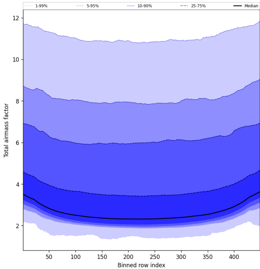
Figure 47: Along track statistics of “Total airmass factor” for 2025-02-09 to 2025-02-10
