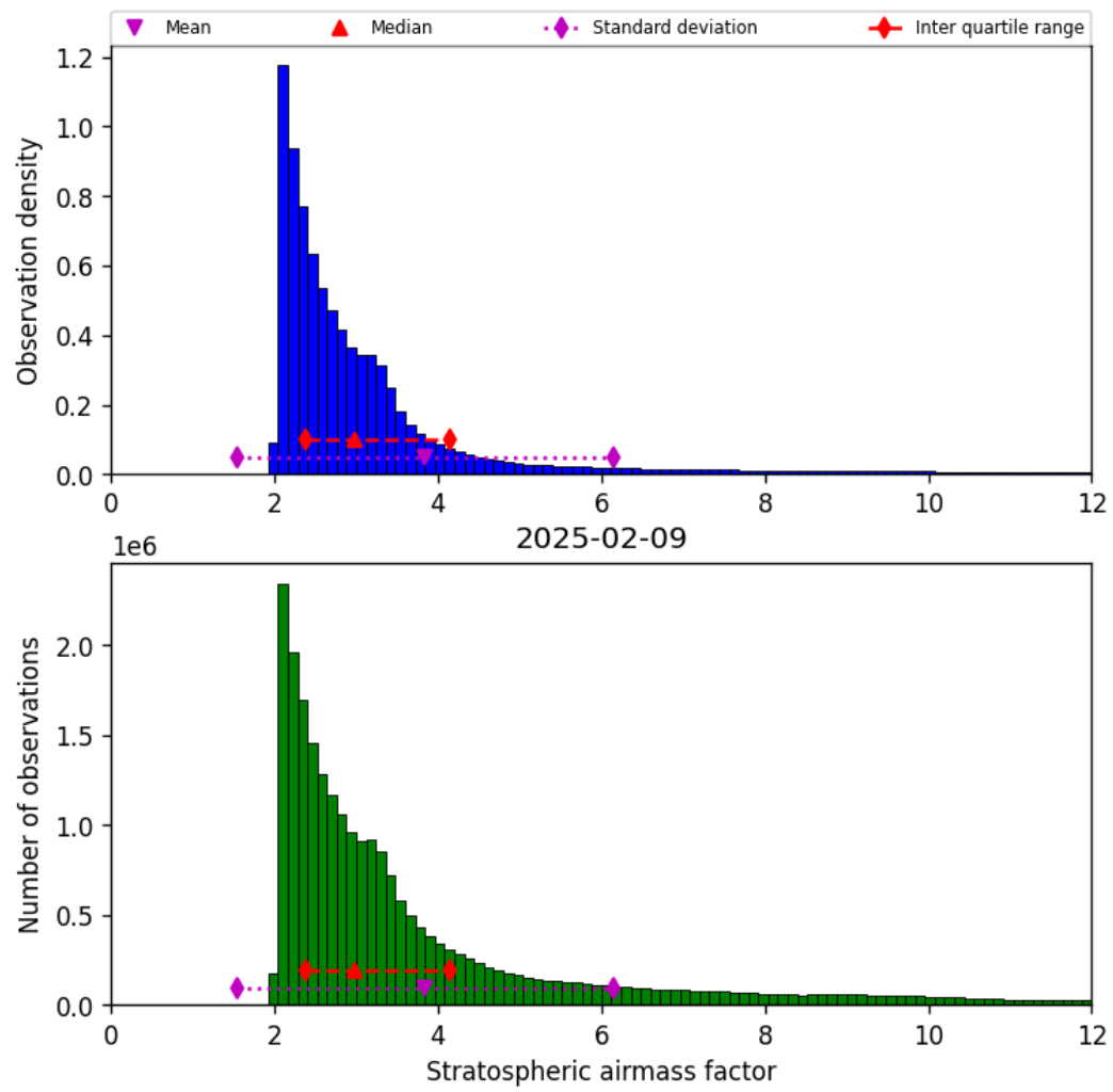
Figure 42: Histogram of “Stratospheric airmass factor” for 2025-02-09 to 2025-02-10
