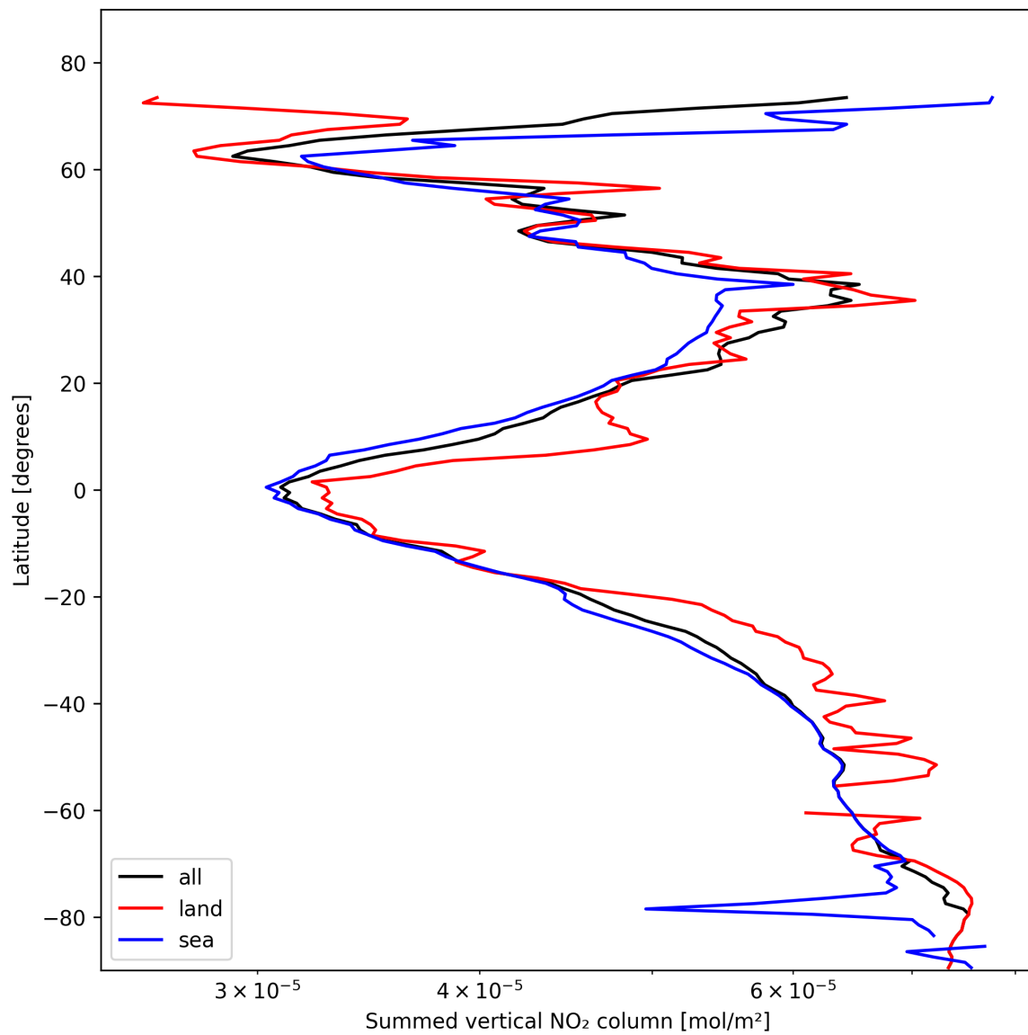
Figure 21: Zonal average of “Summed vertical NO 2 column” for 2025-02-09 to 2025-02-10.
