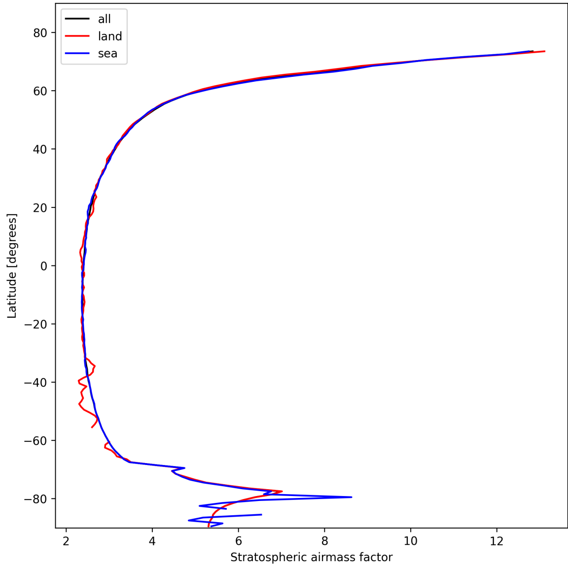
Figure 25: Zonal average of “Stratospheric air mass factor” for 2025-02-09 to 2025-02-10.
