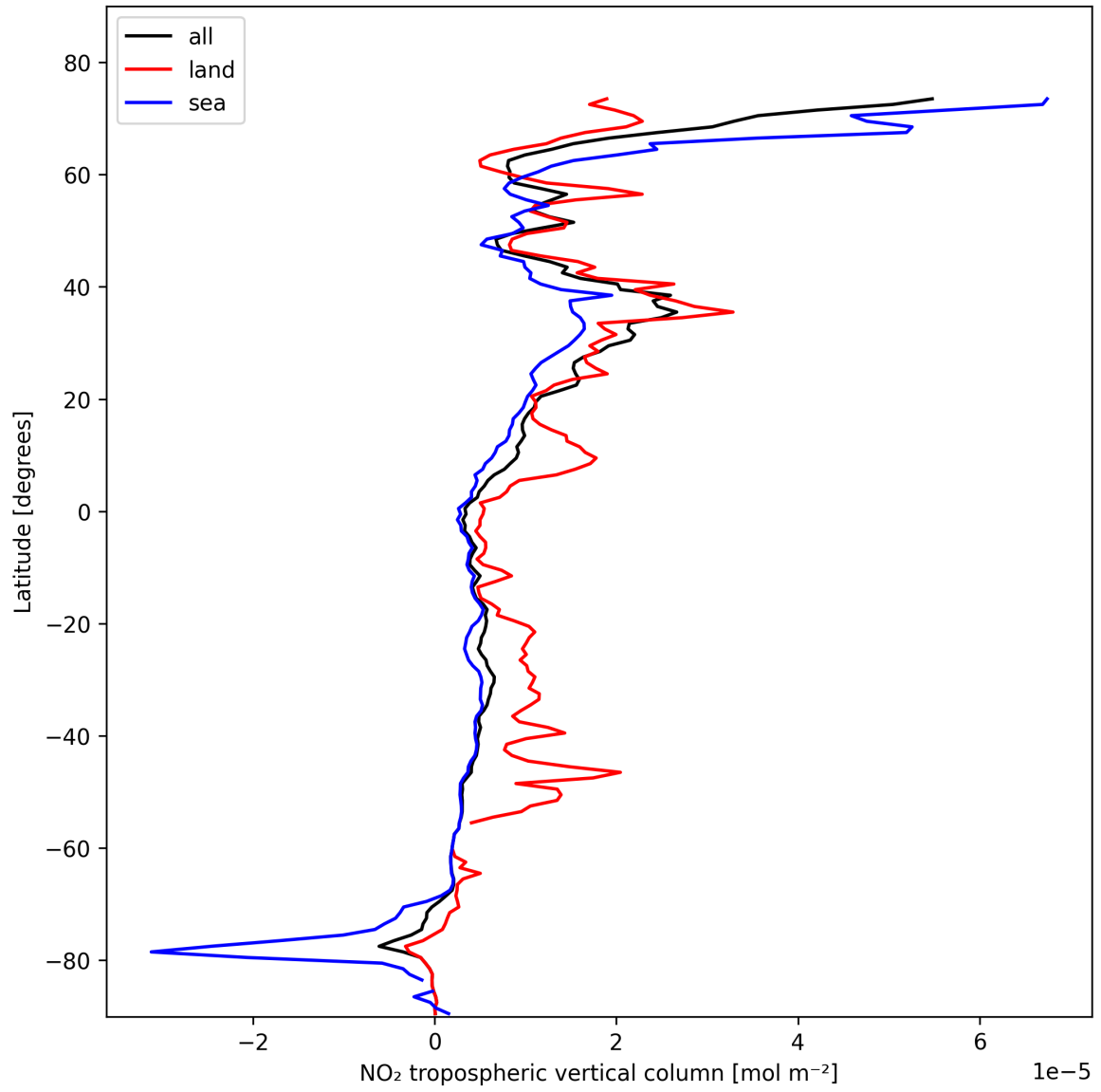
Figure 10: Zonal average of “NO 2 tropospheric vertical column” for 2025-02-09 to 2025-02-10.
