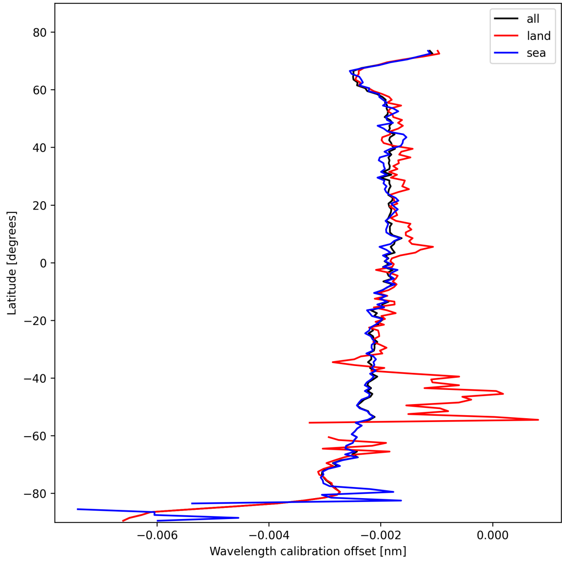
Figure 16: Zonal average of “Wavelength calibration offset” for 2025-02-09 to 2025-02-10.
