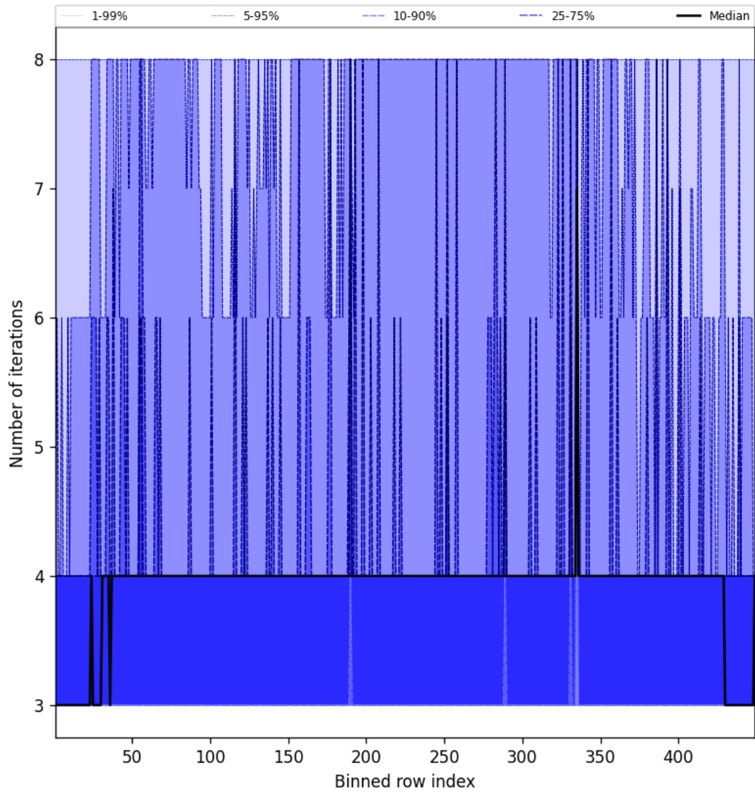
Figure 49: Along track statistics of “Number of iterations” for 2025-02-09 to 2025-02-10
