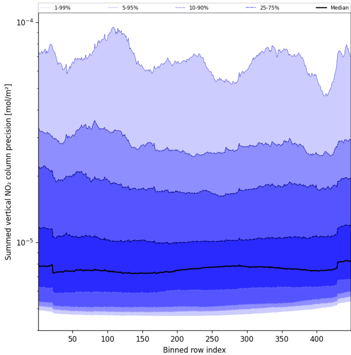
Figure 56: Along track statistics of “Summed vertical NO 2 column precision” for 2025-02-09 to 2025-02-10
