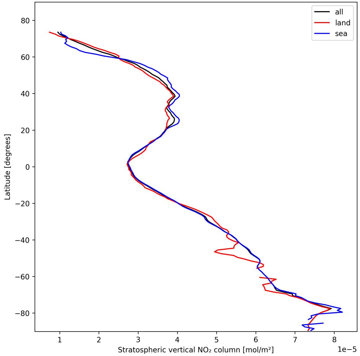
Figure 17: Zonal average of “Stratospheric vertical NO 2 column” for 2025-02-09 to 2025-02-10.
