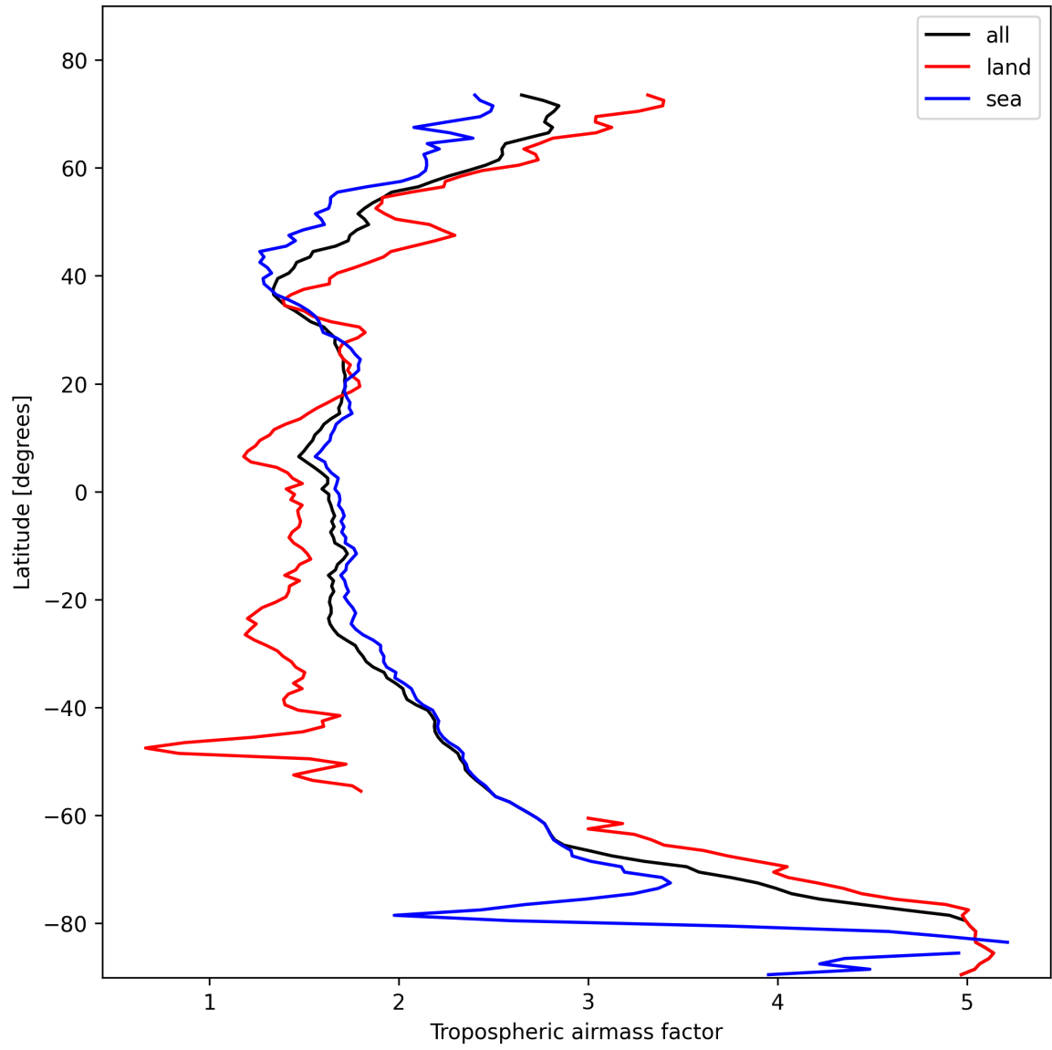
Figure 12: Zonal average of “Tropospheric air mass factor” for 2025-02-09 to 2025-02-10.
