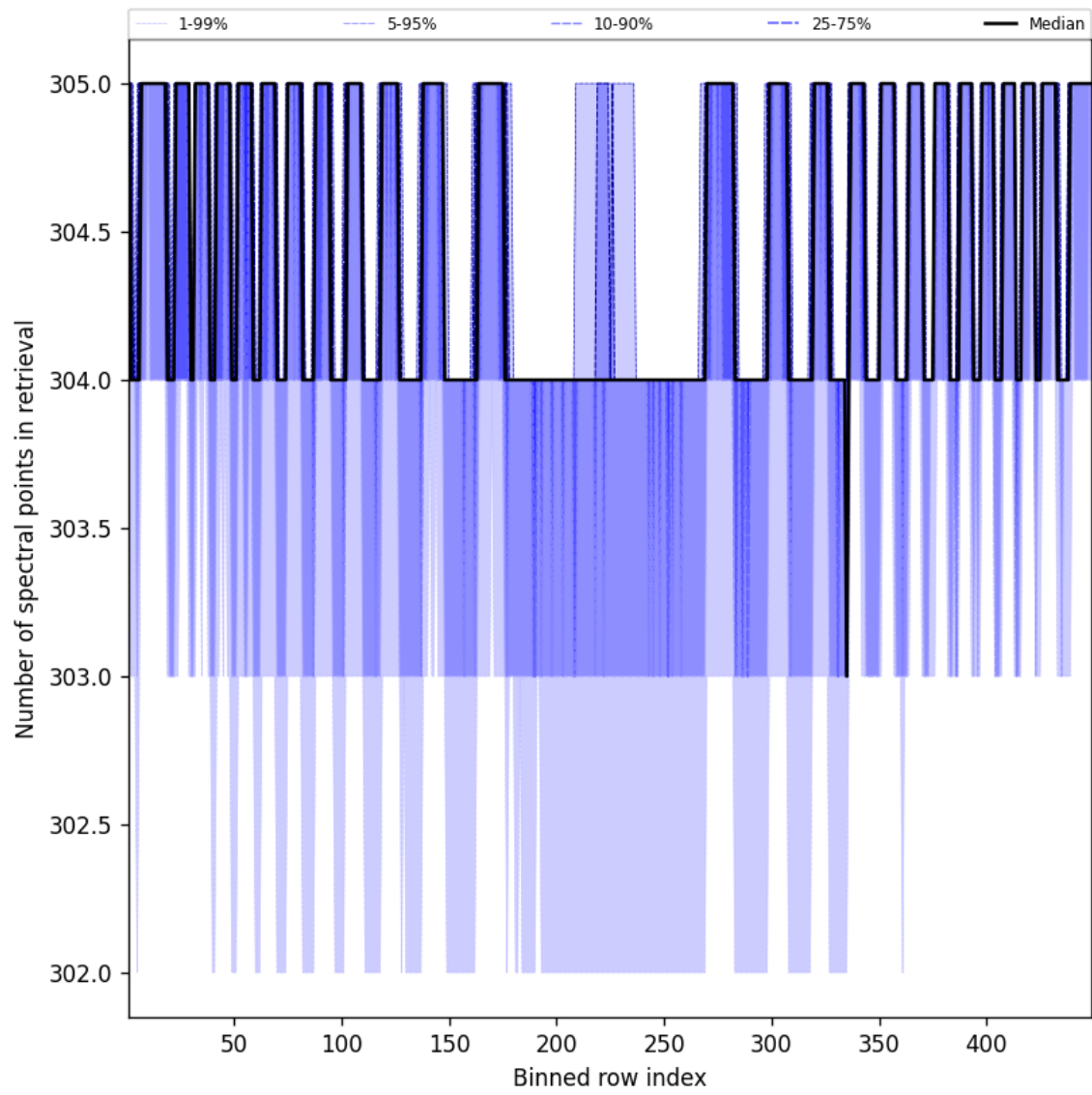
Figure 48: Along track statistics of “Number of spectral points in retrieval” for 2025-02-09 to 2025-02-10
