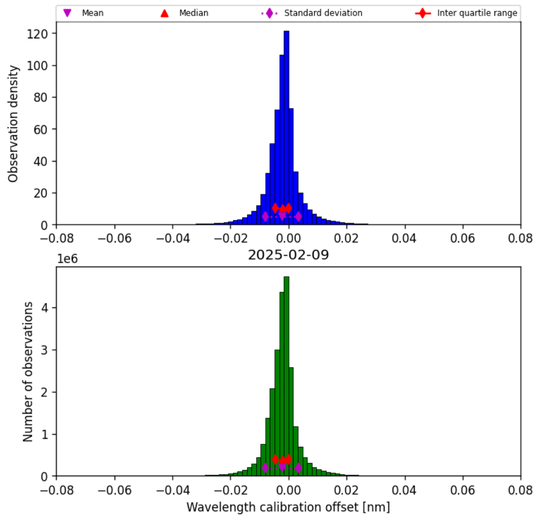
Figure 33: Histogram of “Wavelength calibration offset” for 2025-02-09 to 2025-02-10
