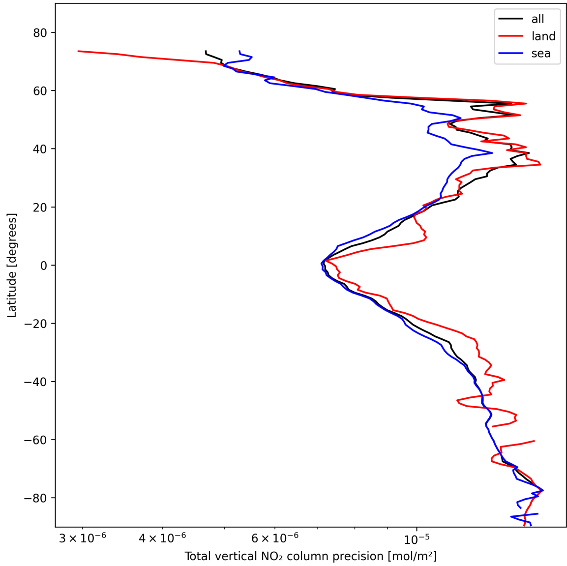
Figure 20: Zonal average of “Total vertical NO 2 column precision” for 2025-02-09 to 2025-02-10.
