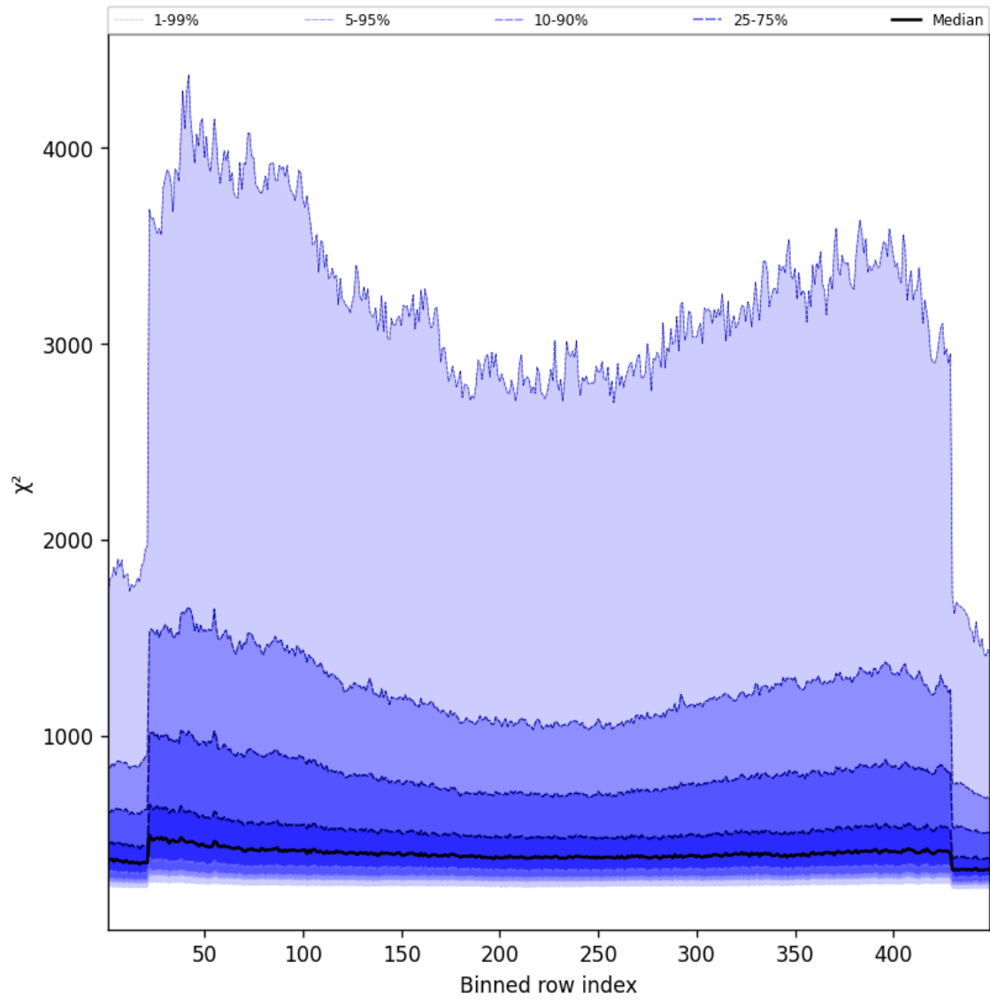
Figure 57: Along track statistics of “ \chi^2 ” for 2025-02-09 to 2025-02-10
