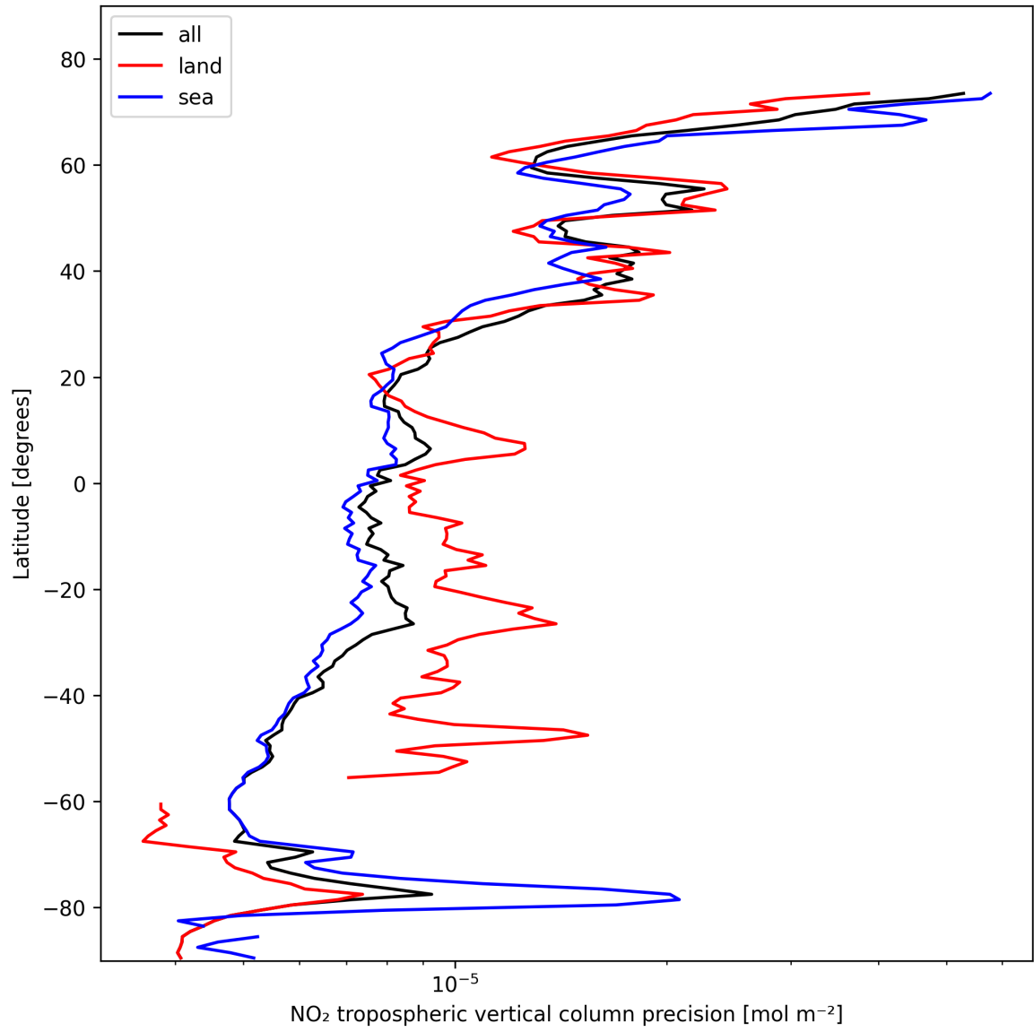
Figure 11: Zonal average of “NO 2 tropospheric vertical column precision” for 2025-02-09 to 2025-02-10.
