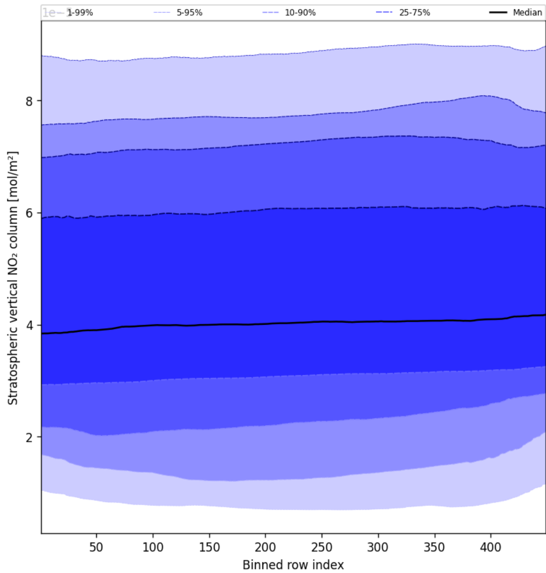
Figure 51: Along track statistics of "Stratospheric vertical NO 2 column" for 2025-02-09 to 2025-02-10
