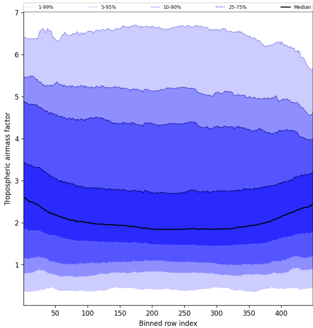
Figure 46: Along track statistics of “Tropospheric airmass factor” for 2025-02-09 to 2025-02-10
