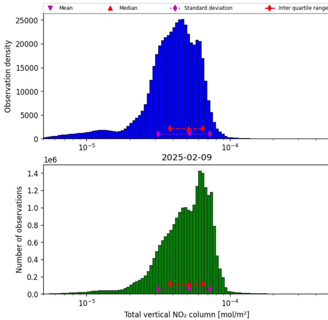
Figure 36: Histogram of “Total vertical NO 2 column” for 2025-02-09 to 2025-02-10
