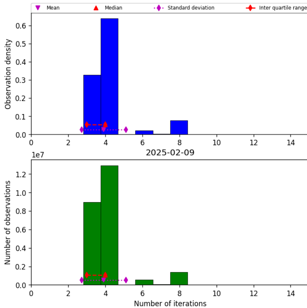
Figure 32: Histogram of “Number of iterations” for 2025-02-09 to 2025-02-10
