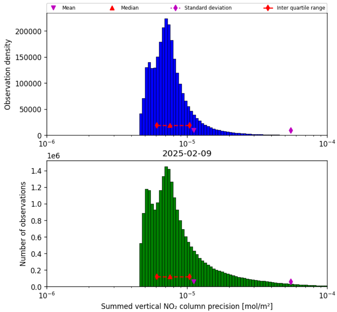
Figure 39: Histogram of “Summed vertical NO 2 column precision” for 2025-02-09 to 2025-02-10
