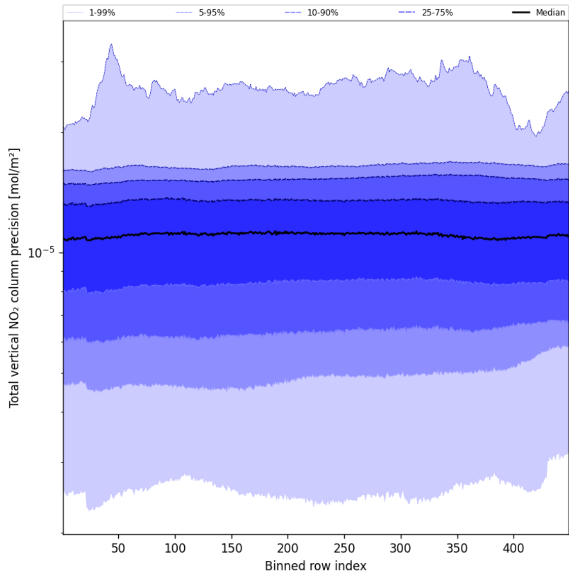
Figure 54: Along track statistics of “Total vertical NO 2 column precision” for 2025-02-09 to 2025-02-10
