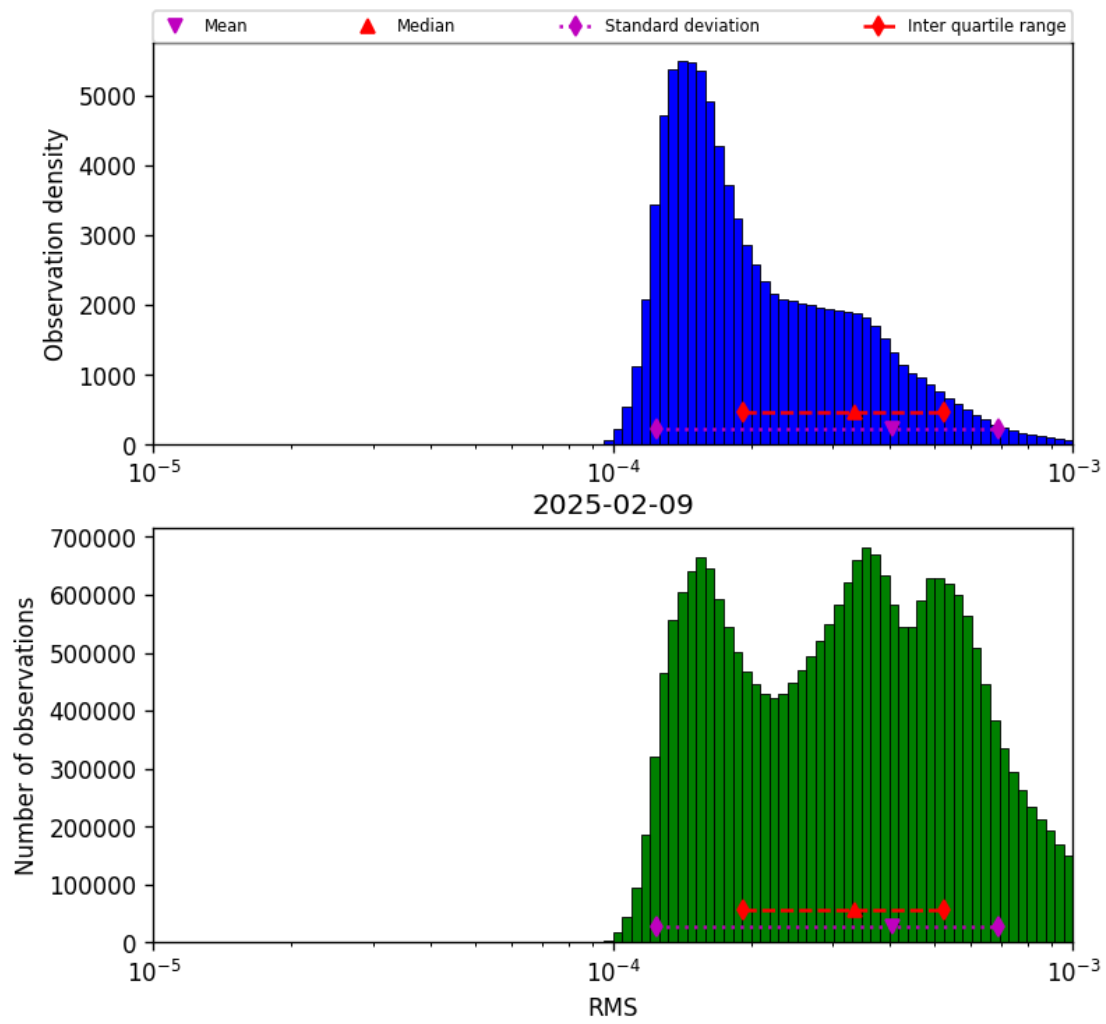
Figure 41: Histogram of “RMS” for 2025-02-09 to 2025-02-10
