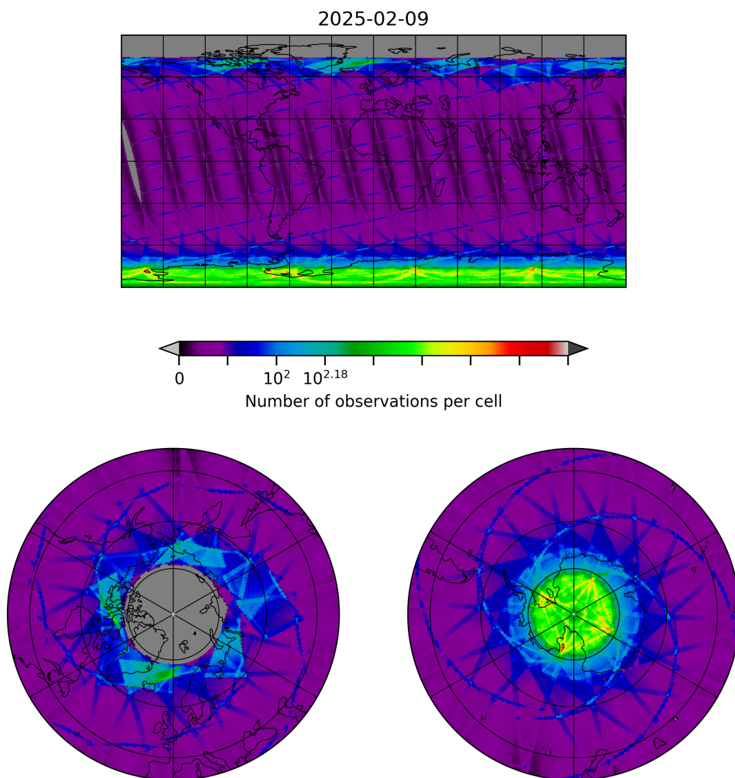
Figure 8: Map of the number of observations for 2025-02-09 to 2025-02-10
