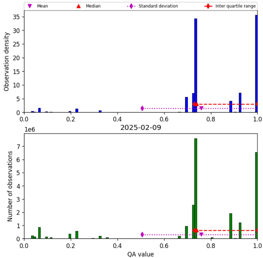
Figure 26: Histogram of “QA value” for 2025-02-09 to 2025-02-10
