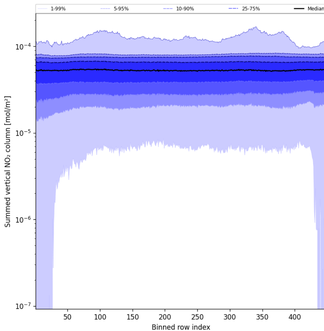
Figure 55: Along track statistics of “Summed vertical NO 2 column” for 2025-02-09 to 2025-02-10
