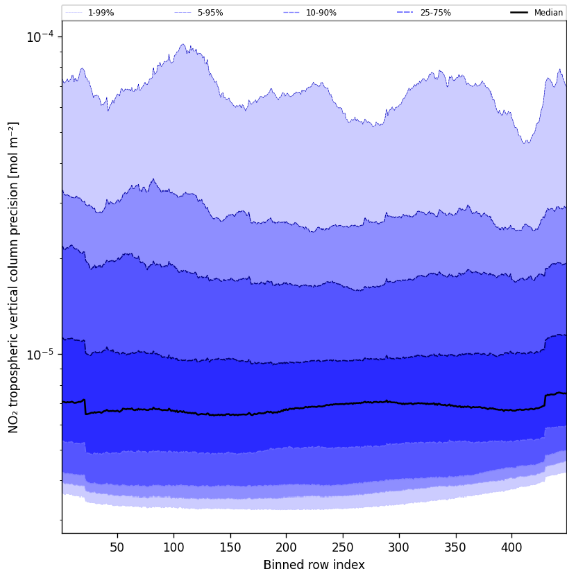
Figure 45: Along track statistics of “NO 2 tropospheric vertical column precision” for 2025-02-09 to 2025-02-10
