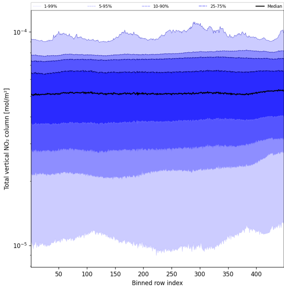
Figure 53: Along track statistics of “Total vertical NO 2 column” for 2025-02-09 to 2025-02-10
