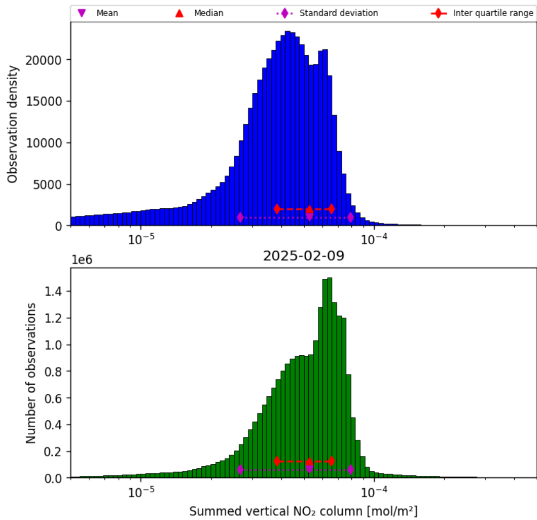
Figure 38: Histogram of "Summed vertical NO 2 column" for 2025-02-09 to 2025-02-10
