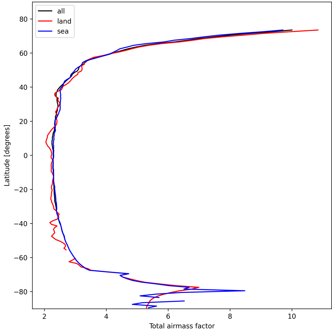
Figure 13: Zonal average of “Total airmass factor” for 2025-02-09 to 2025-02-10.
