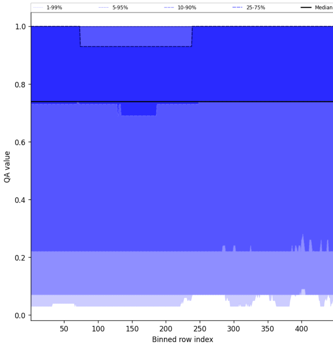
Figure 43: Along track statistics of “QA value” for 2025-02-09 to 2025-02-10
