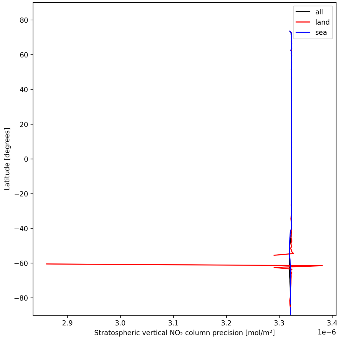
Figure 18: Zonal average of "Stratospheric vertical NO 2 column precision" for 2025-02-09 to 2025-02-10.
