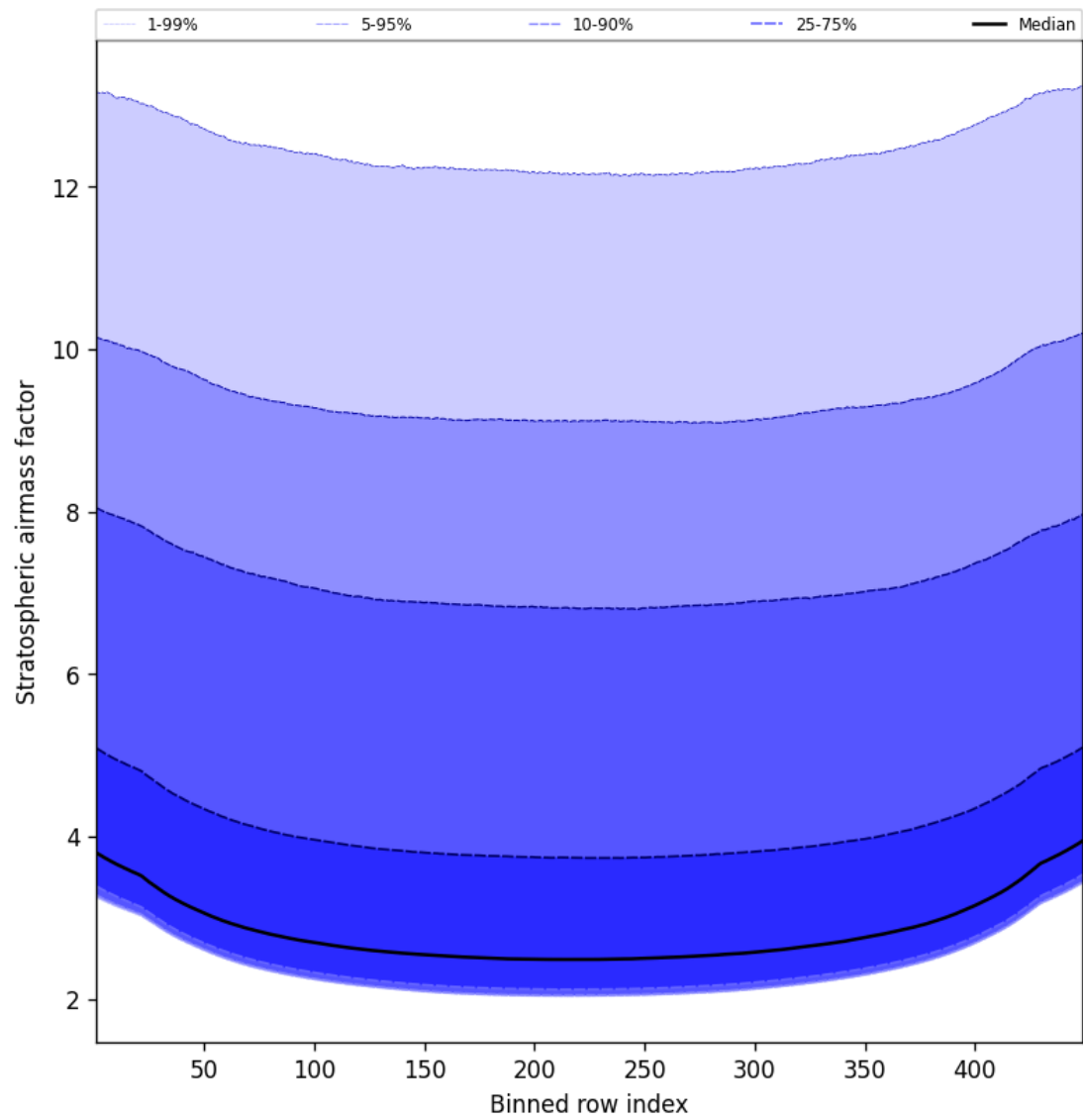
Figure 59: Along track statistics of “Stratospheric airmass factor” for 2025-02-09 to 2025-02-10
