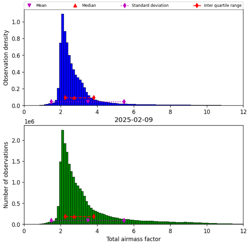
Figure 30: Histogram of “Total airmass factor” for 2025-02-09 to 2025-02-10
