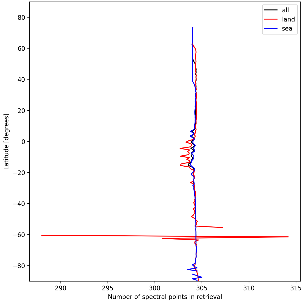
Figure 14: Zonal average of “Number of spectral points in retrieval” for 2025-02-09 to 2025-02-10.
