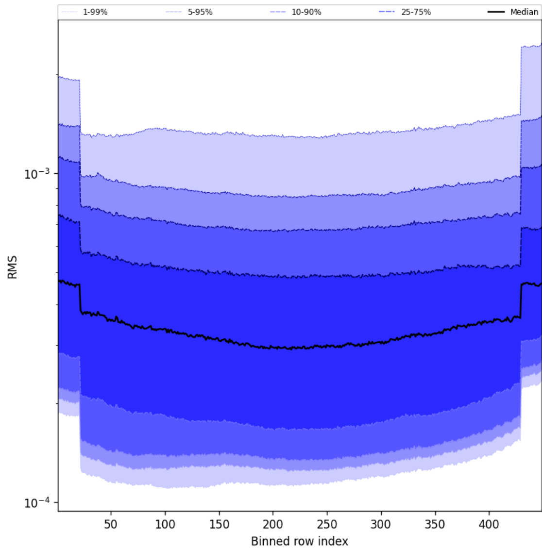
Figure 58: Along track statistics of “RMS” for 2025-02-09 to 2025-02-10
