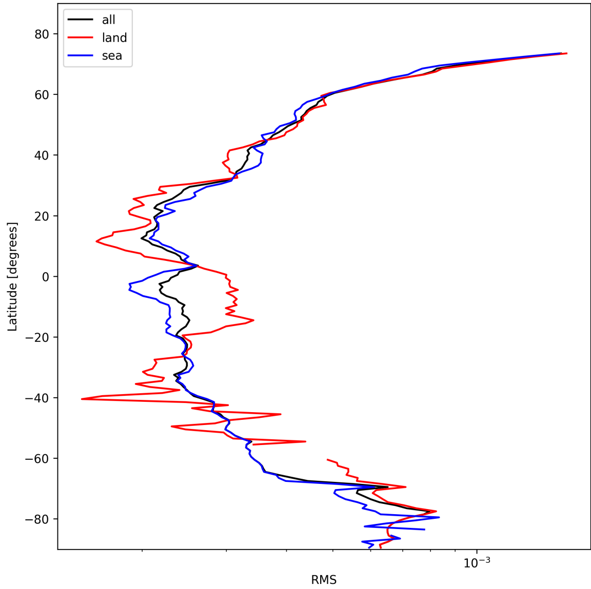
Figure 24: Zonal average of “RMS” for 2025-02-09 to 2025-02-10.
