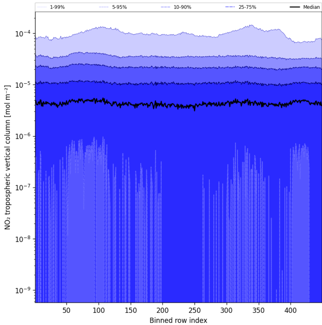
Figure 44: Along track statistics of "NO 2 tropospheric vertical column" for 2025-02-09 to 2025-02-10
