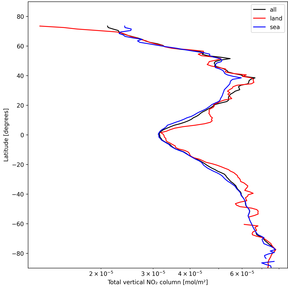
Figure 19: Zonal average of “Total vertical NO 2 column” for 2025-02-09 to 2025-02-10.
