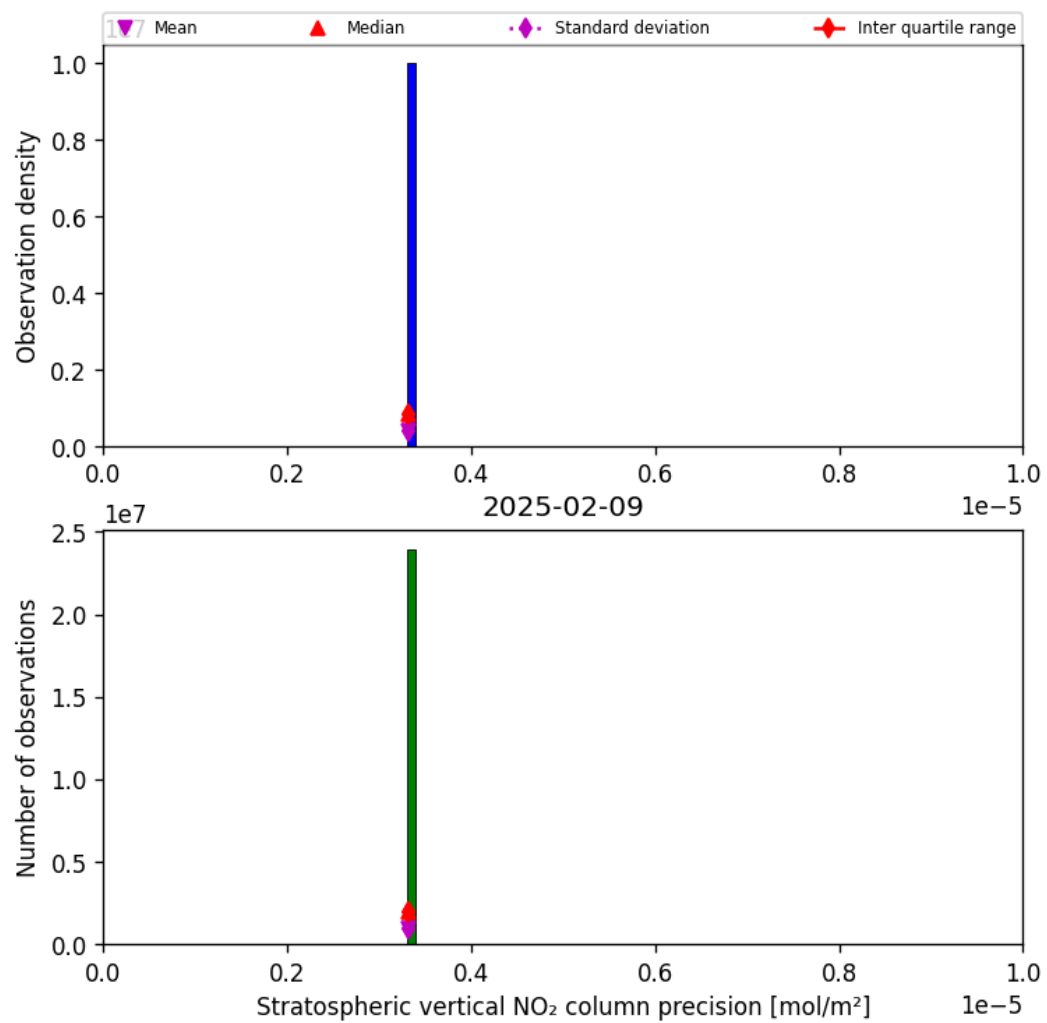
Figure 35: Histogram of “Stratospheric vertical NO 2 column precision” for 2025-02-09 to 2025-02-10
