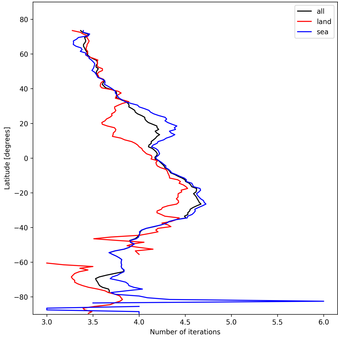
Figure 15: Zonal average of “Number of iterations” for 2025-02-09 to 2025-02-10.
