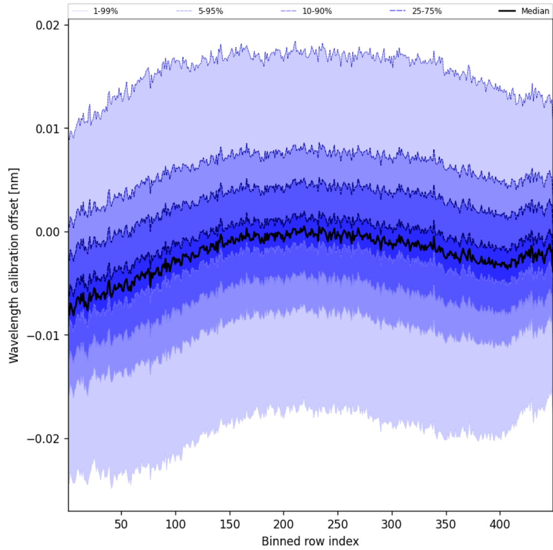
Figure 50: Along track statistics of “Wavelength calibration offset” for 2025-02-09 to 2025-02-10
