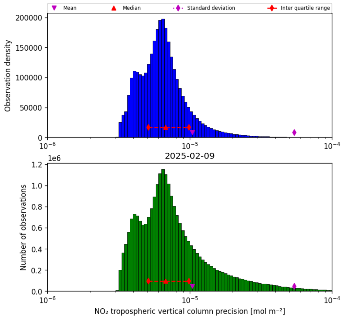
Figure 28: Histogram of “NO 2 tropospheric vertical column precision” for 2025-02-09 to 2025-02-10
