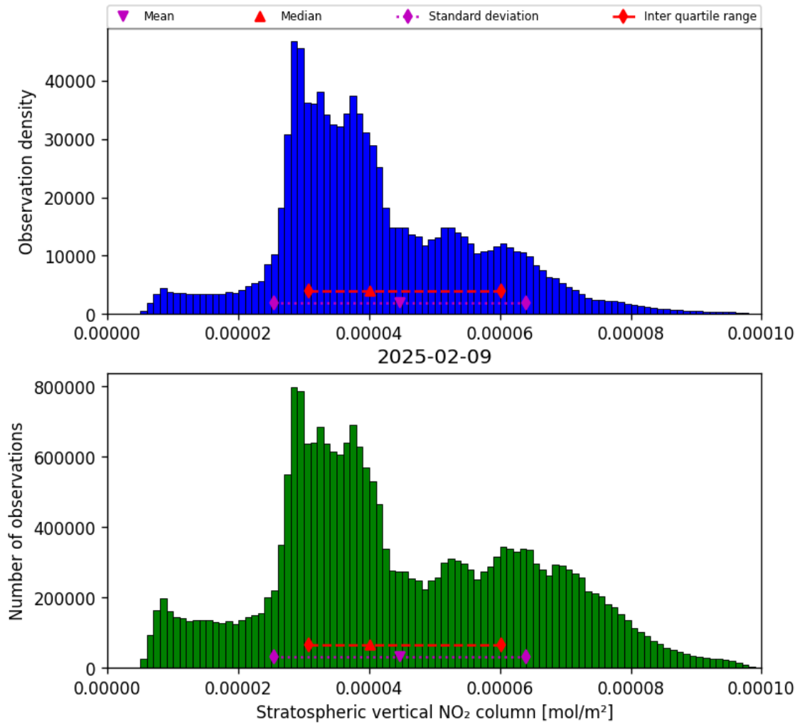
Figure 34: Histogram of “Stratospheric vertical NO 2 column” for 2025-02-09 to 2025-02-10
