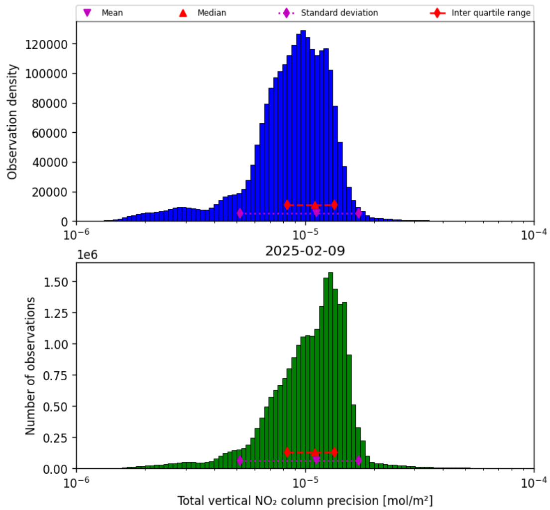
Figure 37: Histogram of “Total vertical NO 2 column precision” for 2025-02-09 to 2025-02-10
