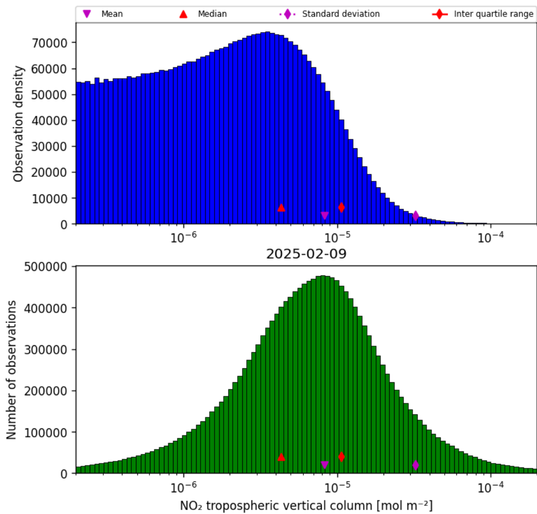
Figure 27: Histogram of “NO 2 tropospheric vertical column” for 2025-02-09 to 2025-02-10
