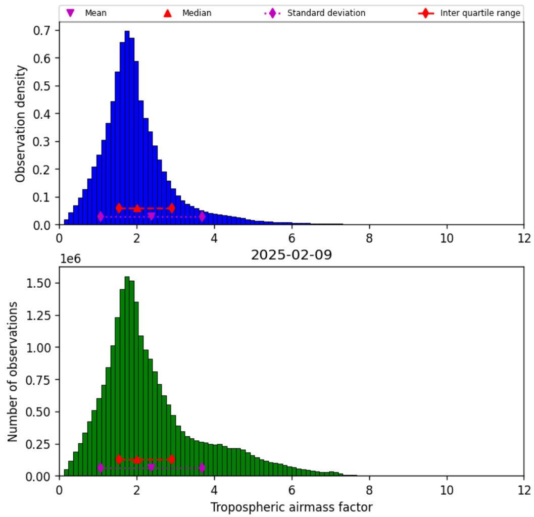
Figure 29: Histogram of “Tropospheric airmass factor” for 2025-02-09 to 2025-02-10
