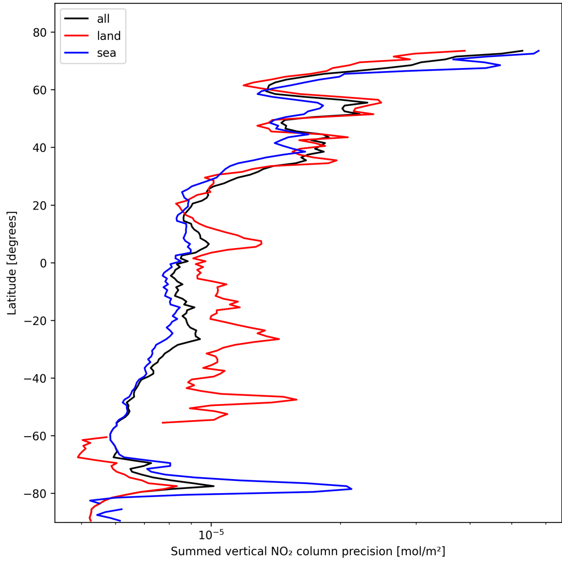
Figure 22: Zonal average of “Summed vertical NO 2 column precision” for 2025-02-09 to 2025-02-10.
