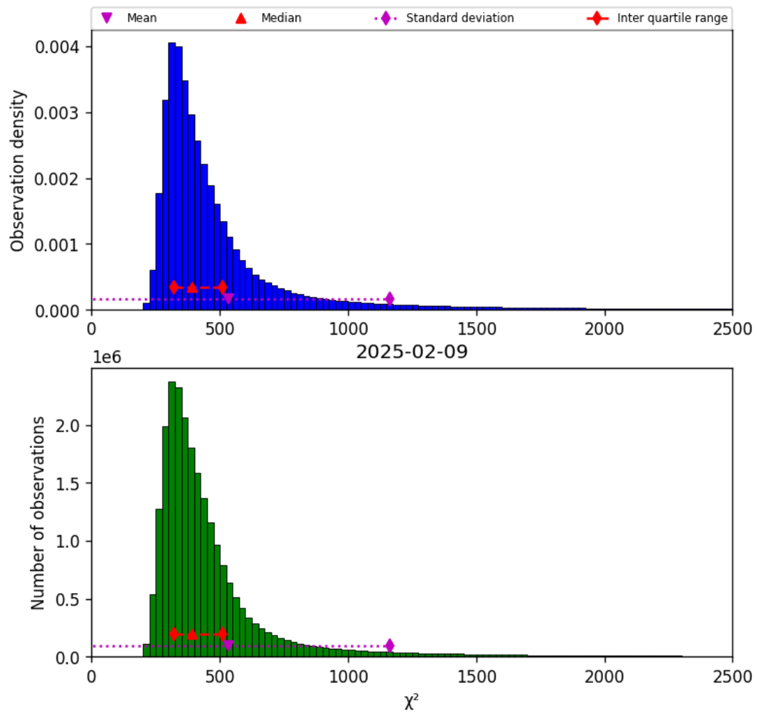
Figure 40: Histogram of “ \chi^2 ” for 2025-02-09 to 2025-02-10
