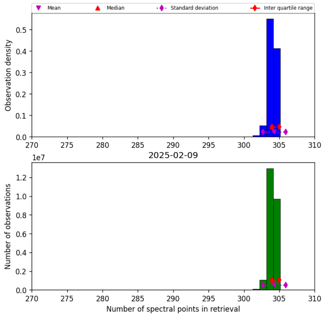
Figure 31: Histogram of “Number of spectral points in retrieval” for 2025-02-09 to 2025-02-10
