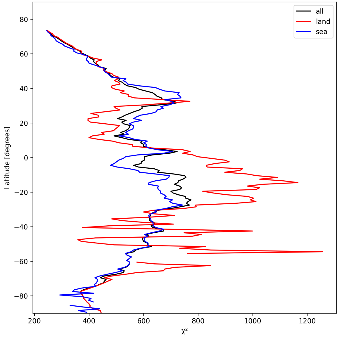
Figure 23: Zonal average of “ \chi^2 ” for 2025-02-09 to 2025-02-10.
