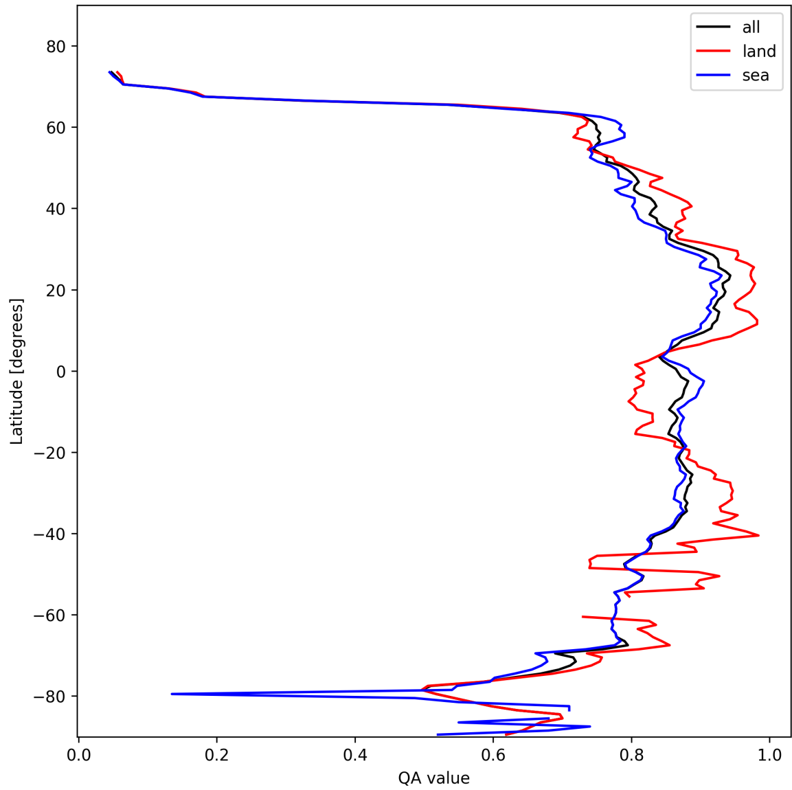
Figure 9: Zonal average of “QA value” for 2025-02-09 to 2025-02-10.
