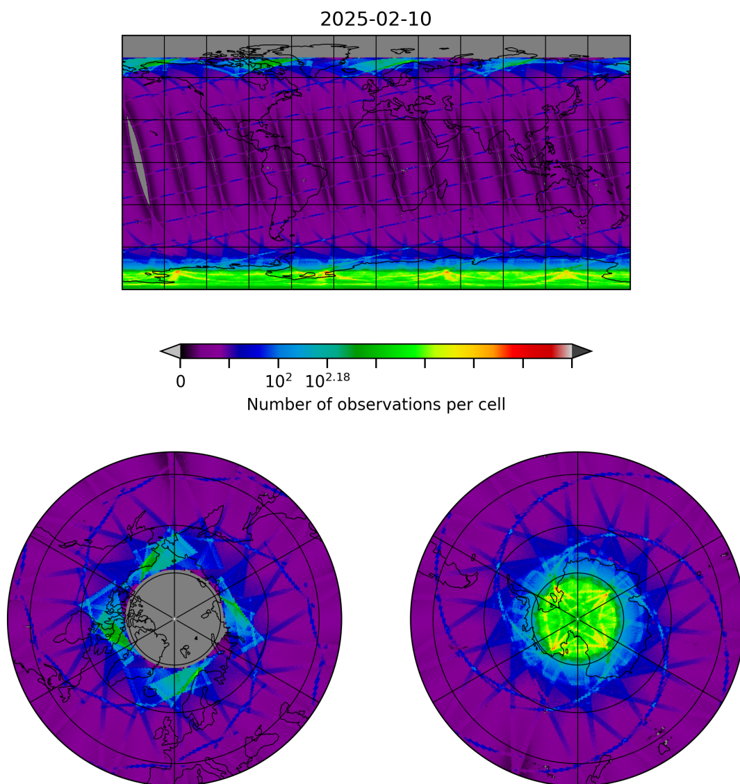
Figure 8: Map of the number of observations for 2025-02-10 to 2025-02-11
