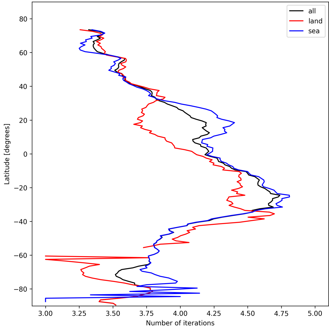
Figure 15: Zonal average of “Number of iterations” for 2025-02-10 to 2025-02-11.
