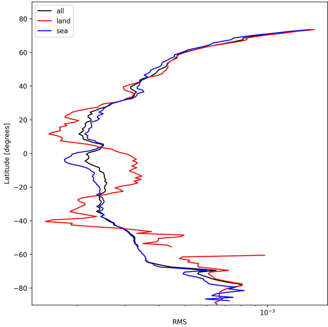
Figure 24: Zonal average of “RMS” for 2025-02-10 to 2025-02-11.
