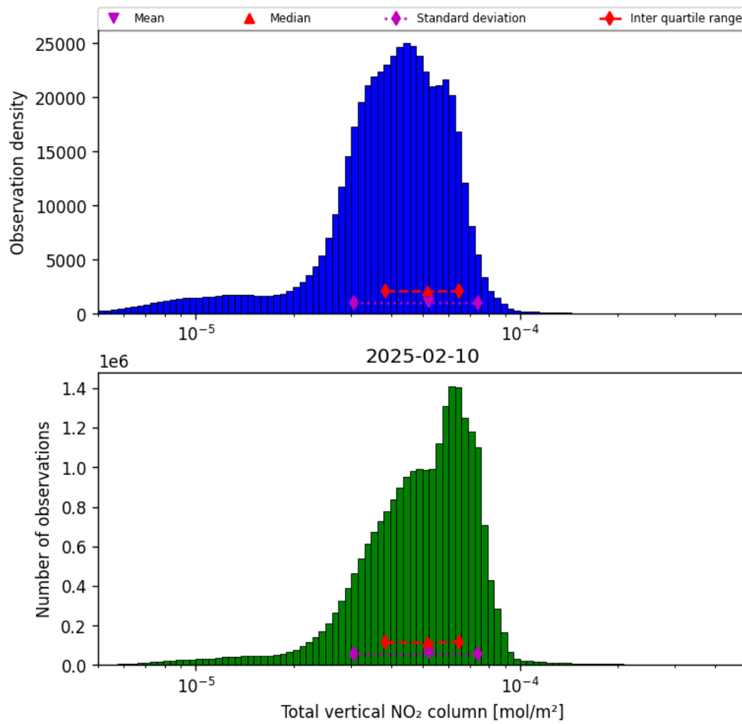
Figure 36: Histogram of “Total vertical NO 2 column” for 2025-02-10 to 2025-02-11
