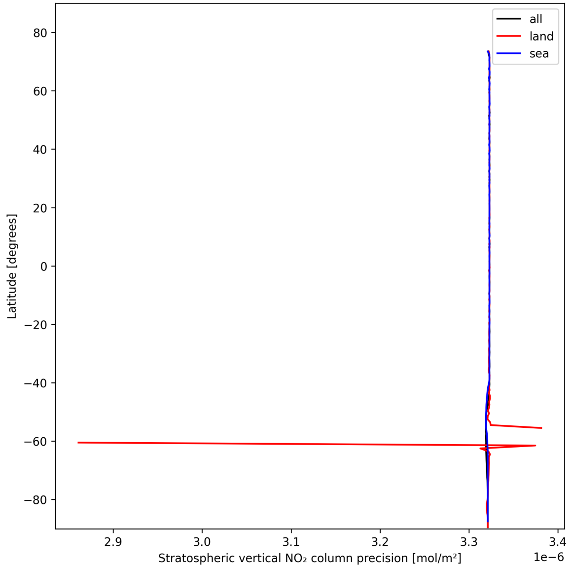
Figure 18: Zonal average of "Stratospheric vertical NO 2 column precision" for 2025-02-10 to 2025-02-11.
