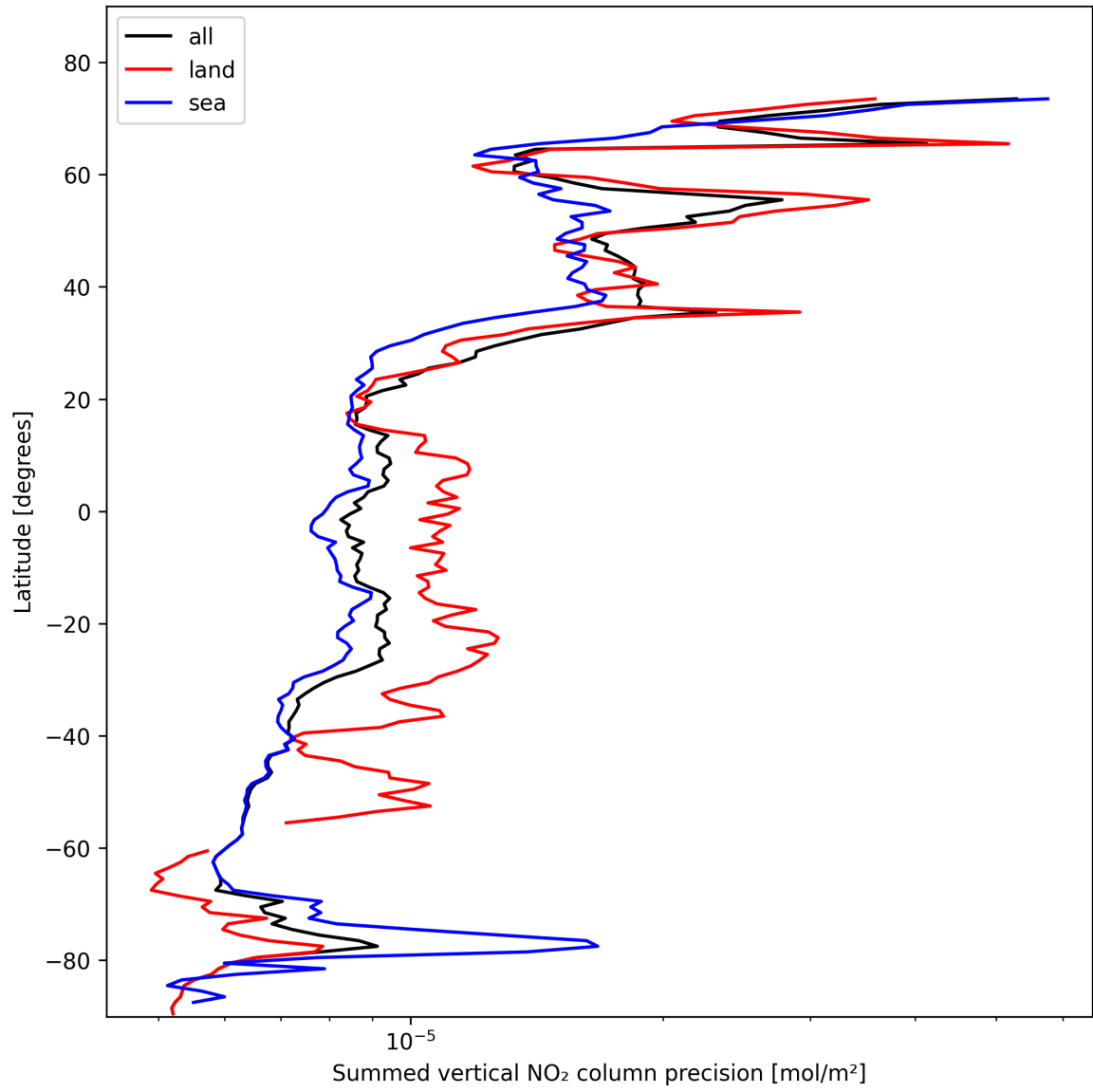
Figure 22: Zonal average of “Summed vertical NO 2 column precision” for 2025-02-10 to 2025-02-11.
