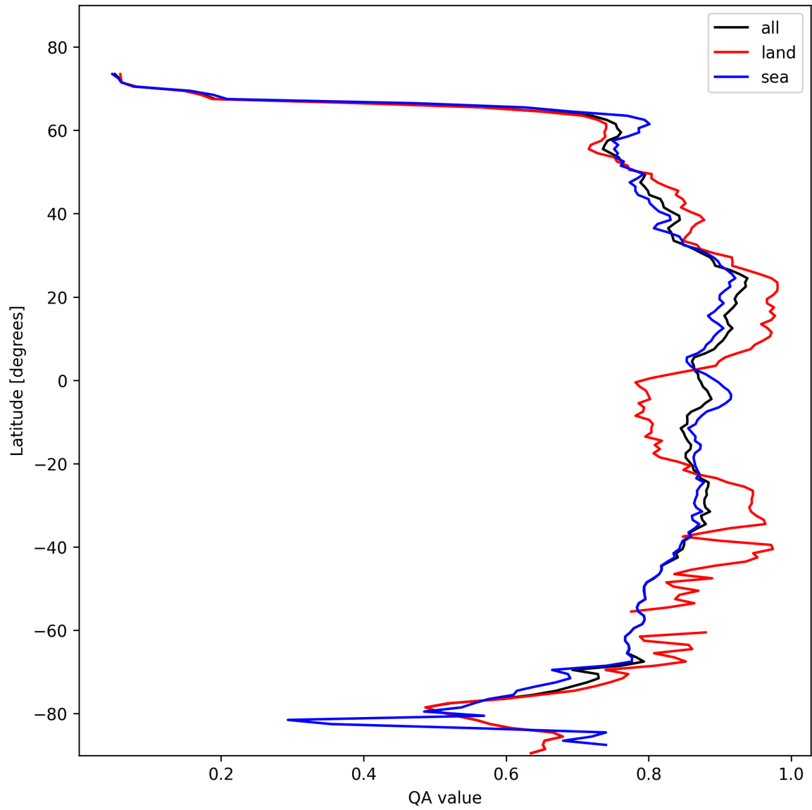
Figure 9: Zonal average of “QA value” for 2025-02-10 to 2025-02-11.
