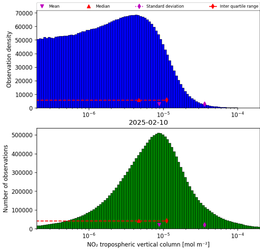
Figure 27: Histogram of “NO 2 tropospheric vertical column” for 2025-02-10 to 2025-02-11
