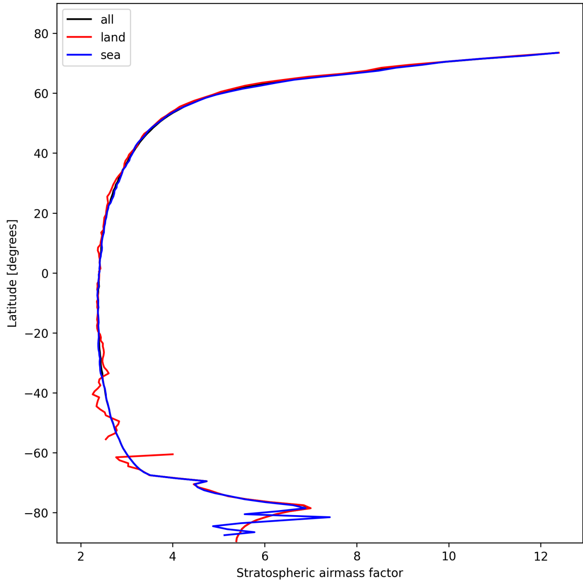
Figure 25: Zonal average of “Stratospheric air mass factor” for 2025-02-10 to 2025-02-11.
