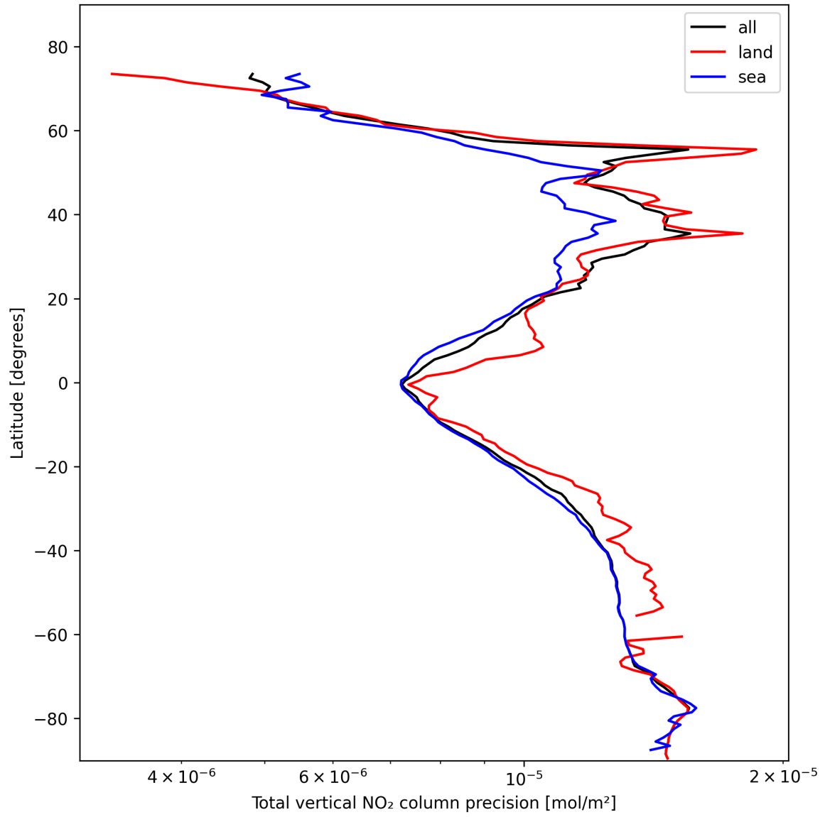
Figure 20: Zonal average of “Total vertical NO 2 column precision” for 2025-02-10 to 2025-02-11.
