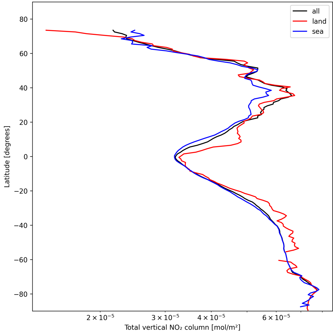
Figure 19: Zonal average of “Total vertical NO 2 column” for 2025-02-10 to 2025-02-11.
