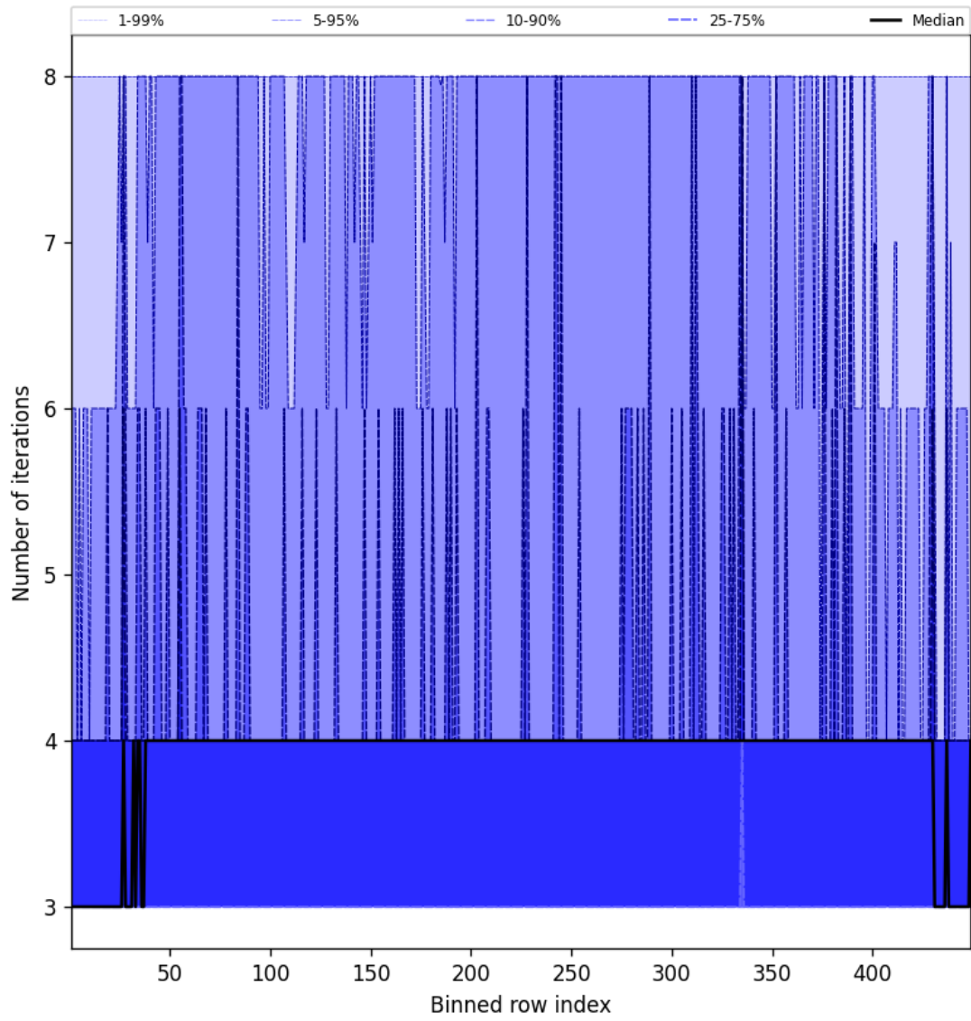
Figure 49: Along track statistics of “Number of iterations” for 2025-02-10 to 2025-02-11
