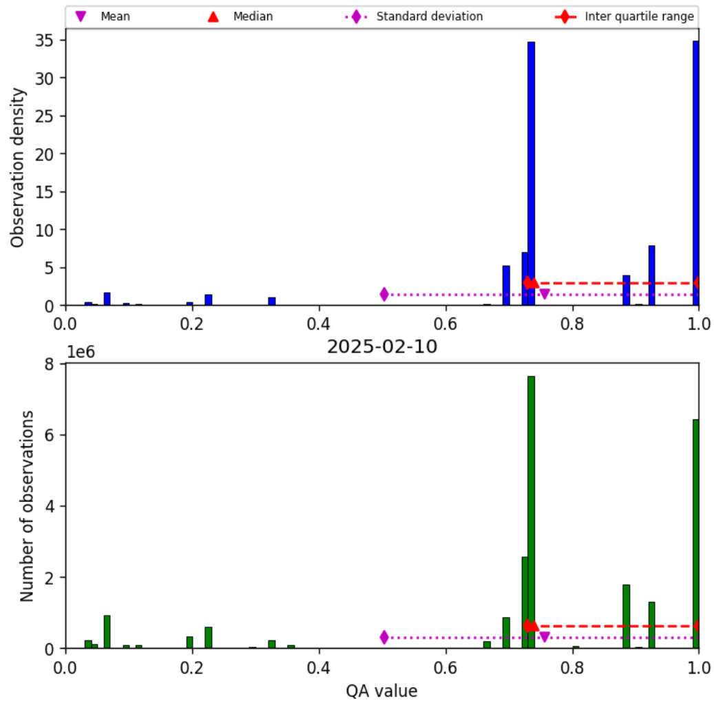
Figure 26: Histogram of “QA value” for 2025-02-10 to 2025-02-11
