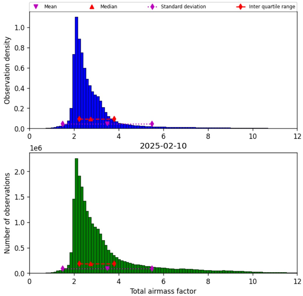
Figure 30: Histogram of “Total airmass factor” for 2025-02-10 to 2025-02-11
