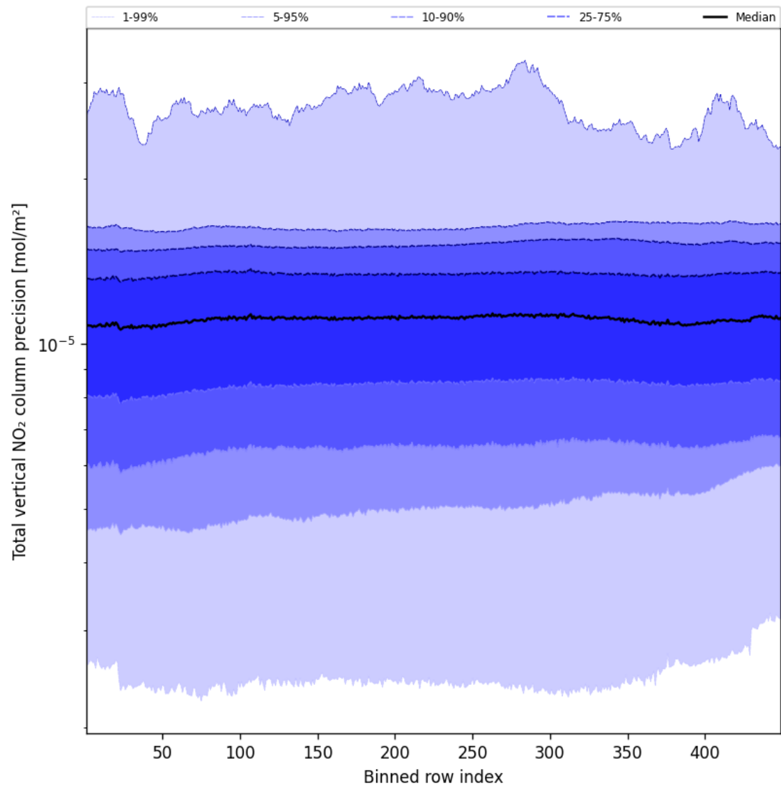
Figure 54: Along track statistics of “Total vertical NO 2 column precision” for 2025-02-10 to 2025-02-11
