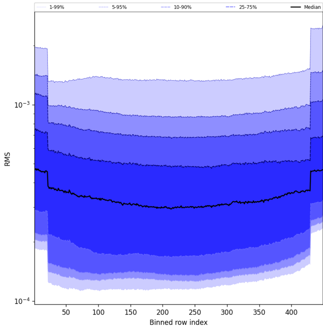
Figure 58: Along track statistics of “RMS” for 2025-02-10 to 2025-02-11
