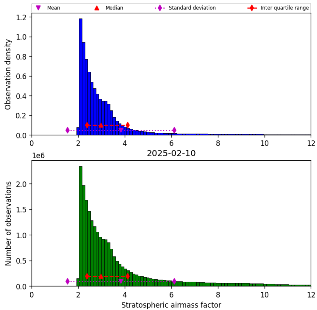
Figure 42: Histogram of “Stratospheric airmass factor” for 2025-02-10 to 2025-02-11
