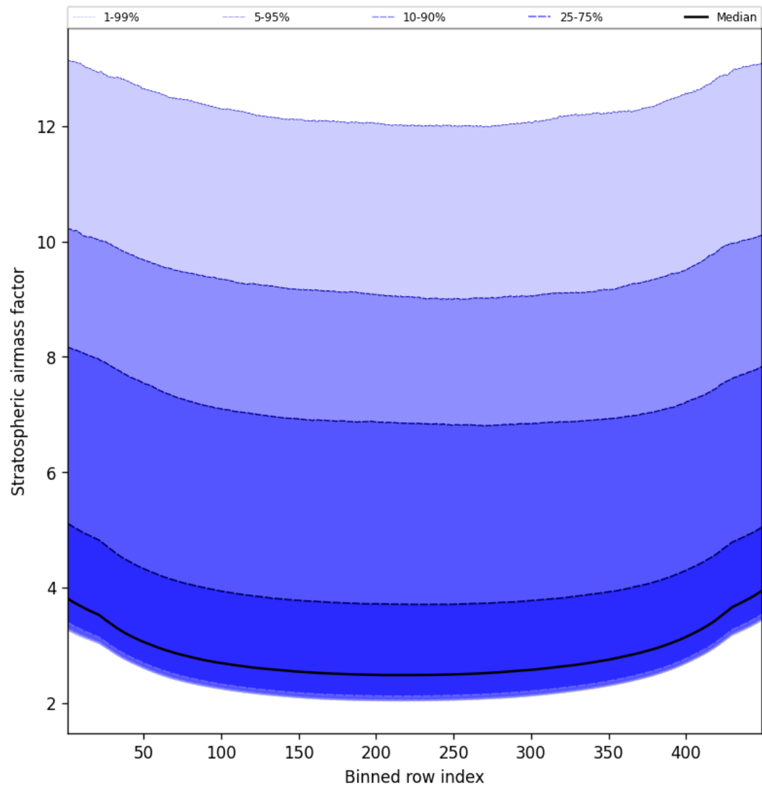
Figure 59: Along track statistics of “Stratospheric airmass factor” for 2025-02-10 to 2025-02-11
