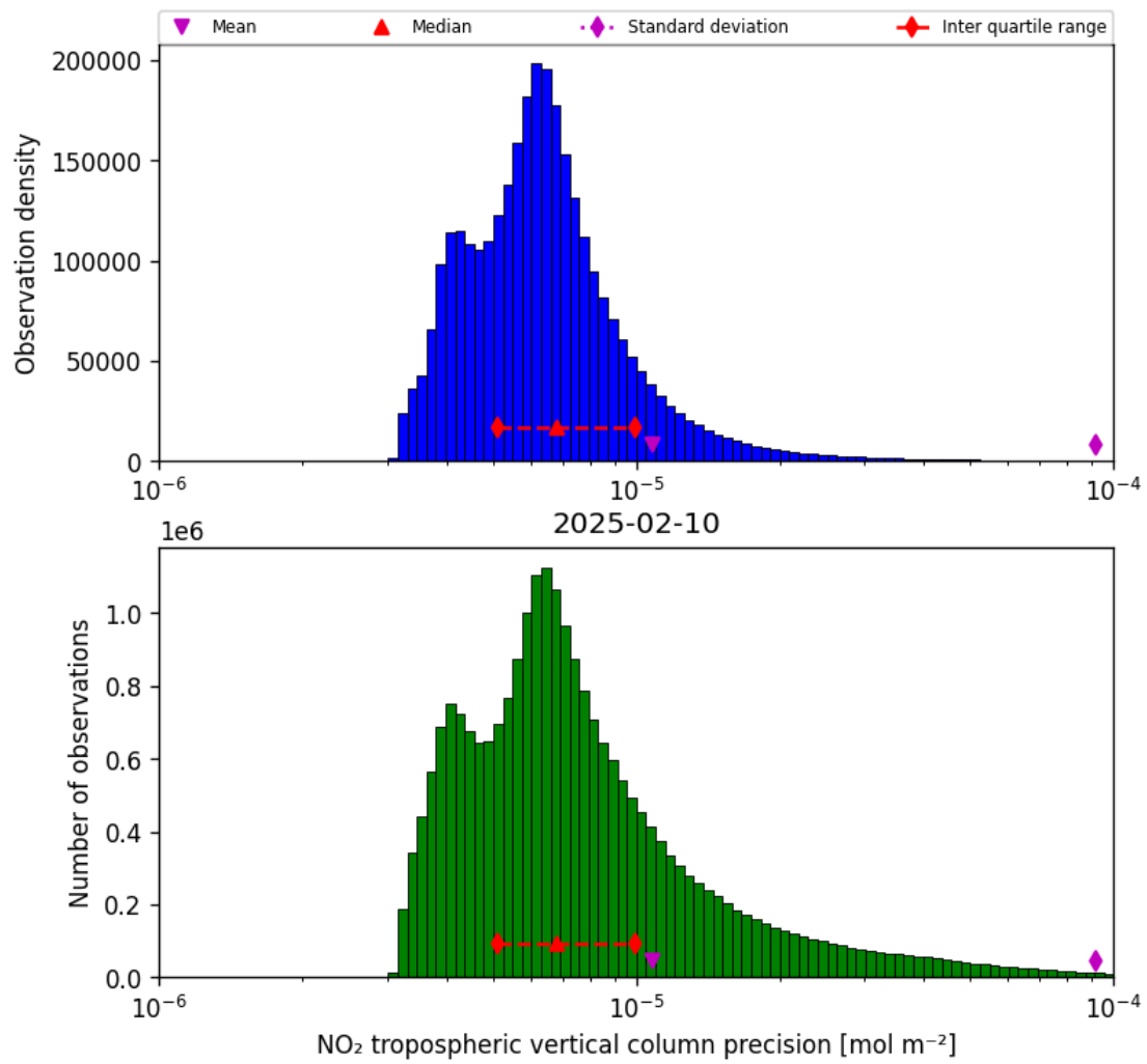
Figure 28: Histogram of “NO 2 tropospheric vertical column precision” for 2025-02-10 to 2025-02-11
