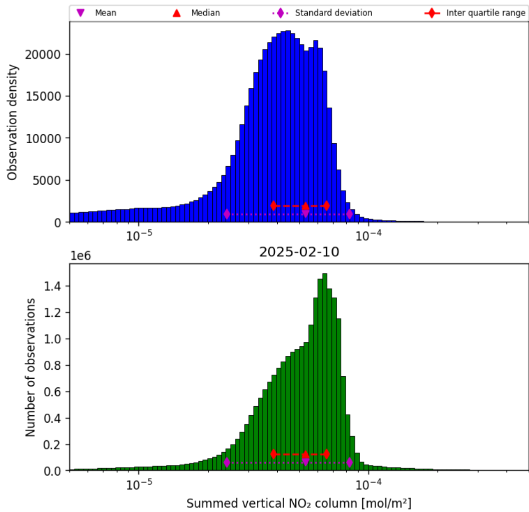
Figure 38: Histogram of “Summed vertical NO 2 column” for 2025-02-10 to 2025-02-11
