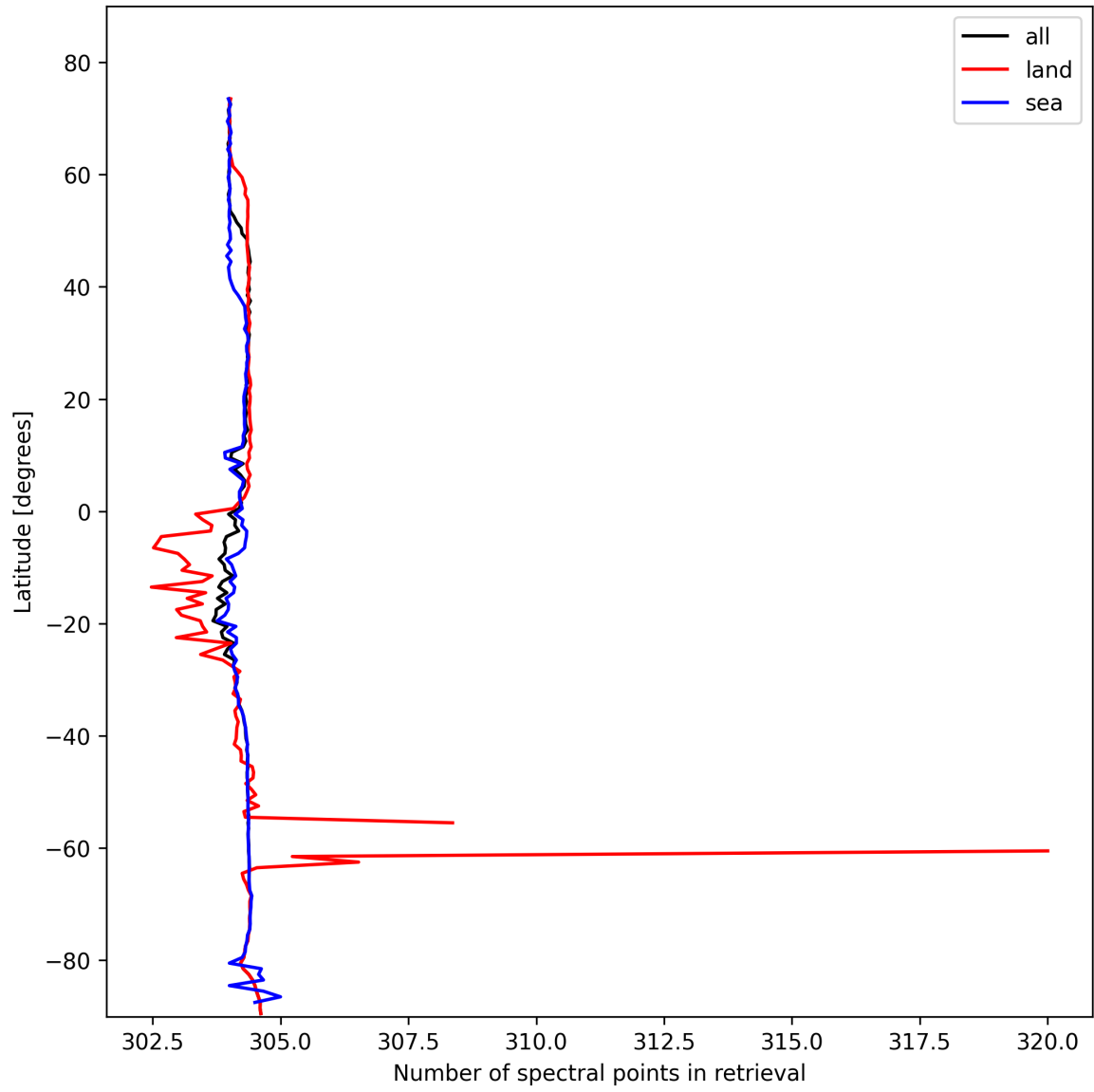
Figure 14: Zonal average of “Number of spectral points in retrieval” for 2025-02-10 to 2025-02-11.
