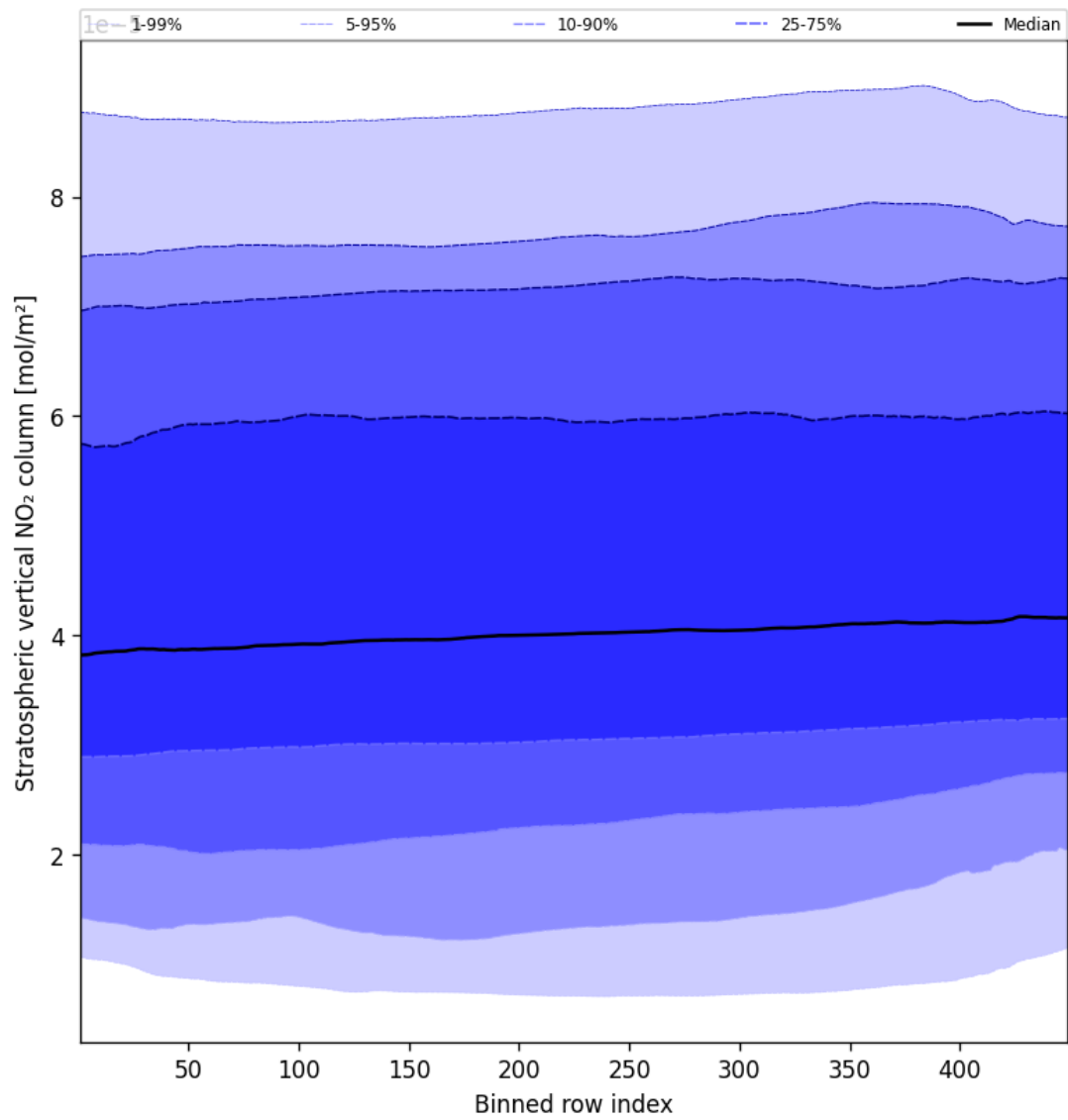
Figure 51: Along track statistics of “Stratospheric vertical NO 2 column” for 2025-02-10 to 2025-02-11
