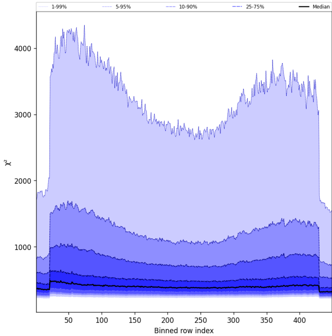
Figure 57: Along track statistics of “ \chi^2 ” for 2025-02-10 to 2025-02-11
