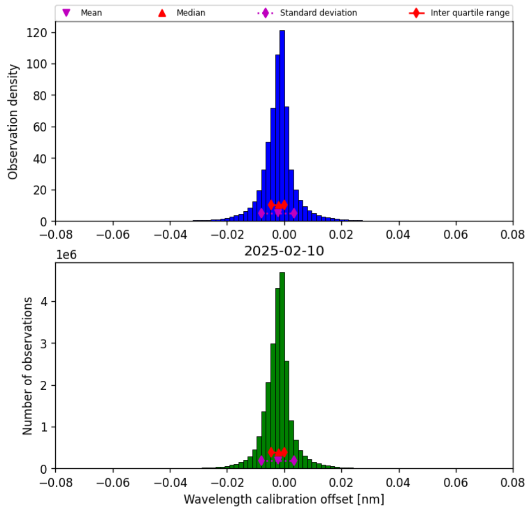
Figure 33: Histogram of “Wavelength calibration offset” for 2025-02-10 to 2025-02-11
