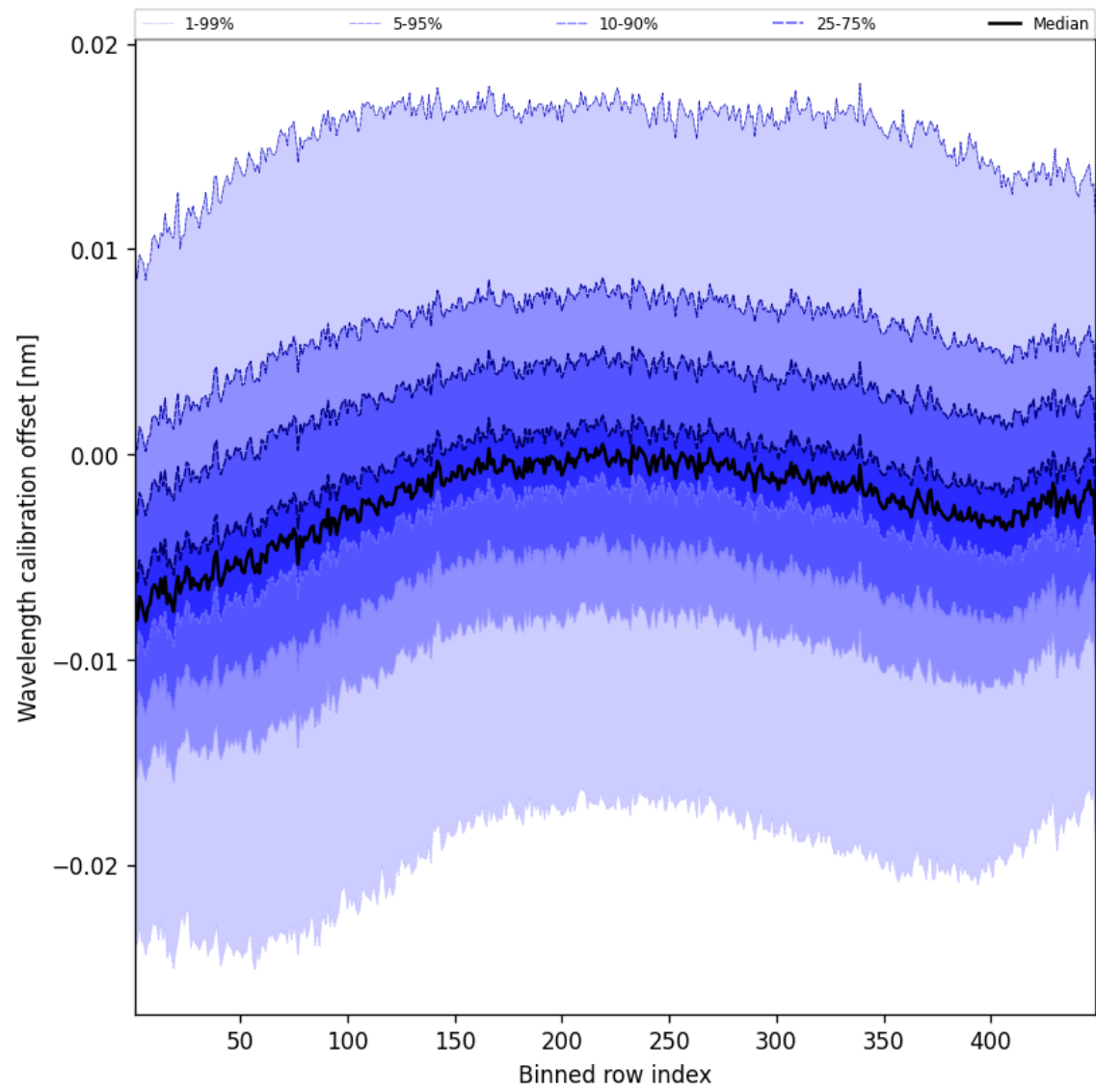
Figure 50: Along track statistics of “Wavelength calibration offset” for 2025-02-10 to 2025-02-11
