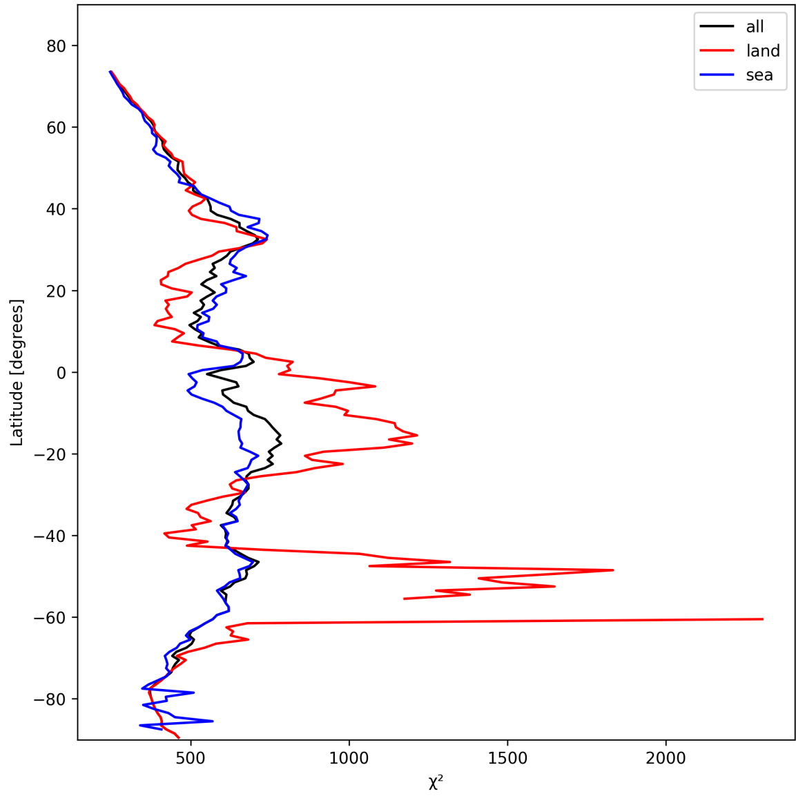
Figure 23: Zonal average of “ \chi^2 ” for 2025-02-10 to 2025-02-11.
