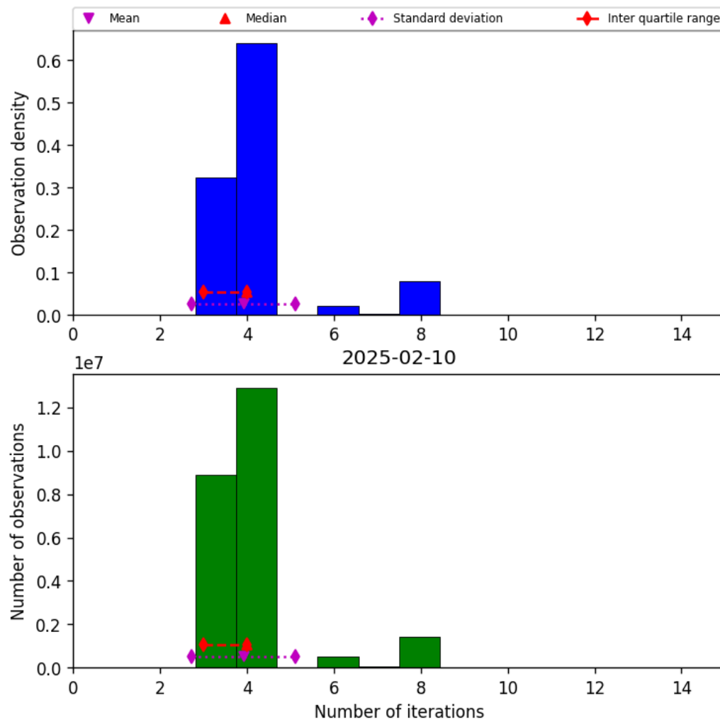
Figure 32: Histogram of “Number of iterations” for 2025-02-10 to 2025-02-11
