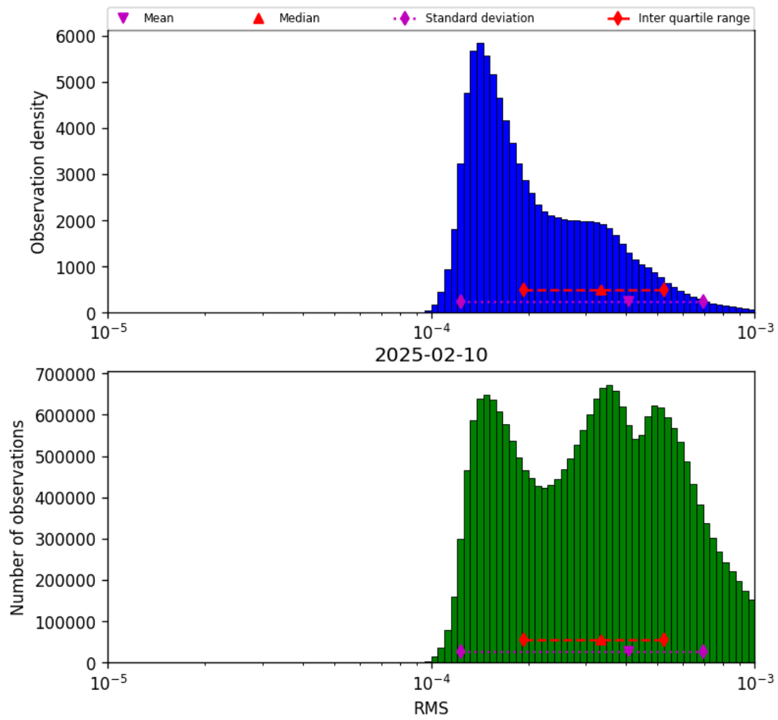
Figure 41: Histogram of “RMS” for 2025-02-10 to 2025-02-11
