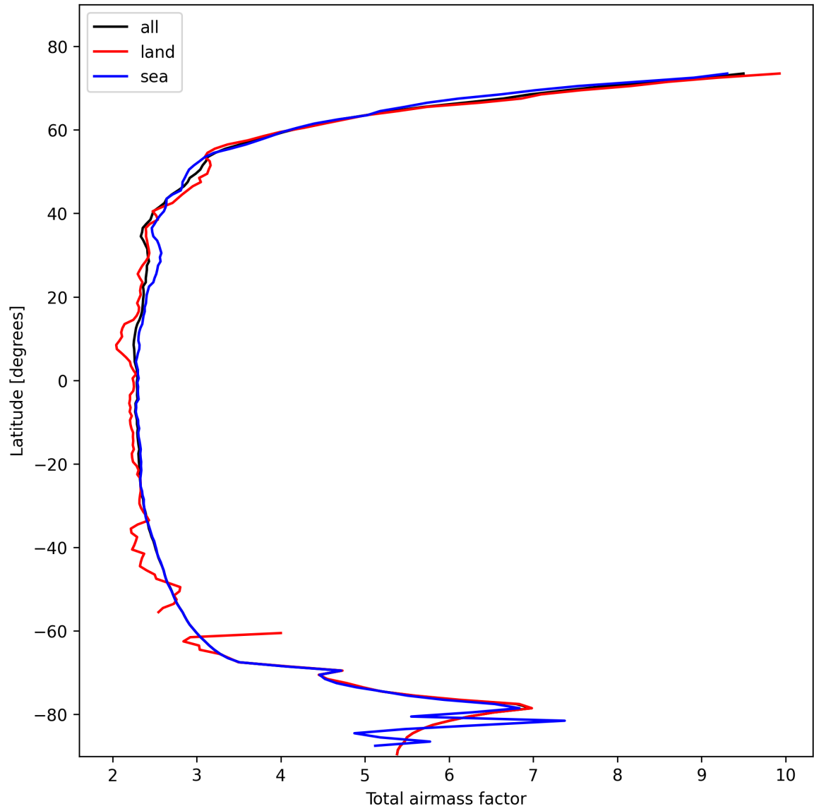
Figure 13: Zonal average of “Total airmass factor” for 2025-02-10 to 2025-02-11.
