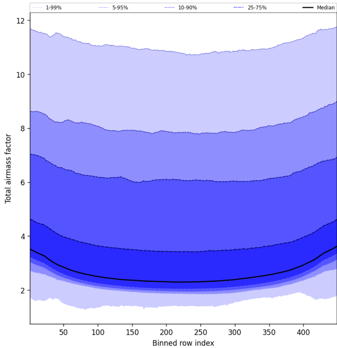
Figure 47: Along track statistics of “Total airmass factor” for 2025-02-10 to 2025-02-11
