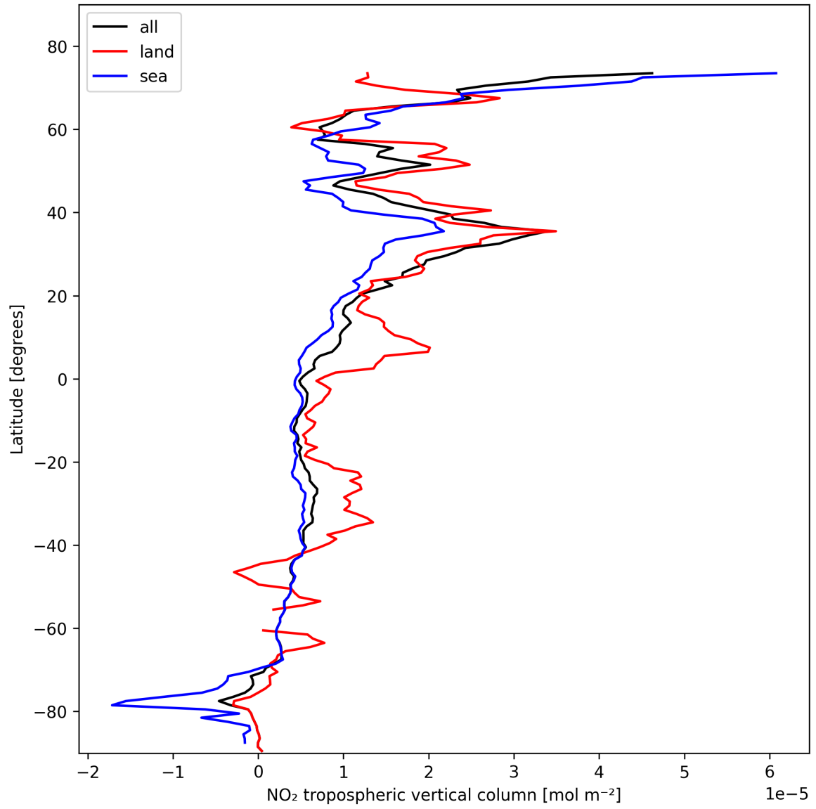
Figure 10: Zonal average of “NO 2 tropospheric vertical column” for 2025-02-10 to 2025-02-11.
