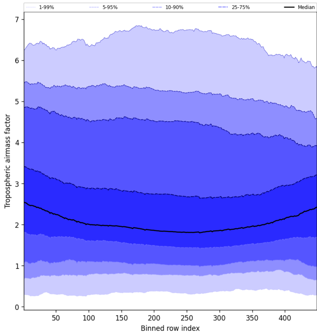
Figure 46: Along track statistics of “Tropospheric airmass factor” for 2025-02-10 to 2025-02-11
