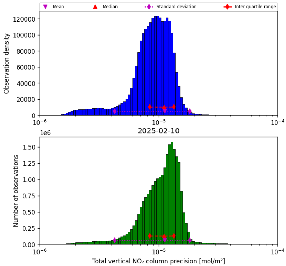
Figure 37: Histogram of “Total vertical NO 2 column precision” for 2025-02-10 to 2025-02-11
