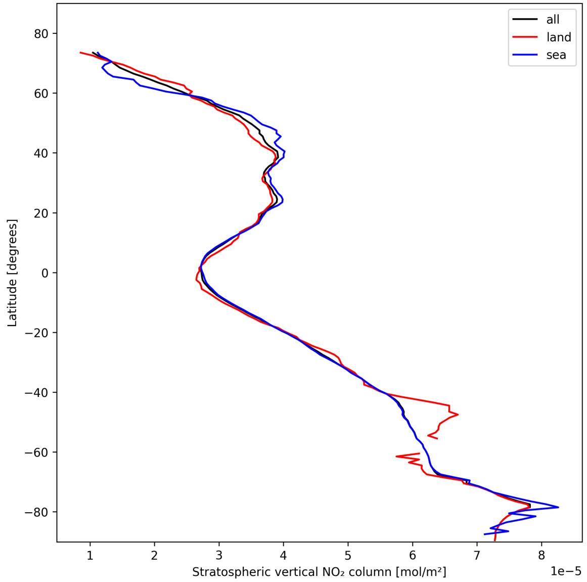
Figure 17: Zonal average of “Stratospheric vertical NO 2 column” for 2025-02-10 to 2025-02-11.
