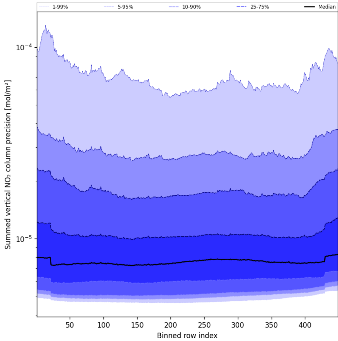
Figure 56: Along track statistics of “Summed vertical NO 2 column precision” for 2025-02-10 to 2025-02-11
