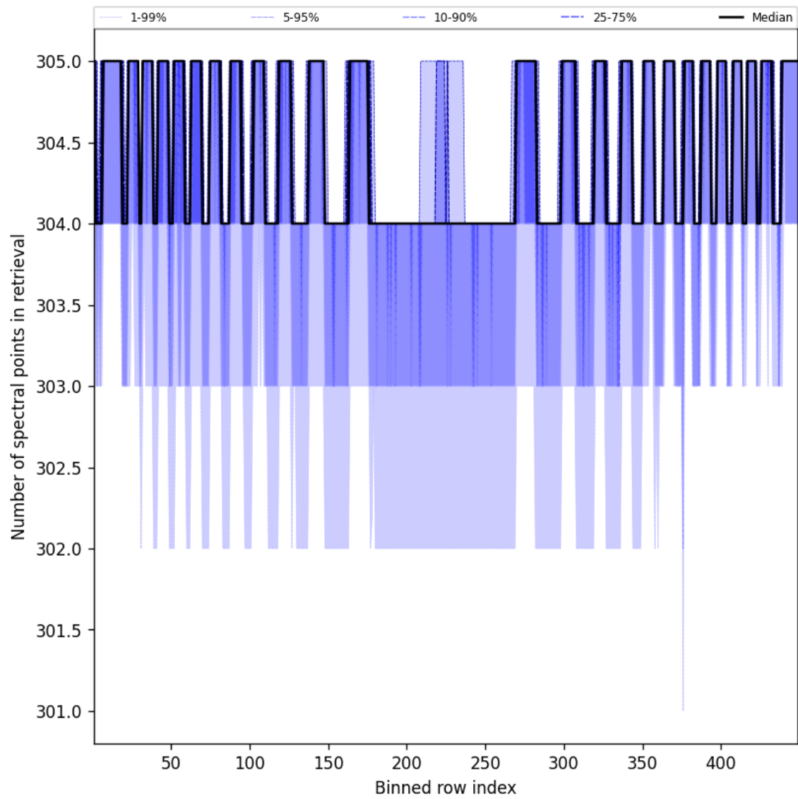
Figure 48: Along track statistics of “Number of spectral points in retrieval” for 2025-02-10 to 2025-02-11
