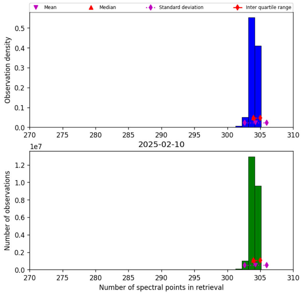
Figure 31: Histogram of “Number of spectral points in retrieval” for 2025-02-10 to 2025-02-11
