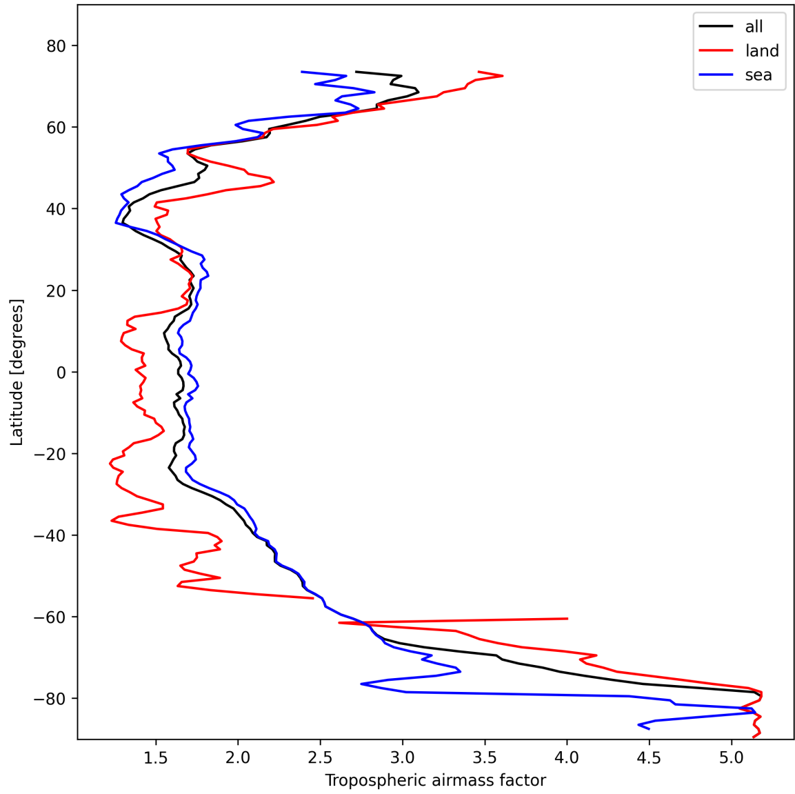
Figure 12: Zonal average of “Tropospheric airmass factor” for 2025-02-10 to 2025-02-11.
