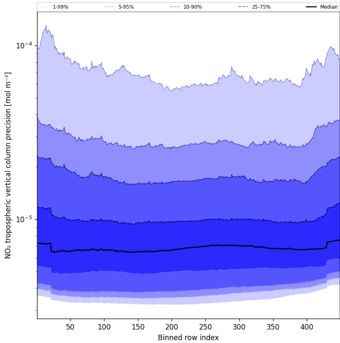
Figure 45: Along track statistics of “NO 2 tropospheric vertical column precision” for 2025-02-10 to 2025-02-11
