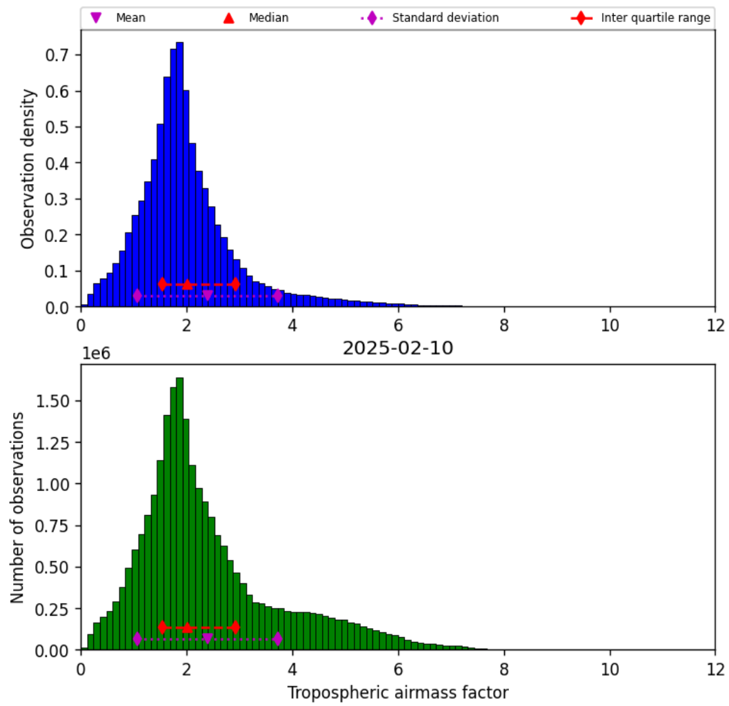
Figure 29: Histogram of “Tropospheric airmass factor” for 2025-02-10 to 2025-02-11
