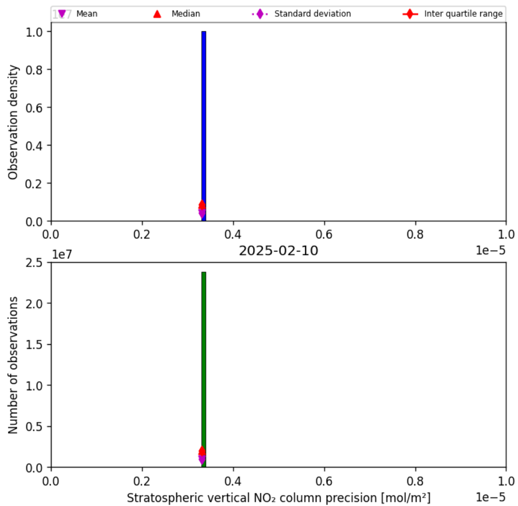
Figure 35: Histogram of “Stratospheric vertical NO 2 column precision” for 2025-02-10 to 2025-02-11
