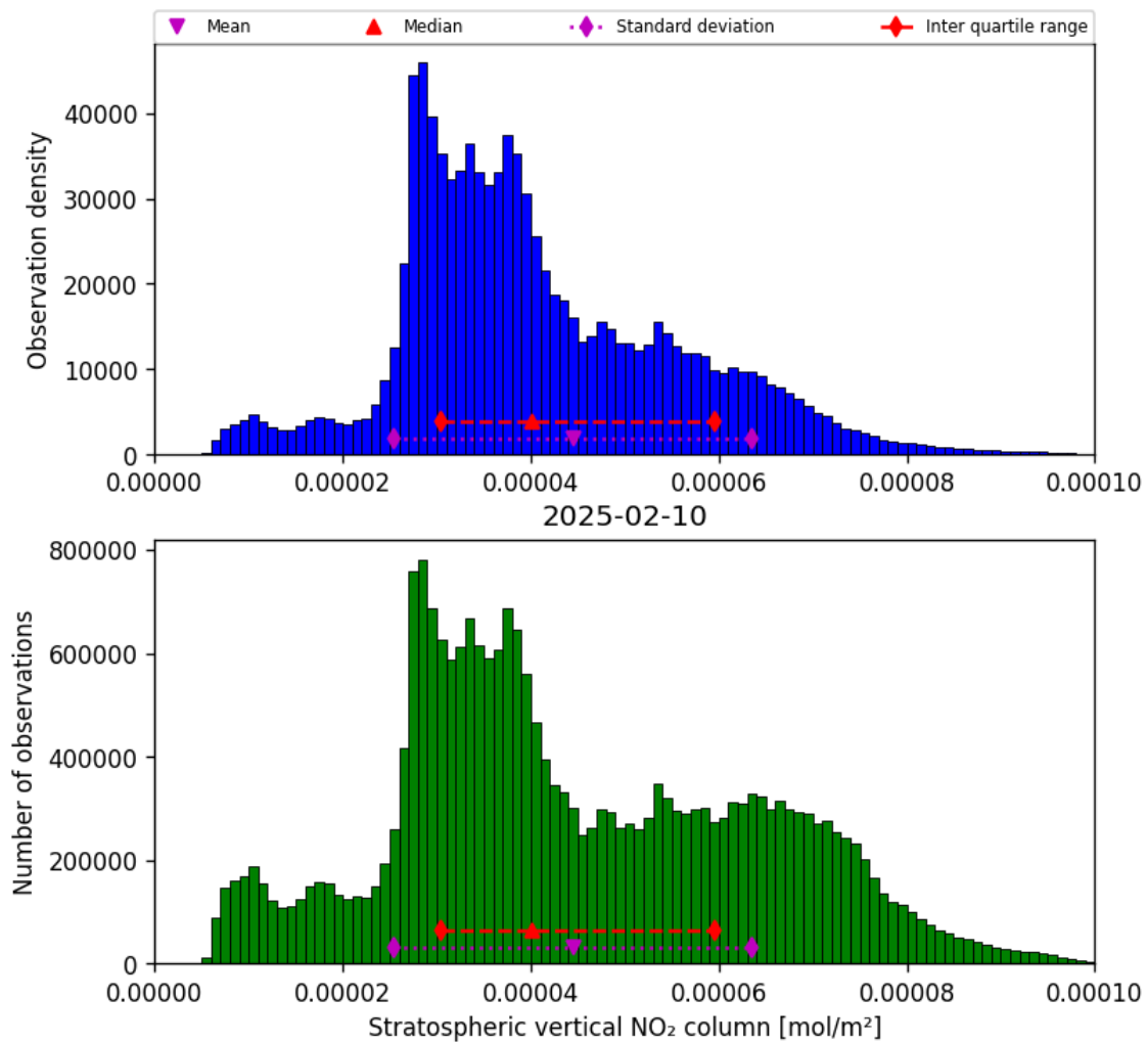
Figure 34: Histogram of “Stratospheric vertical NO 2 column” for 2025-02-10 to 2025-02-11
