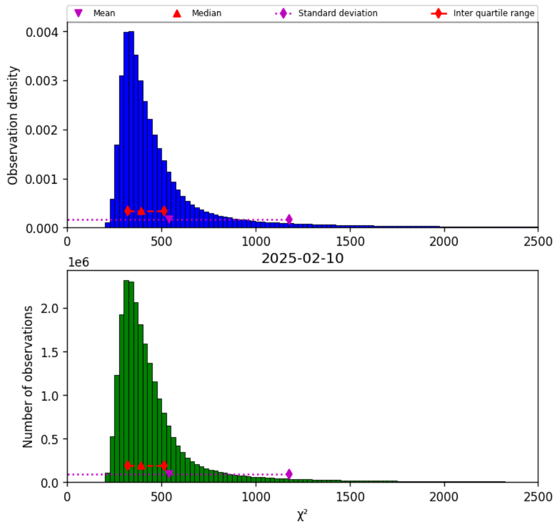
Figure 40: Histogram of “ \chi^2 ” for 2025-02-10 to 2025-02-11
