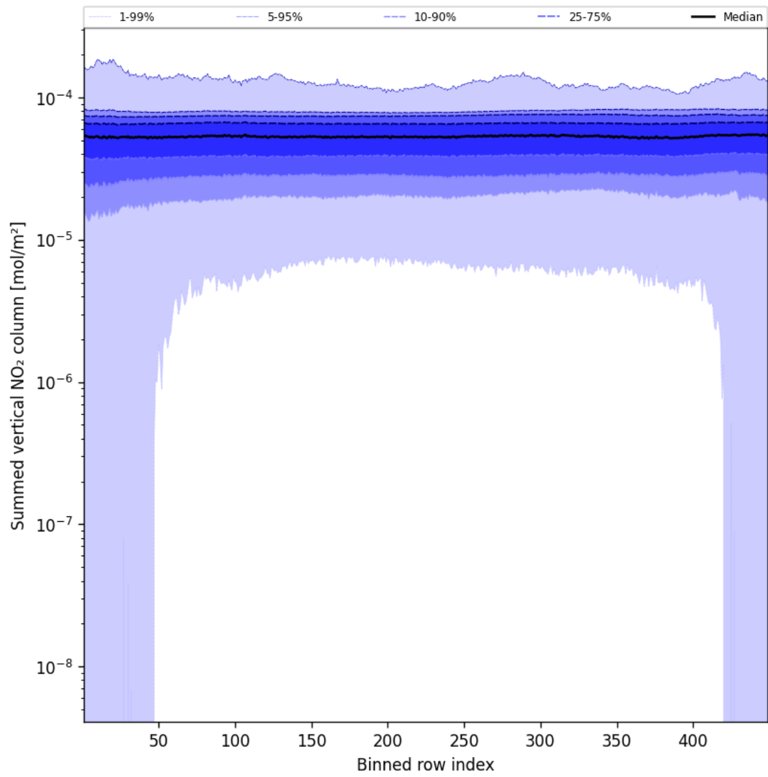
Figure 55: Along track statistics of “Summed vertical NO 2 column” for 2025-02-10 to 2025-02-11
