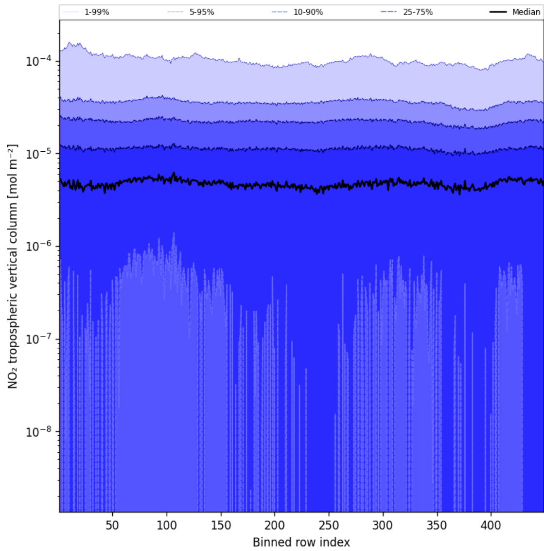
Figure 44: Along track statistics of “NO 2 tropospheric vertical column” for 2025-02-10 to 2025-02-11
