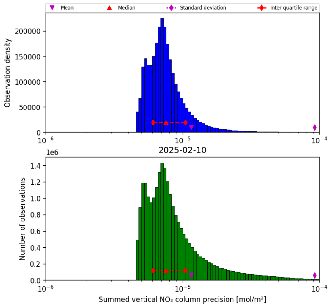
Figure 39: Histogram of “Summed vertical NO 2 column precision” for 2025-02-10 to 2025-02-11
