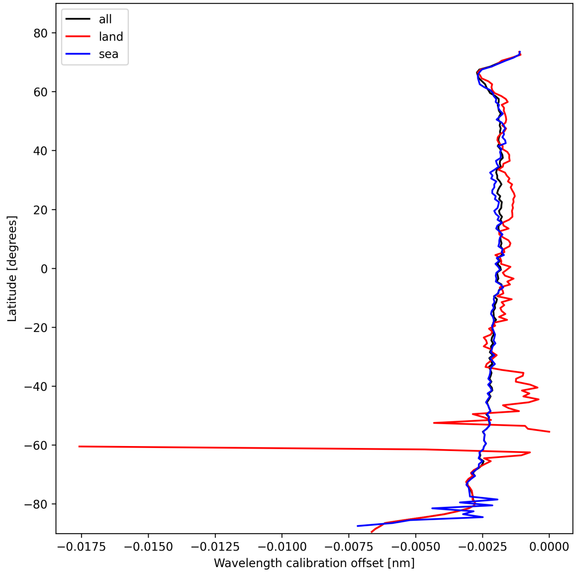
Figure 16: Zonal average of “Wavelength calibration offset” for 2025-02-10 to 2025-02-11.
