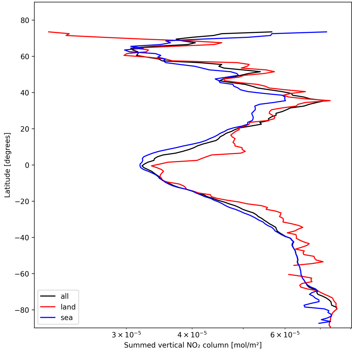
Figure 21: Zonal average of “Summed vertical NO 2 column” for 2025-02-10 to 2025-02-11.
