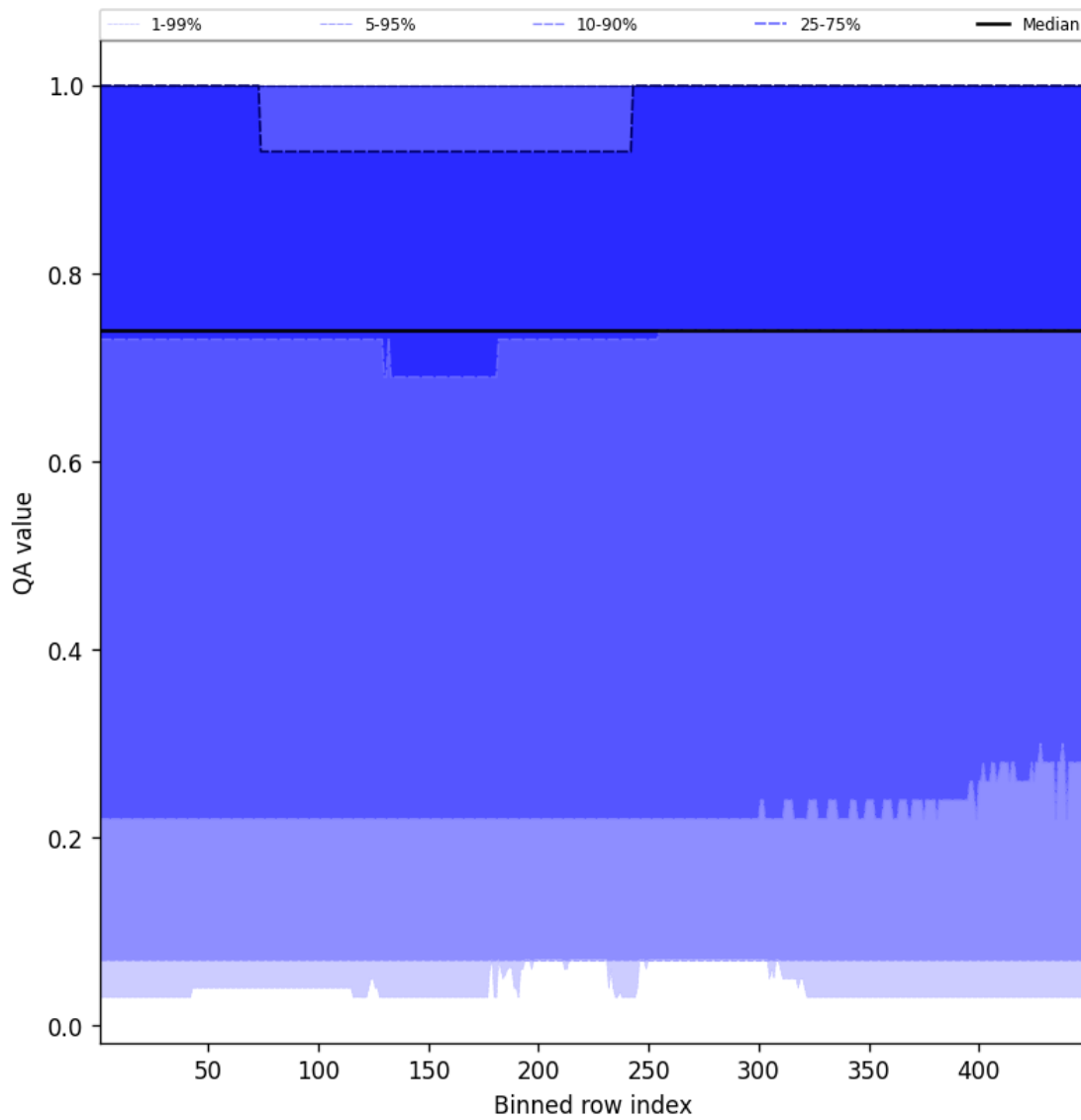
Figure 43: Along track statistics of “QA value” for 2025-02-10 to 2025-02-11
