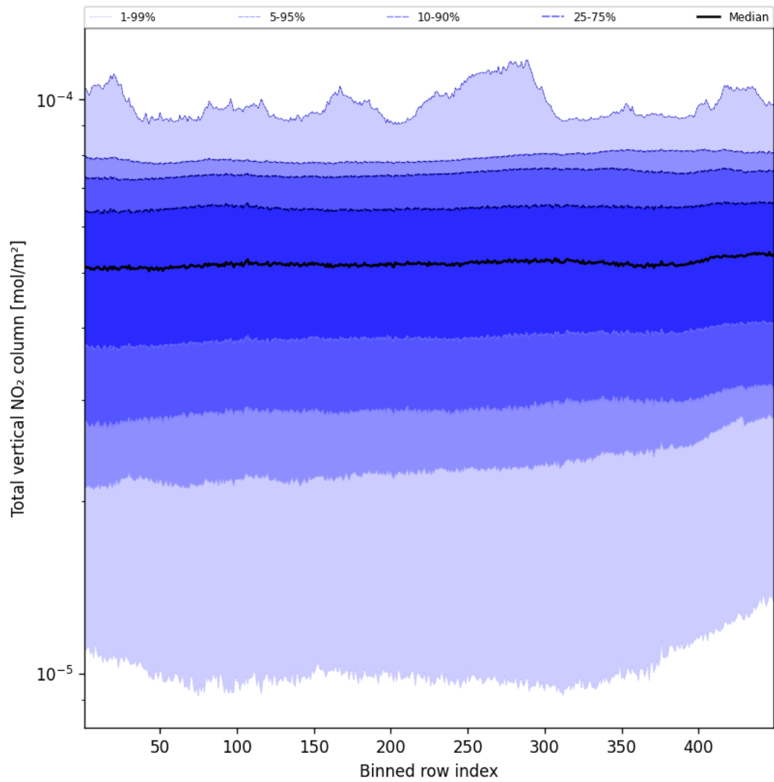
Figure 53: Along track statistics of “Total vertical NO 2 column” for 2025-02-10 to 2025-02-11
