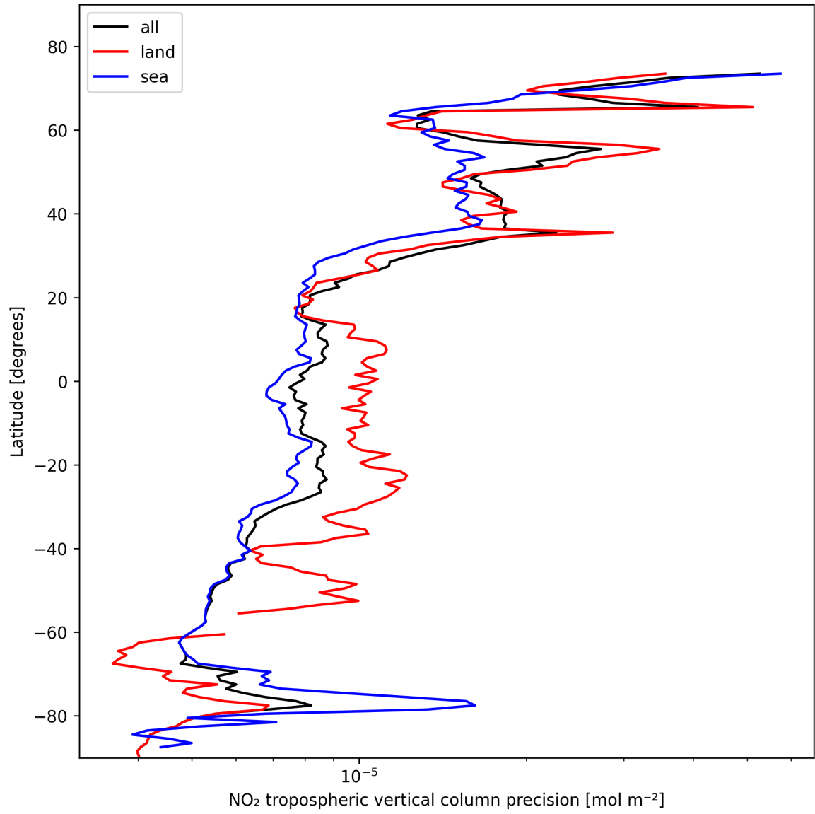
Figure 11: Zonal average of “NO 2 tropospheric vertical column precision” for 2025-02-10 to 2025-02-11.
