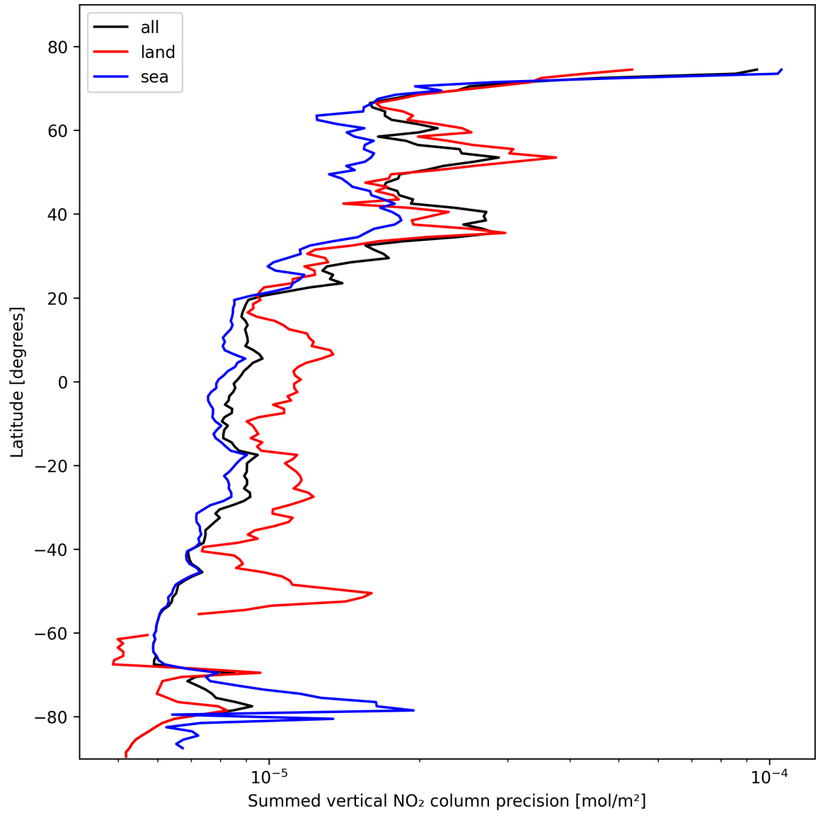
Figure 22: Zonal average of “Summed vertical NO 2 column precision” for 2025-02-12 to 2025-02-13.
