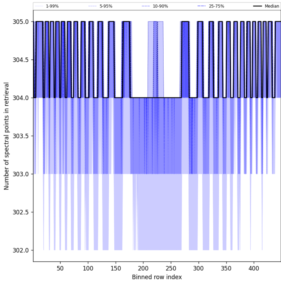
Figure 48: Along track statistics of “Number of spectral points in retrieval” for 2025-02-12 to 2025-02-13
