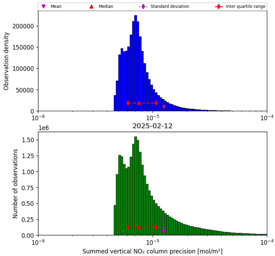
Figure 39: Histogram of “Summed vertical NO 2 column precision” for 2025-02-12 to 2025-02-13
