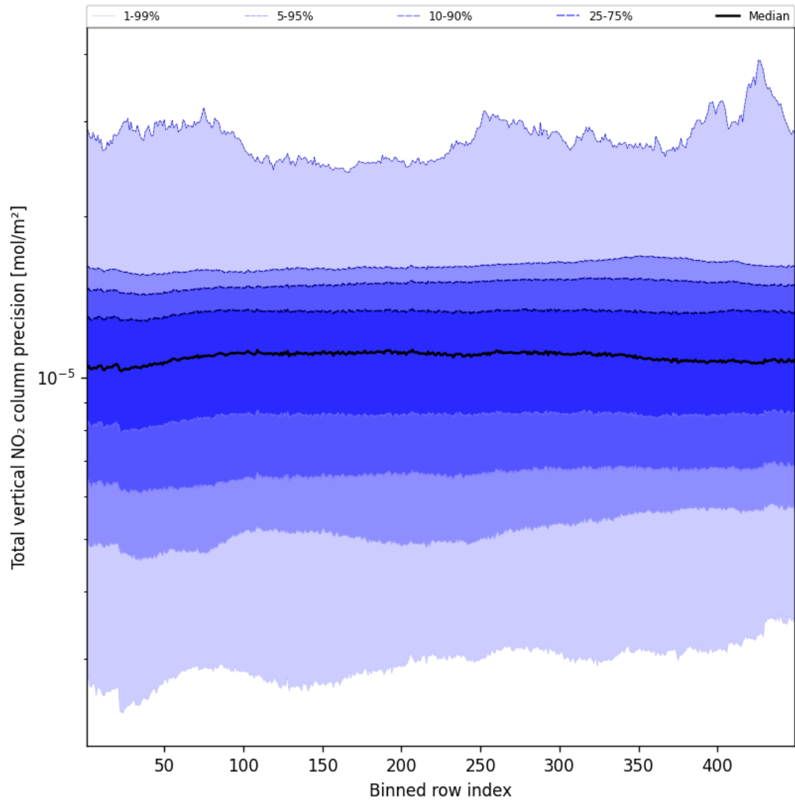
Figure 54: Along track statistics of “Total vertical NO 2 column precision” for 2025-02-12 to 2025-02-13
