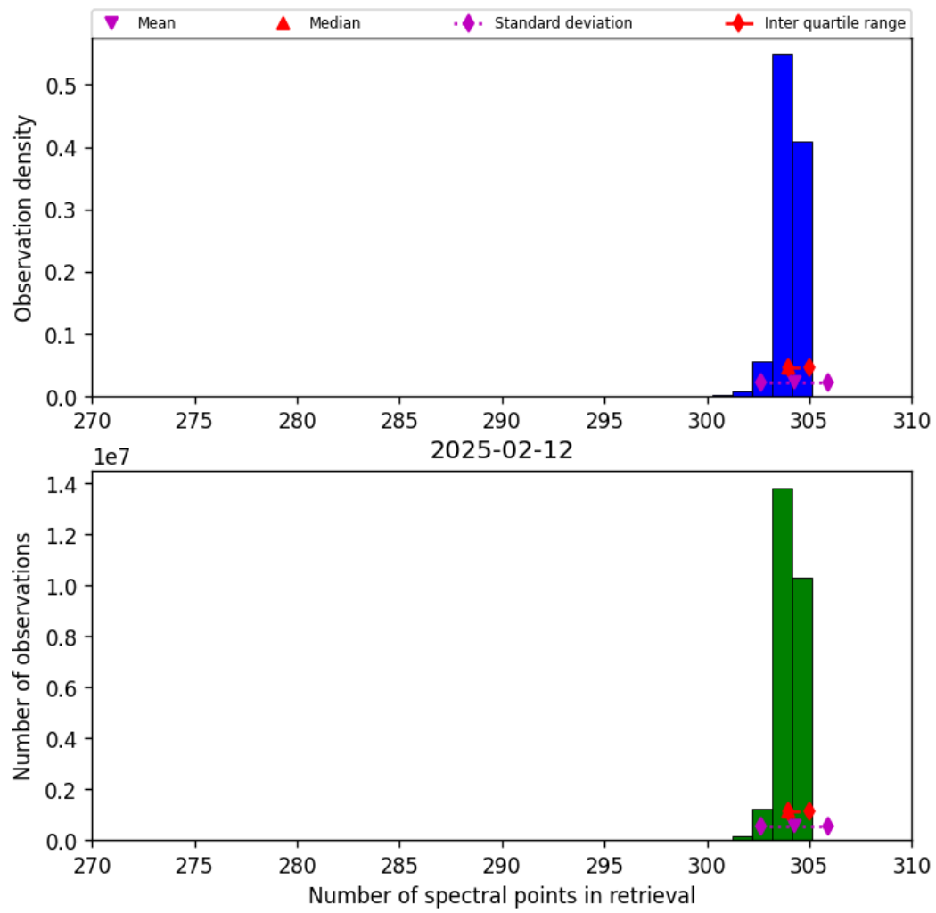
Figure 31: Histogram of “Number of spectral points in retrieval” for 2025-02-12 to 2025-02-13
