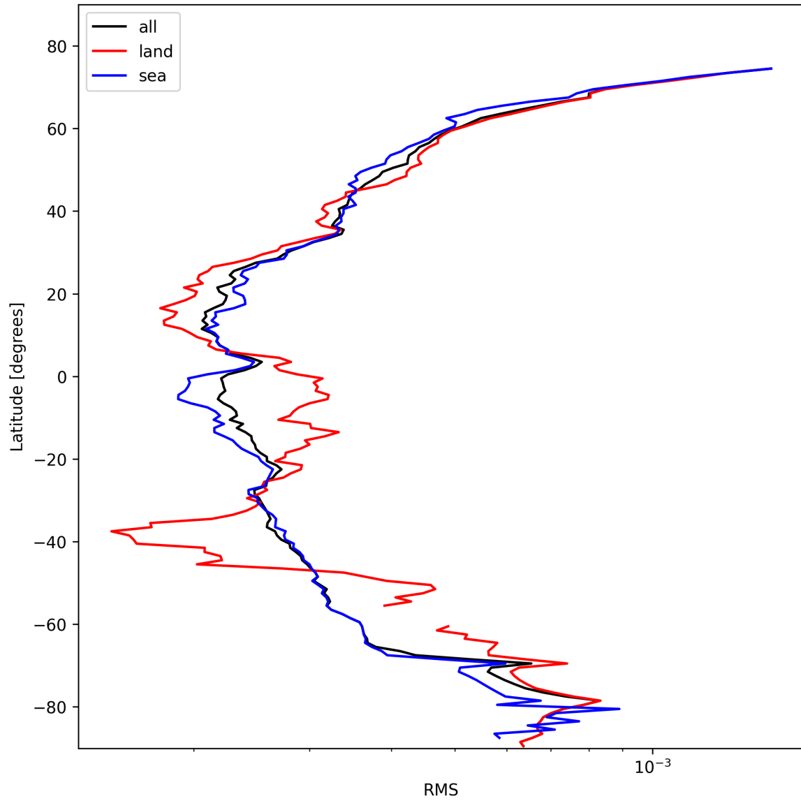
Figure 24: Zonal average of “RMS” for 2025-02-12 to 2025-02-13.
