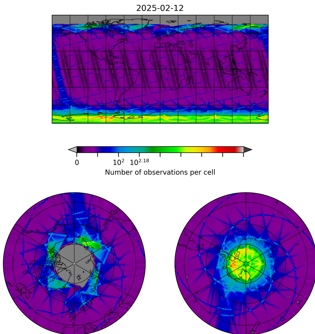
Figure 8: Map of the number of observations for 2025-02-12 to 2025-02-13
