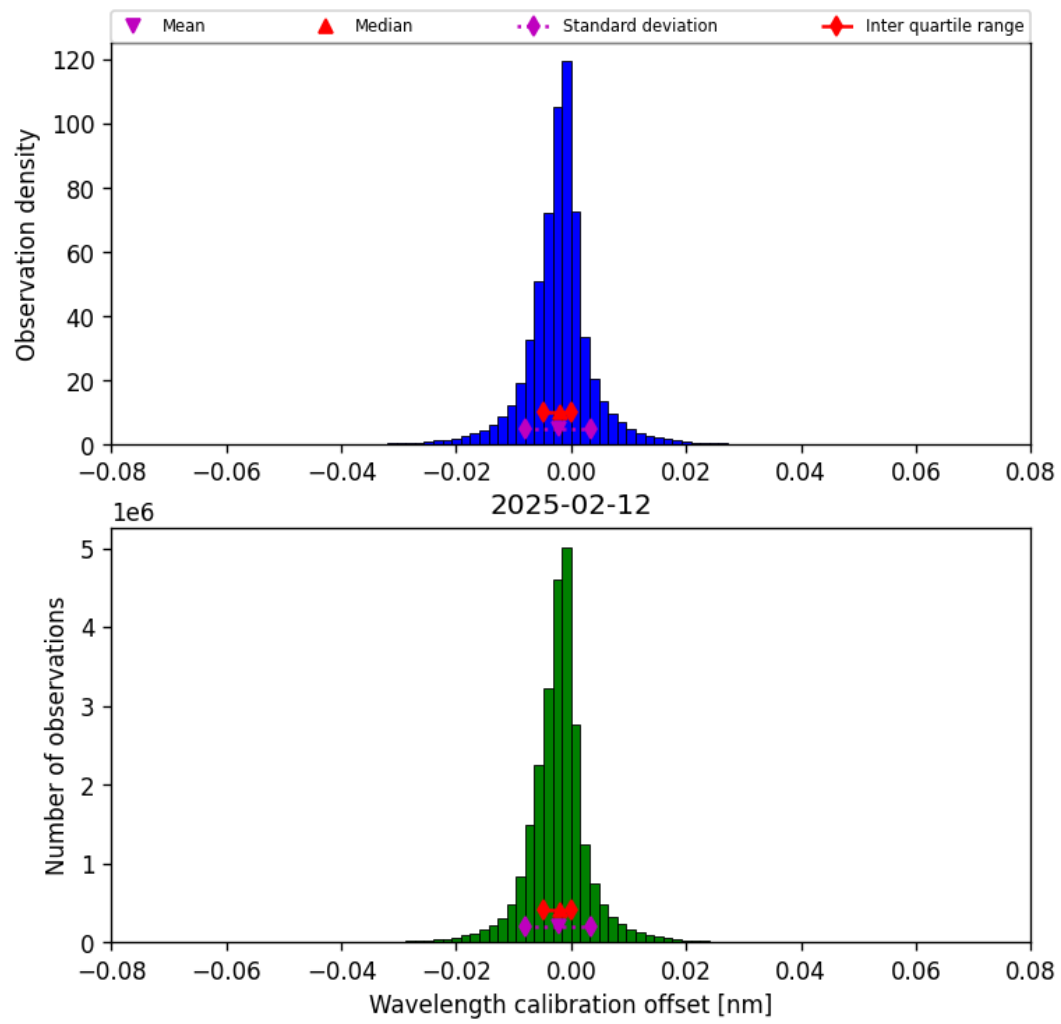
Figure 33: Histogram of “Wavelength calibration offset” for 2025-02-12 to 2025-02-13
