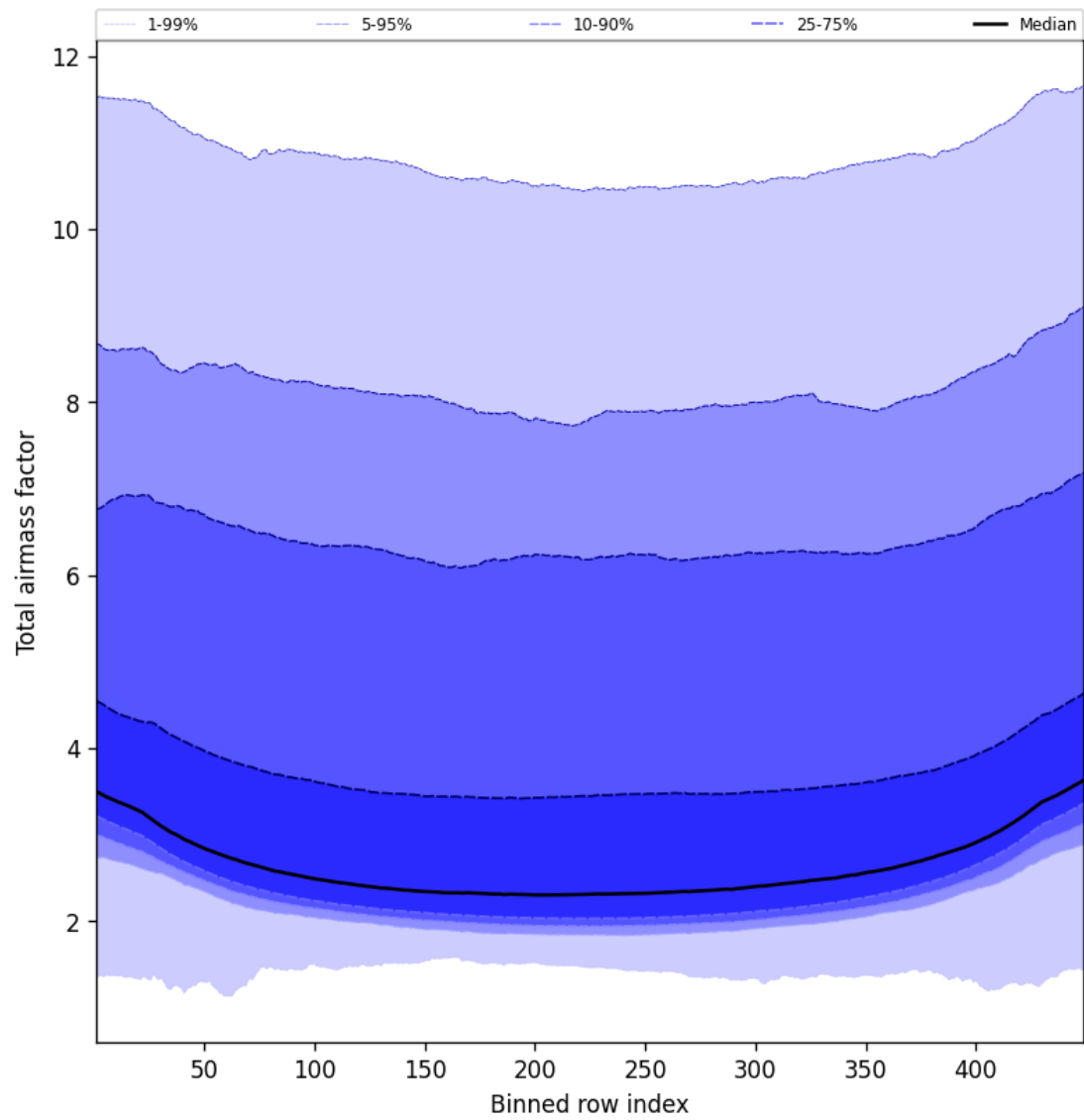
Figure 47: Along track statistics of “Total airmass factor” for 2025-02-12 to 2025-02-13
