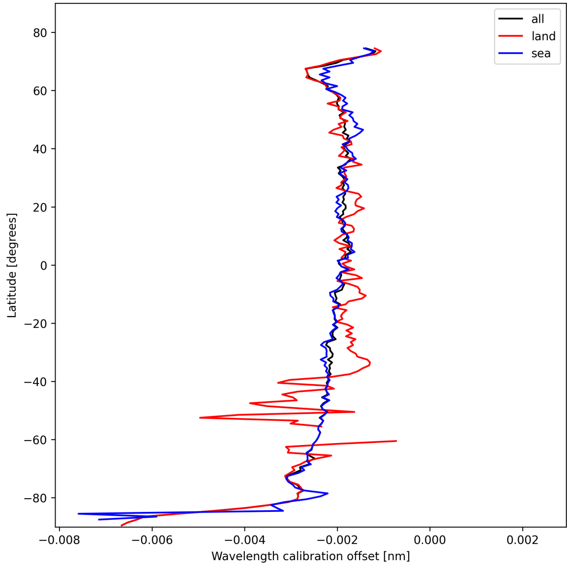
Figure 16: Zonal average of “Wavelength calibration offset” for 2025-02-12 to 2025-02-13.
