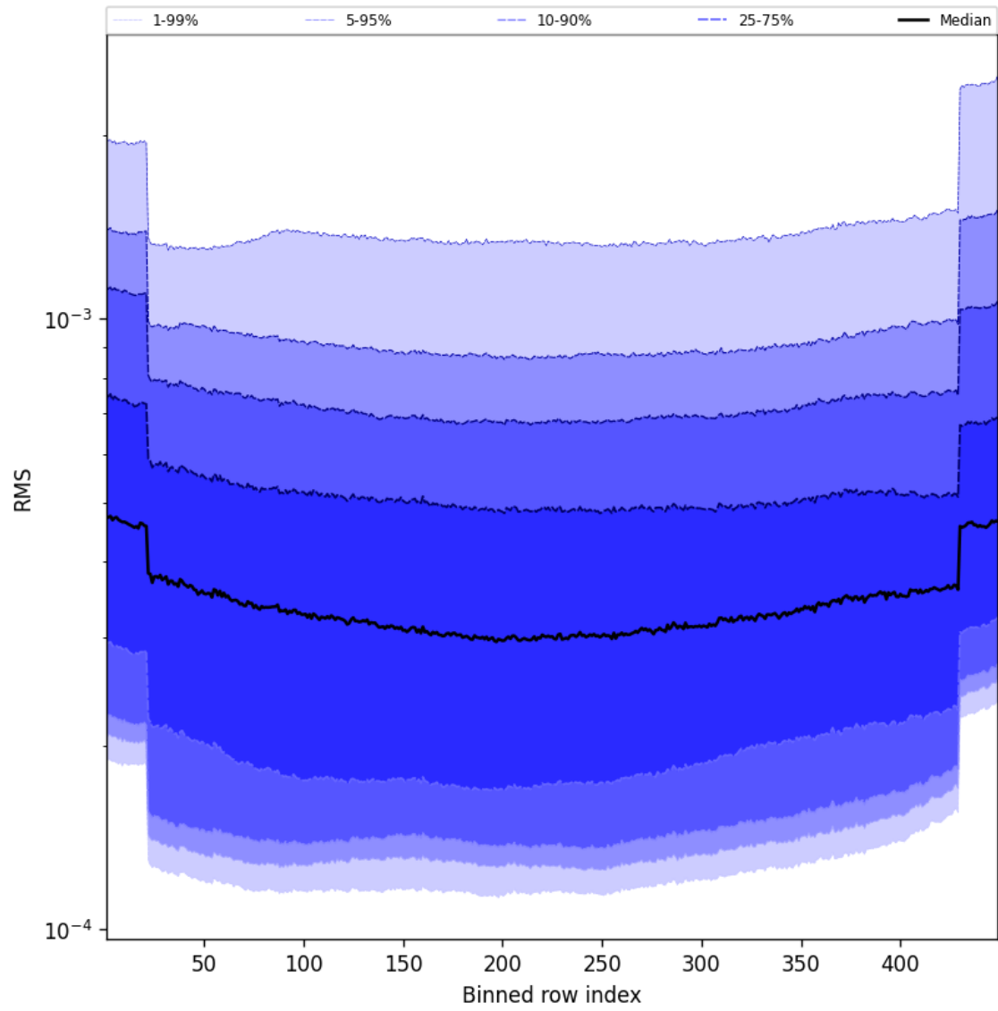
Figure 58: Along track statistics of “RMS” for 2025-02-12 to 2025-02-13
