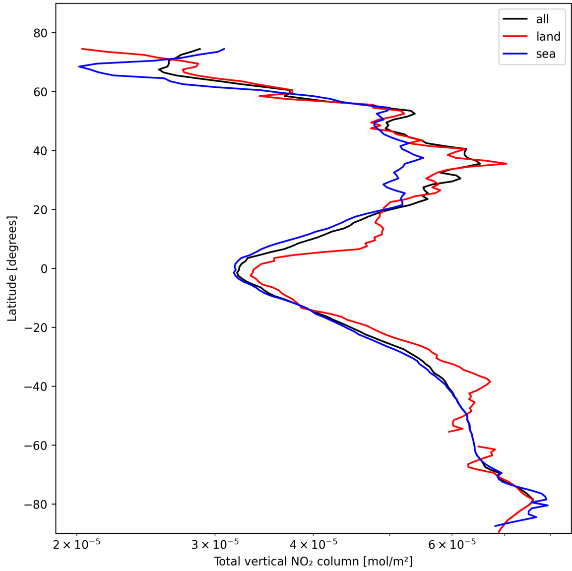
Figure 19: Zonal average of “Total vertical NO 2 column” for 2025-02-12 to 2025-02-13.
