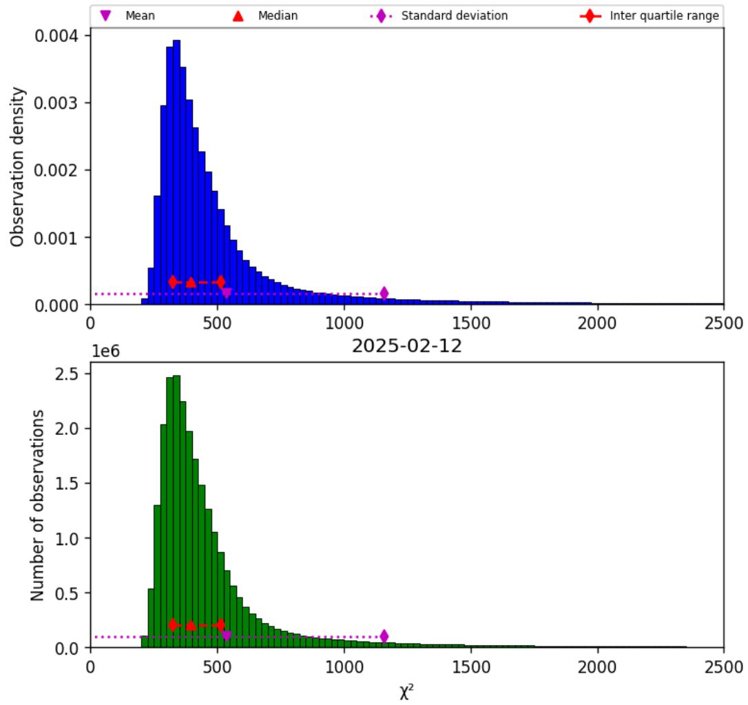
Figure 40: Histogram of “ \chi^2 ” for 2025-02-12 to 2025-02-13
