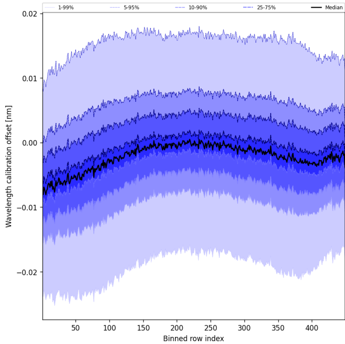
Figure 50: Along track statistics of “Wavelength calibration offset” for 2025-02-12 to 2025-02-13
