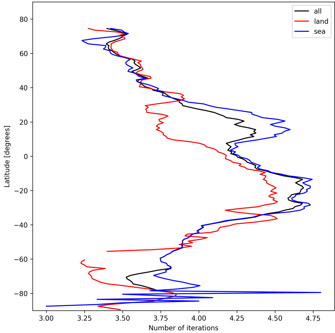
Figure 15: Zonal average of “Number of iterations” for 2025-02-12 to 2025-02-13.
