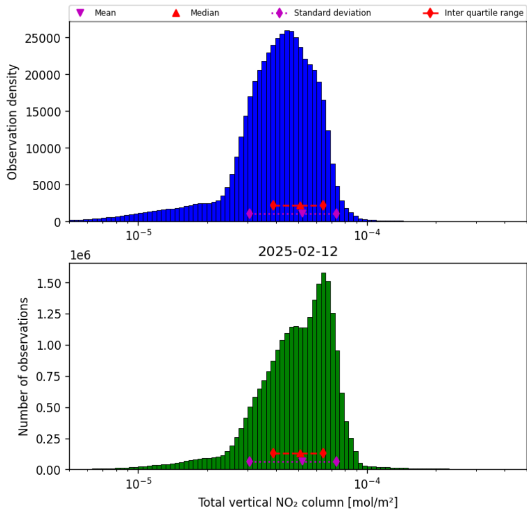
Figure 36: Histogram of "Total vertical NO 2 column" for 2025-02-12 to 2025-02-13
