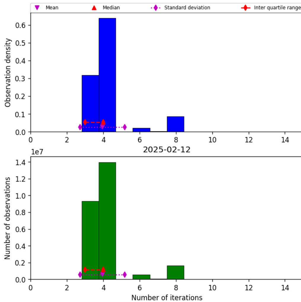
Figure 32: Histogram of “Number of iterations” for 2025-02-12 to 2025-02-13
