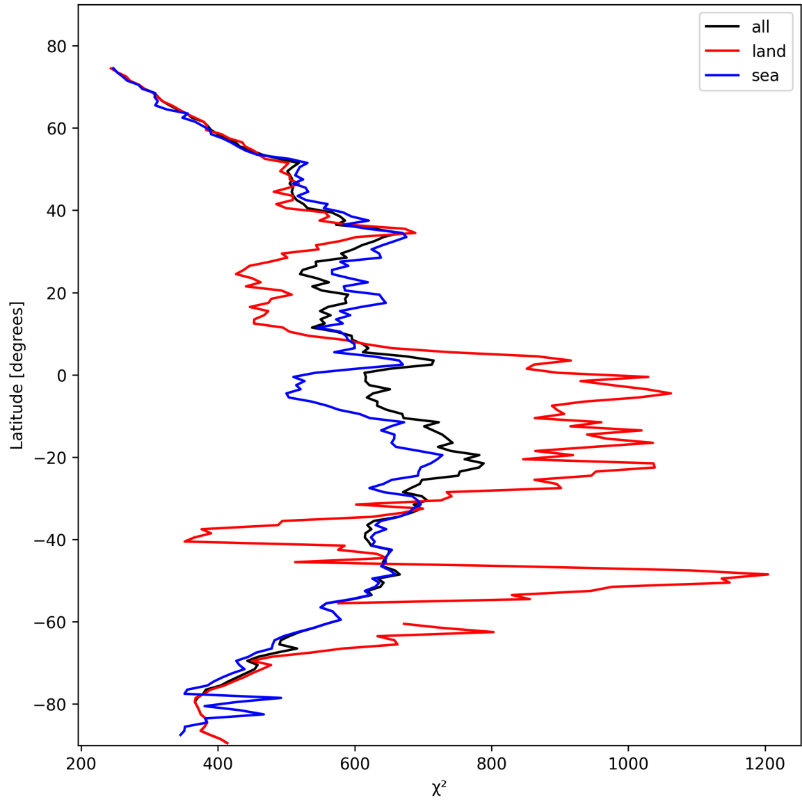
Figure 23: Zonal average of “ \chi^2 ” for 2025-02-12 to 2025-02-13.
