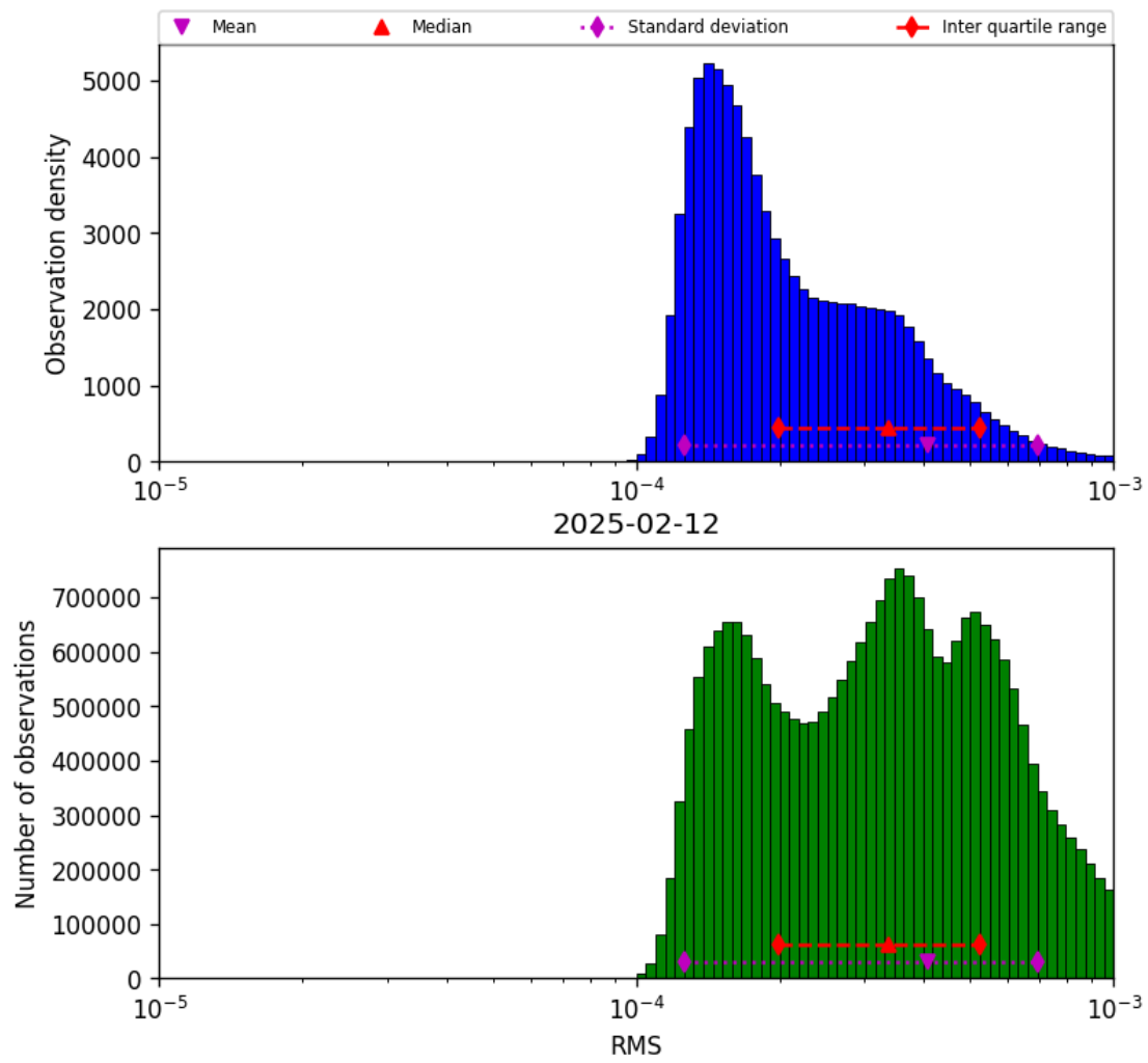
Figure 41: Histogram of “RMS” for 2025-02-12 to 2025-02-13
