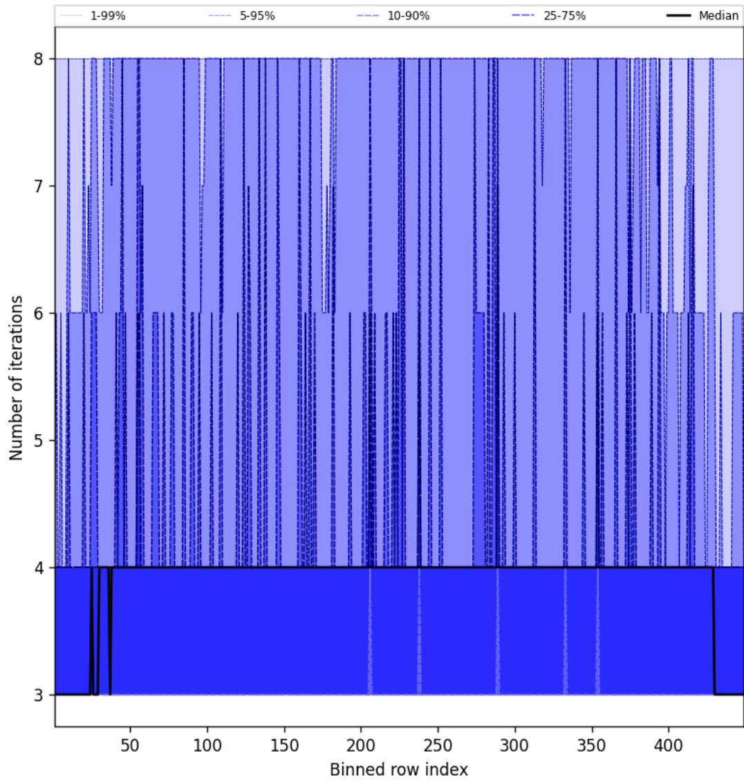
Figure 49: Along track statistics of “Number of iterations” for 2025-02-12 to 2025-02-13
