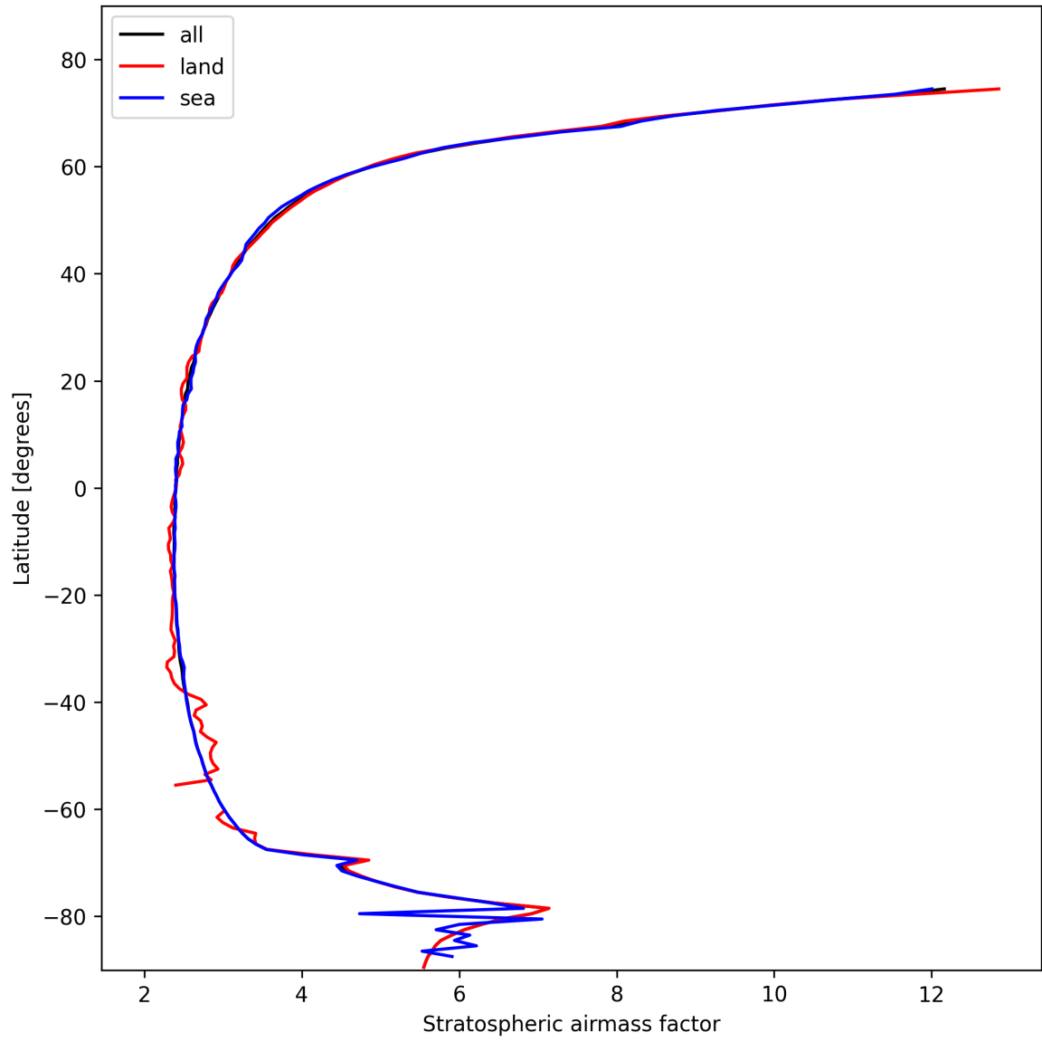
Figure 25: Zonal average of “Stratospheric airmass factor” for 2025-02-12 to 2025-02-13.
