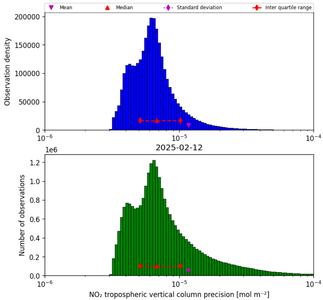
Figure 28: Histogram of “NO 2 tropospheric vertical column precision” for 2025-02-12 to 2025-02-13
