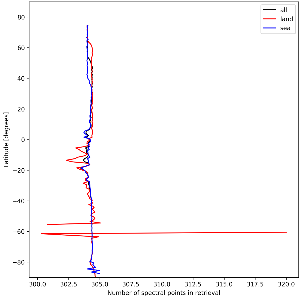
Figure 14: Zonal average of “Number of spectral points in retrieval” for 2025-02-12 to 2025-02-13.
