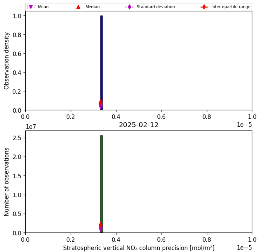
Figure 35: Histogram of “Stratospheric vertical NO 2 column precision” for 2025-02-12 to 2025-02-13
