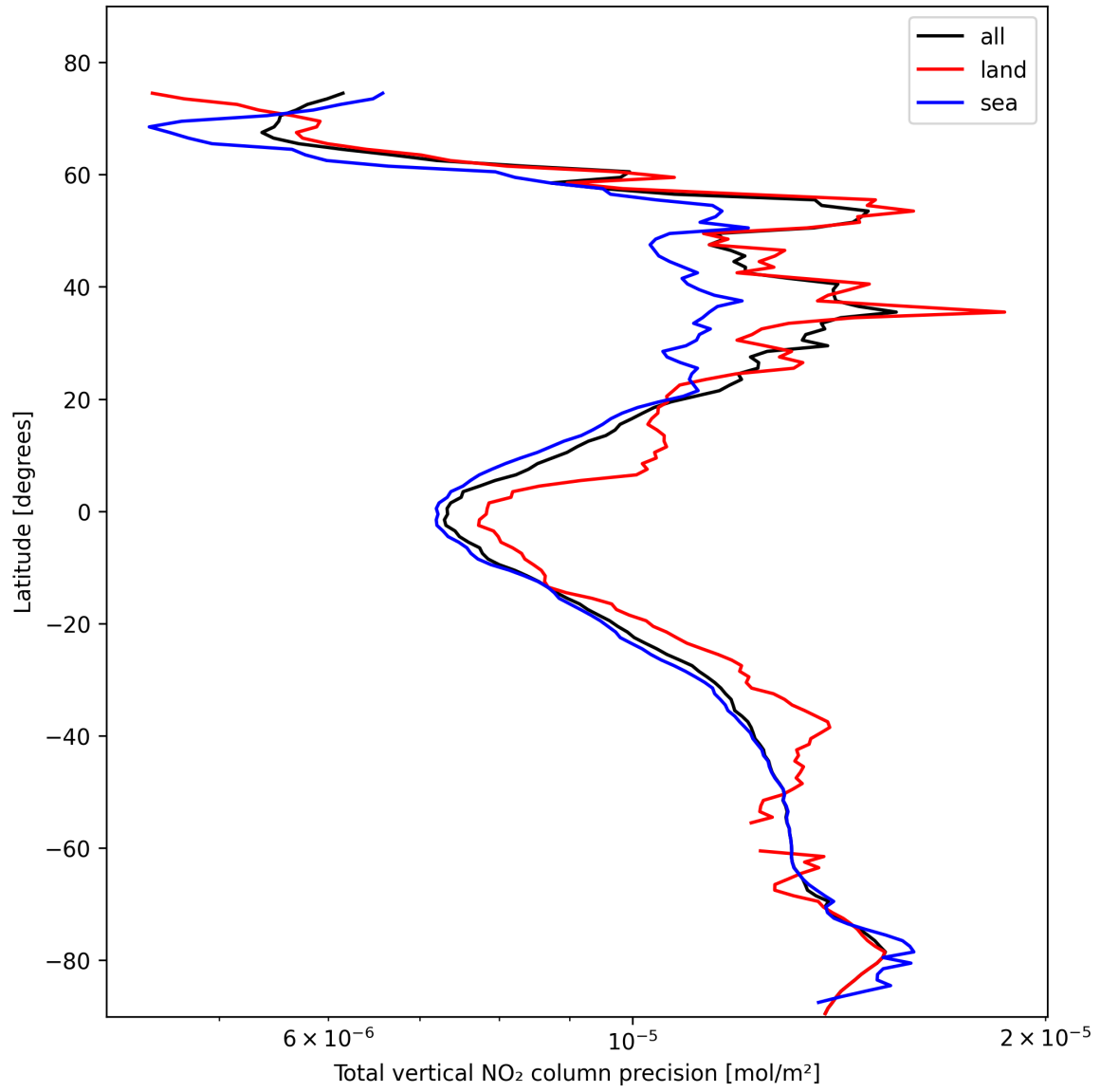
Figure 20: Zonal average of “Total vertical NO 2 column precision” for 2025-02-12 to 2025-02-13.
