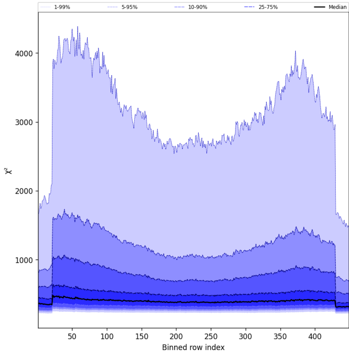
Figure 57: Along track statistics of “ \chi^2 ” for 2025-02-12 to 2025-02-13
