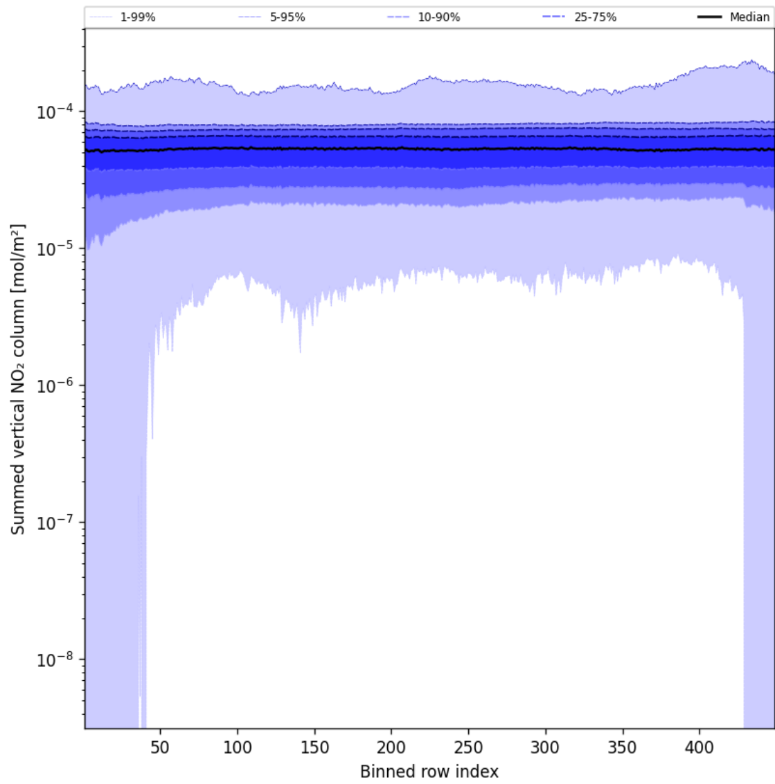
Figure 55: Along track statistics of “Summed vertical NO 2 column” for 2025-02-12 to 2025-02-13
