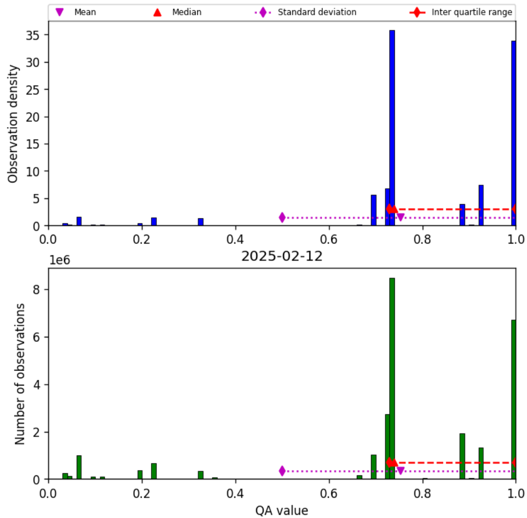
Figure 26: Histogram of “QA value” for 2025-02-12 to 2025-02-13
