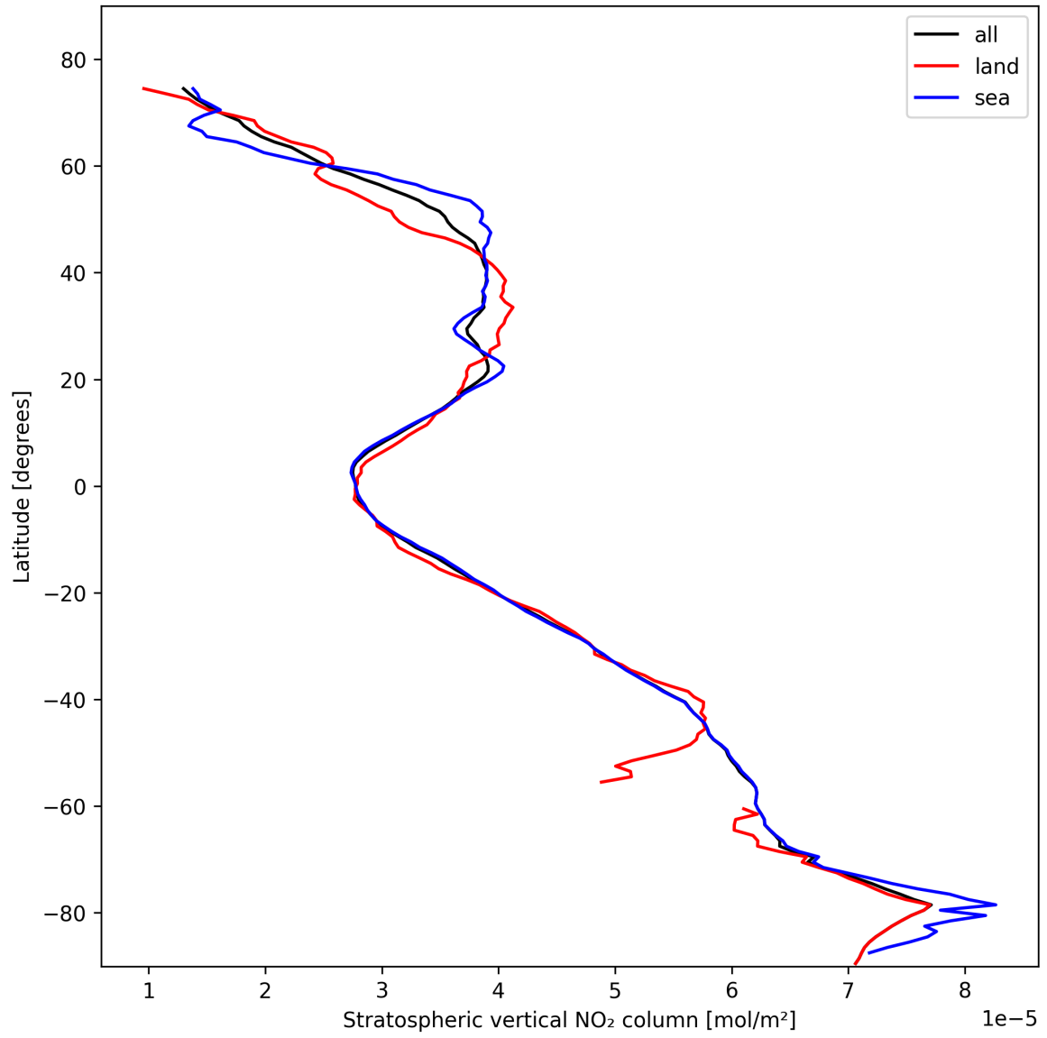
Figure 17: Zonal average of “Stratospheric vertical NO 2 column” for 2025-02-12 to 2025-02-13.
