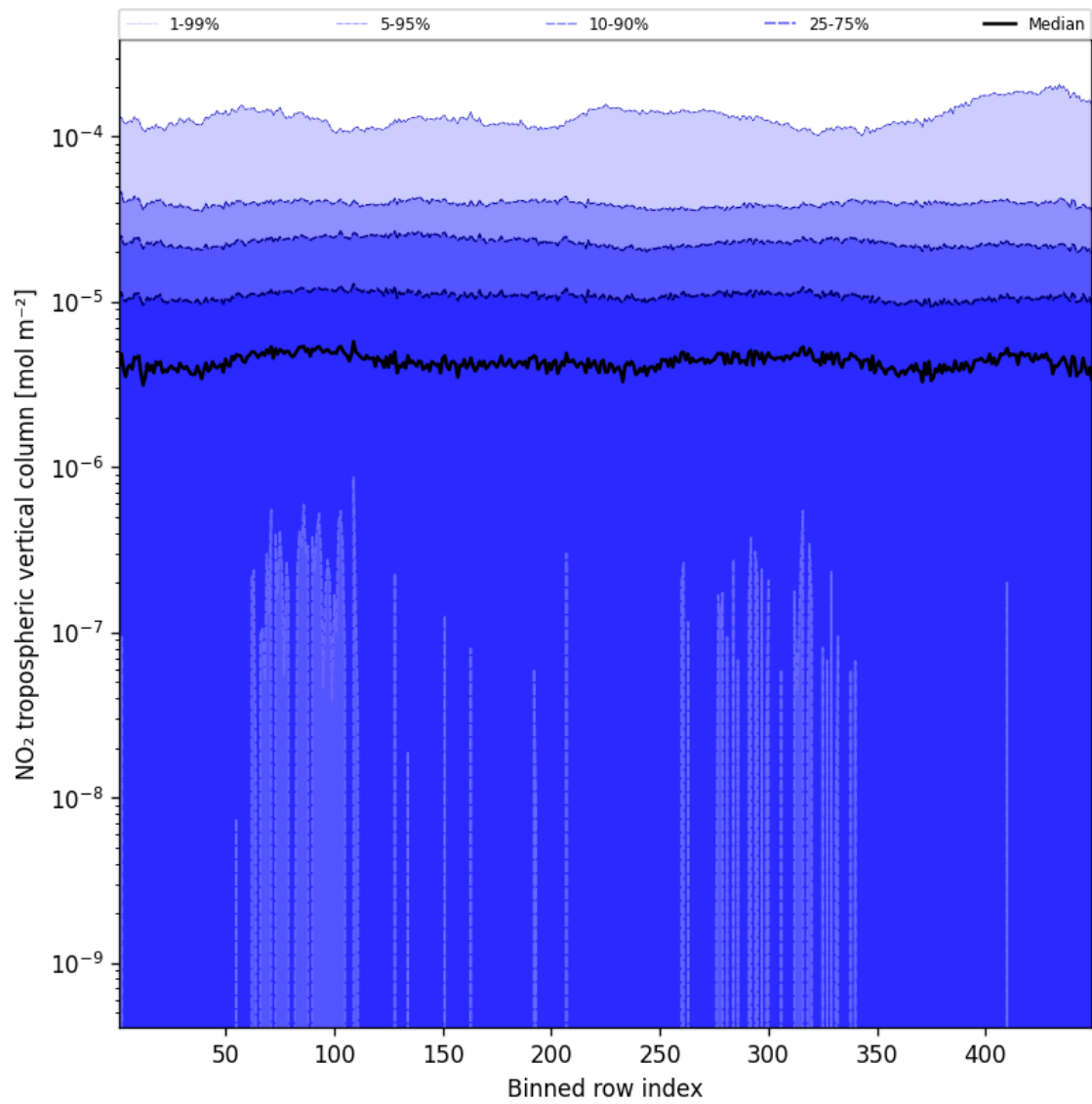
Figure 44: Along track statistics of “NO 2 tropospheric vertical column” for 2025-02-12 to 2025-02-13
