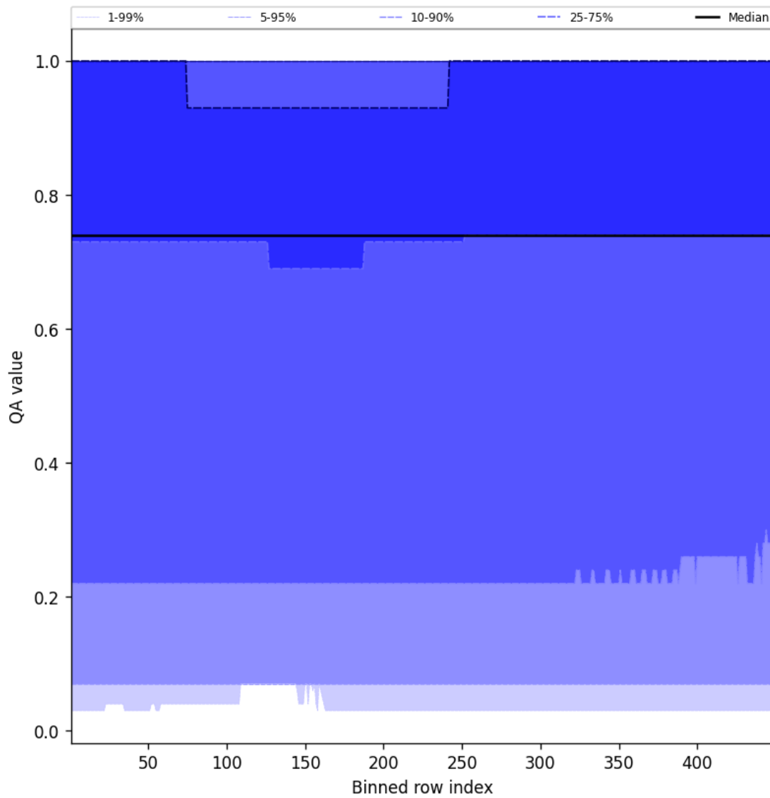
Figure 43: Along track statistics of “QA value” for 2025-02-12 to 2025-02-13
