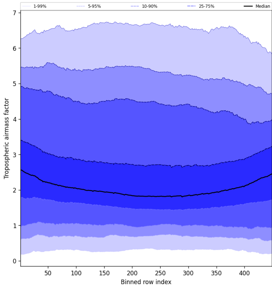
Figure 46: Along track statistics of “Tropospheric airmass factor” for 2025-02-12 to 2025-02-13
