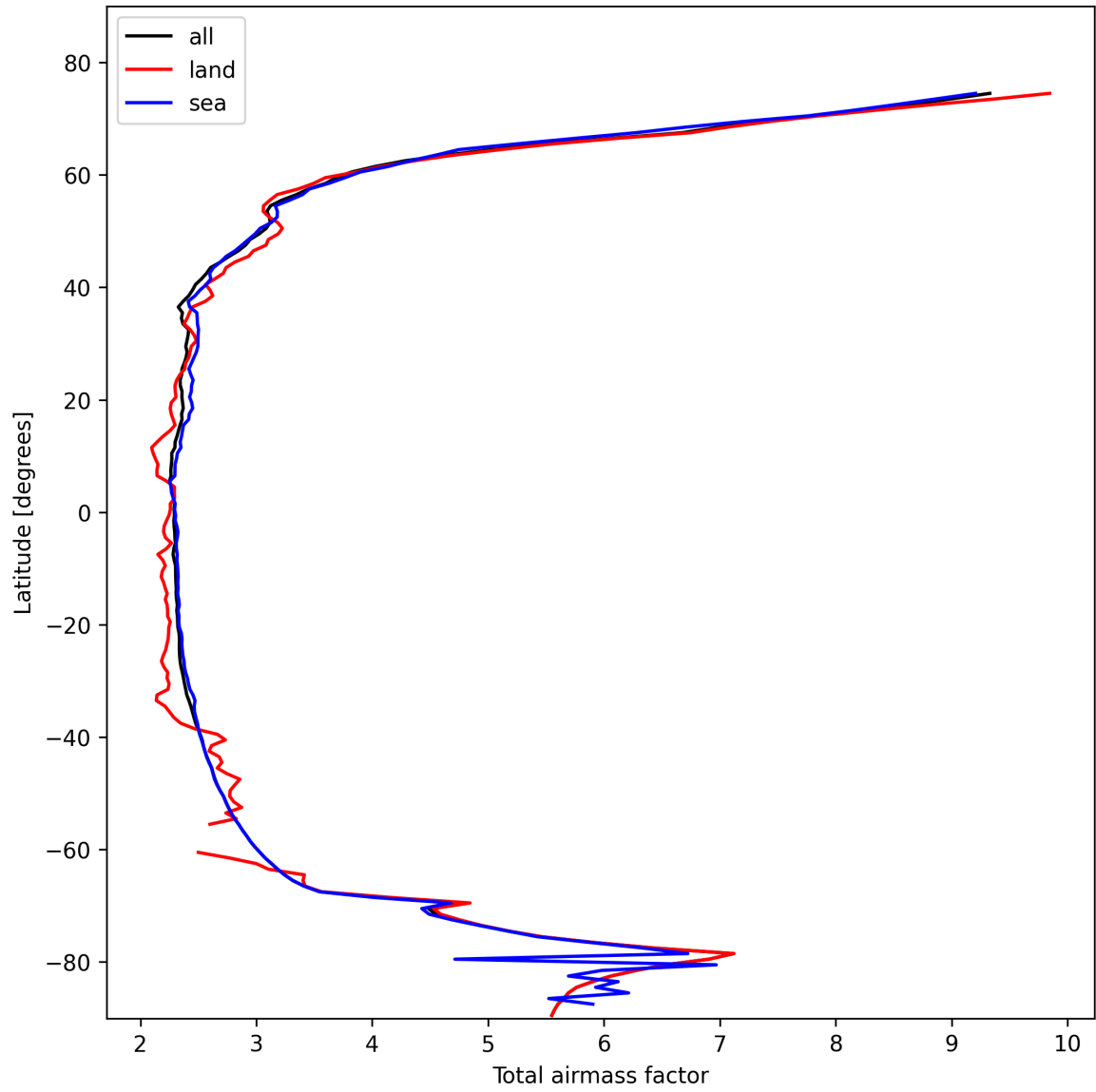
Figure 13: Zonal average of “Total airmass factor” for 2025-02-12 to 2025-02-13.
