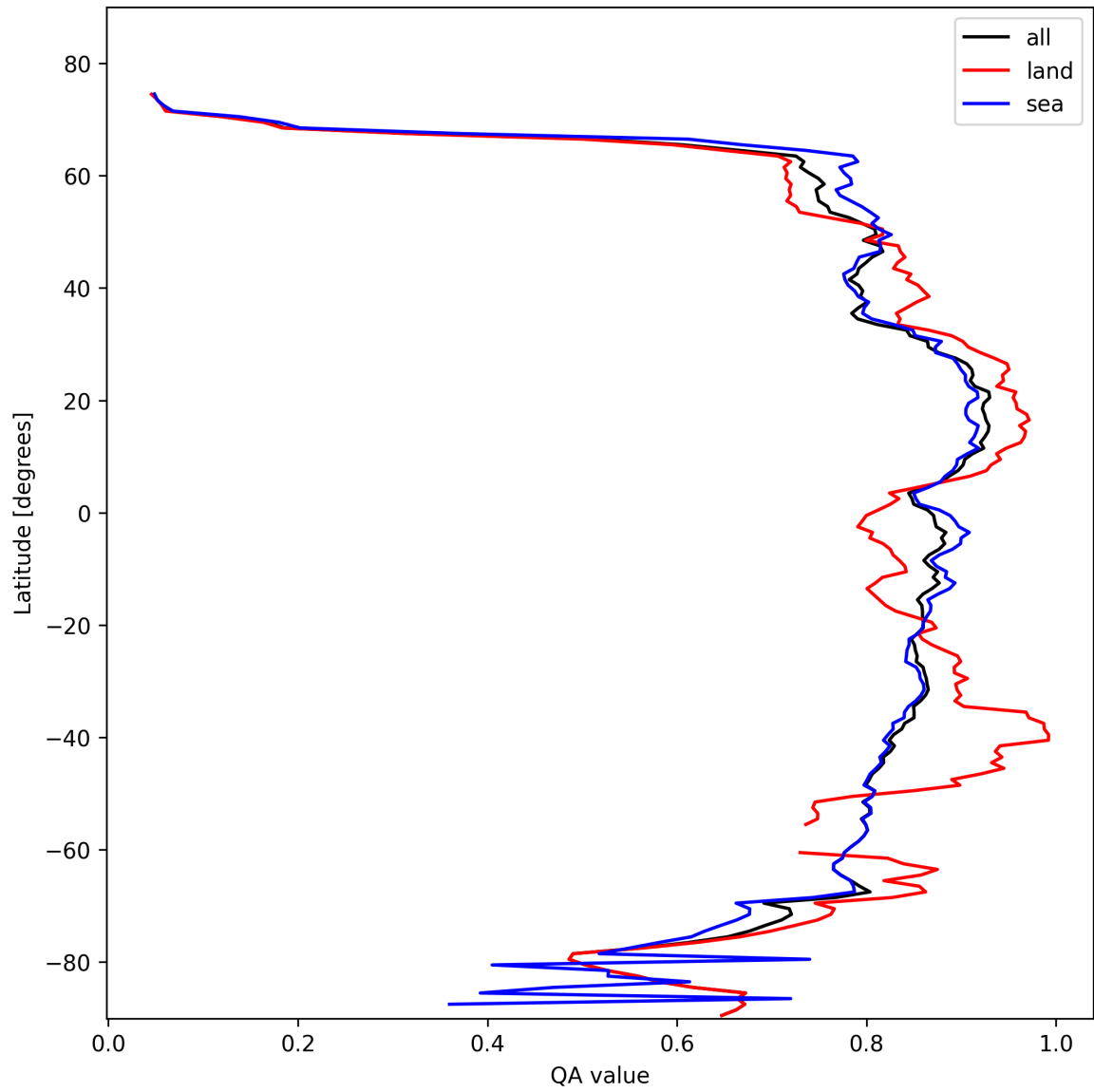
Figure 9: Zonal average of “QA value” for 2025-02-12 to 2025-02-13.
