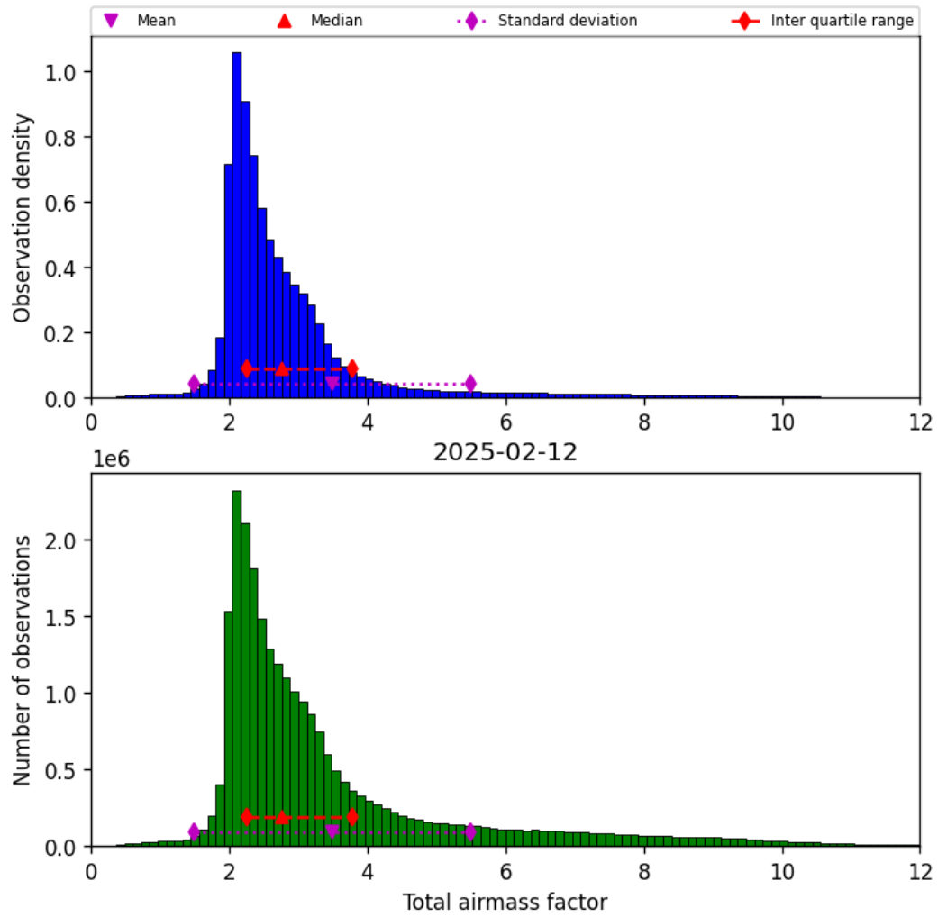
Figure 30: Histogram of “Total airmass factor” for 2025-02-12 to 2025-02-13
