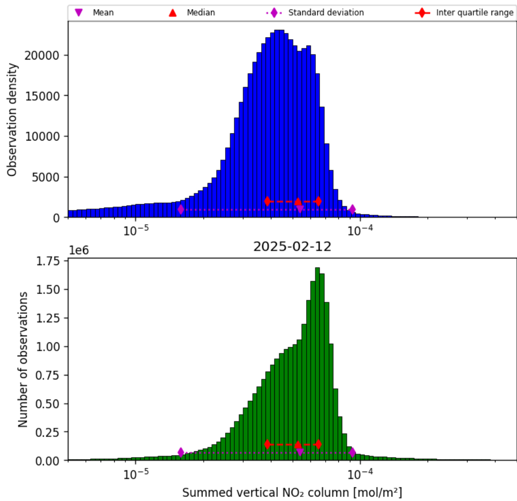
Figure 38: Histogram of “Summed vertical NO 2 column” for 2025-02-12 to 2025-02-13
