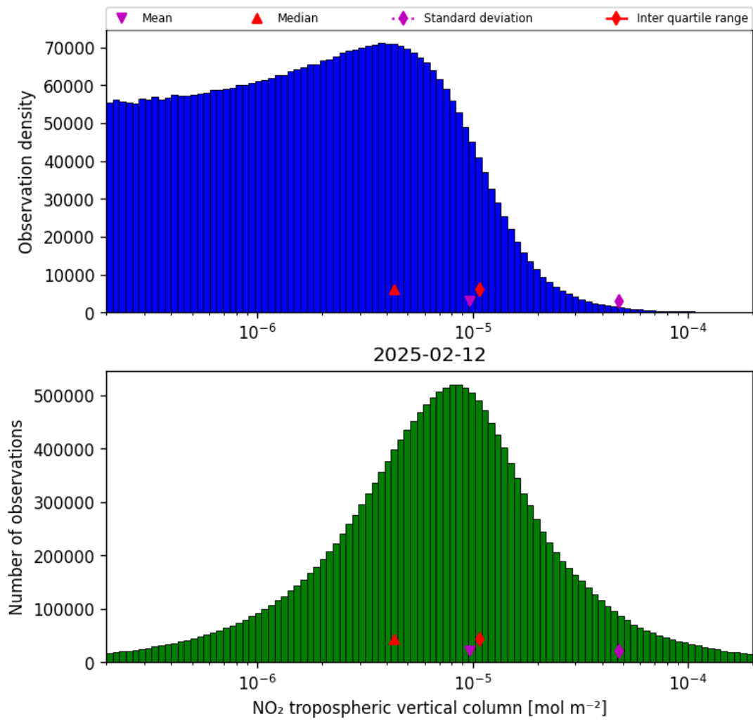
Figure 27: Histogram of “NO 2 tropospheric vertical column” for 2025-02-12 to 2025-02-13
