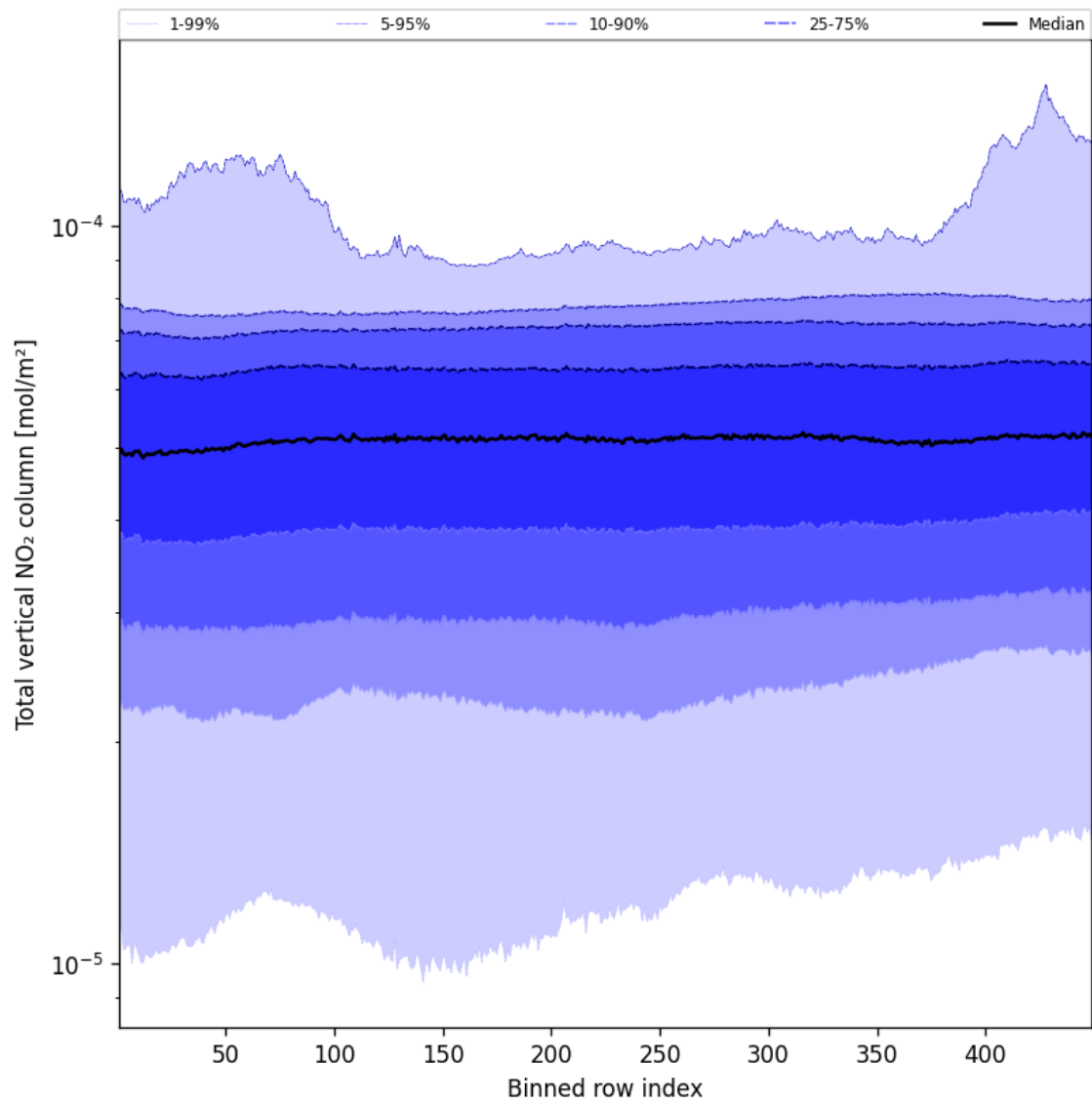
Figure 53: Along track statistics of “Total vertical NO 2 column” for 2025-02-12 to 2025-02-13
