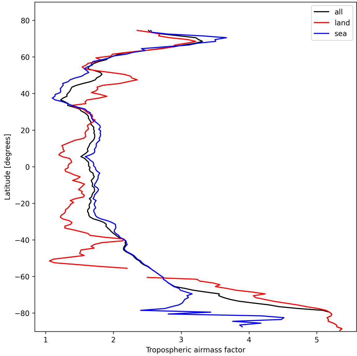
Figure 12: Zonal average of “Tropospheric airmass factor” for 2025-02-12 to 2025-02-13.
