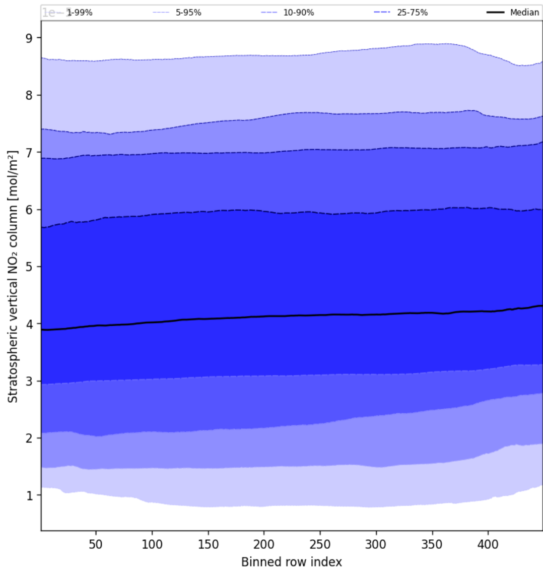
Figure 51: Along track statistics of “Stratospheric vertical NO 2 column” for 2025-02-12 to 2025-02-13
