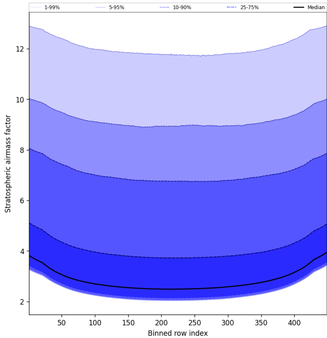
Figure 59: Along track statistics of “Stratospheric airmass factor” for 2025-02-12 to 2025-02-13
