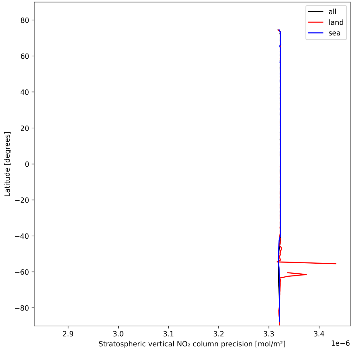
Figure 18: Zonal average of “Stratospheric vertical NO 2 column precision” for 2025-02-12 to 2025-02-13.
