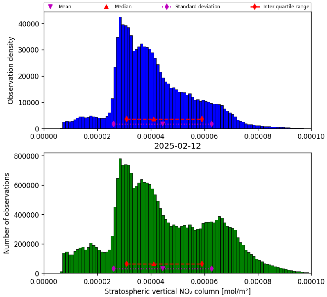
Figure 34: Histogram of “Stratospheric vertical NO 2 column” for 2025-02-12 to 2025-02-13
