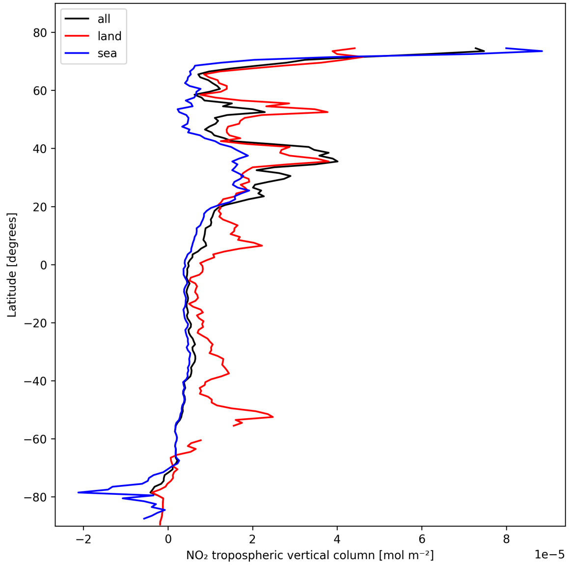
Figure 10: Zonal average of “NO 2 tropospheric vertical column” for 2025-02-12 to 2025-02-13.
