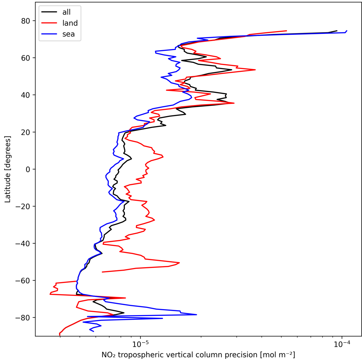
Figure 11: Zonal average of “NO 2 tropospheric vertical column precision” for 2025-02-12 to 2025-02-13.
