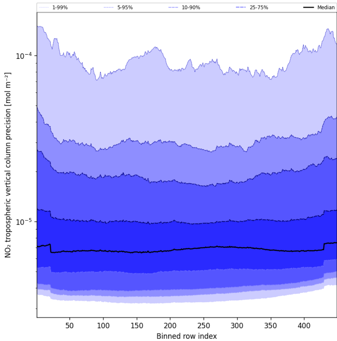
Figure 45: Along track statistics of “NO 2 tropospheric vertical column precision” for 2025-02-12 to 2025-02-13
