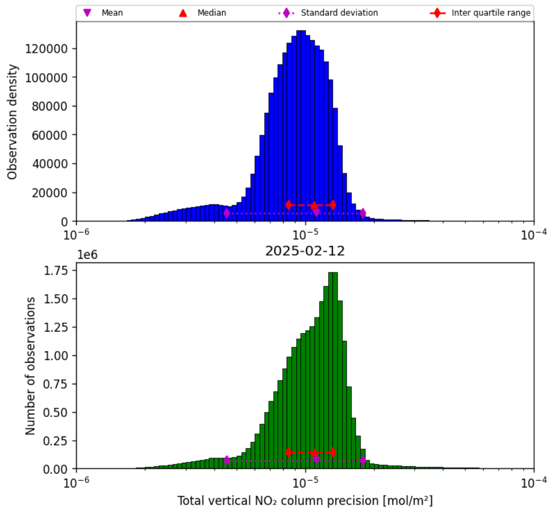
Figure 37: Histogram of “Total vertical NO 2 column precision” for 2025-02-12 to 2025-02-13
