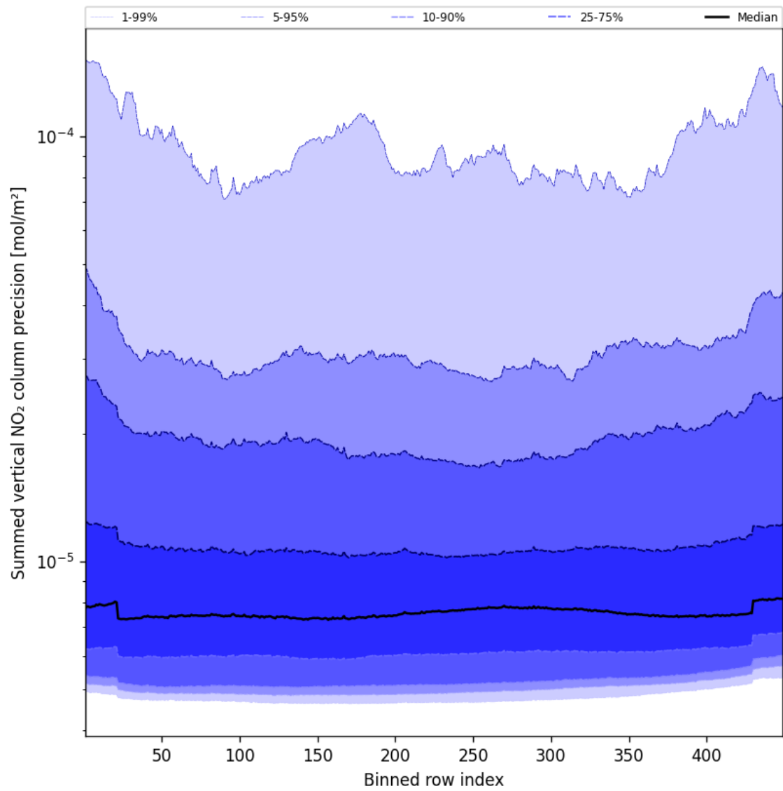
Figure 56: Along track statistics of “Summed vertical NO 2 column precision” for 2025-02-12 to 2025-02-13
