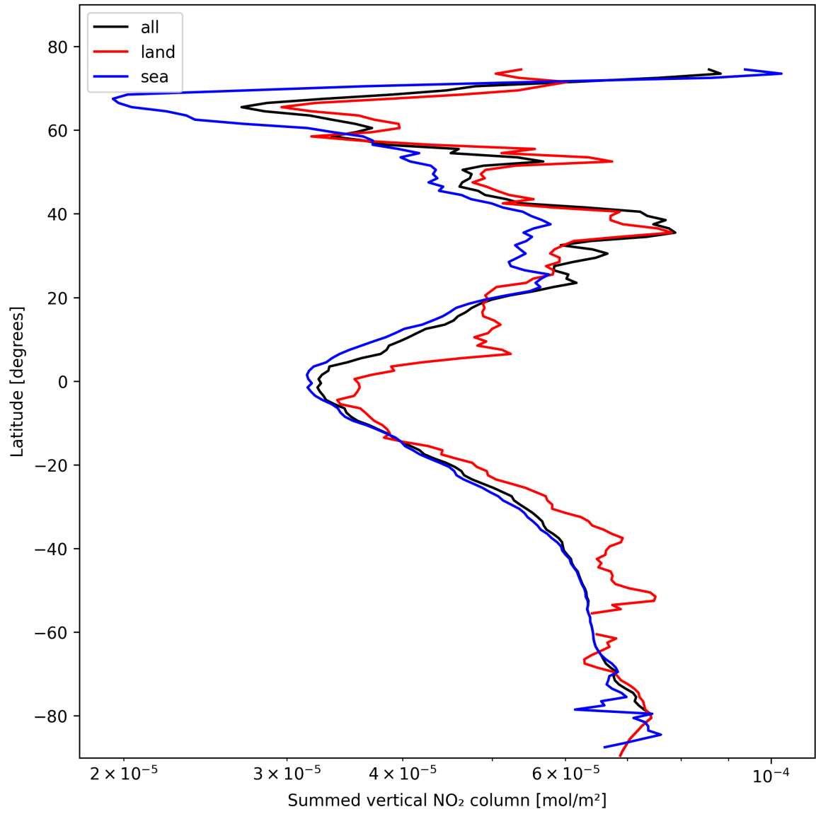
Figure 21: Zonal average of “Summed vertical NO 2 column” for 2025-02-12 to 2025-02-13.
