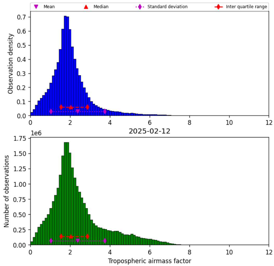
Figure 29: Histogram of “Tropospheric airmass factor” for 2025-02-12 to 2025-02-13
