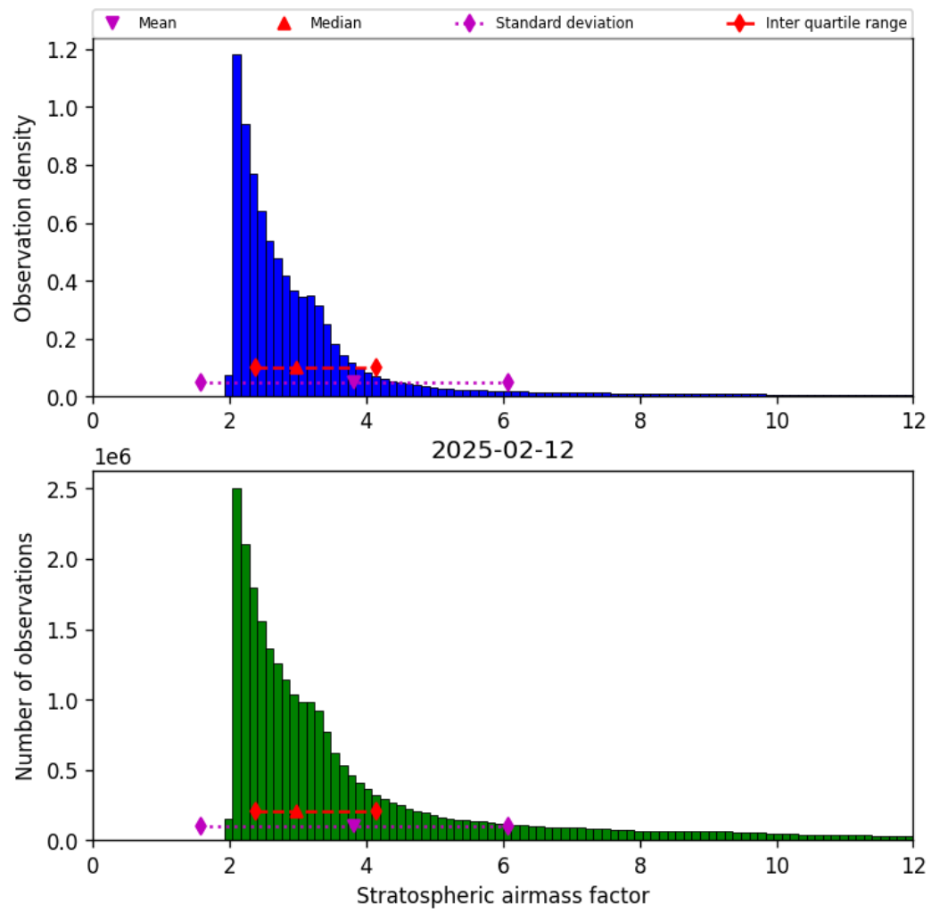
Figure 42: Histogram of “Stratospheric airmass factor” for 2025-02-12 to 2025-02-13
