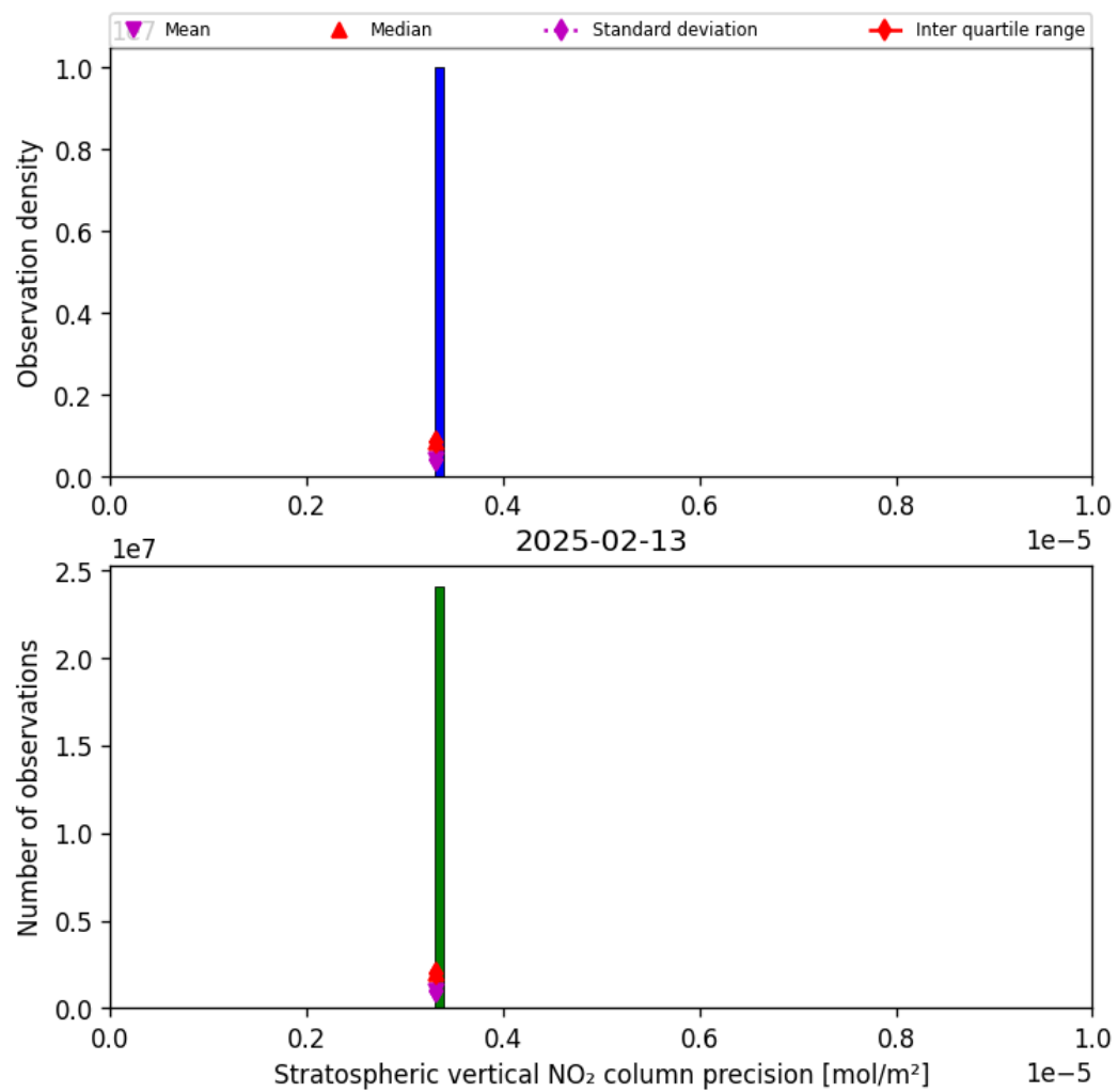
Figure 35: Histogram of “Stratospheric vertical NO 2 column precision” for 2025-02-13 to 2025-02-14
