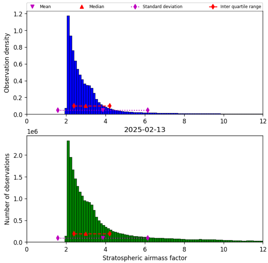
Figure 42: Histogram of “Stratospheric airmass factor” for 2025-02-13 to 2025-02-14
