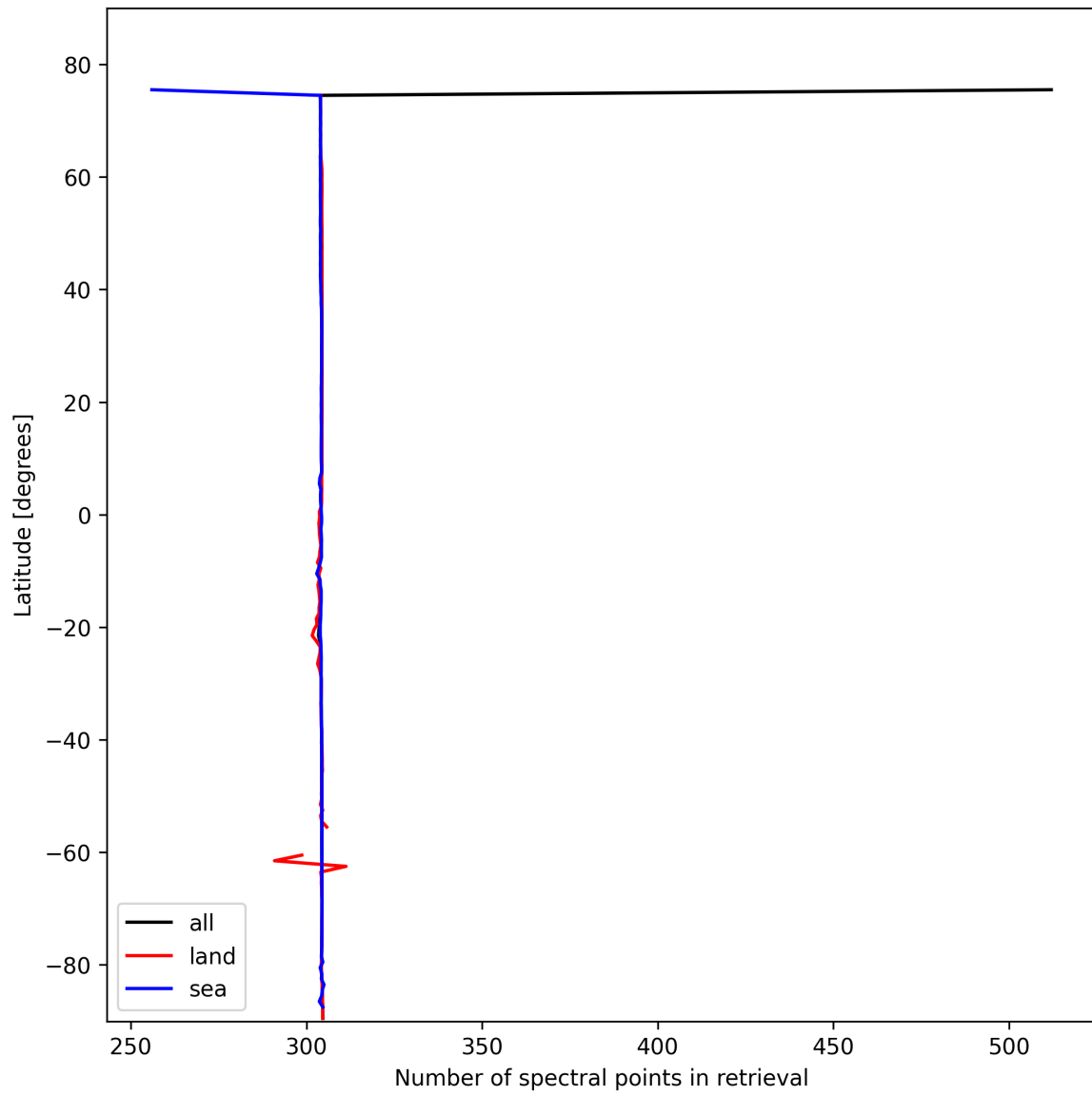
Figure 14: Zonal average of “Number of spectral points in retrieval” for 2025-02-13 to 2025-02-14.
