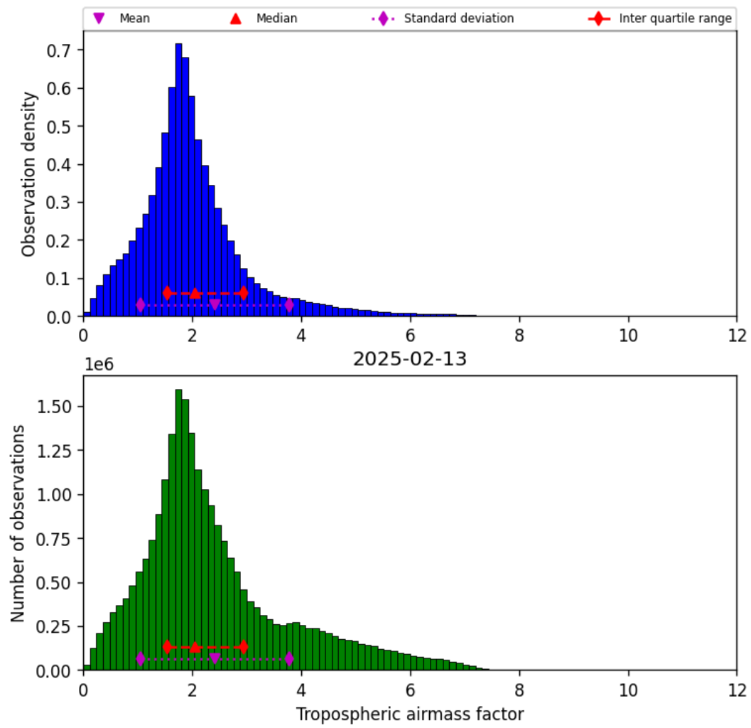
Figure 29: Histogram of “Tropospheric airmass factor” for 2025-02-13 to 2025-02-14
