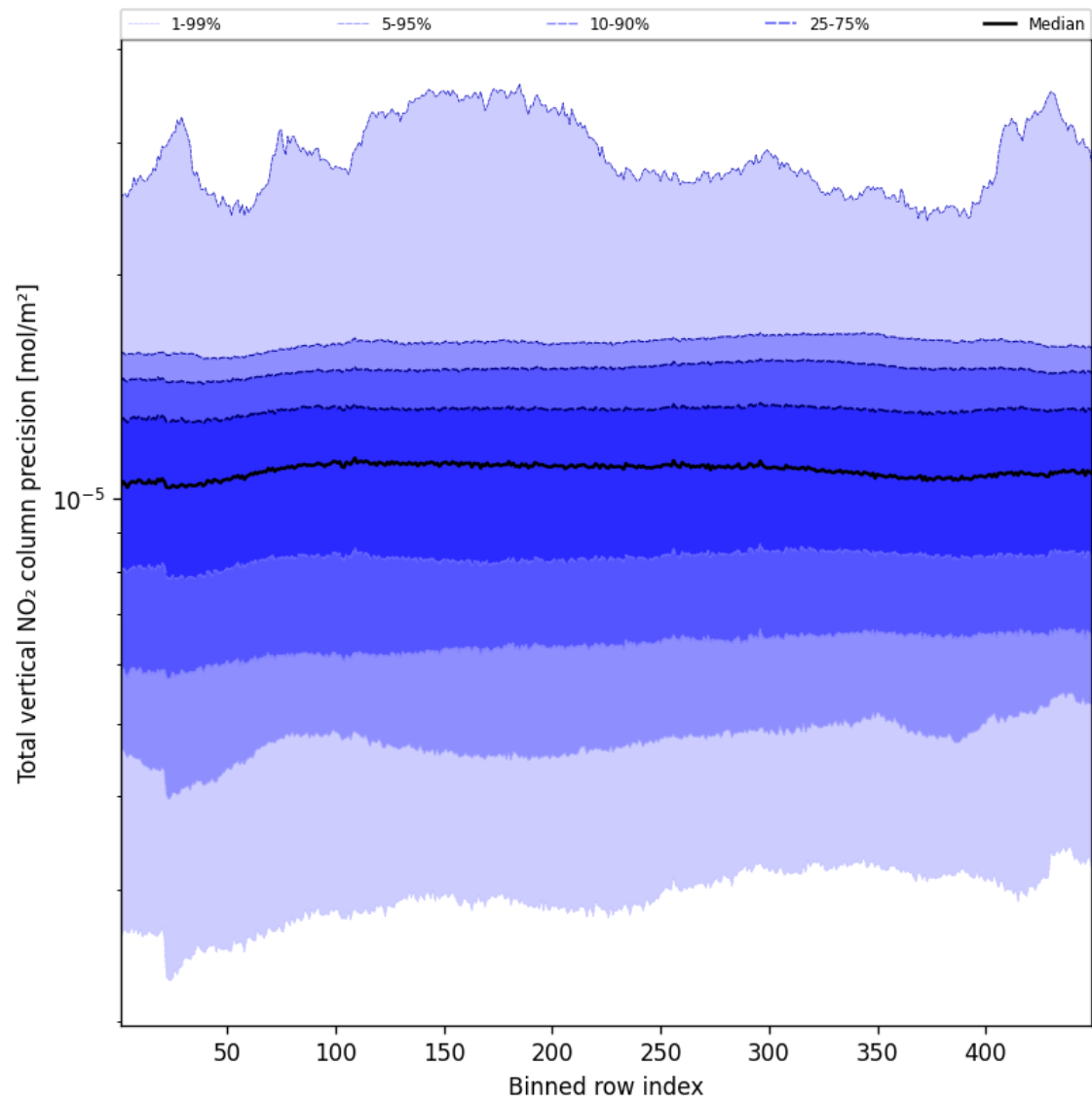
Figure 54: Along track statistics of “Total vertical NO 2 column precision” for 2025-02-13 to 2025-02-14
