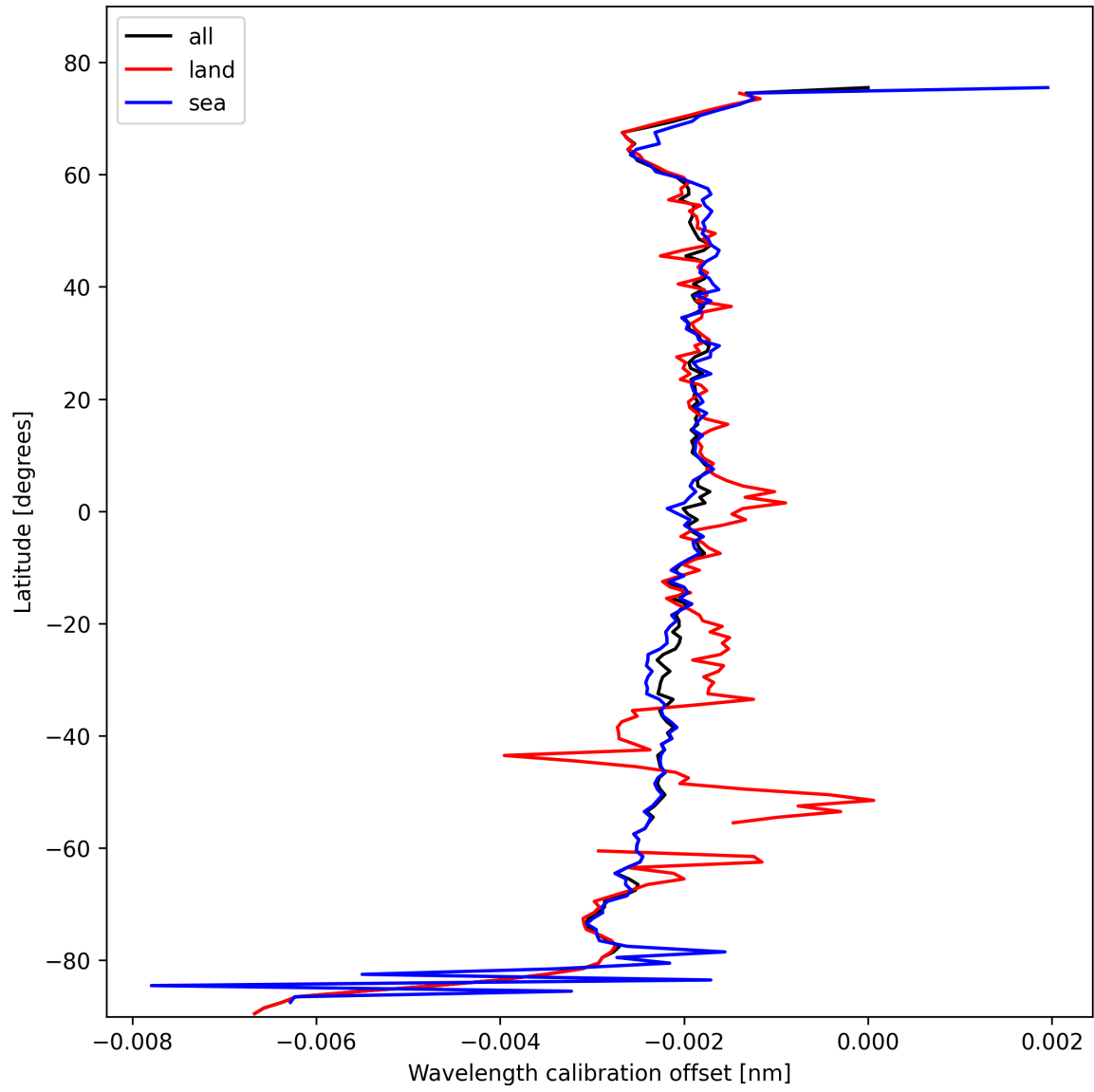
Figure 16: Zonal average of “Wavelength calibration offset” for 2025-02-13 to 2025-02-14.
