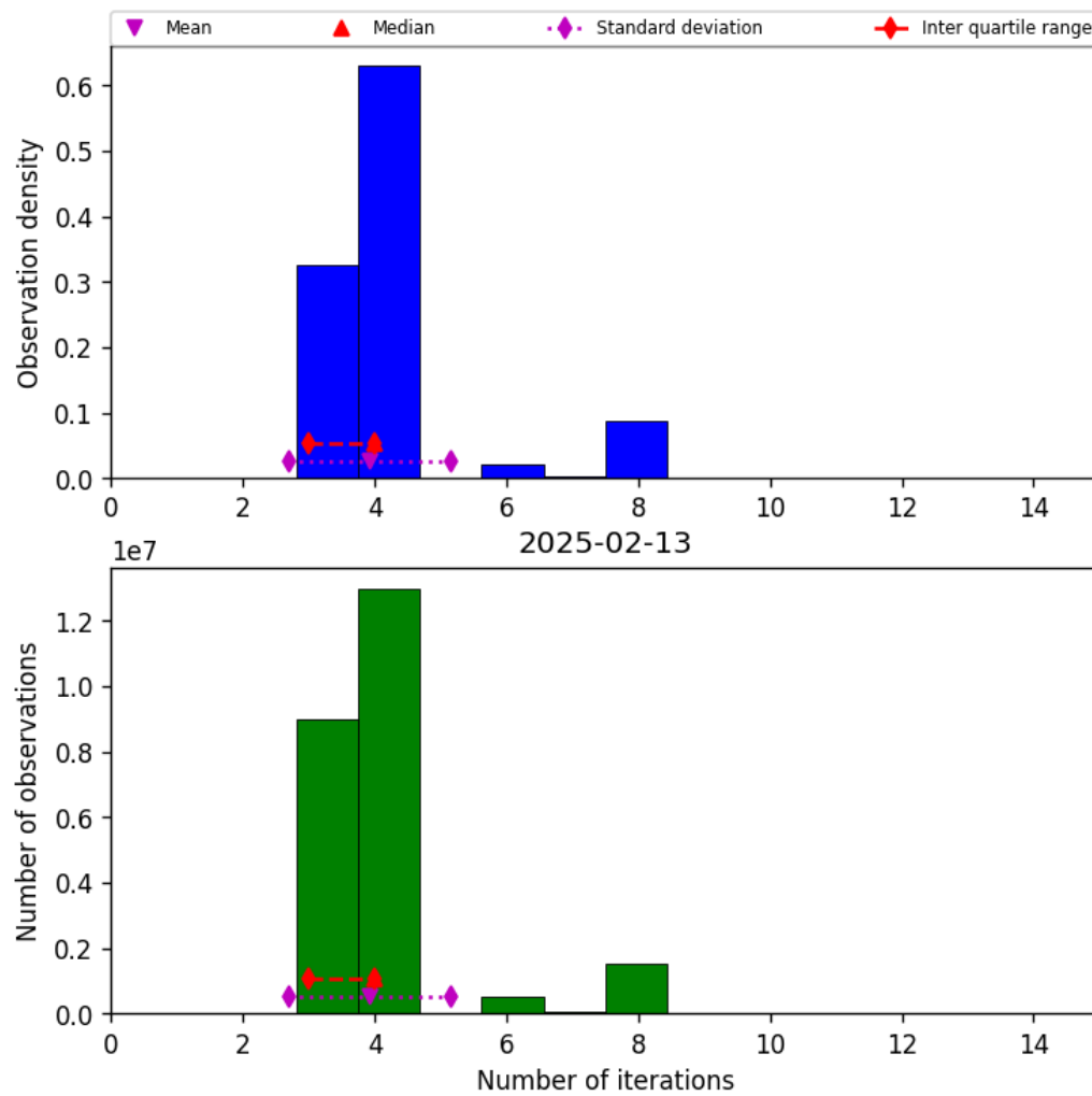
Figure 32: Histogram of “Number of iterations” for 2025-02-13 to 2025-02-14
