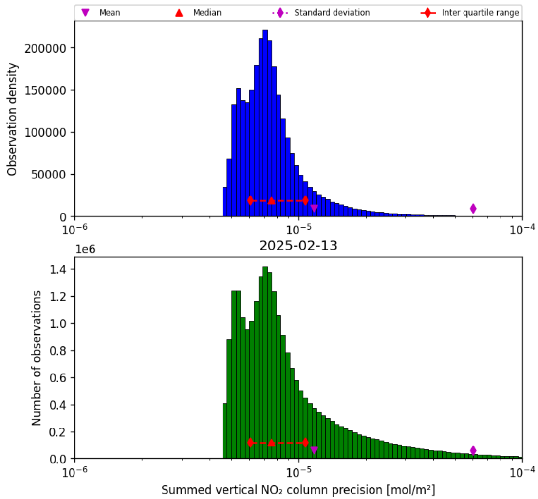
Figure 39: Histogram of “Summed vertical NO 2 column precision” for 2025-02-13 to 2025-02-14
