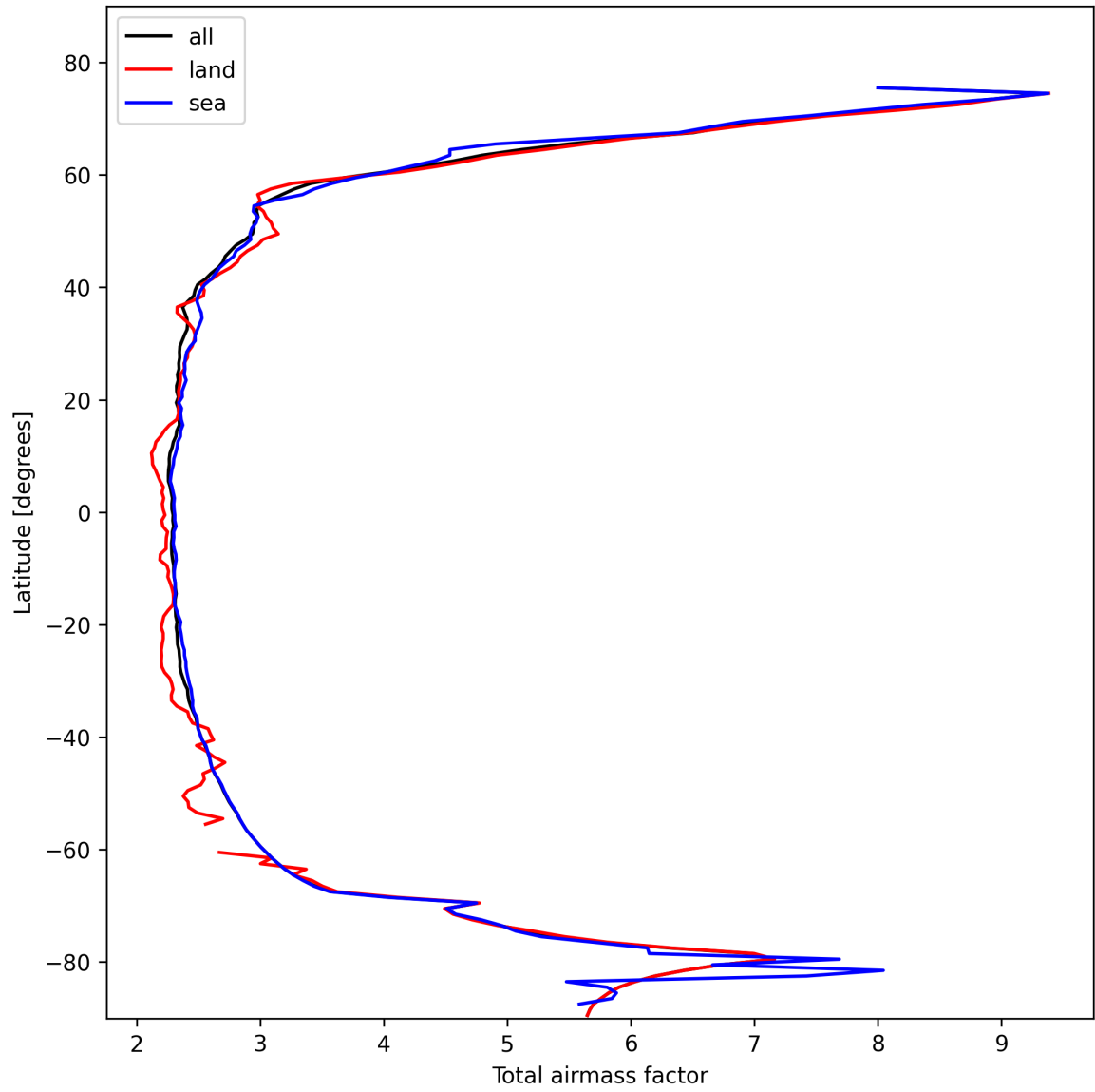
Figure 13: Zonal average of “Total airmass factor” for 2025-02-13 to 2025-02-14.
