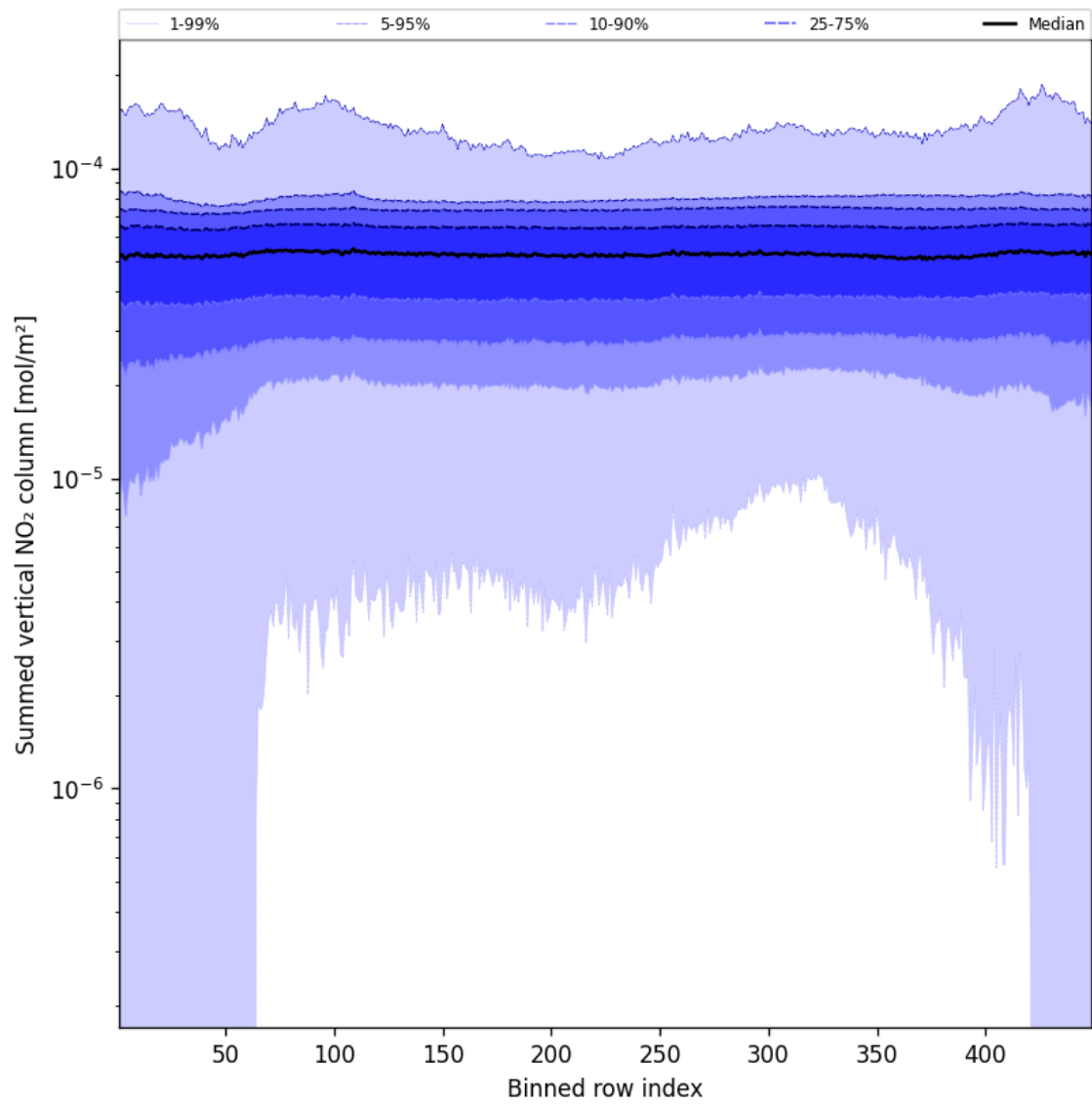
Figure 55: Along track statistics of “Summed vertical NO 2 column” for 2025-02-13 to 2025-02-14
