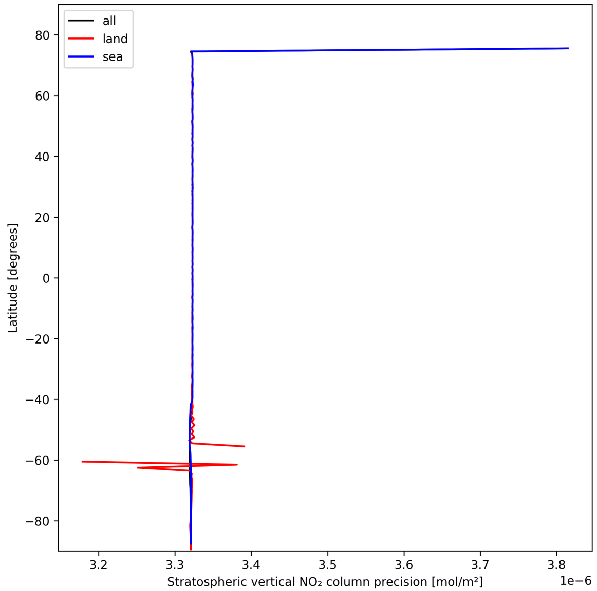
Figure 18: Zonal average of "Stratospheric vertical NO 2 column precision" for 2025-02-13 to 2025-02-14.
