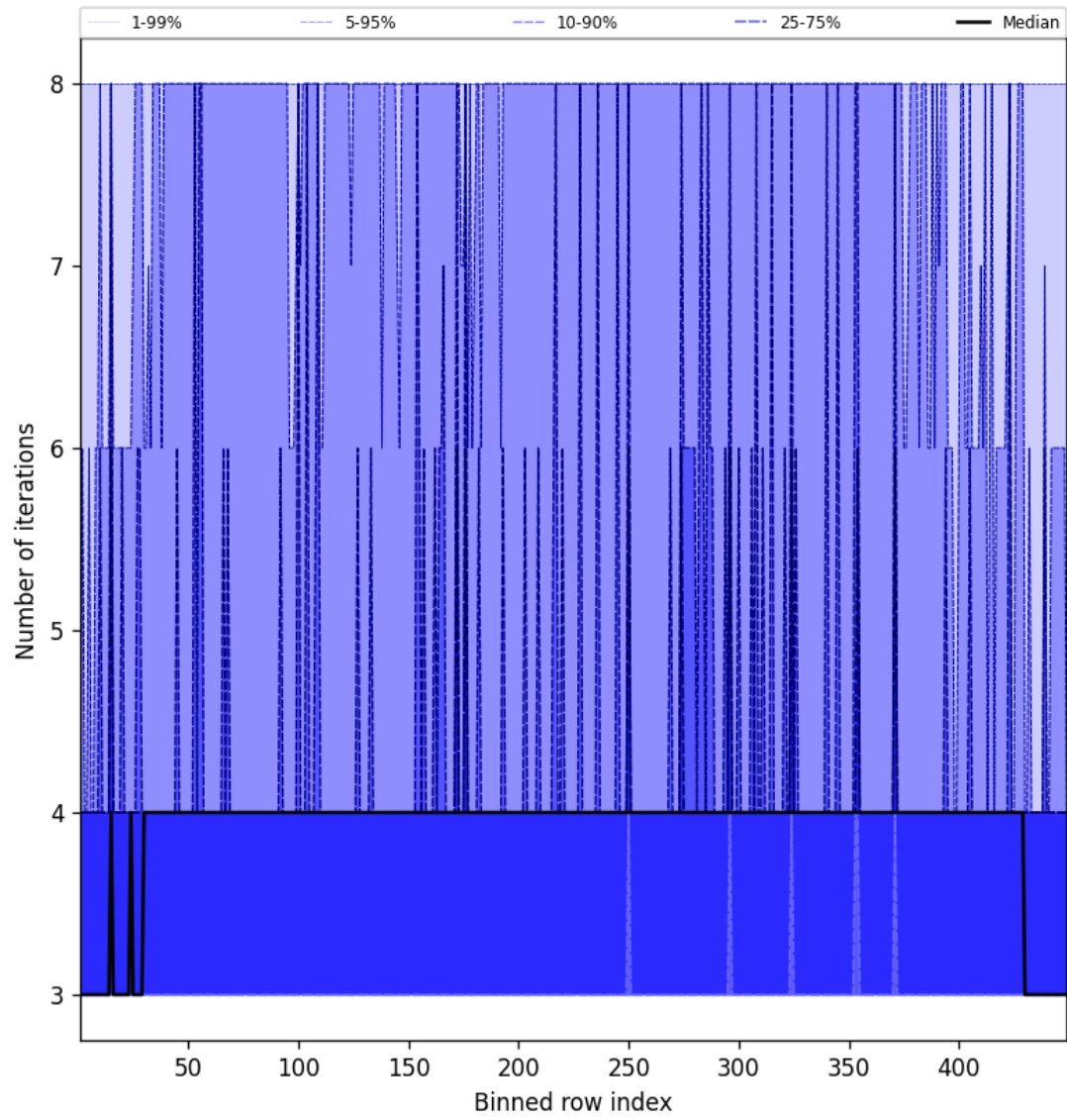
Figure 49: Along track statistics of “Number of iterations” for 2025-02-13 to 2025-02-14
