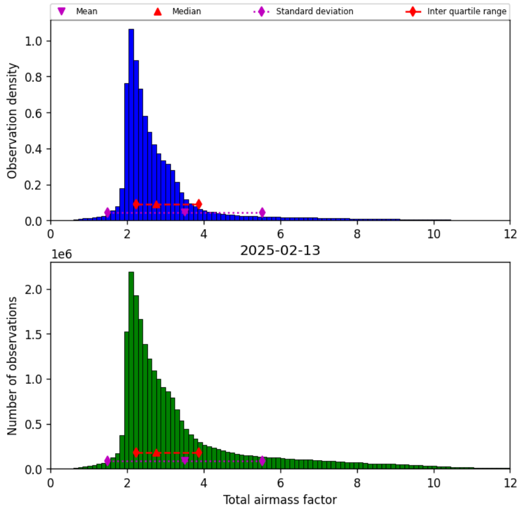
Figure 30: Histogram of “Total airmass factor” for 2025-02-13 to 2025-02-14
