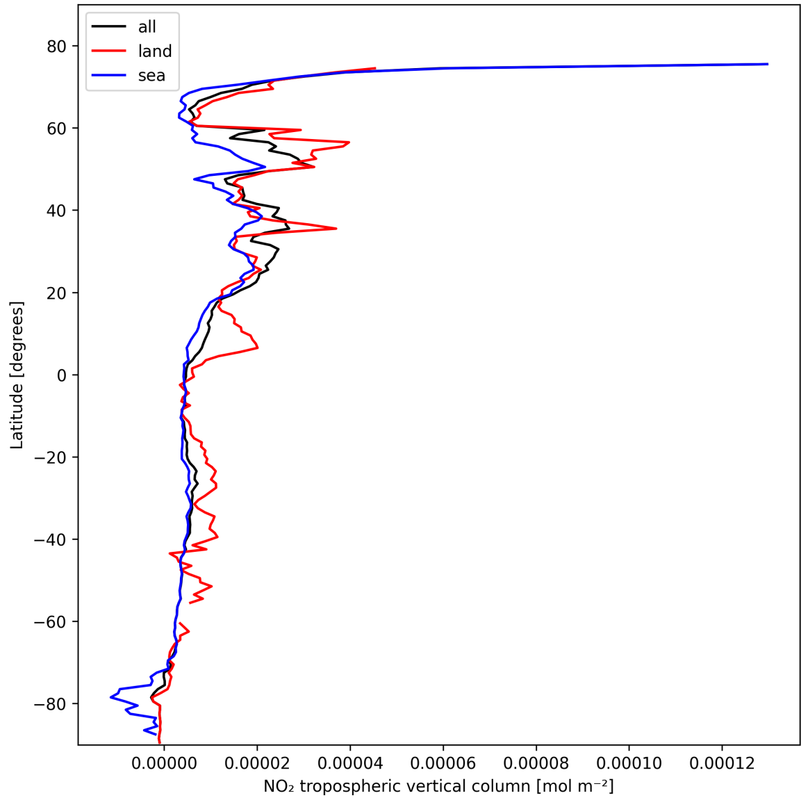
Figure 10: Zonal average of “NO 2 tropospheric vertical column” for 2025-02-13 to 2025-02-14.
