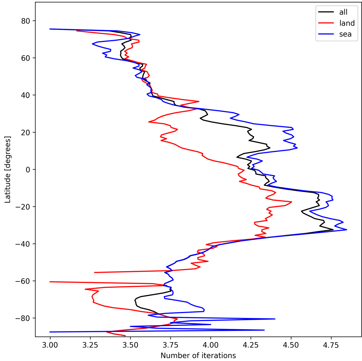
Figure 15: Zonal average of “Number of iterations” for 2025-02-13 to 2025-02-14.
