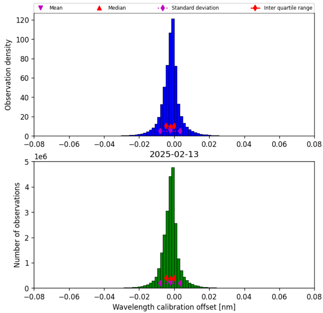
Figure 33: Histogram of “Wavelength calibration offset” for 2025-02-13 to 2025-02-14
