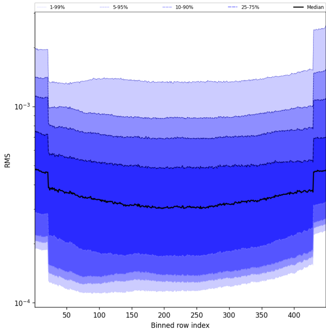
Figure 58: Along track statistics of “RMS” for 2025-02-13 to 2025-02-14
