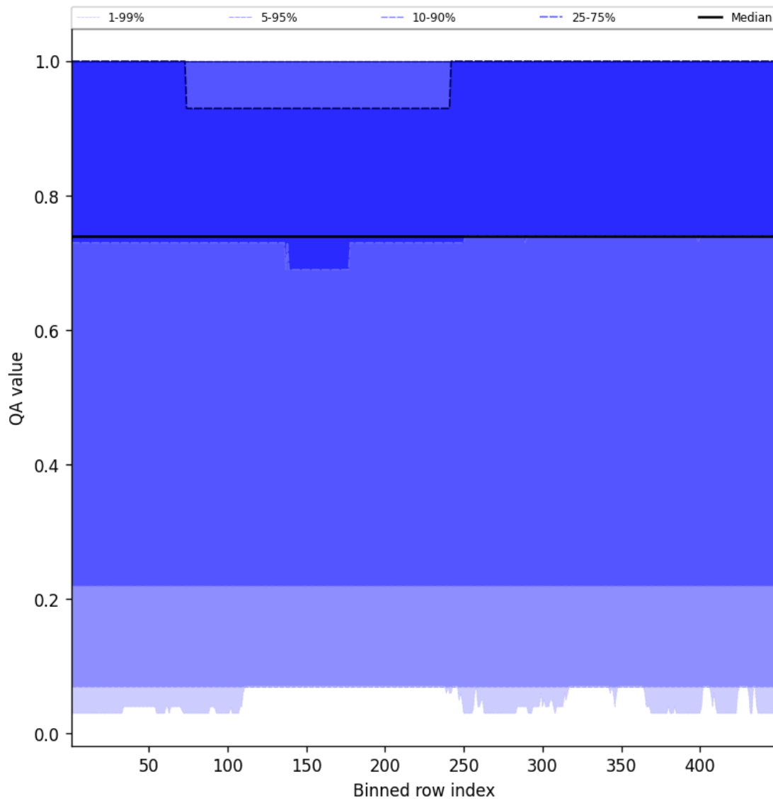
Figure 43: Along track statistics of “QA value” for 2025-02-13 to 2025-02-14
