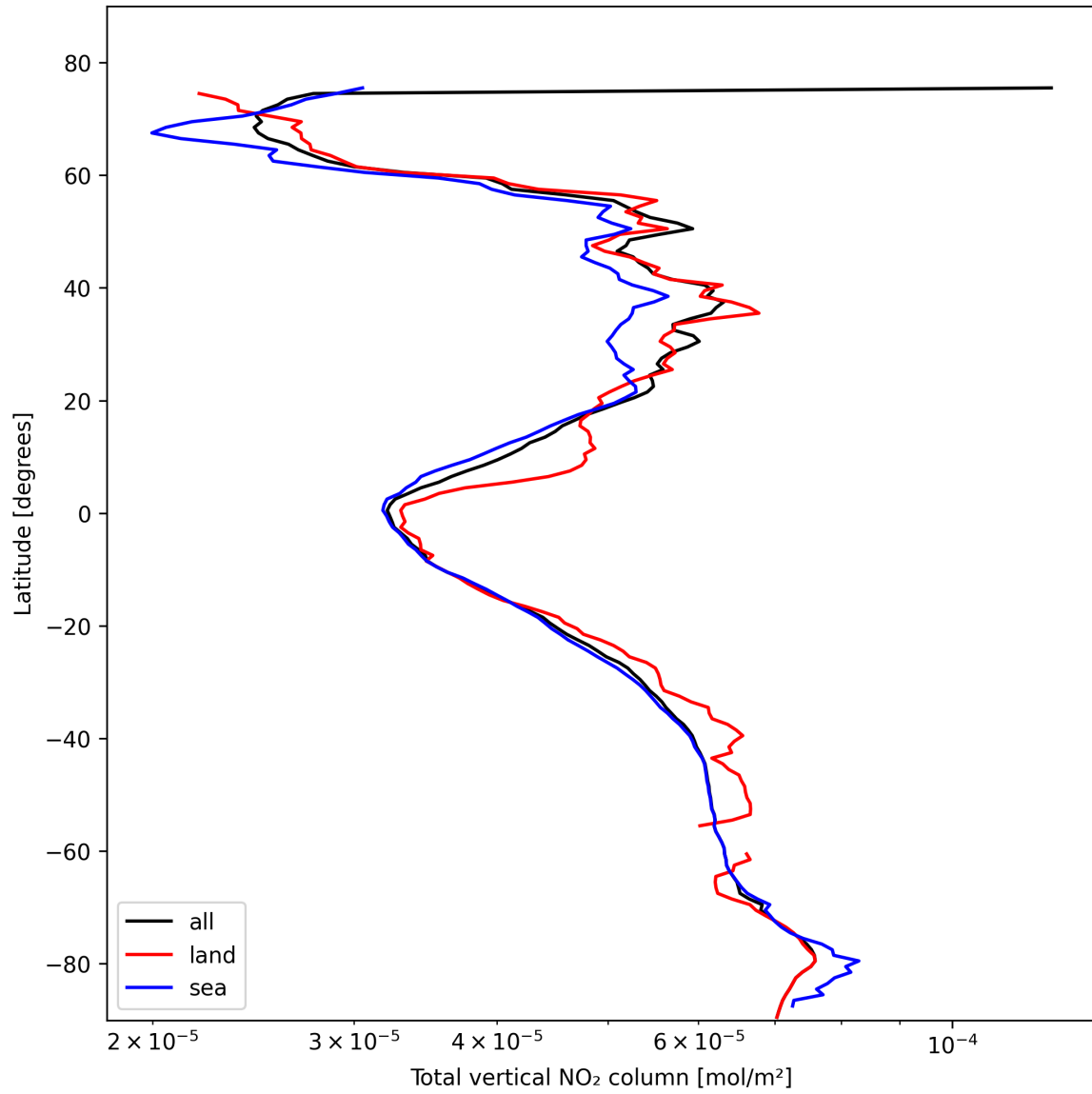
Figure 19: Zonal average of “Total vertical NO 2 column” for 2025-02-13 to 2025-02-14.
