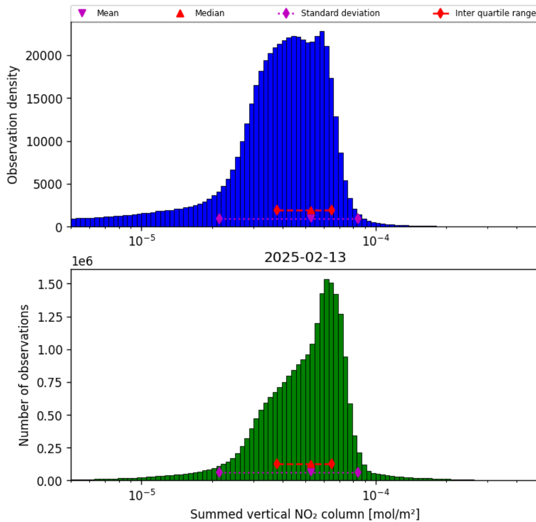
Figure 38: Histogram of “Summed vertical NO 2 column” for 2025-02-13 to 2025-02-14
