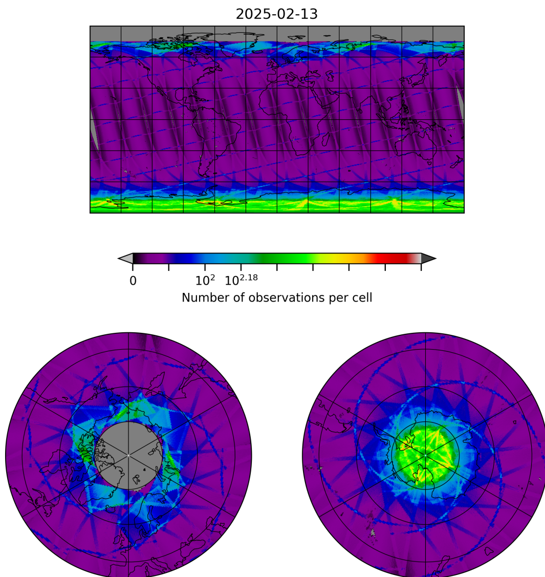
Figure 8: Map of the number of observations for 2025-02-13 to 2025-02-14
