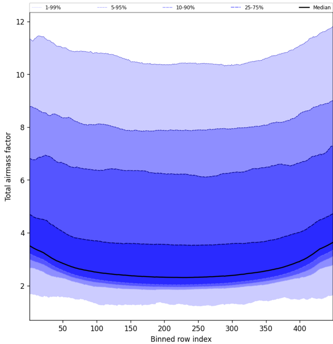
Figure 47: Along track statistics of “Total airmass factor” for 2025-02-13 to 2025-02-14
