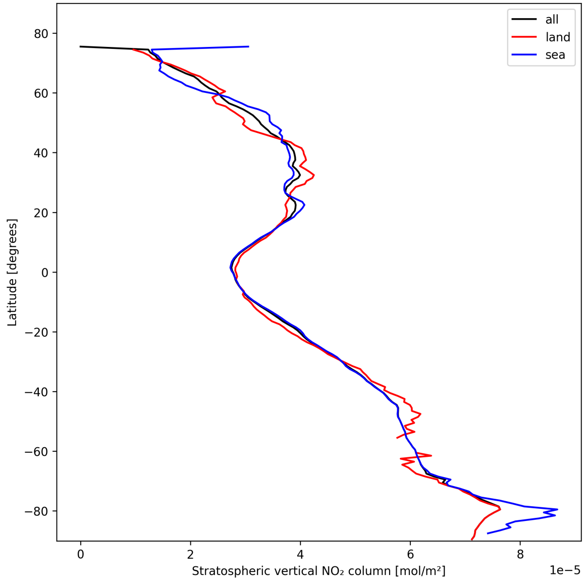
Figure 17: Zonal average of “Stratospheric vertical NO 2 column” for 2025-02-13 to 2025-02-14.
