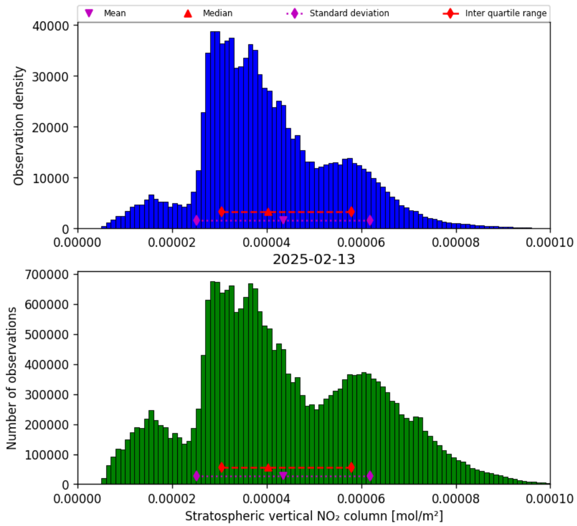
Figure 34: Histogram of “Stratospheric vertical NO 2 column” for 2025-02-13 to 2025-02-14
