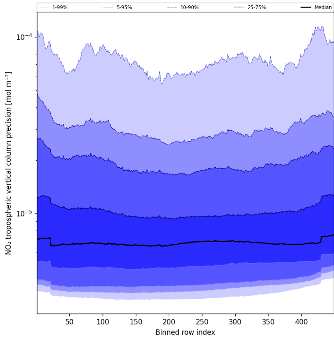
Figure 45: Along track statistics of “NO 2 tropospheric vertical column precision” for 2025-02-13 to 2025-02-14
