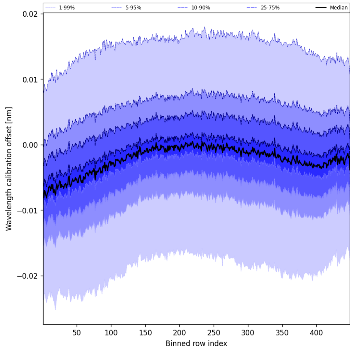
Figure 50: Along track statistics of “Wavelength calibration offset” for 2025-02-13 to 2025-02-14
