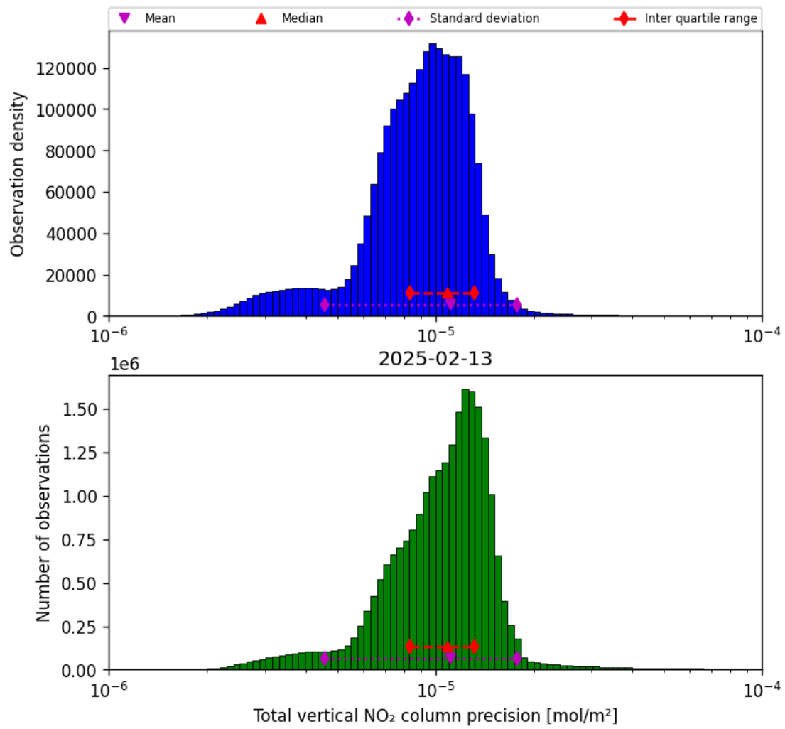
Figure 37: Histogram of “Total vertical NO 2 column precision” for 2025-02-13 to 2025-02-14
