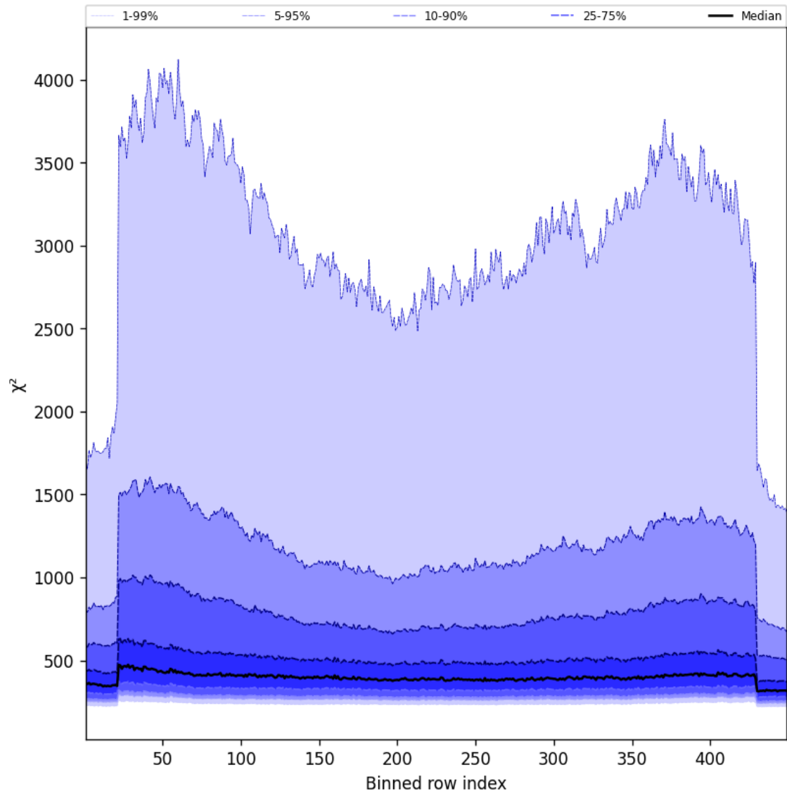
Figure 57: Along track statistics of “ \chi^2 ” for 2025-02-13 to 2025-02-14
