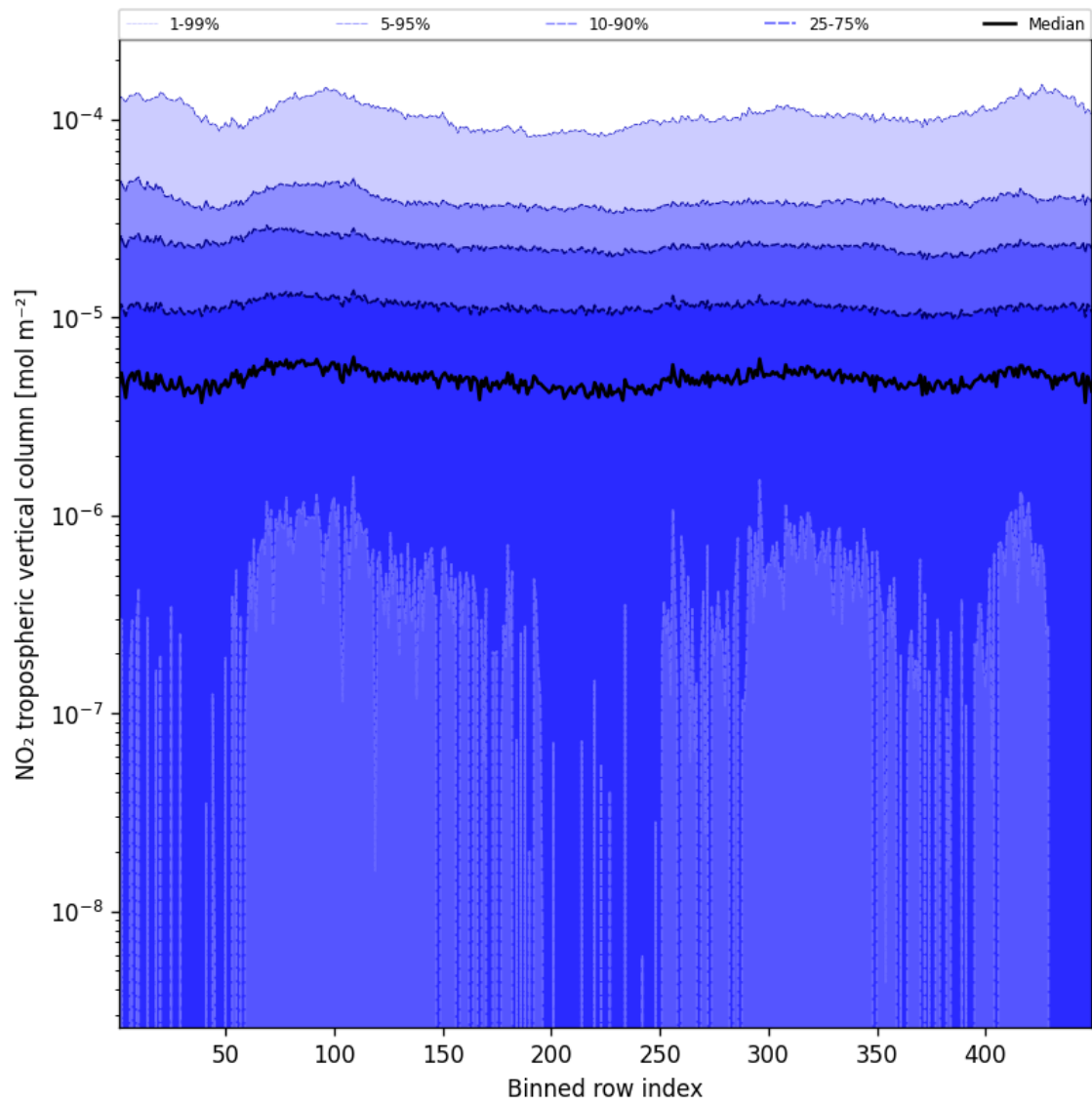
Figure 44: Along track statistics of “NO 2 tropospheric vertical column” for 2025-02-13 to 2025-02-14
