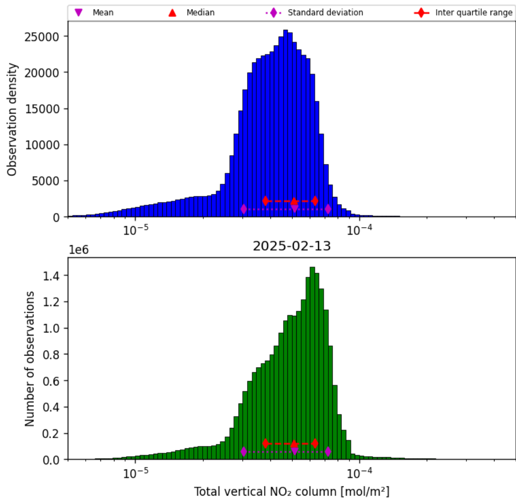
Figure 36: Histogram of “Total vertical NO 2 column” for 2025-02-13 to 2025-02-14
