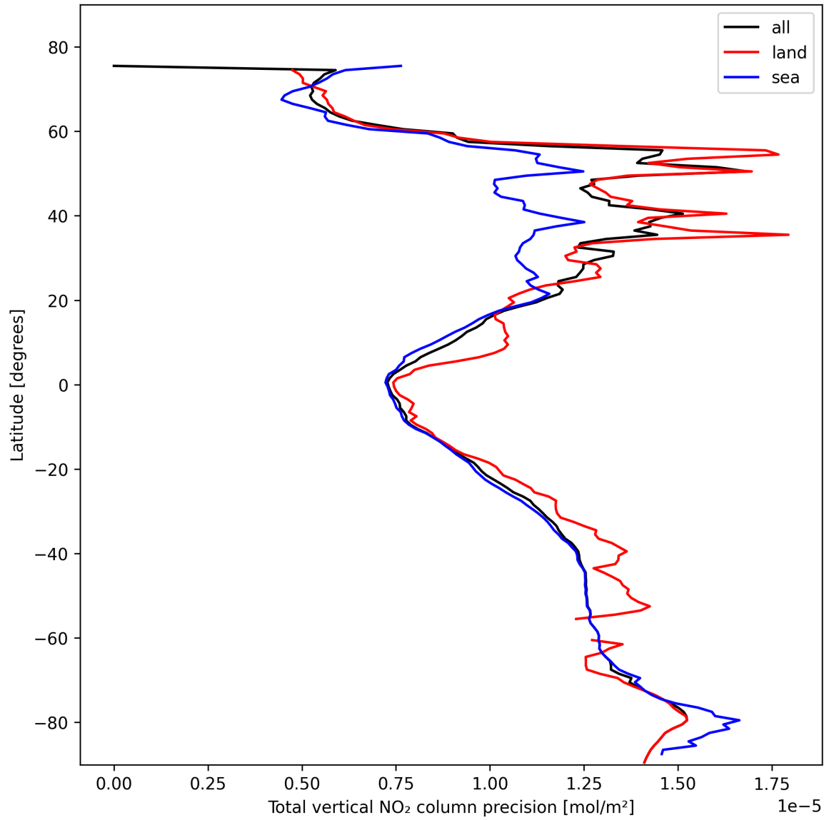
Figure 20: Zonal average of “Total vertical NO 2 column precision” for 2025-02-13 to 2025-02-14.
