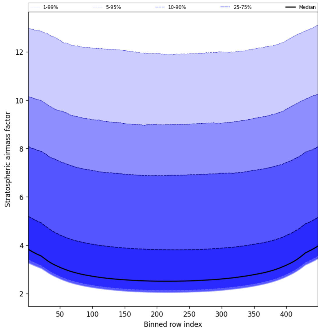
Figure 59: Along track statistics of “Stratospheric airmass factor” for 2025-02-13 to 2025-02-14
