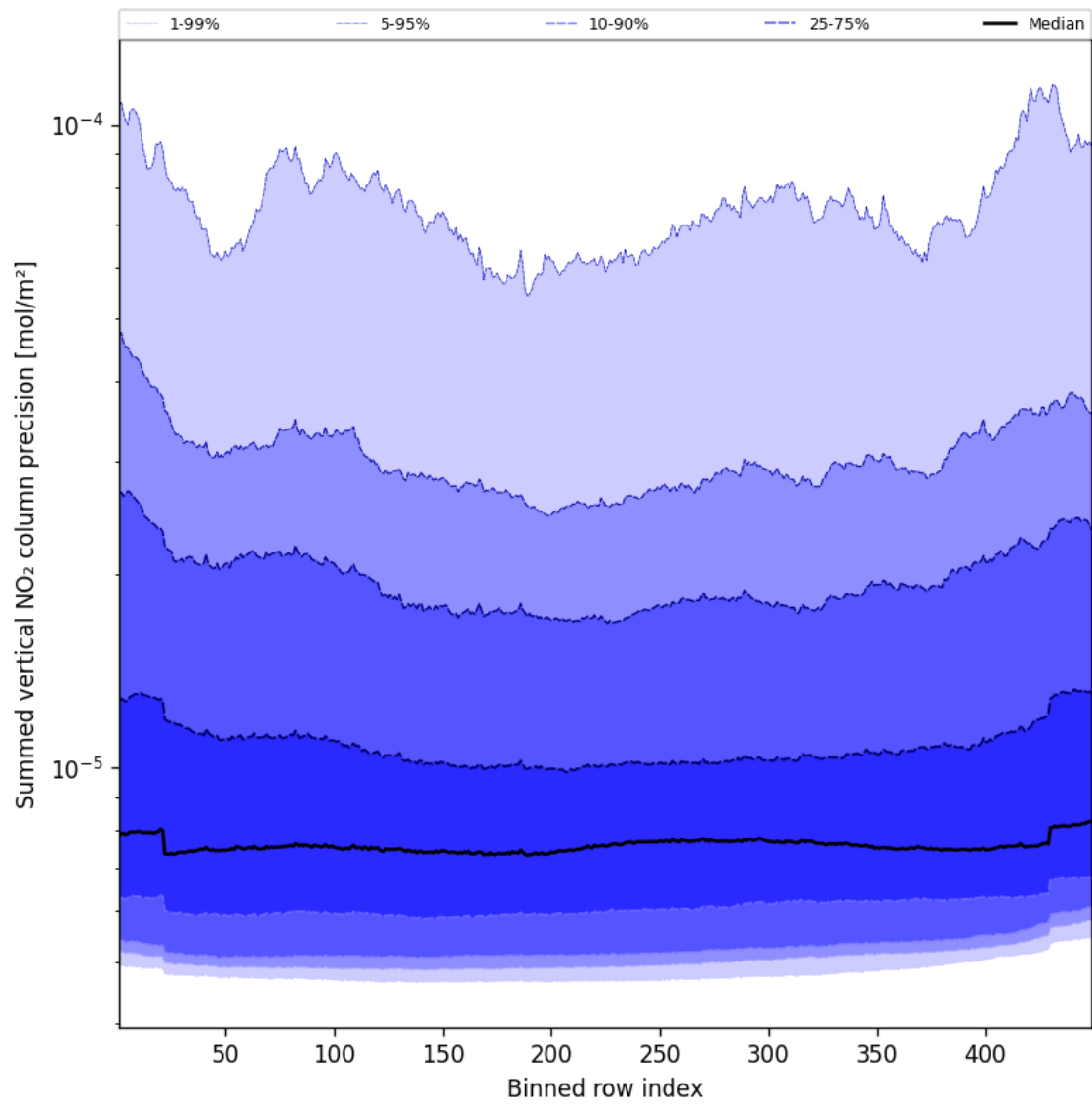
Figure 56: Along track statistics of “Summed vertical NO 2 column precision” for 2025-02-13 to 2025-02-14
