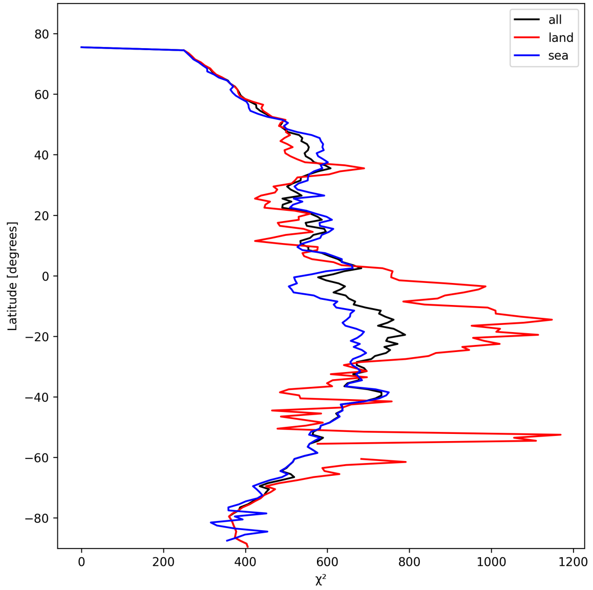
Figure 23: Zonal average of “ \chi^2 ” for 2025-02-13 to 2025-02-14.
