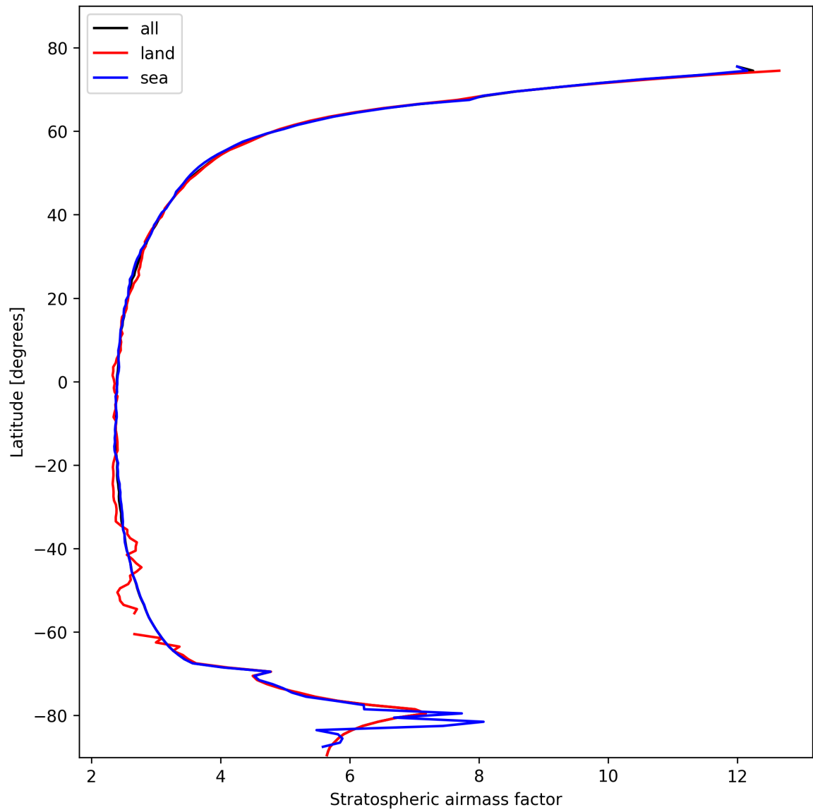
Figure 25: Zonal average of “Stratospheric airmass factor” for 2025-02-13 to 2025-02-14.
