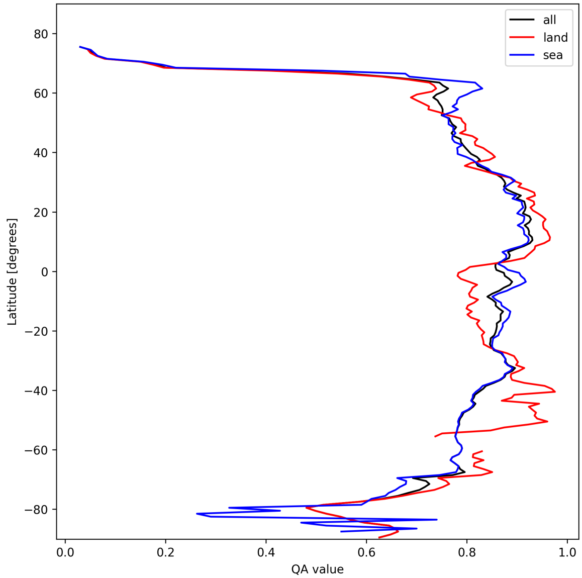
Figure 9: Zonal average of “QA value” for 2025-02-13 to 2025-02-14.
