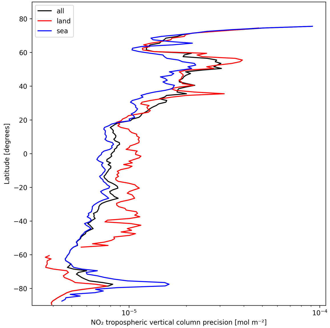
Figure 11: Zonal average of “NO 2 tropospheric vertical column precision” for 2025-02-13 to 2025-02-14.
