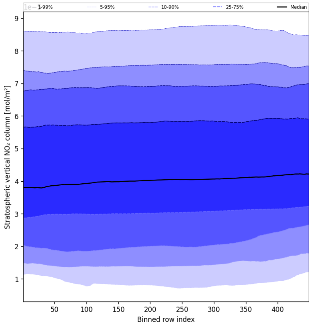
Figure 51: Along track statistics of “Stratospheric vertical NO 2 column” for 2025-02-13 to 2025-02-14
