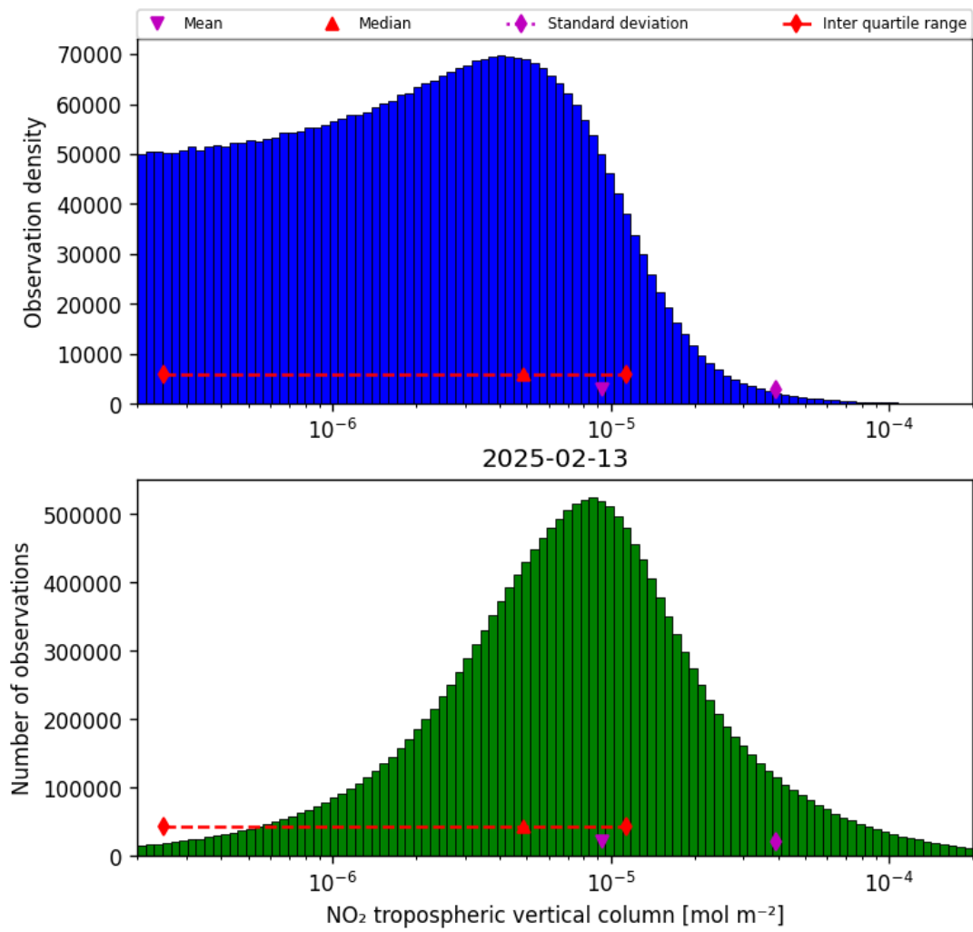
Figure 27: Histogram of “NO 2 tropospheric vertical column” for 2025-02-13 to 2025-02-14
