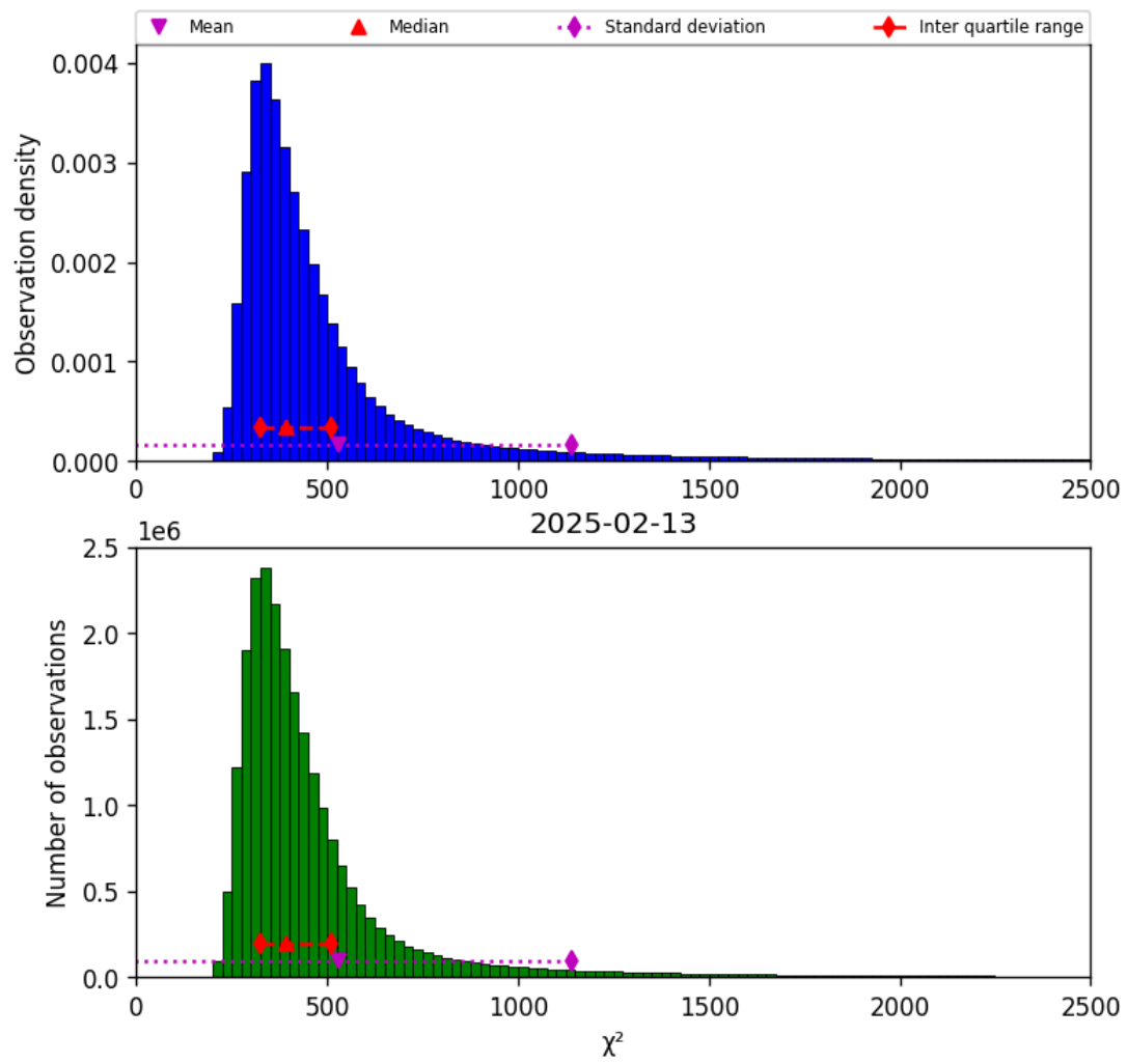
Figure 40: Histogram of “ \chi^2 ” for 2025-02-13 to 2025-02-14
