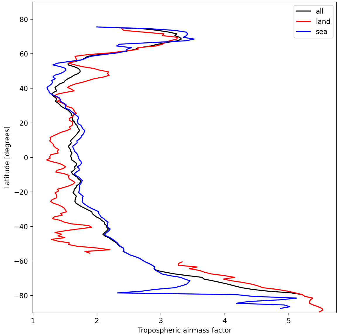
Figure 12: Zonal average of “Tropospheric airmass factor” for 2025-02-13 to 2025-02-14.
