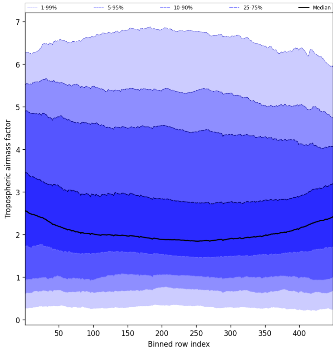
Figure 46: Along track statistics of “Tropospheric airmass factor” for 2025-02-13 to 2025-02-14
