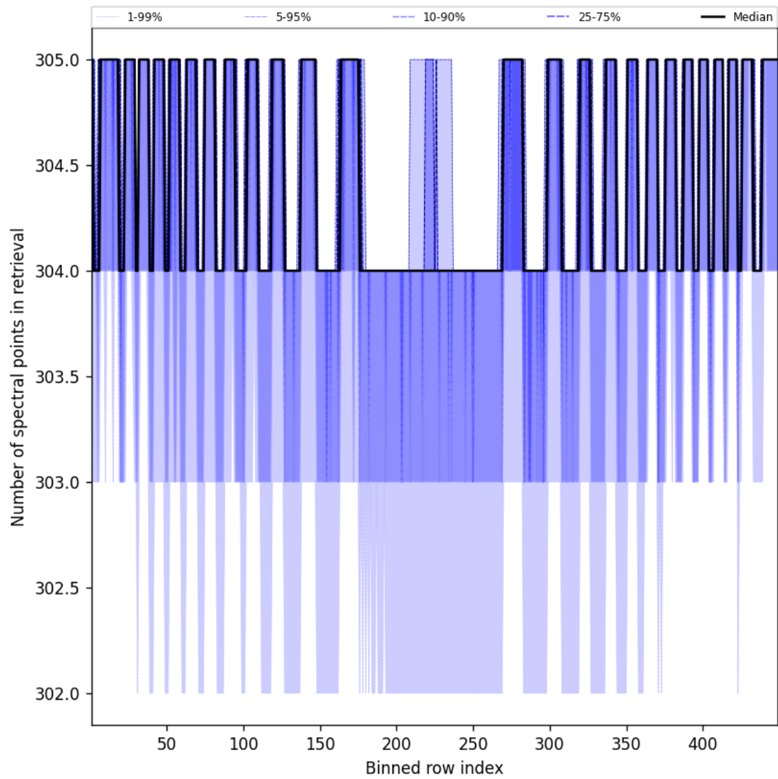
Figure 48: Along track statistics of “Number of spectral points in retrieval” for 2025-02-13 to 2025-02-14
