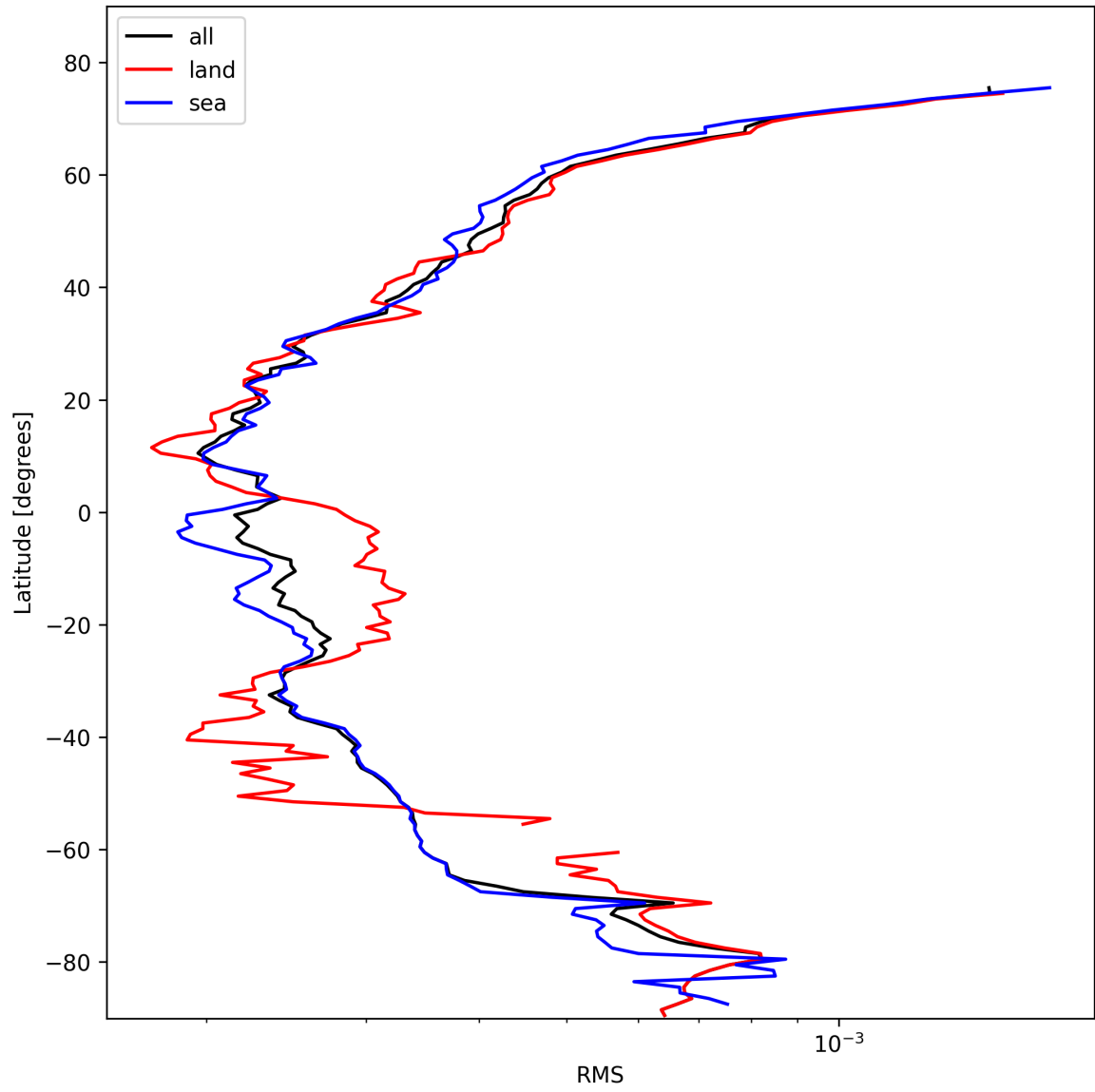
Figure 24: Zonal average of “RMS” for 2025-02-13 to 2025-02-14.
