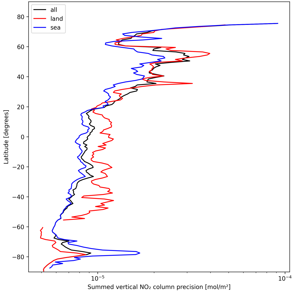
Figure 22: Zonal average of “Summed vertical NO 2 column precision” for 2025-02-13 to 2025-02-14.
