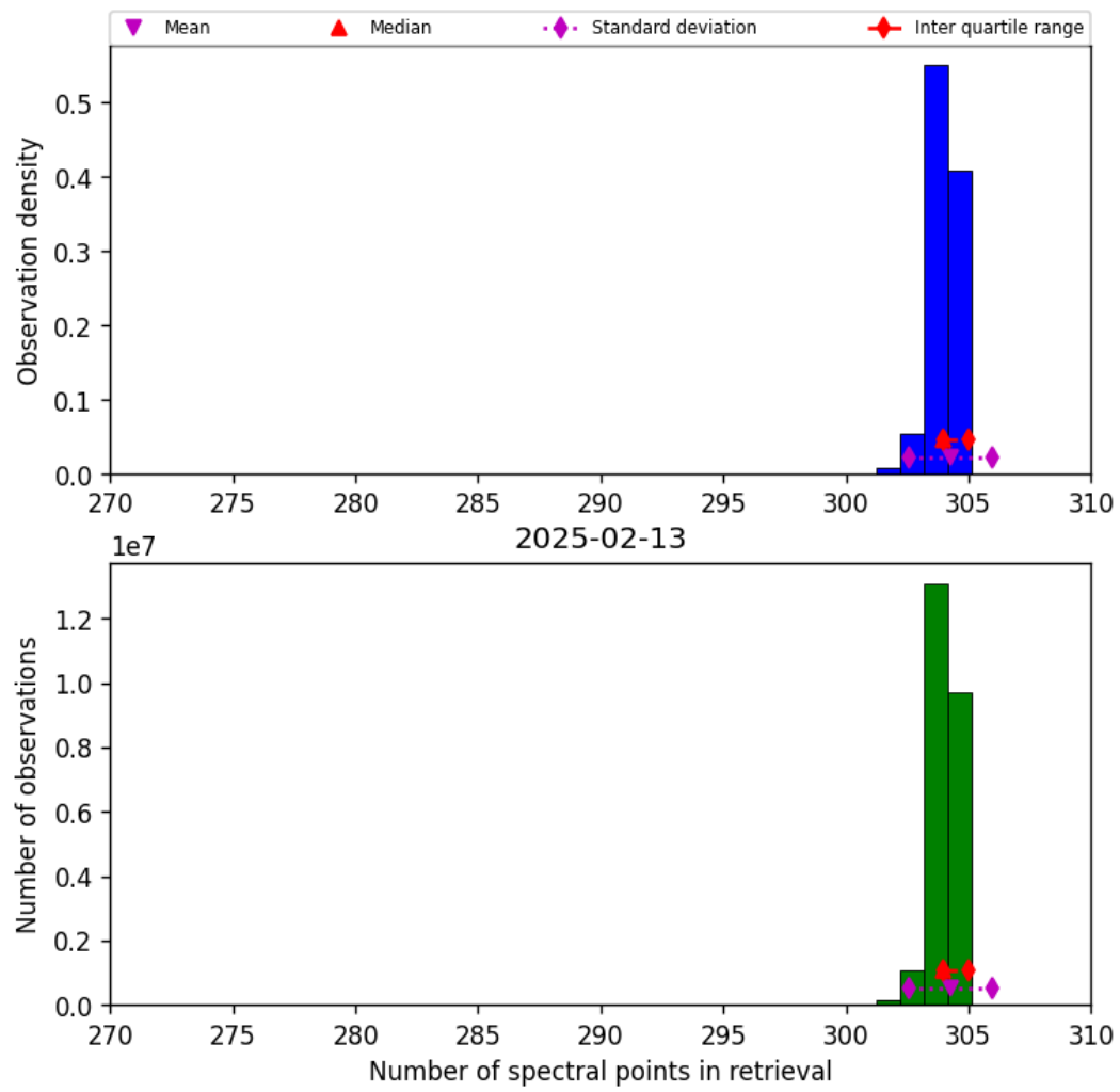
Figure 31: Histogram of “Number of spectral points in retrieval” for 2025-02-13 to 2025-02-14
