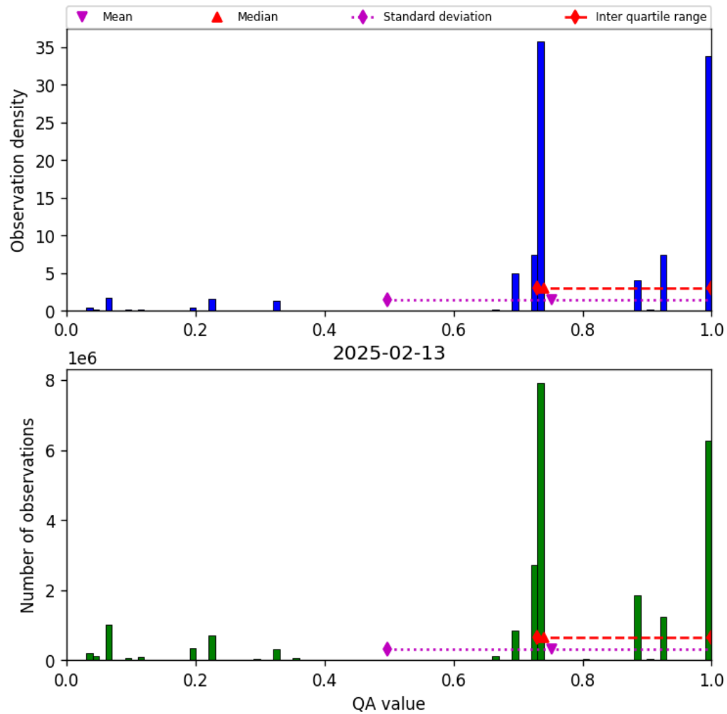
Figure 26: Histogram of “QA value” for 2025-02-13 to 2025-02-14
