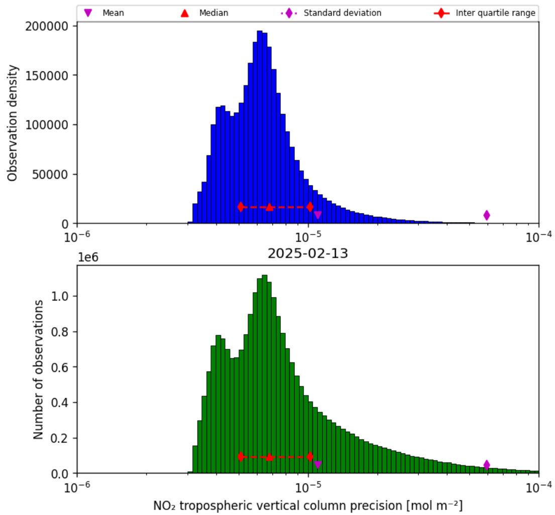
Figure 28: Histogram of “NO 2 tropospheric vertical column precision” for 2025-02-13 to 2025-02-14
