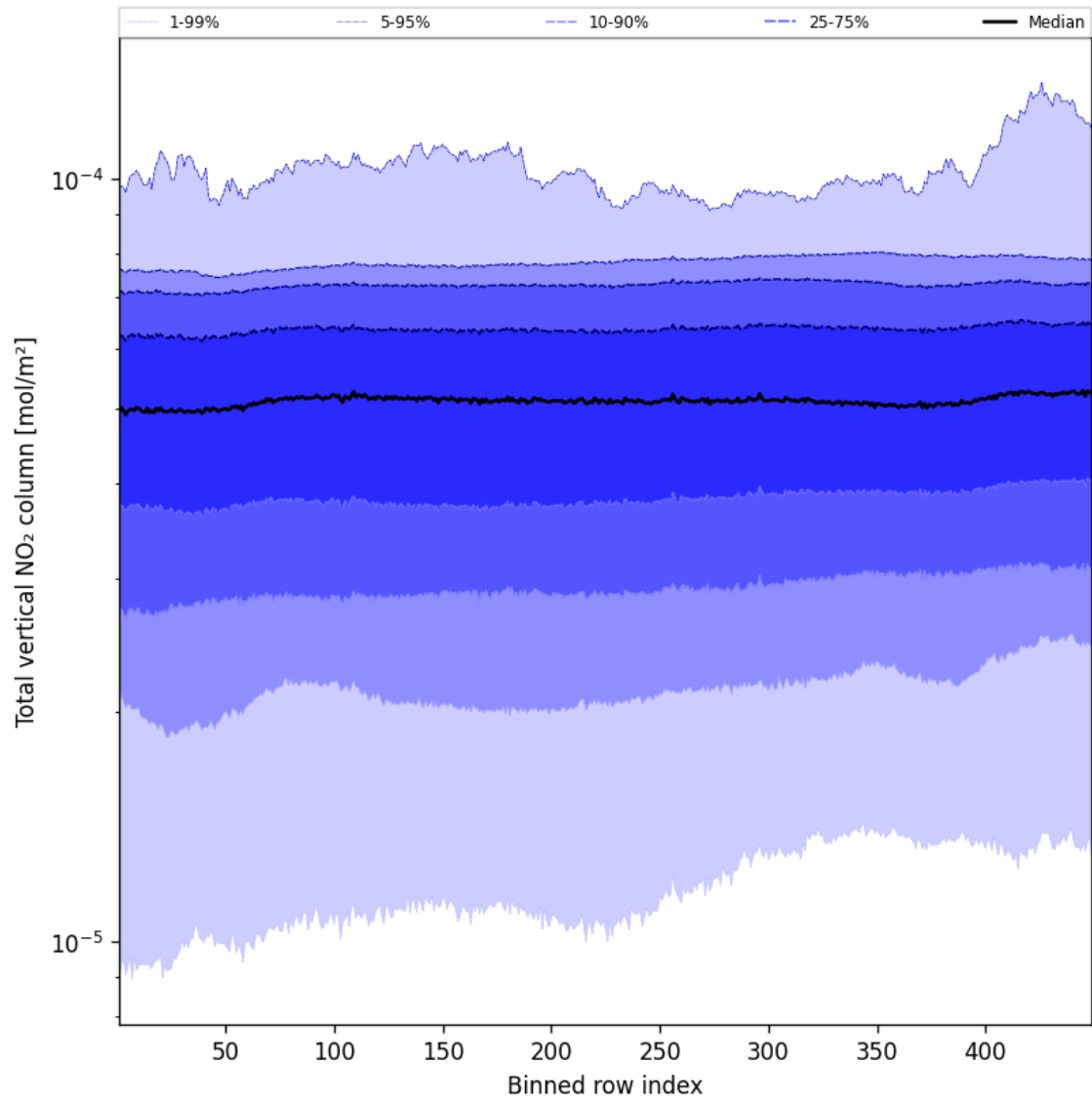
Figure 53: Along track statistics of “Total vertical NO 2 column” for 2025-02-13 to 2025-02-14
