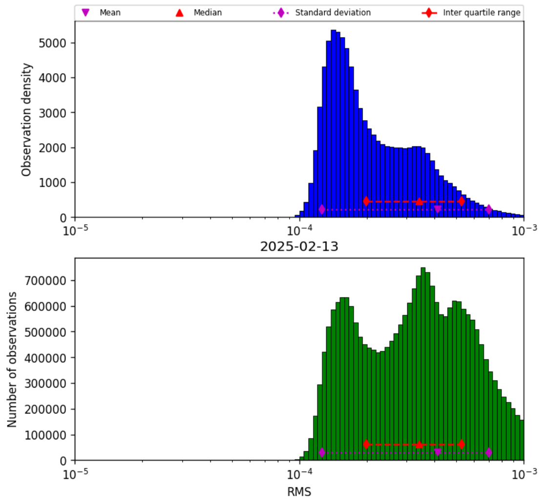
Figure 41: Histogram of “RMS” for 2025-02-13 to 2025-02-14
