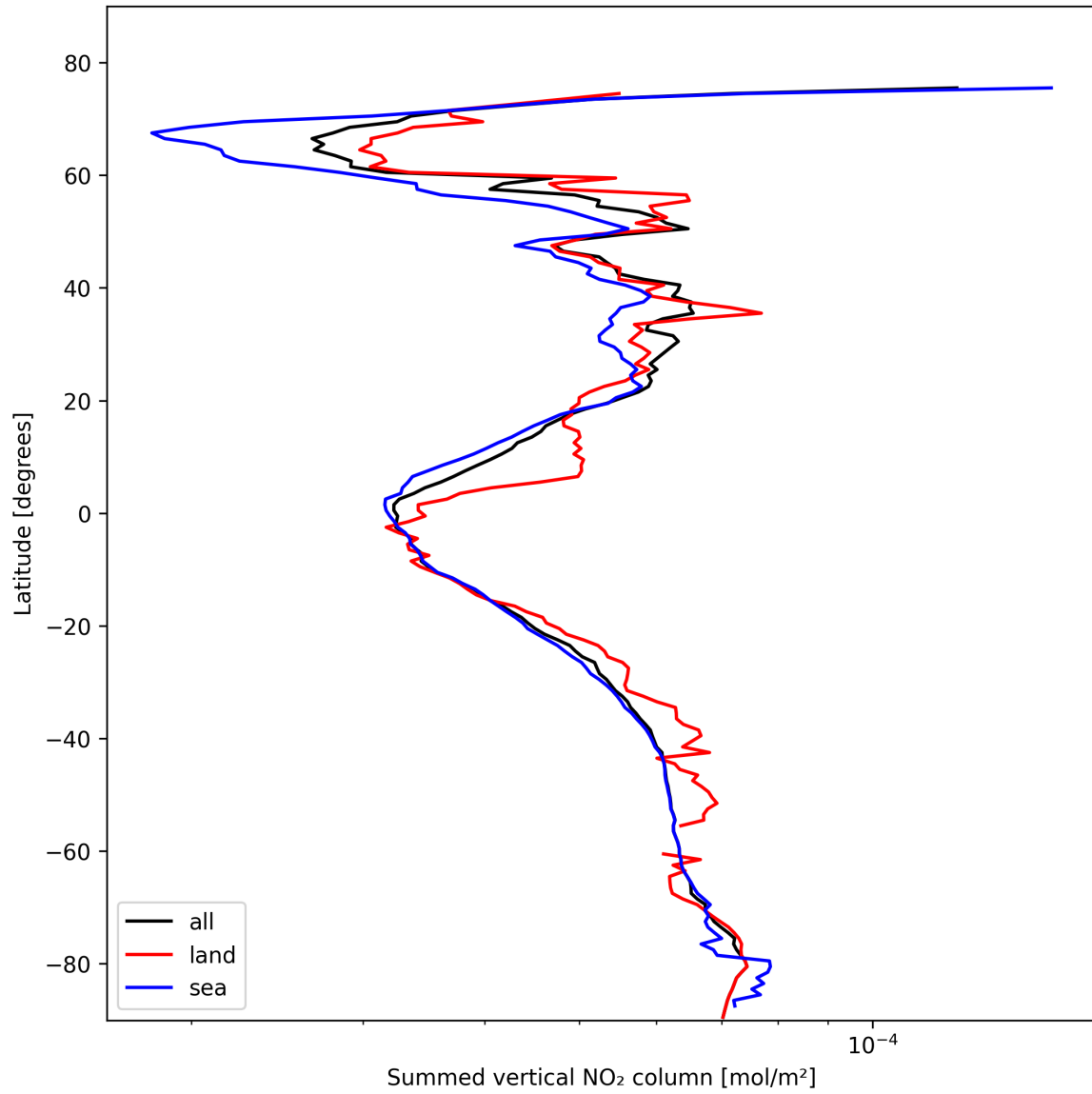
Figure 21: Zonal average of “Summed vertical NO 2 column” for 2025-02-13 to 2025-02-14.
