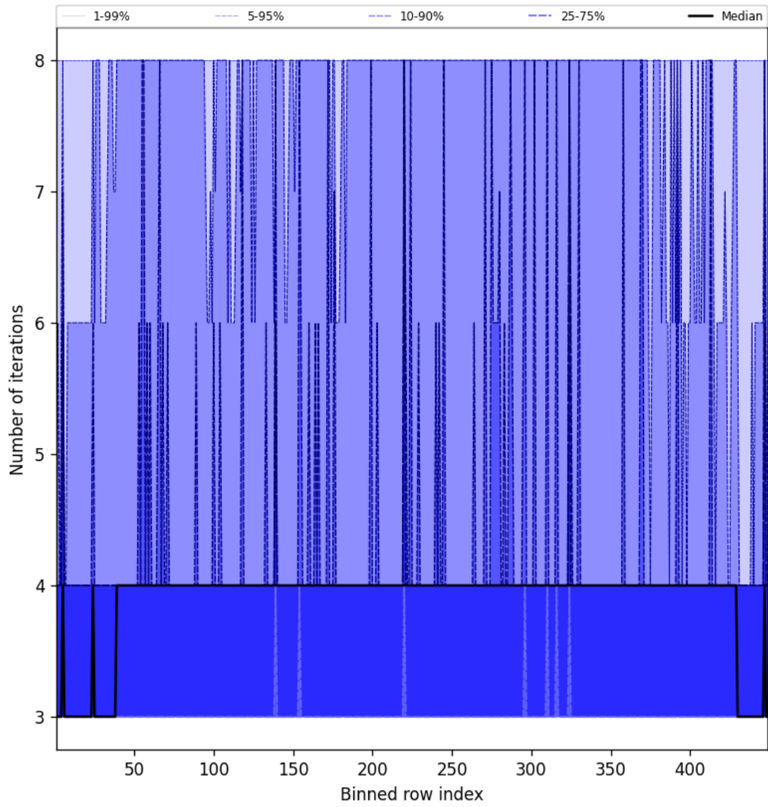
Figure 49: Along track statistics of “Number of iterations” for 2025-02-14 to 2025-02-15
