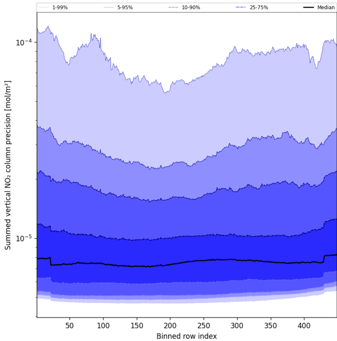
Figure 56: Along track statistics of “Summed vertical NO 2 column precision” for 2025-02-14 to 2025-02-15
