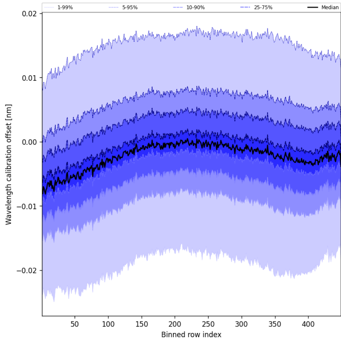
Figure 50: Along track statistics of “Wavelength calibration offset” for 2025-02-14 to 2025-02-15
