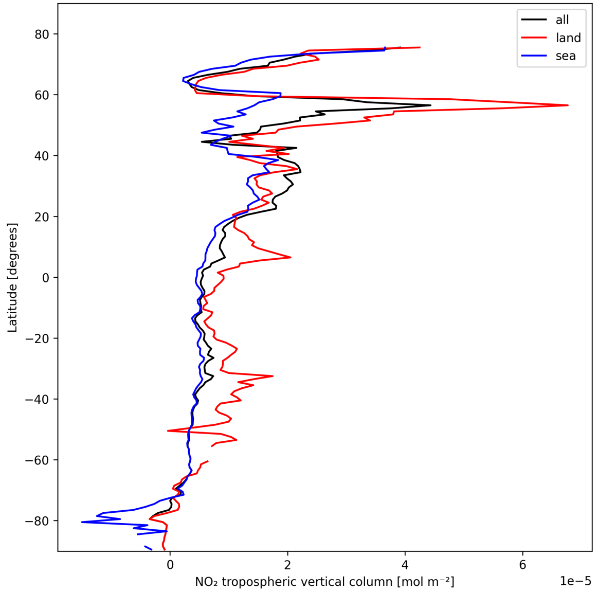
Figure 10: Zonal average of “NO 2 tropospheric vertical column” for 2025-02-14 to 2025-02-15.
