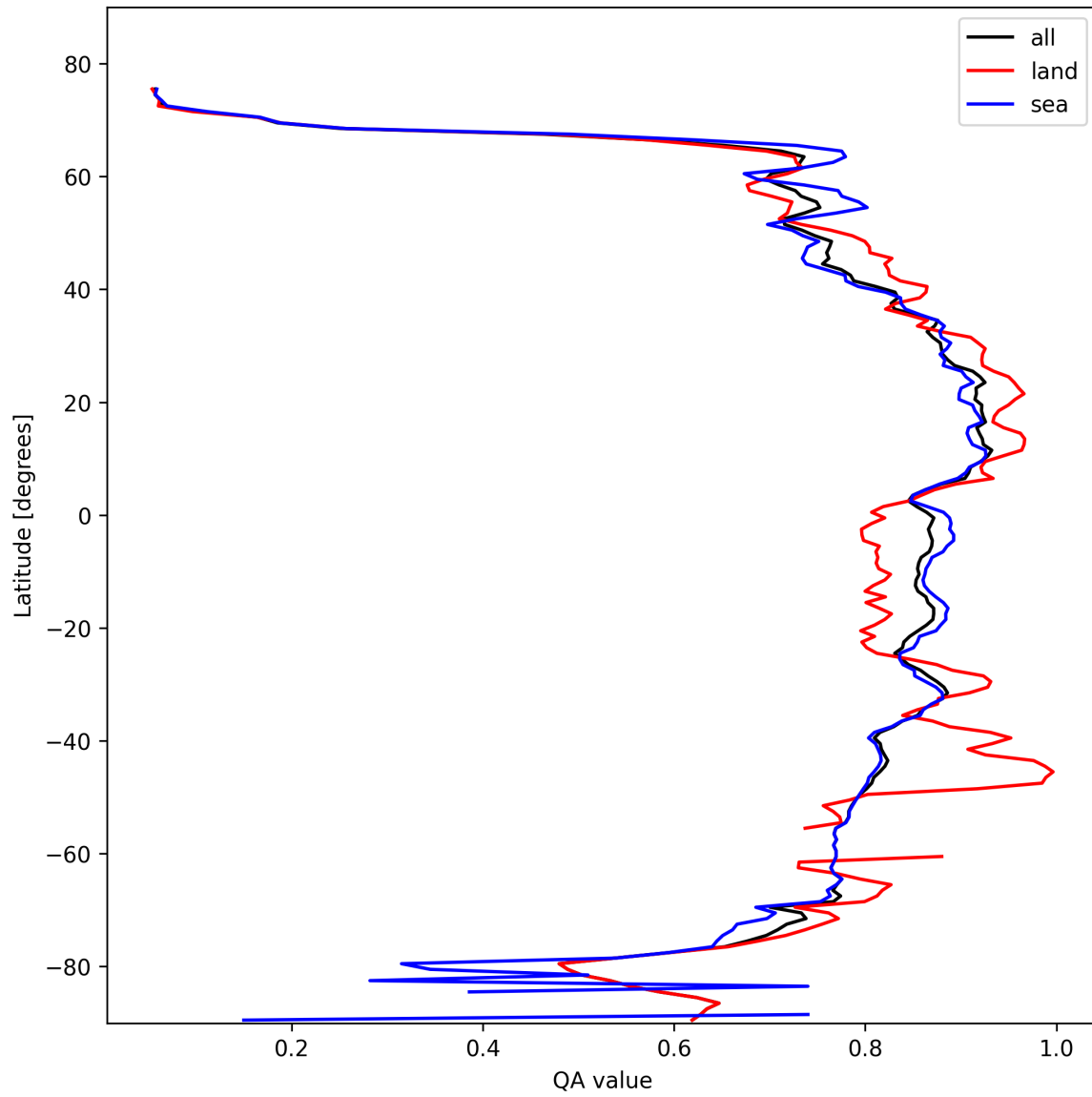
Figure 9: Zonal average of “QA value” for 2025-02-14 to 2025-02-15.
