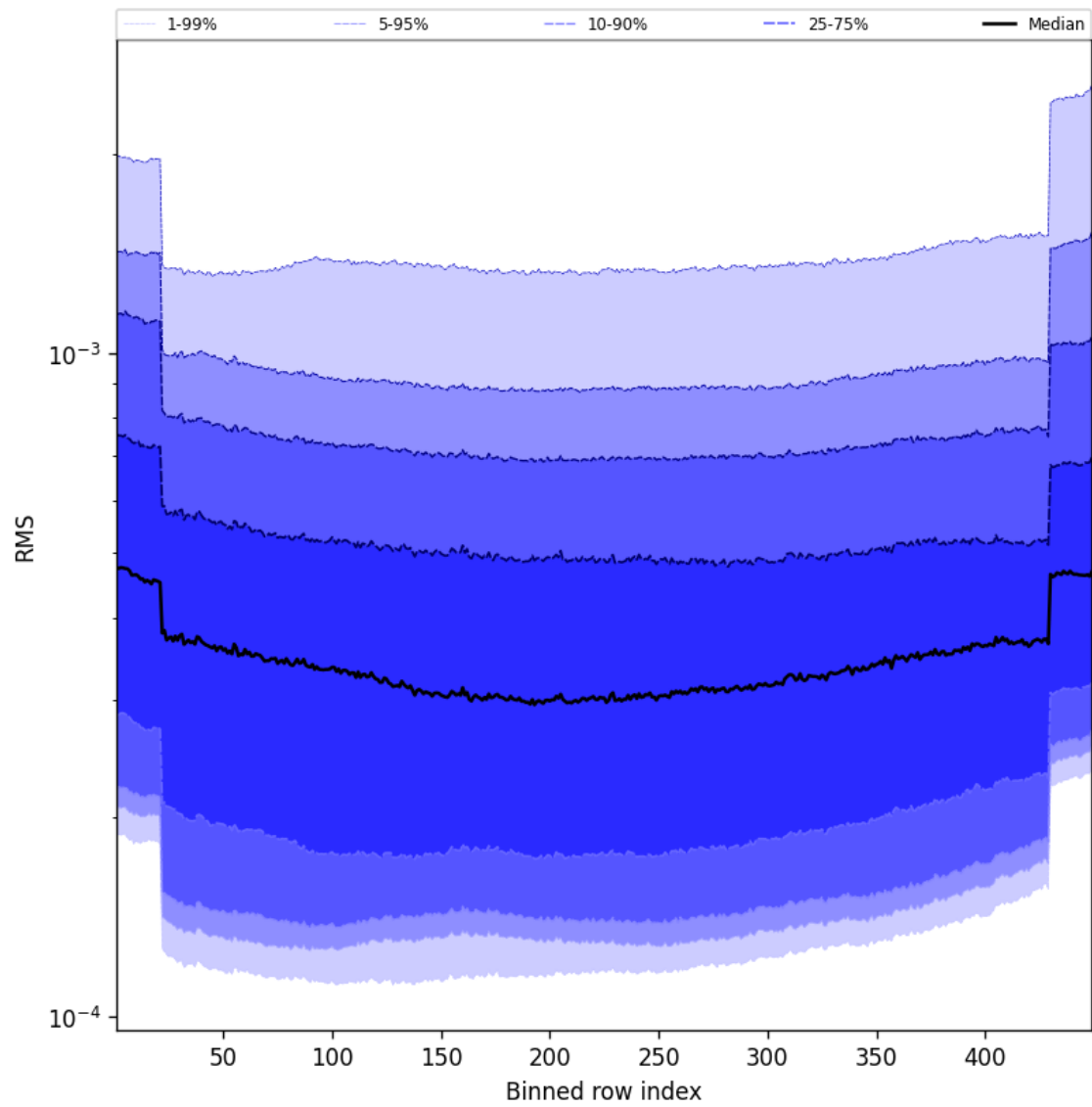
Figure 58: Along track statistics of “RMS” for 2025-02-14 to 2025-02-15
