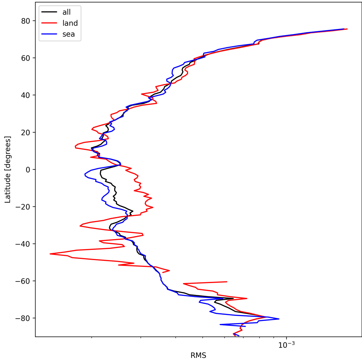
Figure 24: Zonal average of “RMS” for 2025-02-14 to 2025-02-15.
