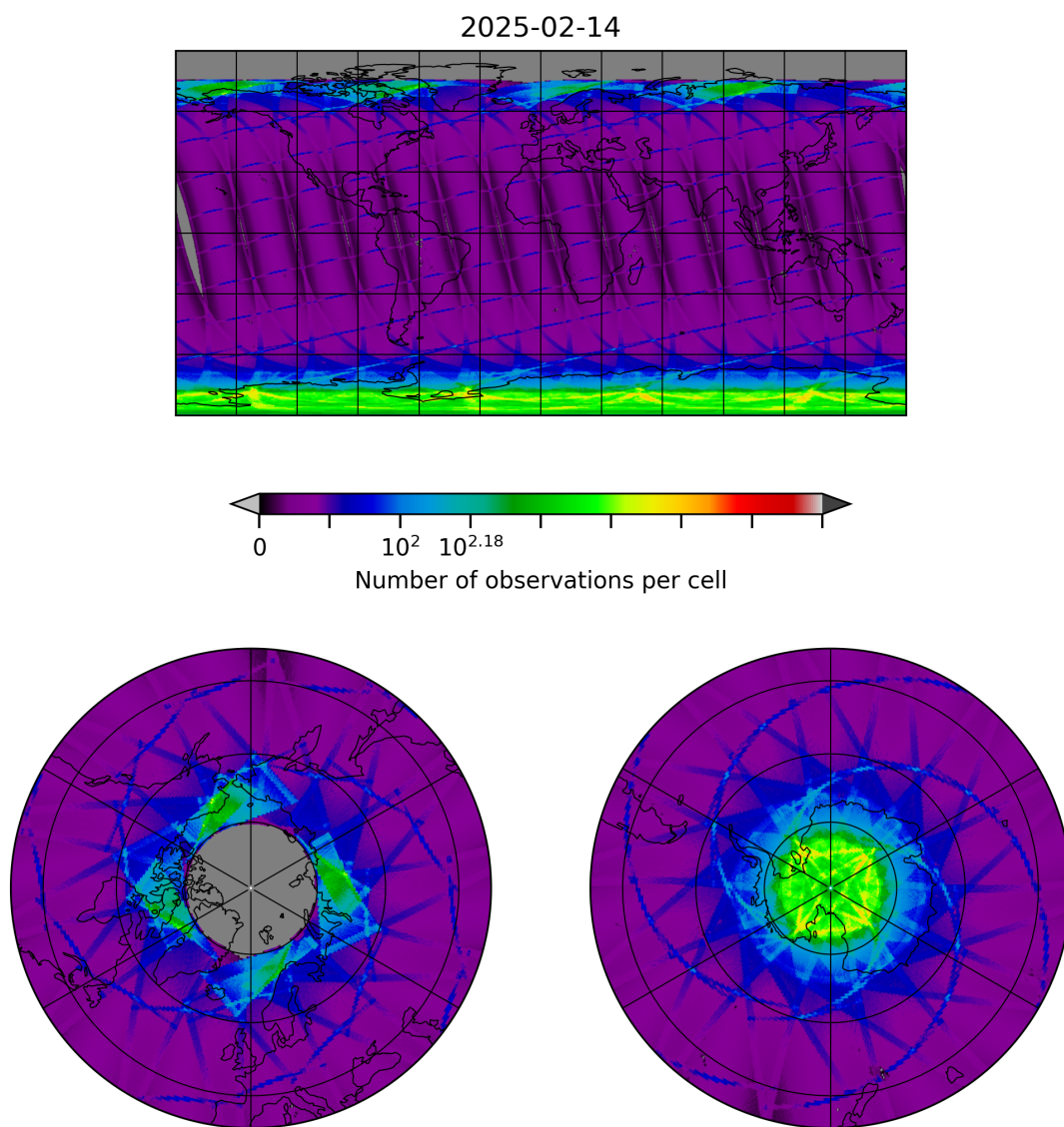
Figure 8: Map of the number of observations for 2025-02-14 to 2025-02-15
