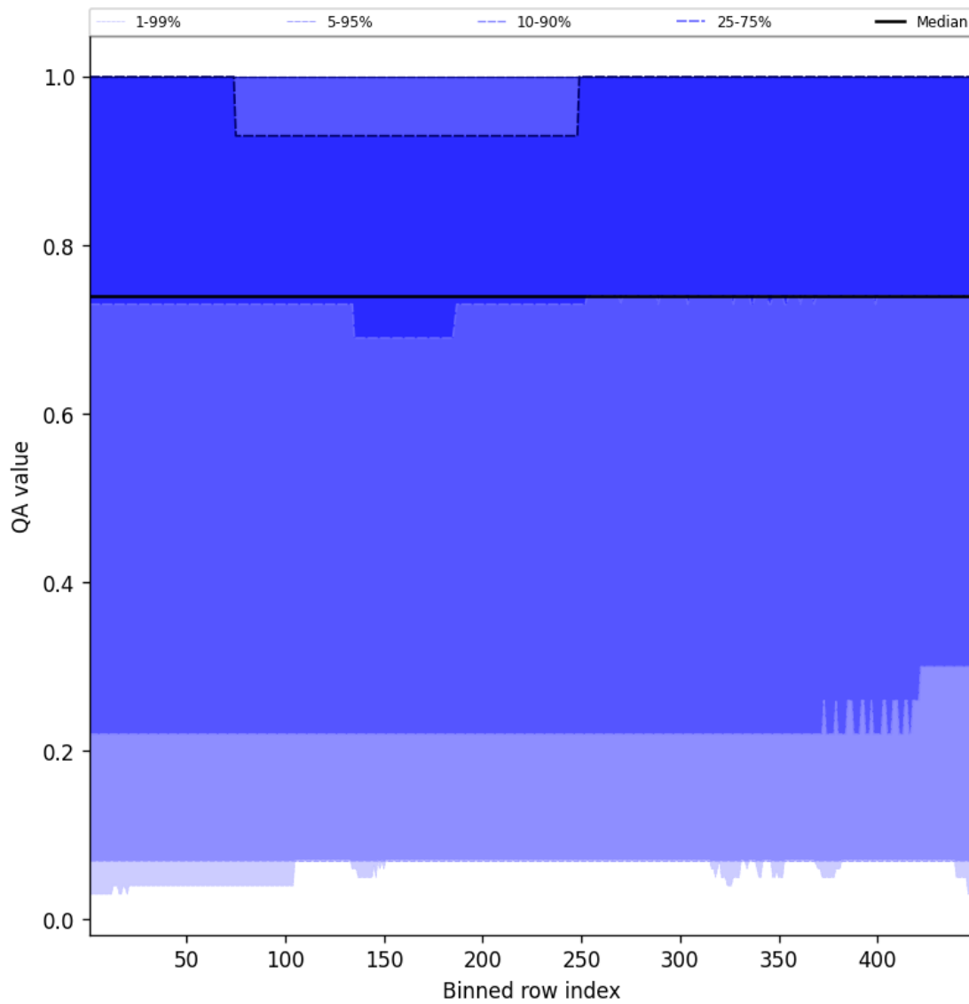
Figure 43: Along track statistics of “QA value” for 2025-02-14 to 2025-02-15
