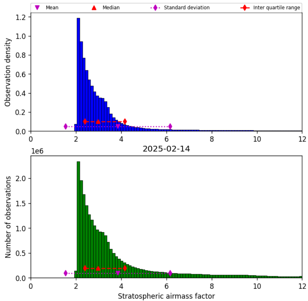
Figure 42: Histogram of “Stratospheric airmass factor” for 2025-02-14 to 2025-02-15
