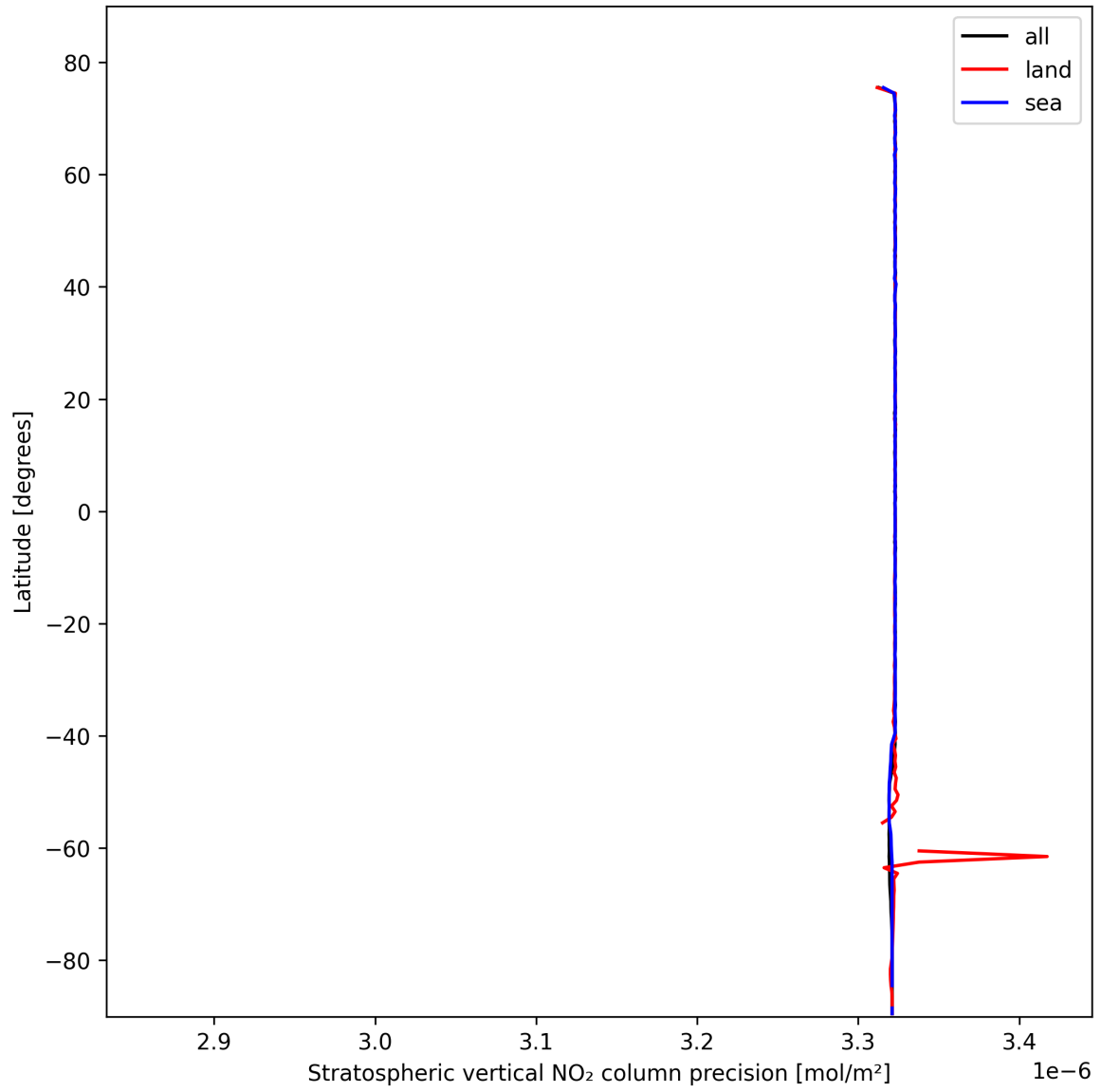
Figure 18: Zonal average of “Stratospheric vertical NO 2 column precision” for 2025-02-14 to 2025-02-15.
