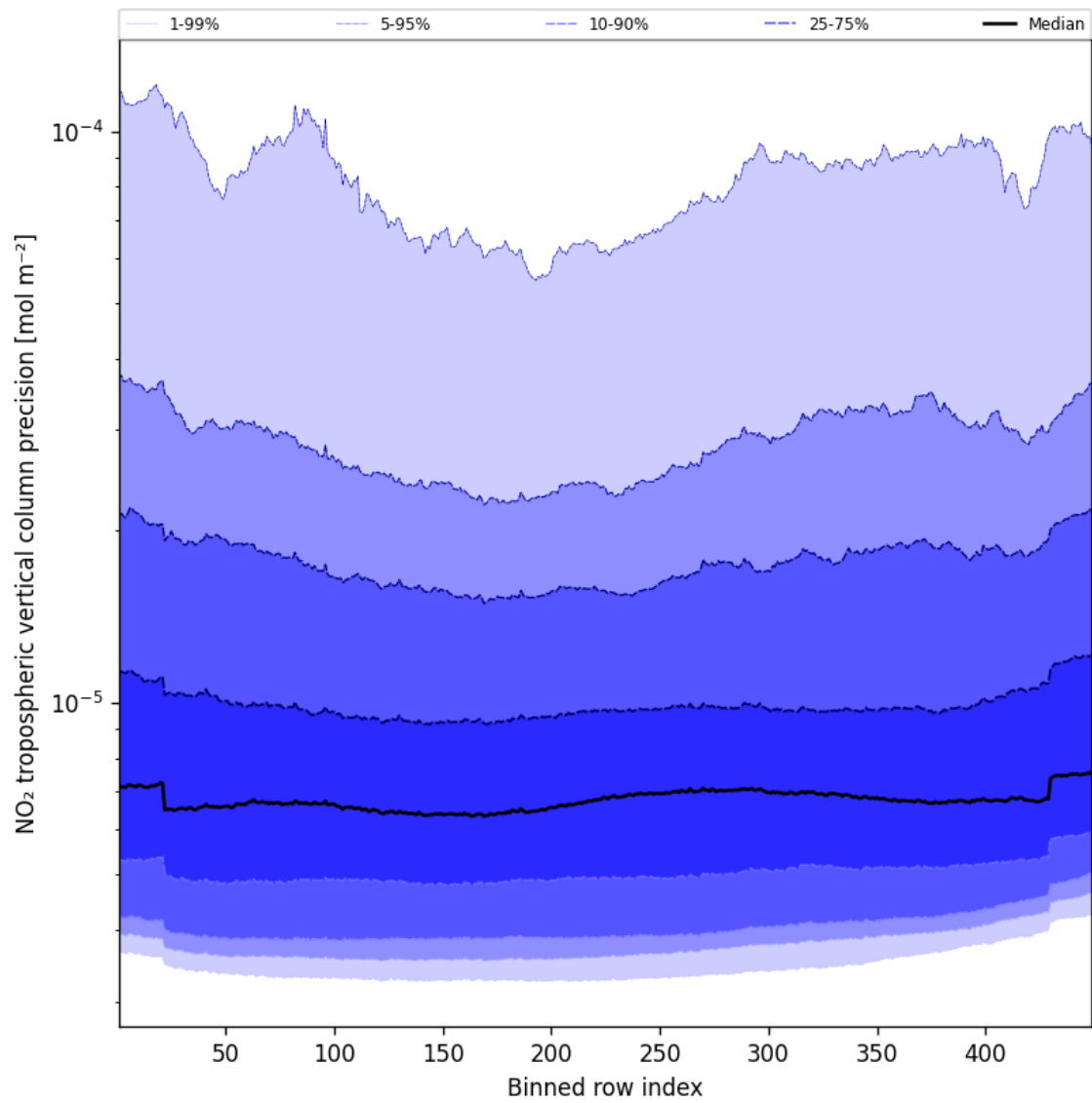
Figure 45: Along track statistics of “NO 2 tropospheric vertical column precision” for 2025-02-14 to 2025-02-15
