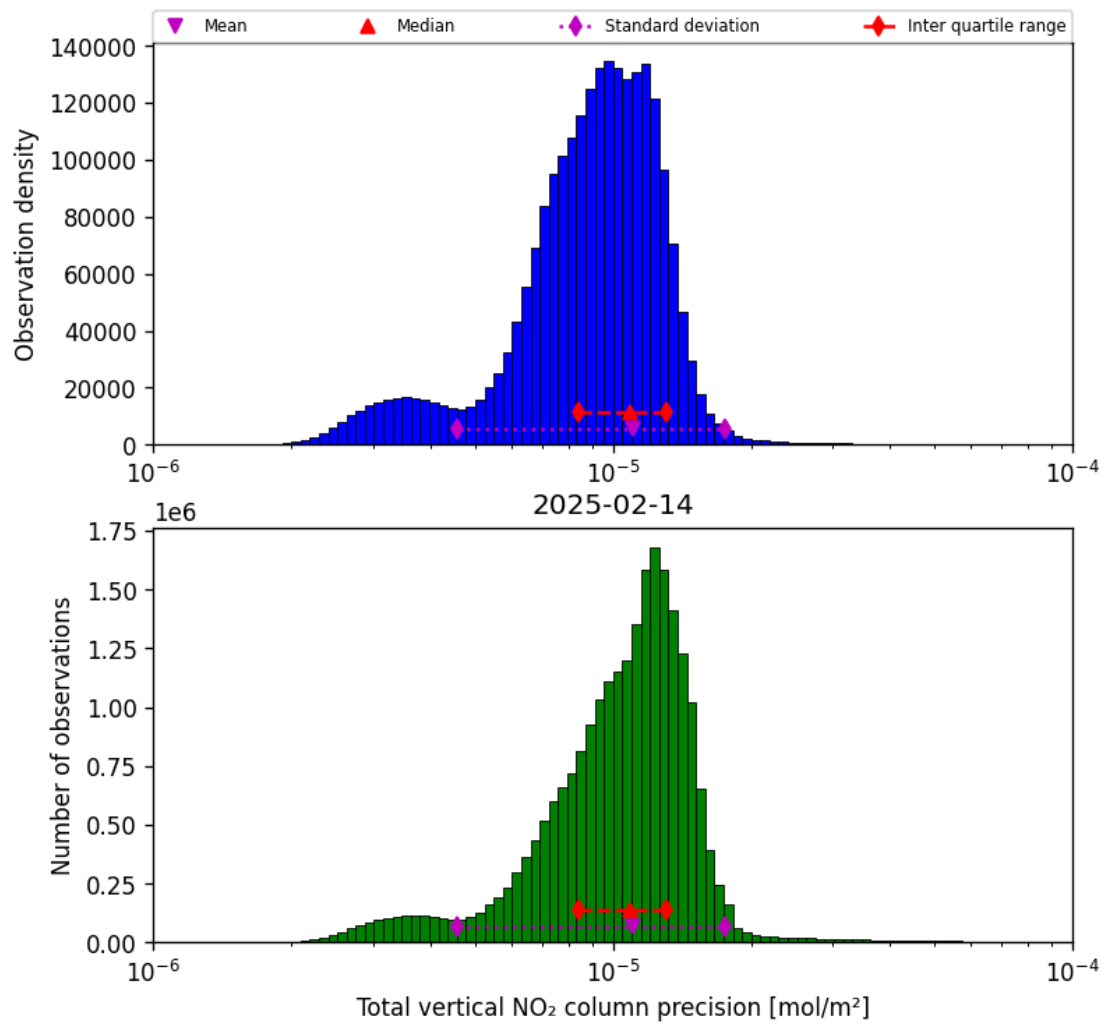
Figure 37: Histogram of “Total vertical NO 2 column precision” for 2025-02-14 to 2025-02-15
