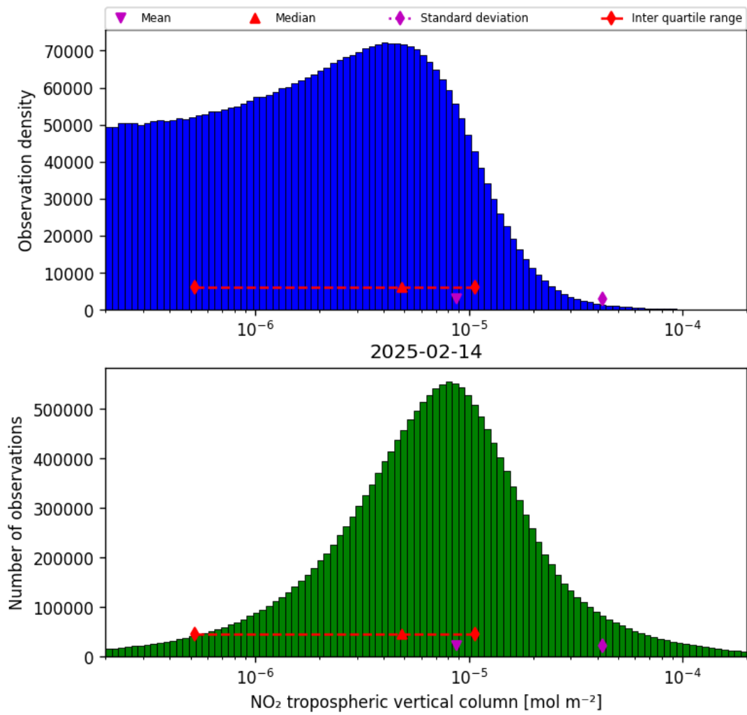
Figure 27: Histogram of “NO 2 tropospheric vertical column” for 2025-02-14 to 2025-02-15
