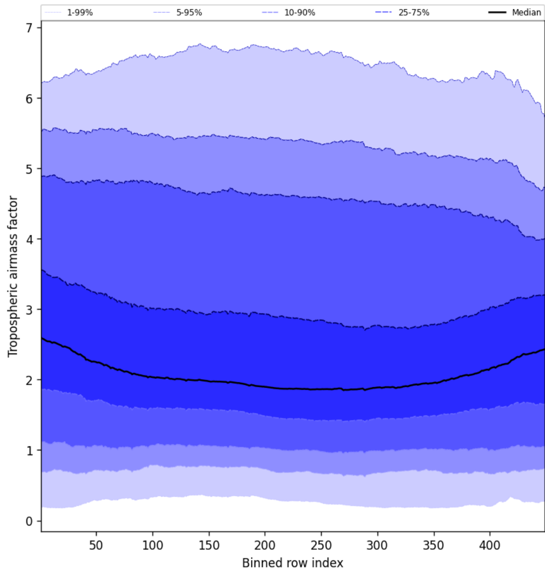
Figure 46: Along track statistics of “Tropospheric airmass factor” for 2025-02-14 to 2025-02-15
