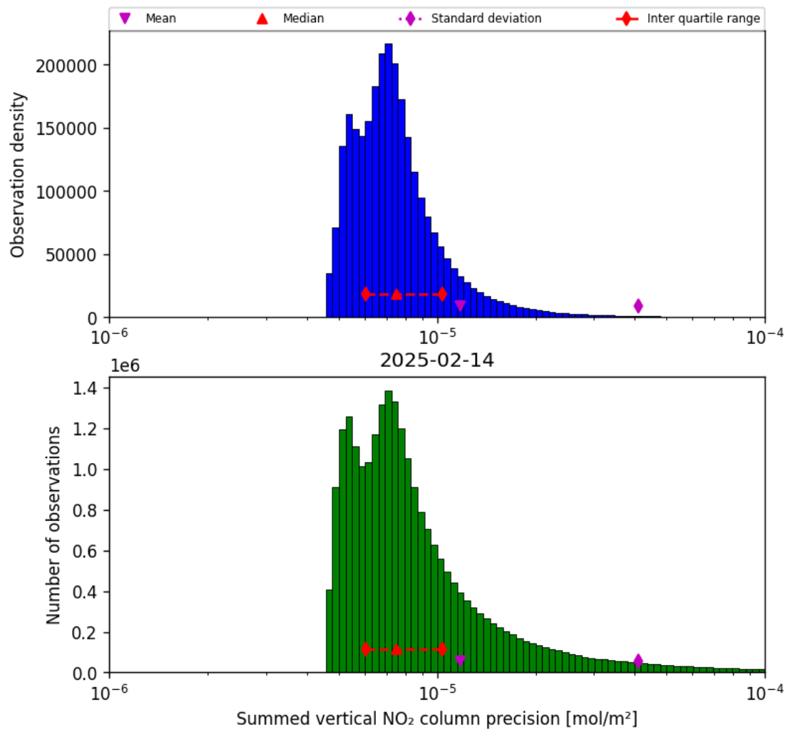
Figure 39: Histogram of “Summed vertical NO 2 column precision” for 2025-02-14 to 2025-02-15
