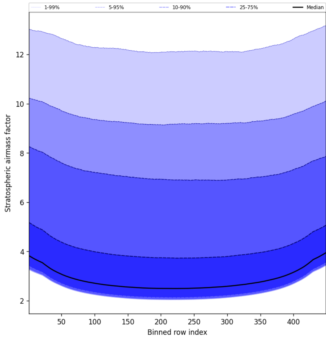
Figure 59: Along track statistics of “Stratospheric airmass factor” for 2025-02-14 to 2025-02-15
