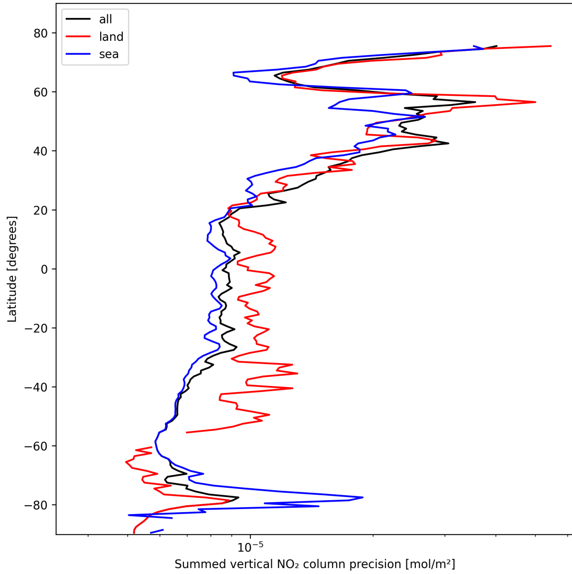
Figure 22: Zonal average of “Summed vertical NO 2 column precision” for 2025-02-14 to 2025-02-15.
