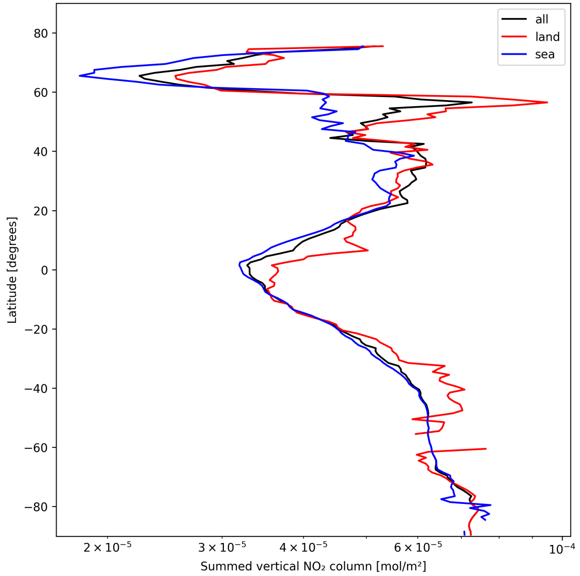
Figure 21: Zonal average of “Summed vertical NO 2 column” for 2025-02-14 to 2025-02-15.
