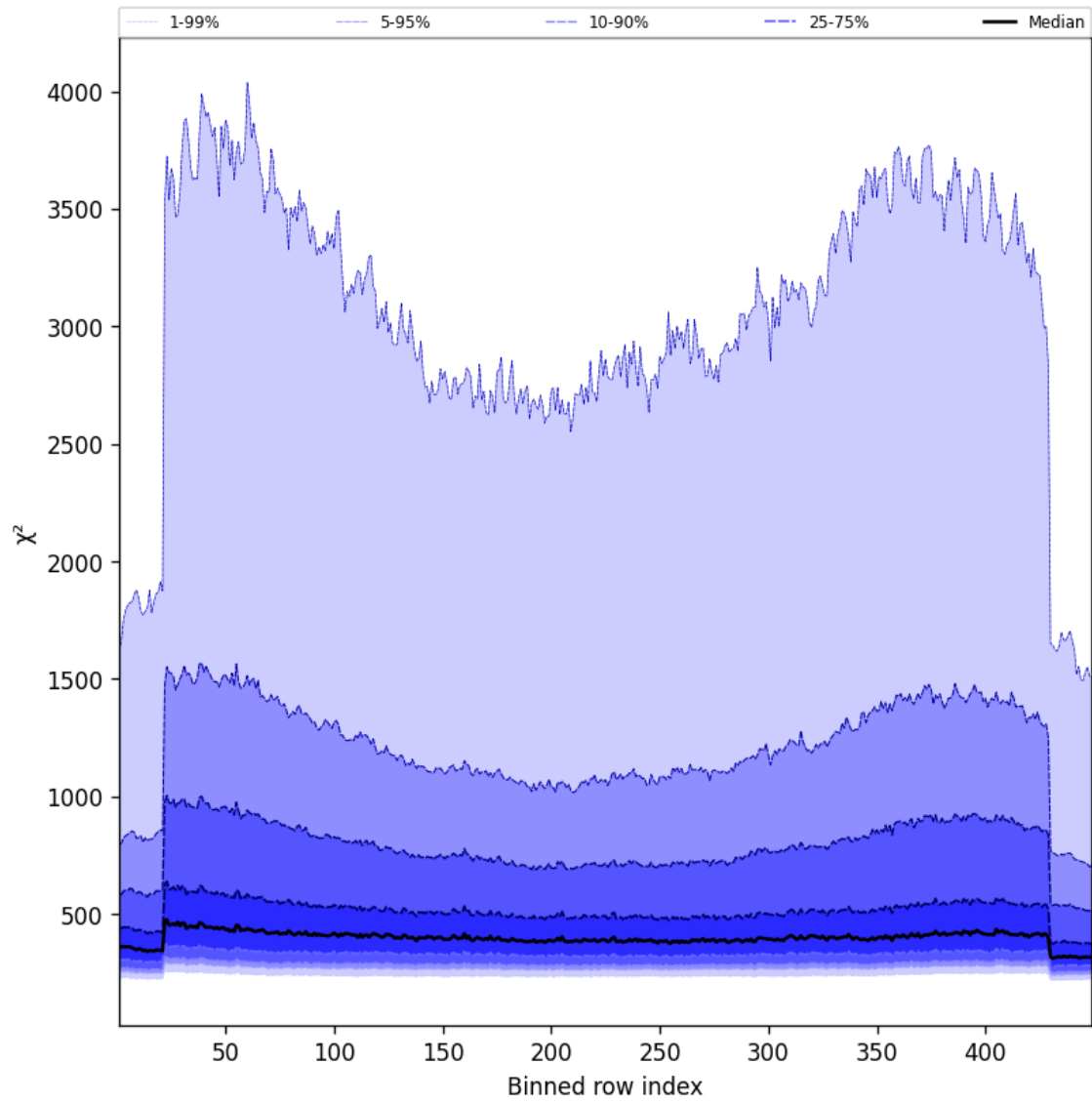
Figure 57: Along track statistics of “ \chi^2 ” for 2025-02-14 to 2025-02-15
