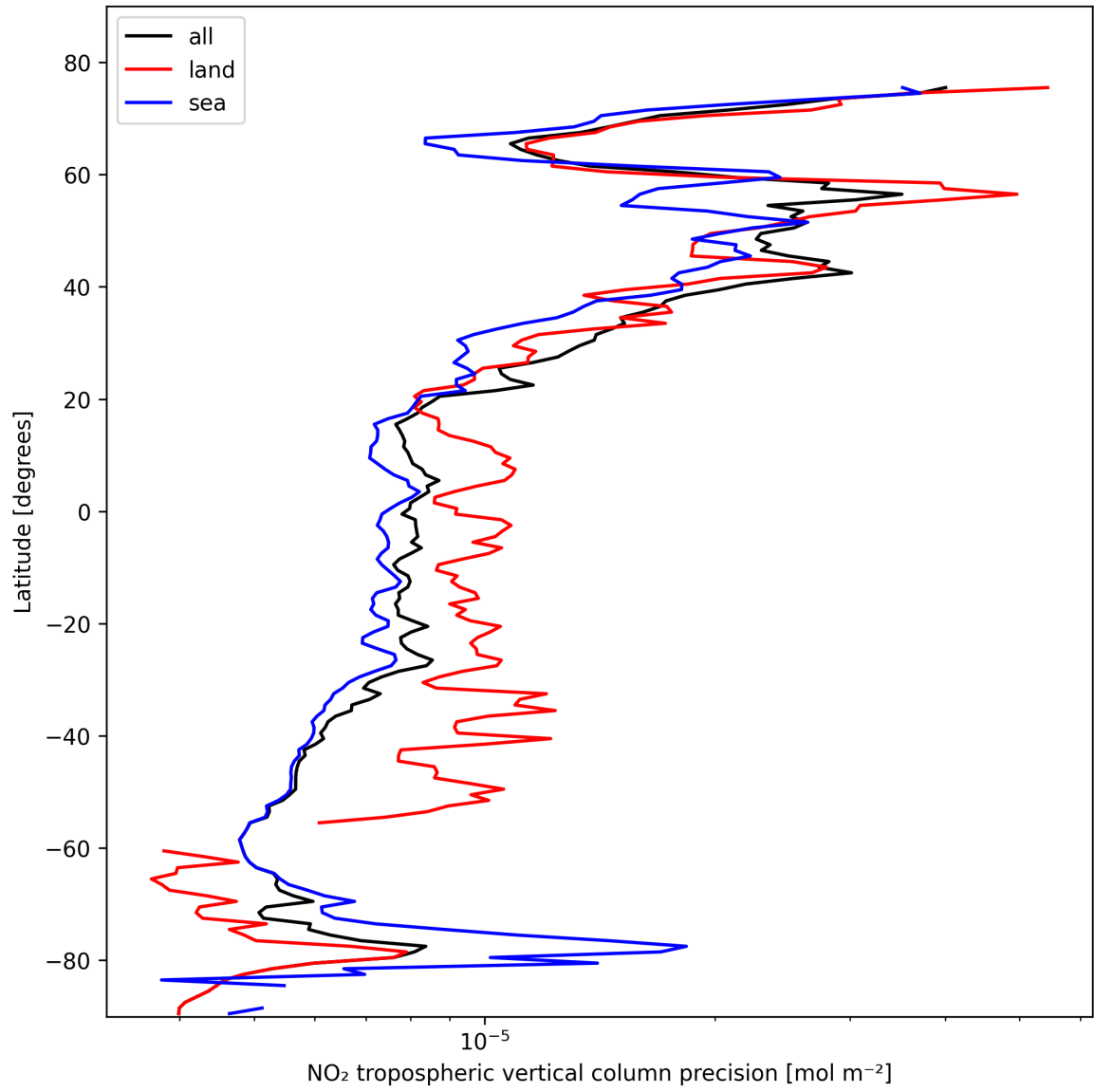
Figure 11: Zonal average of “NO 2 tropospheric vertical column precision” for 2025-02-14 to 2025-02-15.
