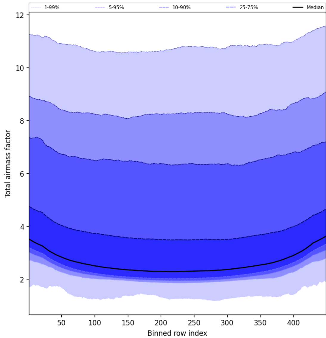
Figure 47: Along track statistics of “Total airmass factor” for 2025-02-14 to 2025-02-15
