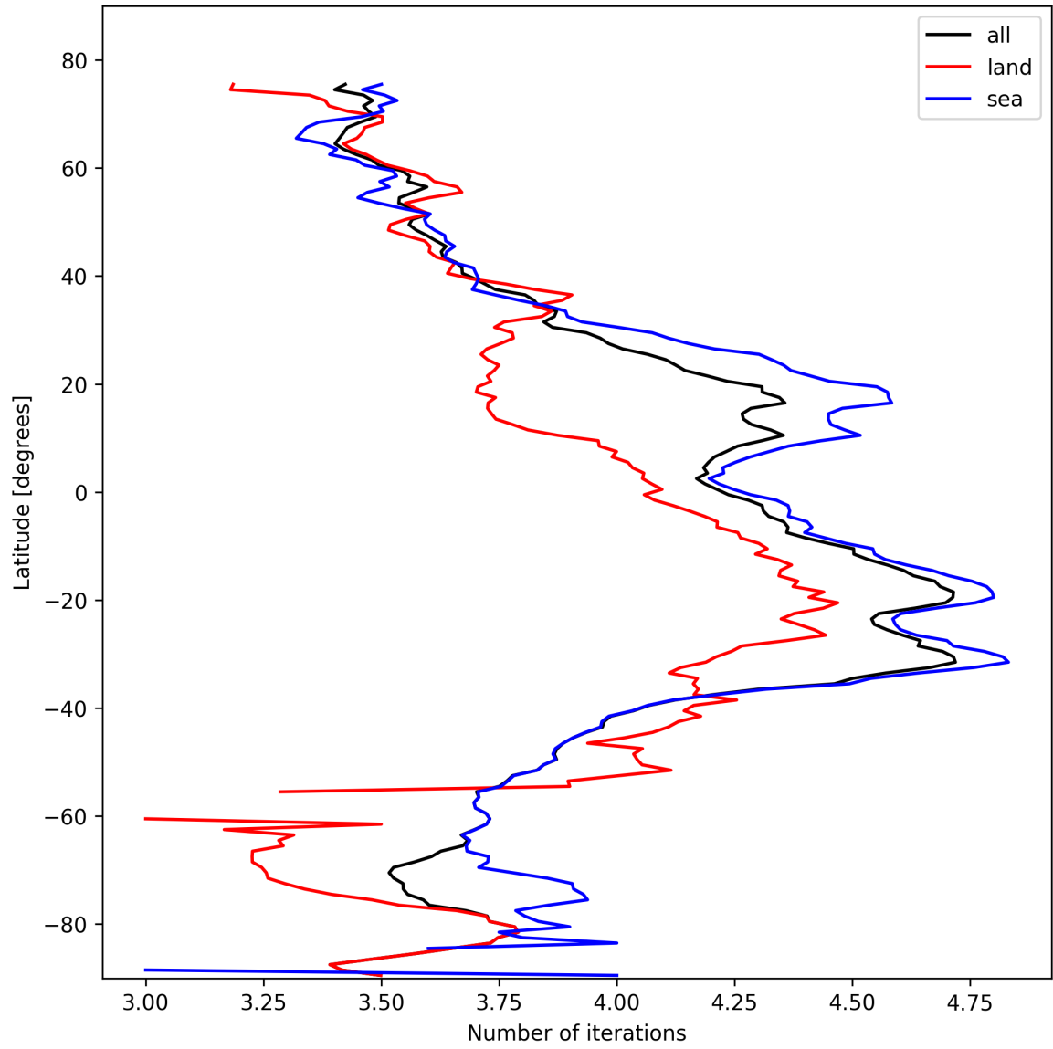
Figure 15: Zonal average of “Number of iterations” for 2025-02-14 to 2025-02-15.
