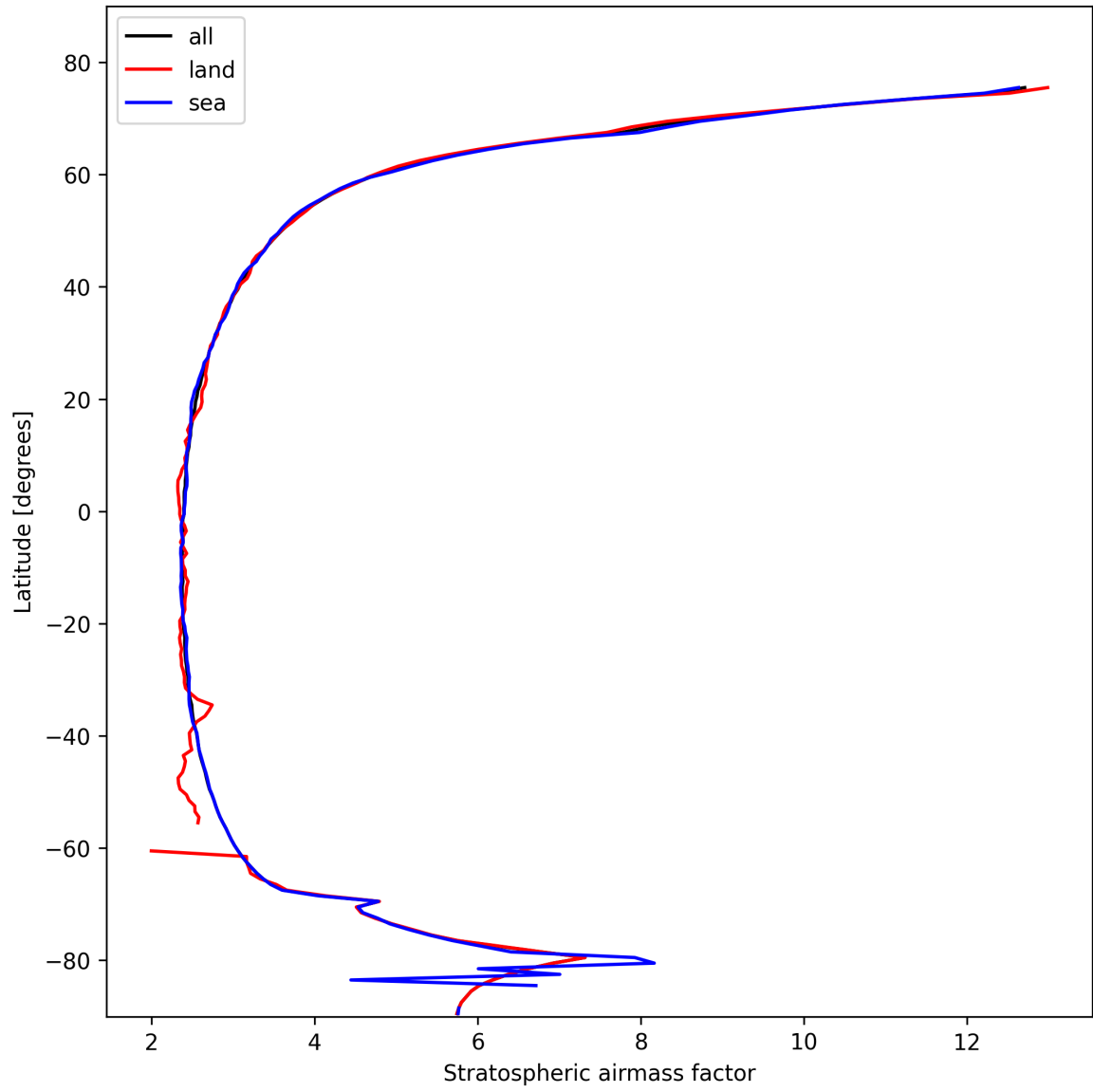
Figure 25: Zonal average of “Stratospheric air mass factor” for 2025-02-14 to 2025-02-15.
