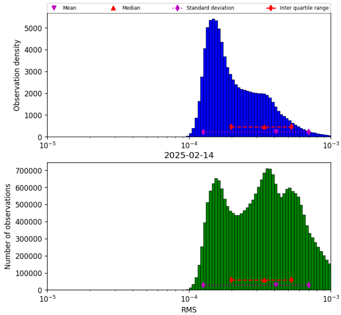
Figure 41: Histogram of “RMS” for 2025-02-14 to 2025-02-15
