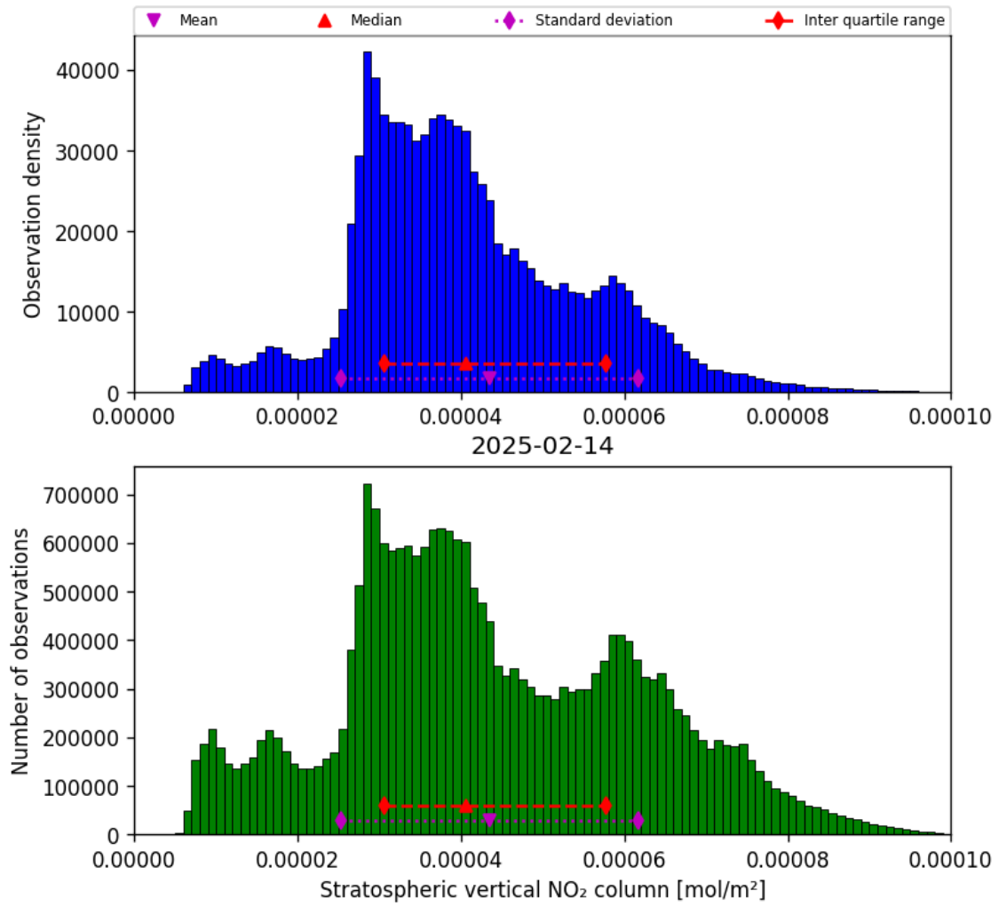
Figure 34: Histogram of “Stratospheric vertical NO 2 column” for 2025-02-14 to 2025-02-15
