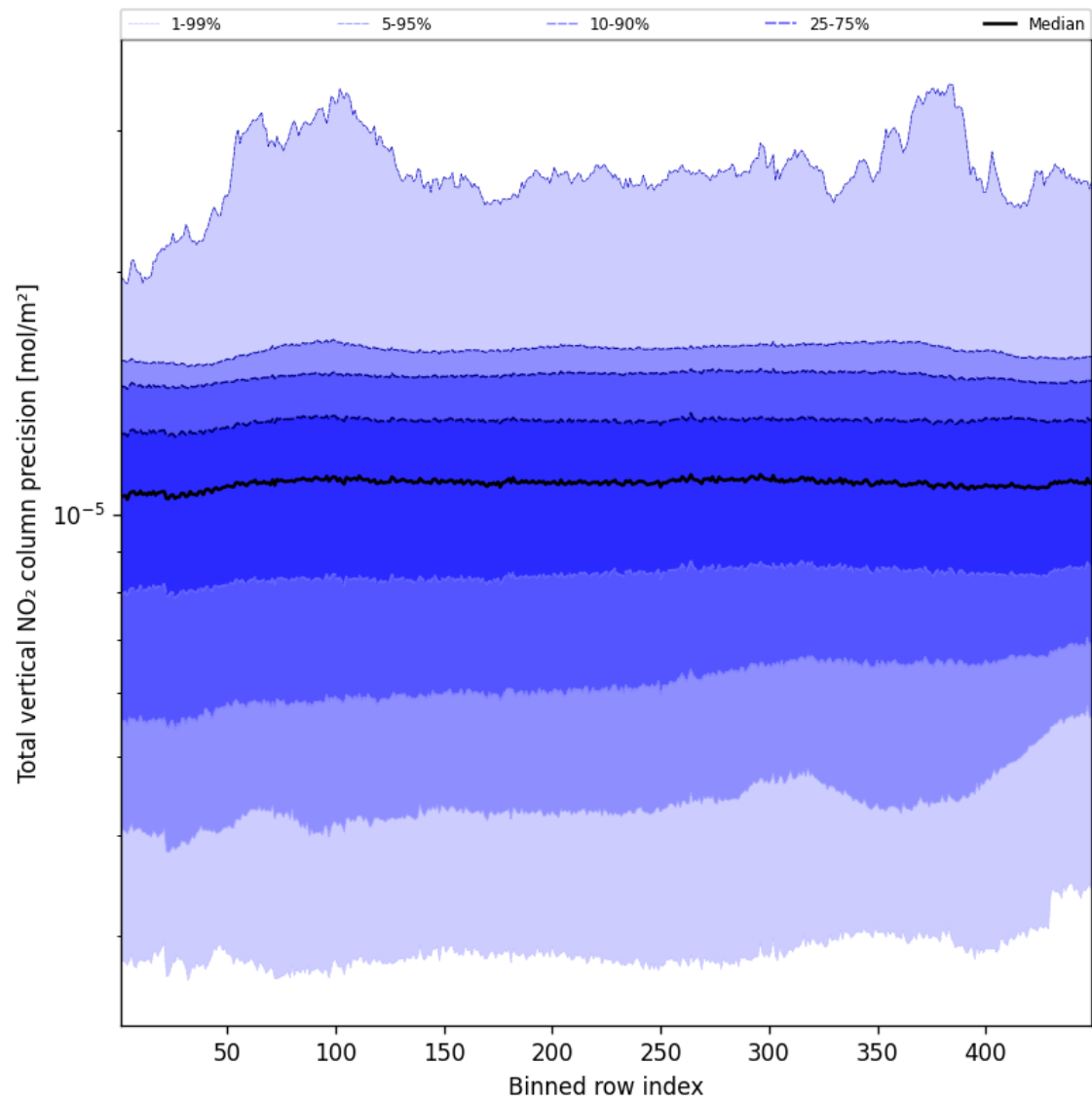
Figure 54: Along track statistics of “Total vertical NO 2 column precision” for 2025-02-14 to 2025-02-15
