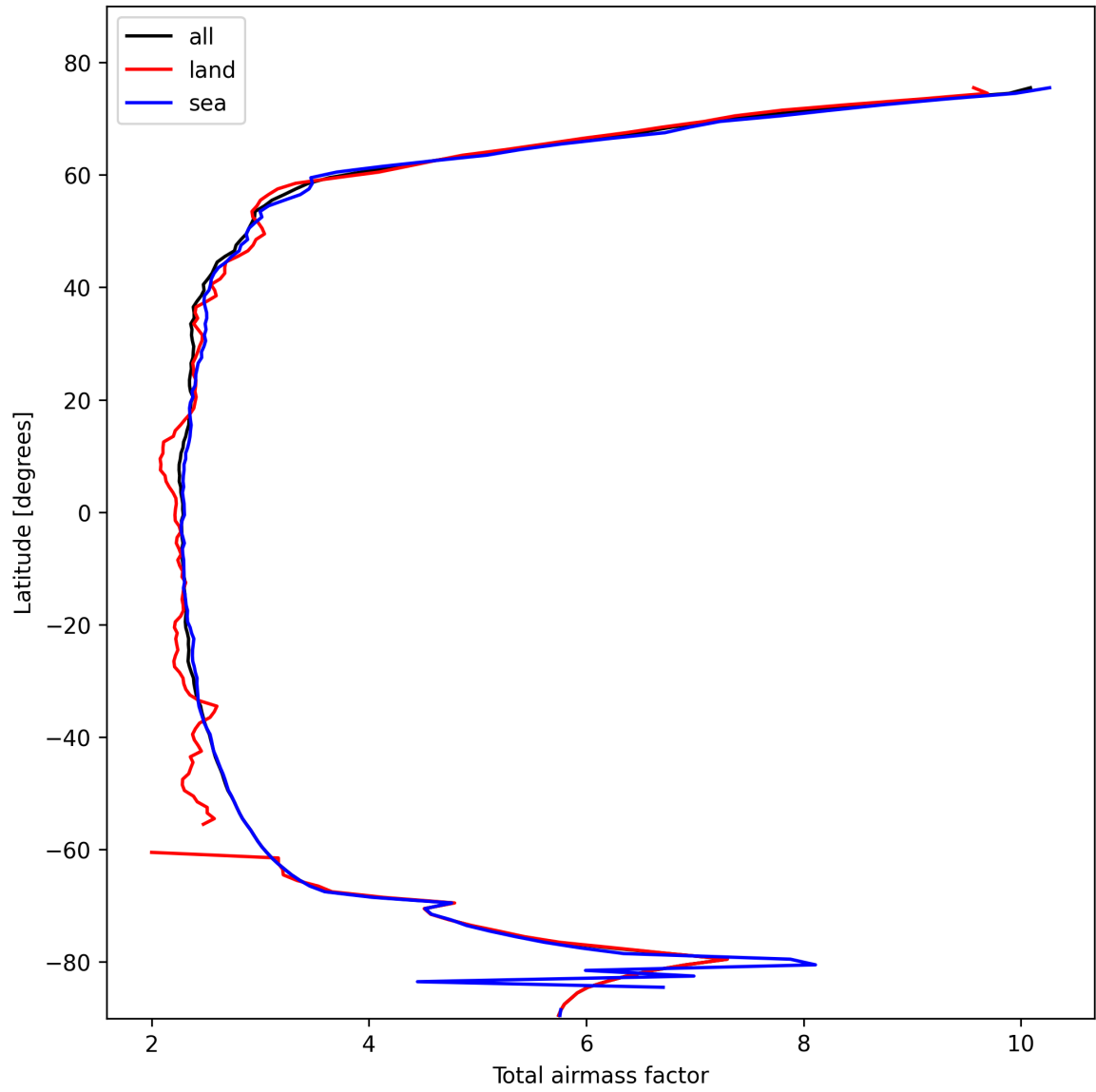
Figure 13: Zonal average of “Total airmass factor” for 2025-02-14 to 2025-02-15.
