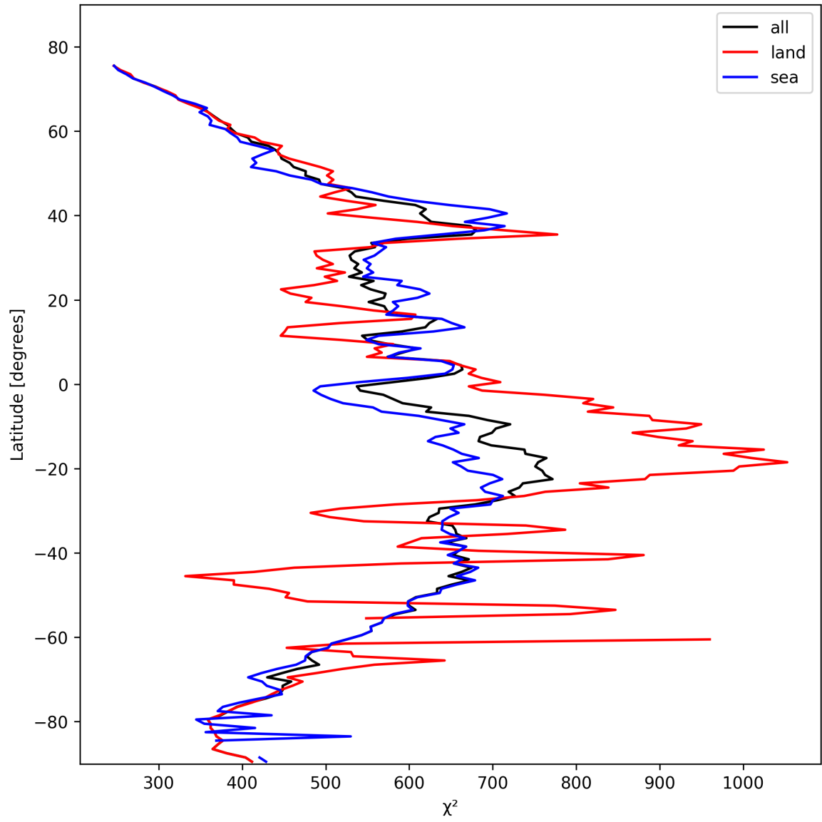
Figure 23: Zonal average of “ \chi^2 ” for 2025-02-14 to 2025-02-15.
