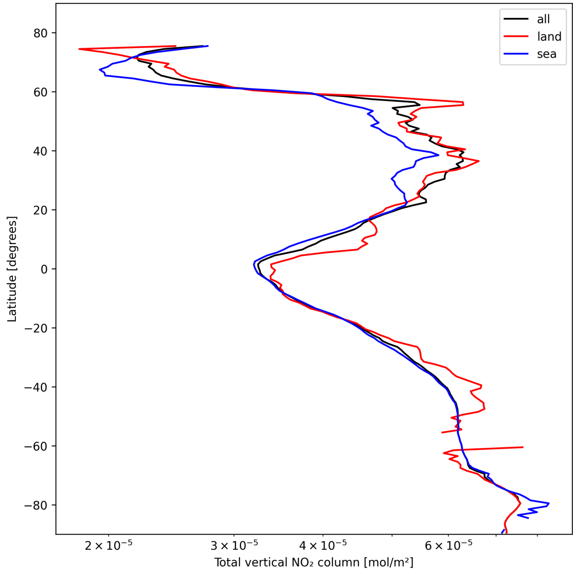
Figure 19: Zonal average of “Total vertical NO 2 column” for 2025-02-14 to 2025-02-15.
