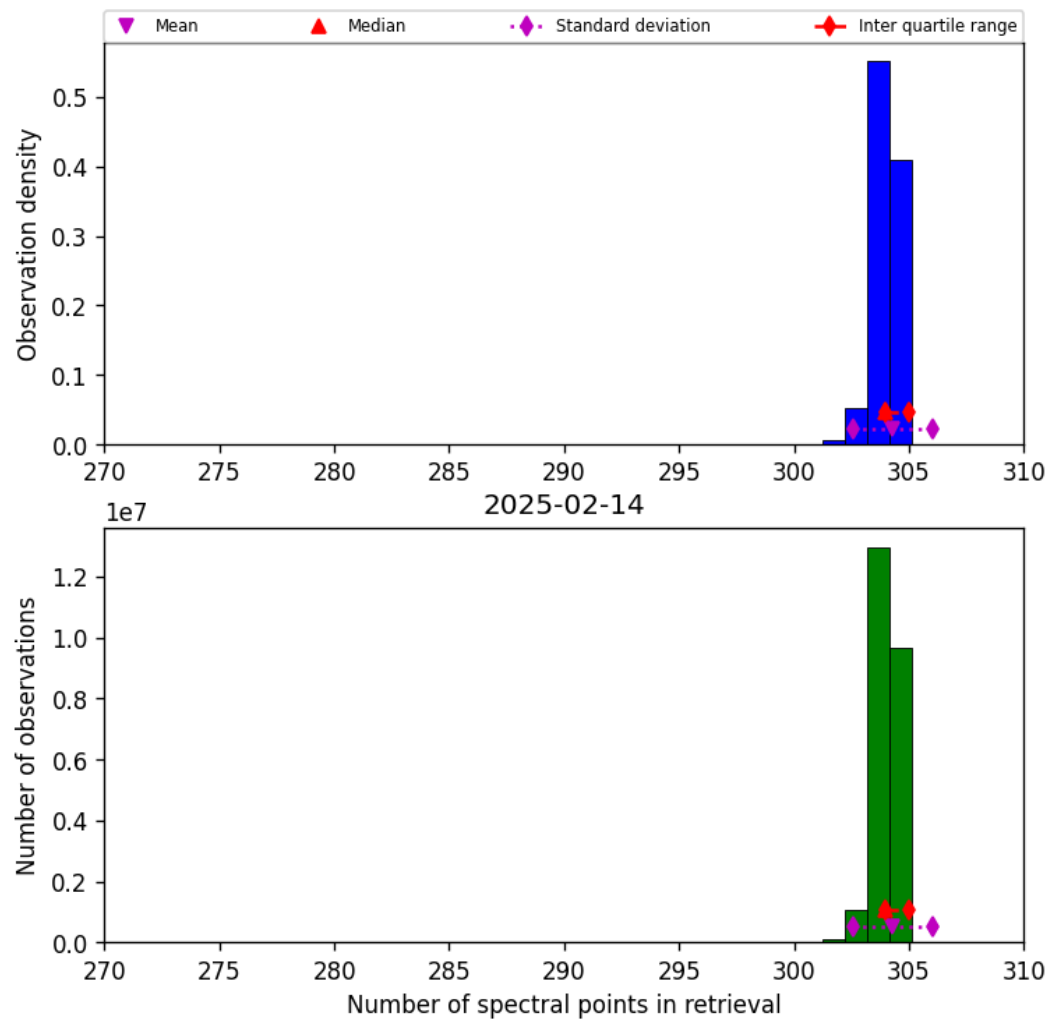
Figure 31: Histogram of “Number of spectral points in retrieval” for 2025-02-14 to 2025-02-15
