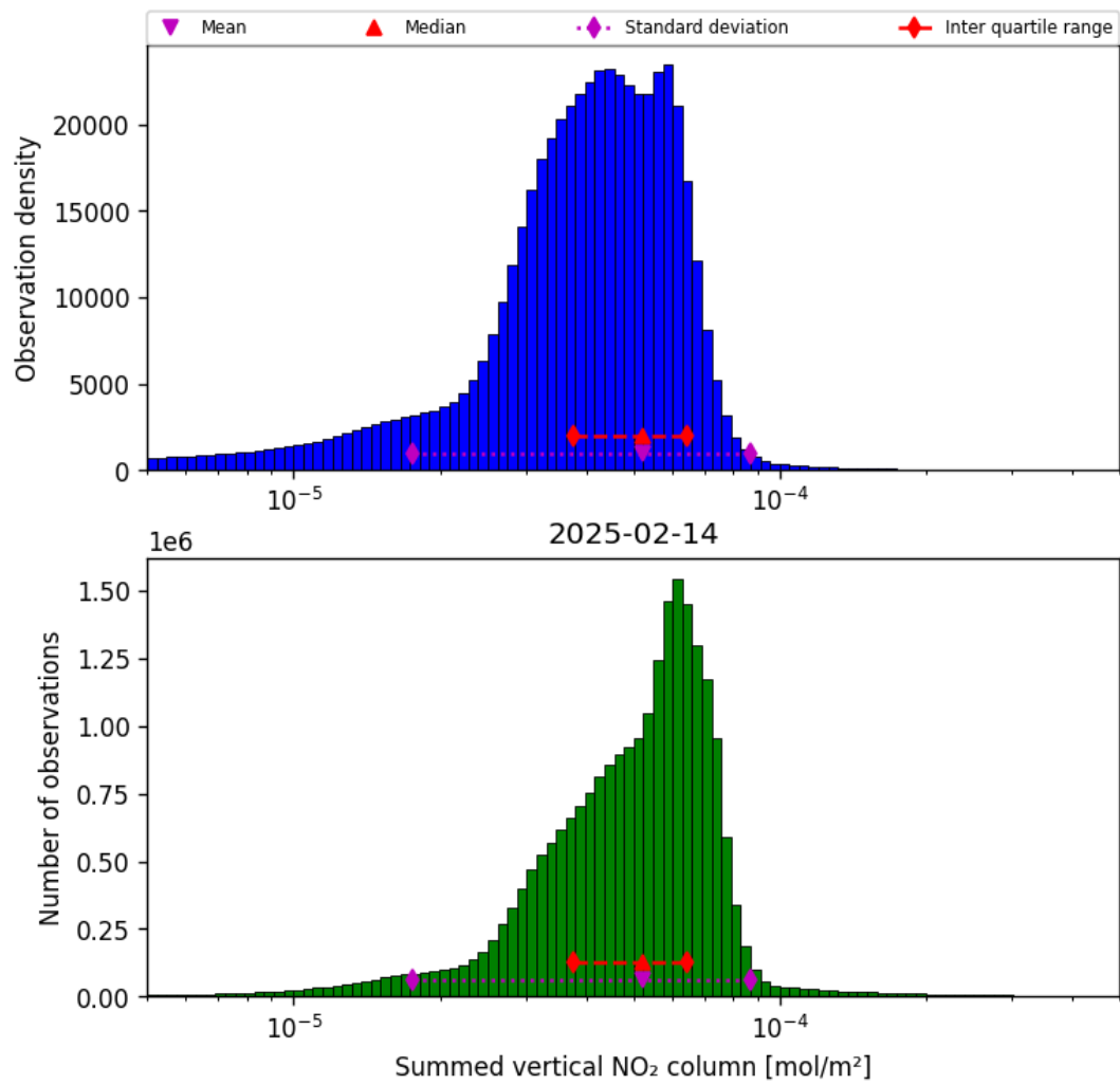
Figure 38: Histogram of “Summed vertical NO 2 column” for 2025-02-14 to 2025-02-15
