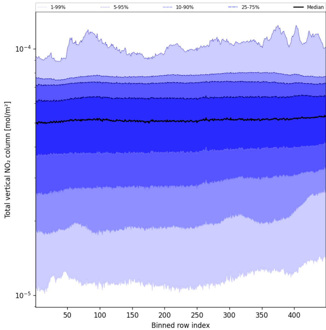
Figure 53: Along track statistics of “Total vertical NO 2 column” for 2025-02-14 to 2025-02-15
