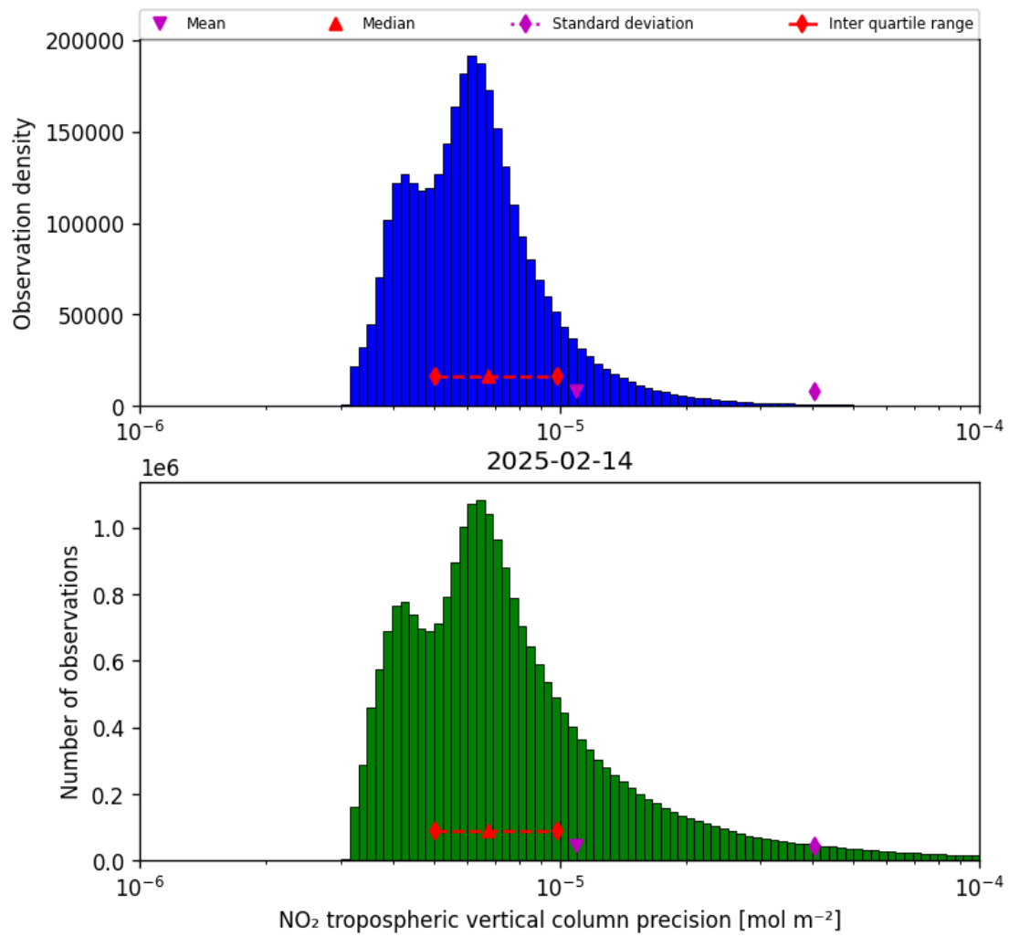
Figure 28: Histogram of “NO 2 tropospheric vertical column precision” for 2025-02-14 to 2025-02-15
