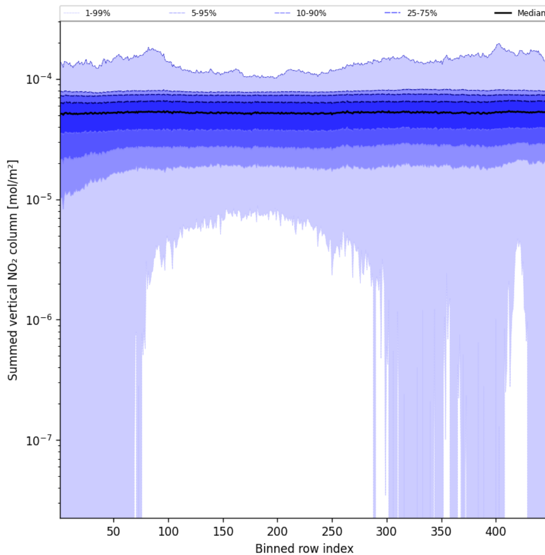
Figure 55: Along track statistics of “Summed vertical NO 2 column” for 2025-02-14 to 2025-02-15
