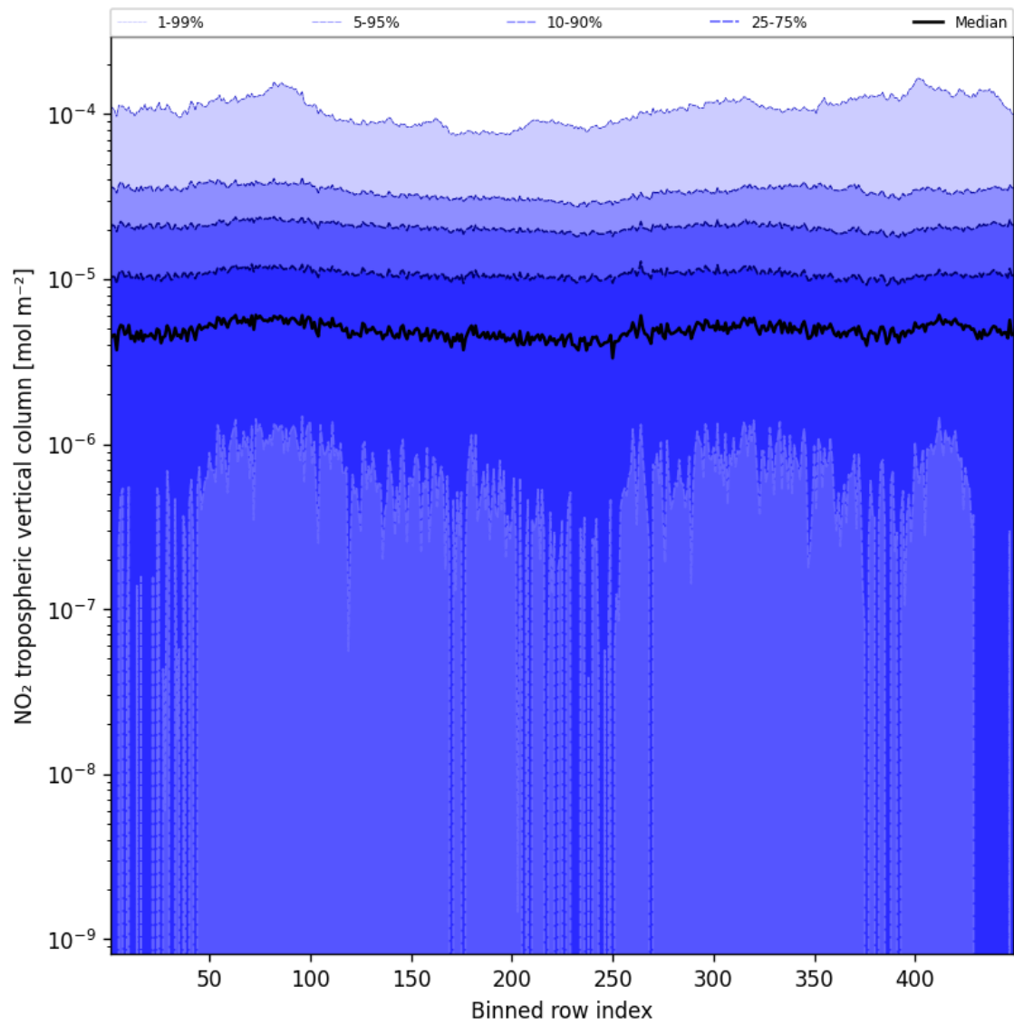
Figure 44: Along track statistics of “NO 2 tropospheric vertical column” for 2025-02-14 to 2025-02-15
