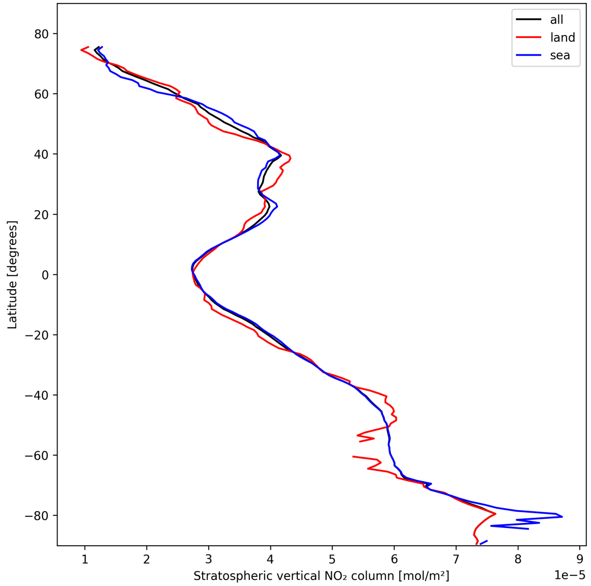
Figure 17: Zonal average of “Stratospheric vertical NO 2 column” for 2025-02-14 to 2025-02-15.
