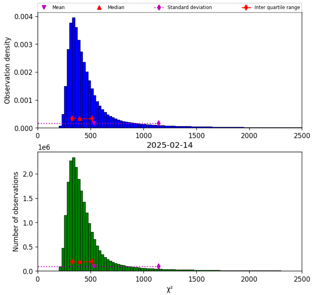
Figure 40: Histogram of “ \chi^2 ” for 2025-02-14 to 2025-02-15
