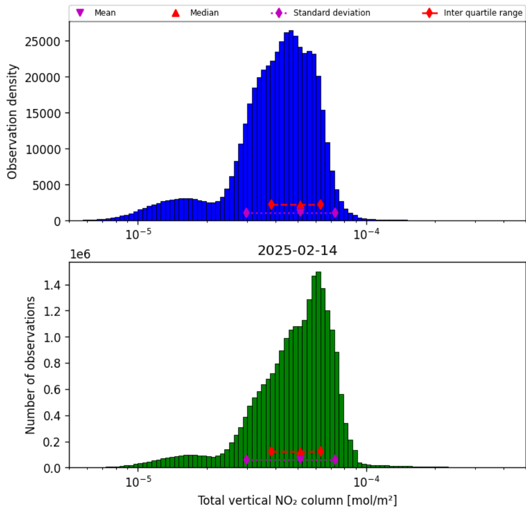
Figure 36: Histogram of "Total vertical NO 2 column" for 2025-02-14 to 2025-02-15
