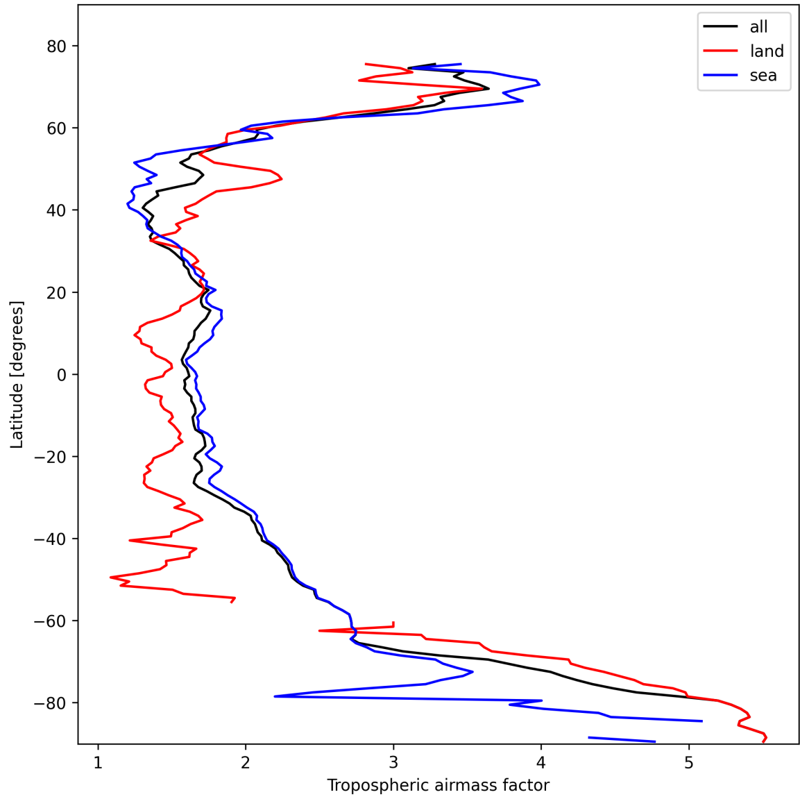
Figure 12: Zonal average of “Tropospheric airmass factor” for 2025-02-14 to 2025-02-15.
