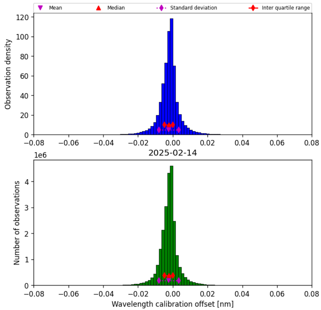
Figure 33: Histogram of “Wavelength calibration offset” for 2025-02-14 to 2025-02-15
