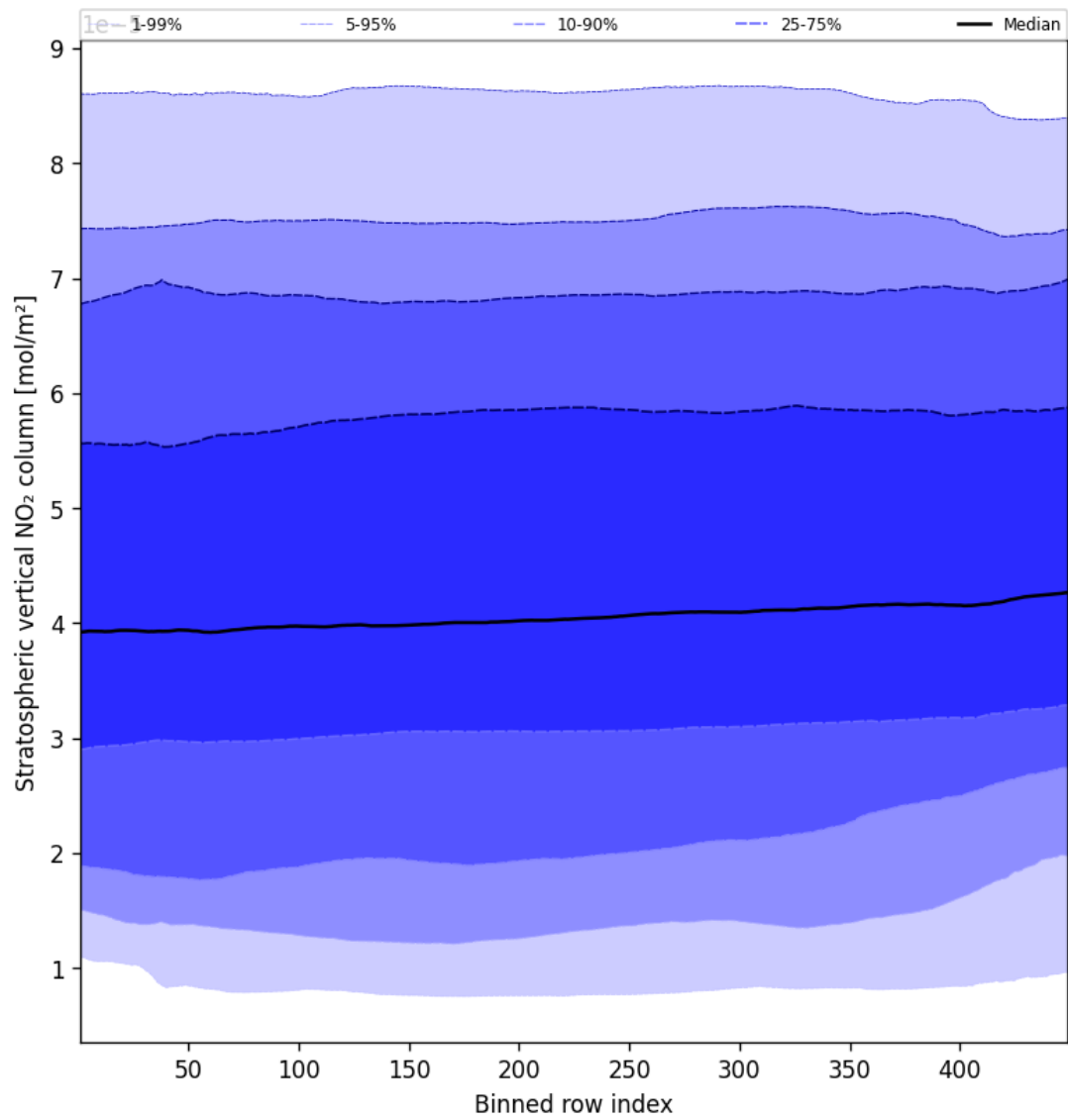
Figure 51: Along track statistics of “Stratospheric vertical NO 2 column” for 2025-02-14 to 2025-02-15
