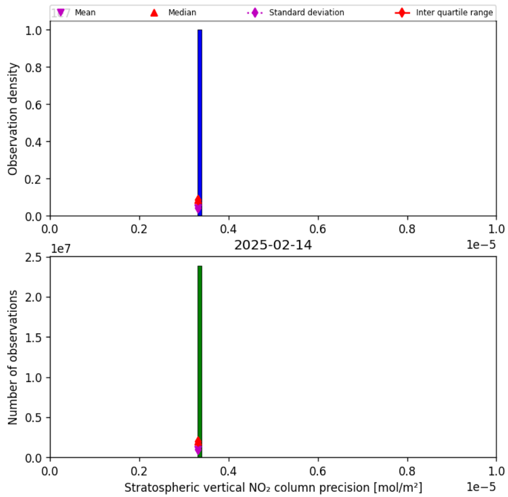
Figure 35: Histogram of “Stratospheric vertical NO 2 column precision” for 2025-02-14 to 2025-02-15
