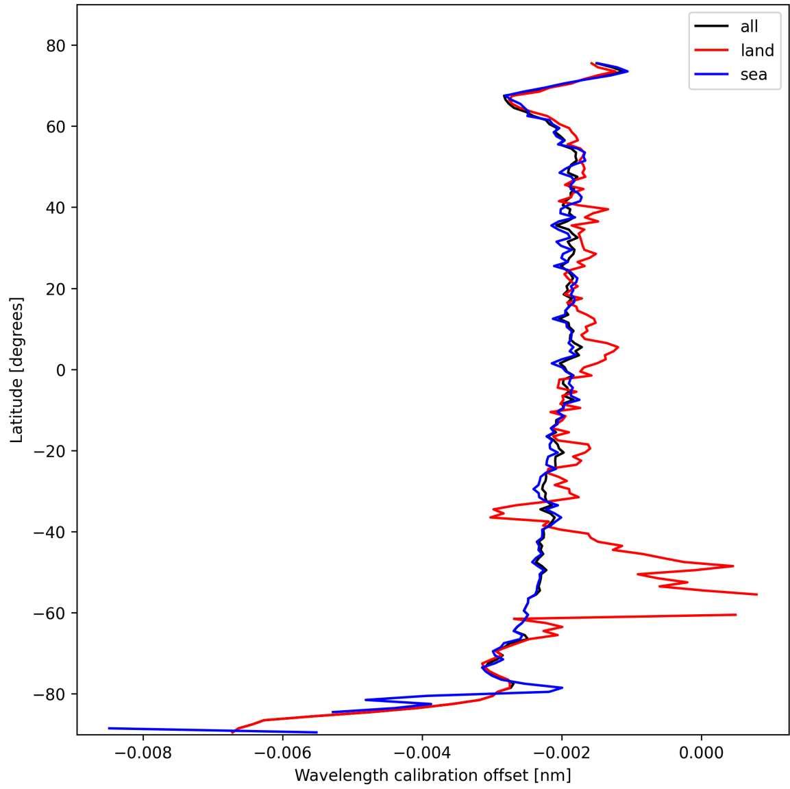
Figure 16: Zonal average of “Wavelength calibration offset” for 2025-02-14 to 2025-02-15.
