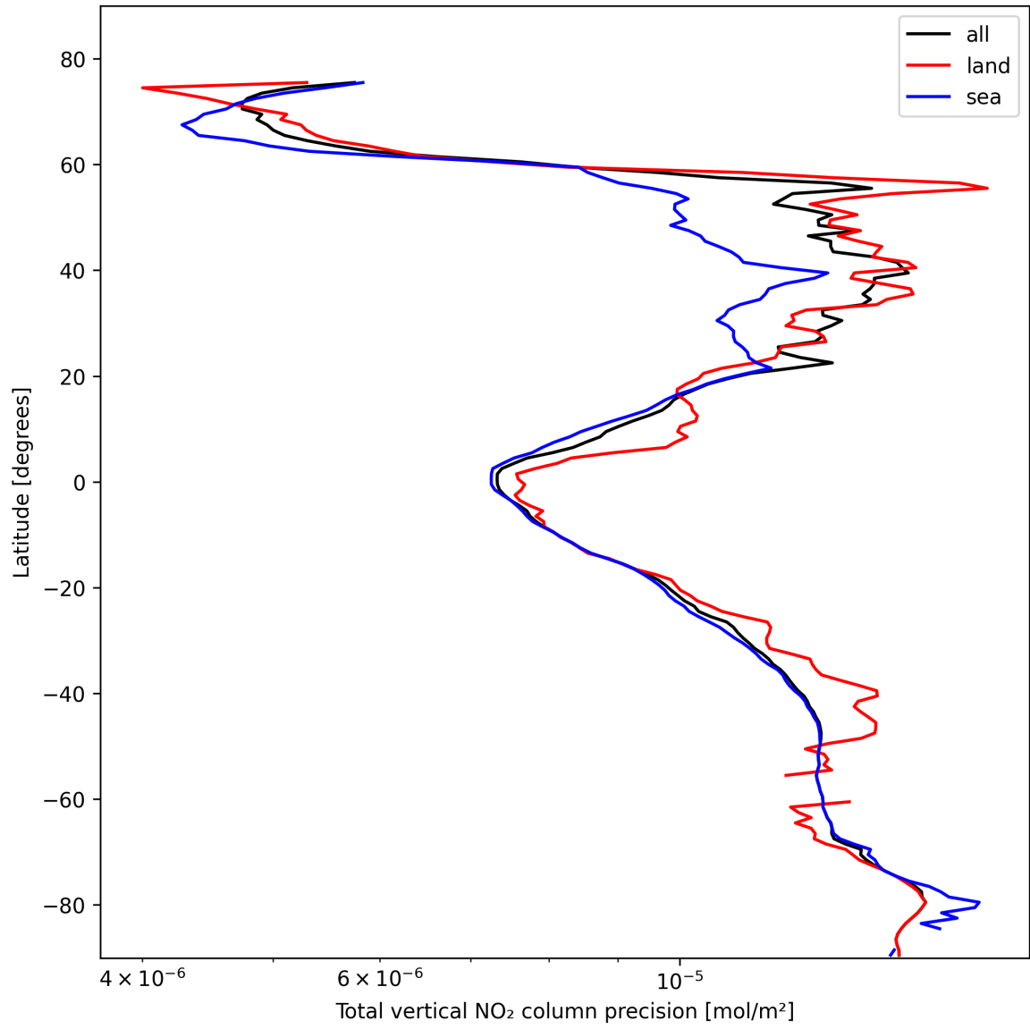
Figure 20: Zonal average of “Total vertical NO 2 column precision” for 2025-02-14 to 2025-02-15.
