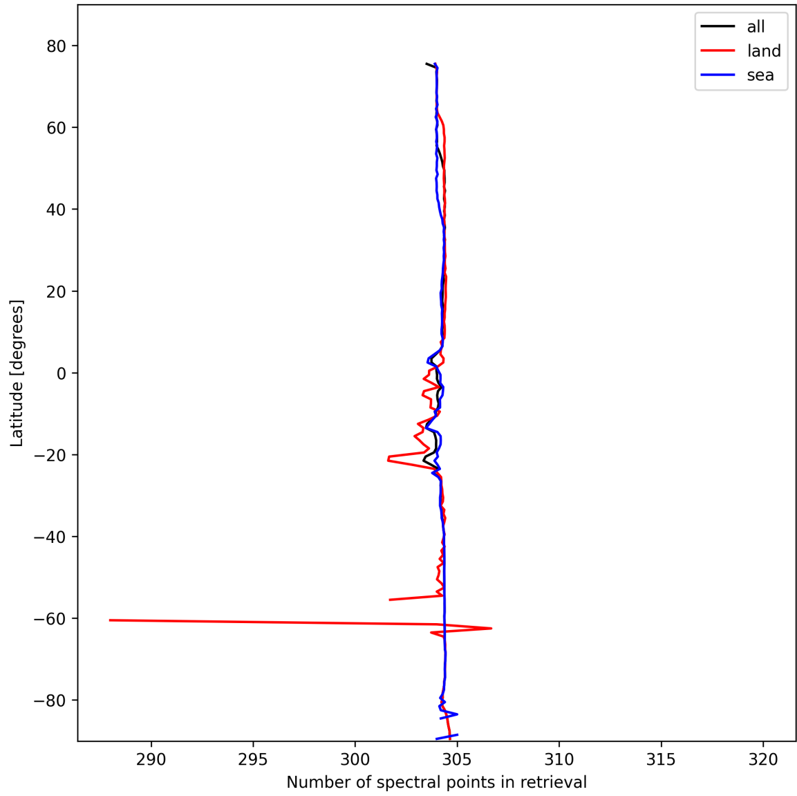
Figure 14: Zonal average of “Number of spectral points in retrieval” for 2025-02-14 to 2025-02-15.
