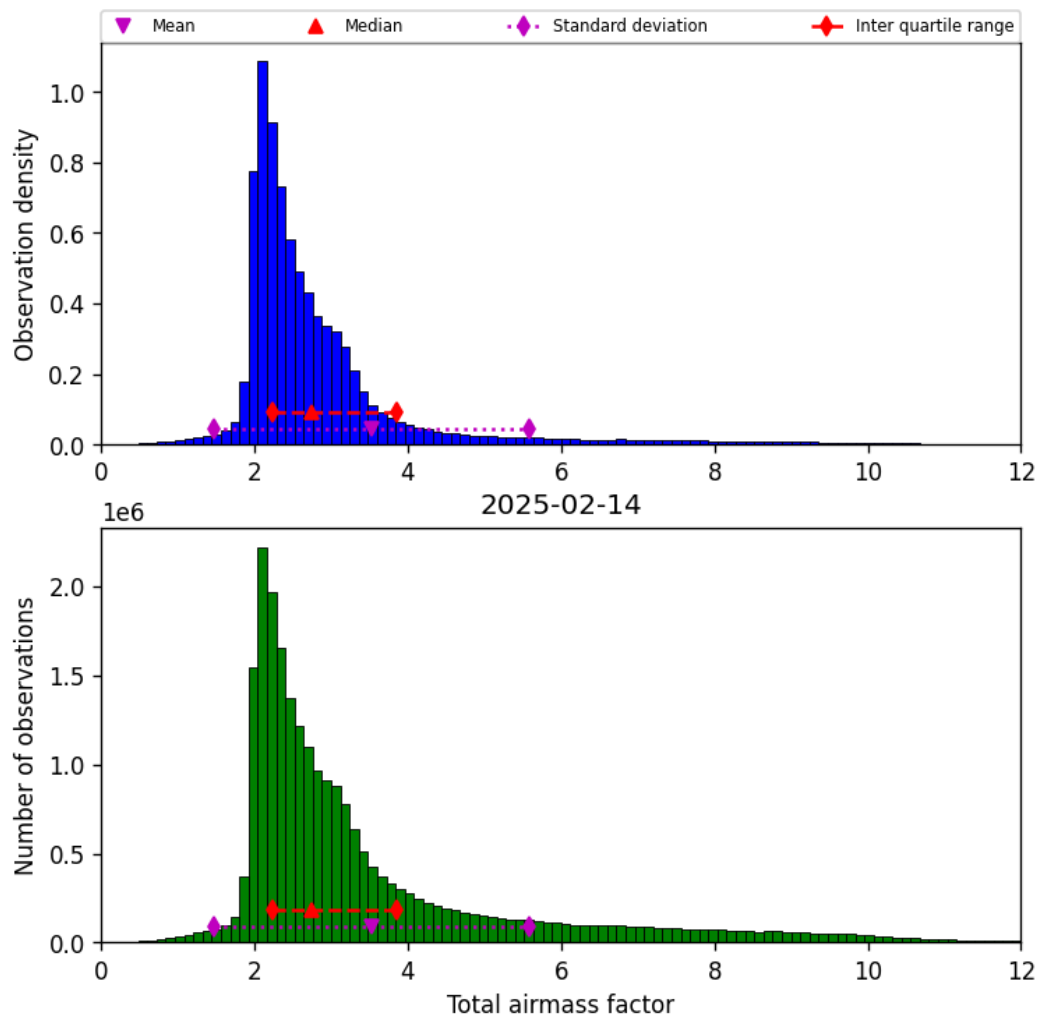
Figure 30: Histogram of “Total airmass factor” for 2025-02-14 to 2025-02-15
