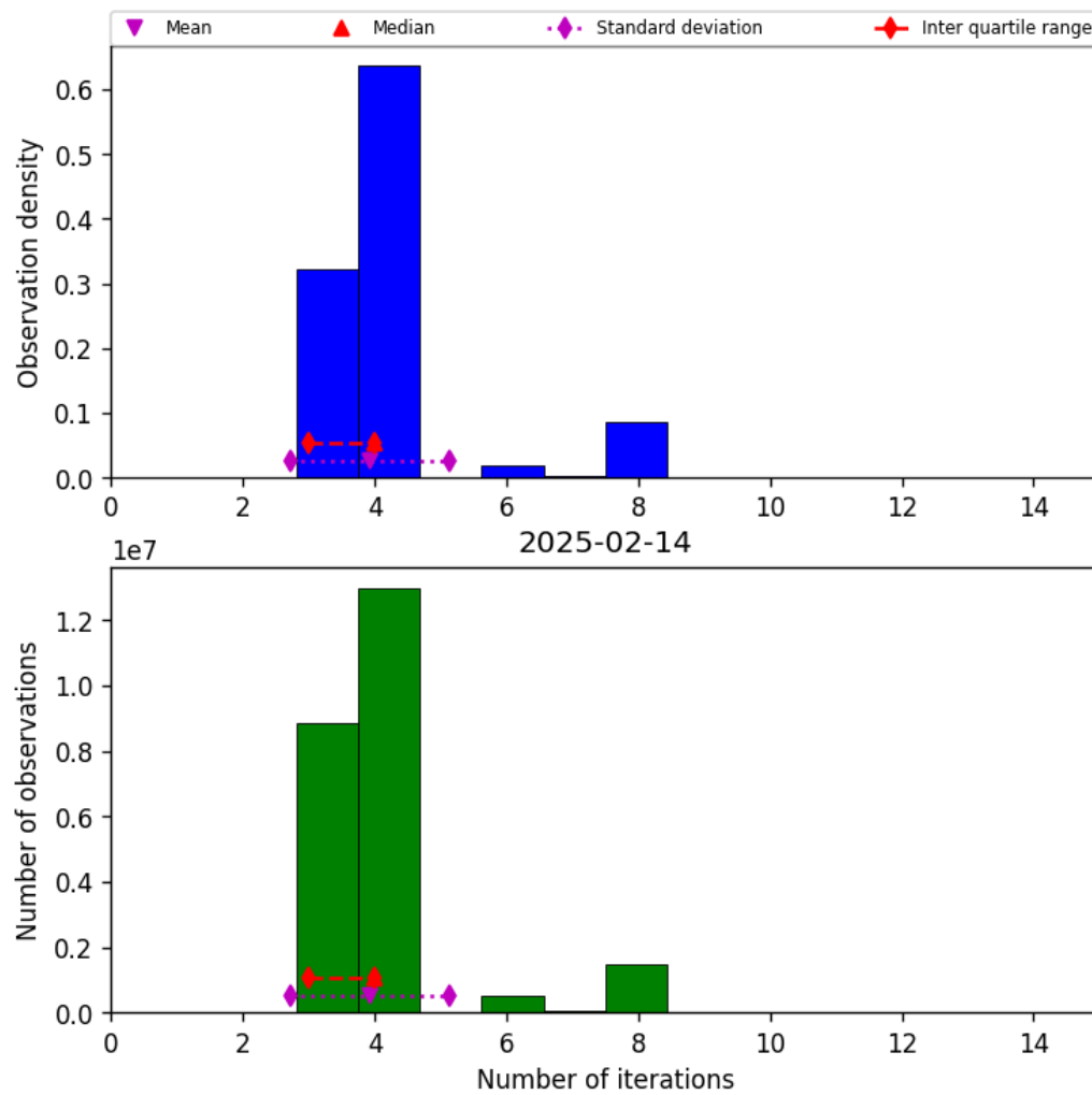
Figure 32: Histogram of “Number of iterations” for 2025-02-14 to 2025-02-15
