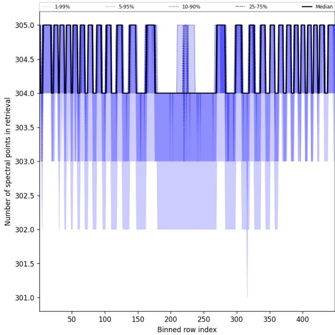
Figure 48: Along track statistics of “Number of spectral points in retrieval” for 2025-02-14 to 2025-02-15
