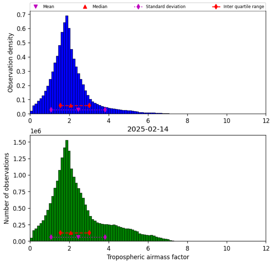
Figure 29: Histogram of “Tropospheric airmass factor” for 2025-02-14 to 2025-02-15
