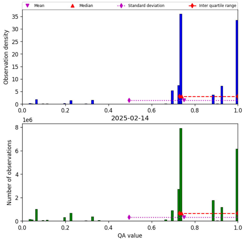
Figure 26: Histogram of “QA value” for 2025-02-14 to 2025-02-15
