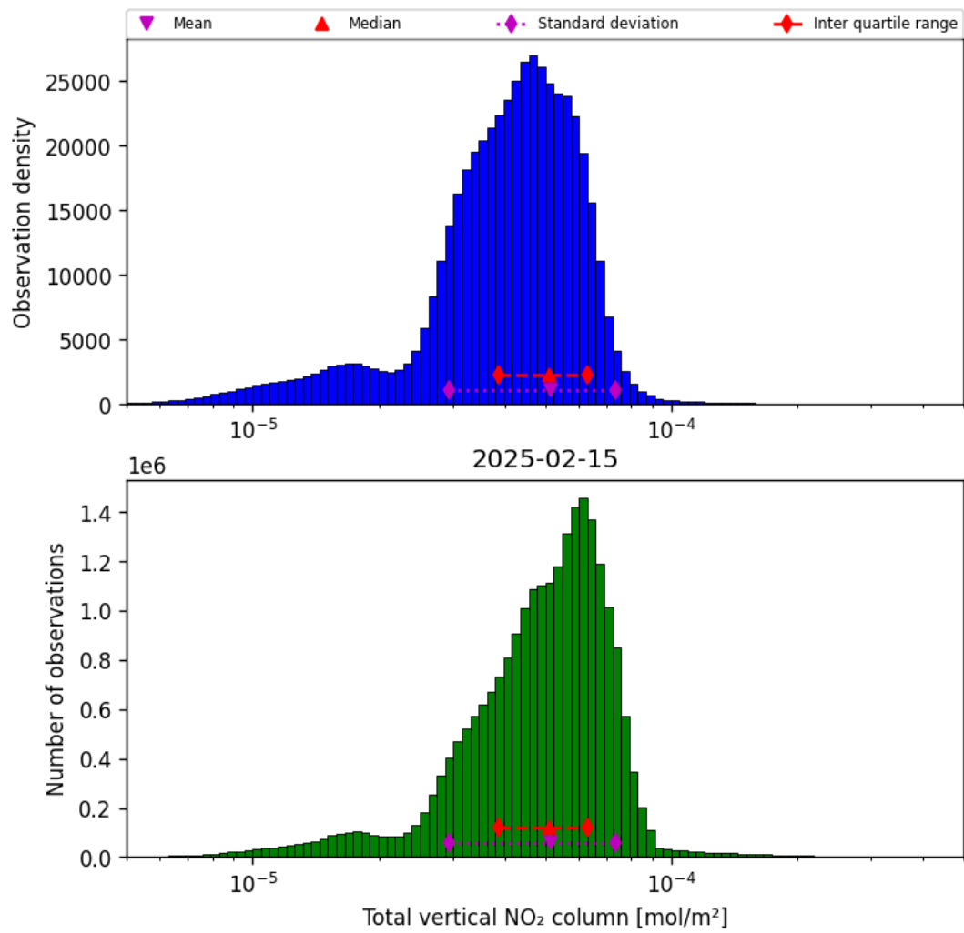
Figure 36: Histogram of “Total vertical NO 2 column” for 2025-02-15 to 2025-02-16
