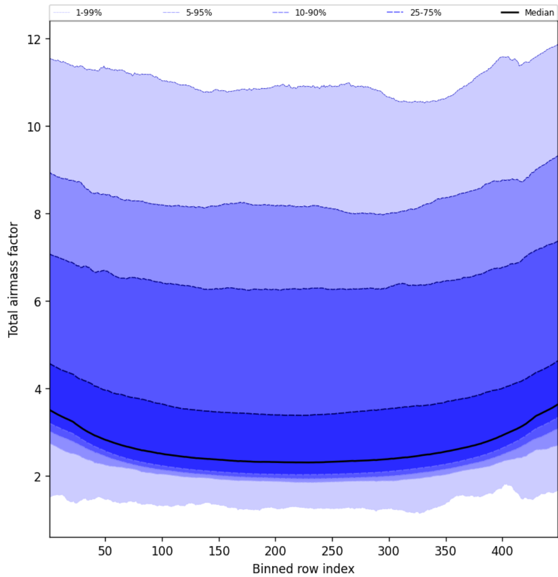
Figure 47: Along track statistics of “Total airmass factor” for 2025-02-15 to 2025-02-16
