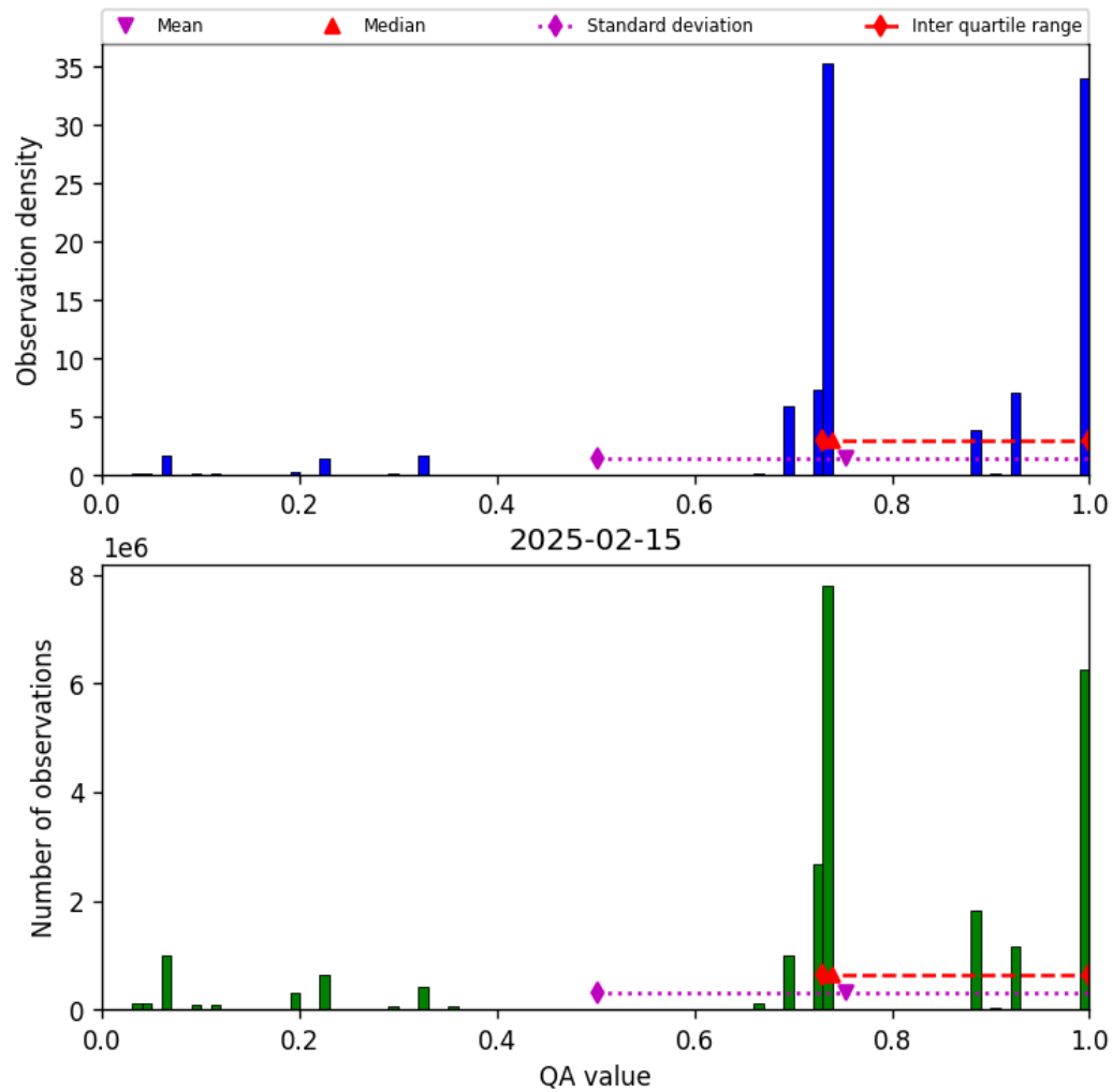
Figure 26: Histogram of “QA value” for 2025-02-15 to 2025-02-16
