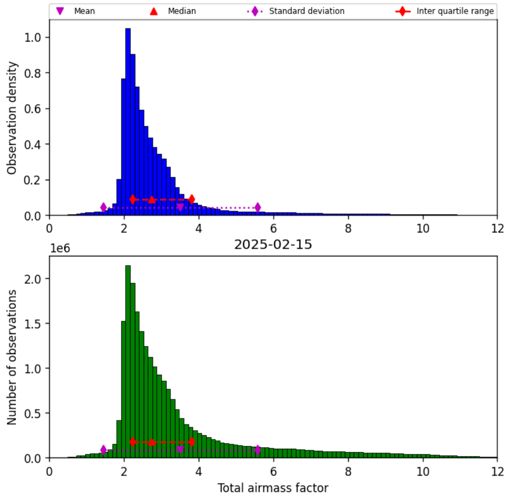
Figure 30: Histogram of “Total airmass factor” for 2025-02-15 to 2025-02-16
