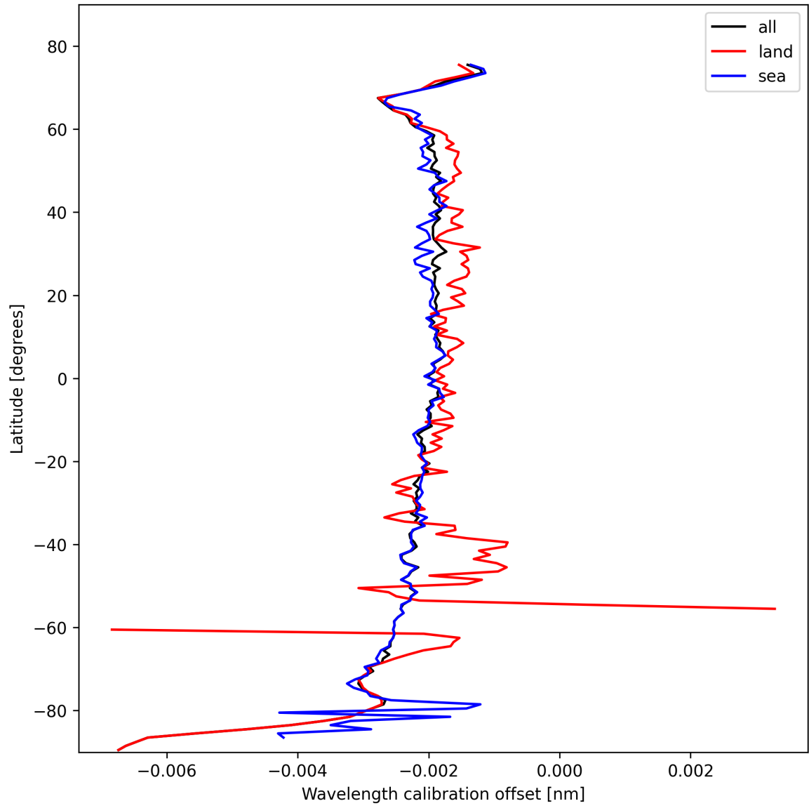
Figure 16: Zonal average of “Wavelength calibration offset” for 2025-02-15 to 2025-02-16.
