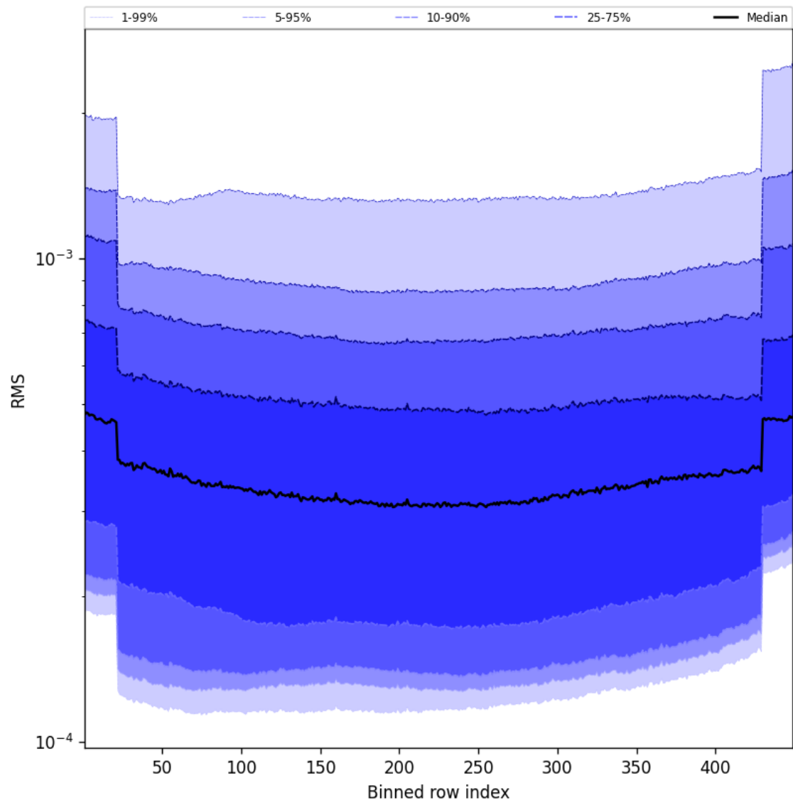
Figure 58: Along track statistics of “RMS” for 2025-02-15 to 2025-02-16
