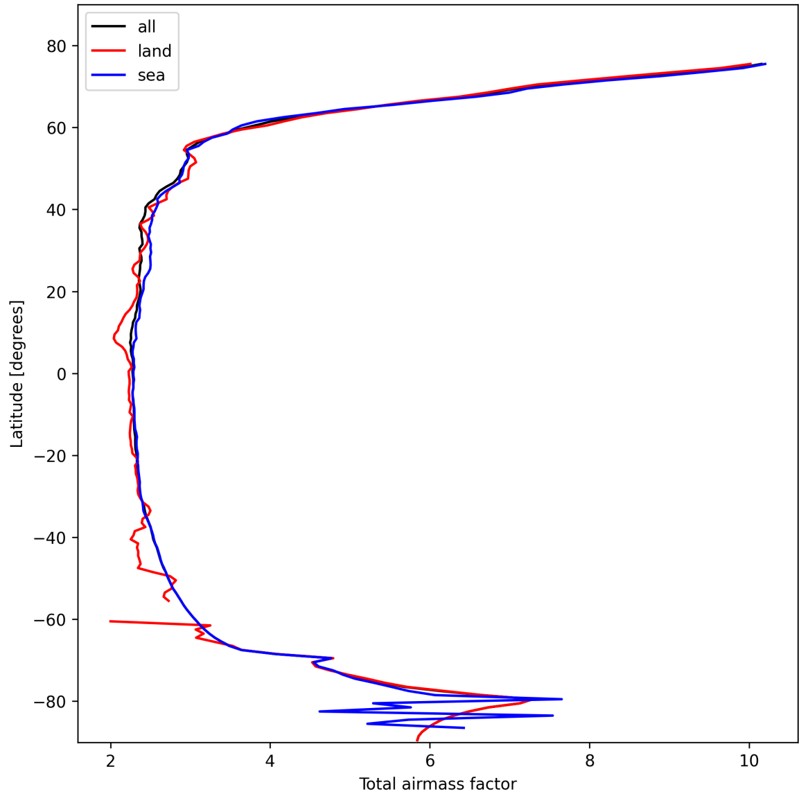
Figure 13: Zonal average of “Total airmass factor” for 2025-02-15 to 2025-02-16.
