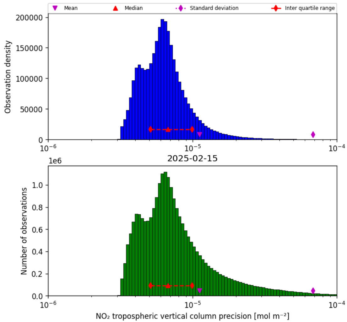
Figure 28: Histogram of “NO 2 tropospheric vertical column precision” for 2025-02-15 to 2025-02-16
