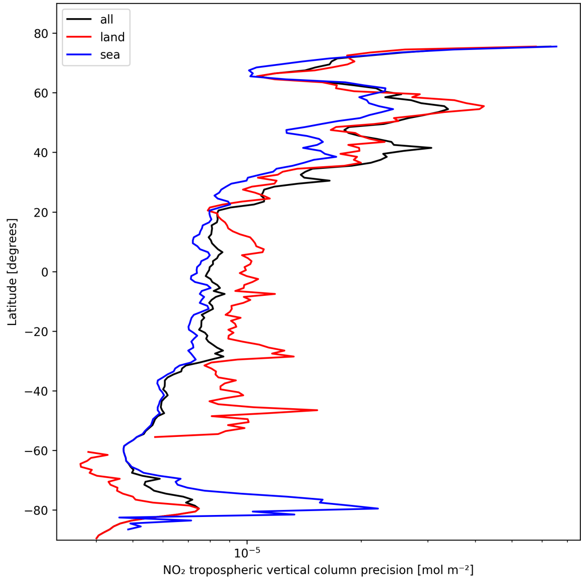
Figure 11: Zonal average of “NO 2 tropospheric vertical column precision” for 2025-02-15 to 2025-02-16.
