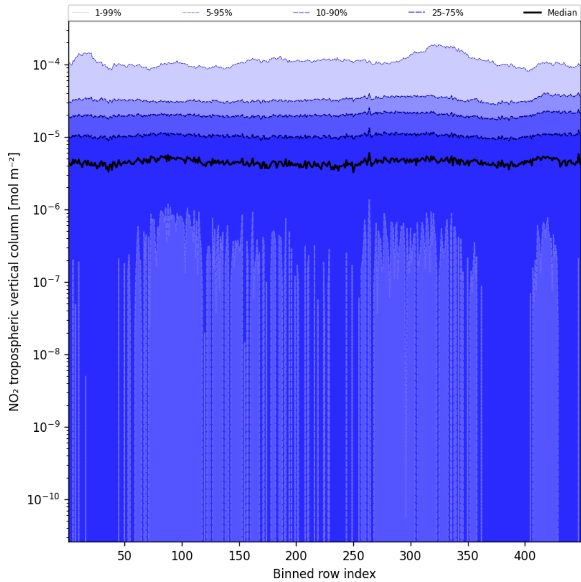
Figure 44: Along track statistics of “NO 2 tropospheric vertical column” for 2025-02-15 to 2025-02-16
