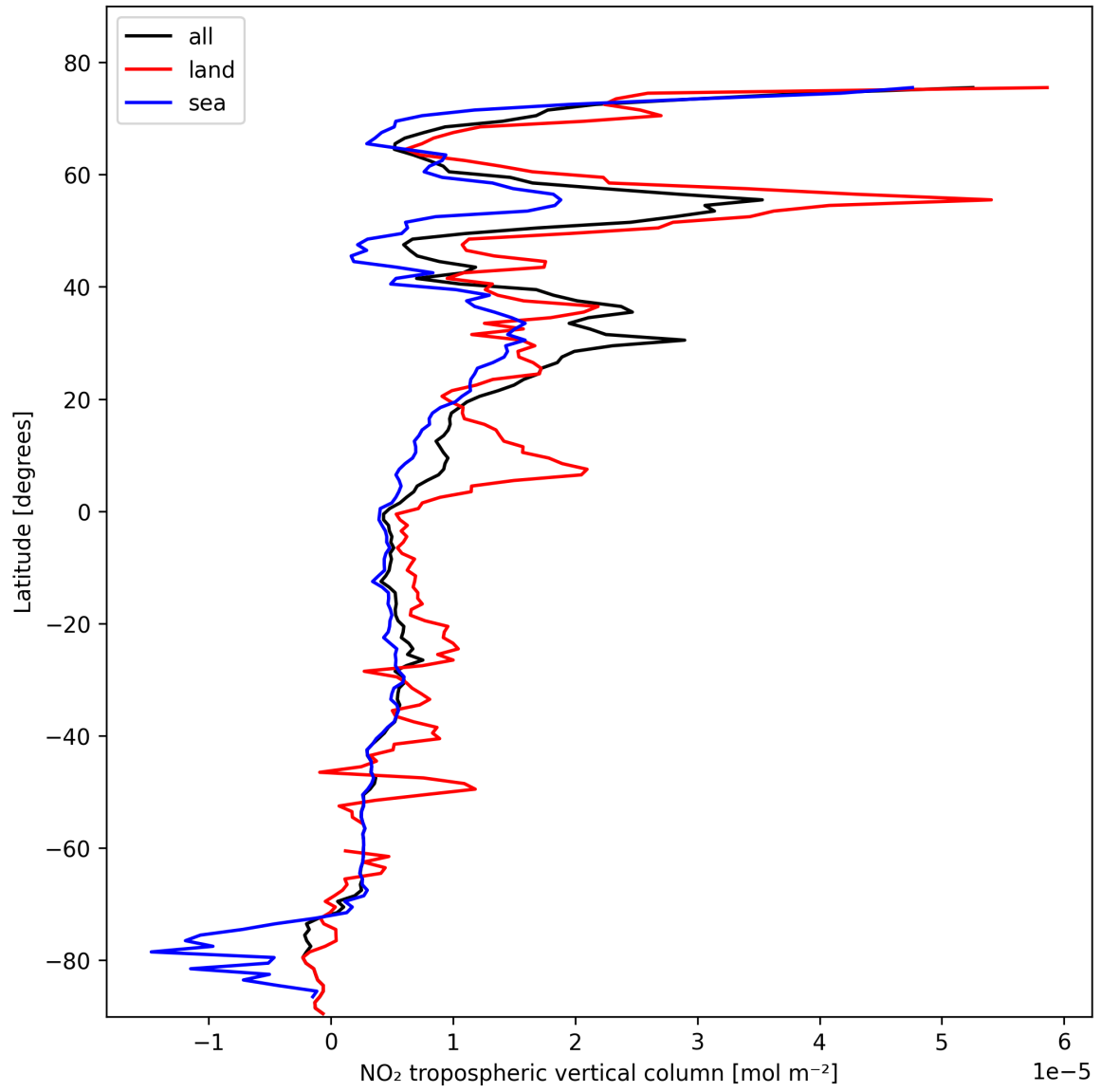
Figure 10: Zonal average of “NO 2 tropospheric vertical column” for 2025-02-15 to 2025-02-16.
