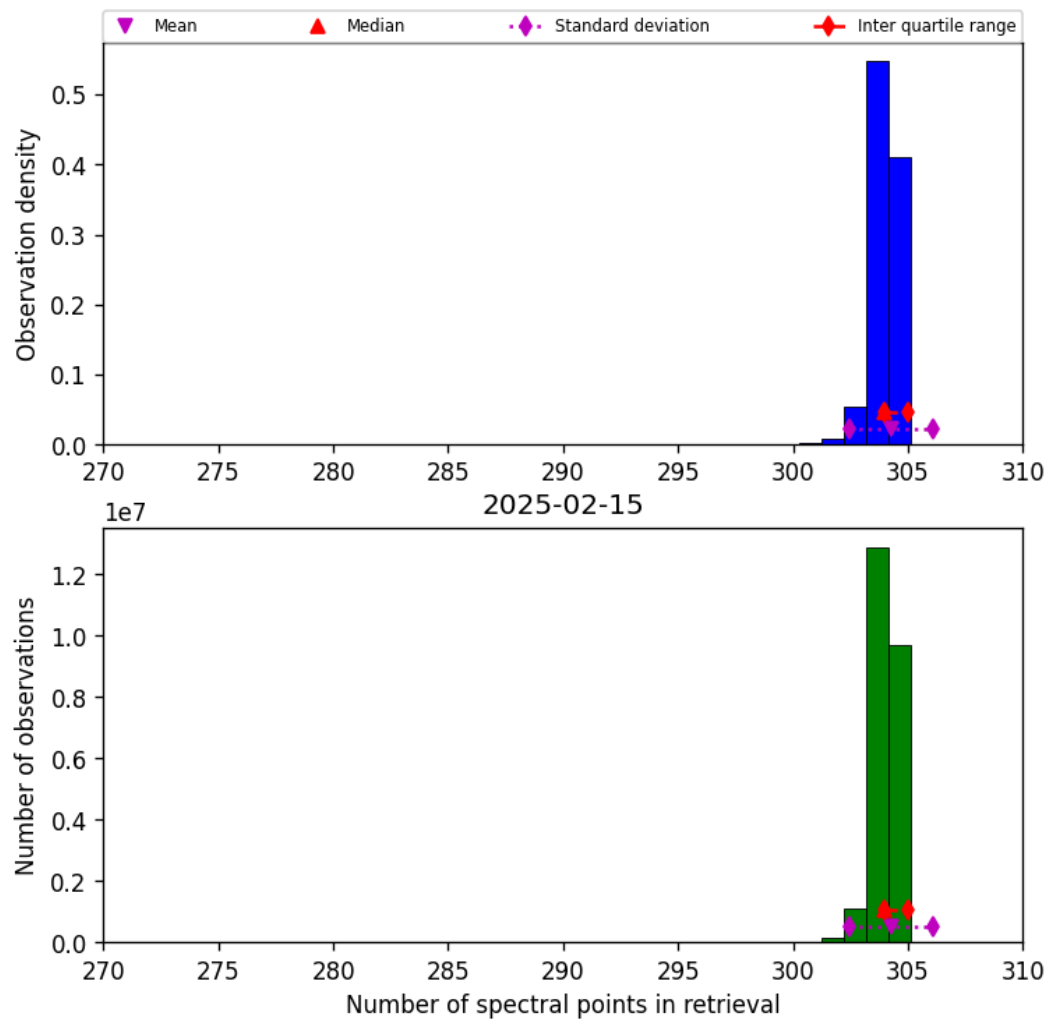
Figure 31: Histogram of “Number of spectral points in retrieval” for 2025-02-15 to 2025-02-16
