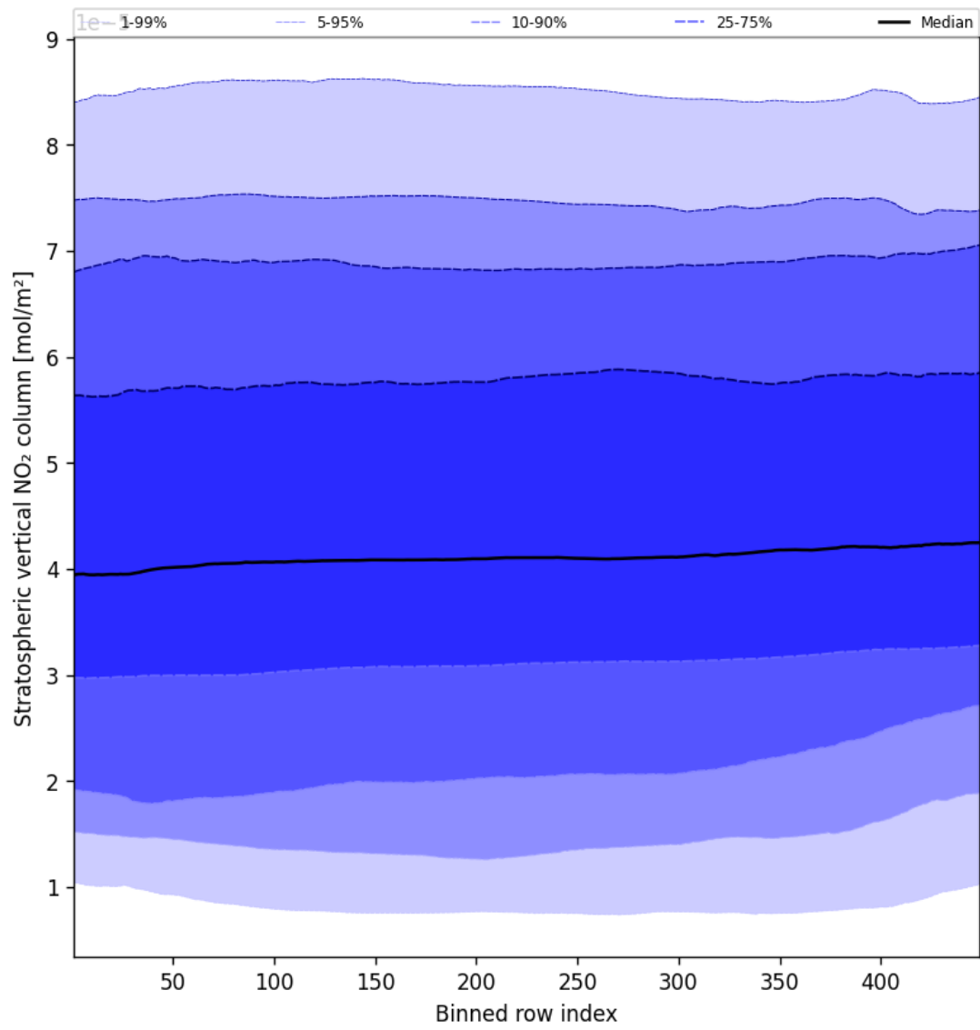
Figure 51: Along track statistics of “Stratospheric vertical NO 2 column” for 2025-02-15 to 2025-02-16
