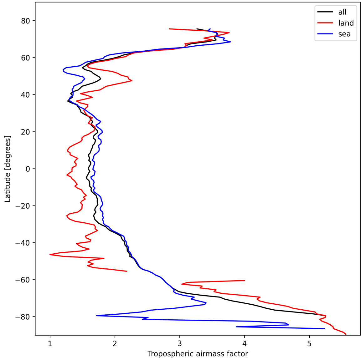
Figure 12: Zonal average of “Tropospheric airmass factor” for 2025-02-15 to 2025-02-16.
