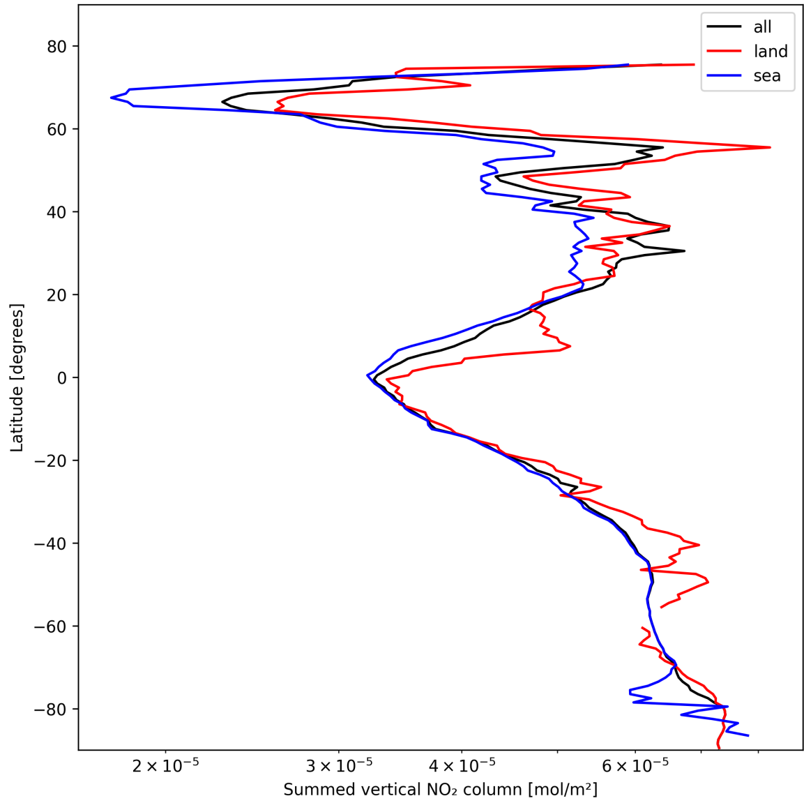
Figure 21: Zonal average of “Summed vertical NO 2 column” for 2025-02-15 to 2025-02-16.
