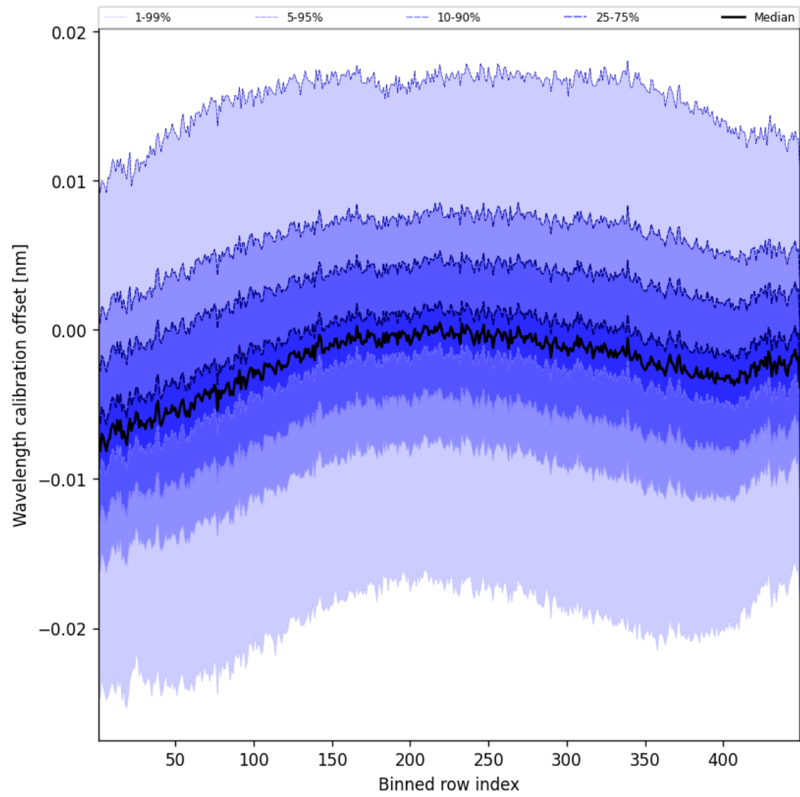
Figure 50: Along track statistics of “Wavelength calibration offset” for 2025-02-15 to 2025-02-16
