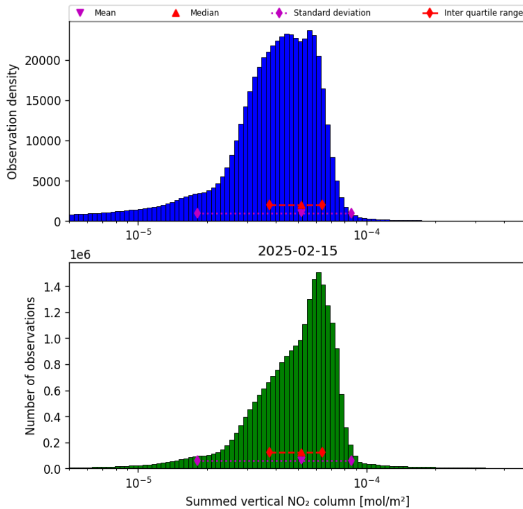
Figure 38: Histogram of “Summed vertical NO 2 column” for 2025-02-15 to 2025-02-16
