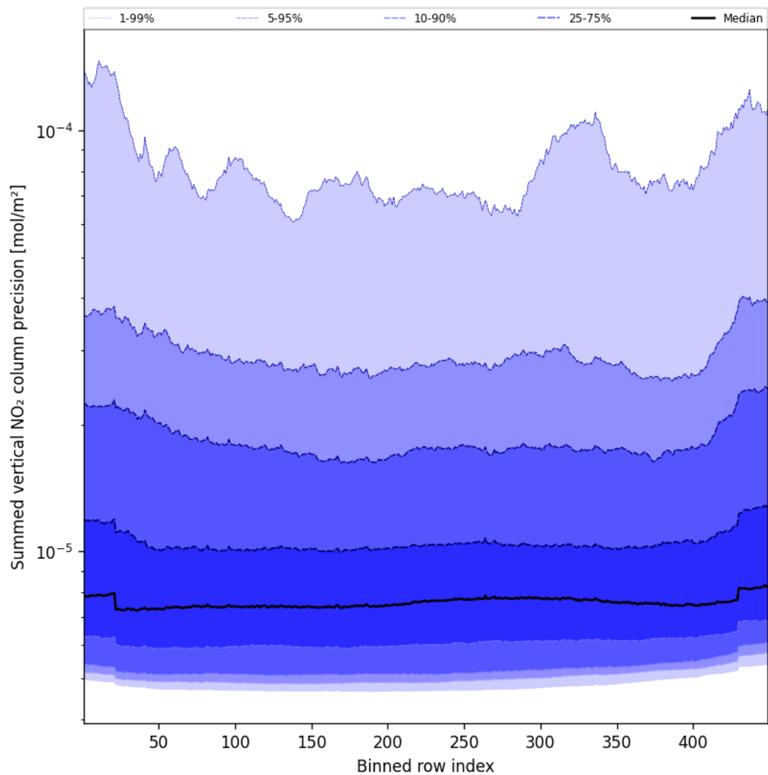
Figure 56: Along track statistics of “Summed vertical NO 2 column precision” for 2025-02-15 to 2025-02-16
