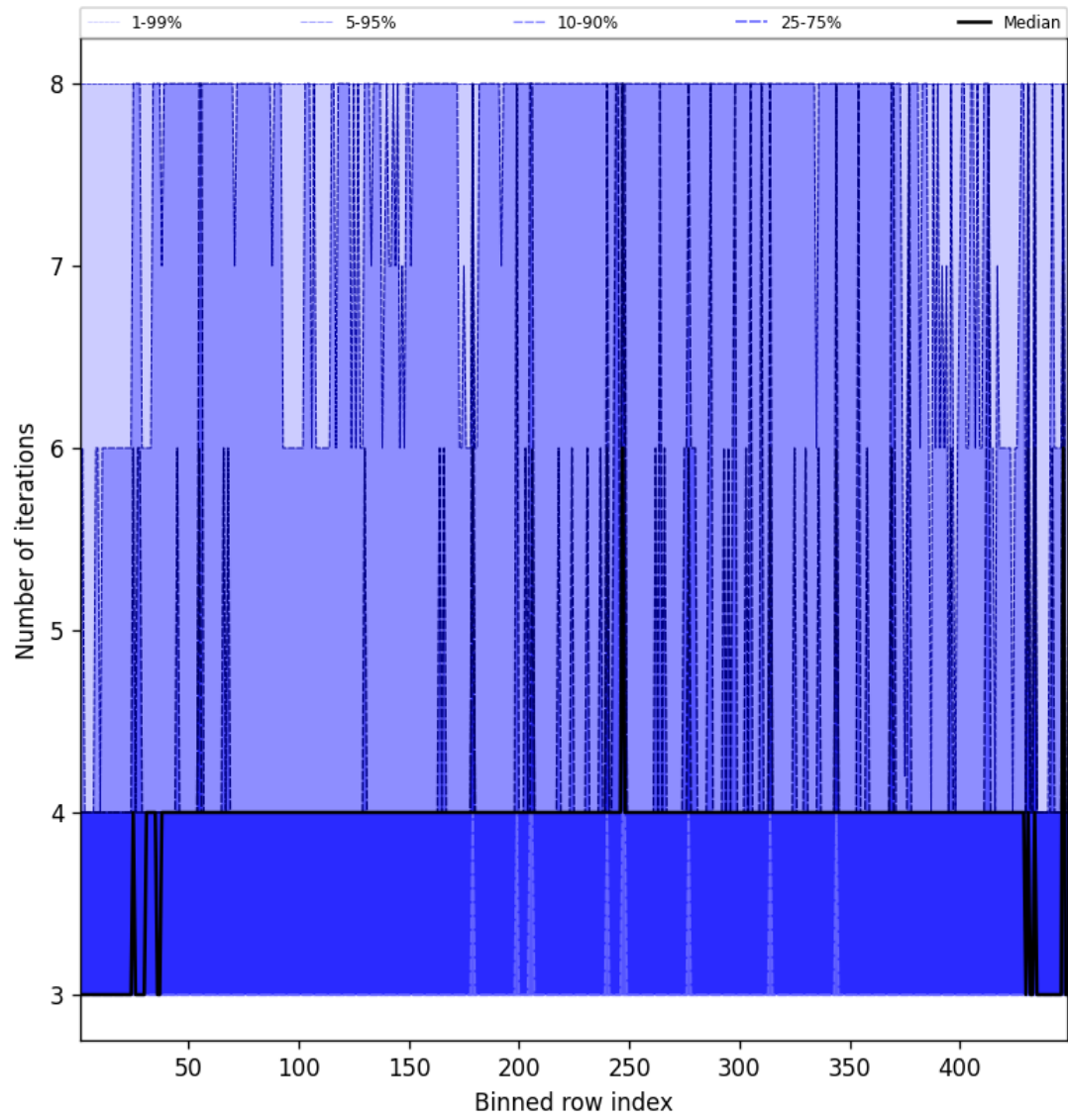
Figure 49: Along track statistics of “Number of iterations” for 2025-02-15 to 2025-02-16
