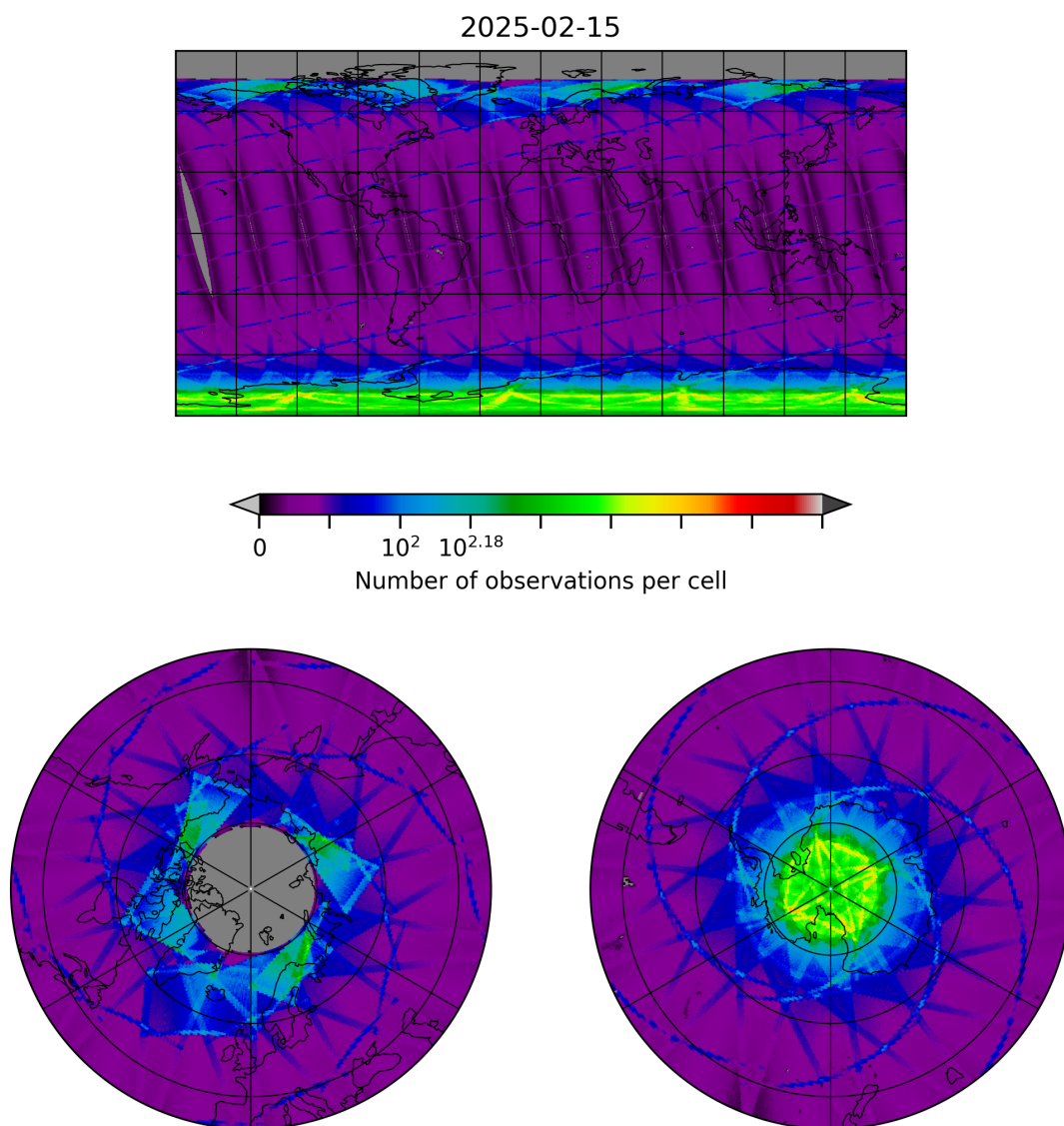
Figure 8: Map of the number of observations for 2025-02-15 to 2025-02-16
