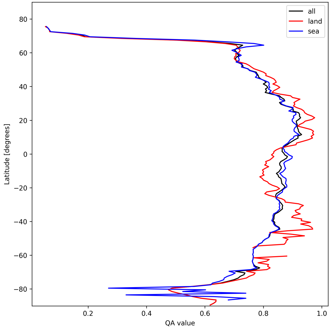
Figure 9: Zonal average of “QA value” for 2025-02-15 to 2025-02-16.
