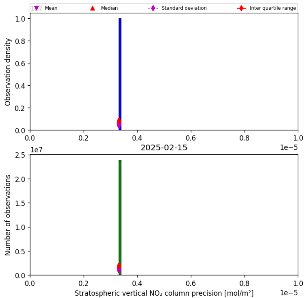
Figure 35: Histogram of “Stratospheric vertical NO 2 column precision” for 2025-02-15 to 2025-02-16
