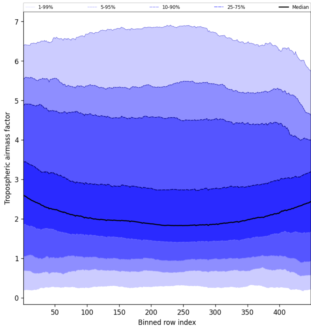
Figure 46: Along track statistics of "Tropospheric airmass factor" for 2025-02-15 to 2025-02-16
