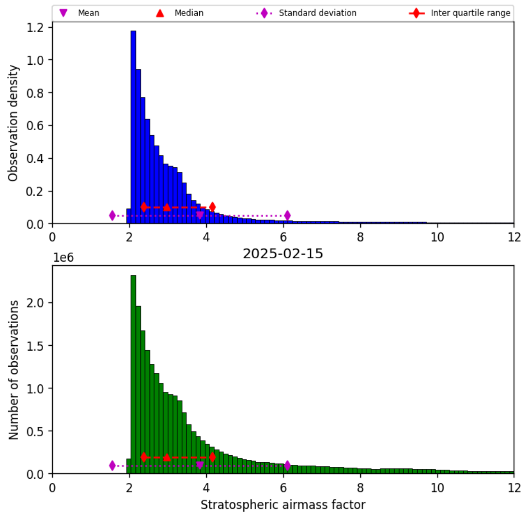
Figure 42: Histogram of “Stratospheric airmass factor” for 2025-02-15 to 2025-02-16
