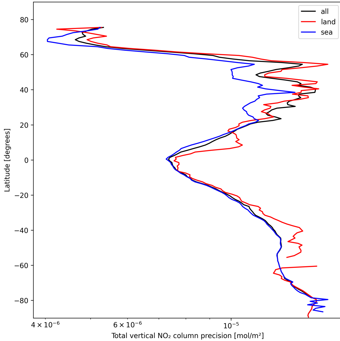
Figure 20: Zonal average of “Total vertical NO 2 column precision” for 2025-02-15 to 2025-02-16.
