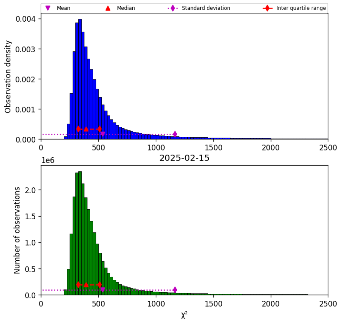
Figure 40: Histogram of “ \chi^2 ” for 2025-02-15 to 2025-02-16
