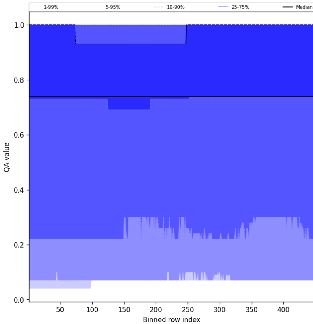
Figure 43: Along track statistics of "QA value" for 2025-02-15 to 2025-02-16
