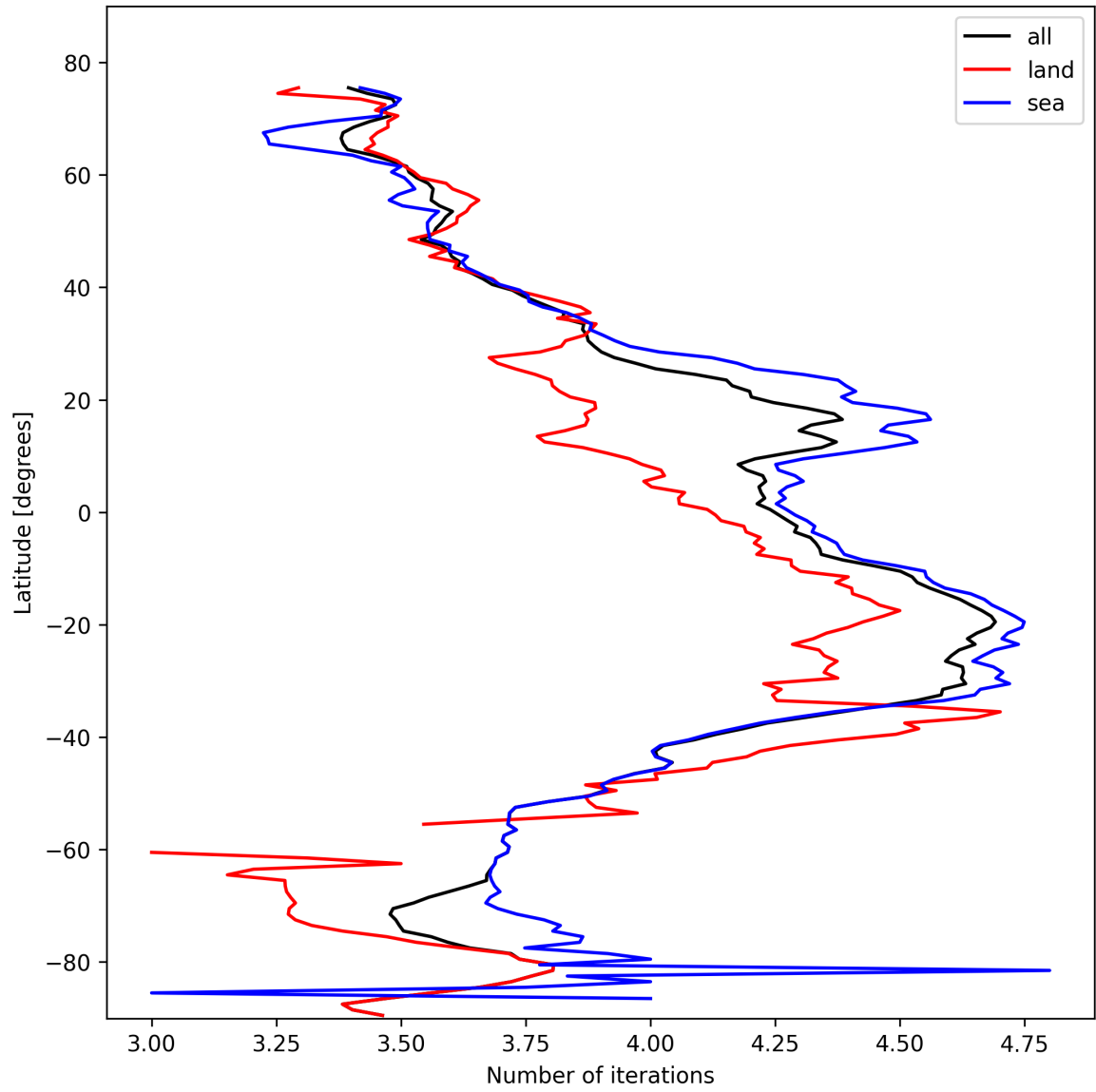
Figure 15: Zonal average of “Number of iterations” for 2025-02-15 to 2025-02-16.
