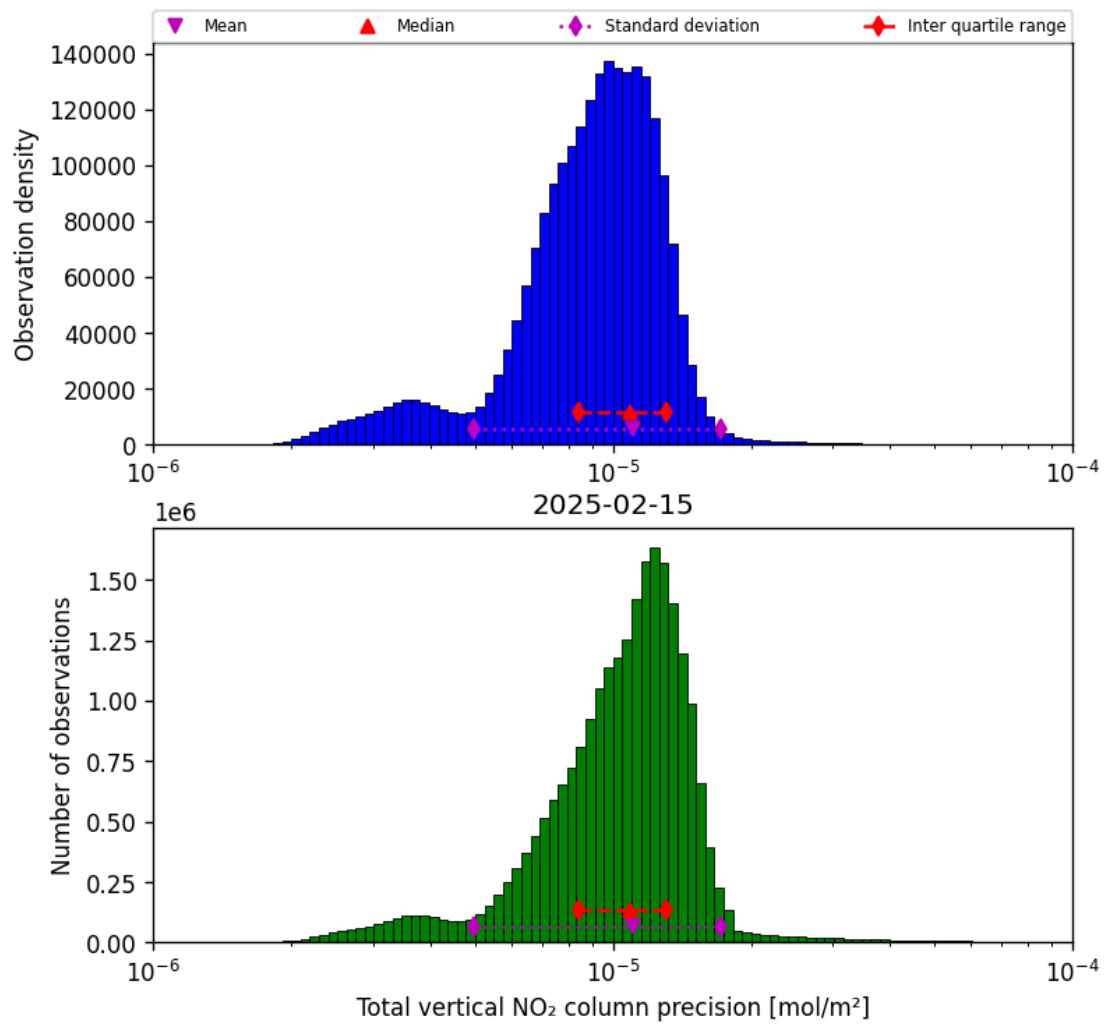
Figure 37: Histogram of “Total vertical NO 2 column precision” for 2025-02-15 to 2025-02-16
