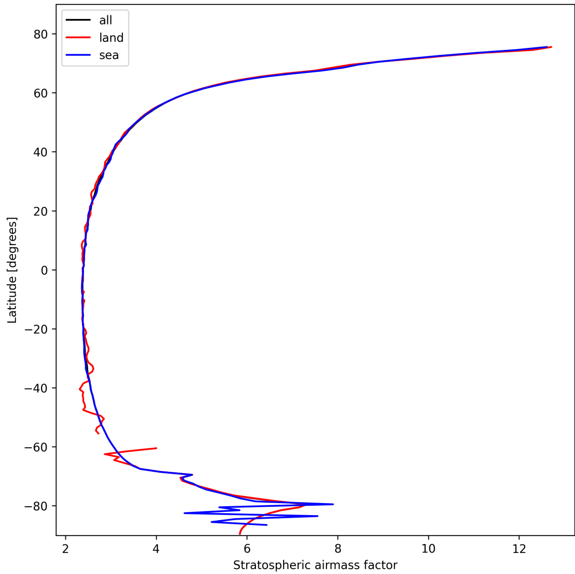
Figure 25: Zonal average of “Stratospheric airmass factor” for 2025-02-15 to 2025-02-16.
