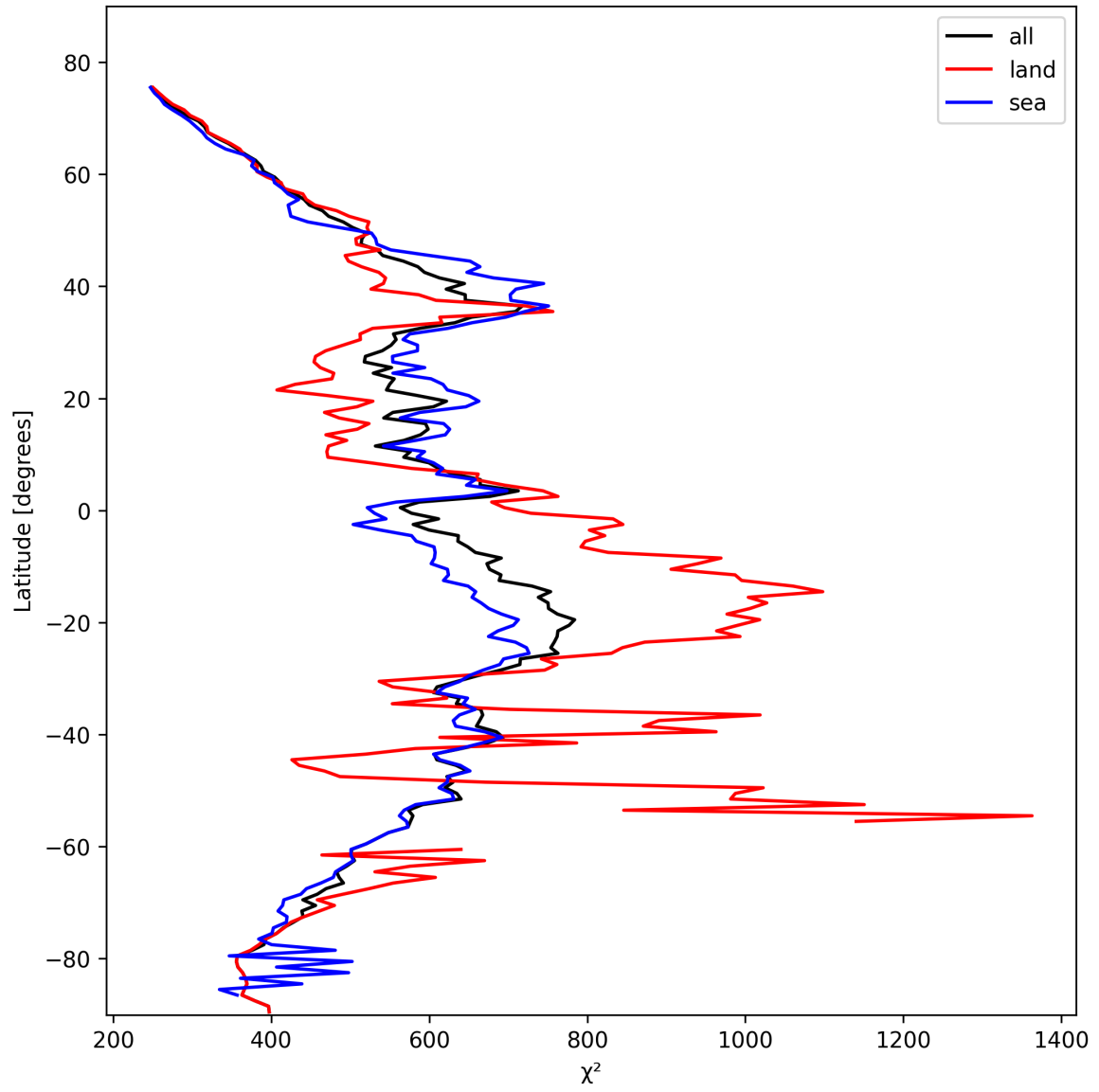
Figure 23: Zonal average of “ \chi^2 ” for 2025-02-15 to 2025-02-16.
