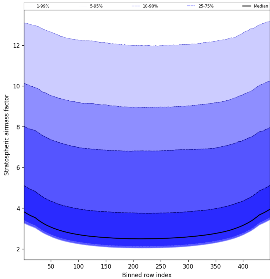
Figure 59: Along track statistics of “Stratospheric airmass factor” for 2025-02-15 to 2025-02-16
