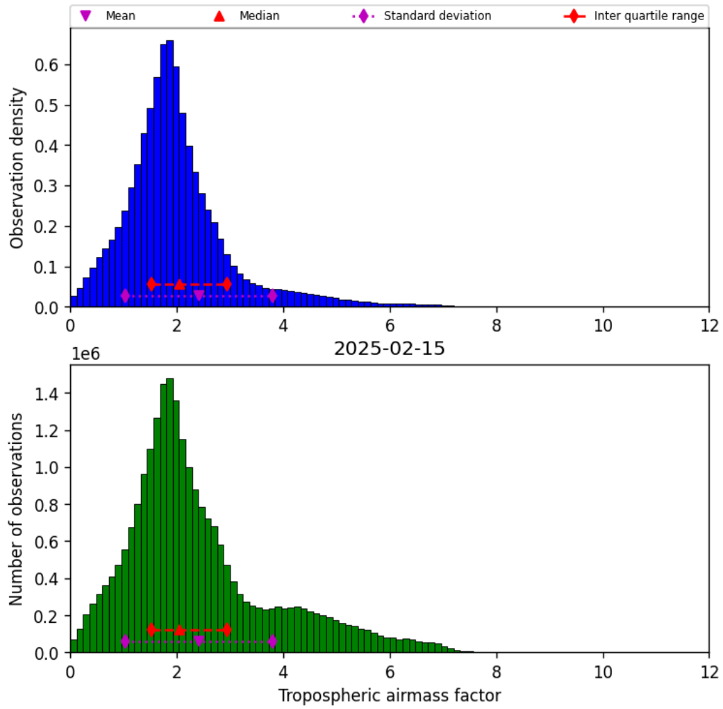
Figure 29: Histogram of “Tropospheric airmass factor” for 2025-02-15 to 2025-02-16
