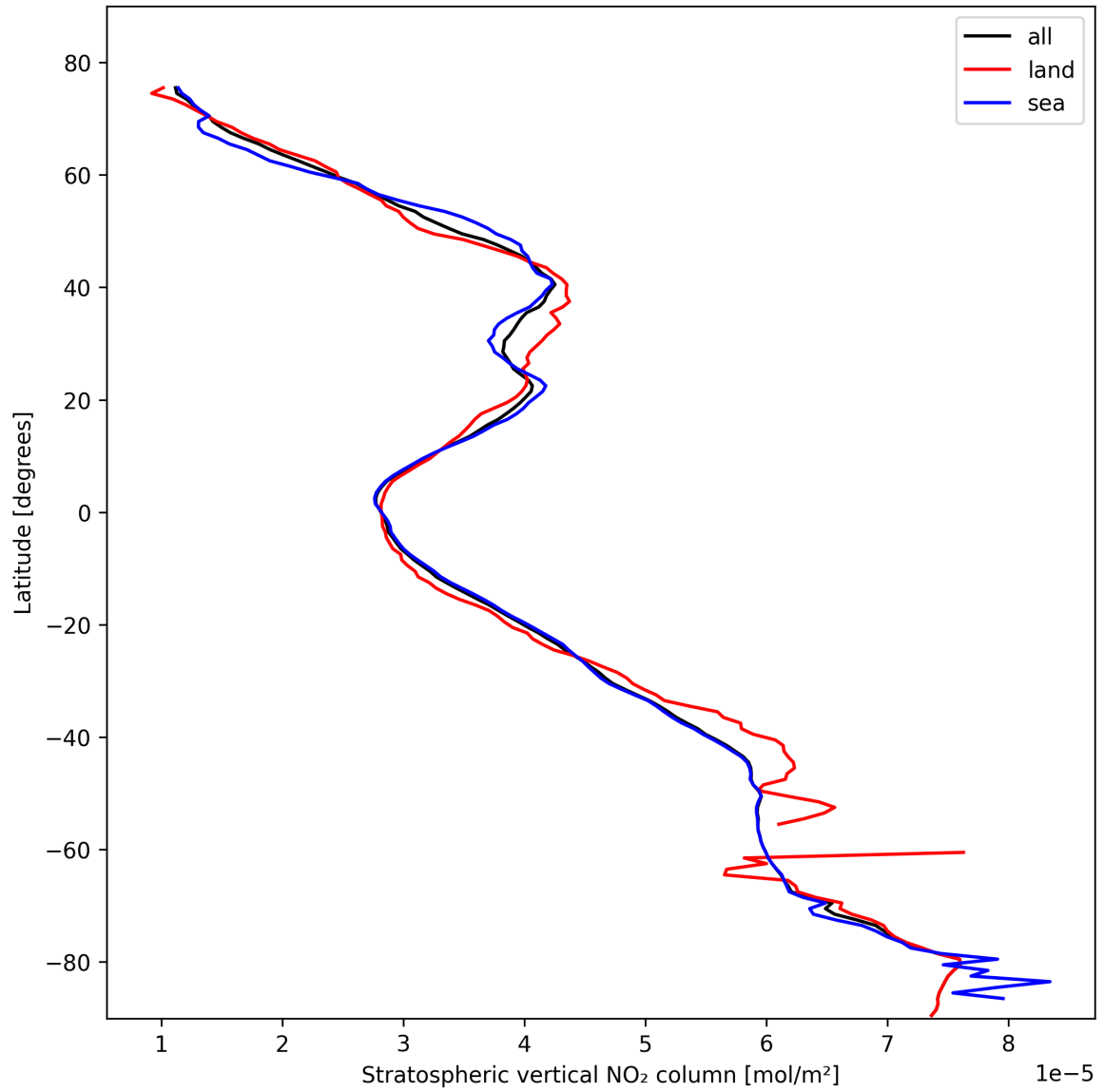
Figure 17: Zonal average of “Stratospheric vertical NO 2 column” for 2025-02-15 to 2025-02-16.
