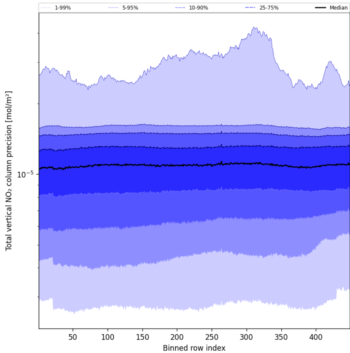
Figure 54: Along track statistics of “Total vertical NO 2 column precision” for 2025-02-15 to 2025-02-16
