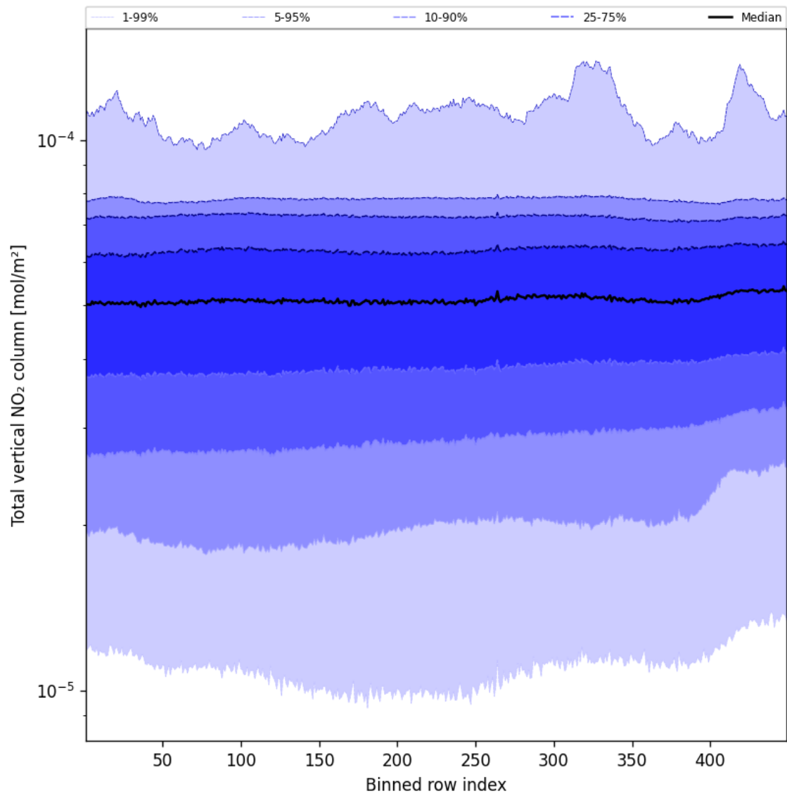
Figure 53: Along track statistics of “Total vertical NO 2 column” for 2025-02-15 to 2025-02-16
