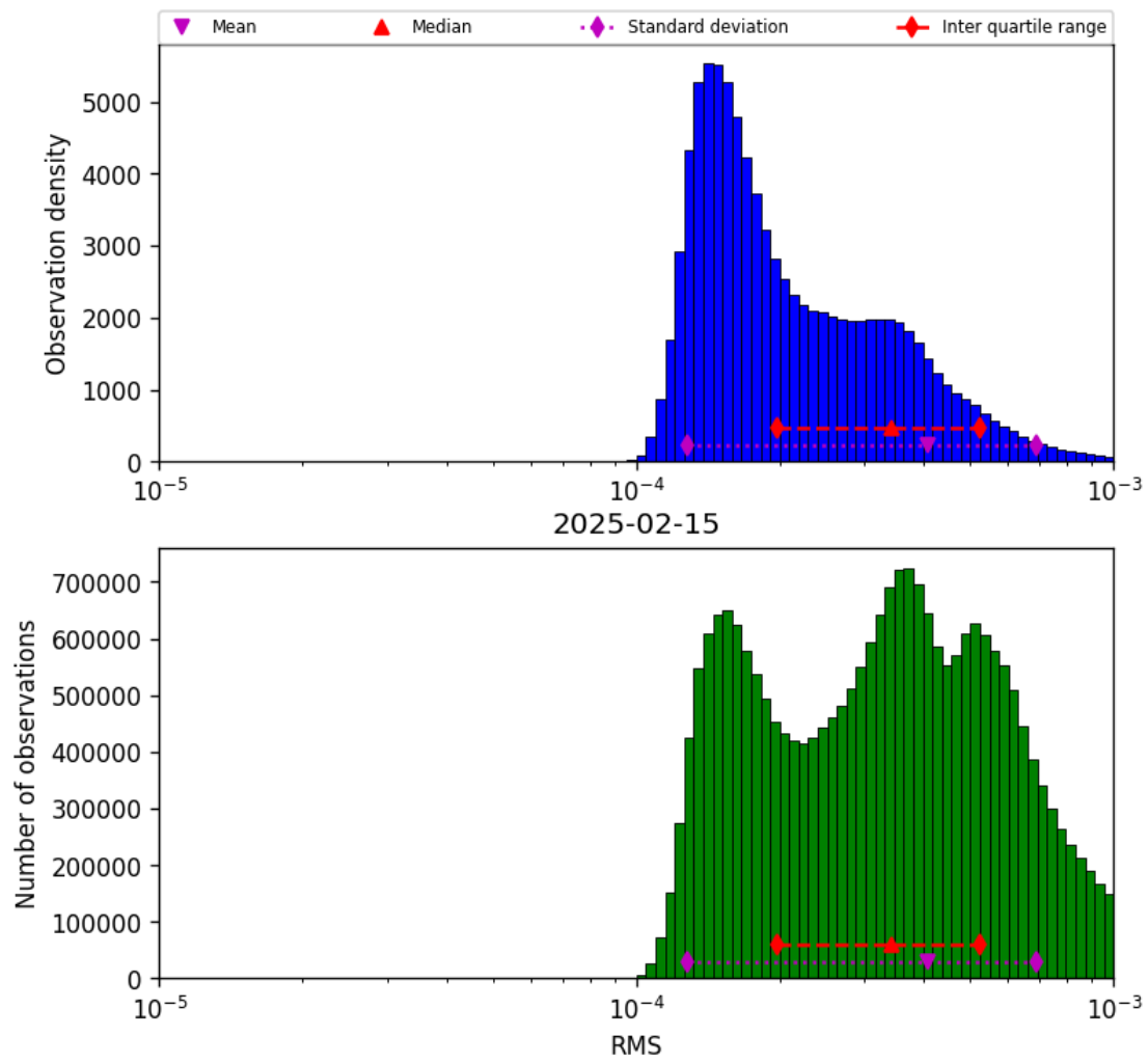
Figure 41: Histogram of “RMS” for 2025-02-15 to 2025-02-16
