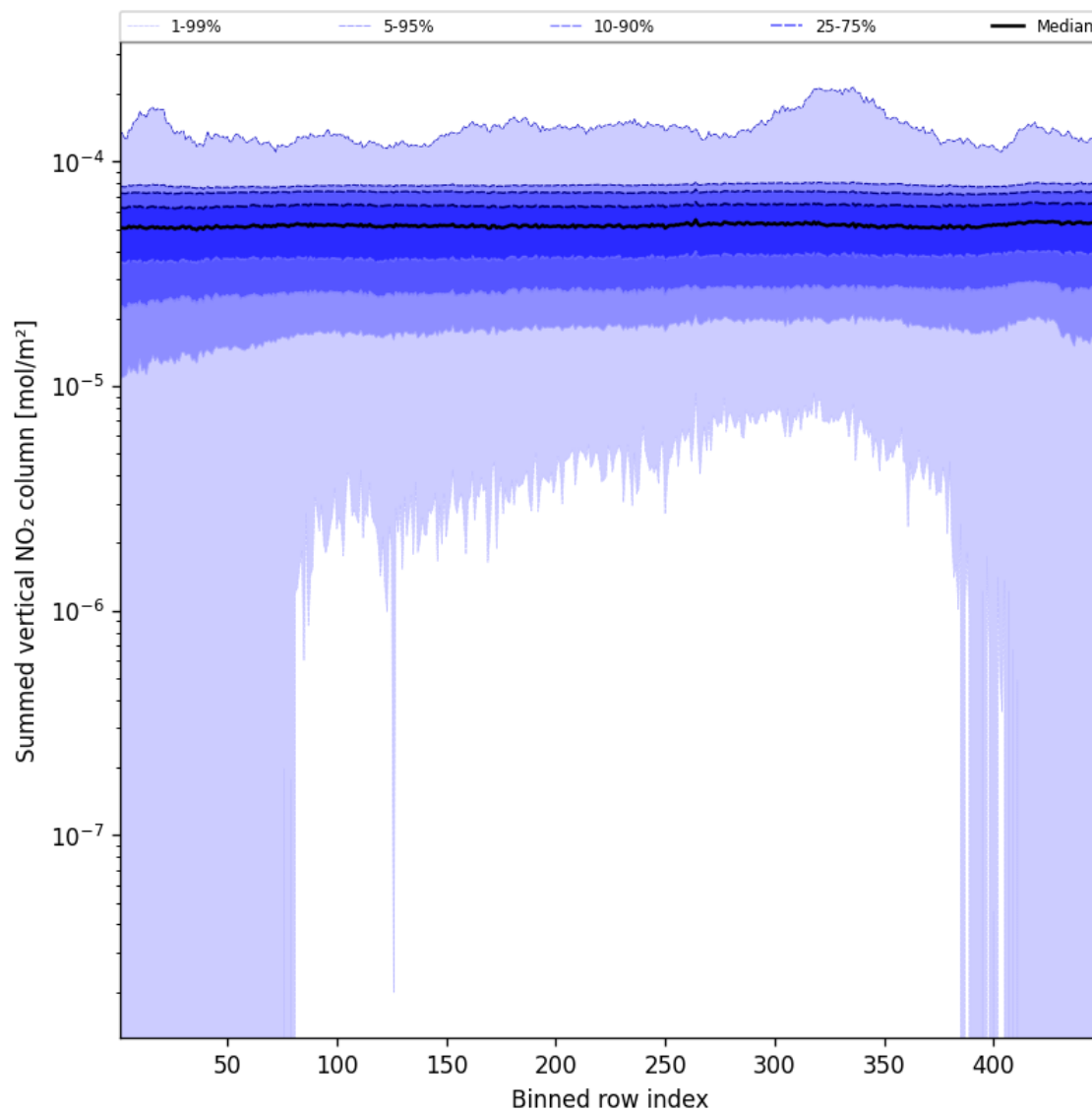
Figure 55: Along track statistics of “Summed vertical NO 2 column” for 2025-02-15 to 2025-02-16
