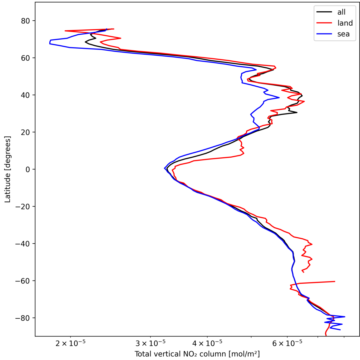
Figure 19: Zonal average of “Total vertical NO 2 column” for 2025-02-15 to 2025-02-16.
