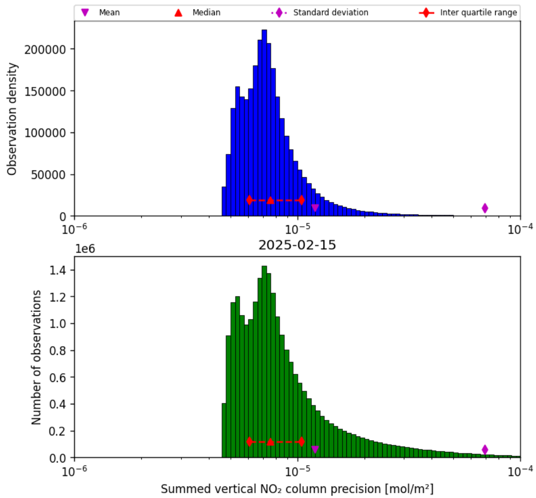
Figure 39: Histogram of "Summed vertical NO 2 column precision" for 2025-02-15 to 2025-02-16
