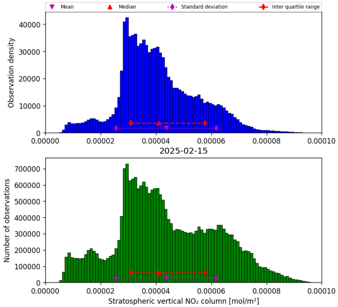
Figure 34: Histogram of “Stratospheric vertical NO 2 column” for 2025-02-15 to 2025-02-16
