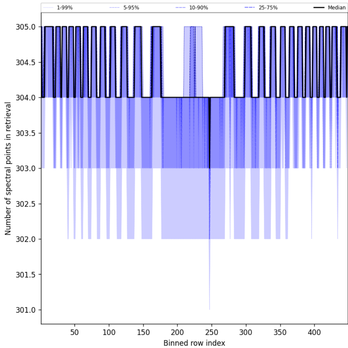
Figure 48: Along track statistics of “Number of spectral points in retrieval” for 2025-02-15 to 2025-02-16
