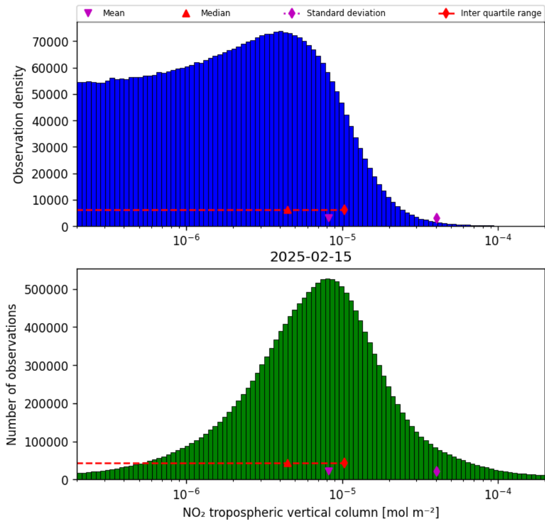
Figure 27: Histogram of “NO 2 tropospheric vertical column” for 2025-02-15 to 2025-02-16
