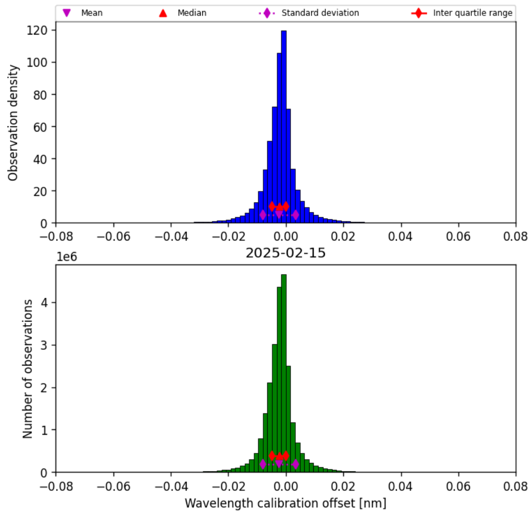
Figure 33: Histogram of “Wavelength calibration offset” for 2025-02-15 to 2025-02-16
