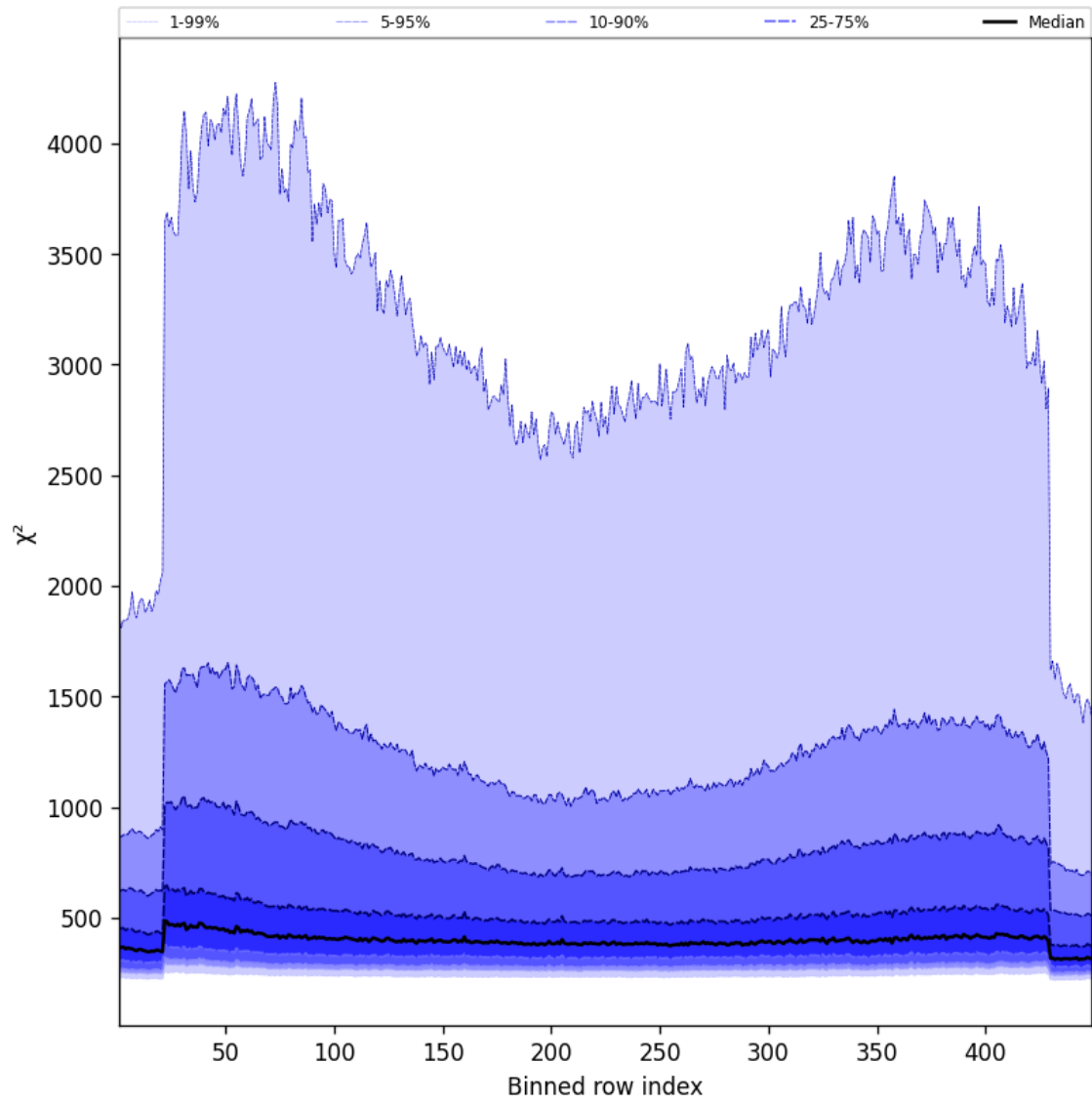
Figure 57: Along track statistics of “ \chi^2 ” for 2025-02-15 to 2025-02-16
