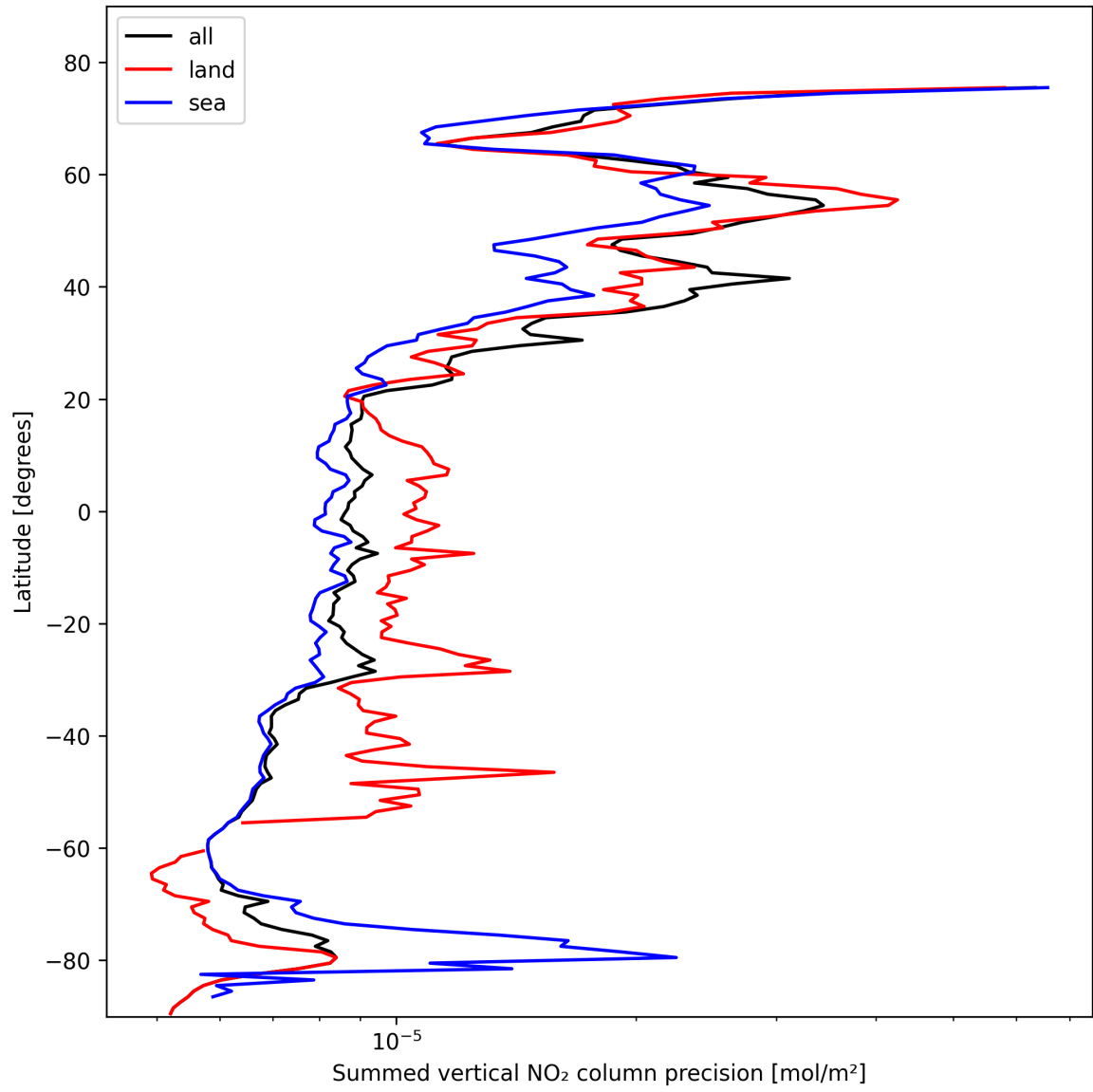
Figure 22: Zonal average of "Summed vertical NO 2 column precision" for 2025-02-15 to 2025-02-16.
