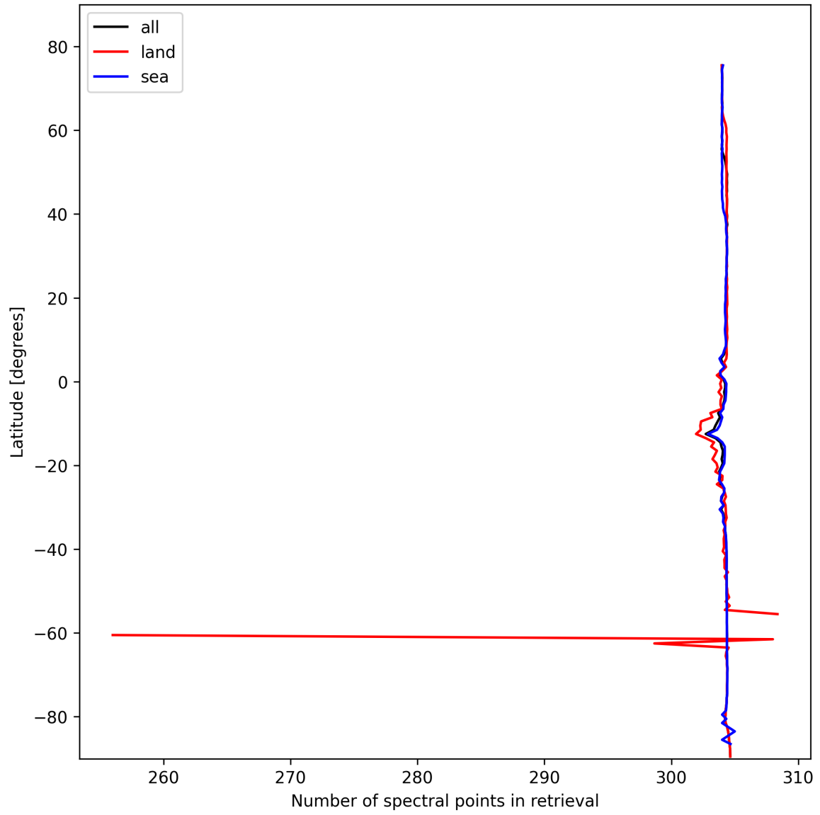
Figure 14: Zonal average of “Number of spectral points in retrieval” for 2025-02-15 to 2025-02-16.
