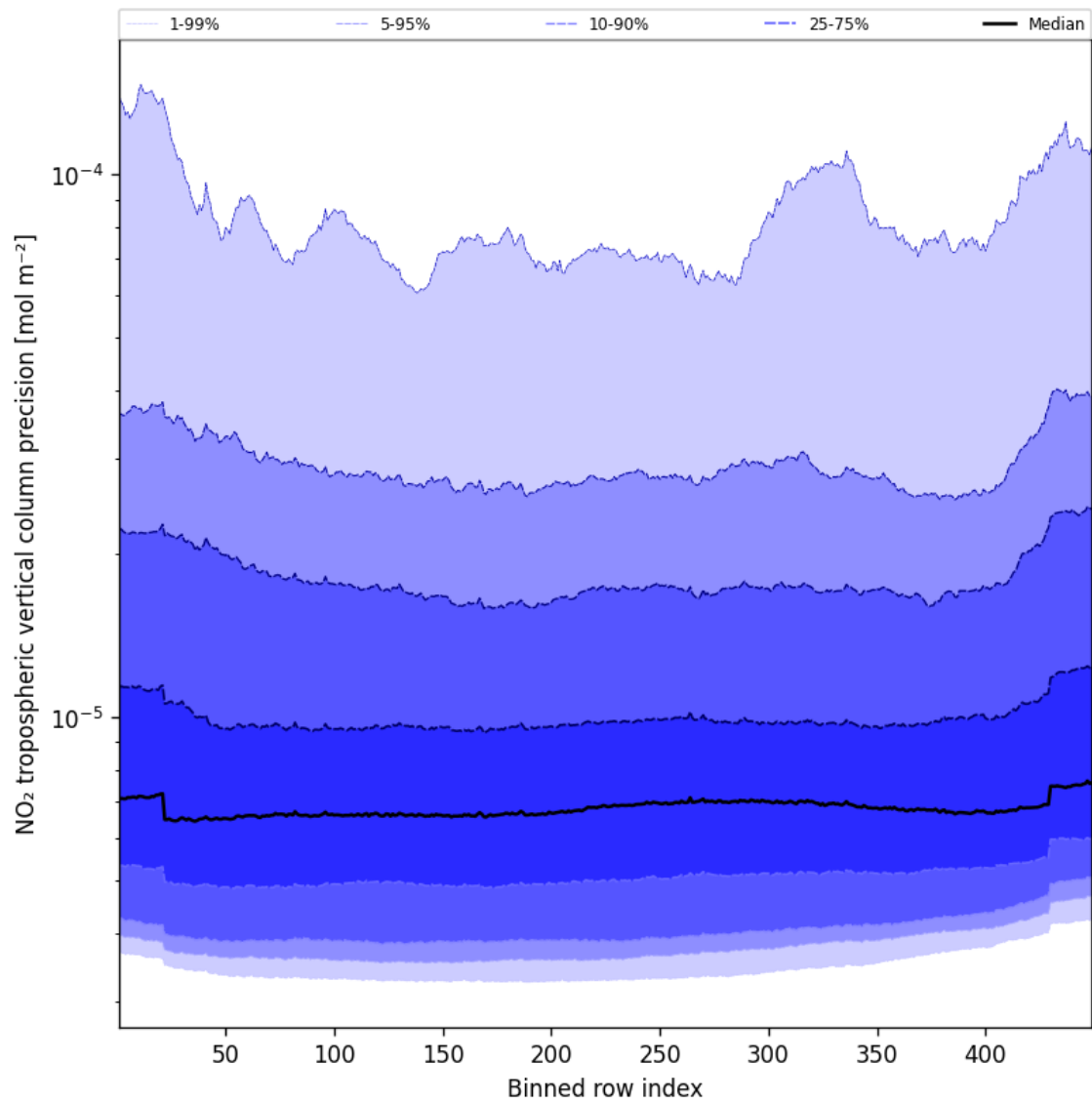
Figure 45: Along track statistics of “NO 2 tropospheric vertical column precision” for 2025-02-15 to 2025-02-16
