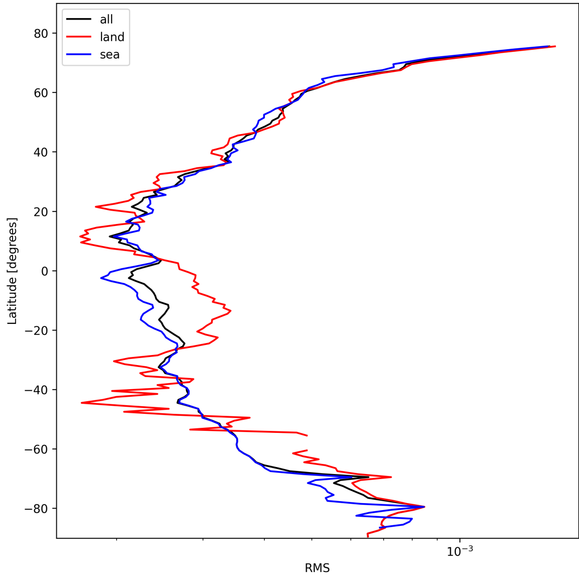
Figure 24: Zonal average of “RMS” for 2025-02-15 to 2025-02-16.
