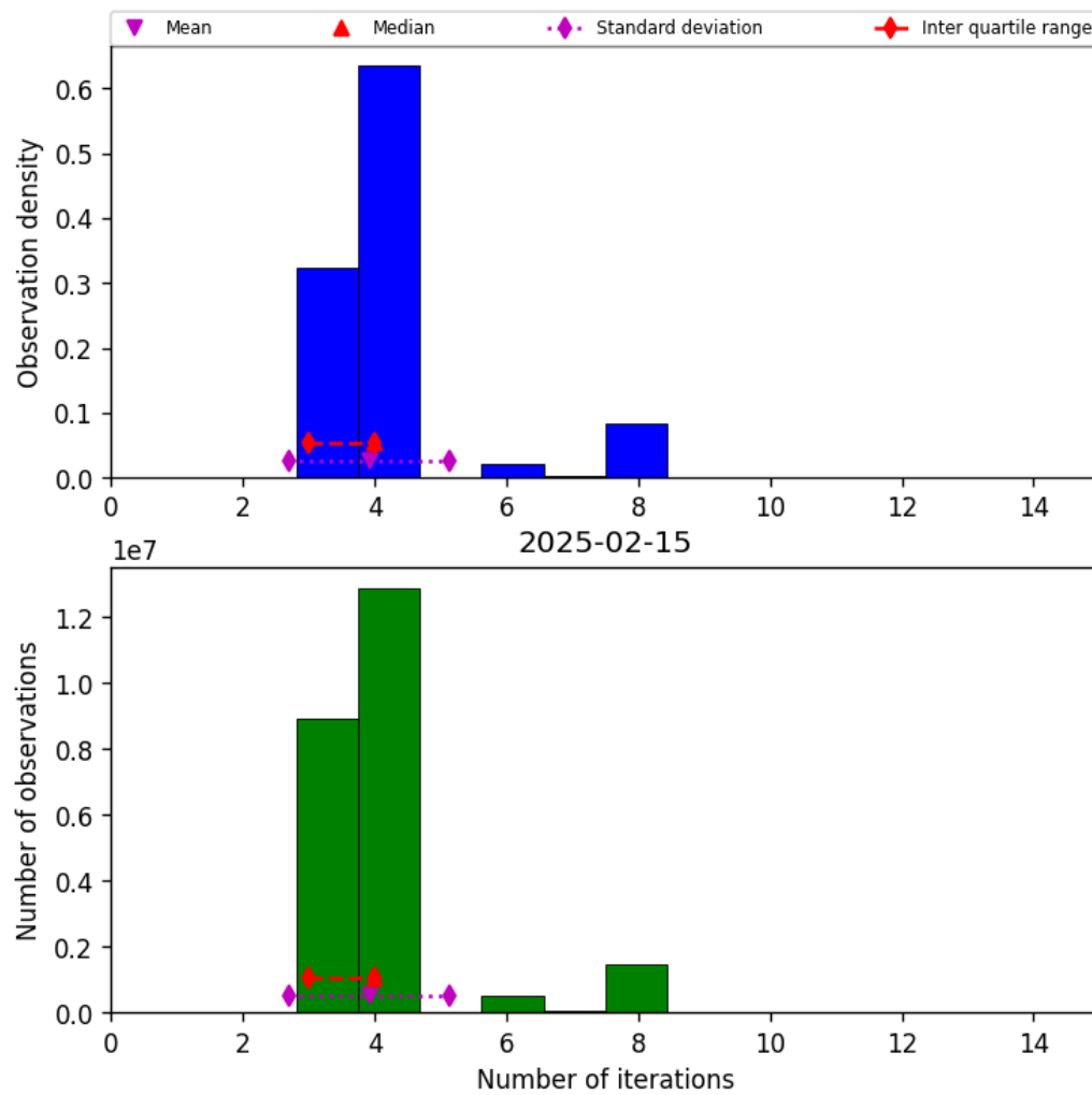
Figure 32: Histogram of “Number of iterations” for 2025-02-15 to 2025-02-16
