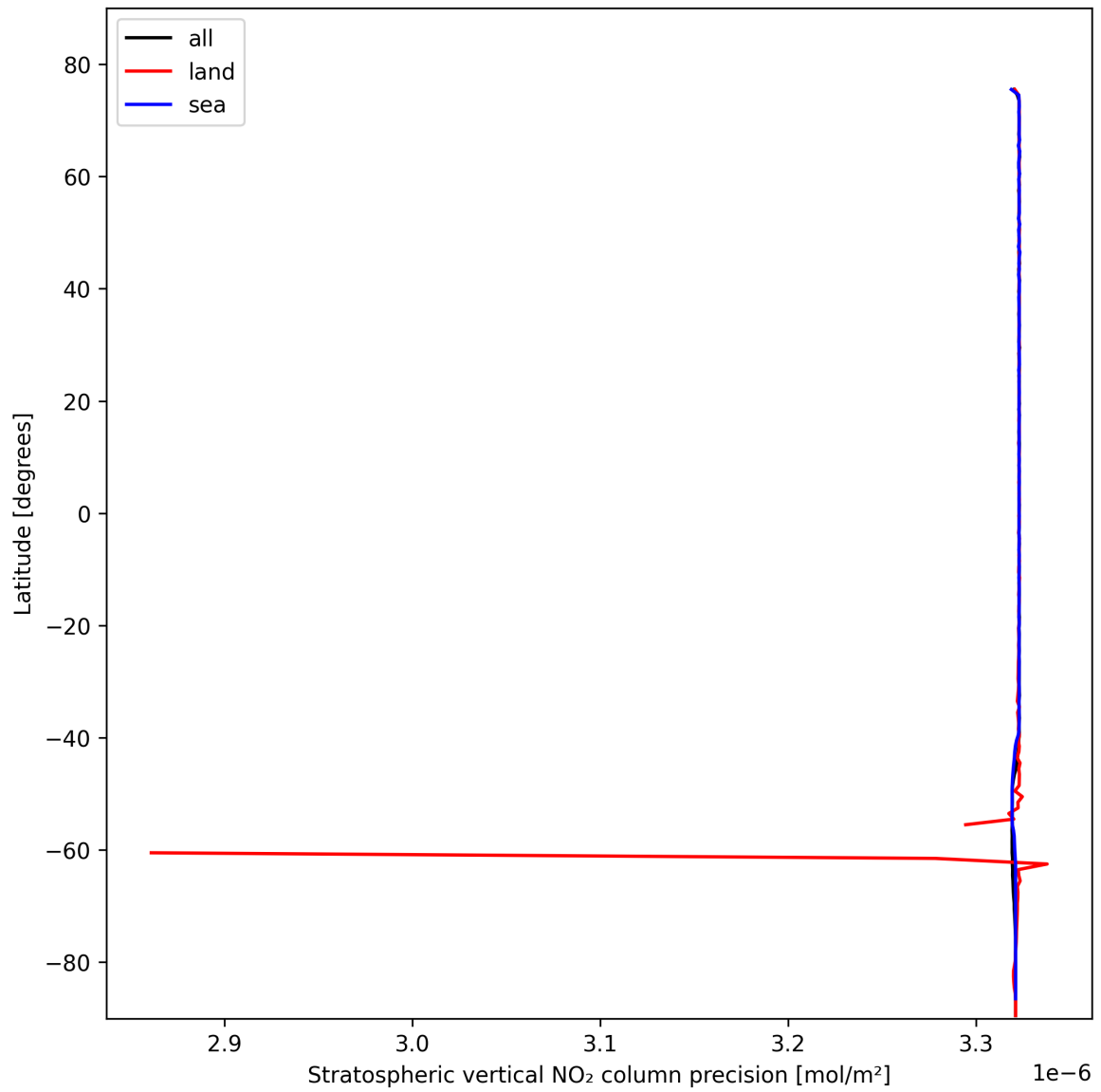
Figure 18: Zonal average of “Stratospheric vertical NO 2 column precision” for 2025-02-15 to 2025-02-16.
