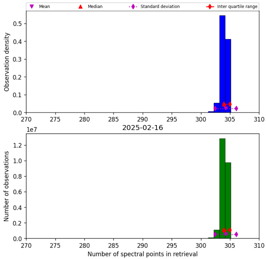
Figure 31: Histogram of “Number of spectral points in retrieval” for 2025-02-16 to 2025-02-16
