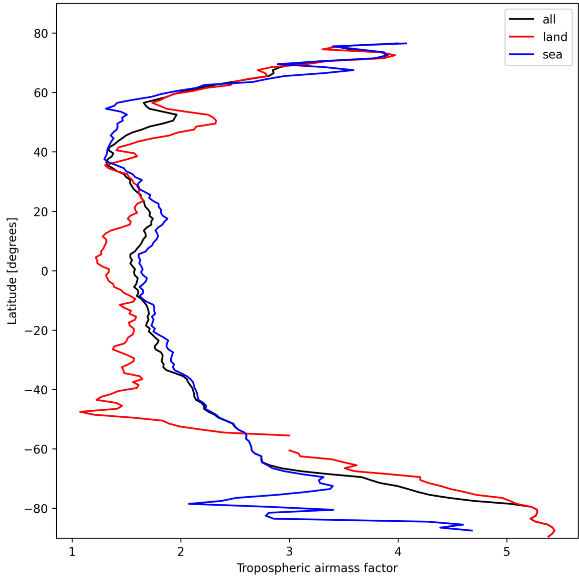
Figure 12: Zonal average of “Tropospheric air mass factor” for 2025-02-16 to 2025-02-16.
