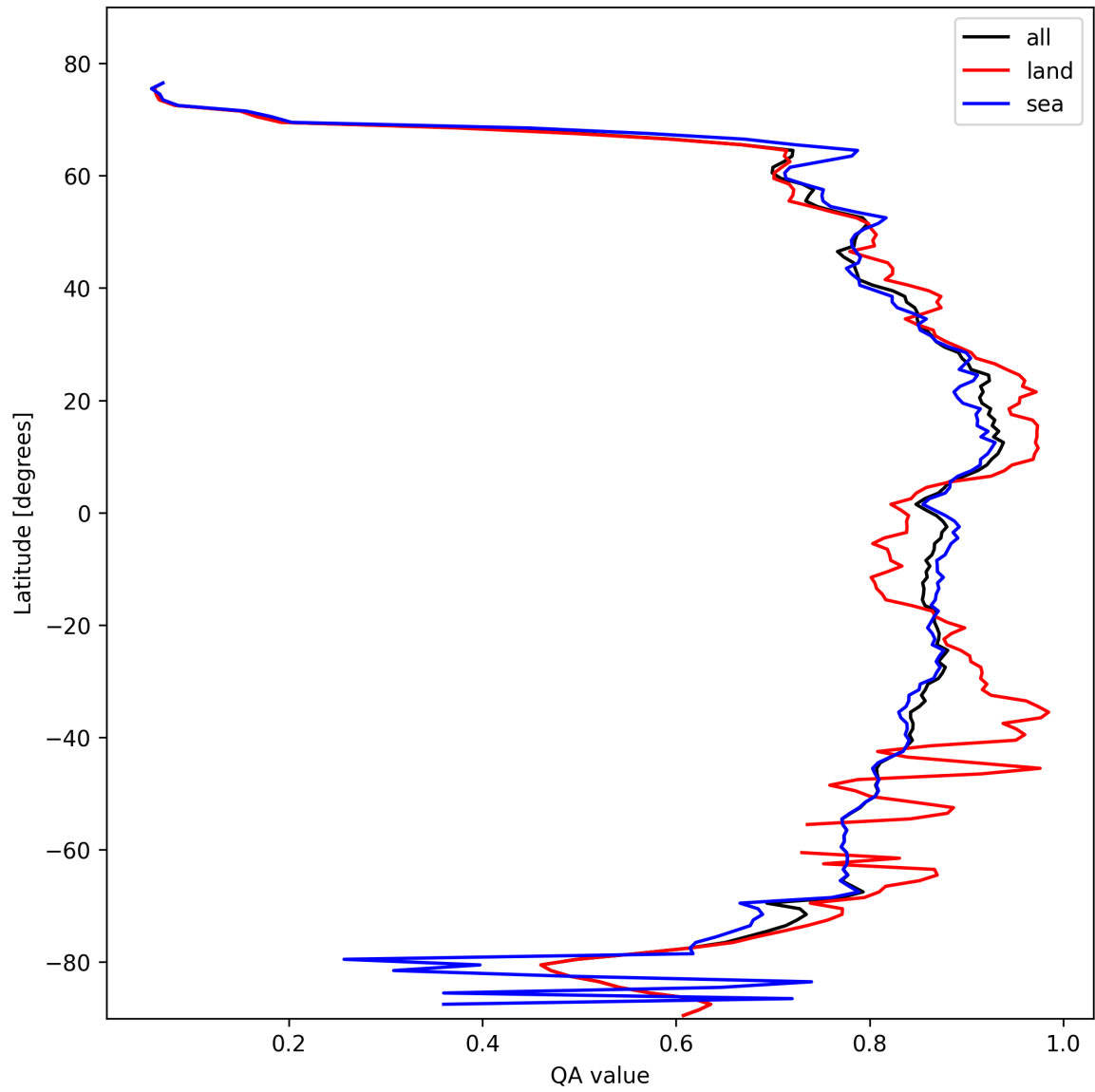
Figure 9: Zonal average of “QA value” for 2025-02-16 to 2025-02-16.
