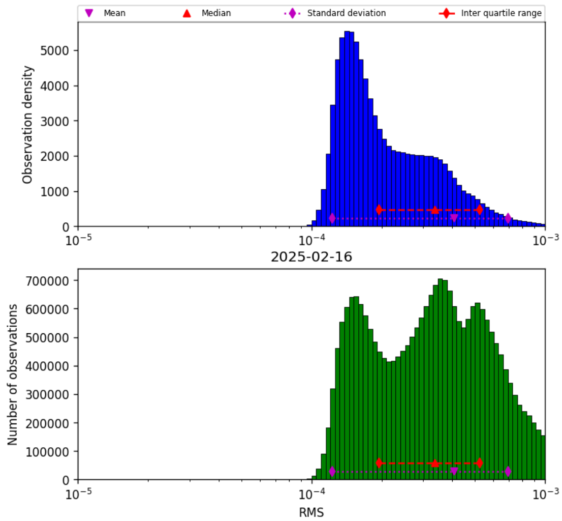
Figure 41: Histogram of “RMS” for 2025-02-16 to 2025-02-16
