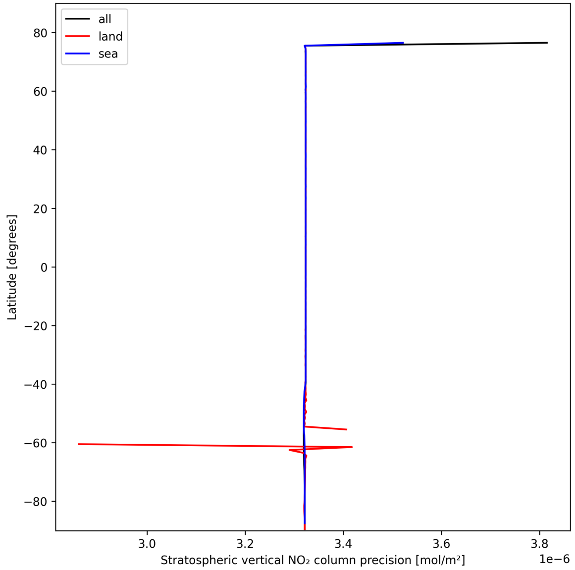
Figure 18: Zonal average of “Stratospheric vertical NO 2 column precision” for 2025-02-16 to 2025-02-16.
