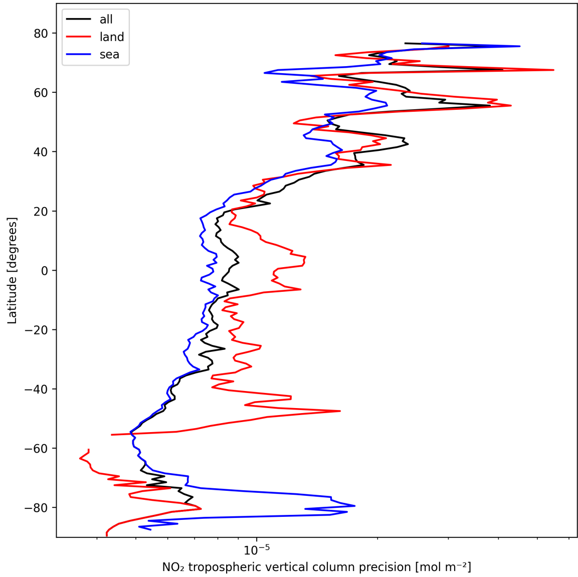
Figure 11: Zonal average of “NO 2 tropospheric vertical column precision” for 2025-02-16 to 2025-02-16.
