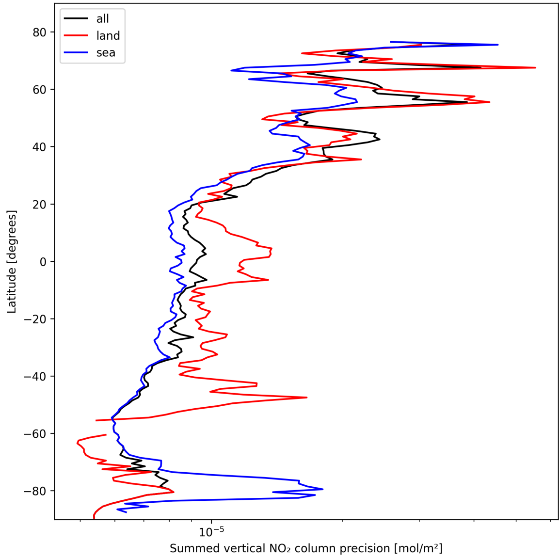
Figure 22: Zonal average of “Summed vertical NO 2 column precision” for 2025-02-16 to 2025-02-16.
