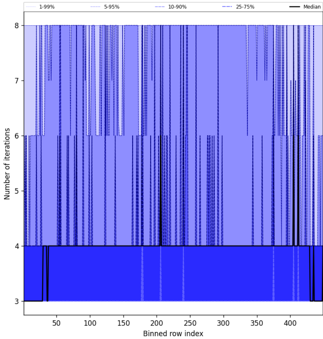
Figure 49: Along track statistics of “Number of iterations” for 2025-02-16 to 2025-02-16
