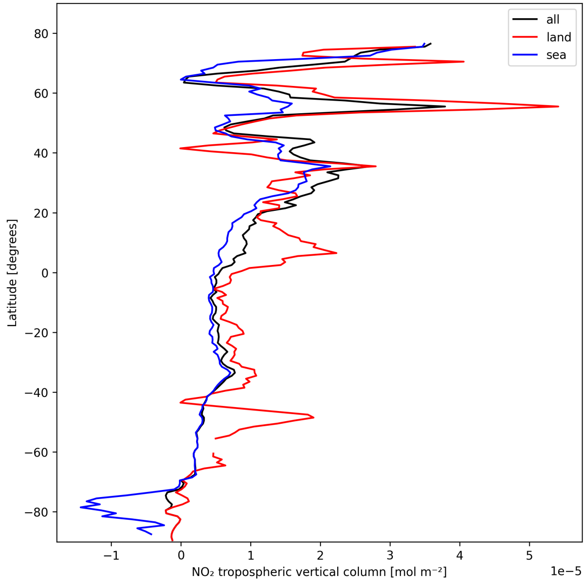
Figure 10: Zonal average of “NO 2 tropospheric vertical column” for 2025-02-16 to 2025-02-16.
