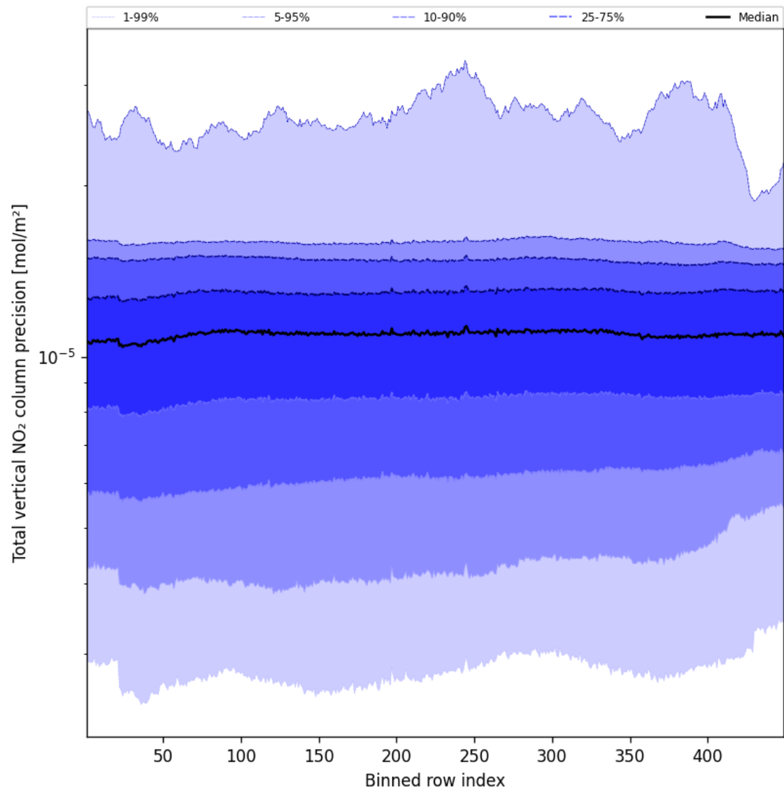
Figure 54: Along track statistics of “Total vertical NO 2 column precision” for 2025-02-16 to 2025-02-16
