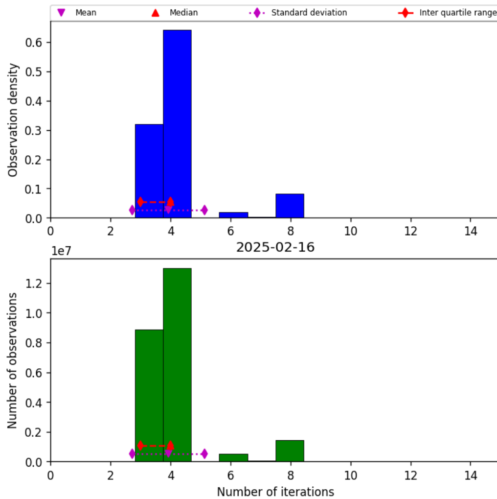
Figure 32: Histogram of “Number of iterations” for 2025-02-16 to 2025-02-16
