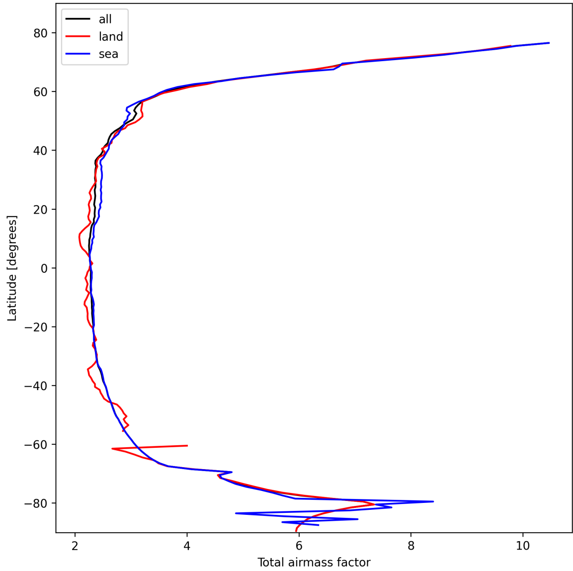
Figure 13: Zonal average of “Total airmass factor” for 2025-02-16 to 2025-02-16.
