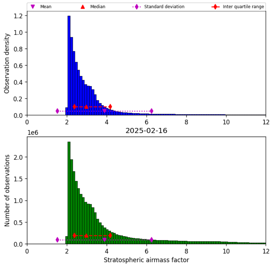
Figure 42: Histogram of “Stratospheric airmass factor” for 2025-02-16 to 2025-02-16
