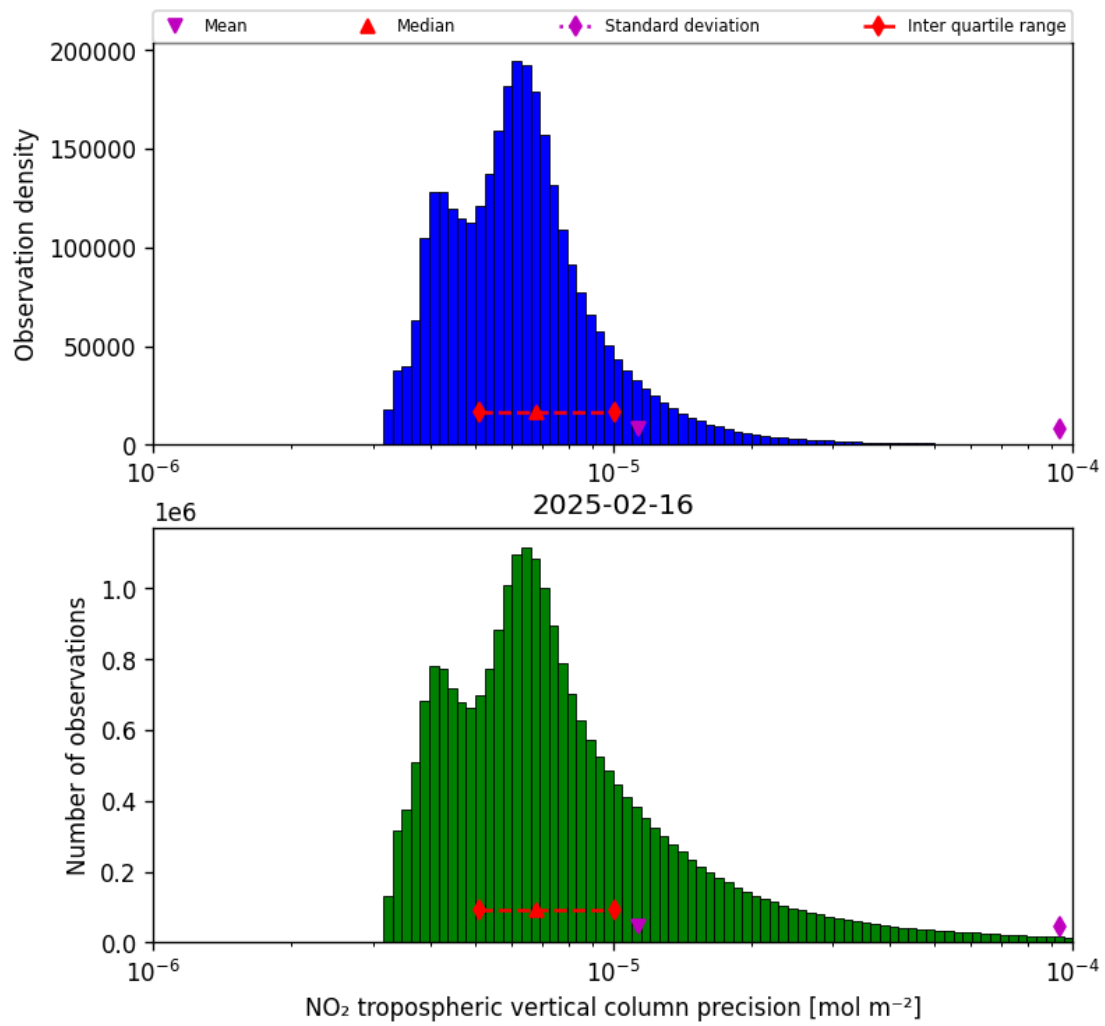
Figure 28: Histogram of "NO 2 tropospheric vertical column precision" for 2025-02-16 to 2025-02-16
