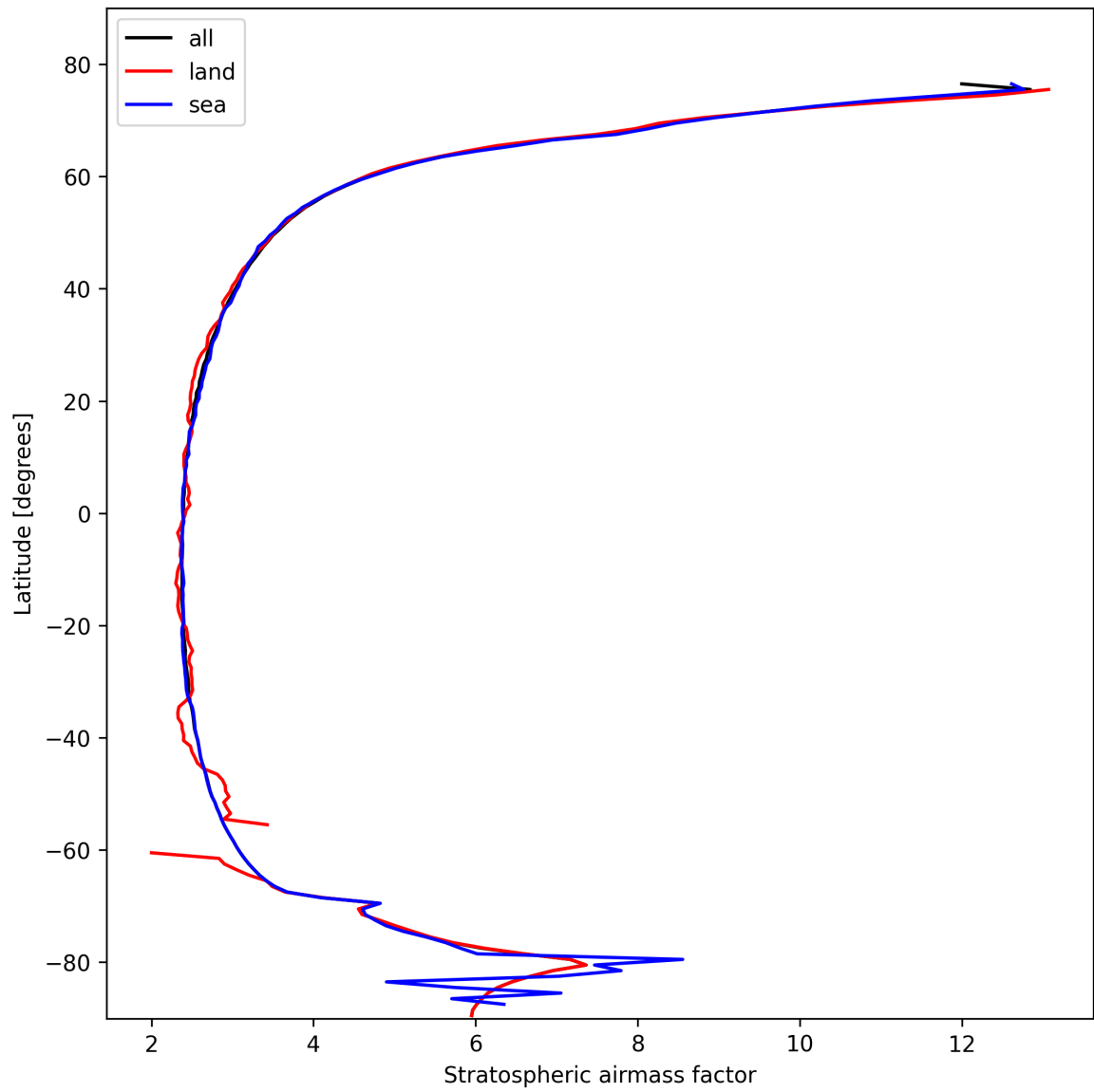
Figure 25: Zonal average of “Stratospheric airmass factor” for 2025-02-16 to 2025-02-16.
