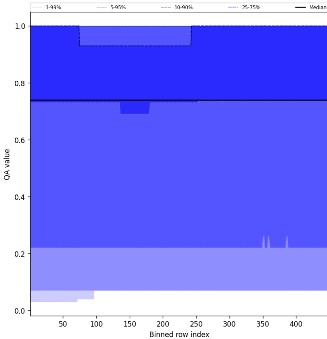
Figure 43: Along track statistics of “QA value” for 2025-02-16 to 2025-02-16
