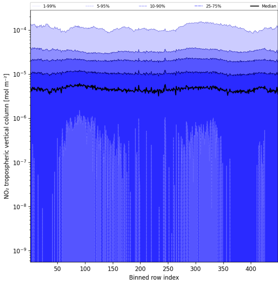
Figure 44: Along track statistics of “NO 2 tropospheric vertical column” for 2025-02-16 to 2025-02-16
