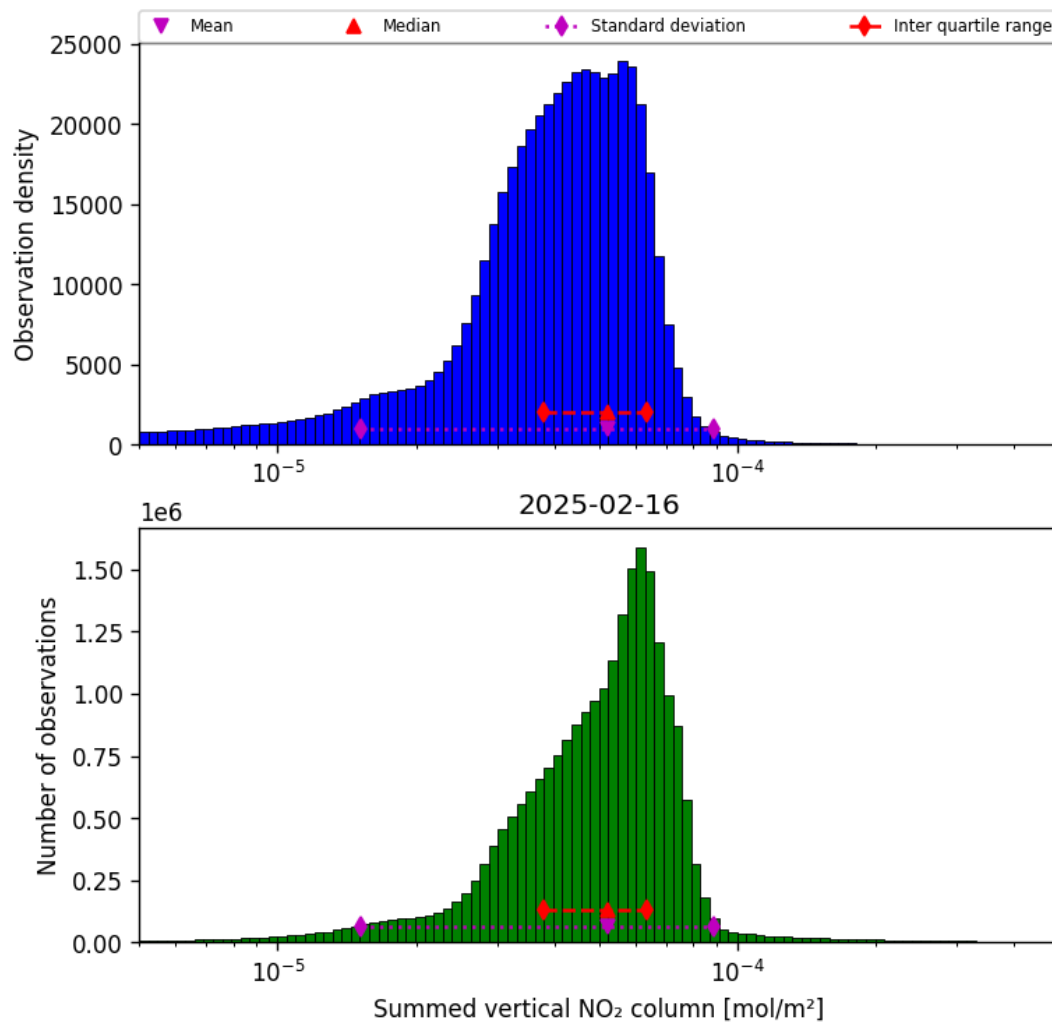
Figure 38: Histogram of “Summed vertical NO 2 column” for 2025-02-16 to 2025-02-16
