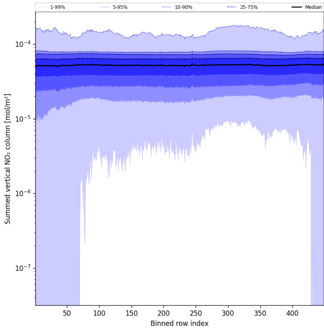
Figure 55: Along track statistics of “Summed vertical NO 2 column” for 2025-02-16 to 2025-02-16
