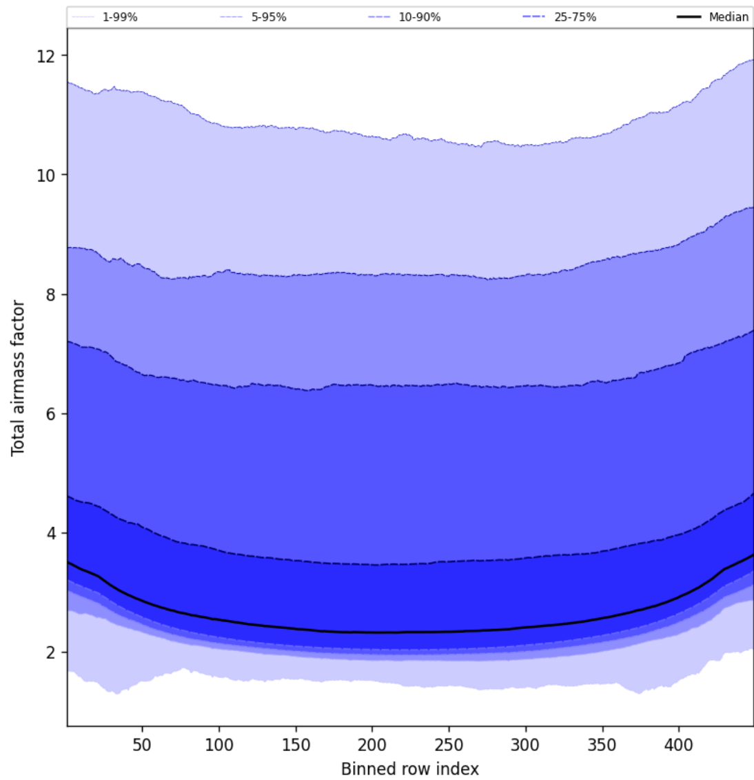
Figure 47: Along track statistics of “Total airmass factor” for 2025-02-16 to 2025-02-16
