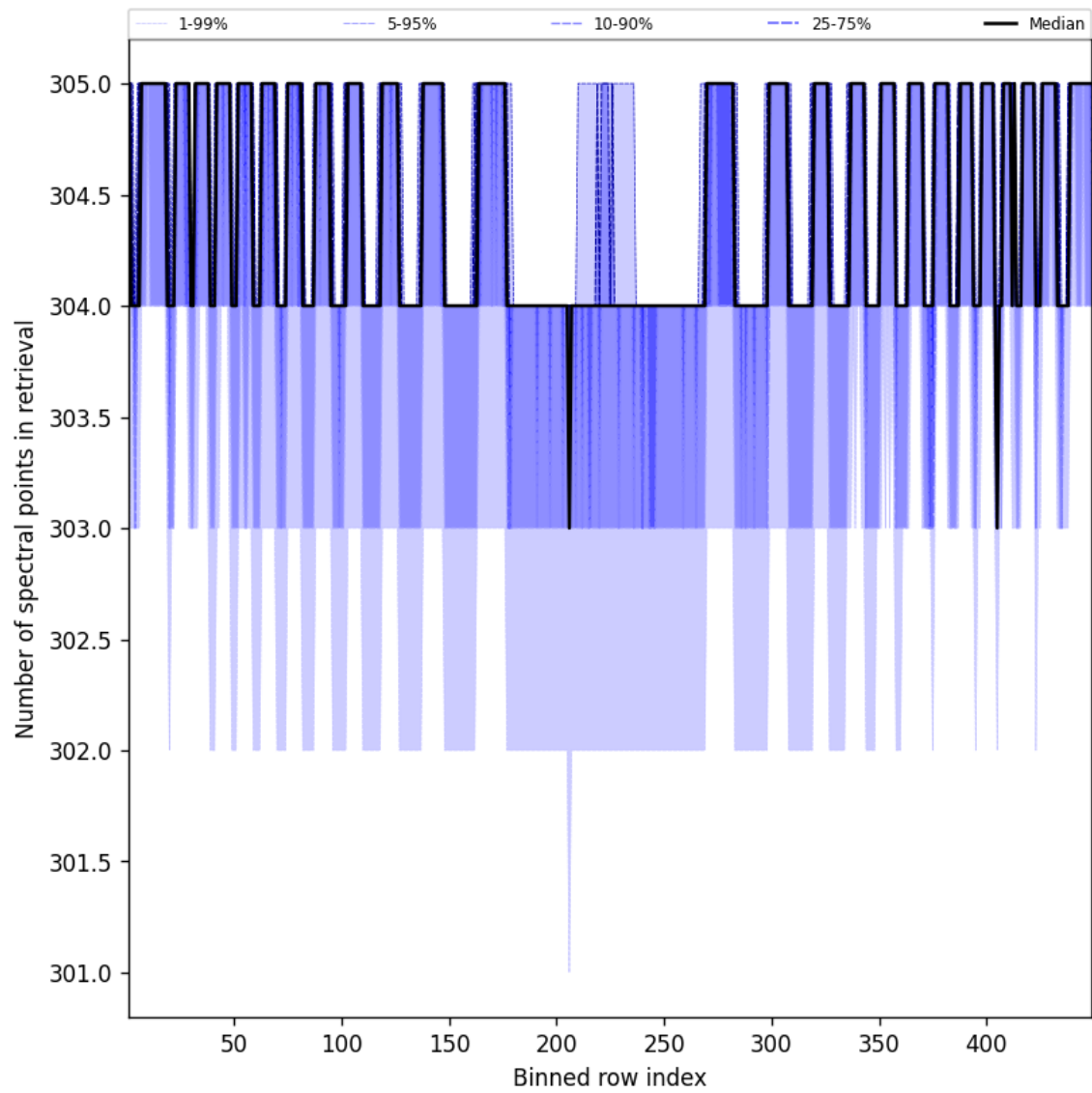
Figure 48: Along track statistics of “Number of spectral points in retrieval” for 2025-02-16 to 2025-02-16
