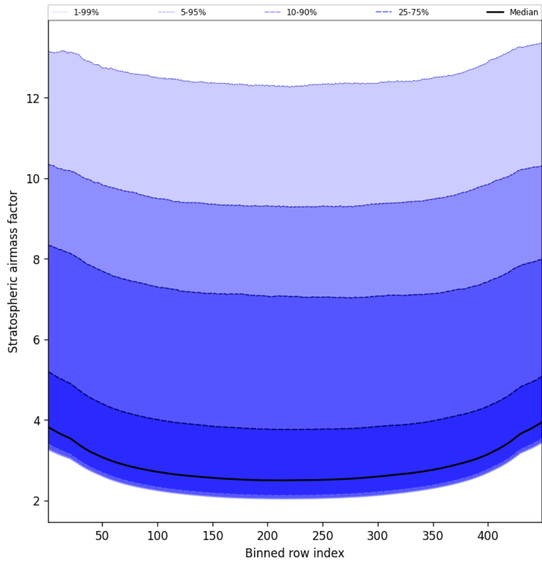
Figure 59: Along track statistics of “Stratospheric airmass factor” for 2025-02-16 to 2025-02-16
