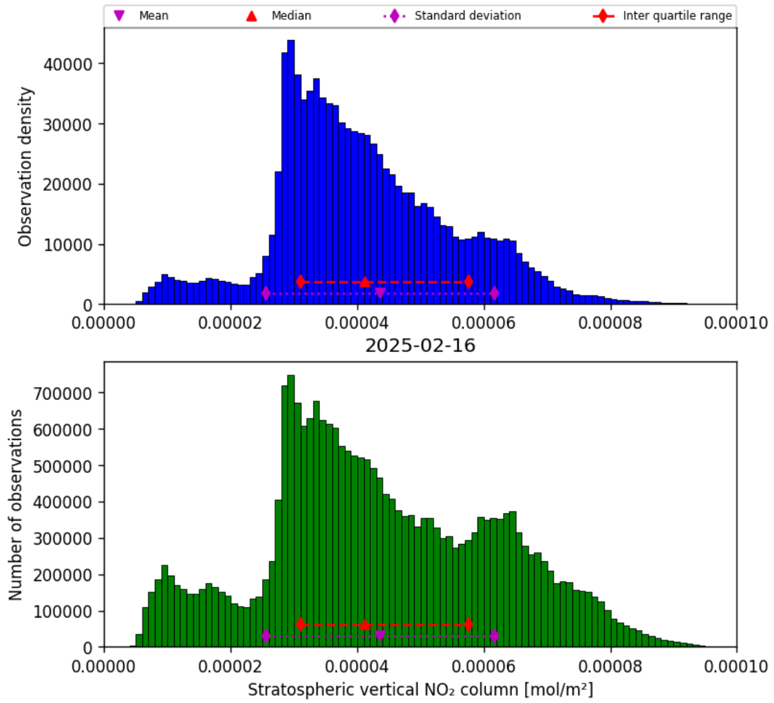
Figure 34: Histogram of “Stratospheric vertical NO 2 column” for 2025-02-16 to 2025-02-16
