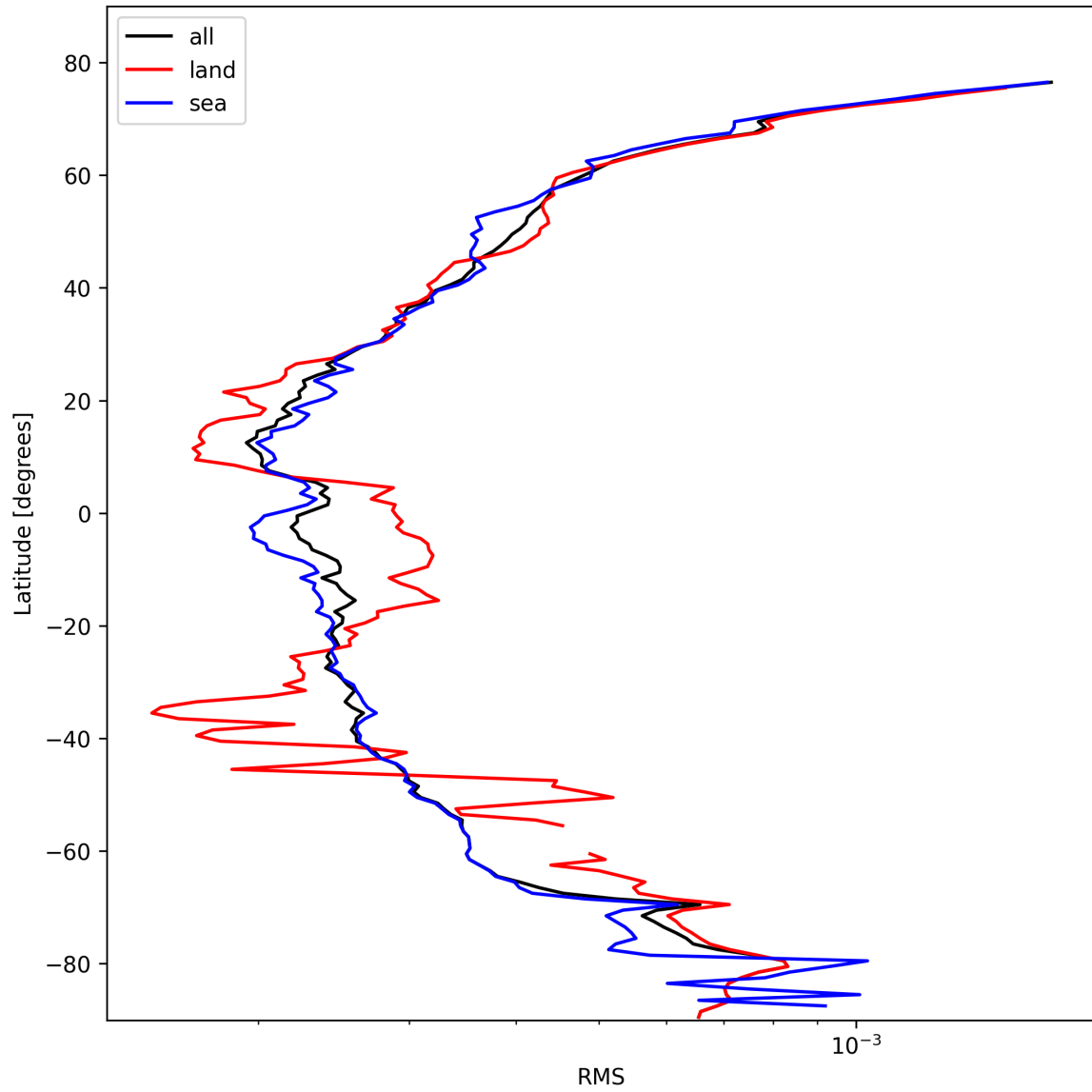
Figure 24: Zonal average of “RMS” for 2025-02-16 to 2025-02-16.
