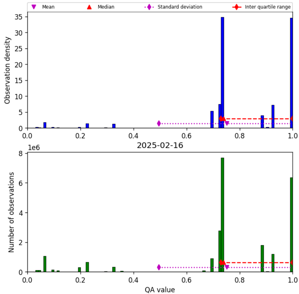
Figure 26: Histogram of “QA value” for 2025-02-16 to 2025-02-16
