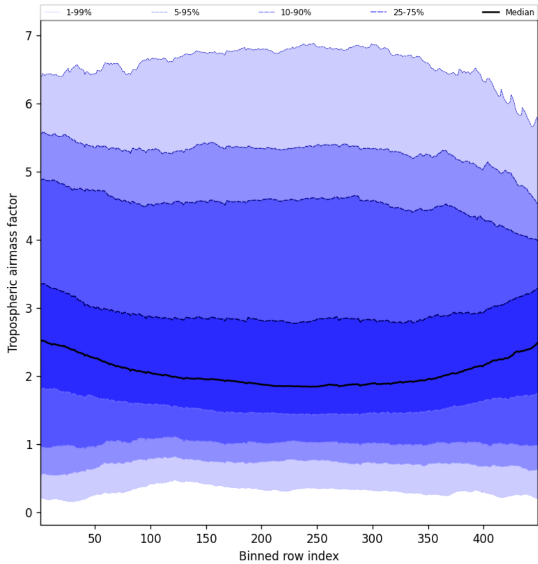
Figure 46: Along track statistics of “Tropospheric airmass factor” for 2025-02-16 to 2025-02-16
