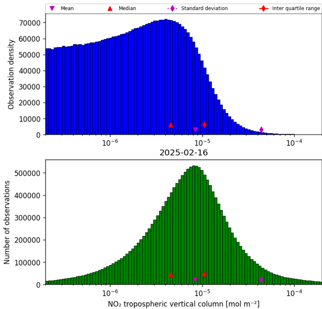
Figure 27: Histogram of “NO 2 tropospheric vertical column” for 2025-02-16 to 2025-02-16
