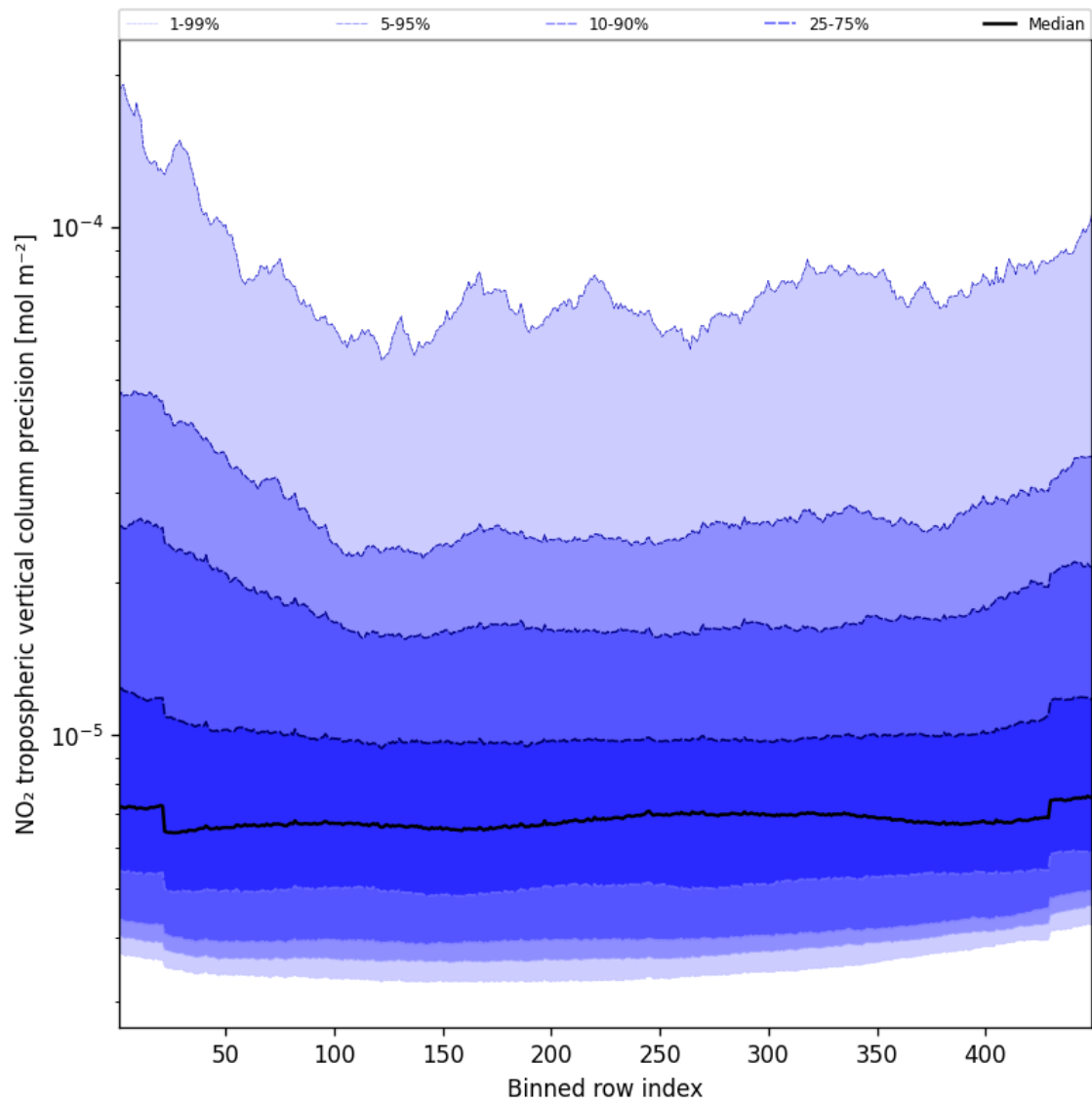
Figure 45: Along track statistics of “NO 2 tropospheric vertical column precision” for 2025-02-16 to 2025-02-16
