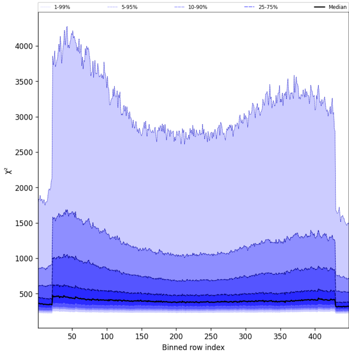
Figure 57: Along track statistics of “ \chi^2 ” for 2025-02-16 to 2025-02-16
