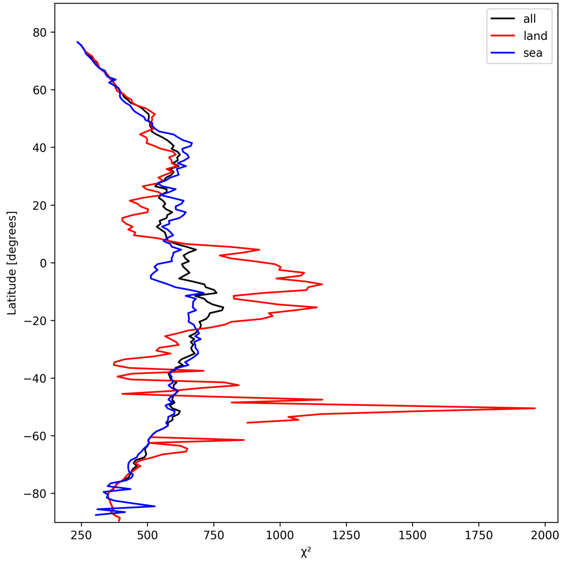
Figure 23: Zonal average of “ \chi^2 ” for 2025-02-16 to 2025-02-16.
