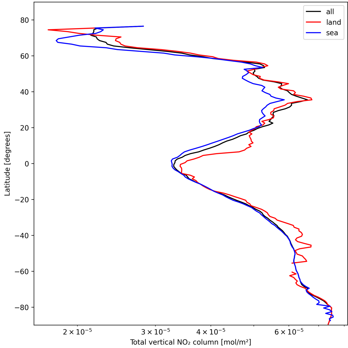
Figure 19: Zonal average of “Total vertical NO 2 column” for 2025-02-16 to 2025-02-16.
