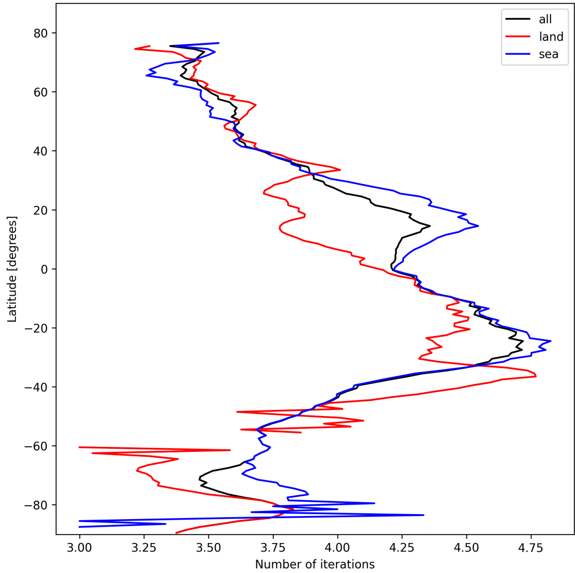
Figure 15: Zonal average of “Number of iterations” for 2025-02-16 to 2025-02-16.
