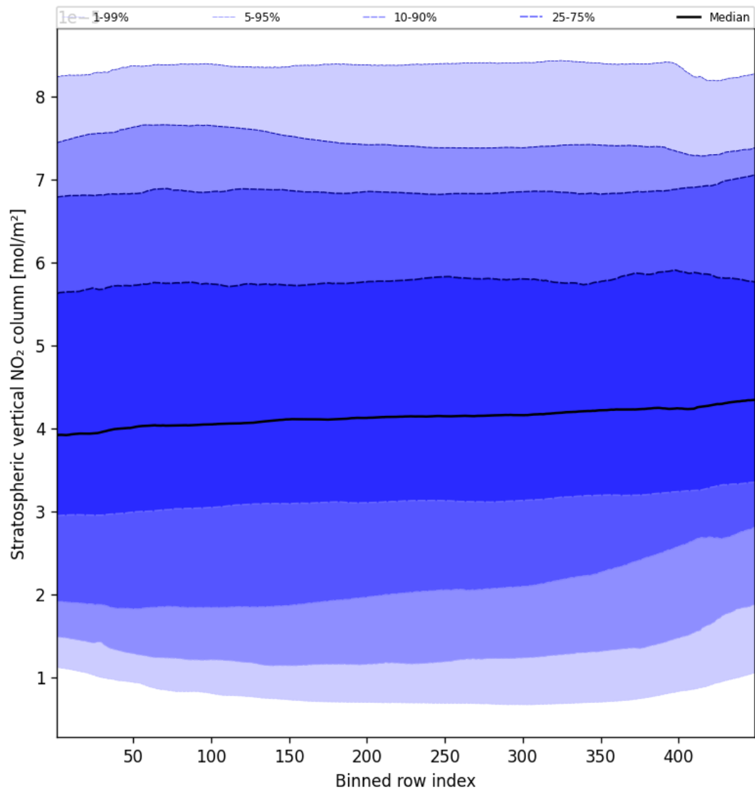
Figure 51: Along track statistics of “Stratospheric vertical NO 2 column” for 2025-02-16 to 2025-02-16
