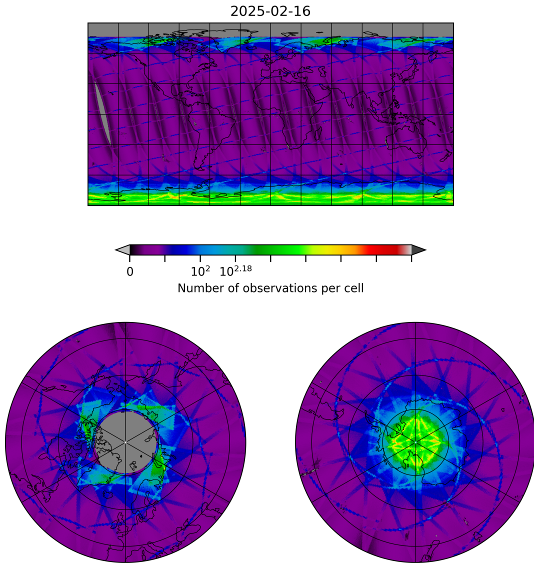
Figure 8: Map of the number of observations for 2025-02-16 to 2025-02-16
