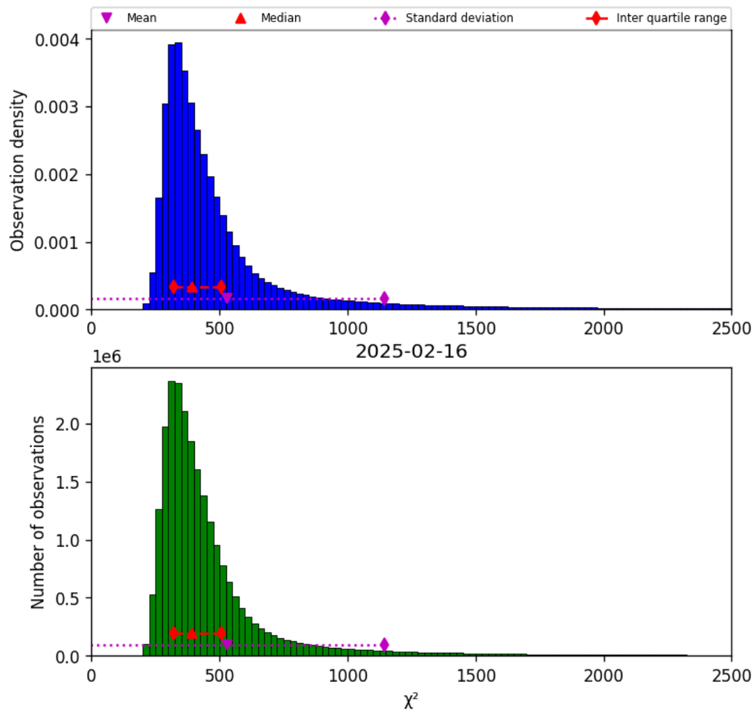
Figure 40: Histogram of “ \chi^2 ” for 2025-02-16 to 2025-02-16
