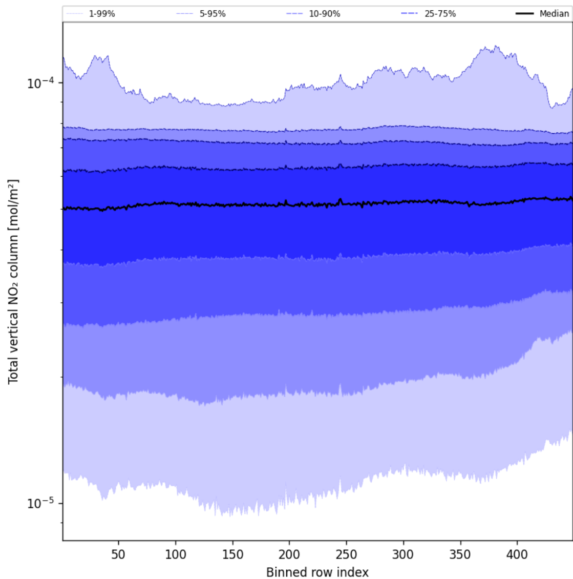
Figure 53: Along track statistics of “Total vertical NO 2 column” for 2025-02-16 to 2025-02-16
