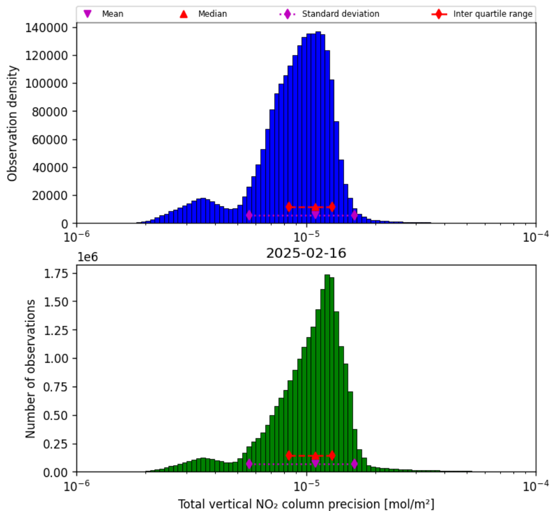
Figure 37: Histogram of "Total vertical NO 2 column precision" for 2025-02-16 to 2025-02-16
