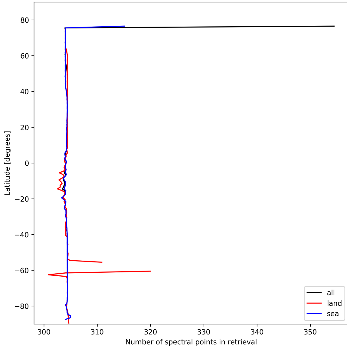
Figure 14: Zonal average of “Number of spectral points in retrieval” for 2025-02-16 to 2025-02-16.
