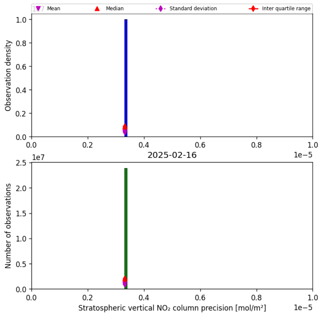
Figure 35: Histogram of “Stratospheric vertical NO 2 column precision” for 2025-02-16 to 2025-02-16
