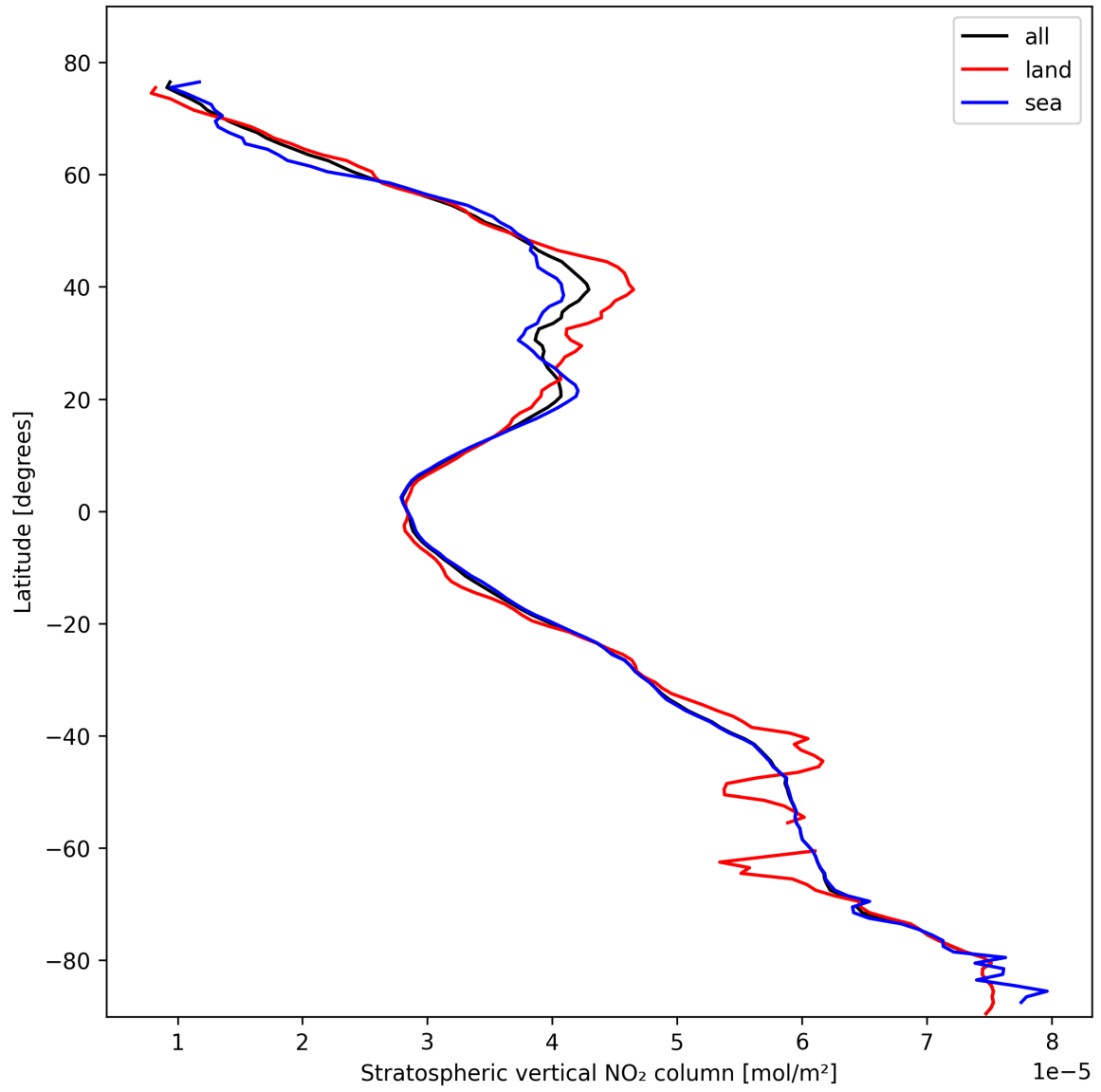
Figure 17: Zonal average of “Stratospheric vertical NO 2 column” for 2025-02-16 to 2025-02-16.
