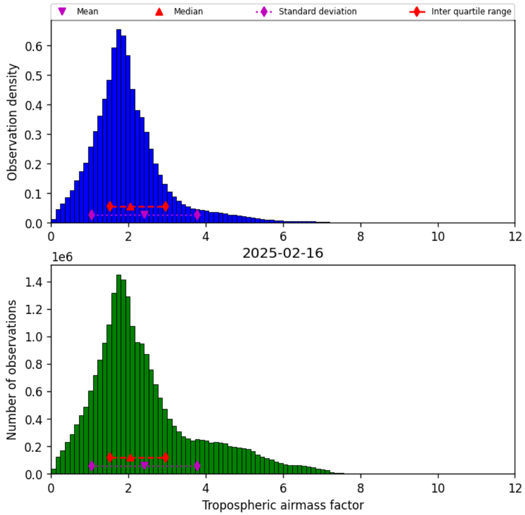
Figure 29: Histogram of “Tropospheric airmass factor” for 2025-02-16 to 2025-02-16
