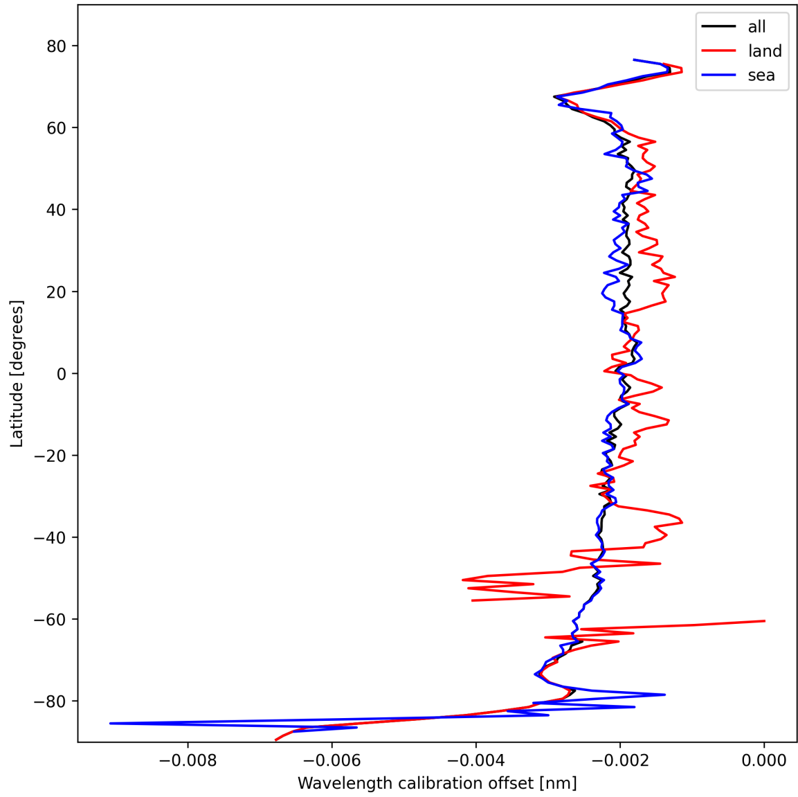
Figure 16: Zonal average of “Wavelength calibration offset” for 2025-02-16 to 2025-02-16.
