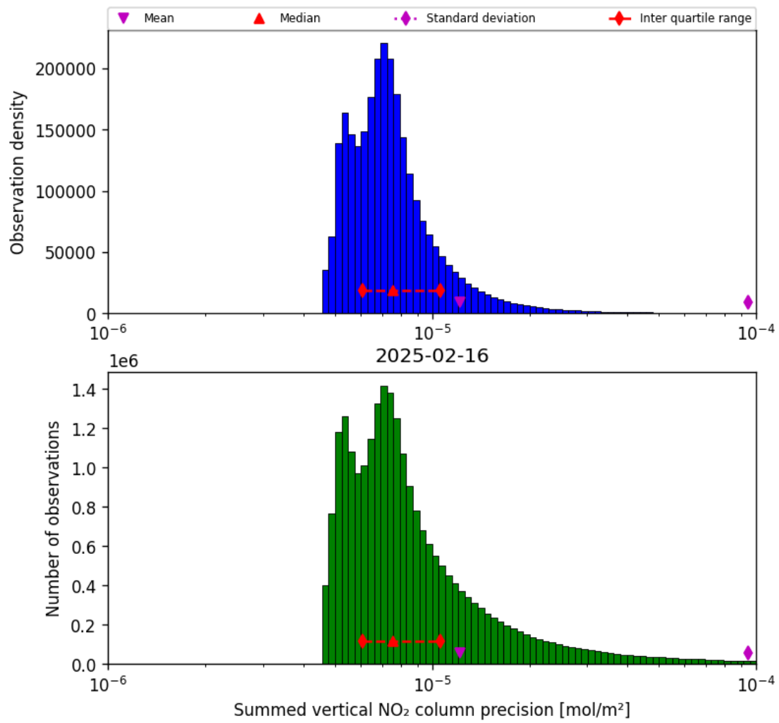
Figure 39: Histogram of "Summed vertical NO 2 column precision" for 2025-02-16 to 2025-02-16
