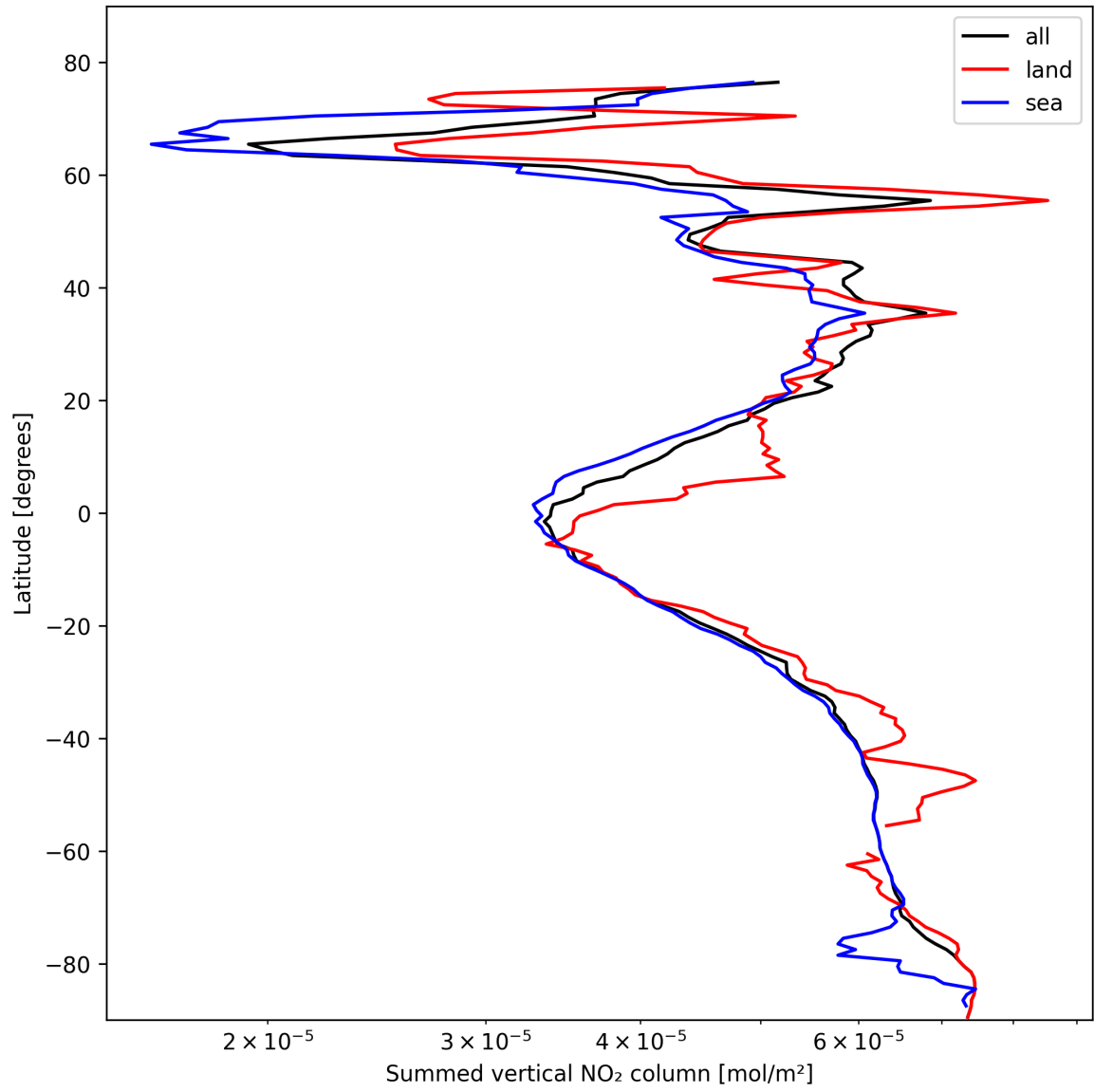
Figure 21: Zonal average of “Summed vertical NO 2 column” for 2025-02-16 to 2025-02-16.
