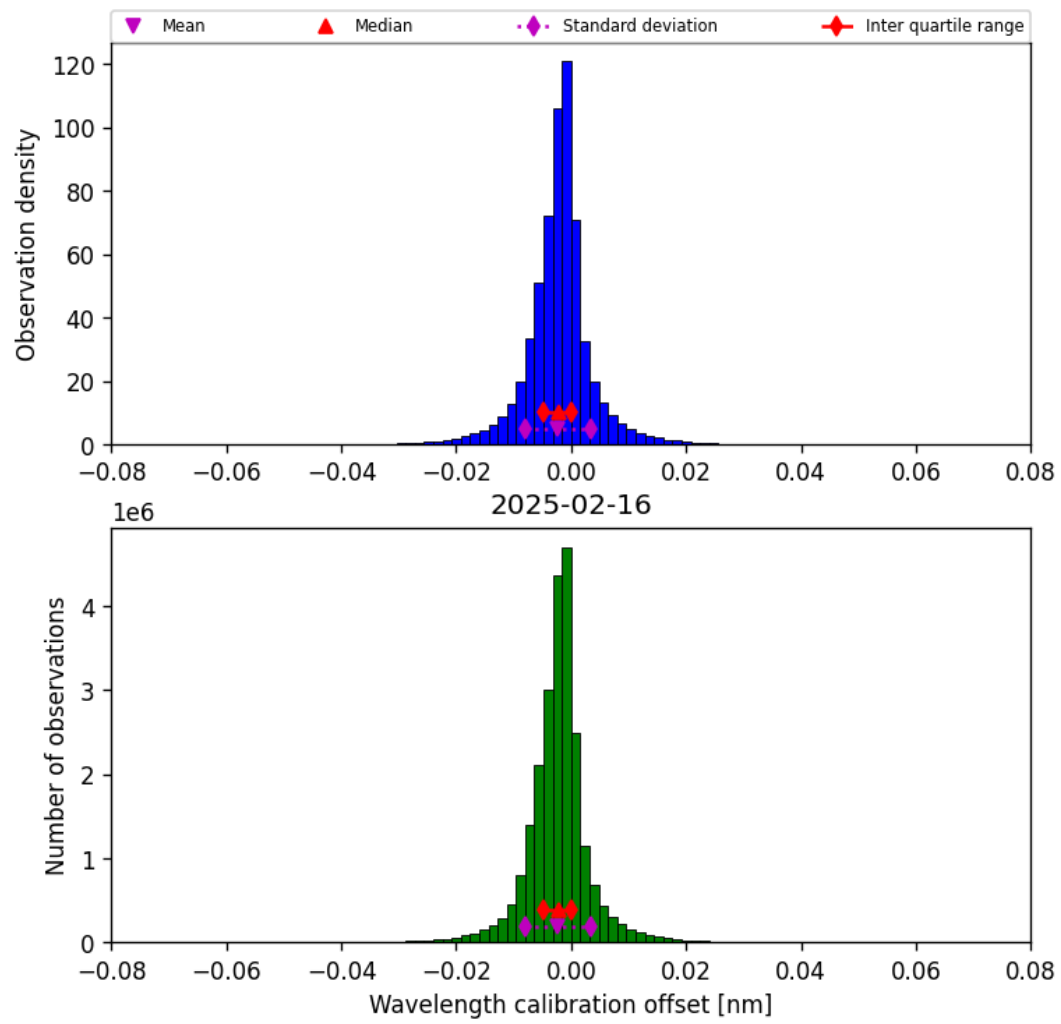
Figure 33: Histogram of “Wavelength calibration offset” for 2025-02-16 to 2025-02-16
