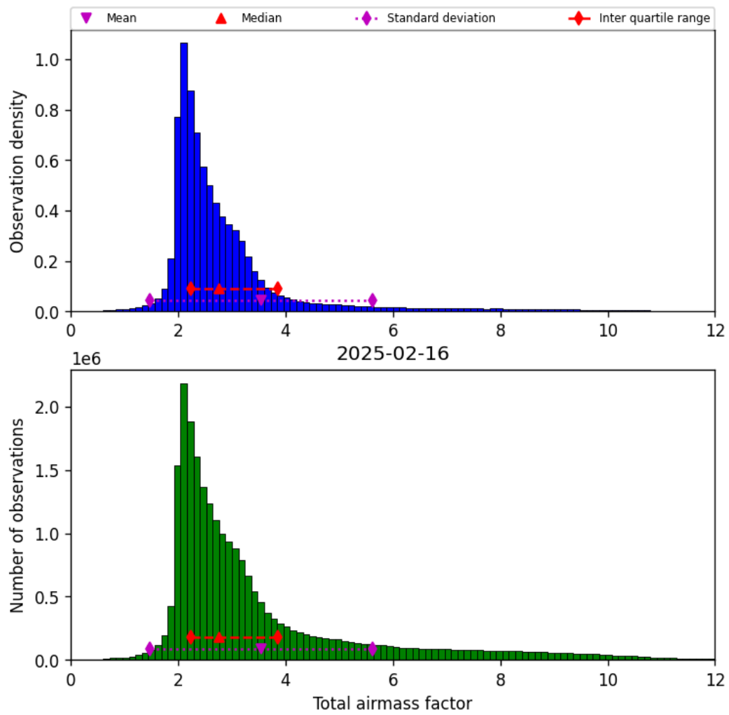
Figure 30: Histogram of “Total airmass factor” for 2025-02-16 to 2025-02-16
