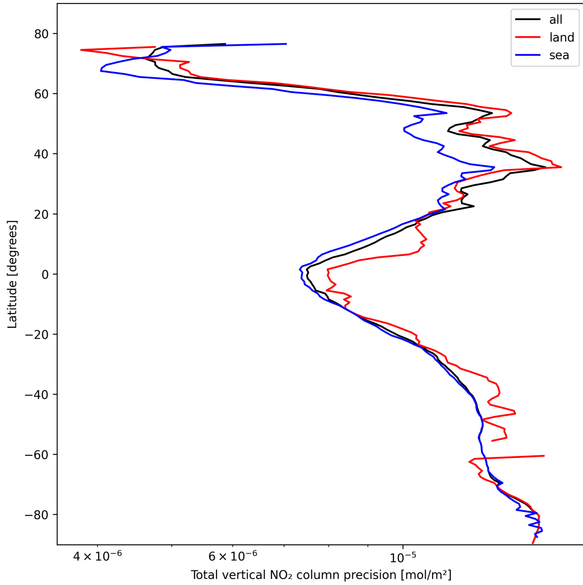
Figure 20: Zonal average of “Total vertical NO 2 column precision” for 2025-02-16 to 2025-02-16.
