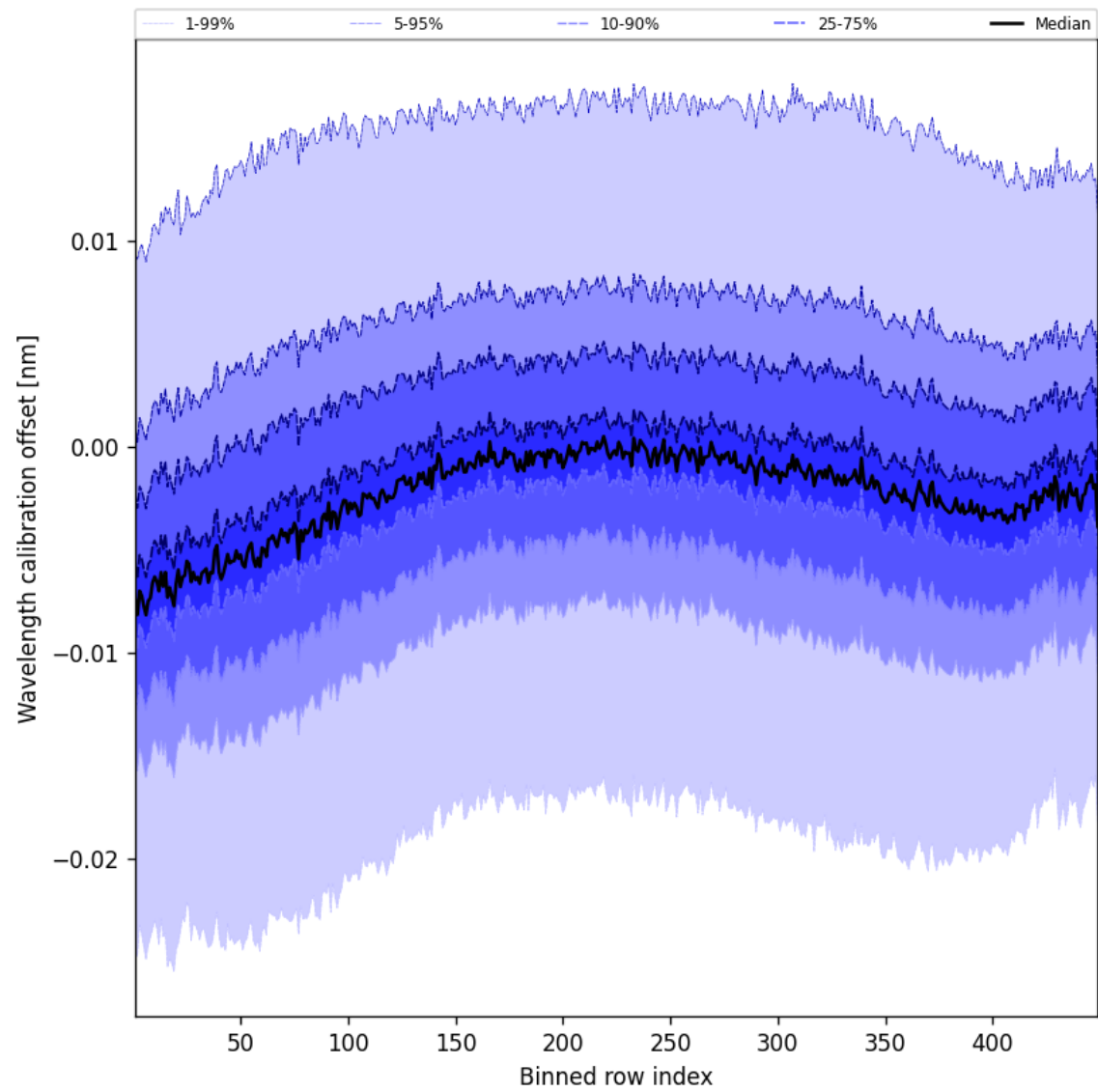
Figure 50: Along track statistics of “Wavelength calibration offset” for 2025-02-16 to 2025-02-16
