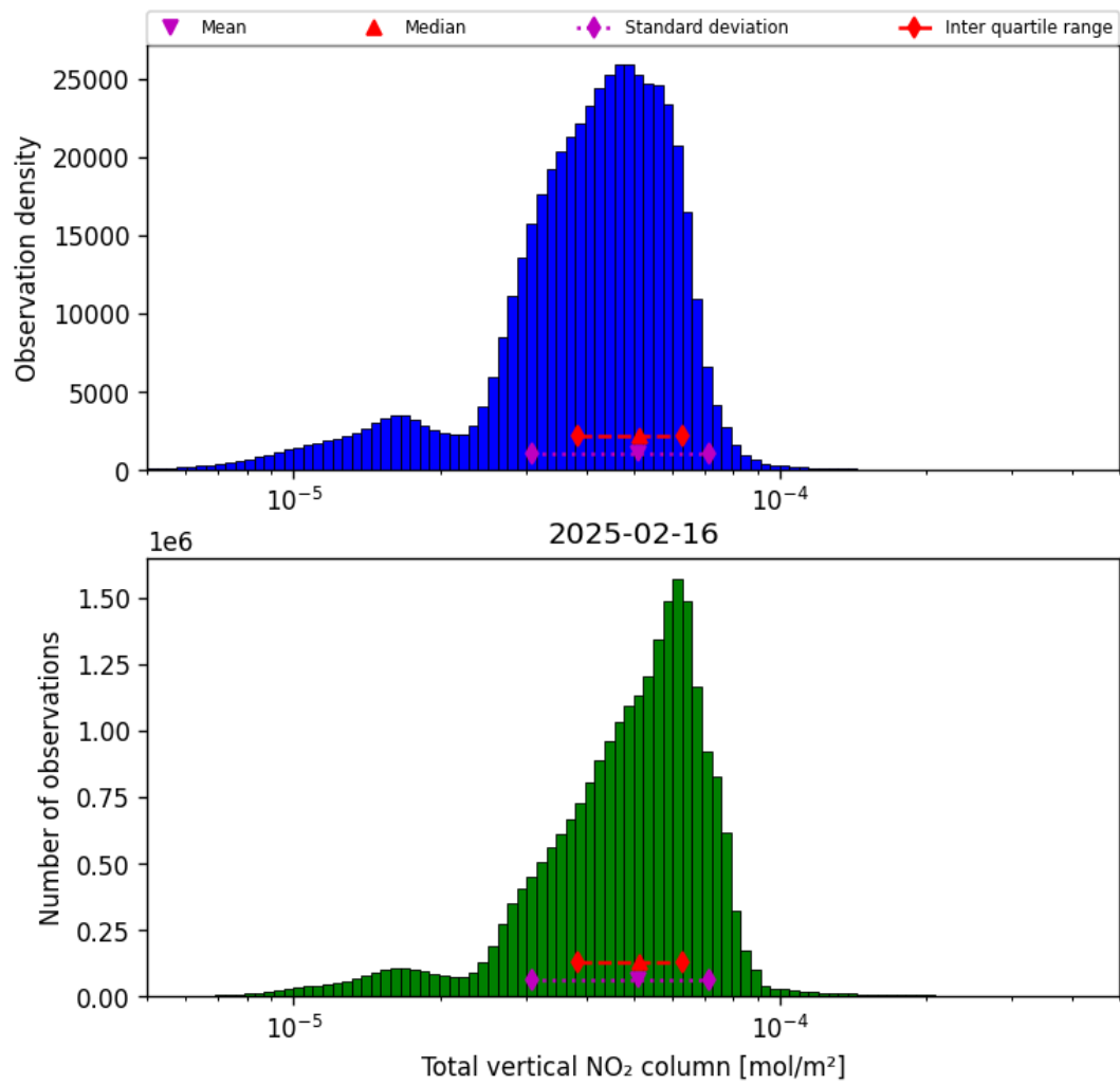
Figure 36: Histogram of "Total vertical NO 2 column" for 2025-02-16 to 2025-02-16
