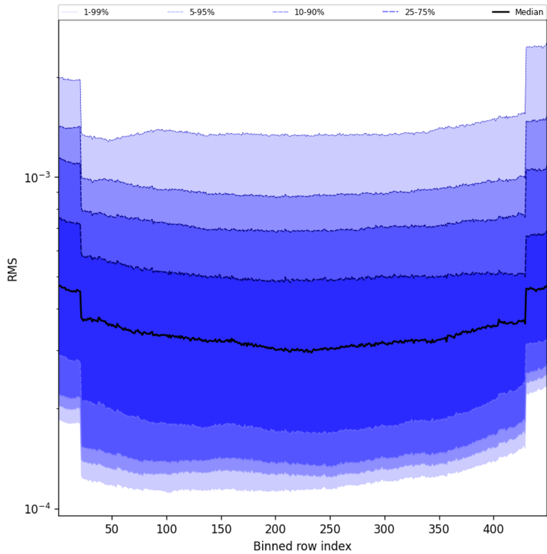
Figure 58: Along track statistics of “RMS” for 2025-02-16 to 2025-02-16
