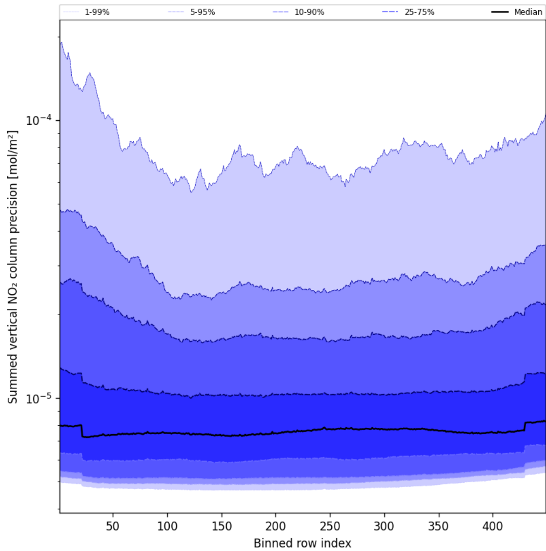
Figure 56: Along track statistics of “Summed vertical NO 2 column precision” for 2025-02-16 to 2025-02-16
