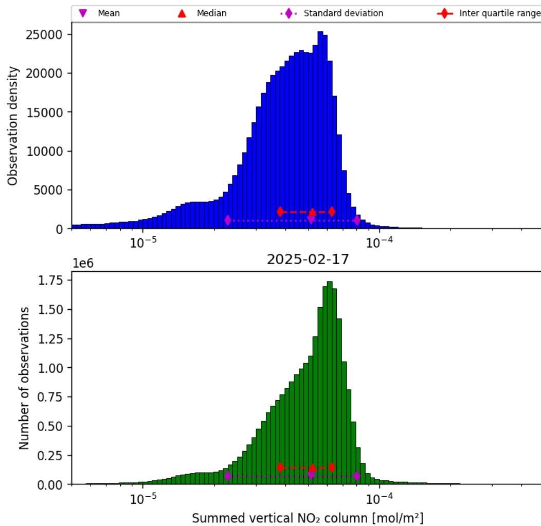
Figure 38: Histogram of "Summed vertical NO 2 column" for 2025-02-17 to 2025-02-18
