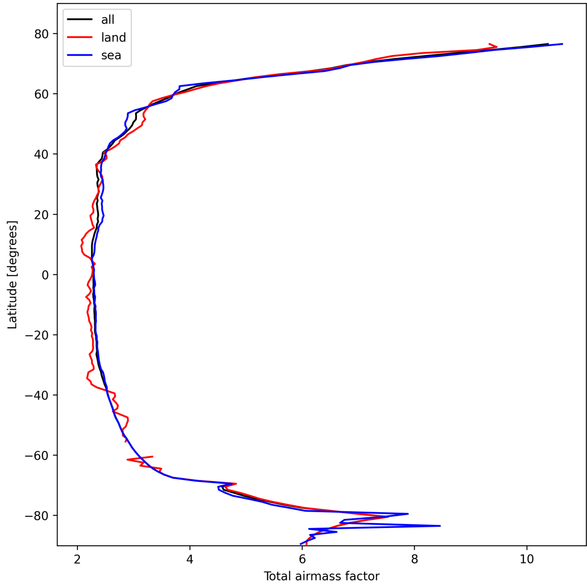
Figure 13: Zonal average of “Total airmass factor” for 2025-02-17 to 2025-02-18.
