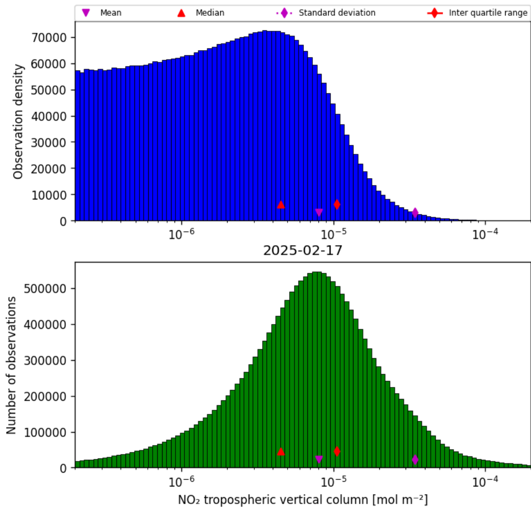
Figure 27: Histogram of “NO 2 tropospheric vertical column” for 2025-02-17 to 2025-02-18
