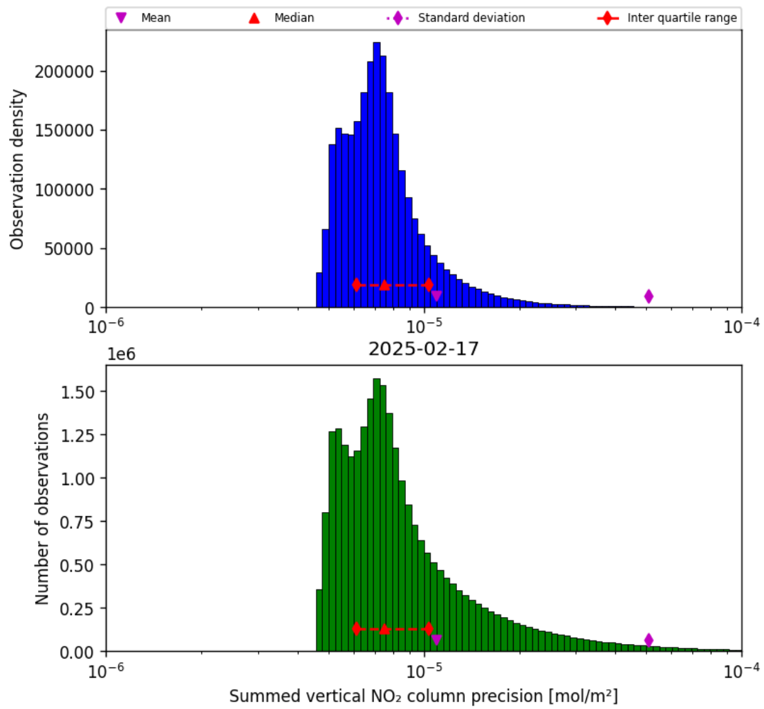
Figure 39: Histogram of "Summed vertical NO 2 column precision" for 2025-02-17 to 2025-02-18
