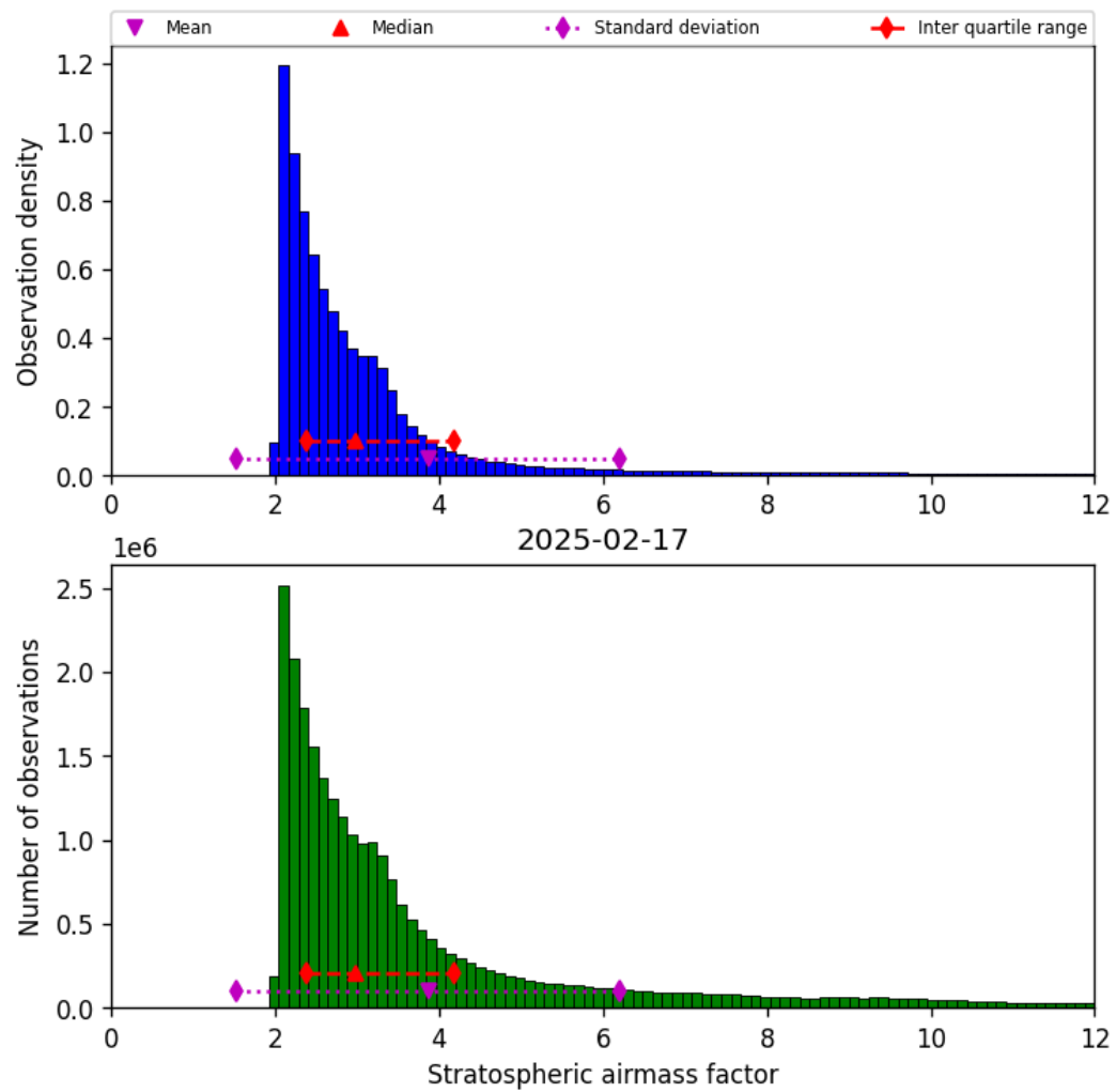
Figure 42: Histogram of “Stratospheric airmass factor” for 2025-02-17 to 2025-02-18
