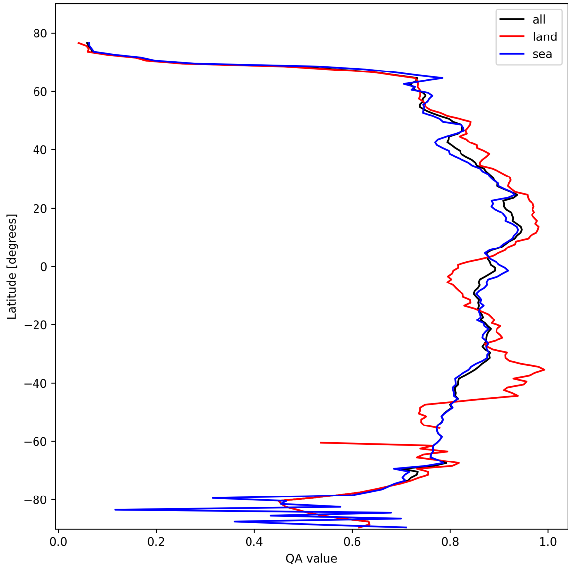
Figure 9: Zonal average of “QA value” for 2025-02-17 to 2025-02-18.
