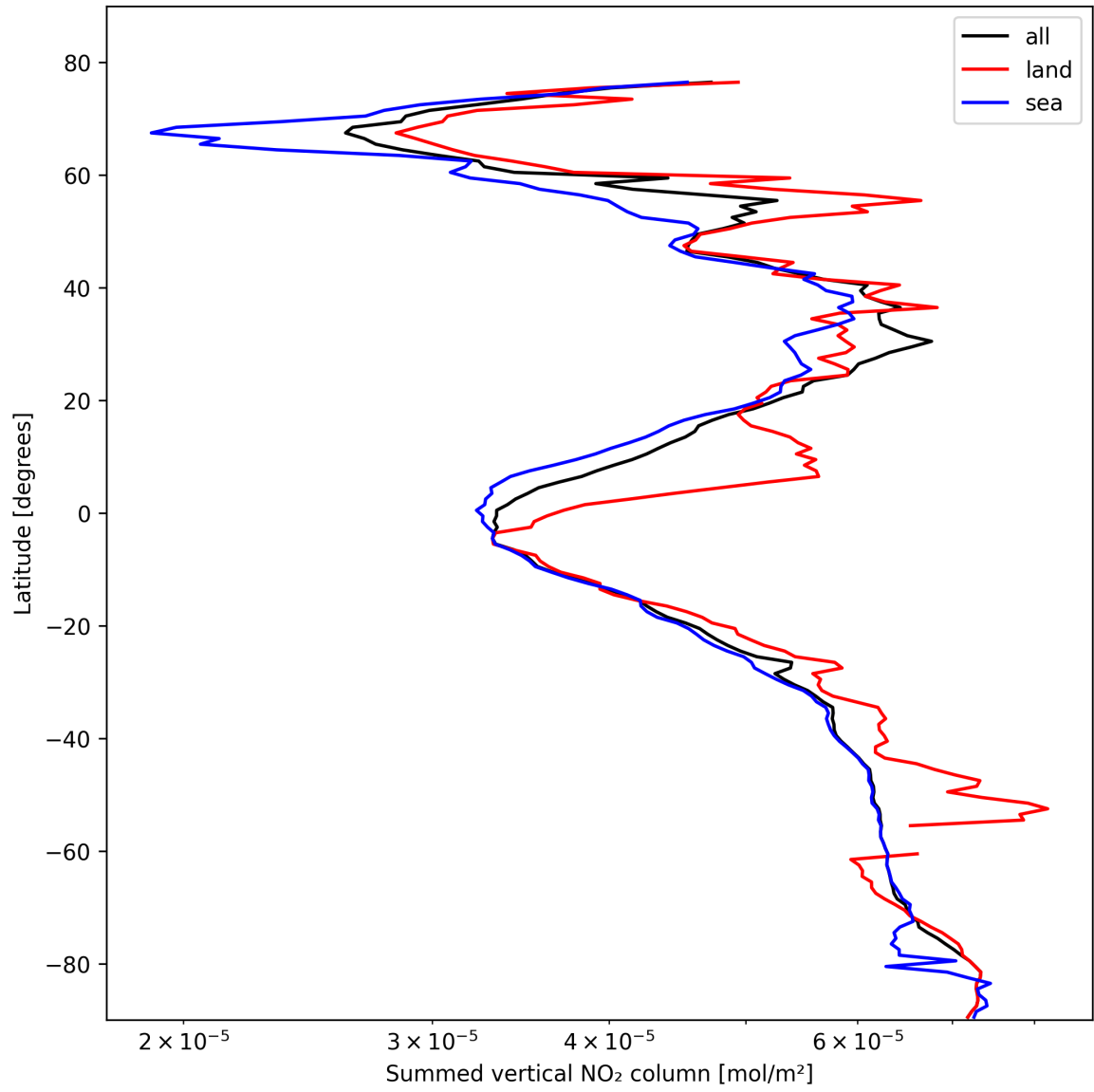
Figure 21: Zonal average of “Summed vertical NO 2 column” for 2025-02-17 to 2025-02-18.
