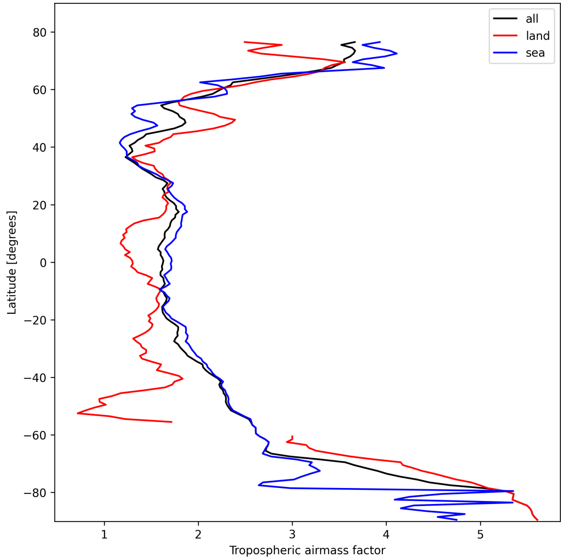
Figure 12: Zonal average of “Tropospheric airmass factor” for 2025-02-17 to 2025-02-18.
