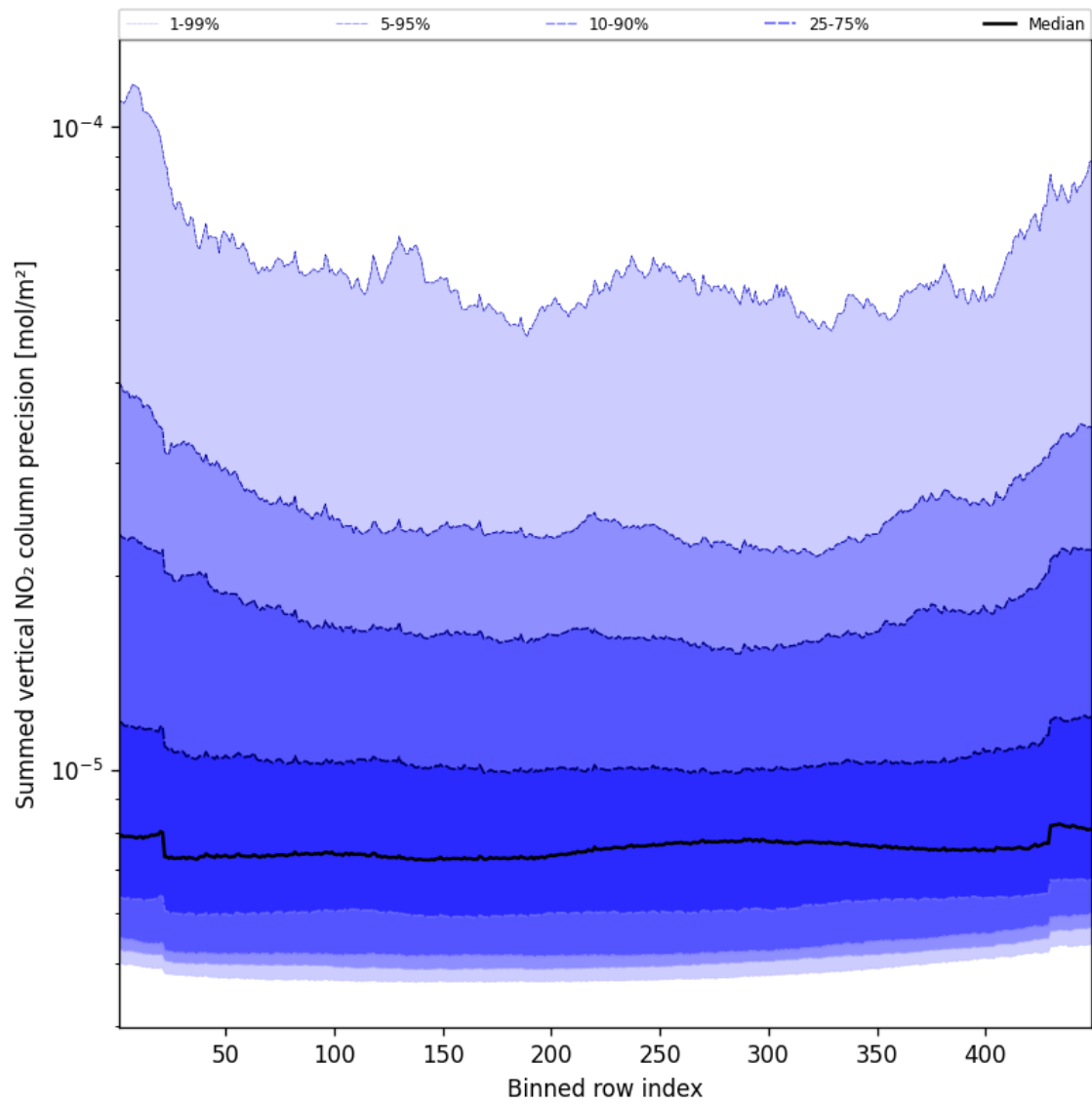
Figure 56: Along track statistics of “Summed vertical NO 2 column precision” for 2025-02-17 to 2025-02-18
