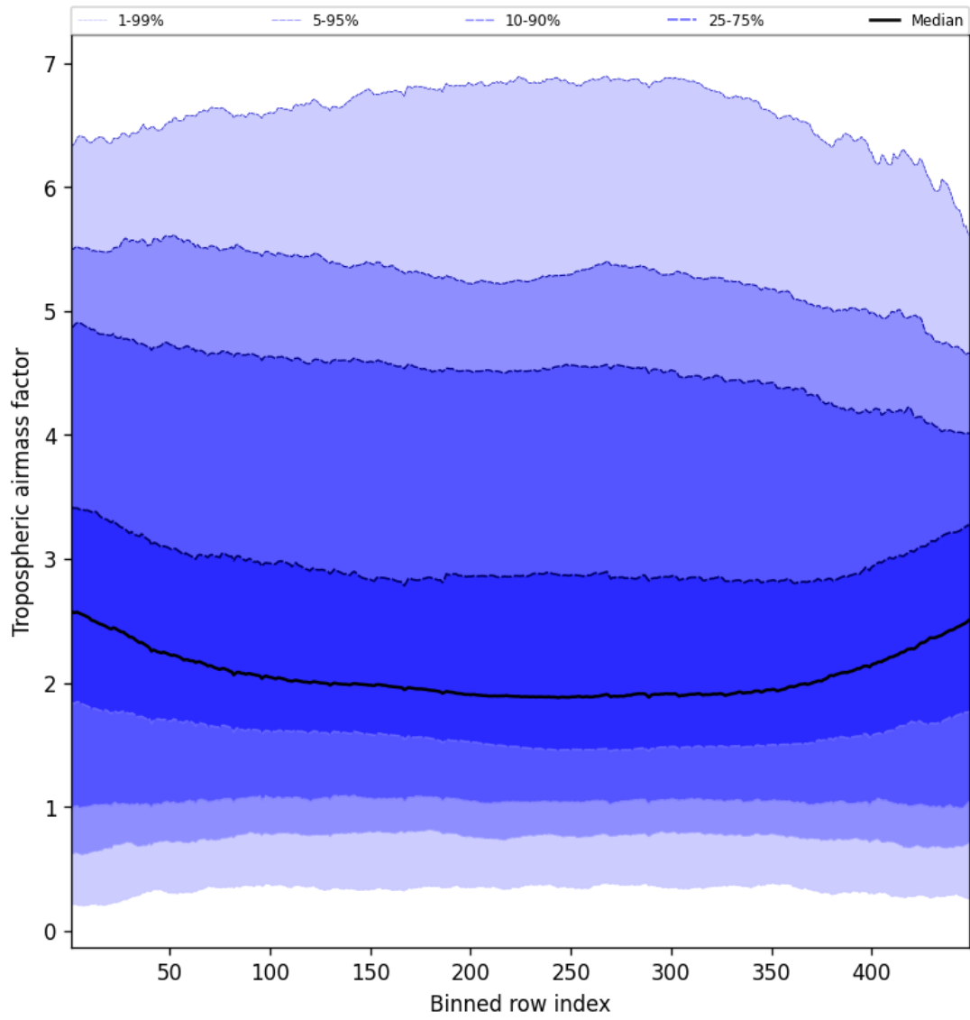
Figure 46: Along track statistics of “Tropospheric airmass factor” for 2025-02-17 to 2025-02-18
