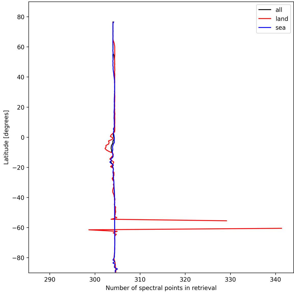
Figure 14: Zonal average of “Number of spectral points in retrieval” for 2025-02-17 to 2025-02-18.
