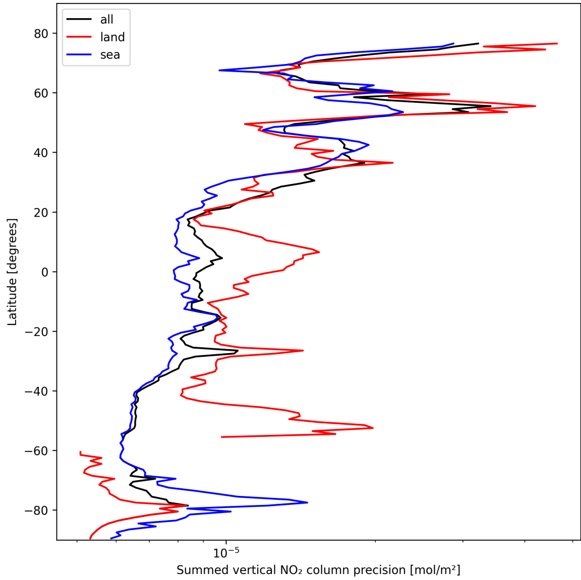
Figure 22: Zonal average of “Summed vertical NO 2 column precision” for 2025-02-17 to 2025-02-18.
