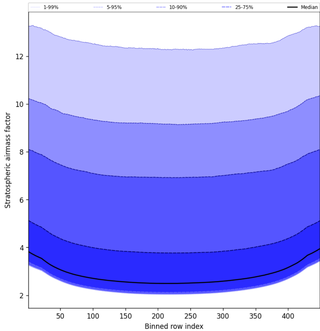
Figure 59: Along track statistics of “Stratospheric airmass factor” for 2025-02-17 to 2025-02-18
