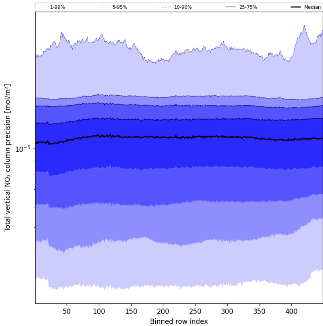
Figure 54: Along track statistics of “Total vertical NO 2 column precision” for 2025-02-17 to 2025-02-18
