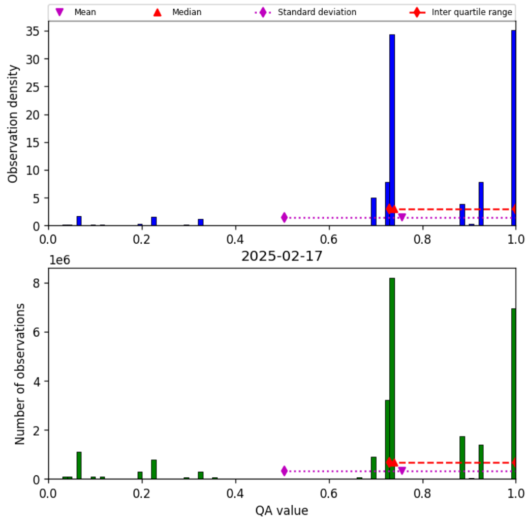
Figure 26: Histogram of “QA value” for 2025-02-17 to 2025-02-18
