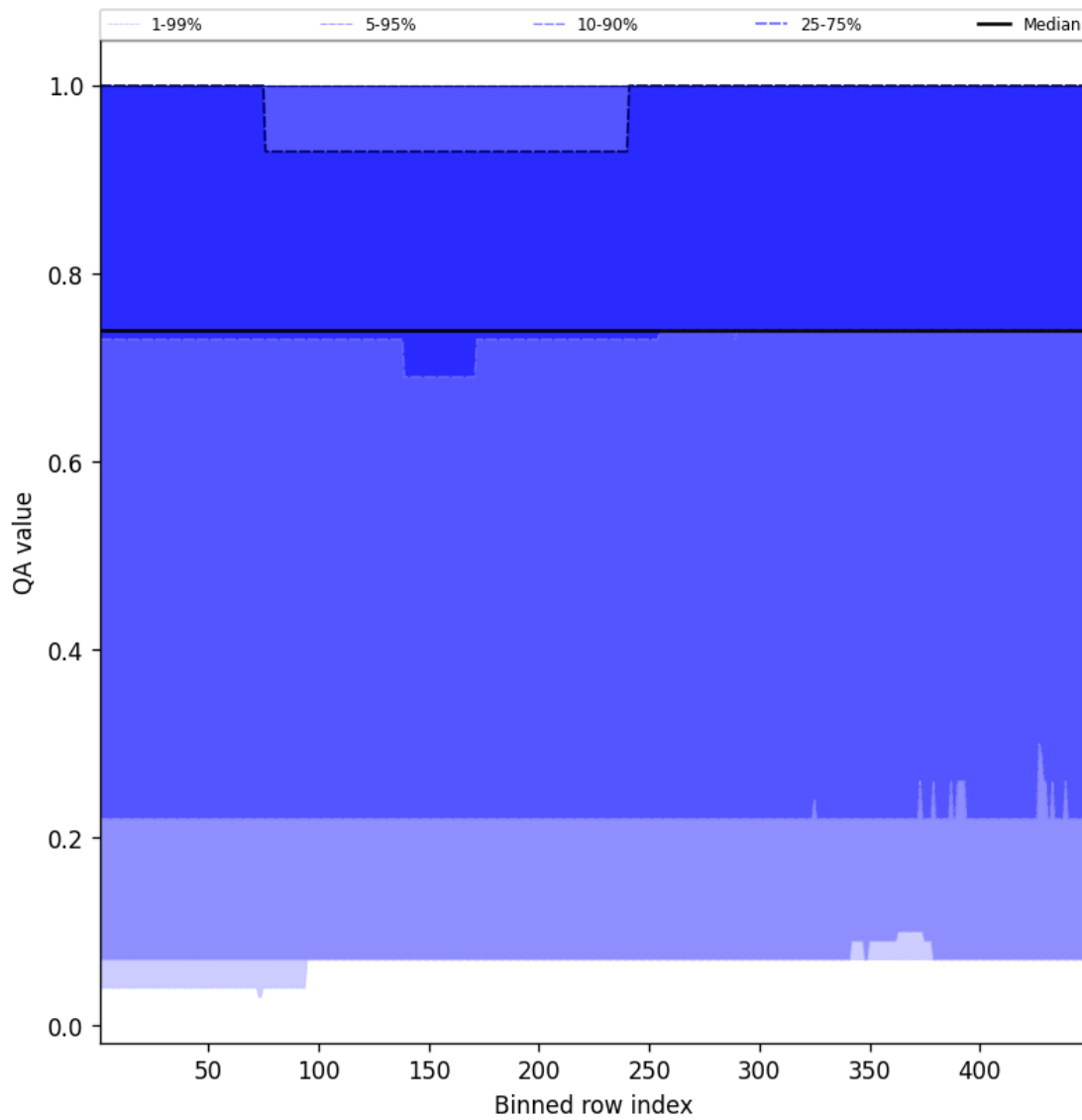
Figure 43: Along track statistics of “QA value” for 2025-02-17 to 2025-02-18
