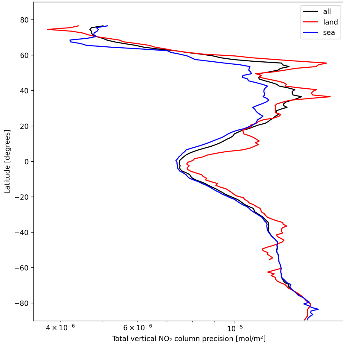
Figure 20: Zonal average of “Total vertical NO 2 column precision” for 2025-02-17 to 2025-02-18.
