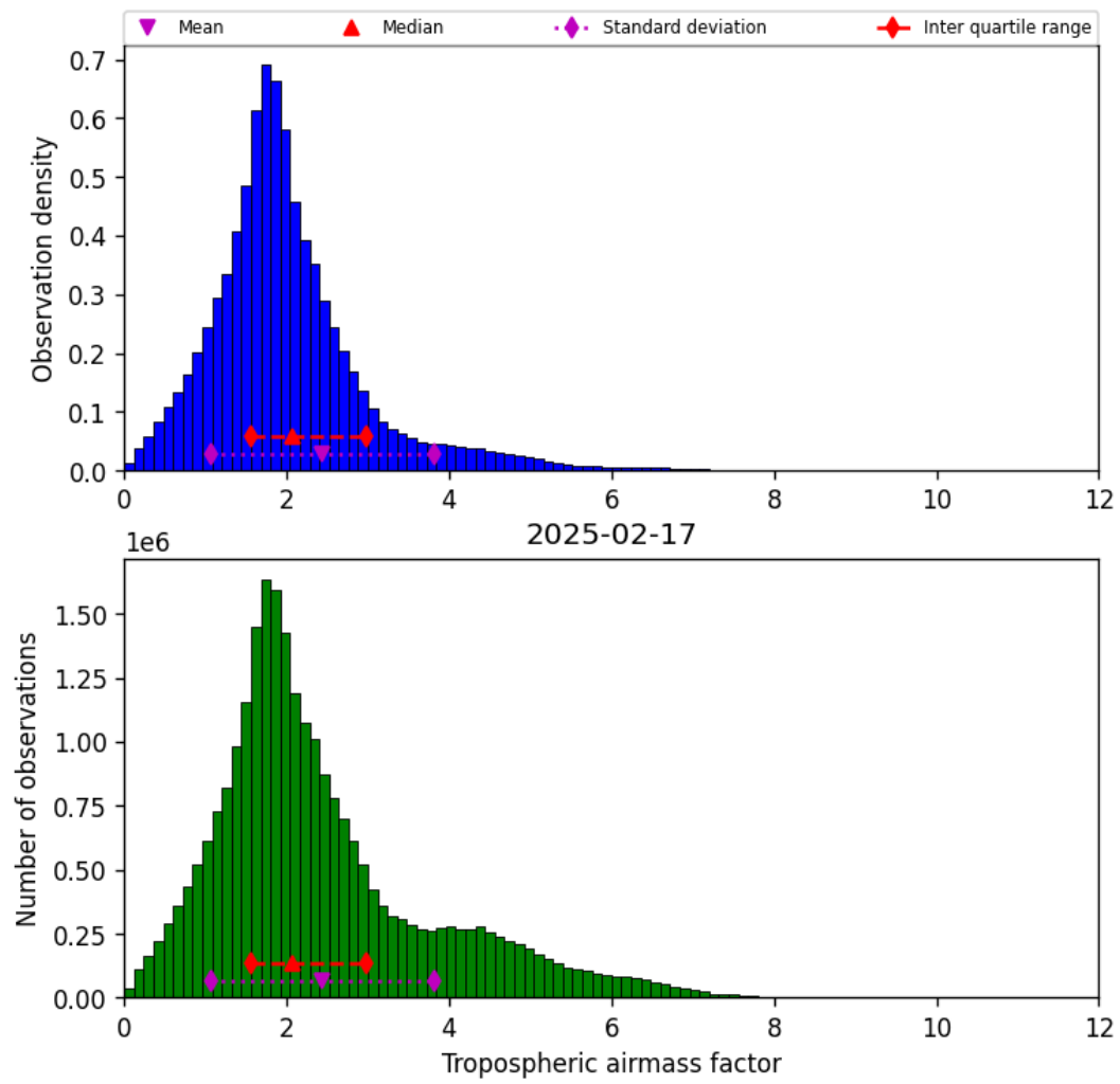
Figure 29: Histogram of “Tropospheric airmass factor” for 2025-02-17 to 2025-02-18
