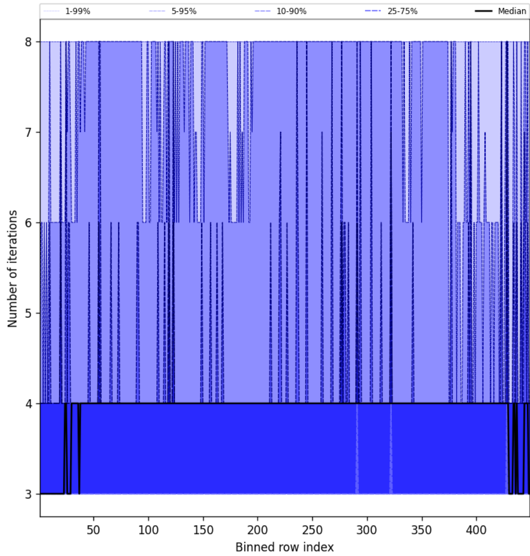
Figure 49: Along track statistics of “Number of iterations” for 2025-02-17 to 2025-02-18
