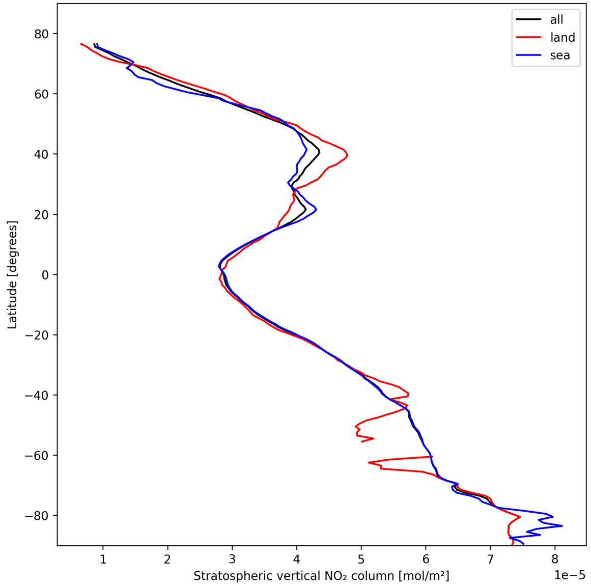
Figure 17: Zonal average of “Stratospheric vertical NO 2 column” for 2025-02-17 to 2025-02-18.
