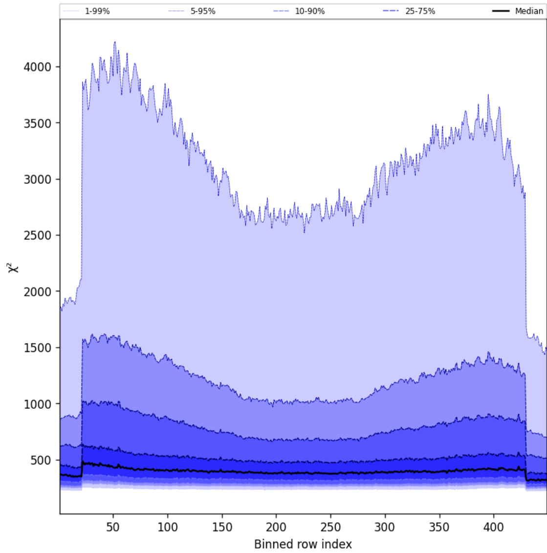
Figure 57: Along track statistics of “ \chi^2 ” for 2025-02-17 to 2025-02-18
