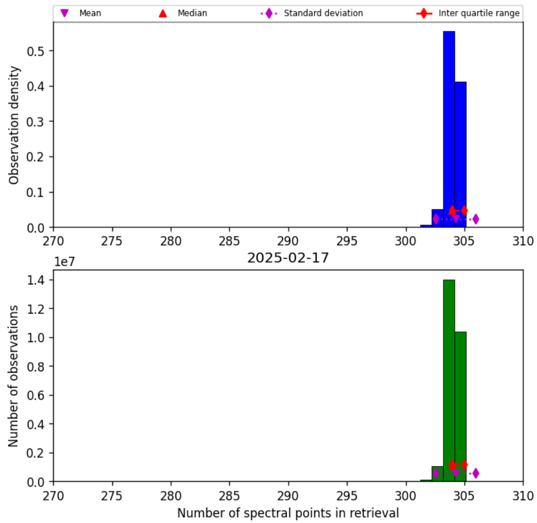
Figure 31: Histogram of “Number of spectral points in retrieval” for 2025-02-17 to 2025-02-18
