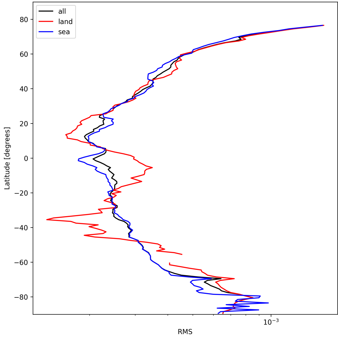
Figure 24: Zonal average of “RMS” for 2025-02-17 to 2025-02-18.
