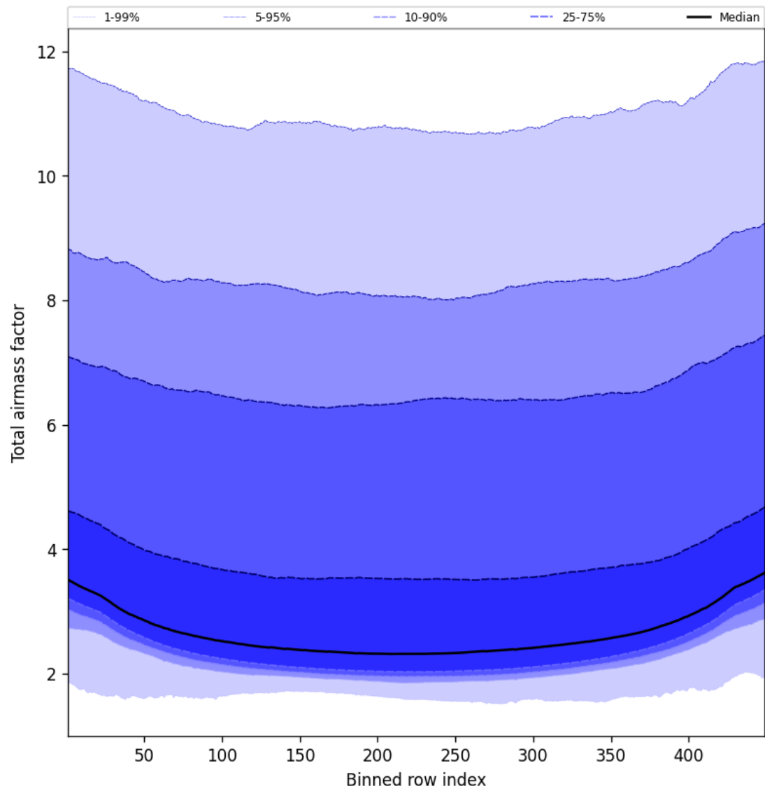
Figure 47: Along track statistics of “Total airmass factor” for 2025-02-17 to 2025-02-18
