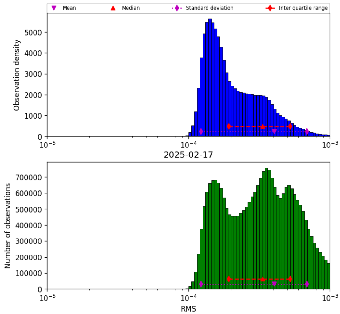
Figure 41: Histogram of “RMS” for 2025-02-17 to 2025-02-18
