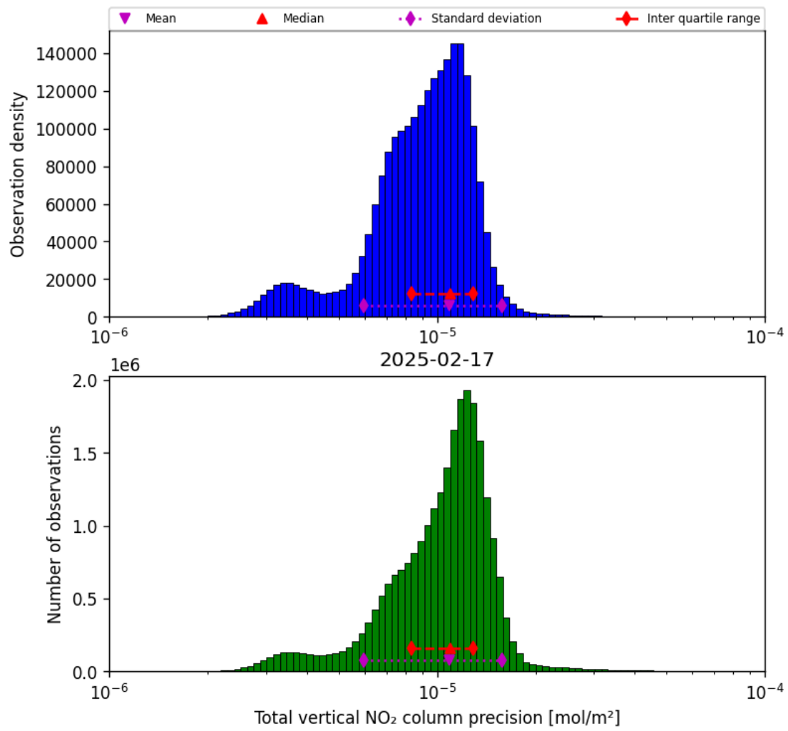
Figure 37: Histogram of “Total vertical NO 2 column precision” for 2025-02-17 to 2025-02-18
