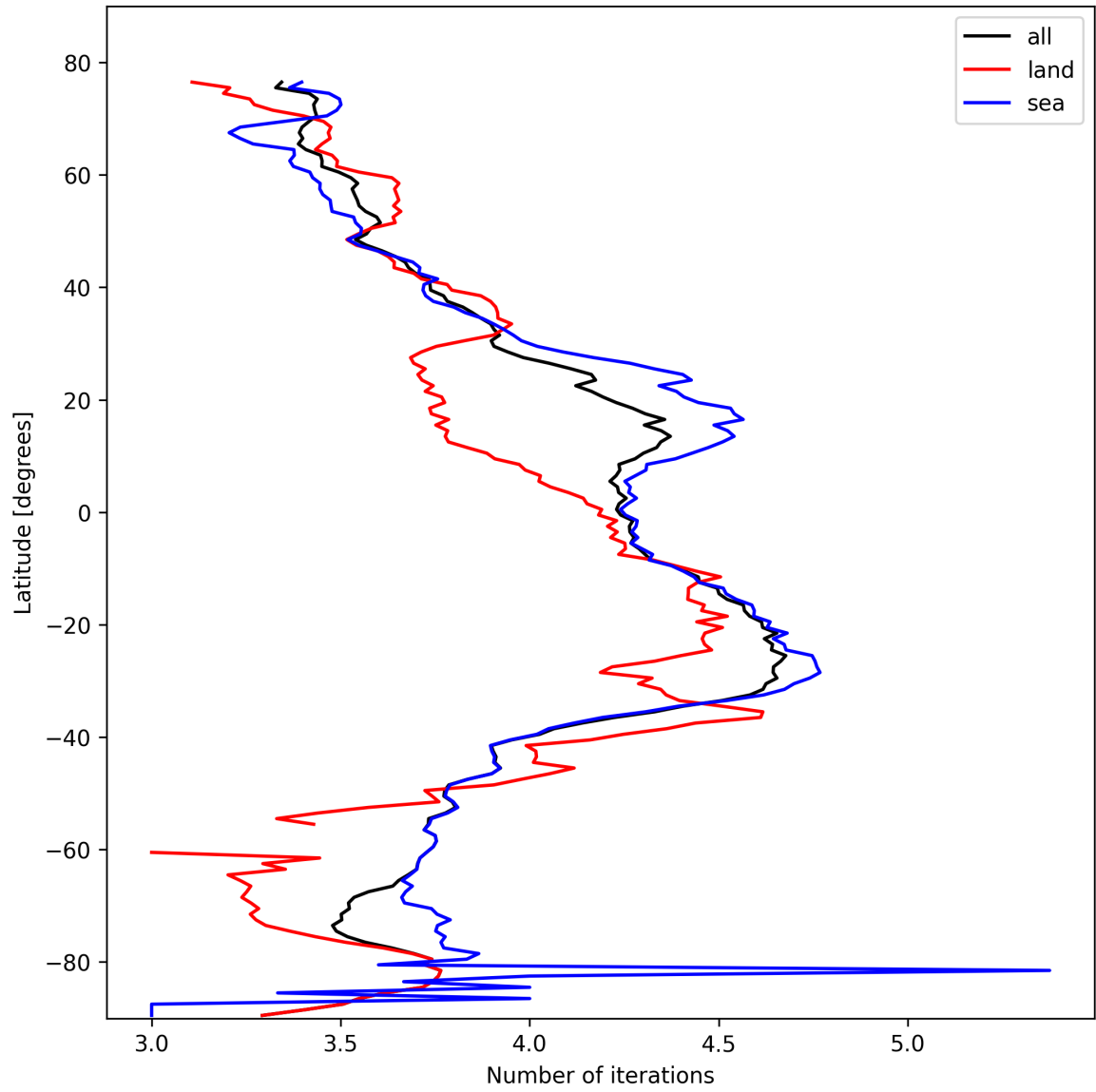
Figure 15: Zonal average of “Number of iterations” for 2025-02-17 to 2025-02-18.
