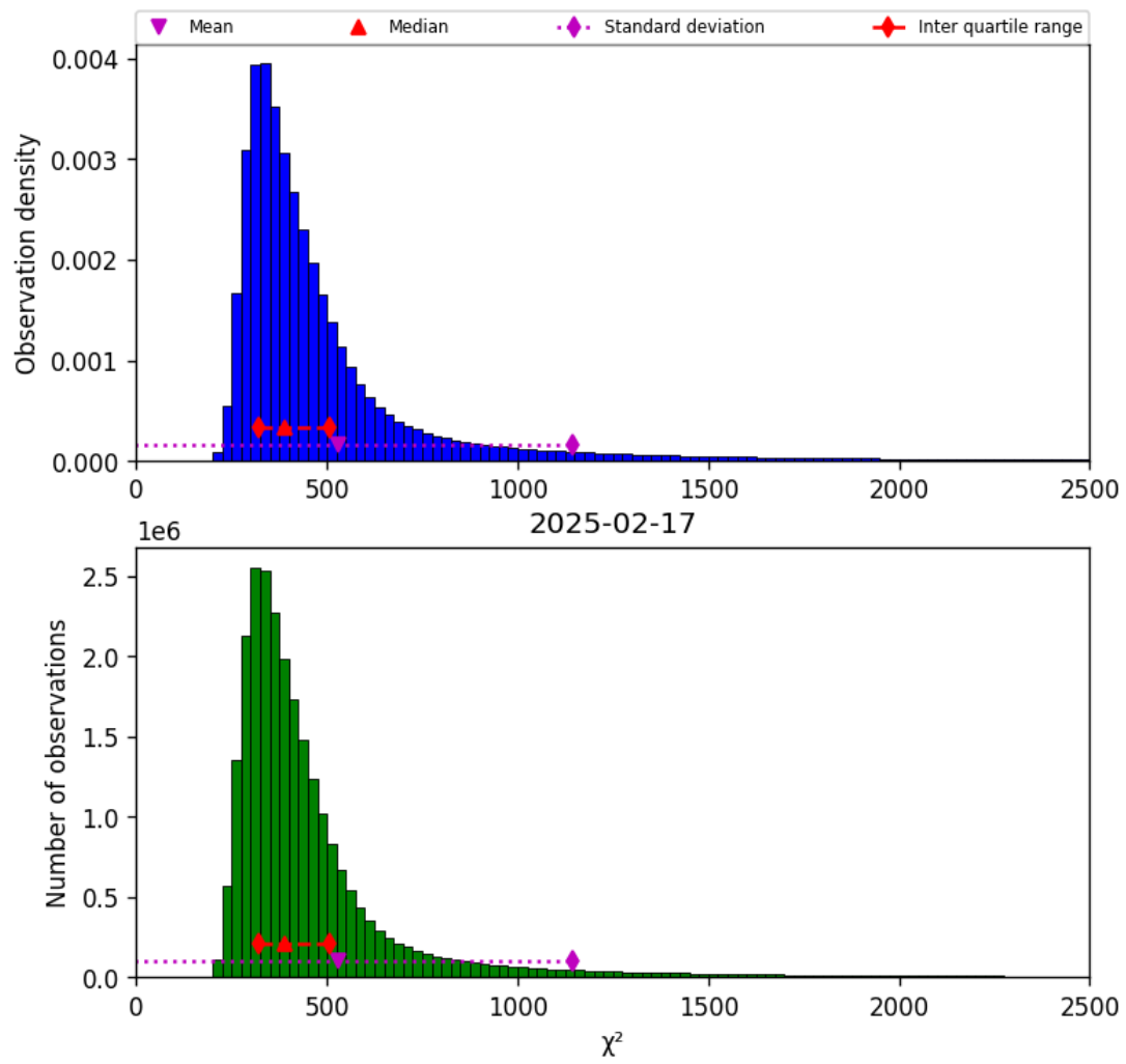
Figure 40: Histogram of “ \chi^2 ” for 2025-02-17 to 2025-02-18
