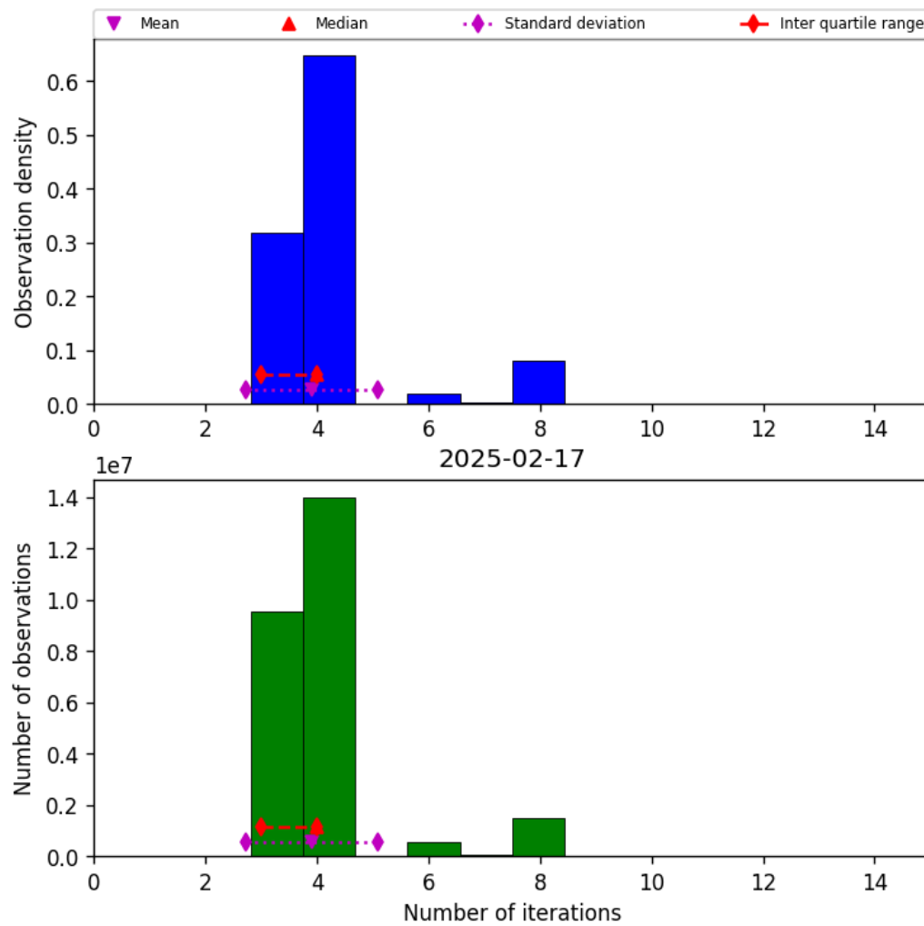
Figure 32: Histogram of “Number of iterations” for 2025-02-17 to 2025-02-18
