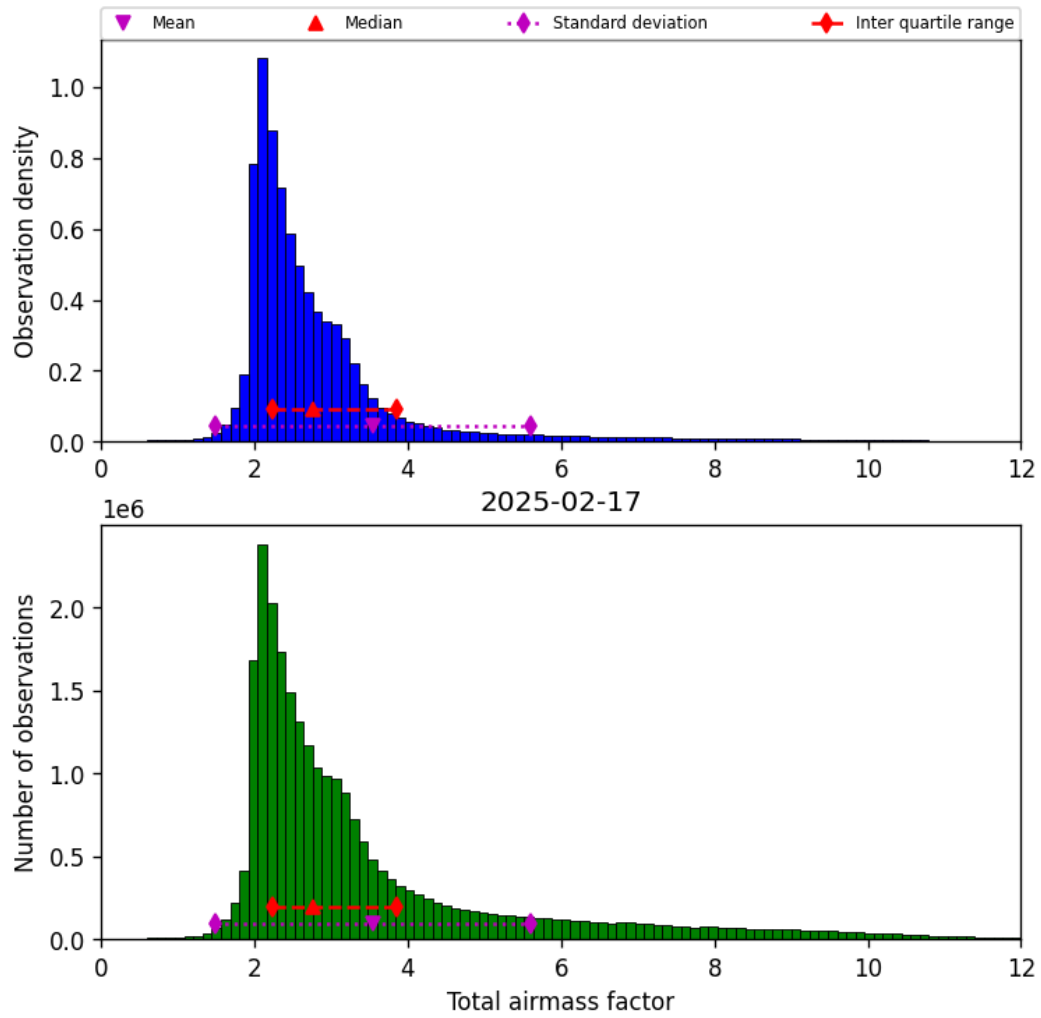
Figure 30: Histogram of “Total airmass factor” for 2025-02-17 to 2025-02-18
