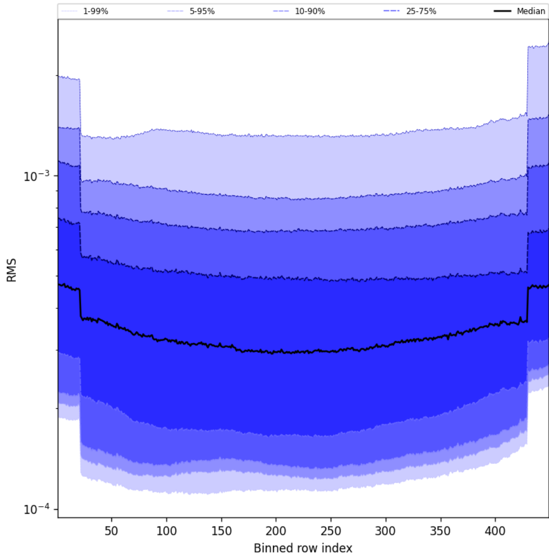
Figure 58: Along track statistics of “RMS” for 2025-02-17 to 2025-02-18
