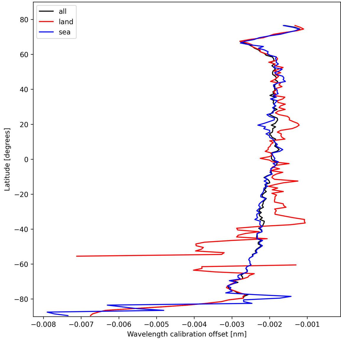
Figure 16: Zonal average of “Wavelength calibration offset” for 2025-02-17 to 2025-02-18.
