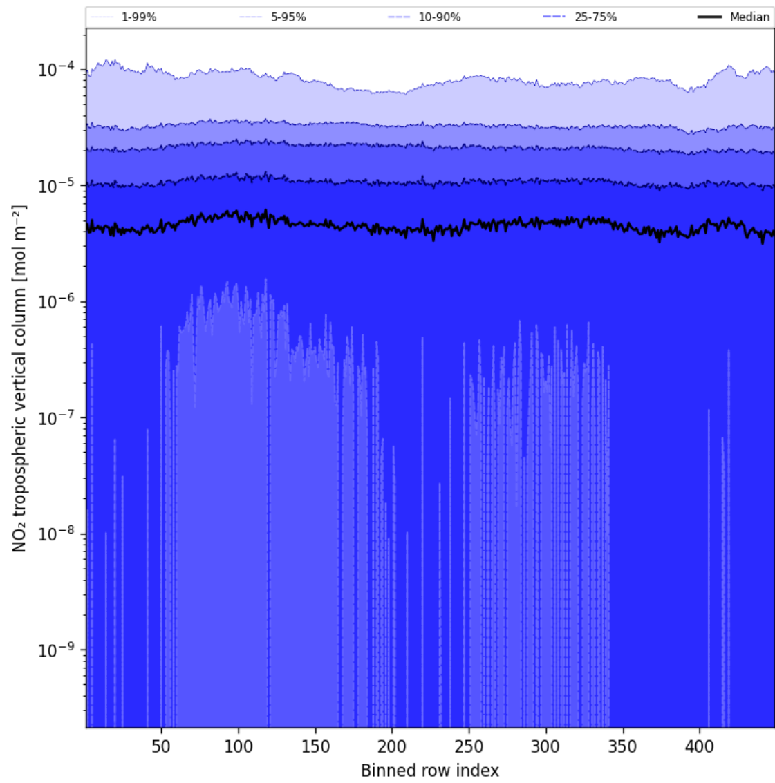
Figure 44: Along track statistics of “NO 2 tropospheric vertical column” for 2025-02-17 to 2025-02-18
