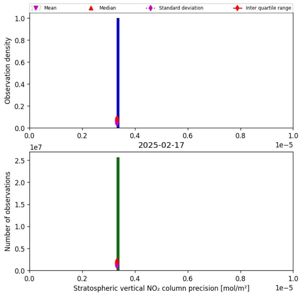
Figure 35: Histogram of “Stratospheric vertical NO 2 column precision” for 2025-02-17 to 2025-02-18
