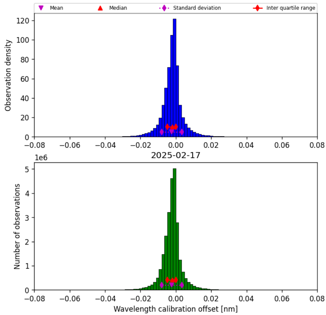
Figure 33: Histogram of “Wavelength calibration offset” for 2025-02-17 to 2025-02-18
