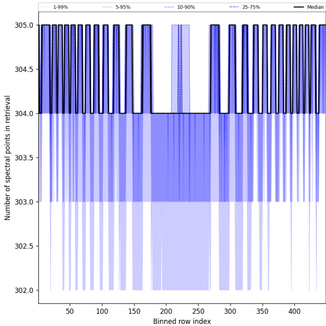
Figure 48: Along track statistics of “Number of spectral points in retrieval” for 2025-02-17 to 2025-02-18
