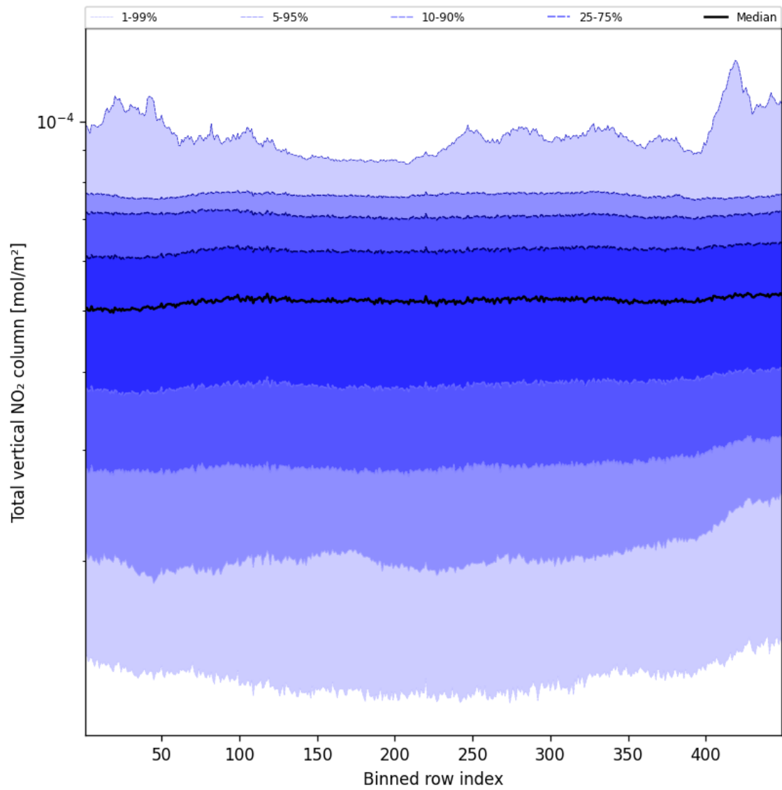
Figure 53: Along track statistics of “Total vertical NO 2 column” for 2025-02-17 to 2025-02-18
