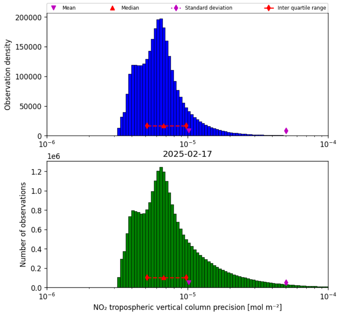
Figure 28: Histogram of “NO 2 tropospheric vertical column precision” for 2025-02-17 to 2025-02-18
