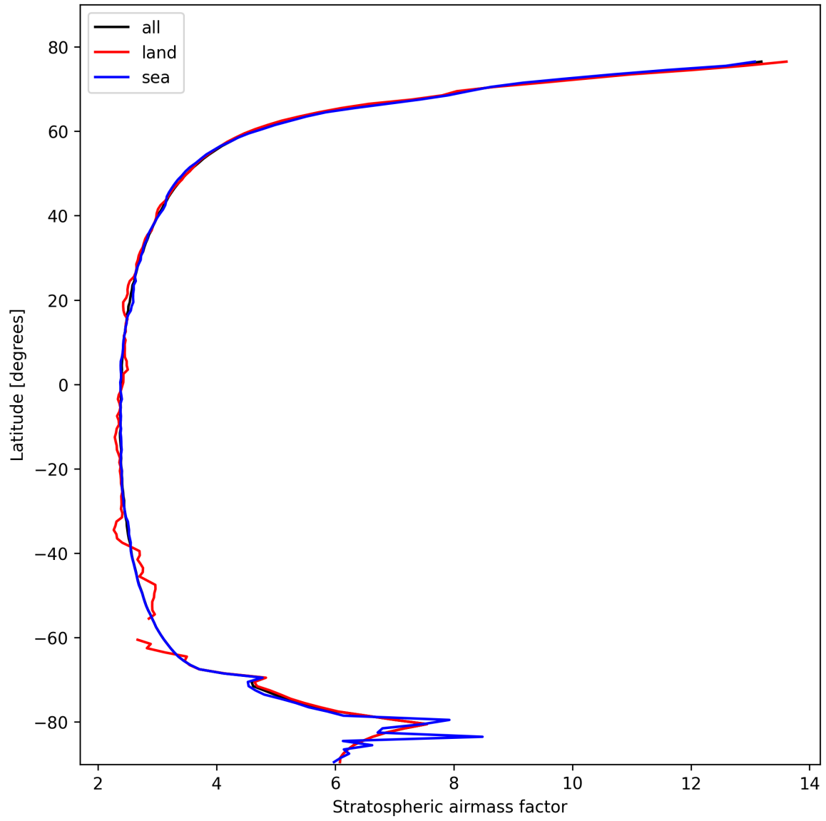
Figure 25: Zonal average of “Stratospheric air mass factor” for 2025-02-17 to 2025-02-18.
