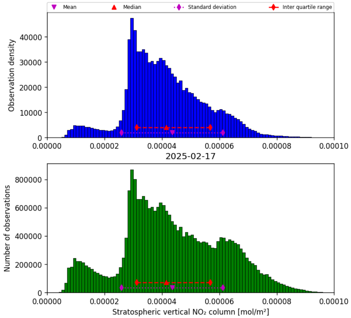
Figure 34: Histogram of “Stratospheric vertical NO 2 column” for 2025-02-17 to 2025-02-18
