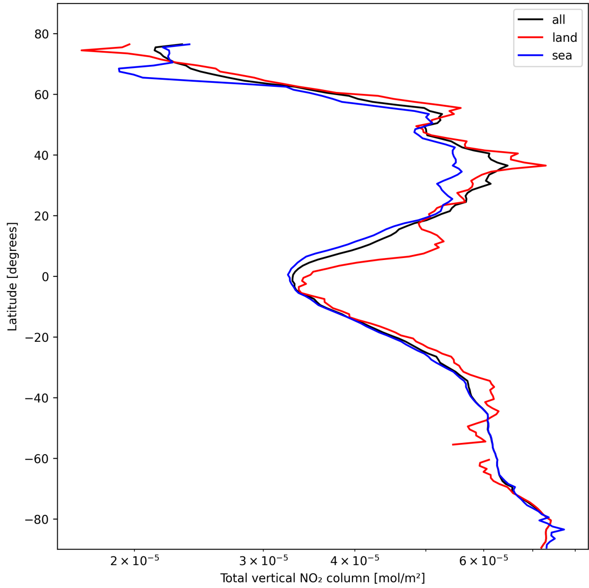
Figure 19: Zonal average of “Total vertical NO 2 column” for 2025-02-17 to 2025-02-18.
