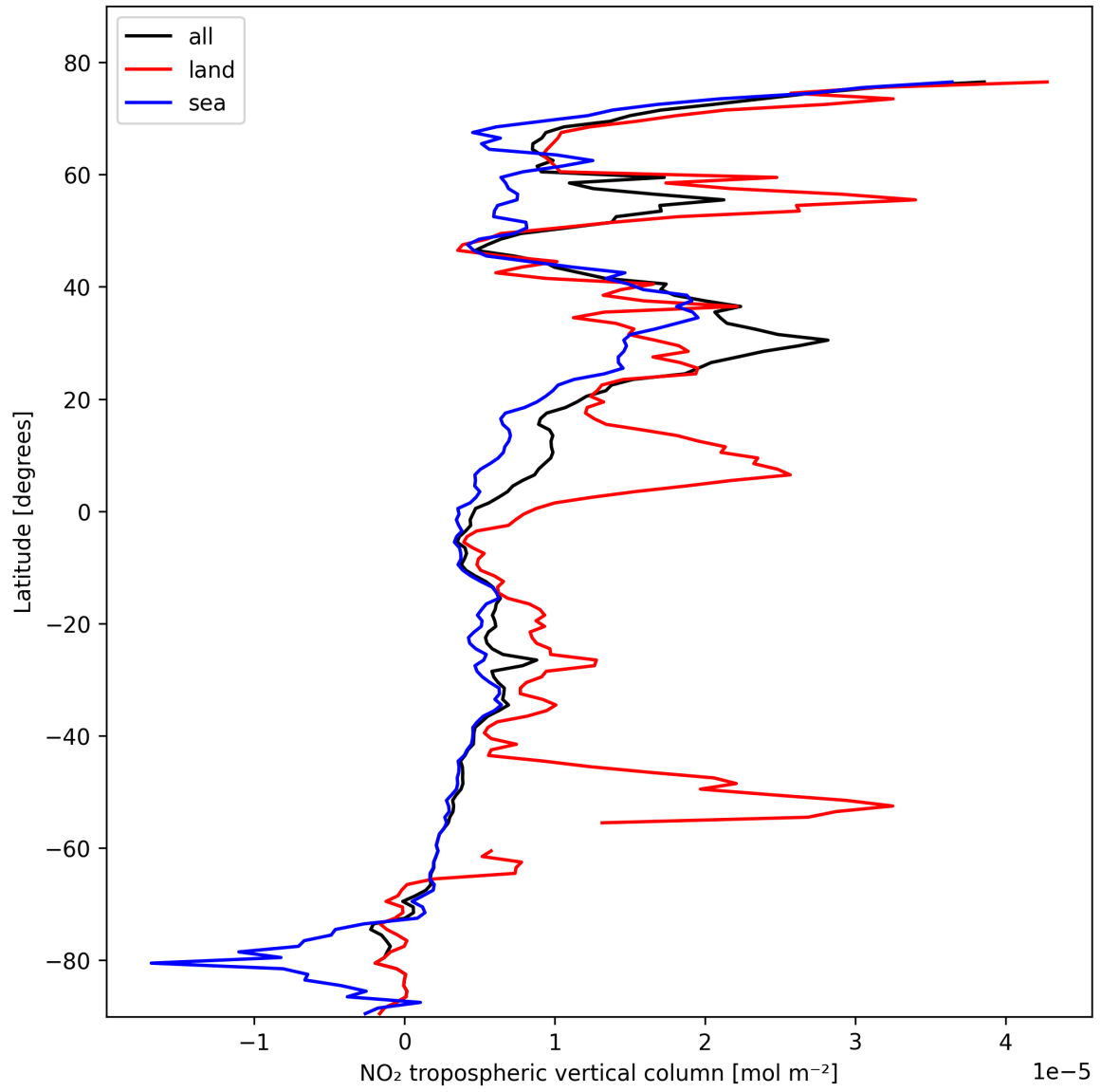
Figure 10: Zonal average of “NO 2 tropospheric vertical column” for 2025-02-17 to 2025-02-18.
