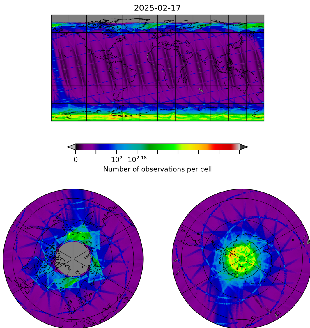
Figure 8: Map of the number of observations for 2025-02-17 to 2025-02-18
