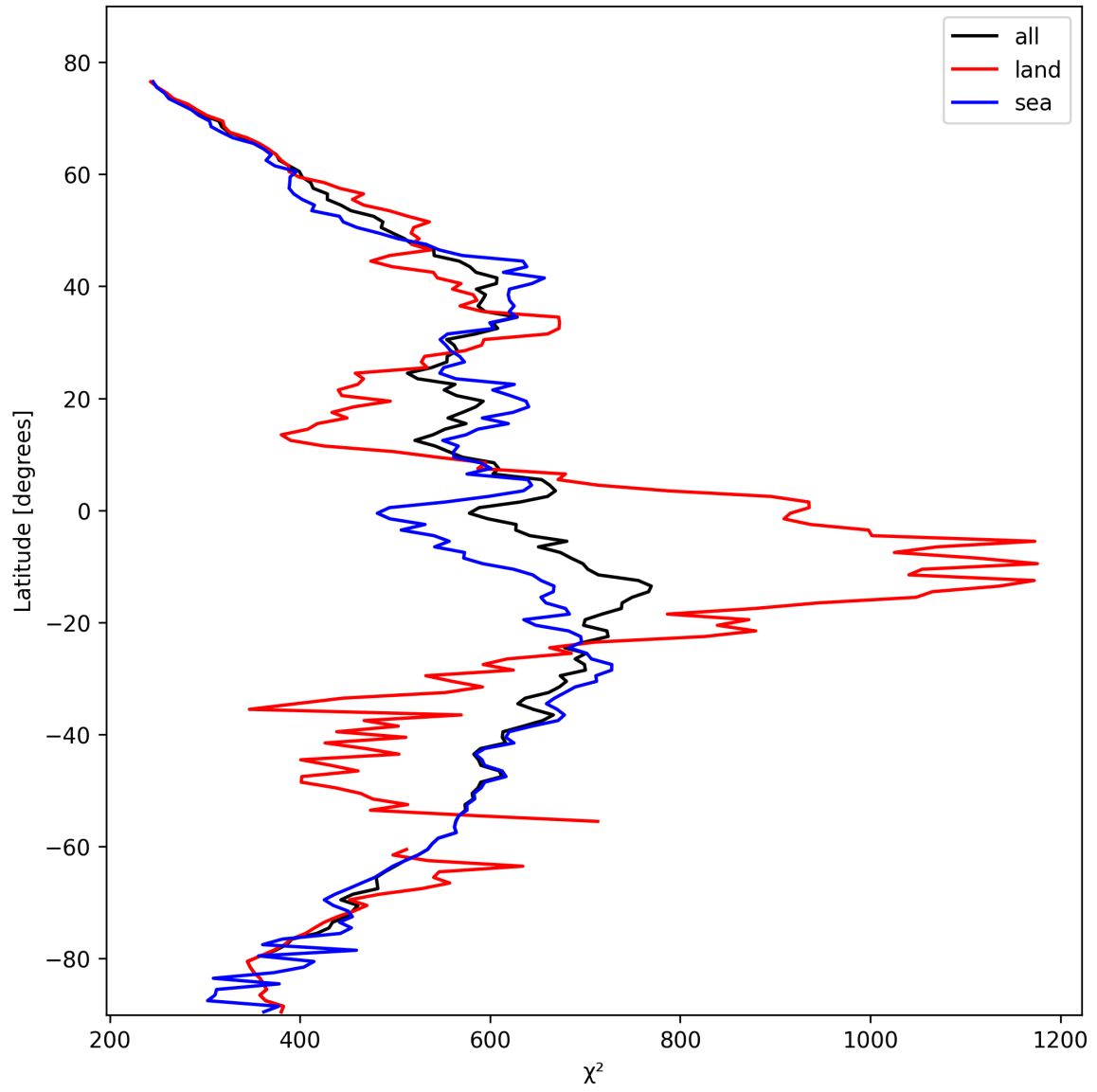
Figure 23: Zonal average of “ \chi^2 ” for 2025-02-17 to 2025-02-18.
