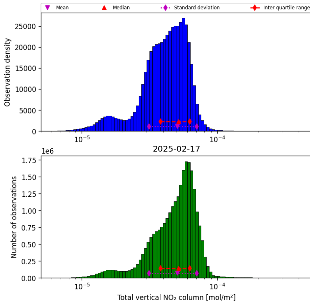
Figure 36: Histogram of “Total vertical NO 2 column” for 2025-02-17 to 2025-02-18
