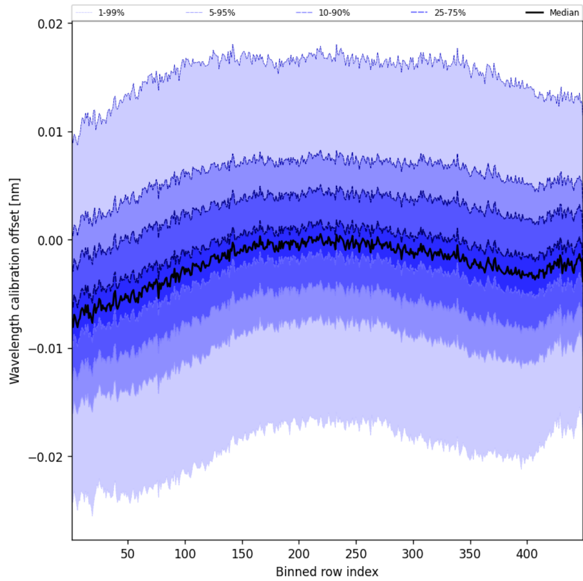
Figure 50: Along track statistics of “Wavelength calibration offset” for 2025-02-17 to 2025-02-18
