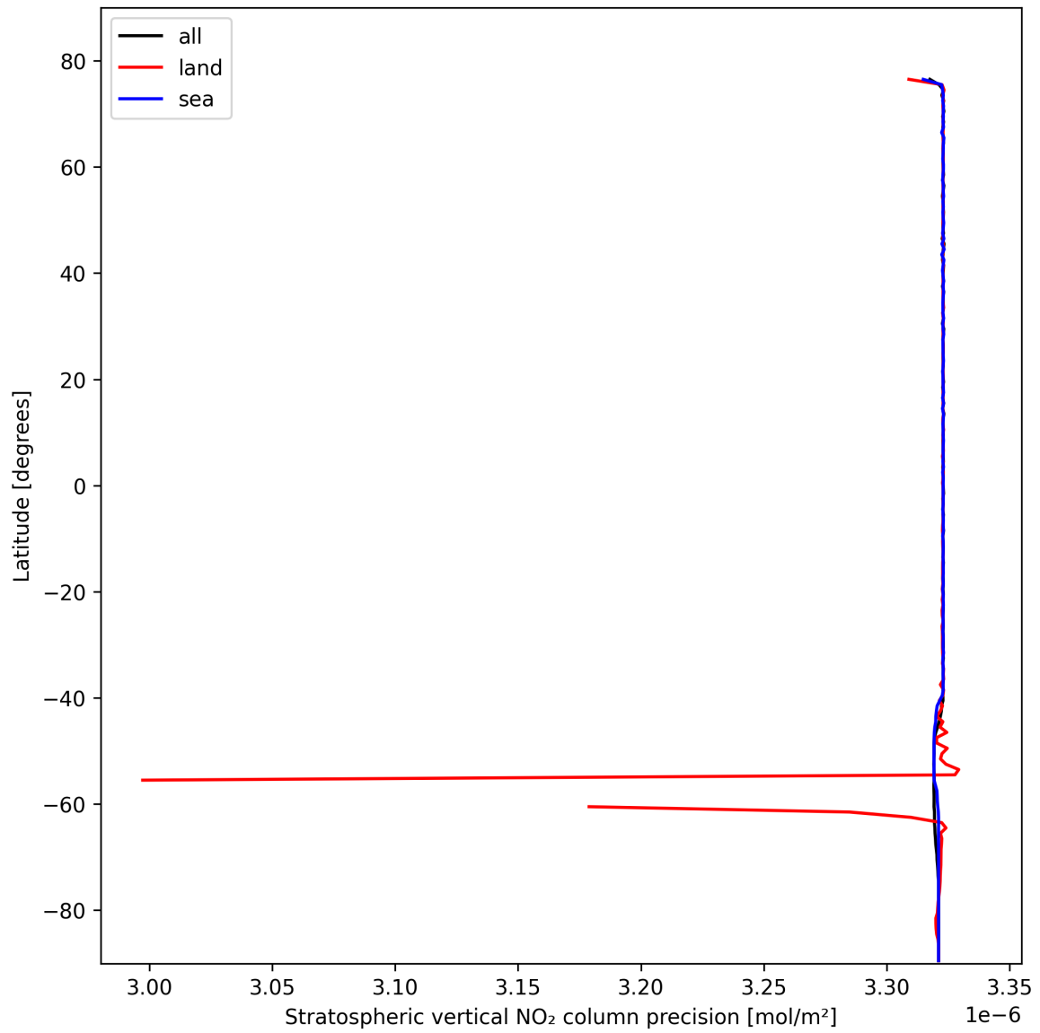
Figure 18: Zonal average of “Stratospheric vertical NO 2 column precision” for 2025-02-17 to 2025-02-18.
