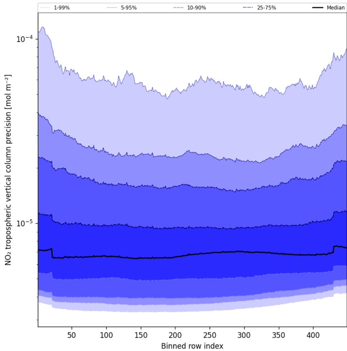
Figure 45: Along track statistics of “NO 2 tropospheric vertical column precision” for 2025-02-17 to 2025-02-18
