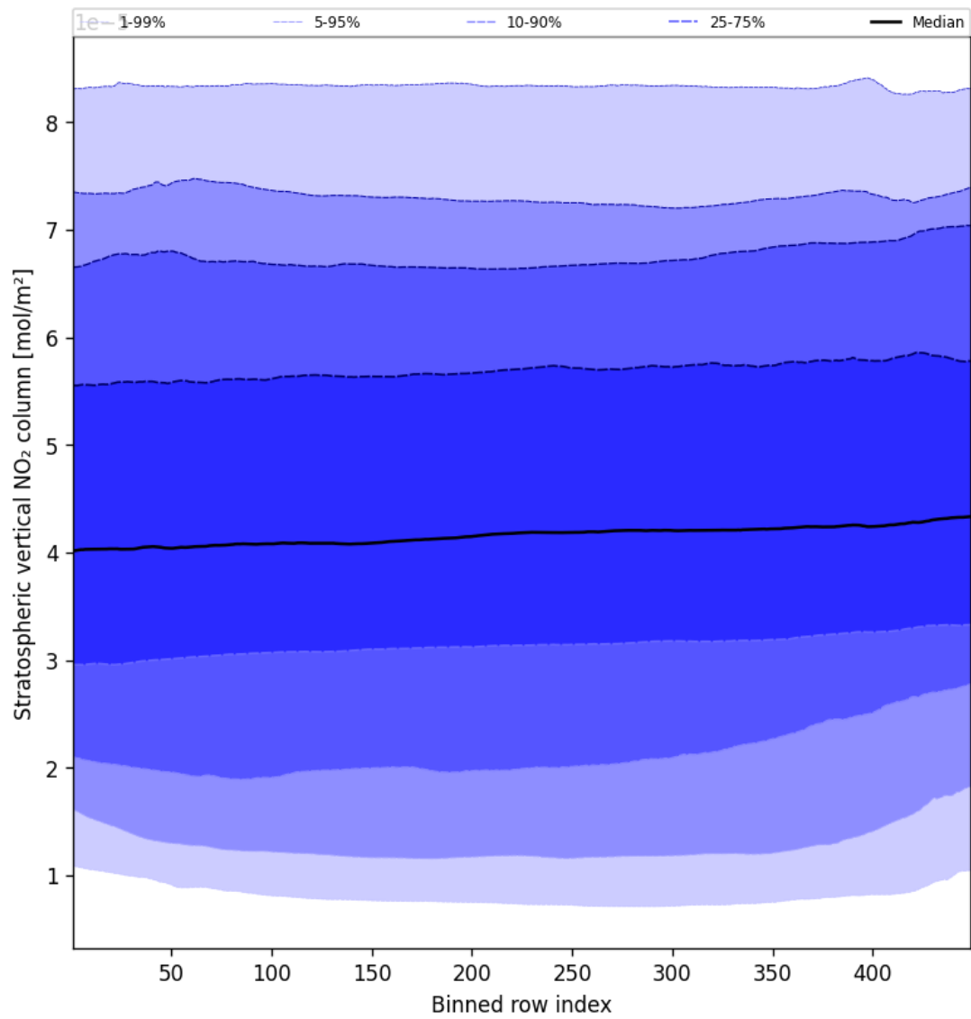
Figure 51: Along track statistics of “Stratospheric vertical NO 2 column” for 2025-02-17 to 2025-02-18
