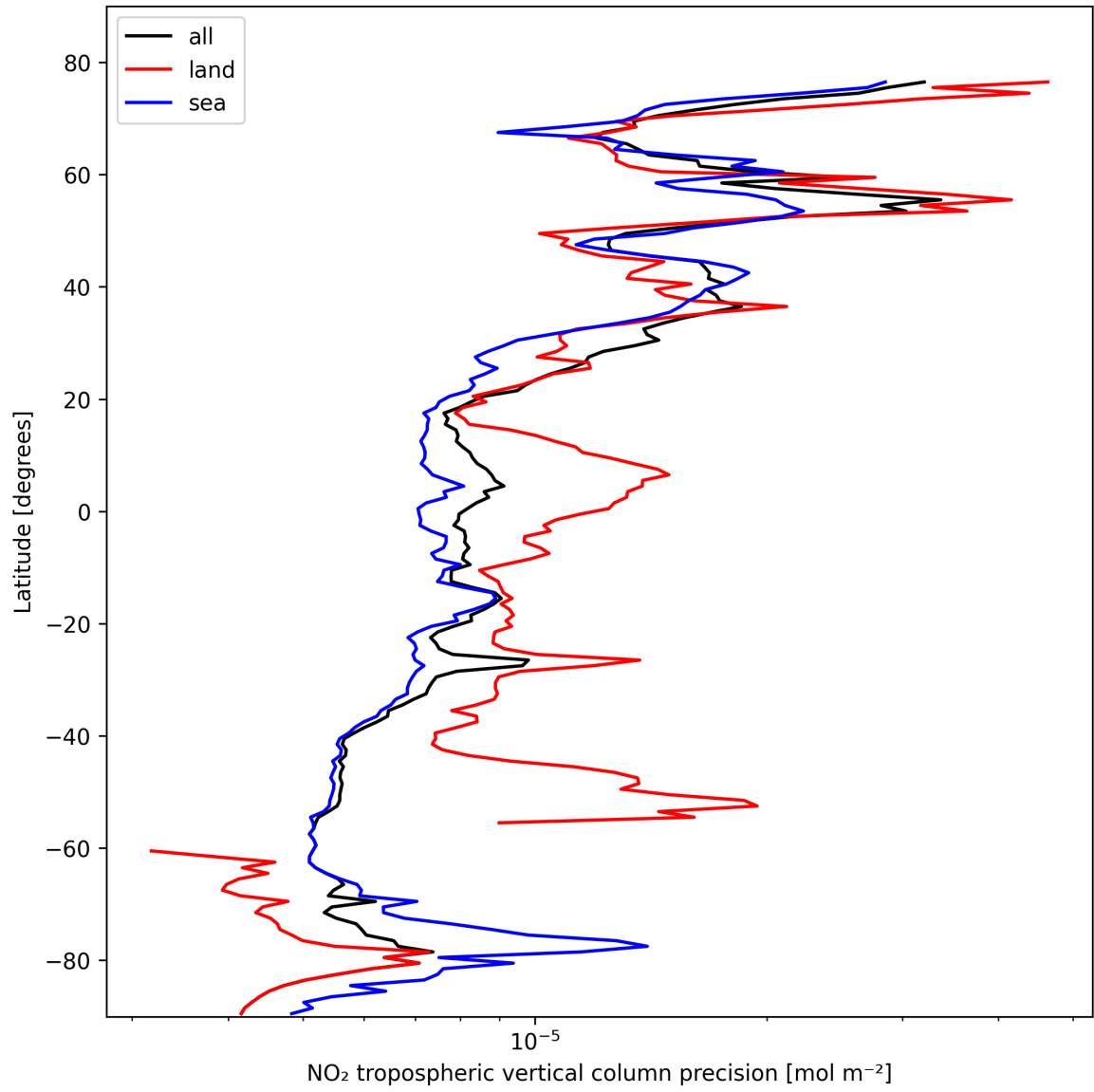
Figure 11: Zonal average of “NO 2 tropospheric vertical column precision” for 2025-02-17 to 2025-02-18.
