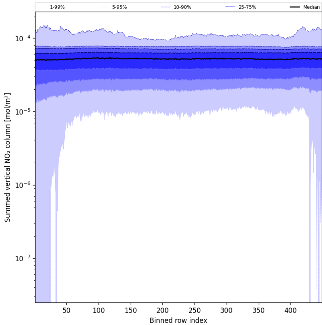
Figure 55: Along track statistics of “Summed vertical NO 2 column” for 2025-02-17 to 2025-02-18
