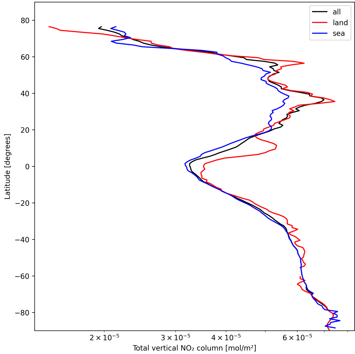
Figure 19: Zonal average of “Total vertical NO 2 column” for 2025-02-18 to 2025-02-19.
