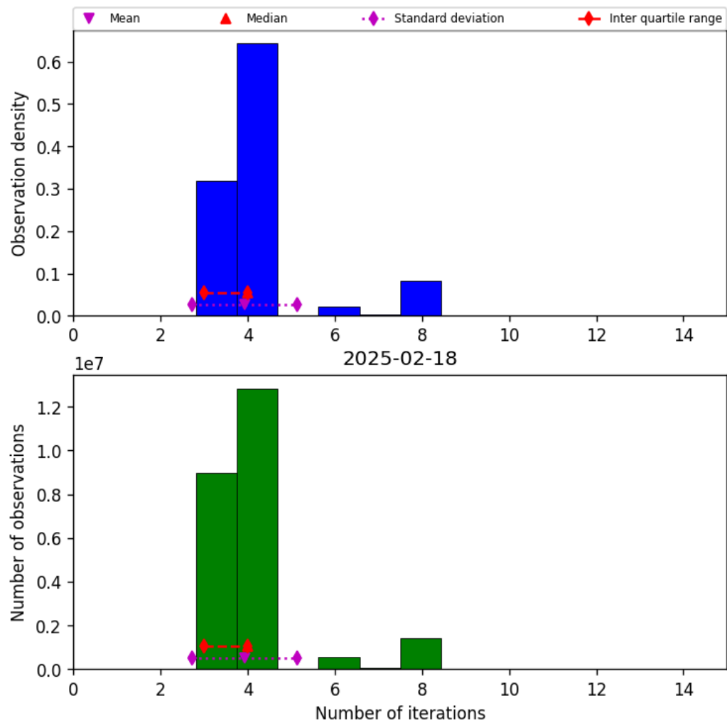
Figure 32: Histogram of “Number of iterations” for 2025-02-18 to 2025-02-19
