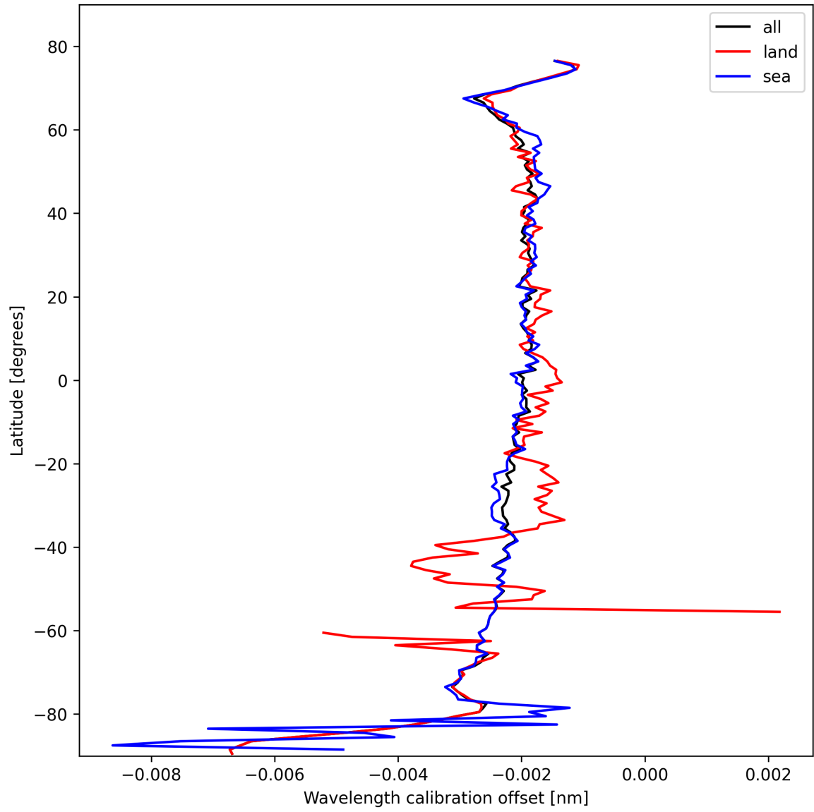
Figure 16: Zonal average of “Wavelength calibration offset” for 2025-02-18 to 2025-02-19.
