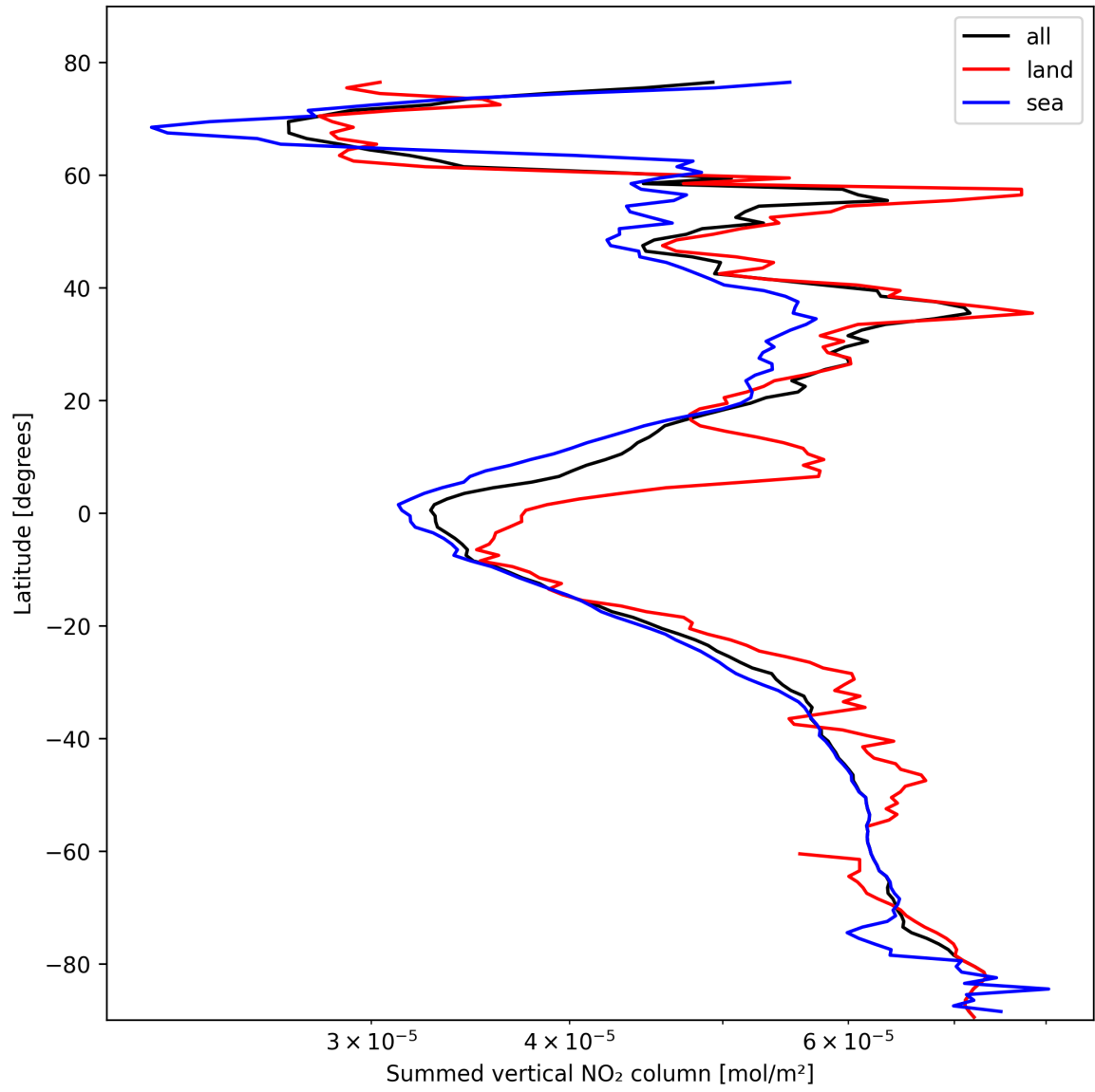
Figure 21: Zonal average of “Summed vertical NO 2 column” for 2025-02-18 to 2025-02-19.
