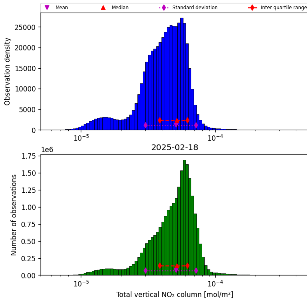
Figure 36: Histogram of “Total vertical NO 2 column” for 2025-02-18 to 2025-02-19
