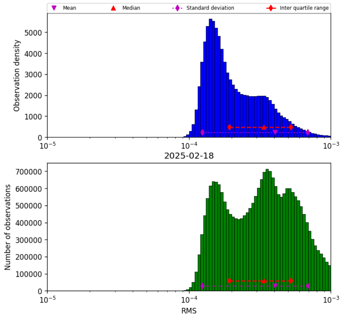
Figure 41: Histogram of “RMS” for 2025-02-18 to 2025-02-19
