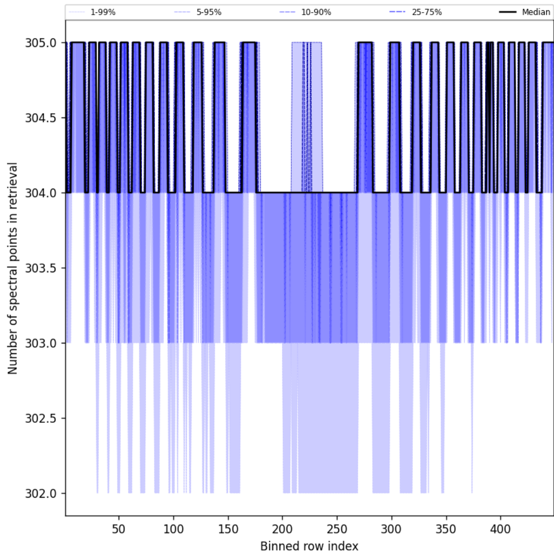
Figure 48: Along track statistics of “Number of spectral points in retrieval” for 2025-02-18 to 2025-02-19
