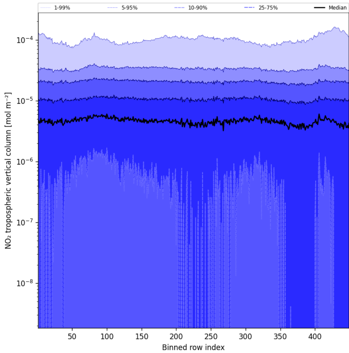
Figure 44: Along track statistics of “NO 2 tropospheric vertical column” for 2025-02-18 to 2025-02-19
