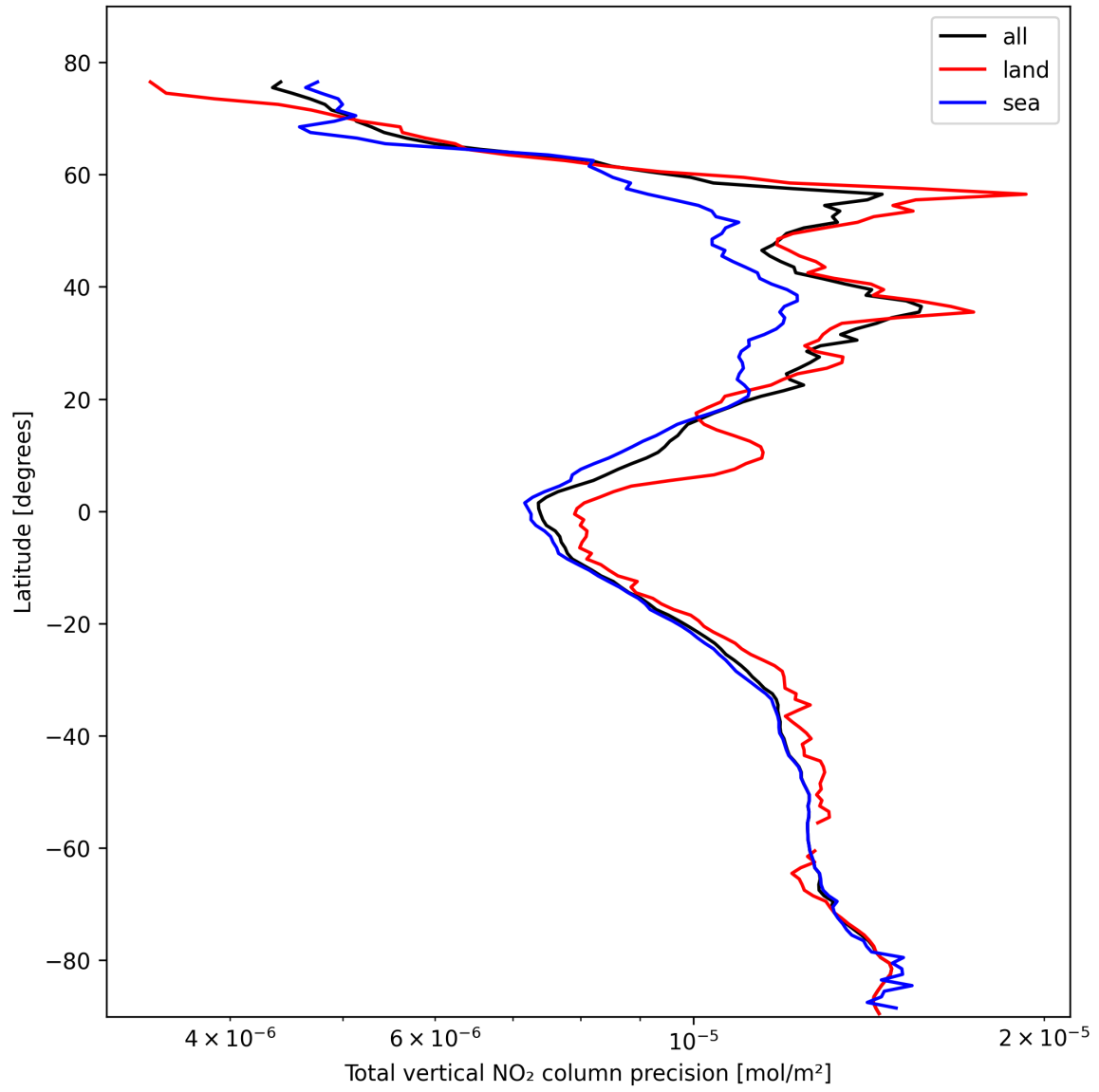
Figure 20: Zonal average of “Total vertical NO 2 column precision” for 2025-02-18 to 2025-02-19.
