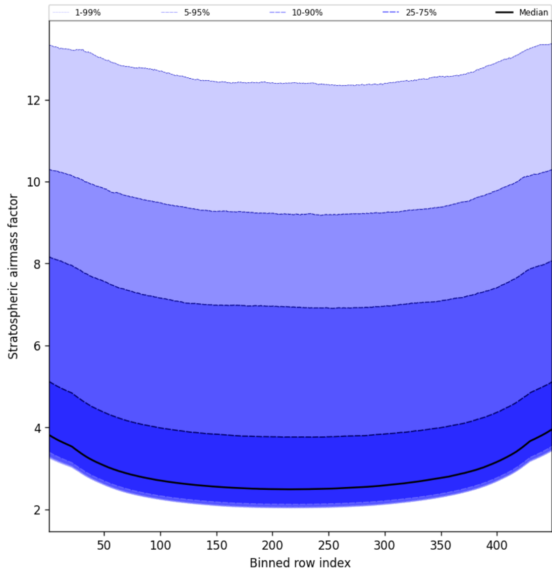
Figure 59: Along track statistics of “Stratospheric airmass factor” for 2025-02-18 to 2025-02-19
