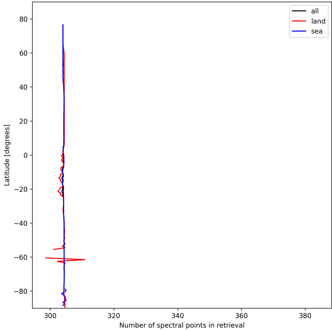
Figure 14: Zonal average of “Number of spectral points in retrieval” for 2025-02-18 to 2025-02-19.
