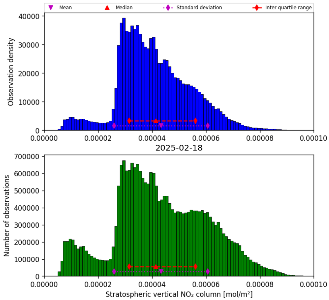
Figure 34: Histogram of “Stratospheric vertical NO 2 column” for 2025-02-18 to 2025-02-19
