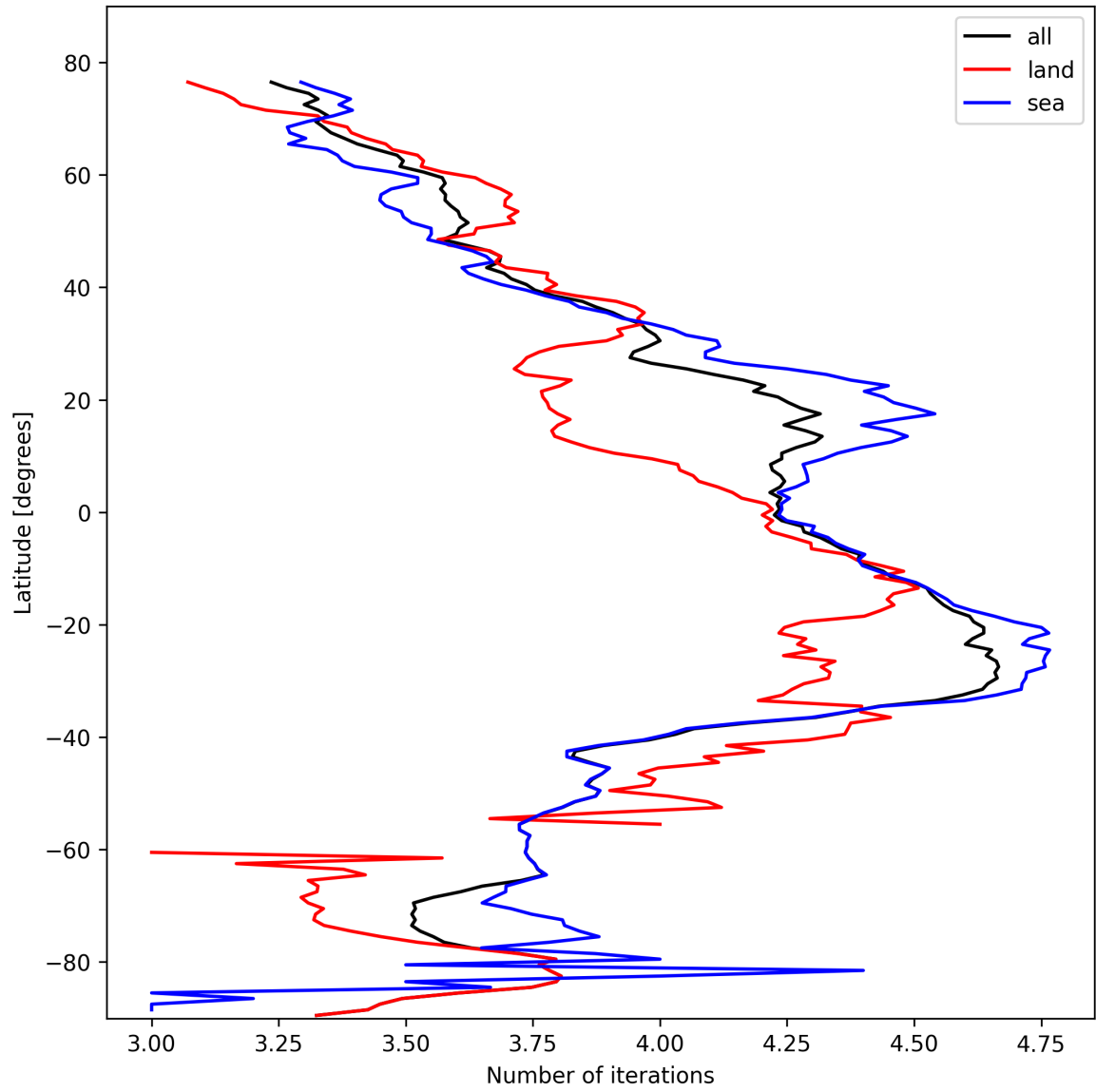
Figure 15: Zonal average of “Number of iterations” for 2025-02-18 to 2025-02-19.
