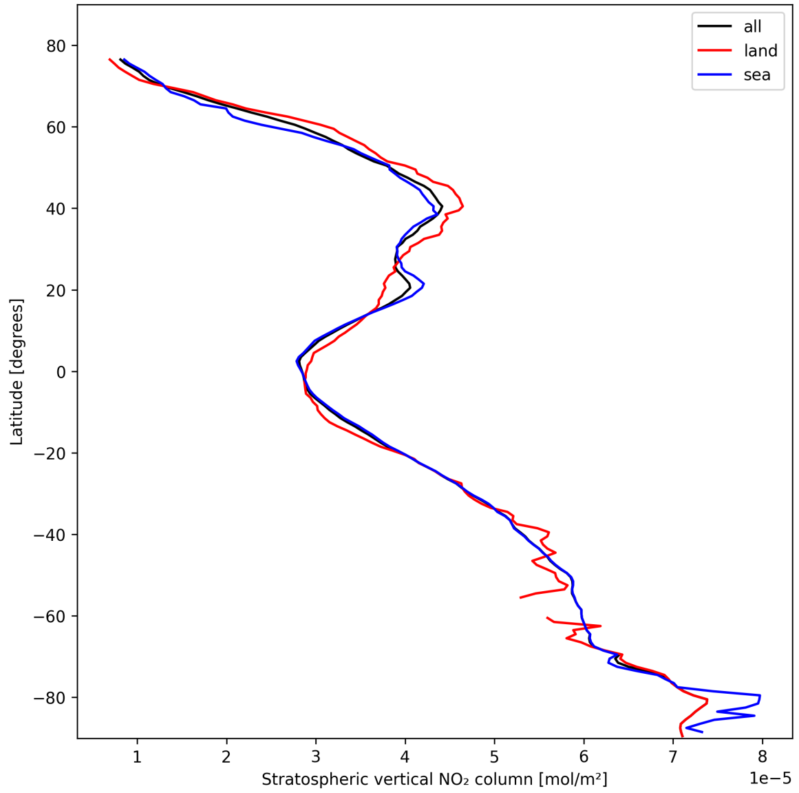
Figure 17: Zonal average of “Stratospheric vertical NO 2 column” for 2025-02-18 to 2025-02-19.
