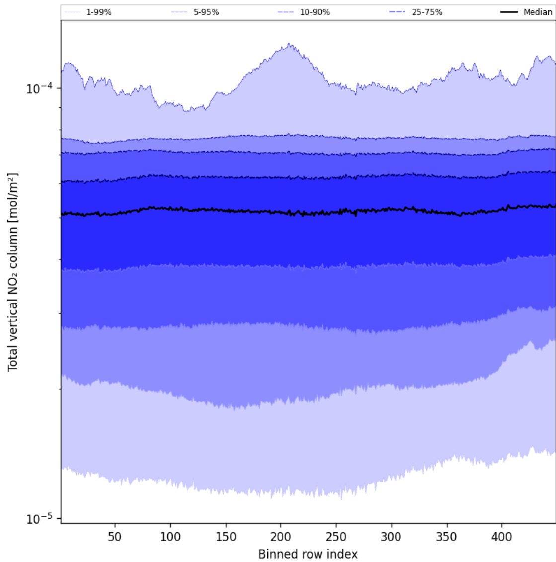
Figure 53: Along track statistics of “Total vertical NO 2 column” for 2025-02-18 to 2025-02-19
