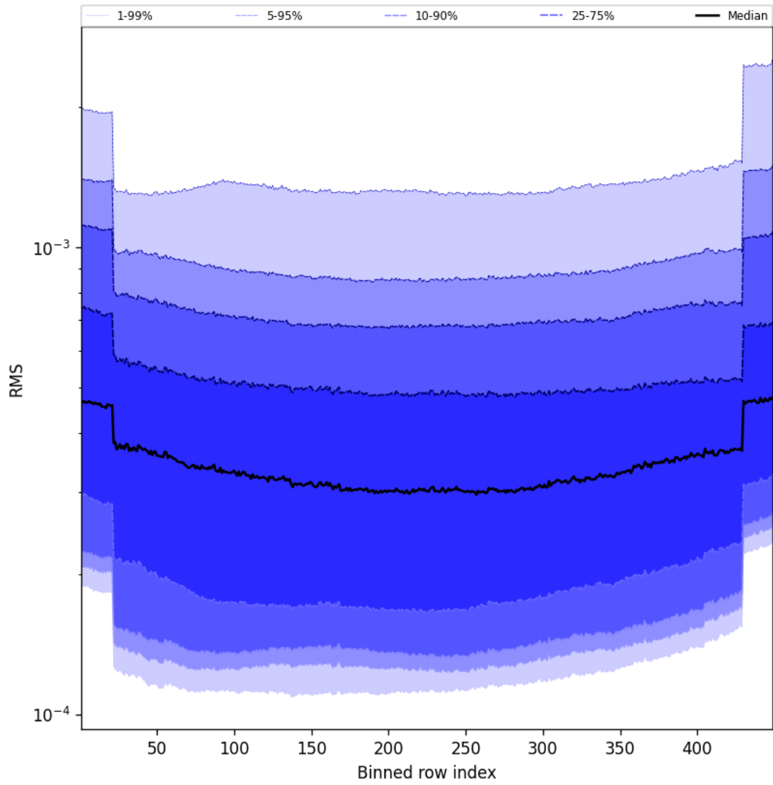
Figure 58: Along track statistics of “RMS” for 2025-02-18 to 2025-02-19
