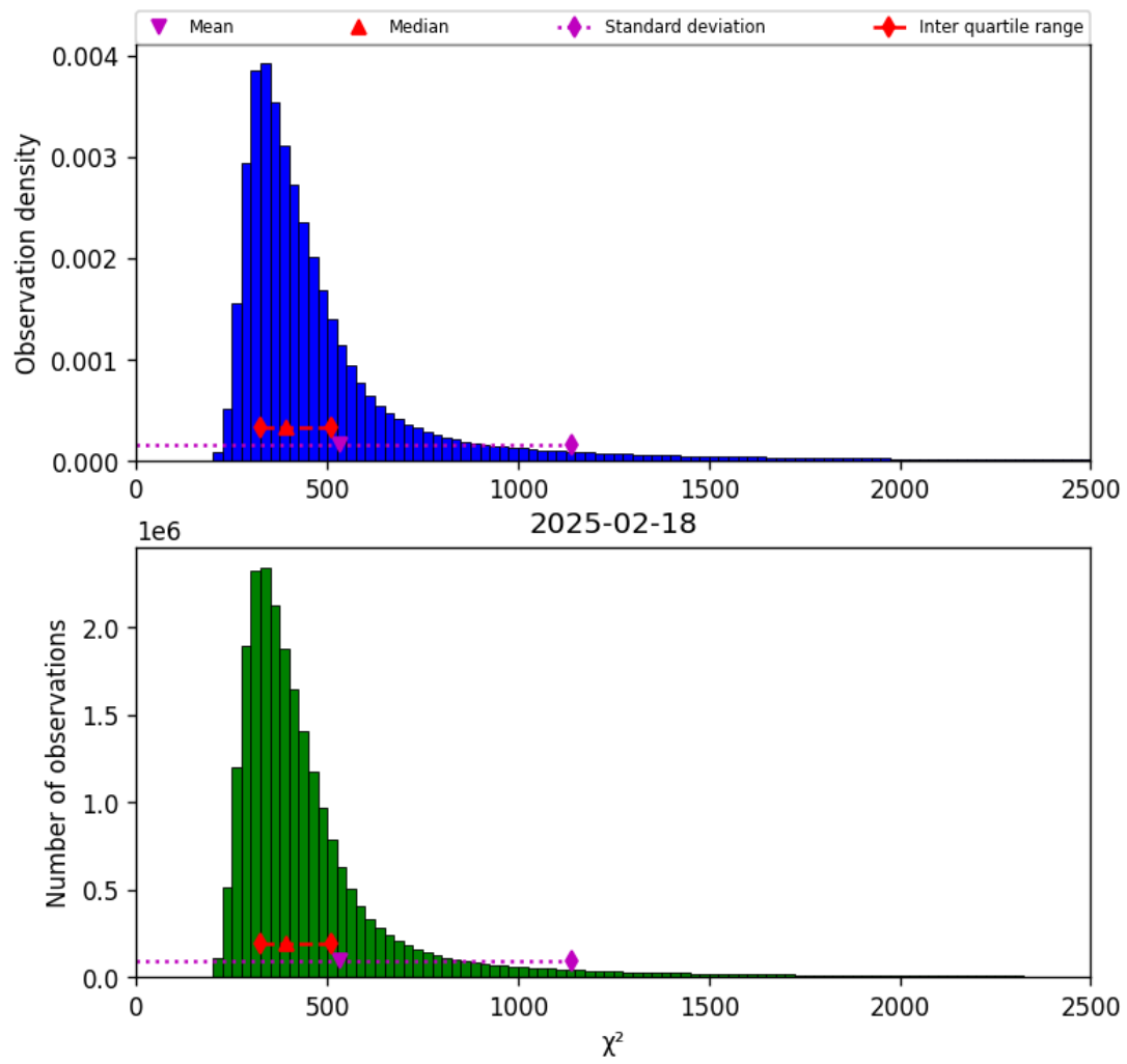
Figure 40: Histogram of “ \chi^2 ” for 2025-02-18 to 2025-02-19
