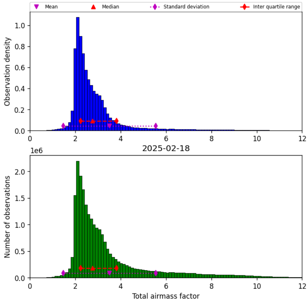
Figure 30: Histogram of “Total airmass factor” for 2025-02-18 to 2025-02-19
