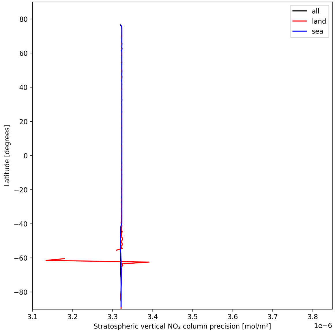
Figure 18: Zonal average of “Stratospheric vertical NO 2 column precision” for 2025-02-18 to 2025-02-19.
