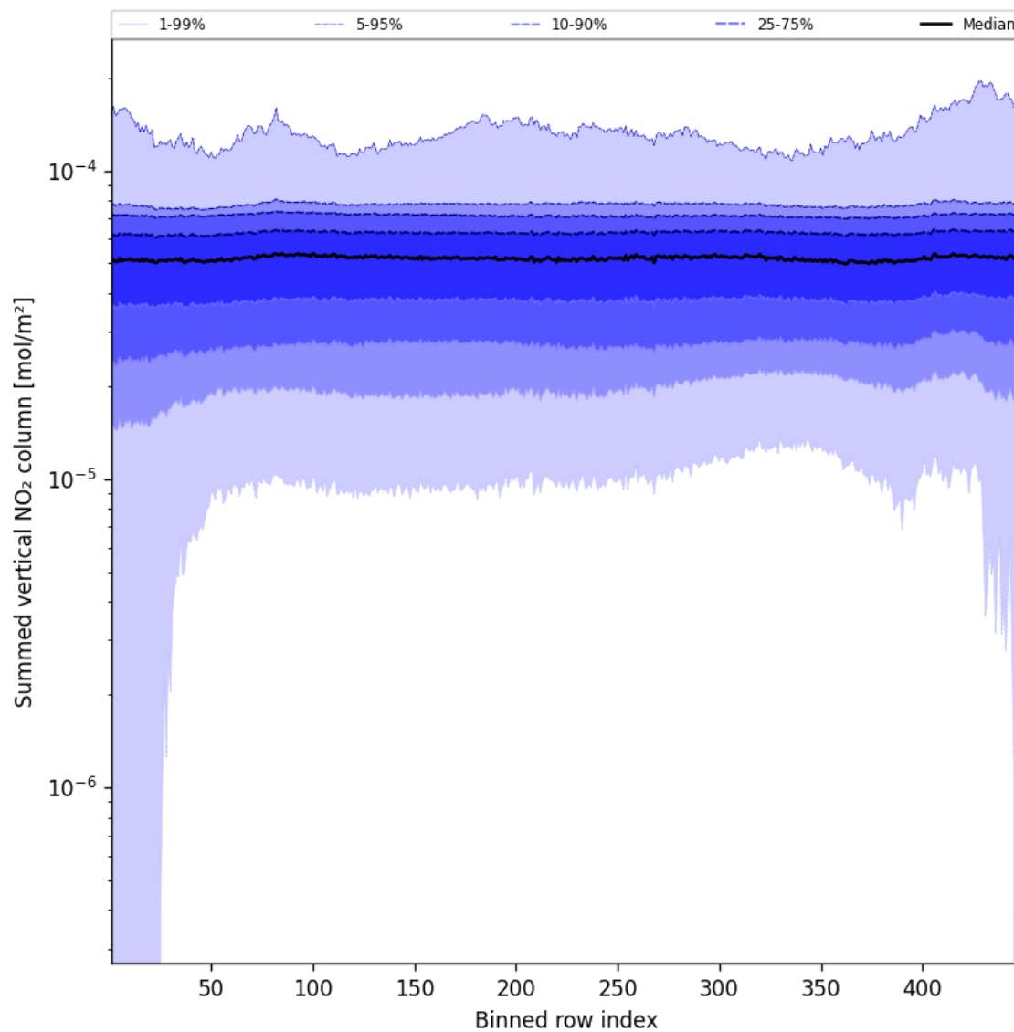
Figure 55: Along track statistics of “Summed vertical NO 2 column” for 2025-02-18 to 2025-02-19
