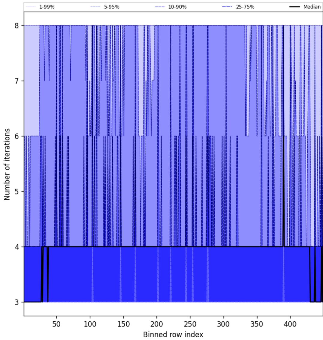
Figure 49: Along track statistics of “Number of iterations” for 2025-02-18 to 2025-02-19
