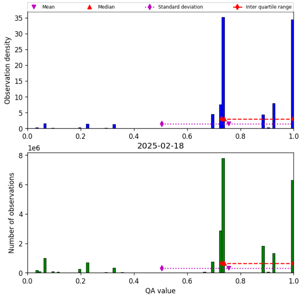
Figure 26: Histogram of “QA value” for 2025-02-18 to 2025-02-19
