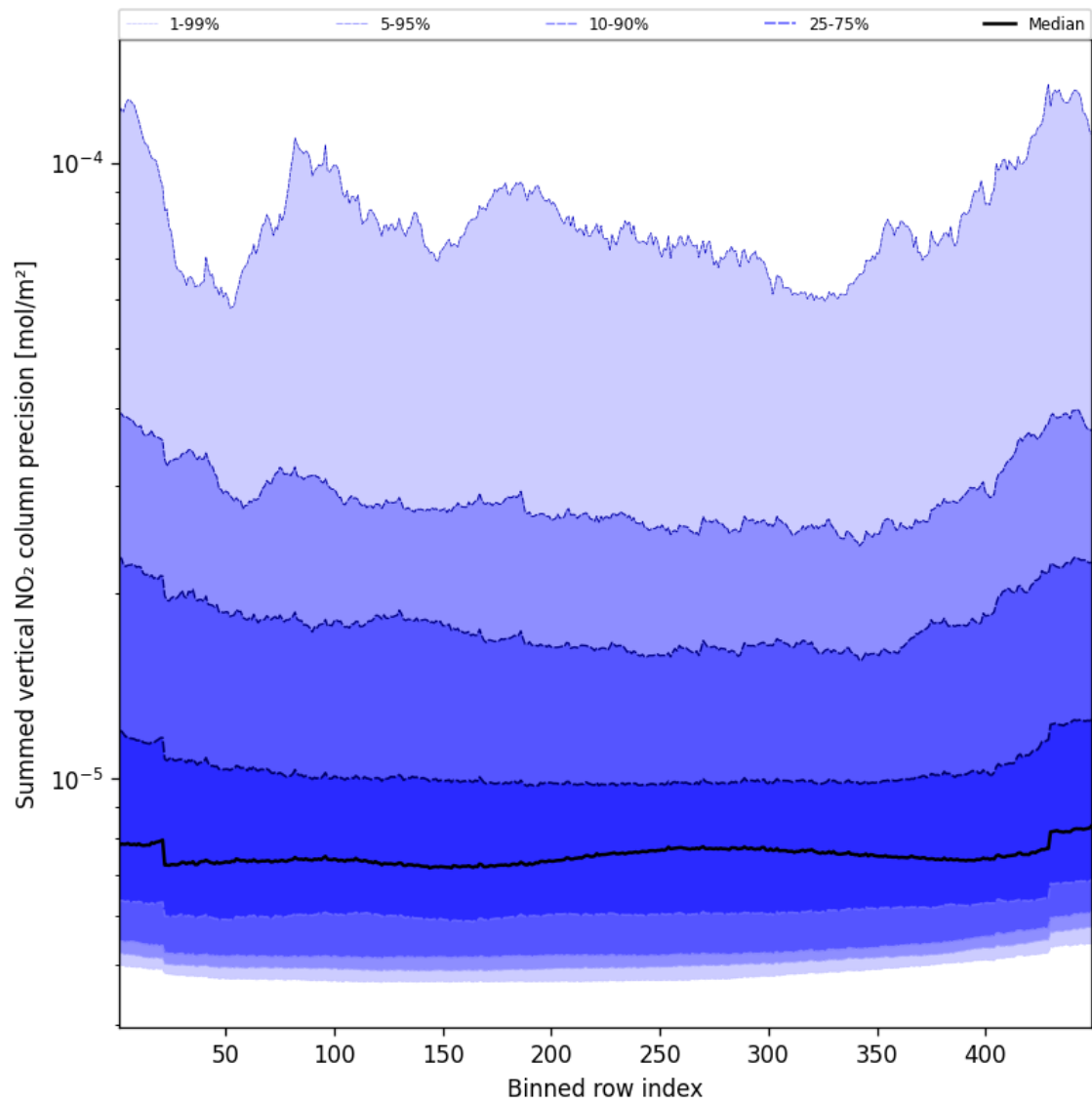
Figure 56: Along track statistics of “Summed vertical NO 2 column precision” for 2025-02-18 to 2025-02-19
