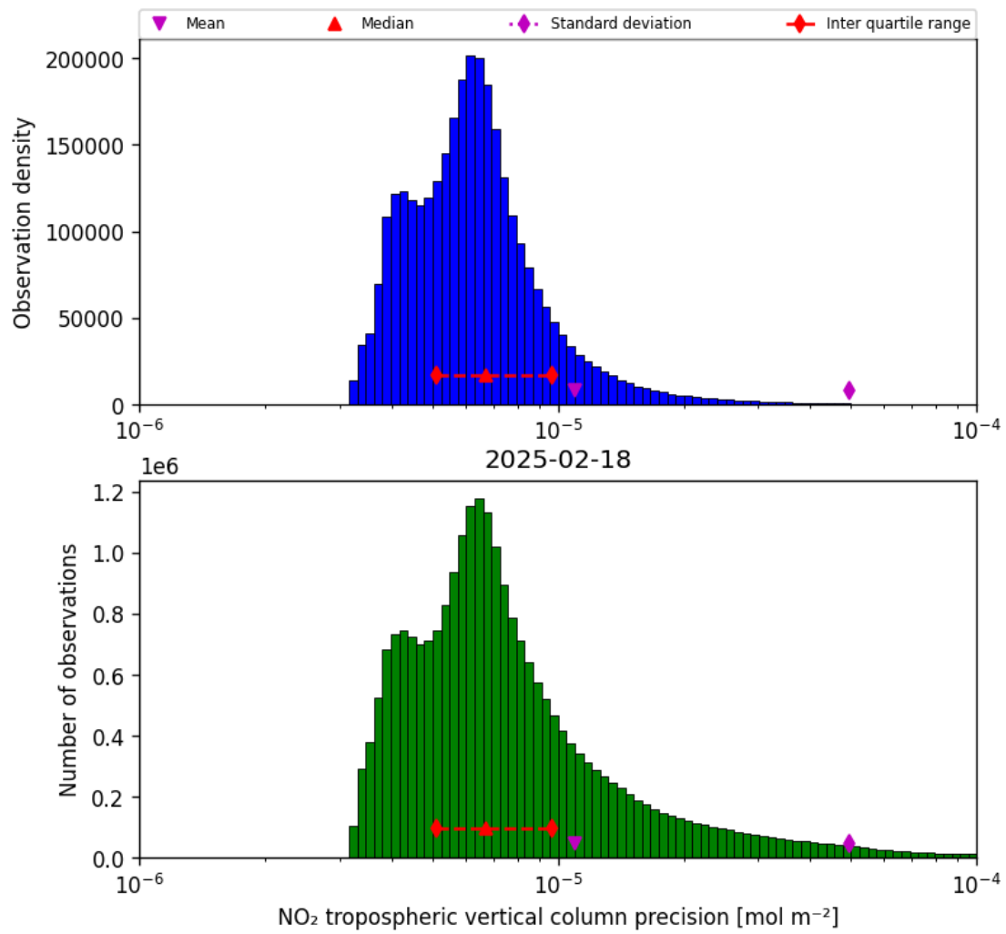
Figure 28: Histogram of “NO 2 tropospheric vertical column precision” for 2025-02-18 to 2025-02-19
