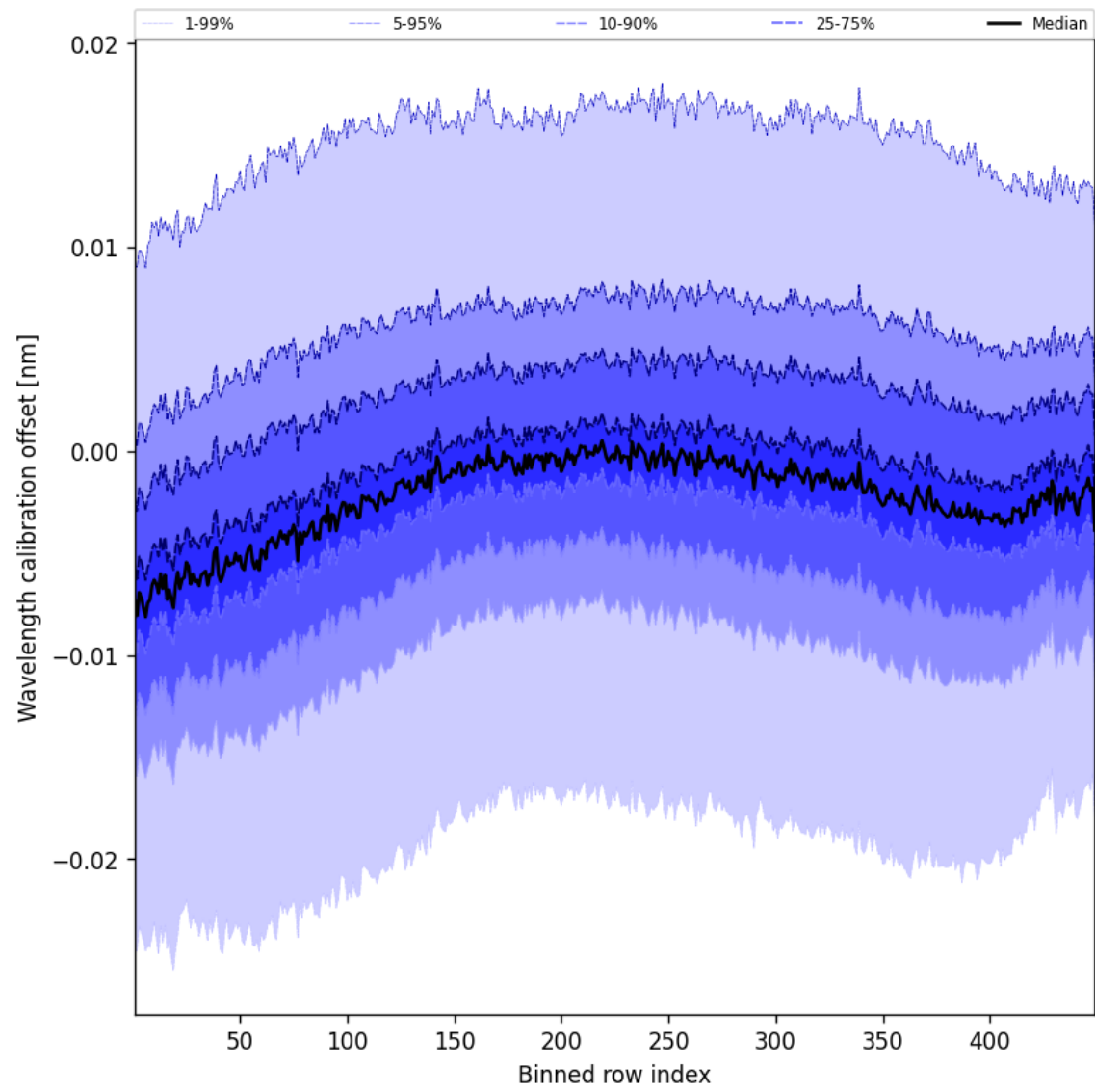
Figure 50: Along track statistics of “Wavelength calibration offset” for 2025-02-18 to 2025-02-19
