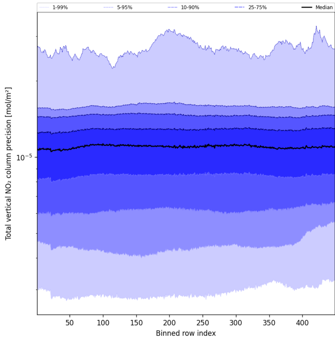
Figure 54: Along track statistics of “Total vertical NO 2 column precision” for 2025-02-18 to 2025-02-19
