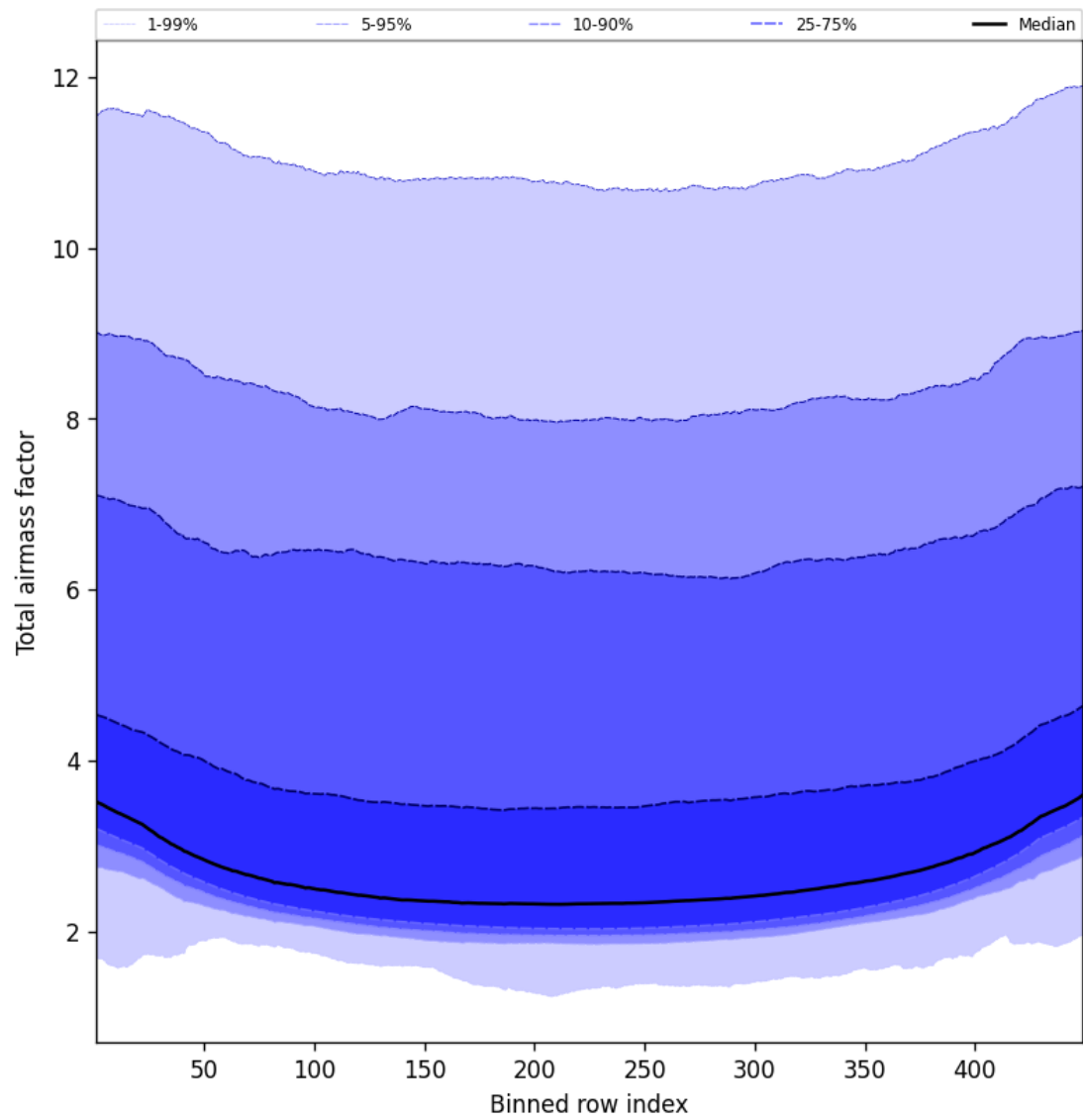
Figure 47: Along track statistics of “Total airmass factor” for 2025-02-18 to 2025-02-19
