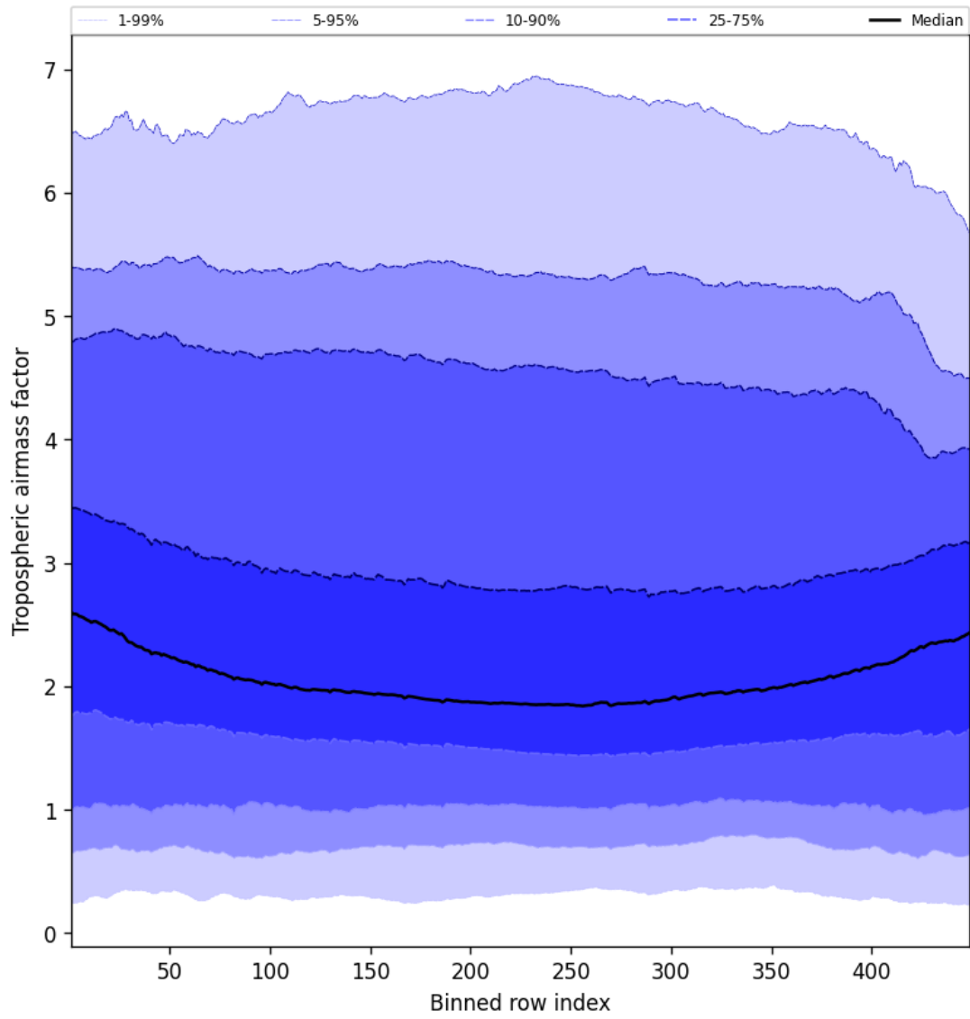
Figure 46: Along track statistics of “Tropospheric air mass factor” for 2025-02-18 to 2025-02-19
