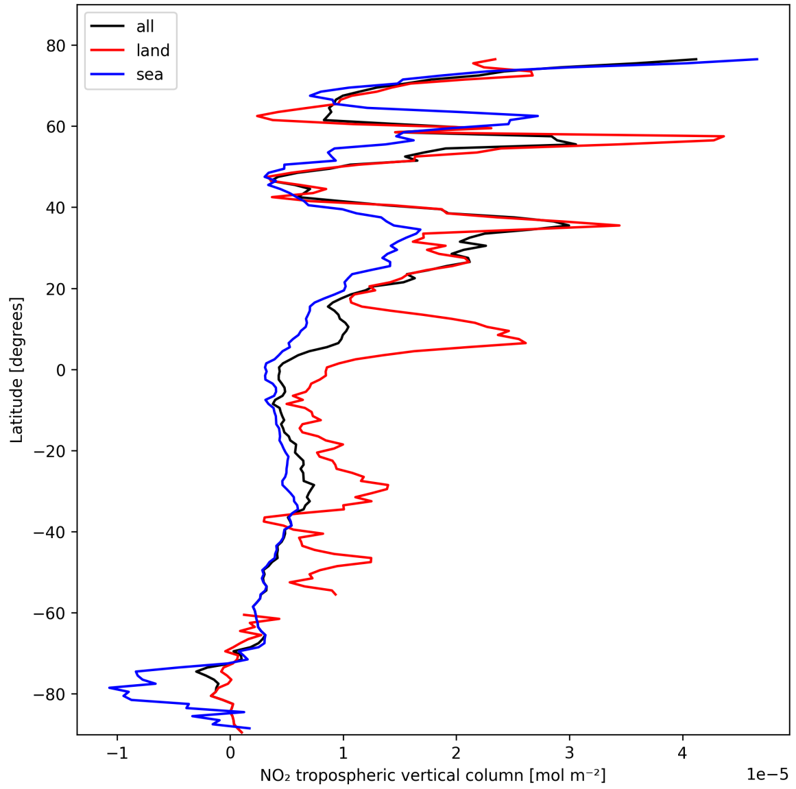
Figure 10: Zonal average of “NO 2 tropospheric vertical column” for 2025-02-18 to 2025-02-19.
