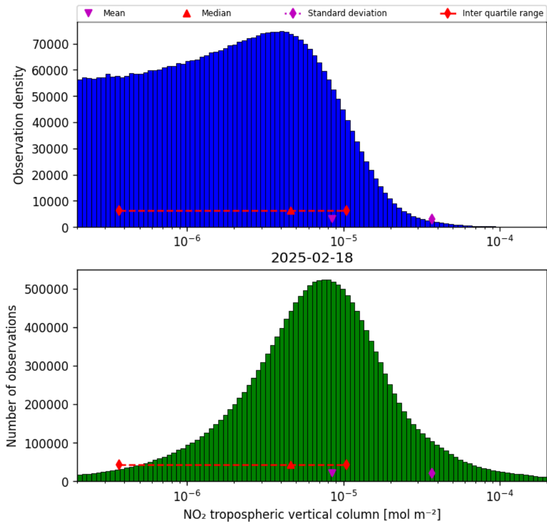
Figure 27: Histogram of “NO 2 tropospheric vertical column” for 2025-02-18 to 2025-02-19
