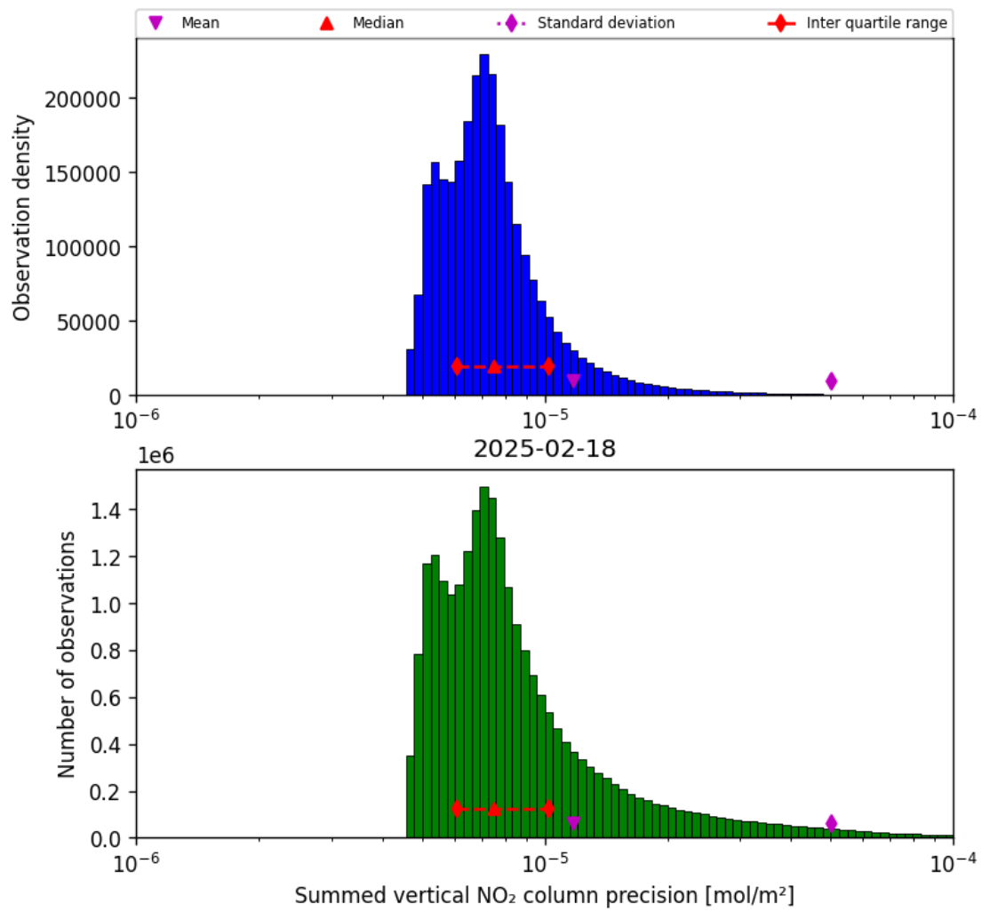
Figure 39: Histogram of “Summed vertical NO 2 column precision” for 2025-02-18 to 2025-02-19
