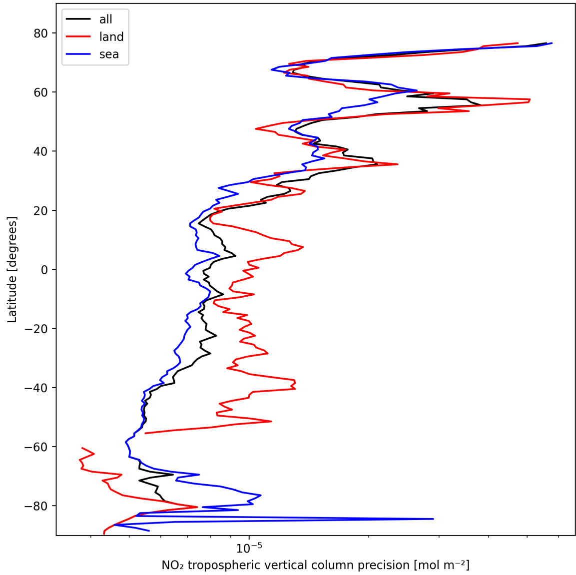
Figure 11: Zonal average of “NO 2 tropospheric vertical column precision” for 2025-02-18 to 2025-02-19.
