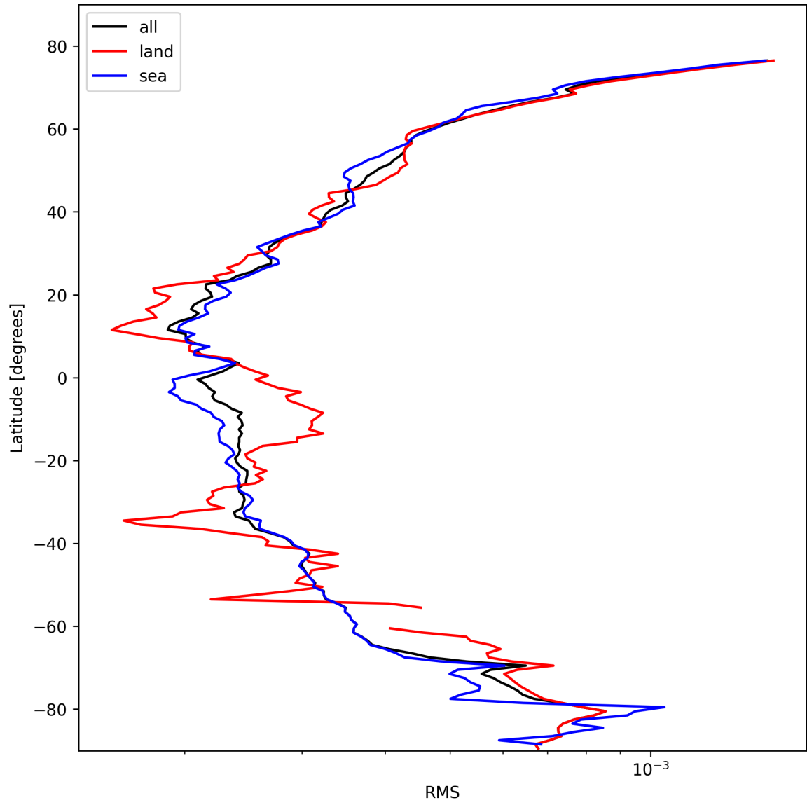
Figure 24: Zonal average of “RMS” for 2025-02-18 to 2025-02-19.
