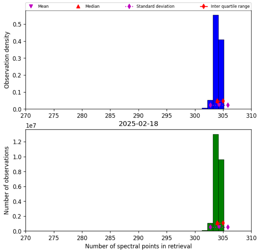
Figure 31: Histogram of “Number of spectral points in retrieval” for 2025-02-18 to 2025-02-19
