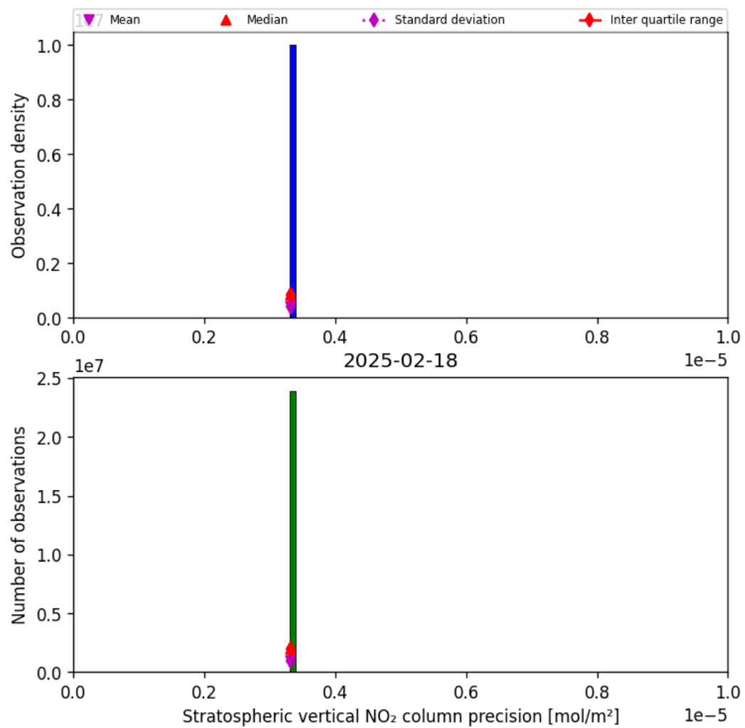
Figure 35: Histogram of “Stratospheric vertical NO 2 column precision” for 2025-02-18 to 2025-02-19
