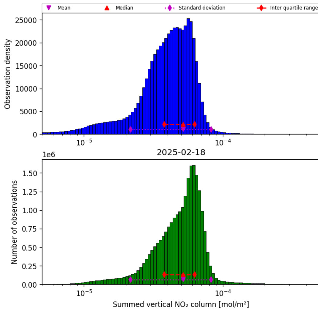
Figure 38: Histogram of “Summed vertical NO 2 column” for 2025-02-18 to 2025-02-19
