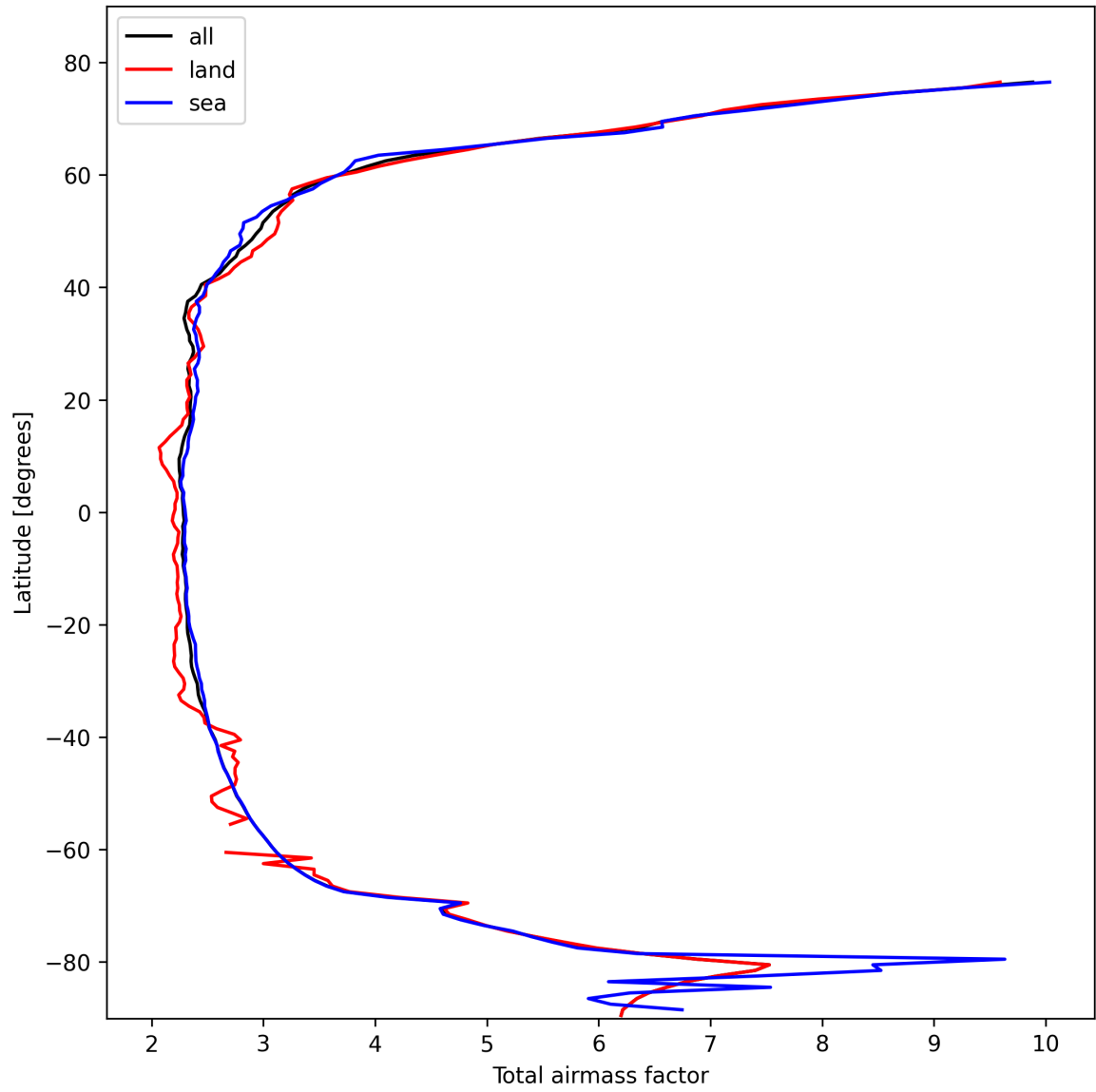
Figure 13: Zonal average of “Total airmass factor” for 2025-02-18 to 2025-02-19.
