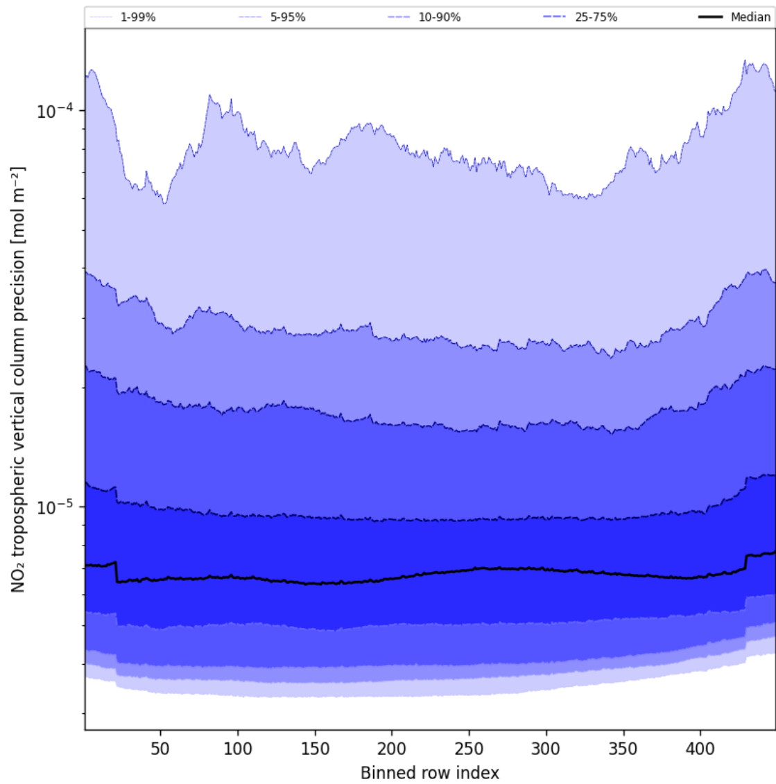
Figure 45: Along track statistics of “NO 2 tropospheric vertical column precision” for 2025-02-18 to 2025-02-19
