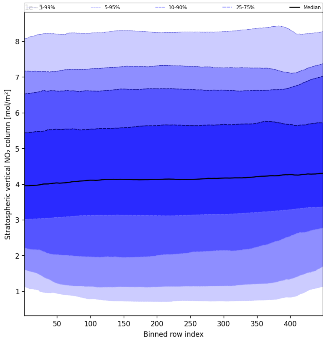
Figure 51: Along track statistics of “Stratospheric vertical NO 2 column” for 2025-02-18 to 2025-02-19
