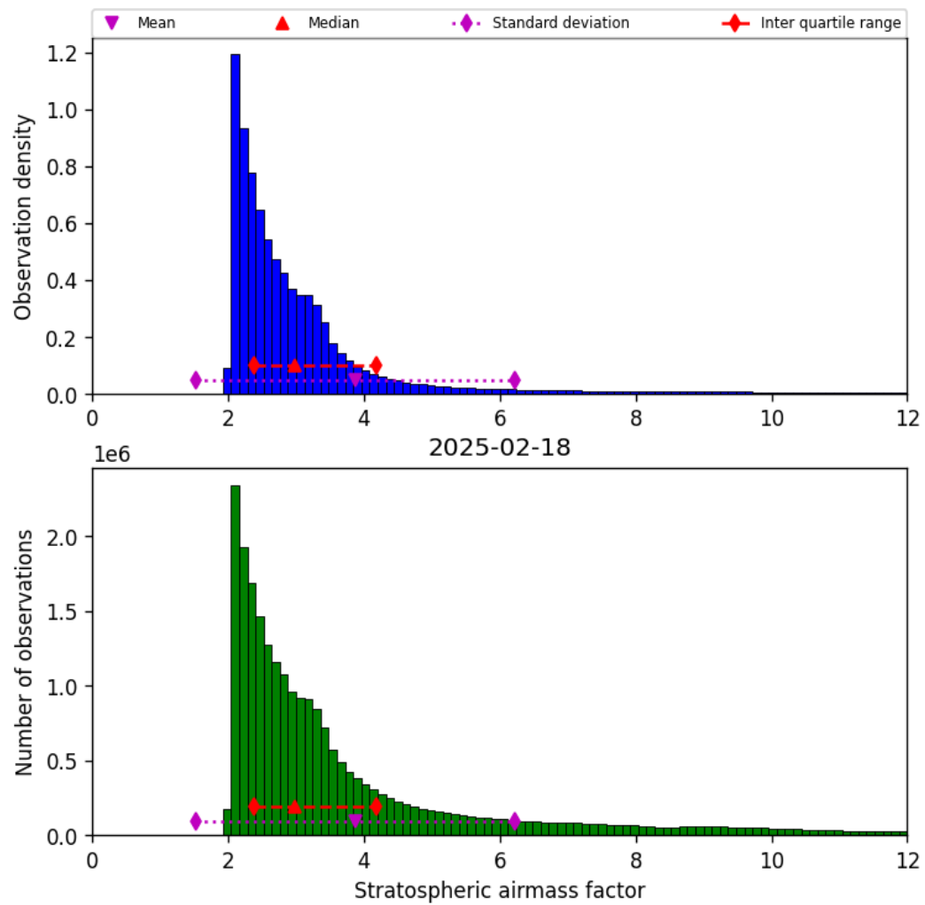
Figure 42: Histogram of “Stratospheric airmass factor” for 2025-02-18 to 2025-02-19
