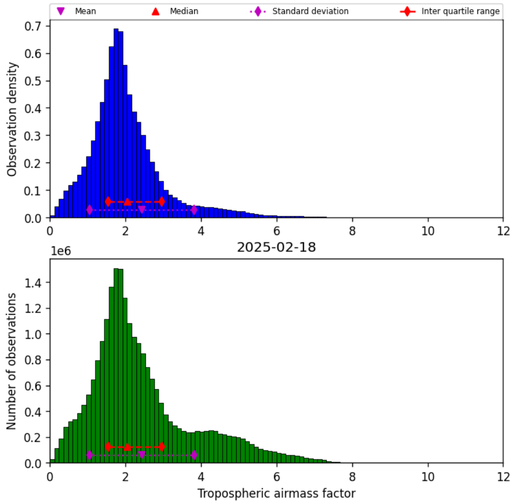
Figure 29: Histogram of “Tropospheric airmass factor” for 2025-02-18 to 2025-02-19
