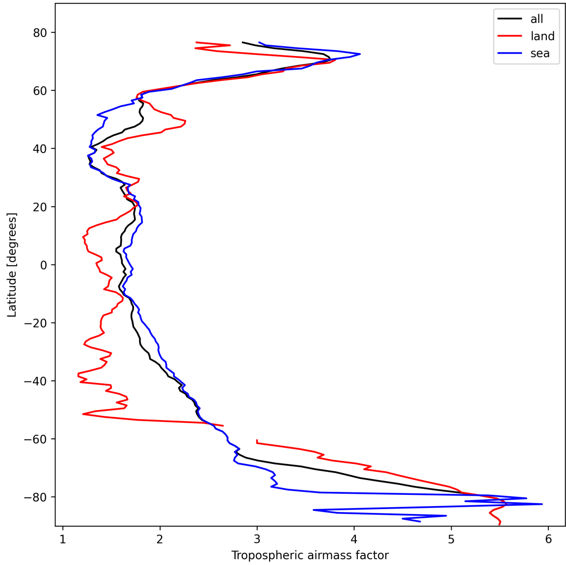
Figure 12: Zonal average of “Tropospheric air mass factor” for 2025-02-18 to 2025-02-19.
