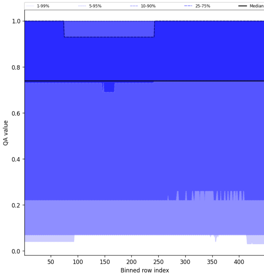
Figure 43: Along track statistics of “QA value” for 2025-02-18 to 2025-02-19
