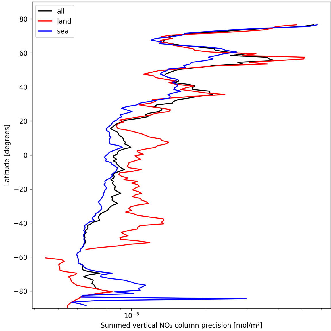
Figure 22: Zonal average of “Summed vertical NO 2 column precision” for 2025-02-18 to 2025-02-19.
