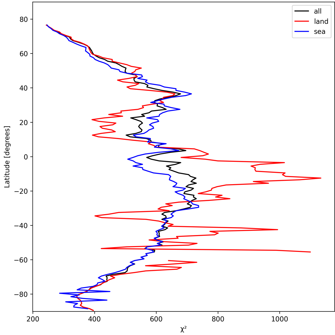
Figure 23: Zonal average of “ \chi^2 ” for 2025-02-18 to 2025-02-19.
