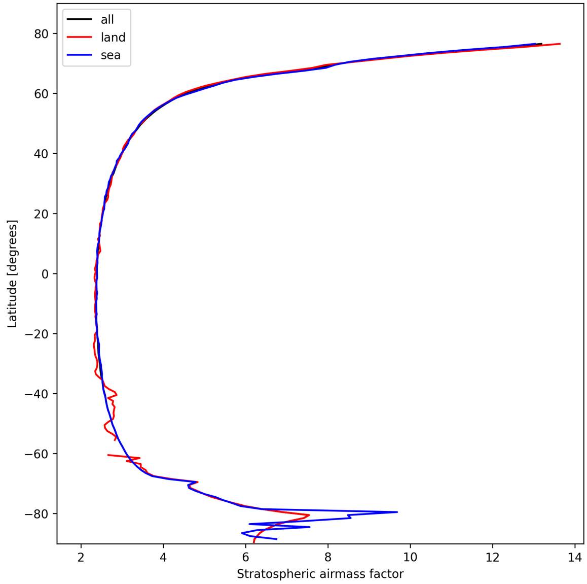
Figure 25: Zonal average of “Stratospheric air mass factor” for 2025-02-18 to 2025-02-19.
