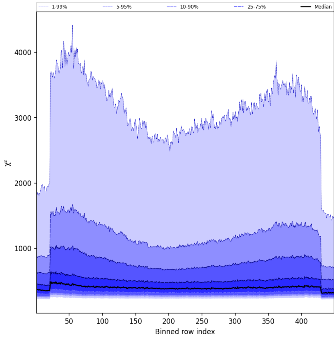
Figure 57: Along track statistics of “ \chi^2 ” for 2025-02-18 to 2025-02-19
