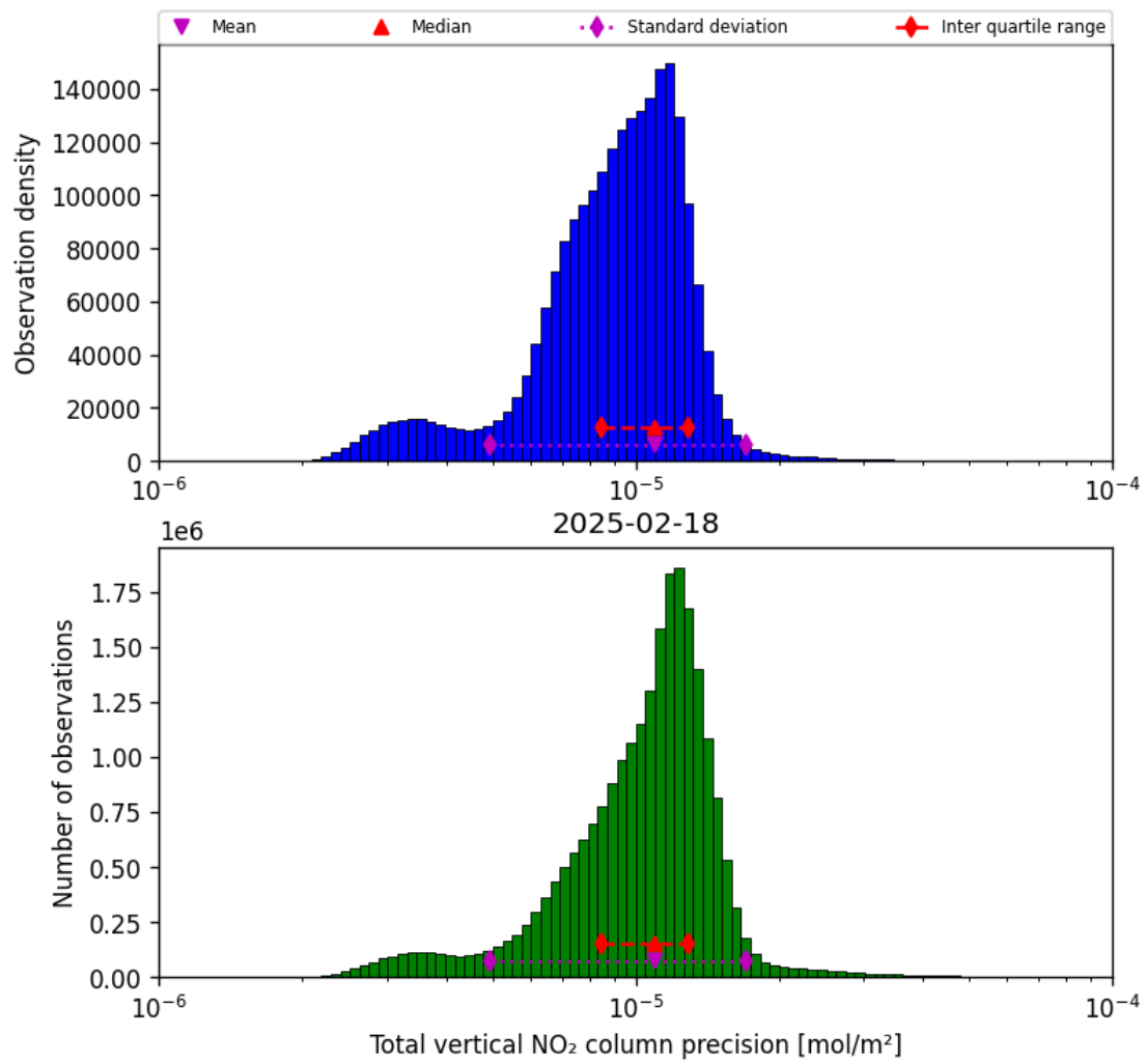
Figure 37: Histogram of “Total vertical NO 2 column precision” for 2025-02-18 to 2025-02-19
