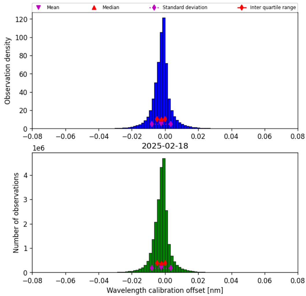
Figure 33: Histogram of “Wavelength calibration offset” for 2025-02-18 to 2025-02-19
