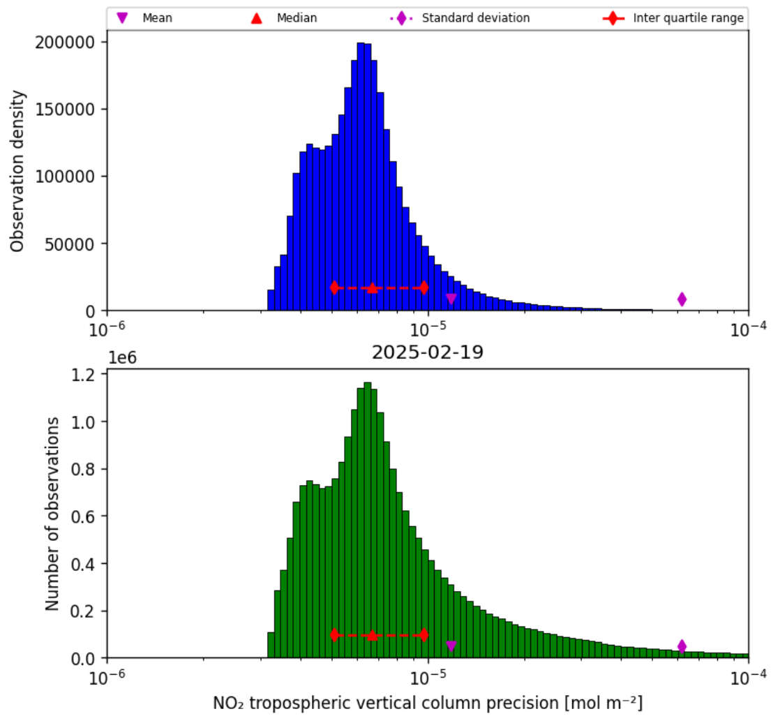
Figure 28: Histogram of “NO 2 tropospheric vertical column precision” for 2025-02-19 to 2025-02-20
