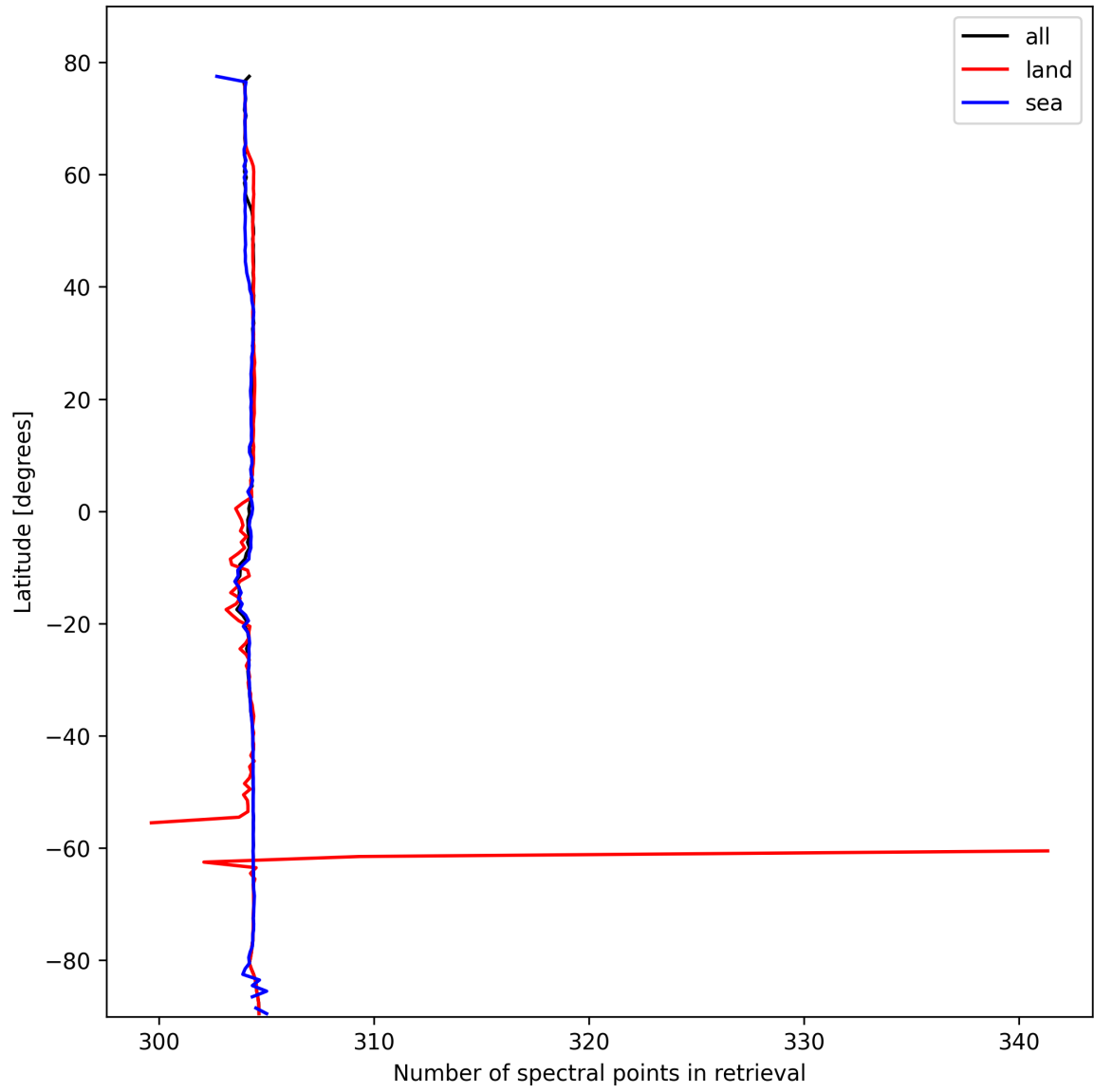
Figure 14: Zonal average of “Number of spectral points in retrieval” for 2025-02-19 to 2025-02-20.
