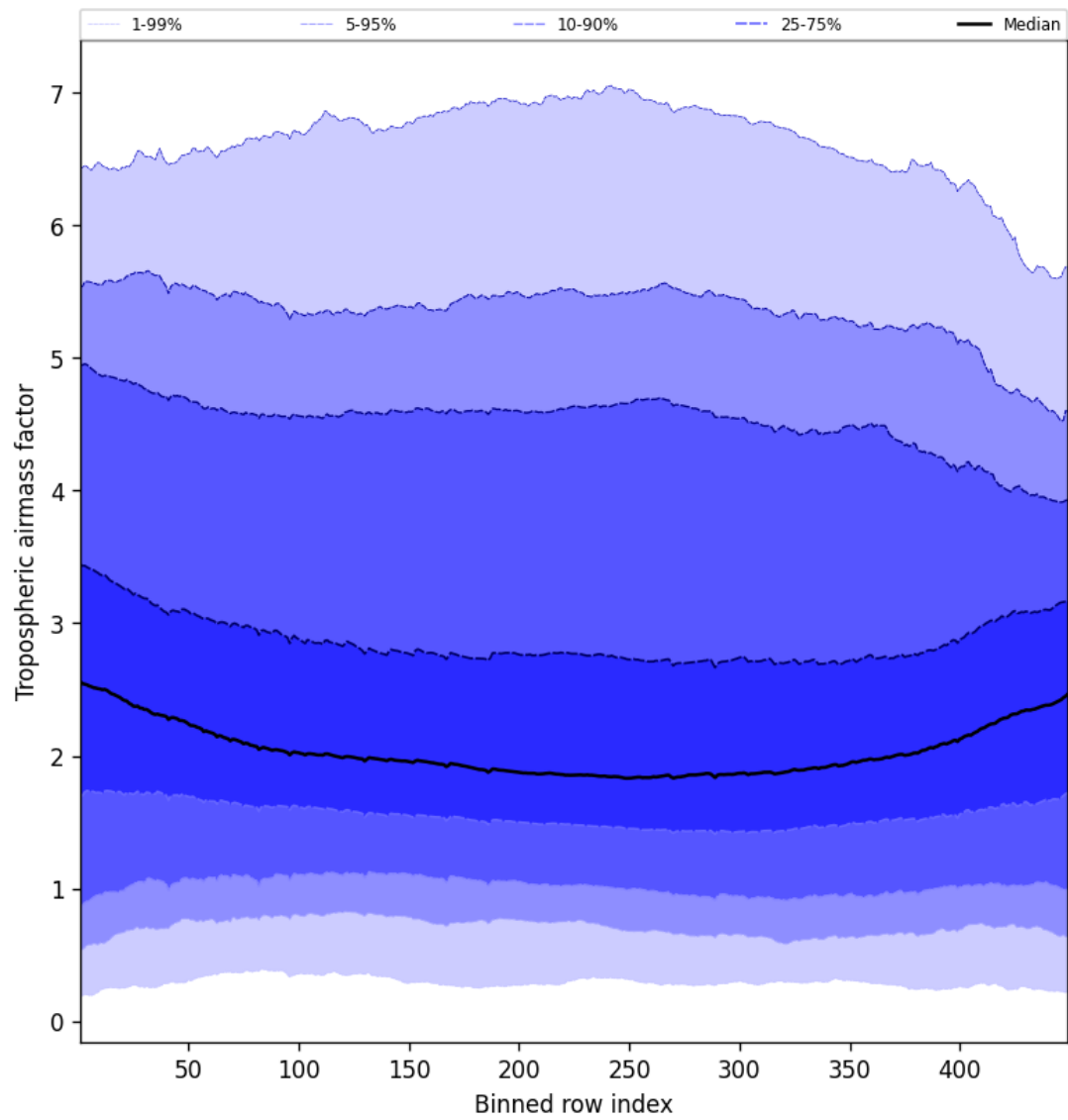
Figure 46: Along track statistics of “Tropospheric airmass factor” for 2025-02-19 to 2025-02-20
