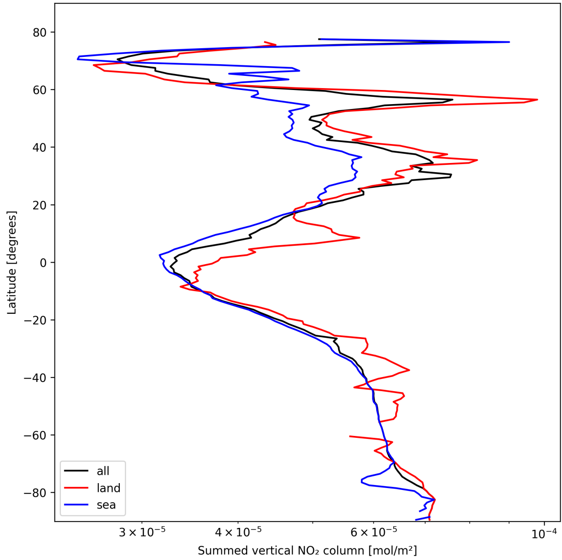
Figure 21: Zonal average of “Summed vertical NO 2 column” for 2025-02-19 to 2025-02-20.
