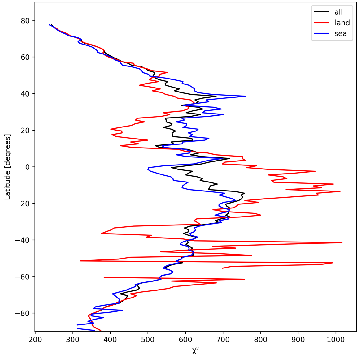
Figure 23: Zonal average of “ \chi^2 ” for 2025-02-19 to 2025-02-20.
