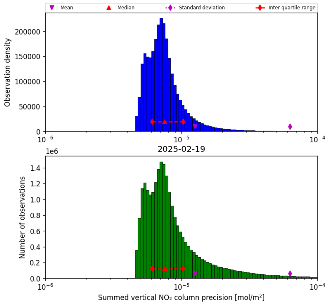
Figure 39: Histogram of "Summed vertical NO 2 column precision" for 2025-02-19 to 2025-02-20
