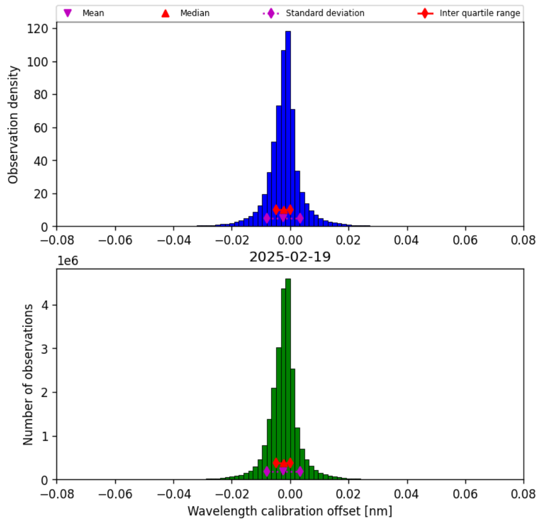
Figure 33: Histogram of “Wavelength calibration offset” for 2025-02-19 to 2025-02-20
