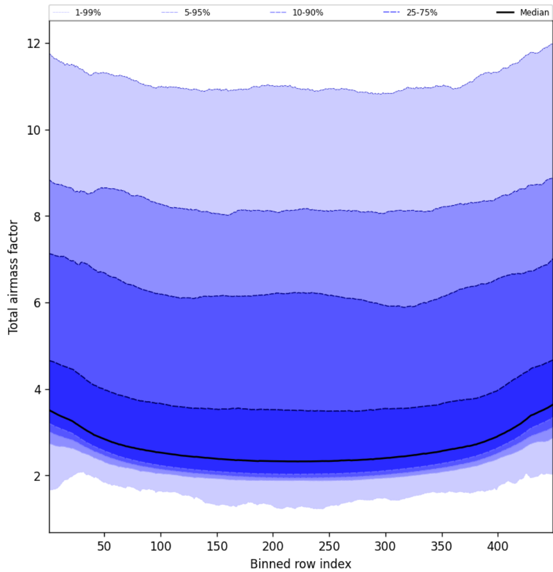
Figure 47: Along track statistics of “Total airmass factor” for 2025-02-19 to 2025-02-20
