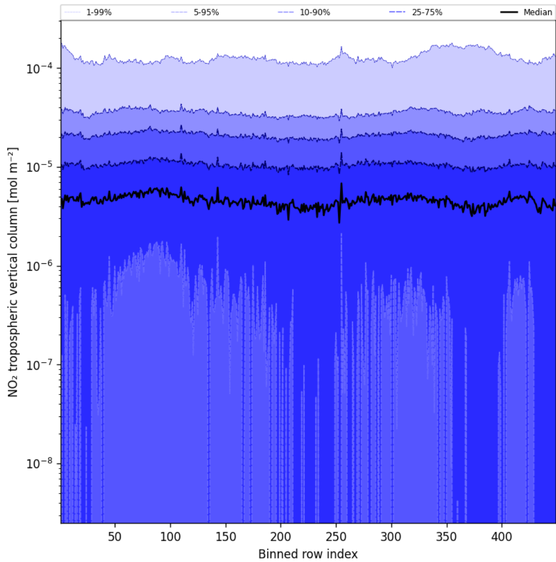
Figure 44: Along track statistics of “NO 2 tropospheric vertical column” for 2025-02-19 to 2025-02-20
