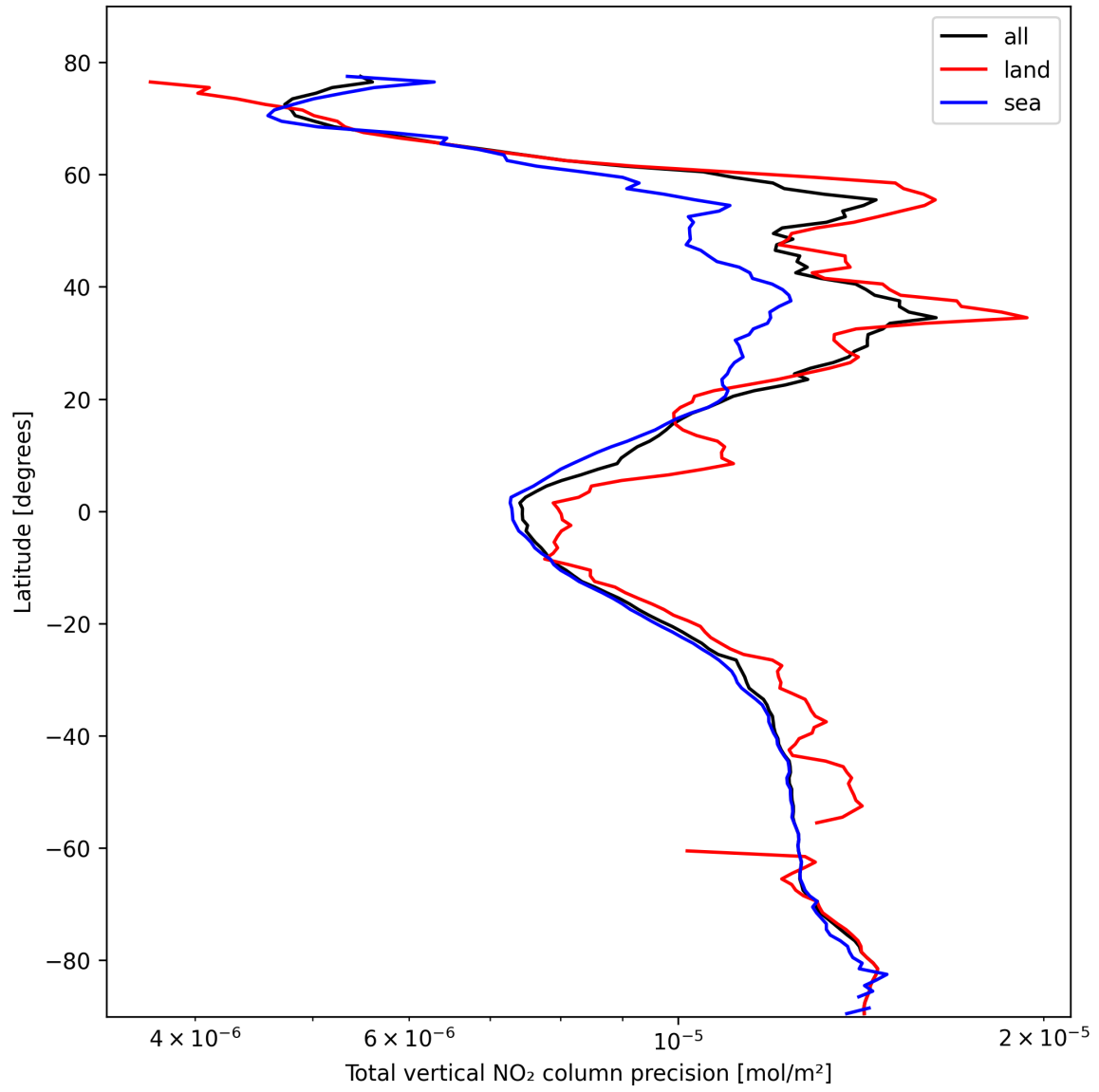
Figure 20: Zonal average of “Total vertical NO 2 column precision” for 2025-02-19 to 2025-02-20.
