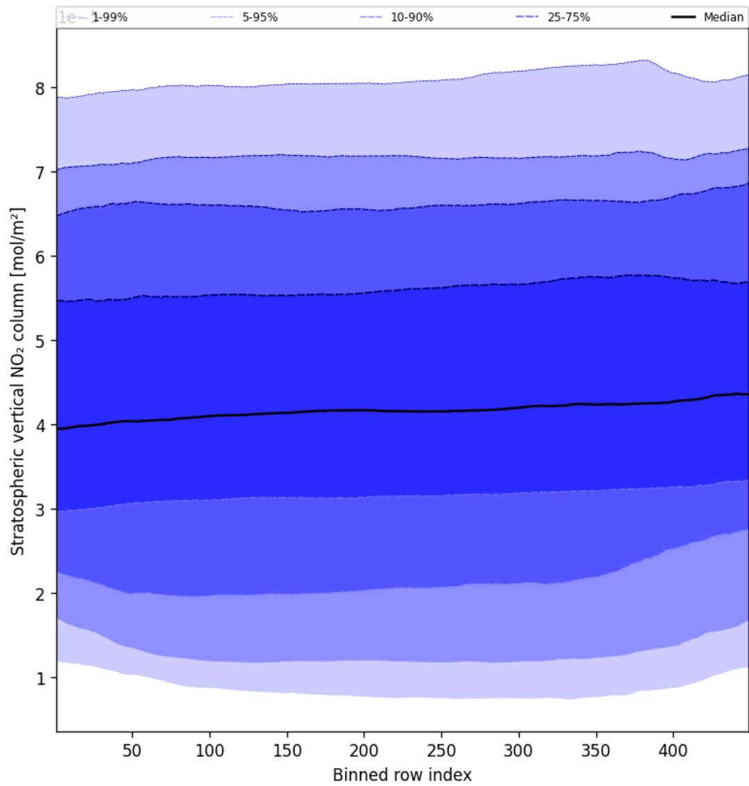
Figure 51: Along track statistics of “Stratospheric vertical NO 2 column” for 2025-02-19 to 2025-02-20
