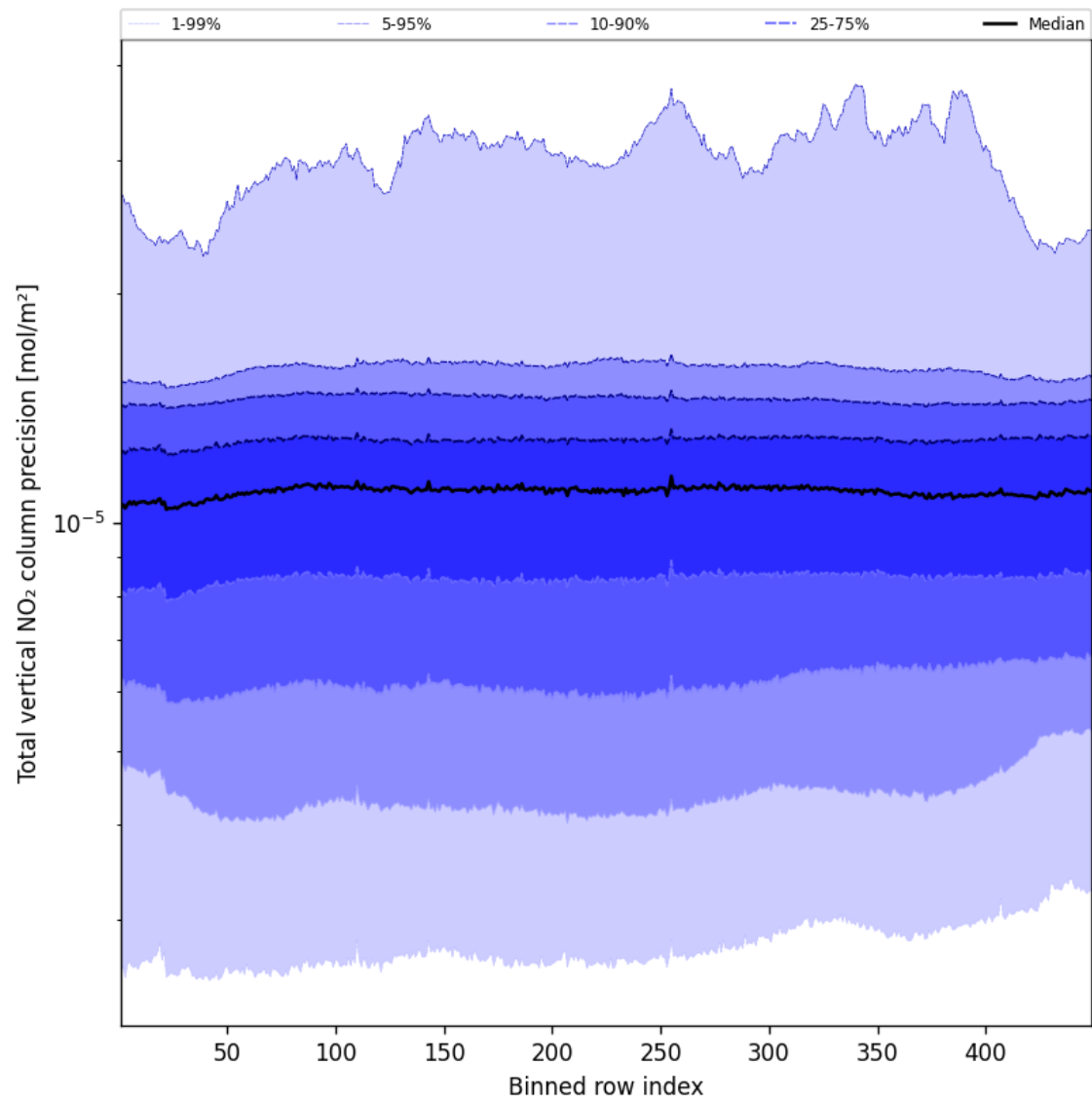
Figure 54: Along track statistics of “Total vertical NO 2 column precision” for 2025-02-19 to 2025-02-20
