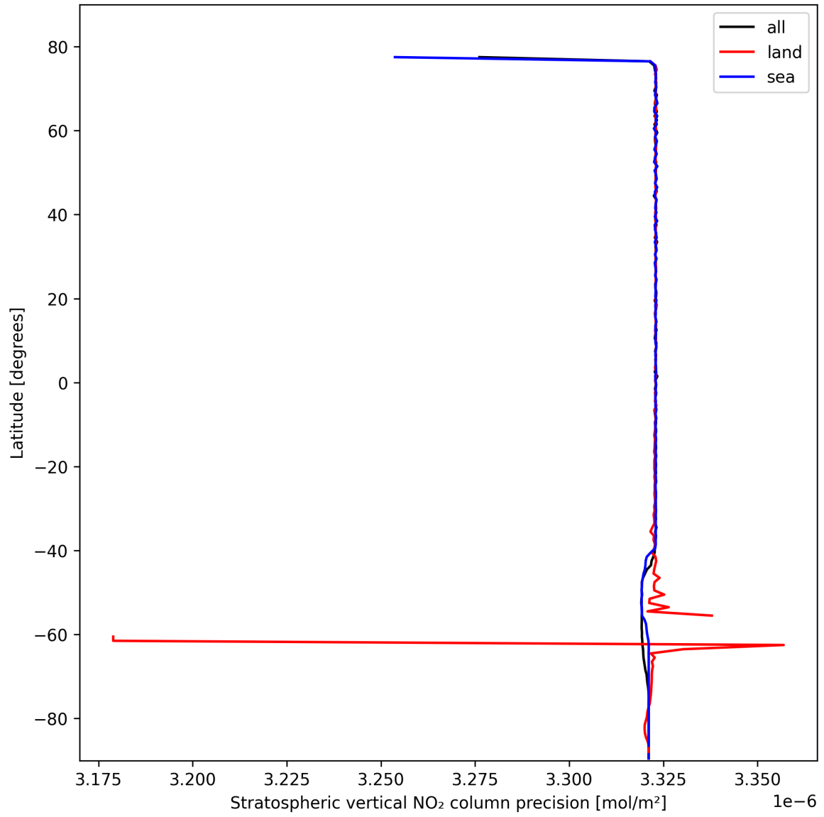
Figure 18: Zonal average of “Stratospheric vertical NO 2 column precision” for 2025-02-19 to 2025-02-20.
