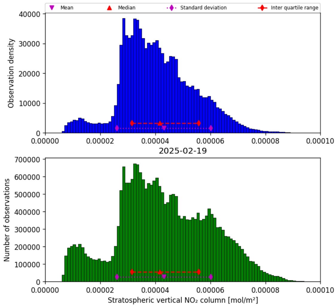
Figure 34: Histogram of “Stratospheric vertical NO 2 column” for 2025-02-19 to 2025-02-20
