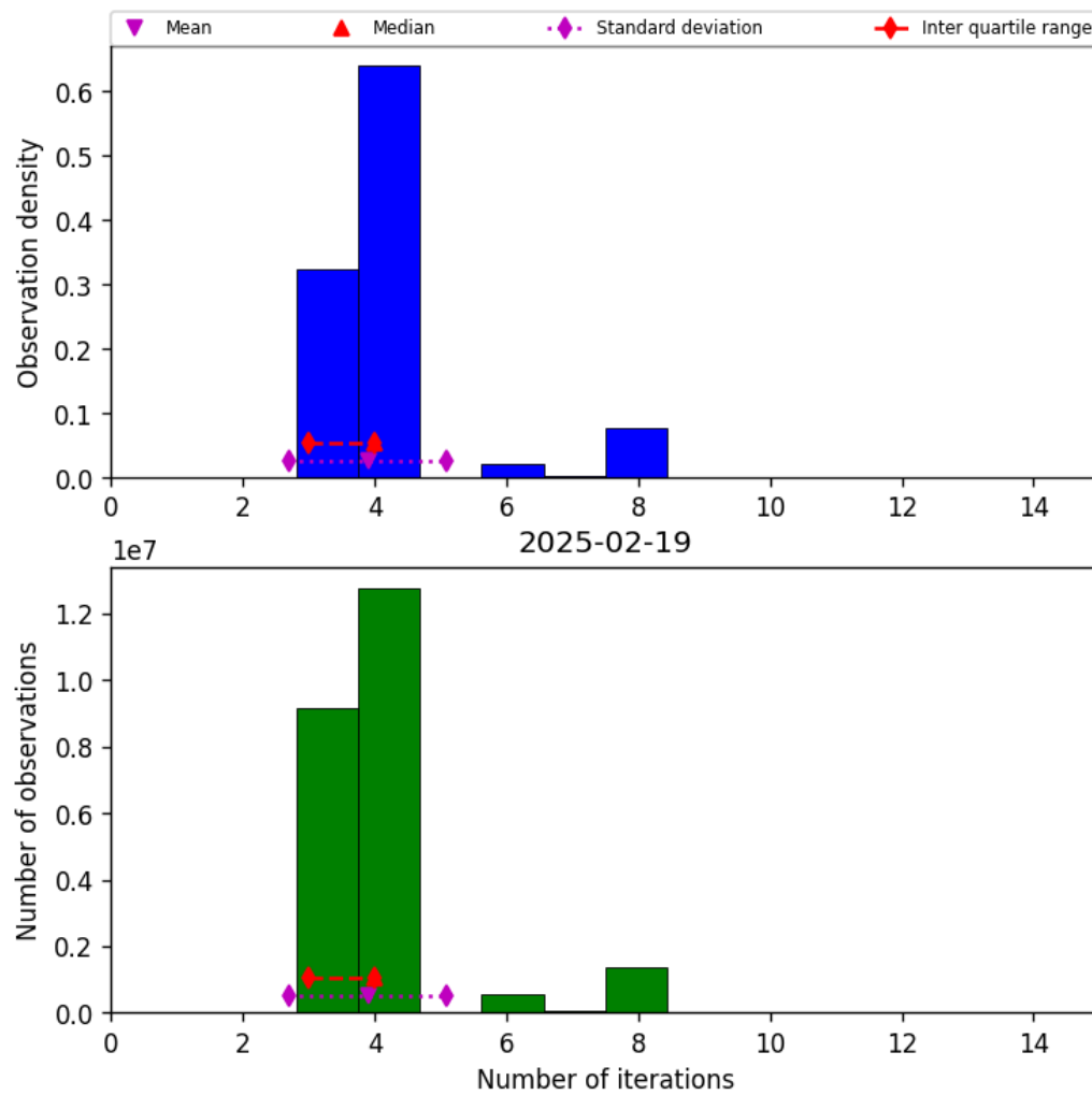
Figure 32: Histogram of “Number of iterations” for 2025-02-19 to 2025-02-20
