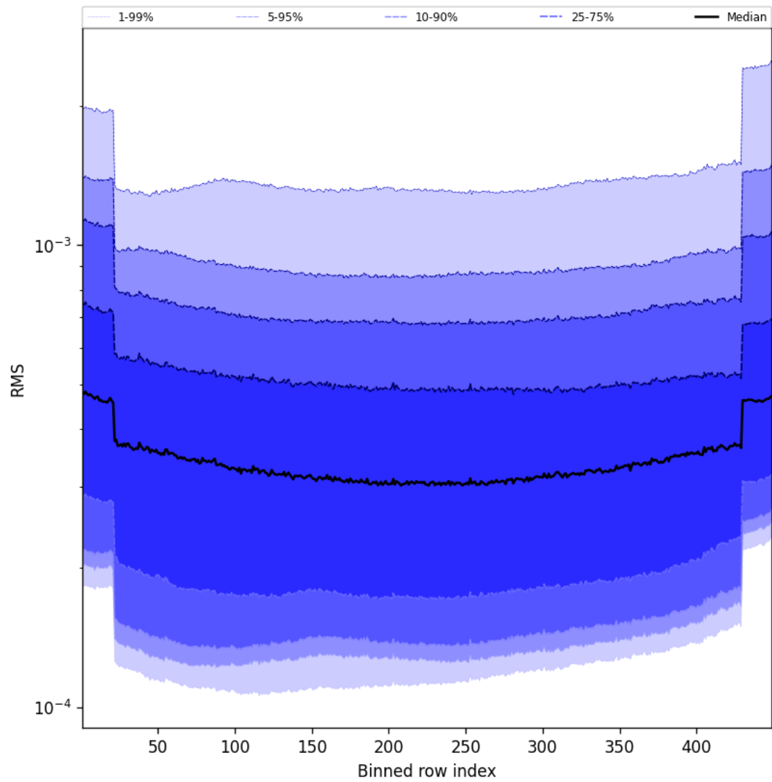
Figure 58: Along track statistics of “RMS” for 2025-02-19 to 2025-02-20
