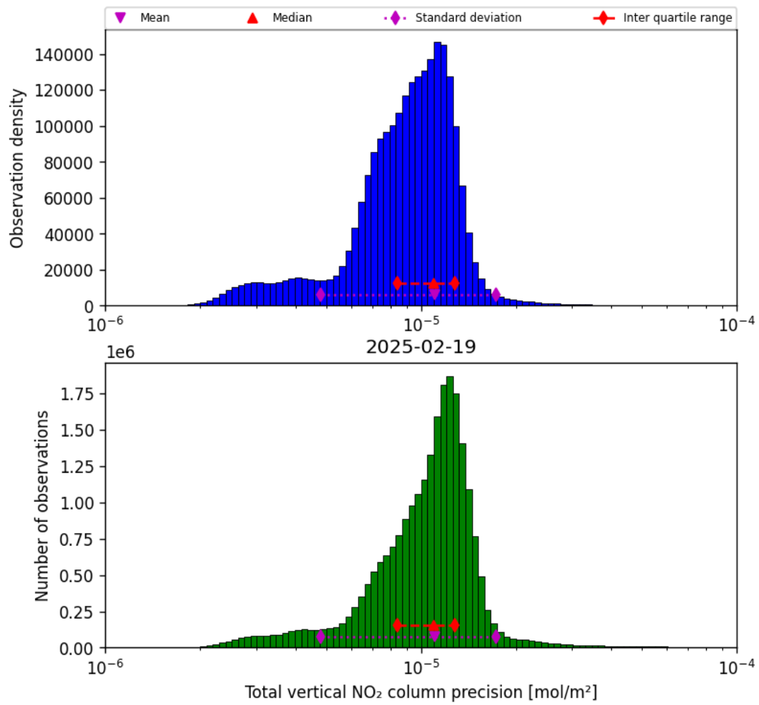
Figure 37: Histogram of "Total vertical NO 2 column precision" for 2025-02-19 to 2025-02-20
