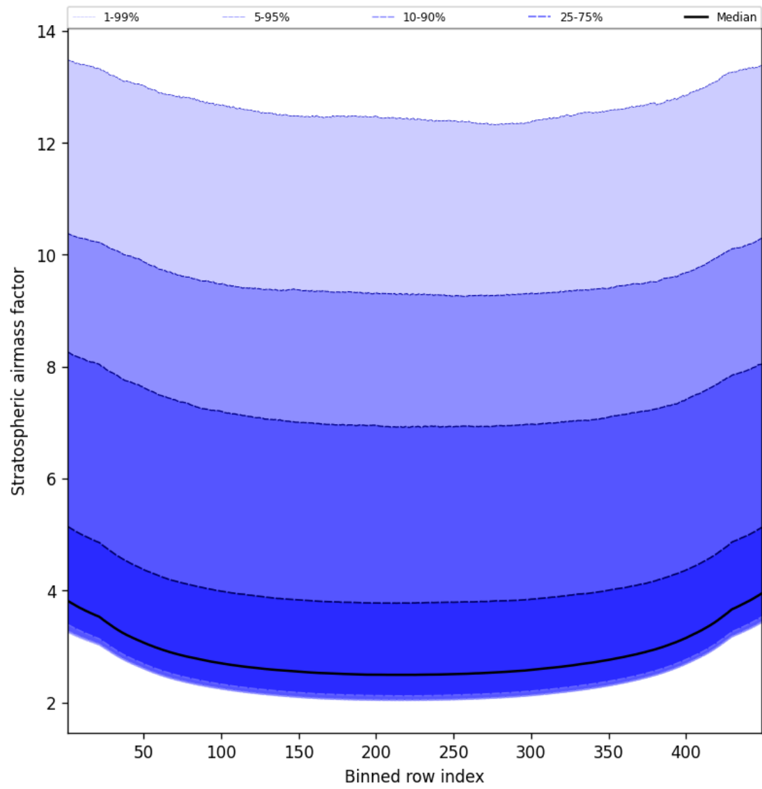
Figure 59: Along track statistics of “Stratospheric airmass factor” for 2025-02-19 to 2025-02-20
