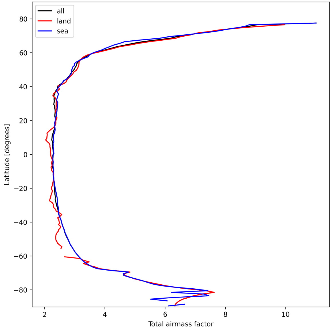
Figure 13: Zonal average of “Total airmass factor” for 2025-02-19 to 2025-02-20.
