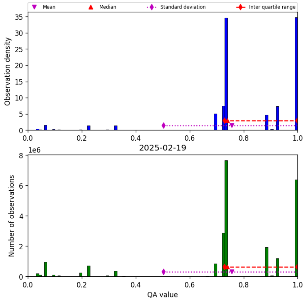
Figure 26: Histogram of “QA value” for 2025-02-19 to 2025-02-20
