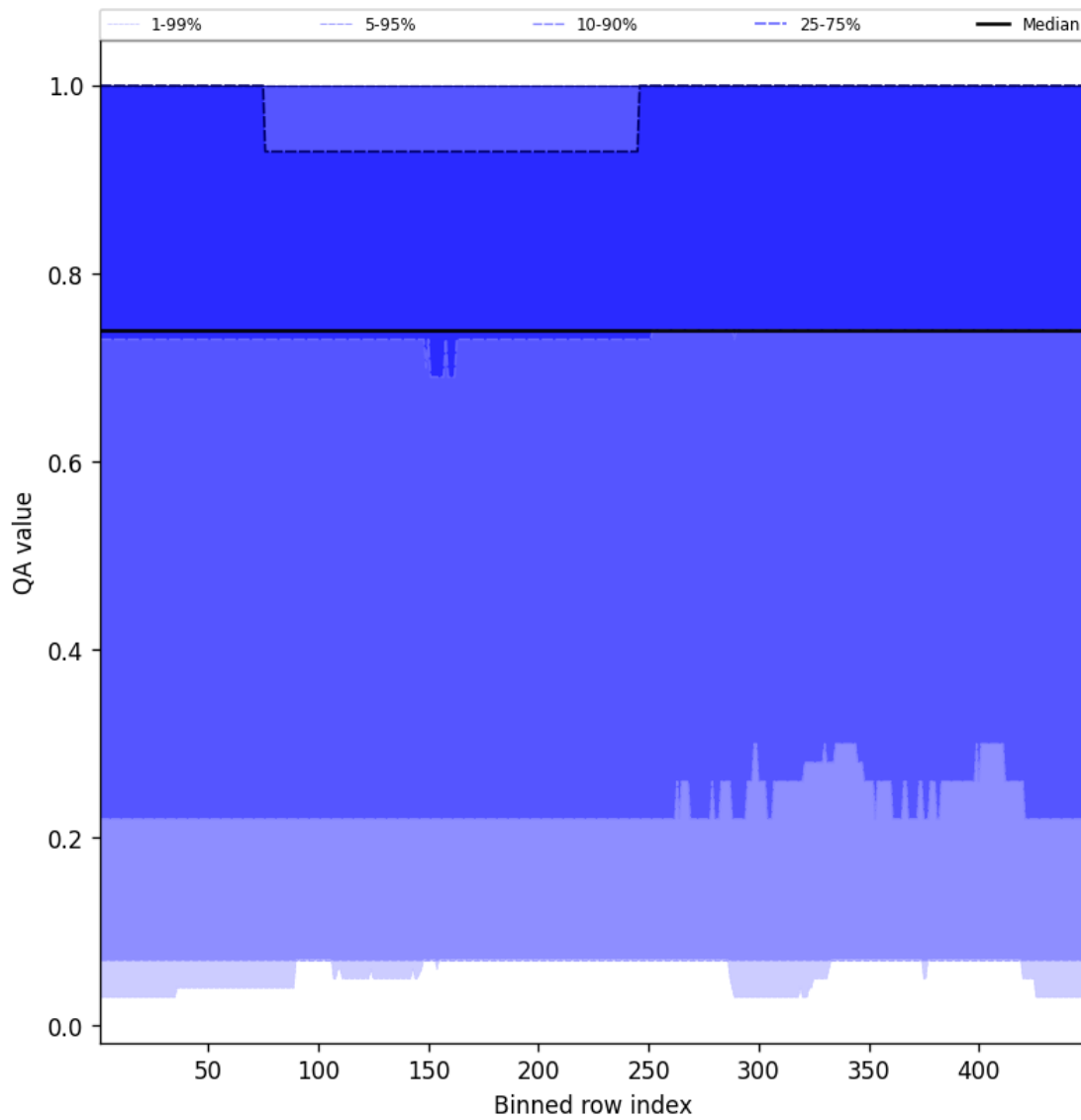
Figure 43: Along track statistics of “QA value” for 2025-02-19 to 2025-02-20
