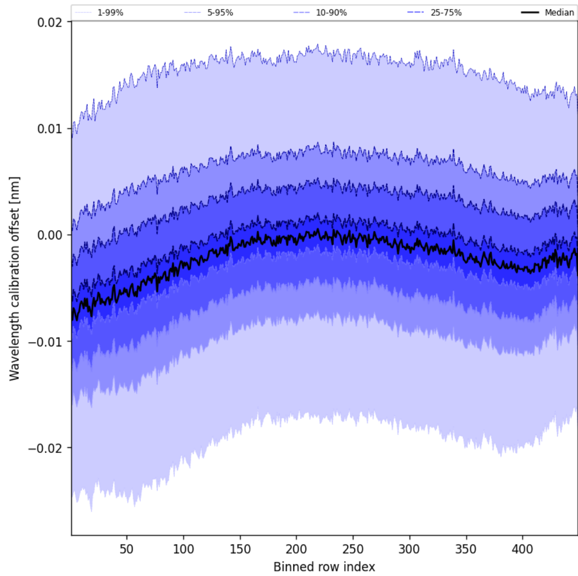
Figure 50: Along track statistics of “Wavelength calibration offset” for 2025-02-19 to 2025-02-20
