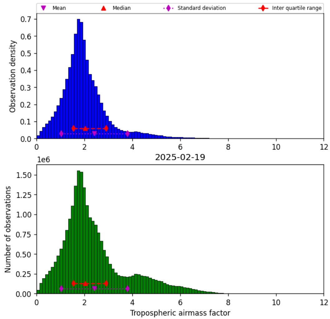
Figure 29: Histogram of “Tropospheric airmass factor” for 2025-02-19 to 2025-02-20
