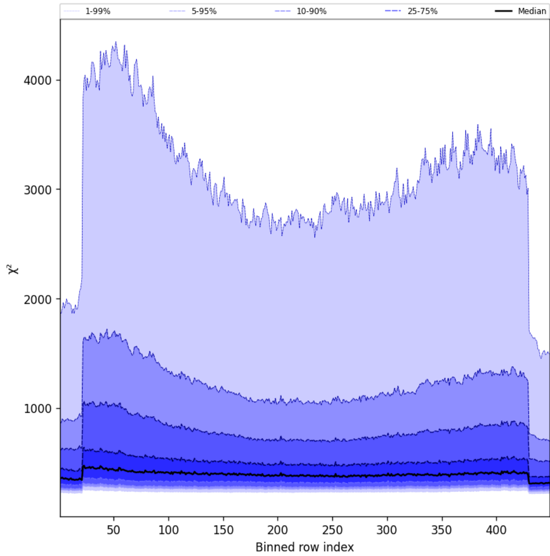
Figure 57: Along track statistics of “ \chi^2 ” for 2025-02-19 to 2025-02-20
