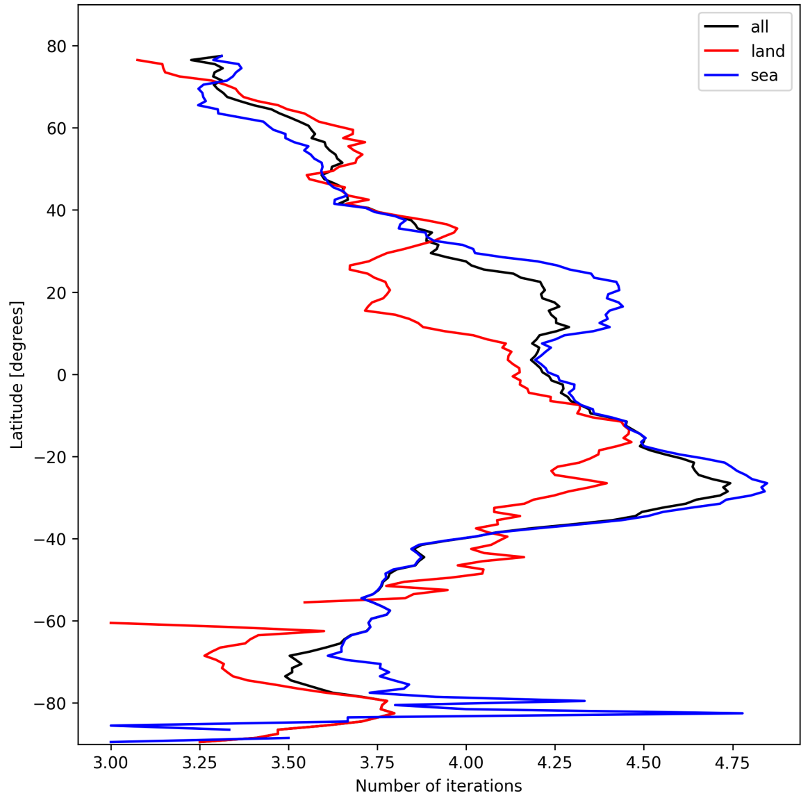
Figure 15: Zonal average of “Number of iterations” for 2025-02-19 to 2025-02-20.
