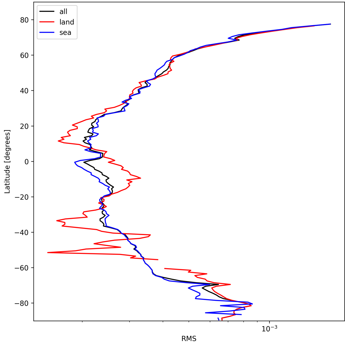
Figure 24: Zonal average of “RMS” for 2025-02-19 to 2025-02-20.
