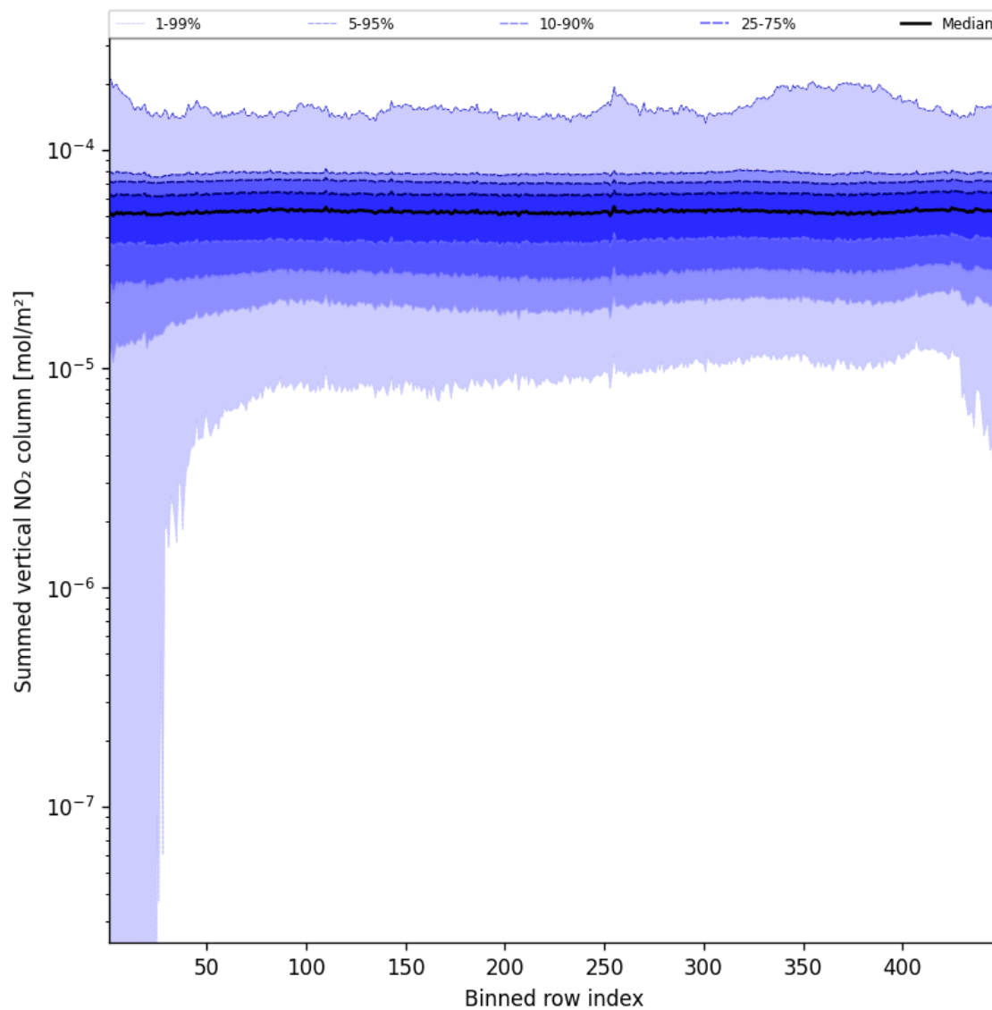
Figure 55: Along track statistics of “Summed vertical NO 2 column” for 2025-02-19 to 2025-02-20
