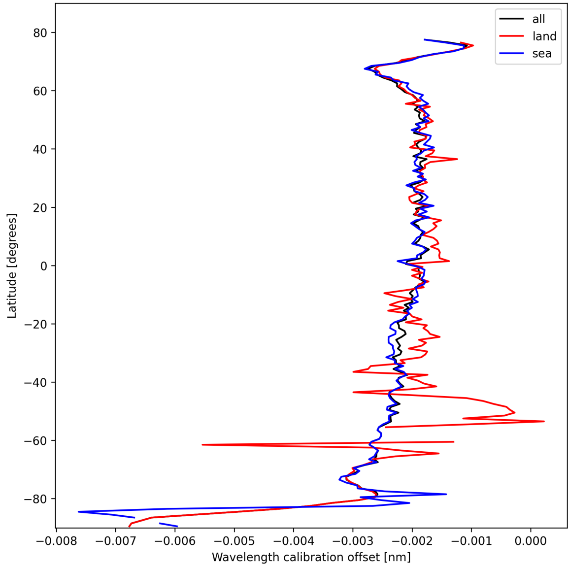
Figure 16: Zonal average of “Wavelength calibration offset” for 2025-02-19 to 2025-02-20.
