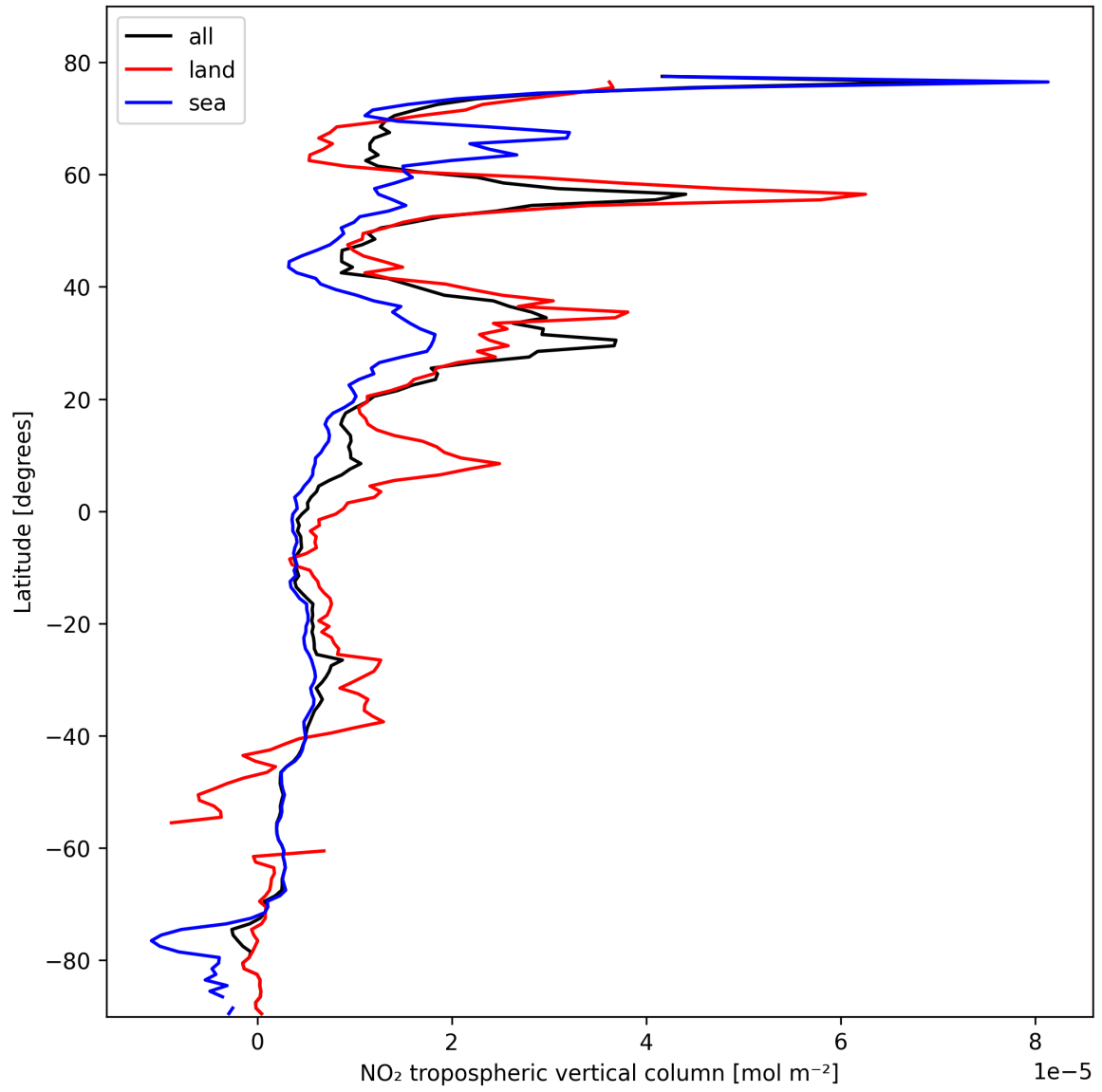
Figure 10: Zonal average of “NO 2 tropospheric vertical column” for 2025-02-19 to 2025-02-20.
