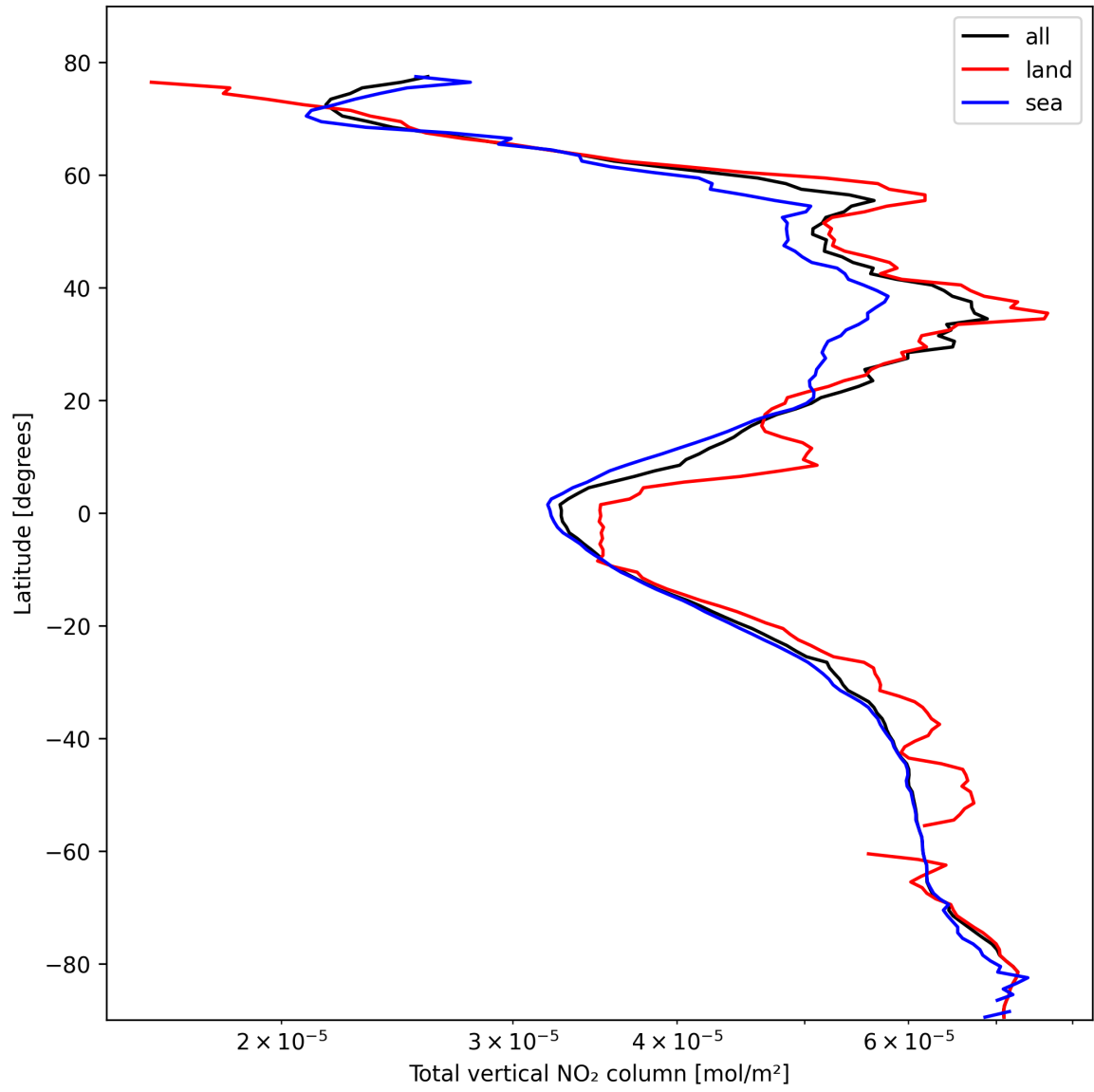
Figure 19: Zonal average of “Total vertical NO 2 column” for 2025-02-19 to 2025-02-20.
