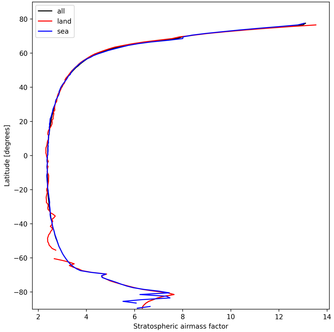
Figure 25: Zonal average of “Stratospheric airmass factor” for 2025-02-19 to 2025-02-20.
