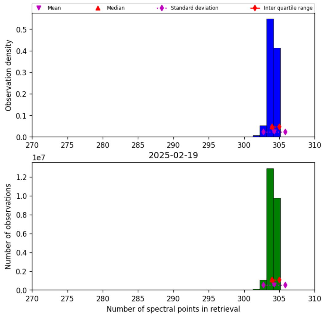
Figure 31: Histogram of “Number of spectral points in retrieval” for 2025-02-19 to 2025-02-20
