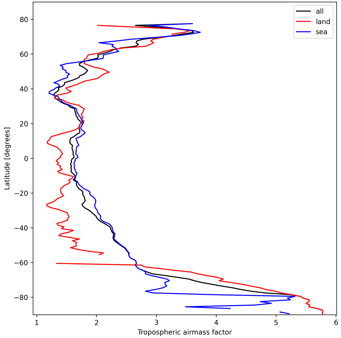
Figure 12: Zonal average of “Tropospheric airmass factor” for 2025-02-19 to 2025-02-20.
