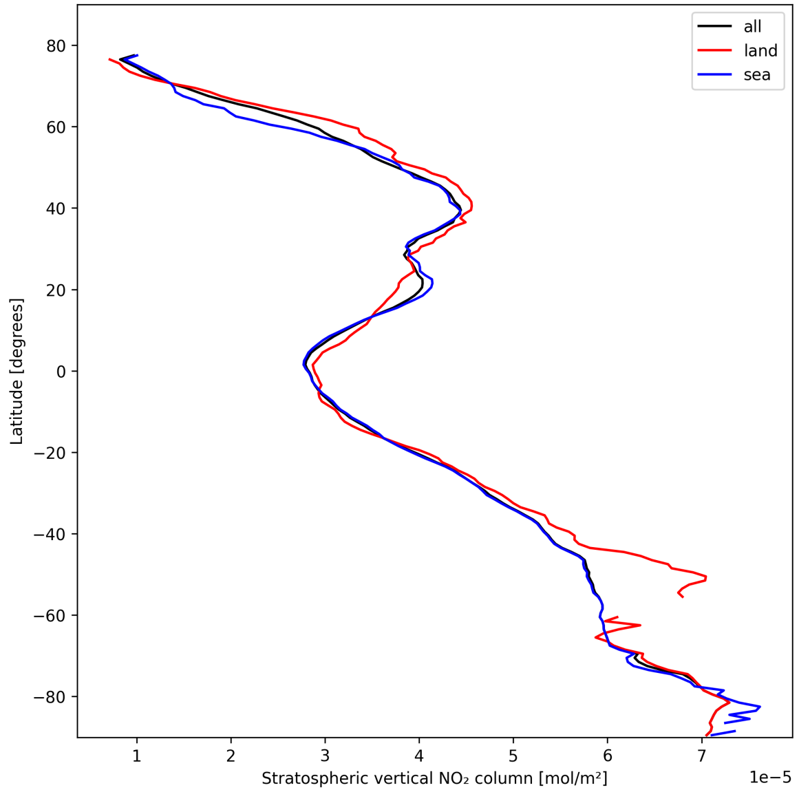
Figure 17: Zonal average of “Stratospheric vertical NO 2 column” for 2025-02-19 to 2025-02-20.
