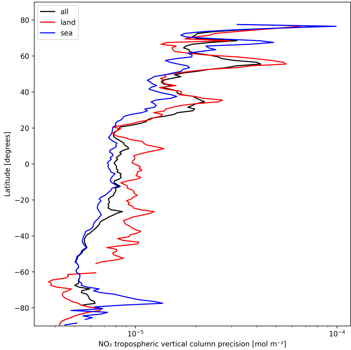
Figure 11: Zonal average of “NO 2 tropospheric vertical column precision” for 2025-02-19 to 2025-02-20.
