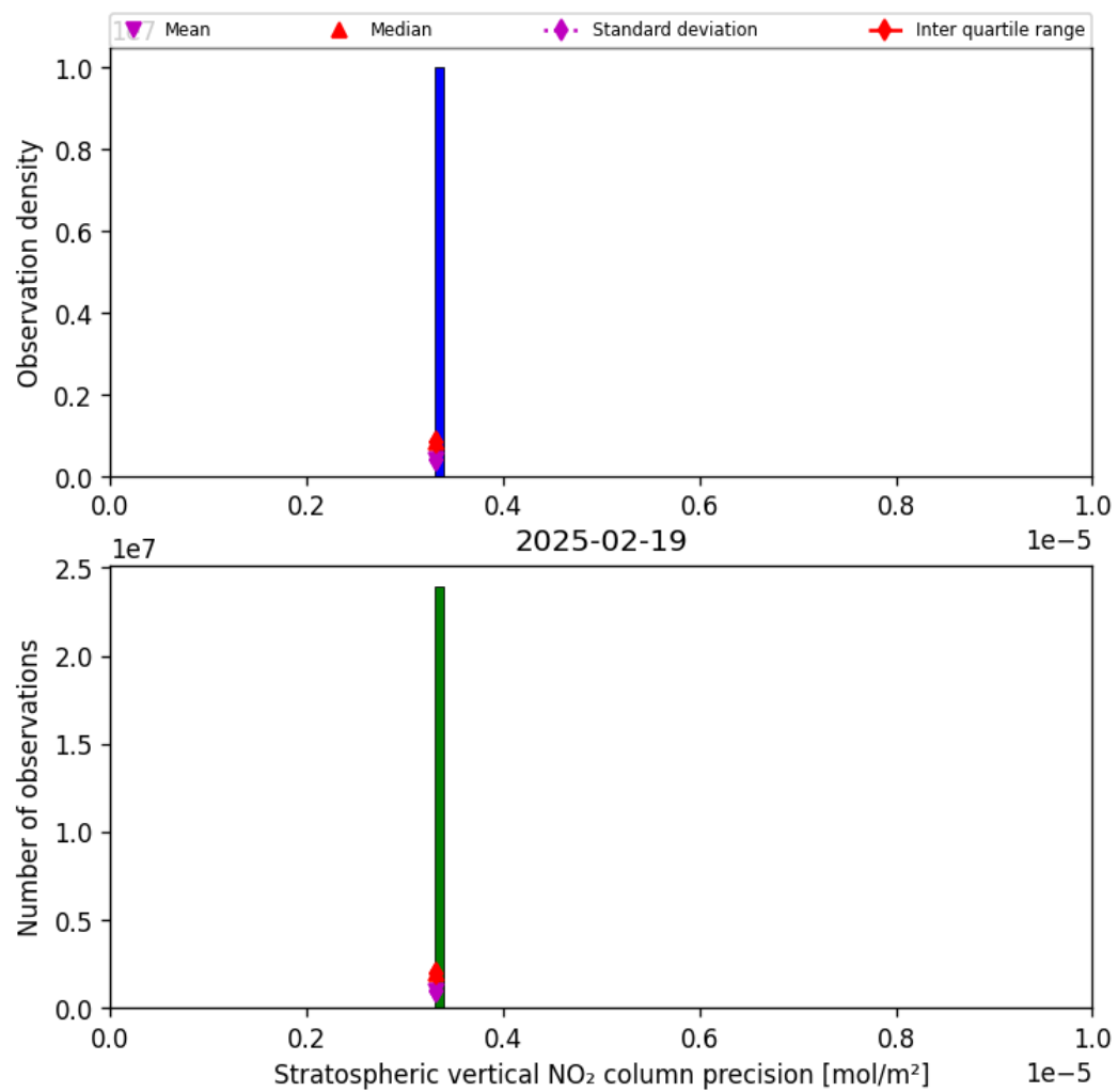
Figure 35: Histogram of “Stratospheric vertical NO 2 column precision” for 2025-02-19 to 2025-02-20
