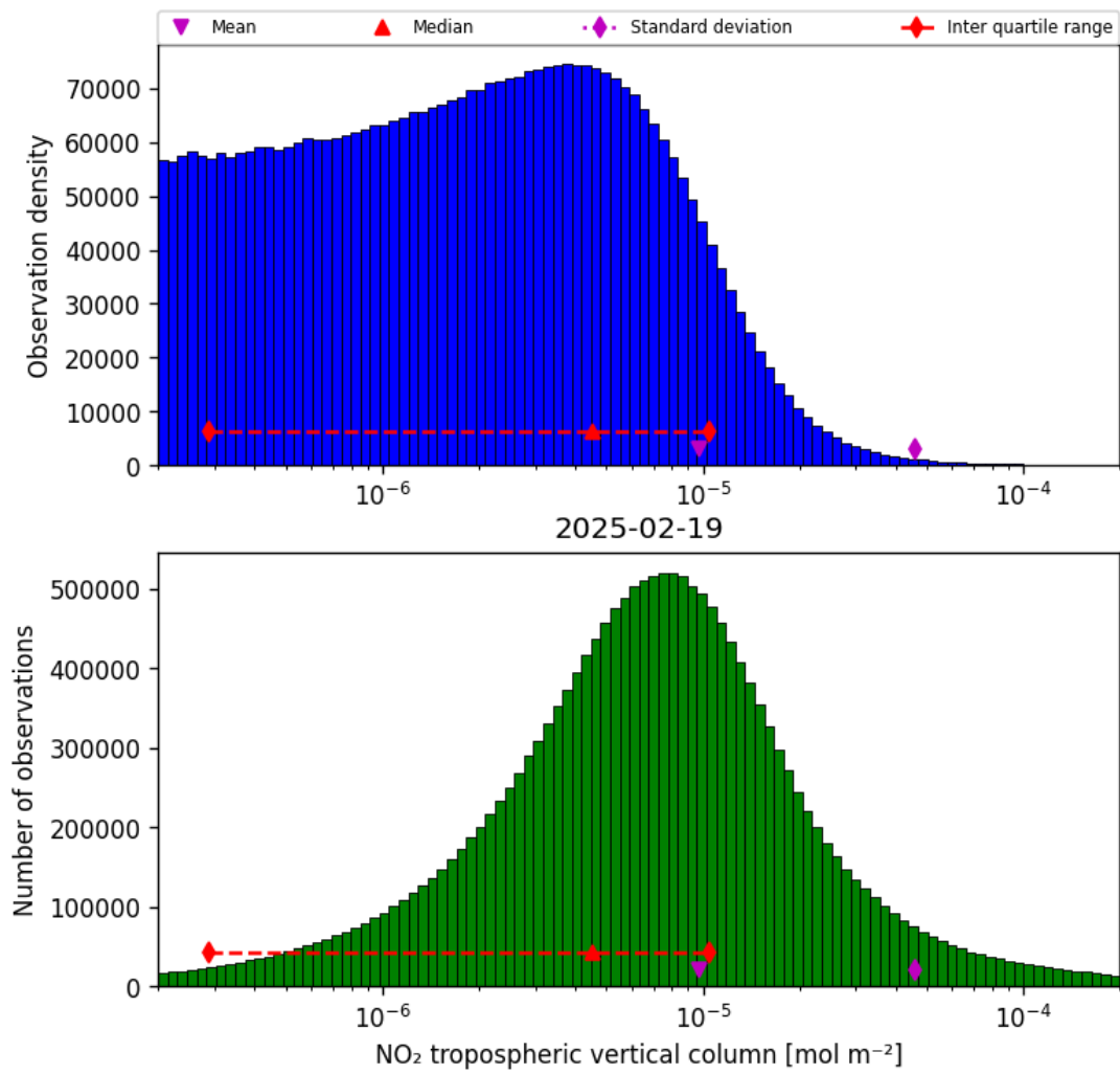
Figure 27: Histogram of “NO 2 tropospheric vertical column” for 2025-02-19 to 2025-02-20
