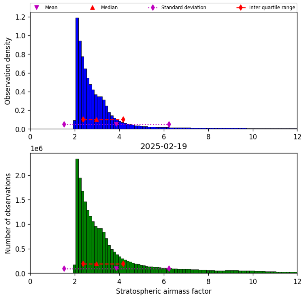
Figure 42: Histogram of “Stratospheric airmass factor” for 2025-02-19 to 2025-02-20
