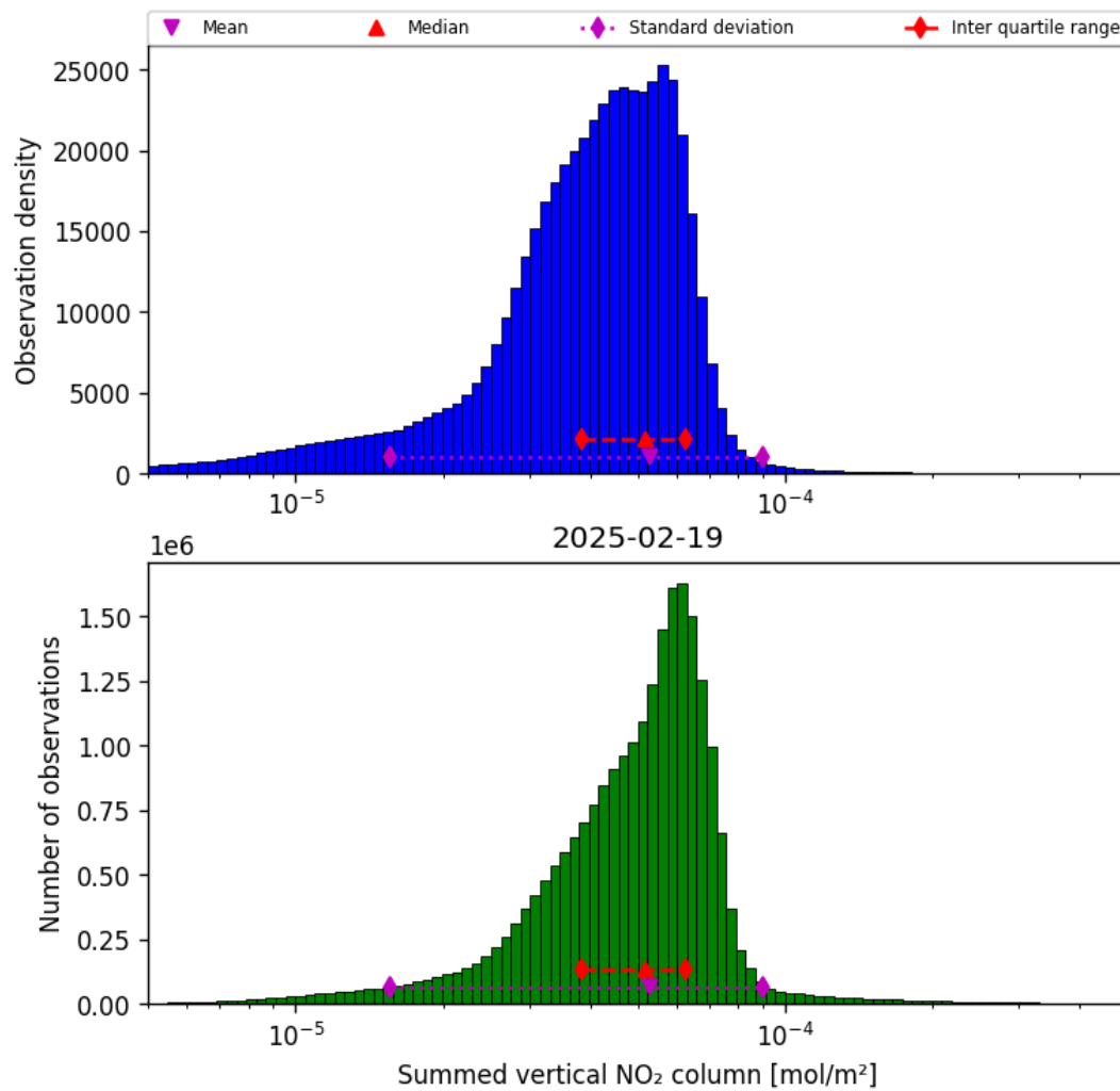
Figure 38: Histogram of “Summed vertical NO 2 column” for 2025-02-19 to 2025-02-20
