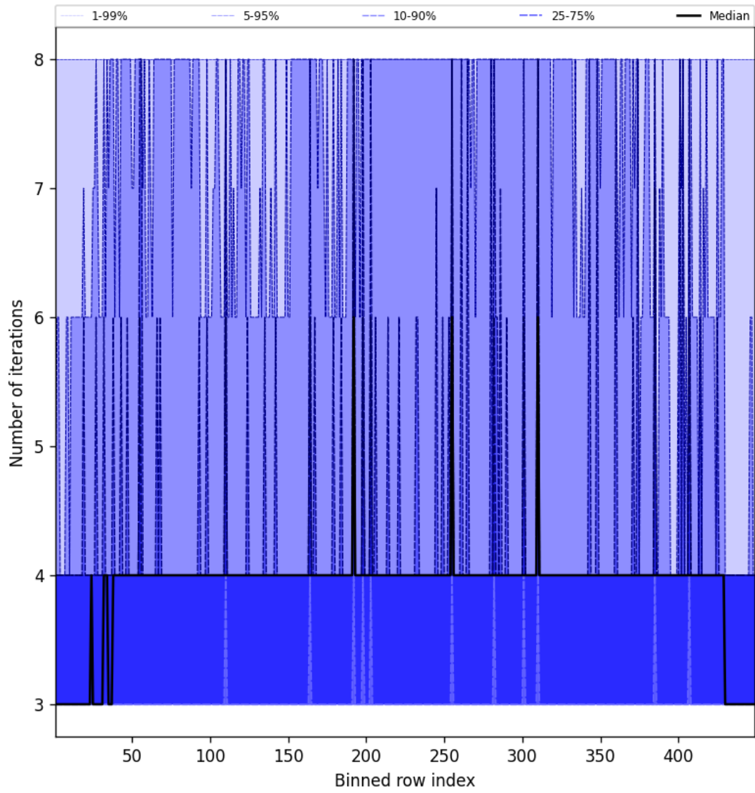
Figure 49: Along track statistics of “Number of iterations” for 2025-02-19 to 2025-02-20
