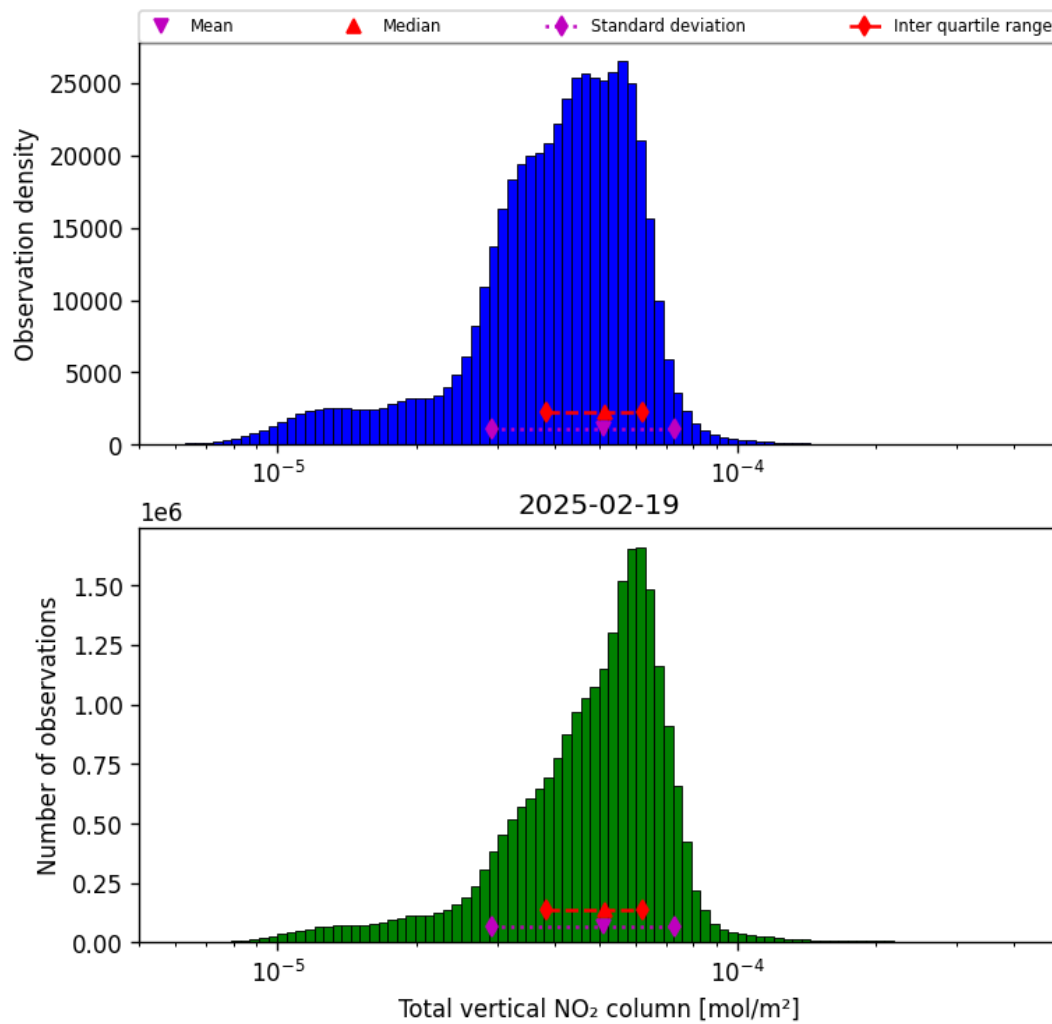
Figure 36: Histogram of “Total vertical NO 2 column” for 2025-02-19 to 2025-02-20
