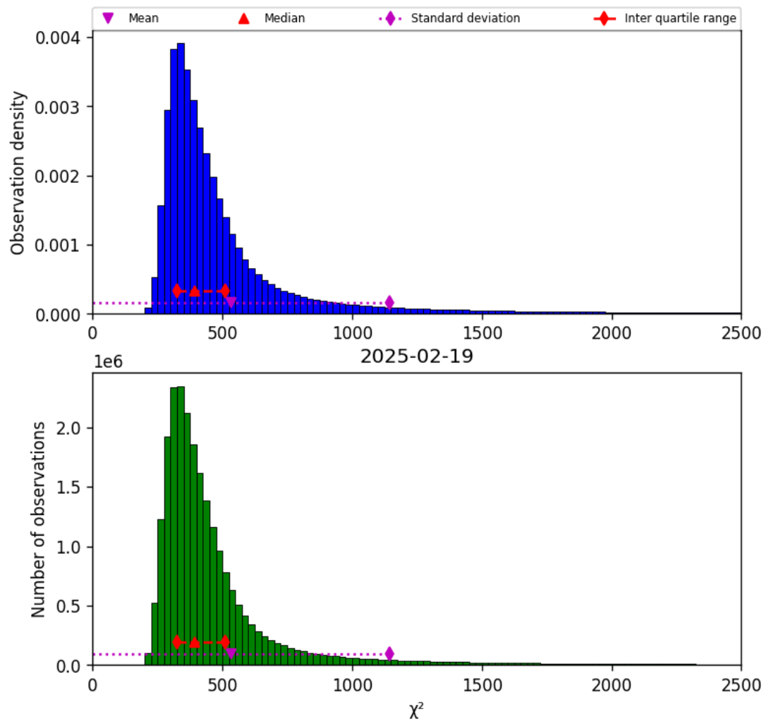
Figure 40: Histogram of “ \chi^2 ” for 2025-02-19 to 2025-02-20
