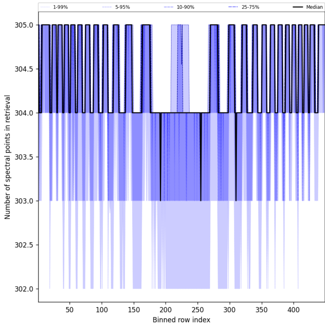
Figure 48: Along track statistics of “Number of spectral points in retrieval” for 2025-02-19 to 2025-02-20
