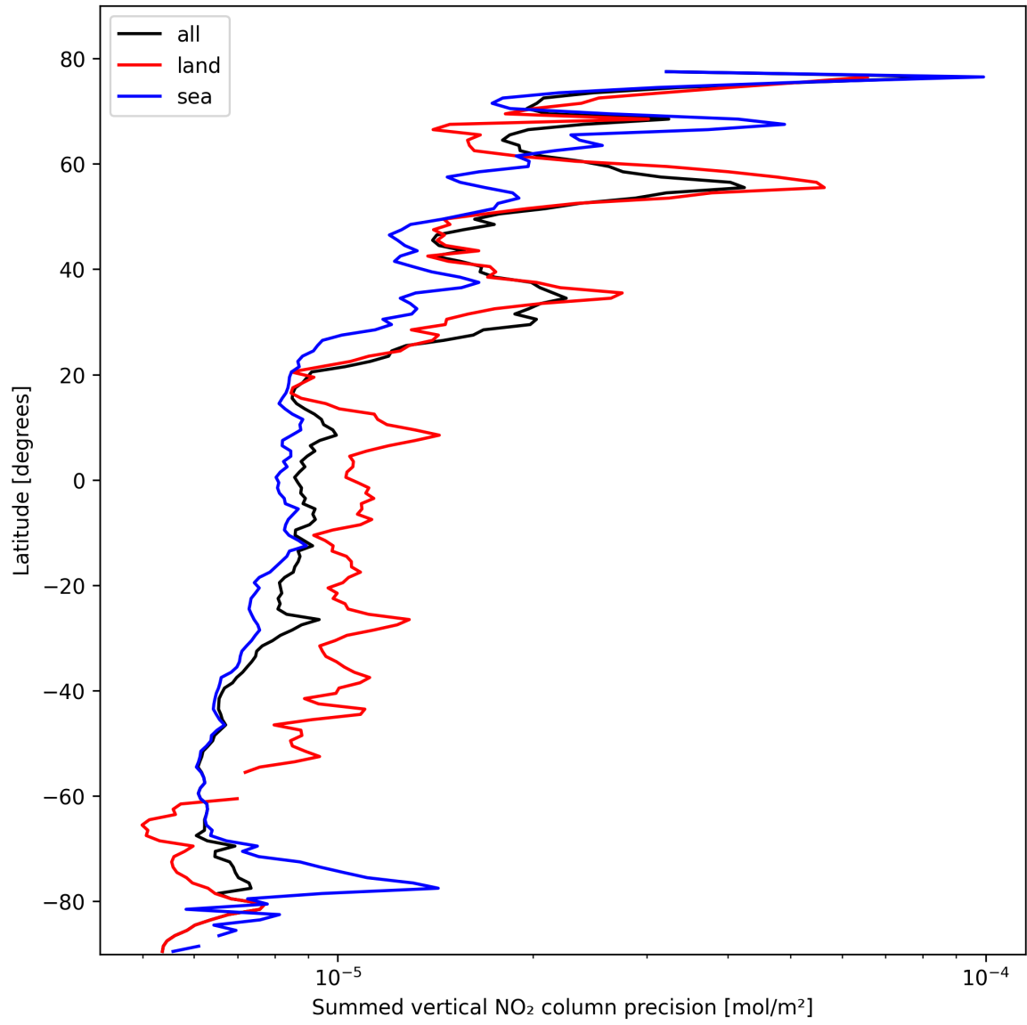
Figure 22: Zonal average of “Summed vertical NO 2 column precision” for 2025-02-19 to 2025-02-20.
