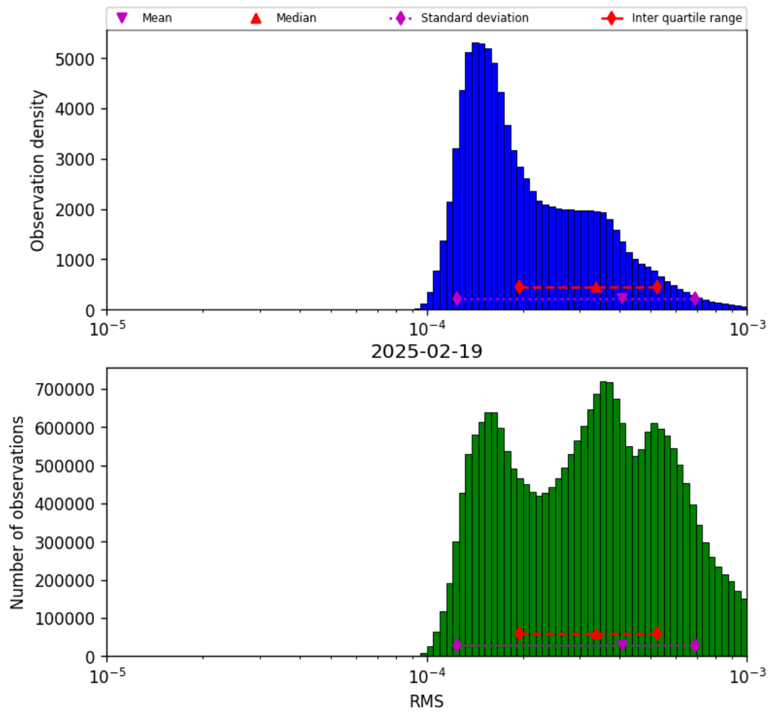
Figure 41: Histogram of “RMS” for 2025-02-19 to 2025-02-20
