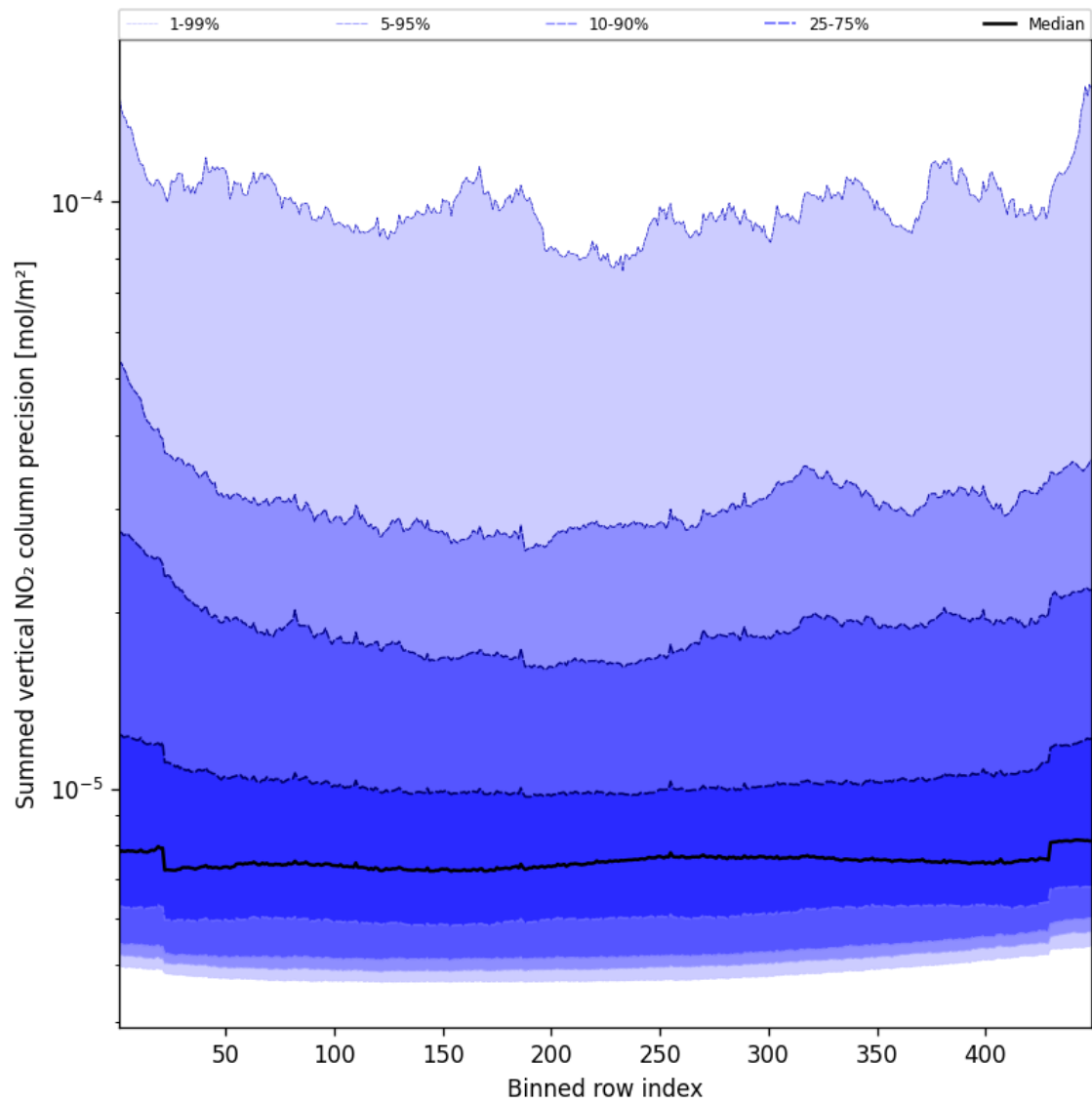
Figure 56: Along track statistics of “Summed vertical NO 2 column precision” for 2025-02-19 to 2025-02-20
