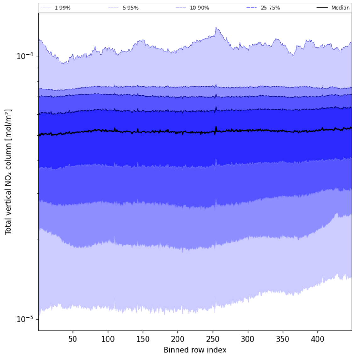
Figure 53: Along track statistics of “Total vertical NO 2 column” for 2025-02-19 to 2025-02-20
