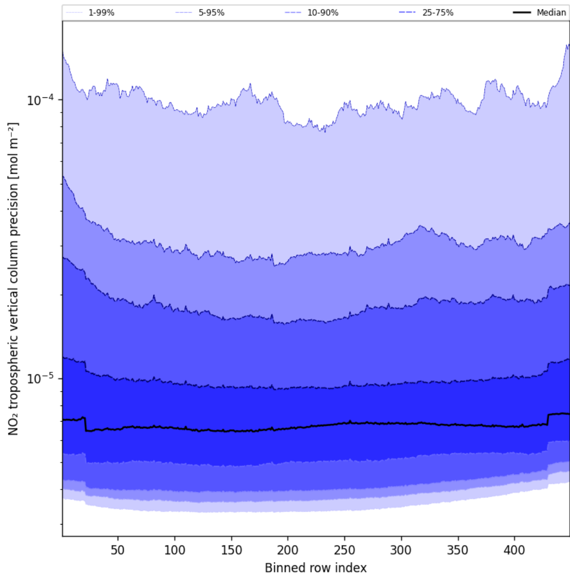
Figure 45: Along track statistics of “NO 2 tropospheric vertical column precision” for 2025-02-19 to 2025-02-20
