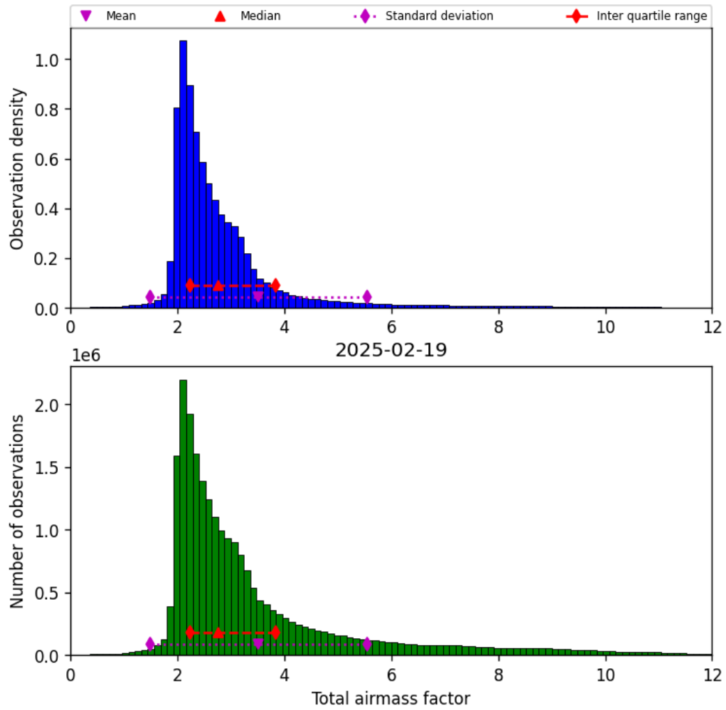
Figure 30: Histogram of “Total airmass factor” for 2025-02-19 to 2025-02-20
