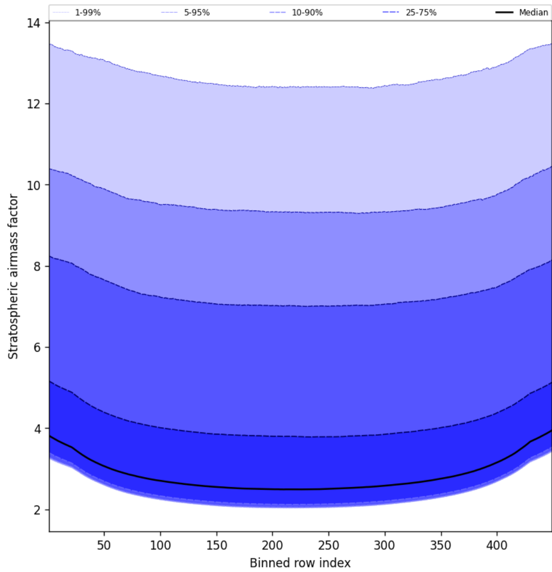
Figure 59: Along track statistics of “Stratospheric airmass factor” for 2025-02-20 to 2025-02-21
