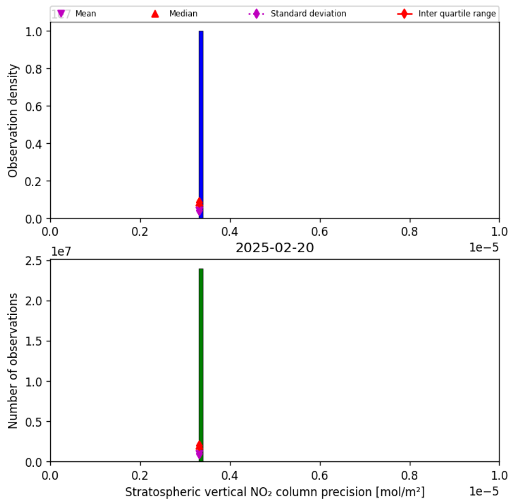
Figure 35: Histogram of “Stratospheric vertical NO 2 column precision” for 2025-02-20 to 2025-02-21
