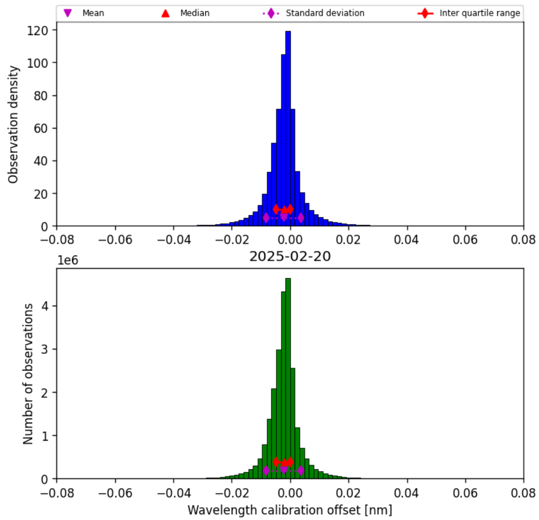
Figure 33: Histogram of “Wavelength calibration offset” for 2025-02-20 to 2025-02-21
