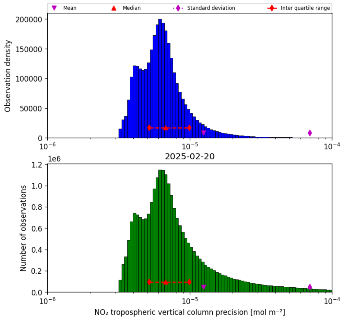
Figure 28: Histogram of “NO 2 tropospheric vertical column precision” for 2025-02-20 to 2025-02-21
