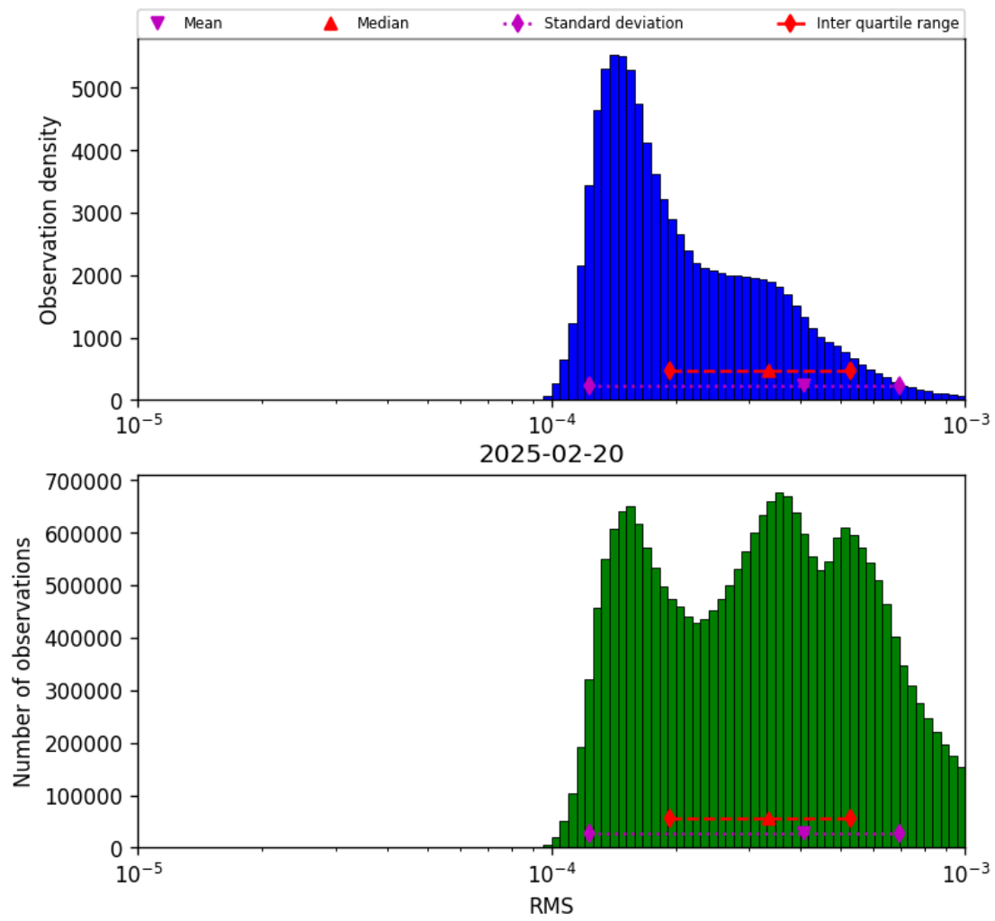
Figure 41: Histogram of “RMS” for 2025-02-20 to 2025-02-21
