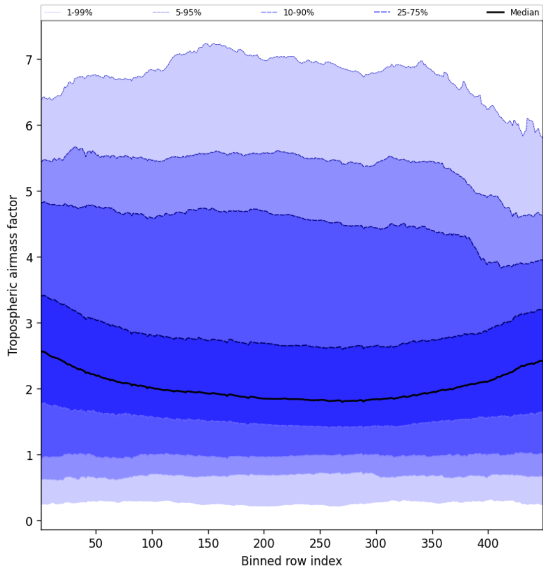
Figure 46: Along track statistics of “Tropospheric air mass factor” for 2025-02-20 to 2025-02-21
