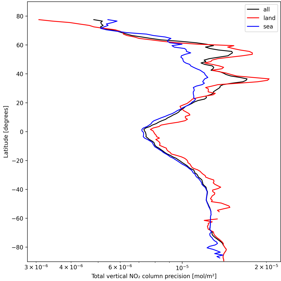
Figure 20: Zonal average of "Total vertical NO 2 column precision" for 2025-02-20 to 2025-02-21.
