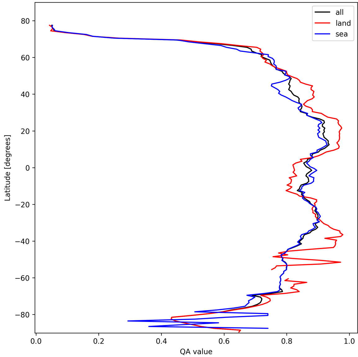
Figure 9: Zonal average of “QA value” for 2025-02-20 to 2025-02-21.
