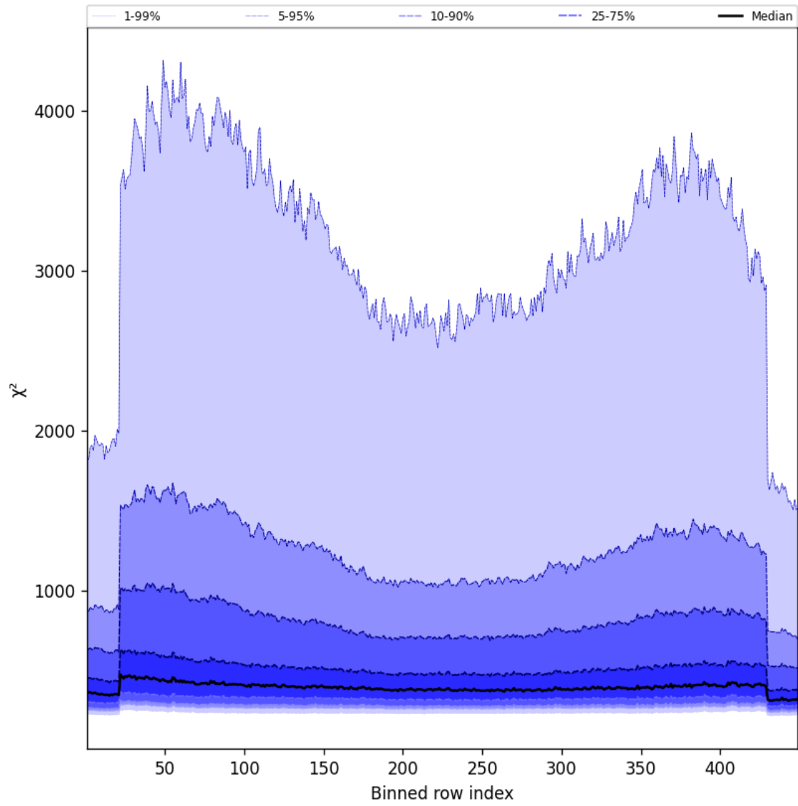
Figure 57: Along track statistics of “ \chi^2 ” for 2025-02-20 to 2025-02-21
