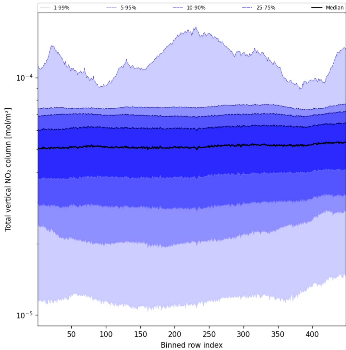
Figure 53: Along track statistics of “Total vertical NO 2 column” for 2025-02-20 to 2025-02-21
