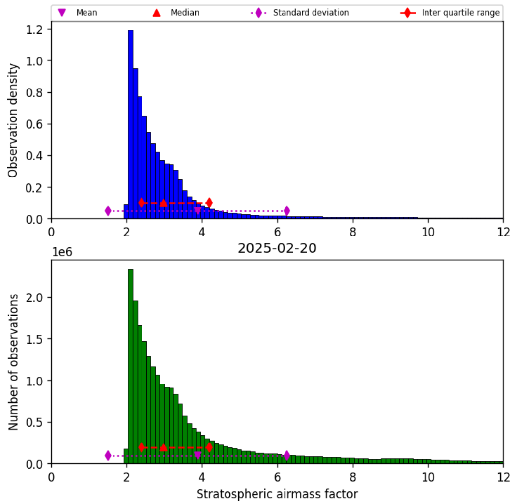
Figure 42: Histogram of “Stratospheric airmass factor” for 2025-02-20 to 2025-02-21
