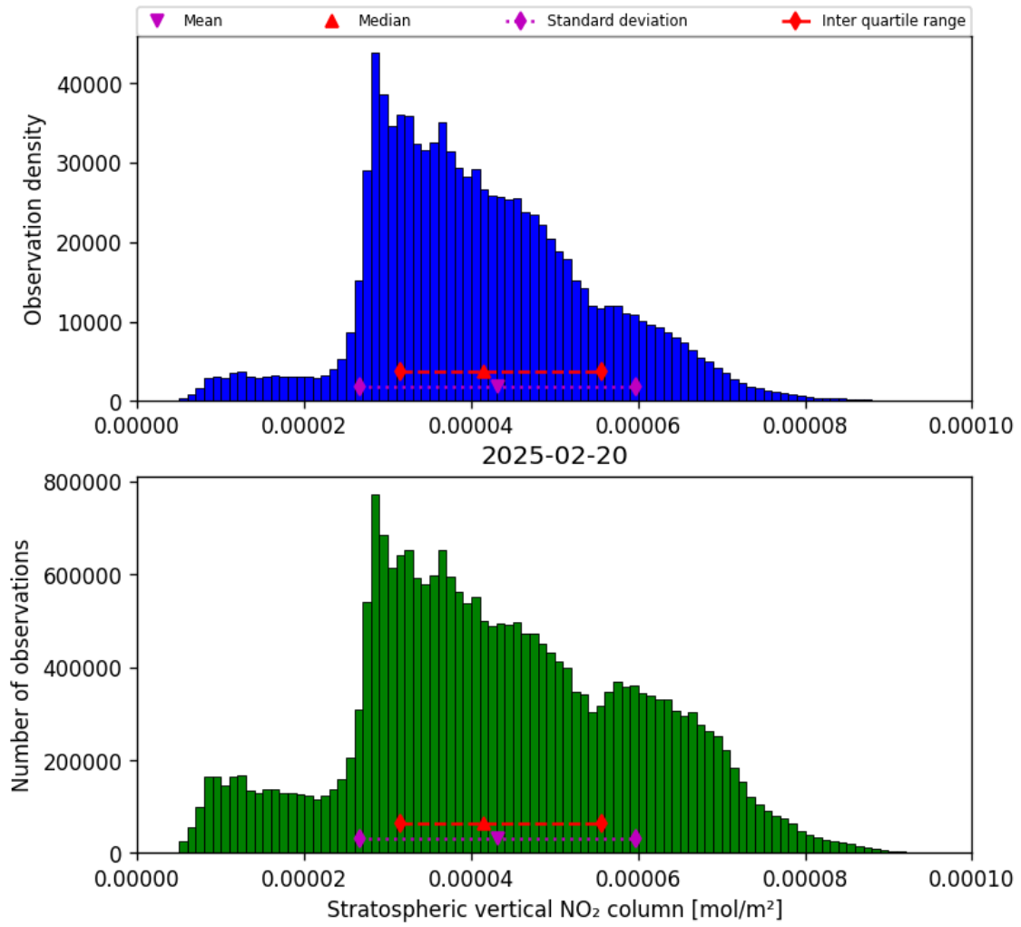
Figure 34: Histogram of “Stratospheric vertical NO 2 column” for 2025-02-20 to 2025-02-21
