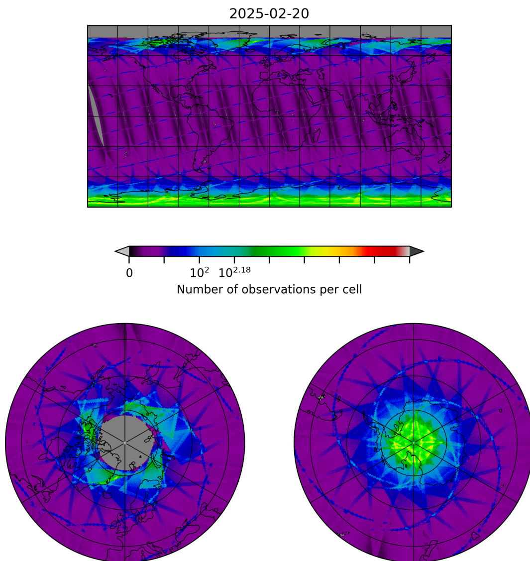
Figure 8: Map of the number of observations for 2025-02-20 to 2025-02-21
