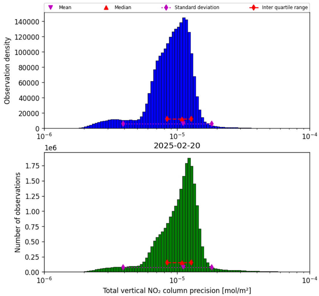
Figure 37: Histogram of “Total vertical NO 2 column precision” for 2025-02-20 to 2025-02-21
