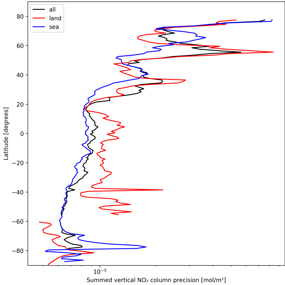
Figure 22: Zonal average of “Summed vertical NO 2 column precision” for 2025-02-20 to 2025-02-21.
