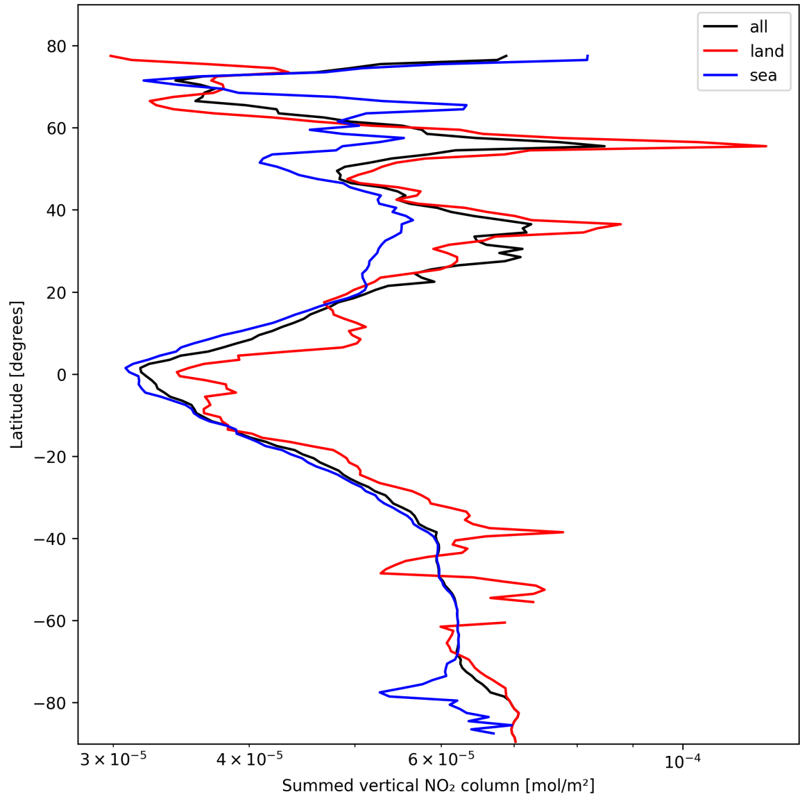
Figure 21: Zonal average of “Summed vertical NO 2 column” for 2025-02-20 to 2025-02-21.
