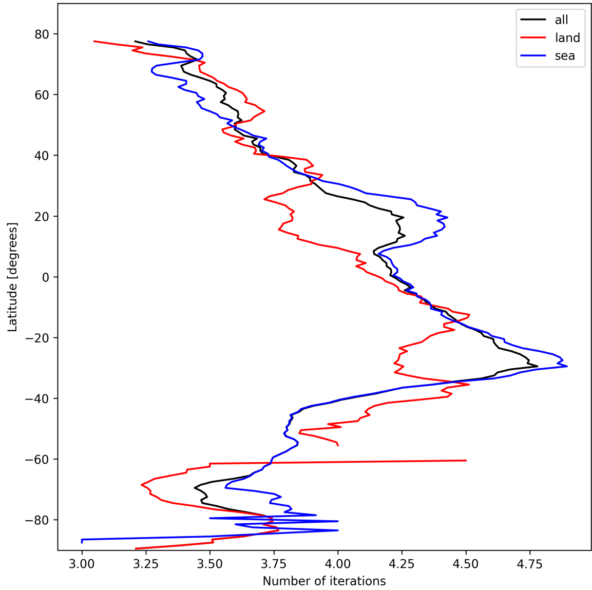
Figure 15: Zonal average of “Number of iterations” for 2025-02-20 to 2025-02-21.
