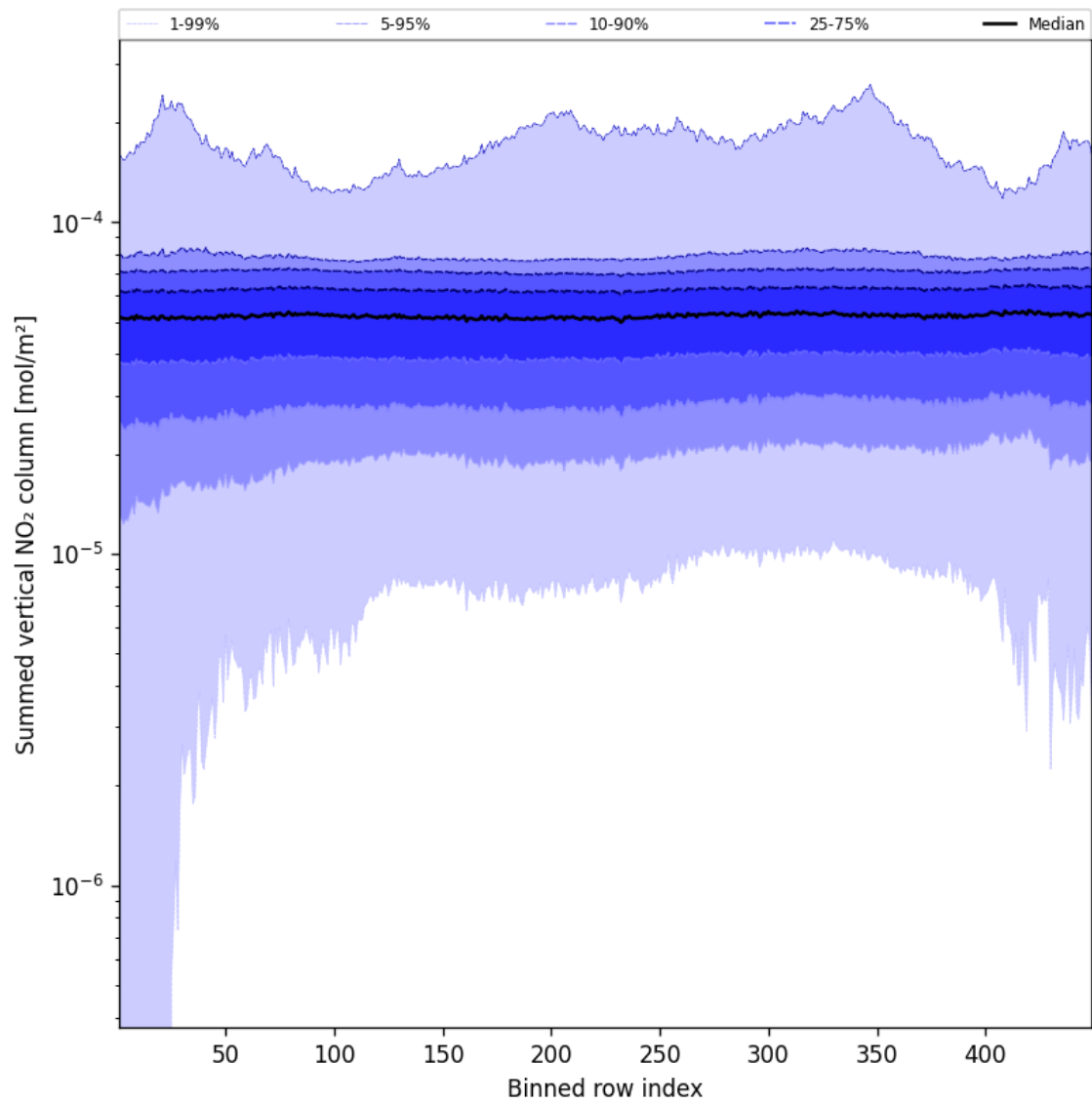
Figure 55: Along track statistics of “Summed vertical NO 2 column” for 2025-02-20 to 2025-02-21
