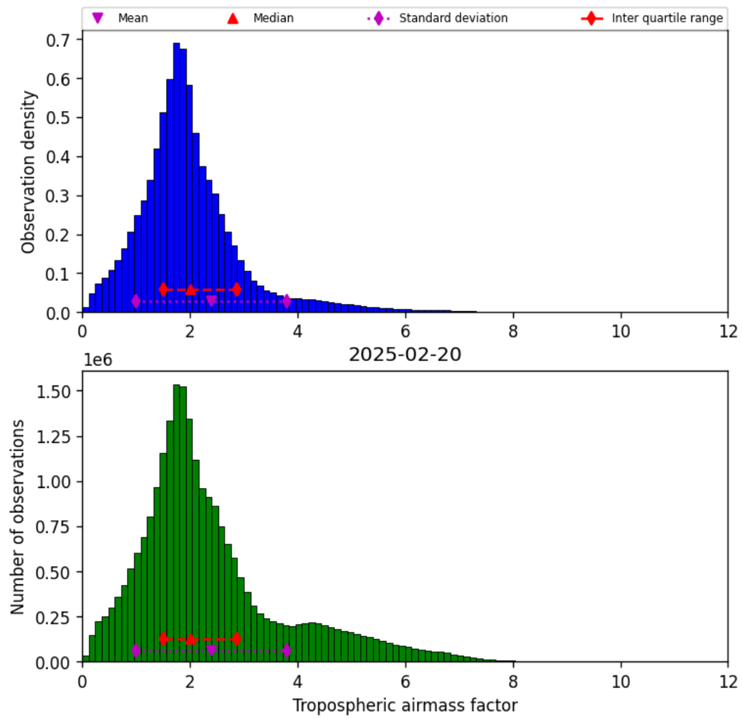
Figure 29: Histogram of “Tropospheric airmass factor” for 2025-02-20 to 2025-02-21
