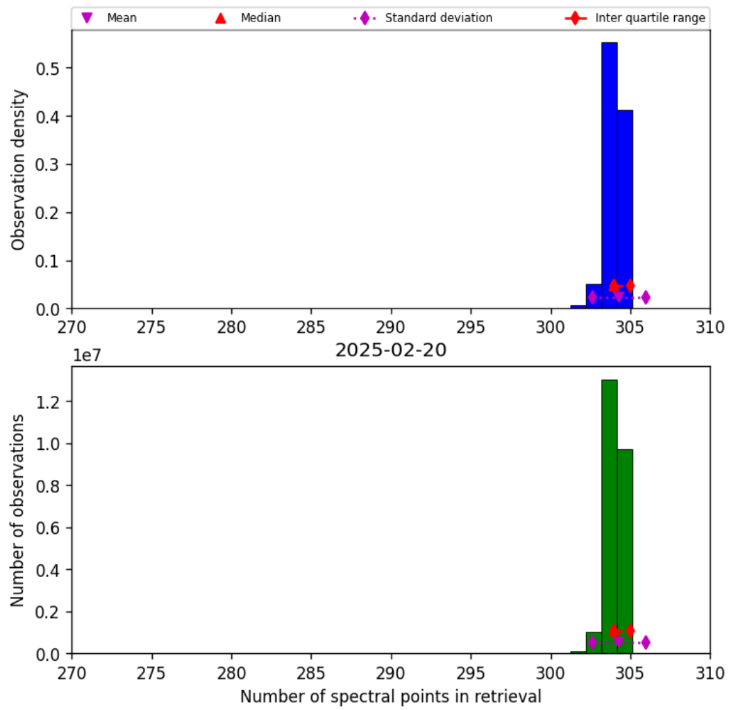
Figure 31: Histogram of “Number of spectral points in retrieval” for 2025-02-20 to 2025-02-21
