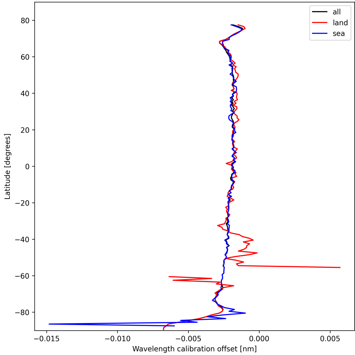
Figure 16: Zonal average of “Wavelength calibration offset” for 2025-02-20 to 2025-02-21.
