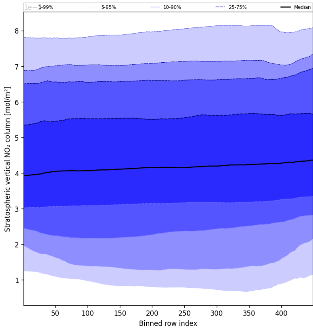
Figure 51: Along track statistics of “Stratospheric vertical NO 2 column” for 2025-02-20 to 2025-02-21
