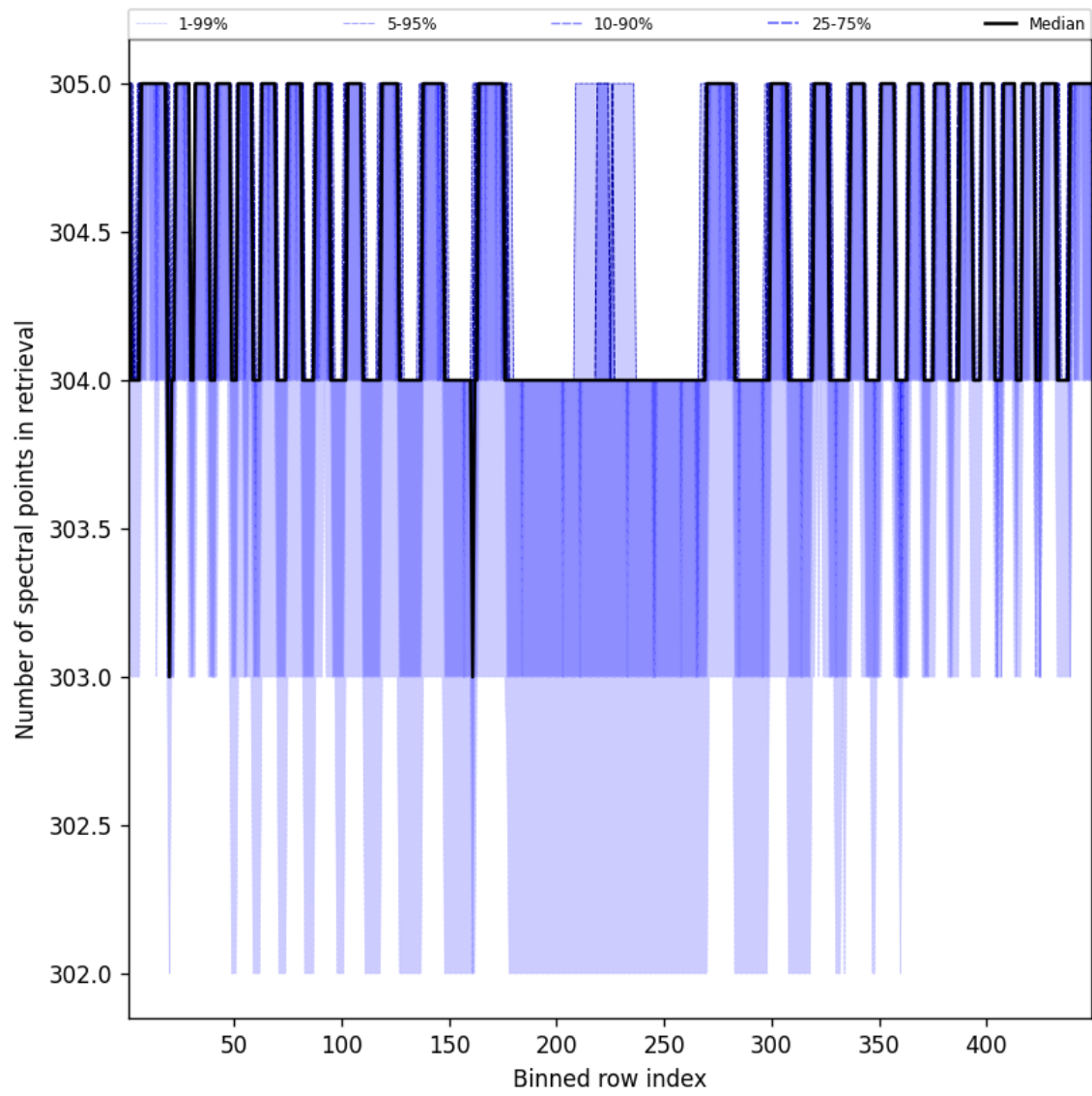
Figure 48: Along track statistics of “Number of spectral points in retrieval” for 2025-02-20 to 2025-02-21
