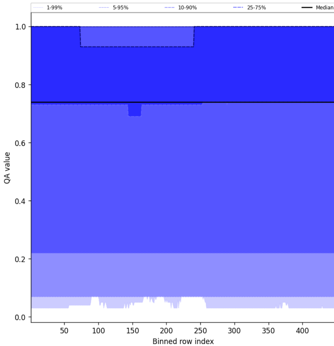
Figure 43: Along track statistics of “QA value” for 2025-02-20 to 2025-02-21
