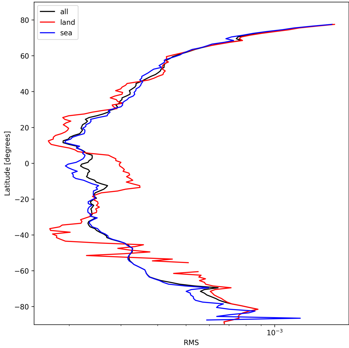
Figure 24: Zonal average of “RMS” for 2025-02-20 to 2025-02-21.
