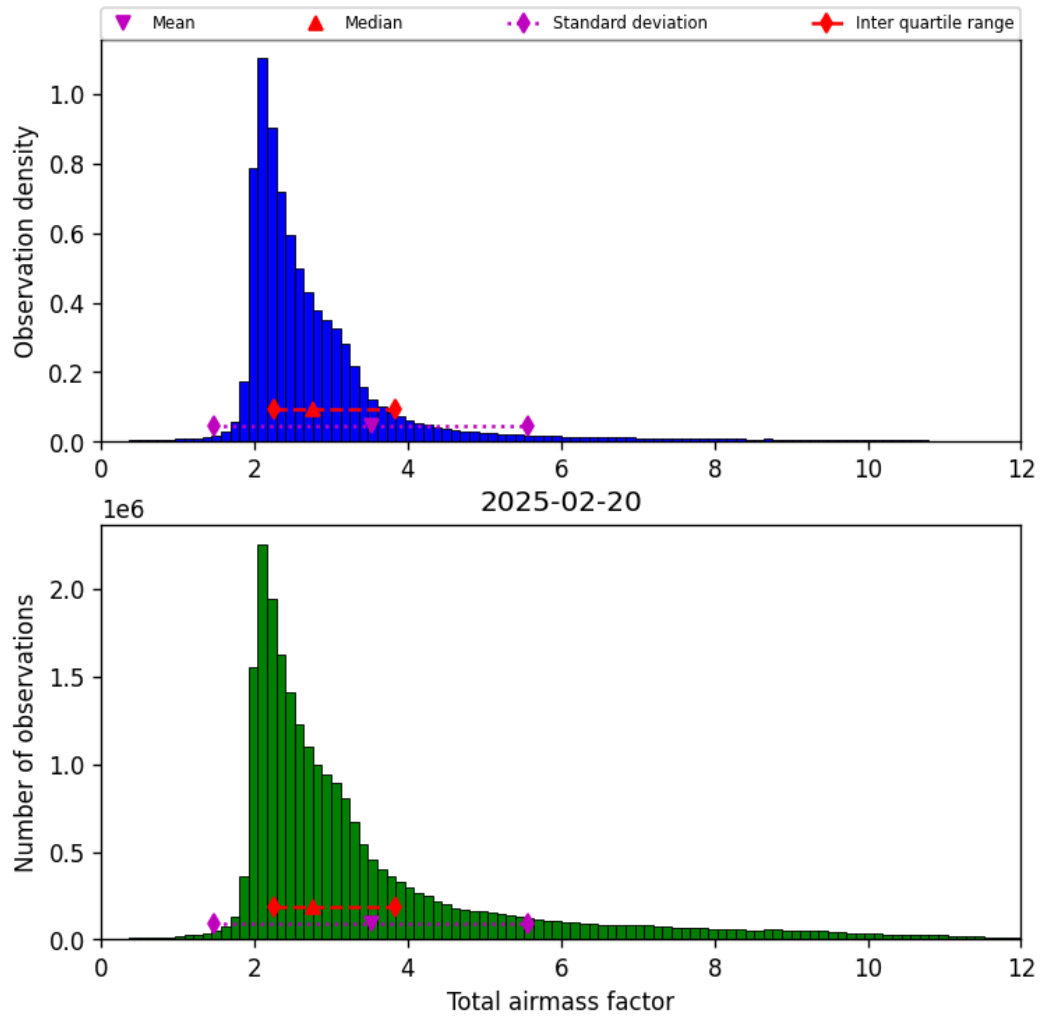
Figure 30: Histogram of “Total airmass factor” for 2025-02-20 to 2025-02-21
