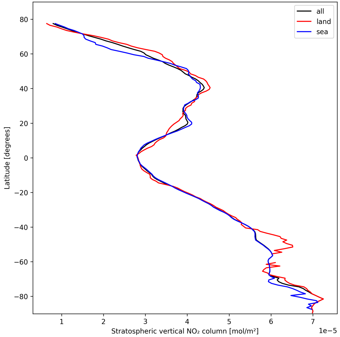
Figure 17: Zonal average of “Stratospheric vertical NO 2 column” for 2025-02-20 to 2025-02-21.
