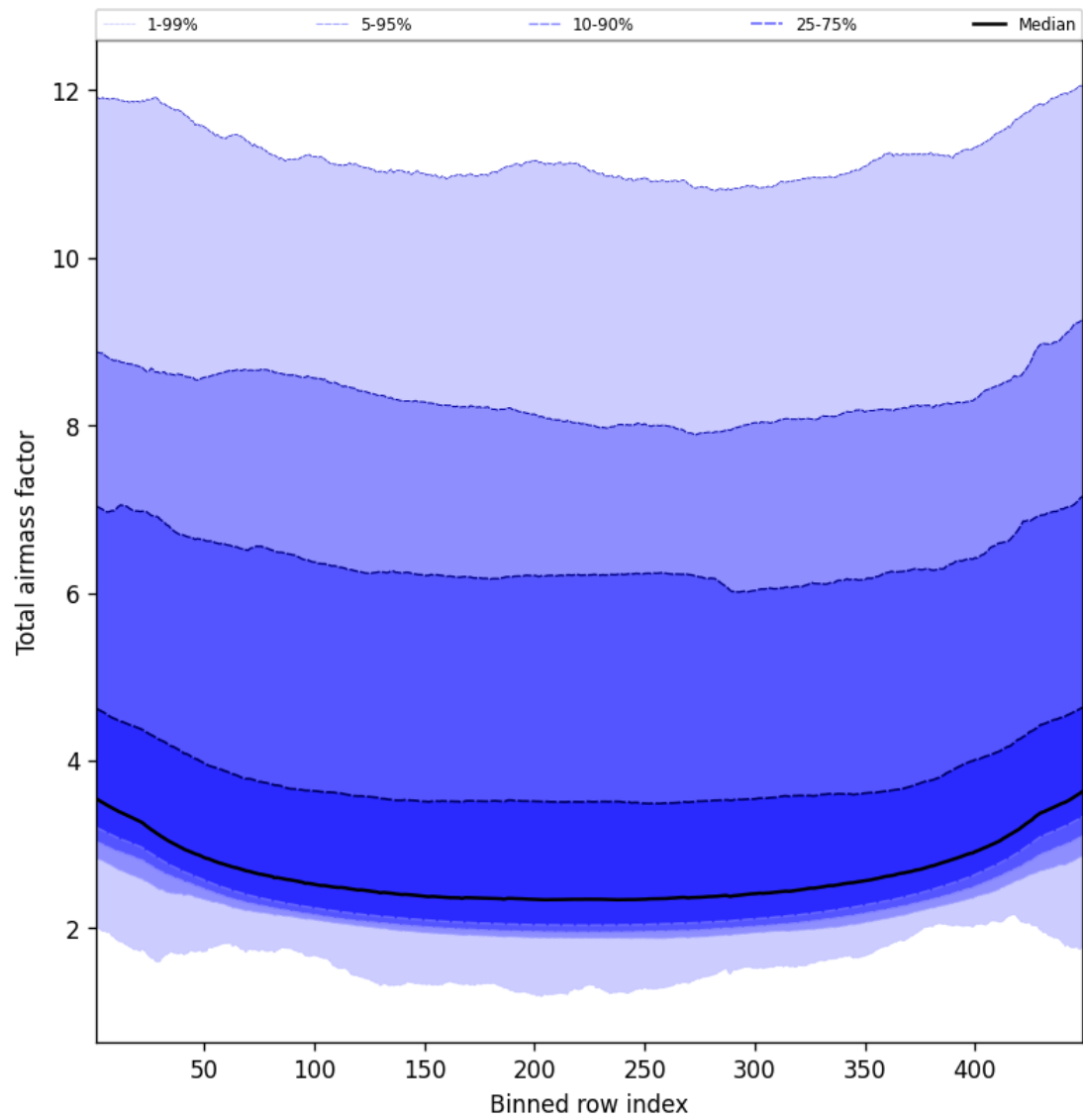
Figure 47: Along track statistics of “Total airmass factor” for 2025-02-20 to 2025-02-21
