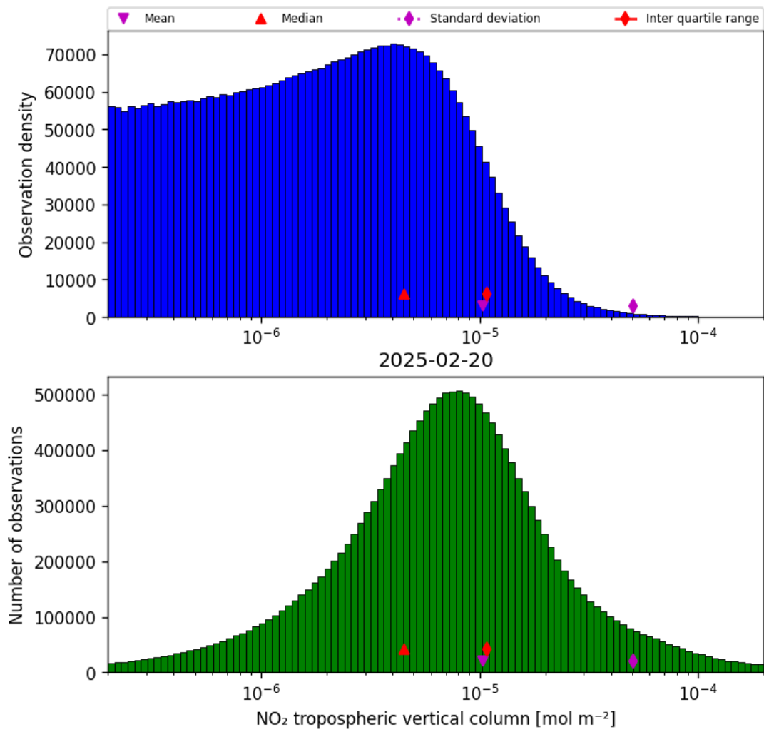
Figure 27: Histogram of “NO 2 tropospheric vertical column” for 2025-02-20 to 2025-02-21
