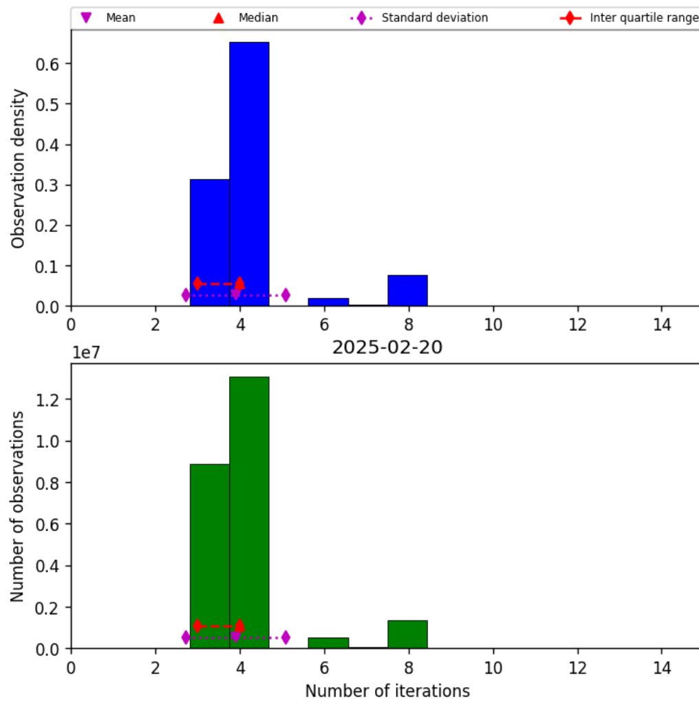
Figure 32: Histogram of “Number of iterations” for 2025-02-20 to 2025-02-21
