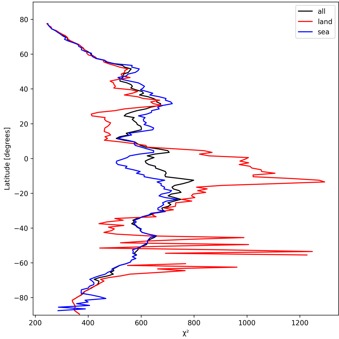
Figure 23: Zonal average of “ \chi^2 ” for 2025-02-20 to 2025-02-21.
