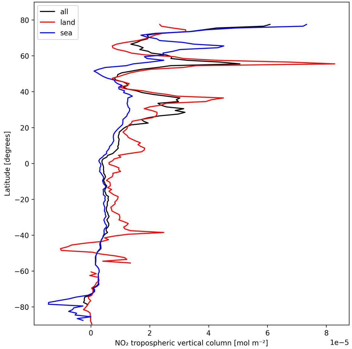
Figure 10: Zonal average of “NO 2 tropospheric vertical column” for 2025-02-20 to 2025-02-21.
