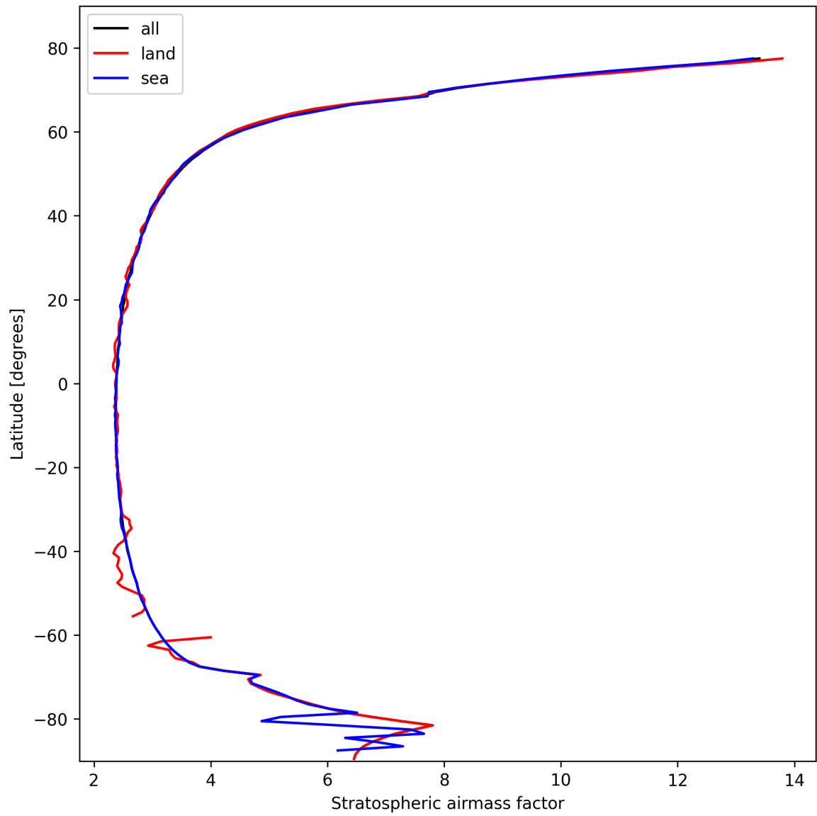
Figure 25: Zonal average of “Stratospheric airmass factor” for 2025-02-20 to 2025-02-21.
