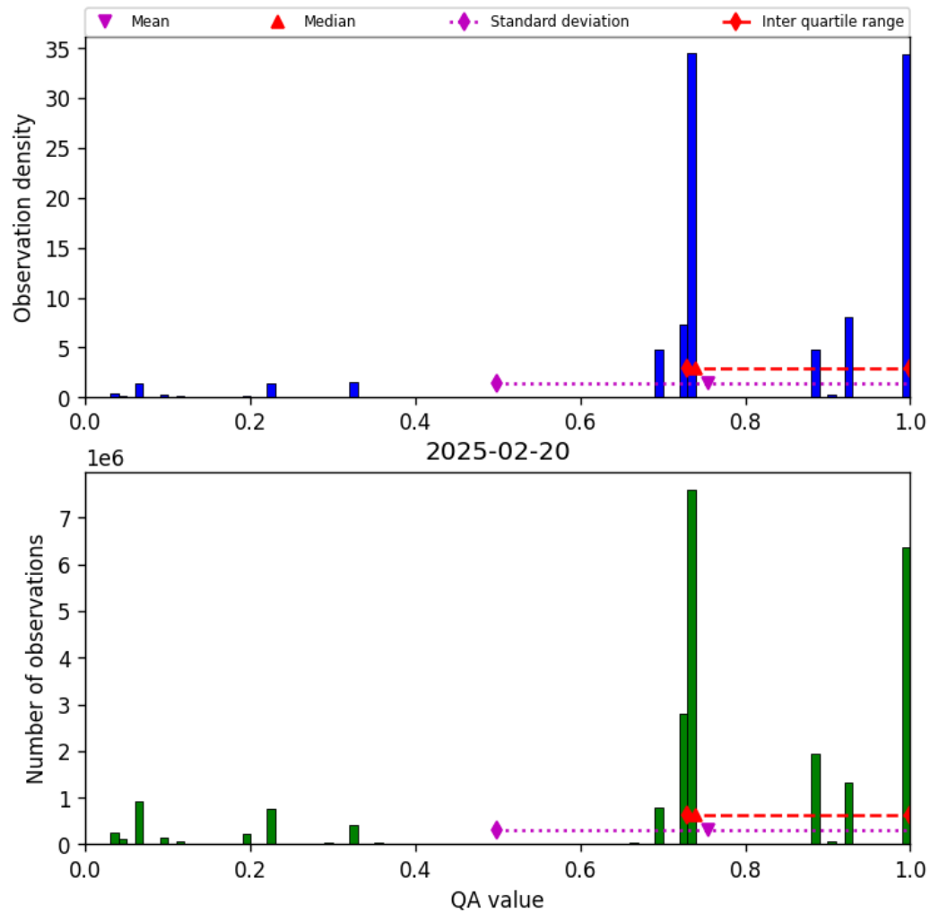
Figure 26: Histogram of “QA value” for 2025-02-20 to 2025-02-21
