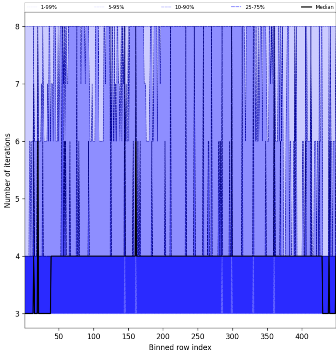
Figure 49: Along track statistics of “Number of iterations” for 2025-02-20 to 2025-02-21
