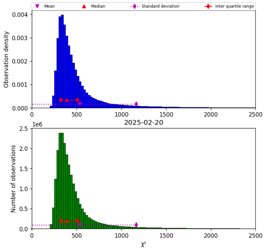
Figure 40: Histogram of “ \chi^2 ” for 2025-02-20 to 2025-02-21
