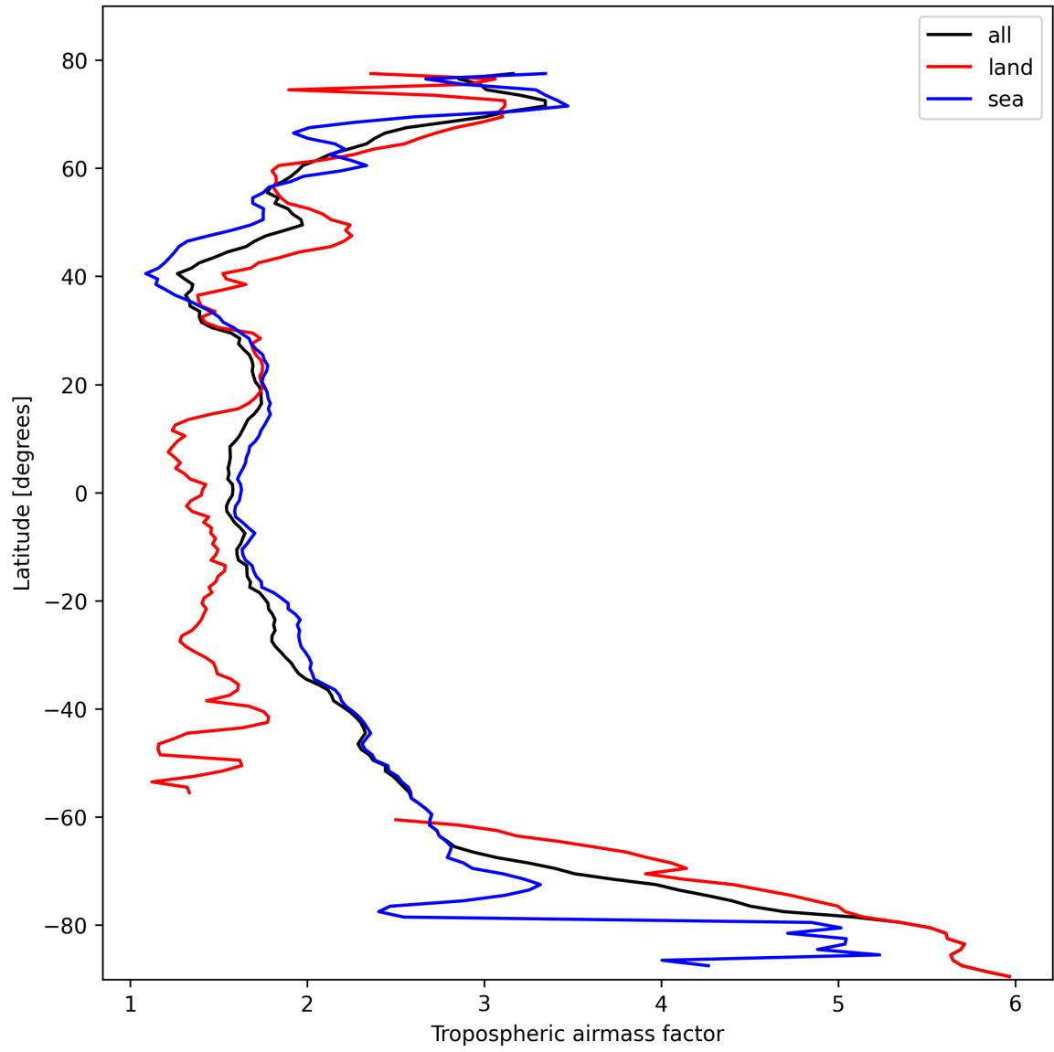
Figure 12: Zonal average of “Tropospheric airmass factor” for 2025-02-20 to 2025-02-21.
