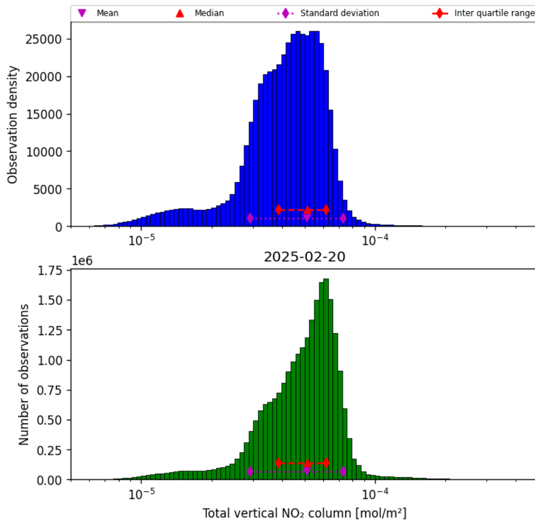
Figure 36: Histogram of "Total vertical NO 2 column" for 2025-02-20 to 2025-02-21
