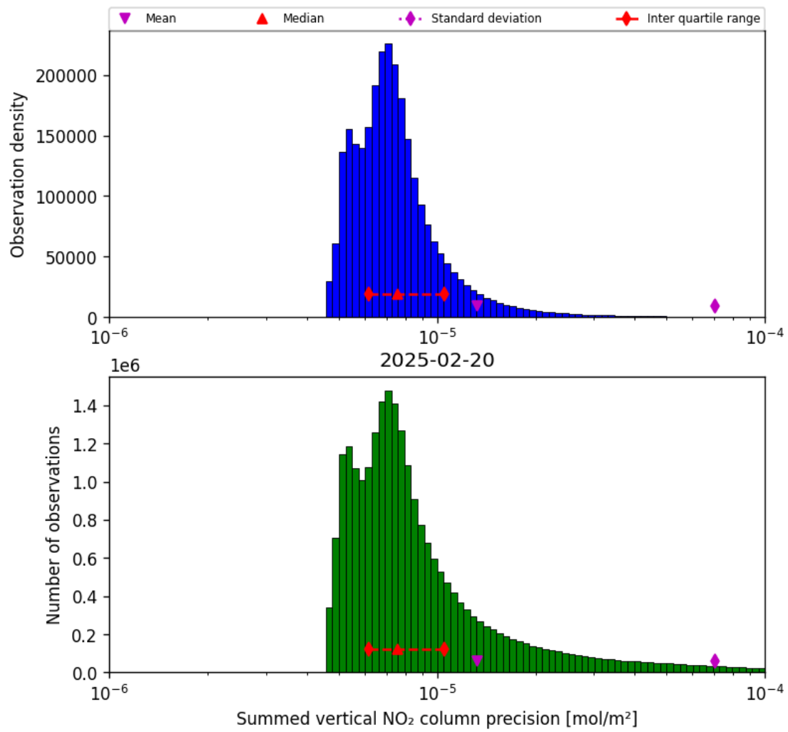
Figure 39: Histogram of “Summed vertical NO 2 column precision” for 2025-02-20 to 2025-02-21
