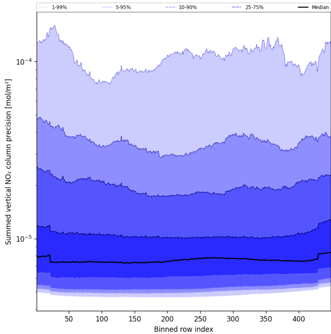
Figure 56: Along track statistics of “Summed vertical NO 2 column precision” for 2025-02-20 to 2025-02-21
