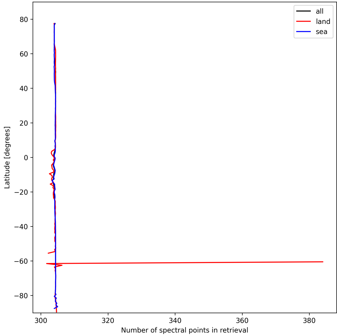
Figure 14: Zonal average of “Number of spectral points in retrieval” for 2025-02-20 to 2025-02-21.
