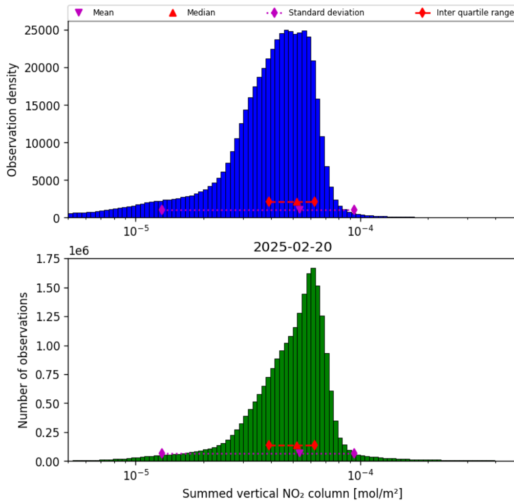
Figure 38: Histogram of “Summed vertical NO 2 column” for 2025-02-20 to 2025-02-21
