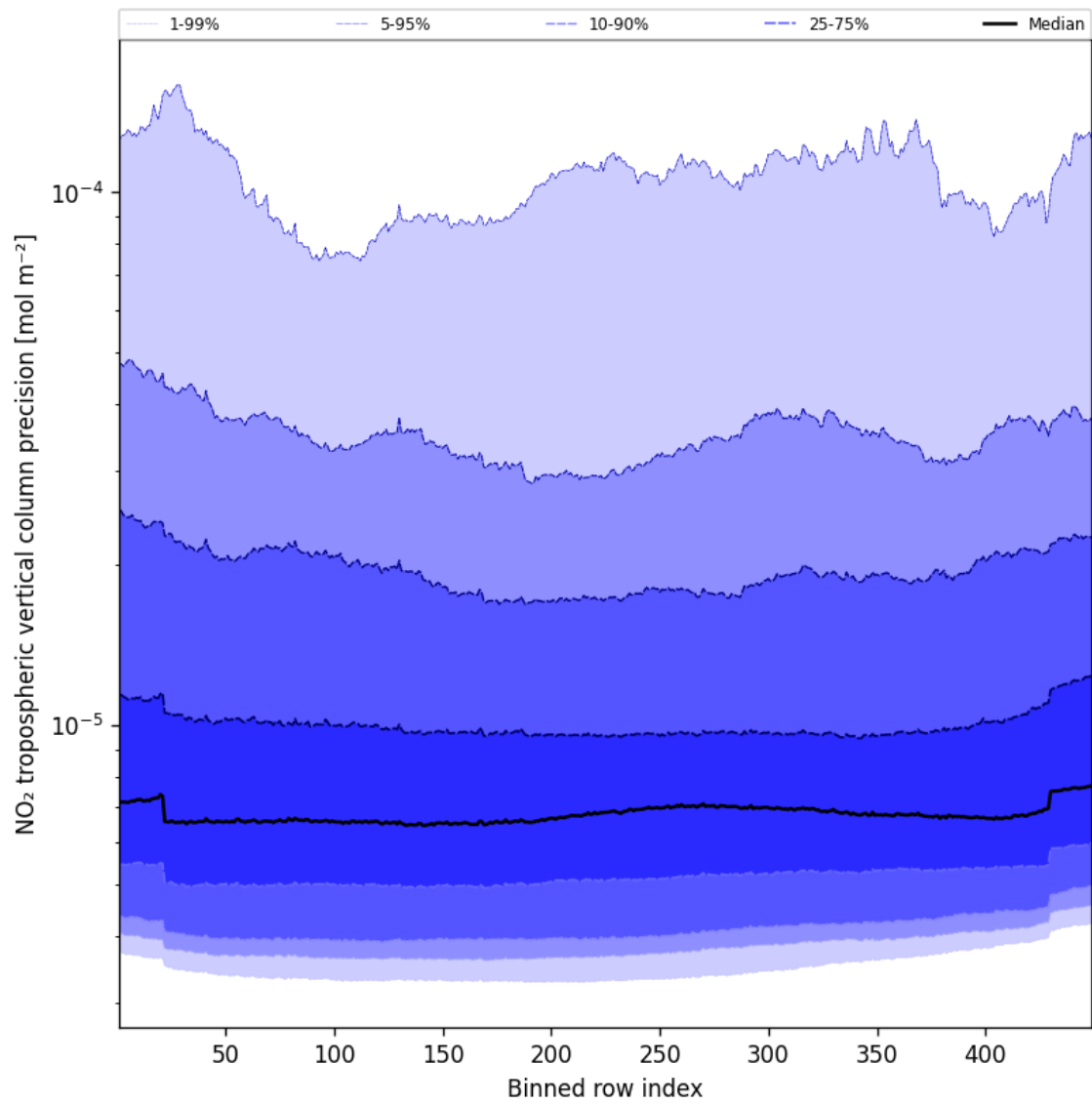
Figure 45: Along track statistics of “NO 2 tropospheric vertical column precision” for 2025-02-20 to 2025-02-21
