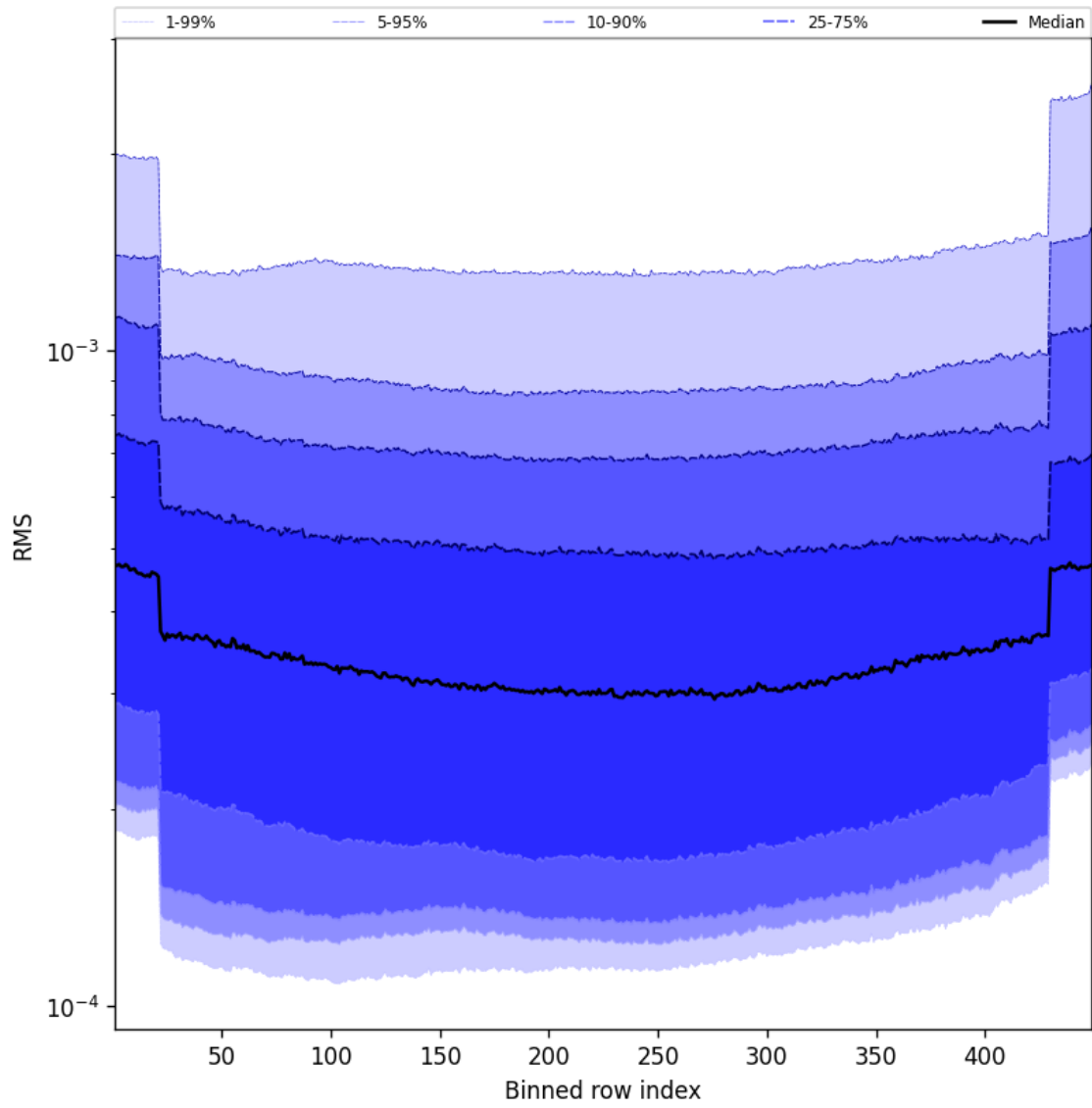
Figure 58: Along track statistics of “RMS” for 2025-02-20 to 2025-02-21
