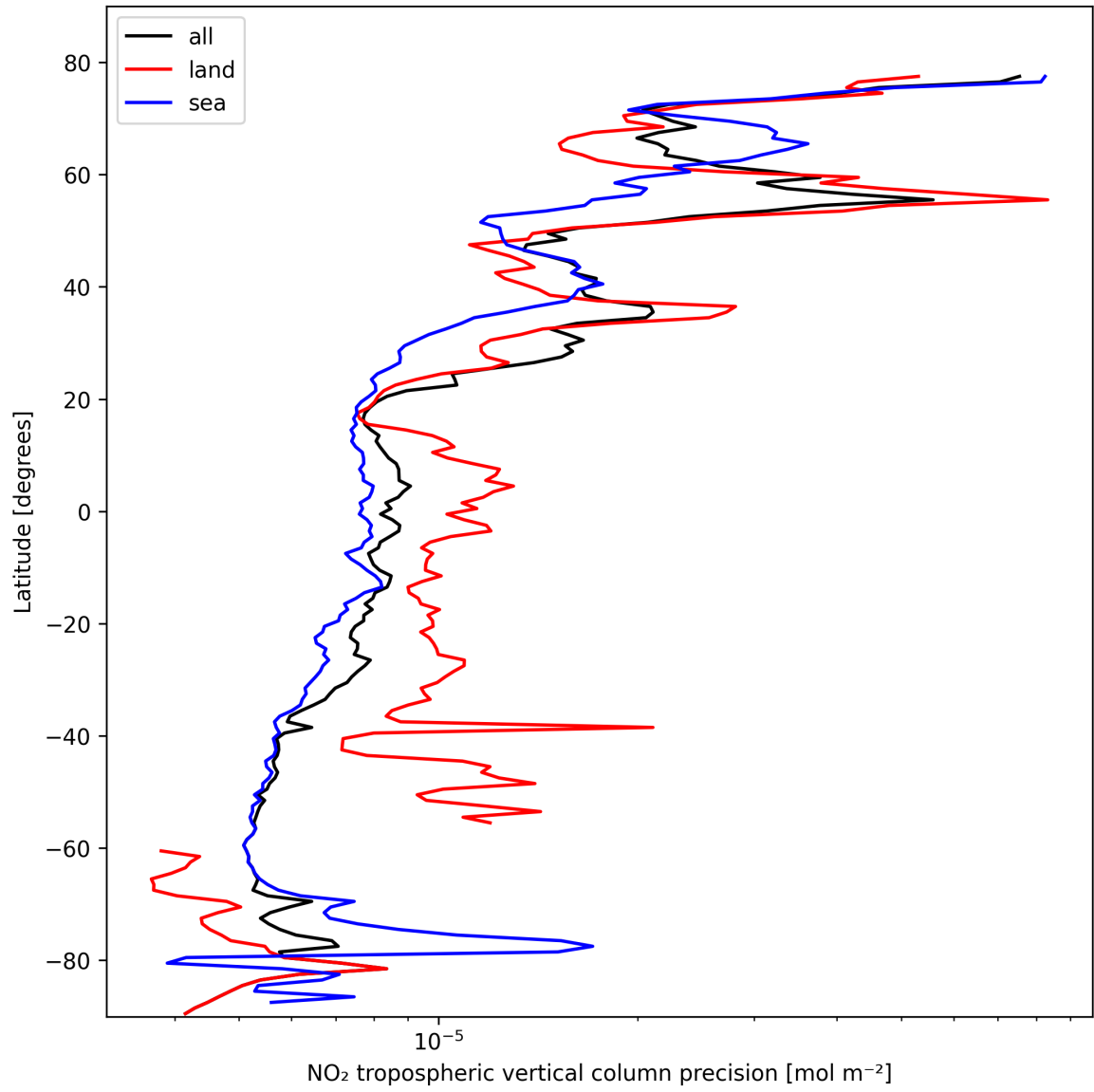
Figure 11: Zonal average of “NO 2 tropospheric vertical column precision” for 2025-02-20 to 2025-02-21.
