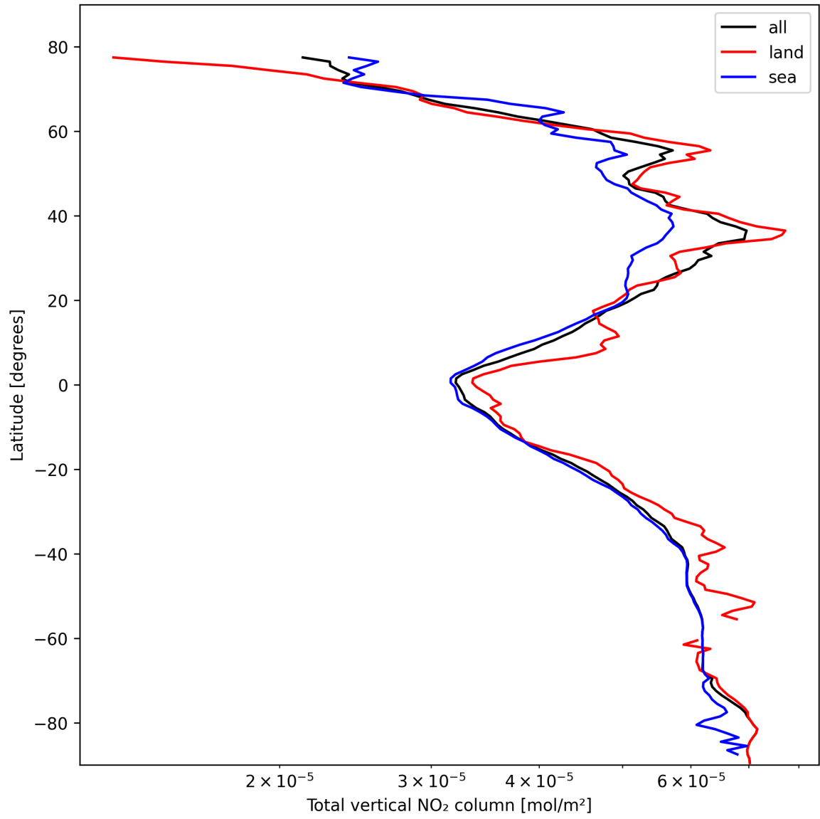
Figure 19: Zonal average of “Total vertical NO 2 column” for 2025-02-20 to 2025-02-21.
