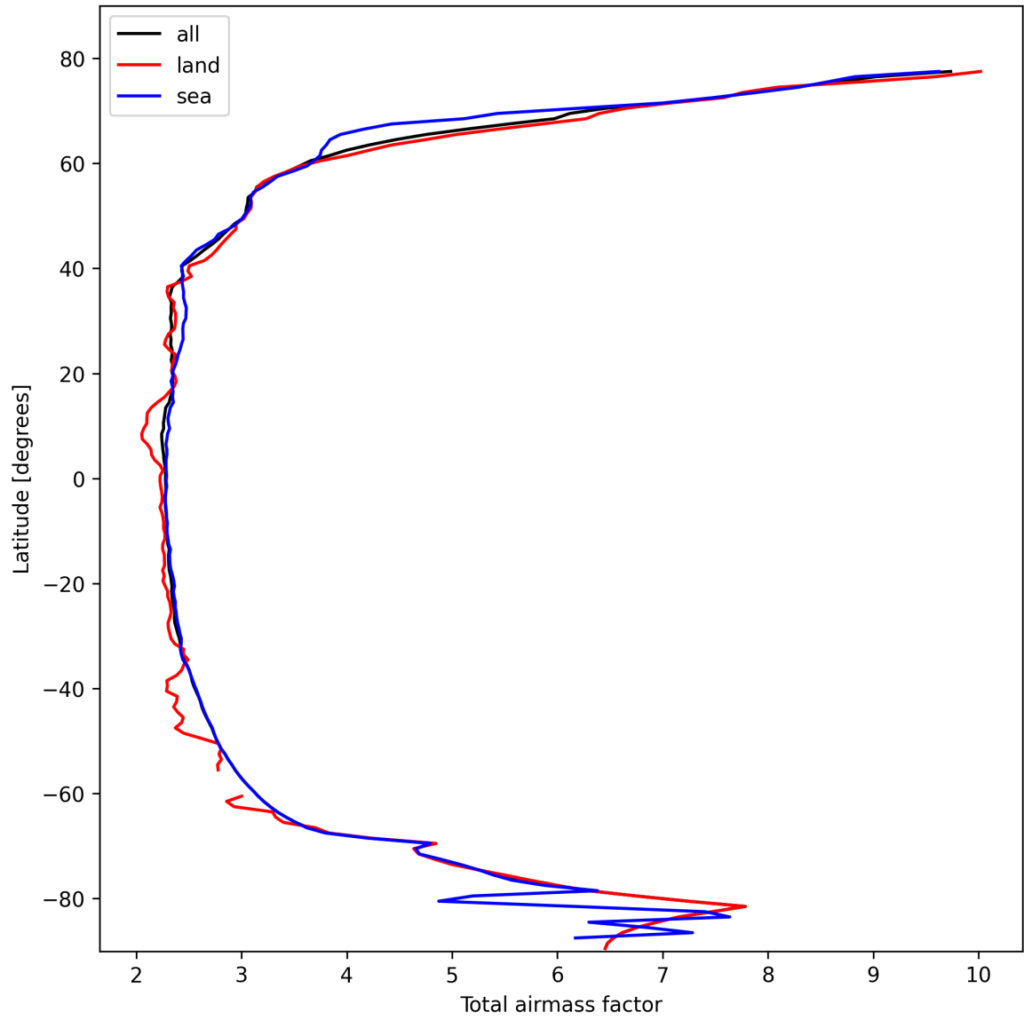
Figure 13: Zonal average of “Total airmass factor” for 2025-02-20 to 2025-02-21.
