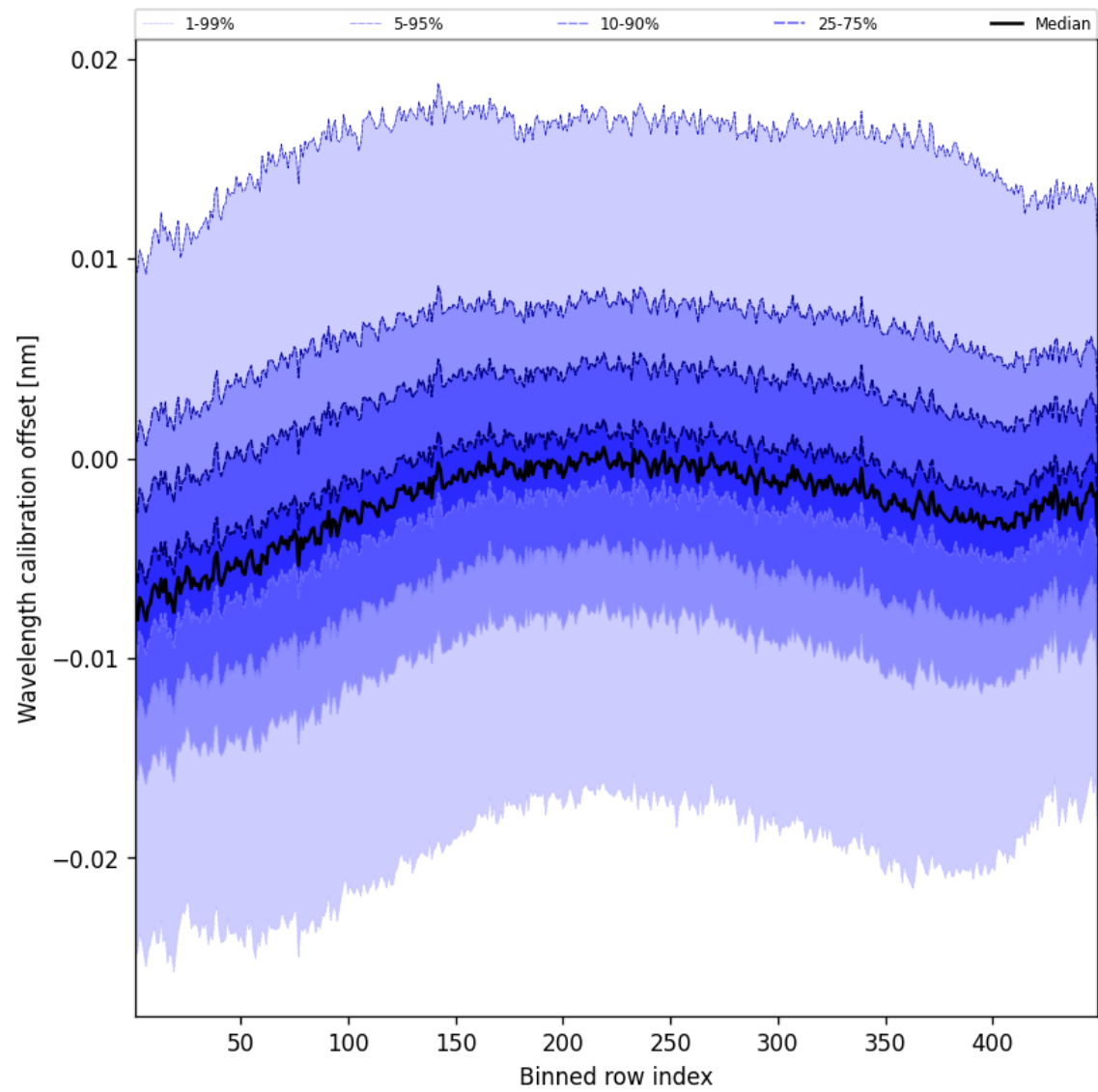
Figure 50: Along track statistics of “Wavelength calibration offset” for 2025-02-20 to 2025-02-21
