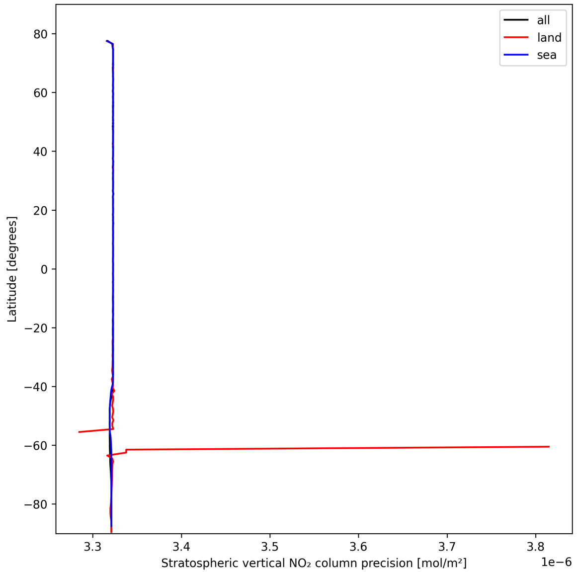
Figure 18: Zonal average of “Stratospheric vertical NO 2 column precision” for 2025-02-20 to 2025-02-21.
