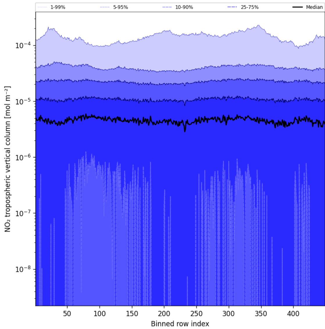
Figure 44: Along track statistics of “NO 2 tropospheric vertical column” for 2025-02-20 to 2025-02-21
