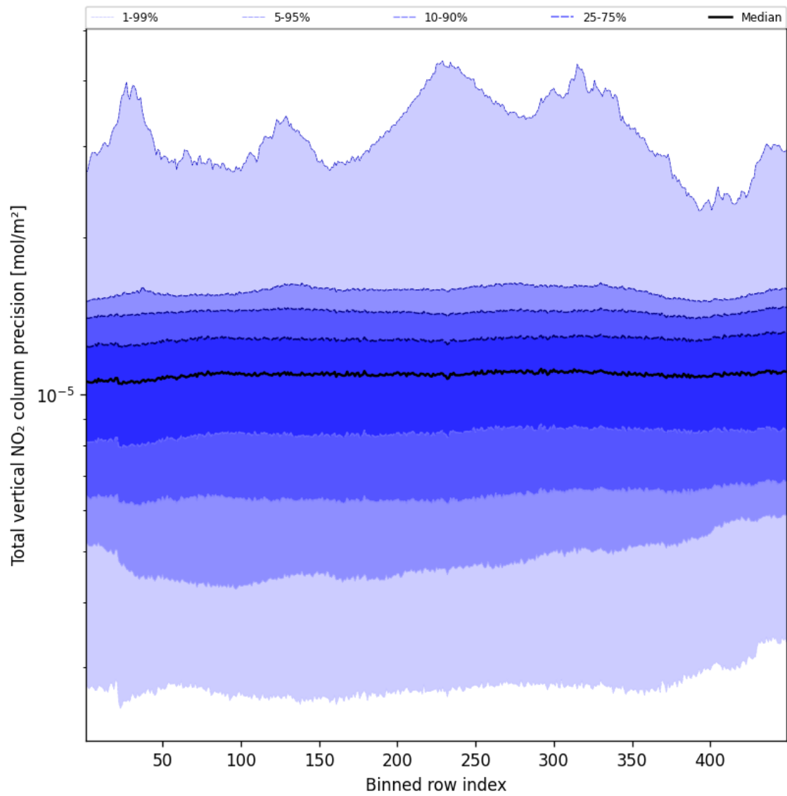
Figure 54: Along track statistics of “Total vertical NO 2 column precision” for 2025-02-20 to 2025-02-21
