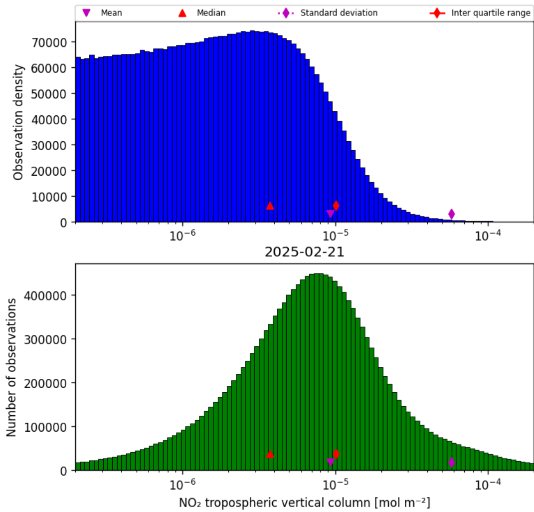
Figure 27: Histogram of “NO 2 tropospheric vertical column” for 2025-02-21 to 2025-02-22
