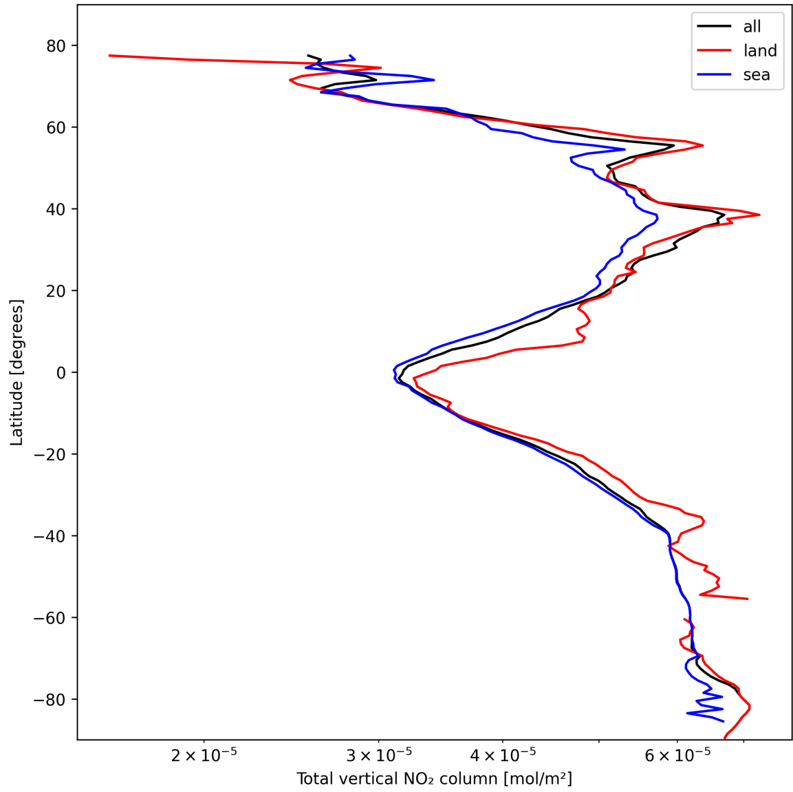
Figure 19: Zonal average of “Total vertical NO 2 column” for 2025-02-21 to 2025-02-22.
