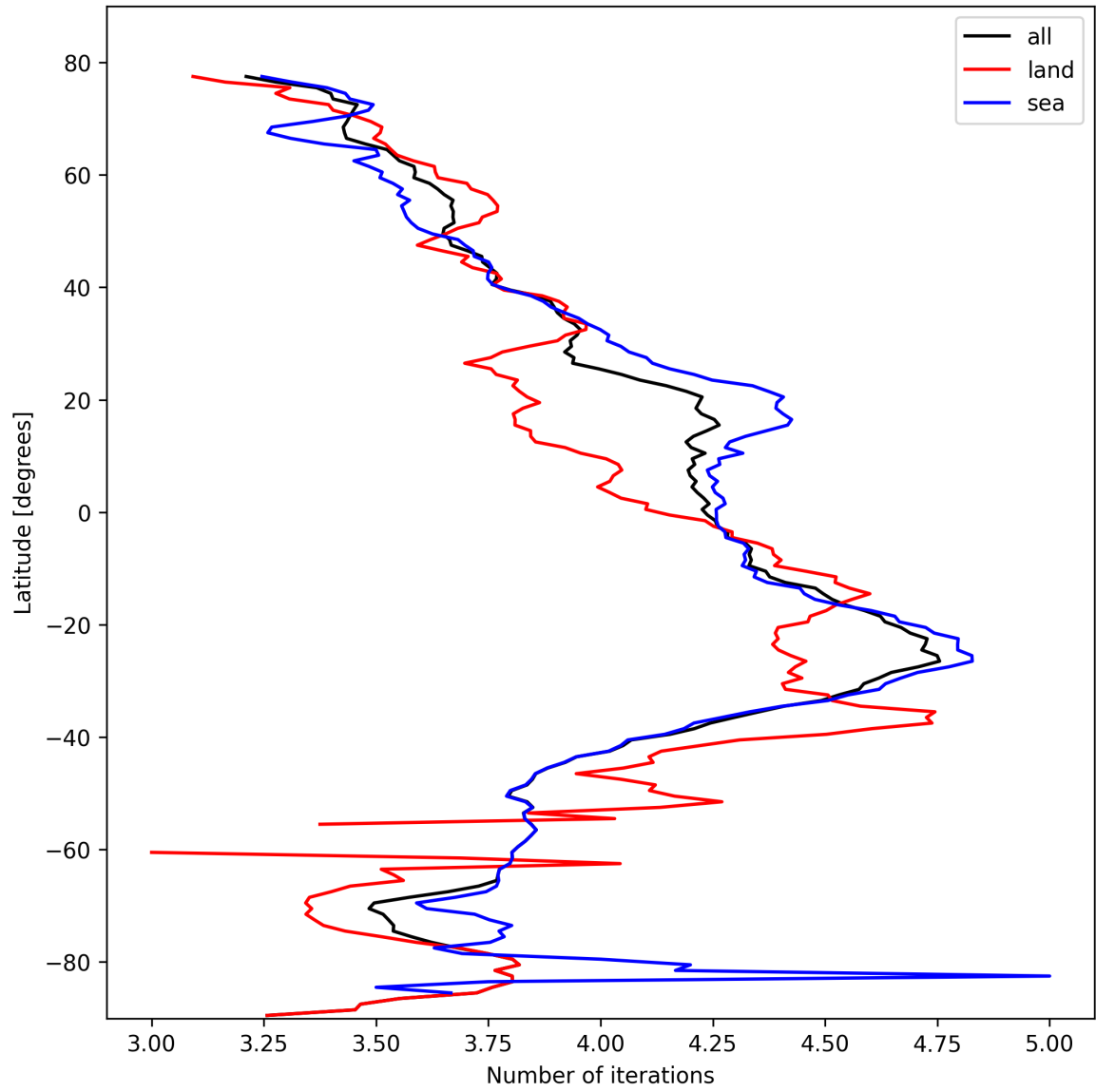
Figure 15: Zonal average of “Number of iterations” for 2025-02-21 to 2025-02-22.
