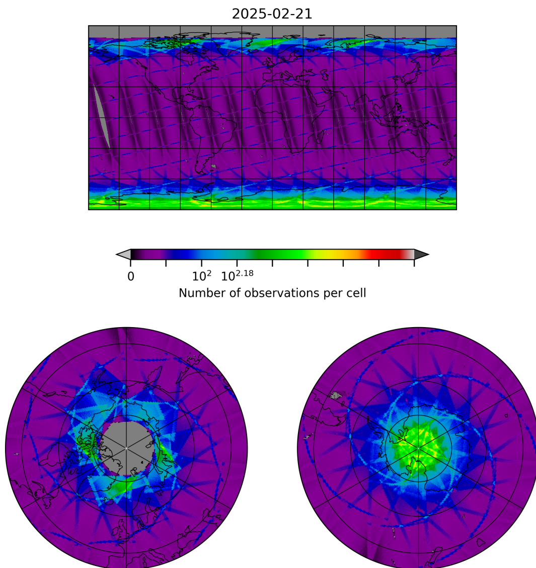
Figure 8: Map of the number of observations for 2025-02-21 to 2025-02-22
