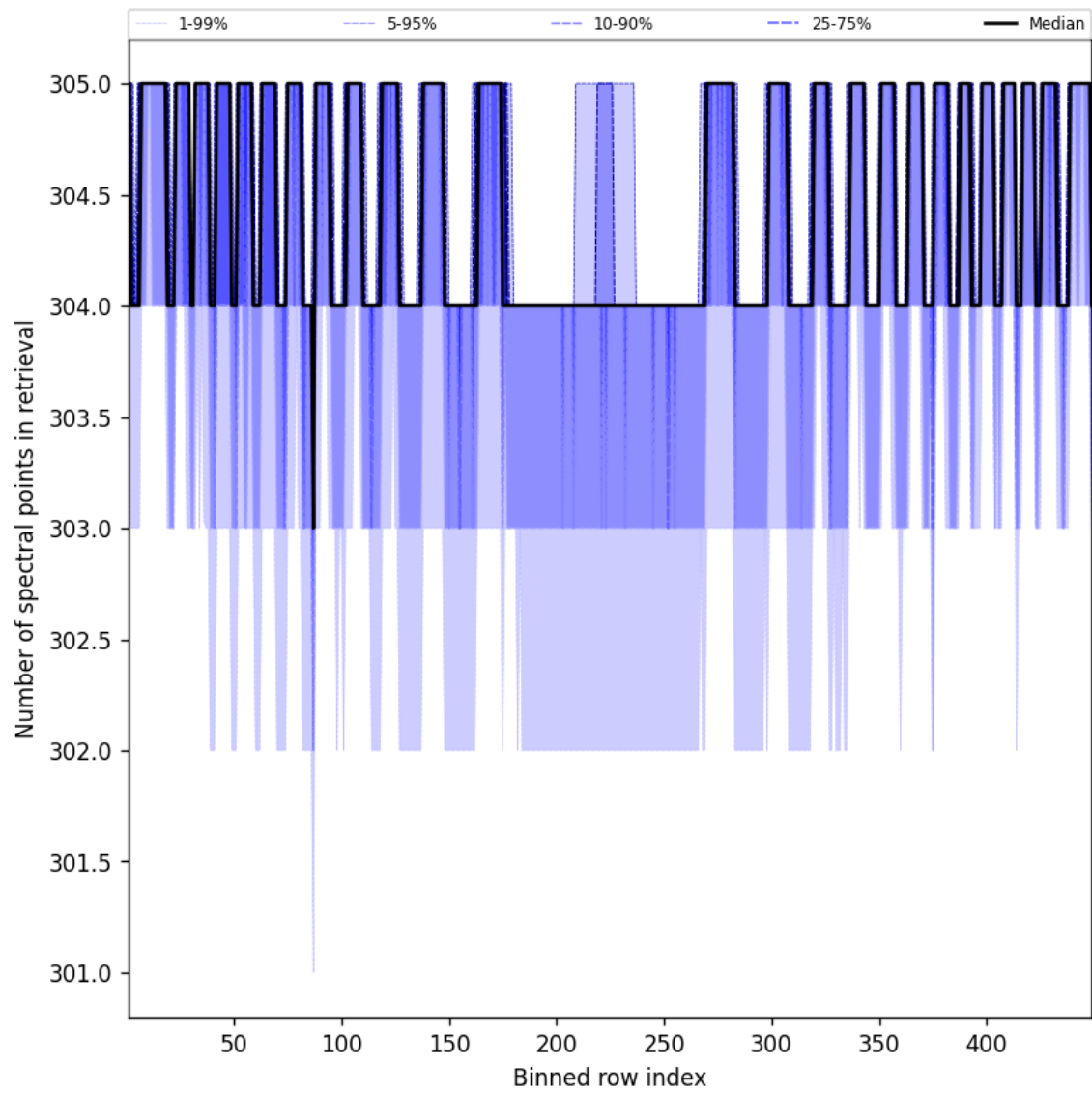
Figure 48: Along track statistics of “Number of spectral points in retrieval” for 2025-02-21 to 2025-02-22
