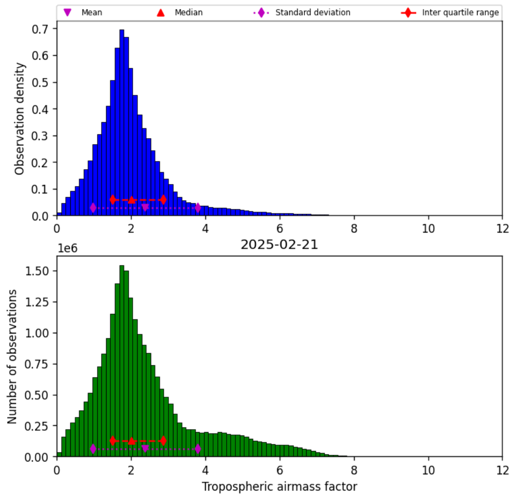
Figure 29: Histogram of “Tropospheric airmass factor” for 2025-02-21 to 2025-02-22
