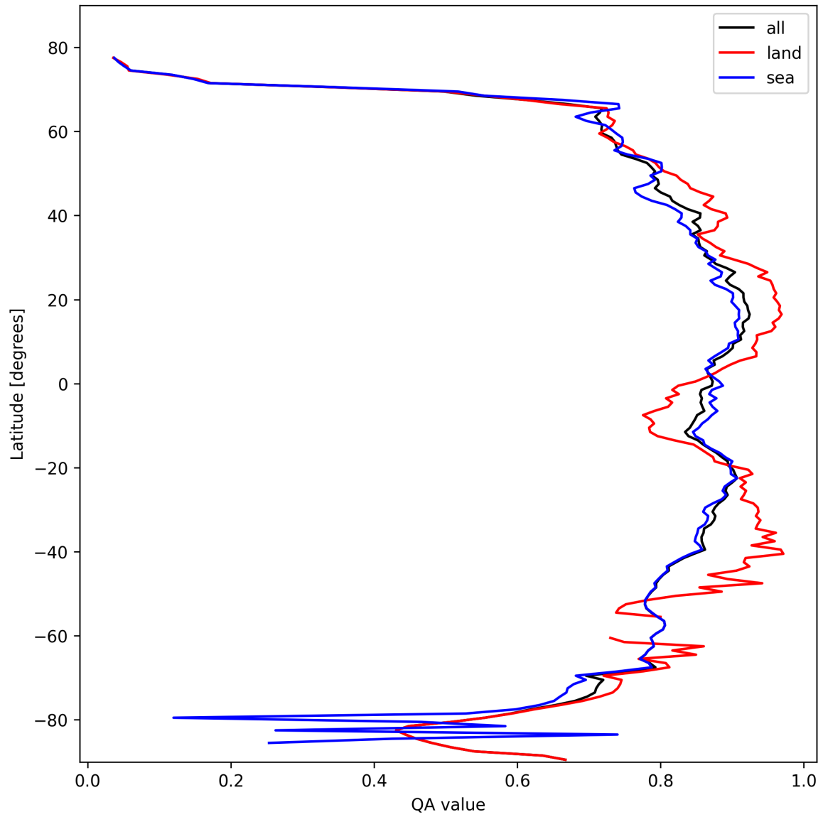
Figure 9: Zonal average of “QA value” for 2025-02-21 to 2025-02-22.
