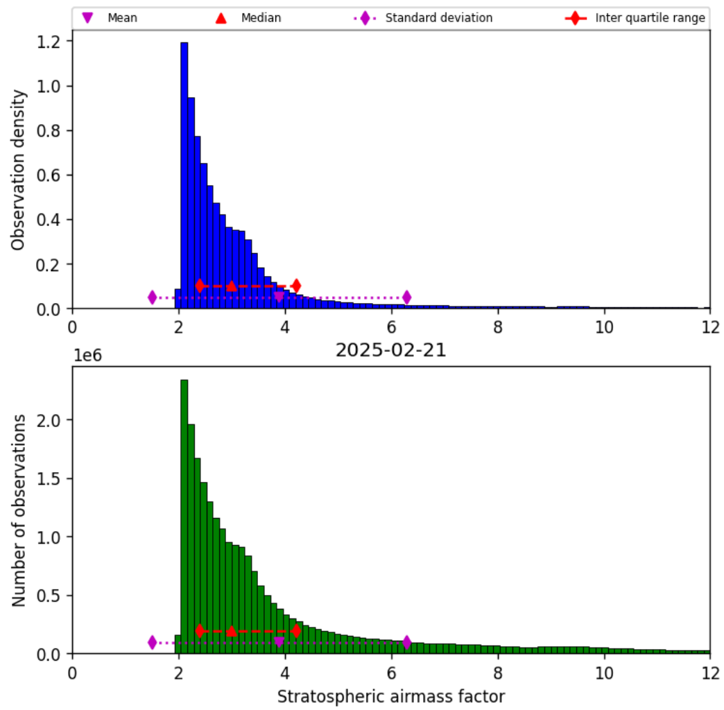
Figure 42: Histogram of “Stratospheric airmass factor” for 2025-02-21 to 2025-02-22
