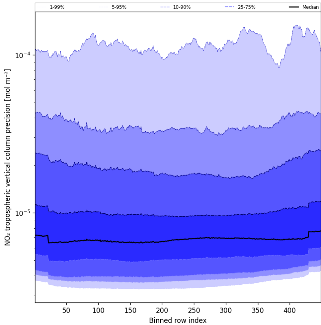
Figure 45: Along track statistics of “NO 2 tropospheric vertical column precision” for 2025-02-21 to 2025-02-22
