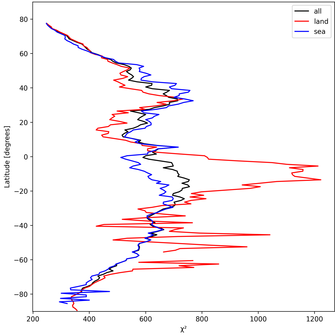
Figure 23: Zonal average of “ \chi^2 ” for 2025-02-21 to 2025-02-22.
