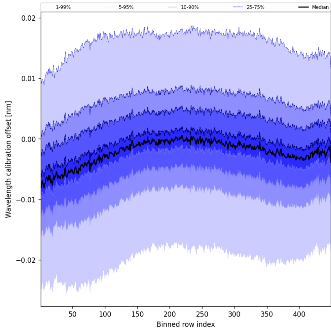
Figure 50: Along track statistics of “Wavelength calibration offset” for 2025-02-21 to 2025-02-22
