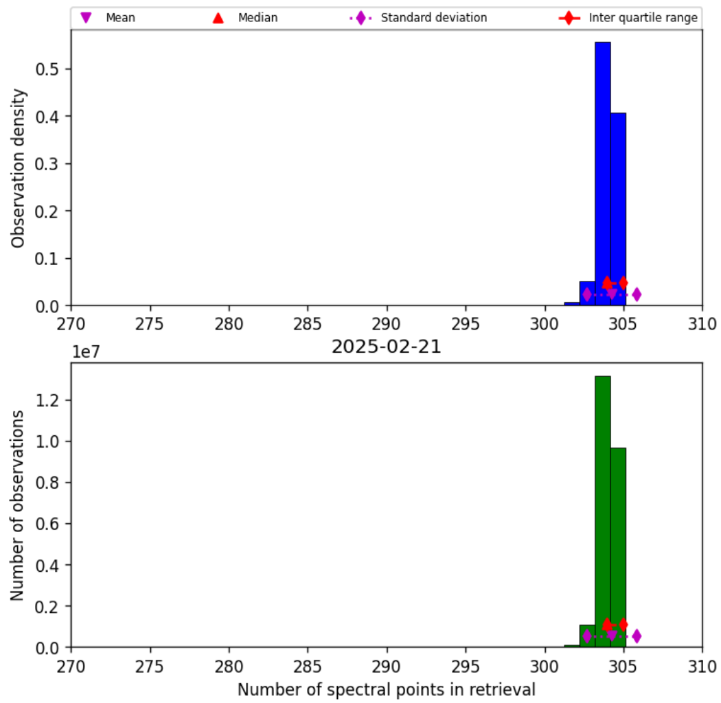
Figure 31: Histogram of “Number of spectral points in retrieval” for 2025-02-21 to 2025-02-22
