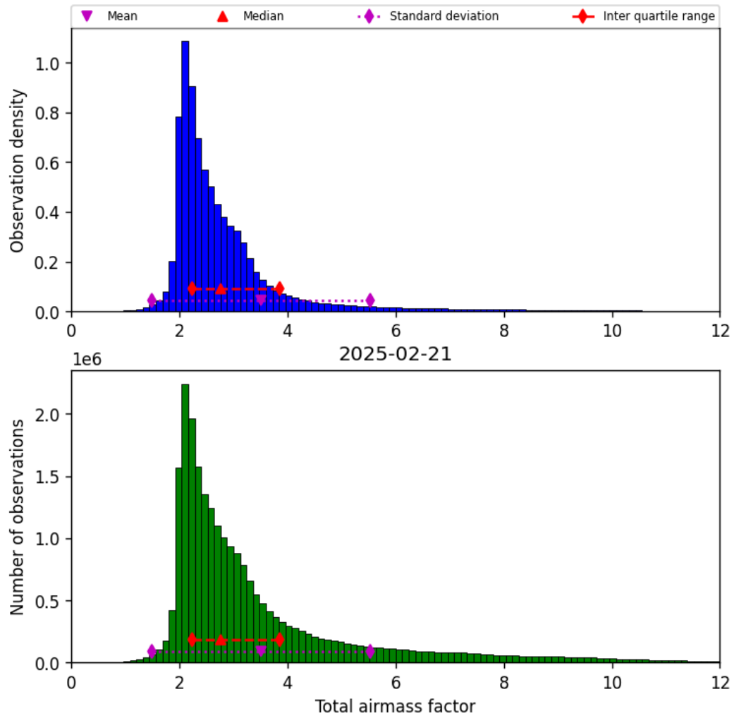
Figure 30: Histogram of “Total airmass factor” for 2025-02-21 to 2025-02-22
