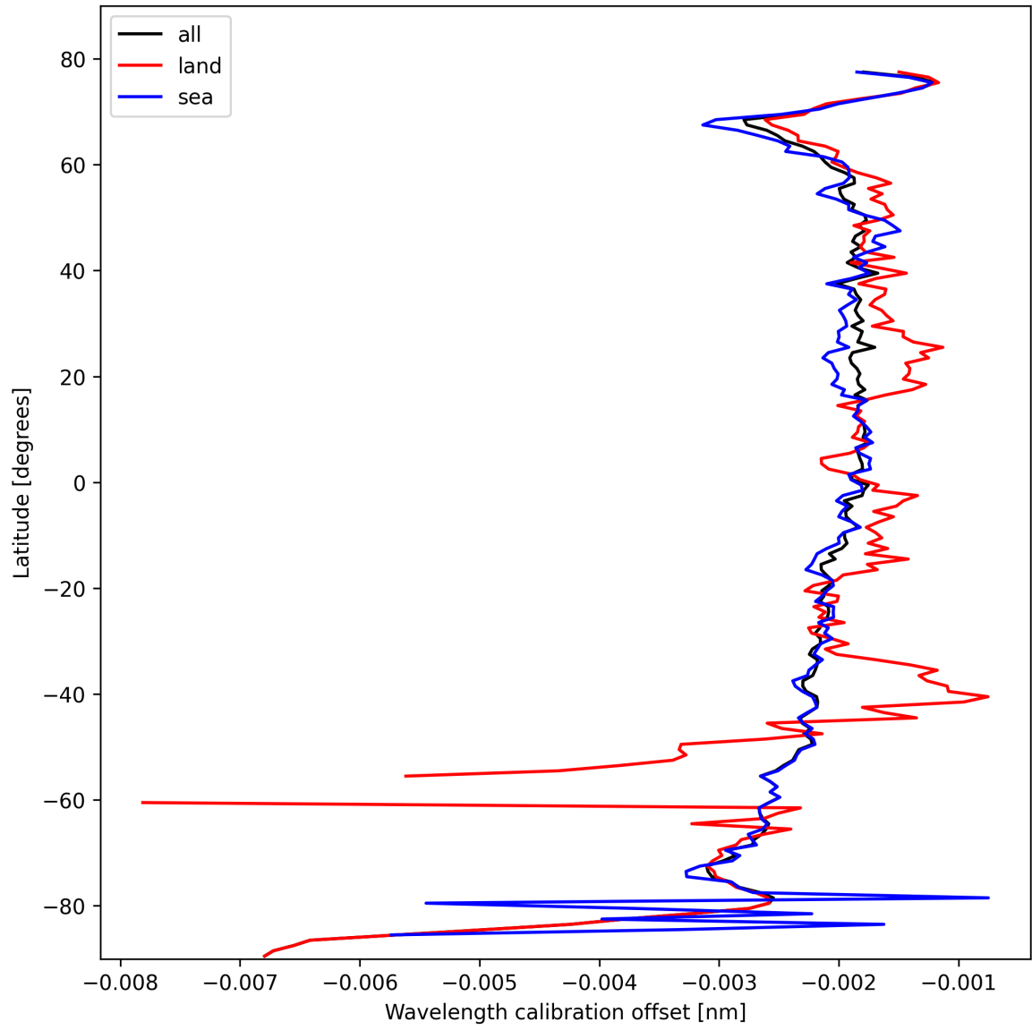
Figure 16: Zonal average of “Wavelength calibration offset” for 2025-02-21 to 2025-02-22.
