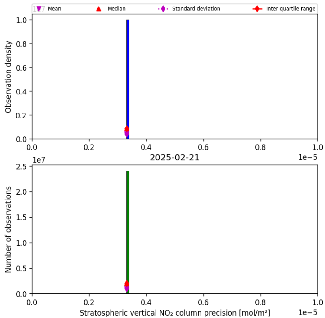
Figure 35: Histogram of “Stratospheric vertical NO 2 column precision” for 2025-02-21 to 2025-02-22
