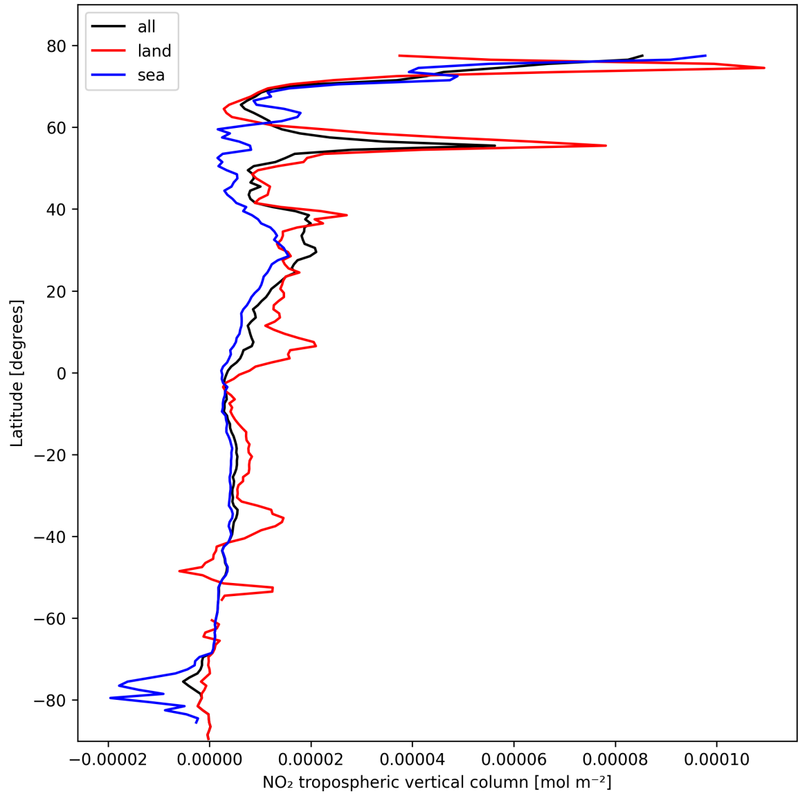
Figure 10: Zonal average of “NO 2 tropospheric vertical column” for 2025-02-21 to 2025-02-22.
