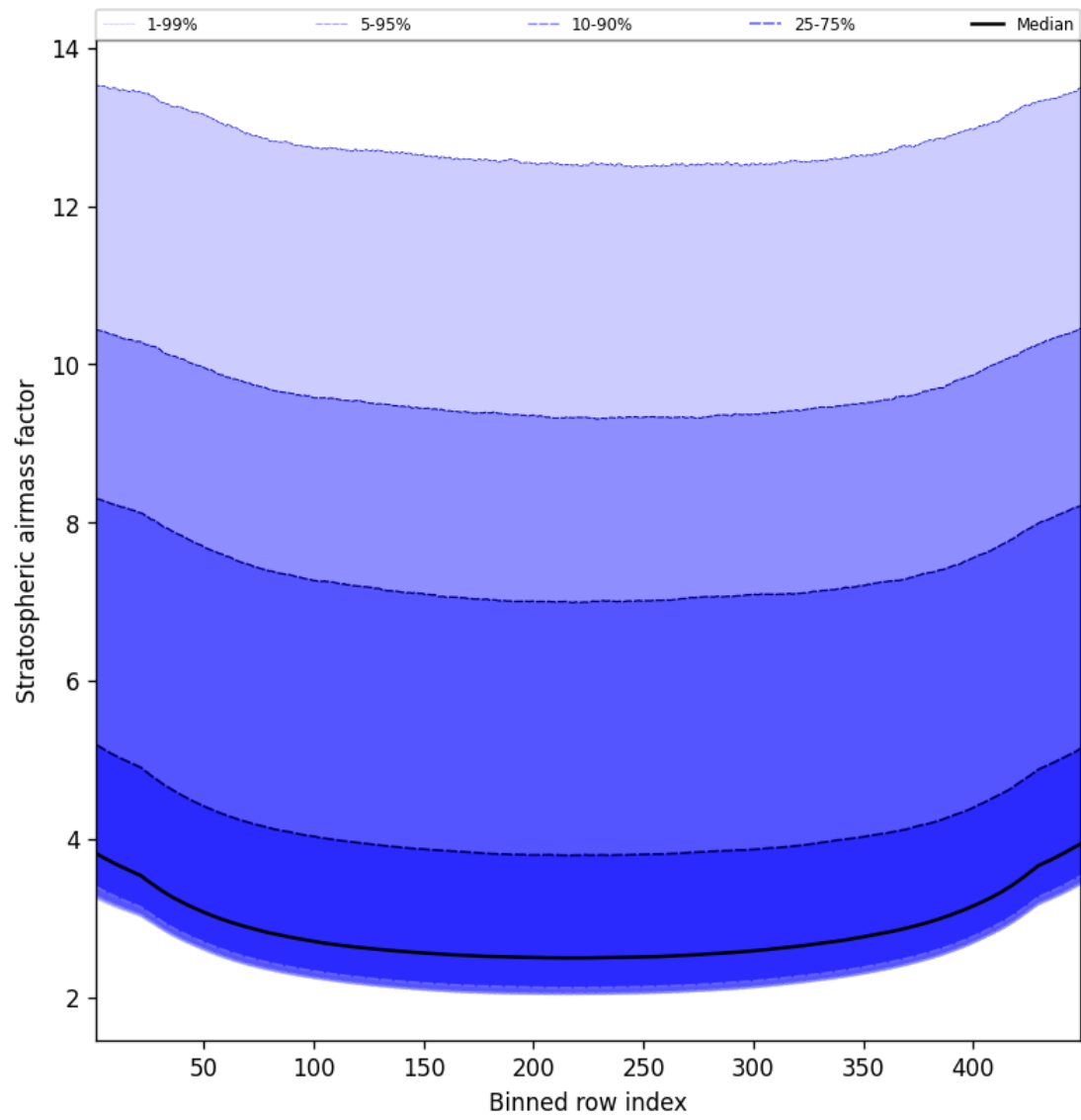
Figure 59: Along track statistics of “Stratospheric airmass factor” for 2025-02-21 to 2025-02-22
