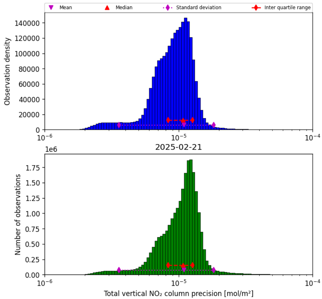
Figure 37: Histogram of “Total vertical NO 2 column precision” for 2025-02-21 to 2025-02-22
