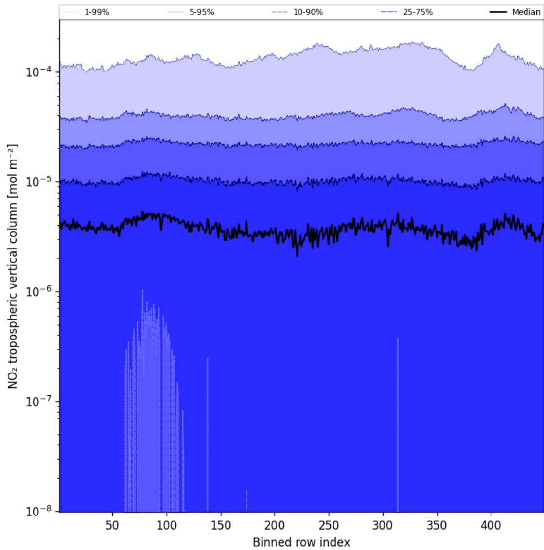
Figure 44: Along track statistics of “NO 2 tropospheric vertical column” for 2025-02-21 to 2025-02-22
