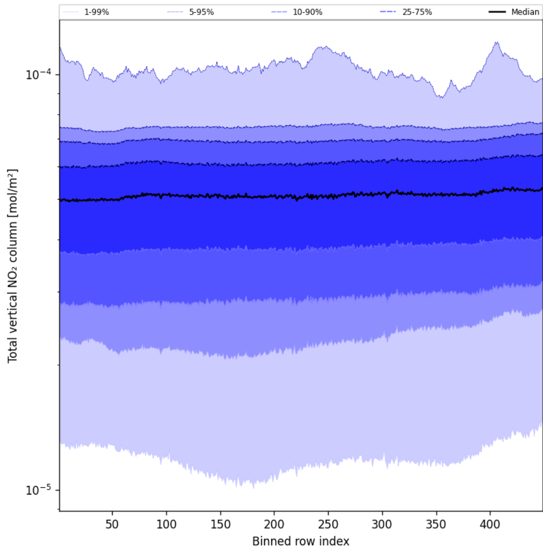
Figure 53: Along track statistics of “Total vertical NO 2 column” for 2025-02-21 to 2025-02-22
