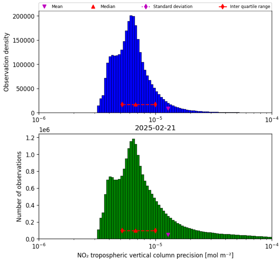
Figure 28: Histogram of “NO 2 tropospheric vertical column precision” for 2025-02-21 to 2025-02-22
