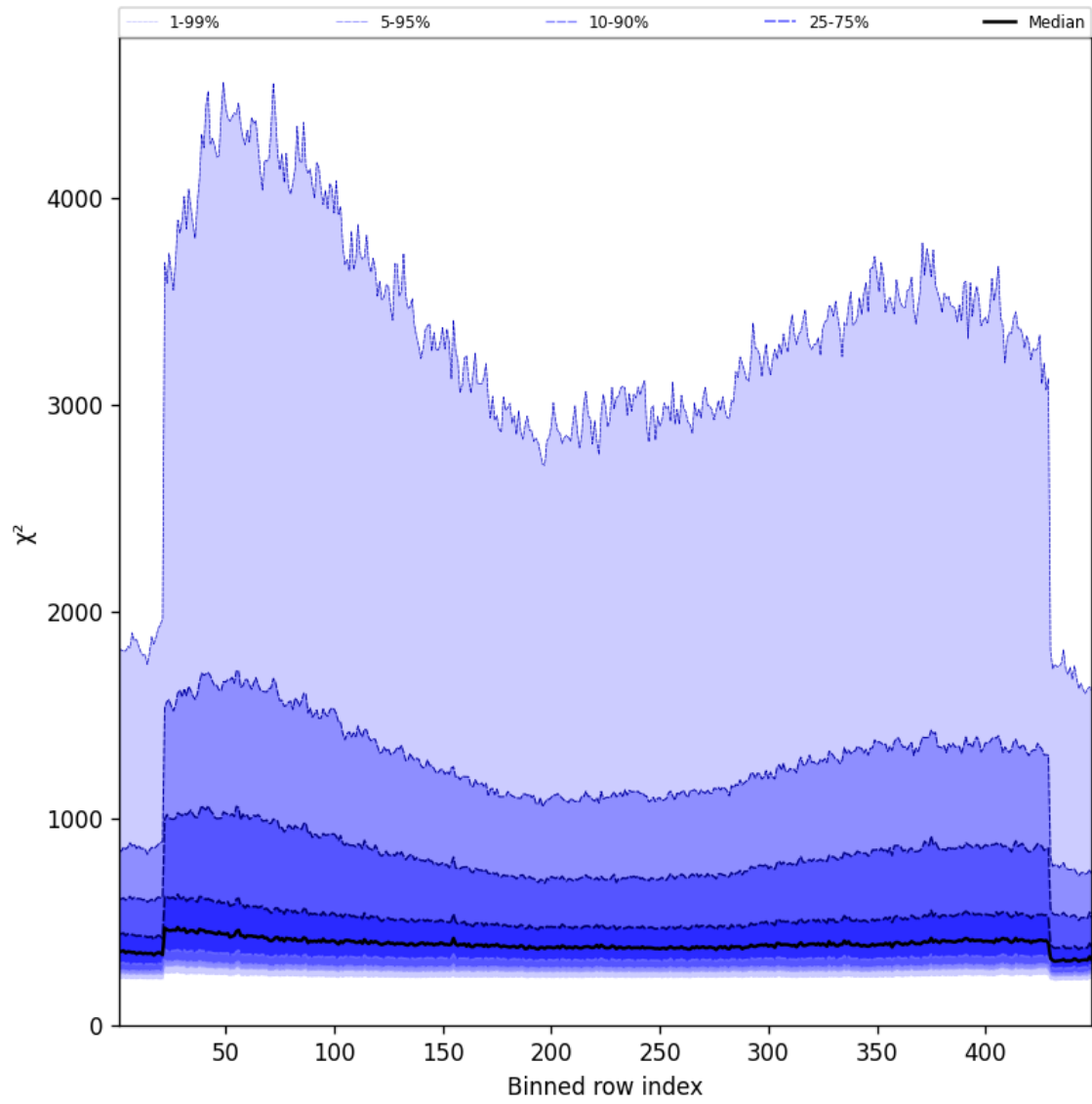
Figure 57: Along track statistics of “ \chi^2 ” for 2025-02-21 to 2025-02-22
