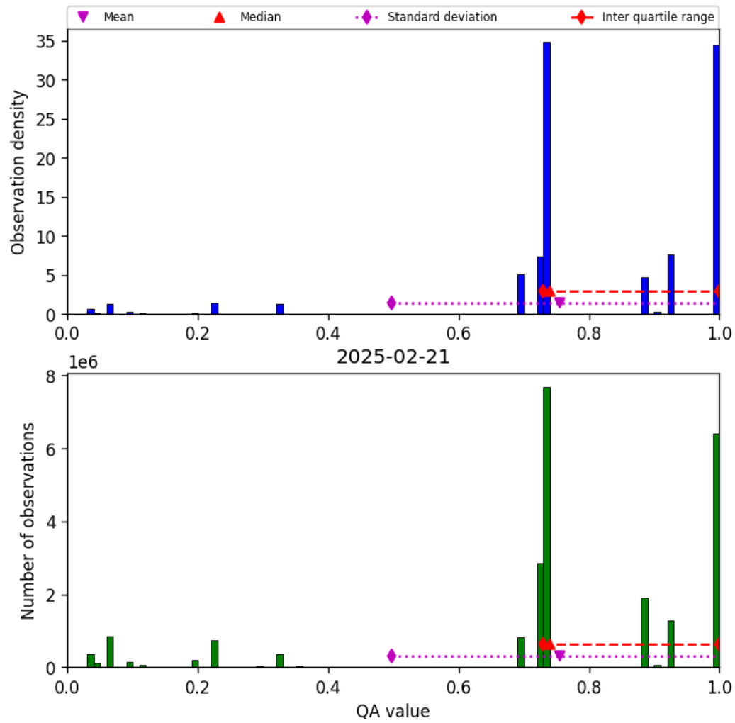
Figure 26: Histogram of “QA value” for 2025-02-21 to 2025-02-22
