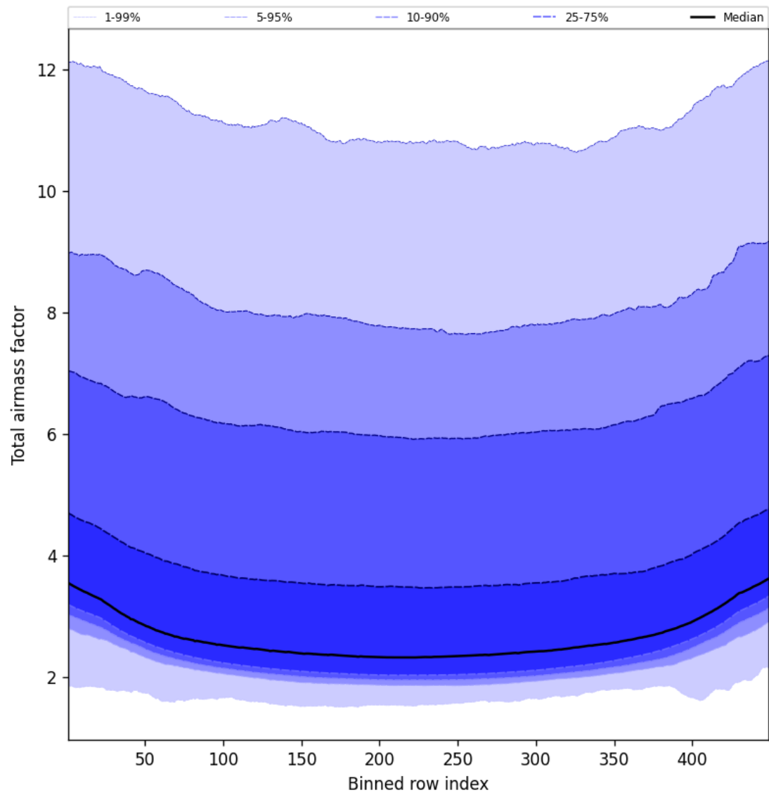
Figure 47: Along track statistics of “Total airmass factor” for 2025-02-21 to 2025-02-22
