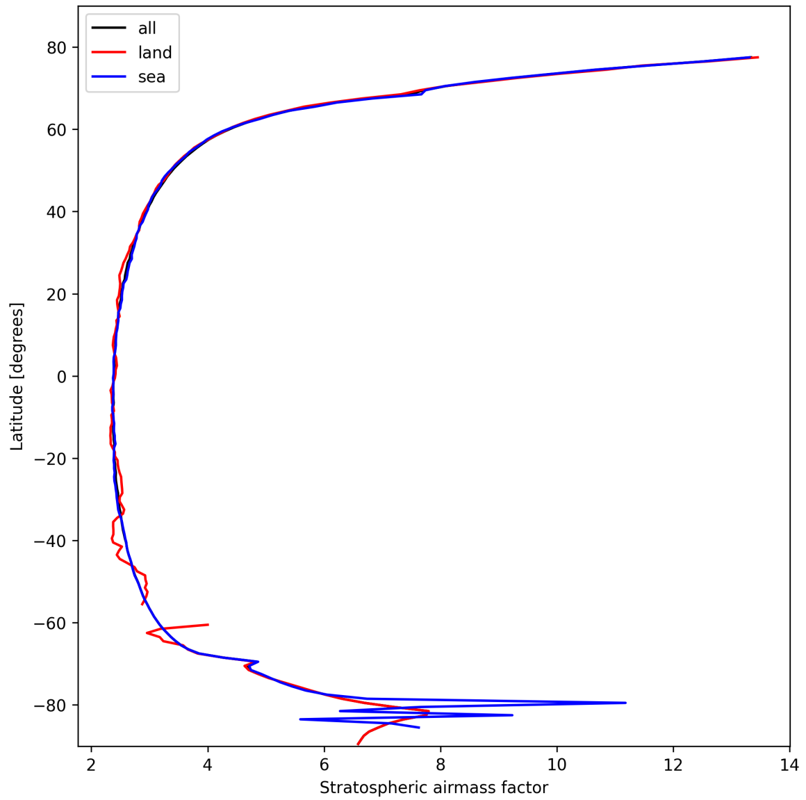
Figure 25: Zonal average of “Stratospheric airmass factor” for 2025-02-21 to 2025-02-22.
