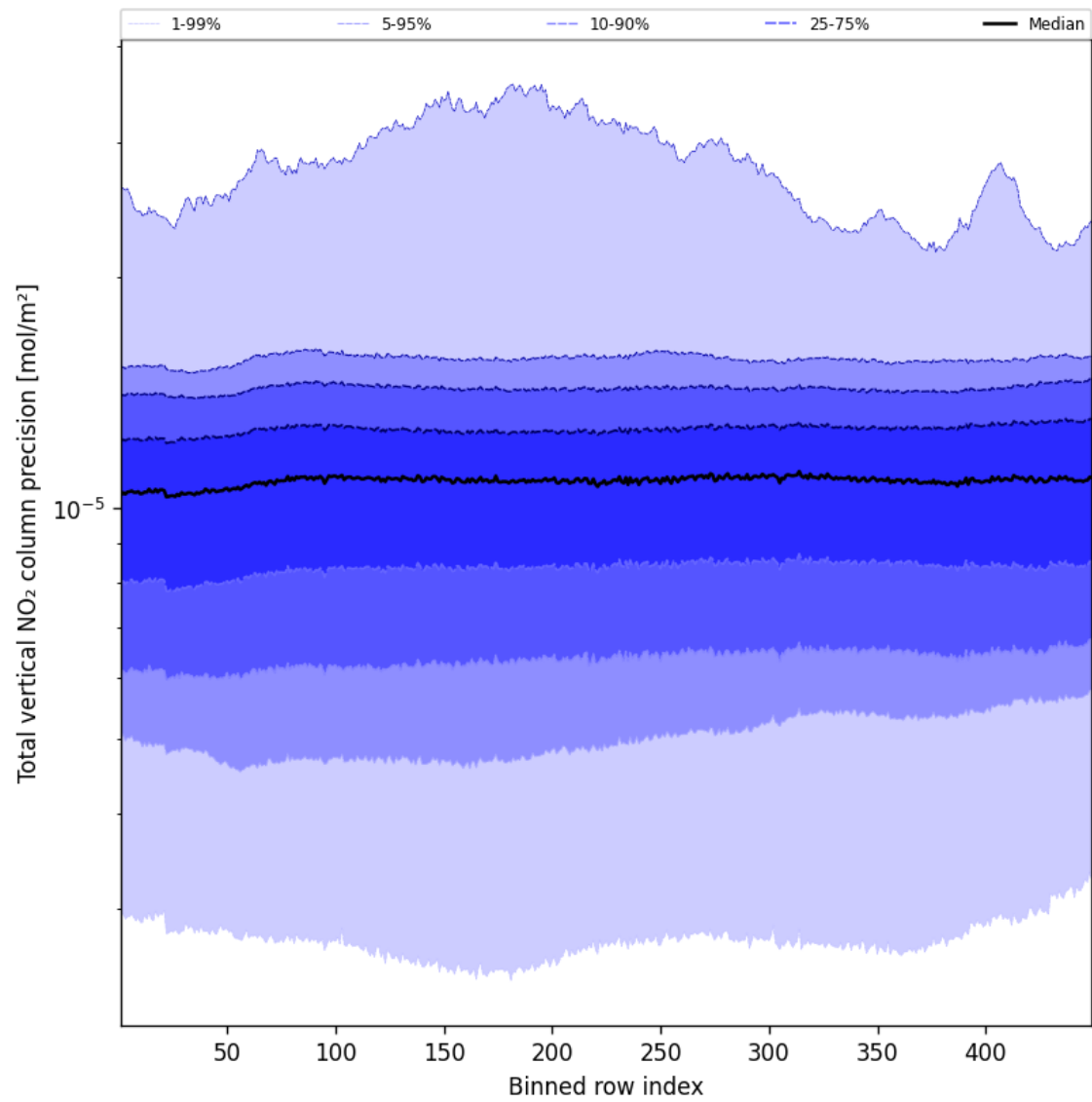
Figure 54: Along track statistics of “Total vertical NO 2 column precision” for 2025-02-21 to 2025-02-22
