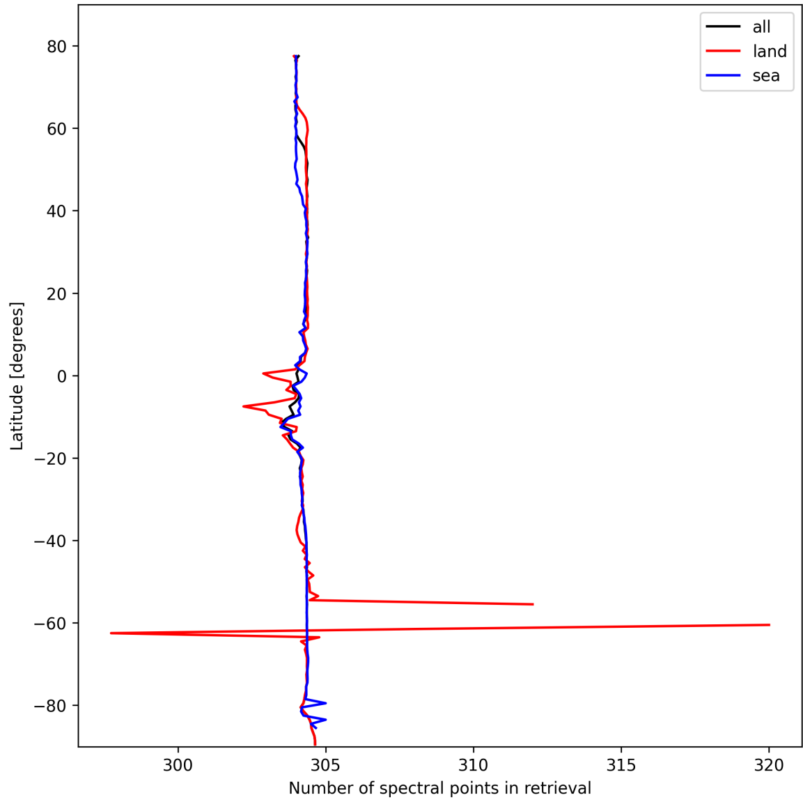
Figure 14: Zonal average of “Number of spectral points in retrieval” for 2025-02-21 to 2025-02-22.
