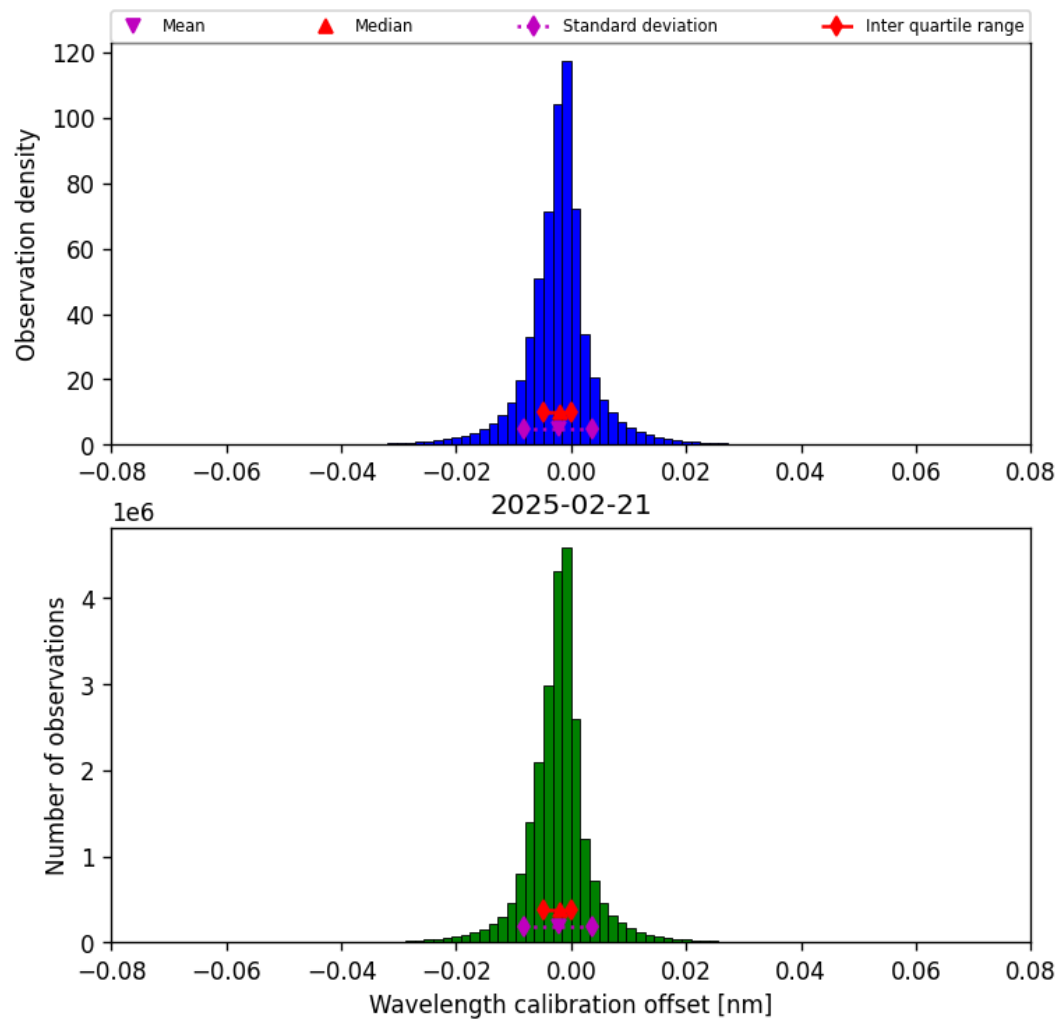
Figure 33: Histogram of “Wavelength calibration offset” for 2025-02-21 to 2025-02-22
