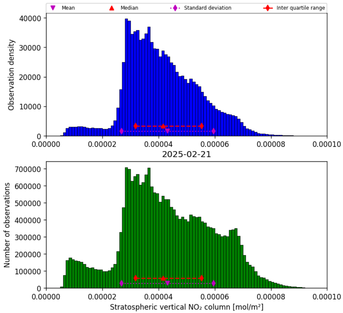
Figure 34: Histogram of “Stratospheric vertical NO 2 column” for 2025-02-21 to 2025-02-22
