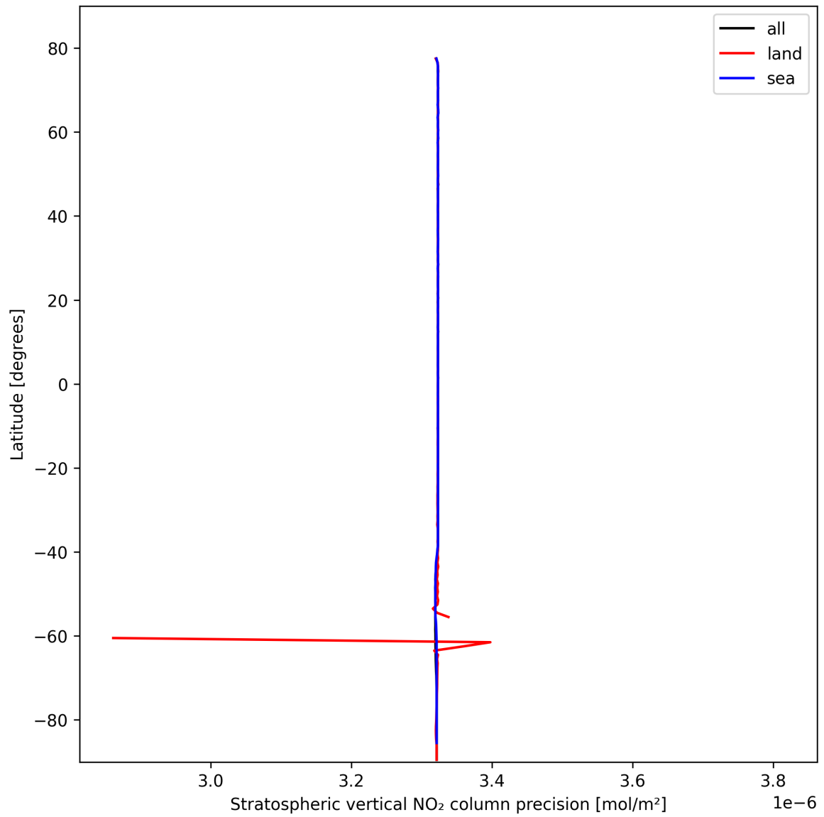
Figure 18: Zonal average of “Stratospheric vertical NO 2 column precision” for 2025-02-21 to 2025-02-22.
