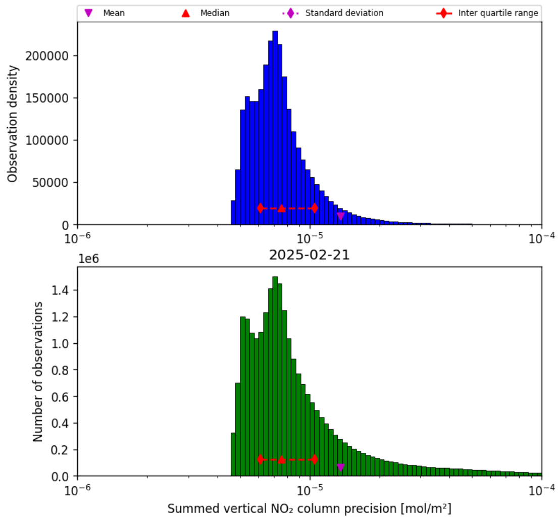
Figure 39: Histogram of "Summed vertical NO 2 column precision" for 2025-02-21 to 2025-02-22
