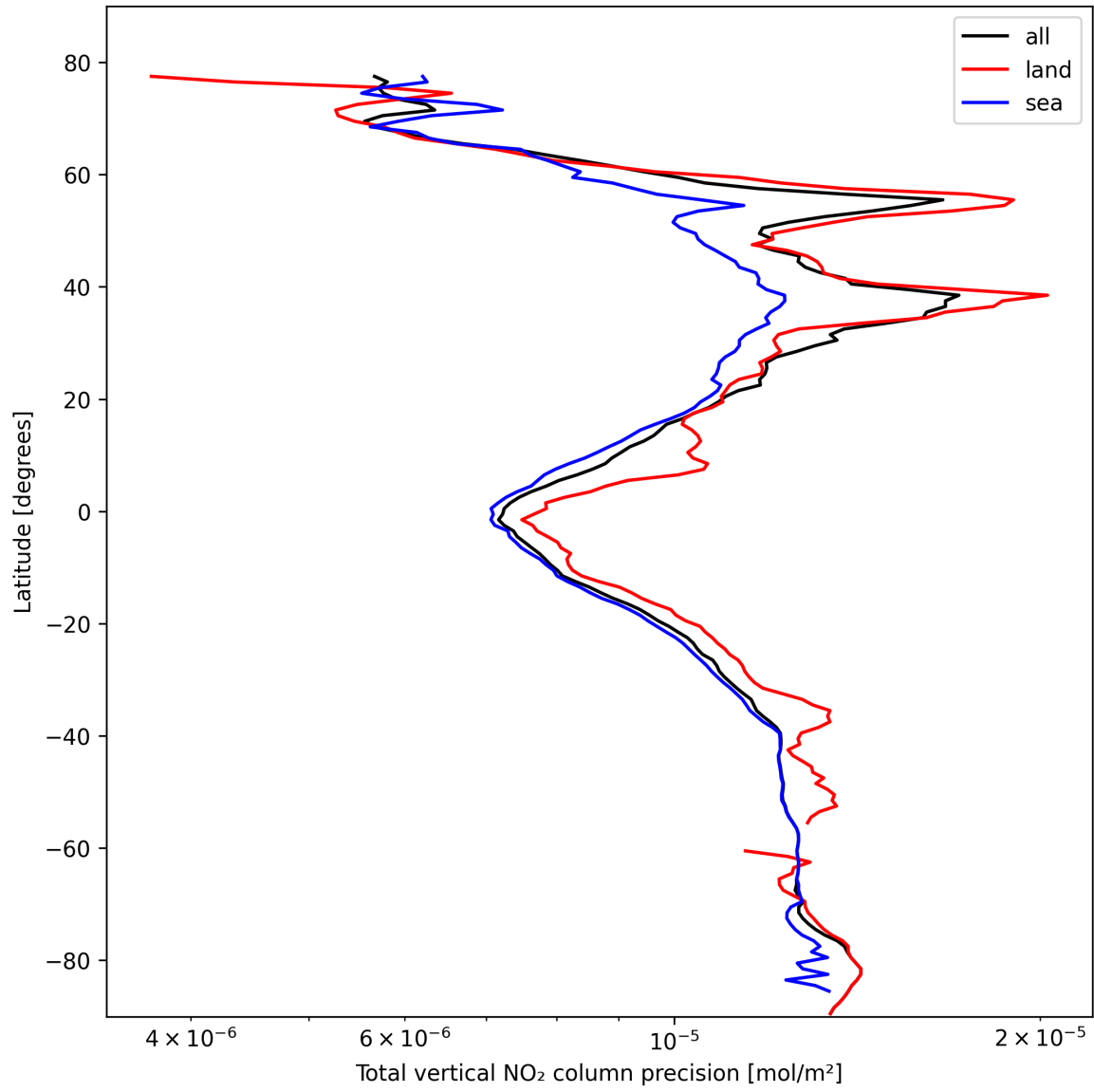
Figure 20: Zonal average of “Total vertical NO 2 column precision” for 2025-02-21 to 2025-02-22.
