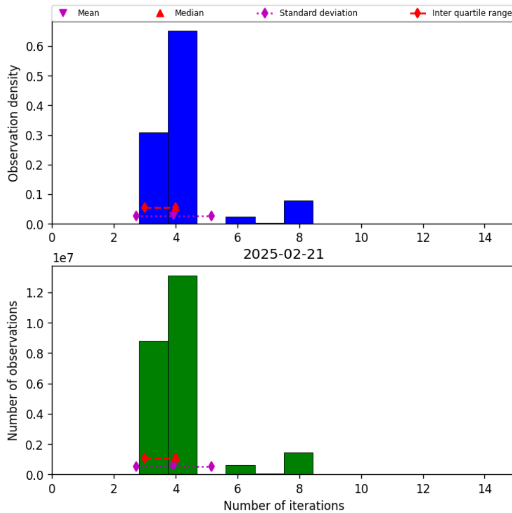
Figure 32: Histogram of “Number of iterations” for 2025-02-21 to 2025-02-22
