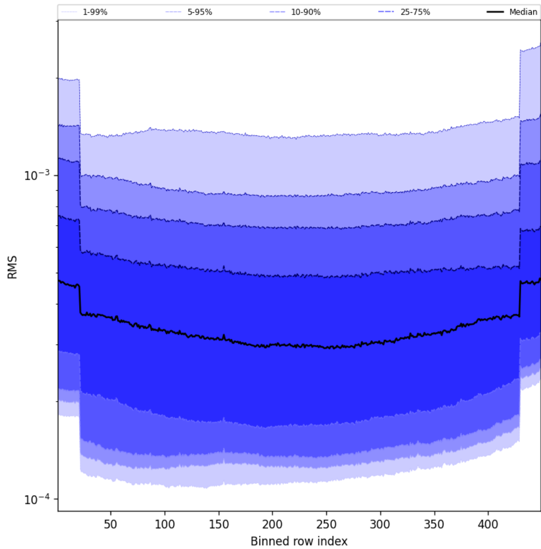
Figure 58: Along track statistics of “RMS” for 2025-02-21 to 2025-02-22
