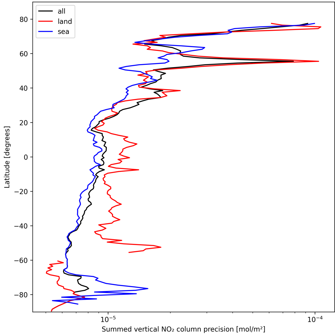
Figure 22: Zonal average of "Summed vertical NO 2 column precision" for 2025-02-21 to 2025-02-22.
