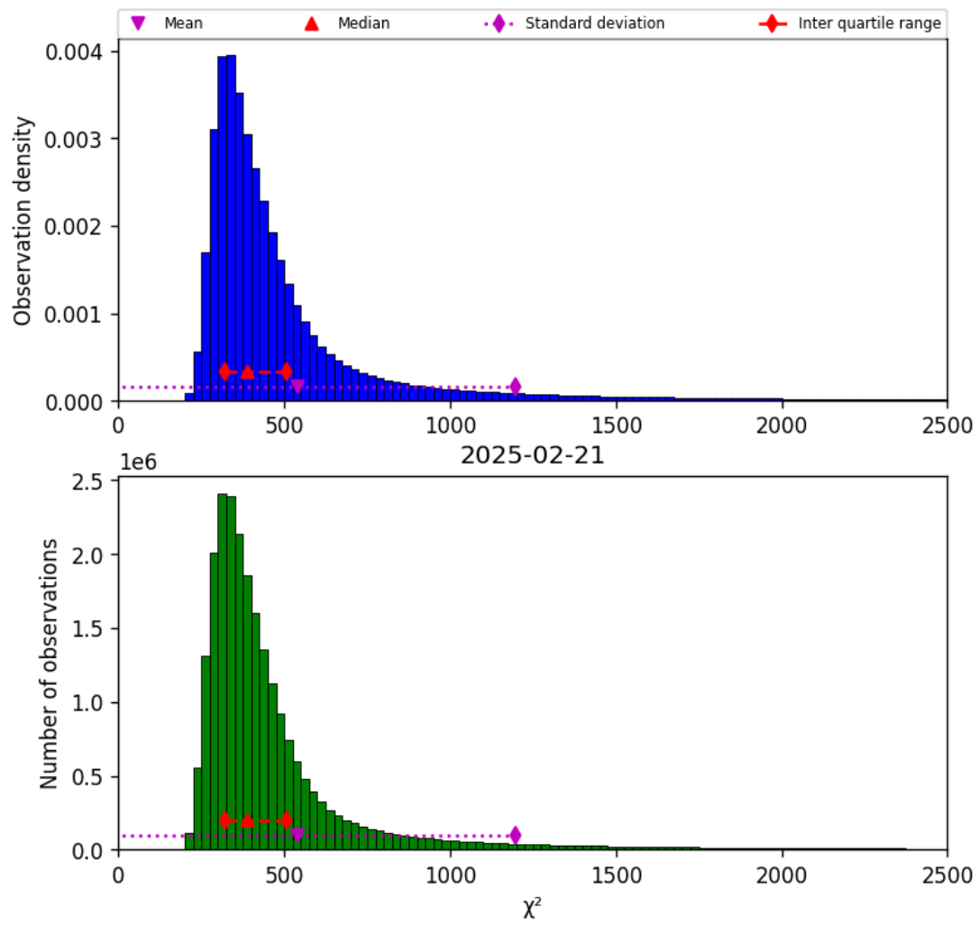
Figure 40: Histogram of “ \chi^2 ” for 2025-02-21 to 2025-02-22
