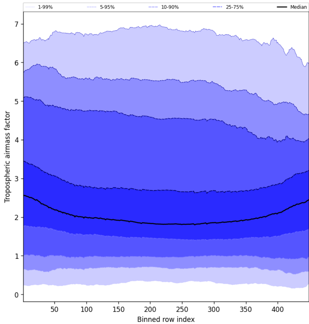
Figure 46: Along track statistics of “Tropospheric airmass factor” for 2025-02-21 to 2025-02-22
