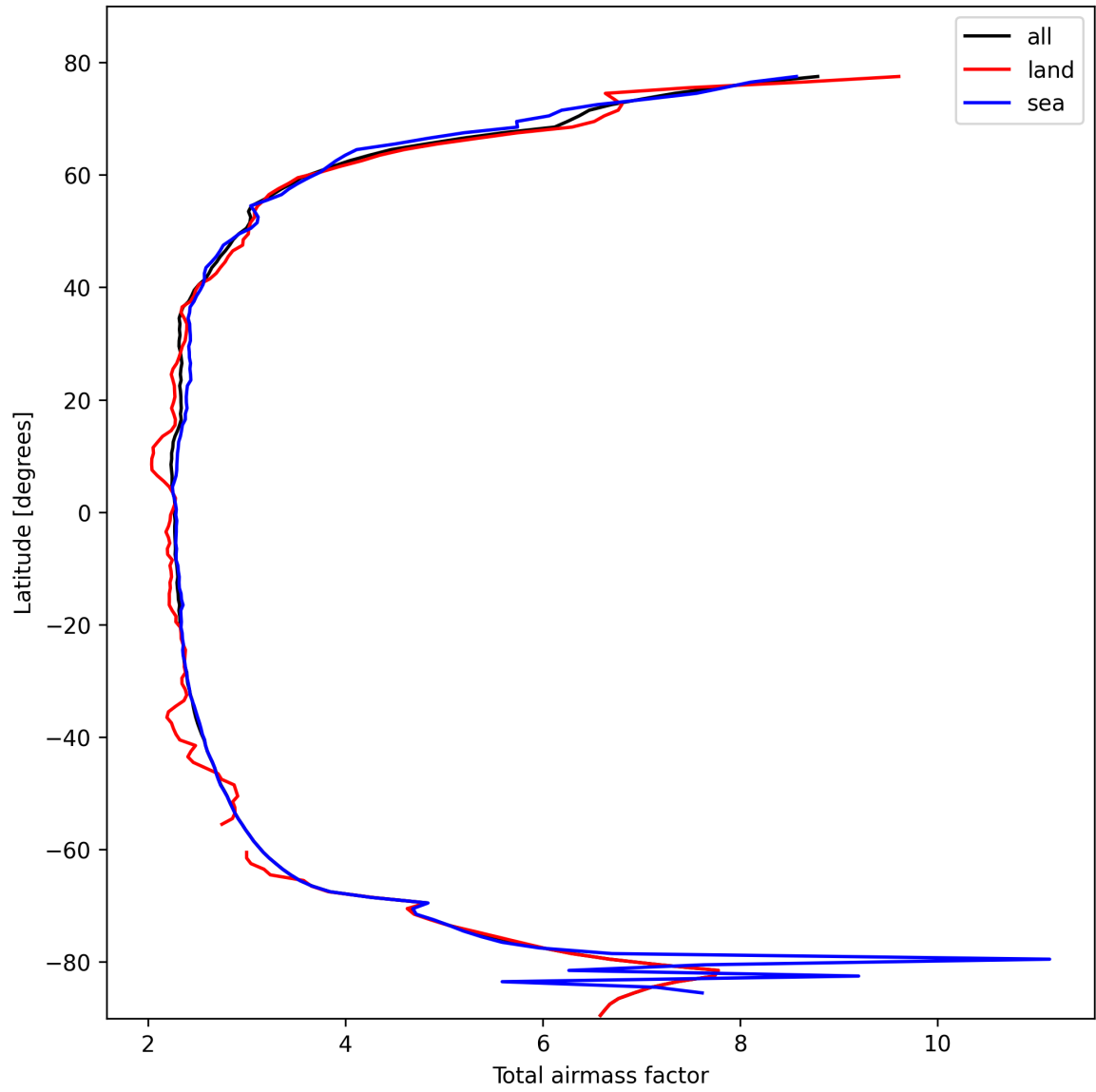
Figure 13: Zonal average of “Total airmass factor” for 2025-02-21 to 2025-02-22.
