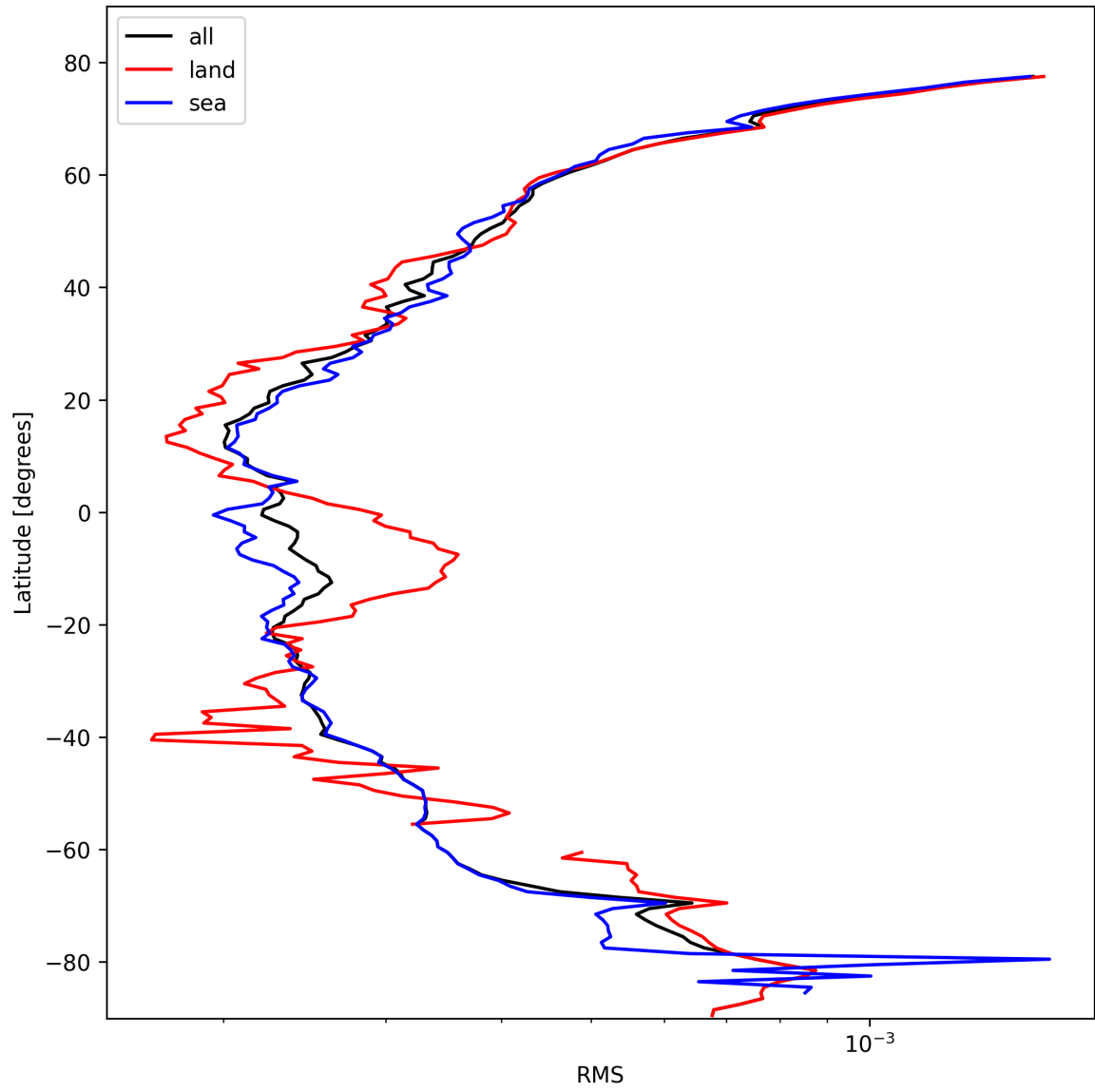
Figure 24: Zonal average of “RMS” for 2025-02-21 to 2025-02-22.
