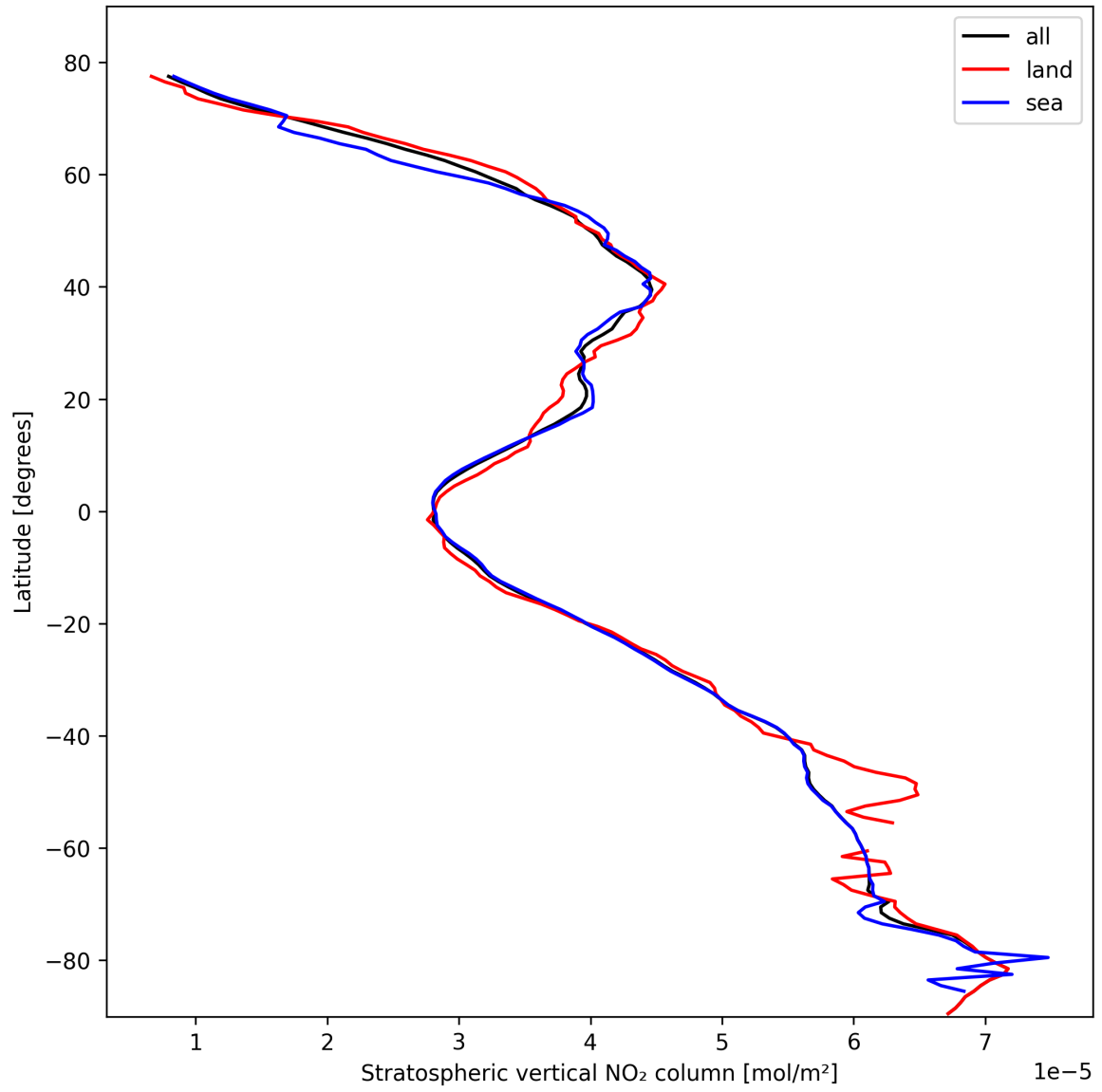
Figure 17: Zonal average of “Stratospheric vertical NO 2 column” for 2025-02-21 to 2025-02-22.
