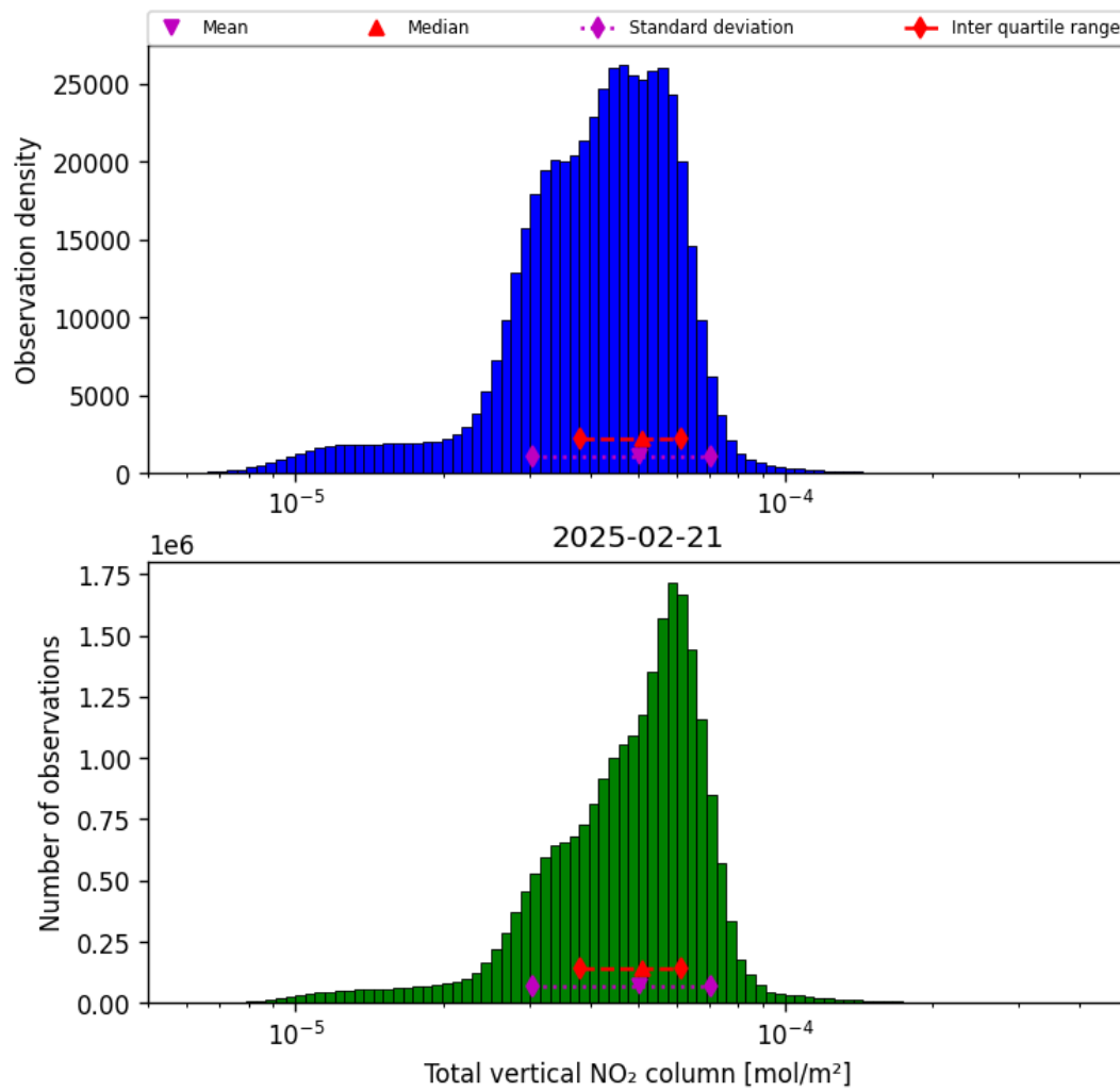
Figure 36: Histogram of “Total vertical NO 2 column” for 2025-02-21 to 2025-02-22
