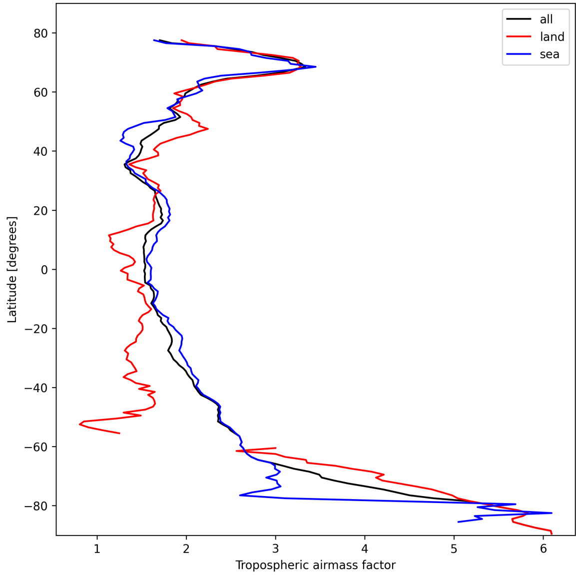
Figure 12: Zonal average of “Tropospheric airmass factor” for 2025-02-21 to 2025-02-22.
