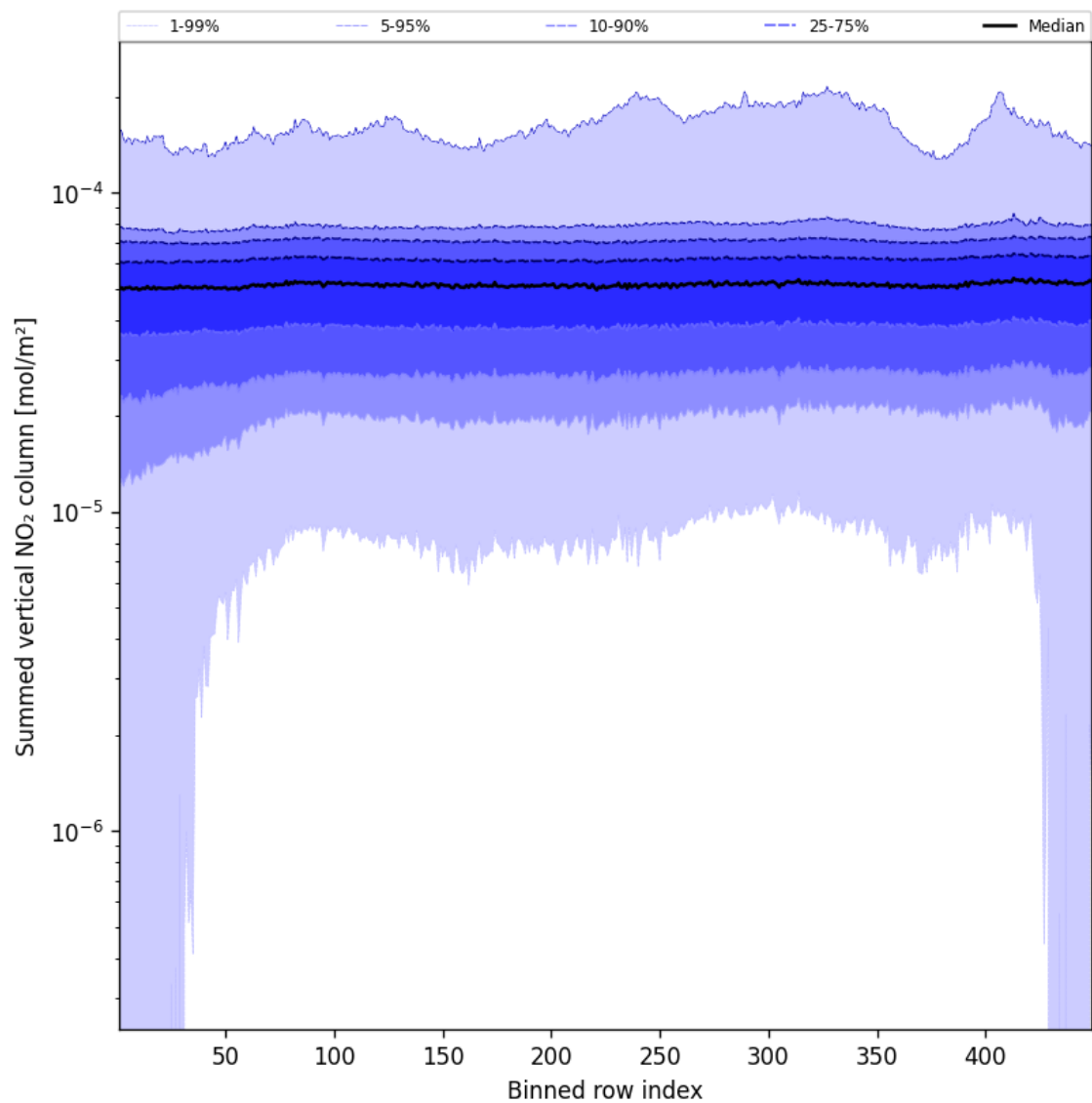
Figure 55: Along track statistics of “Summed vertical NO 2 column” for 2025-02-21 to 2025-02-22
