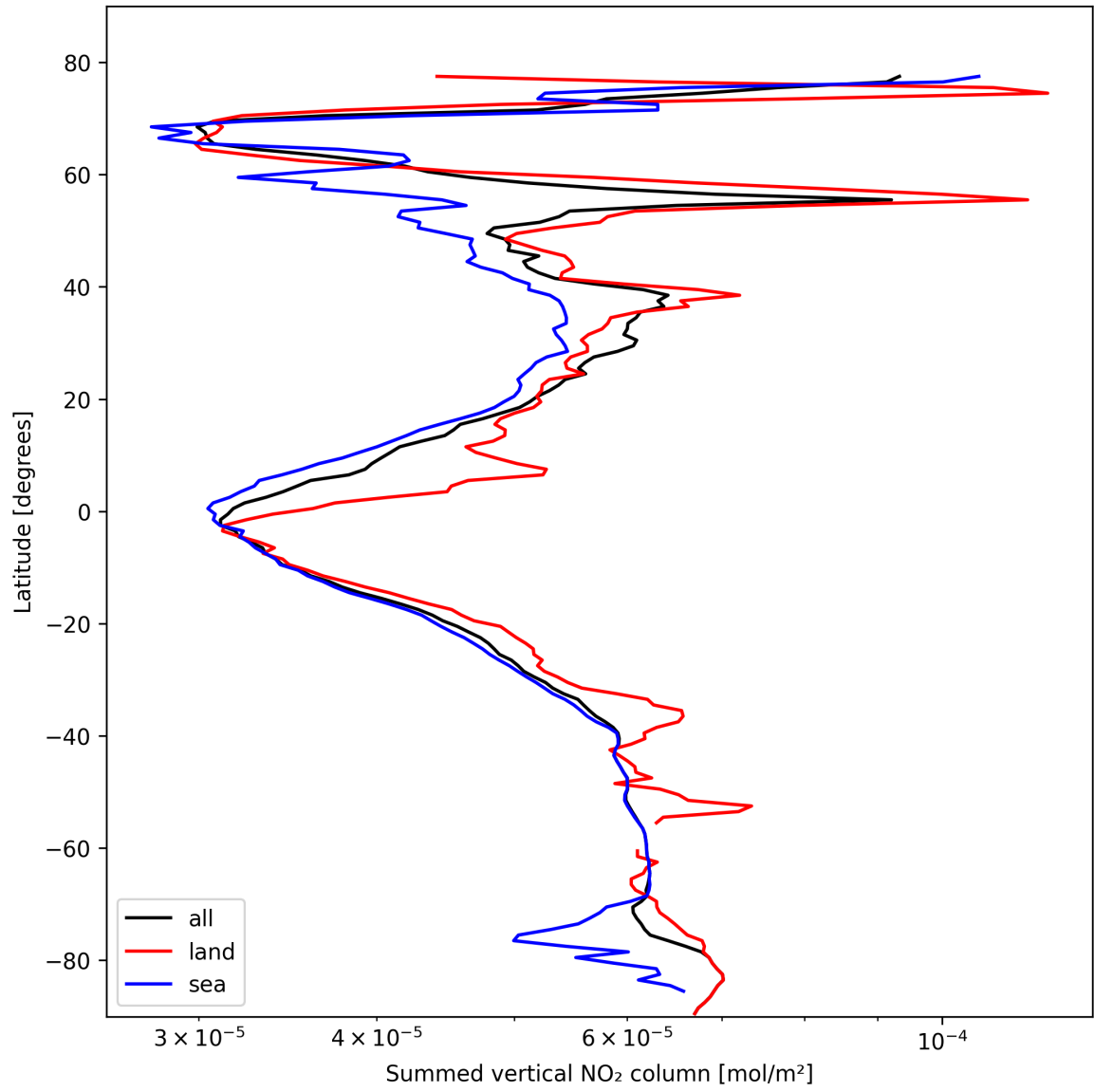
Figure 21: Zonal average of “Summed vertical NO 2 column” for 2025-02-21 to 2025-02-22.
