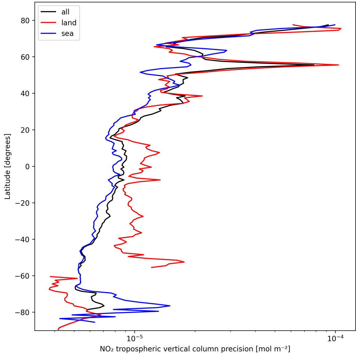
Figure 11: Zonal average of “NO 2 tropospheric vertical column precision” for 2025-02-21 to 2025-02-22.
