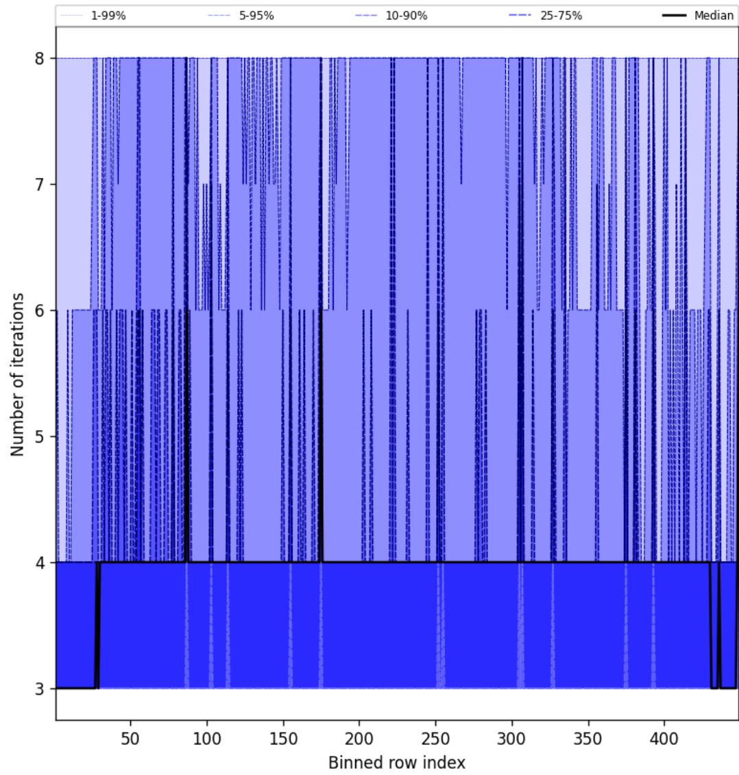
Figure 49: Along track statistics of “Number of iterations” for 2025-02-21 to 2025-02-22
