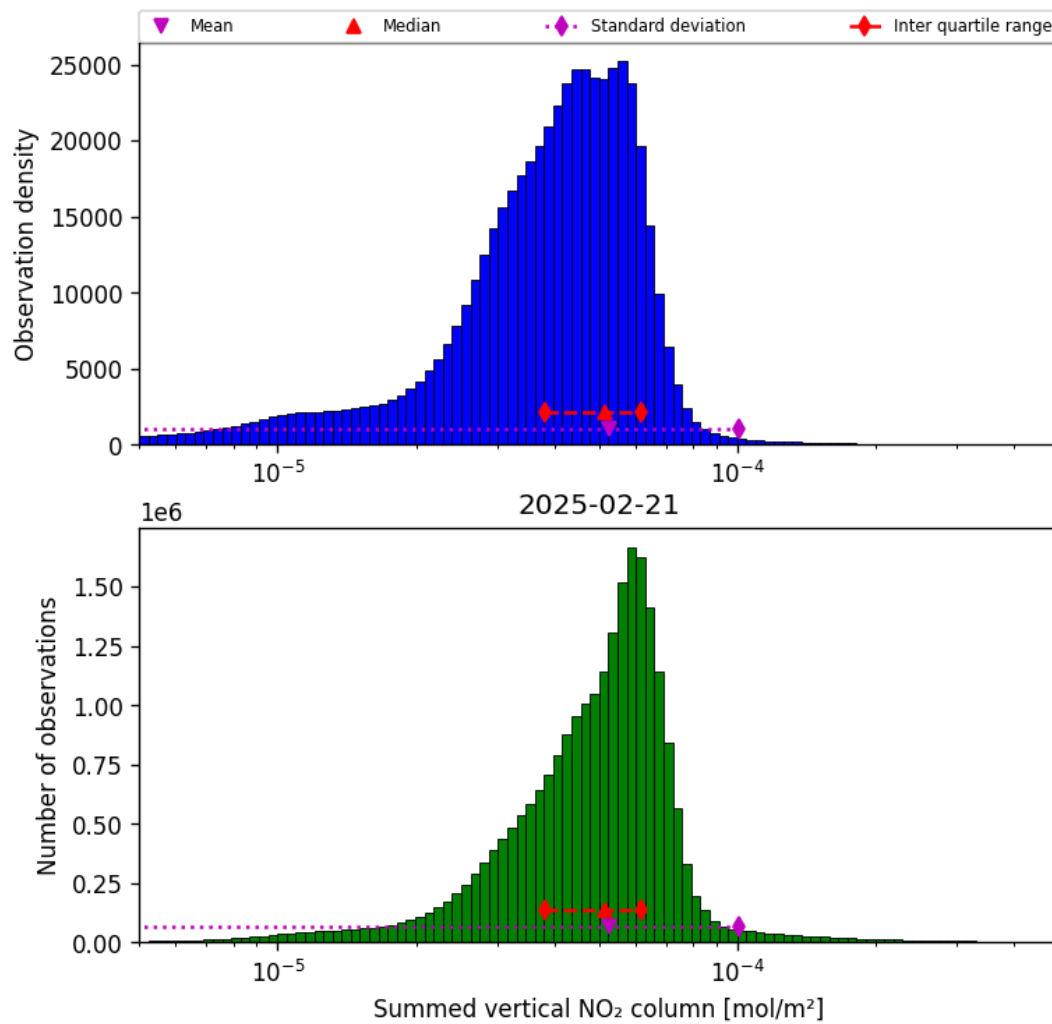
Figure 38: Histogram of "Summed vertical NO 2 column" for 2025-02-21 to 2025-02-22
