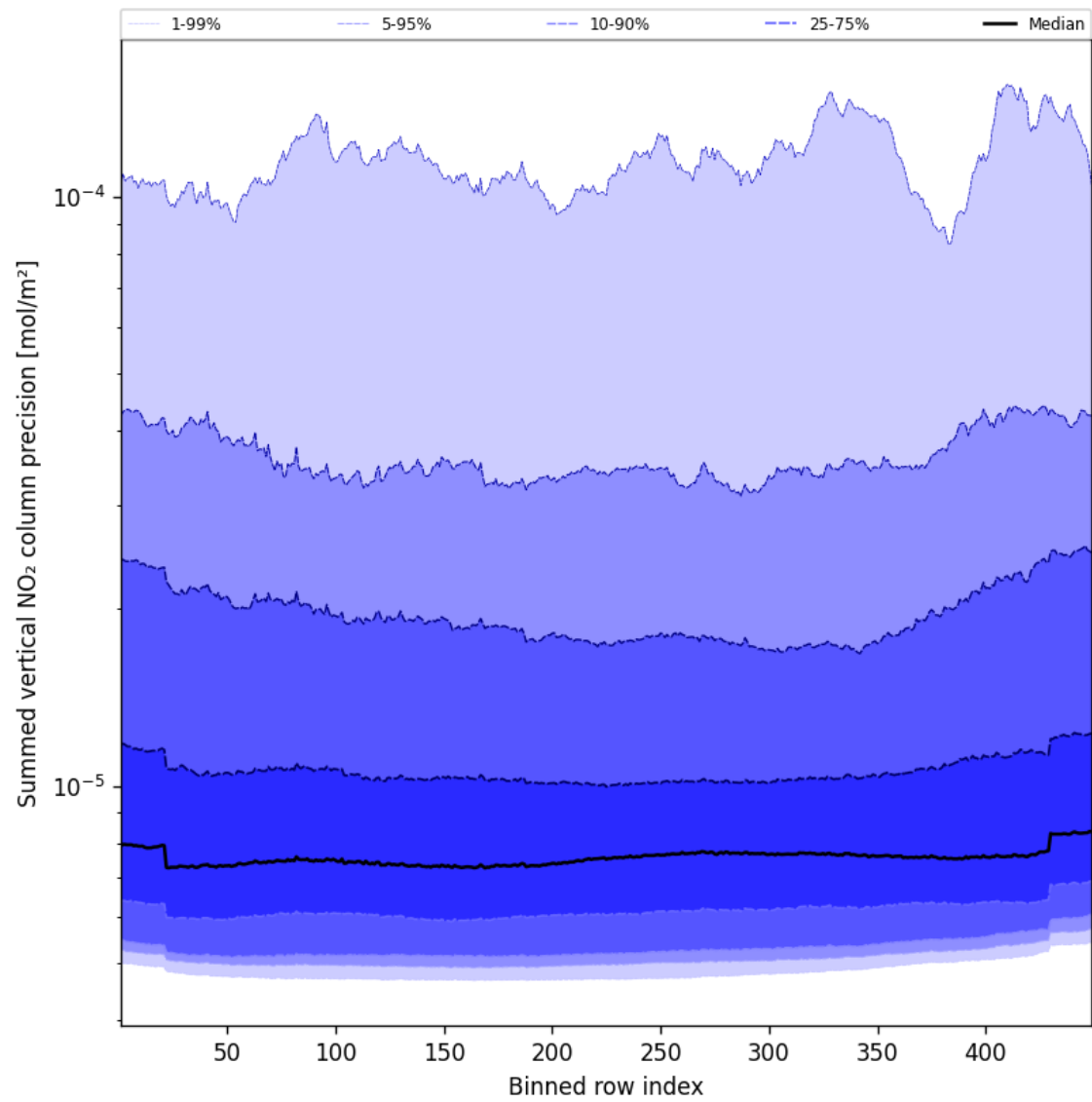
Figure 56: Along track statistics of “Summed vertical NO 2 column precision” for 2025-02-21 to 2025-02-22
