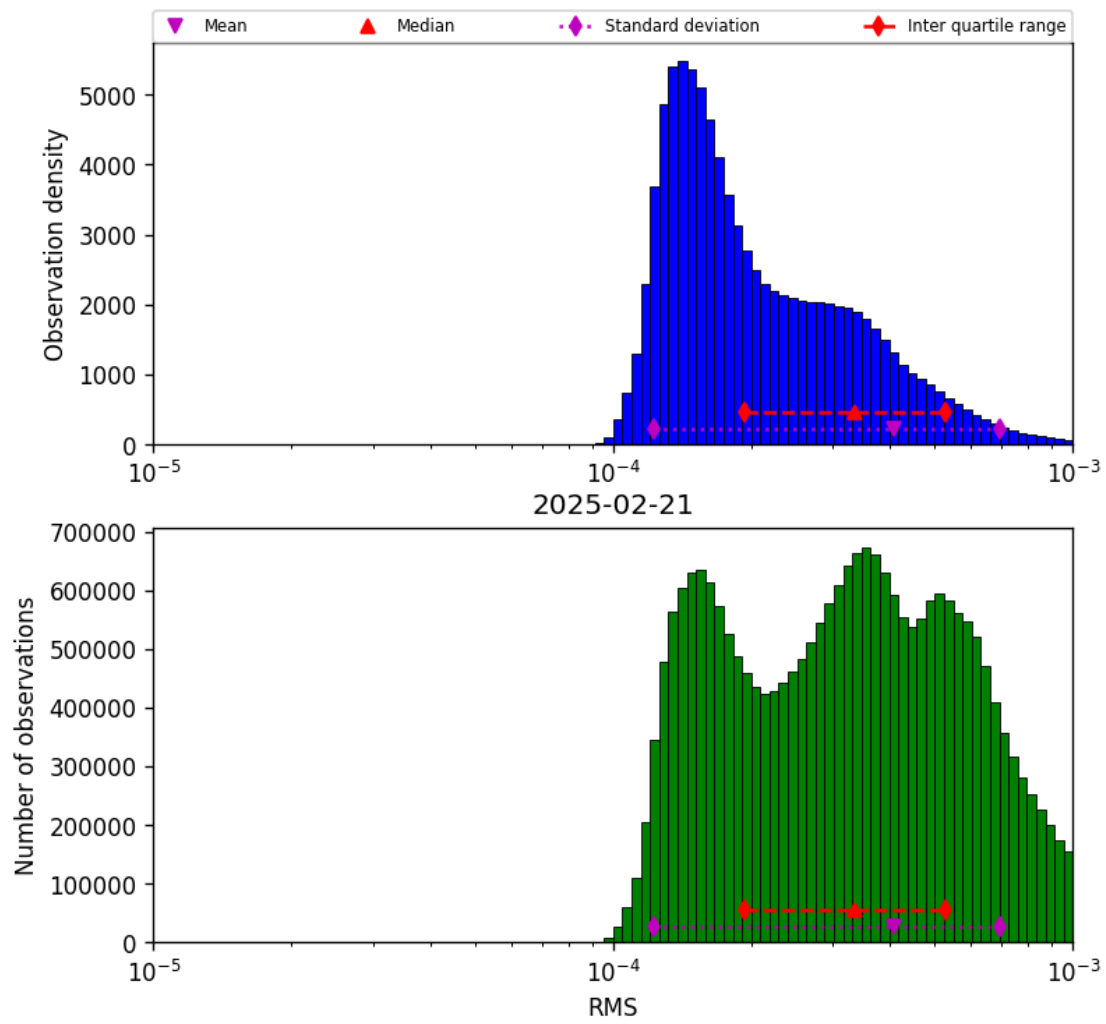
Figure 41: Histogram of “RMS” for 2025-02-21 to 2025-02-22
