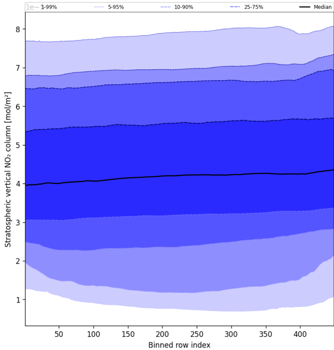
Figure 51: Along track statistics of “Stratospheric vertical NO 2 column” for 2025-02-21 to 2025-02-22
