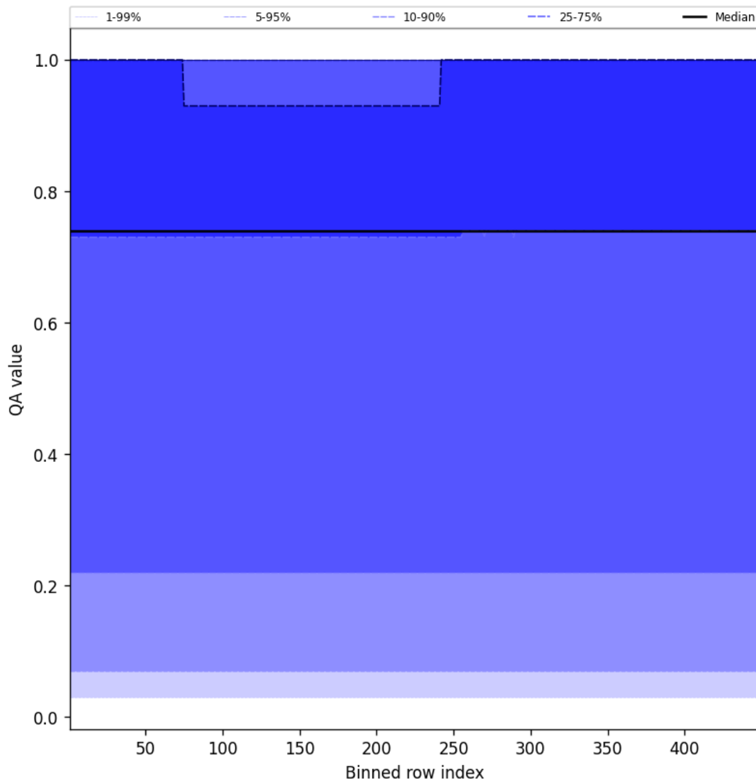
Figure 43: Along track statistics of “QA value” for 2025-02-21 to 2025-02-22
