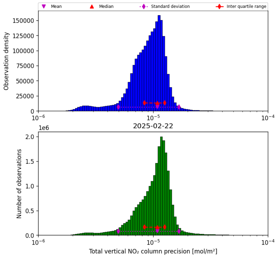
Figure 37: Histogram of "Total vertical NO 2 column precision" for 2025-02-22 to 2025-02-22
