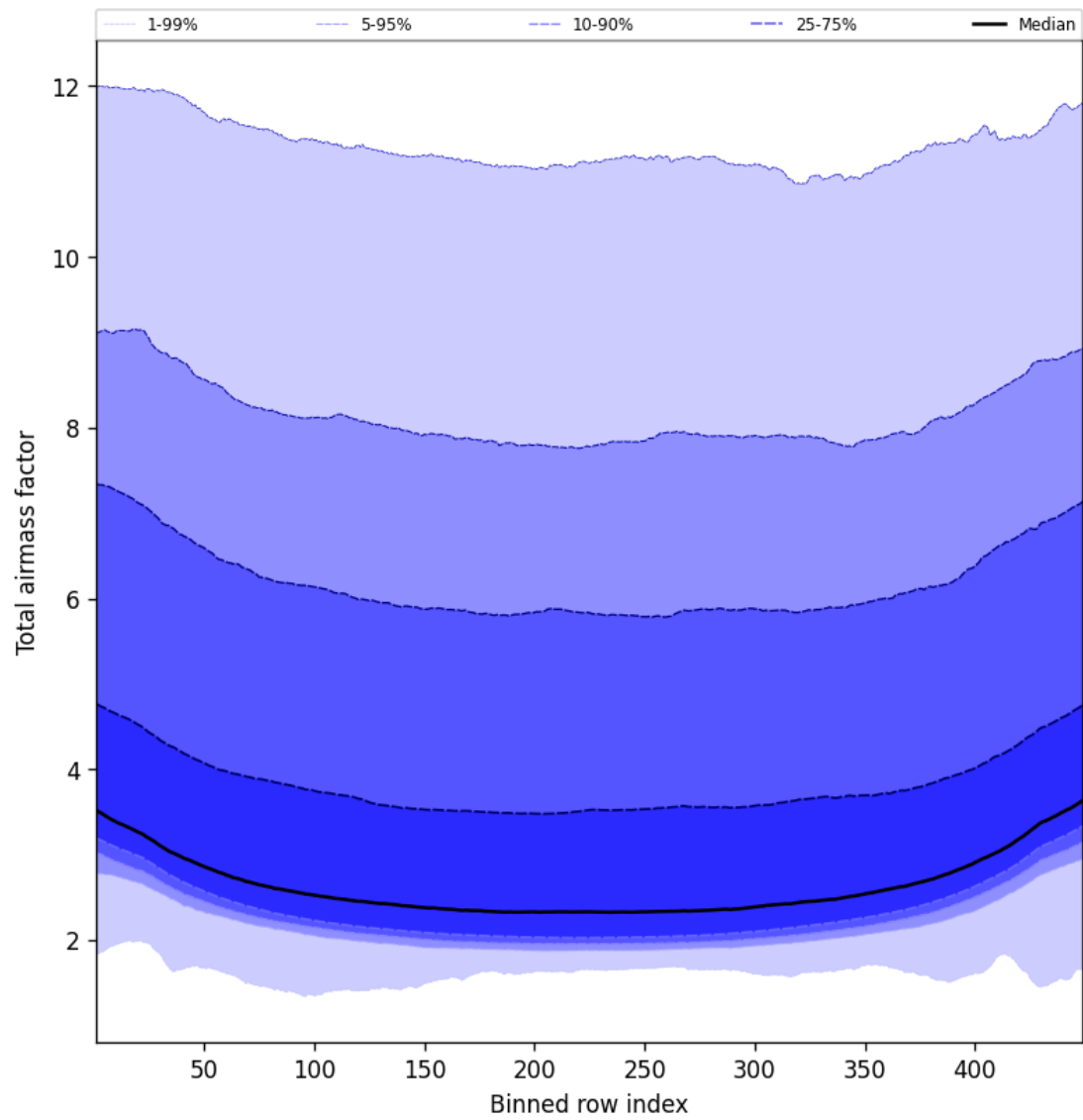
Figure 47: Along track statistics of “Total airmass factor” for 2025-02-22 to 2025-02-22
