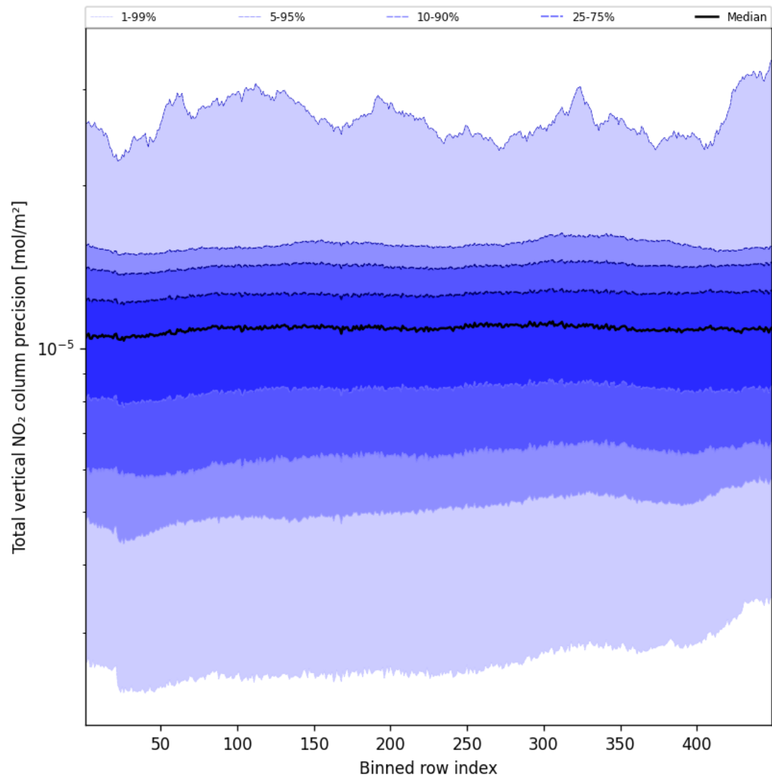
Figure 54: Along track statistics of “Total vertical NO 2 column precision” for 2025-02-22 to 2025-02-22
