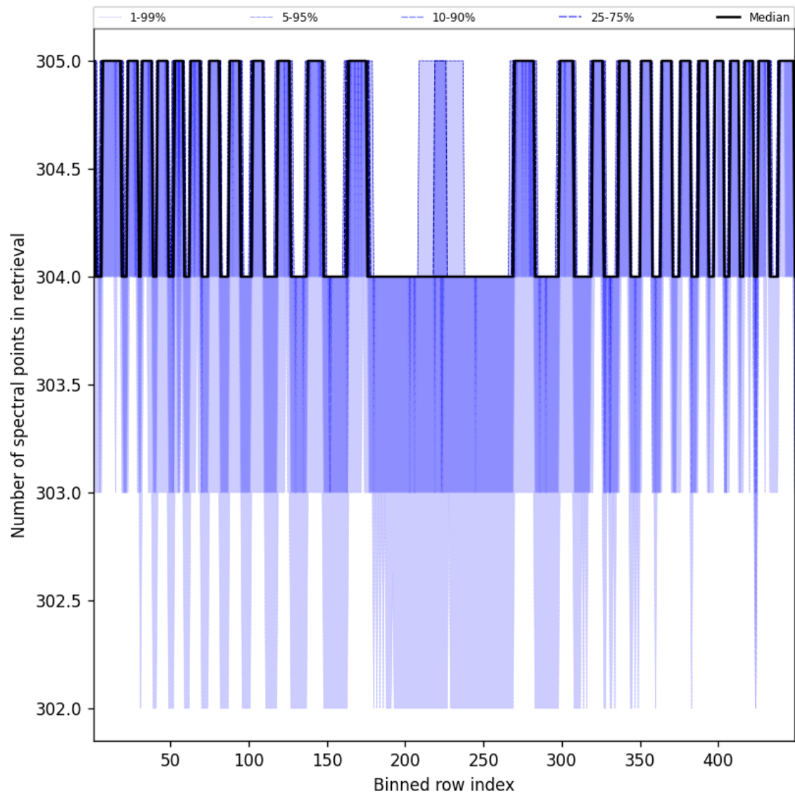
Figure 48: Along track statistics of “Number of spectral points in retrieval” for 2025-02-22 to 2025-02-22
