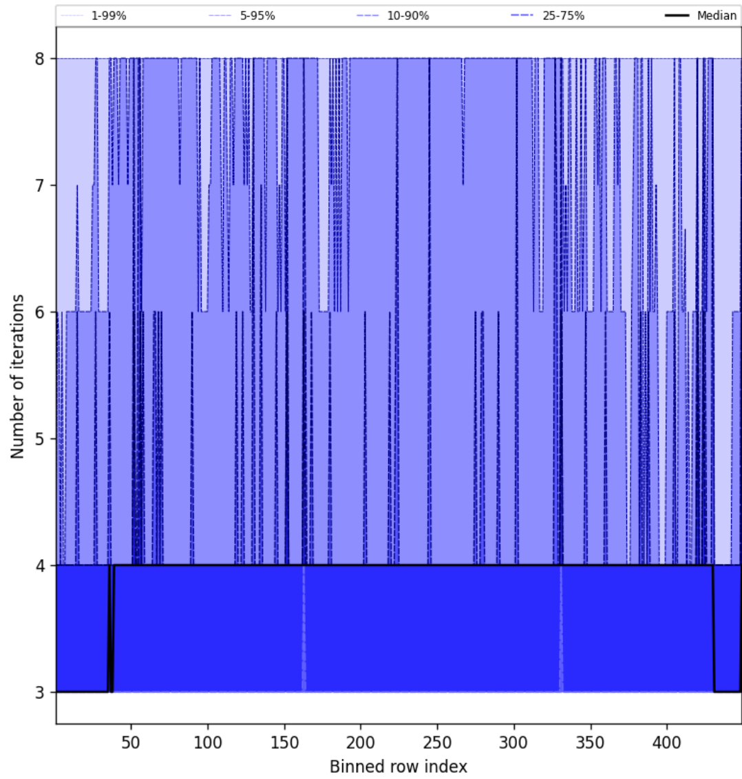
Figure 49: Along track statistics of “Number of iterations” for 2025-02-22 to 2025-02-22
