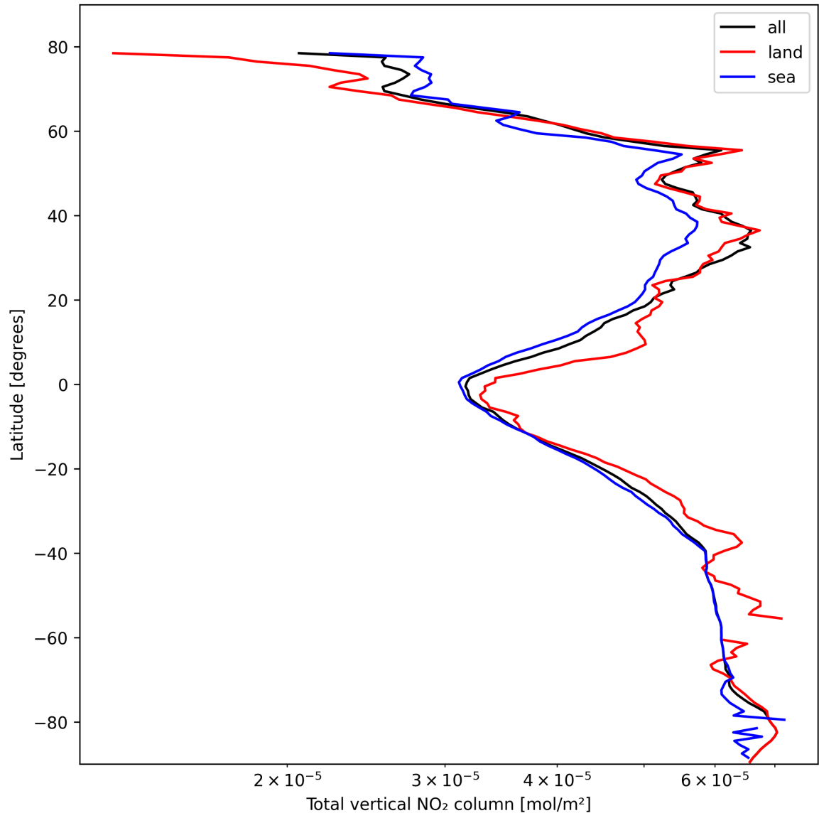
Figure 19: Zonal average of “Total vertical NO 2 column” for 2025-02-22 to 2025-02-22.
