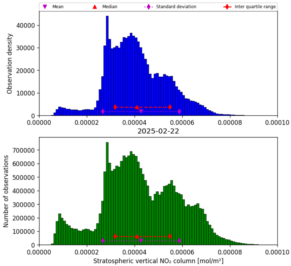
Figure 34: Histogram of “Stratospheric vertical NO 2 column” for 2025-02-22 to 2025-02-22
