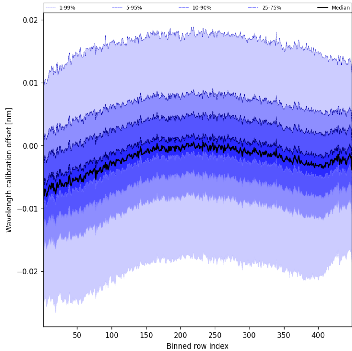
Figure 50: Along track statistics of “Wavelength calibration offset” for 2025-02-22 to 2025-02-22
