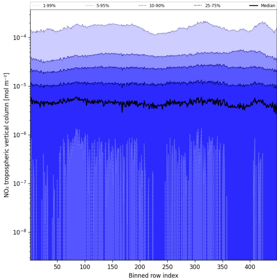
Figure 44: Along track statistics of “NO 2 tropospheric vertical column” for 2025-02-22 to 2025-02-22
