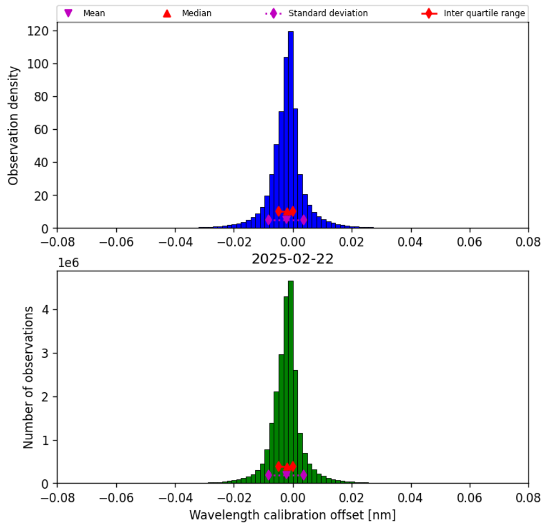
Figure 33: Histogram of “Wavelength calibration offset” for 2025-02-22 to 2025-02-22
