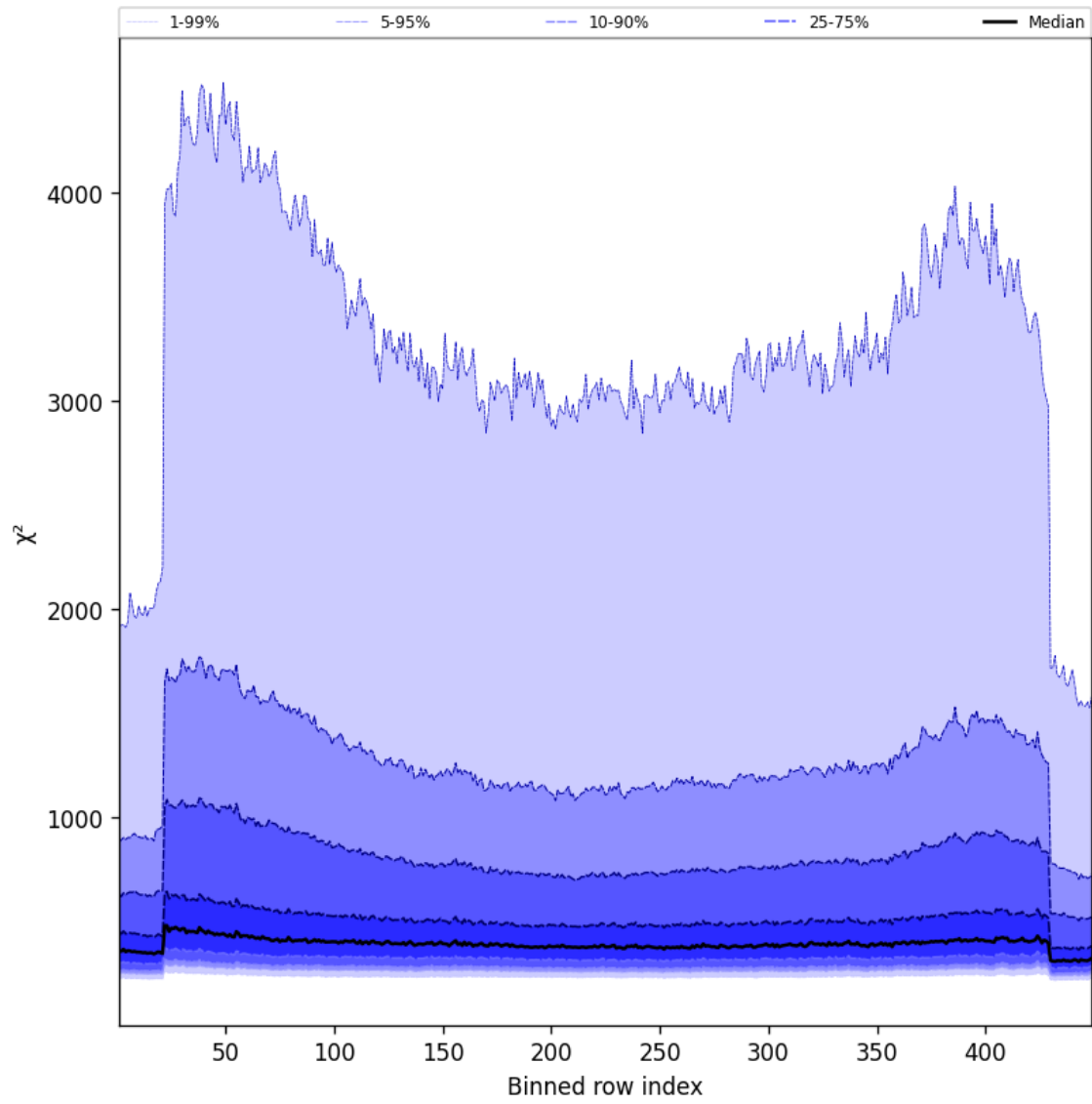
Figure 57: Along track statistics of “ \chi^2 ” for 2025-02-22 to 2025-02-22
