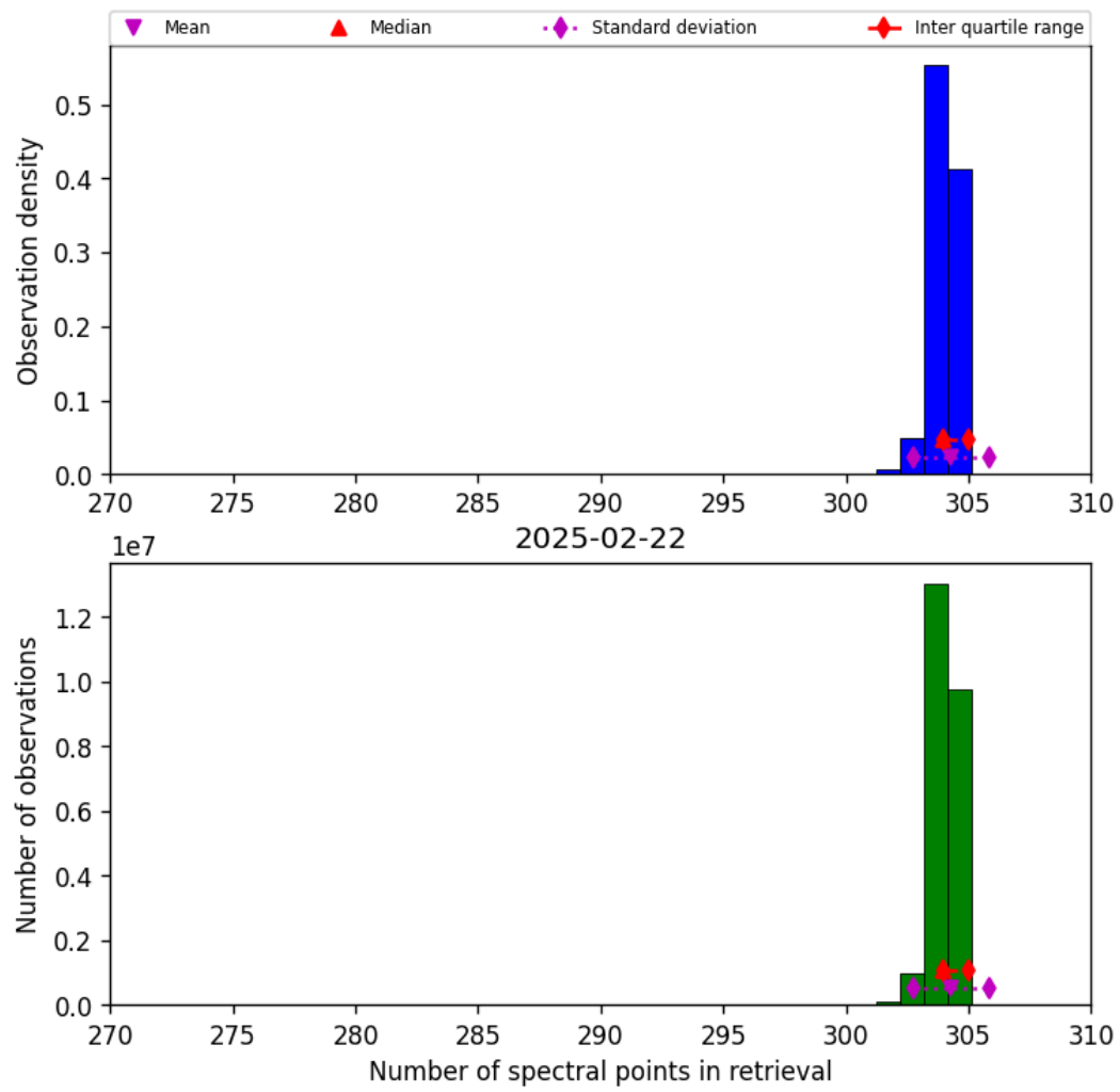
Figure 31: Histogram of “Number of spectral points in retrieval” for 2025-02-22 to 2025-02-22
