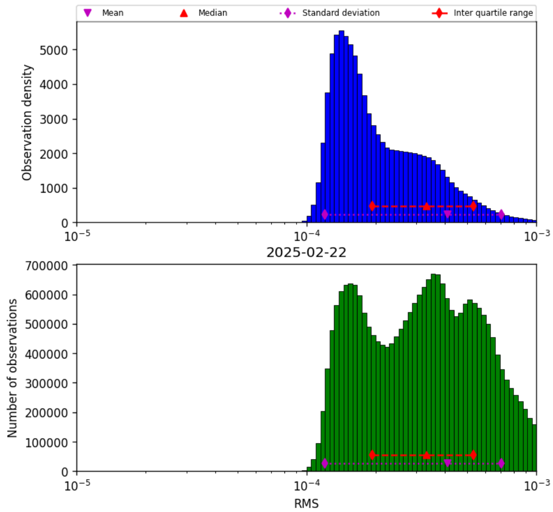
Figure 41: Histogram of “RMS” for 2025-02-22 to 2025-02-22
