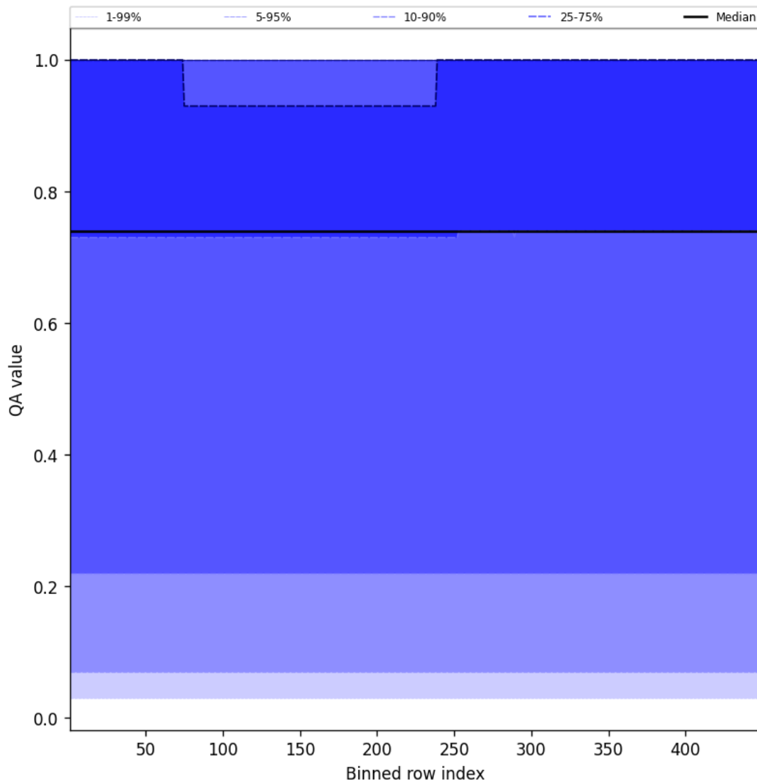
Figure 43: Along track statistics of “QA value” for 2025-02-22 to 2025-02-22
