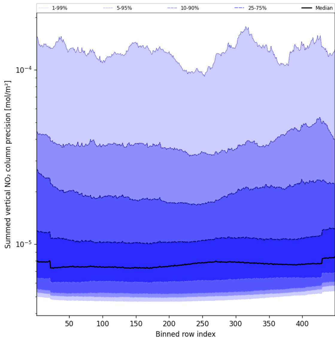
Figure 56: Along track statistics of “Summed vertical NO 2 column precision” for 2025-02-22 to 2025-02-22
