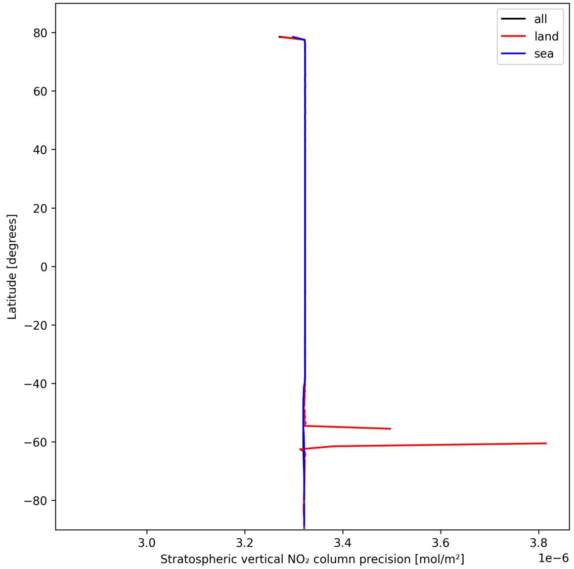
Figure 18: Zonal average of “Stratospheric vertical NO 2 column precision” for 2025-02-22 to 2025-02-22.
