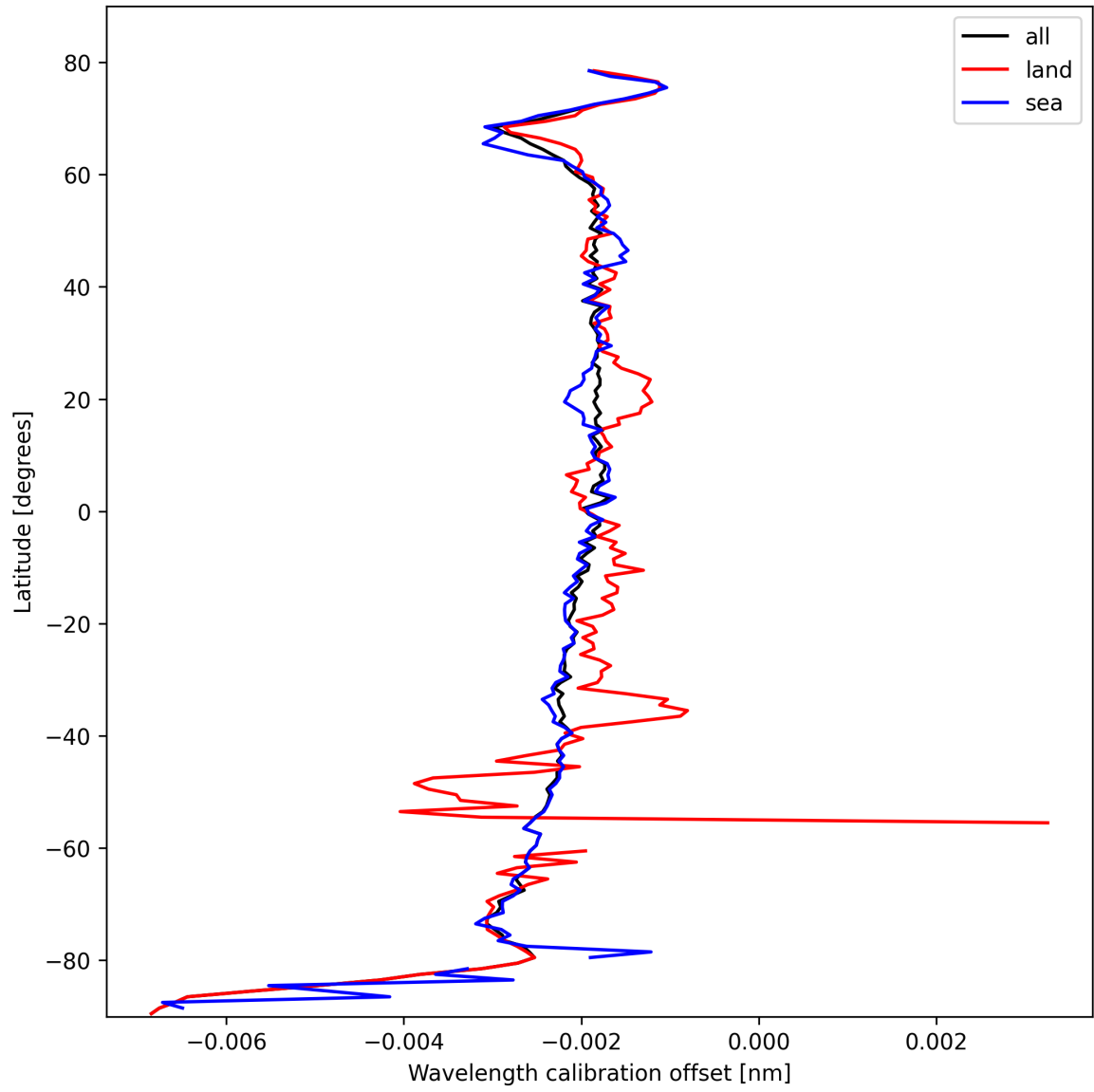
Figure 16: Zonal average of “Wavelength calibration offset” for 2025-02-22 to 2025-02-22.
