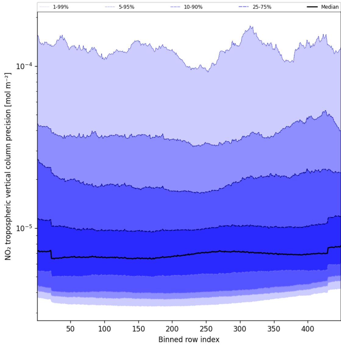
Figure 45: Along track statistics of “NO 2 tropospheric vertical column precision” for 2025-02-22 to 2025-02-22
