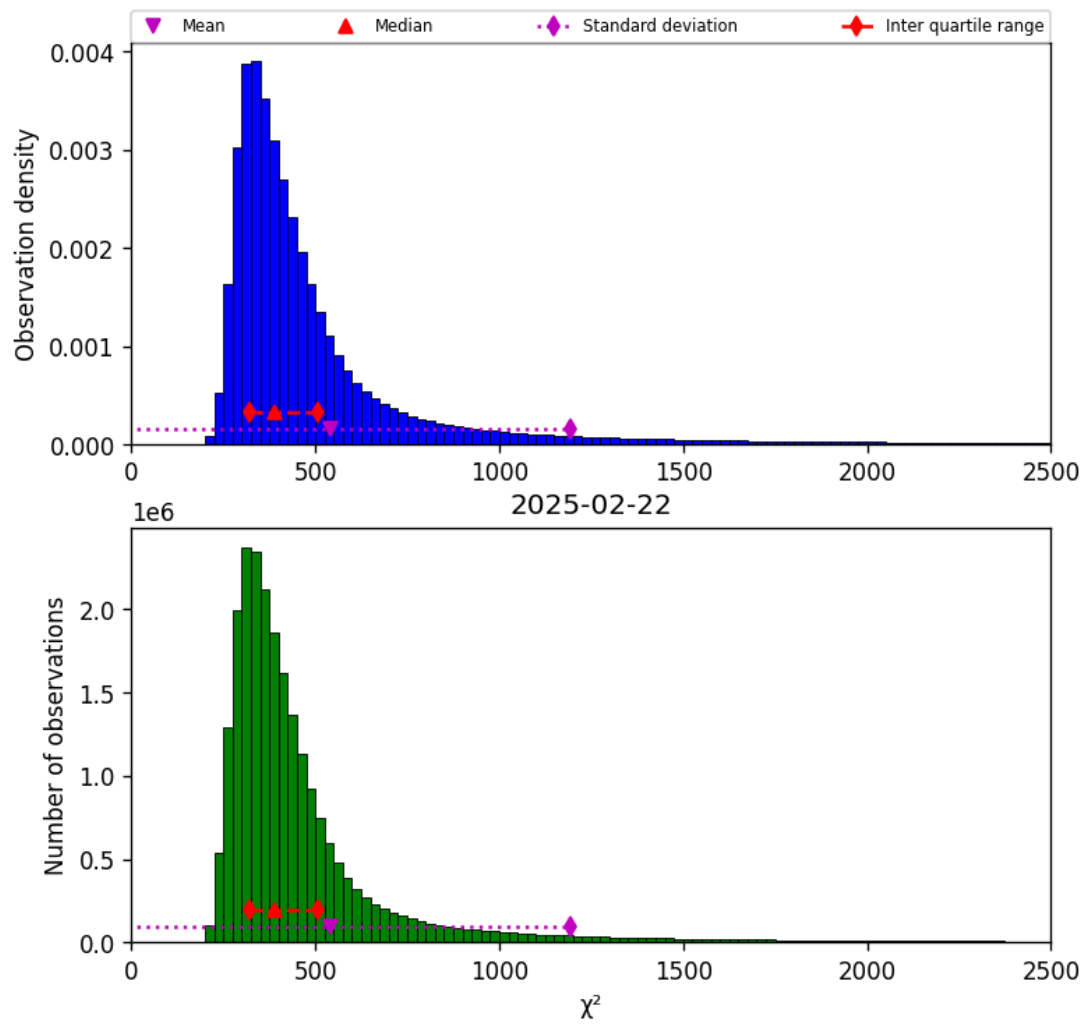
Figure 40: Histogram of “ \chi^2 ” for 2025-02-22 to 2025-02-22
