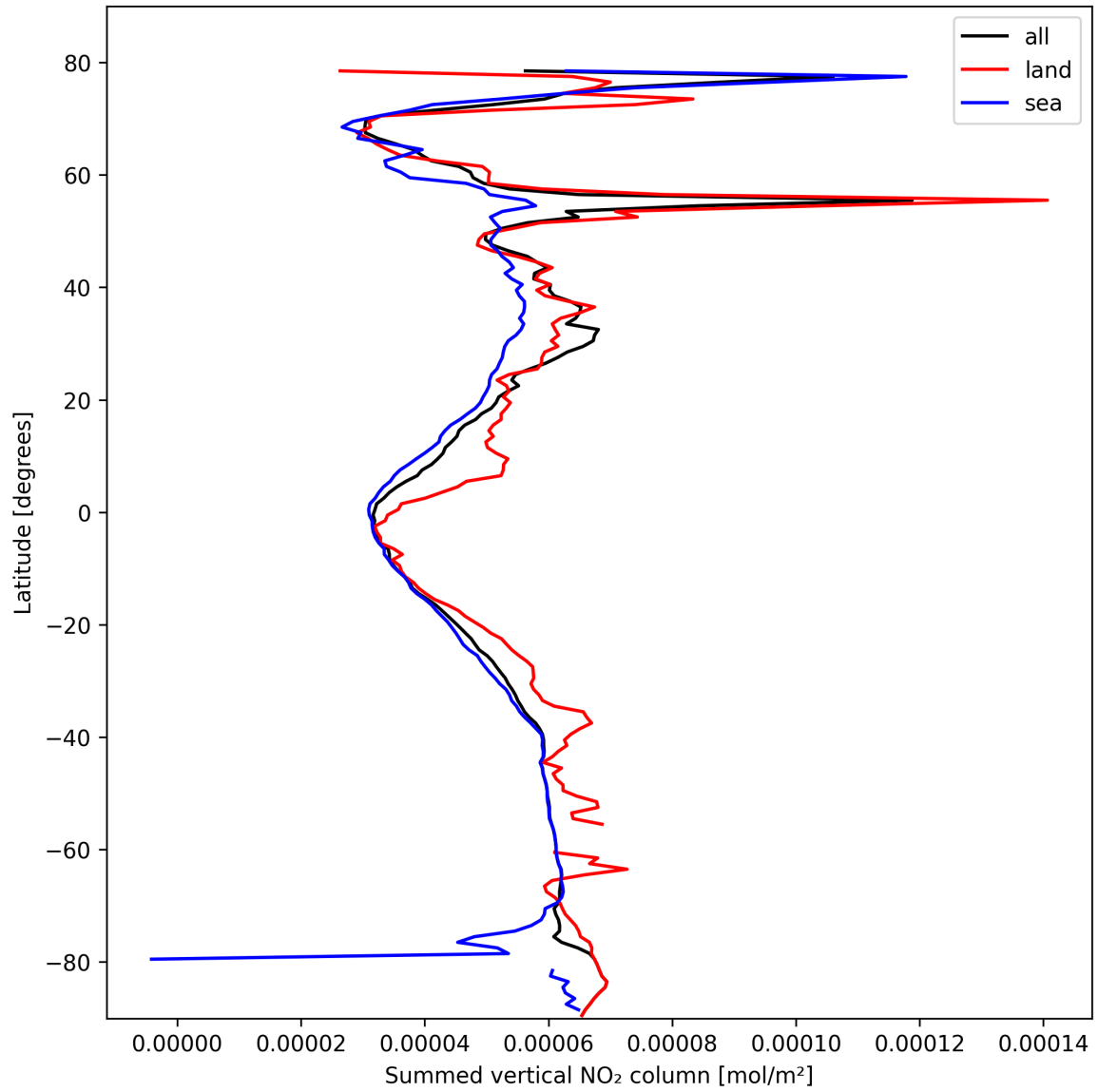
Figure 21: Zonal average of “Summed vertical NO 2 column” for 2025-02-22 to 2025-02-22.
