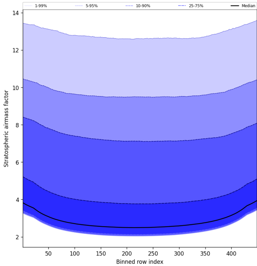
Figure 59: Along track statistics of “Stratospheric airmass factor” for 2025-02-22 to 2025-02-22
