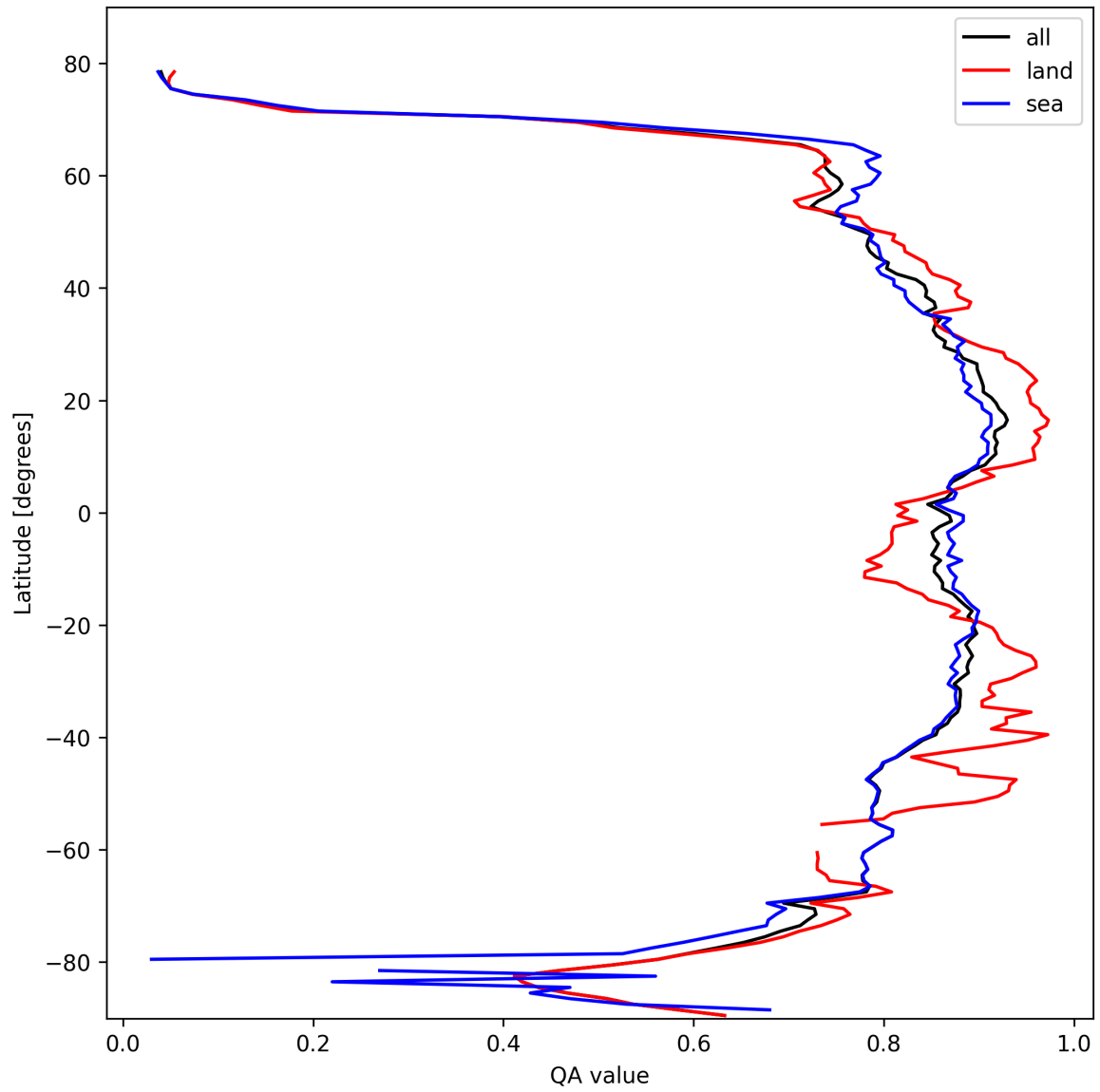
Figure 9: Zonal average of “QA value” for 2025-02-22 to 2025-02-22.
