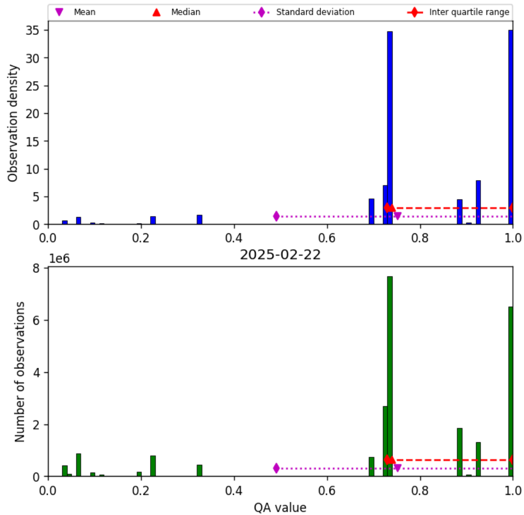
Figure 26: Histogram of “QA value” for 2025-02-22 to 2025-02-22
