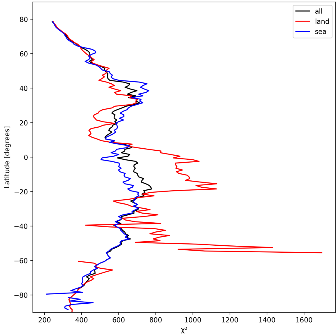
Figure 23: Zonal average of “ \chi^2 ” for 2025-02-22 to 2025-02-22.
