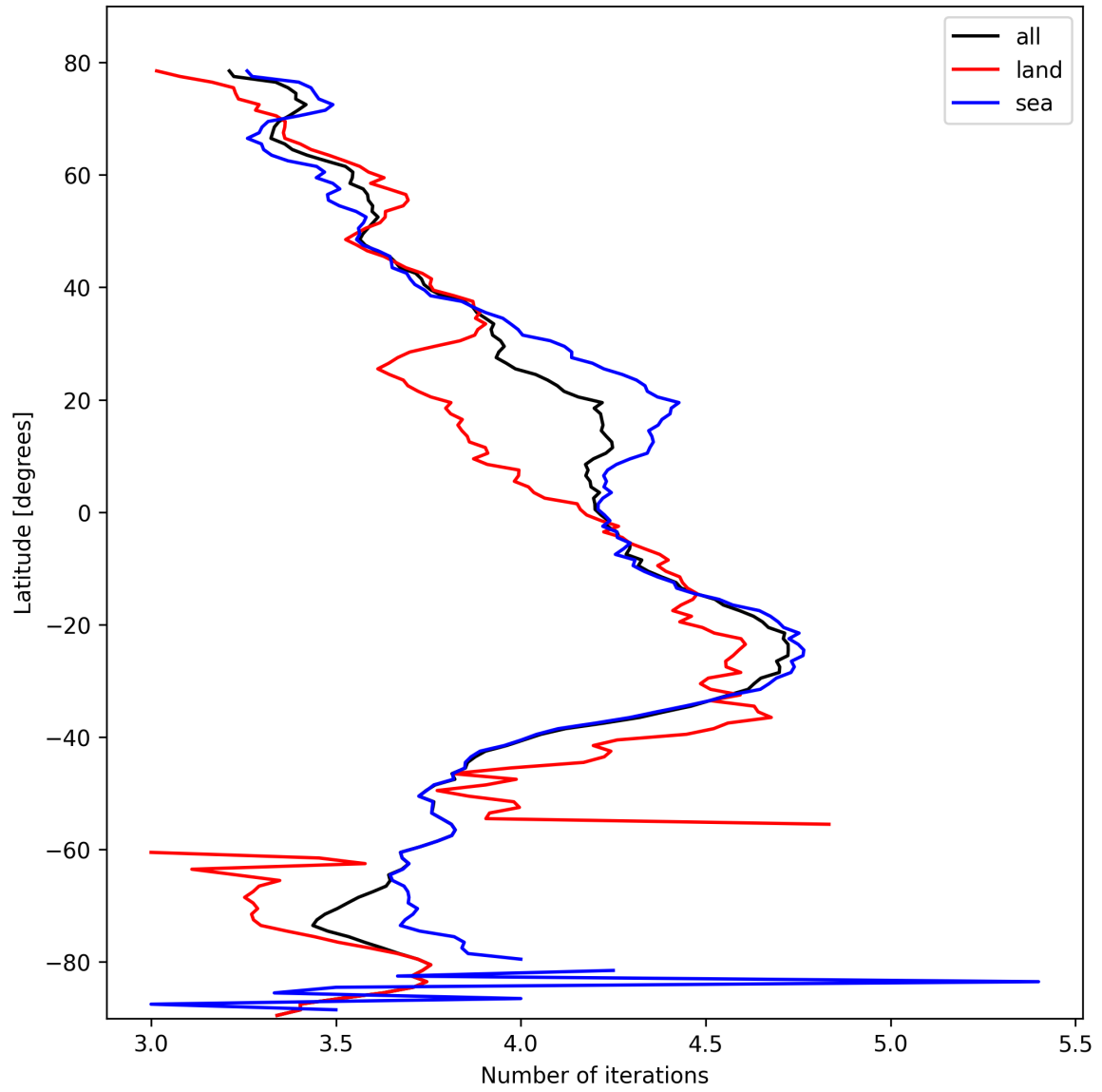
Figure 15: Zonal average of “Number of iterations” for 2025-02-22 to 2025-02-22.
