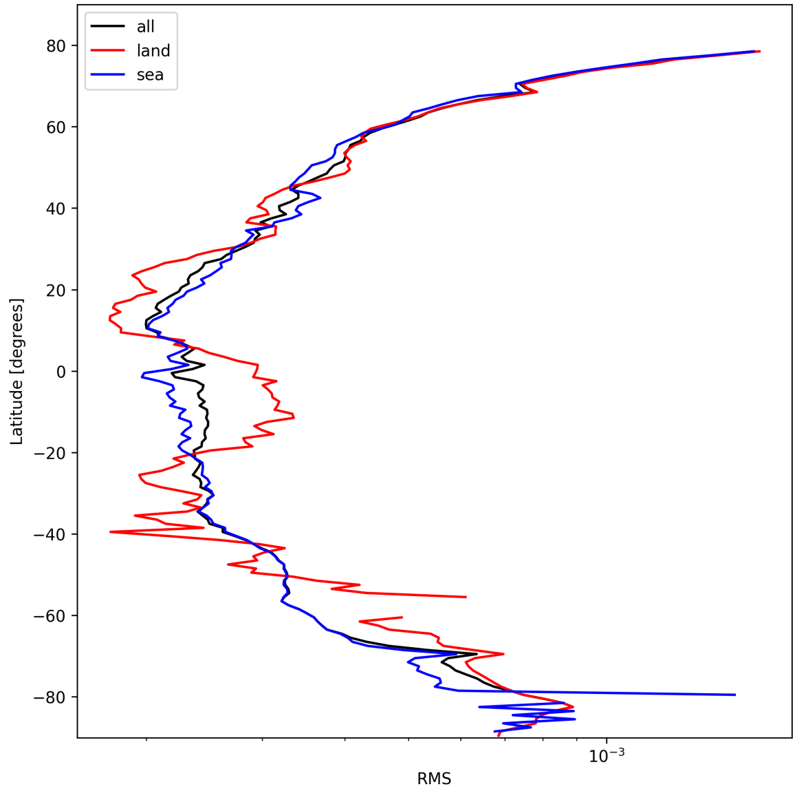
Figure 24: Zonal average of “RMS” for 2025-02-22 to 2025-02-22.
