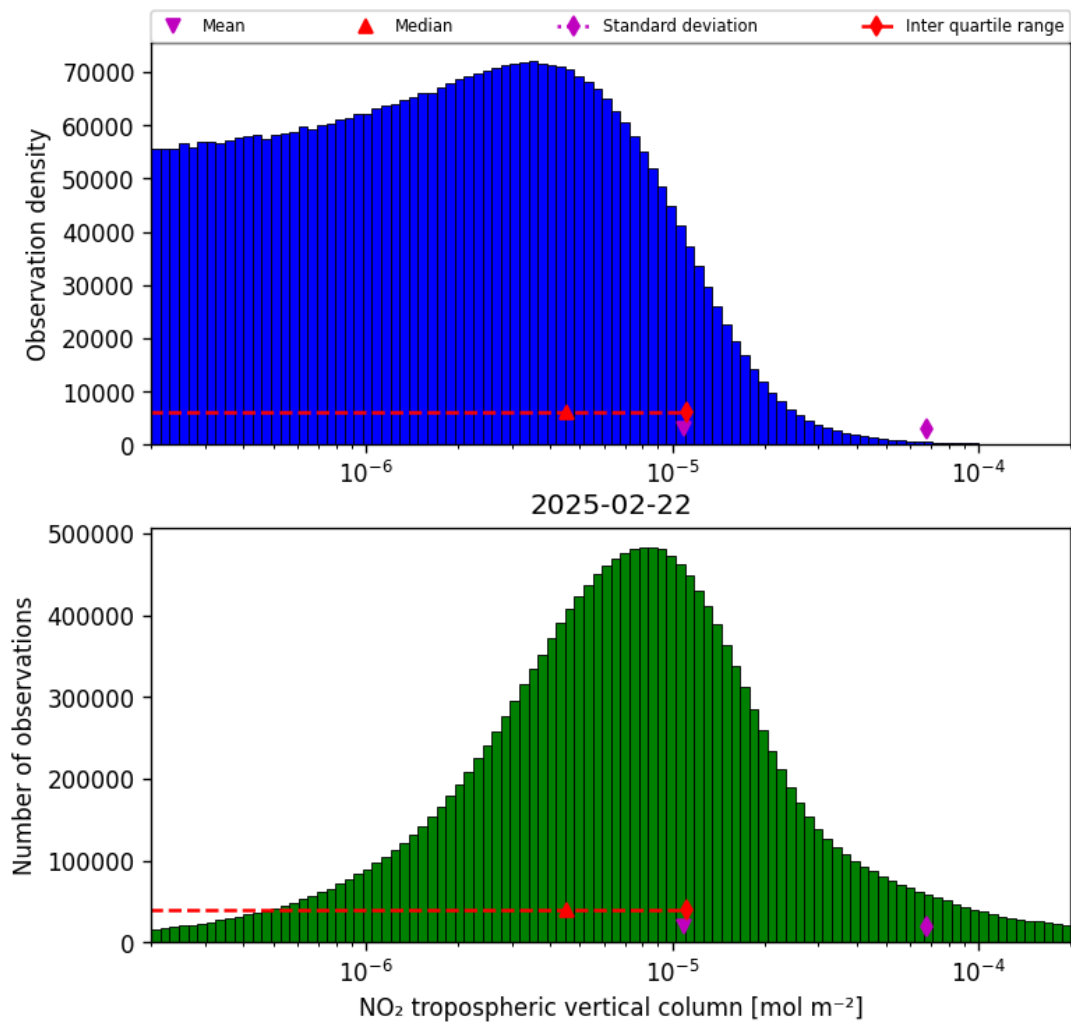
Figure 27: Histogram of “ \text{NO}_2 tropospheric vertical column” for 2025-02-22 to 2025-02-22
