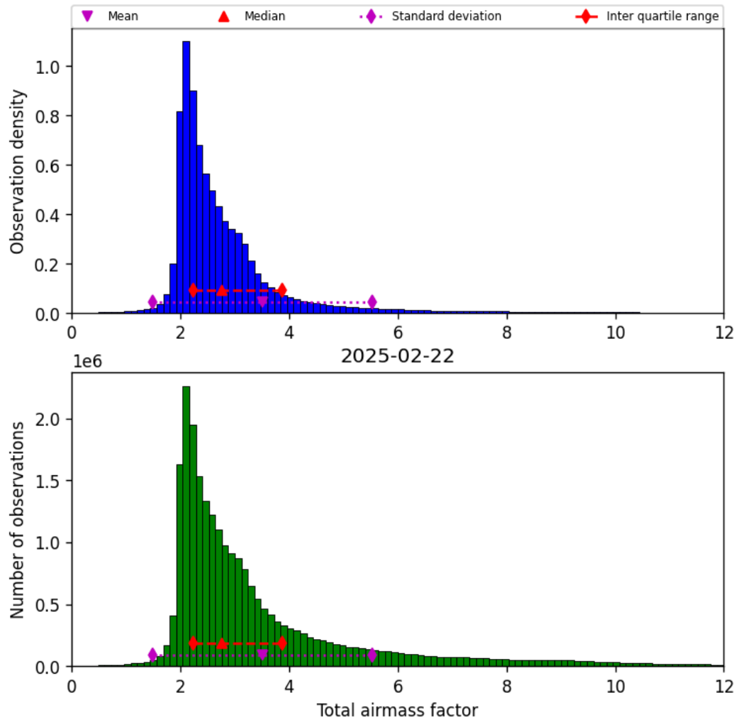
Figure 30: Histogram of “Total airmass factor” for 2025-02-22 to 2025-02-22
