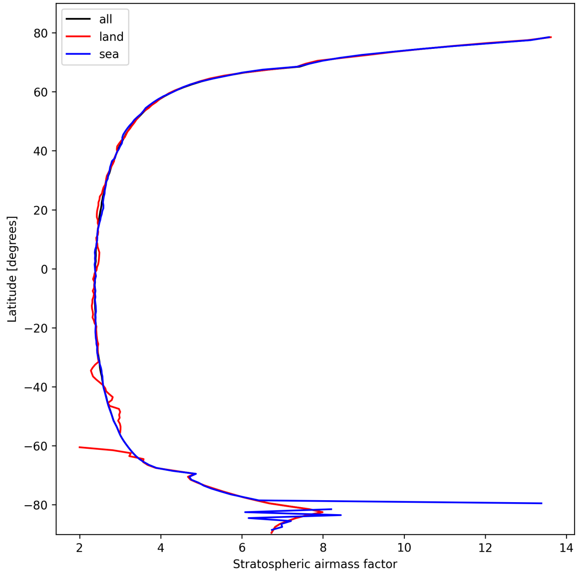
Figure 25: Zonal average of “Stratospheric airmass factor” for 2025-02-22 to 2025-02-22.
