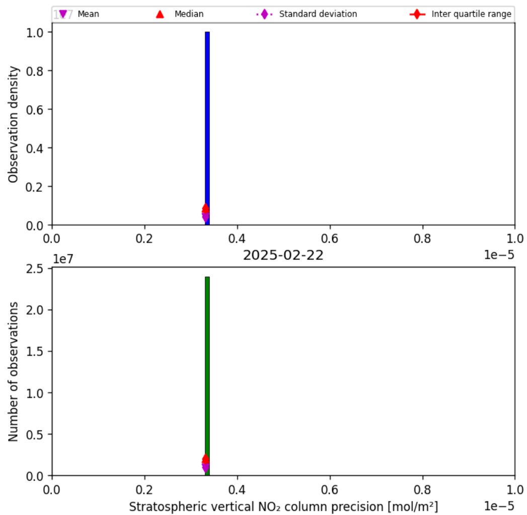
Figure 35: Histogram of “Stratospheric vertical NO 2 column precision” for 2025-02-22 to 2025-02-22
