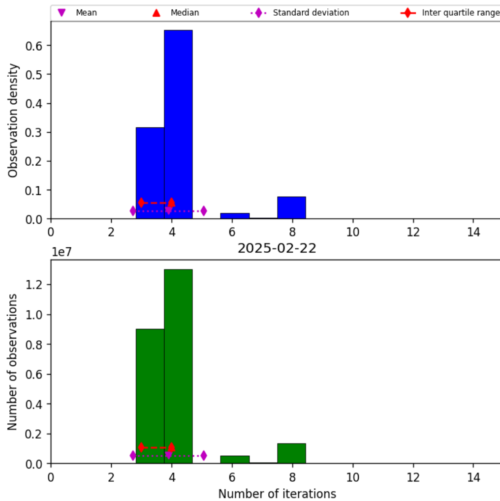
Figure 32: Histogram of “Number of iterations” for 2025-02-22 to 2025-02-22
