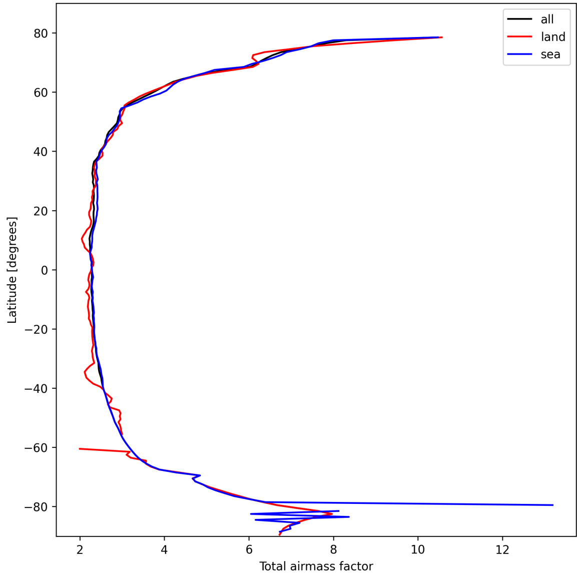
Figure 13: Zonal average of “Total airmass factor” for 2025-02-22 to 2025-02-22.
