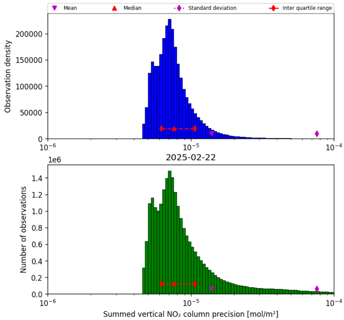
Figure 39: Histogram of "Summed vertical NO 2 column precision" for 2025-02-22 to 2025-02-22
