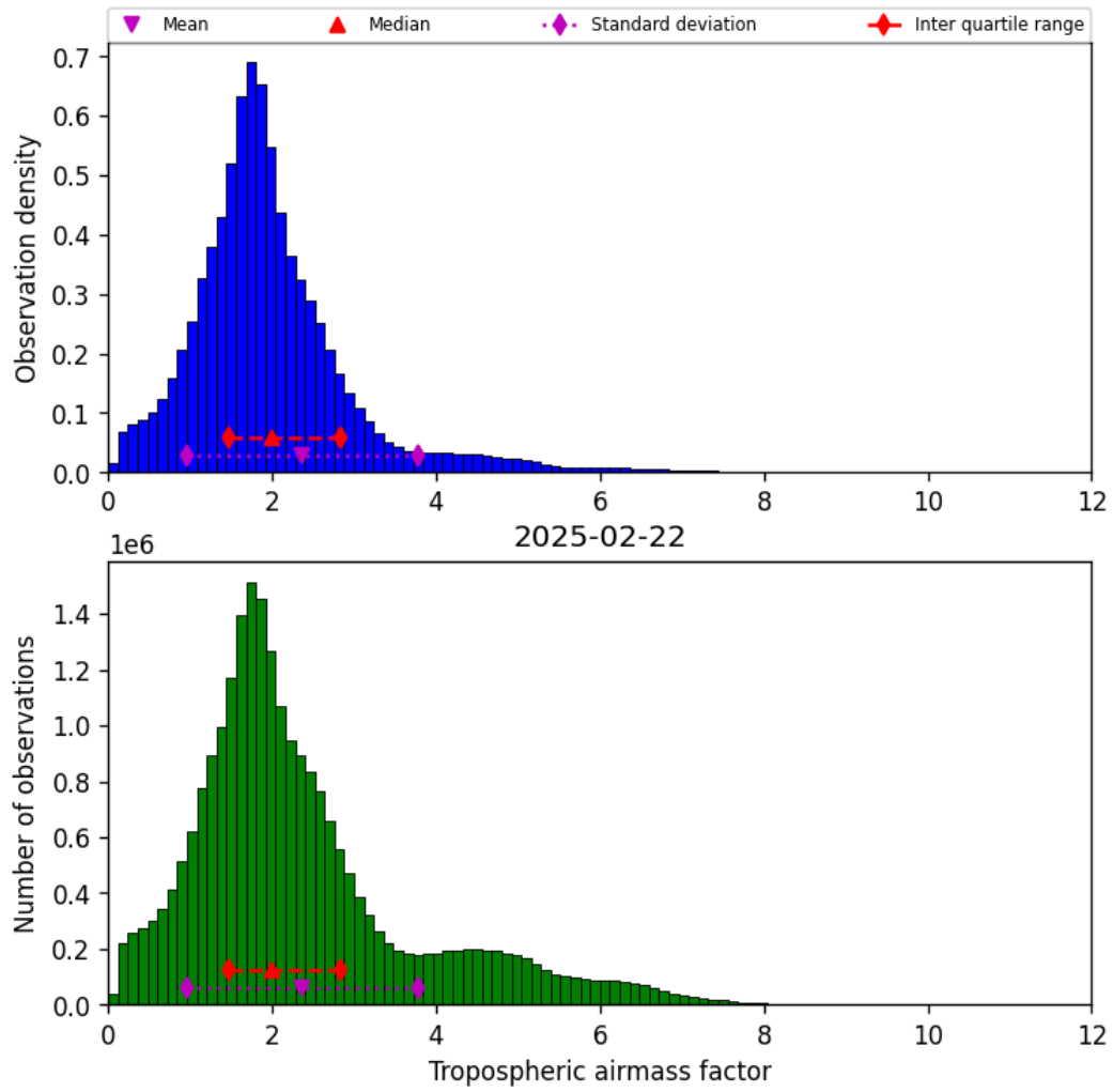
Figure 29: Histogram of “Tropospheric airmass factor” for 2025-02-22 to 2025-02-22
