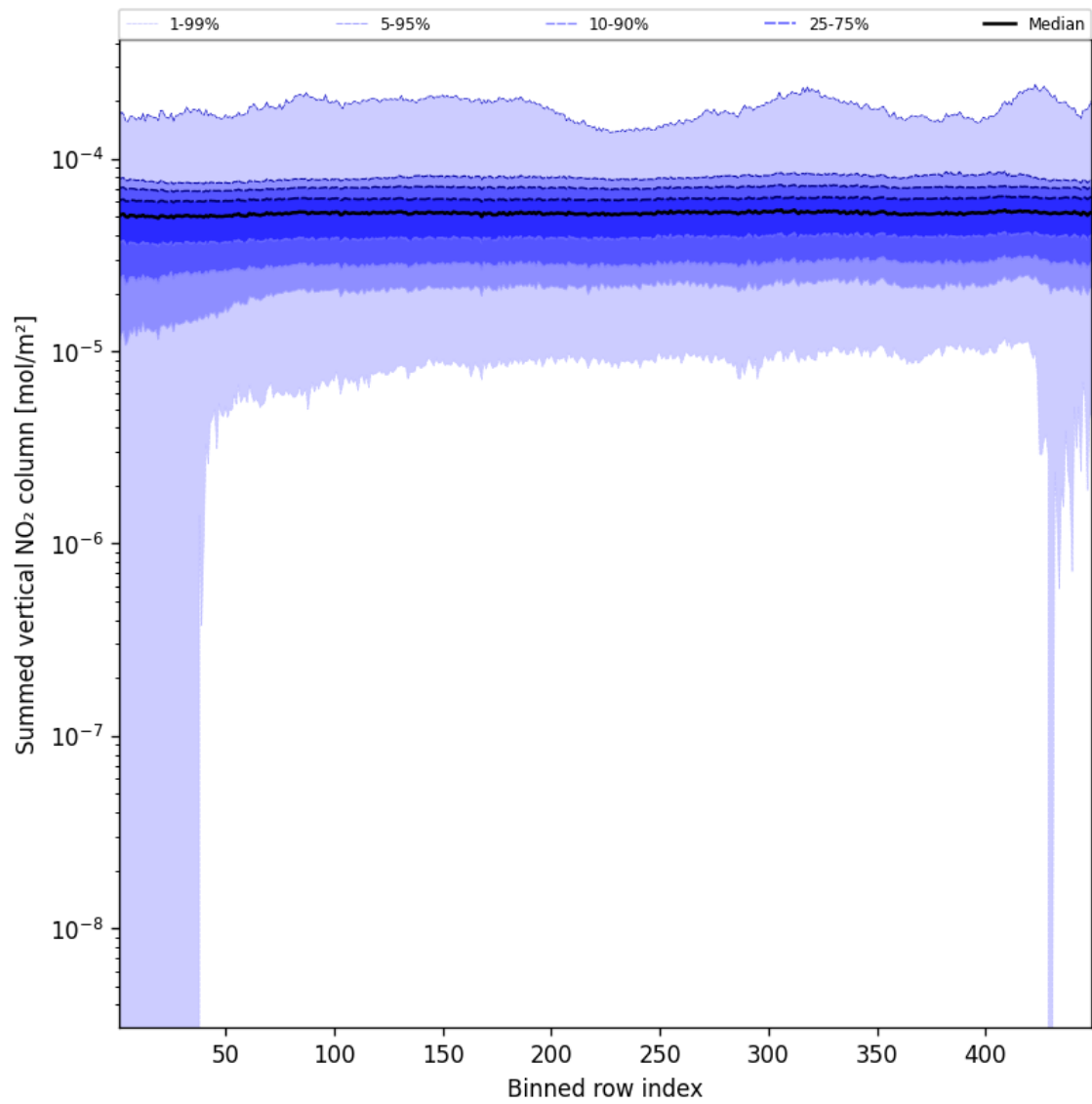
Figure 55: Along track statistics of “Summed vertical NO 2 column” for 2025-02-22 to 2025-02-22
