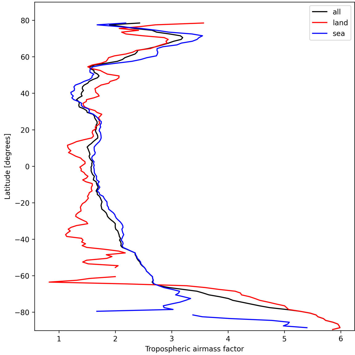
Figure 12: Zonal average of “Tropospheric airmass factor” for 2025-02-22 to 2025-02-22.
