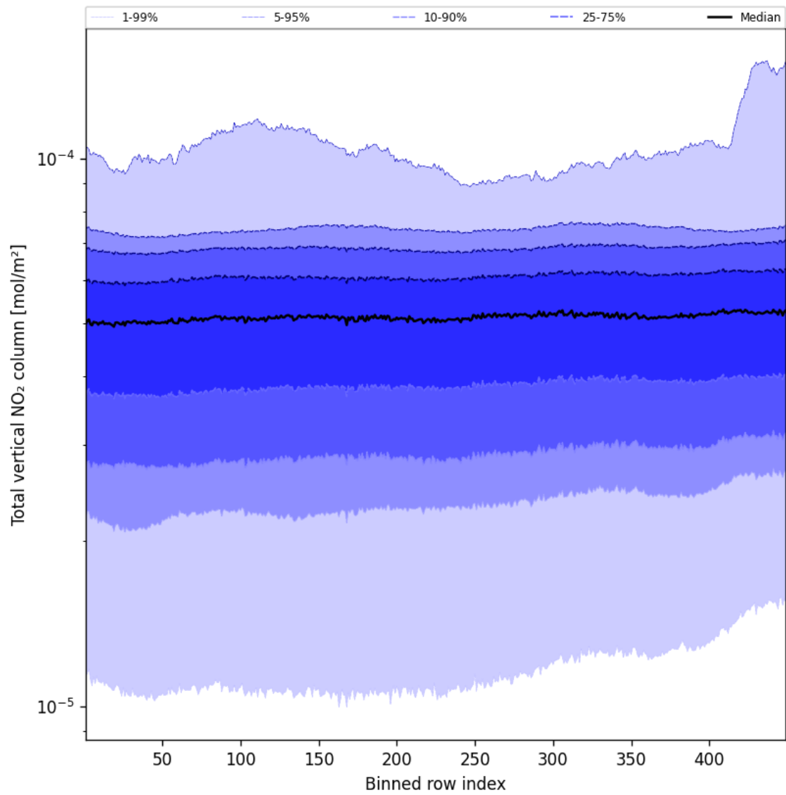
Figure 53: Along track statistics of “Total vertical NO 2 column” for 2025-02-22 to 2025-02-22
