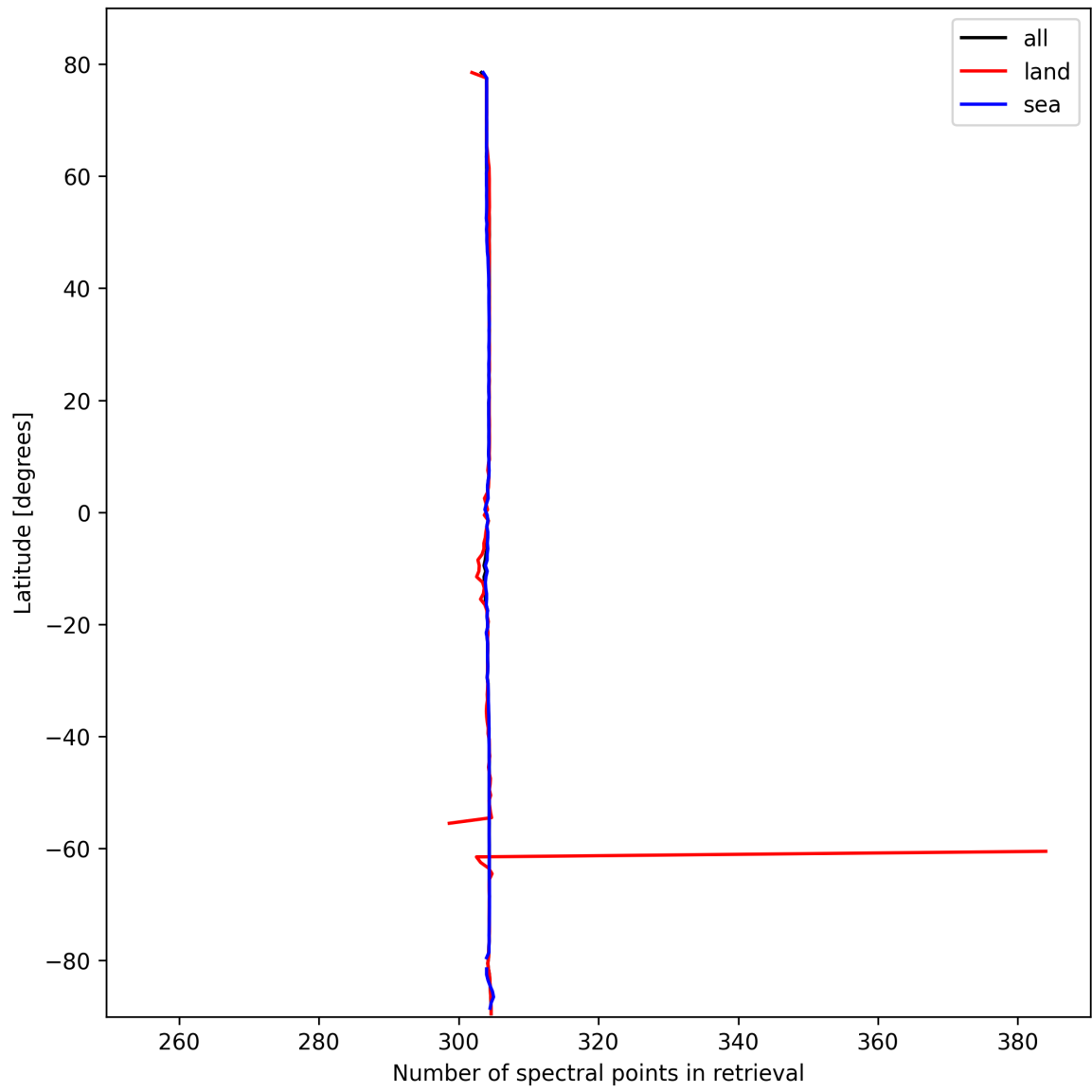
Figure 14: Zonal average of “Number of spectral points in retrieval” for 2025-02-22 to 2025-02-22.
