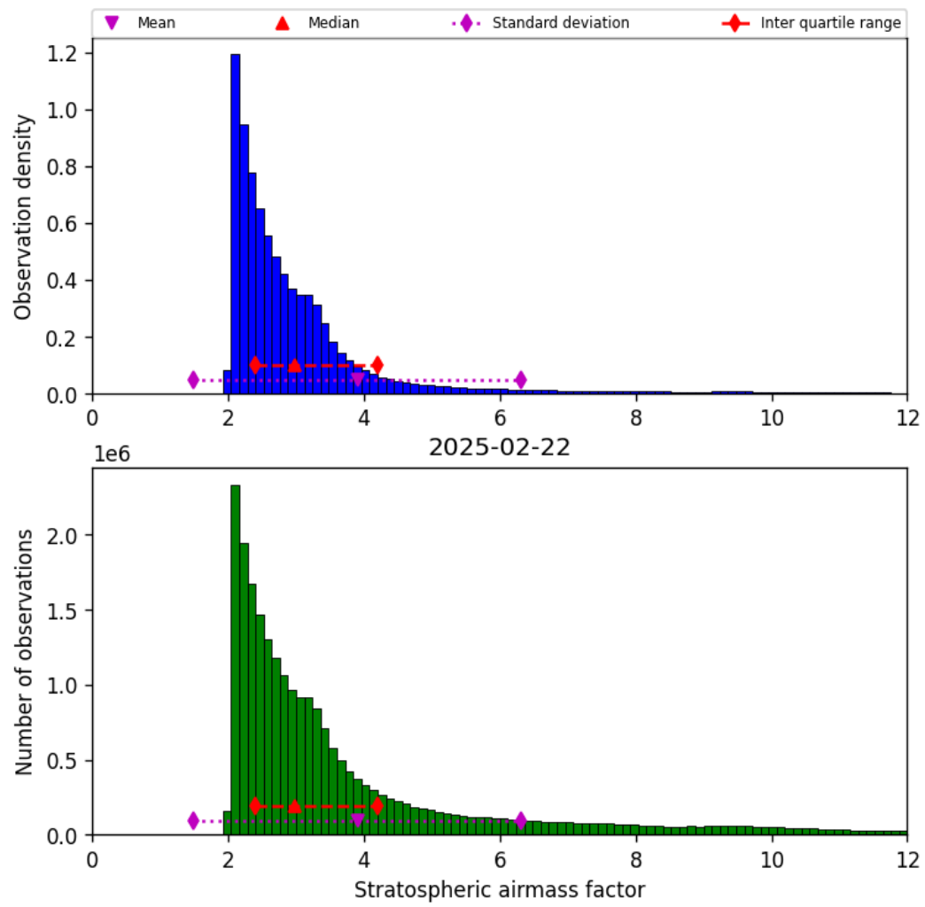
Figure 42: Histogram of “Stratospheric airmass factor” for 2025-02-22 to 2025-02-22
