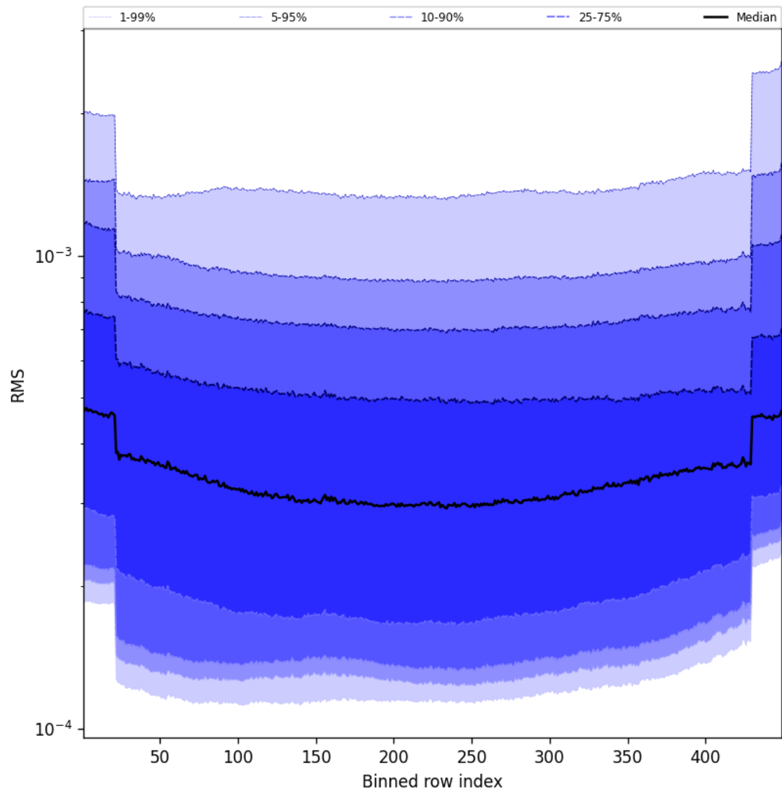
Figure 58: Along track statistics of “RMS” for 2025-02-22 to 2025-02-22
