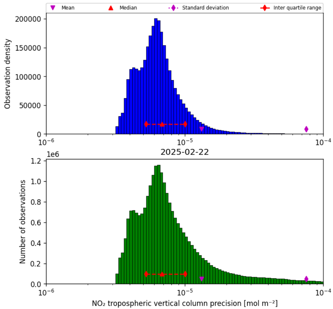
Figure 28: Histogram of “NO 2 tropospheric vertical column precision” for 2025-02-22 to 2025-02-22
