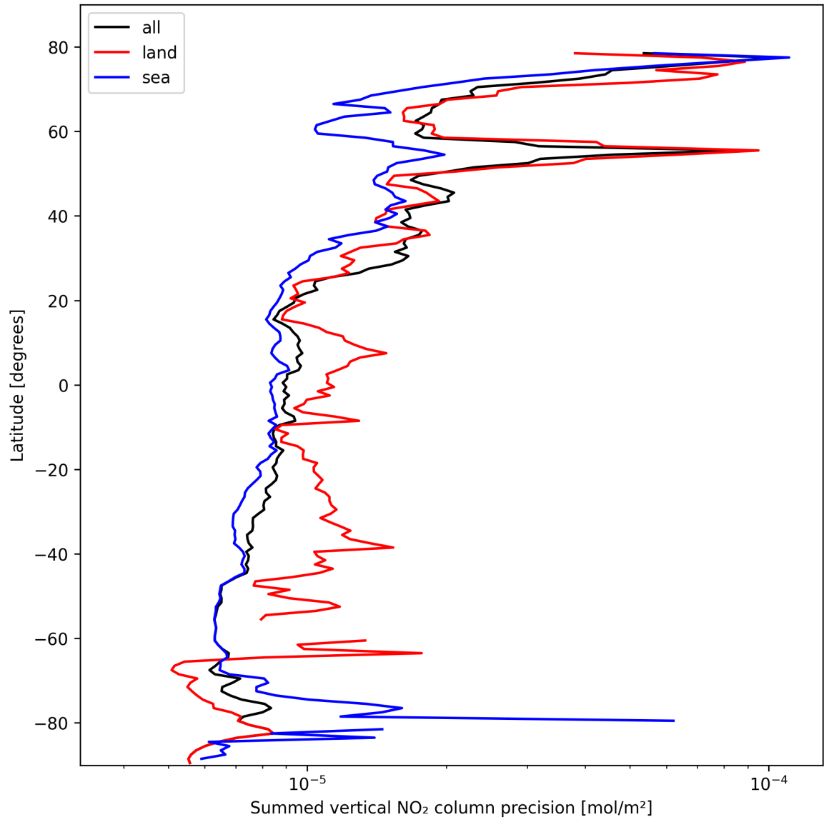
Figure 22: Zonal average of “Summed vertical NO 2 column precision” for 2025-02-22 to 2025-02-22.
