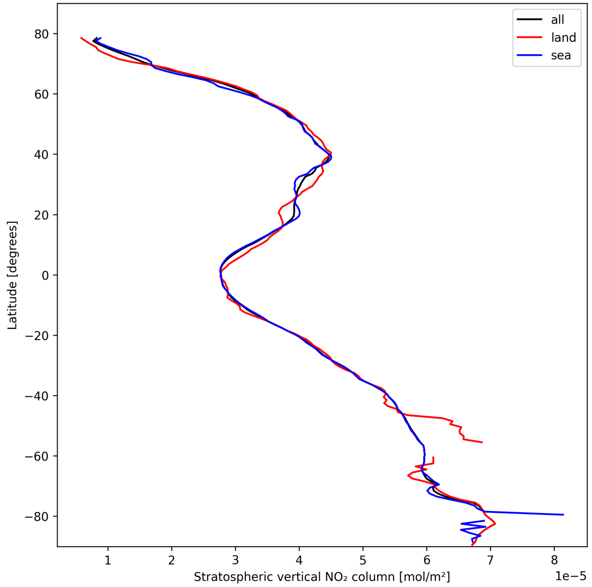
Figure 17: Zonal average of “Stratospheric vertical NO 2 column” for 2025-02-22 to 2025-02-22.
