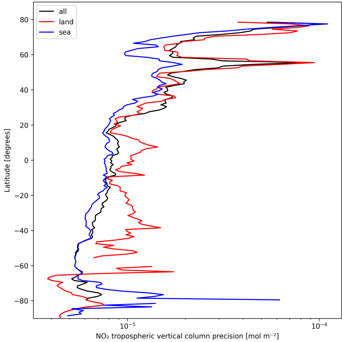
Figure 11: Zonal average of “NO 2 tropospheric vertical column precision” for 2025-02-22 to 2025-02-22.
