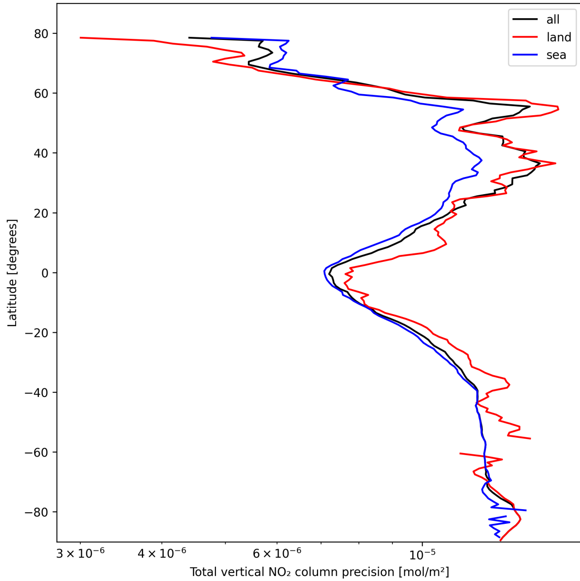
Figure 20: Zonal average of “Total vertical NO 2 column precision” for 2025-02-22 to 2025-02-22.
