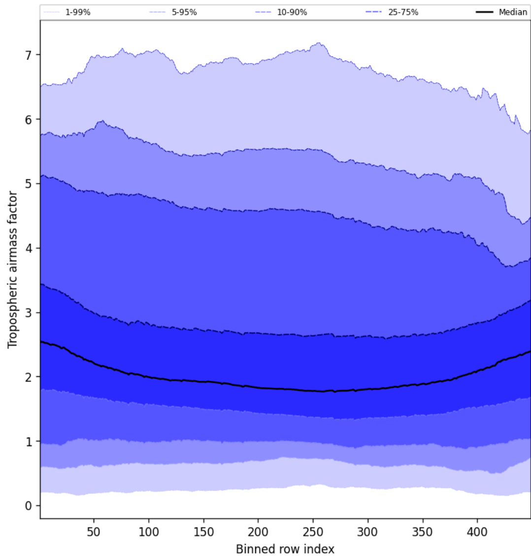
Figure 46: Along track statistics of “Tropospheric airmass factor” for 2025-02-22 to 2025-02-22
