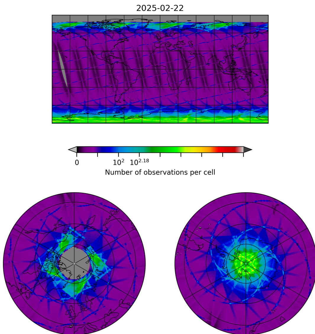
Figure 8: Map of the number of observations for 2025-02-22 to 2025-02-22
