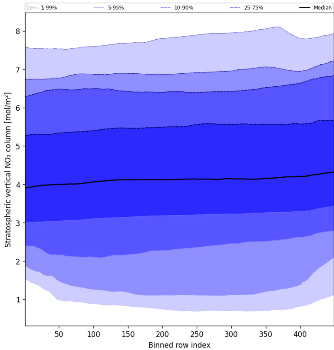
Figure 51: Along track statistics of “Stratospheric vertical NO 2 column” for 2025-02-22 to 2025-02-22
