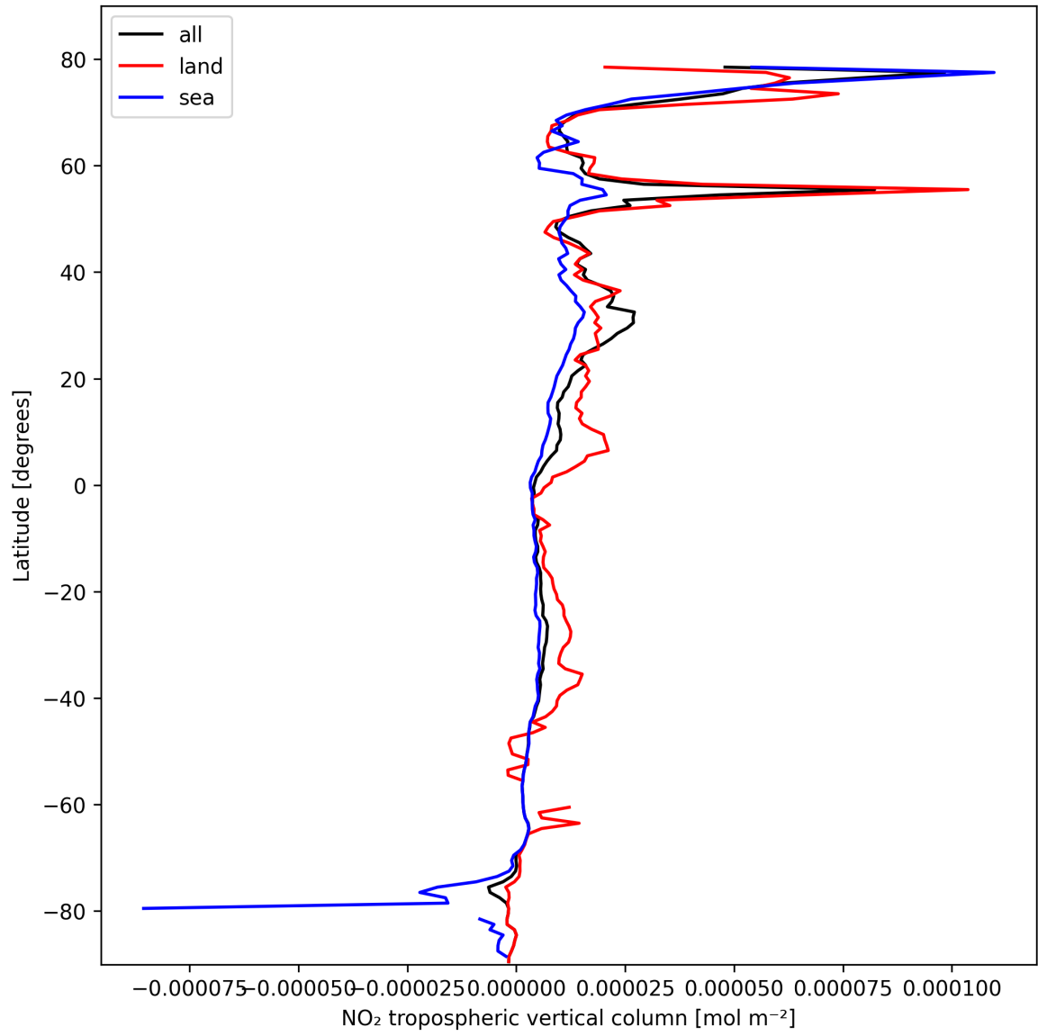
Figure 10: Zonal average of “NO 2 tropospheric vertical column” for 2025-02-22 to 2025-02-22.
