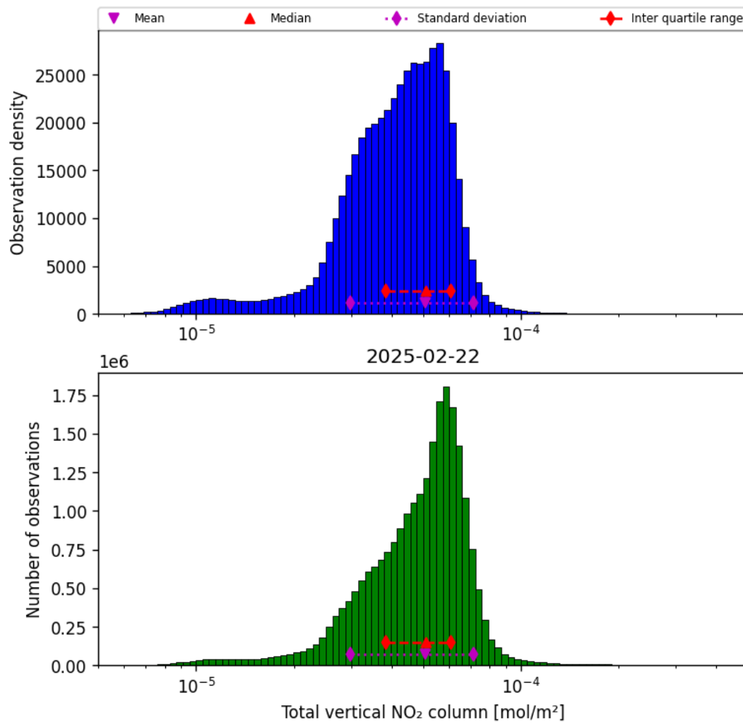
Figure 36: Histogram of "Total vertical NO 2 column" for 2025-02-22 to 2025-02-22
