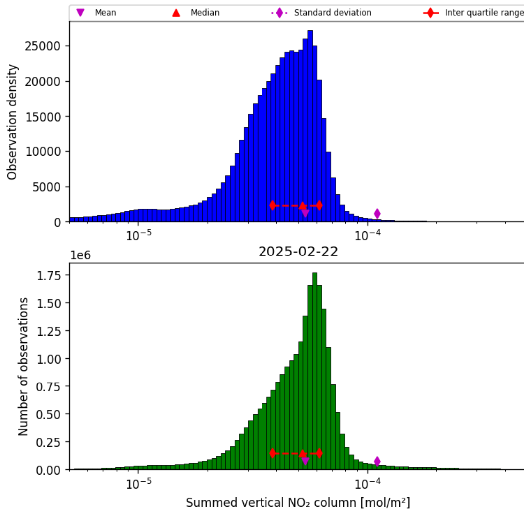
Figure 38: Histogram of “Summed vertical NO 2 column” for 2025-02-22 to 2025-02-22
