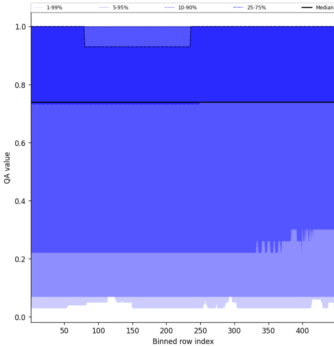
Figure 43: Along track statistics of “QA value” for 2025-02-23 to 2025-02-24
