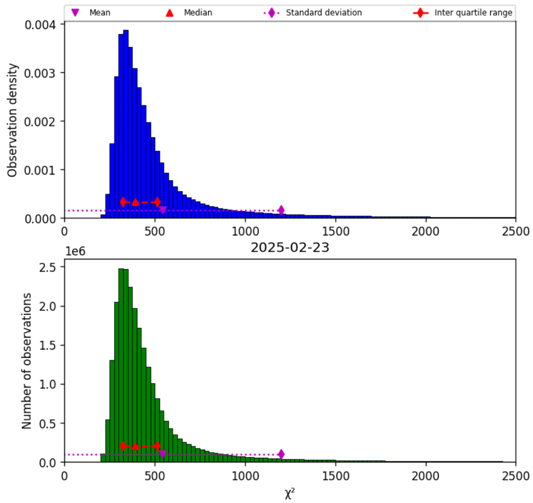
Figure 40: Histogram of “ \chi^2 ” for 2025-02-23 to 2025-02-24
