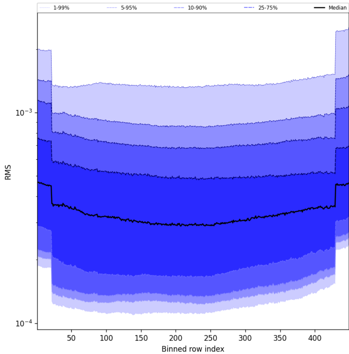
Figure 58: Along track statistics of “RMS” for 2025-02-23 to 2025-02-24
