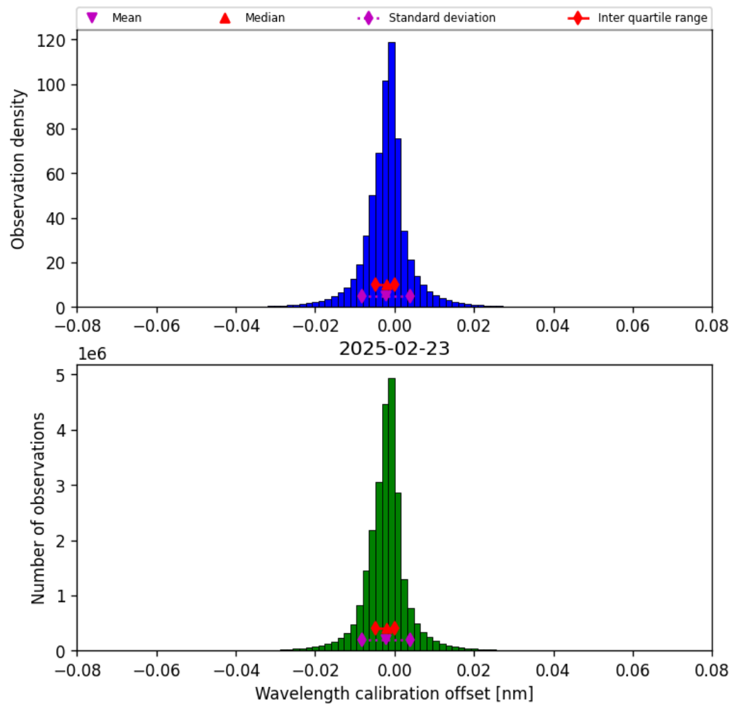
Figure 33: Histogram of “Wavelength calibration offset” for 2025-02-23 to 2025-02-24
