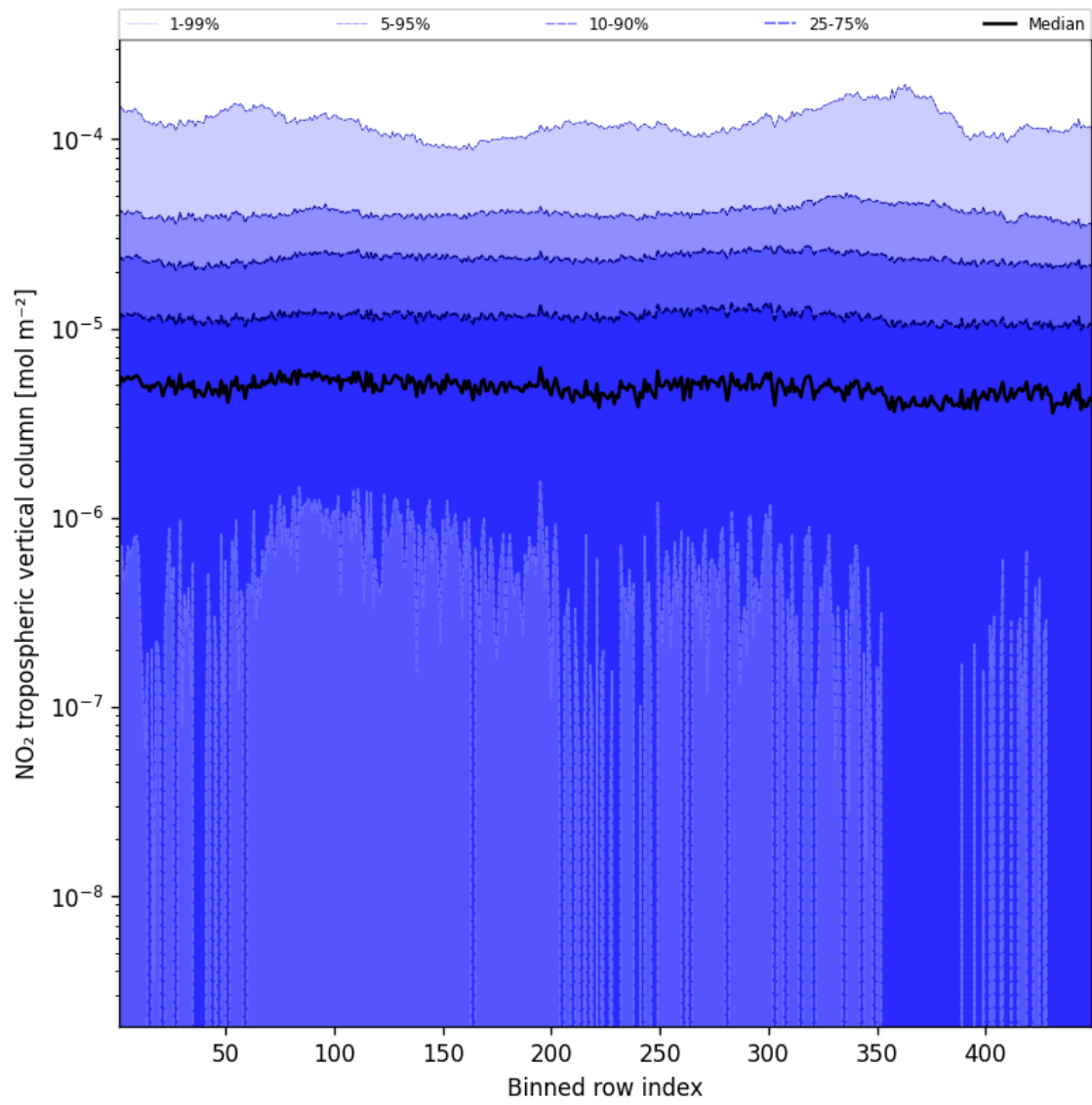
Figure 44: Along track statistics of “NO 2 tropospheric vertical column” for 2025-02-23 to 2025-02-24
