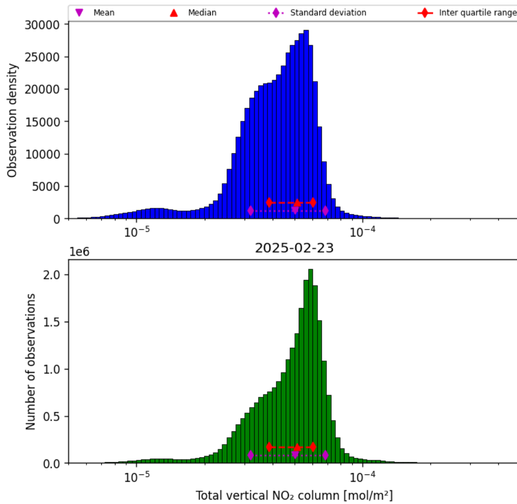
Figure 36: Histogram of "Total vertical NO 2 column" for 2025-02-23 to 2025-02-24
