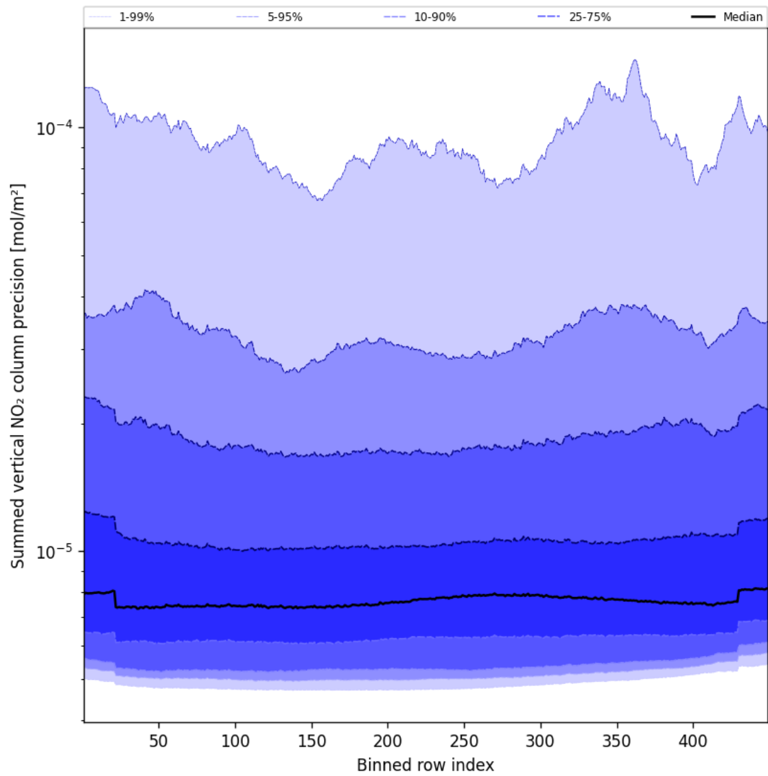
Figure 56: Along track statistics of “Summed vertical NO 2 column precision” for 2025-02-23 to 2025-02-24
