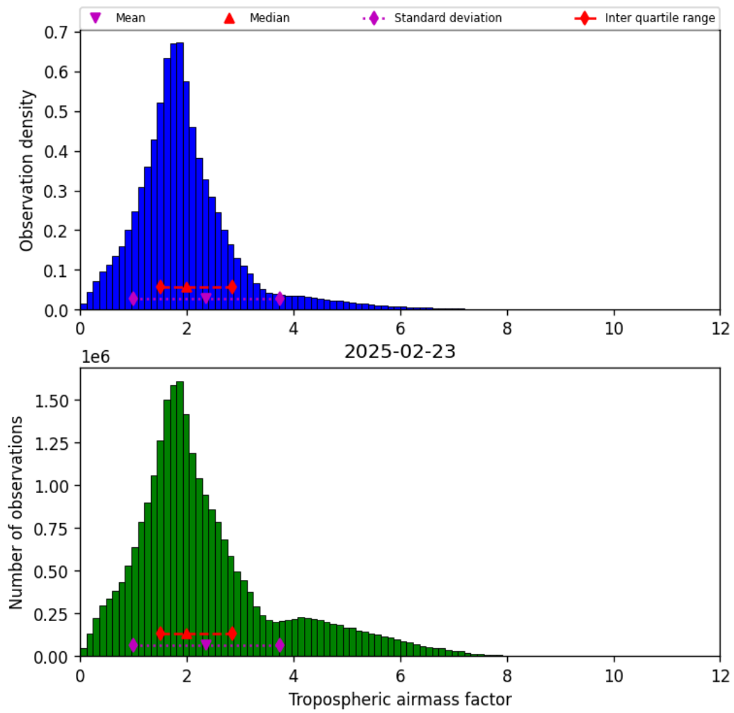
Figure 29: Histogram of “Tropospheric airmass factor” for 2025-02-23 to 2025-02-24
