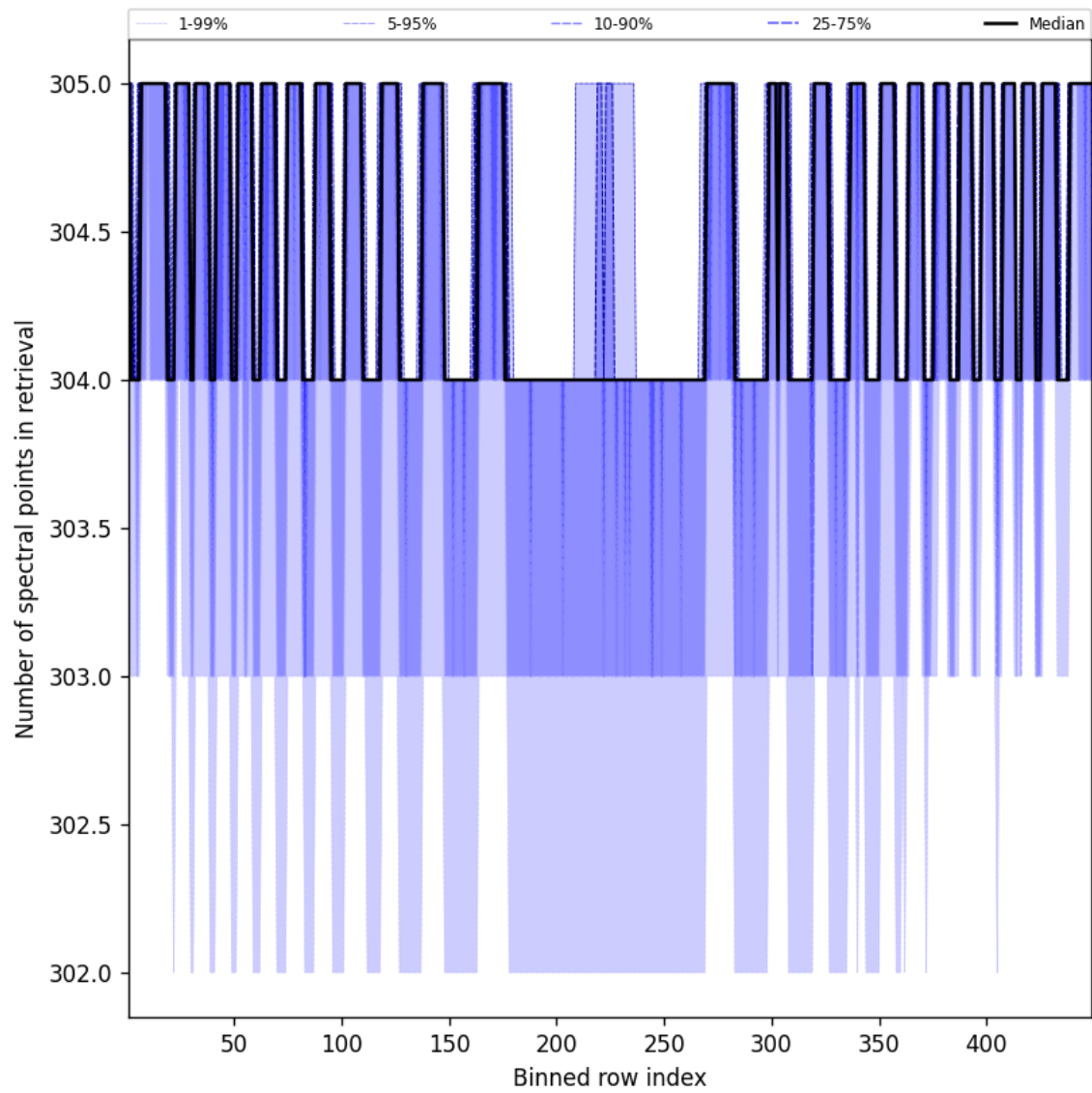
Figure 48: Along track statistics of “Number of spectral points in retrieval” for 2025-02-23 to 2025-02-24
