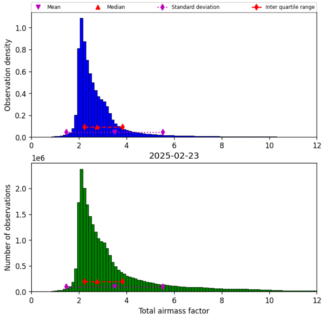
Figure 30: Histogram of “Total airmass factor” for 2025-02-23 to 2025-02-24
