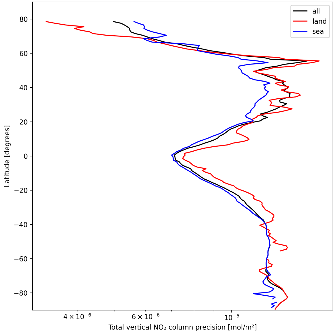
Figure 20: Zonal average of “Total vertical NO 2 column precision” for 2025-02-23 to 2025-02-24.
