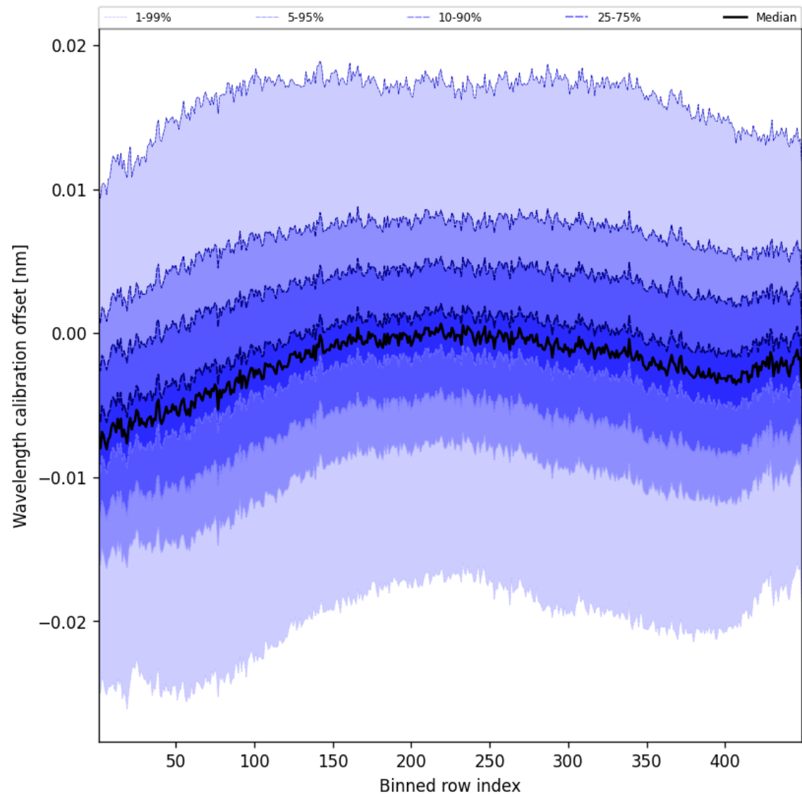
Figure 50: Along track statistics of “Wavelength calibration offset” for 2025-02-23 to 2025-02-24
