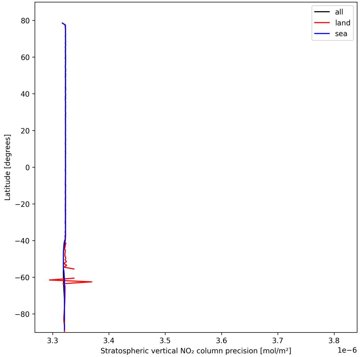
Figure 18: Zonal average of “Stratospheric vertical NO 2 column precision” for 2025-02-23 to 2025-02-24.
