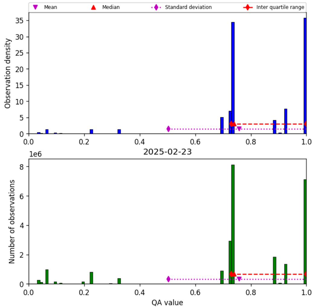
Figure 26: Histogram of “QA value” for 2025-02-23 to 2025-02-24
