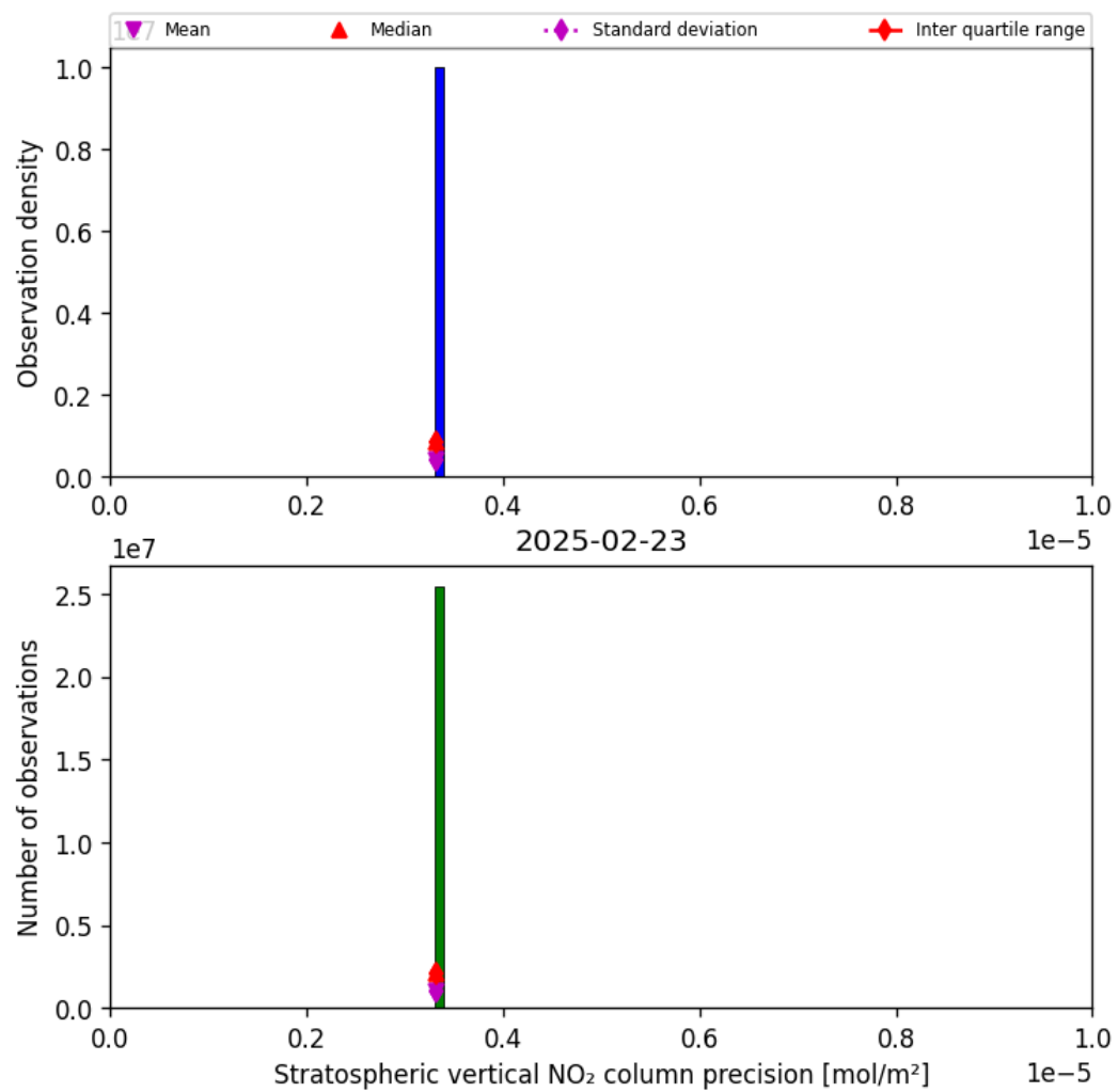
Figure 35: Histogram of “Stratospheric vertical NO 2 column precision” for 2025-02-23 to 2025-02-24
