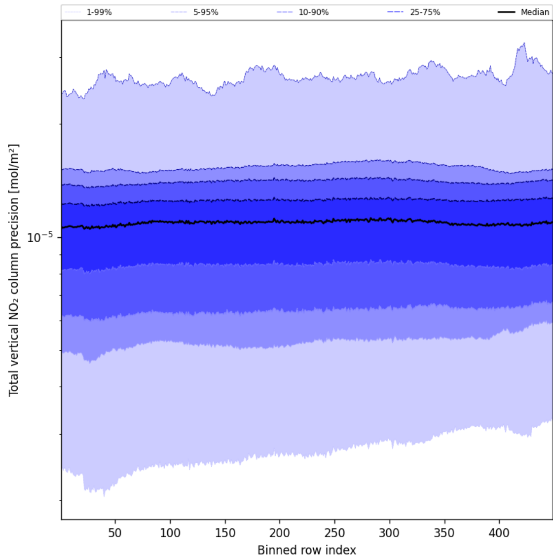
Figure 54: Along track statistics of “Total vertical NO 2 column precision” for 2025-02-23 to 2025-02-24
