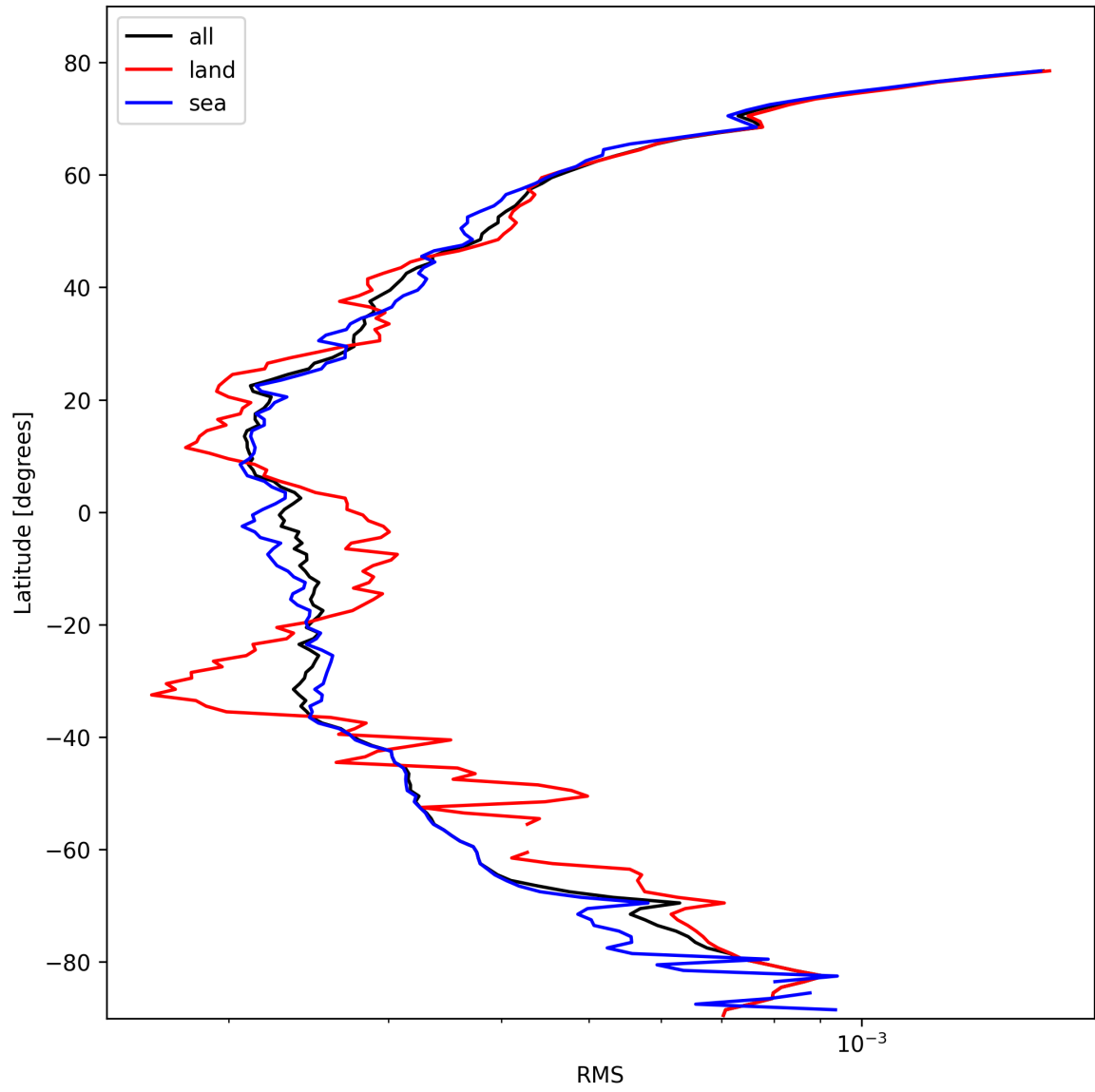
Figure 24: Zonal average of “RMS” for 2025-02-23 to 2025-02-24.
