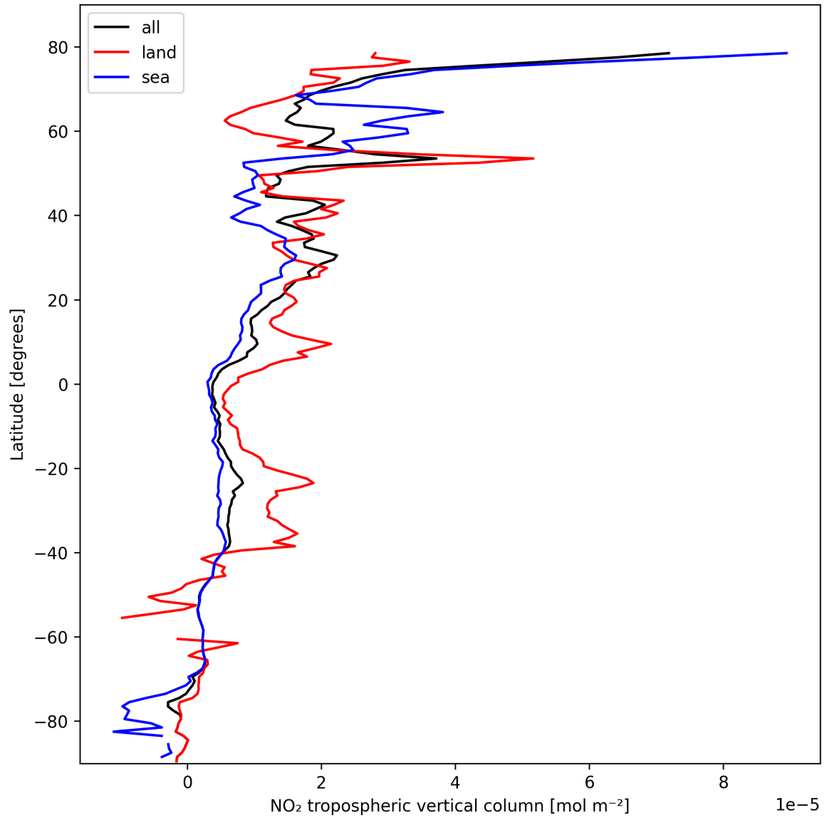
Figure 10: Zonal average of “NO 2 tropospheric vertical column” for 2025-02-23 to 2025-02-24.
