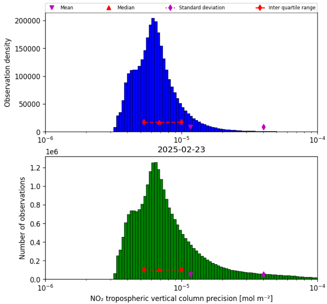
Figure 28: Histogram of “NO 2 tropospheric vertical column precision” for 2025-02-23 to 2025-02-24
