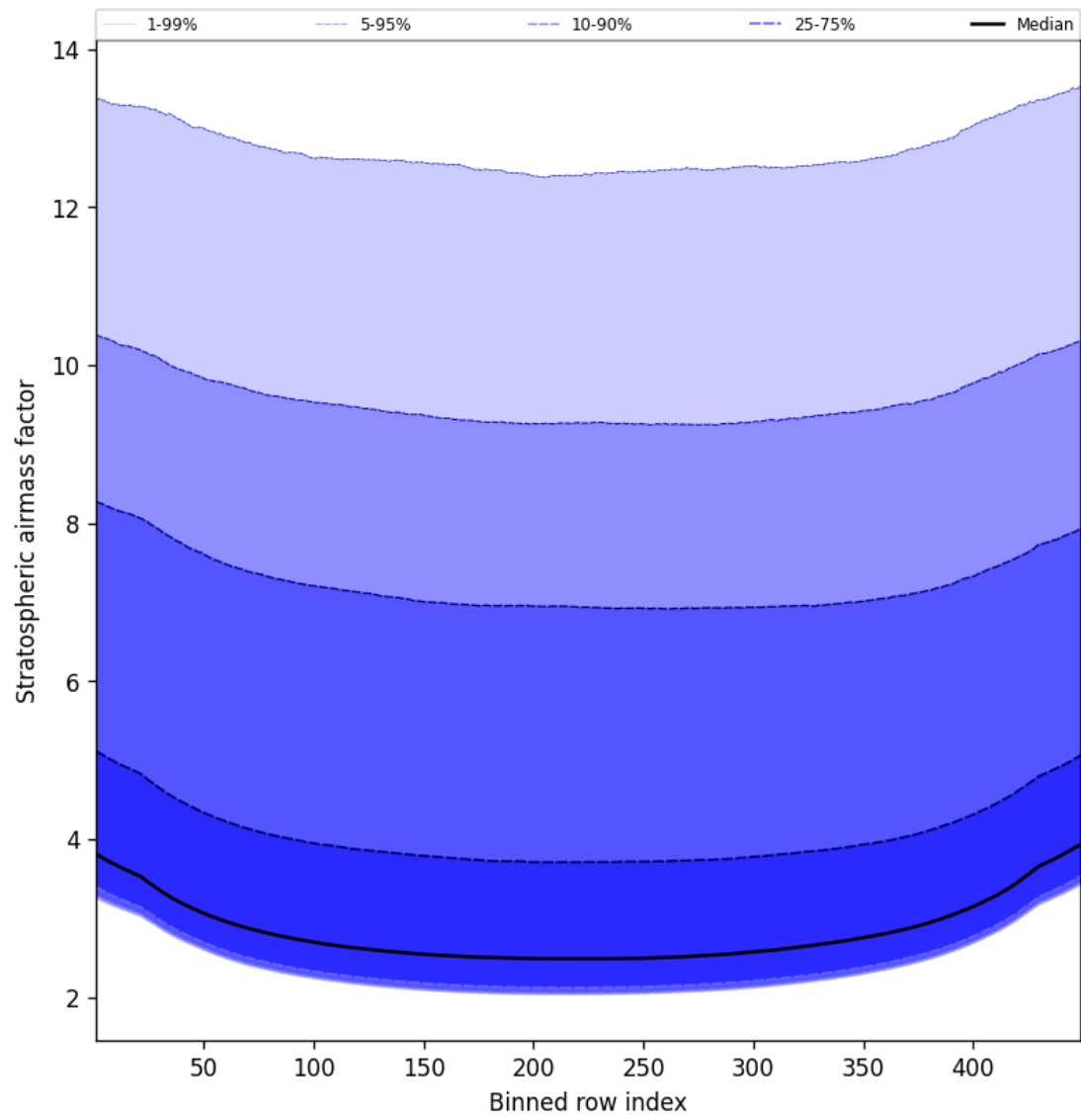
Figure 59: Along track statistics of “Stratospheric airmass factor” for 2025-02-23 to 2025-02-24
