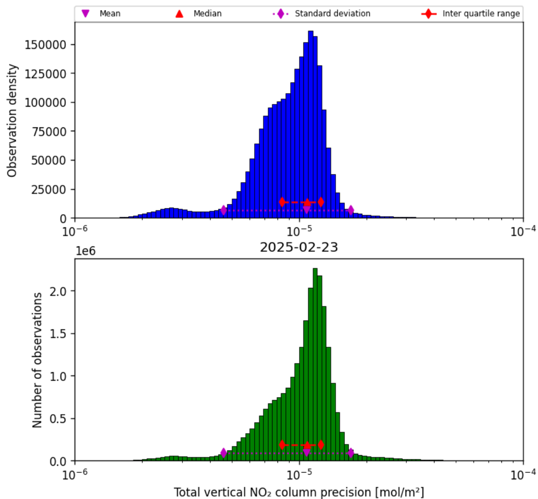
Figure 37: Histogram of “Total vertical NO 2 column precision” for 2025-02-23 to 2025-02-24
