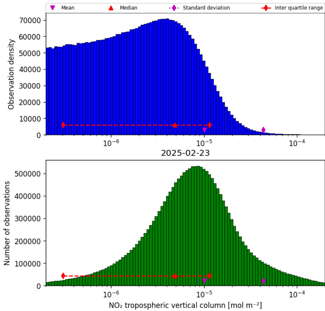
Figure 27: Histogram of “NO 2 tropospheric vertical column” for 2025-02-23 to 2025-02-24
