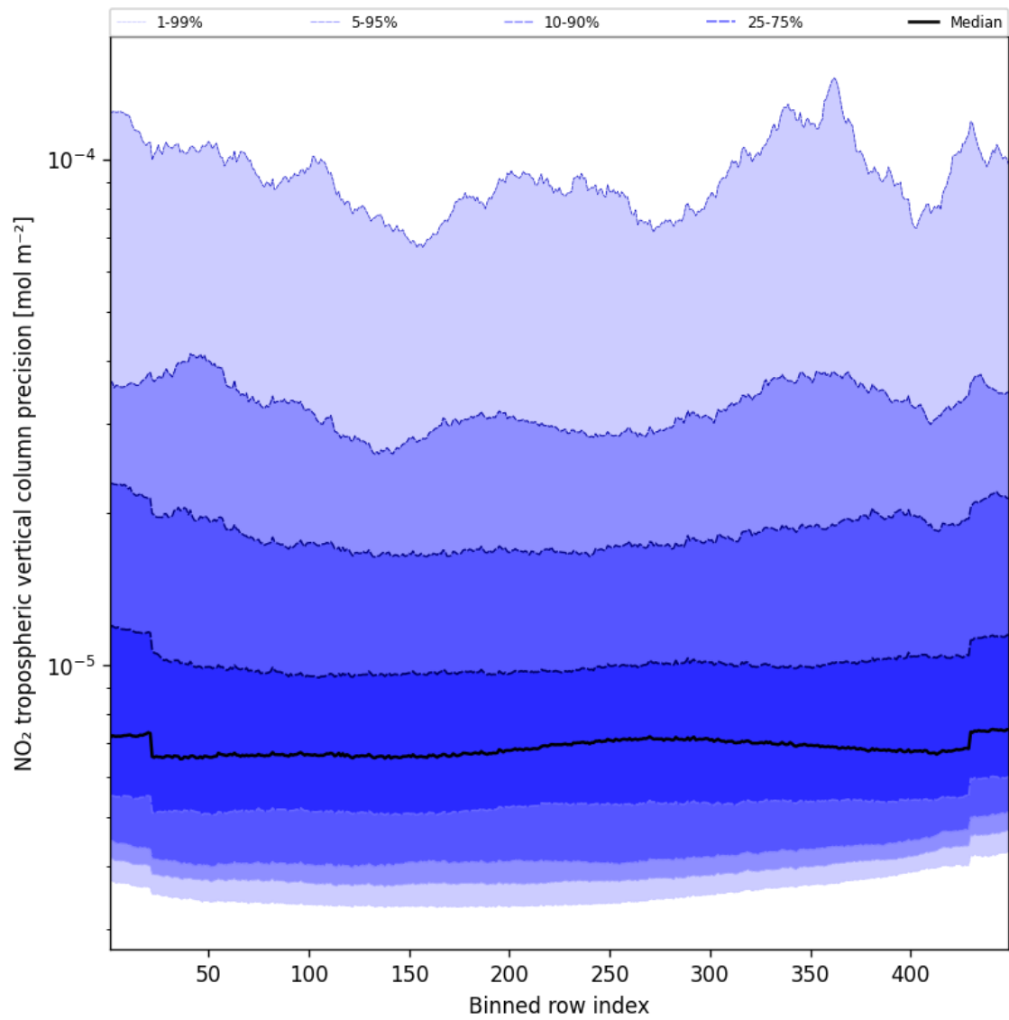
Figure 45: Along track statistics of “NO 2 tropospheric vertical column precision” for 2025-02-23 to 2025-02-24
