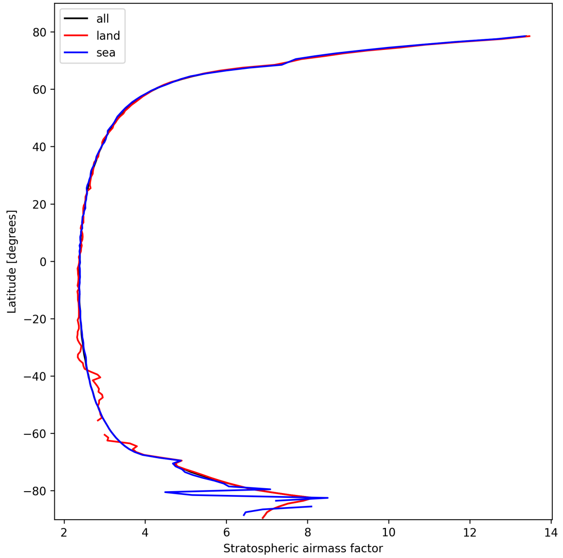
Figure 25: Zonal average of “Stratospheric airmass factor” for 2025-02-23 to 2025-02-24.
