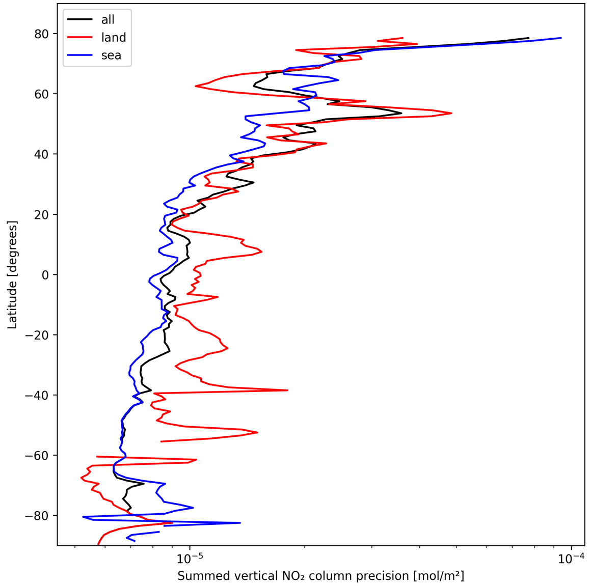
Figure 22: Zonal average of “Summed vertical NO 2 column precision” for 2025-02-23 to 2025-02-24.
