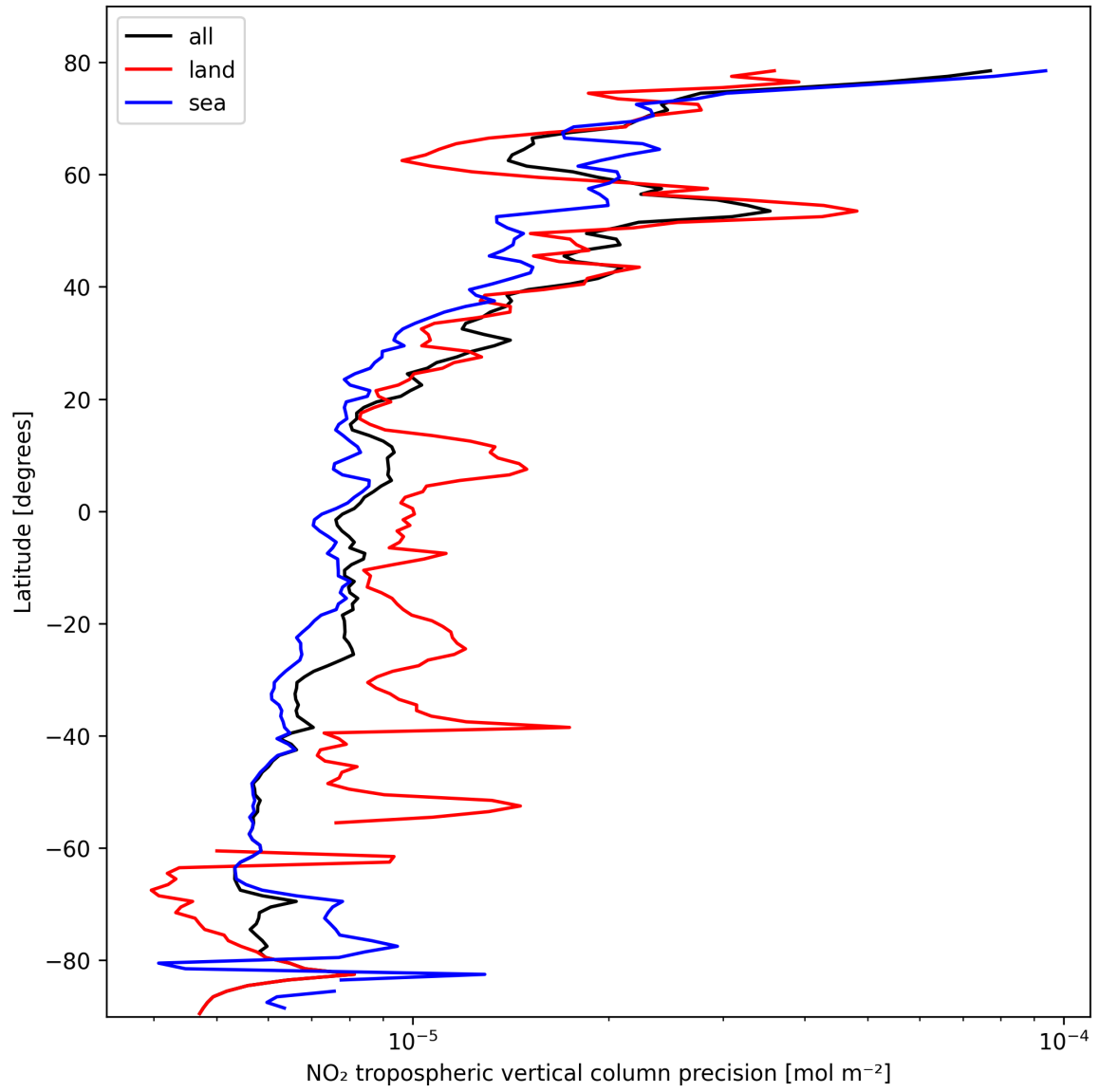
Figure 11: Zonal average of “NO 2 tropospheric vertical column precision” for 2025-02-23 to 2025-02-24.
