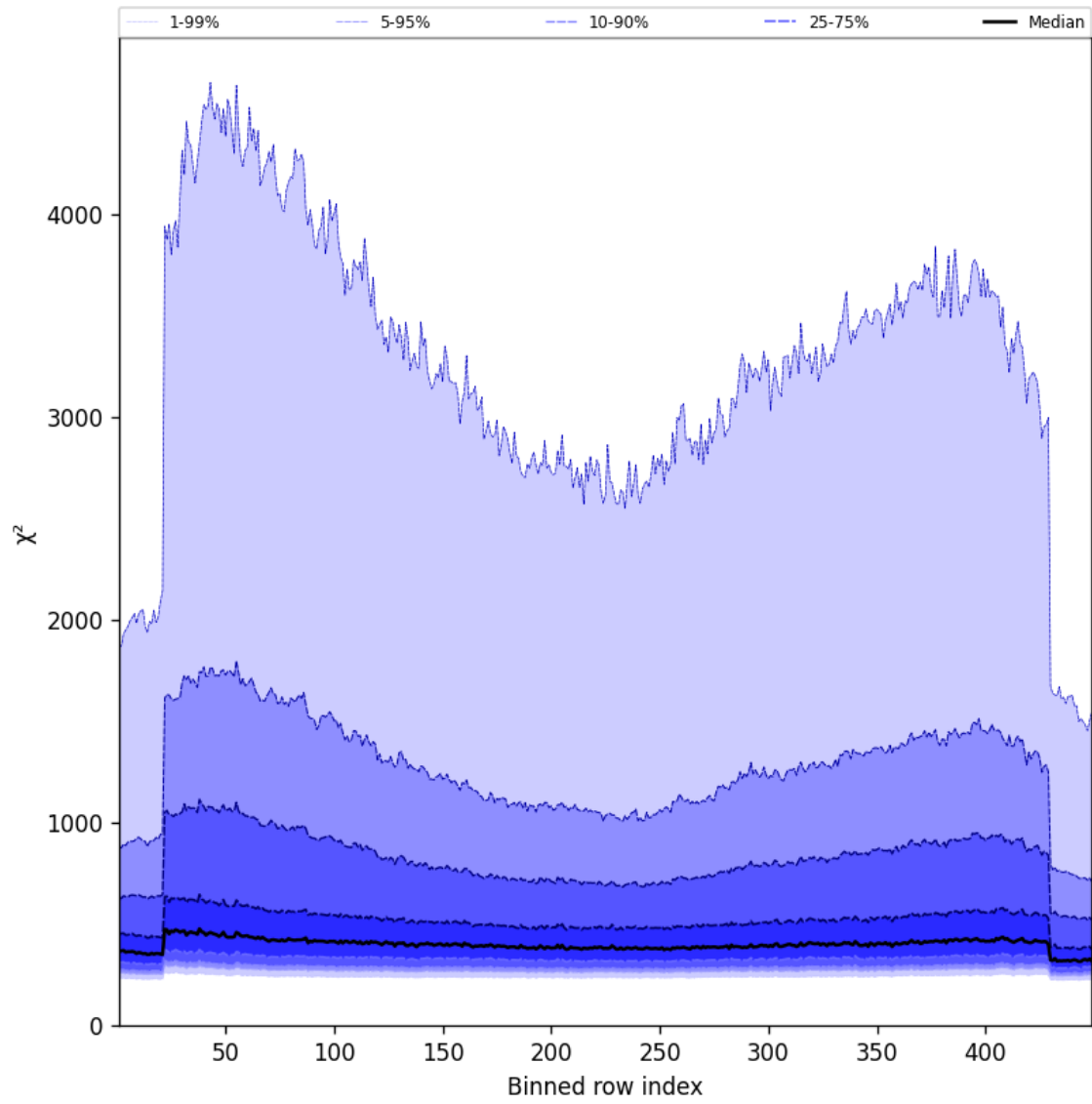
Figure 57: Along track statistics of “ \chi^2 ” for 2025-02-23 to 2025-02-24
