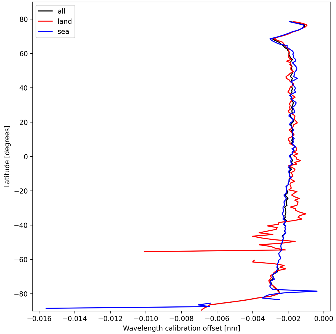
Figure 16: Zonal average of “Wavelength calibration offset” for 2025-02-23 to 2025-02-24.
