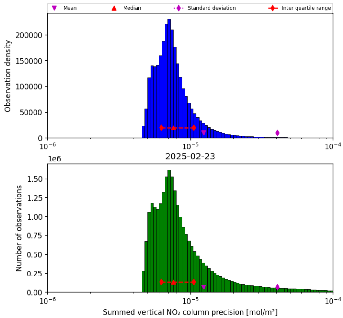
Figure 39: Histogram of “Summed vertical NO 2 column precision” for 2025-02-23 to 2025-02-24
