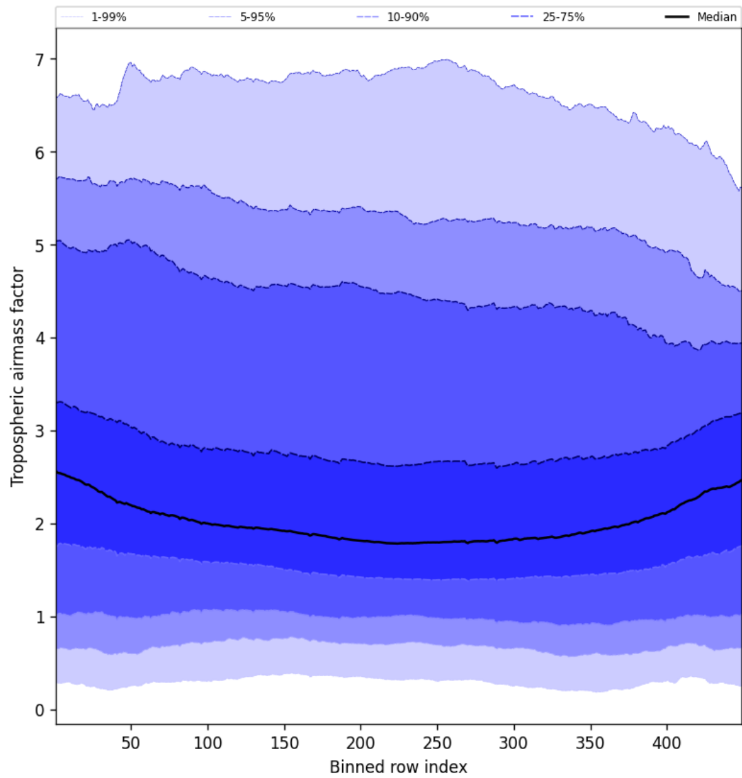
Figure 46: Along track statistics of “Tropospheric airmass factor” for 2025-02-23 to 2025-02-24
