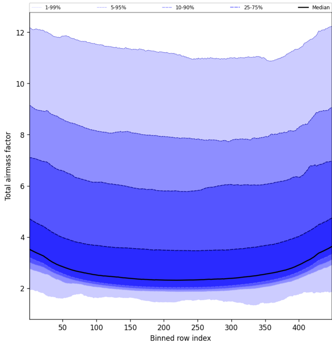
Figure 47: Along track statistics of “Total airmass factor” for 2025-02-23 to 2025-02-24
