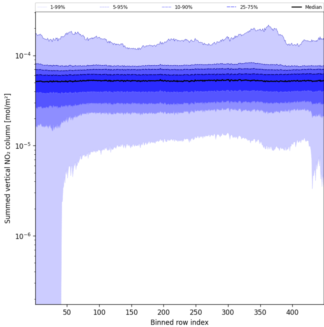
Figure 55: Along track statistics of “Summed vertical NO 2 column” for 2025-02-23 to 2025-02-24
