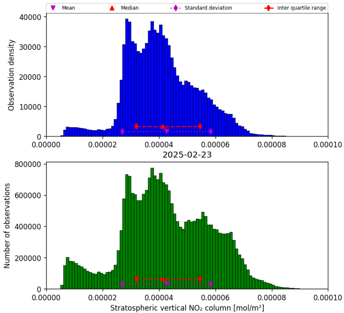
Figure 34: Histogram of “Stratospheric vertical NO 2 column” for 2025-02-23 to 2025-02-24
