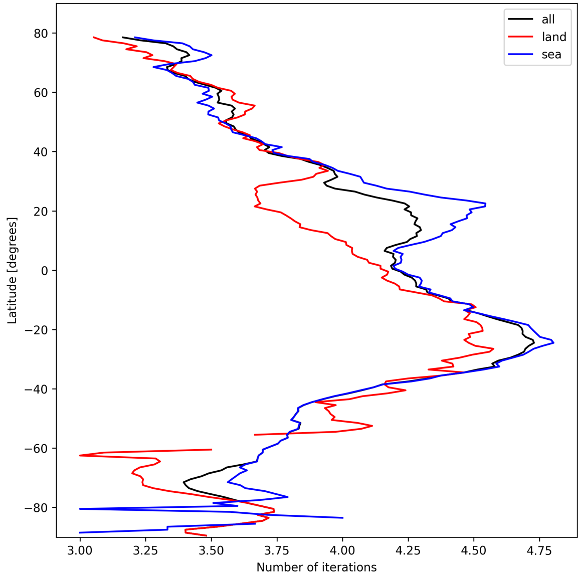
Figure 15: Zonal average of “Number of iterations” for 2025-02-23 to 2025-02-24.
