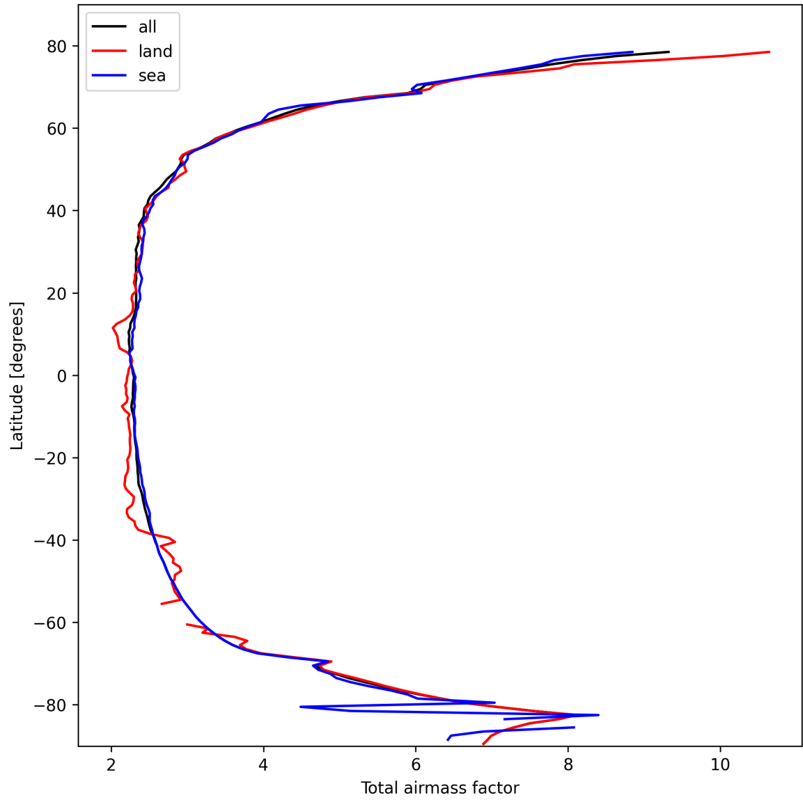
Figure 13: Zonal average of “Total airmass factor” for 2025-02-23 to 2025-02-24.
