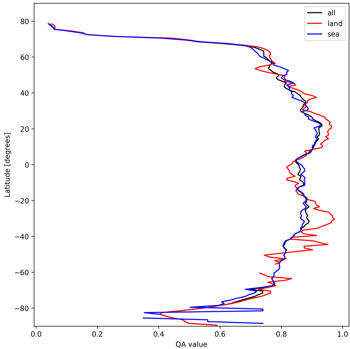
Figure 9: Zonal average of “QA value” for 2025-02-23 to 2025-02-24.
