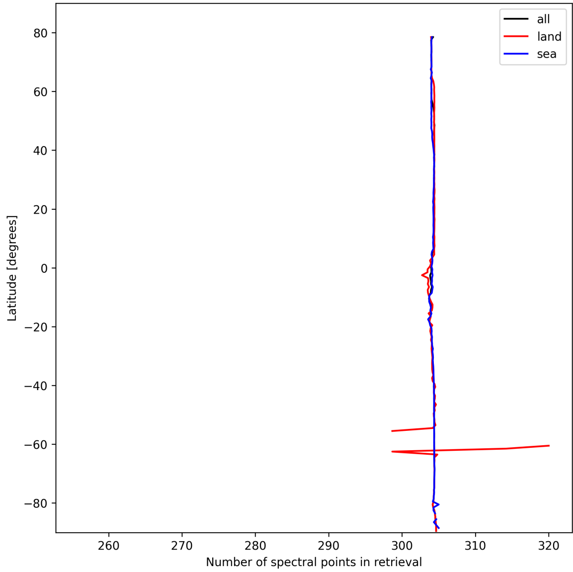
Figure 14: Zonal average of “Number of spectral points in retrieval” for 2025-02-23 to 2025-02-24.
