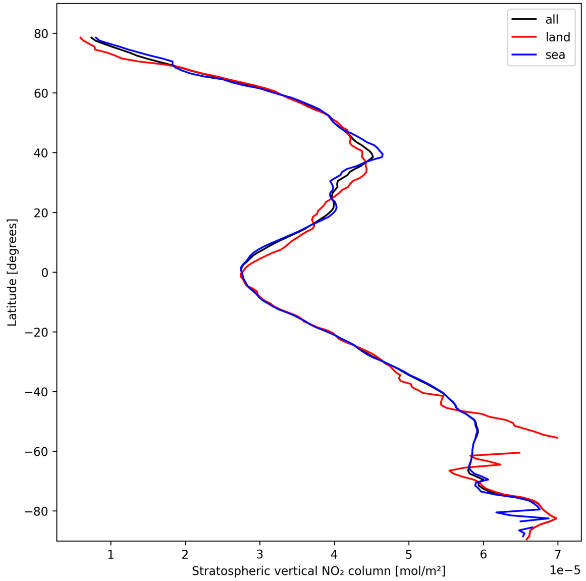
Figure 17: Zonal average of “Stratospheric vertical NO 2 column” for 2025-02-23 to 2025-02-24.
