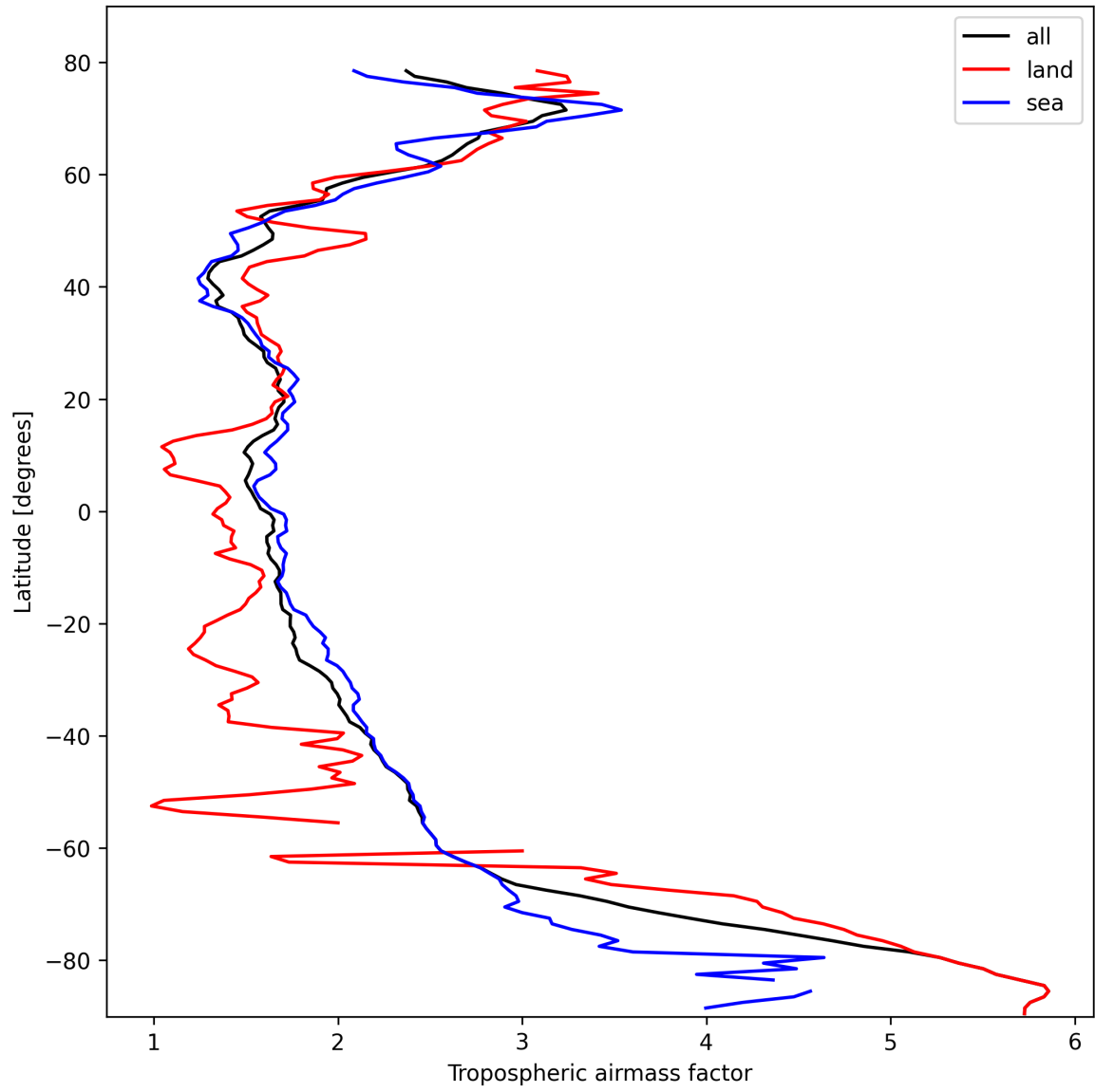
Figure 12: Zonal average of “Tropospheric airmass factor” for 2025-02-23 to 2025-02-24.
