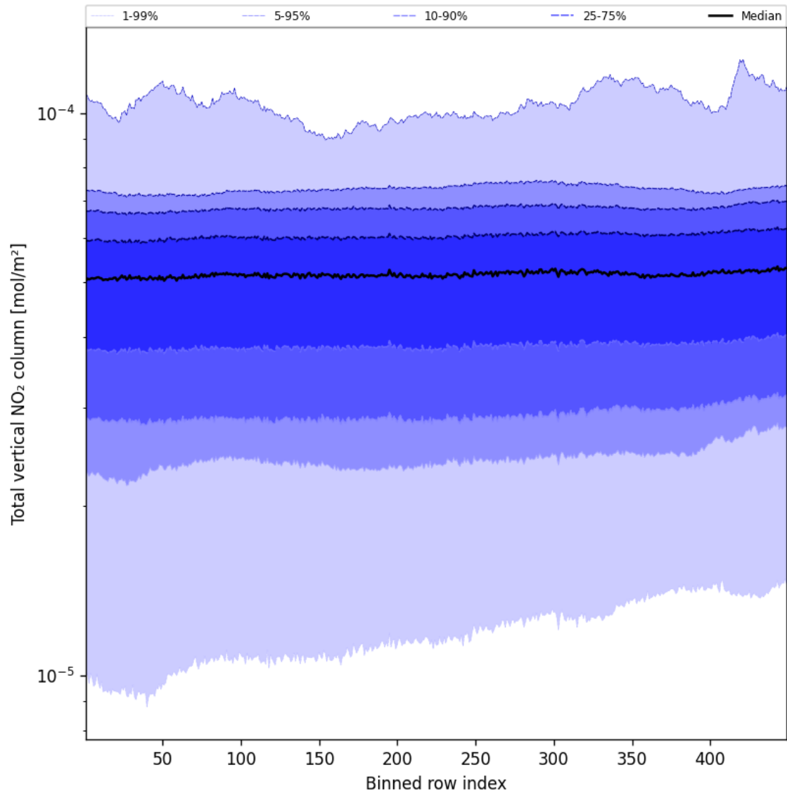
Figure 53: Along track statistics of “Total vertical NO 2 column” for 2025-02-23 to 2025-02-24
