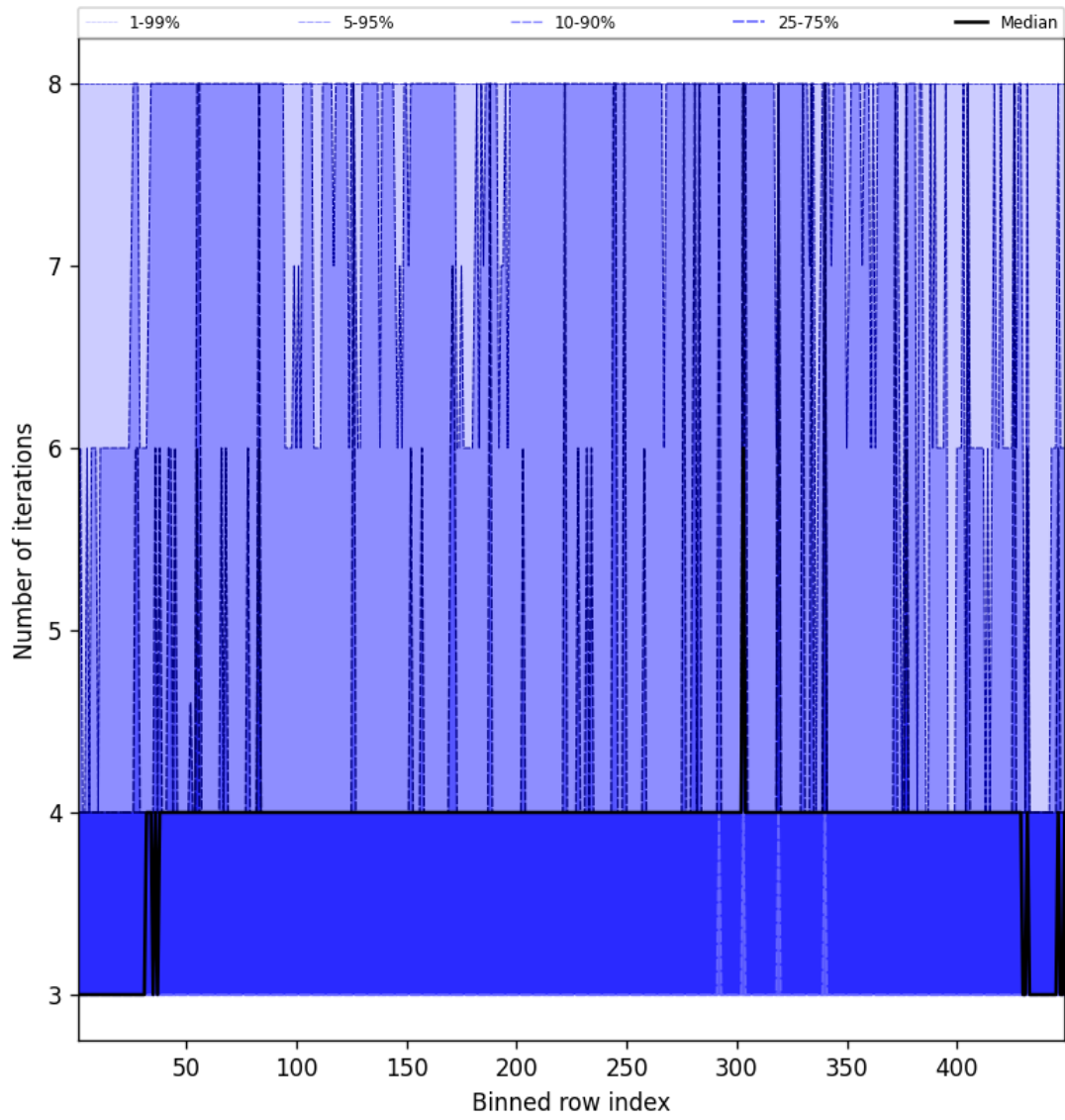
Figure 49: Along track statistics of “Number of iterations” for 2025-02-23 to 2025-02-24
