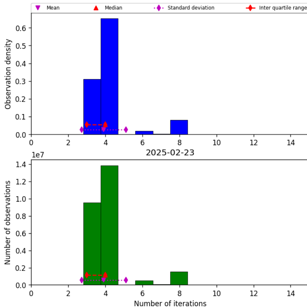
Figure 32: Histogram of “Number of iterations” for 2025-02-23 to 2025-02-24
