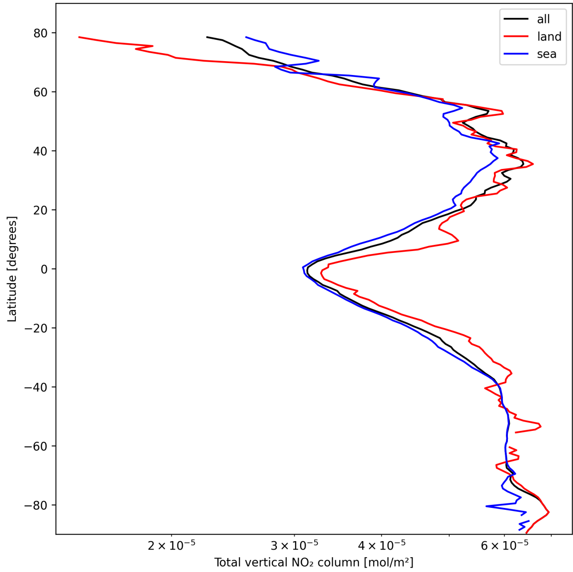
Figure 19: Zonal average of “Total vertical NO 2 column” for 2025-02-23 to 2025-02-24.
