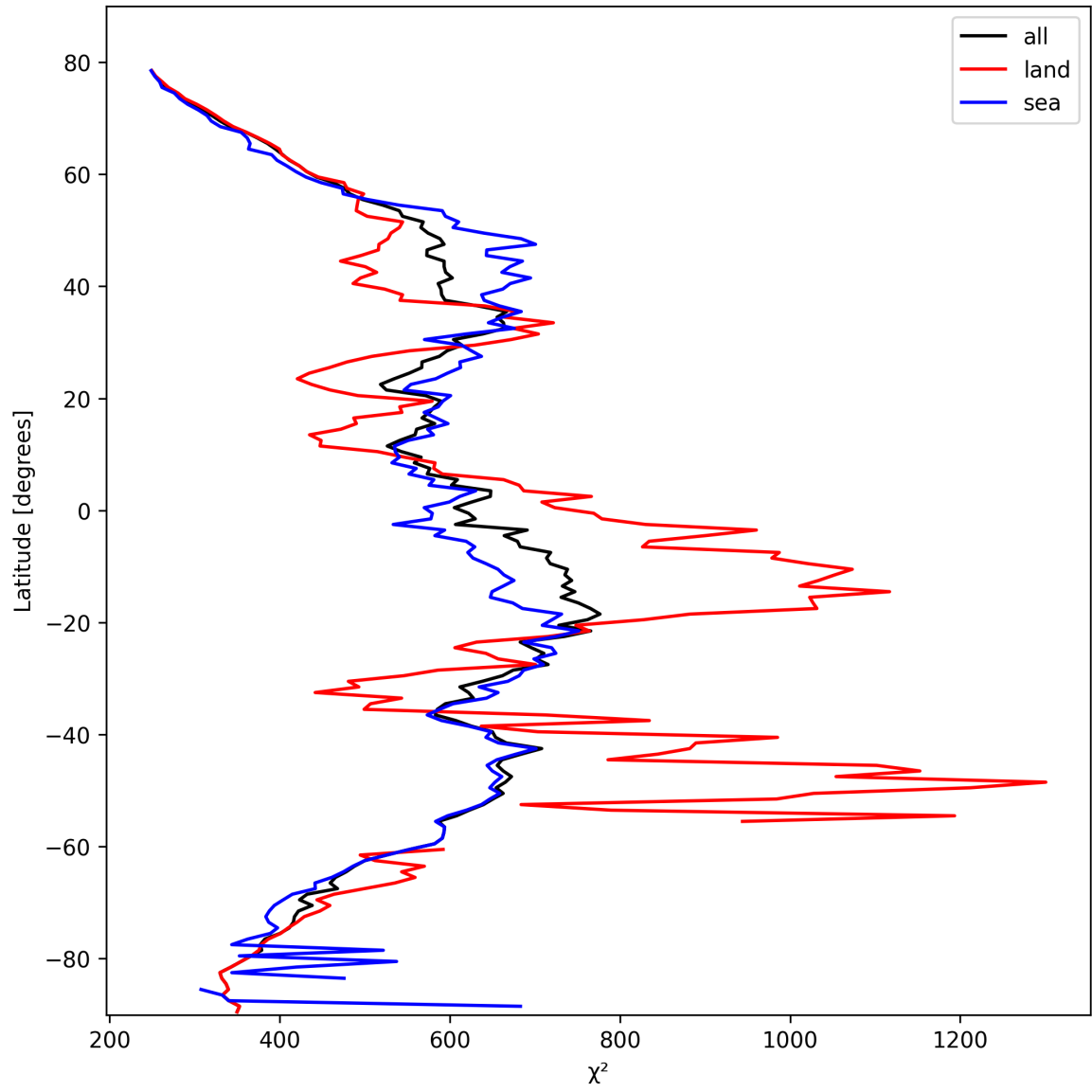
Figure 23: Zonal average of “ \chi^2 ” for 2025-02-23 to 2025-02-24.
