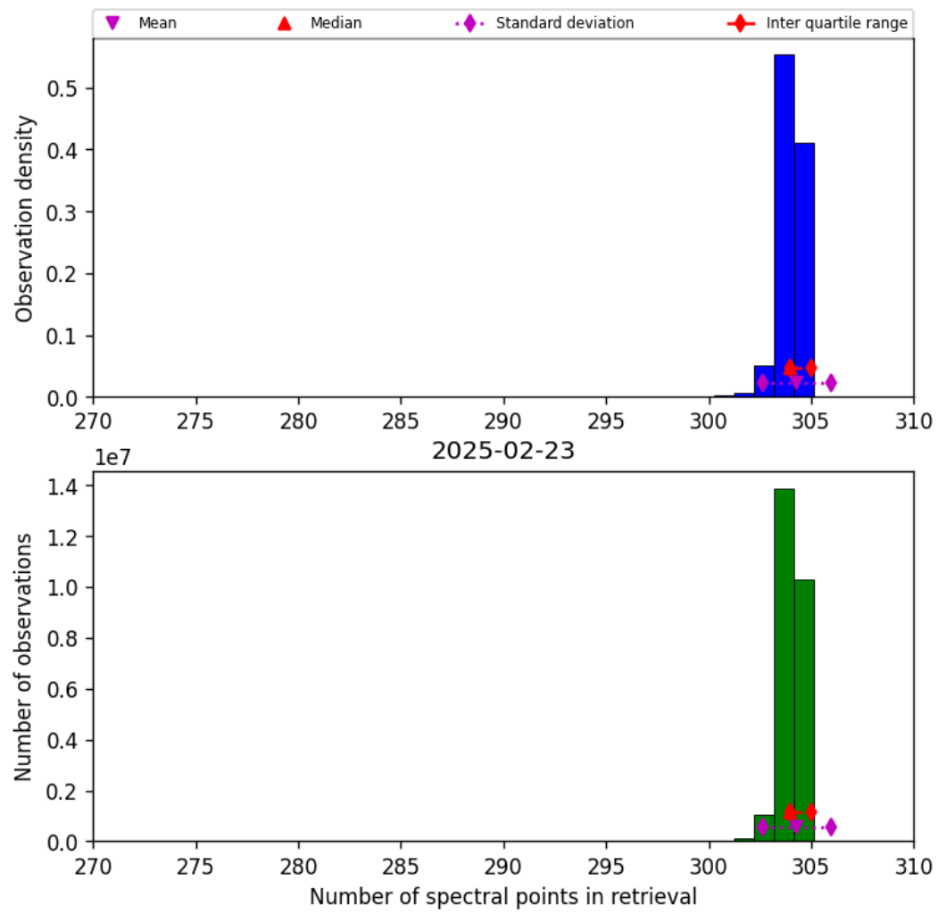
Figure 31: Histogram of “Number of spectral points in retrieval” for 2025-02-23 to 2025-02-24
