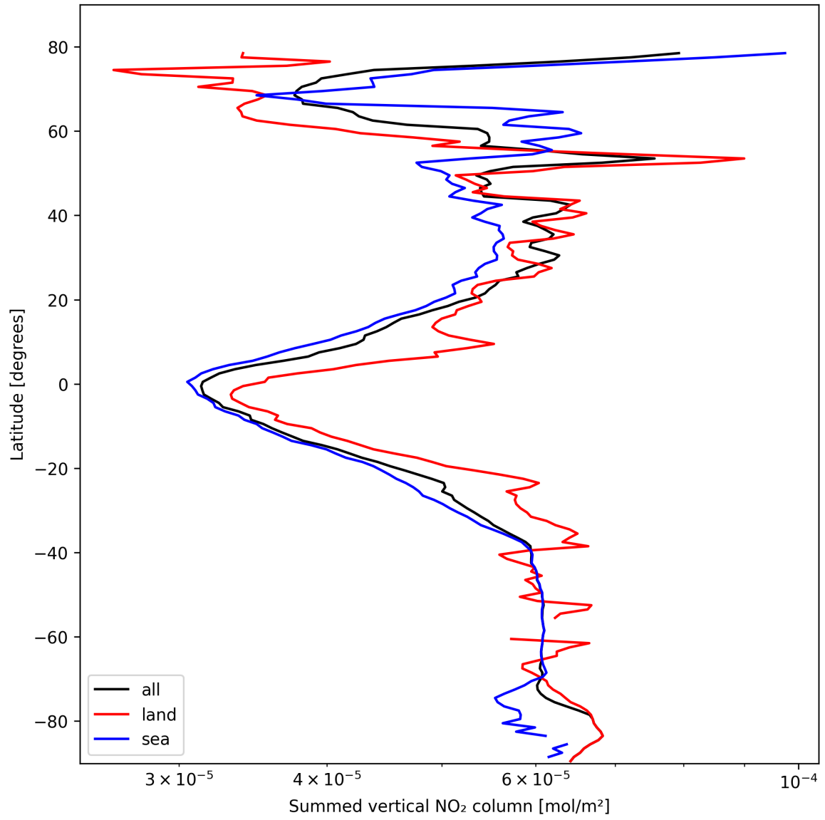
Figure 21: Zonal average of “Summed vertical NO 2 column” for 2025-02-23 to 2025-02-24.
