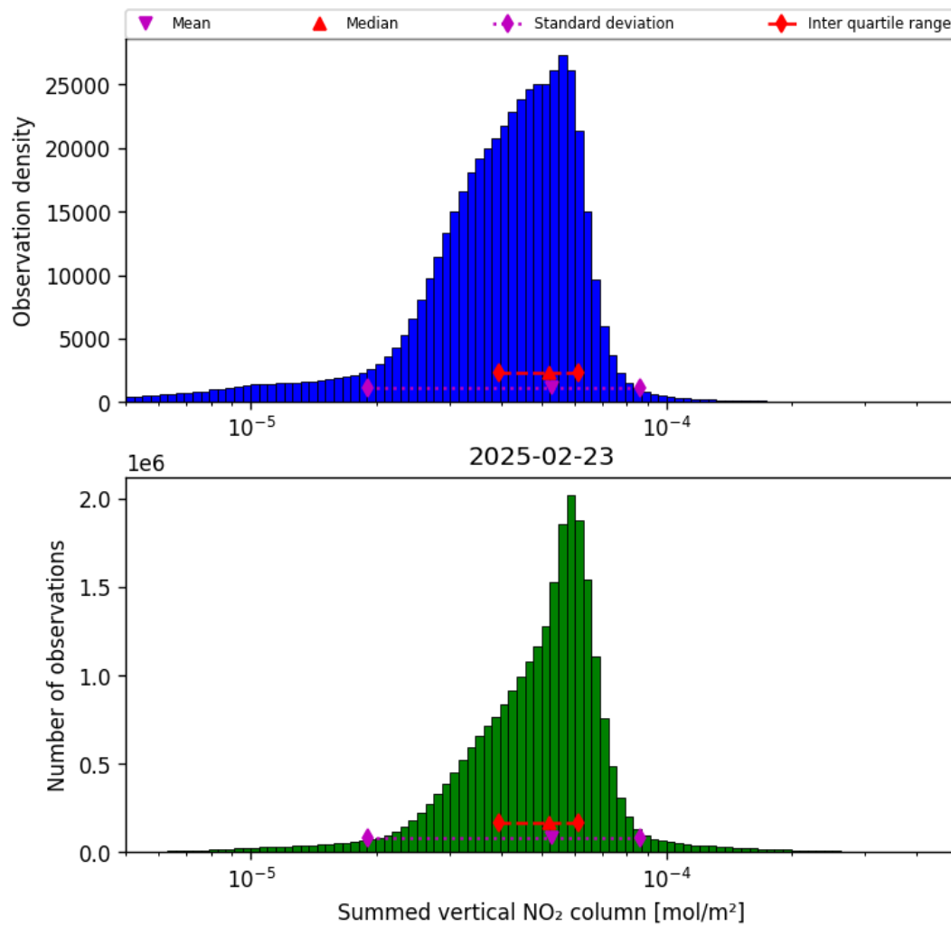
Figure 38: Histogram of “Summed vertical NO 2 column” for 2025-02-23 to 2025-02-24
