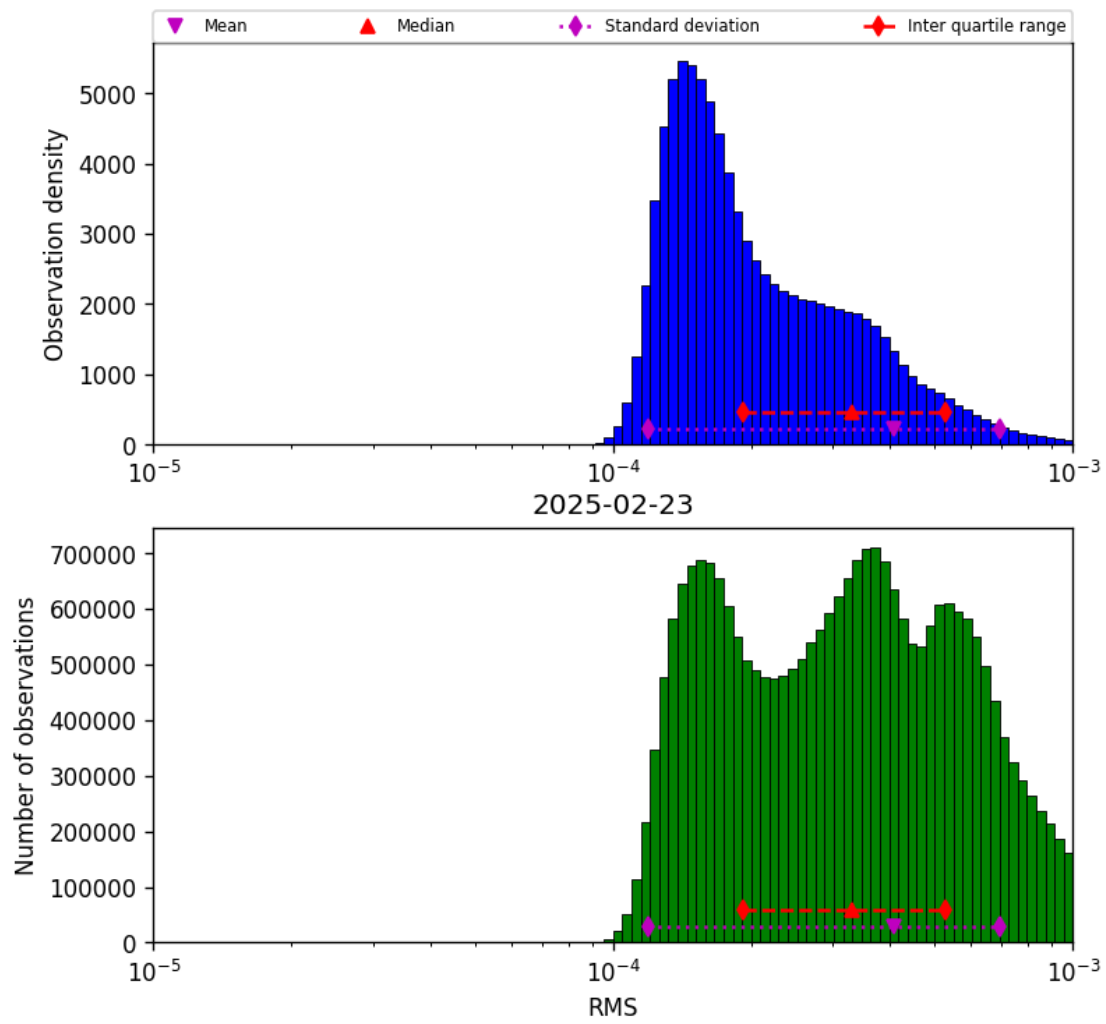
Figure 41: Histogram of “RMS” for 2025-02-23 to 2025-02-24
