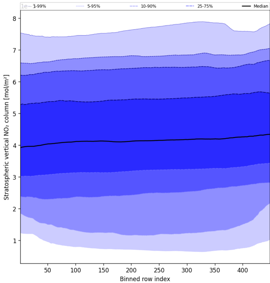
Figure 51: Along track statistics of “Stratospheric vertical NO 2 column” for 2025-02-23 to 2025-02-24
