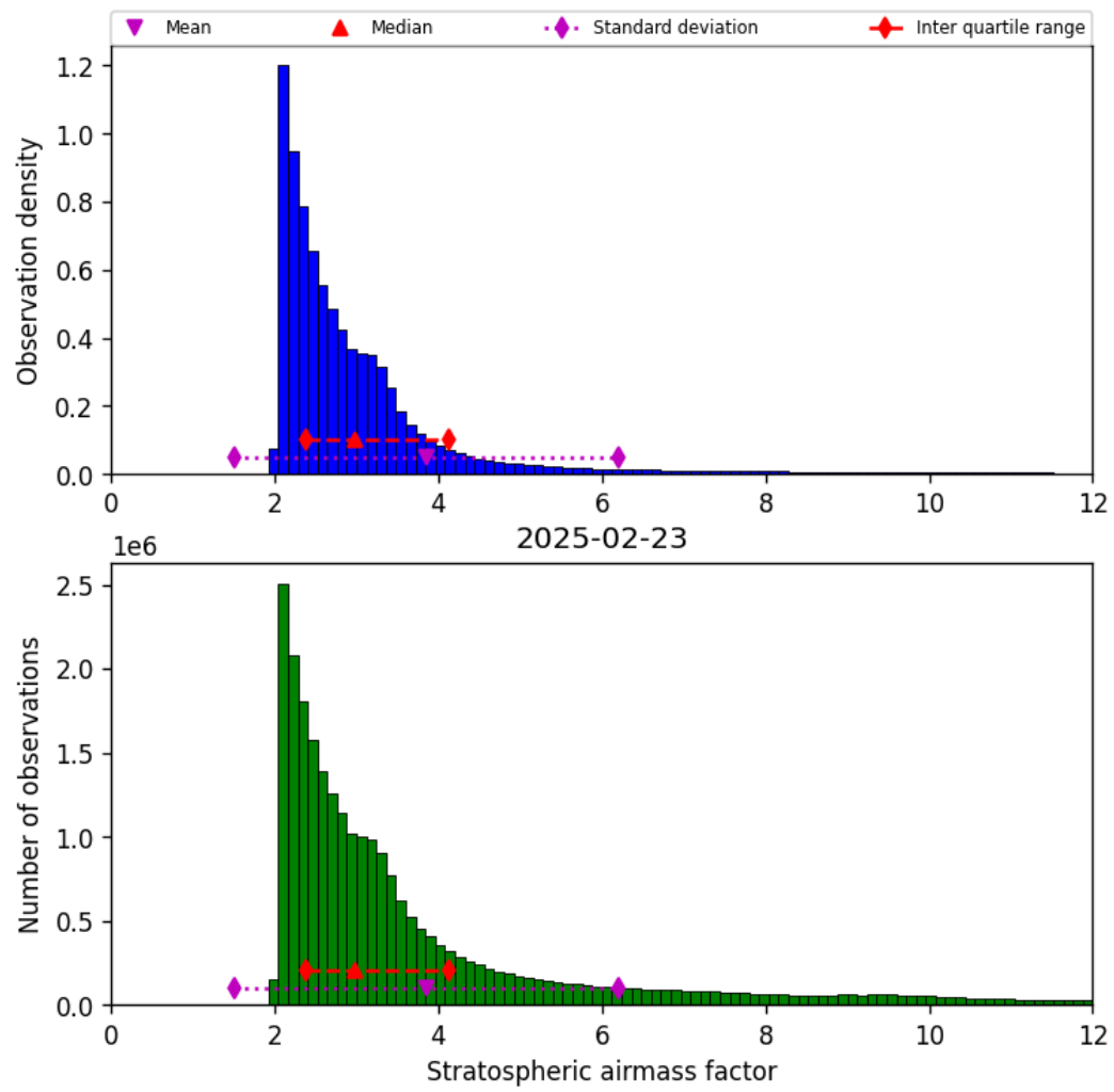
Figure 42: Histogram of “Stratospheric airmass factor” for 2025-02-23 to 2025-02-24
