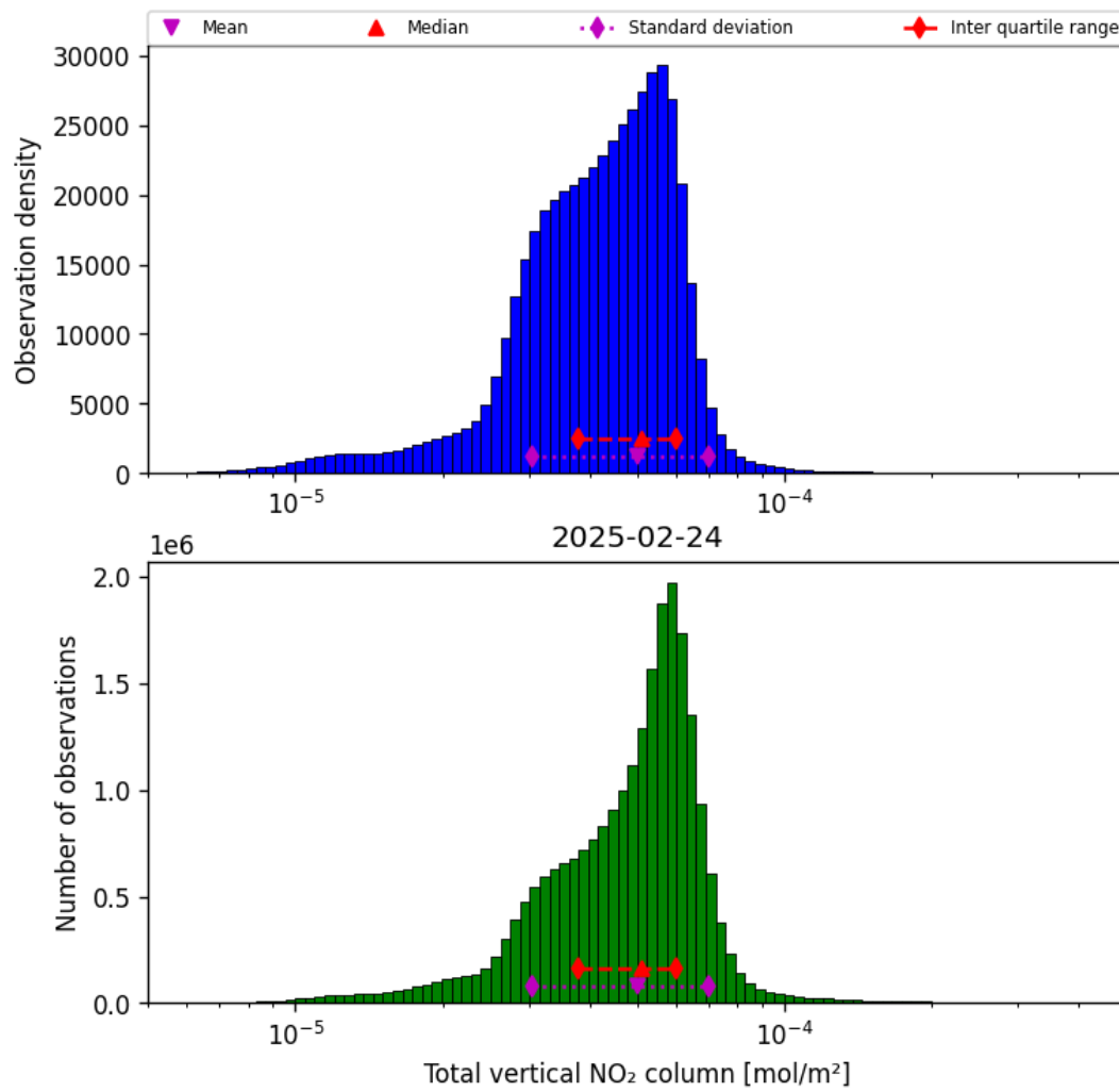
Figure 36: Histogram of "Total vertical NO 2 column" for 2025-02-24 to 2025-02-25
