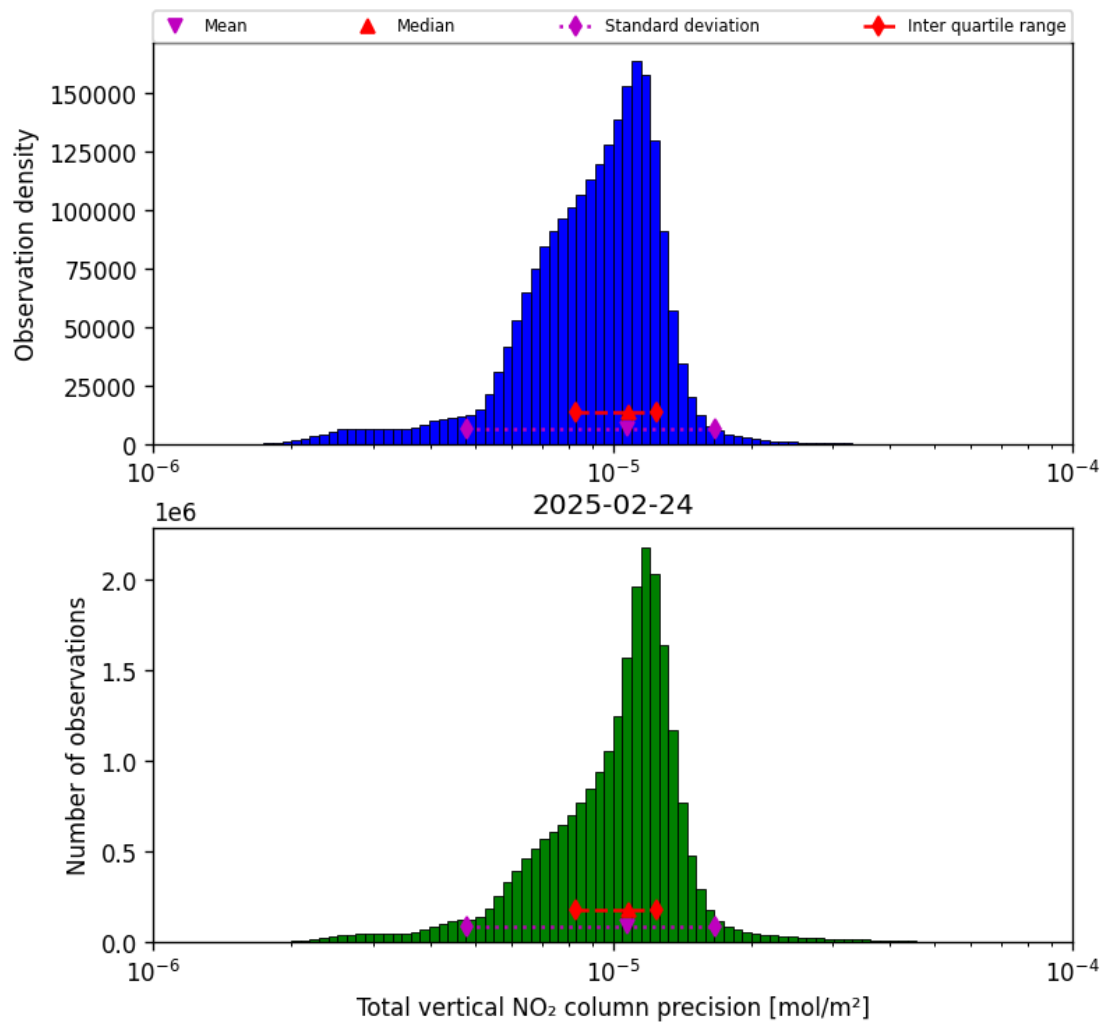
Figure 37: Histogram of “Total vertical NO 2 column precision” for 2025-02-24 to 2025-02-25
