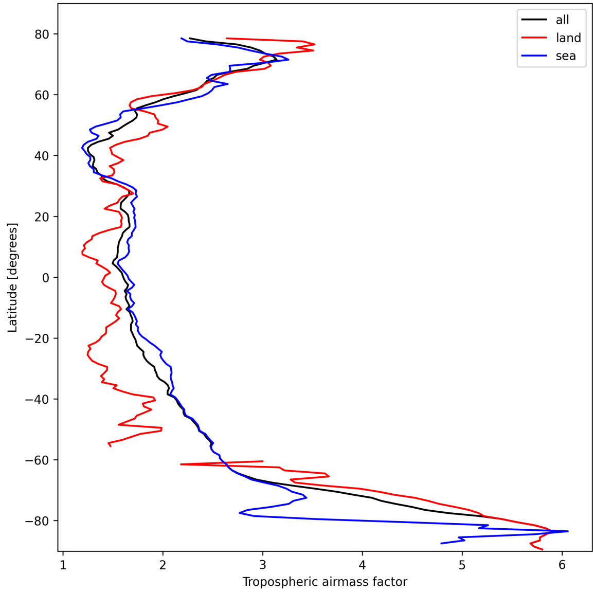
Figure 12: Zonal average of “Tropospheric airmass factor” for 2025-02-24 to 2025-02-25.
