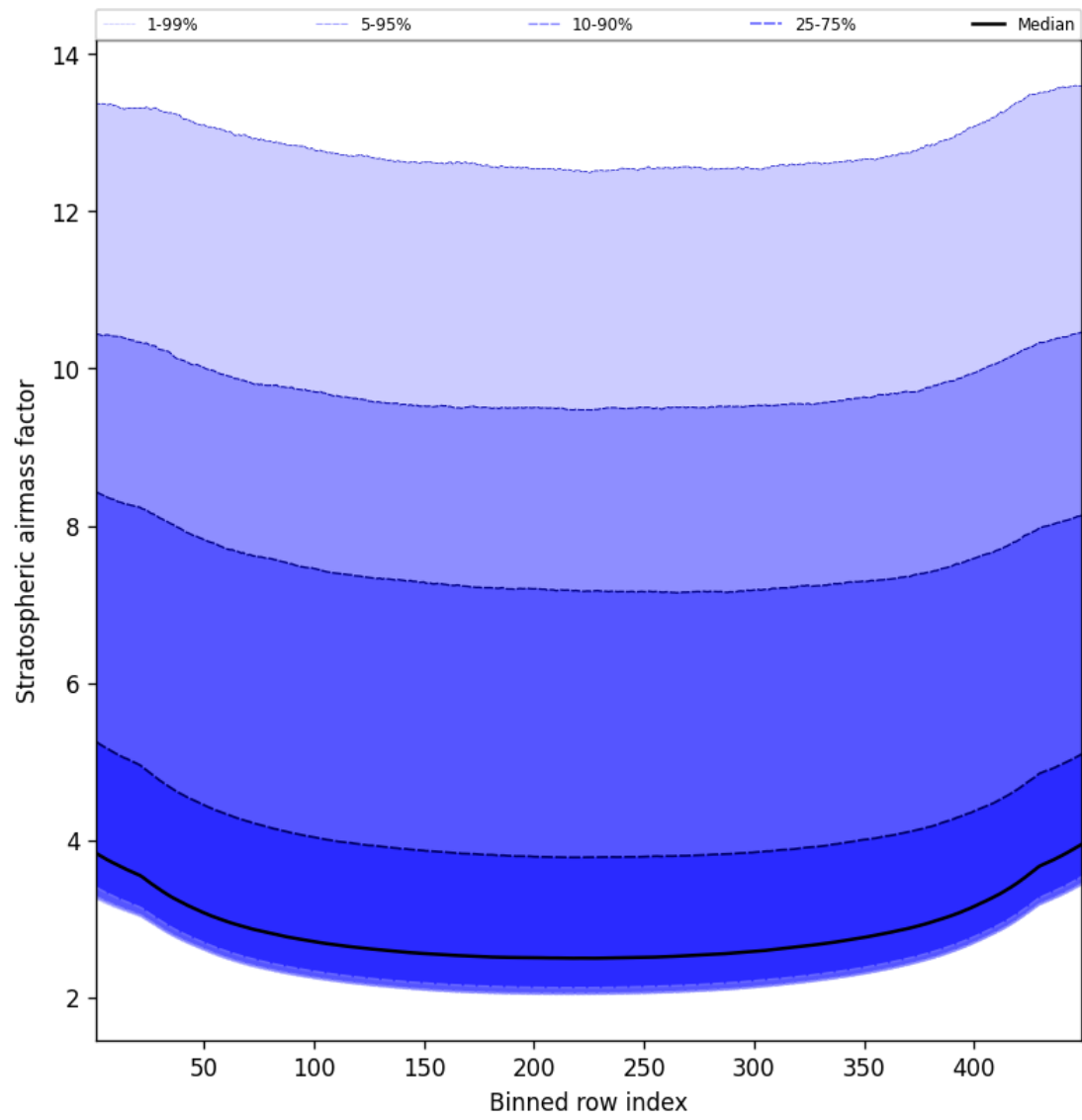
Figure 59: Along track statistics of “Stratospheric airmass factor” for 2025-02-24 to 2025-02-25
