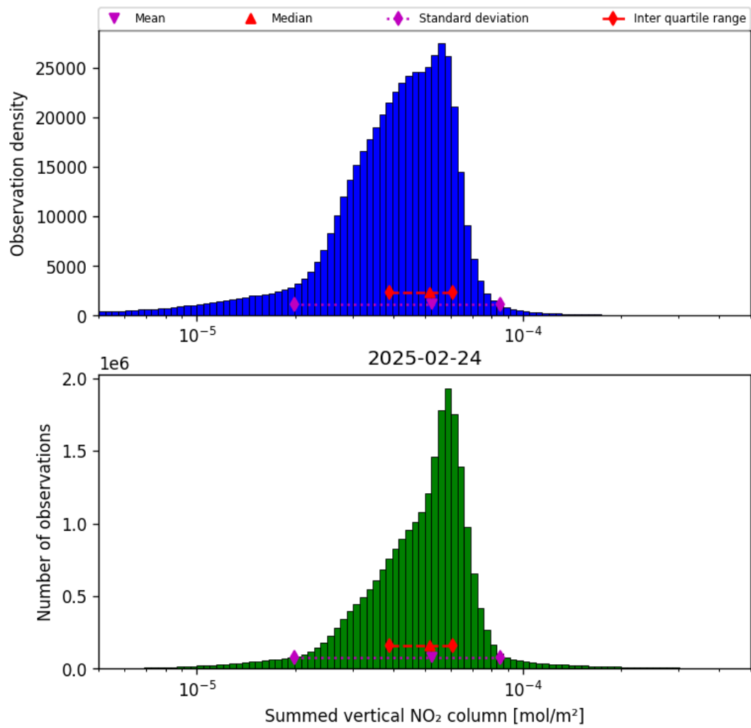
Figure 38: Histogram of “Summed vertical NO 2 column” for 2025-02-24 to 2025-02-25
