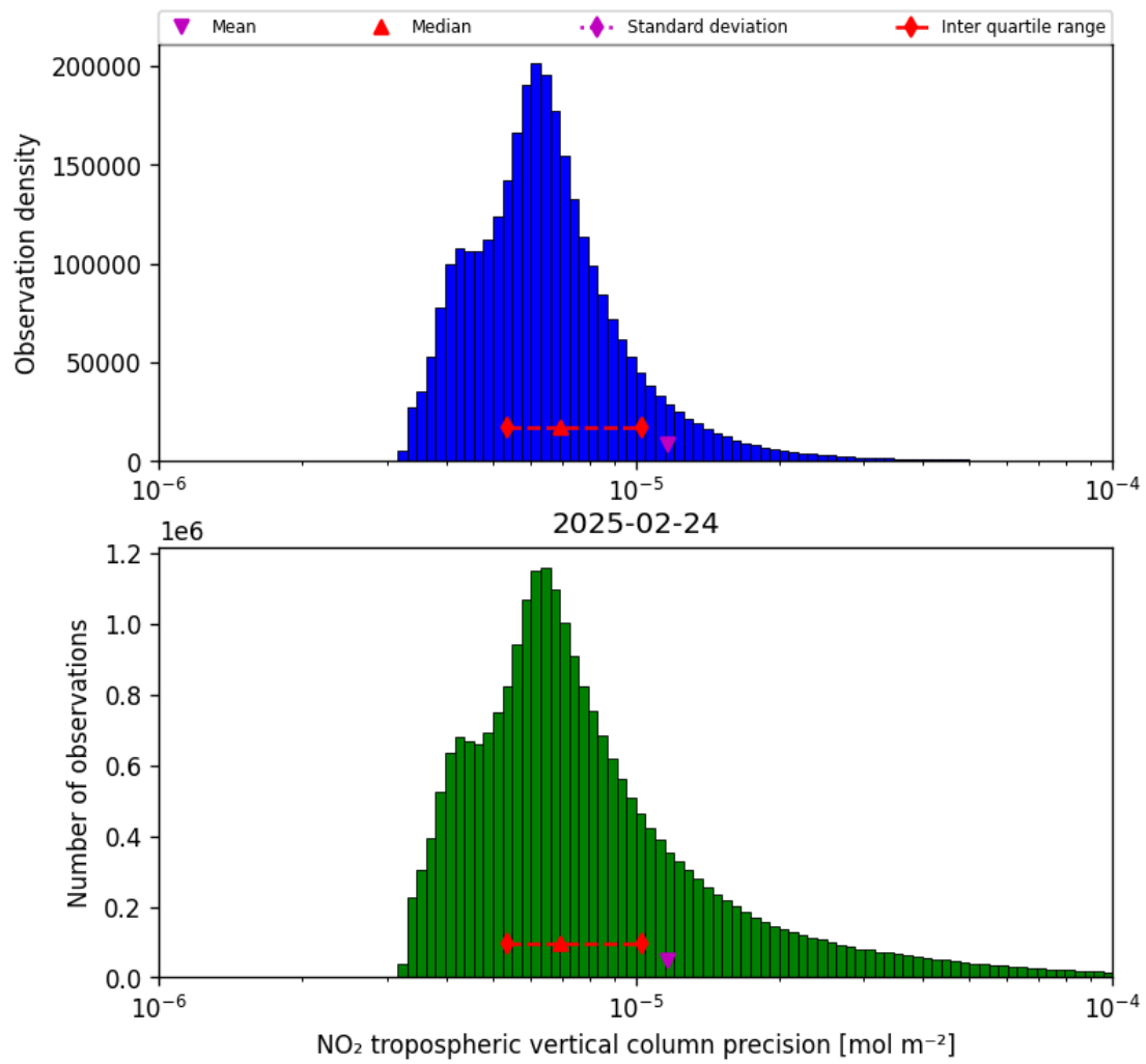
Figure 28: Histogram of “NO 2 tropospheric vertical column precision” for 2025-02-24 to 2025-02-25
