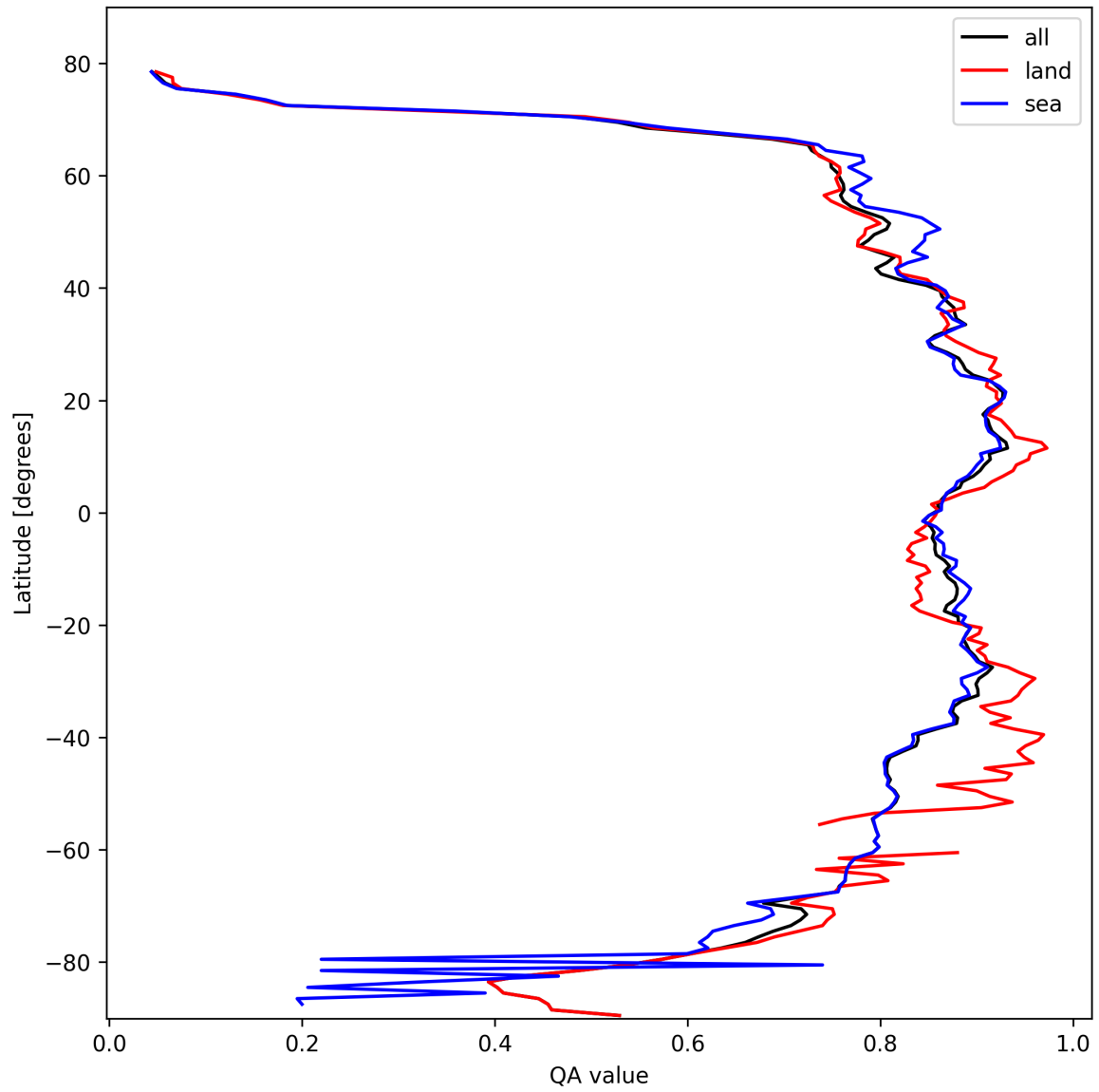
Figure 9: Zonal average of “QA value” for 2025-02-24 to 2025-02-25.
