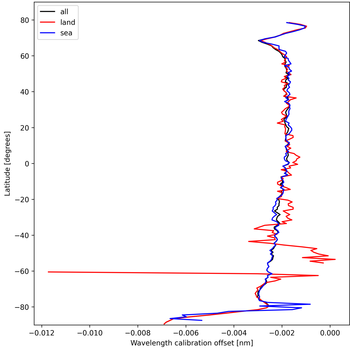
Figure 16: Zonal average of “Wavelength calibration offset” for 2025-02-24 to 2025-02-25.
