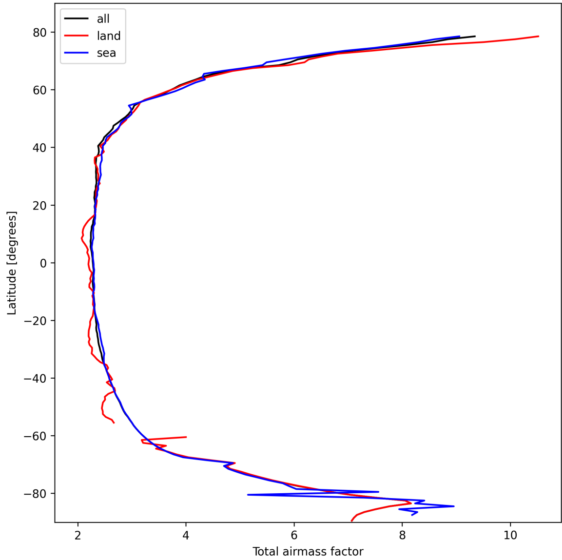
Figure 13: Zonal average of “Total airmass factor” for 2025-02-24 to 2025-02-25.
