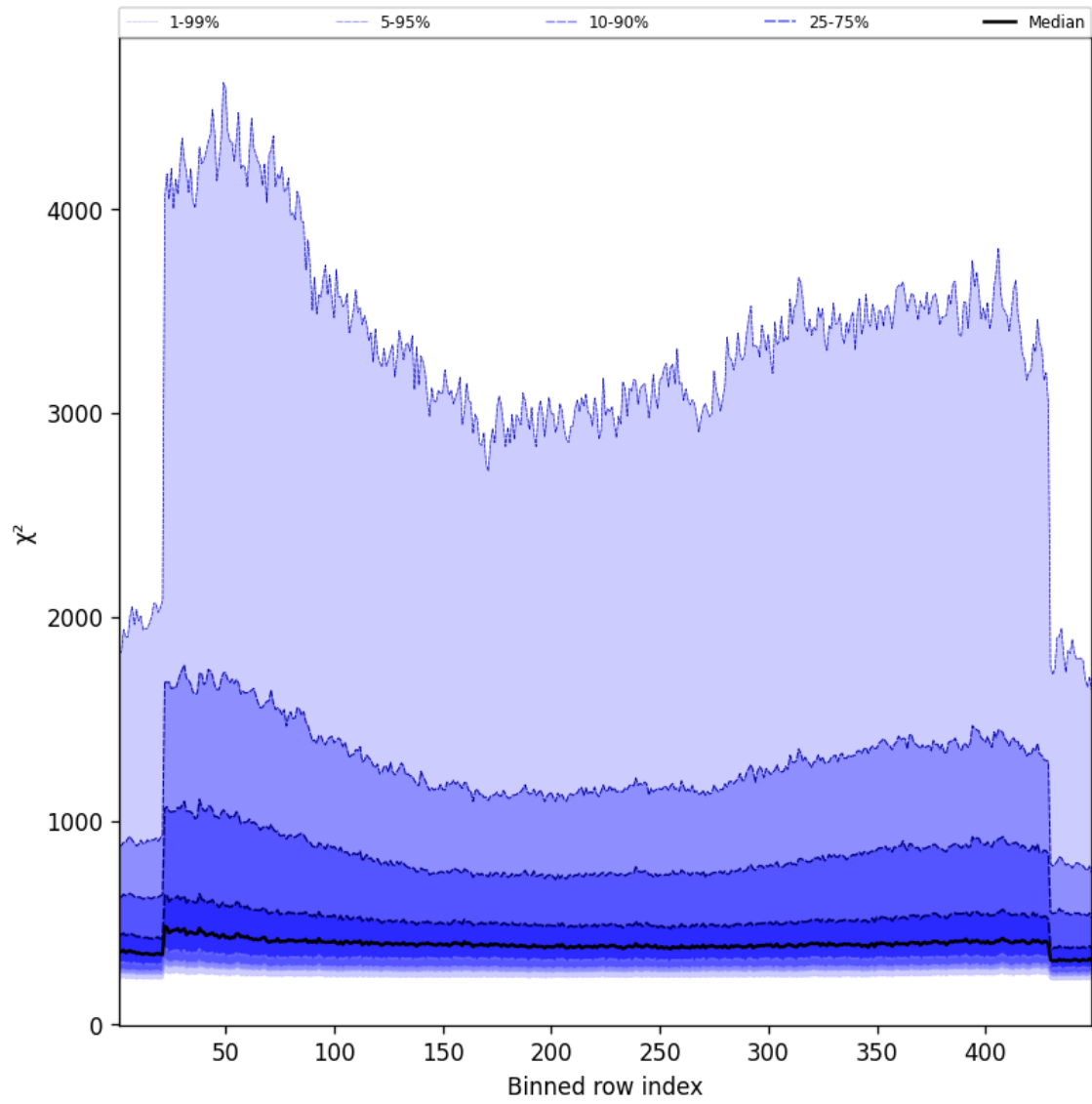
Figure 57: Along track statistics of “ \chi^2 ” for 2025-02-24 to 2025-02-25
