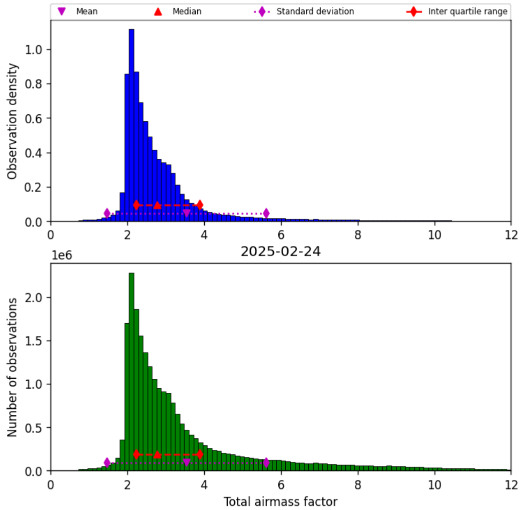
Figure 30: Histogram of “Total airmass factor” for 2025-02-24 to 2025-02-25
