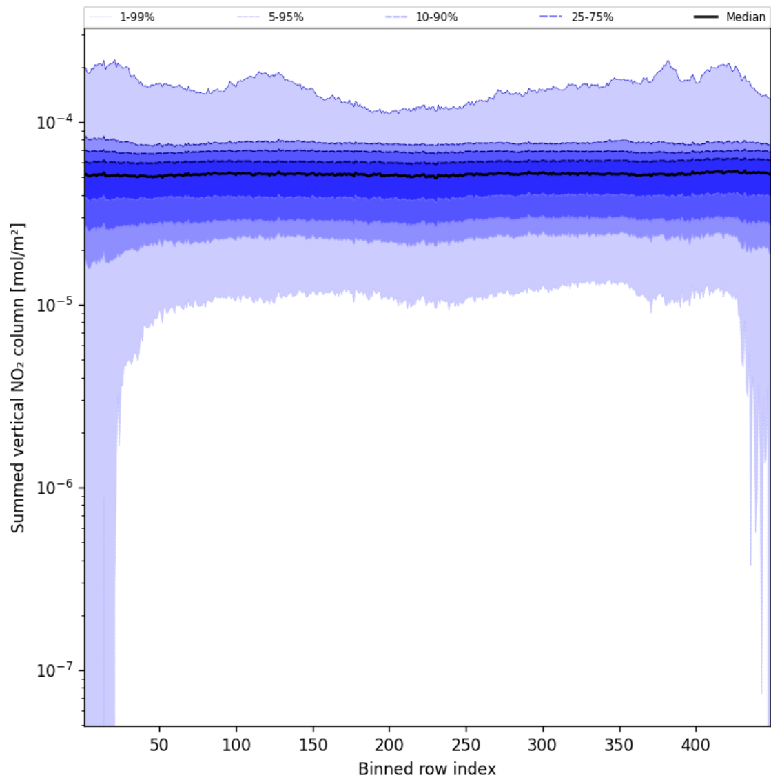
Figure 55: Along track statistics of “Summed vertical NO 2 column” for 2025-02-24 to 2025-02-25
