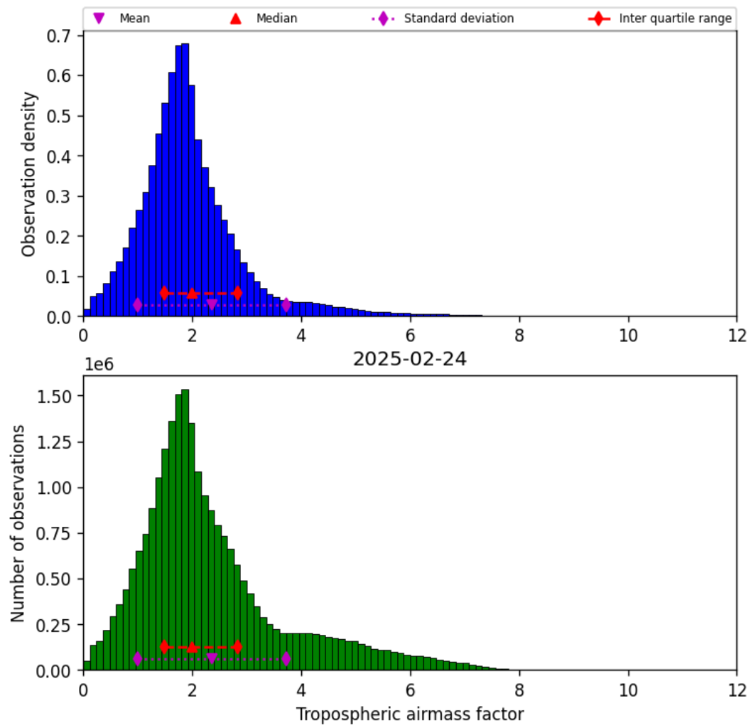
Figure 29: Histogram of “Tropospheric airmass factor” for 2025-02-24 to 2025-02-25
