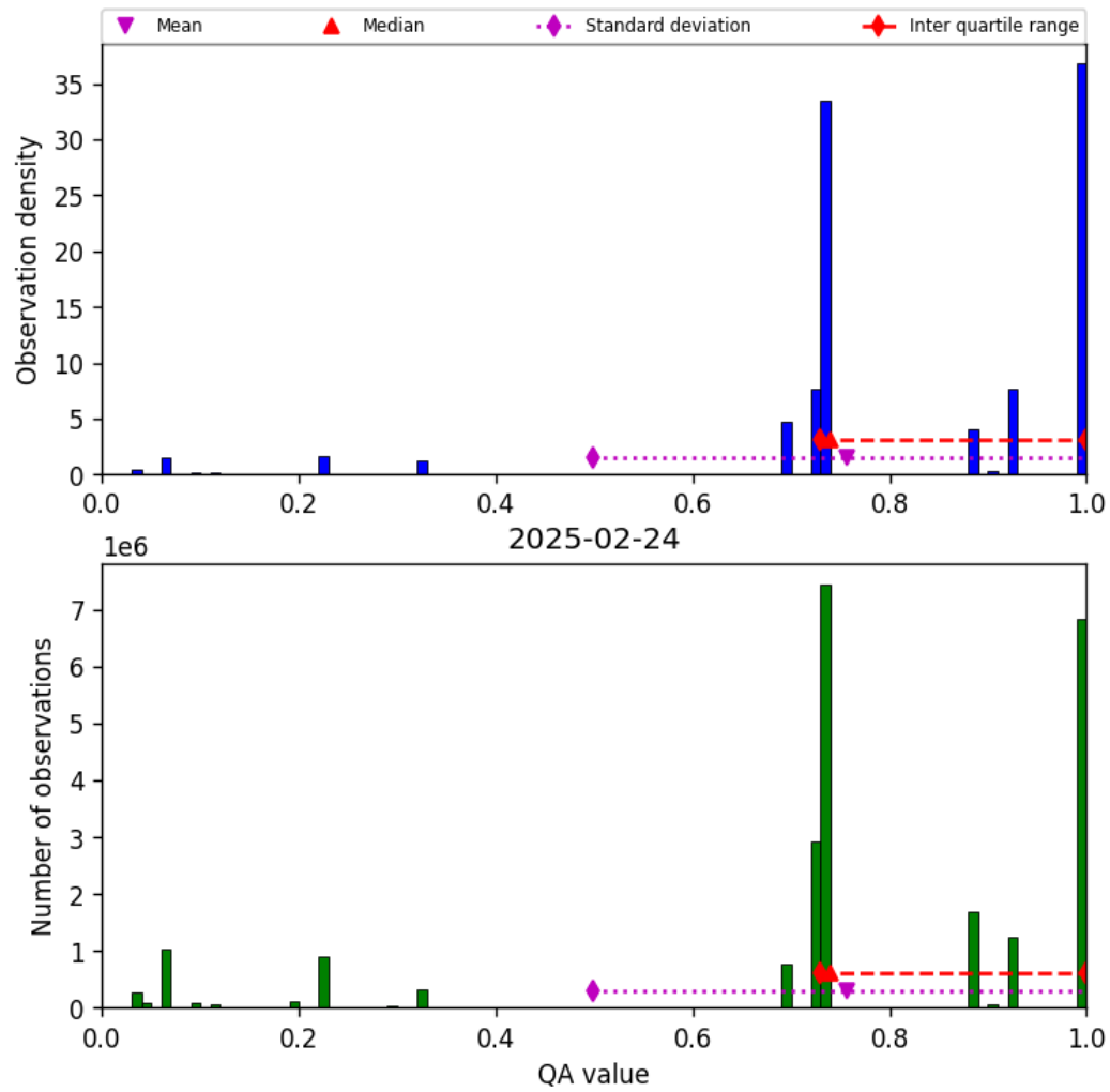
Figure 26: Histogram of “QA value” for 2025-02-24 to 2025-02-25
