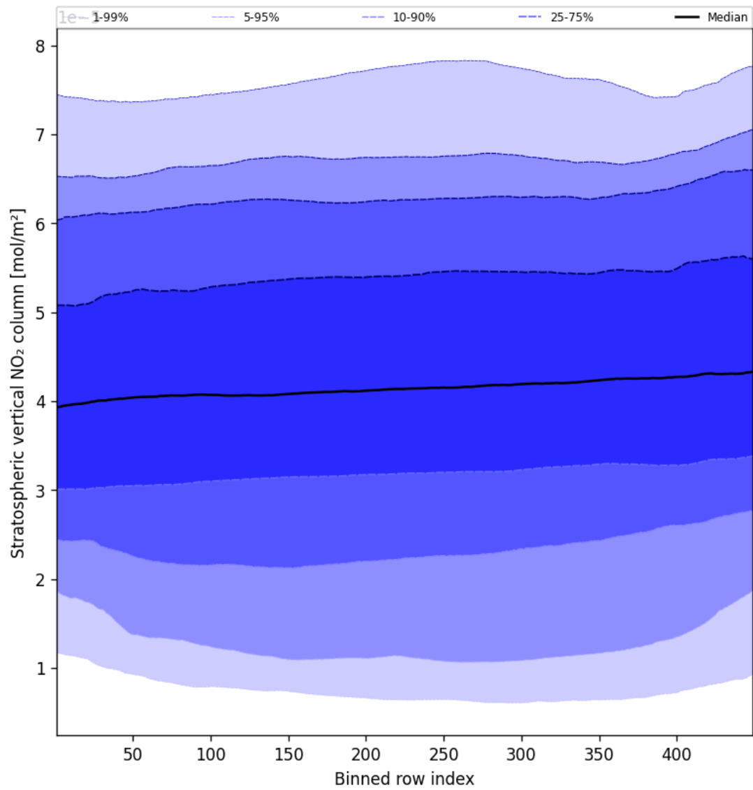
Figure 51: Along track statistics of “Stratospheric vertical NO 2 column” for 2025-02-24 to 2025-02-25
