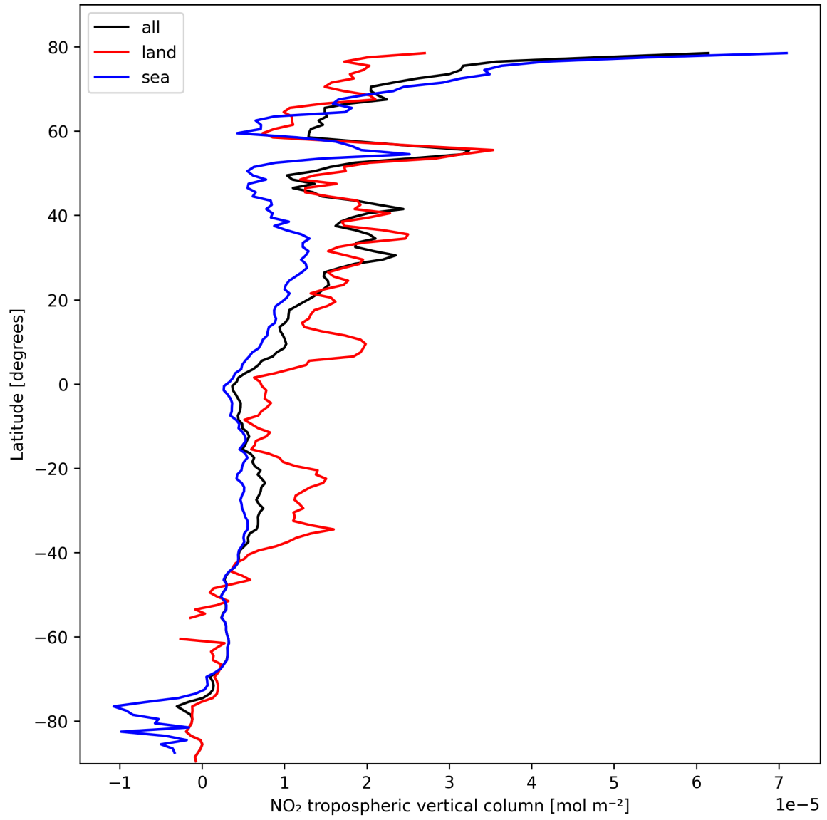
Figure 10: Zonal average of “NO 2 tropospheric vertical column” for 2025-02-24 to 2025-02-25.
