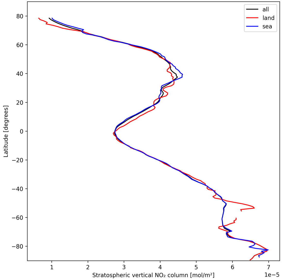
Figure 17: Zonal average of “Stratospheric vertical NO 2 column” for 2025-02-24 to 2025-02-25.
