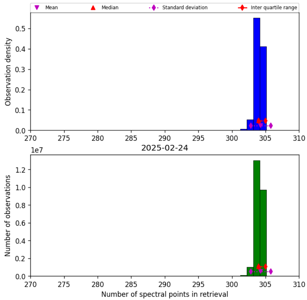
Figure 31: Histogram of “Number of spectral points in retrieval” for 2025-02-24 to 2025-02-25
