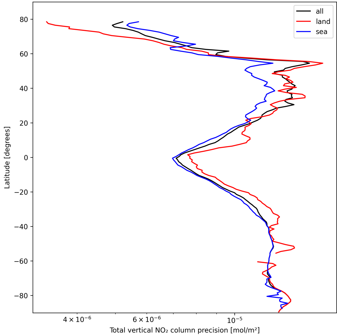
Figure 20: Zonal average of “Total vertical NO 2 column precision” for 2025-02-24 to 2025-02-25.
