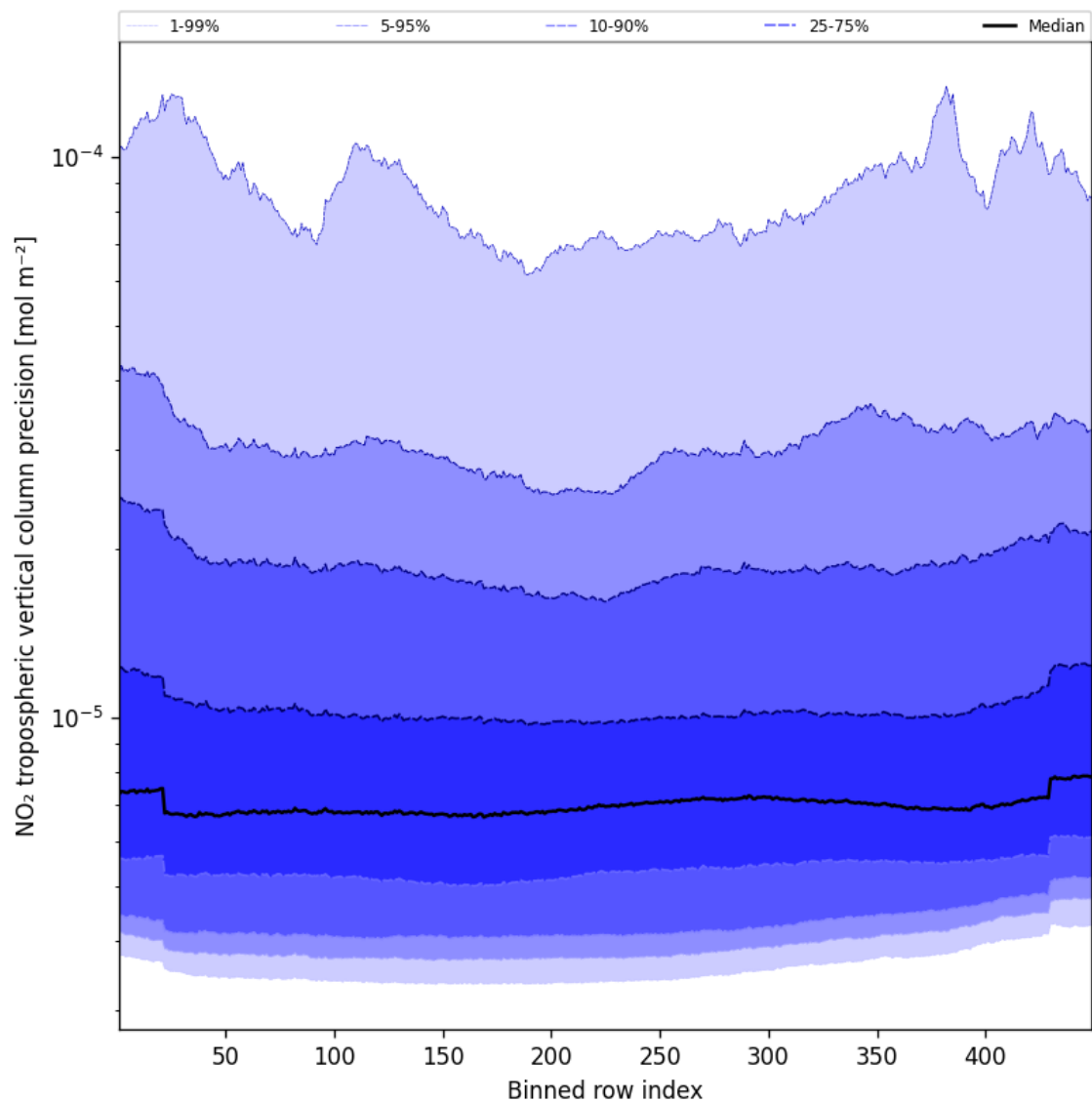
Figure 45: Along track statistics of “NO 2 tropospheric vertical column precision” for 2025-02-24 to 2025-02-25
