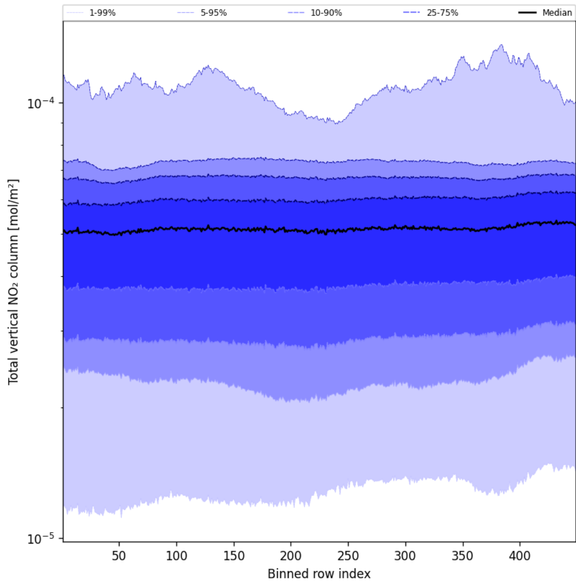
Figure 53: Along track statistics of “Total vertical NO 2 column” for 2025-02-24 to 2025-02-25
