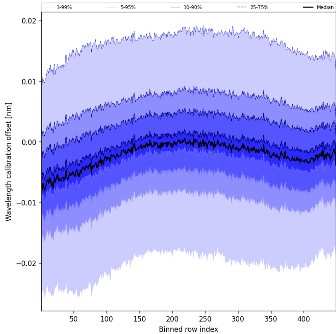
Figure 50: Along track statistics of “Wavelength calibration offset” for 2025-02-24 to 2025-02-25
