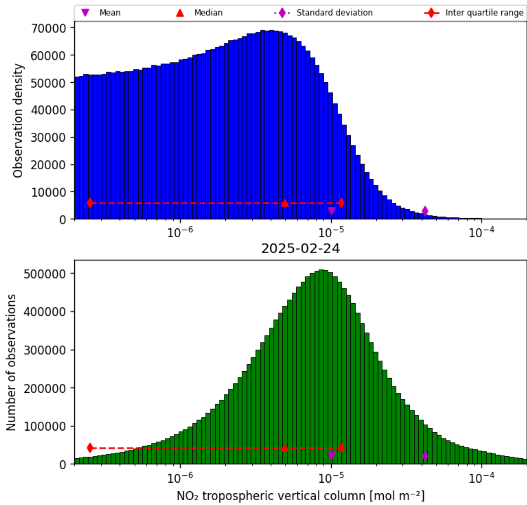
Figure 27: Histogram of “NO 2 tropospheric vertical column” for 2025-02-24 to 2025-02-25
