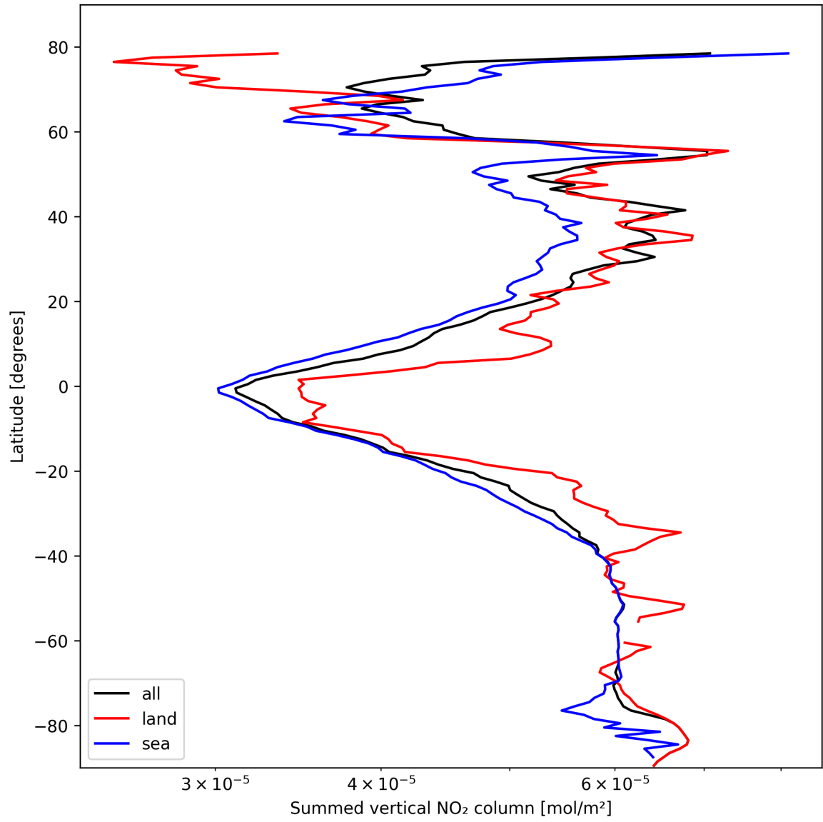
Figure 21: Zonal average of “Summed vertical NO 2 column” for 2025-02-24 to 2025-02-25.
