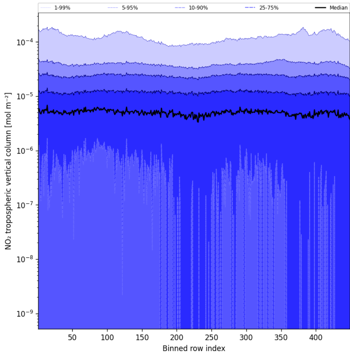
Figure 44: Along track statistics of “NO 2 tropospheric vertical column” for 2025-02-24 to 2025-02-25
