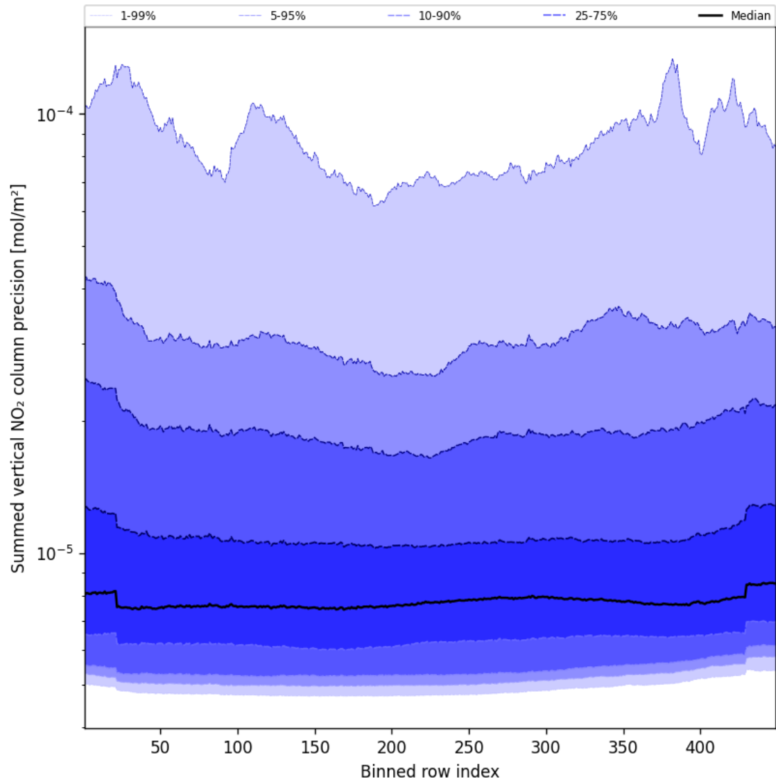
Figure 56: Along track statistics of “Summed vertical NO 2 column precision” for 2025-02-24 to 2025-02-25
