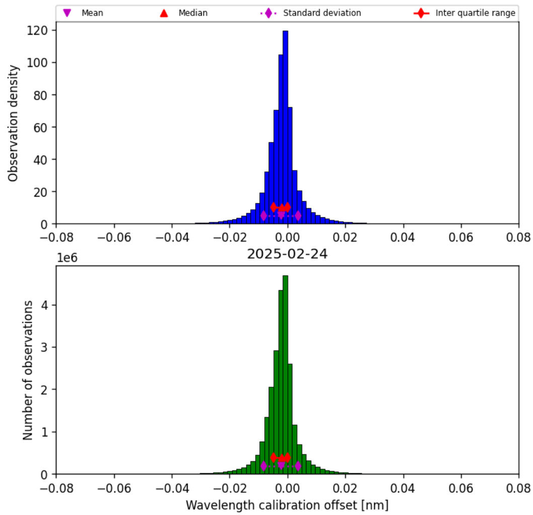
Figure 33: Histogram of “Wavelength calibration offset” for 2025-02-24 to 2025-02-25
