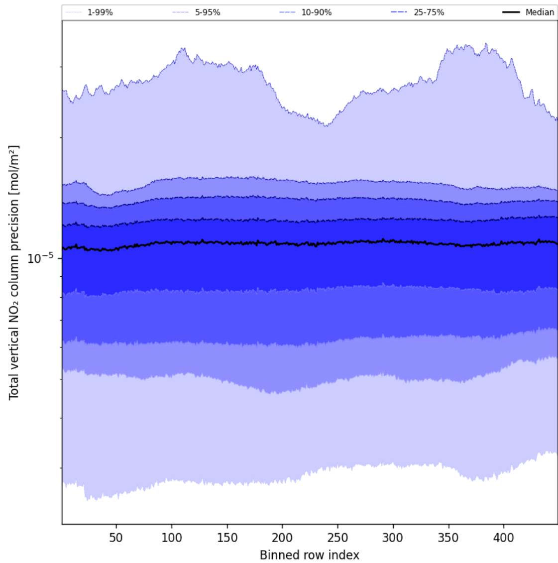
Figure 54: Along track statistics of “Total vertical NO 2 column precision” for 2025-02-24 to 2025-02-25
