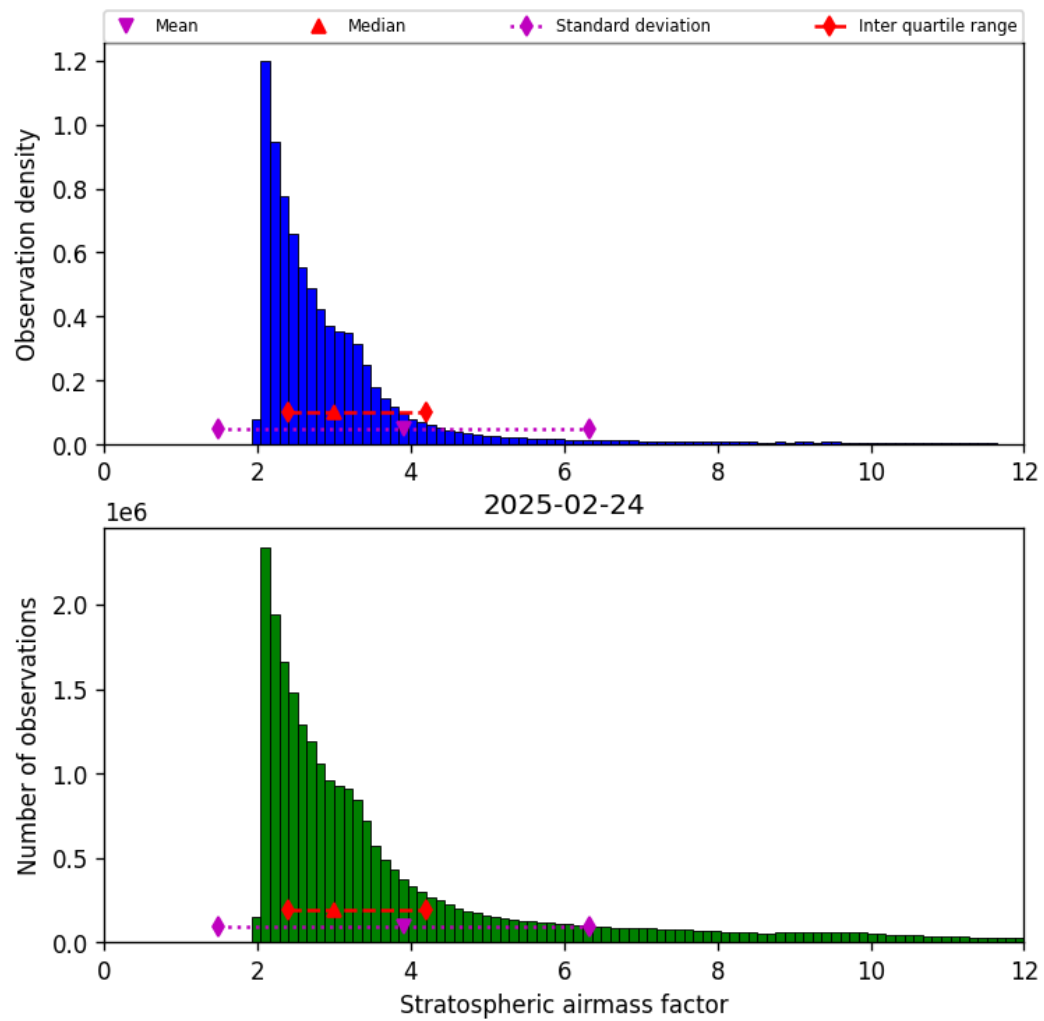
Figure 42: Histogram of “Stratospheric airmass factor” for 2025-02-24 to 2025-02-25
