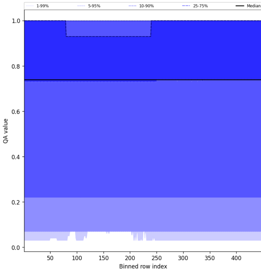
Figure 43: Along track statistics of “QA value” for 2025-02-24 to 2025-02-25
