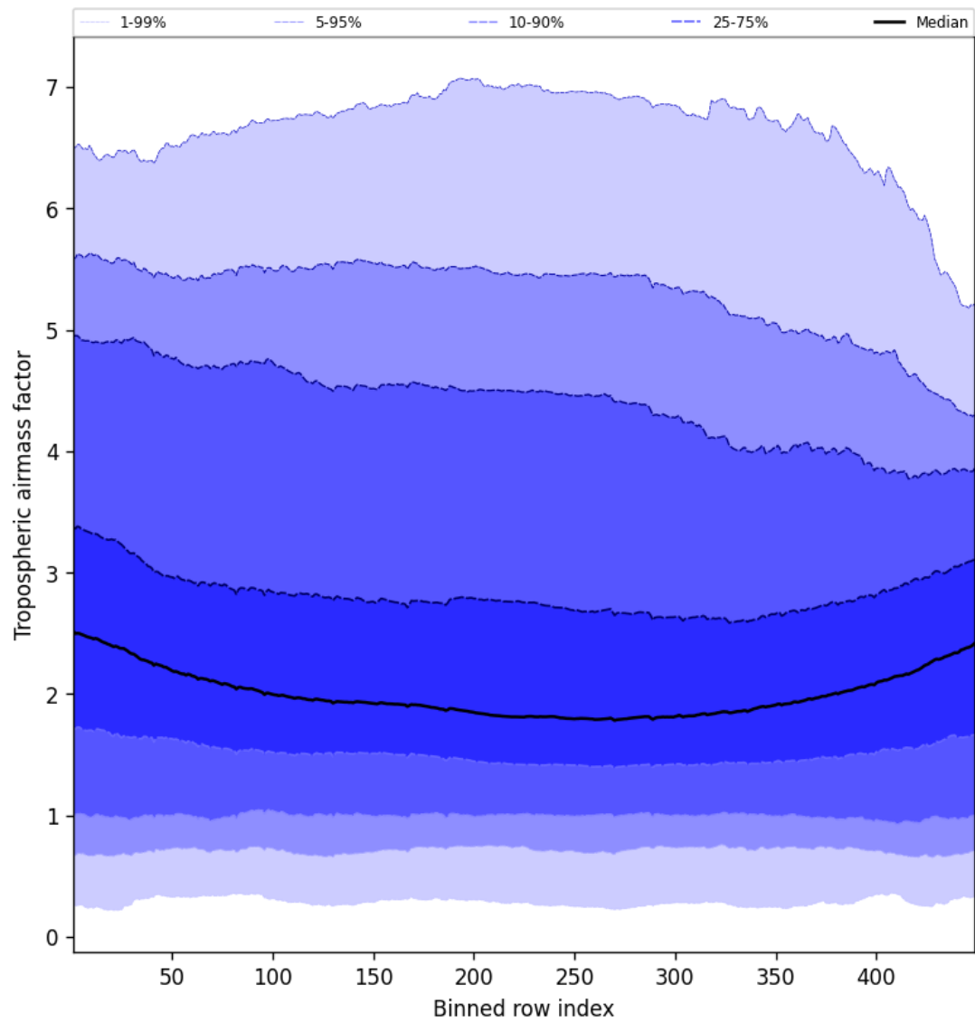
Figure 46: Along track statistics of “Tropospheric air mass factor” for 2025-02-24 to 2025-02-25
