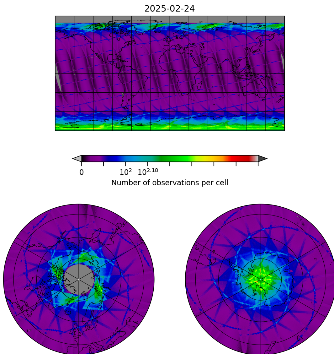
Figure 8: Map of the number of observations for 2025-02-24 to 2025-02-25
