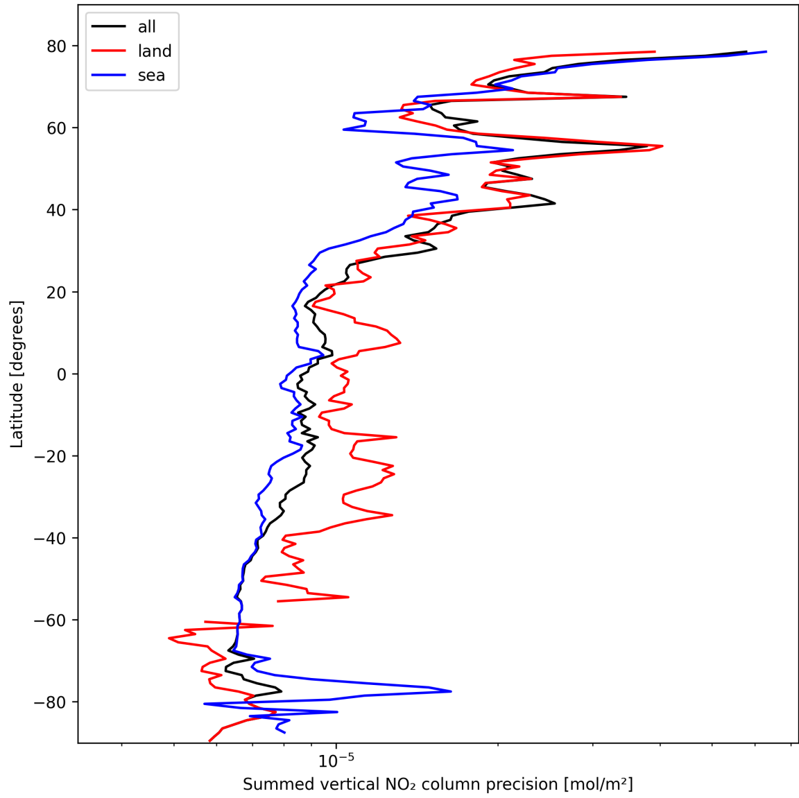
Figure 22: Zonal average of “Summed vertical NO 2 column precision” for 2025-02-24 to 2025-02-25.
