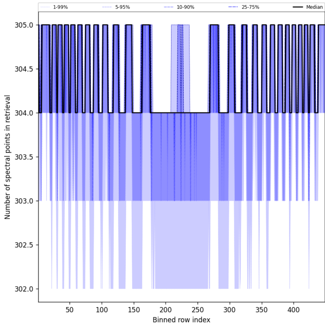
Figure 48: Along track statistics of “Number of spectral points in retrieval” for 2025-02-24 to 2025-02-25
