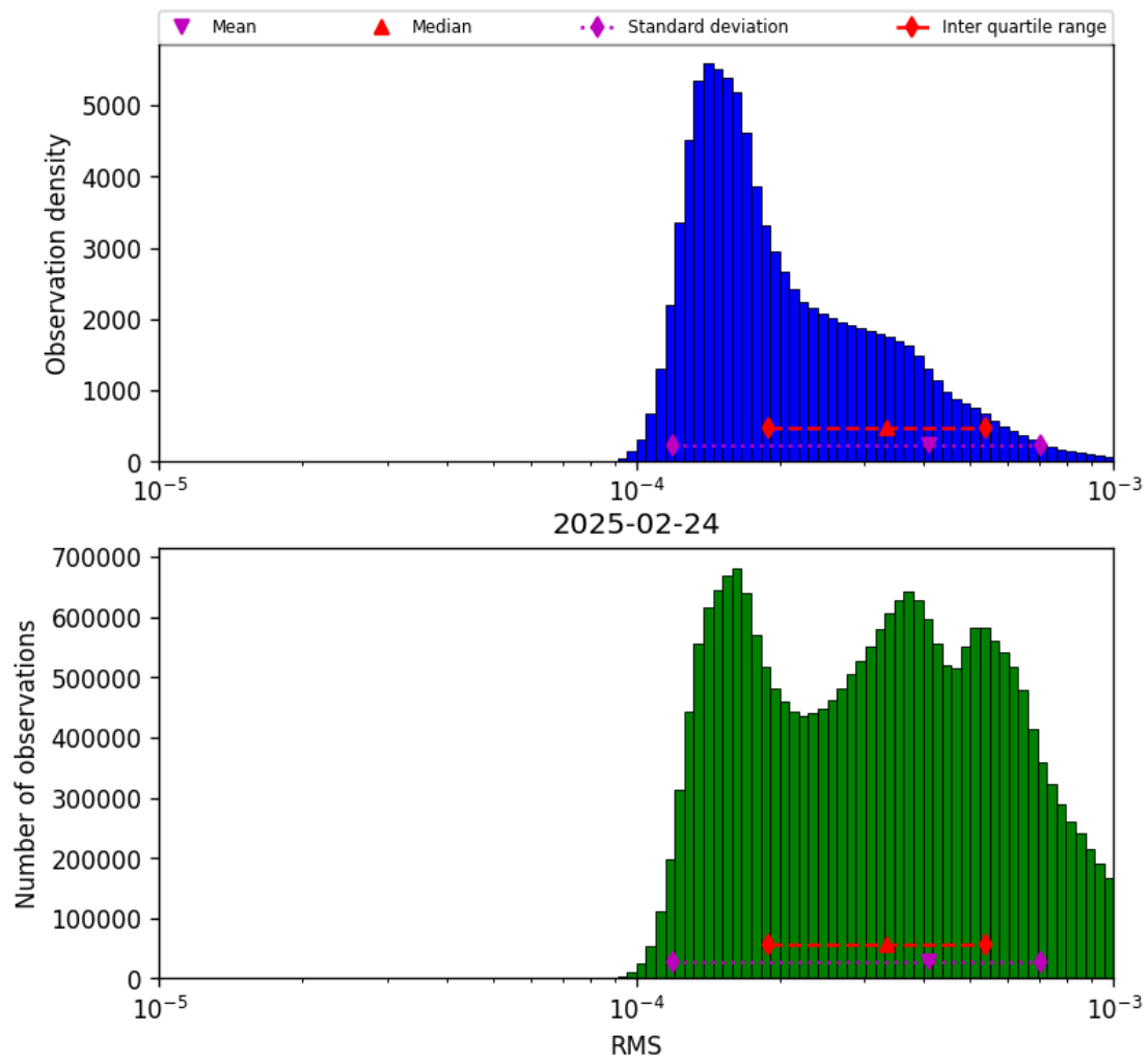
Figure 41: Histogram of “RMS” for 2025-02-24 to 2025-02-25
