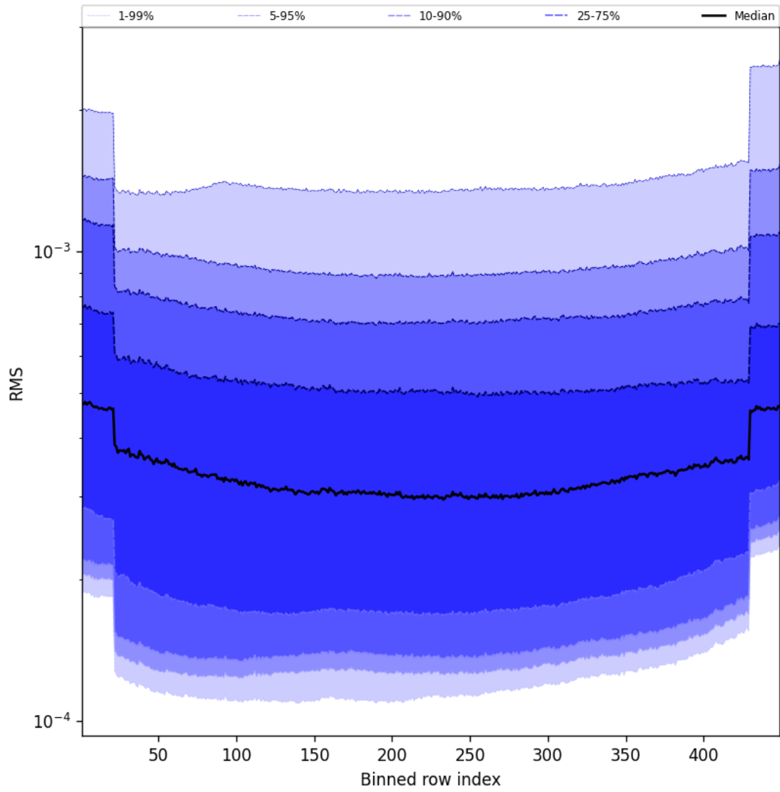
Figure 58: Along track statistics of “RMS” for 2025-02-24 to 2025-02-25
