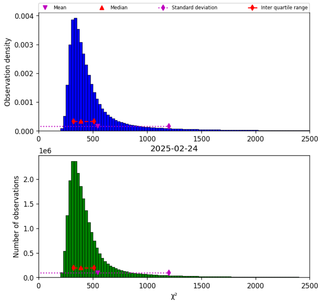
Figure 40: Histogram of “ \chi^2 ” for 2025-02-24 to 2025-02-25
