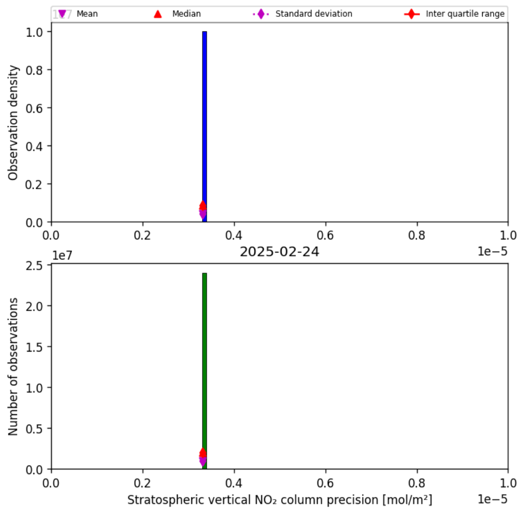
Figure 35: Histogram of “Stratospheric vertical NO 2 column precision” for 2025-02-24 to 2025-02-25
