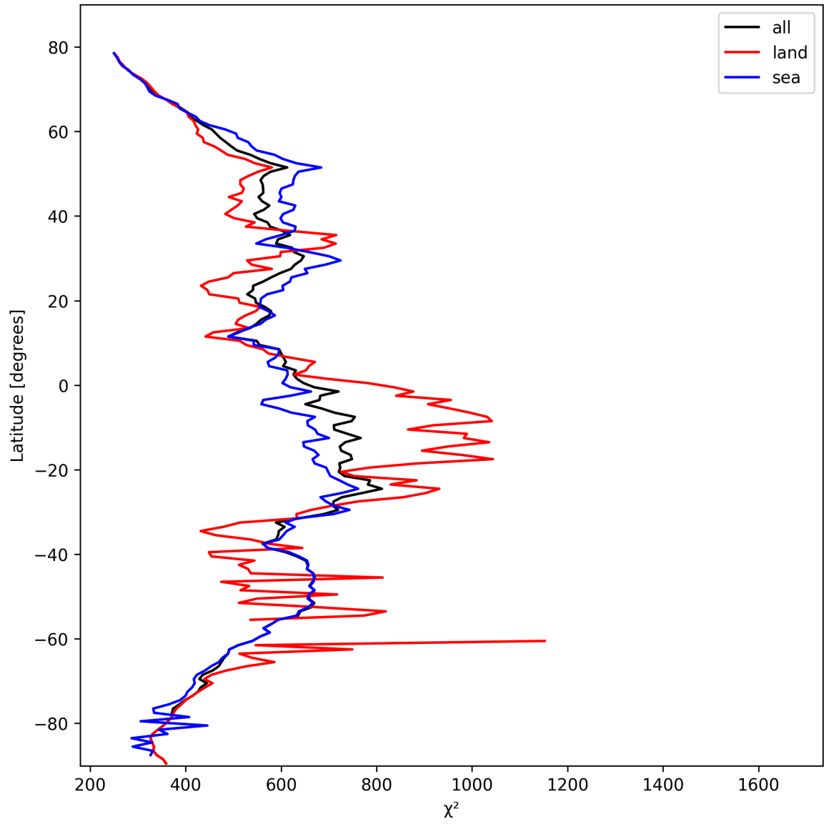
Figure 23: Zonal average of “ \chi^2 ” for 2025-02-24 to 2025-02-25.
