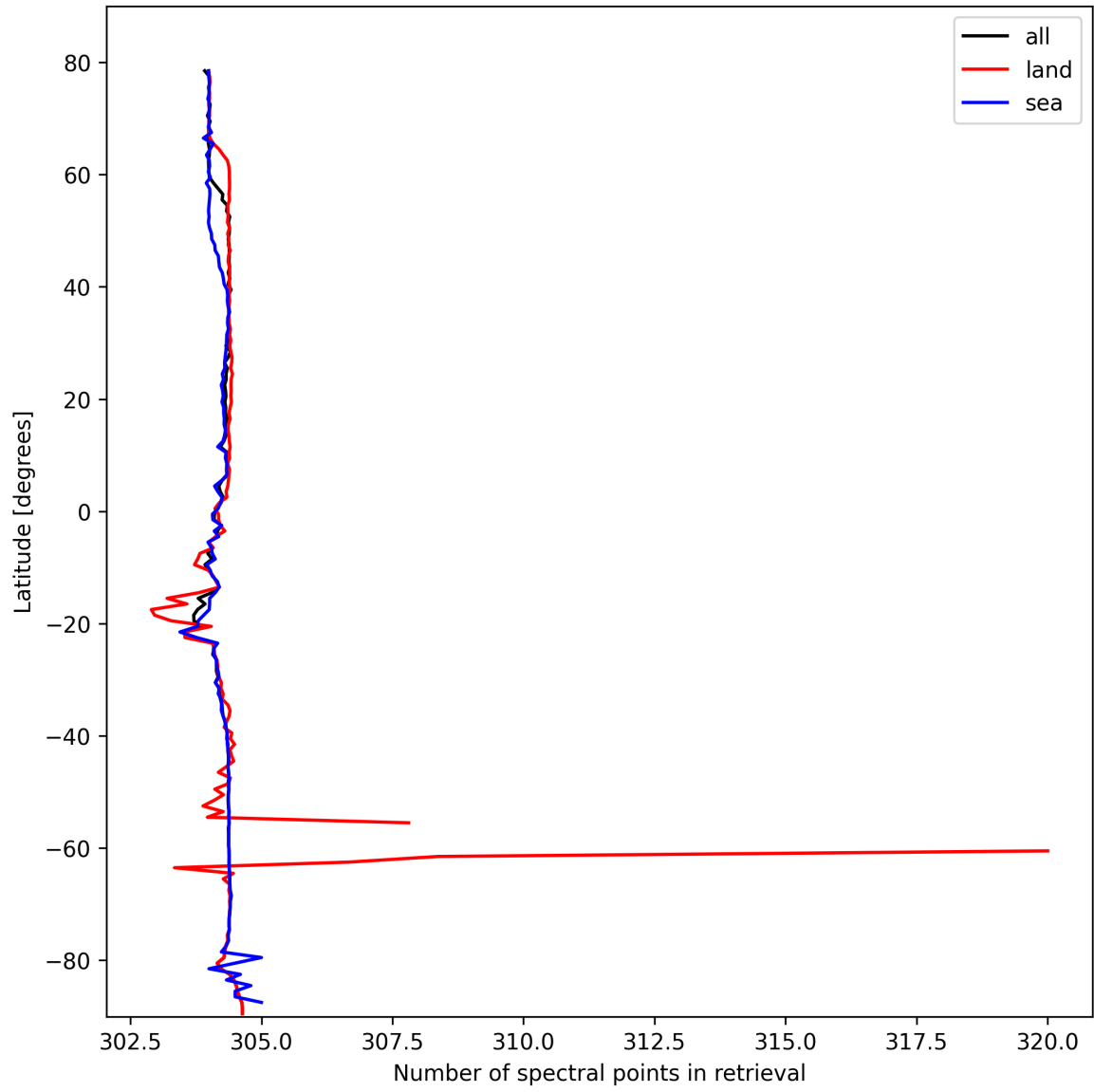
Figure 14: Zonal average of “Number of spectral points in retrieval” for 2025-02-24 to 2025-02-25.
