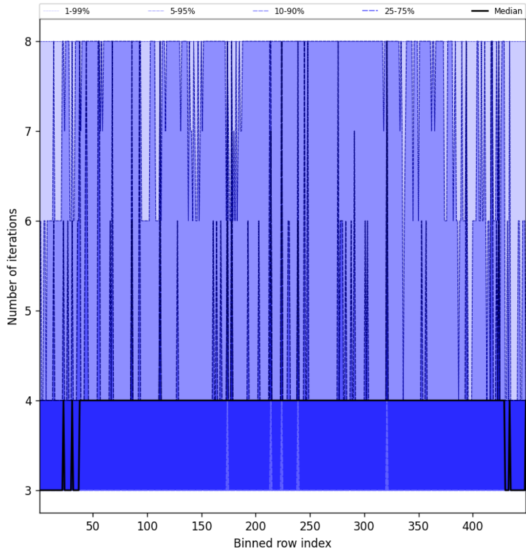
Figure 49: Along track statistics of “Number of iterations” for 2025-02-24 to 2025-02-25
