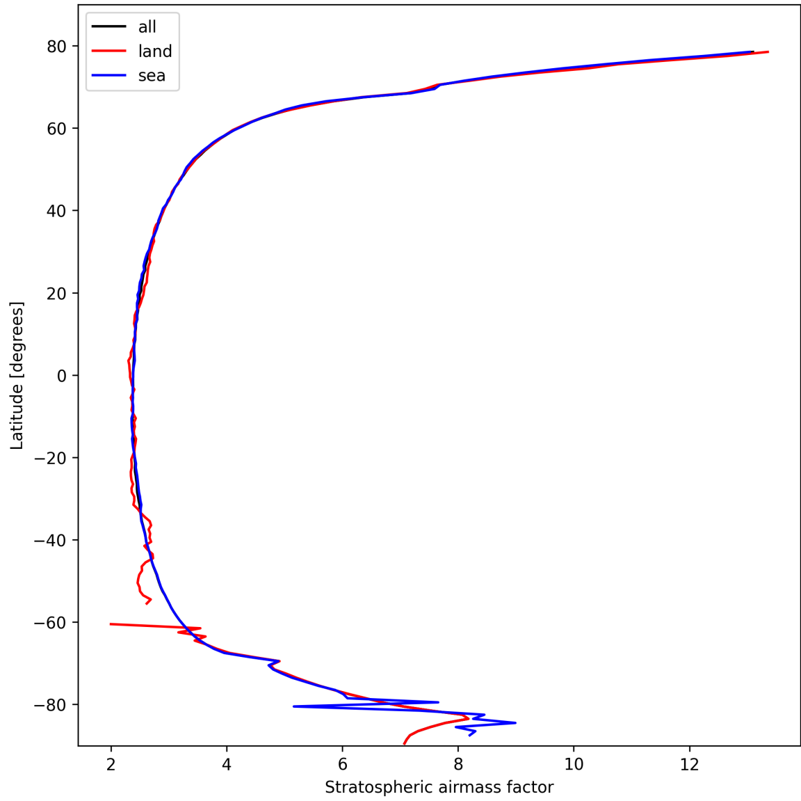
Figure 25: Zonal average of “Stratospheric airmass factor” for 2025-02-24 to 2025-02-25.
