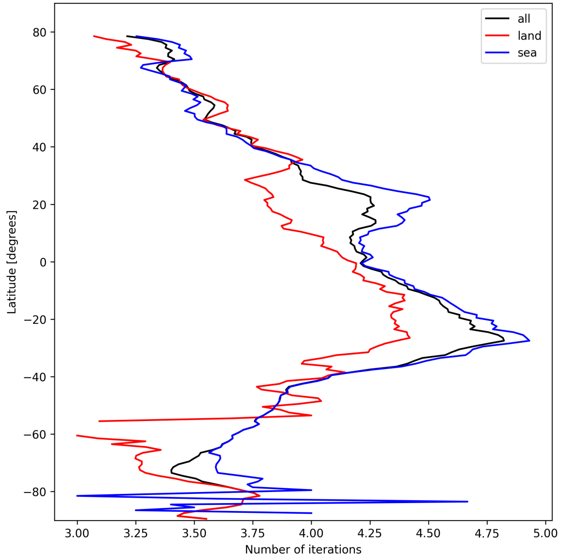
Figure 15: Zonal average of “Number of iterations” for 2025-02-24 to 2025-02-25.
