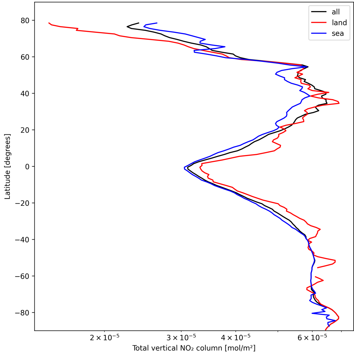
Figure 19: Zonal average of “Total vertical NO 2 column” for 2025-02-24 to 2025-02-25.
