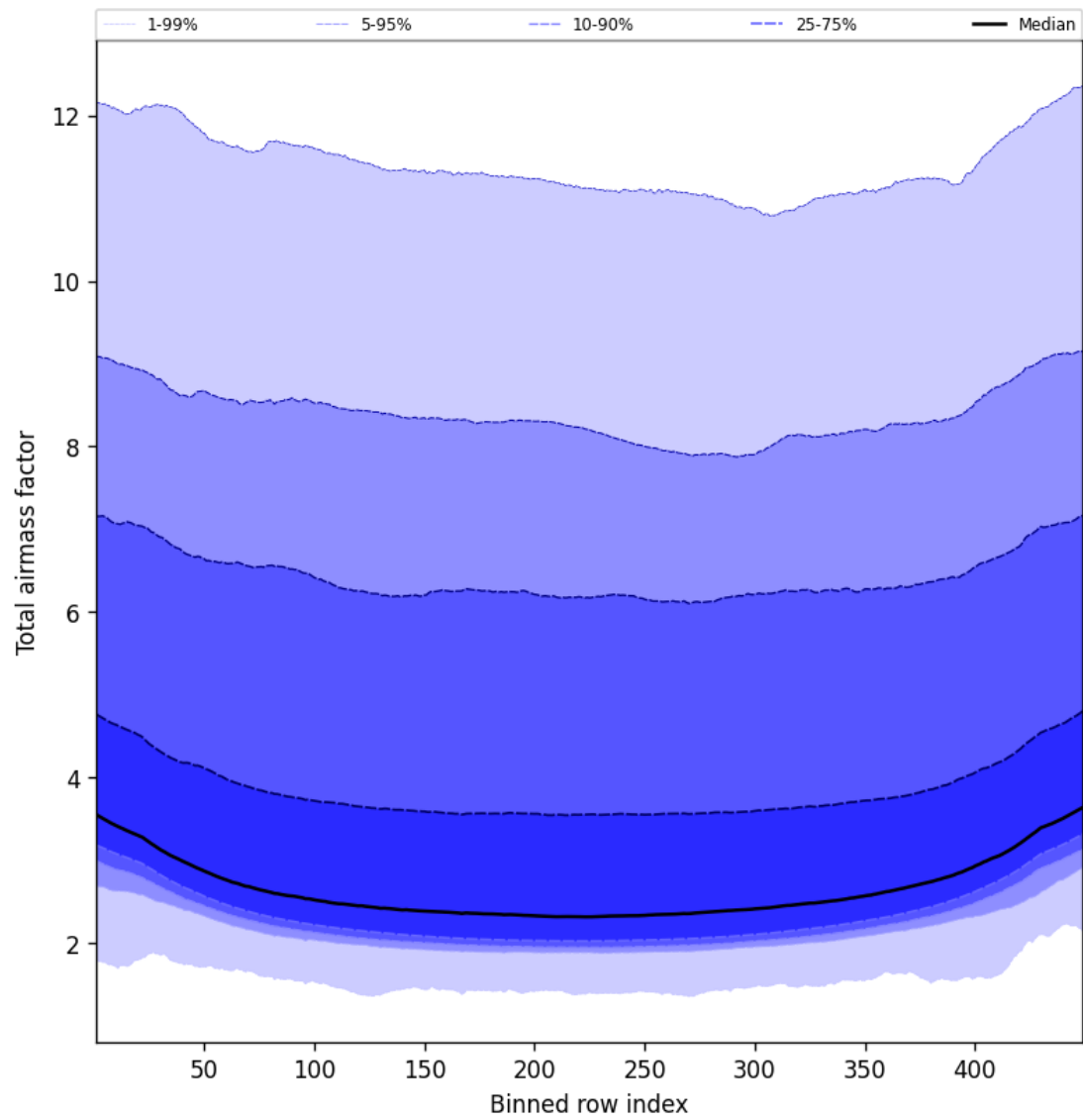
Figure 47: Along track statistics of “Total airmass factor” for 2025-02-24 to 2025-02-25
