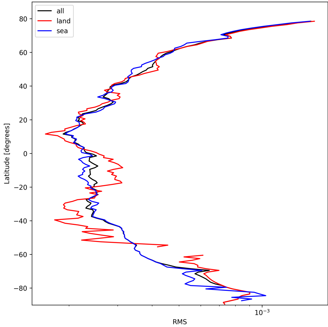
Figure 24: Zonal average of “RMS” for 2025-02-24 to 2025-02-25.
