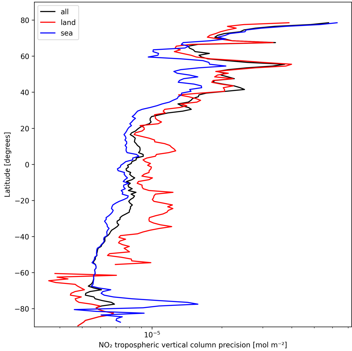
Figure 11: Zonal average of “NO 2 tropospheric vertical column precision” for 2025-02-24 to 2025-02-25.
