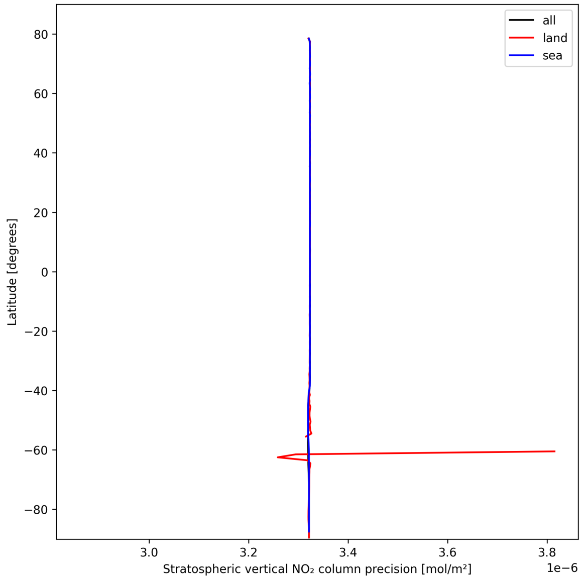
Figure 18: Zonal average of “Stratospheric vertical NO 2 column precision” for 2025-02-24 to 2025-02-25.
