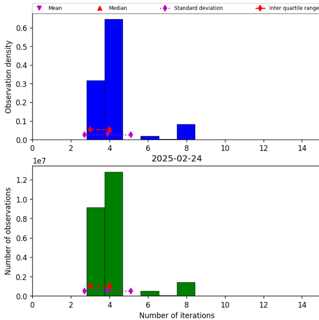
Figure 32: Histogram of “Number of iterations” for 2025-02-24 to 2025-02-25
