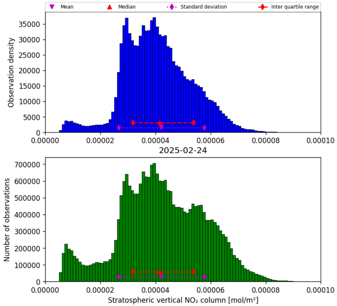
Figure 34: Histogram of “Stratospheric vertical NO 2 column” for 2025-02-24 to 2025-02-25
