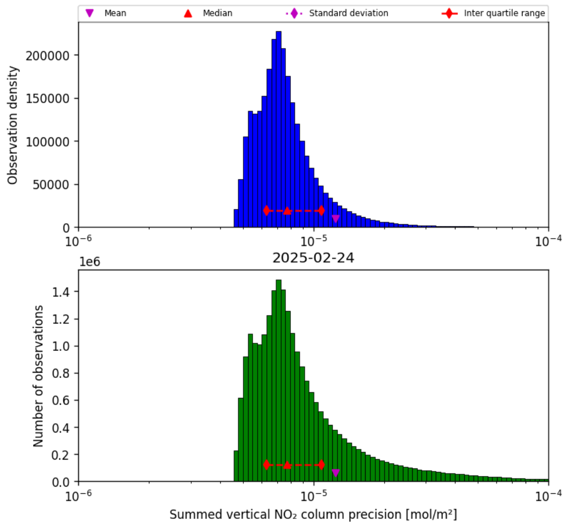
Figure 39: Histogram of “Summed vertical NO 2 column precision” for 2025-02-24 to 2025-02-25
