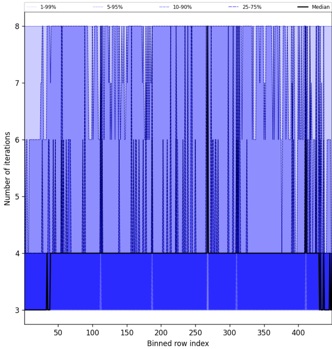
Figure 49: Along track statistics of “Number of iterations” for 2025-02-25 to 2025-02-26
