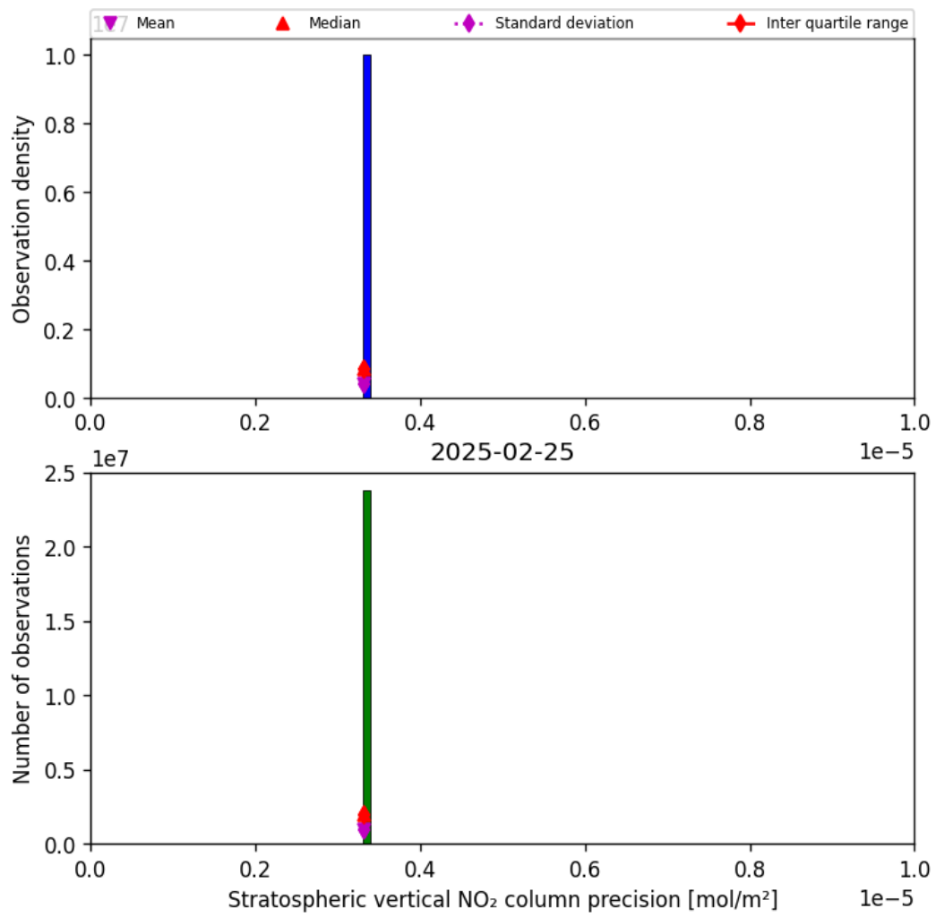
Figure 35: Histogram of “Stratospheric vertical NO 2 column precision” for 2025-02-25 to 2025-02-26
