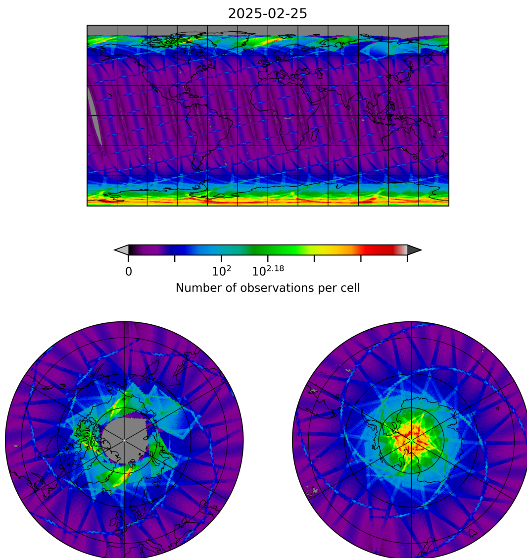
Figure 8: Map of the number of observations for 2025-02-25 to 2025-02-26
