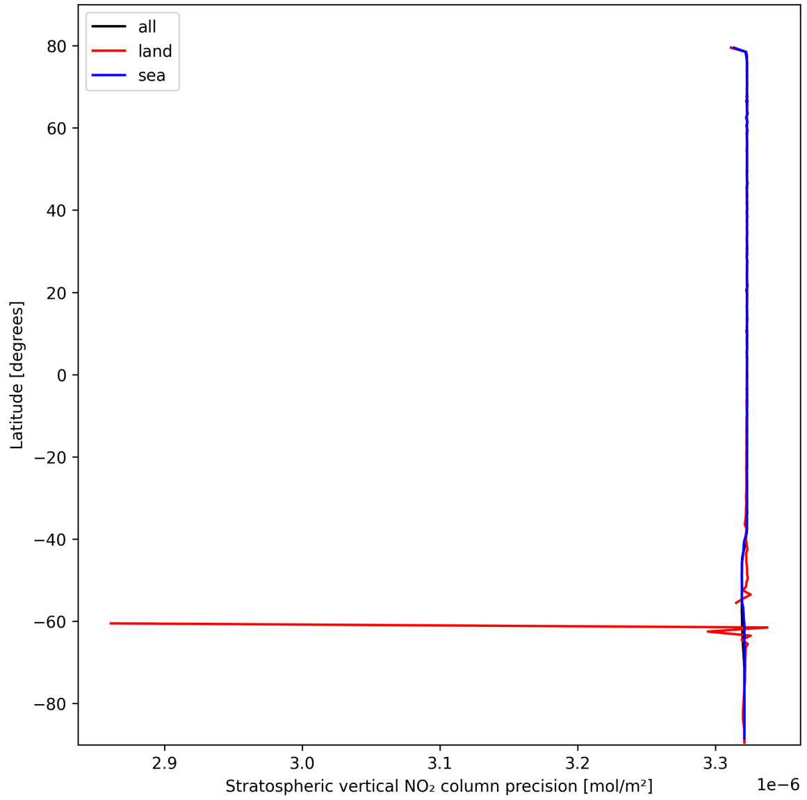
Figure 18: Zonal average of “Stratospheric vertical NO 2 column precision” for 2025-02-25 to 2025-02-26.
