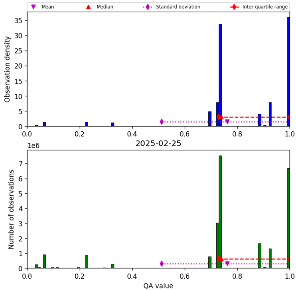
Figure 26: Histogram of “QA value” for 2025-02-25 to 2025-02-26
