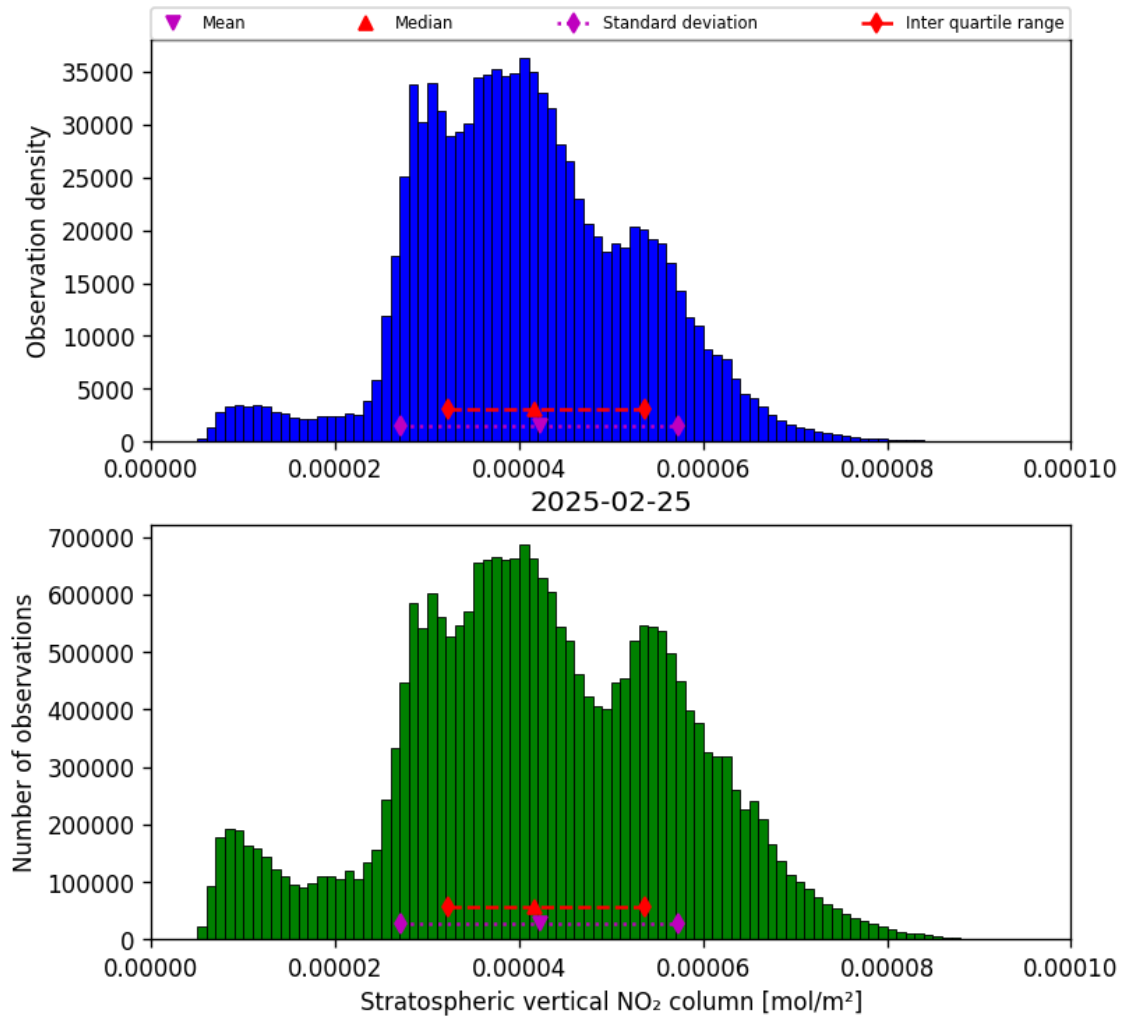
Figure 34: Histogram of “Stratospheric vertical NO 2 column” for 2025-02-25 to 2025-02-26
