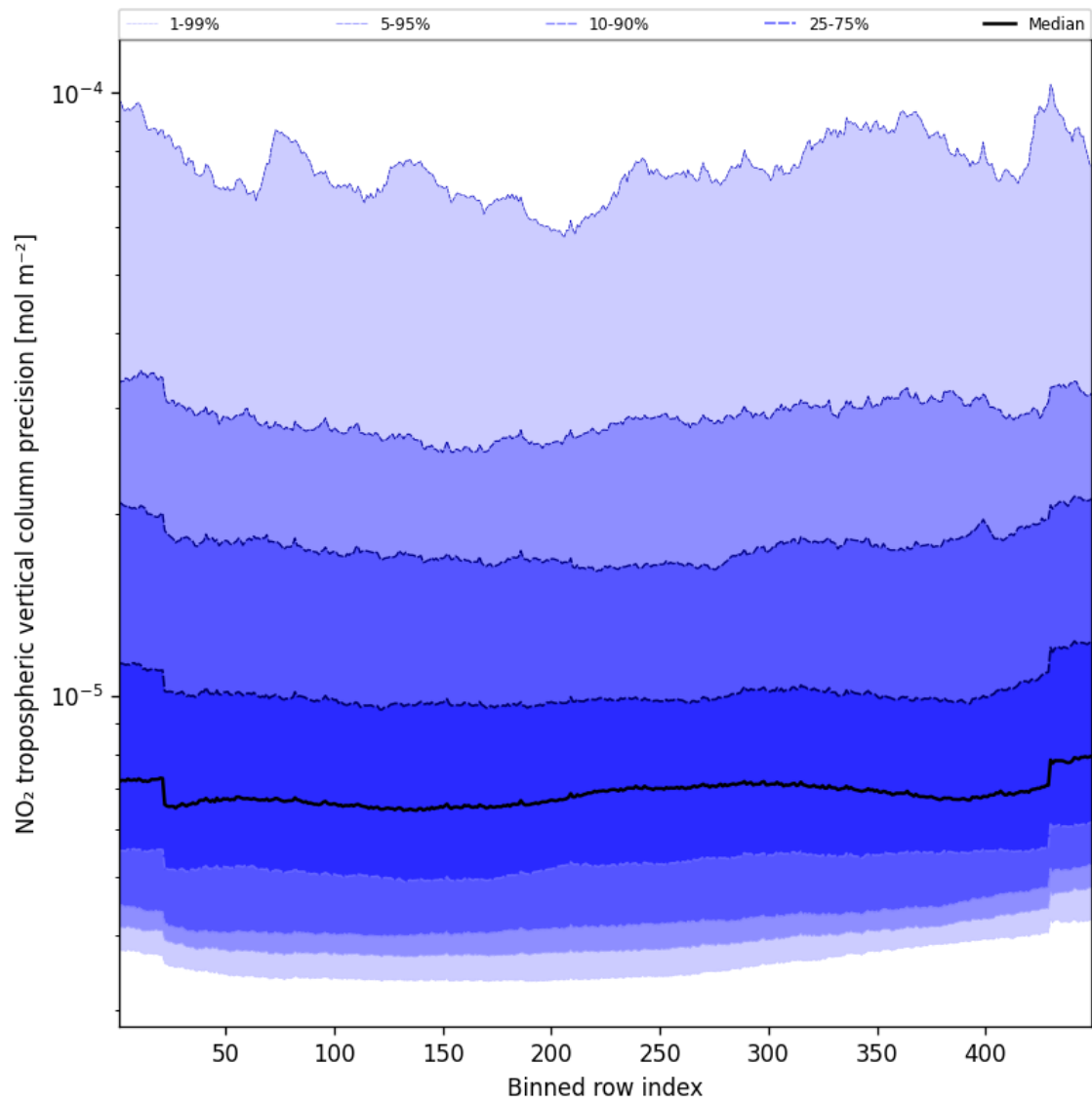
Figure 45: Along track statistics of “NO 2 tropospheric vertical column precision” for 2025-02-25 to 2025-02-26
