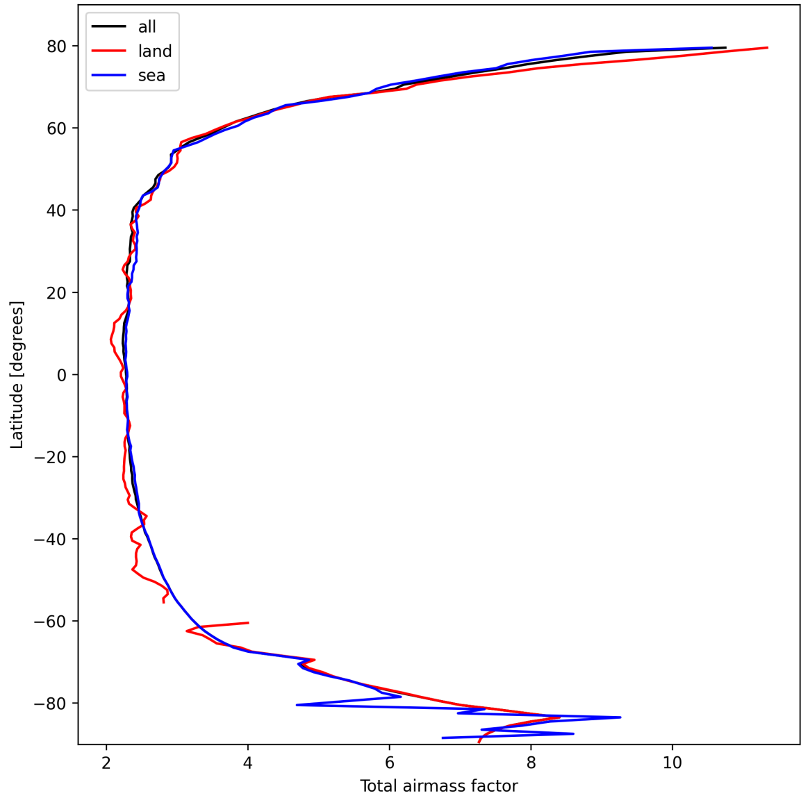
Figure 13: Zonal average of “Total airmass factor” for 2025-02-25 to 2025-02-26.
