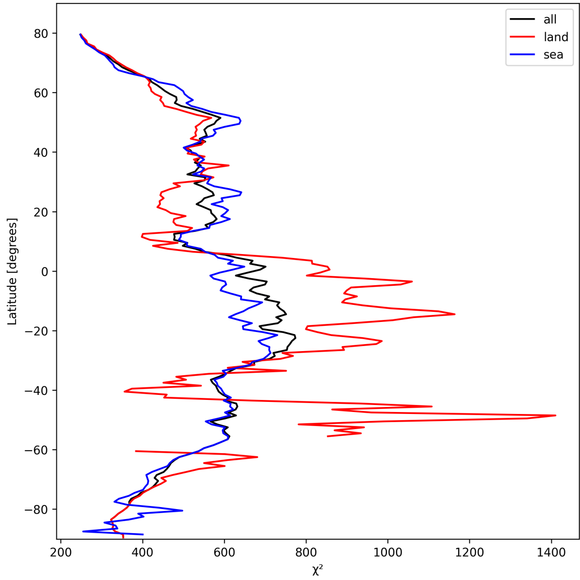
Figure 23: Zonal average of “ \chi^2 ” for 2025-02-25 to 2025-02-26.
