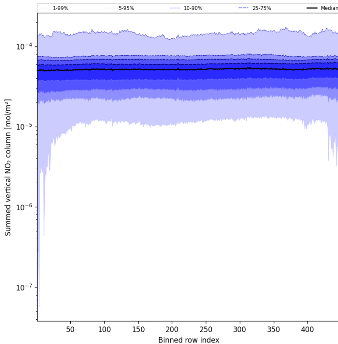
Figure 55: Along track statistics of “Summed vertical NO 2 column” for 2025-02-25 to 2025-02-26
