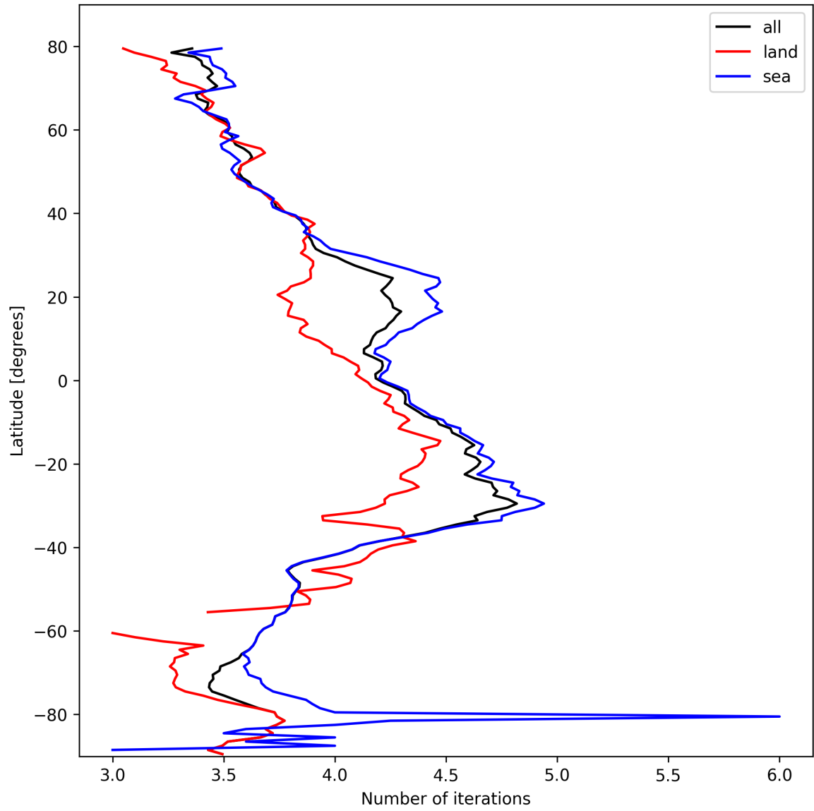
Figure 15: Zonal average of “Number of iterations” for 2025-02-25 to 2025-02-26.
