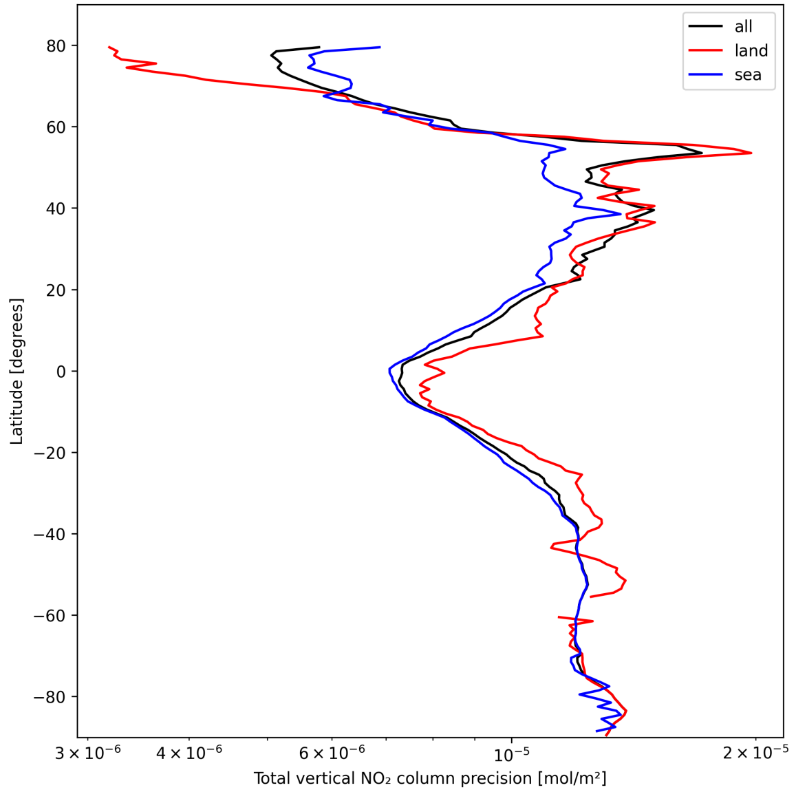
Figure 20: Zonal average of “Total vertical NO 2 column precision” for 2025-02-25 to 2025-02-26.
