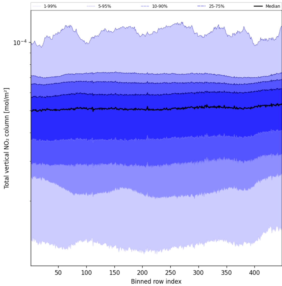
Figure 53: Along track statistics of “Total vertical NO 2 column” for 2025-02-25 to 2025-02-26
