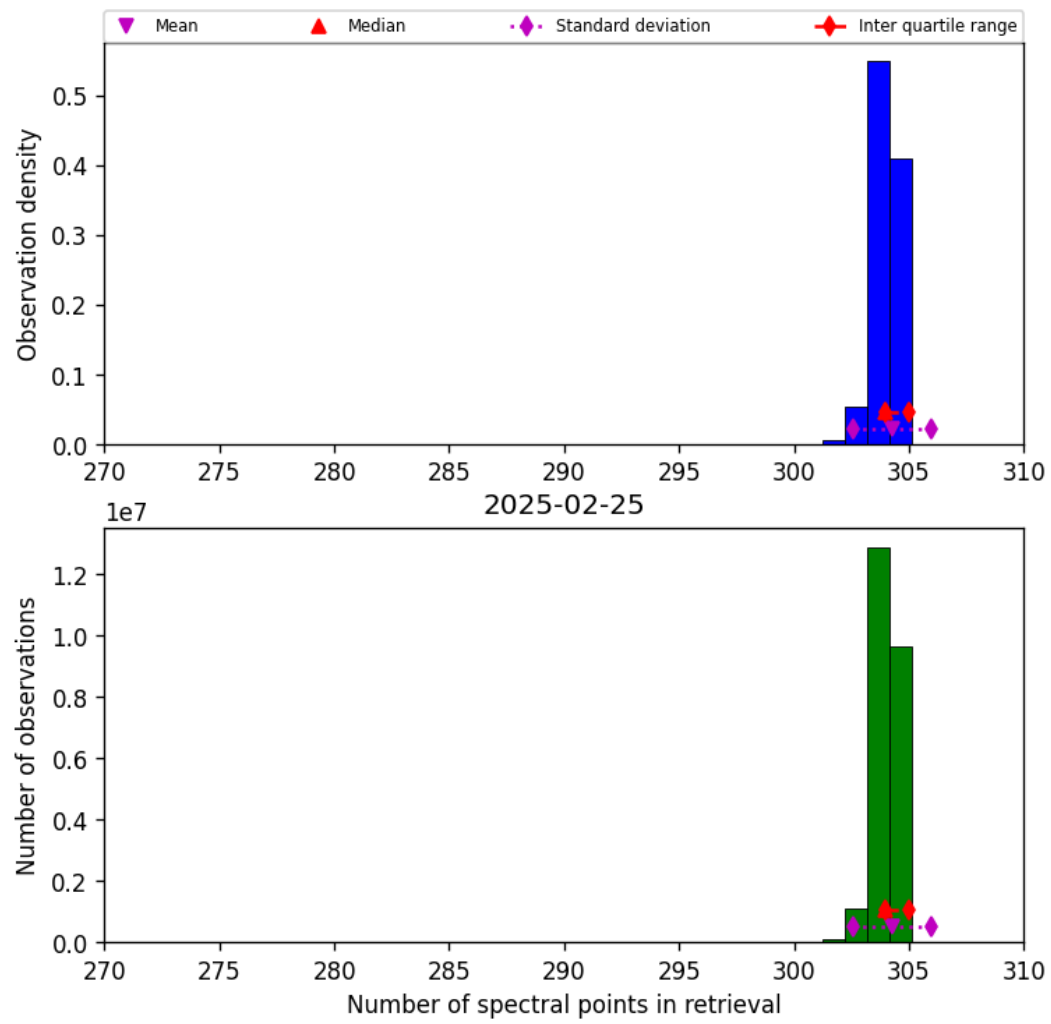
Figure 31: Histogram of “Number of spectral points in retrieval” for 2025-02-25 to 2025-02-26
