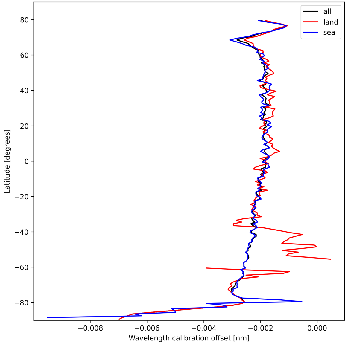
Figure 16: Zonal average of “Wavelength calibration offset” for 2025-02-25 to 2025-02-26.
