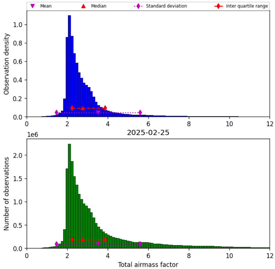
Figure 30: Histogram of “Total airmass factor” for 2025-02-25 to 2025-02-26
