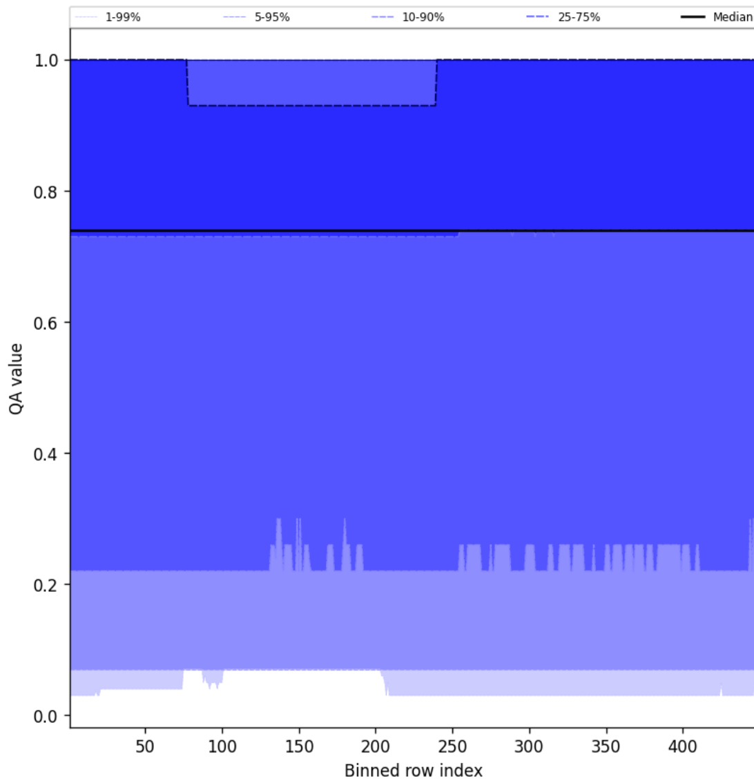
Figure 43: Along track statistics of “QA value” for 2025-02-25 to 2025-02-26
