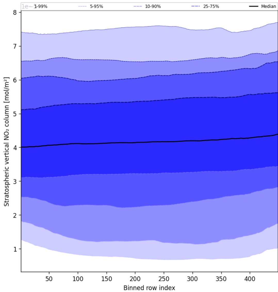
Figure 51: Along track statistics of “Stratospheric vertical NO 2 column” for 2025-02-25 to 2025-02-26
