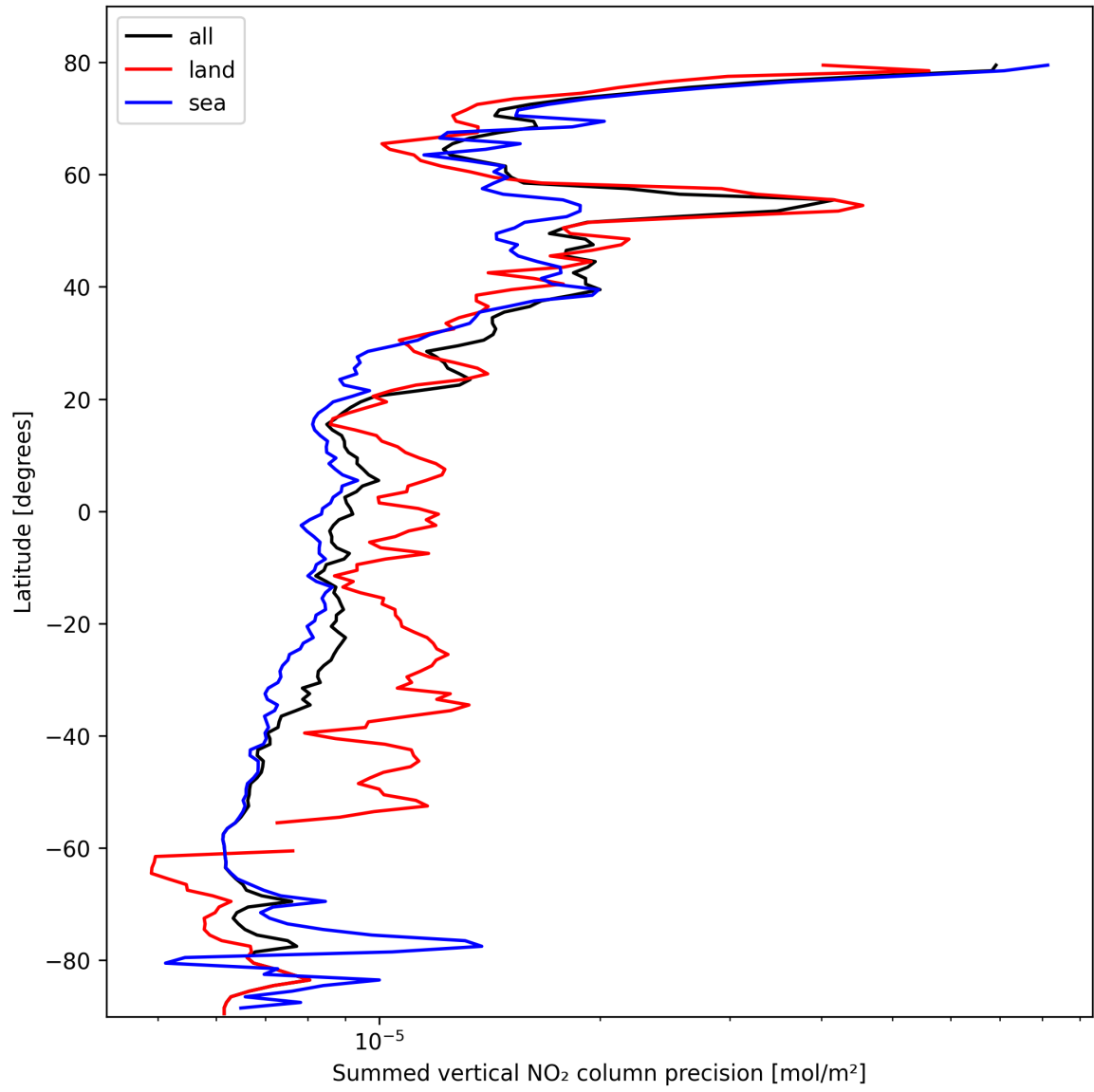
Figure 22: Zonal average of “Summed vertical NO 2 column precision” for 2025-02-25 to 2025-02-26.
