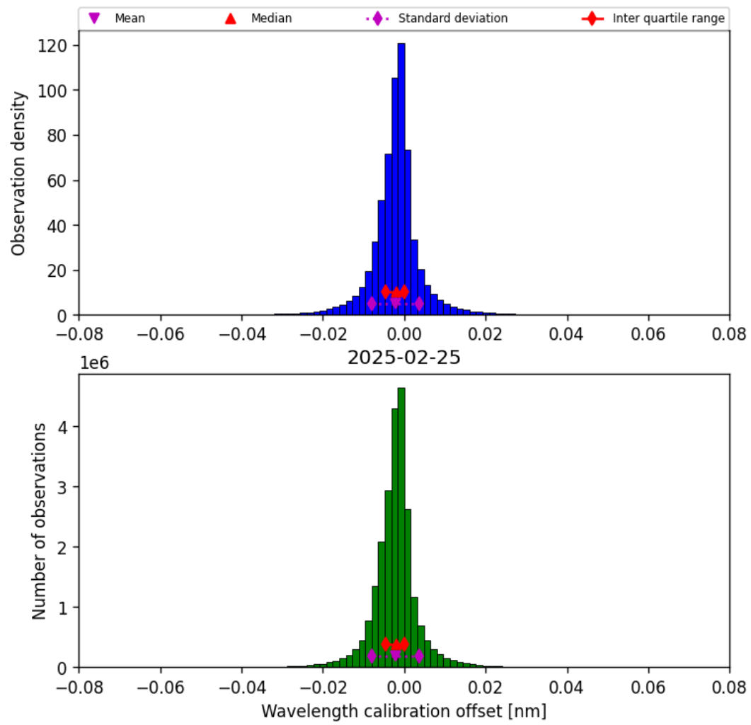
Figure 33: Histogram of “Wavelength calibration offset” for 2025-02-25 to 2025-02-26
