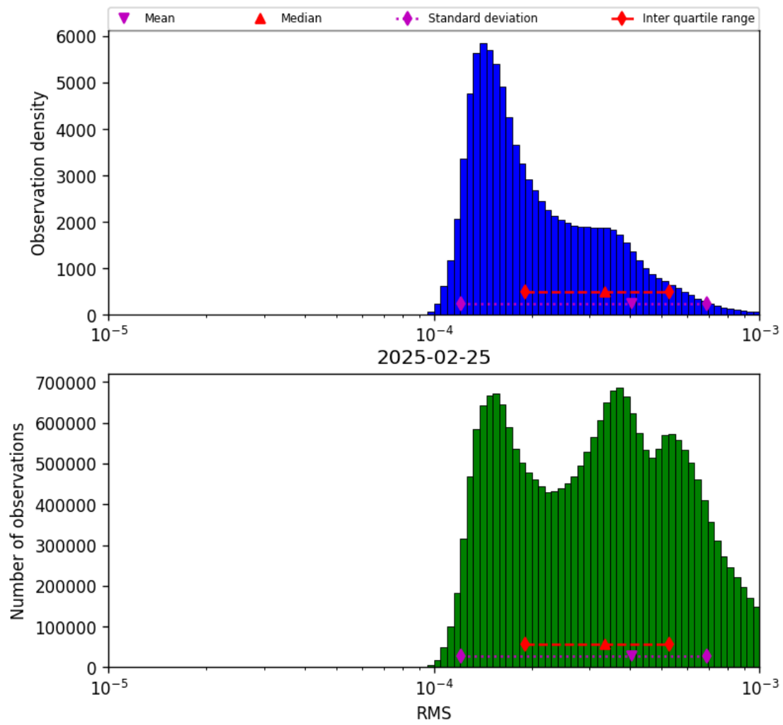
Figure 41: Histogram of “RMS” for 2025-02-25 to 2025-02-26
