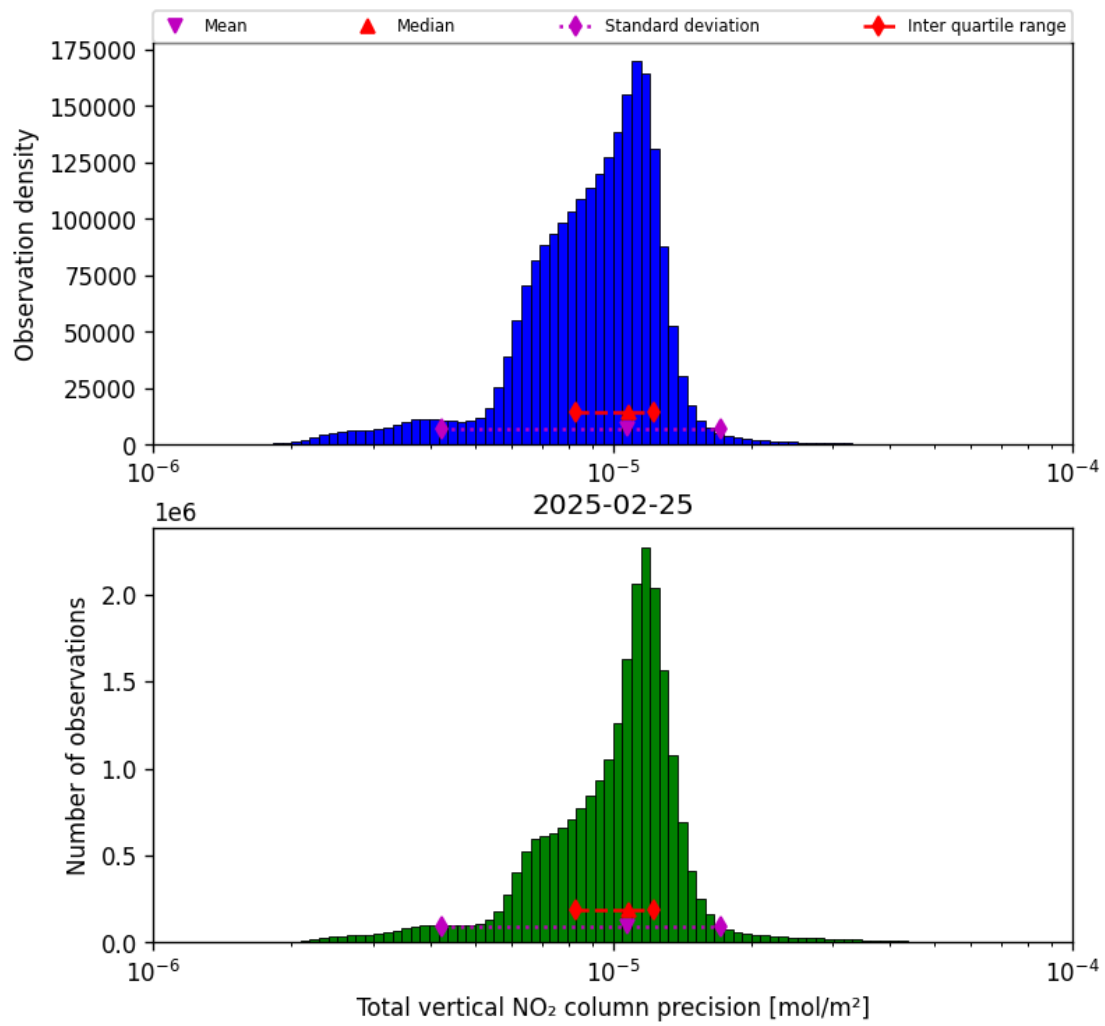
Figure 37: Histogram of “Total vertical NO 2 column precision” for 2025-02-25 to 2025-02-26
