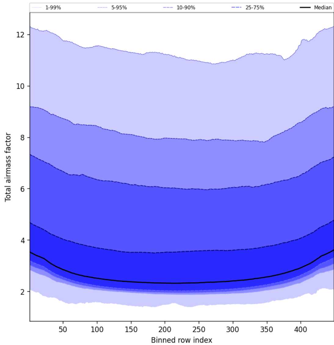
Figure 47: Along track statistics of “Total airmass factor” for 2025-02-25 to 2025-02-26
