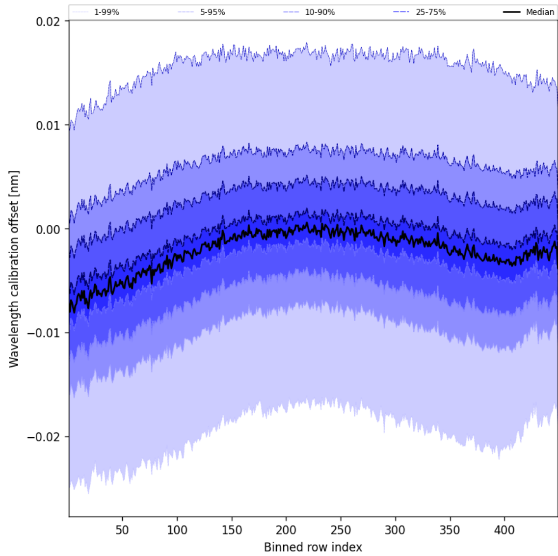
Figure 50: Along track statistics of “Wavelength calibration offset” for 2025-02-25 to 2025-02-26
