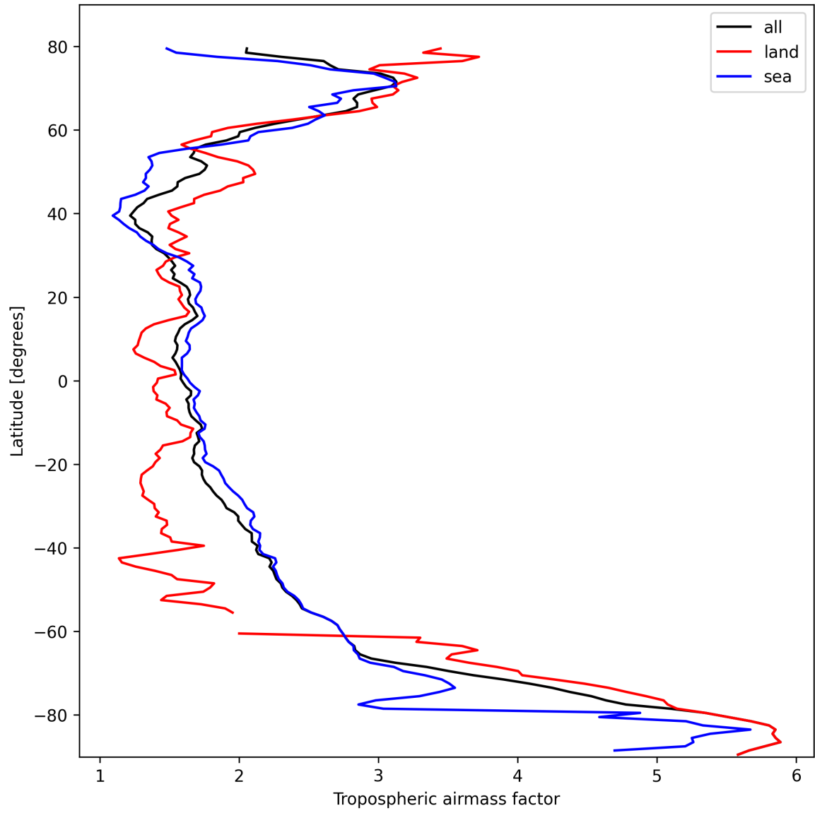
Figure 12: Zonal average of “Tropospheric airmass factor” for 2025-02-25 to 2025-02-26.
