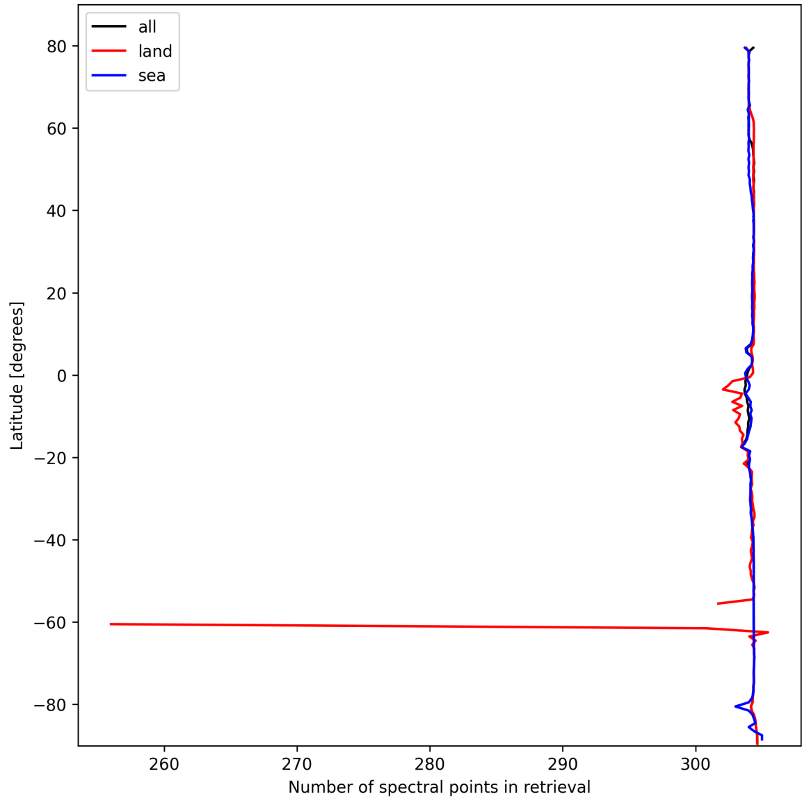
Figure 14: Zonal average of “Number of spectral points in retrieval” for 2025-02-25 to 2025-02-26.
