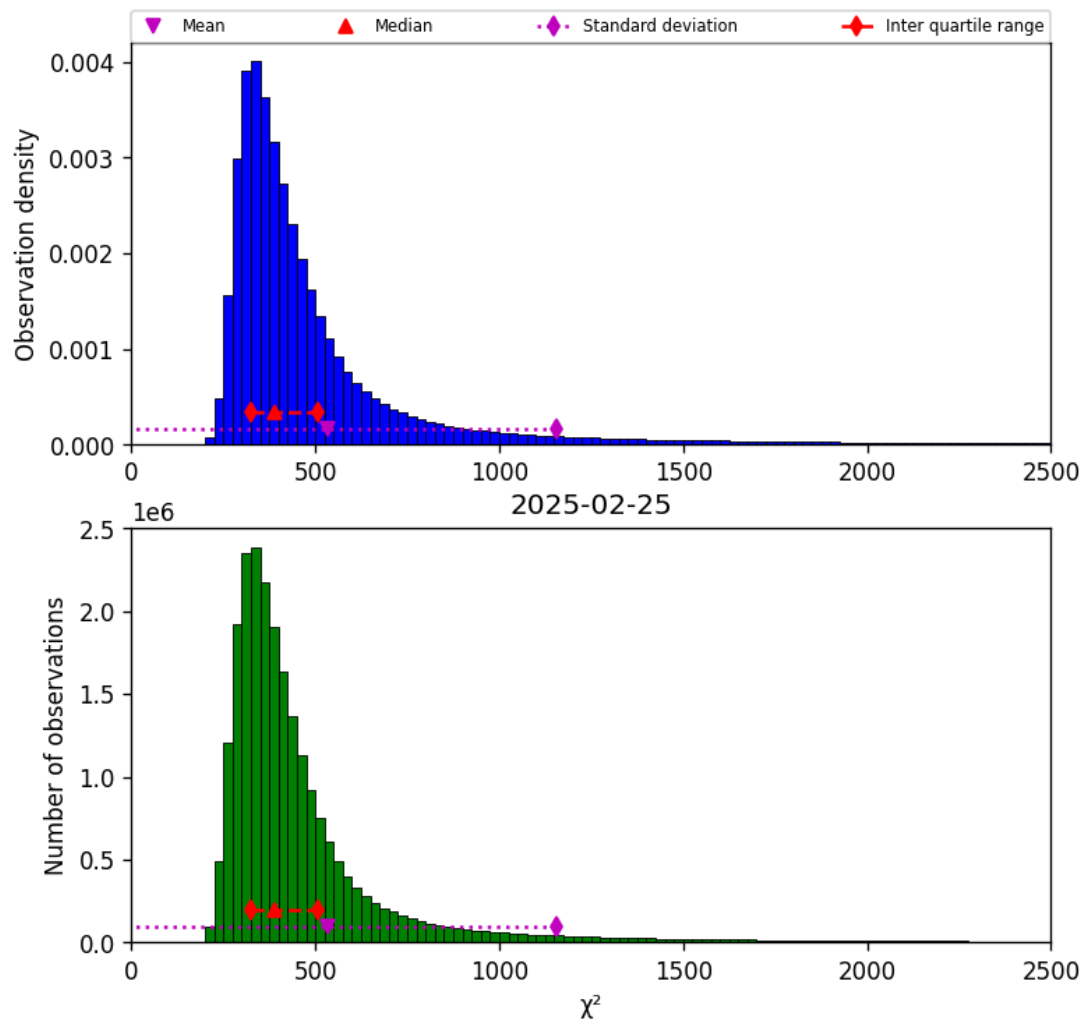
Figure 40: Histogram of “ \chi^2 ” for 2025-02-25 to 2025-02-26
