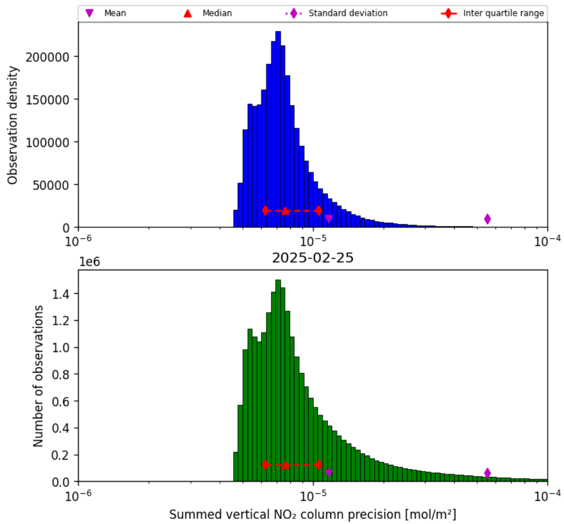
Figure 39: Histogram of "Summed vertical NO 2 column precision" for 2025-02-25 to 2025-02-26
