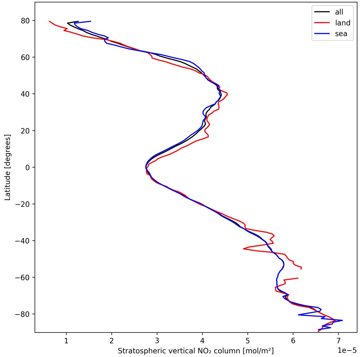
Figure 17: Zonal average of “Stratospheric vertical NO 2 column” for 2025-02-25 to 2025-02-26.
