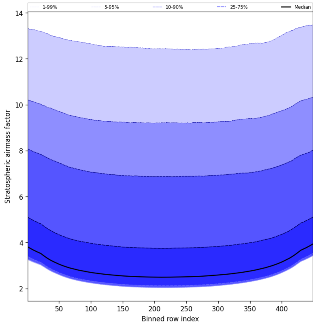
Figure 59: Along track statistics of “Stratospheric airmass factor” for 2025-02-25 to 2025-02-26
