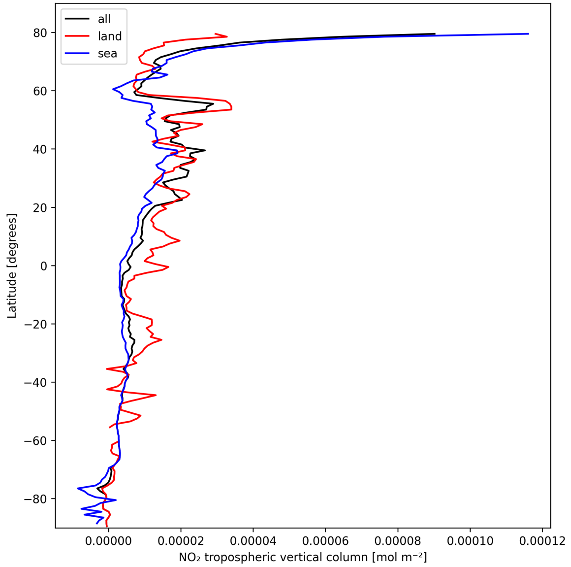
Figure 10: Zonal average of “NO 2 tropospheric vertical column” for 2025-02-25 to 2025-02-26.
