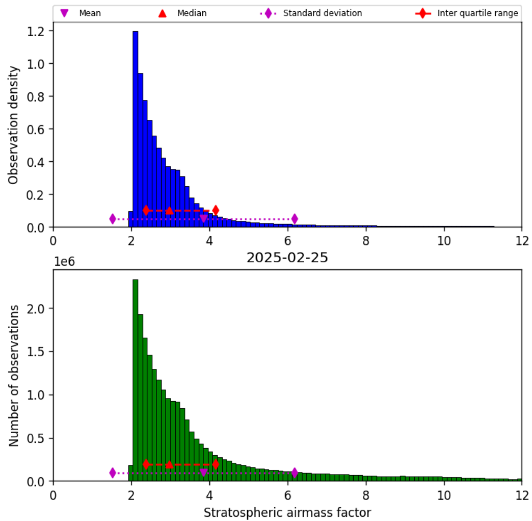
Figure 42: Histogram of “Stratospheric airmass factor” for 2025-02-25 to 2025-02-26
