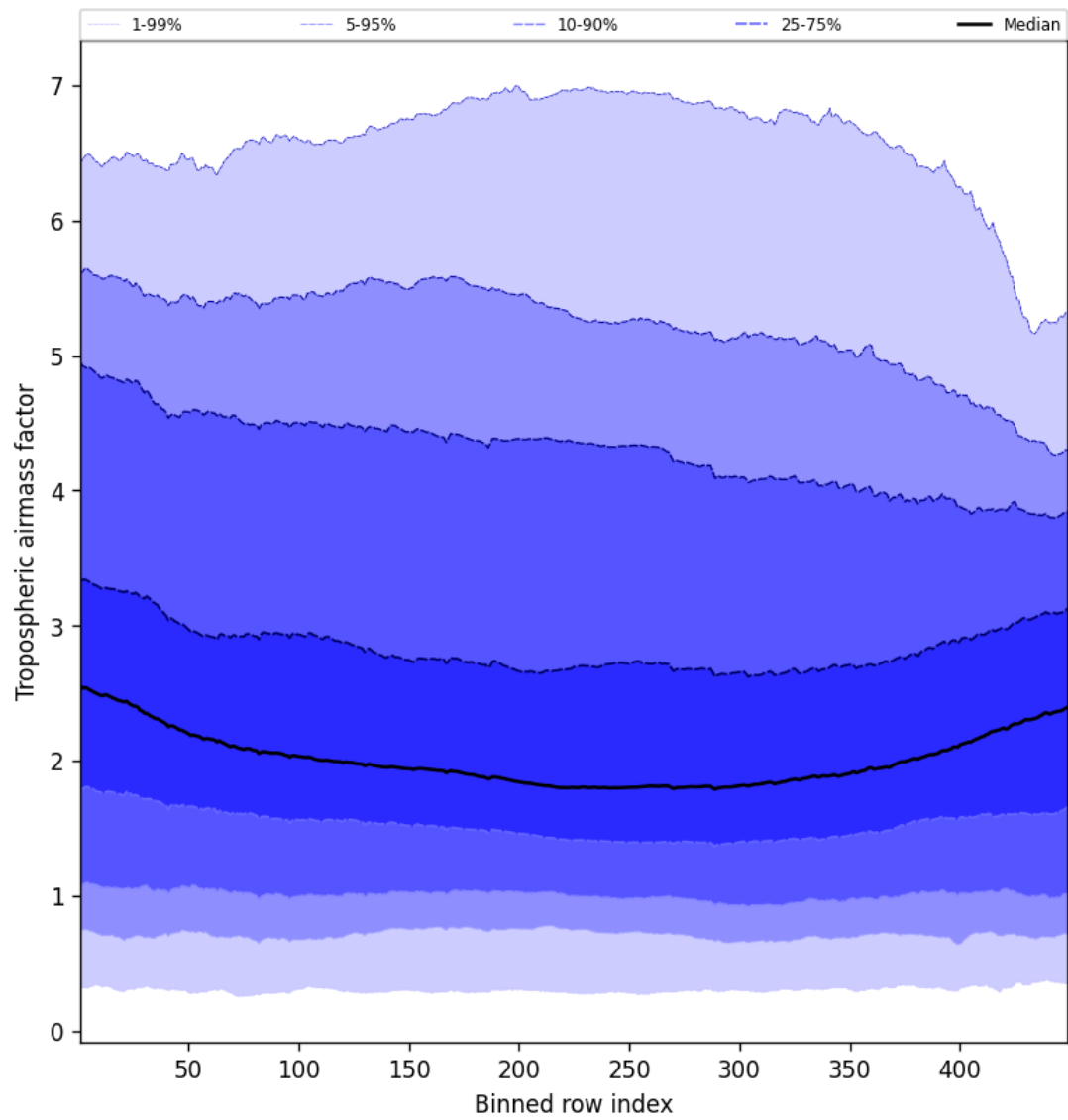
Figure 46: Along track statistics of “Tropospheric airmass factor” for 2025-02-25 to 2025-02-26
