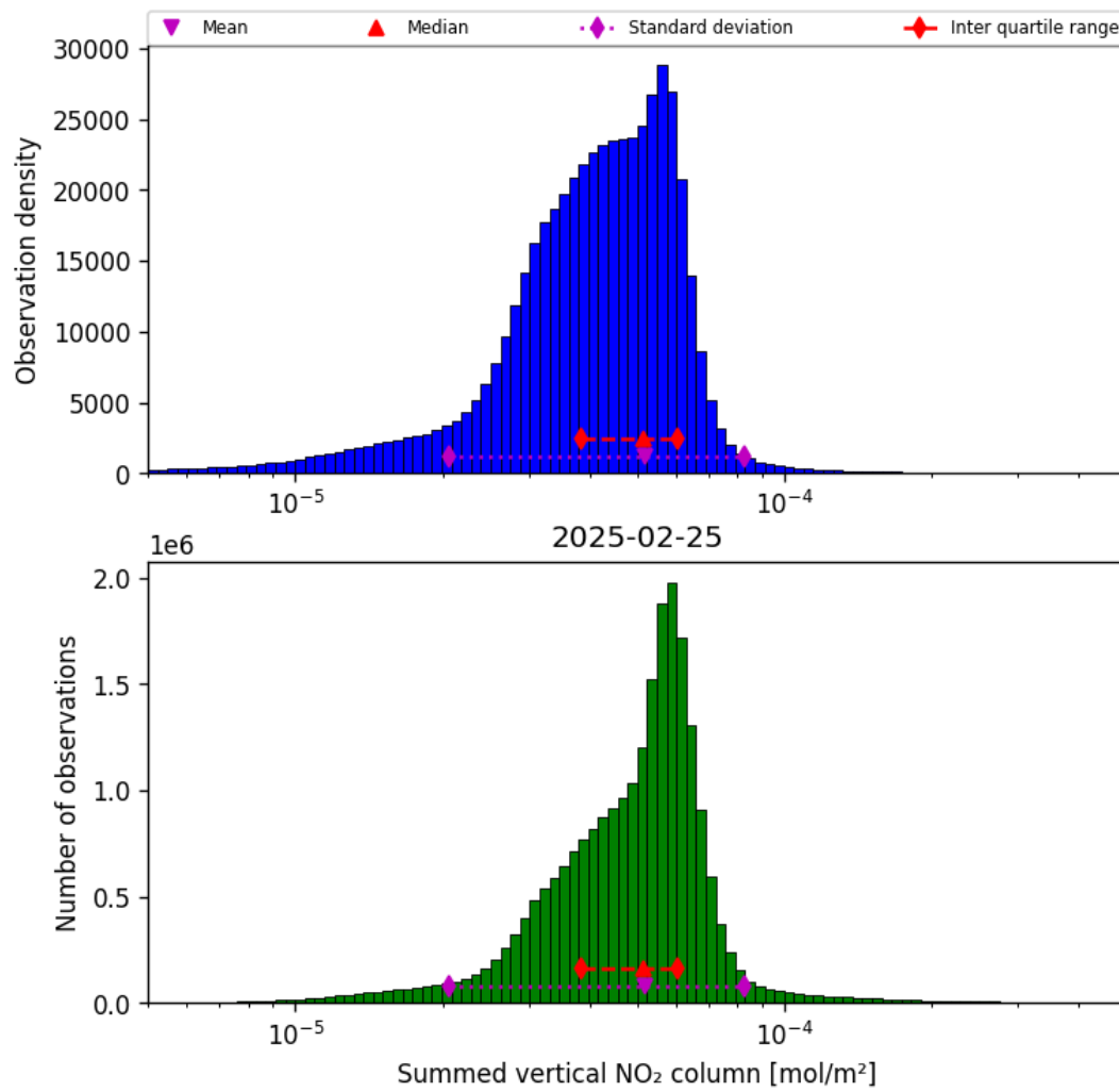
Figure 38: Histogram of "Summed vertical NO 2 column" for 2025-02-25 to 2025-02-26
