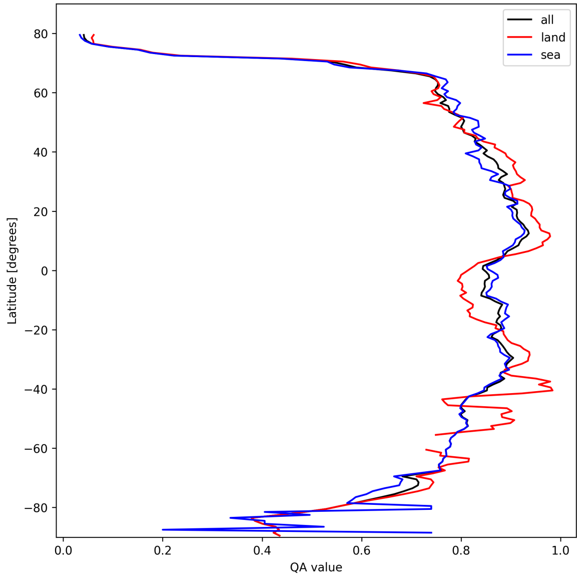
Figure 9: Zonal average of “QA value” for 2025-02-25 to 2025-02-26.
