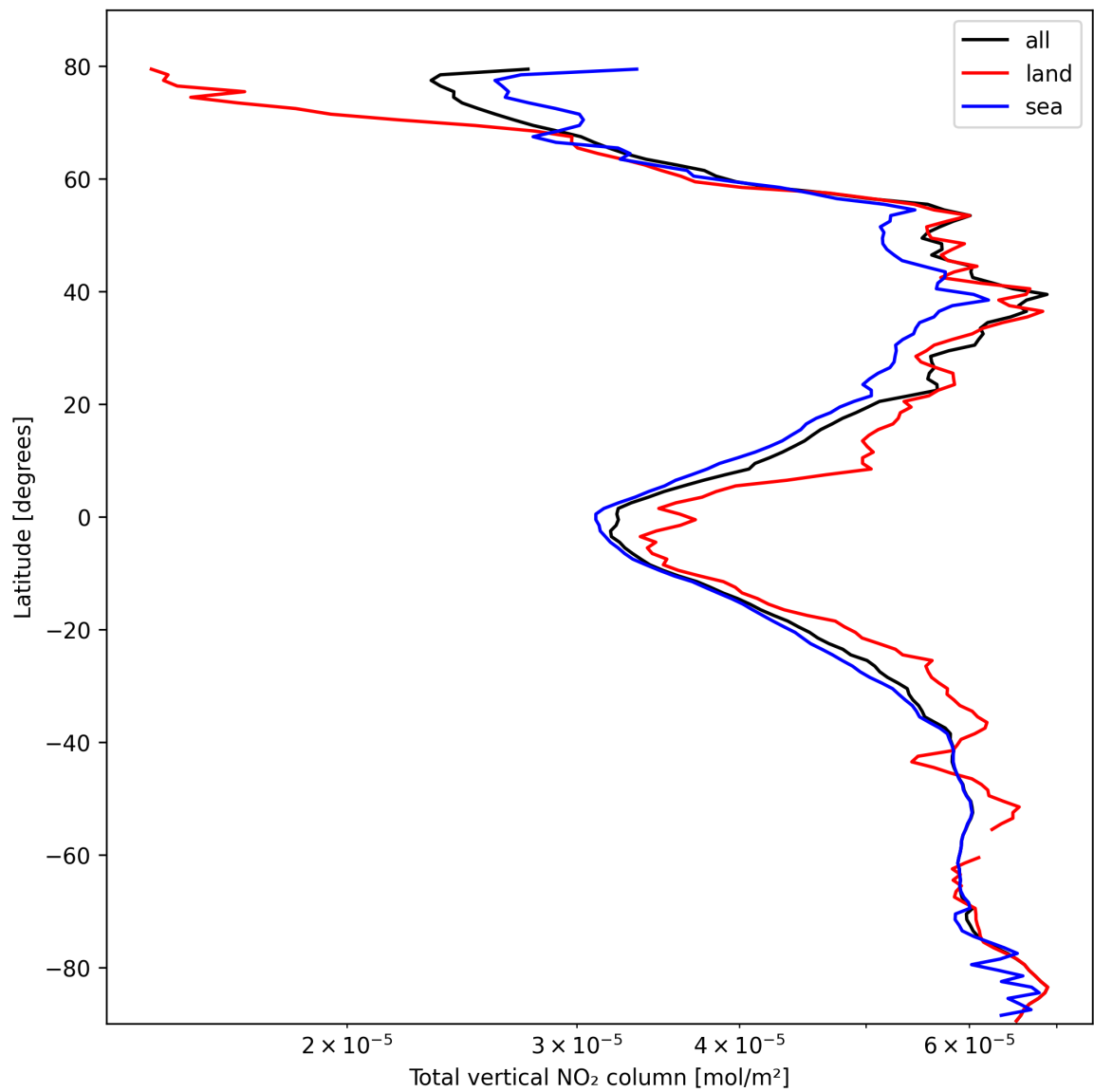
Figure 19: Zonal average of “Total vertical NO 2 column” for 2025-02-25 to 2025-02-26.
