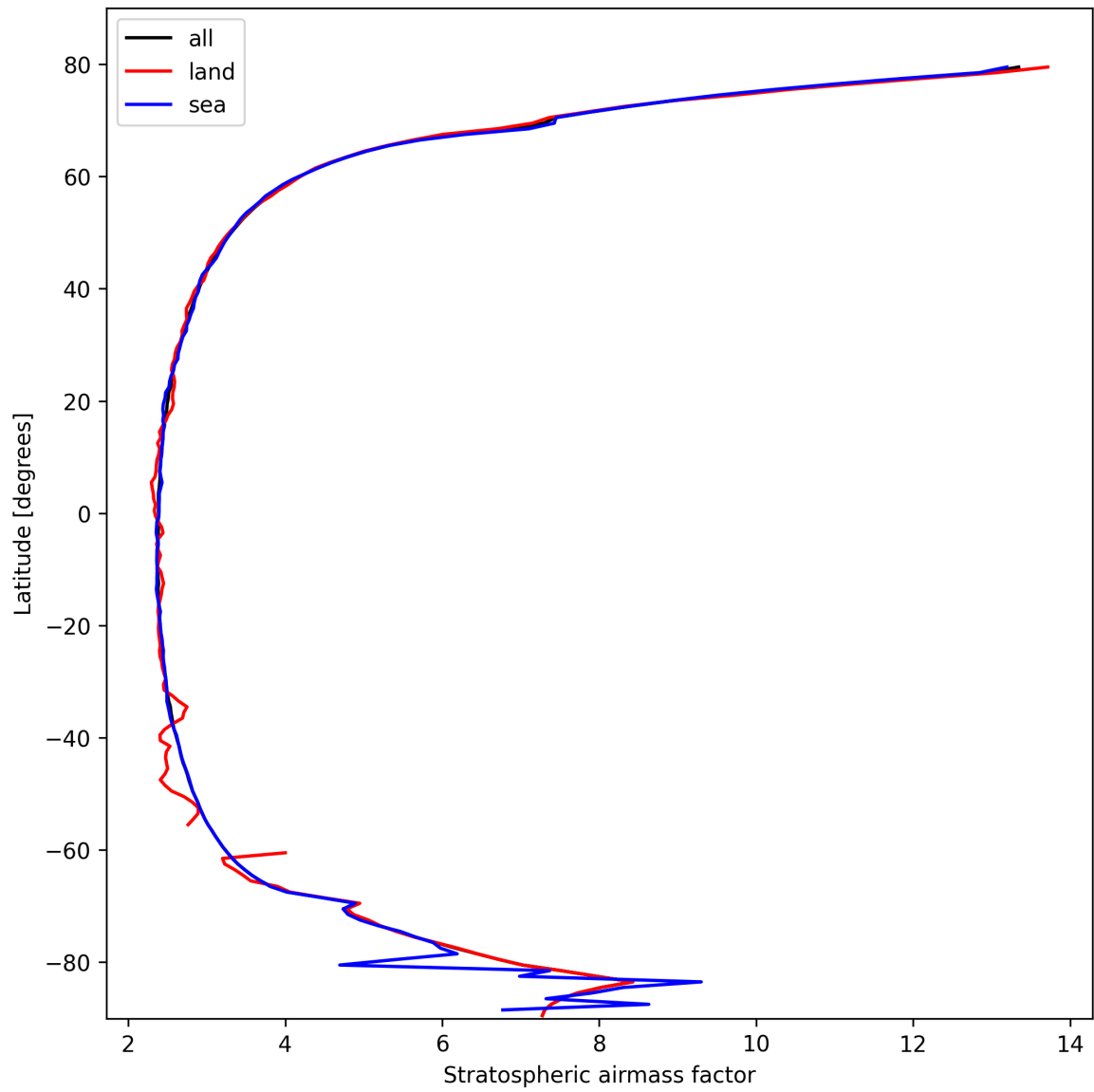
Figure 25: Zonal average of “Stratospheric air mass factor” for 2025-02-25 to 2025-02-26.
