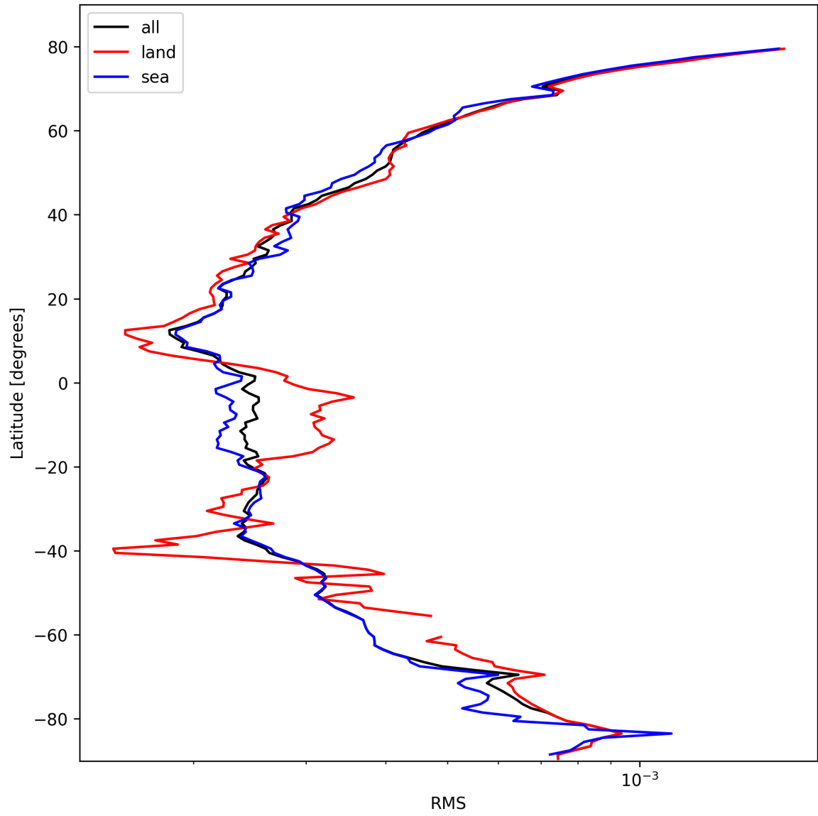
Figure 24: Zonal average of “RMS” for 2025-02-25 to 2025-02-26.
