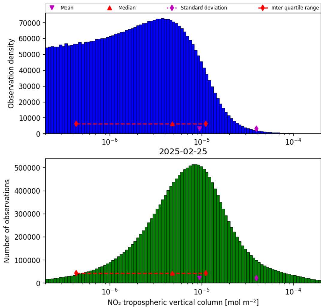
Figure 27: Histogram of “NO 2 tropospheric vertical column” for 2025-02-25 to 2025-02-26
