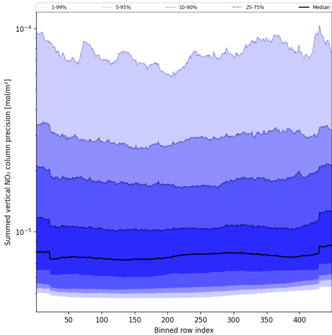
Figure 56: Along track statistics of “Summed vertical NO 2 column precision” for 2025-02-25 to 2025-02-26
