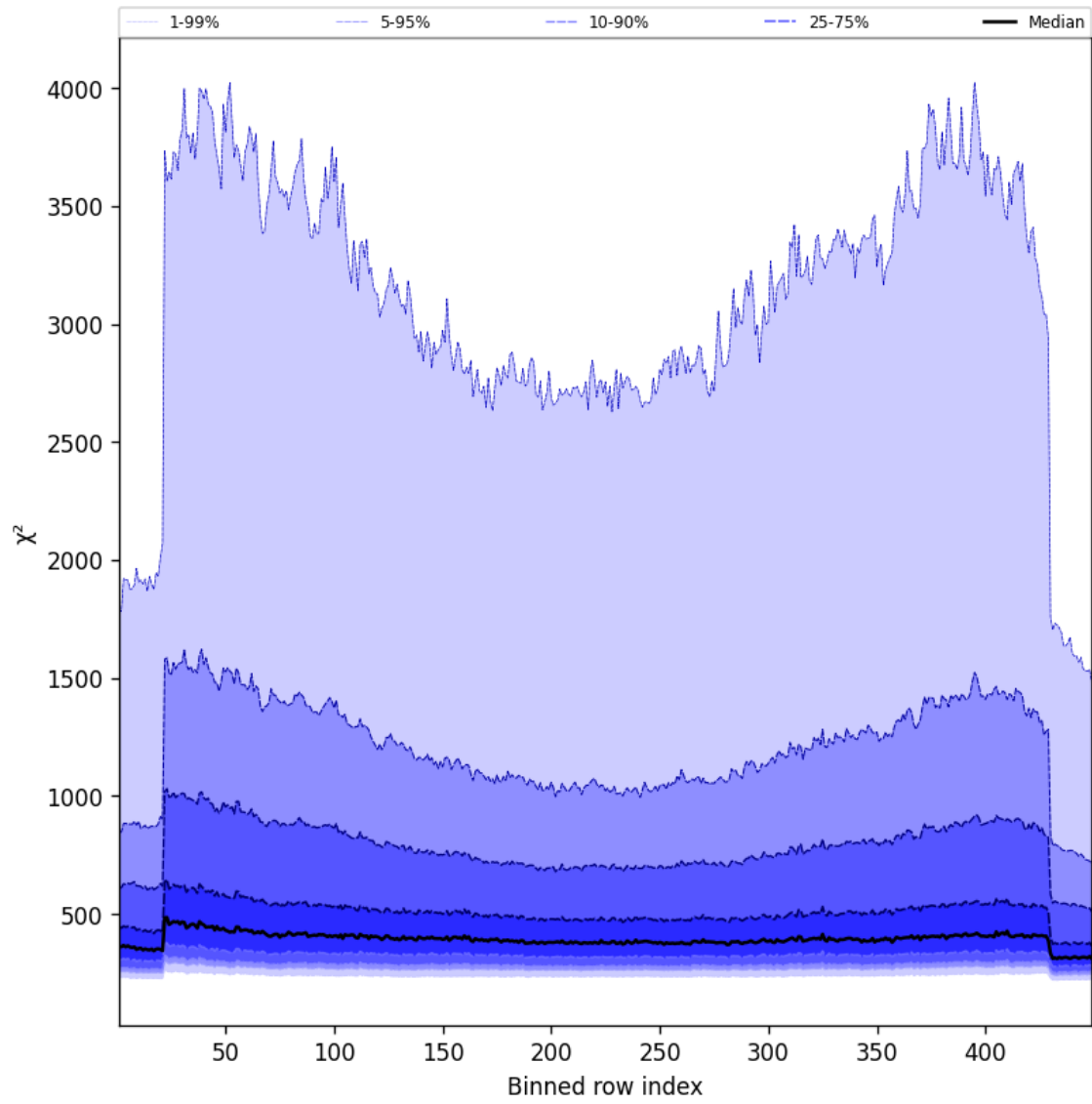
Figure 57: Along track statistics of “ \chi^2 ” for 2025-02-25 to 2025-02-26
