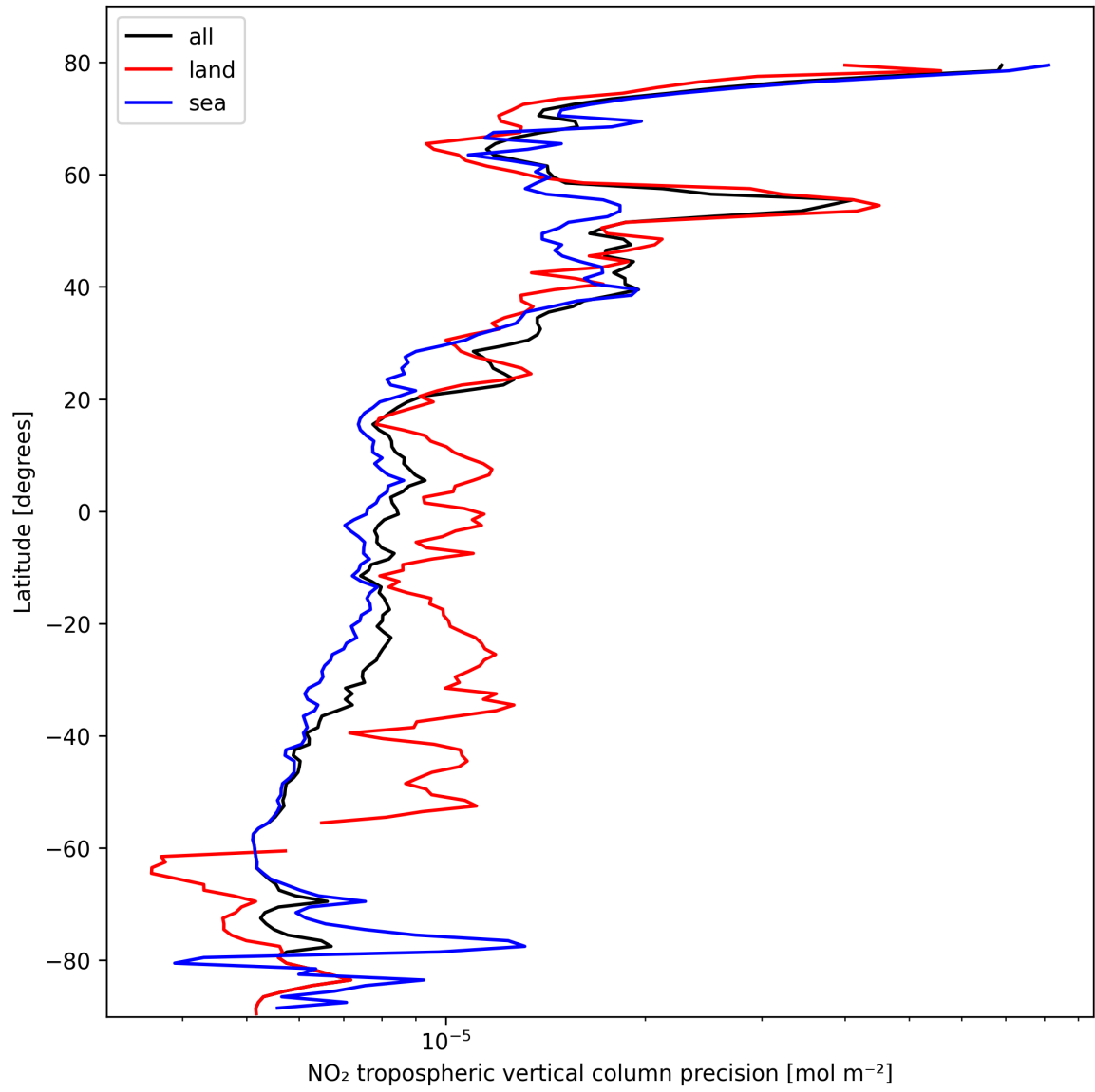
Figure 11: Zonal average of “NO 2 tropospheric vertical column precision” for 2025-02-25 to 2025-02-26.
