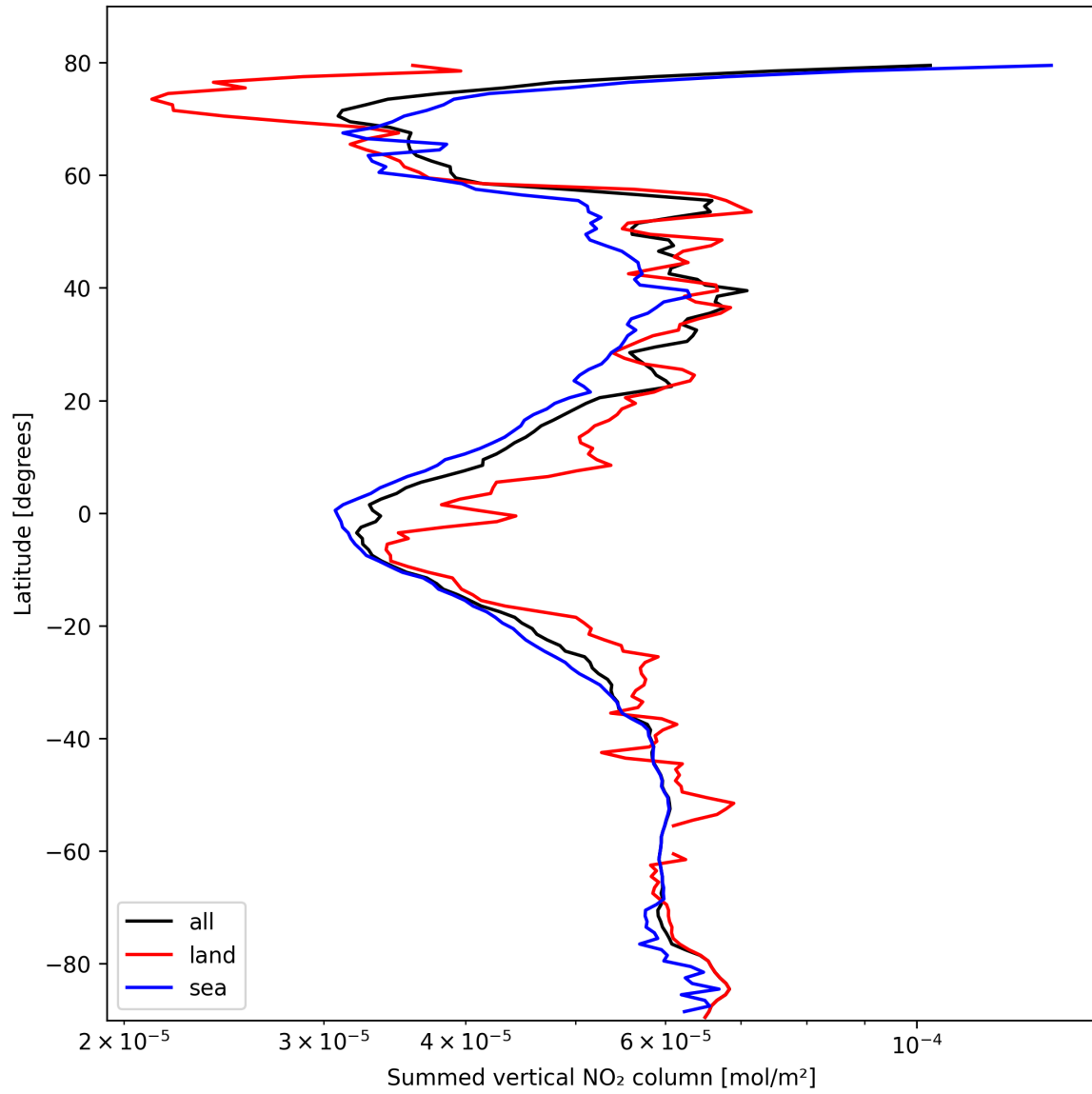
Figure 21: Zonal average of “Summed vertical NO 2 column” for 2025-02-25 to 2025-02-26.
