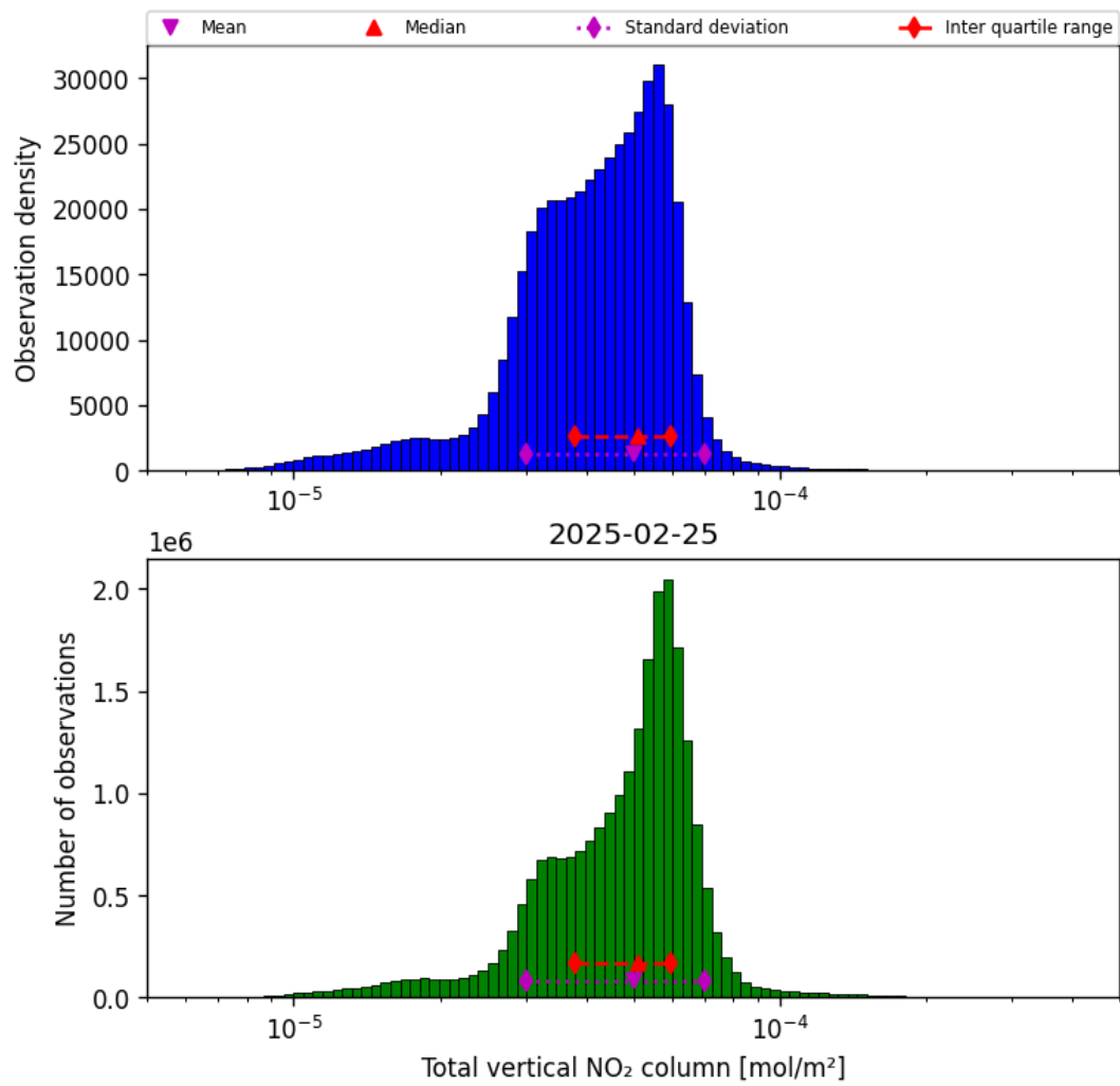
Figure 36: Histogram of “Total vertical NO 2 column” for 2025-02-25 to 2025-02-26
