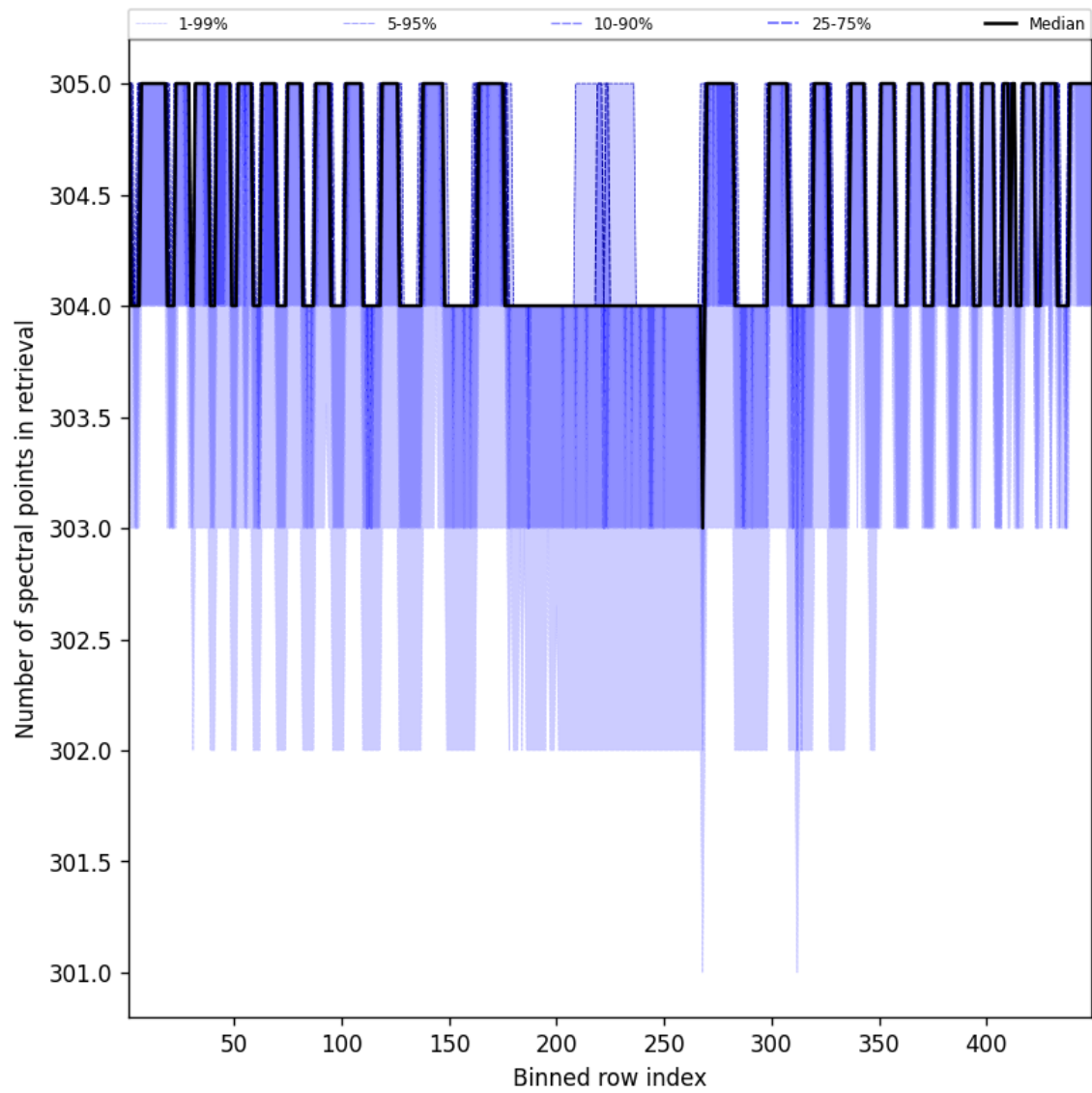
Figure 48: Along track statistics of “Number of spectral points in retrieval” for 2025-02-25 to 2025-02-26
