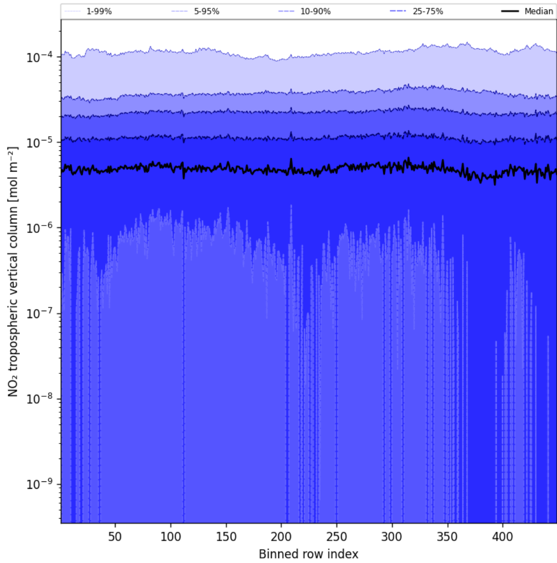
Figure 44: Along track statistics of “NO 2 tropospheric vertical column” for 2025-02-25 to 2025-02-26
