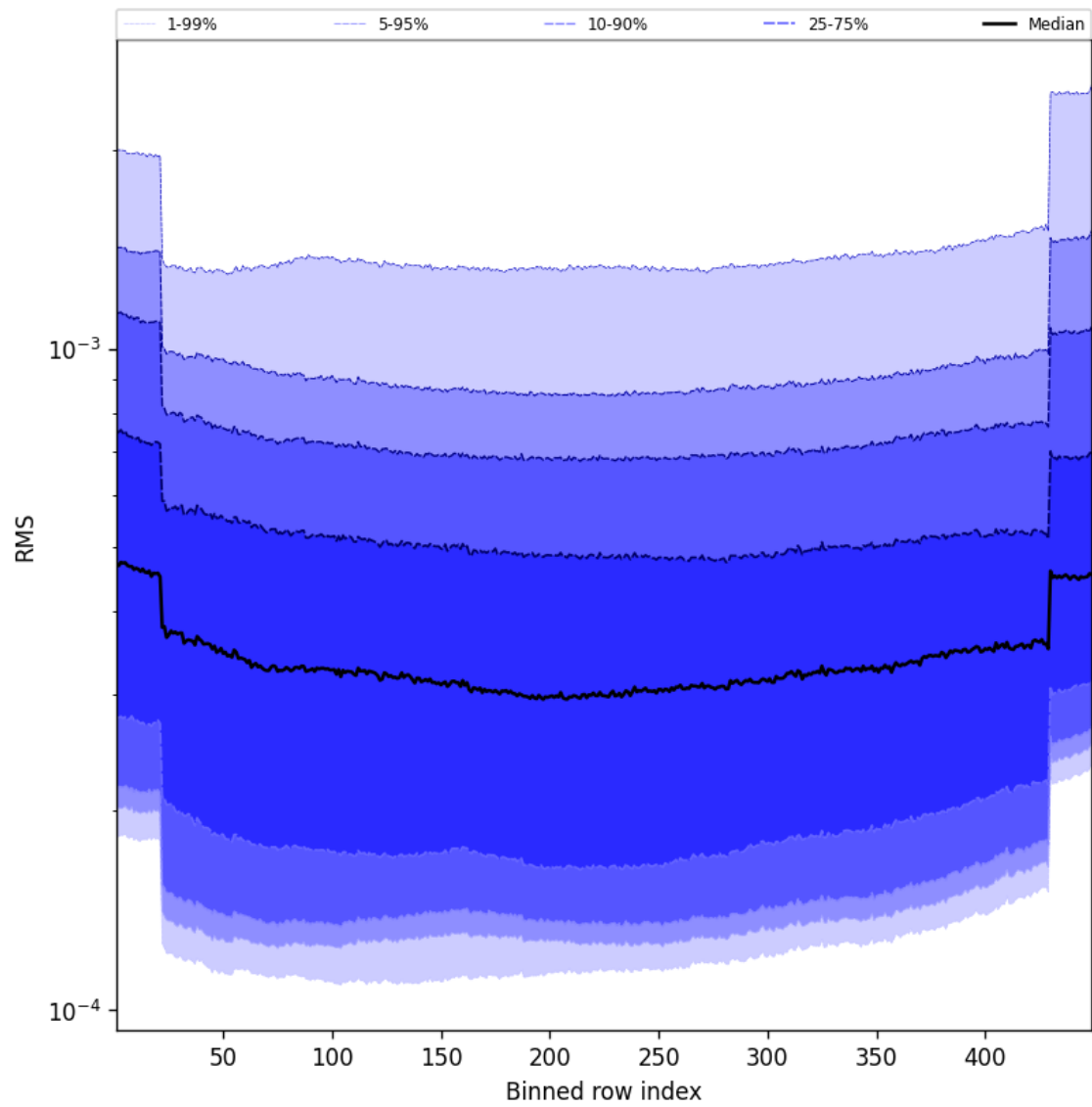
Figure 58: Along track statistics of “RMS” for 2025-02-25 to 2025-02-26
