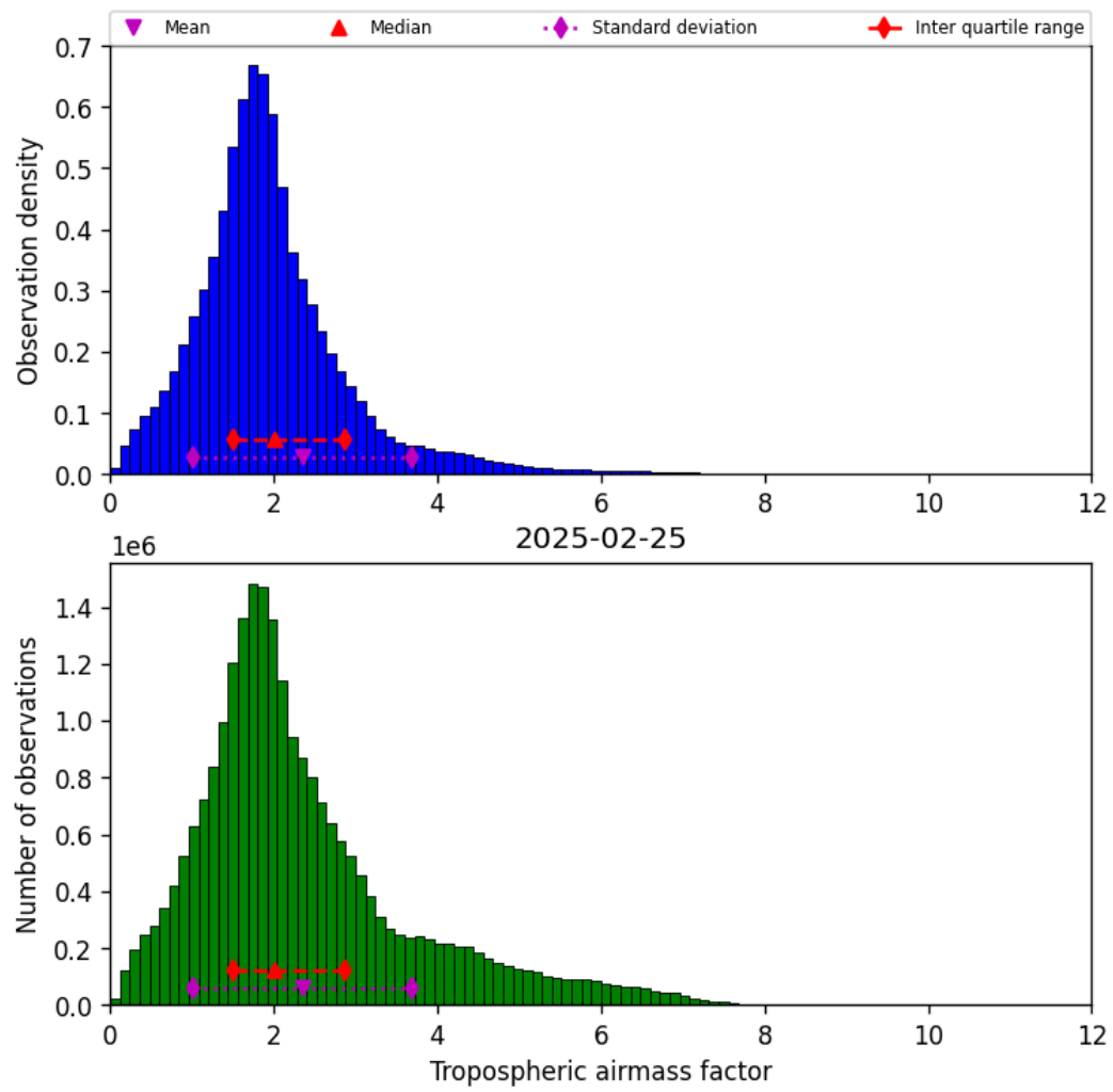
Figure 29: Histogram of “Tropospheric airmass factor” for 2025-02-25 to 2025-02-26
