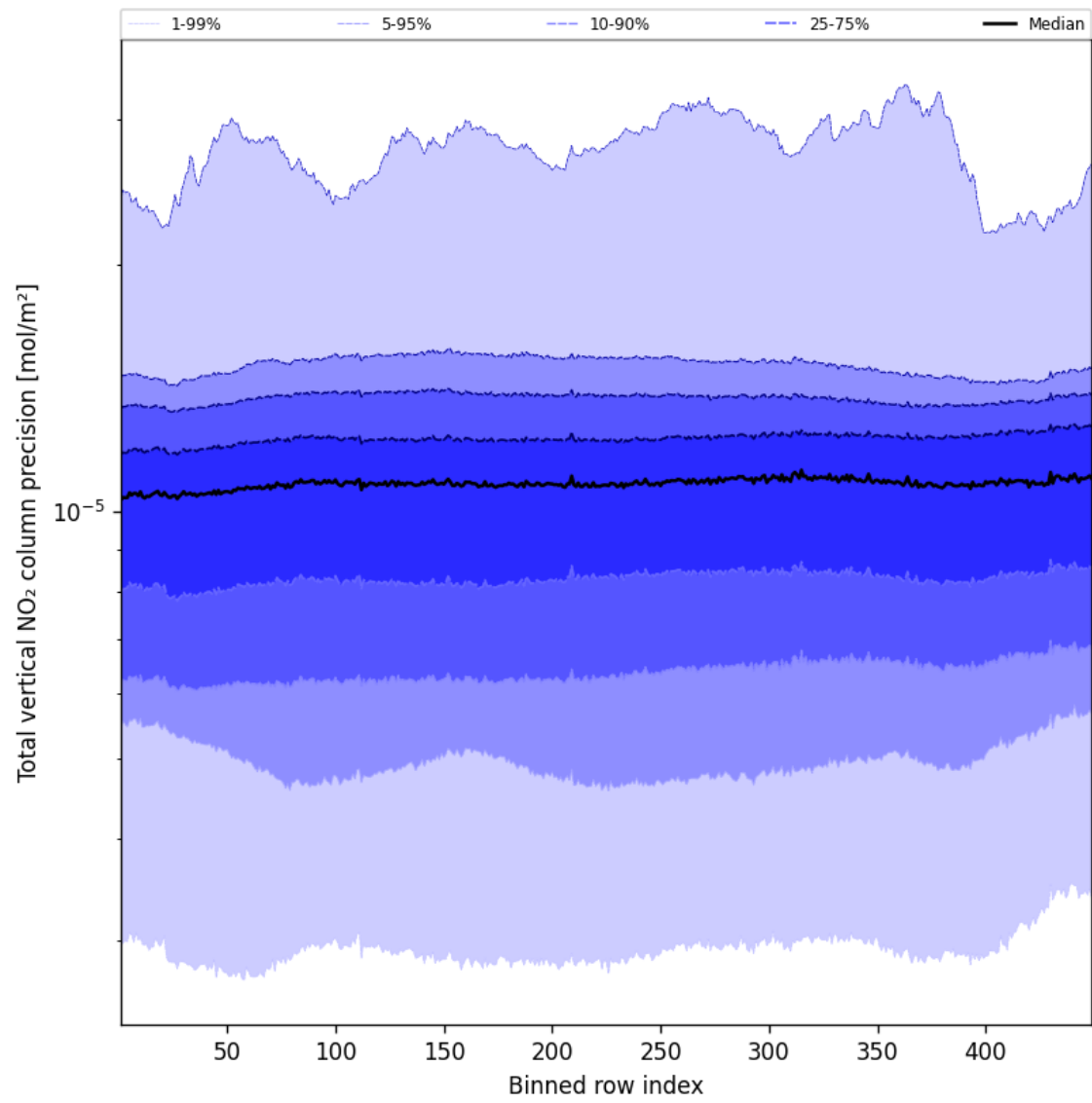
Figure 54: Along track statistics of “Total vertical NO 2 column precision” for 2025-02-25 to 2025-02-26
