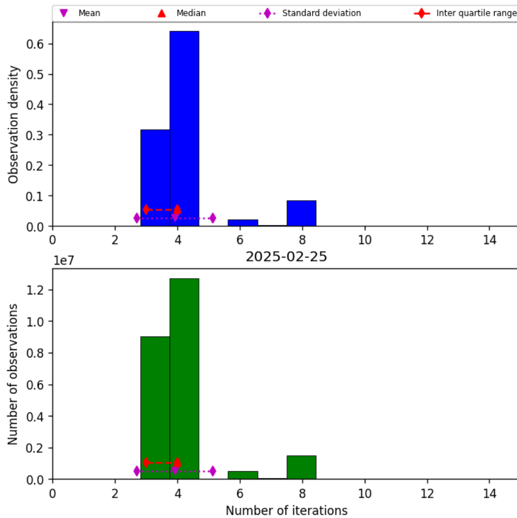
Figure 32: Histogram of “Number of iterations” for 2025-02-25 to 2025-02-26
