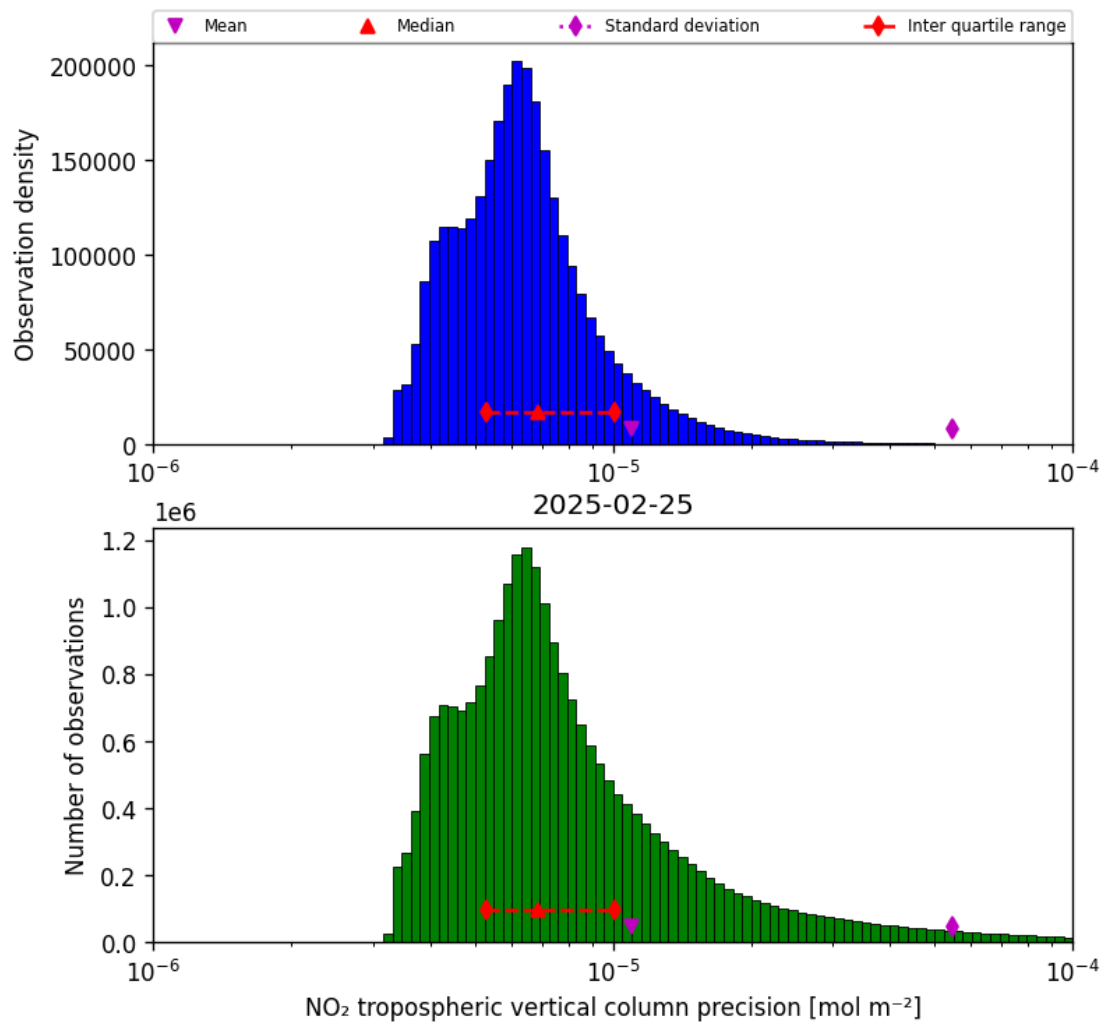
Figure 28: Histogram of “NO 2 tropospheric vertical column precision” for 2025-02-25 to 2025-02-26
