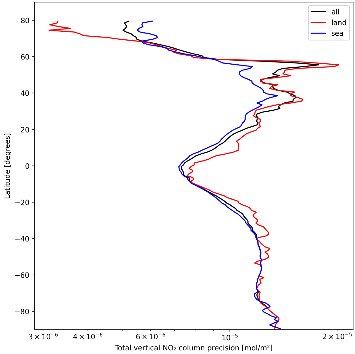
Figure 20: Zonal average of “Total vertical NO 2 column precision” for 2025-02-26 to 2025-02-27.
