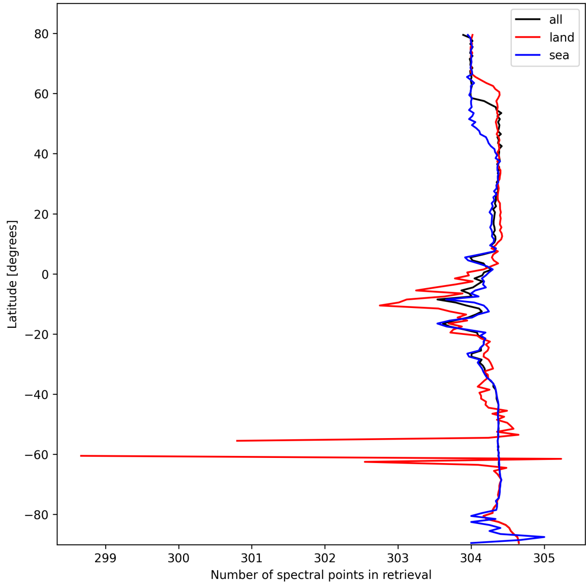
Figure 14: Zonal average of “Number of spectral points in retrieval” for 2025-02-26 to 2025-02-27.
