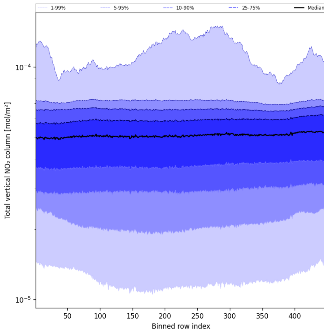
Figure 53: Along track statistics of “Total vertical NO 2 column” for 2025-02-26 to 2025-02-27
