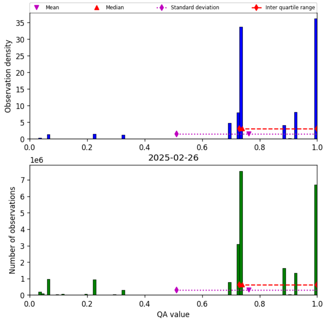
Figure 26: Histogram of “QA value” for 2025-02-26 to 2025-02-27
