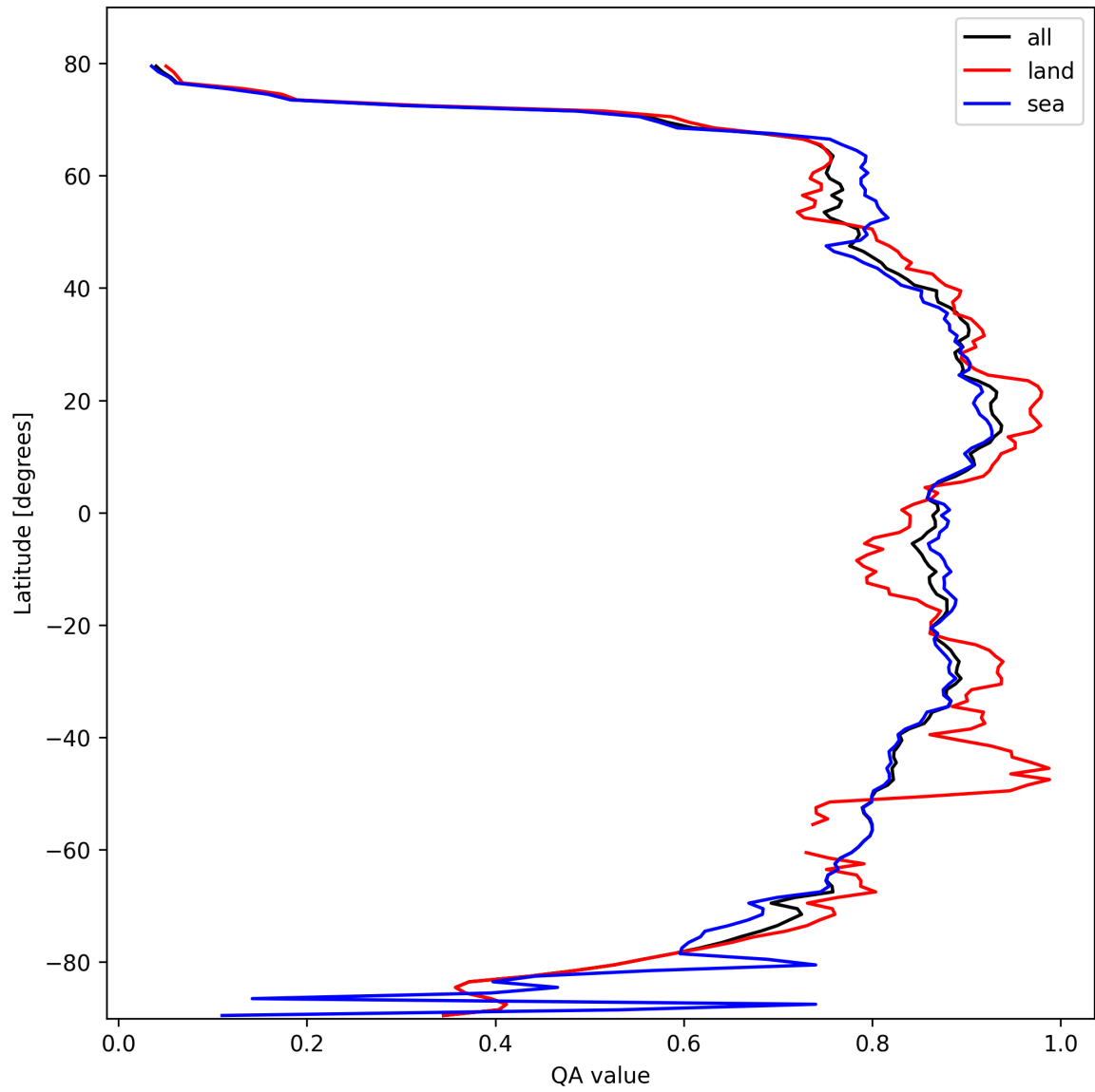
Figure 9: Zonal average of “QA value” for 2025-02-26 to 2025-02-27.
