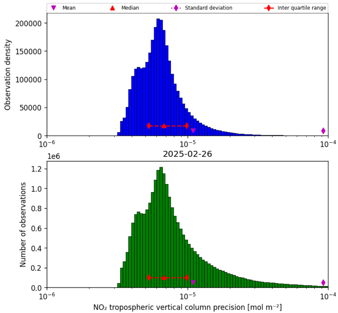
Figure 28: Histogram of “NO 2 tropospheric vertical column precision” for 2025-02-26 to 2025-02-27
