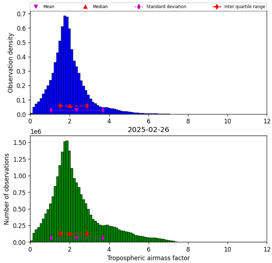
Figure 29: Histogram of “Tropospheric airmass factor” for 2025-02-26 to 2025-02-27
