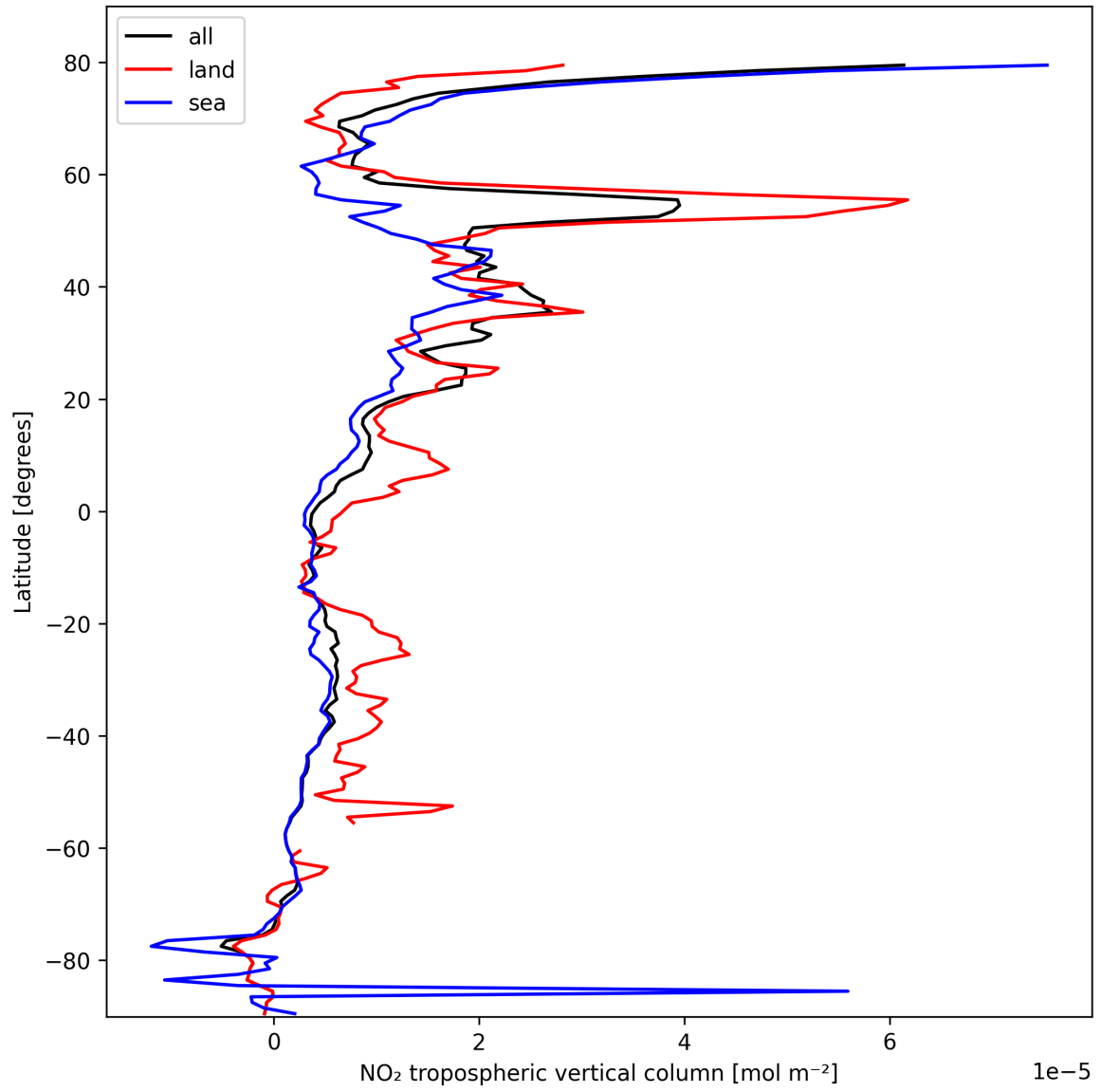
Figure 10: Zonal average of “NO 2 tropospheric vertical column” for 2025-02-26 to 2025-02-27.
