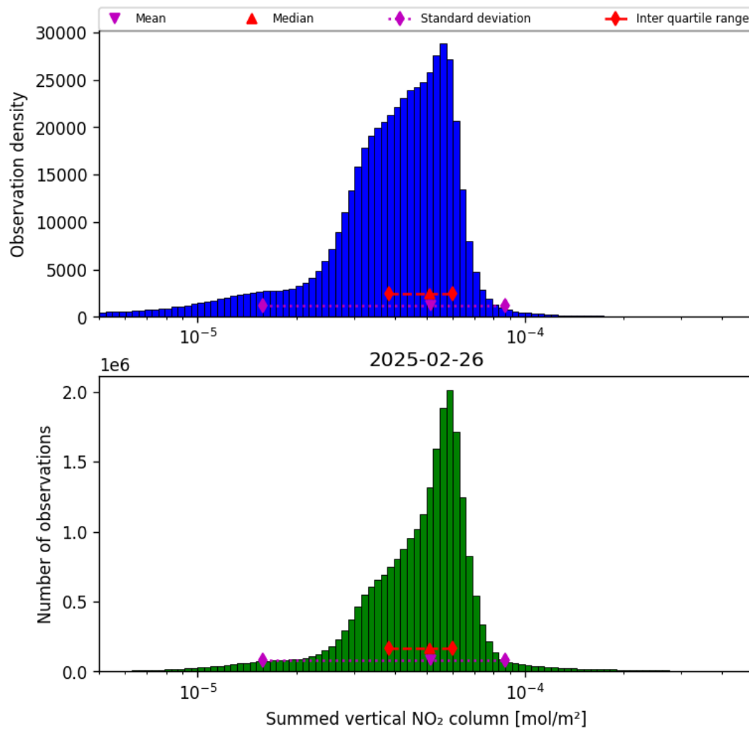
Figure 38: Histogram of “Summed vertical NO 2 column” for 2025-02-26 to 2025-02-27
