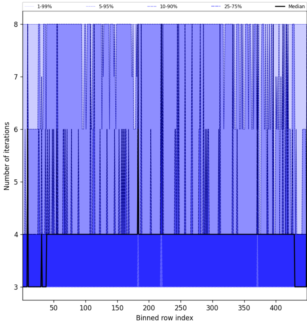
Figure 49: Along track statistics of “Number of iterations” for 2025-02-26 to 2025-02-27
