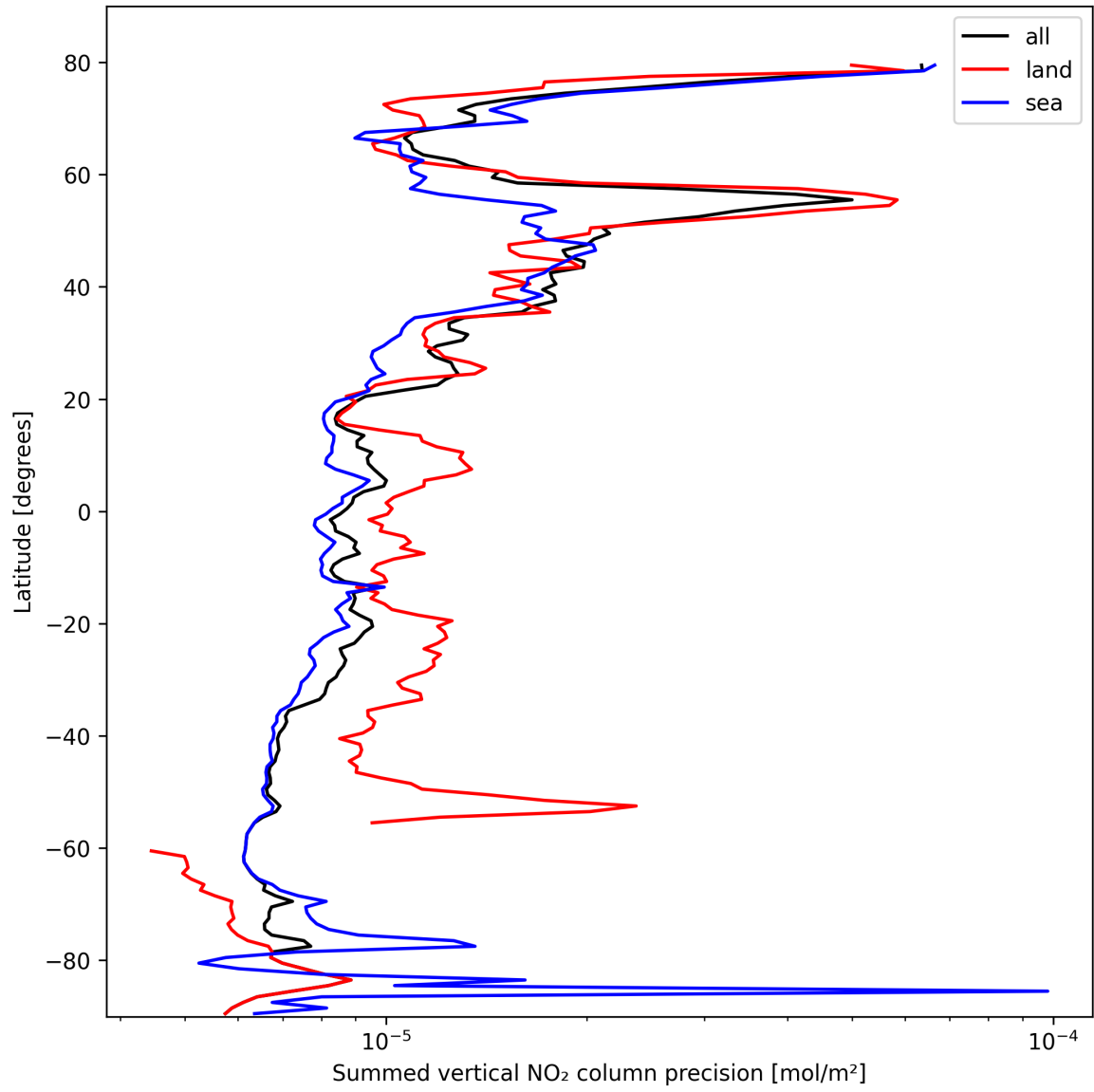
Figure 22: Zonal average of “Summed vertical NO 2 column precision” for 2025-02-26 to 2025-02-27.
