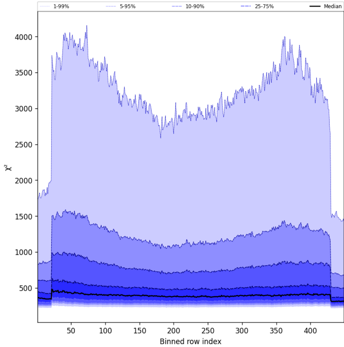
Figure 57: Along track statistics of “ \chi^2 ” for 2025-02-26 to 2025-02-27
