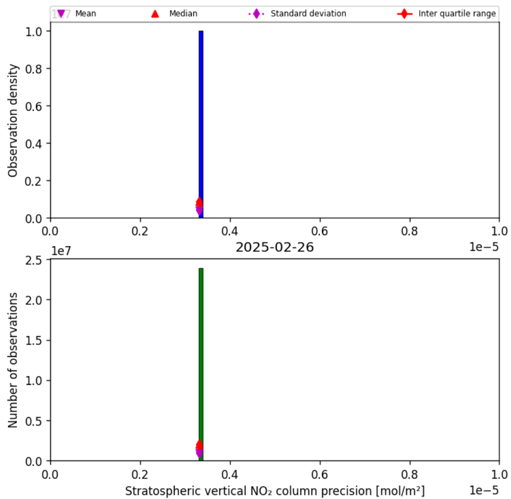
Figure 35: Histogram of “Stratospheric vertical NO 2 column precision” for 2025-02-26 to 2025-02-27
