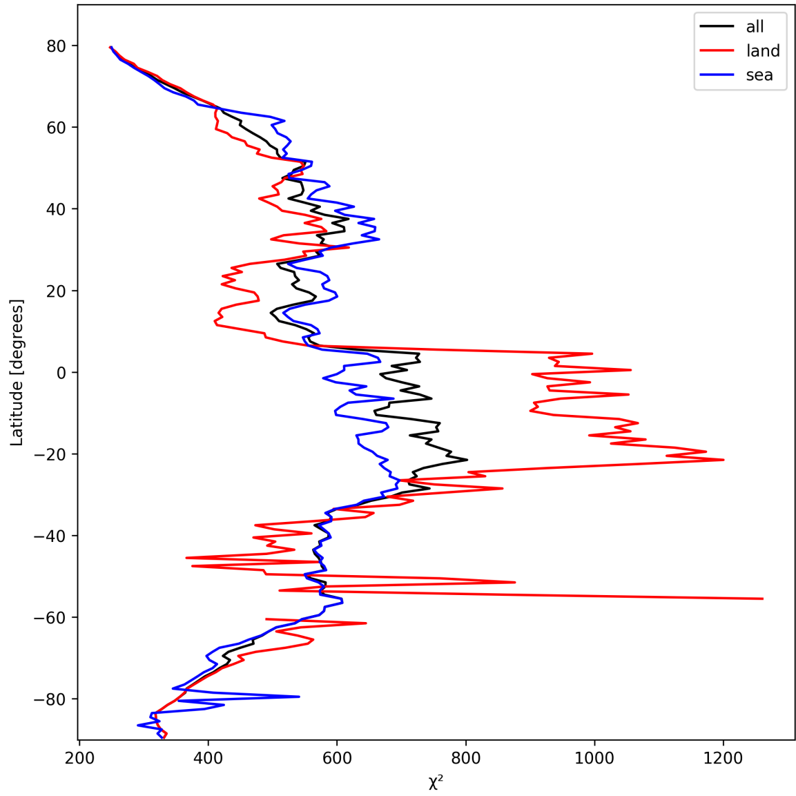
Figure 23: Zonal average of “ \chi^2 ” for 2025-02-26 to 2025-02-27.
