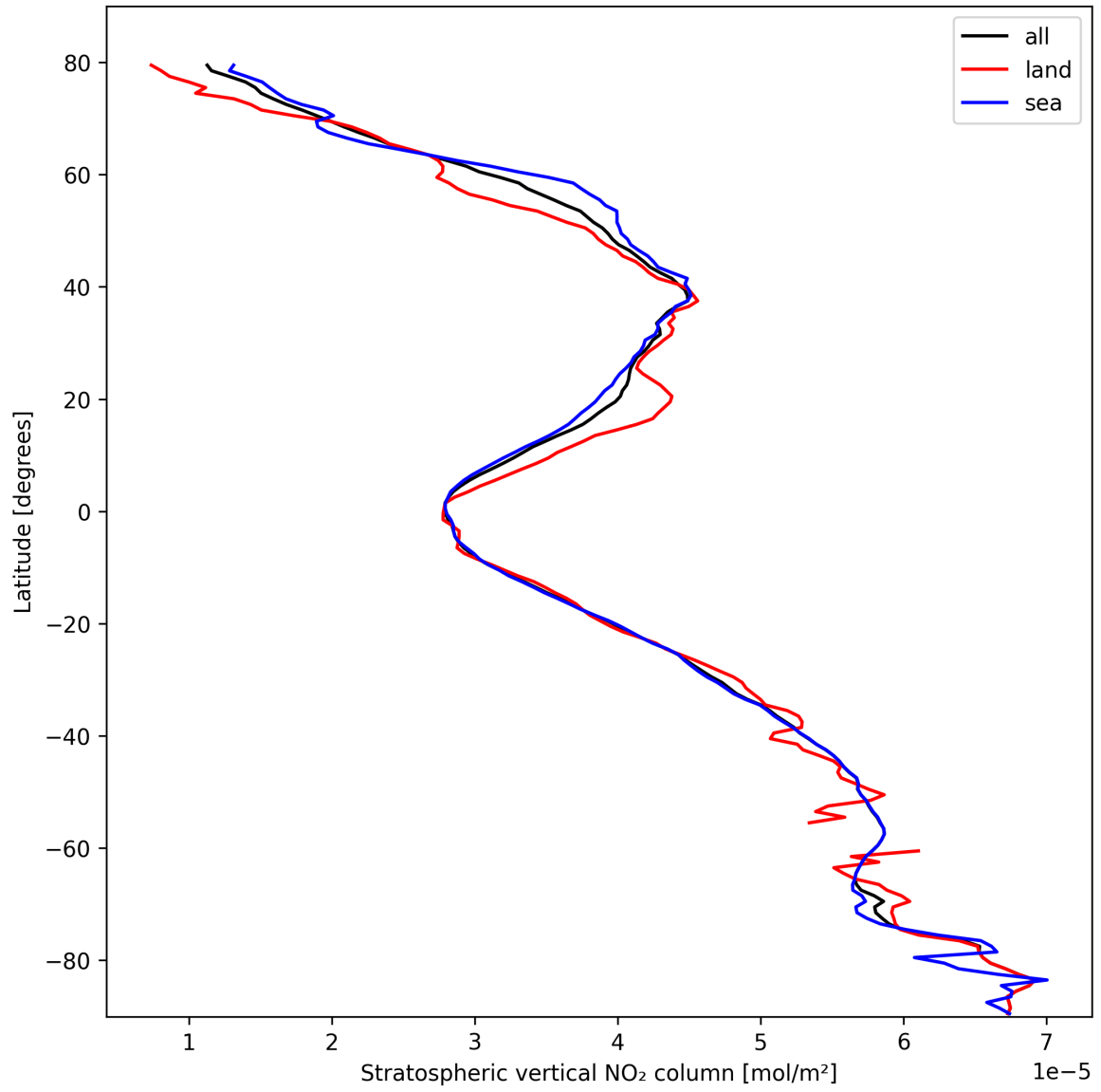
Figure 17: Zonal average of “Stratospheric vertical NO 2 column” for 2025-02-26 to 2025-02-27.
