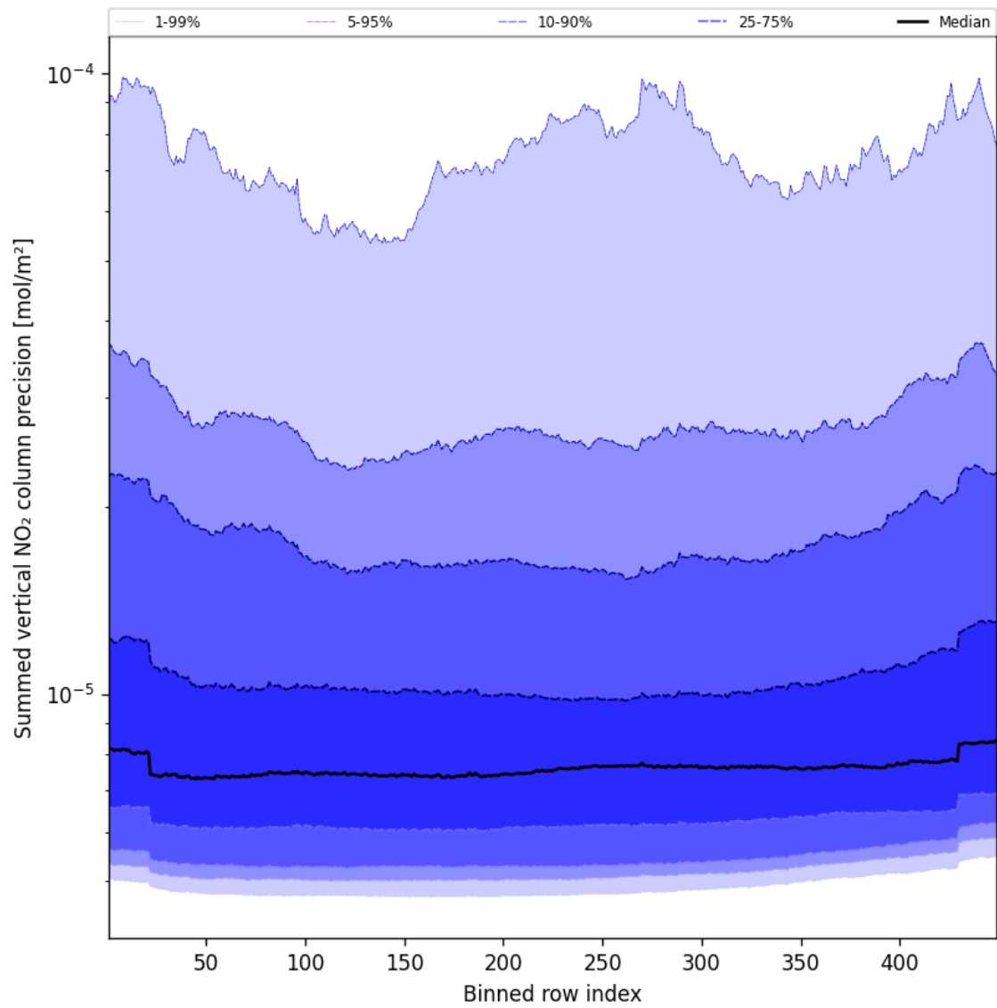
Figure 56: Along track statistics of “Summed vertical NO 2 column precision” for 2025-02-26 to 2025-02-27
