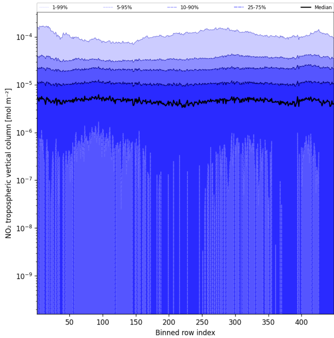
Figure 44: Along track statistics of “NO 2 tropospheric vertical column” for 2025-02-26 to 2025-02-27
