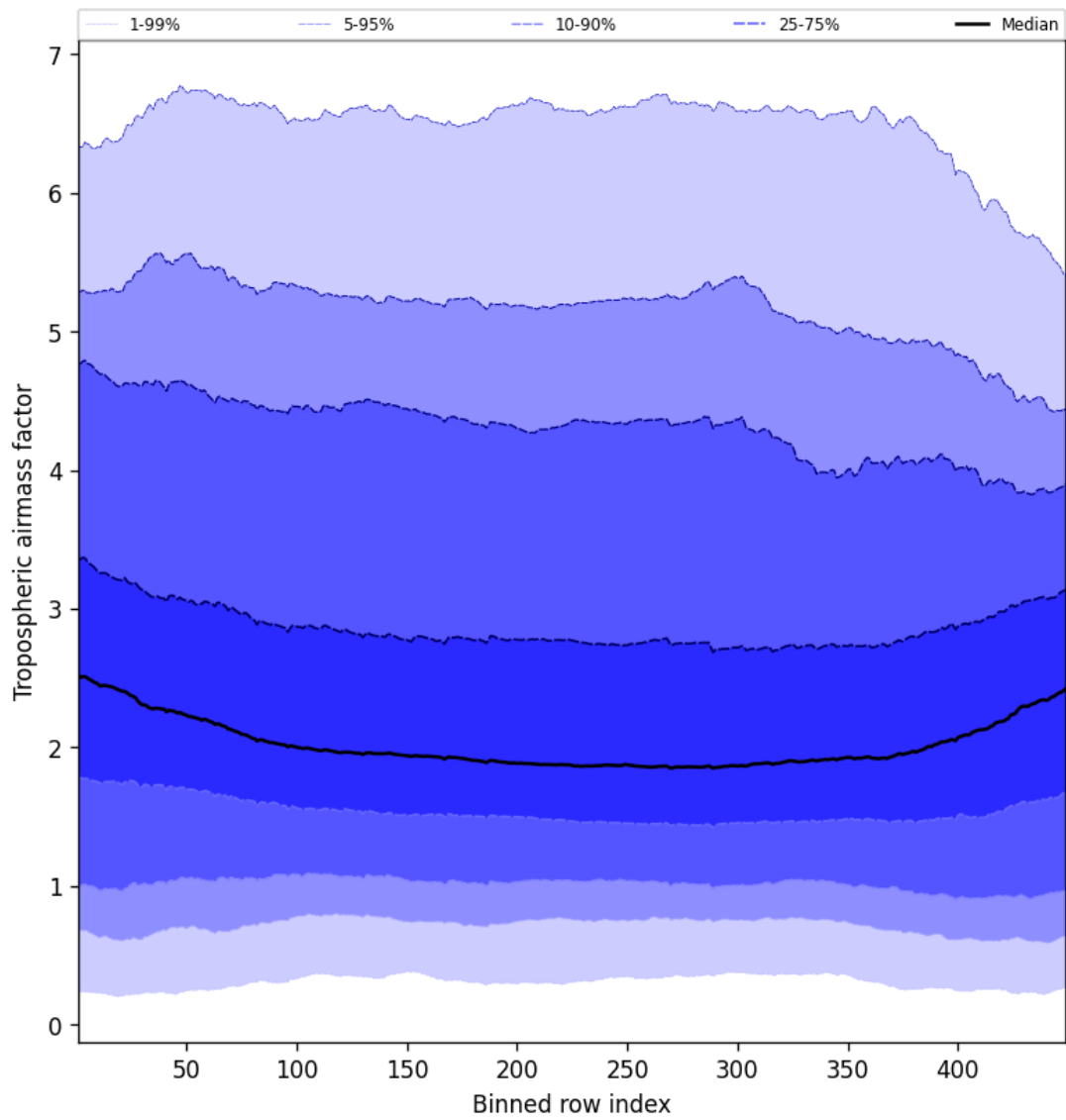
Figure 46: Along track statistics of “Tropospheric air mass factor” for 2025-02-26 to 2025-02-27
