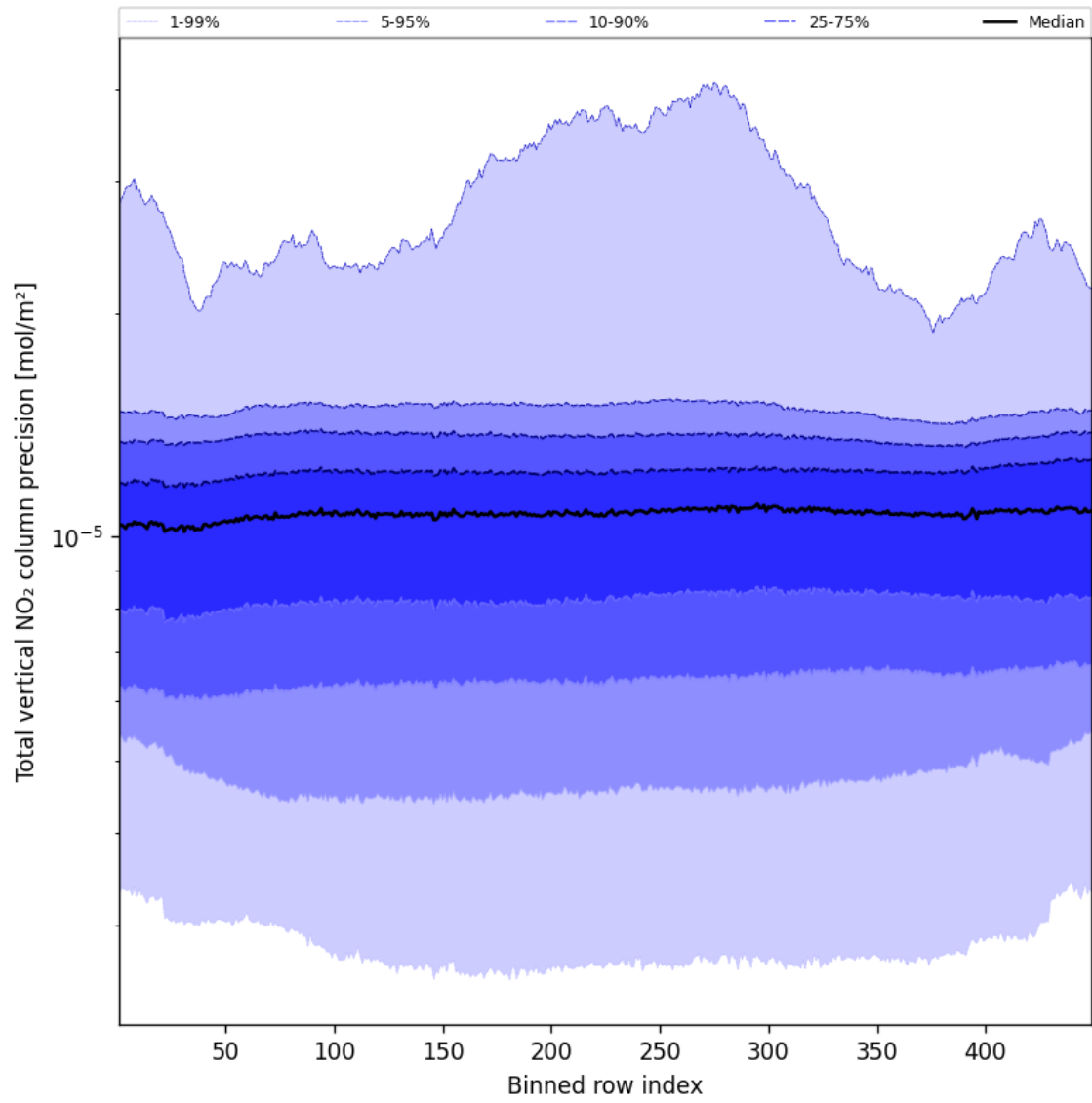
Figure 54: Along track statistics of “Total vertical NO 2 column precision” for 2025-02-26 to 2025-02-27
