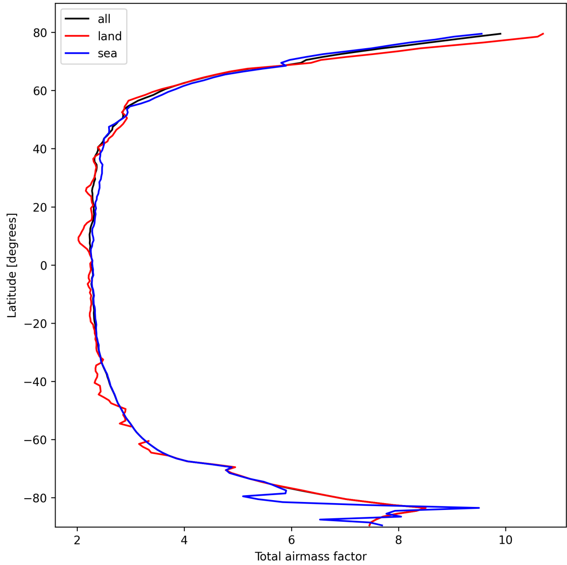
Figure 13: Zonal average of “Total airmass factor” for 2025-02-26 to 2025-02-27.
