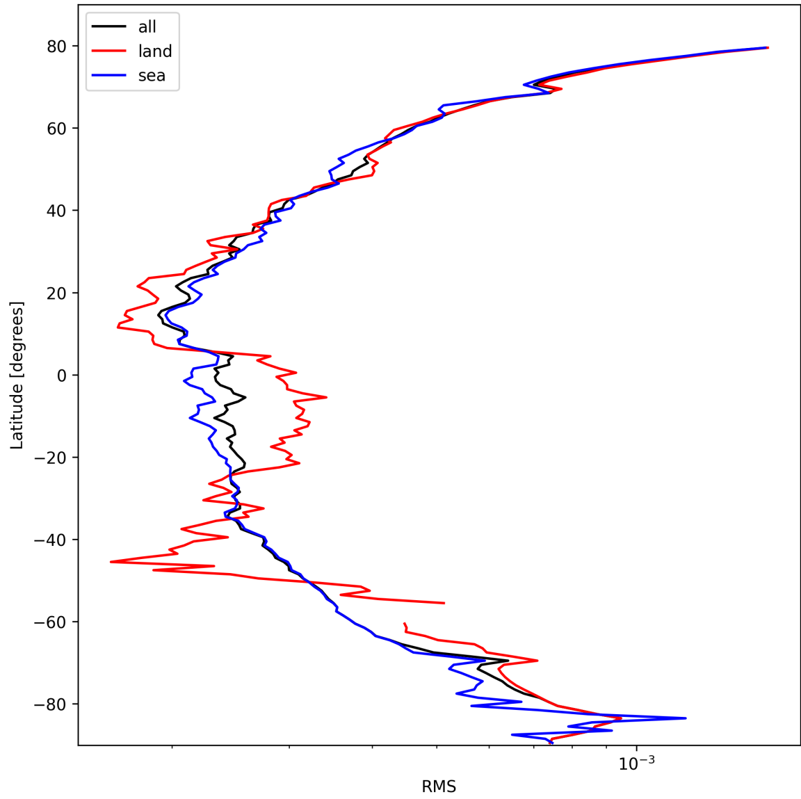
Figure 24: Zonal average of “RMS” for 2025-02-26 to 2025-02-27.
