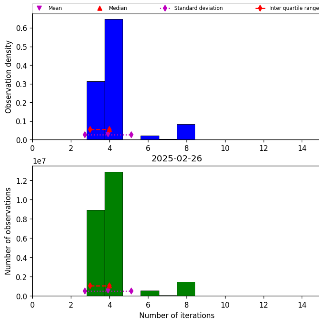
Figure 32: Histogram of “Number of iterations” for 2025-02-26 to 2025-02-27
