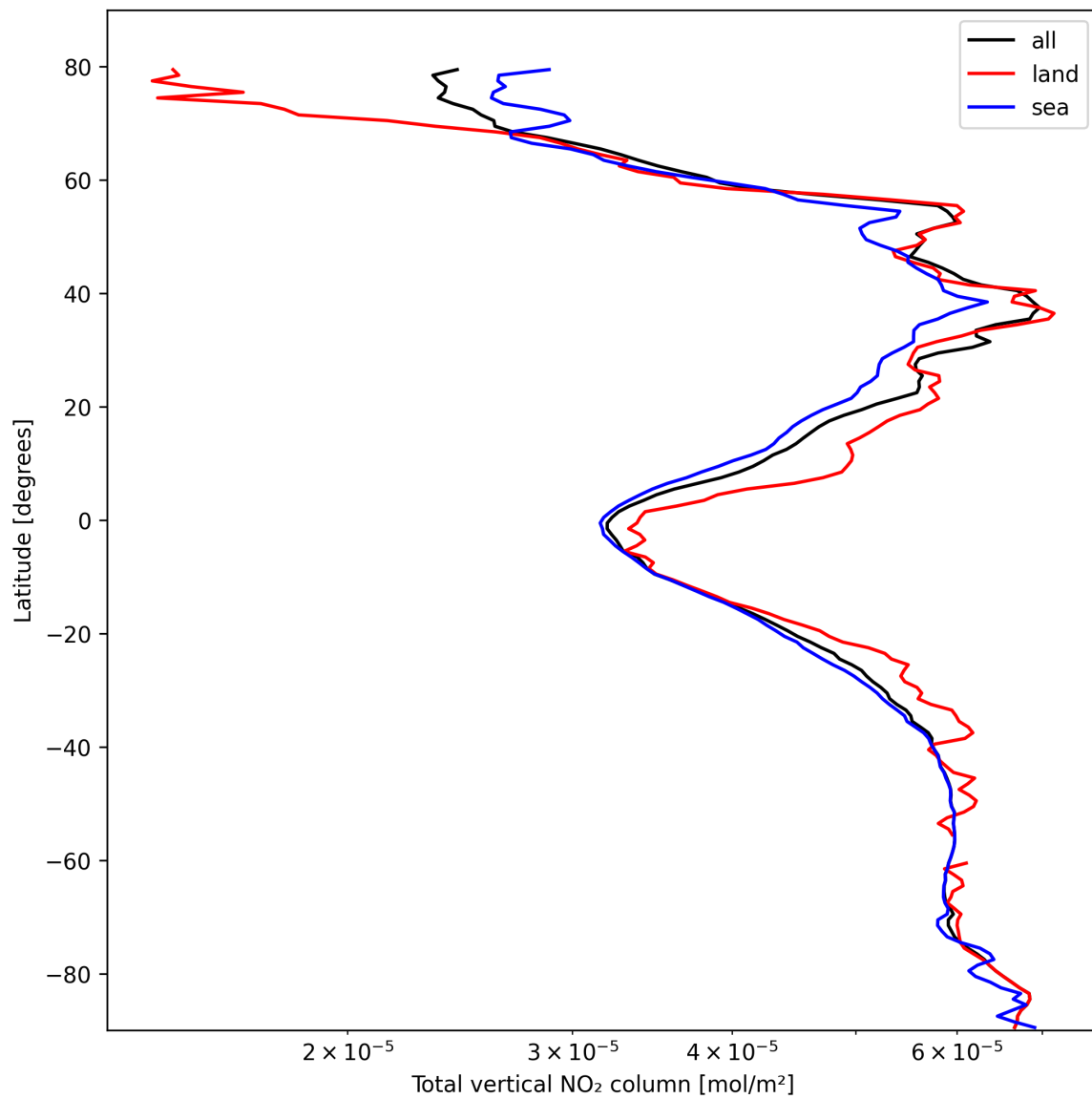
Figure 19: Zonal average of “Total vertical NO 2 column” for 2025-02-26 to 2025-02-27.
