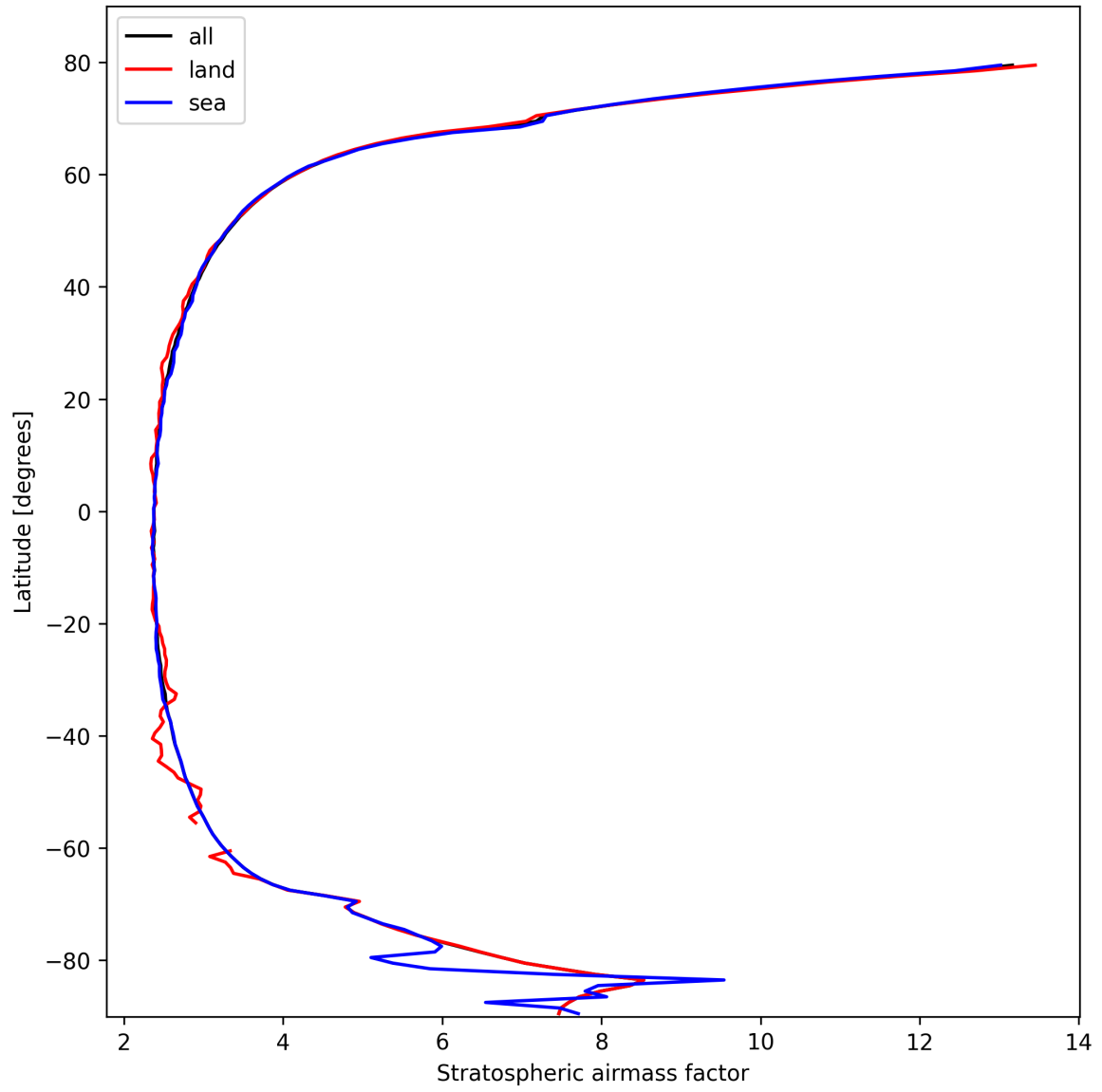
Figure 25: Zonal average of “Stratospheric airmass factor” for 2025-02-26 to 2025-02-27.
