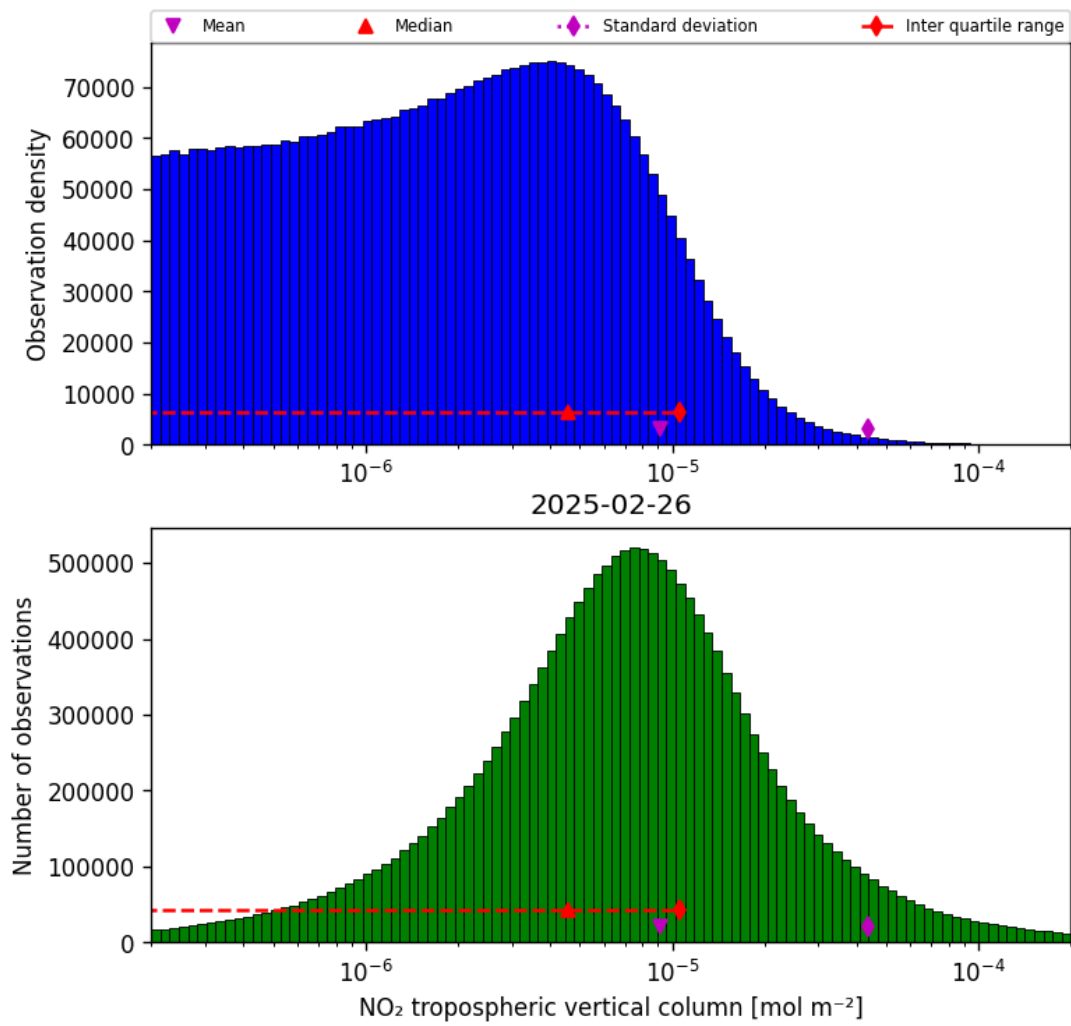
Figure 27: Histogram of “NO 2 tropospheric vertical column” for 2025-02-26 to 2025-02-27
