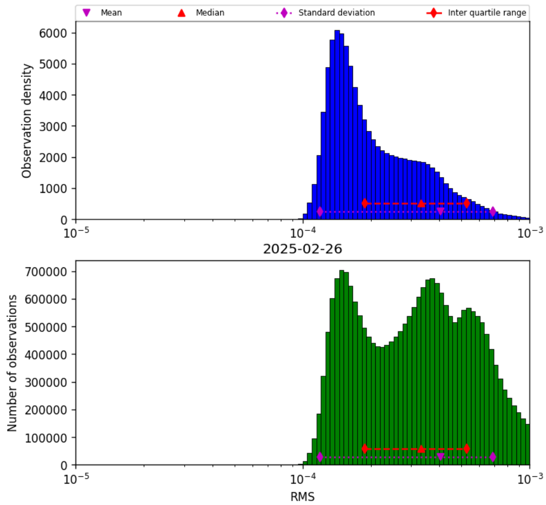
Figure 41: Histogram of “RMS” for 2025-02-26 to 2025-02-27
