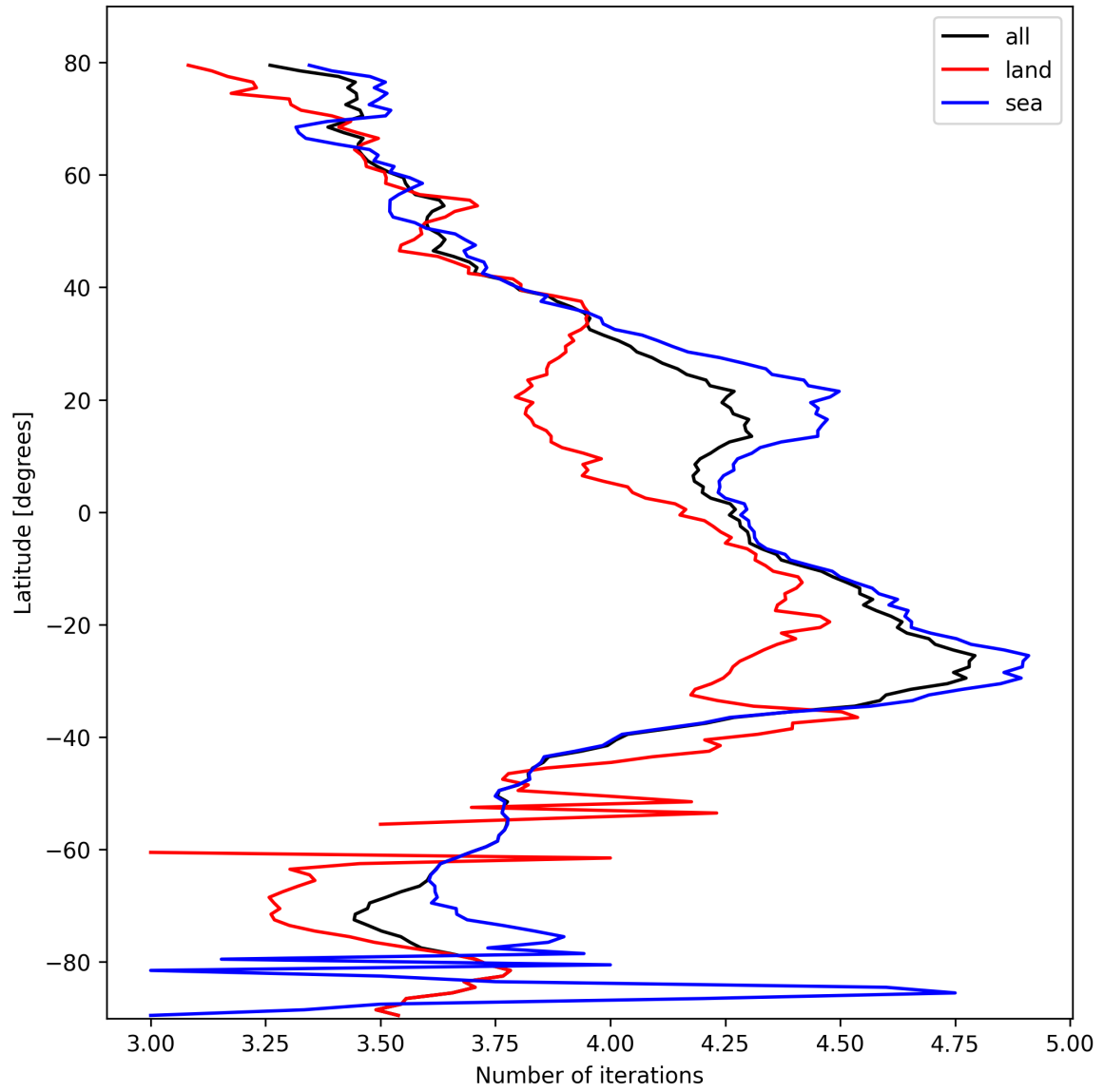
Figure 15: Zonal average of “Number of iterations” for 2025-02-26 to 2025-02-27.
