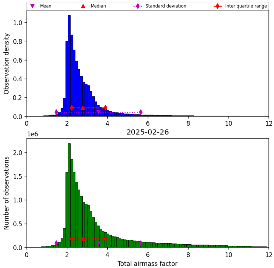
Figure 30: Histogram of “Total airmass factor” for 2025-02-26 to 2025-02-27
