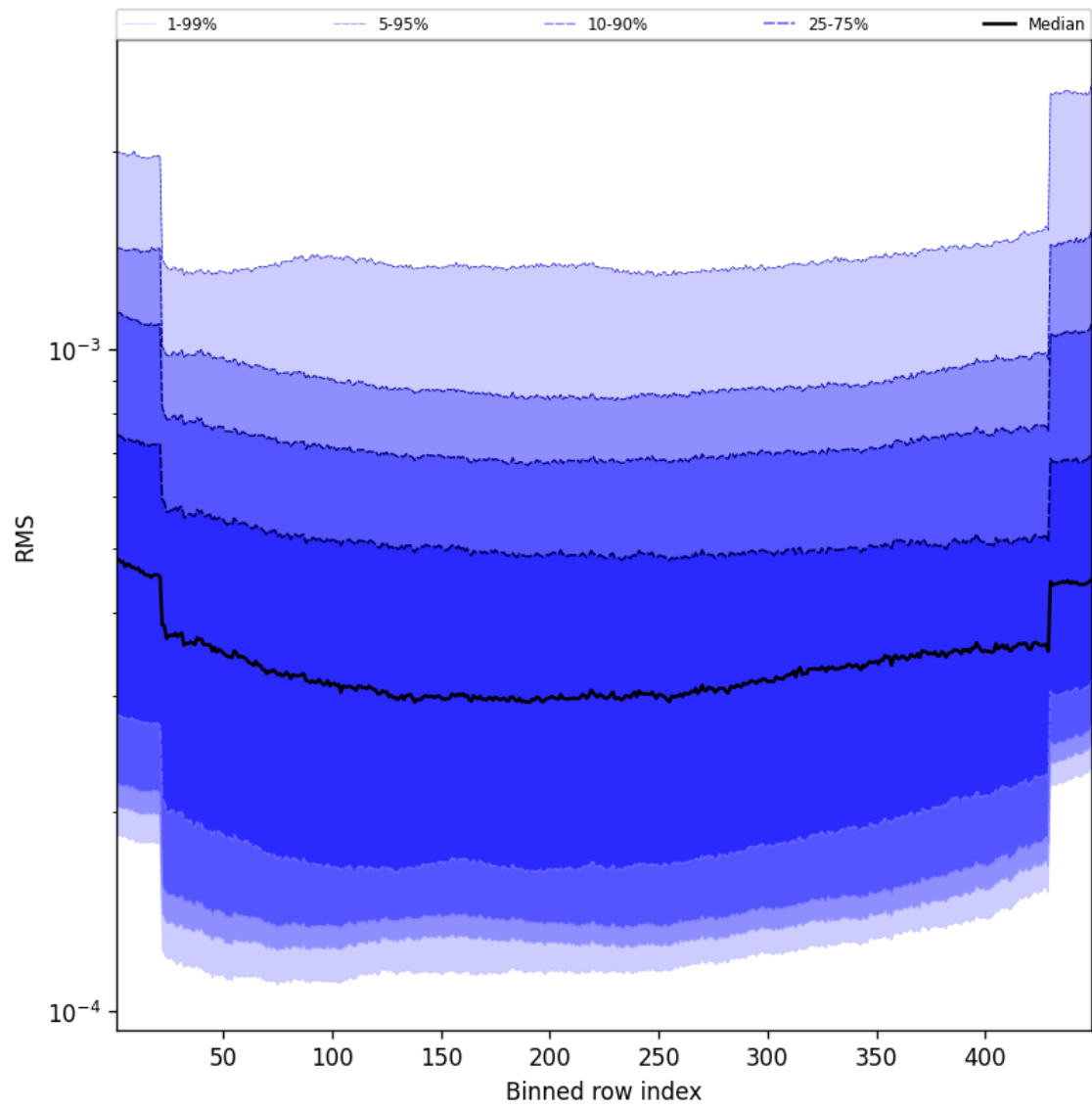
Figure 58: Along track statistics of “RMS” for 2025-02-26 to 2025-02-27
