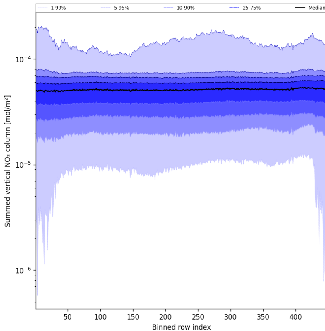
Figure 55: Along track statistics of “Summed vertical NO 2 column” for 2025-02-26 to 2025-02-27
