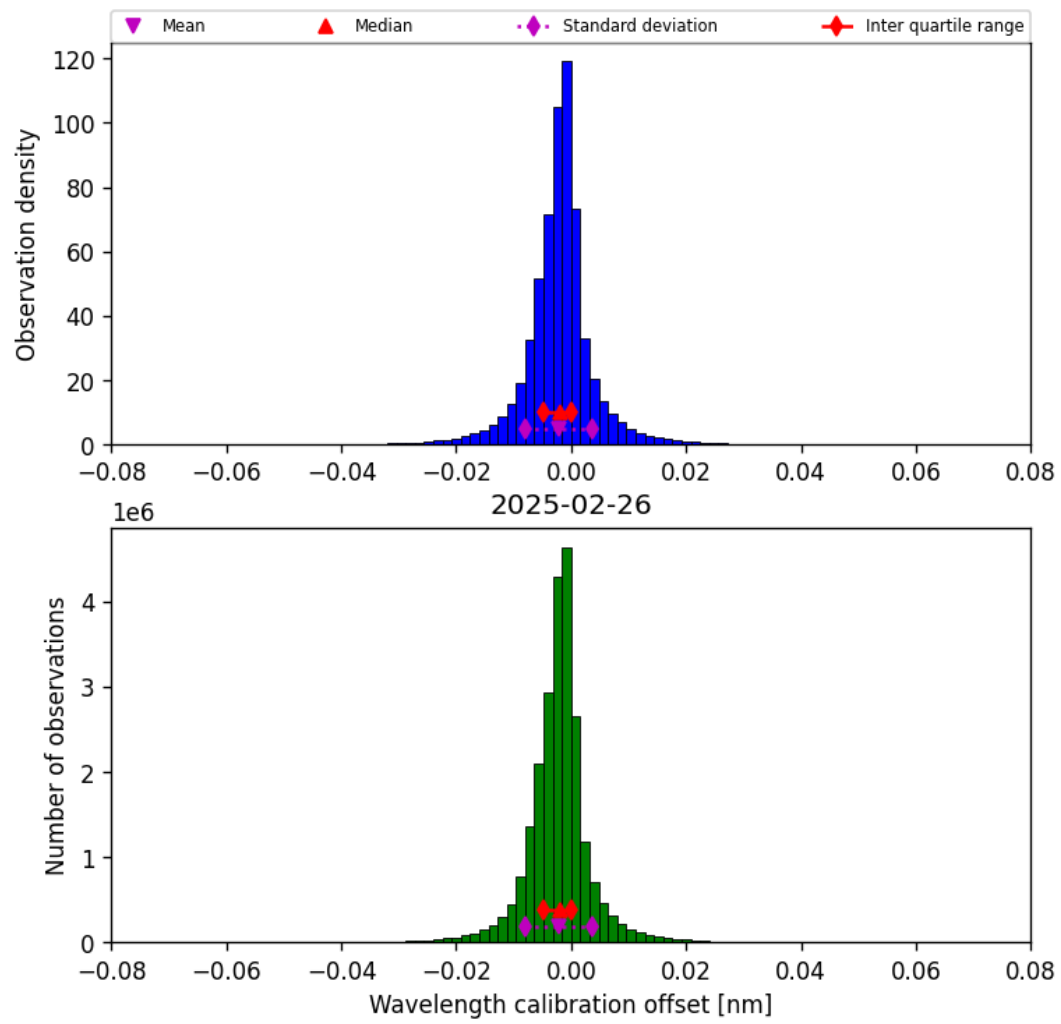
Figure 33: Histogram of “Wavelength calibration offset” for 2025-02-26 to 2025-02-27
