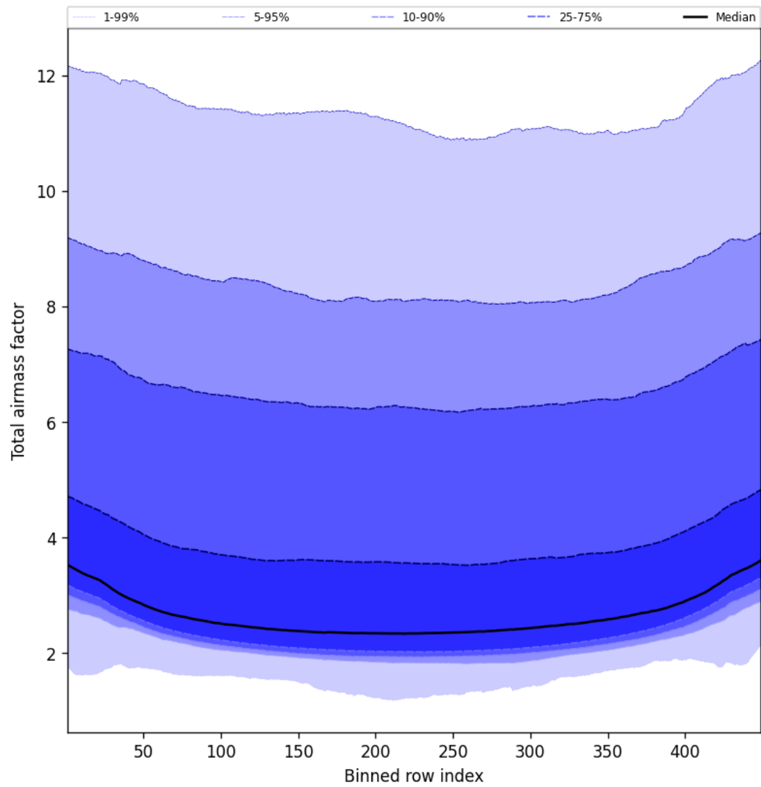
Figure 47: Along track statistics of “Total airmass factor” for 2025-02-26 to 2025-02-27
