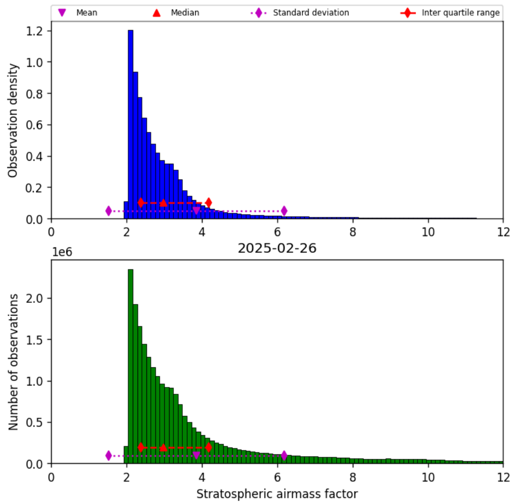
Figure 42: Histogram of “Stratospheric airmass factor” for 2025-02-26 to 2025-02-27
