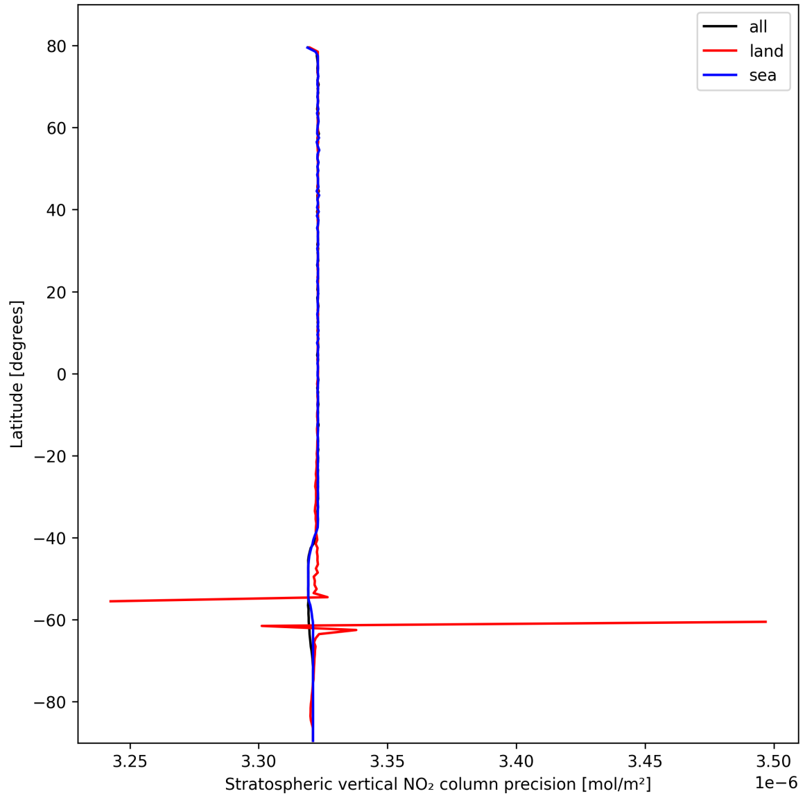
Figure 18: Zonal average of “Stratospheric vertical NO 2 column precision” for 2025-02-26 to 2025-02-27.
