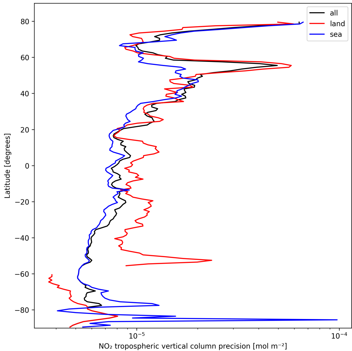
Figure 11: Zonal average of “NO 2 tropospheric vertical column precision” for 2025-02-26 to 2025-02-27.
