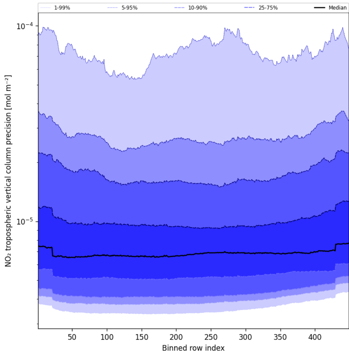
Figure 45: Along track statistics of “NO 2 tropospheric vertical column precision” for 2025-02-26 to 2025-02-27
