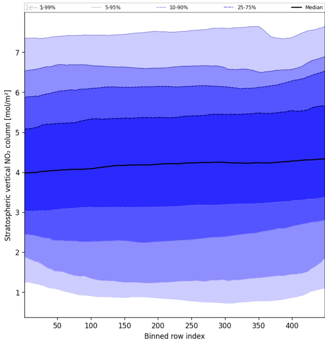
Figure 51: Along track statistics of "Stratospheric vertical NO 2 column" for 2025-02-26 to 2025-02-27
