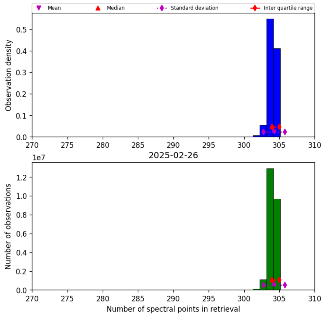
Figure 31: Histogram of “Number of spectral points in retrieval” for 2025-02-26 to 2025-02-27
