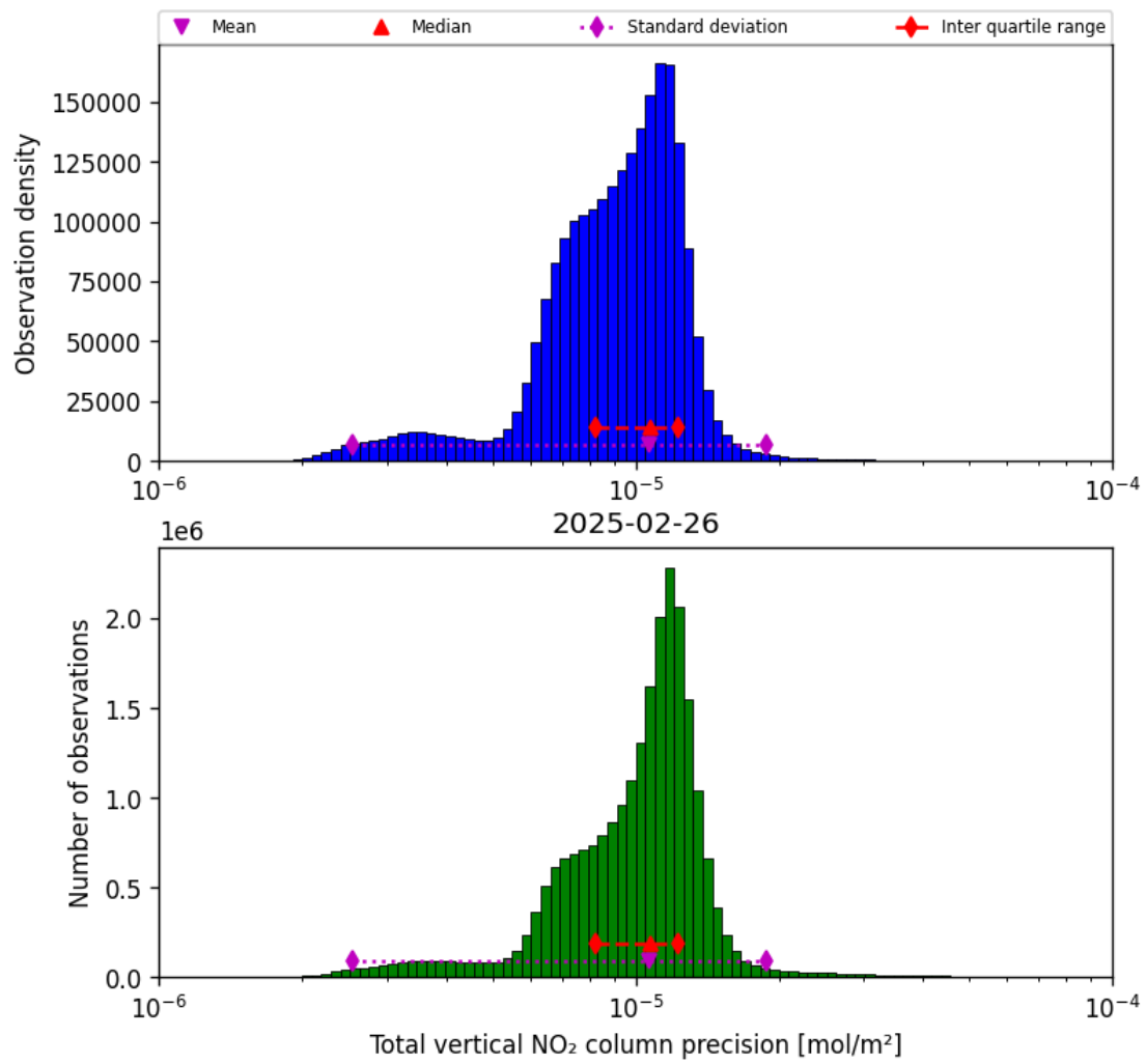
Figure 37: Histogram of “Total vertical NO 2 column precision” for 2025-02-26 to 2025-02-27
