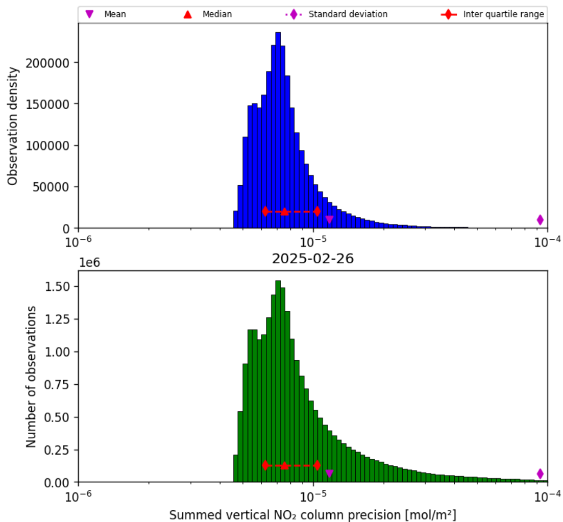
Figure 39: Histogram of “Summed vertical NO 2 column precision” for 2025-02-26 to 2025-02-27
