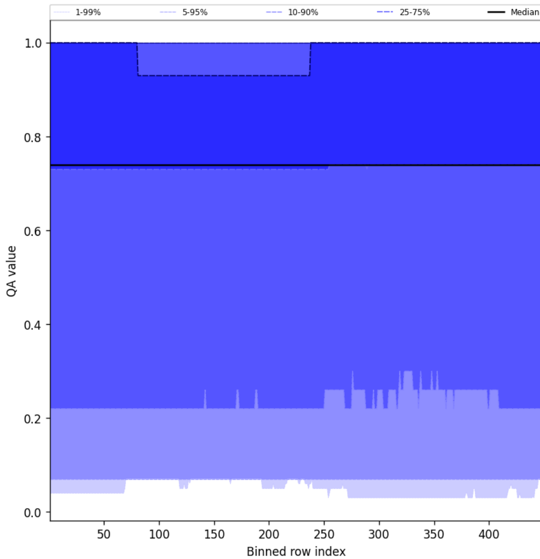
Figure 43: Along track statistics of “QA value” for 2025-02-26 to 2025-02-27
