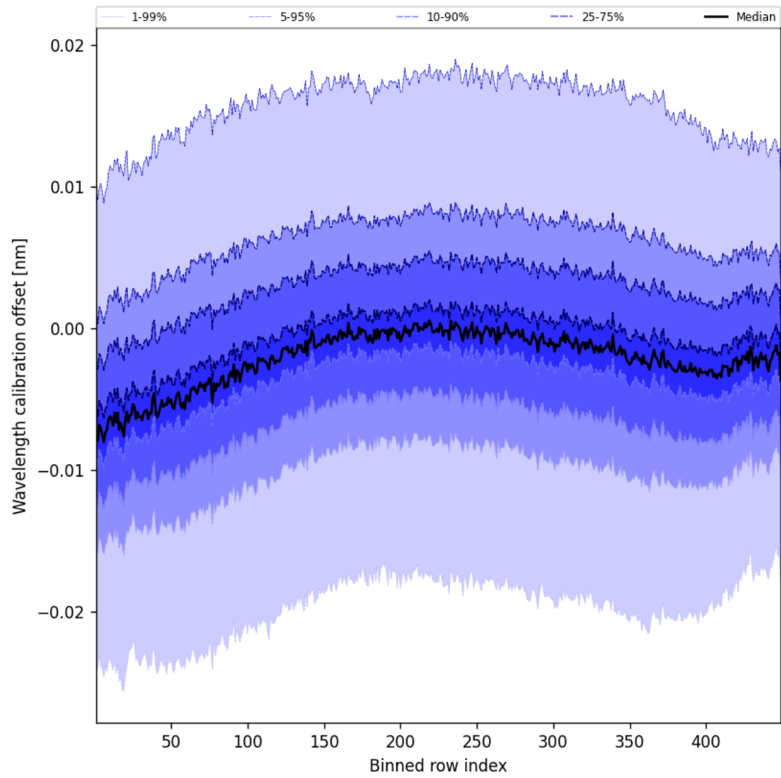
Figure 50: Along track statistics of “Wavelength calibration offset” for 2025-02-26 to 2025-02-27
