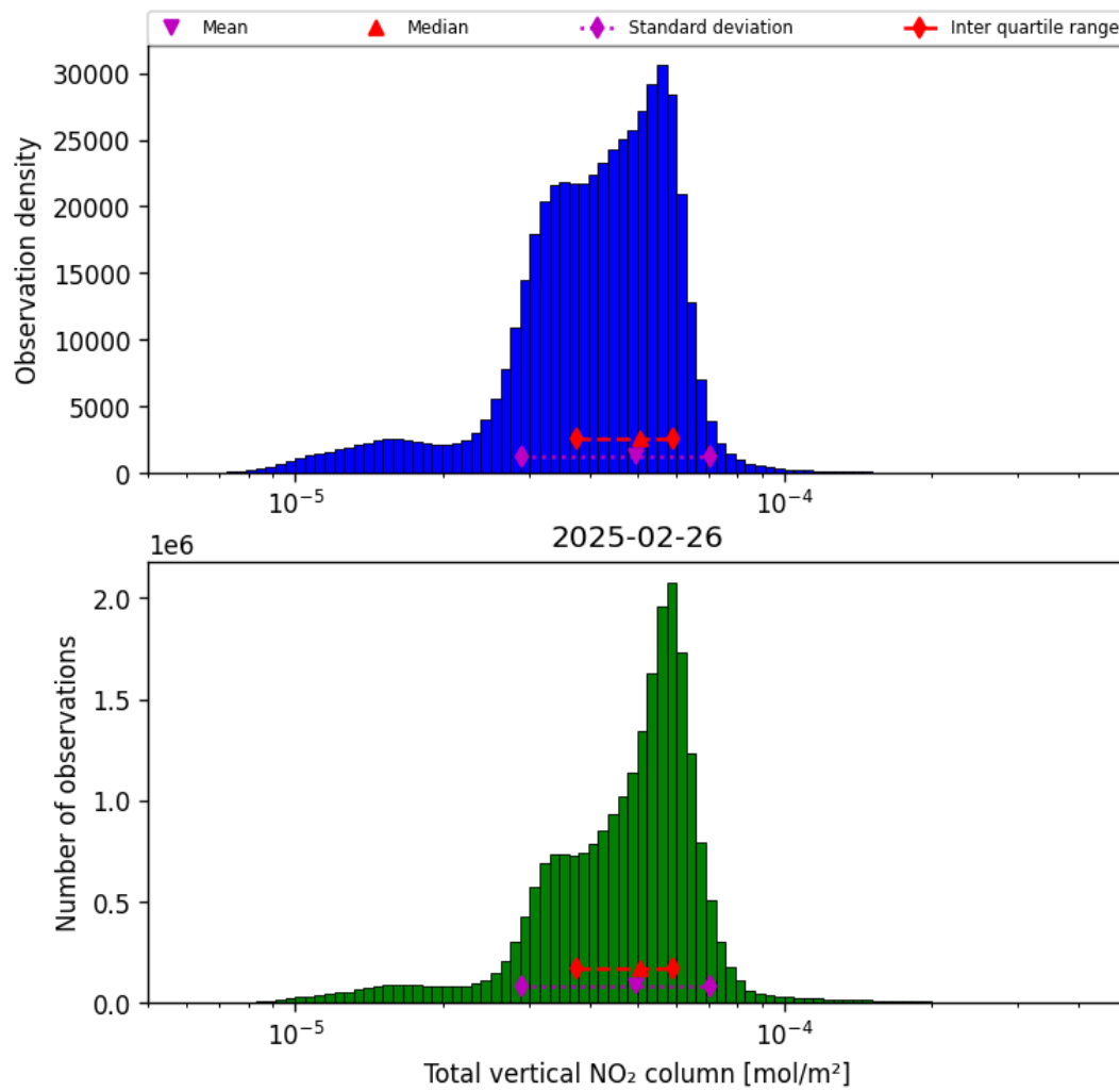
Figure 36: Histogram of "Total vertical NO 2 column" for 2025-02-26 to 2025-02-27
