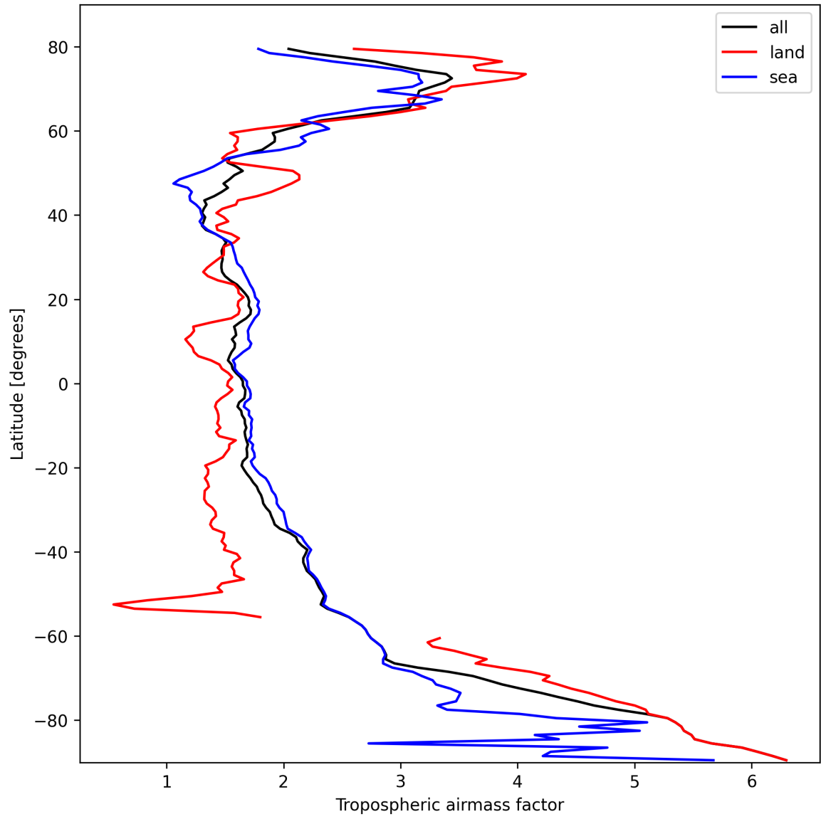
Figure 12: Zonal average of “Tropospheric airmass factor” for 2025-02-26 to 2025-02-27.
