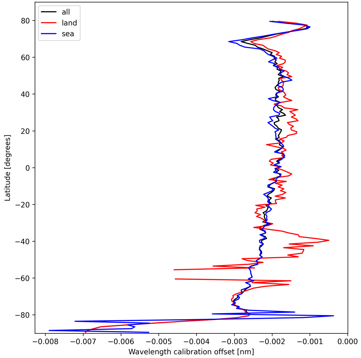
Figure 16: Zonal average of “Wavelength calibration offset” for 2025-02-26 to 2025-02-27.
