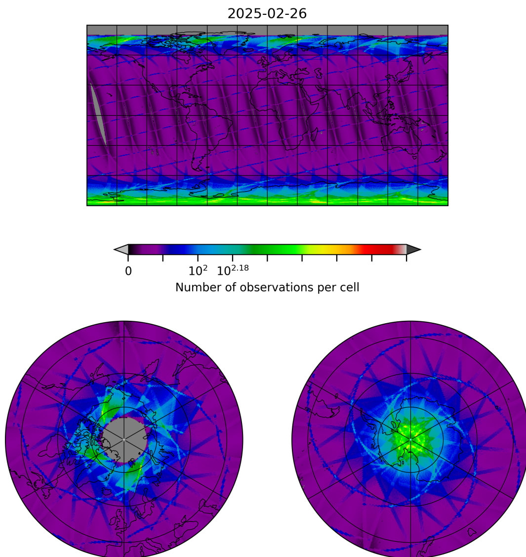
Figure 8: Map of the number of observations for 2025-02-26 to 2025-02-27
