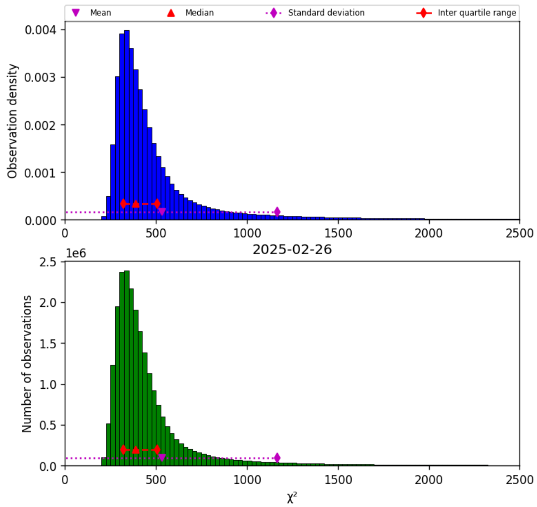
Figure 40: Histogram of “ \chi^2 ” for 2025-02-26 to 2025-02-27
