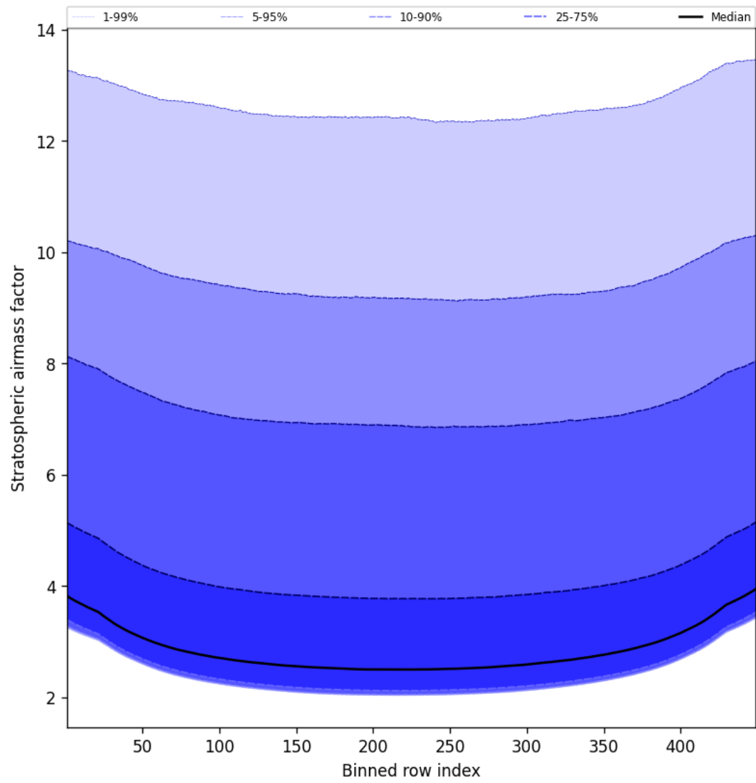
Figure 59: Along track statistics of “Stratospheric airmass factor” for 2025-02-26 to 2025-02-27
