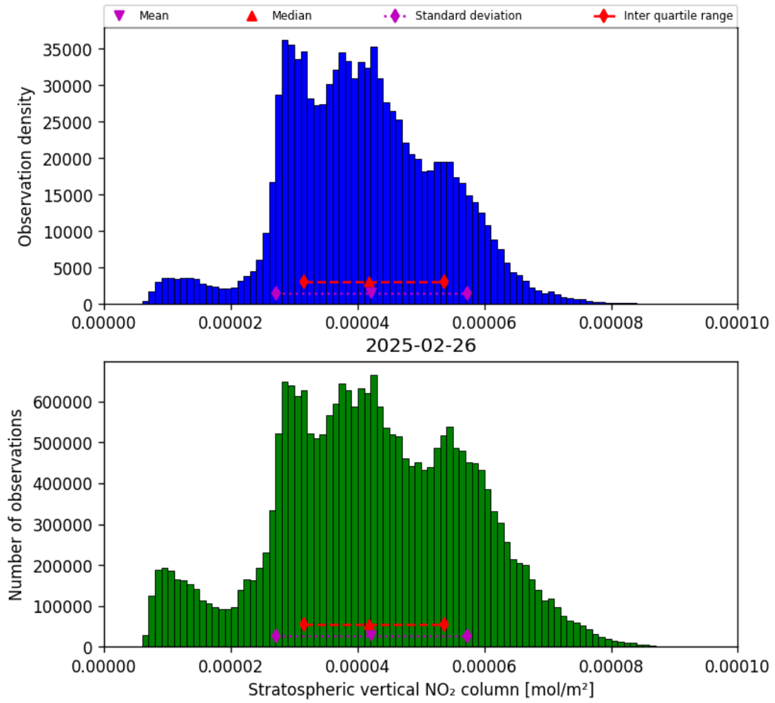
Figure 34: Histogram of “Stratospheric vertical NO 2 column” for 2025-02-26 to 2025-02-27
