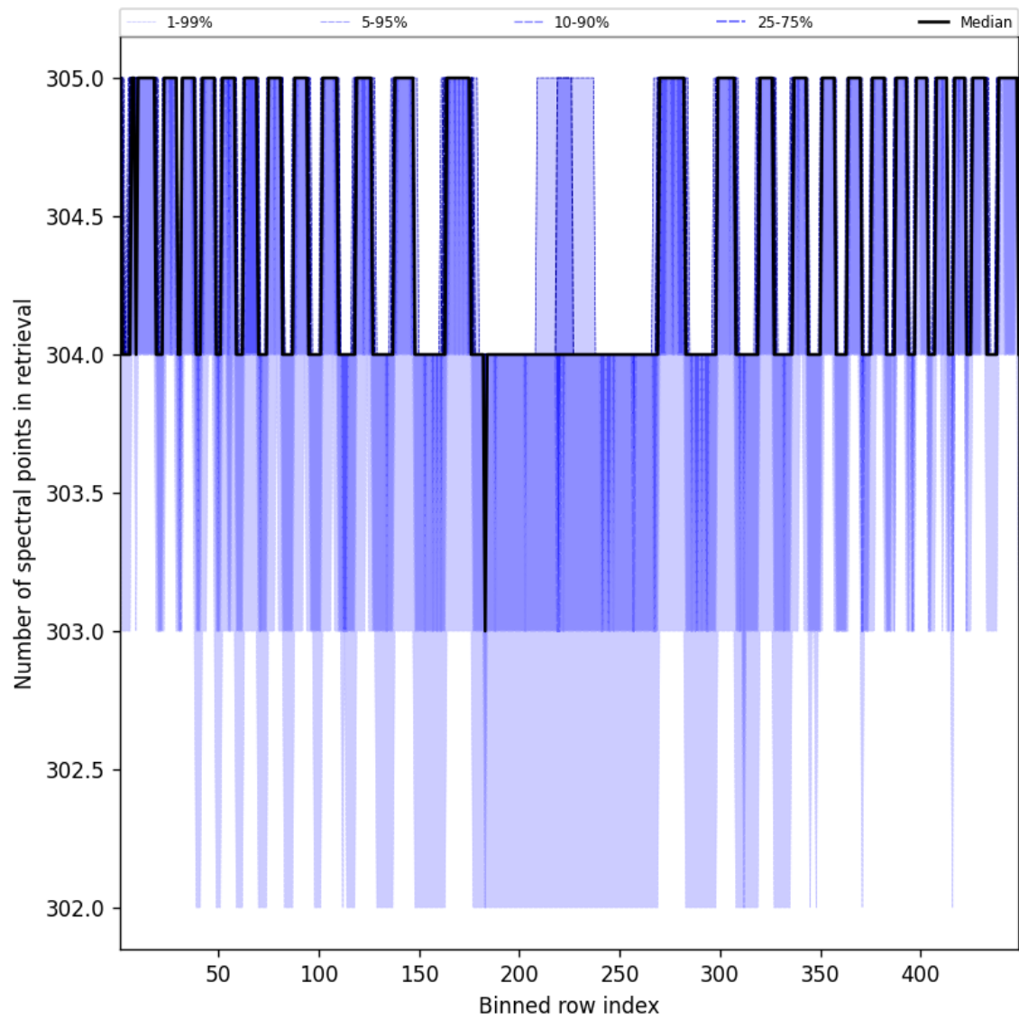
Figure 48: Along track statistics of “Number of spectral points in retrieval” for 2025-02-26 to 2025-02-27
