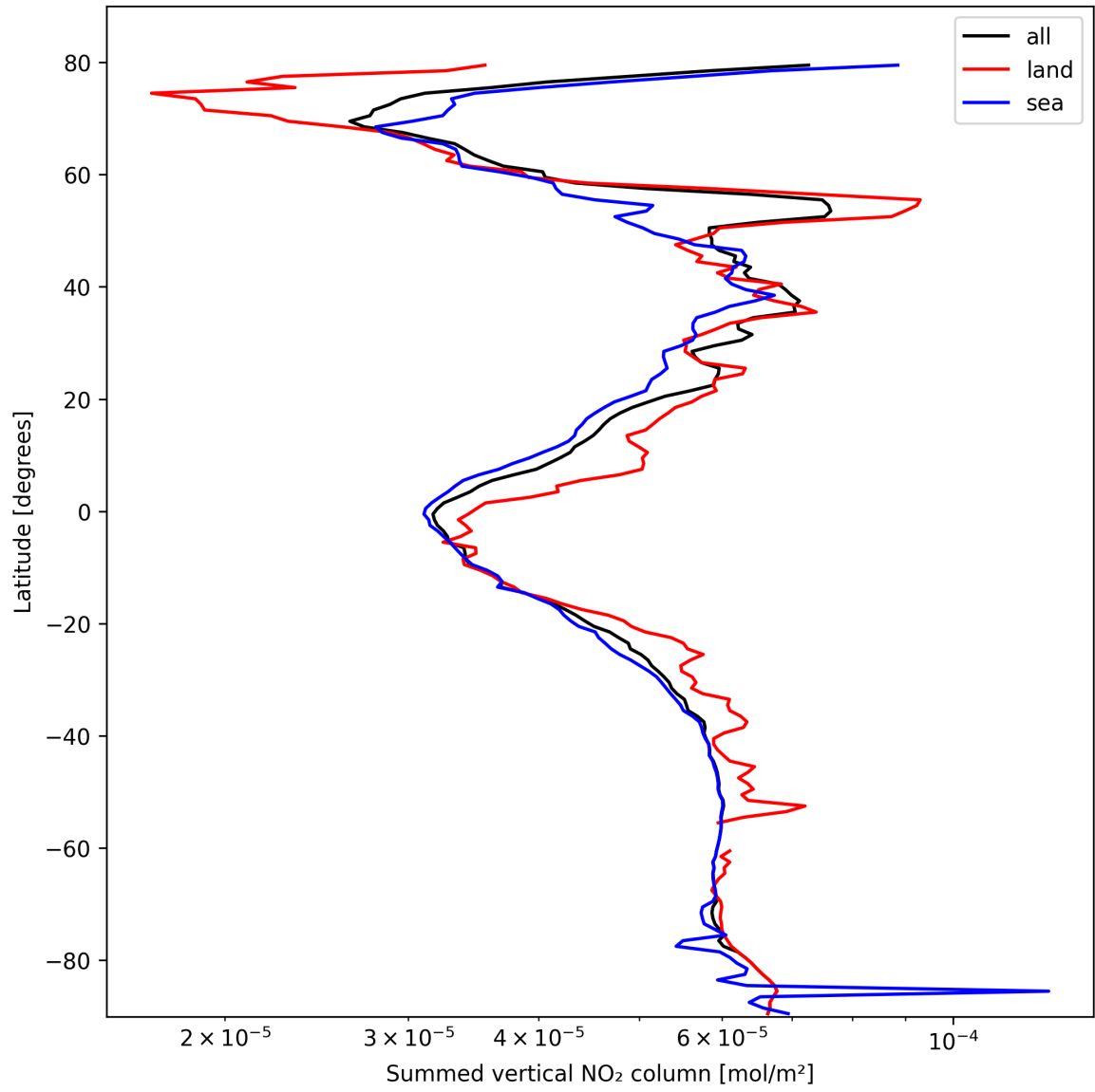
Figure 21: Zonal average of “Summed vertical NO 2 column” for 2025-02-26 to 2025-02-27.
