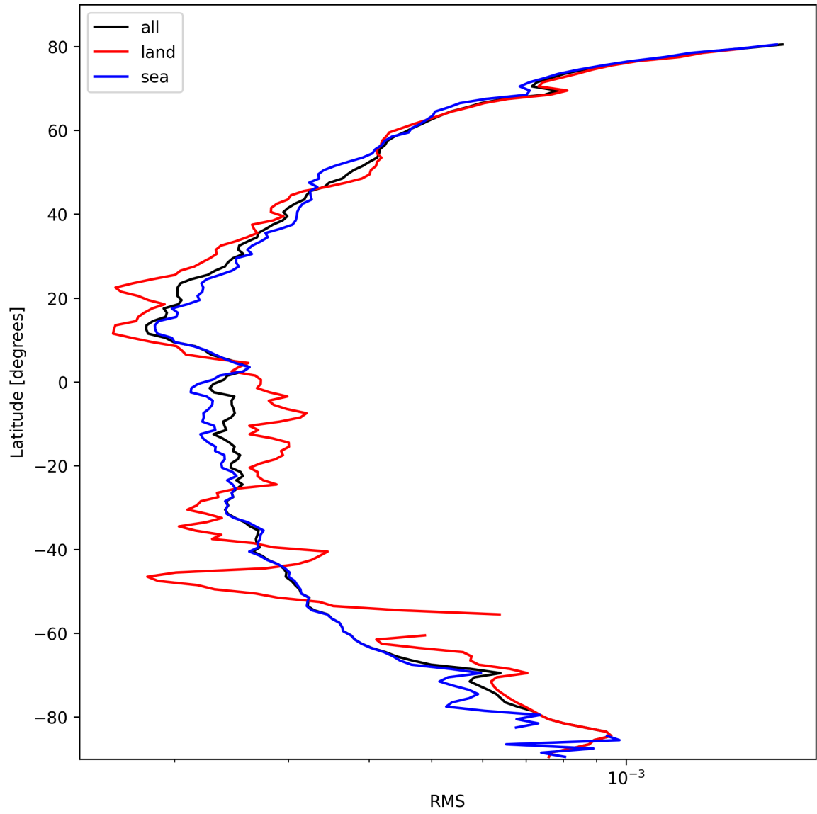
Figure 24: Zonal average of “RMS” for 2025-02-27 to 2025-02-27.
