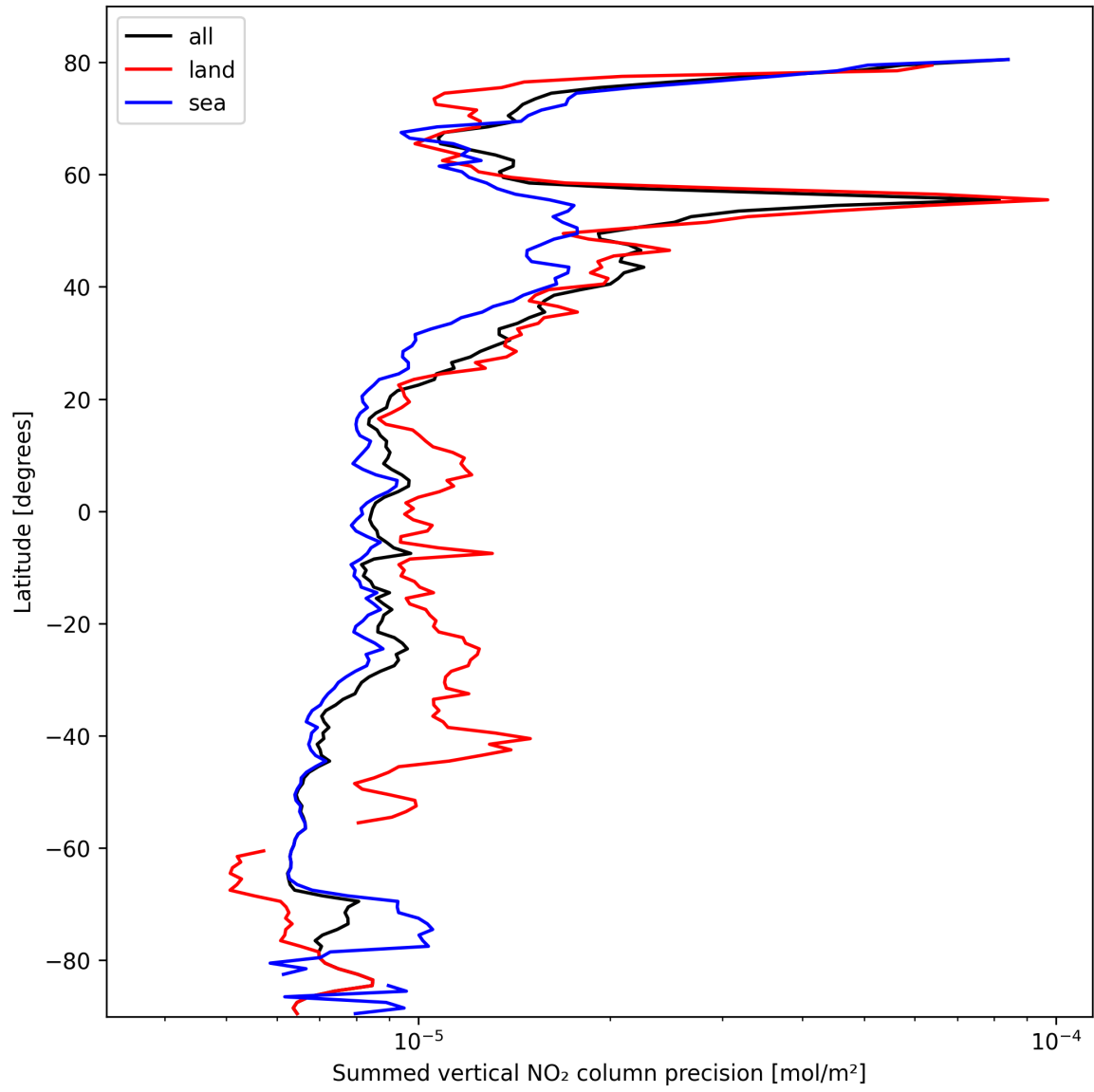
Figure 22: Zonal average of “Summed vertical NO 2 column precision” for 2025-02-27 to 2025-02-27.
