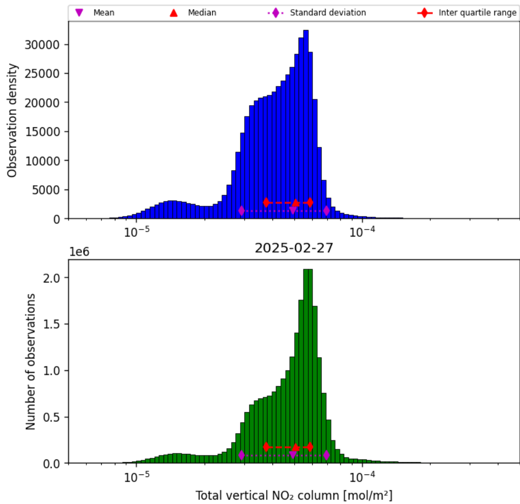
Figure 36: Histogram of "Total vertical NO 2 column" for 2025-02-27 to 2025-02-27
