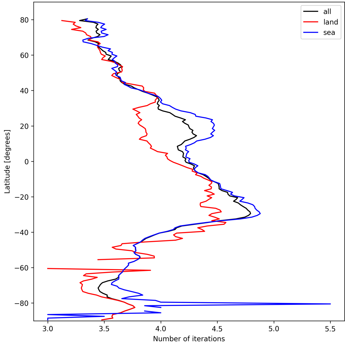
Figure 15: Zonal average of “Number of iterations” for 2025-02-27 to 2025-02-27.
