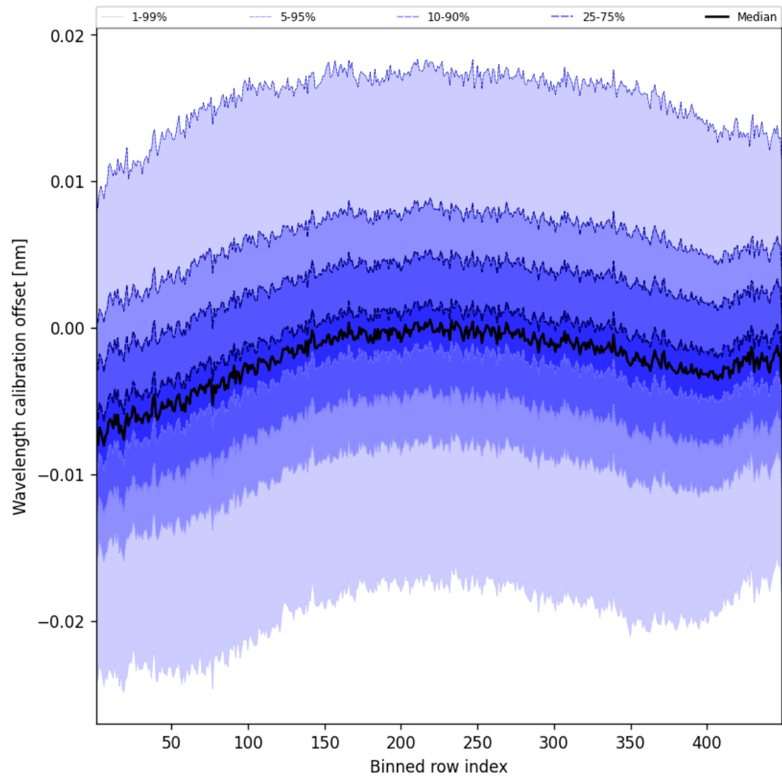
Figure 50: Along track statistics of “Wavelength calibration offset” for 2025-02-27 to 2025-02-27
