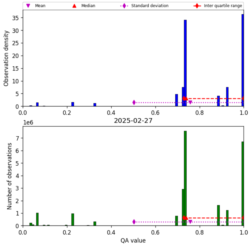
Figure 26: Histogram of “QA value” for 2025-02-27 to 2025-02-27
