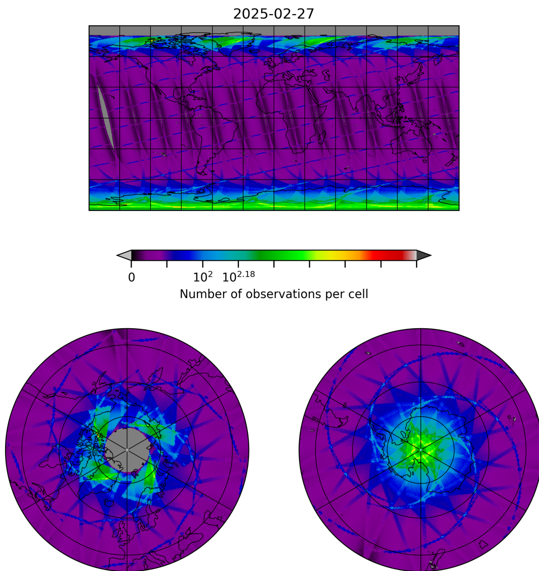
Figure 8: Map of the number of observations for 2025-02-27 to 2025-02-27
