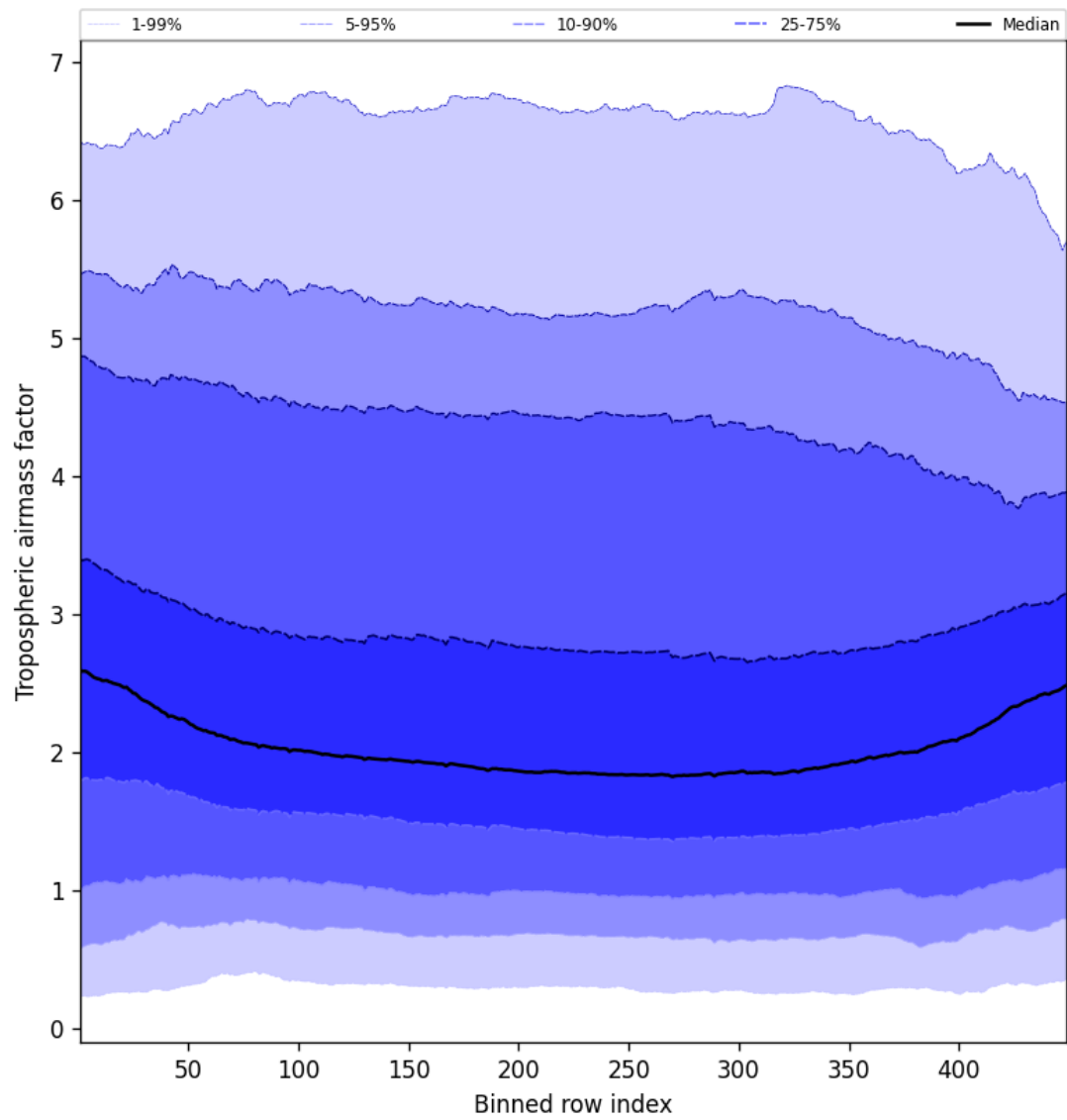
Figure 46: Along track statistics of “Tropospheric airmass factor” for 2025-02-27 to 2025-02-27
