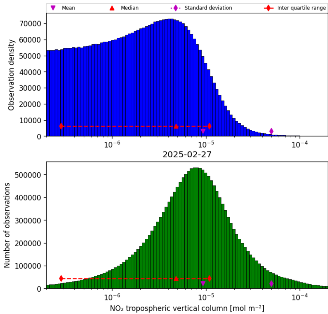
Figure 27: Histogram of “NO 2 tropospheric vertical column” for 2025-02-27 to 2025-02-27
