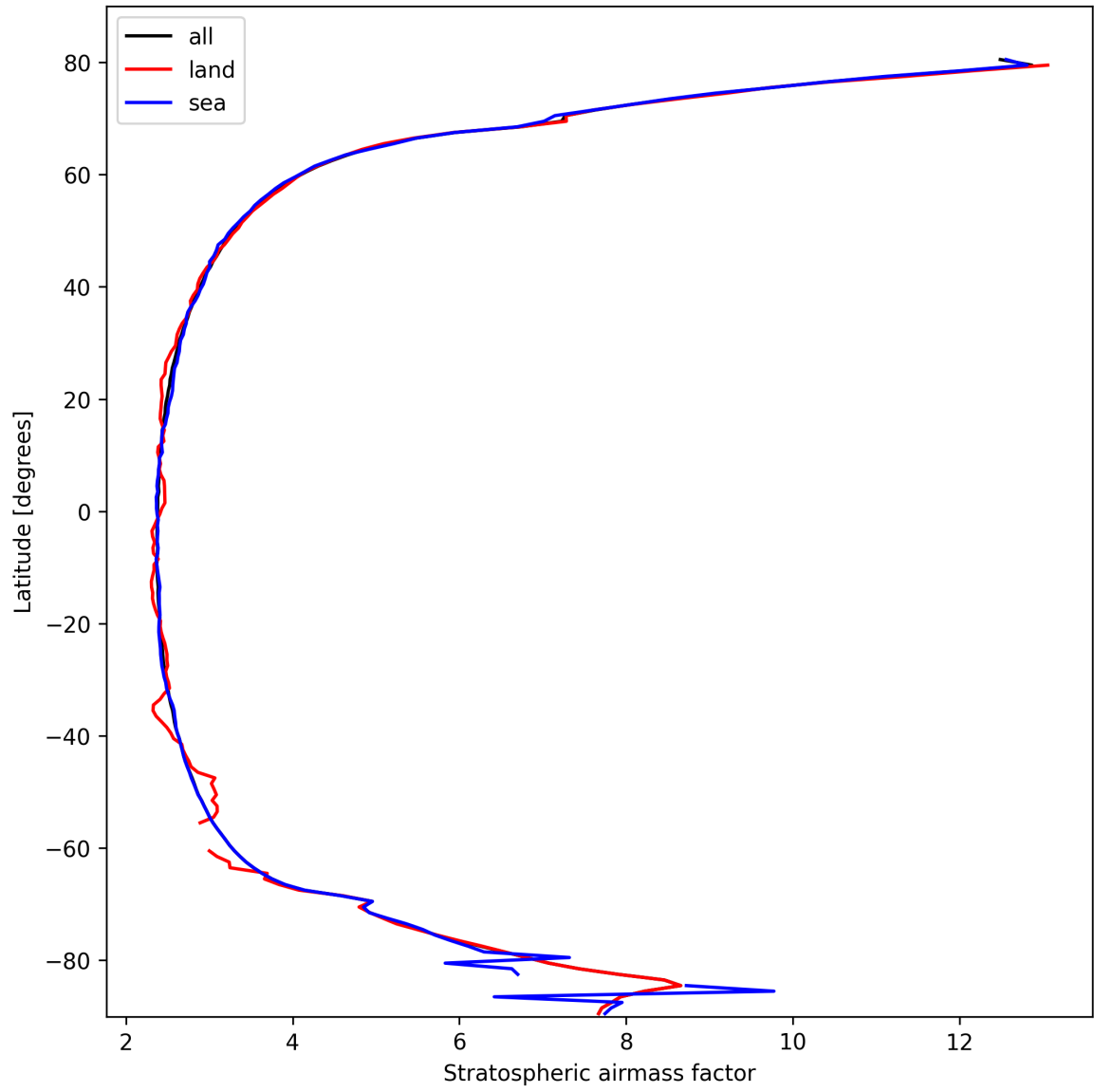
Figure 25: Zonal average of “Stratospheric air mass factor” for 2025-02-27 to 2025-02-27.
