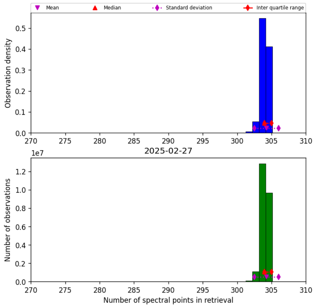
Figure 31: Histogram of “Number of spectral points in retrieval” for 2025-02-27 to 2025-02-27
