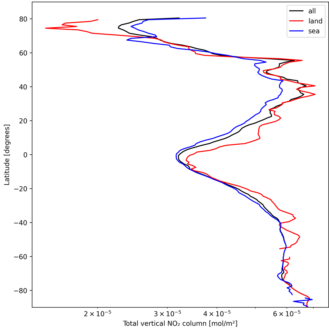
Figure 19: Zonal average of “Total vertical NO 2 column” for 2025-02-27 to 2025-02-27.
