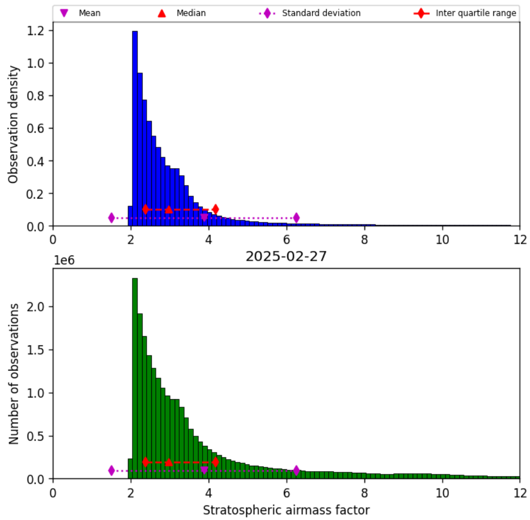
Figure 42: Histogram of “Stratospheric airmass factor” for 2025-02-27 to 2025-02-27
