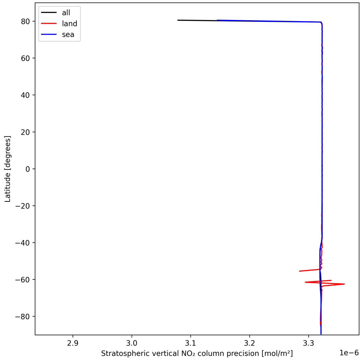
Figure 18: Zonal average of “Stratospheric vertical NO 2 column precision” for 2025-02-27 to 2025-02-27.
