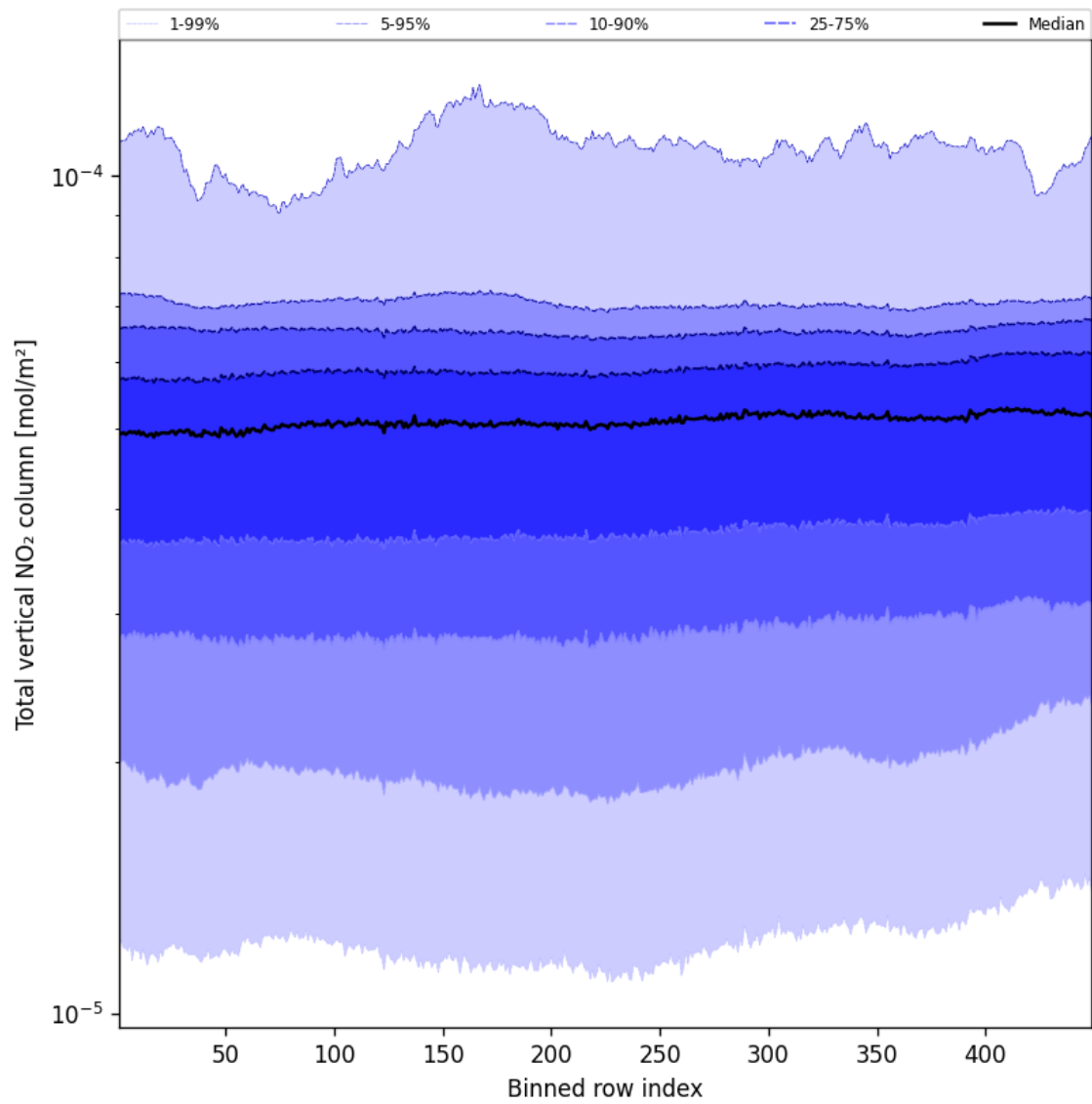
Figure 53: Along track statistics of “Total vertical NO 2 column” for 2025-02-27 to 2025-02-27
