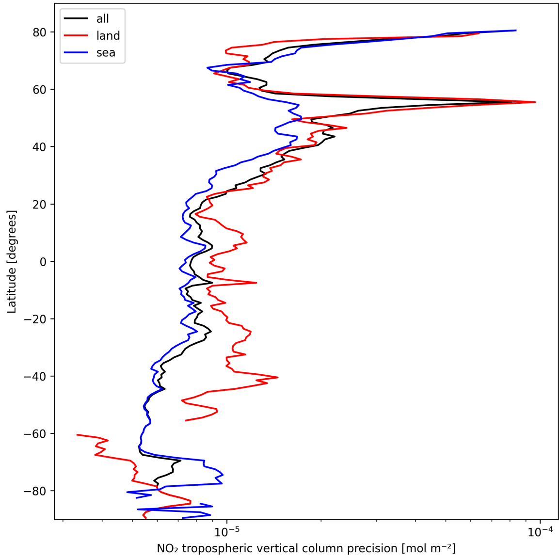
Figure 11: Zonal average of “NO 2 tropospheric vertical column precision” for 2025-02-27 to 2025-02-27.
