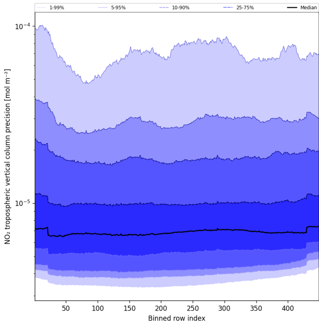
Figure 45: Along track statistics of “NO 2 tropospheric vertical column precision” for 2025-02-27 to 2025-02-27
