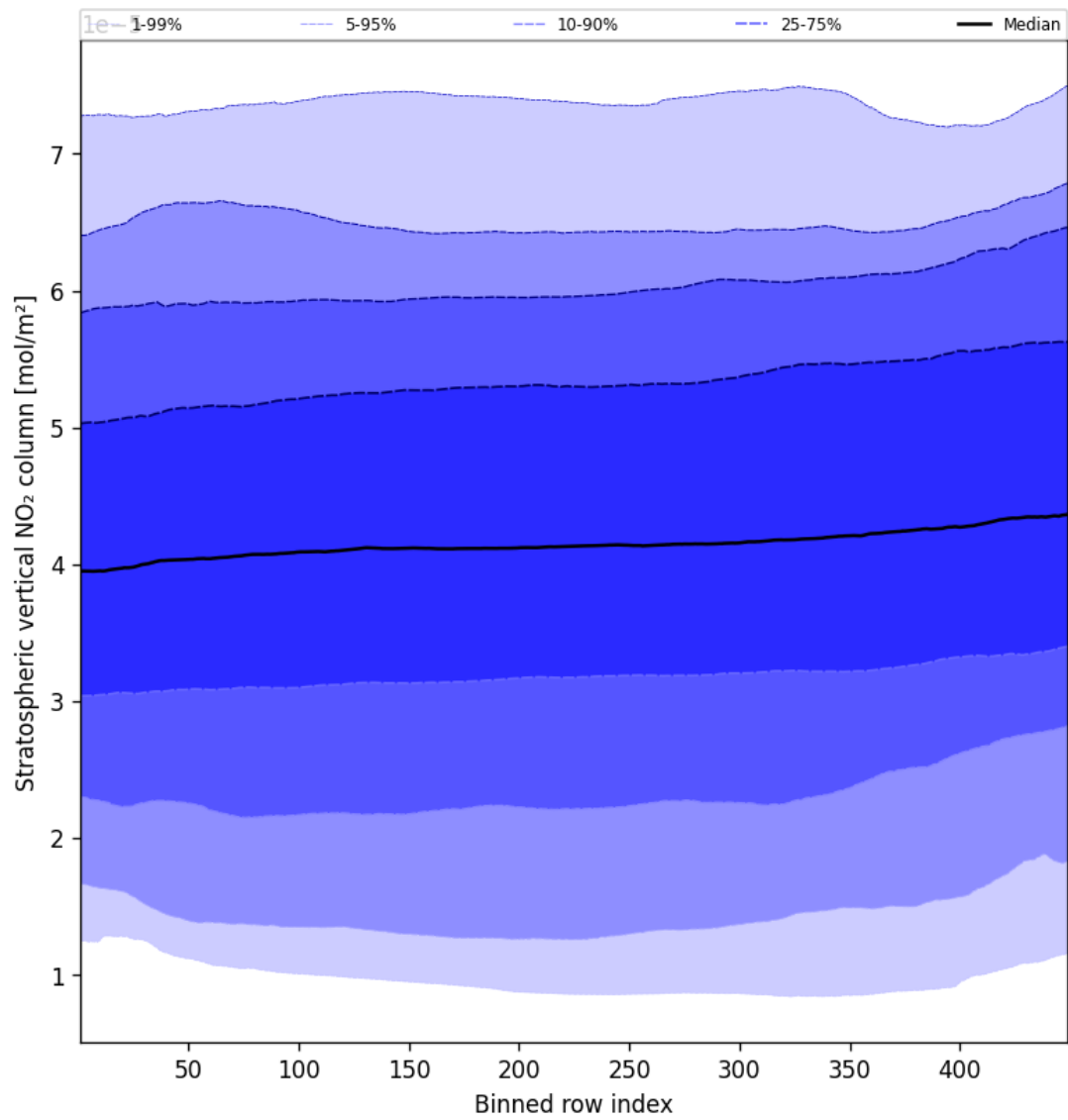
Figure 51: Along track statistics of "Stratospheric vertical NO 2 column" for 2025-02-27 to 2025-02-27
