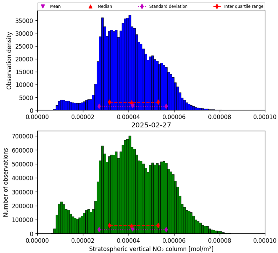
Figure 34: Histogram of “Stratospheric vertical NO 2 column” for 2025-02-27 to 2025-02-27
