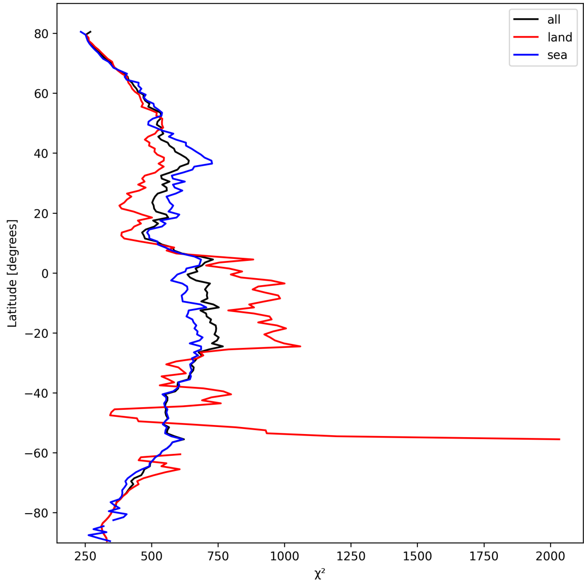
Figure 23: Zonal average of “ \chi^2 ” for 2025-02-27 to 2025-02-27.
