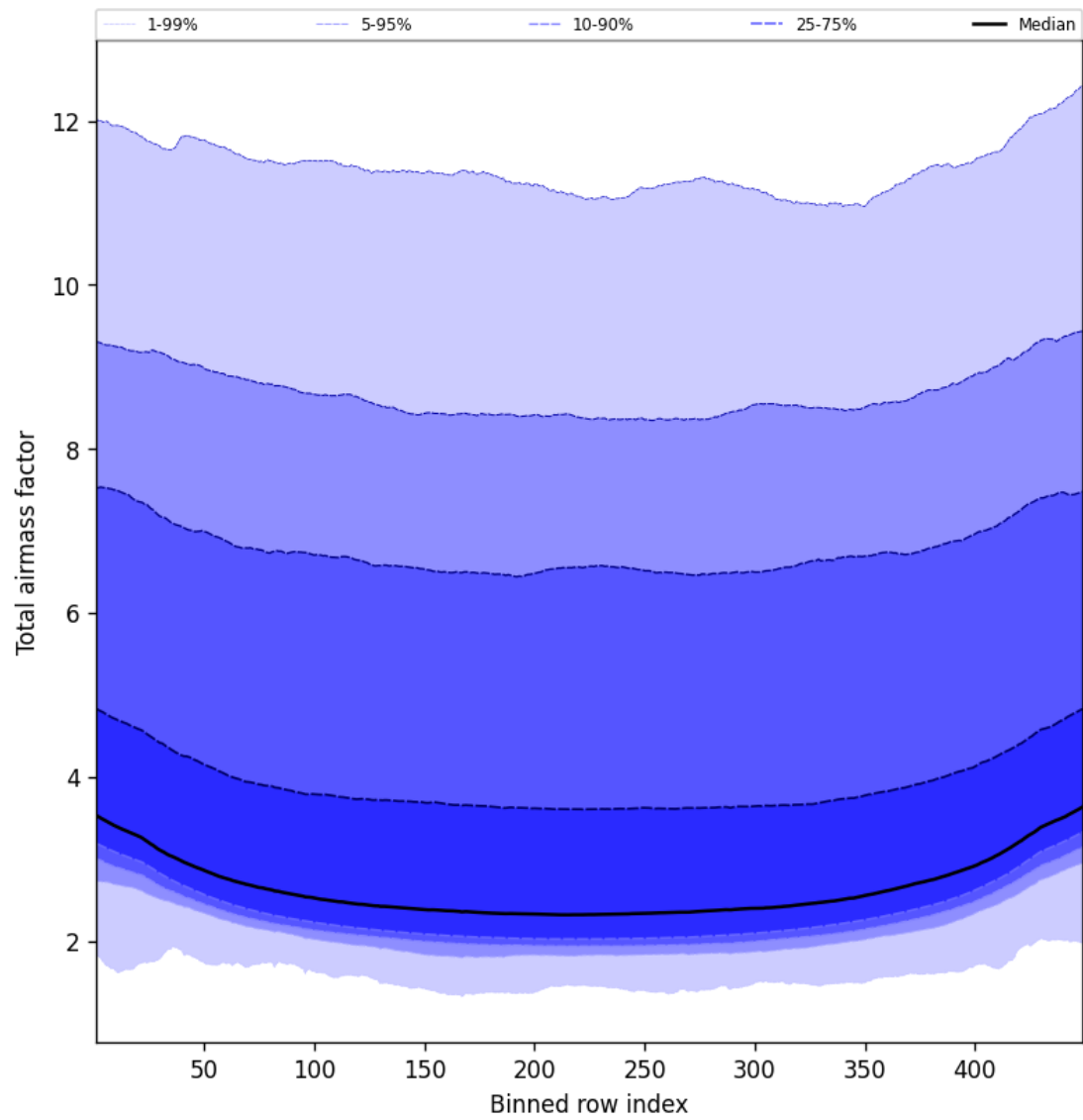
Figure 47: Along track statistics of “Total airmass factor” for 2025-02-27 to 2025-02-27
