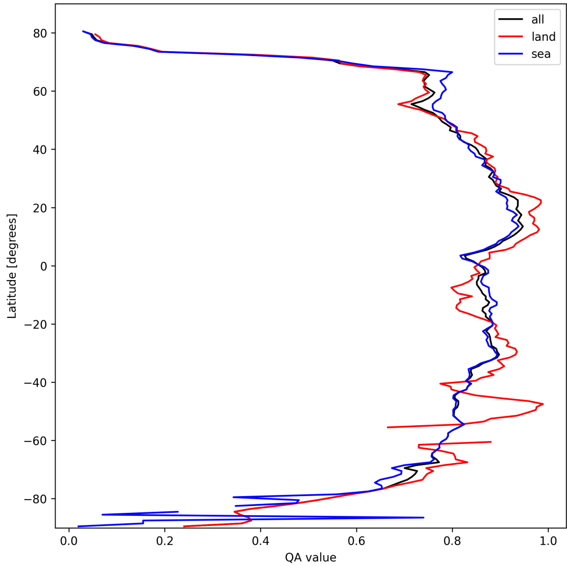
Figure 9: Zonal average of “QA value” for 2025-02-27 to 2025-02-27.
