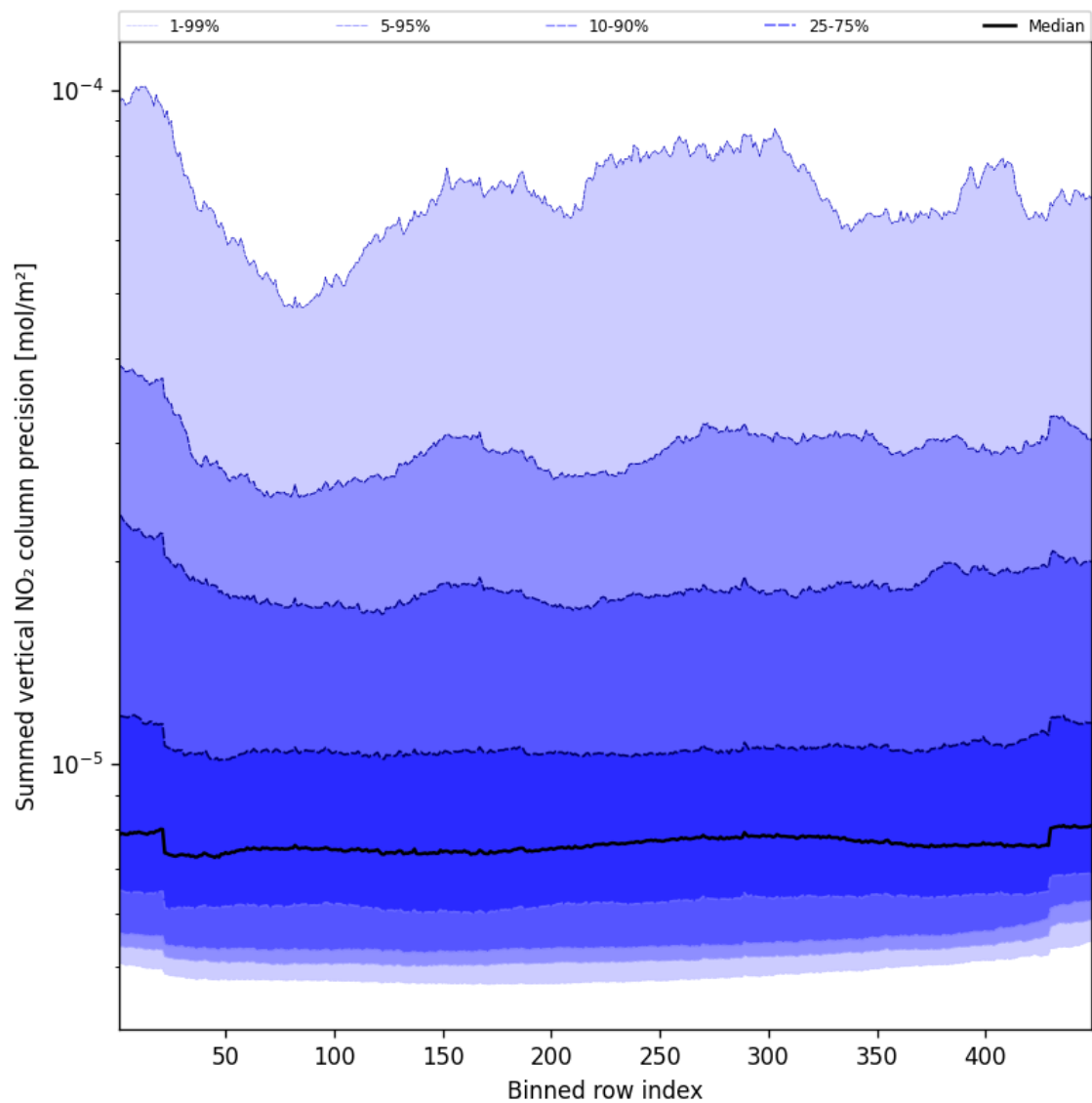
Figure 56: Along track statistics of “Summed vertical NO 2 column precision” for 2025-02-27 to 2025-02-27
