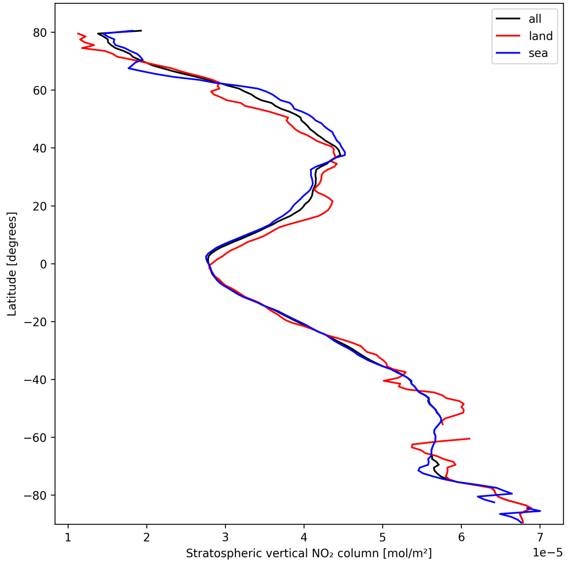
Figure 17: Zonal average of “Stratospheric vertical NO 2 column” for 2025-02-27 to 2025-02-27.
