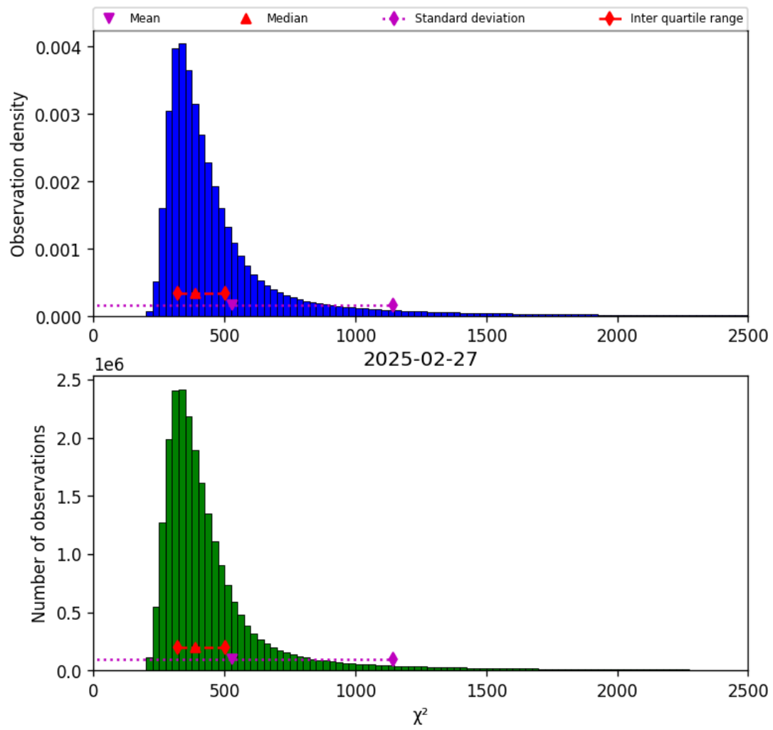
Figure 40: Histogram of “ \chi^2 ” for 2025-02-27 to 2025-02-27
