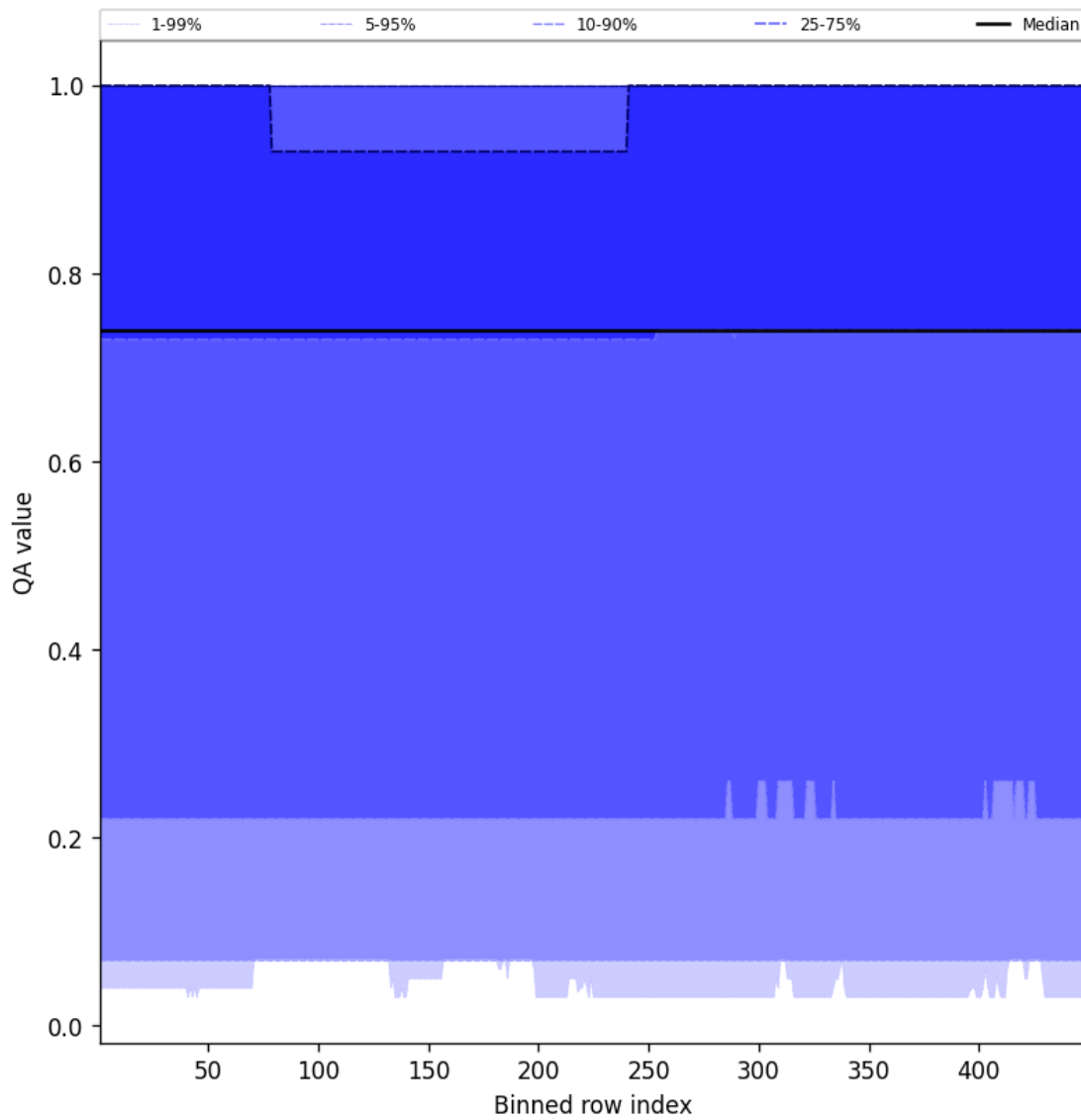
Figure 43: Along track statistics of “QA value” for 2025-02-27 to 2025-02-27
