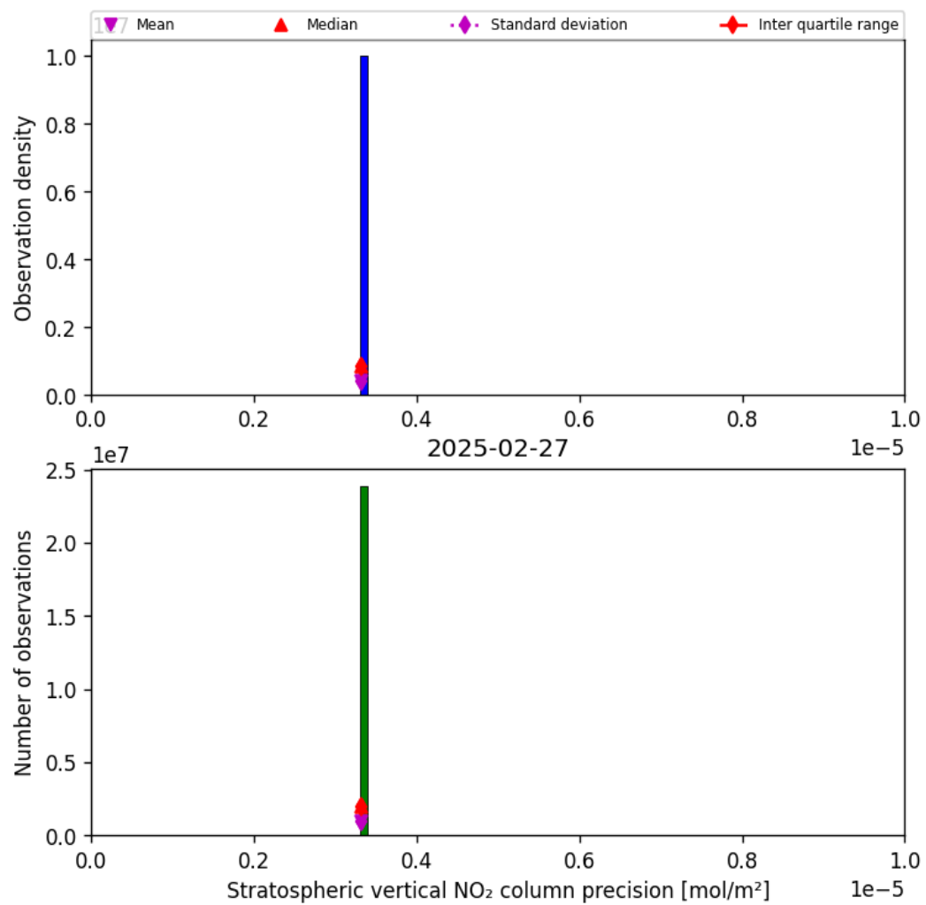
Figure 35: Histogram of “Stratospheric vertical NO 2 column precision” for 2025-02-27 to 2025-02-27
