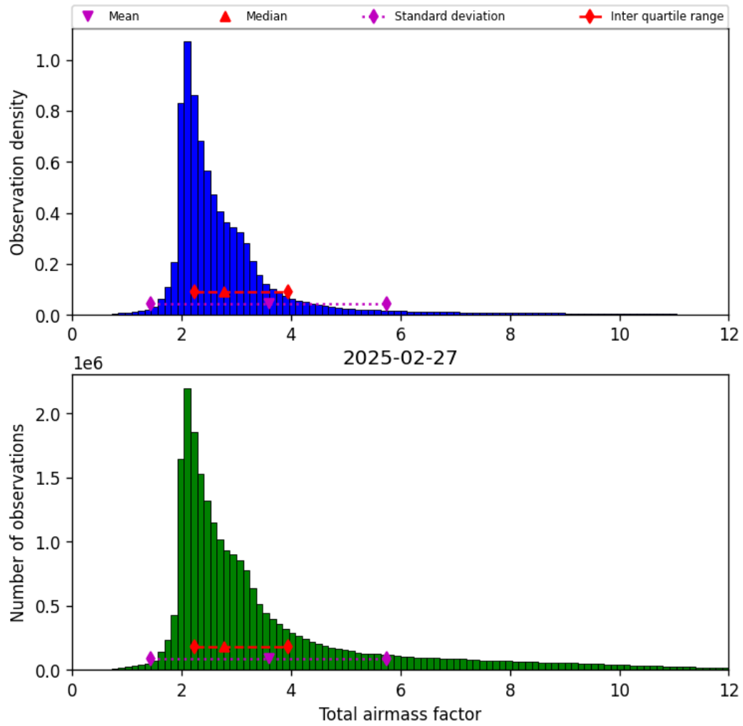
Figure 30: Histogram of “Total airmass factor” for 2025-02-27 to 2025-02-27
