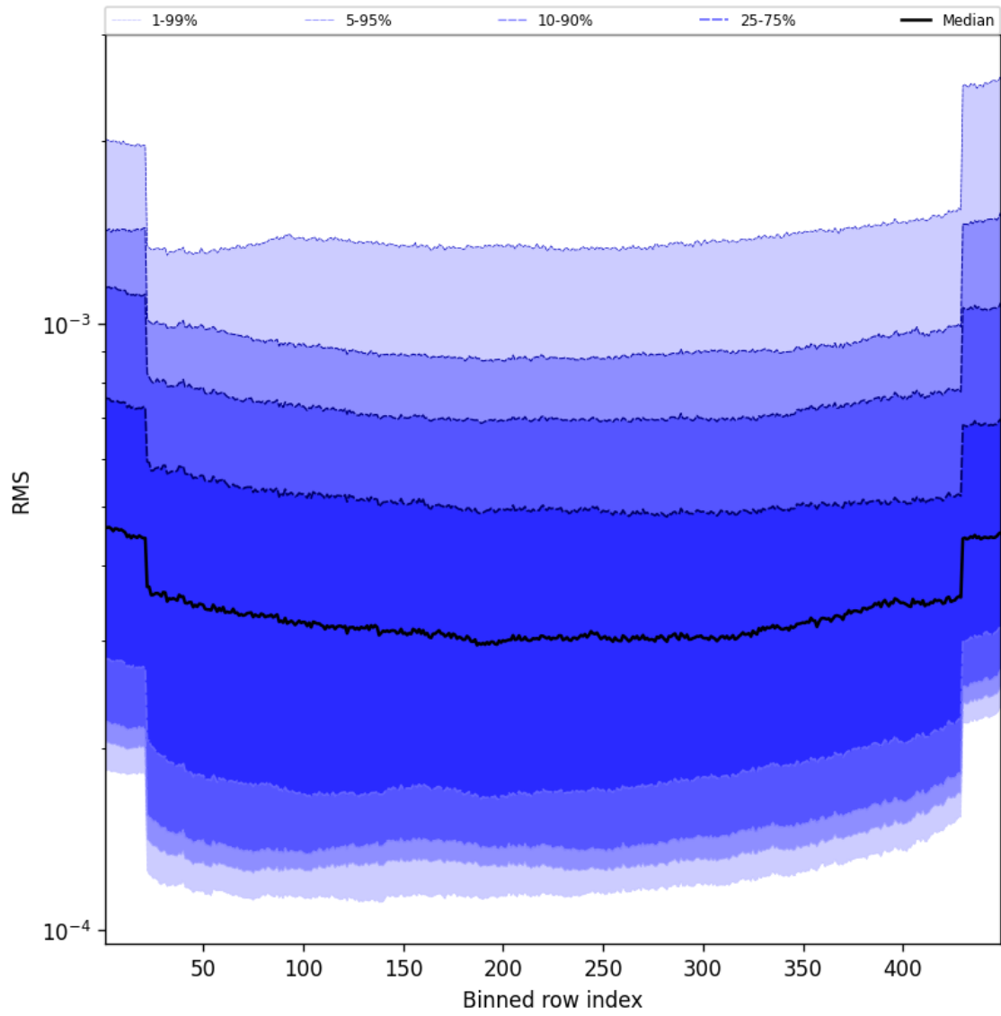
Figure 58: Along track statistics of “RMS” for 2025-02-27 to 2025-02-27
