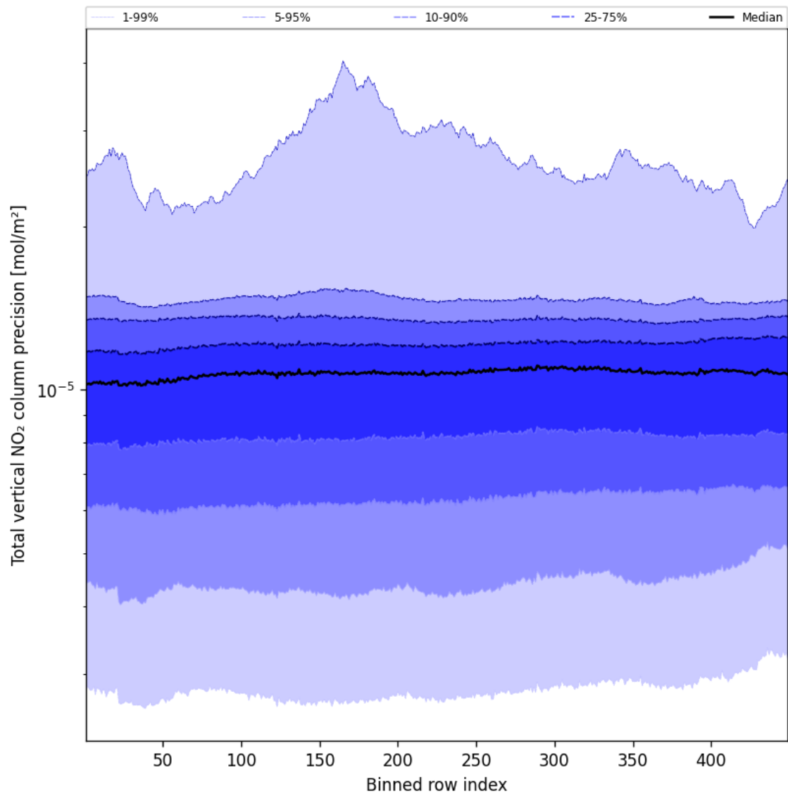
Figure 54: Along track statistics of “Total vertical NO 2 column precision” for 2025-02-27 to 2025-02-27
