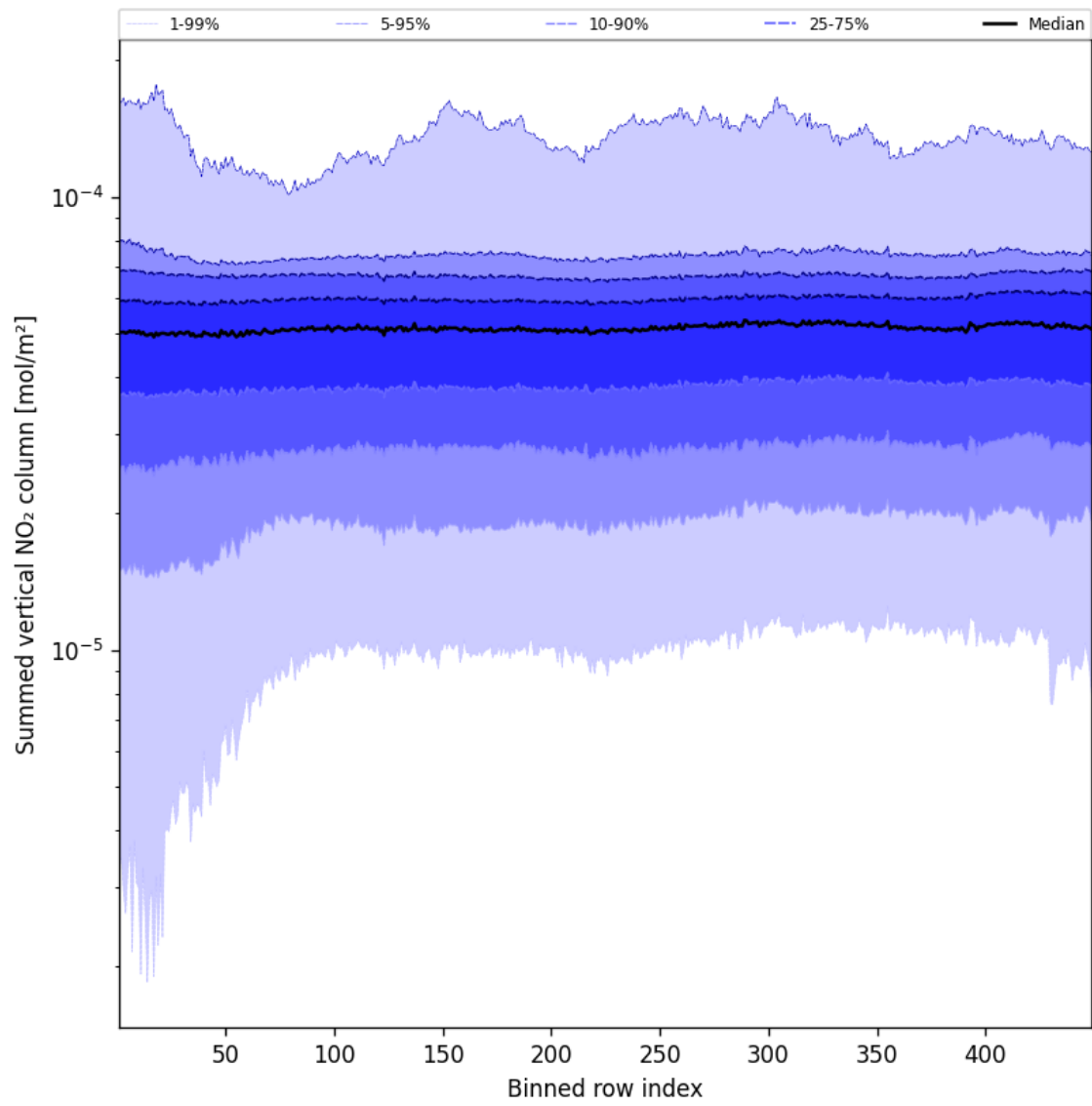
Figure 55: Along track statistics of “Summed vertical NO 2 column” for 2025-02-27 to 2025-02-27
