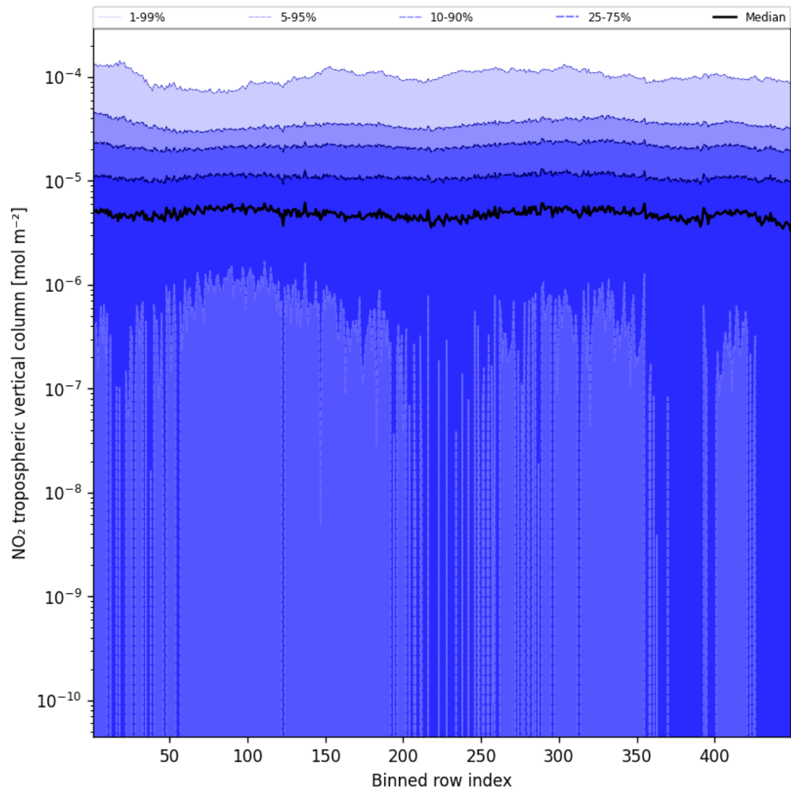
Figure 44: Along track statistics of “NO 2 tropospheric vertical column” for 2025-02-27 to 2025-02-27
