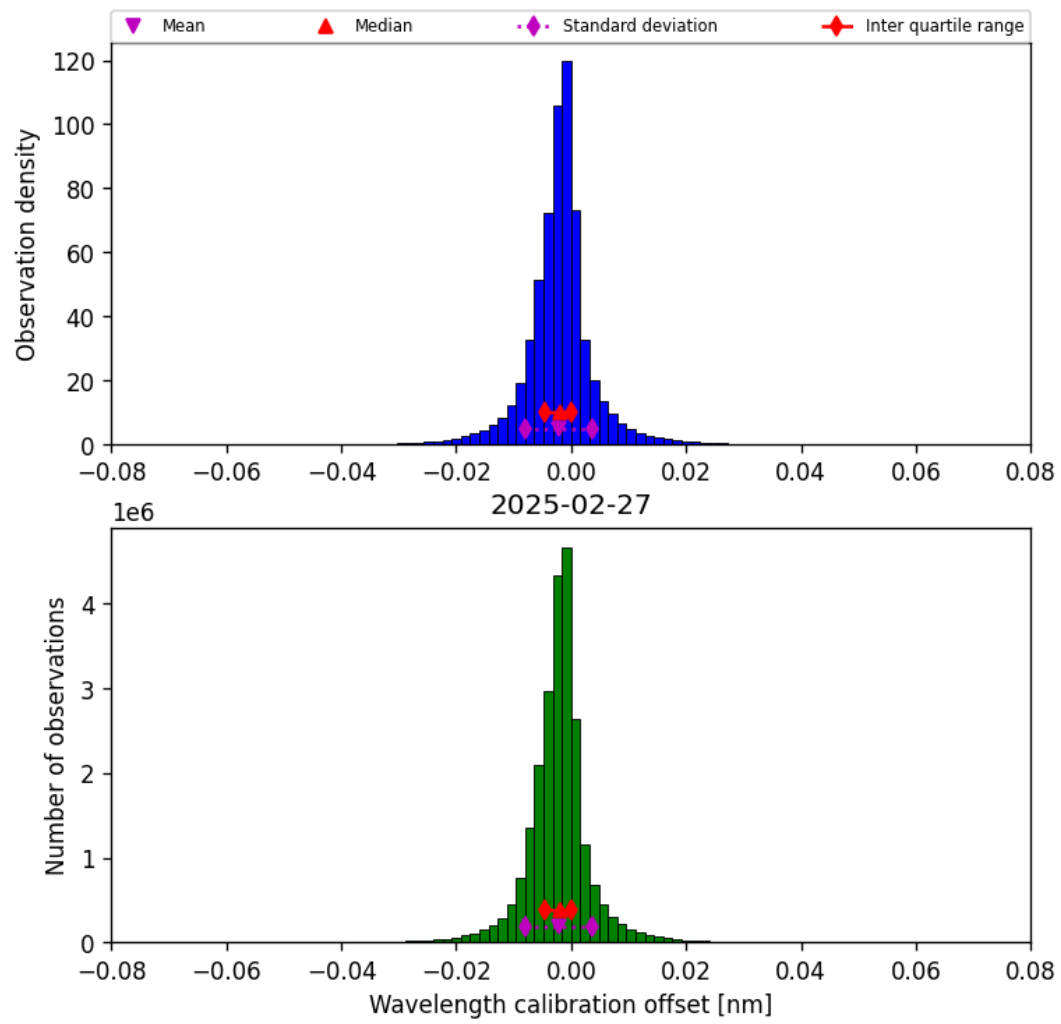
Figure 33: Histogram of “Wavelength calibration offset” for 2025-02-27 to 2025-02-27
