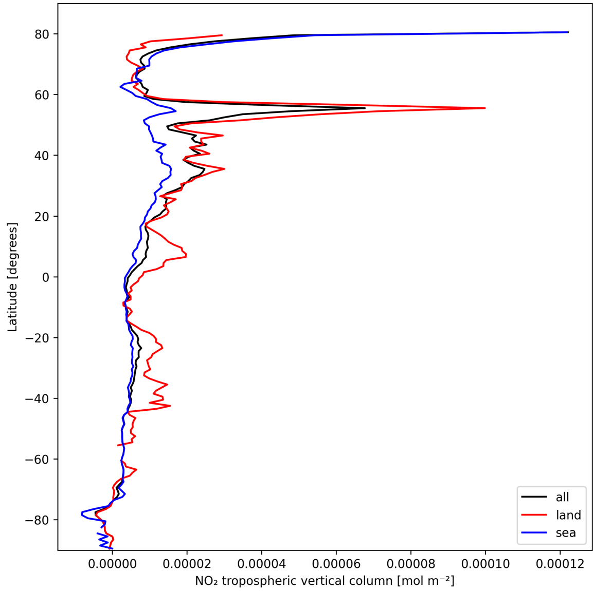
Figure 10: Zonal average of “NO 2 tropospheric vertical column” for 2025-02-27 to 2025-02-27.
