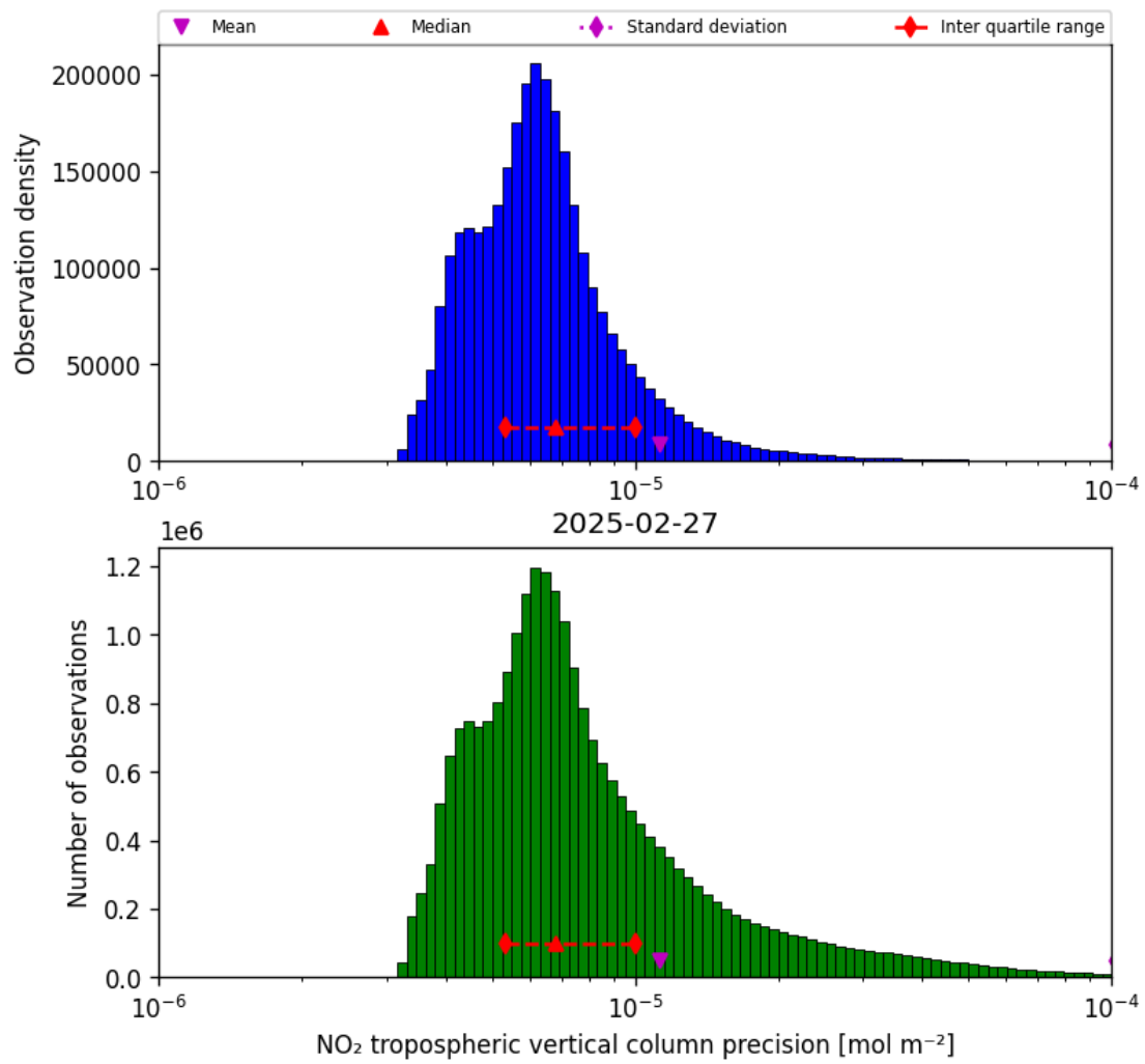
Figure 28: Histogram of “NO 2 tropospheric vertical column precision” for 2025-02-27 to 2025-02-27
