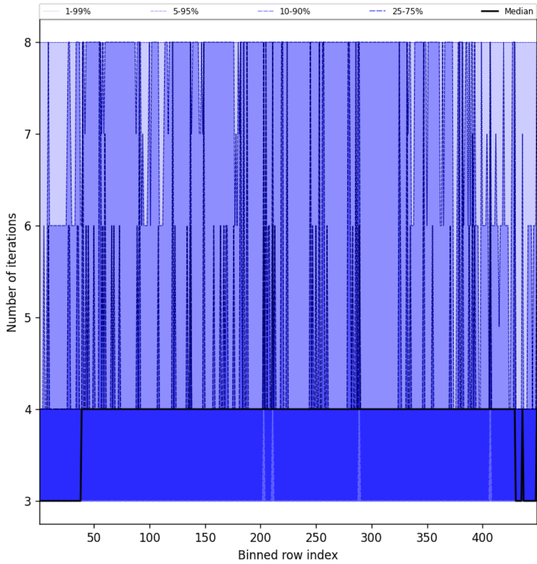
Figure 49: Along track statistics of “Number of iterations” for 2025-02-27 to 2025-02-27
