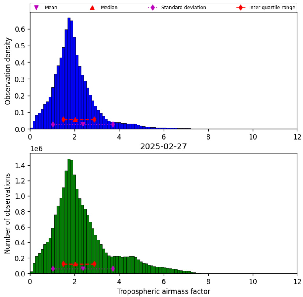
Figure 29: Histogram of “Tropospheric airmass factor” for 2025-02-27 to 2025-02-27
