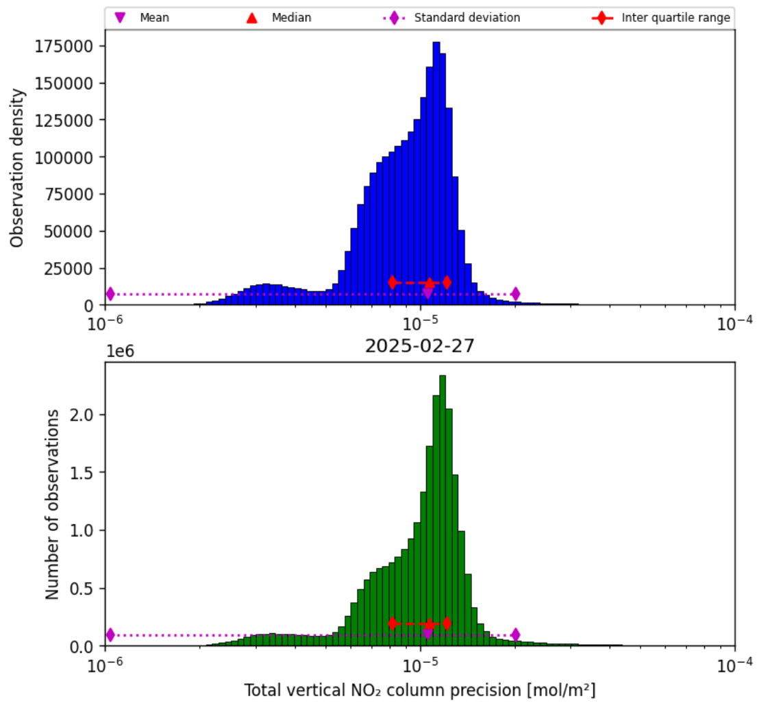
Figure 37: Histogram of "Total vertical NO 2 column precision" for 2025-02-27 to 2025-02-27
