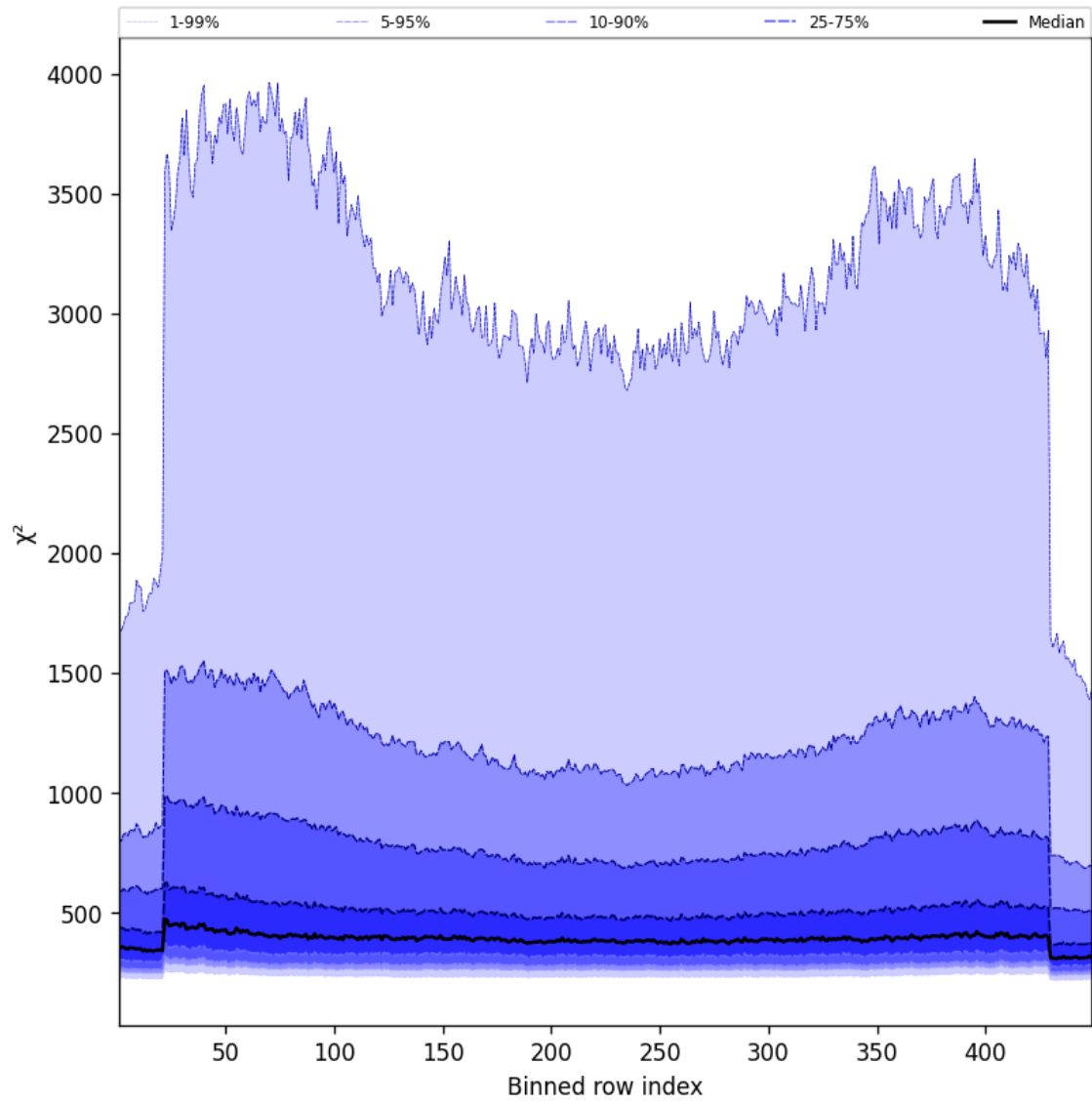
Figure 57: Along track statistics of “ \chi^2 ” for 2025-02-27 to 2025-02-27
