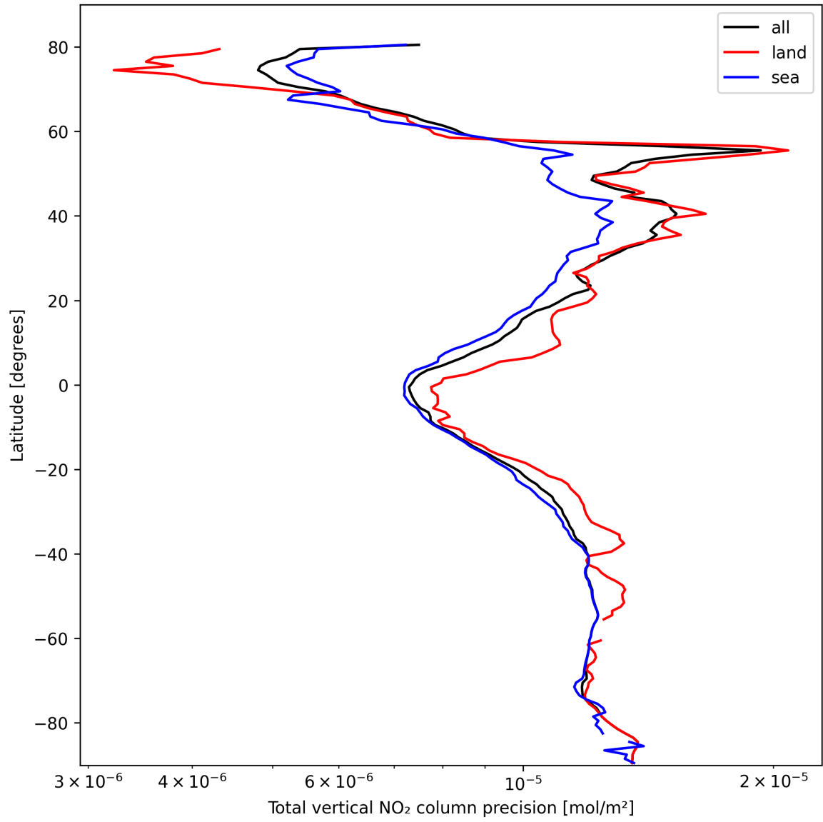
Figure 20: Zonal average of “Total vertical NO 2 column precision” for 2025-02-27 to 2025-02-27.
