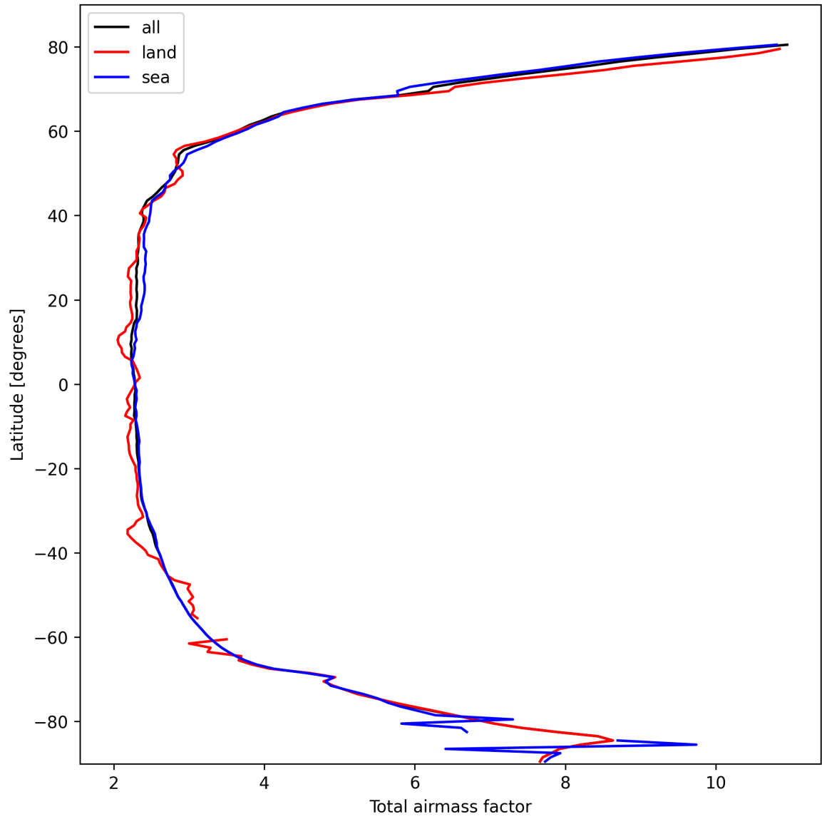
Figure 13: Zonal average of “Total airmass factor” for 2025-02-27 to 2025-02-27.
