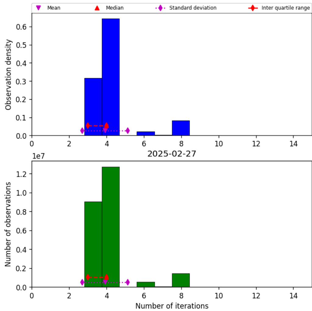
Figure 32: Histogram of “Number of iterations” for 2025-02-27 to 2025-02-27
