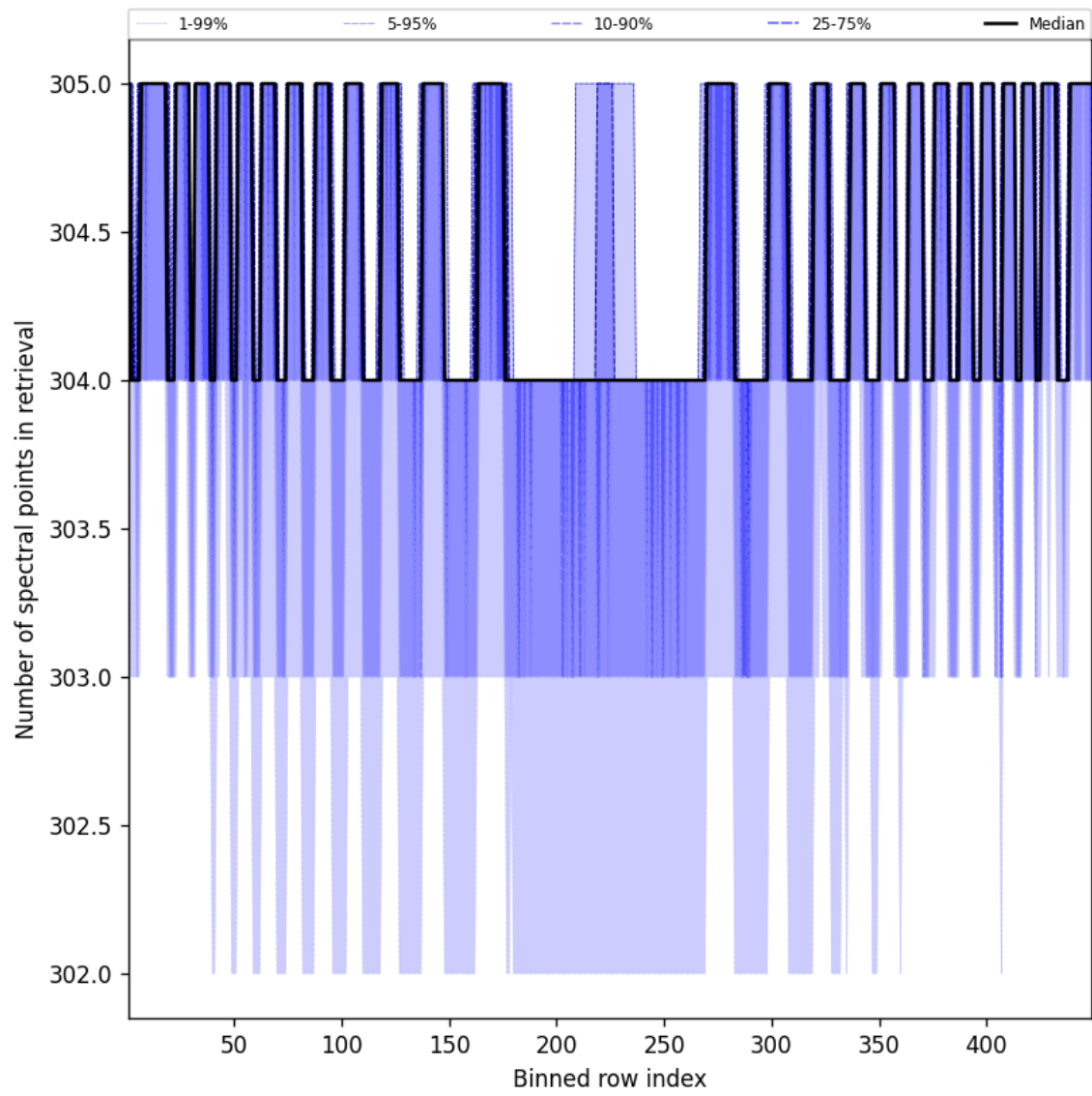
Figure 48: Along track statistics of “Number of spectral points in retrieval” for 2025-02-27 to 2025-02-27
