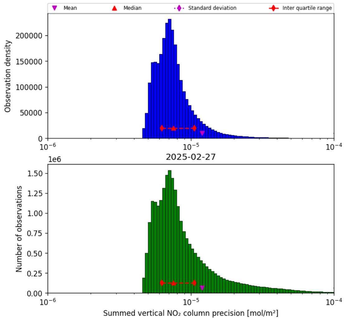
Figure 39: Histogram of "Summed vertical NO 2 column precision" for 2025-02-27 to 2025-02-27
