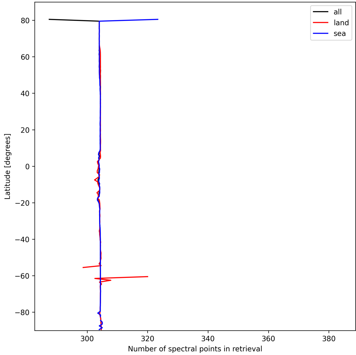
Figure 14: Zonal average of “Number of spectral points in retrieval” for 2025-02-27 to 2025-02-27.
