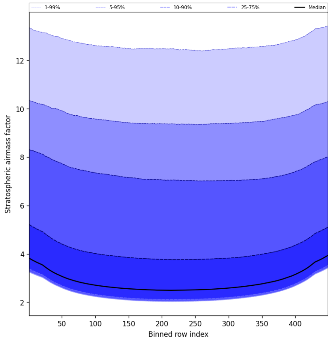
Figure 59: Along track statistics of “Stratospheric airmass factor” for 2025-02-27 to 2025-02-27
