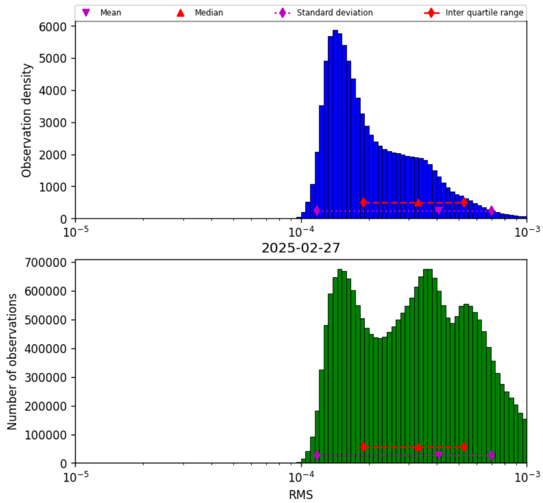
Figure 41: Histogram of “RMS” for 2025-02-27 to 2025-02-27
