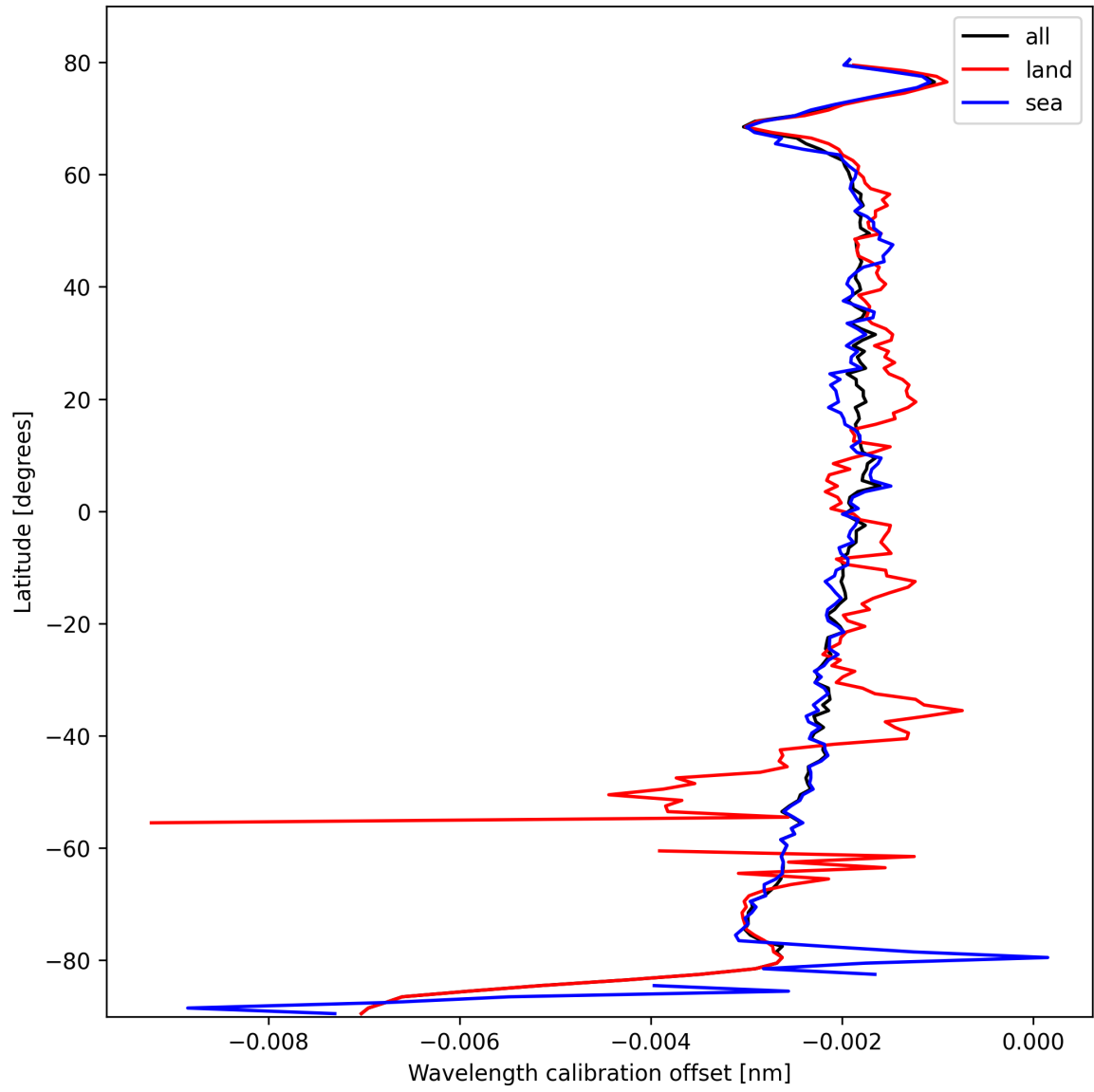
Figure 16: Zonal average of “Wavelength calibration offset” for 2025-02-27 to 2025-02-27.
