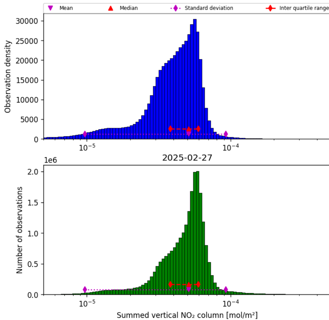
Figure 38: Histogram of “Summed vertical NO 2 column” for 2025-02-27 to 2025-02-27
