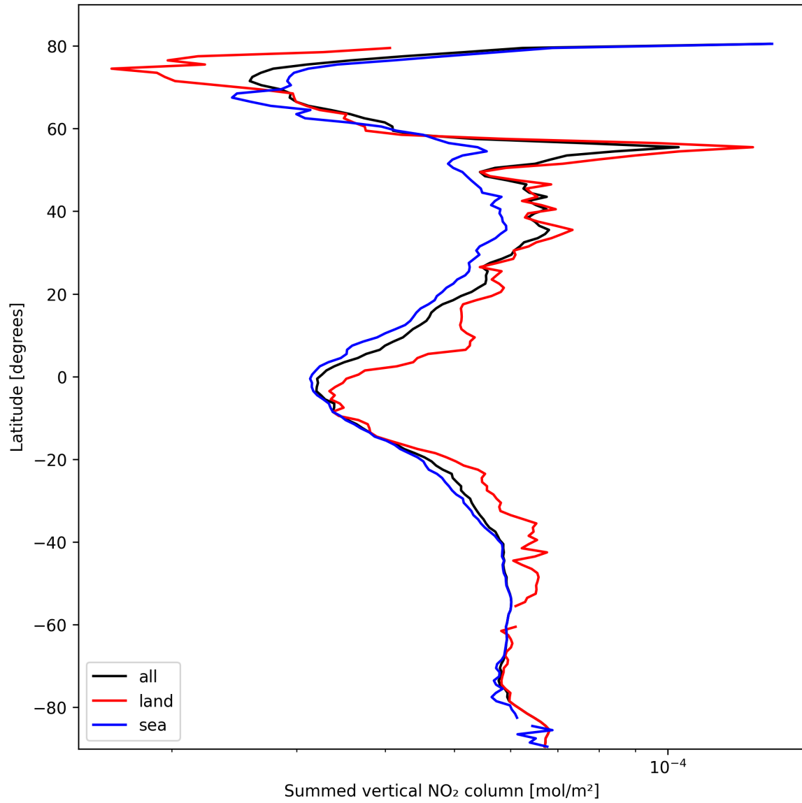
Figure 21: Zonal average of “Summed vertical NO 2 column” for 2025-02-27 to 2025-02-27.
