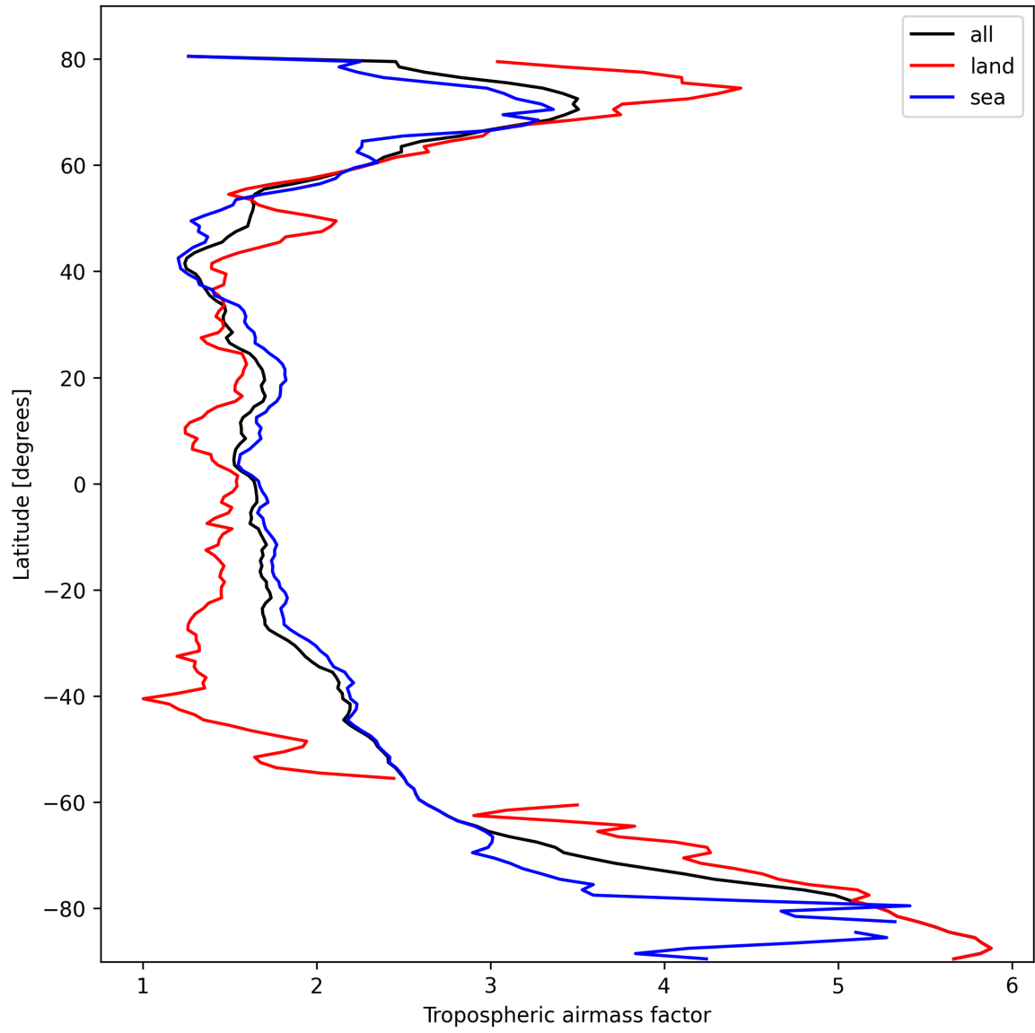
Figure 12: Zonal average of “Tropospheric airmass factor” for 2025-02-27 to 2025-02-27.
