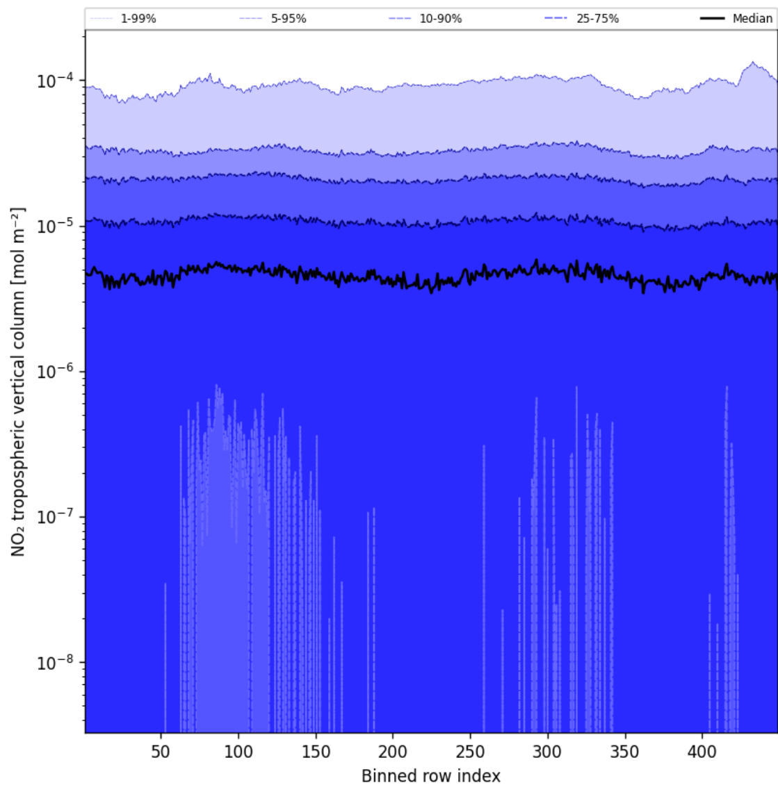
Figure 44: Along track statistics of “NO 2 tropospheric vertical column” for 2025-02-28 to 2025-03-01
