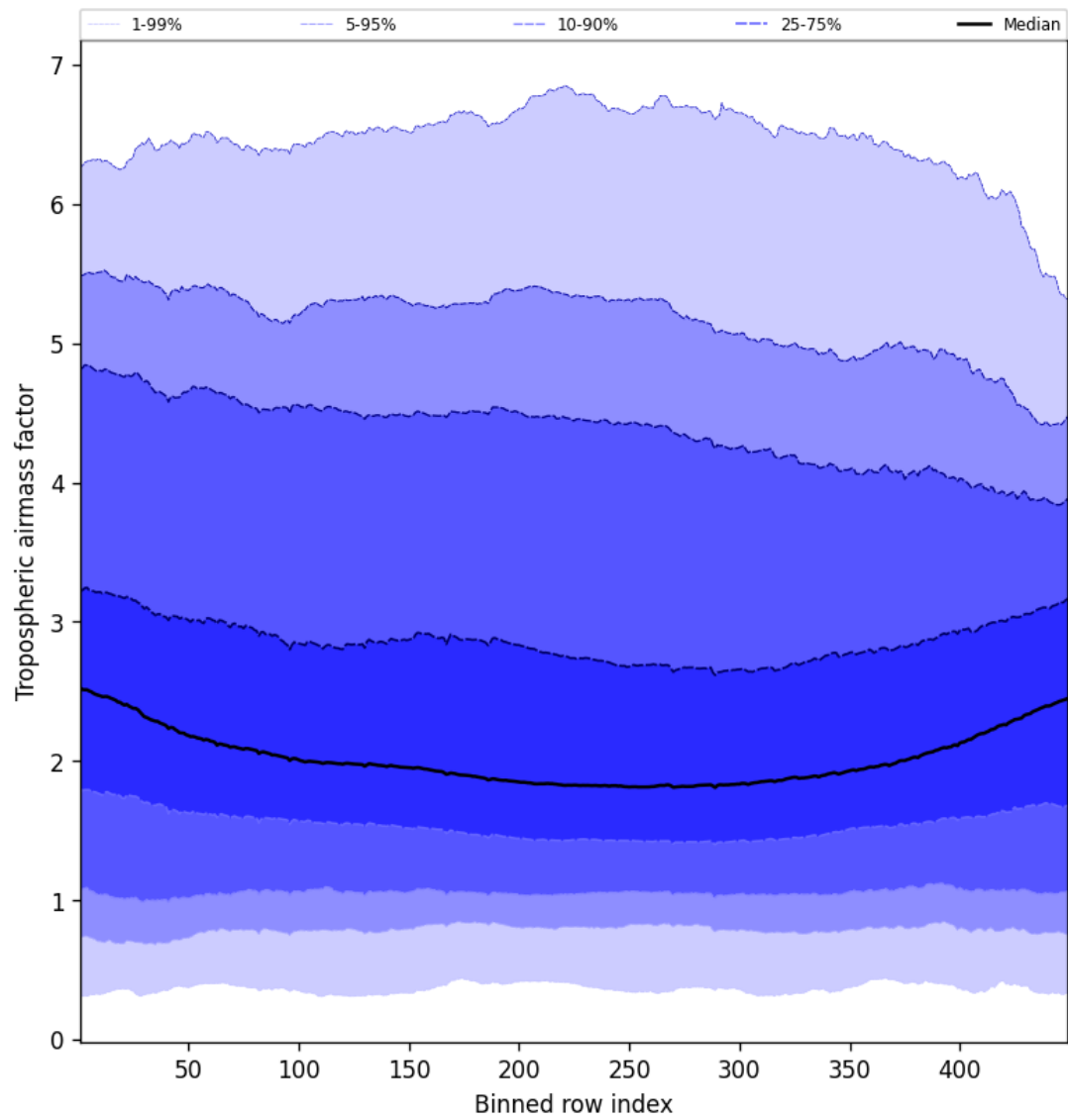
Figure 46: Along track statistics of “Tropospheric air mass factor” for 2025-02-28 to 2025-03-01
