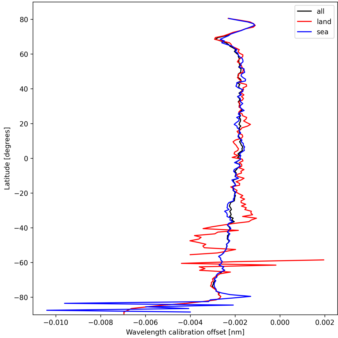
Figure 16: Zonal average of “Wavelength calibration offset” for 2025-02-28 to 2025-03-01.
