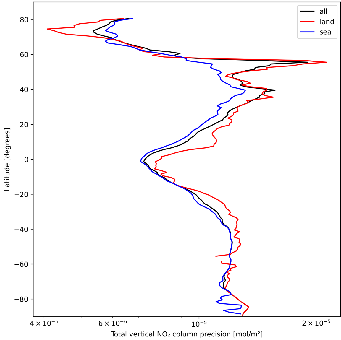
Figure 20: Zonal average of “Total vertical NO 2 column precision” for 2025-02-28 to 2025-03-01.
