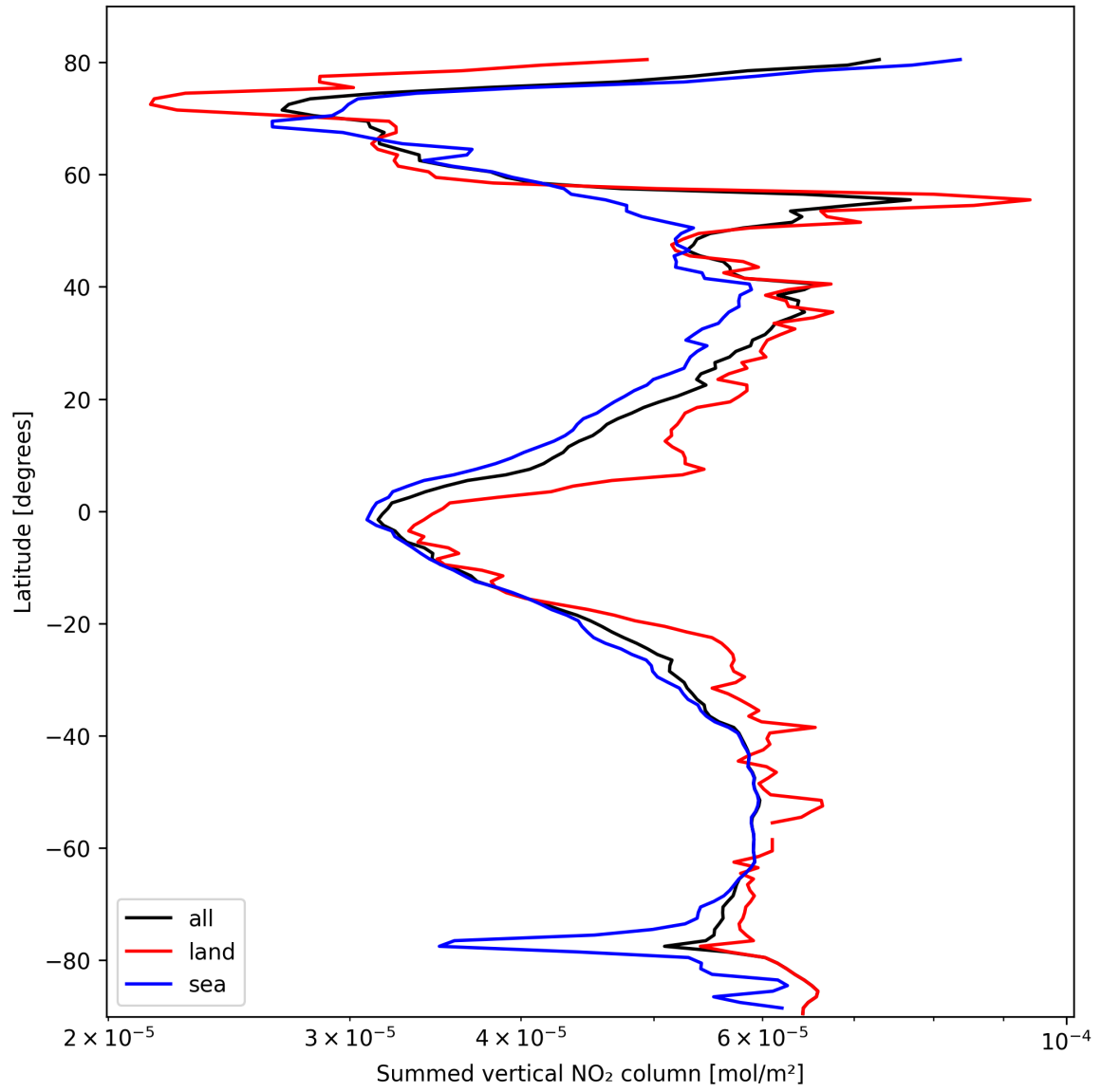
Figure 21: Zonal average of “Summed vertical NO 2 column” for 2025-02-28 to 2025-03-01.
