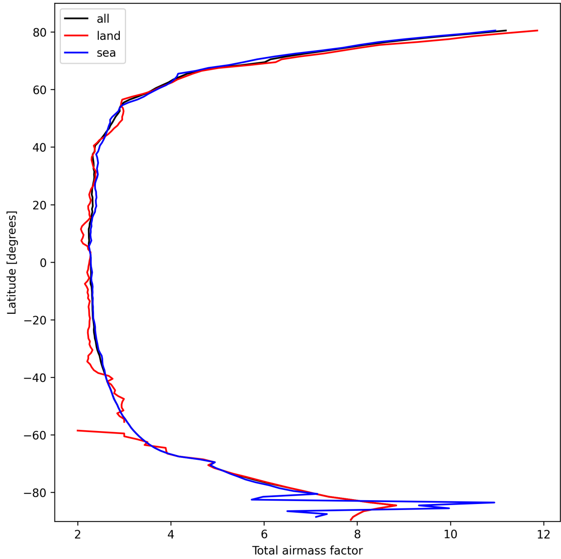
Figure 13: Zonal average of “Total airmass factor” for 2025-02-28 to 2025-03-01.
