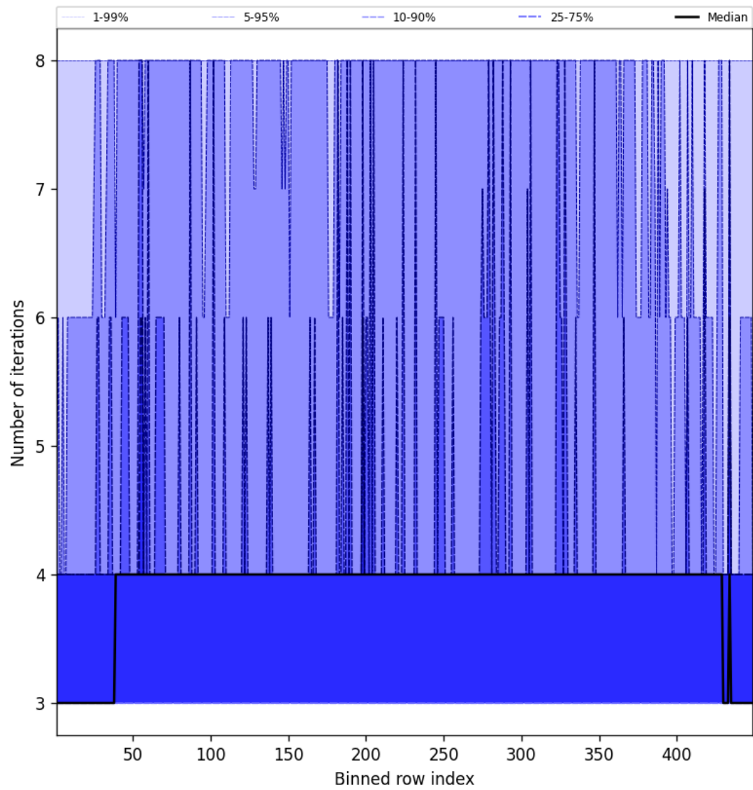
Figure 49: Along track statistics of “Number of iterations” for 2025-02-28 to 2025-03-01
