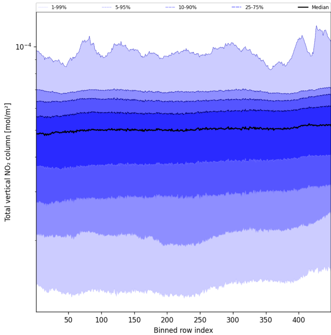
Figure 53: Along track statistics of “Total vertical NO 2 column” for 2025-02-28 to 2025-03-01
