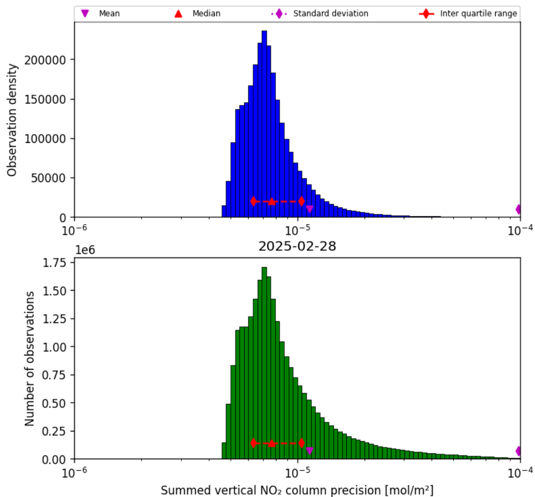
Figure 39: Histogram of "Summed vertical NO 2 column precision" for 2025-02-28 to 2025-03-01
