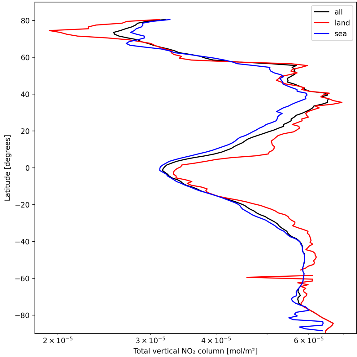
Figure 19: Zonal average of “Total vertical NO 2 column” for 2025-02-28 to 2025-03-01.
