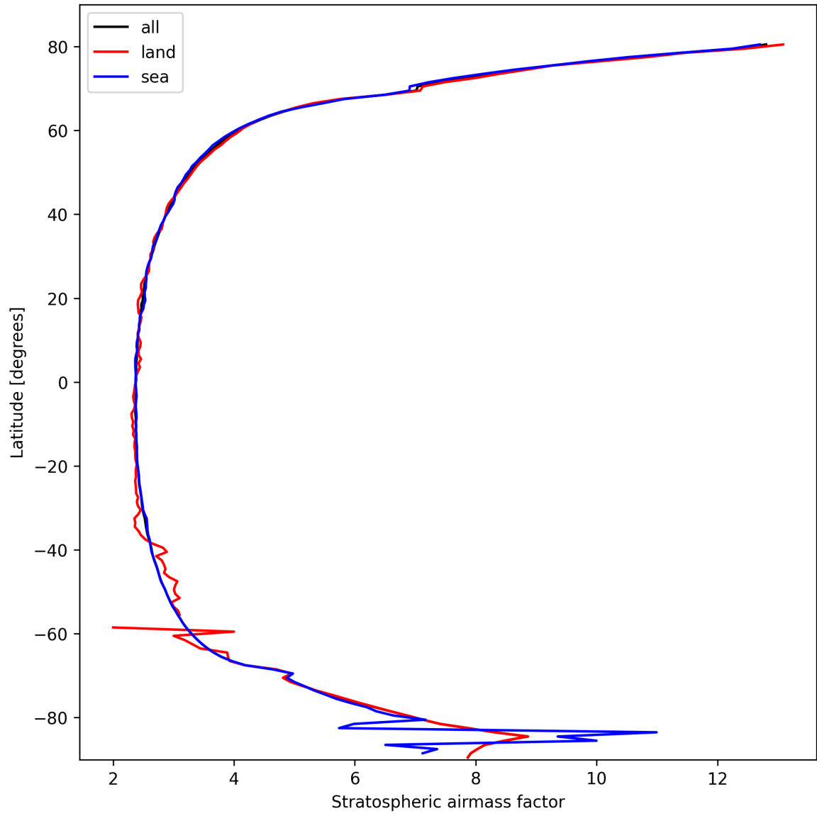
Figure 25: Zonal average of “Stratospheric airmass factor” for 2025-02-28 to 2025-03-01.
