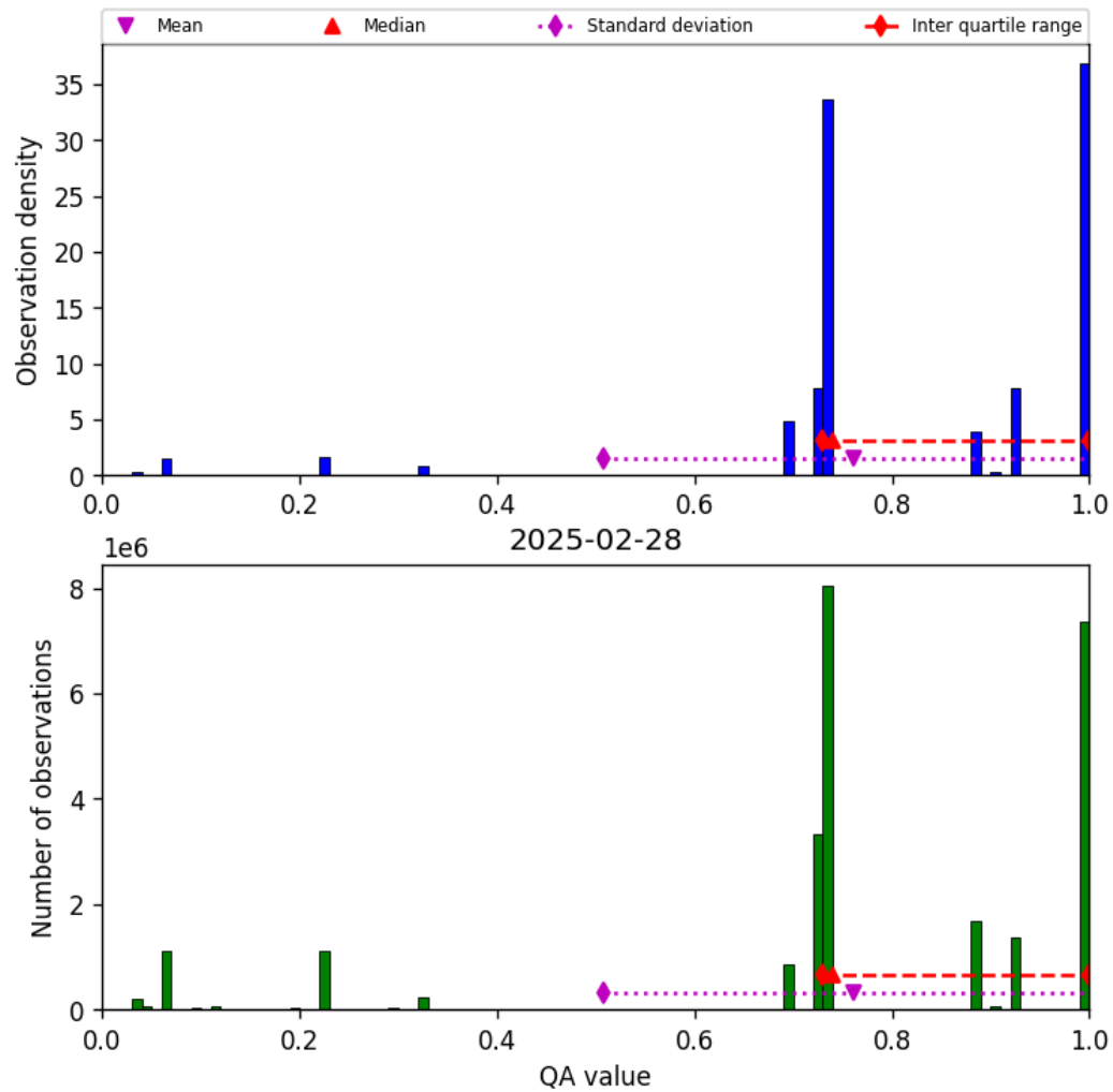
Figure 26: Histogram of “QA value” for 2025-02-28 to 2025-03-01
