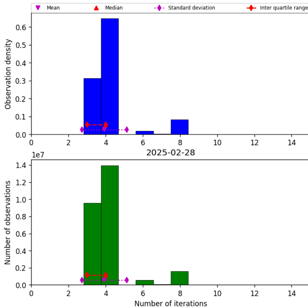
Figure 32: Histogram of “Number of iterations” for 2025-02-28 to 2025-03-01
