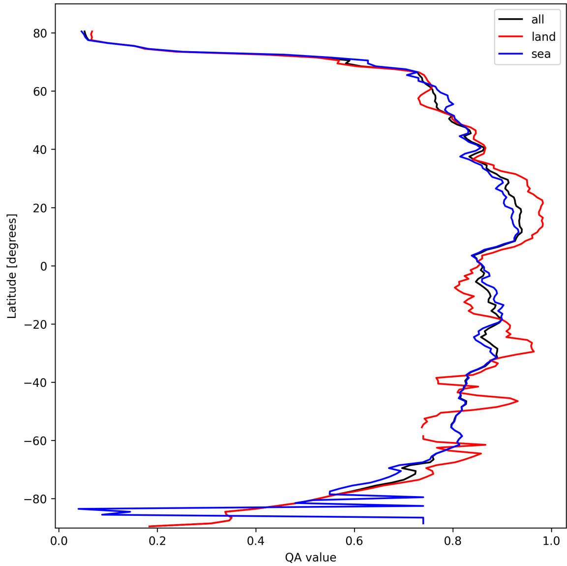
Figure 9: Zonal average of “QA value” for 2025-02-28 to 2025-03-01.
