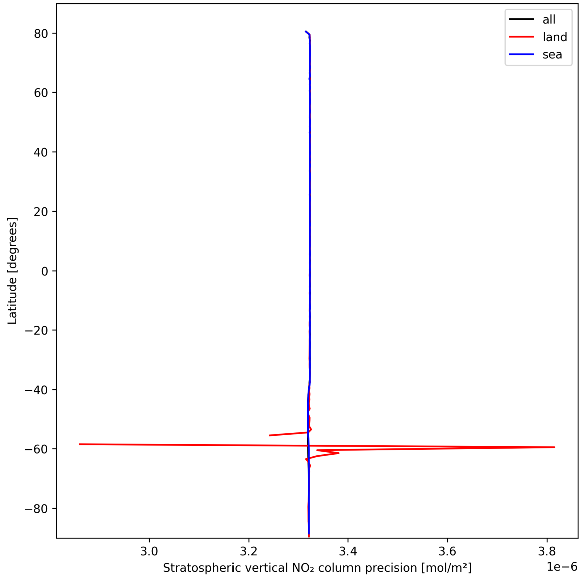
Figure 18: Zonal average of “Stratospheric vertical NO 2 column precision” for 2025-02-28 to 2025-03-01.
