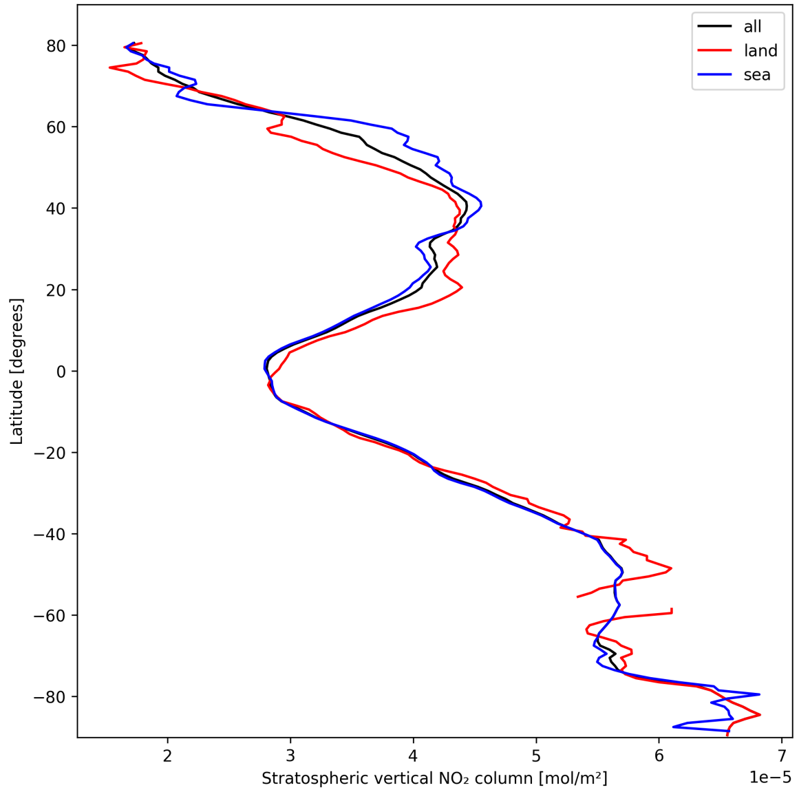
Figure 17: Zonal average of “Stratospheric vertical NO 2 column” for 2025-02-28 to 2025-03-01.
