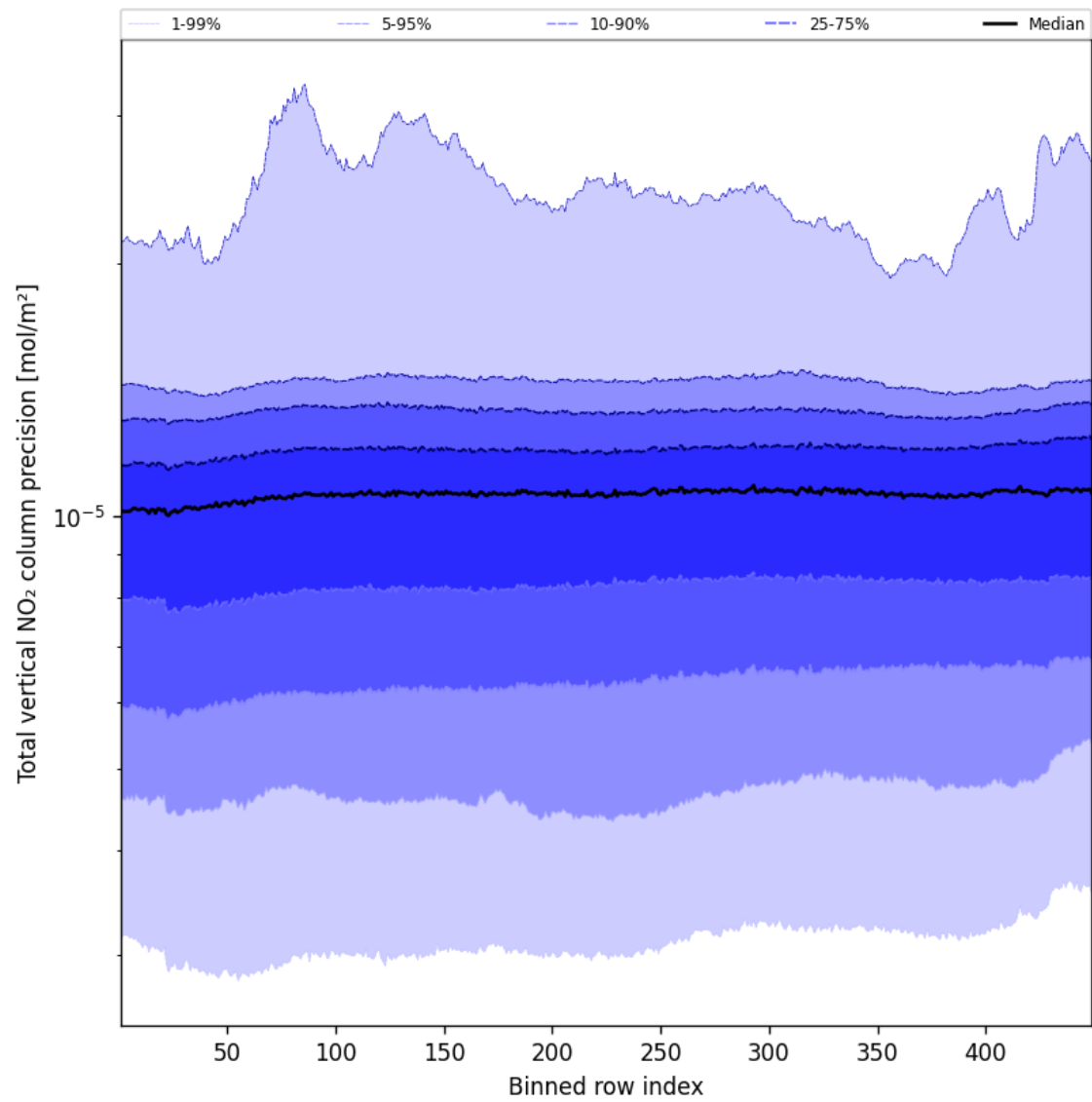
Figure 54: Along track statistics of “Total vertical NO 2 column precision” for 2025-02-28 to 2025-03-01
