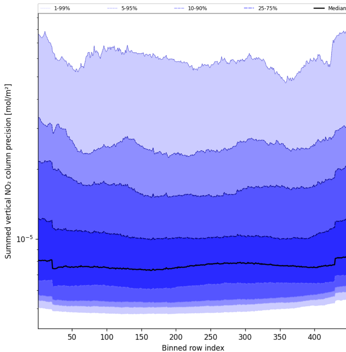
Figure 56: Along track statistics of “Summed vertical NO 2 column precision” for 2025-02-28 to 2025-03-01
