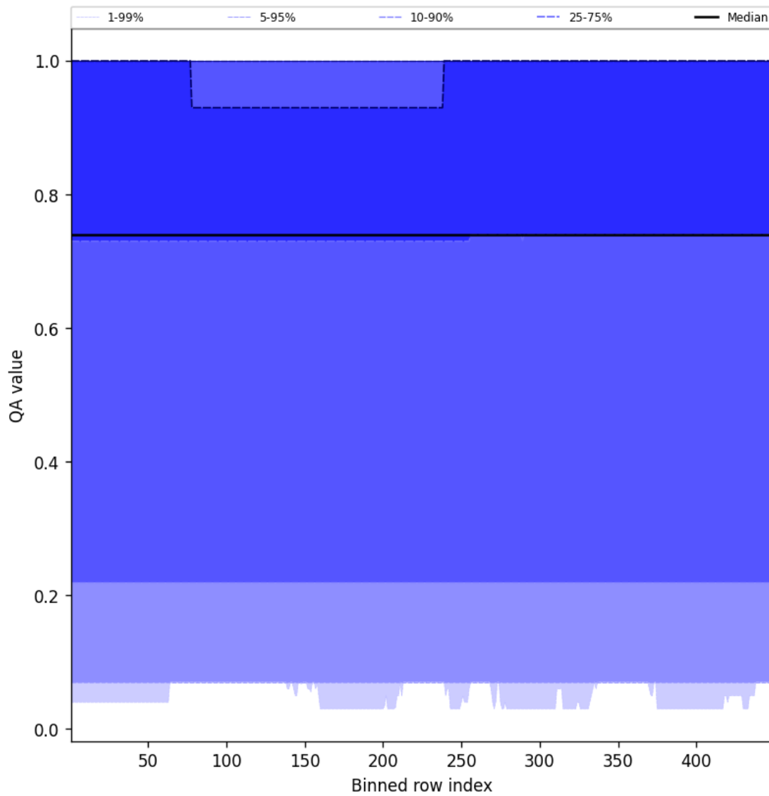
Figure 43: Along track statistics of “QA value” for 2025-02-28 to 2025-03-01
