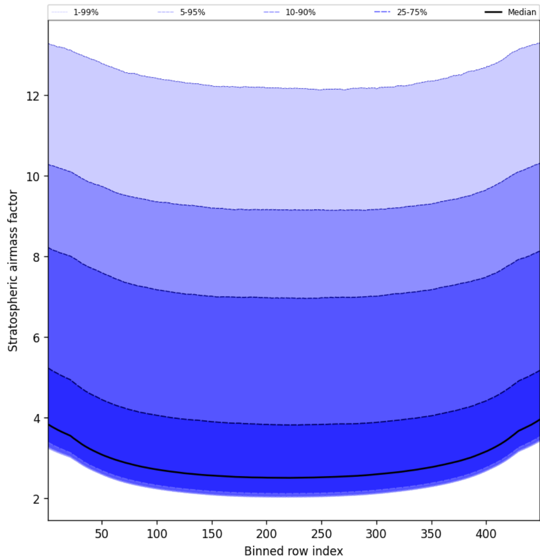
Figure 59: Along track statistics of “Stratospheric airmass factor” for 2025-02-28 to 2025-03-01
