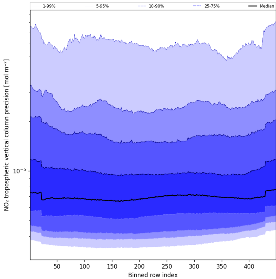
Figure 45: Along track statistics of “NO 2 tropospheric vertical column precision” for 2025-02-28 to 2025-03-01
