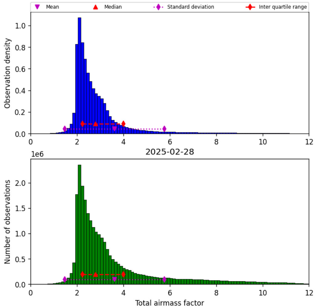
Figure 30: Histogram of “Total airmass factor” for 2025-02-28 to 2025-03-01
