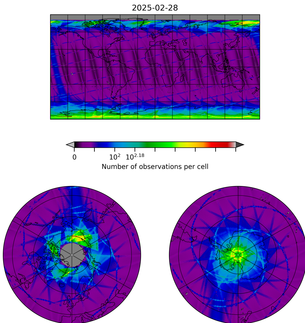
Figure 8: Map of the number of observations for 2025-02-28 to 2025-03-01
