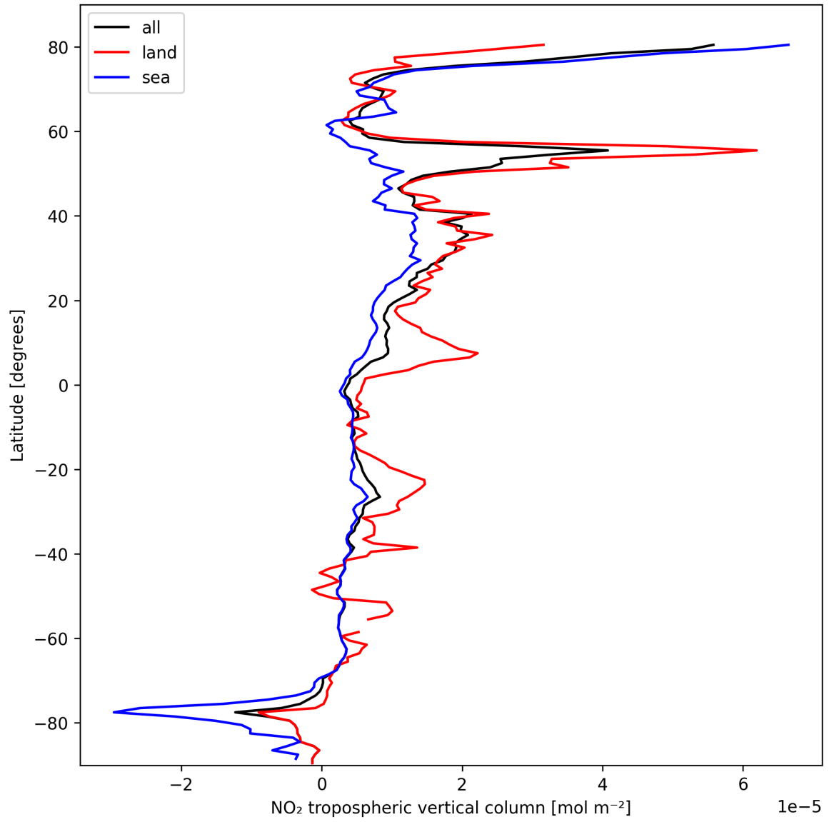
Figure 10: Zonal average of “NO 2 tropospheric vertical column” for 2025-02-28 to 2025-03-01.
