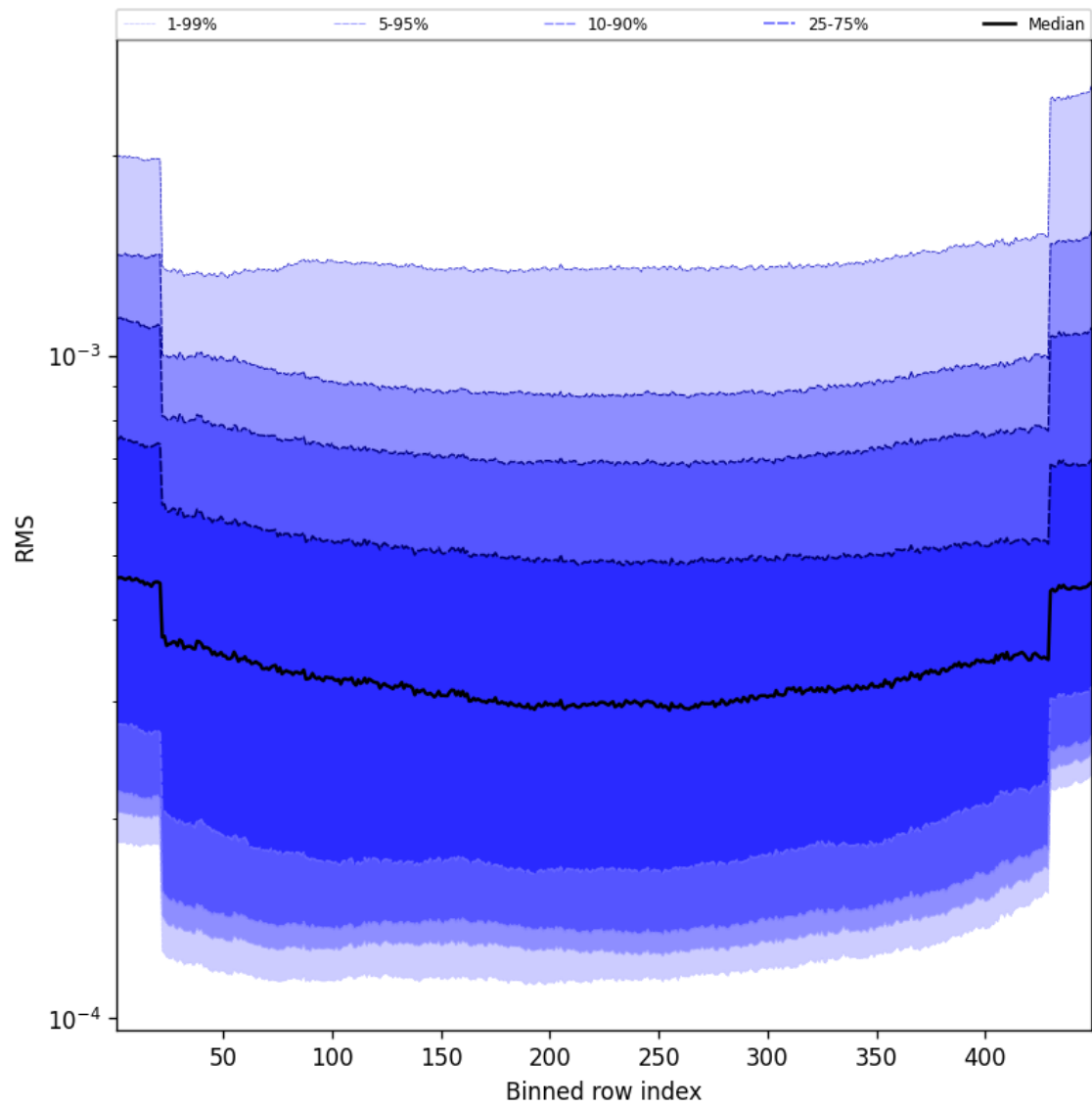
Figure 58: Along track statistics of “RMS” for 2025-02-28 to 2025-03-01
