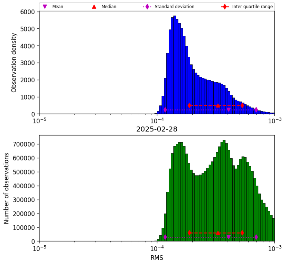
Figure 41: Histogram of “RMS” for 2025-02-28 to 2025-03-01
