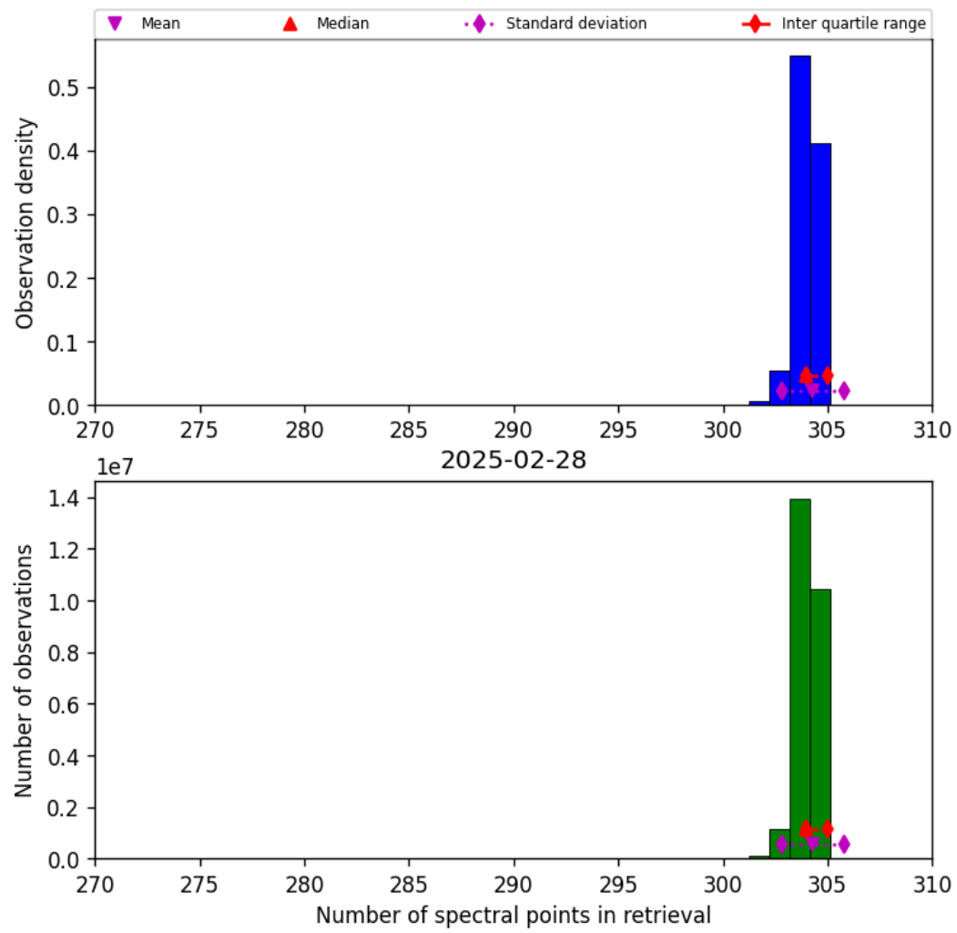
Figure 31: Histogram of “Number of spectral points in retrieval” for 2025-02-28 to 2025-03-01
