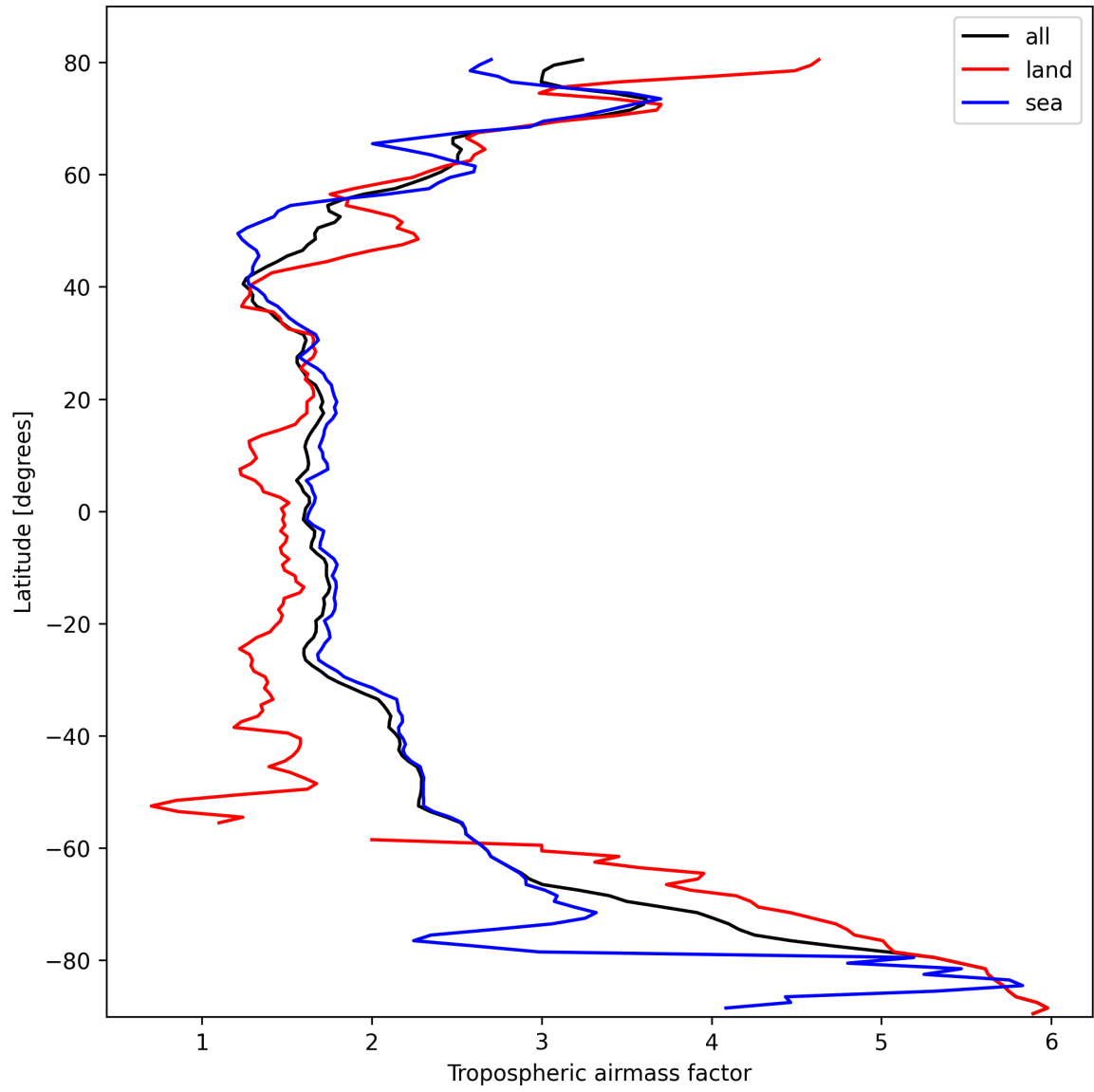
Figure 12: Zonal average of “Tropospheric air mass factor” for 2025-02-28 to 2025-03-01.
