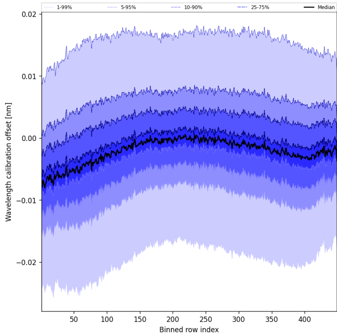
Figure 50: Along track statistics of “Wavelength calibration offset” for 2025-02-28 to 2025-03-01
