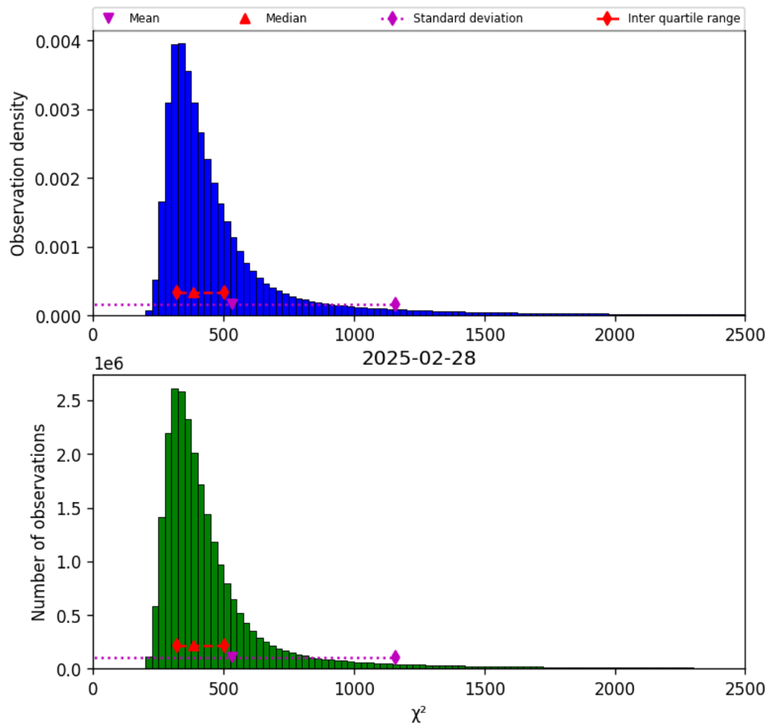
Figure 40: Histogram of “ \chi^2 ” for 2025-02-28 to 2025-03-01
