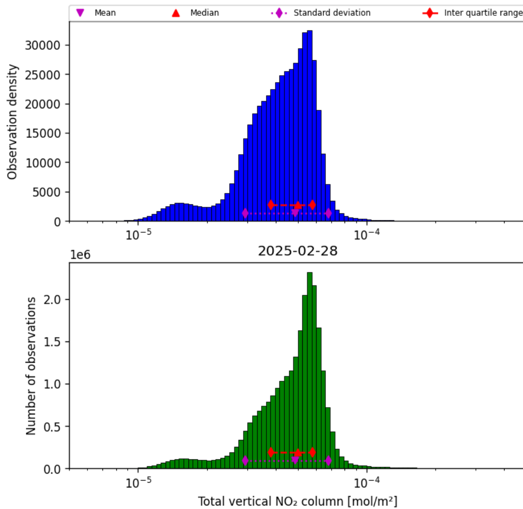
Figure 36: Histogram of “Total vertical NO 2 column” for 2025-02-28 to 2025-03-01
