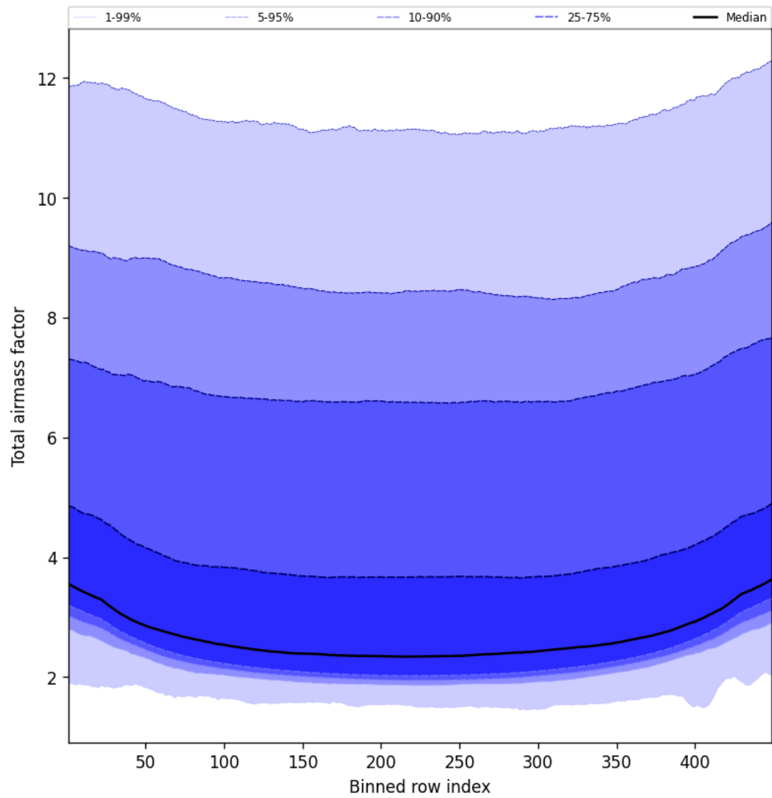
Figure 47: Along track statistics of “Total airmass factor” for 2025-02-28 to 2025-03-01
