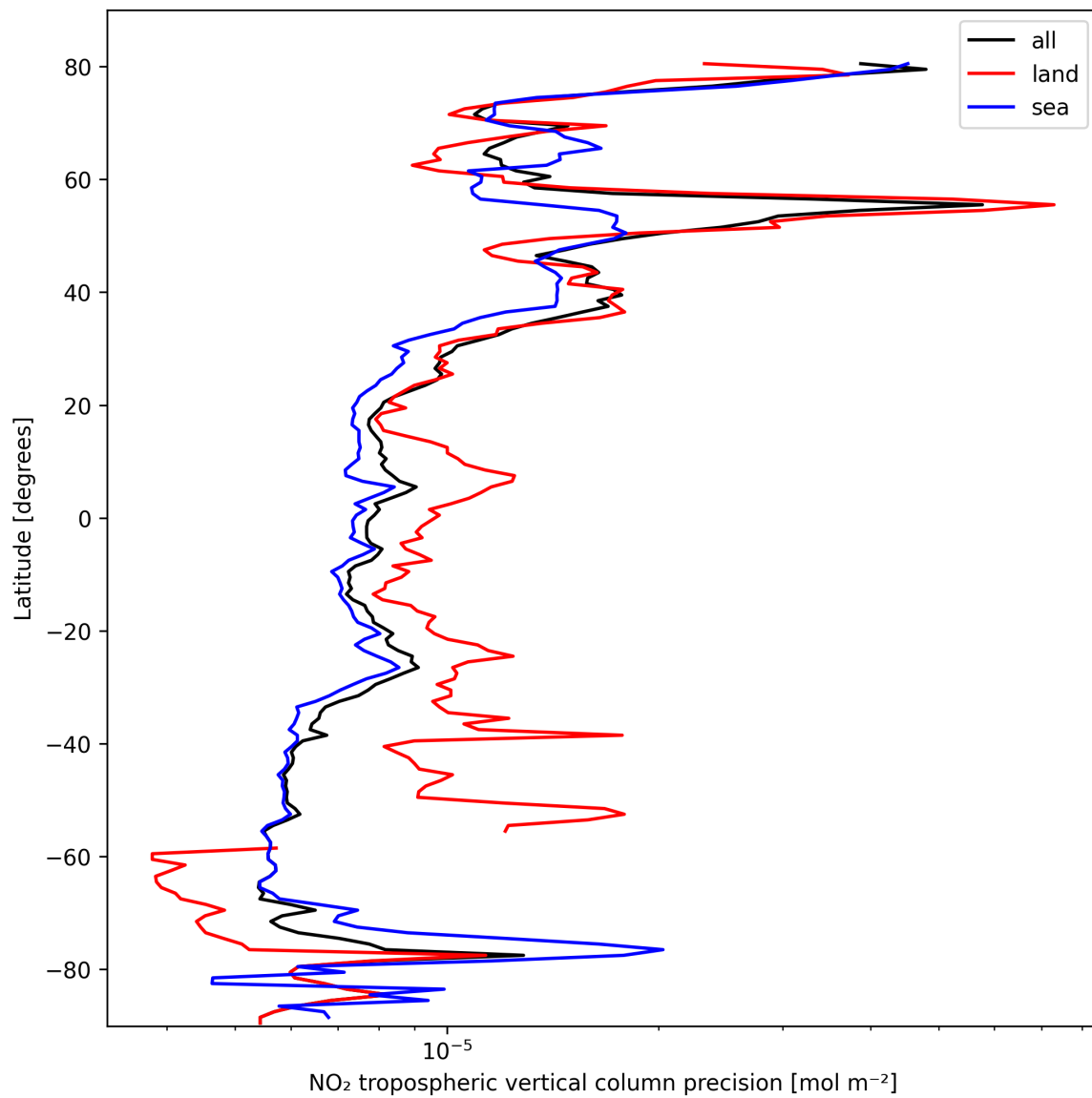
Figure 11: Zonal average of “NO 2 tropospheric vertical column precision” for 2025-02-28 to 2025-03-01.
