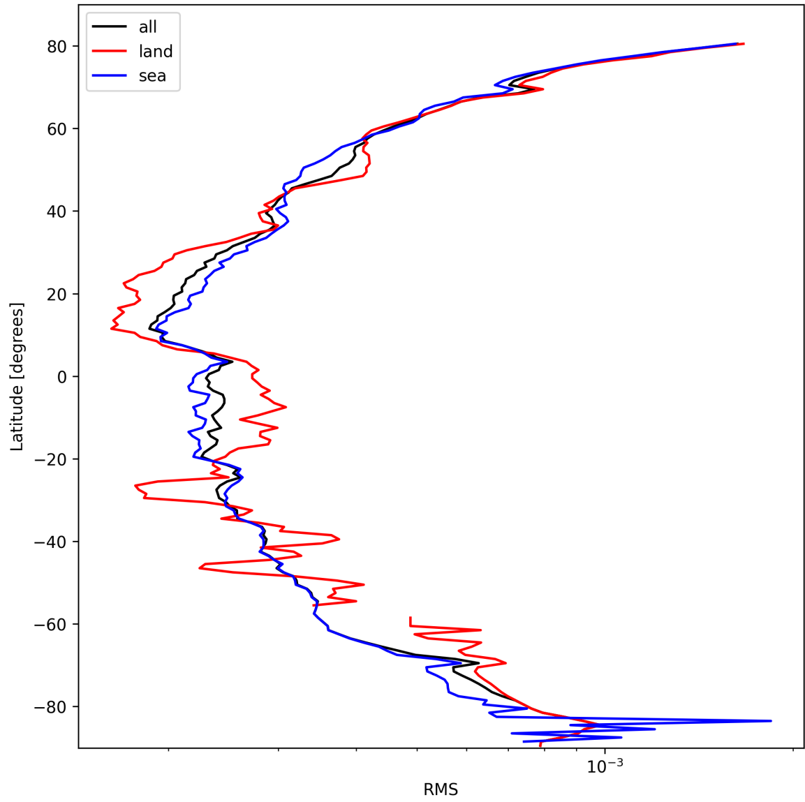
Figure 24: Zonal average of “RMS” for 2025-02-28 to 2025-03-01.
