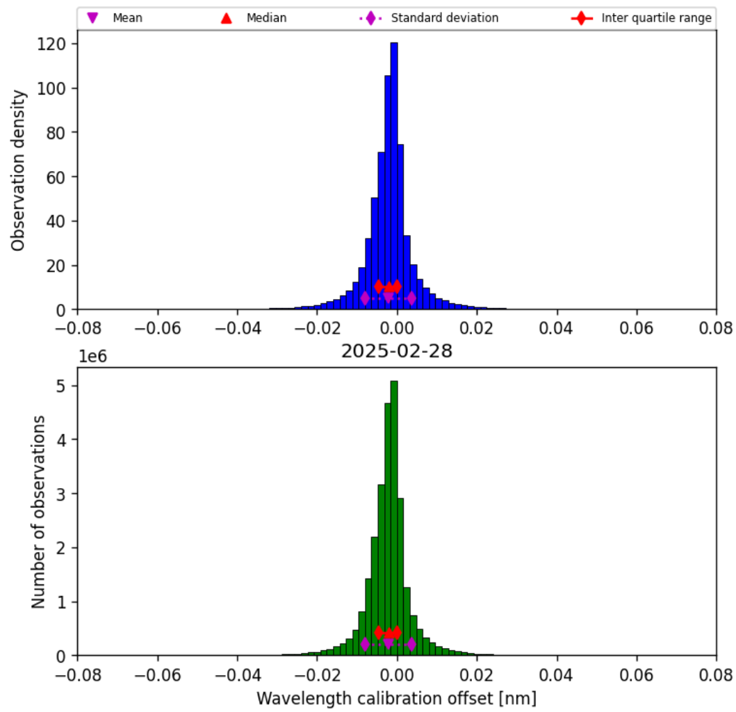
Figure 33: Histogram of “Wavelength calibration offset” for 2025-02-28 to 2025-03-01
