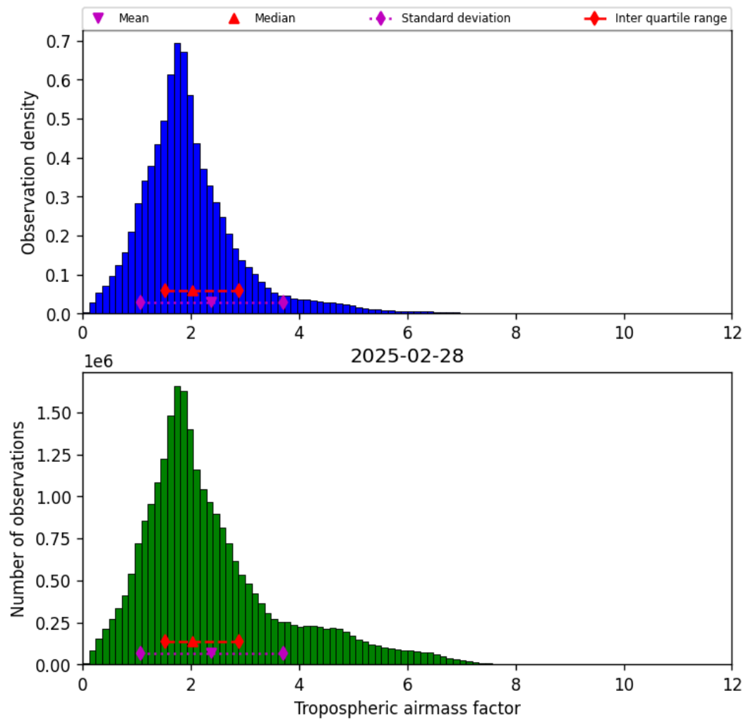
Figure 29: Histogram of “Tropospheric airmass factor” for 2025-02-28 to 2025-03-01
