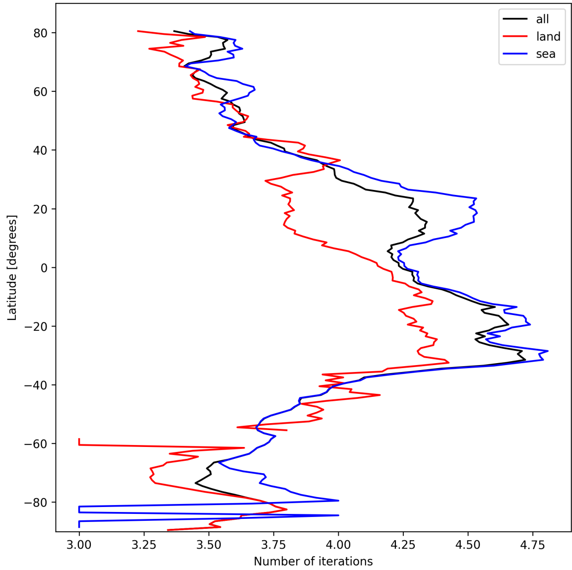
Figure 15: Zonal average of “Number of iterations” for 2025-02-28 to 2025-03-01.
