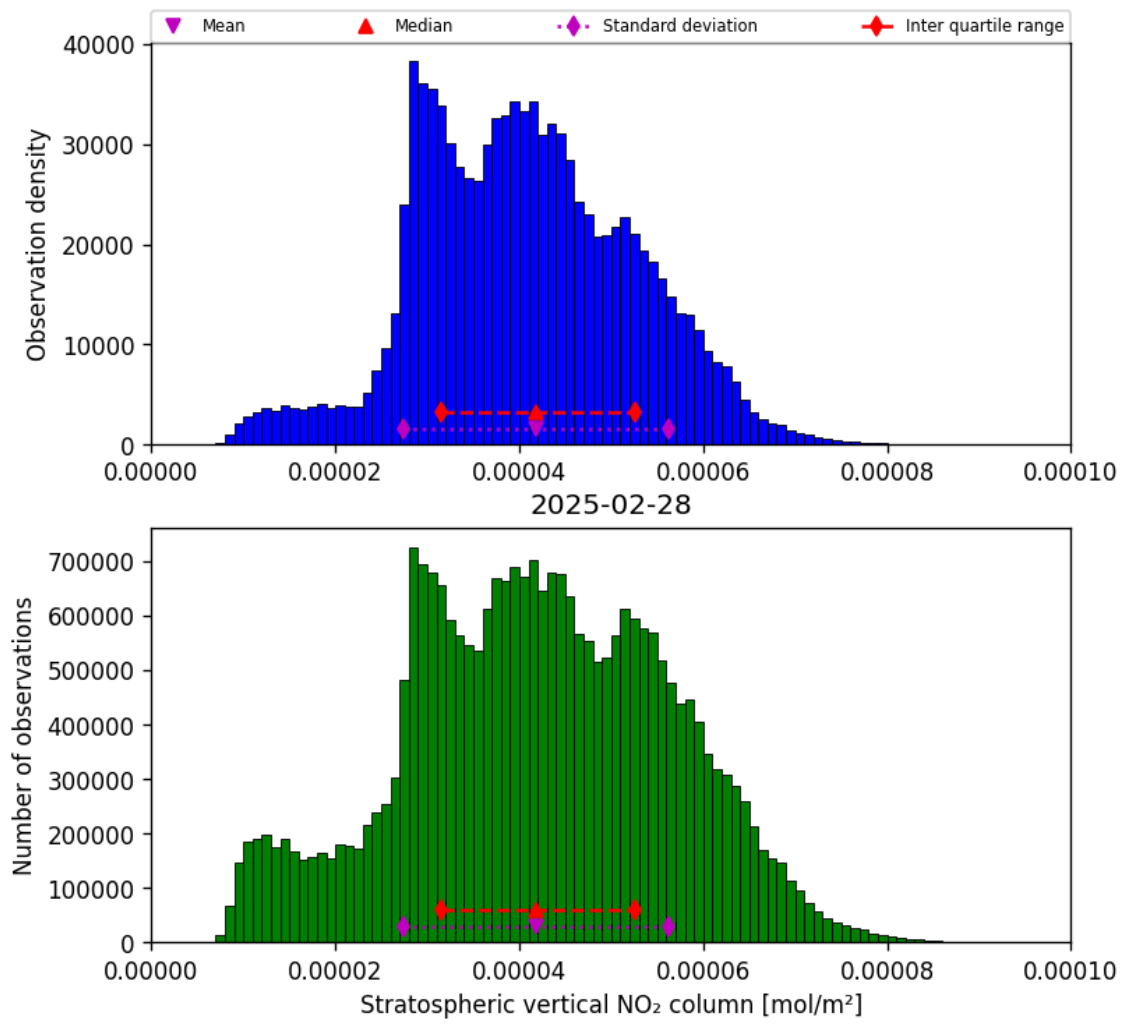
Figure 34: Histogram of “Stratospheric vertical NO 2 column” for 2025-02-28 to 2025-03-01
