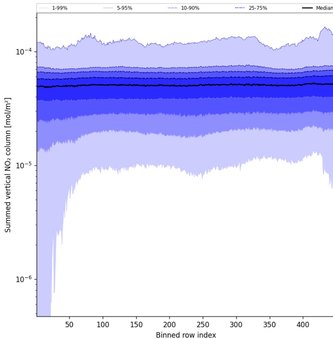
Figure 55: Along track statistics of “Summed vertical NO 2 column” for 2025-02-28 to 2025-03-01
