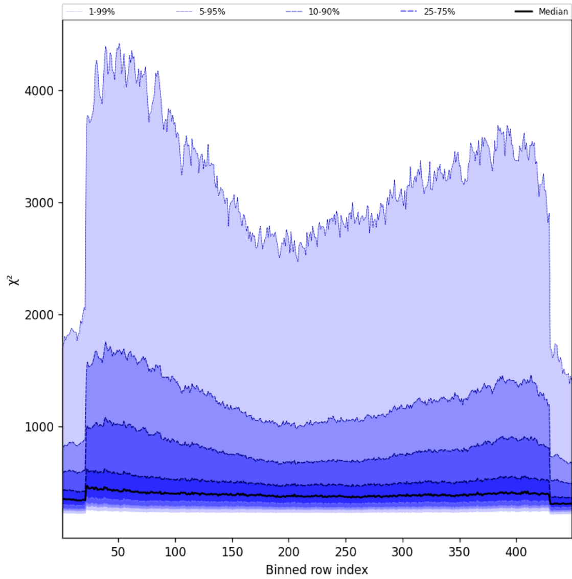
Figure 57: Along track statistics of “ \chi^2 ” for 2025-02-28 to 2025-03-01
