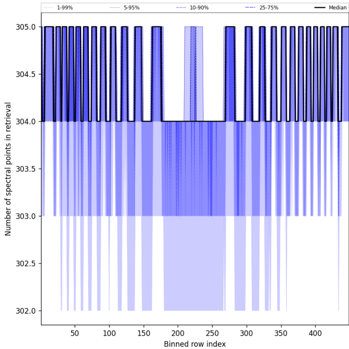
Figure 48: Along track statistics of “Number of spectral points in retrieval” for 2025-02-28 to 2025-03-01
