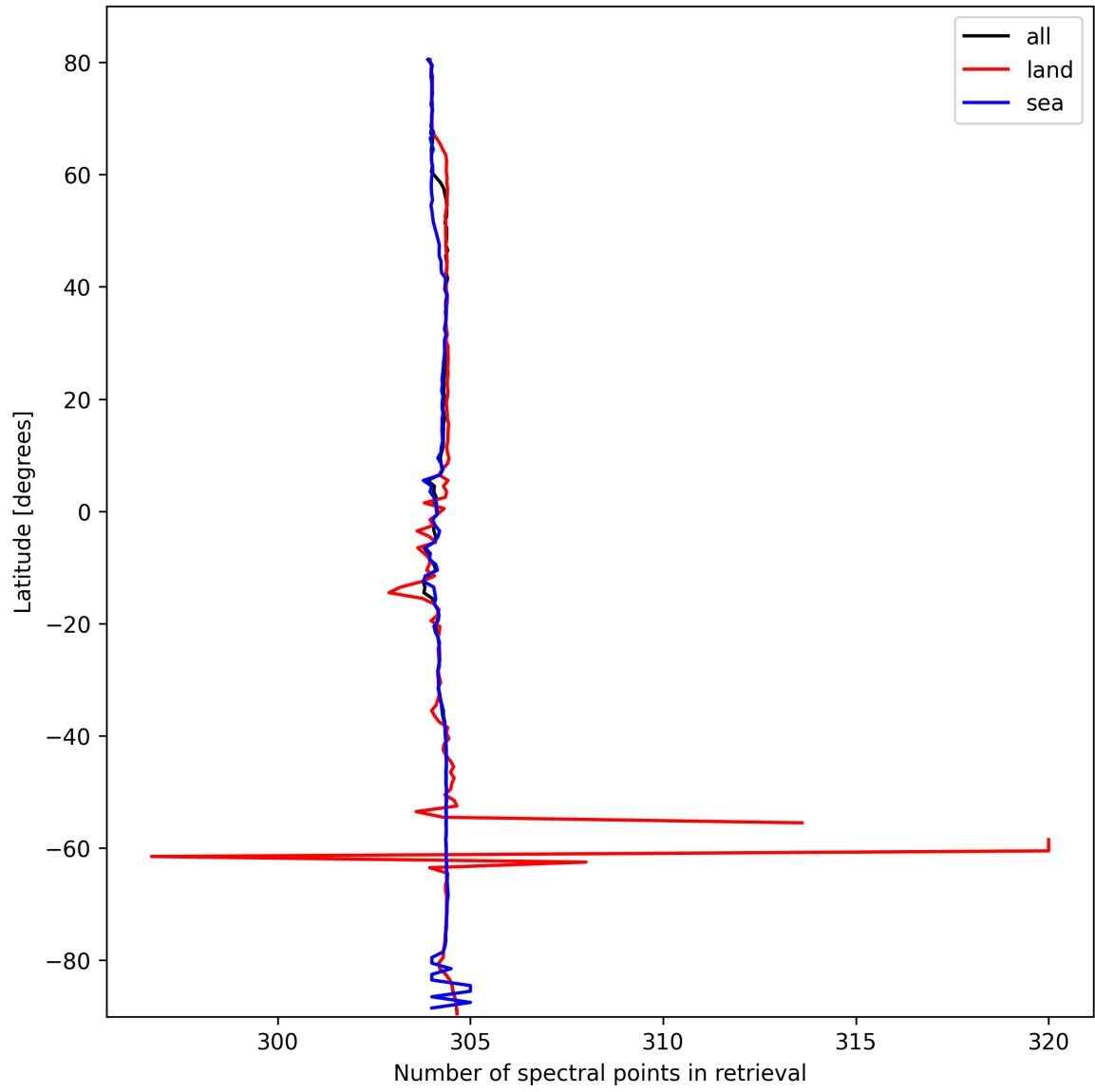
Figure 14: Zonal average of “Number of spectral points in retrieval” for 2025-02-28 to 2025-03-01.
