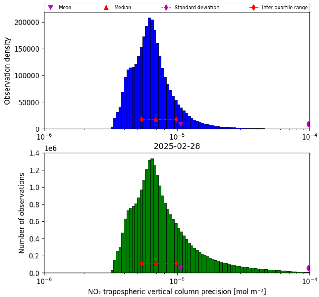
Figure 28: Histogram of “NO 2 tropospheric vertical column precision” for 2025-02-28 to 2025-03-01
