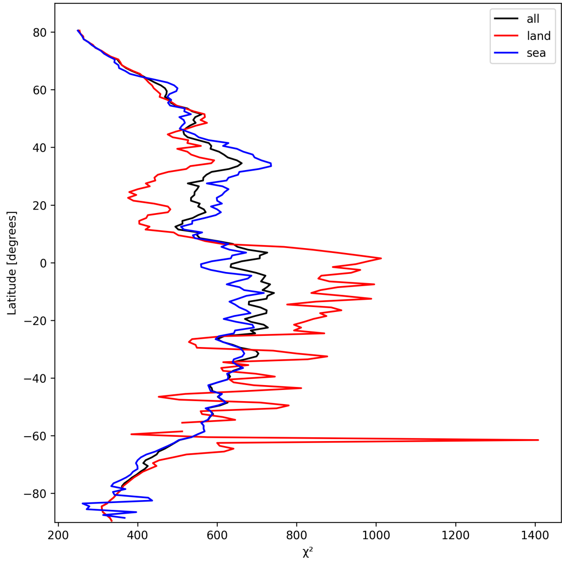
Figure 23: Zonal average of “ \chi^2 ” for 2025-02-28 to 2025-03-01.
