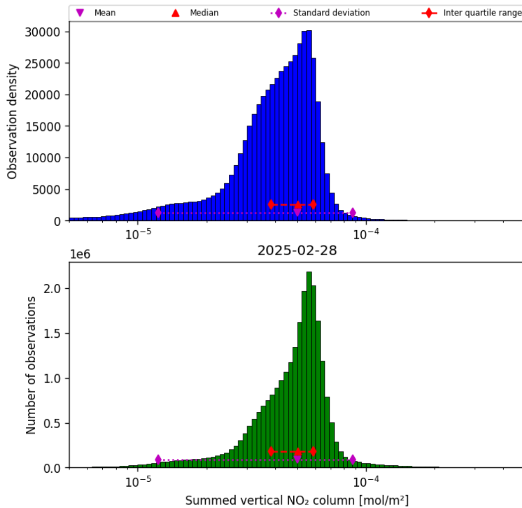
Figure 38: Histogram of “Summed vertical NO 2 column” for 2025-02-28 to 2025-03-01
