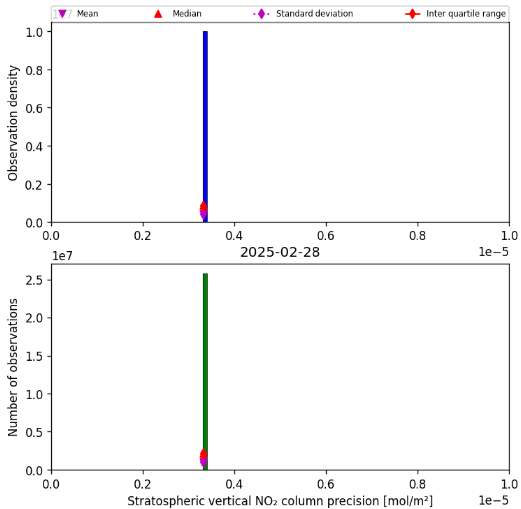
Figure 35: Histogram of “Stratospheric vertical NO 2 column precision” for 2025-02-28 to 2025-03-01
