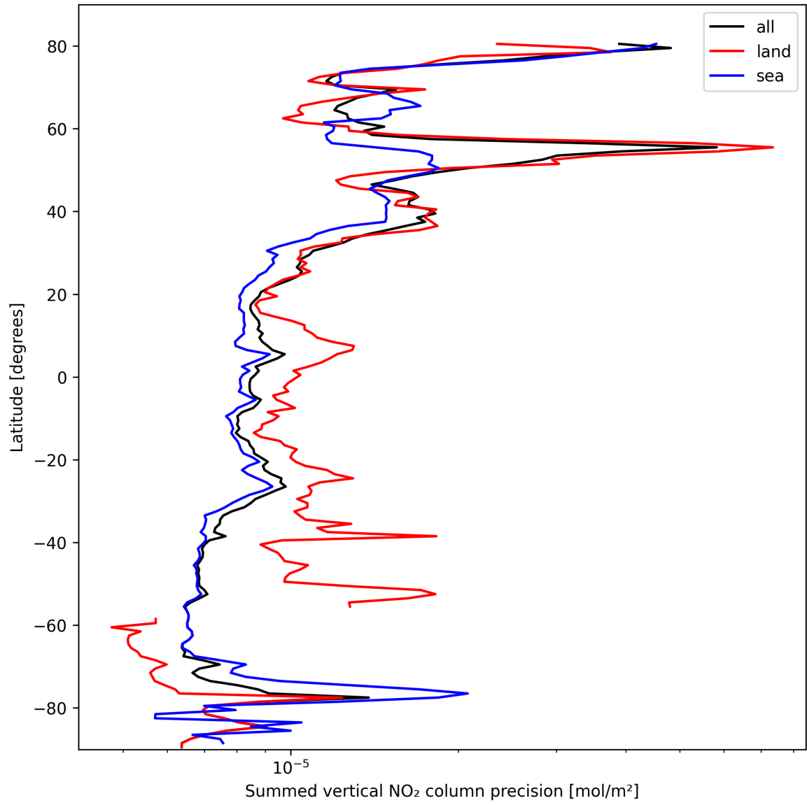
Figure 22: Zonal average of “Summed vertical NO 2 column precision” for 2025-02-28 to 2025-03-01.
