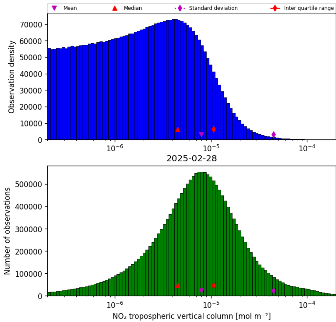
Figure 27: Histogram of “NO 2 tropospheric vertical column” for 2025-02-28 to 2025-03-01
