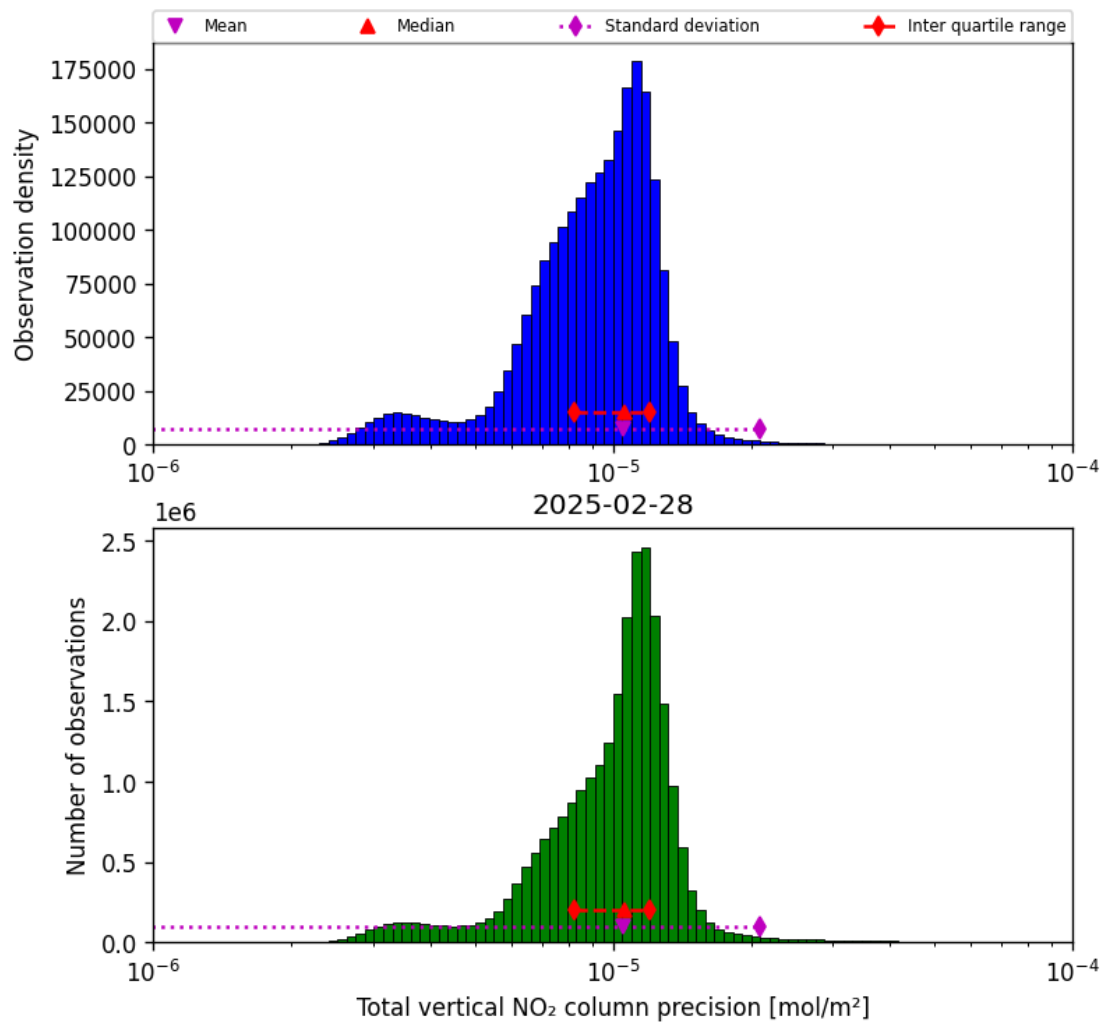
Figure 37: Histogram of “Total vertical NO 2 column precision” for 2025-02-28 to 2025-03-01
