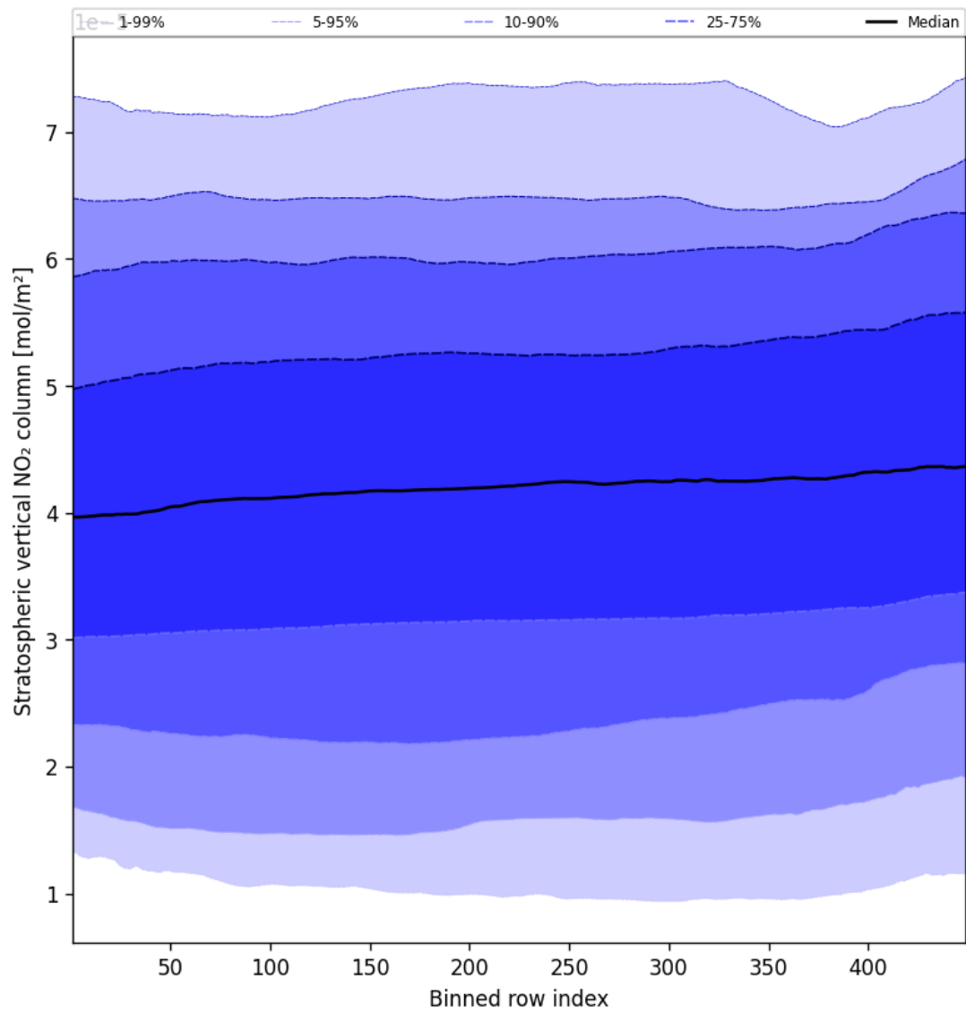
Figure 51: Along track statistics of “Stratospheric vertical NO 2 column” for 2025-02-28 to 2025-03-01
