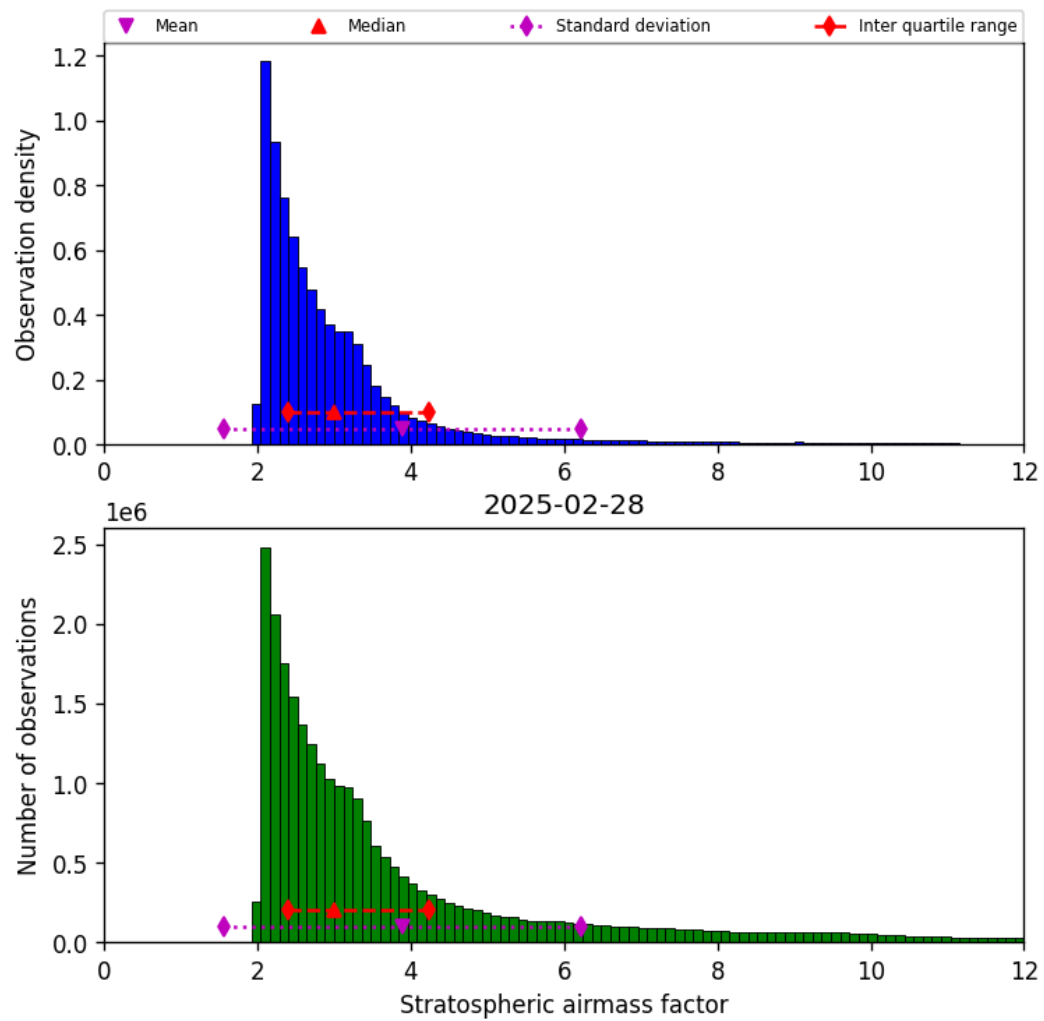
Figure 42: Histogram of “Stratospheric airmass factor” for 2025-02-28 to 2025-03-01
