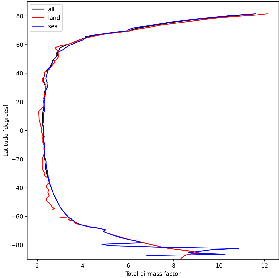
Figure 13: Zonal average of “Total airmass factor” for 2025-03-02 to 2025-03-03.
