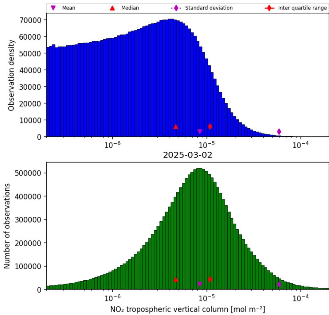
Figure 27: Histogram of “NO 2 tropospheric vertical column” for 2025-03-02 to 2025-03-03
