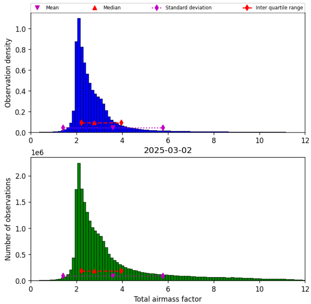
Figure 30: Histogram of “Total airmass factor” for 2025-03-02 to 2025-03-03
