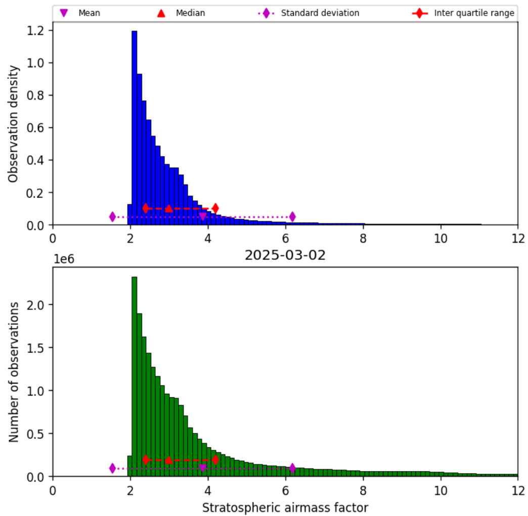
Figure 42: Histogram of “Stratospheric airmass factor” for 2025-03-02 to 2025-03-03
