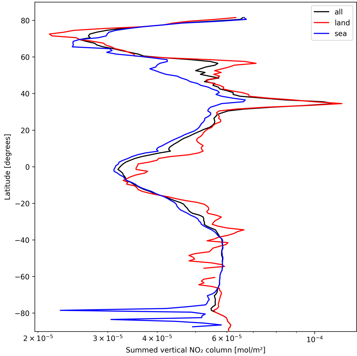
Figure 21: Zonal average of “Summed vertical NO 2 column” for 2025-03-02 to 2025-03-03.
