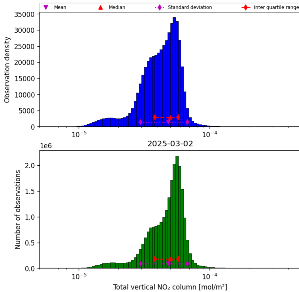
Figure 36: Histogram of “Total vertical NO 2 column” for 2025-03-02 to 2025-03-03
