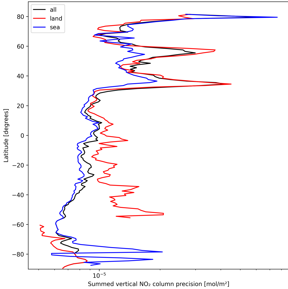
Figure 22: Zonal average of “Summed vertical NO 2 column precision” for 2025-03-02 to 2025-03-03.
