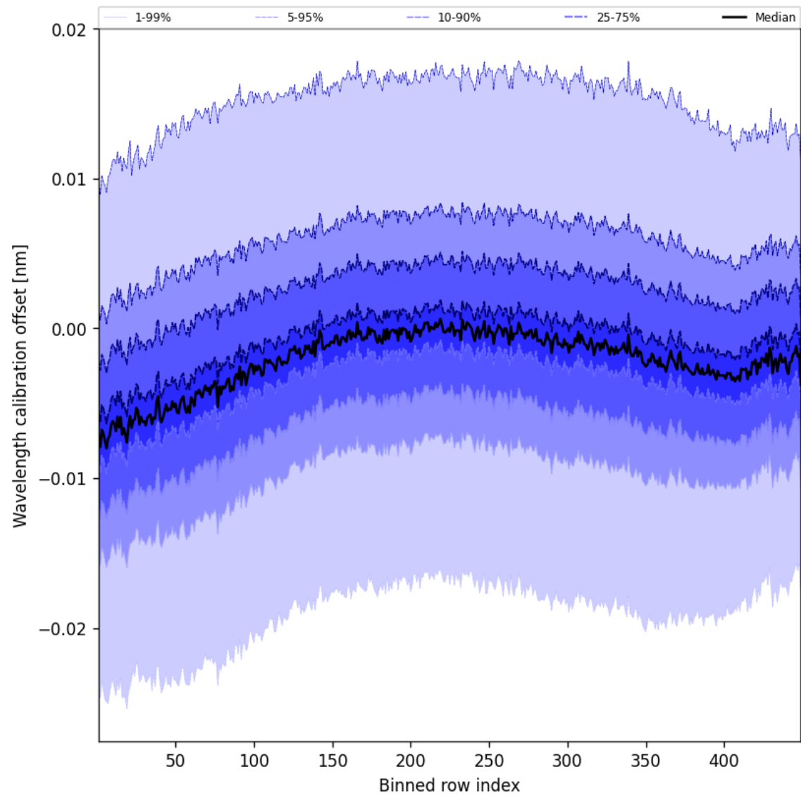
Figure 50: Along track statistics of “Wavelength calibration offset” for 2025-03-02 to 2025-03-03
