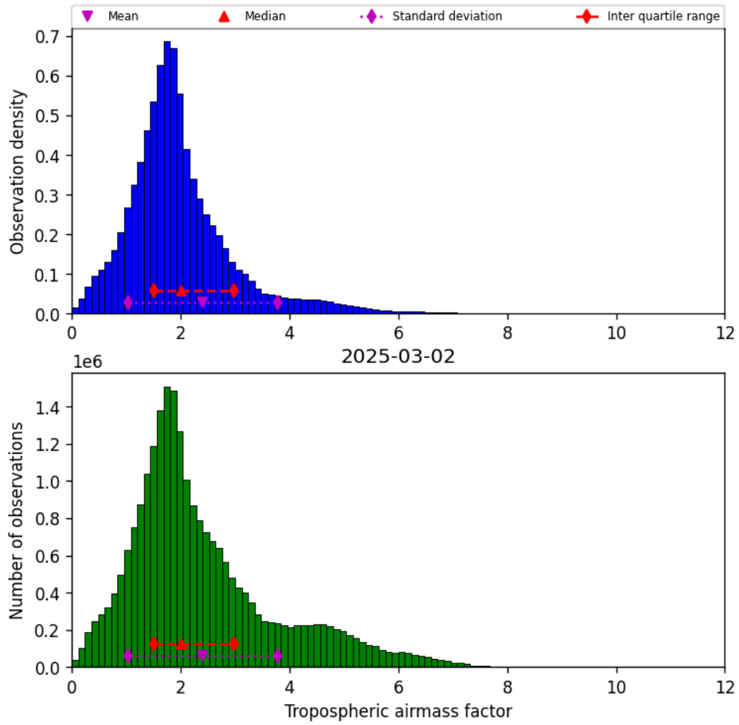
Figure 29: Histogram of “Tropospheric airmass factor” for 2025-03-02 to 2025-03-03
