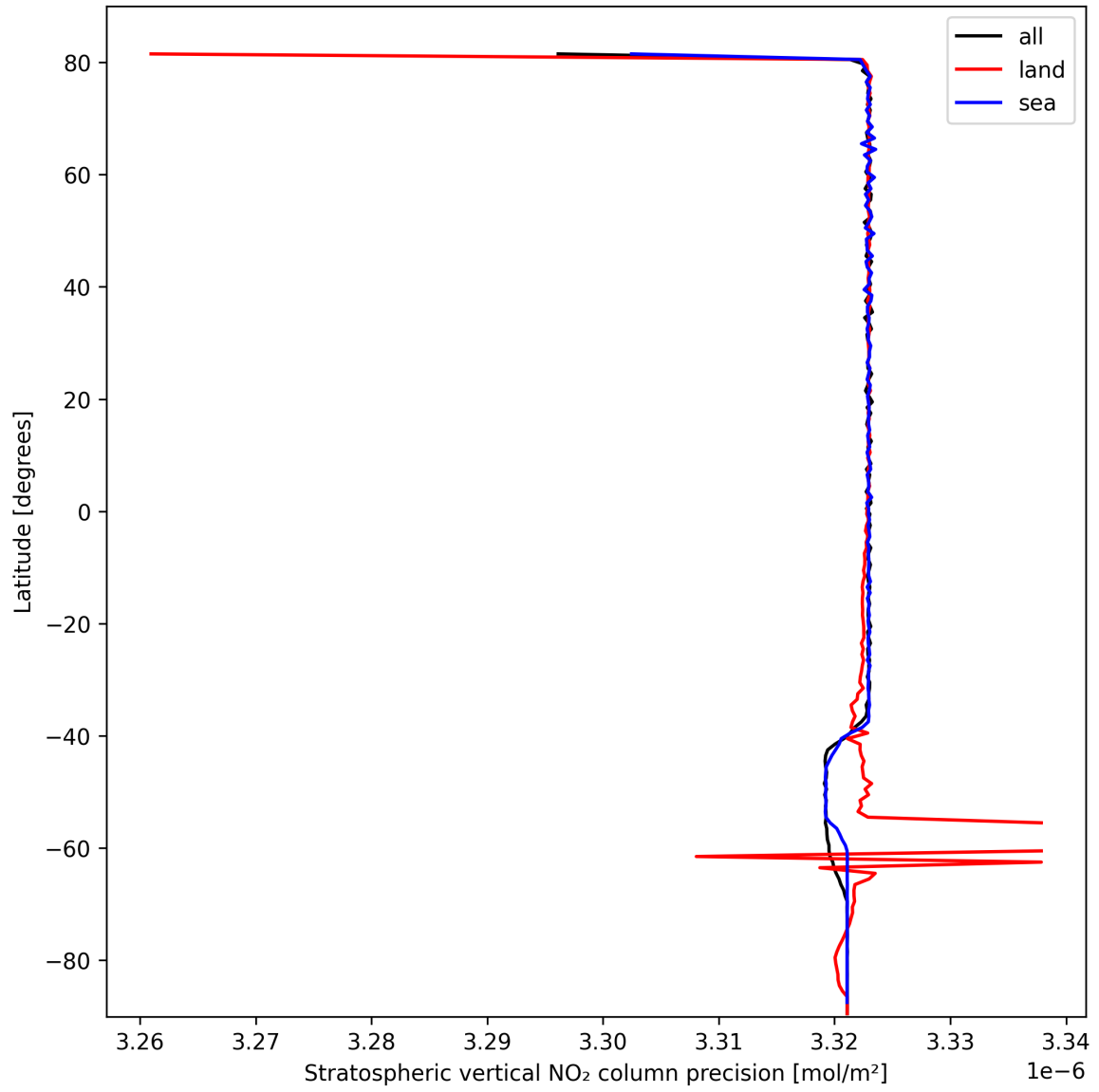
Figure 18: Zonal average of “Stratospheric vertical NO 2 column precision” for 2025-03-02 to 2025-03-03.
