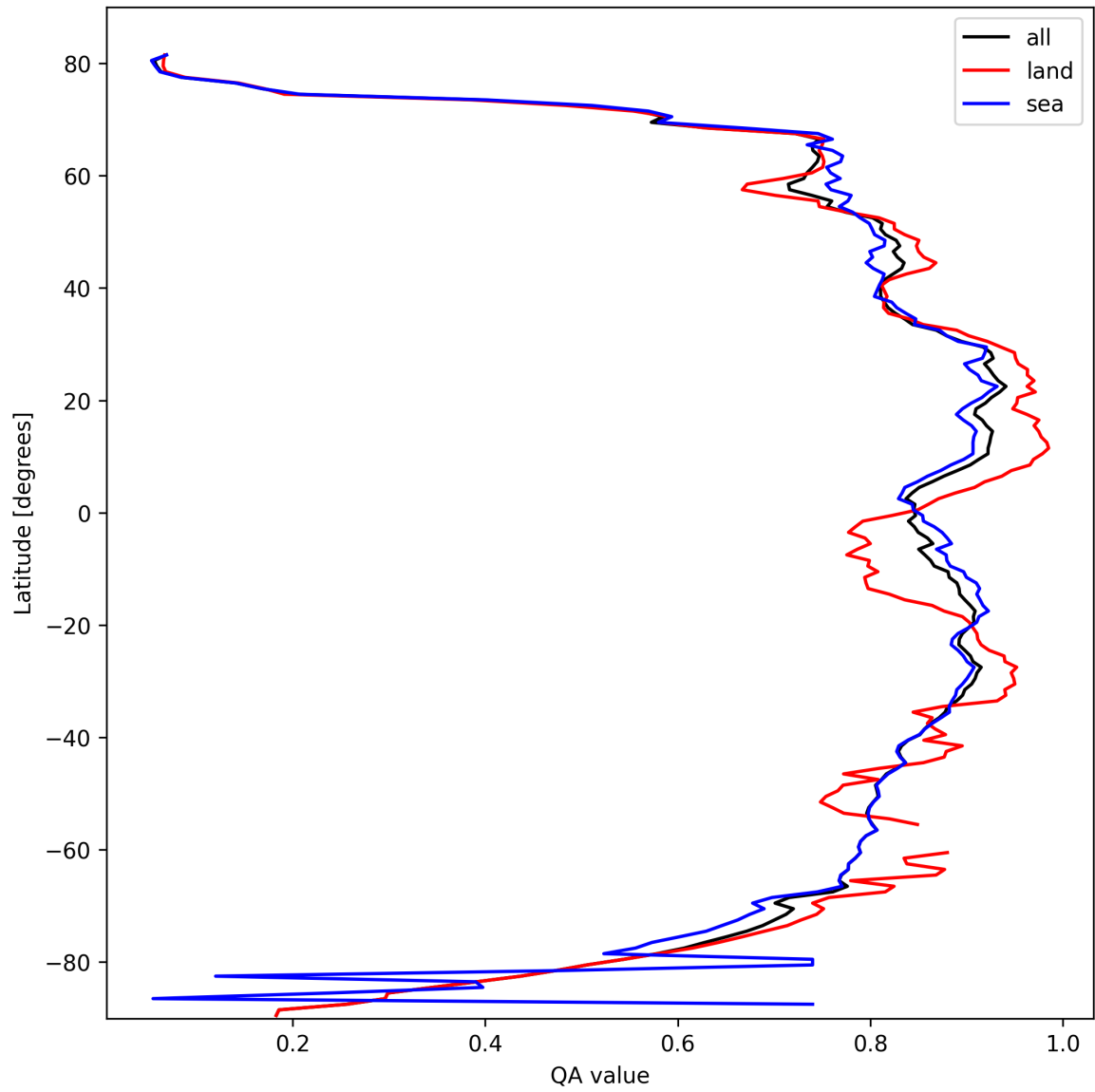
Figure 9: Zonal average of “QA value” for 2025-03-02 to 2025-03-03.
