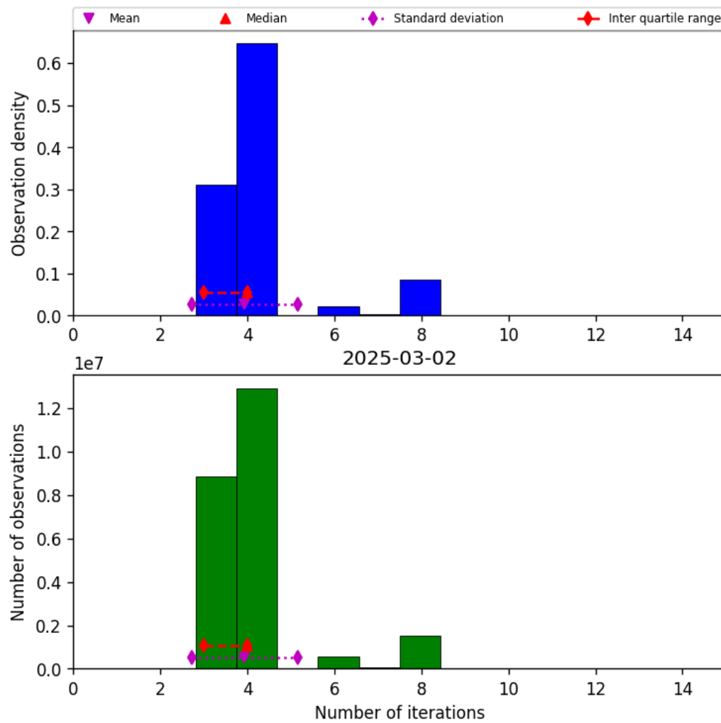
Figure 32: Histogram of “Number of iterations” for 2025-03-02 to 2025-03-03
