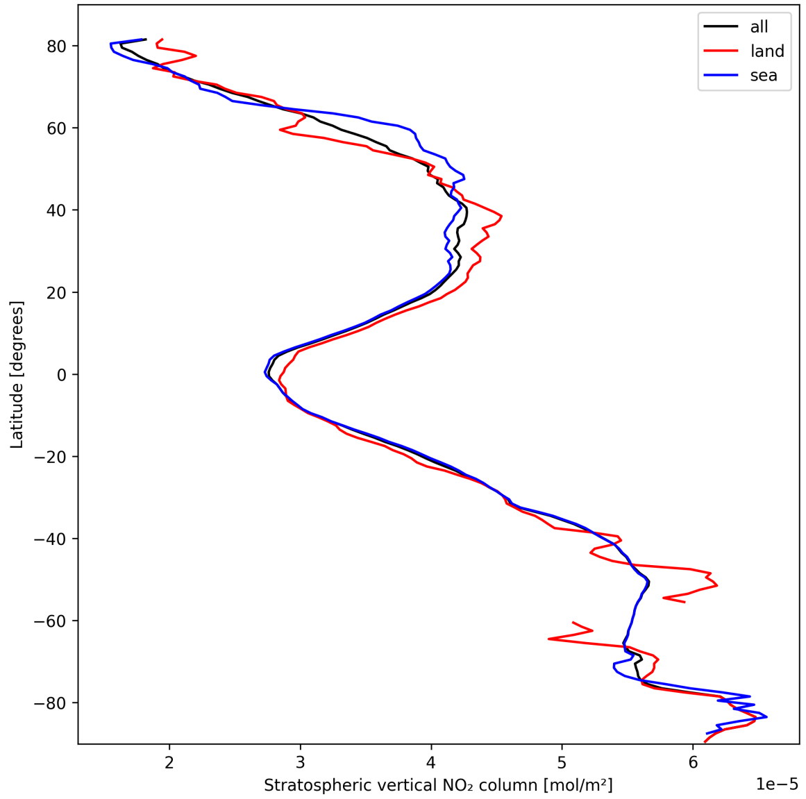
Figure 17: Zonal average of “Stratospheric vertical NO 2 column” for 2025-03-02 to 2025-03-03.
