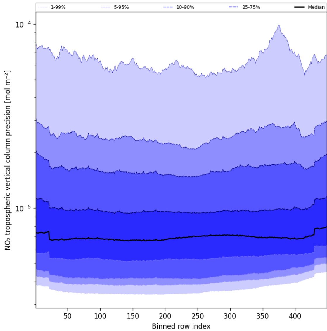
Figure 45: Along track statistics of “NO 2 tropospheric vertical column precision” for 2025-03-02 to 2025-03-03
