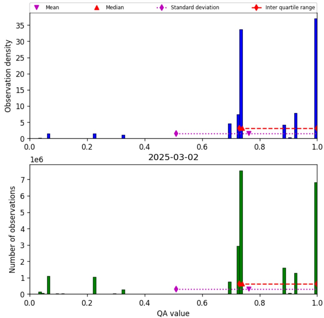
Figure 26: Histogram of “QA value” for 2025-03-02 to 2025-03-03
