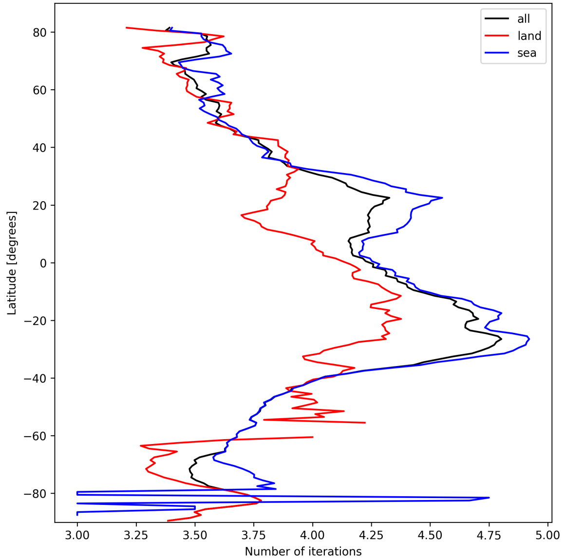
Figure 15: Zonal average of “Number of iterations” for 2025-03-02 to 2025-03-03.
