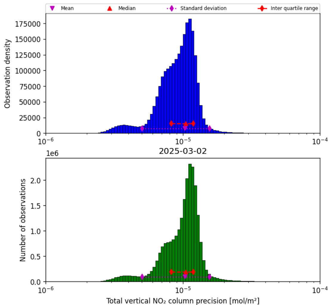
Figure 37: Histogram of “Total vertical NO 2 column precision” for 2025-03-02 to 2025-03-03
