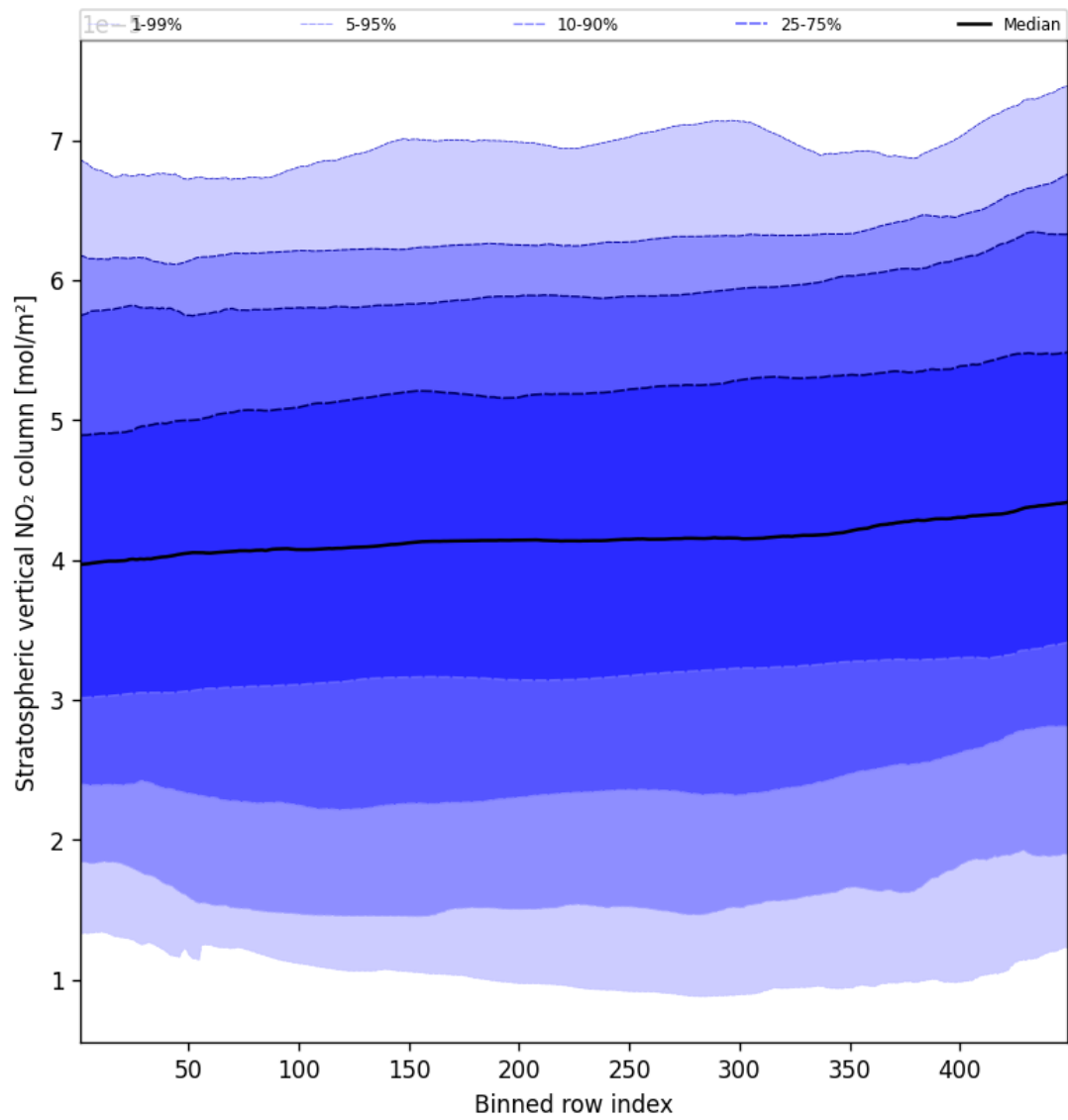
Figure 51: Along track statistics of “Stratospheric vertical NO 2 column” for 2025-03-02 to 2025-03-03
