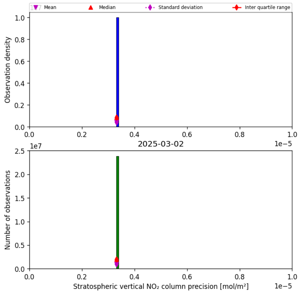
Figure 35: Histogram of “Stratospheric vertical NO 2 column precision” for 2025-03-02 to 2025-03-03
