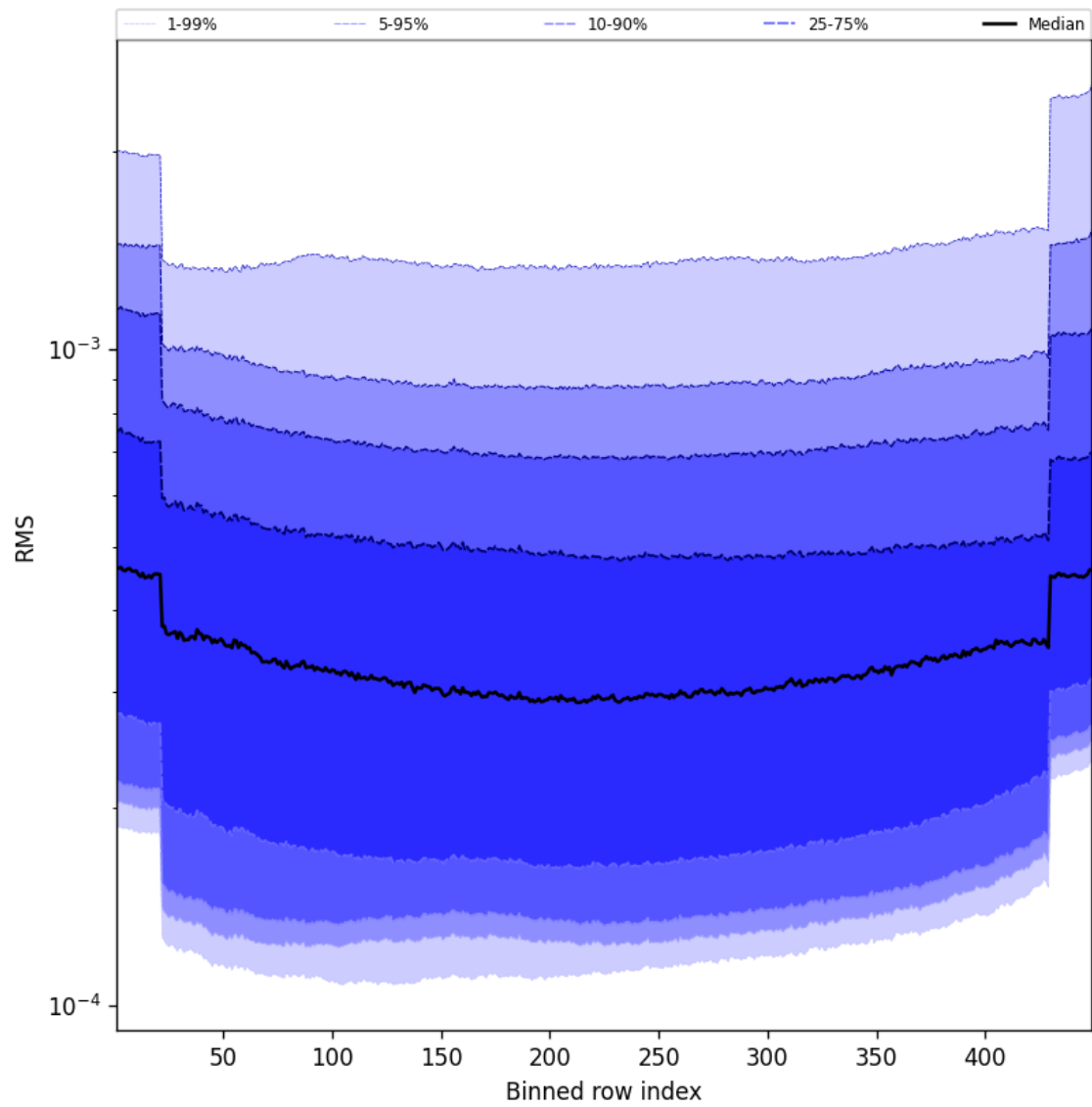
Figure 58: Along track statistics of “RMS” for 2025-03-02 to 2025-03-03
