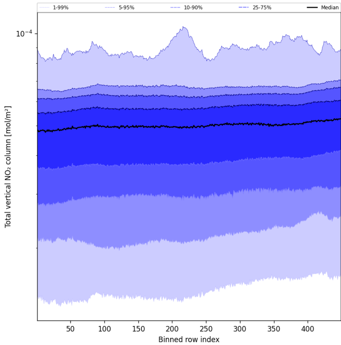
Figure 53: Along track statistics of “Total vertical NO 2 column” for 2025-03-02 to 2025-03-03
