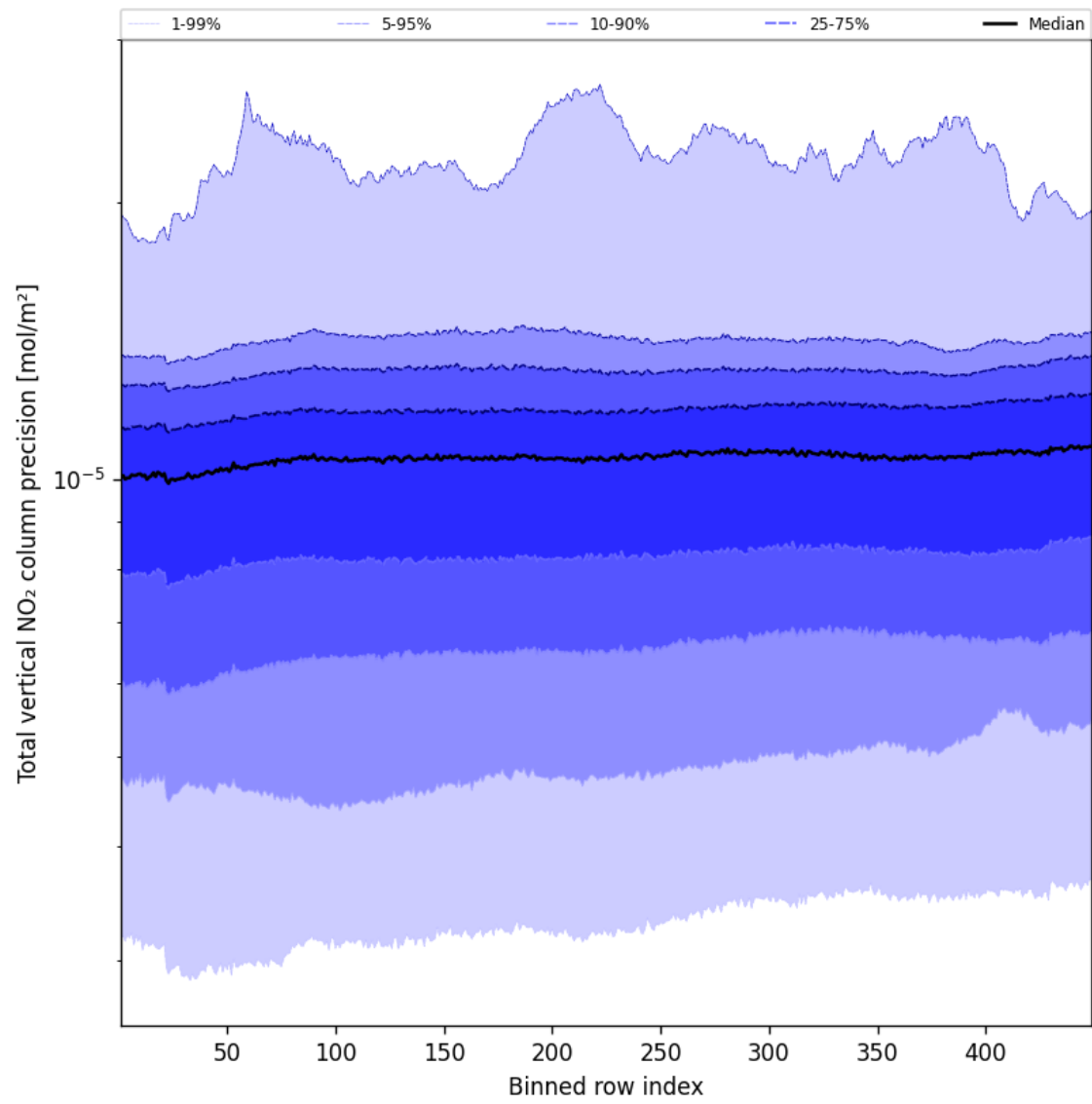
Figure 54: Along track statistics of “Total vertical NO 2 column precision” for 2025-03-02 to 2025-03-03
