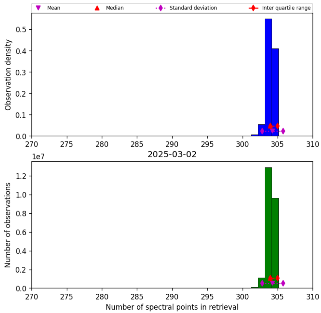
Figure 31: Histogram of “Number of spectral points in retrieval” for 2025-03-02 to 2025-03-03
