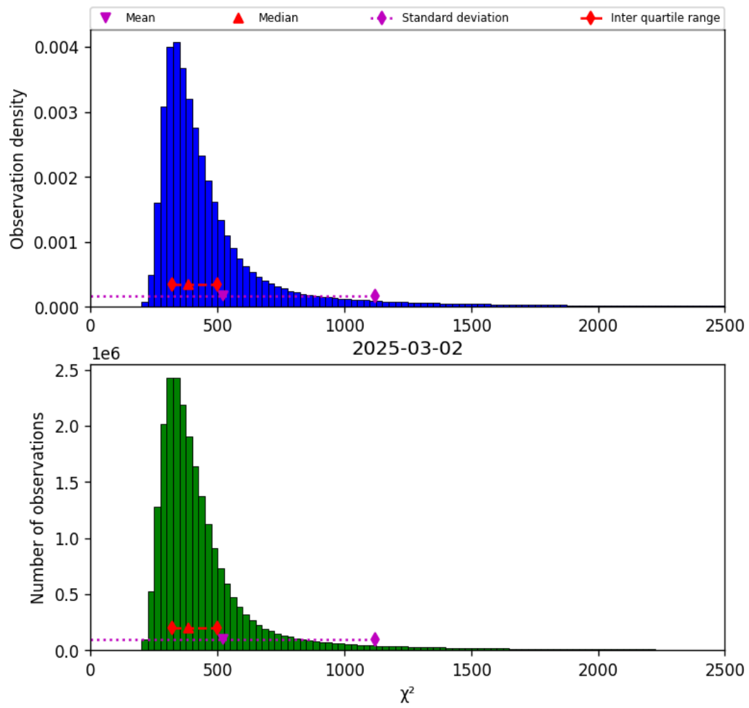
Figure 40: Histogram of “ \chi^2 ” for 2025-03-02 to 2025-03-03
