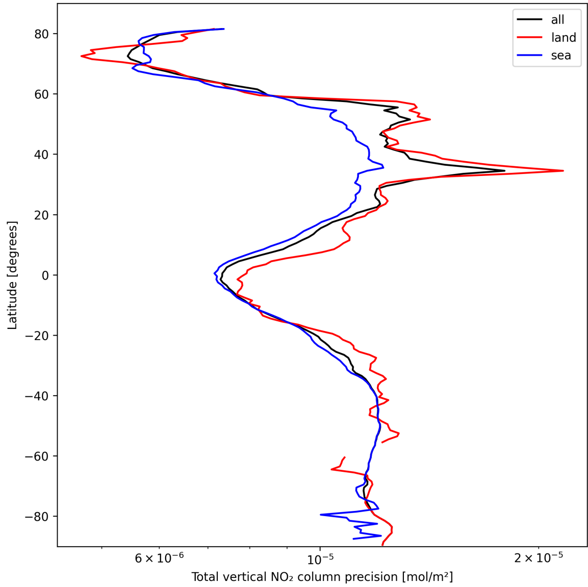
Figure 20: Zonal average of “Total vertical NO 2 column precision” for 2025-03-02 to 2025-03-03.
