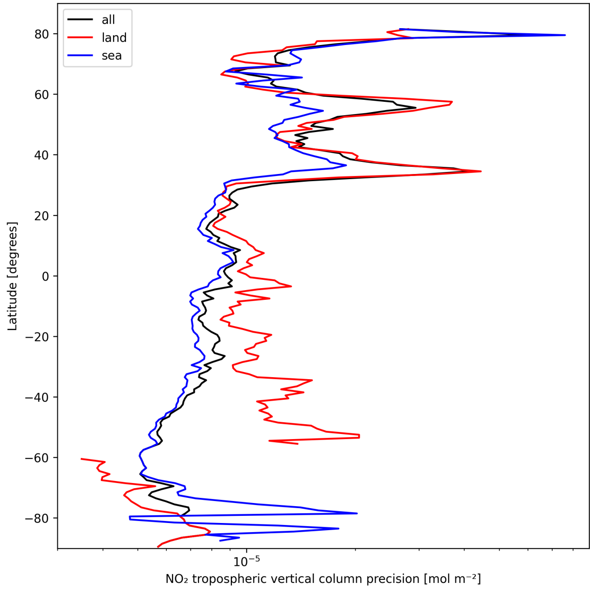
Figure 11: Zonal average of "NO 2 tropospheric vertical column precision" for 2025-03-02 to 2025-03-03.
