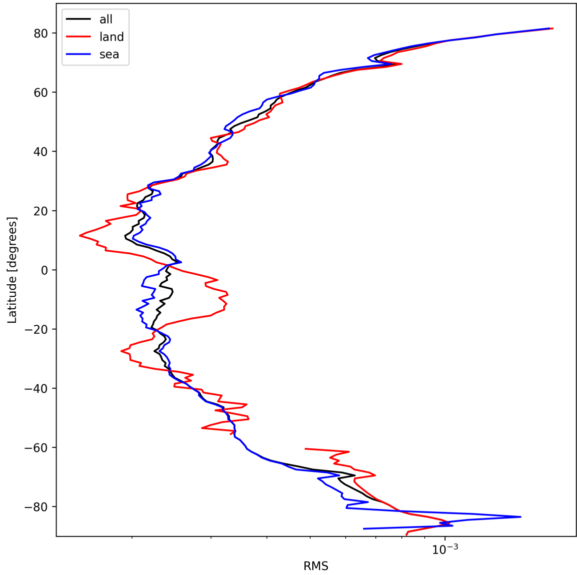
Figure 24: Zonal average of “RMS” for 2025-03-02 to 2025-03-03.
