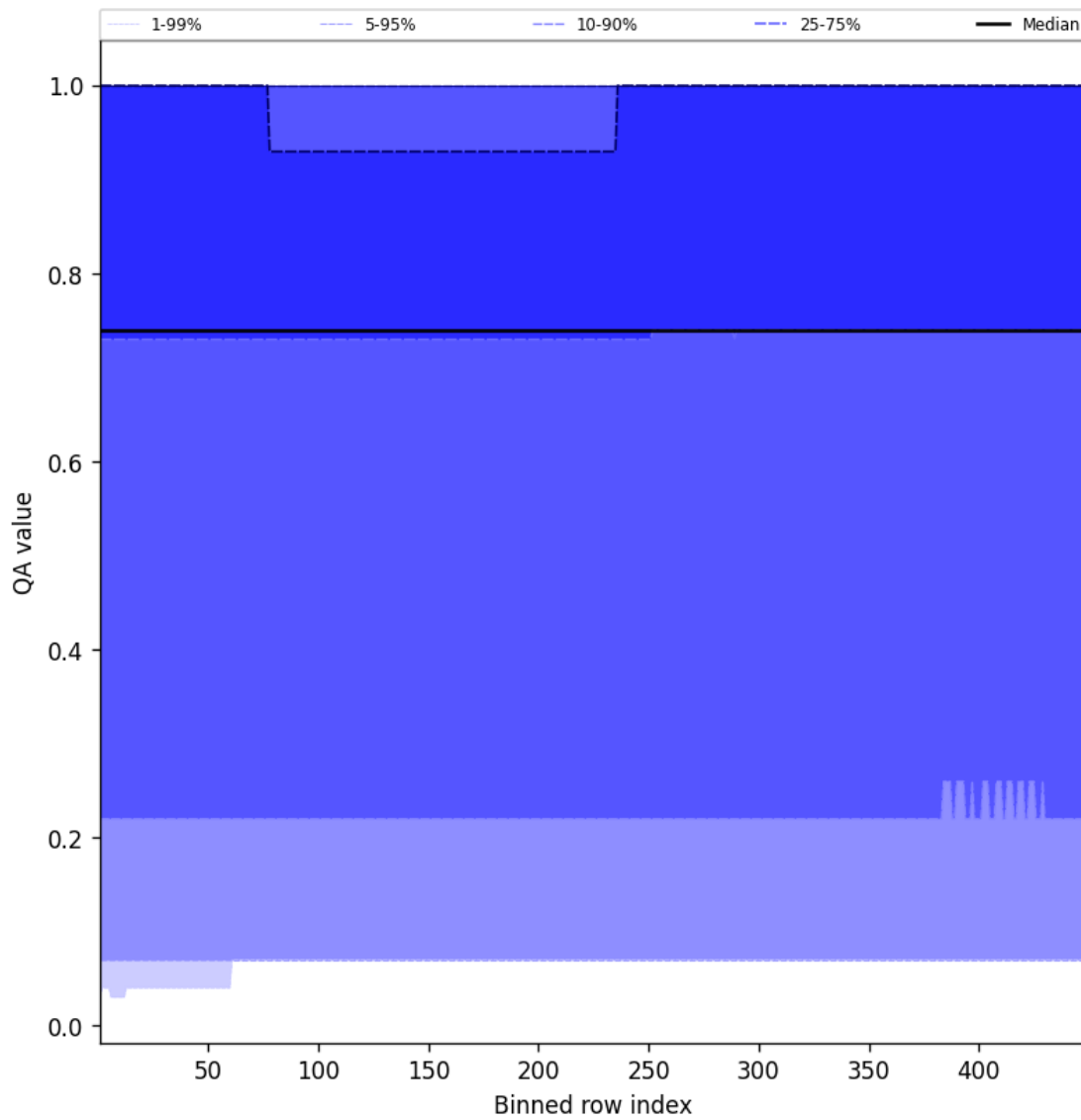
Figure 43: Along track statistics of “QA value” for 2025-03-02 to 2025-03-03
