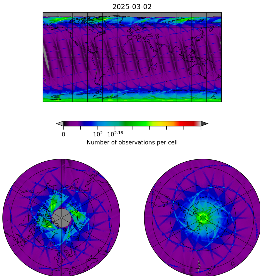
Figure 8: Map of the number of observations for 2025-03-02 to 2025-03-03
