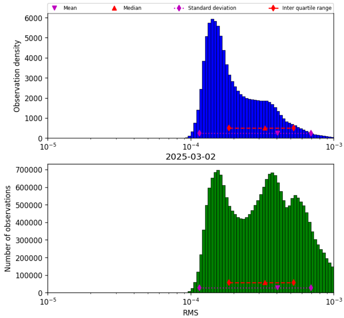
Figure 41: Histogram of “RMS” for 2025-03-02 to 2025-03-03
