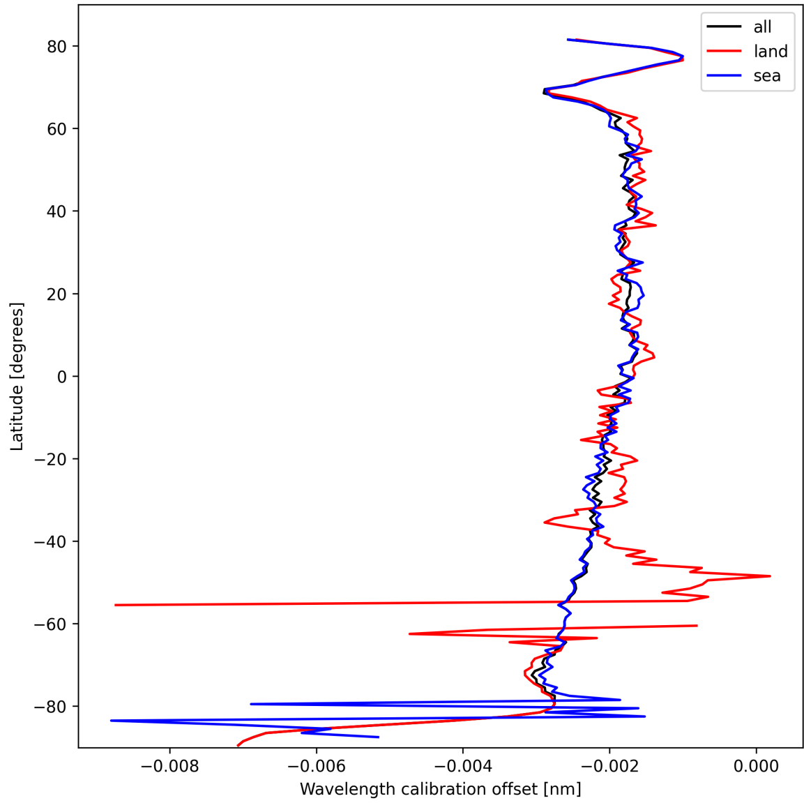
Figure 16: Zonal average of “Wavelength calibration offset” for 2025-03-02 to 2025-03-03.
