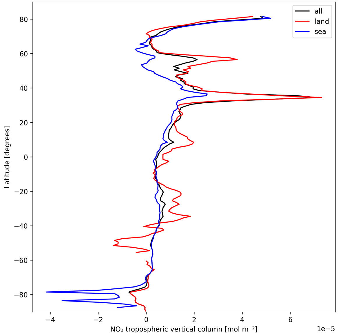
Figure 10: Zonal average of “NO 2 tropospheric vertical column” for 2025-03-02 to 2025-03-03.
