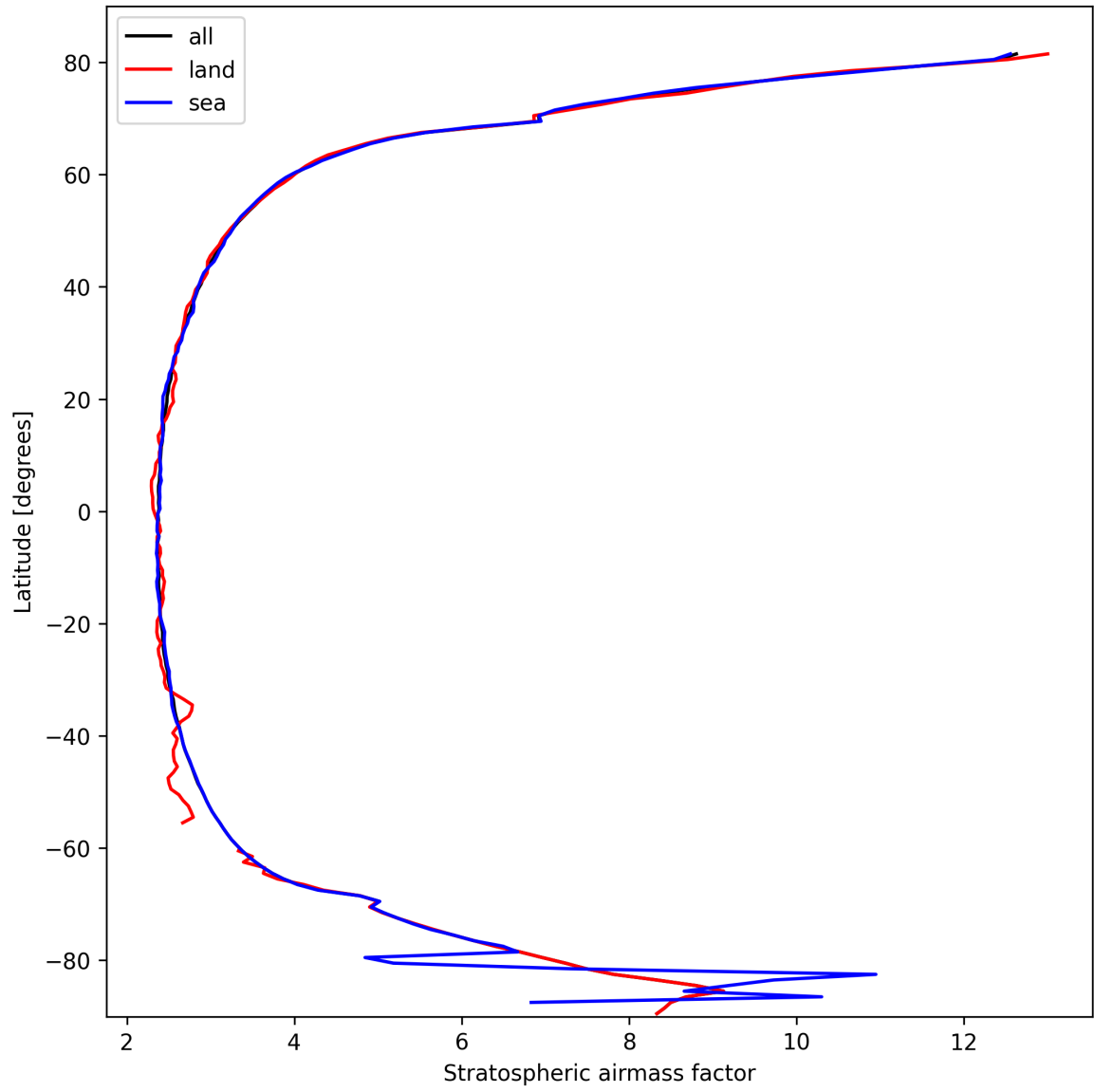
Figure 25: Zonal average of “Stratospheric airmass factor” for 2025-03-02 to 2025-03-03.
