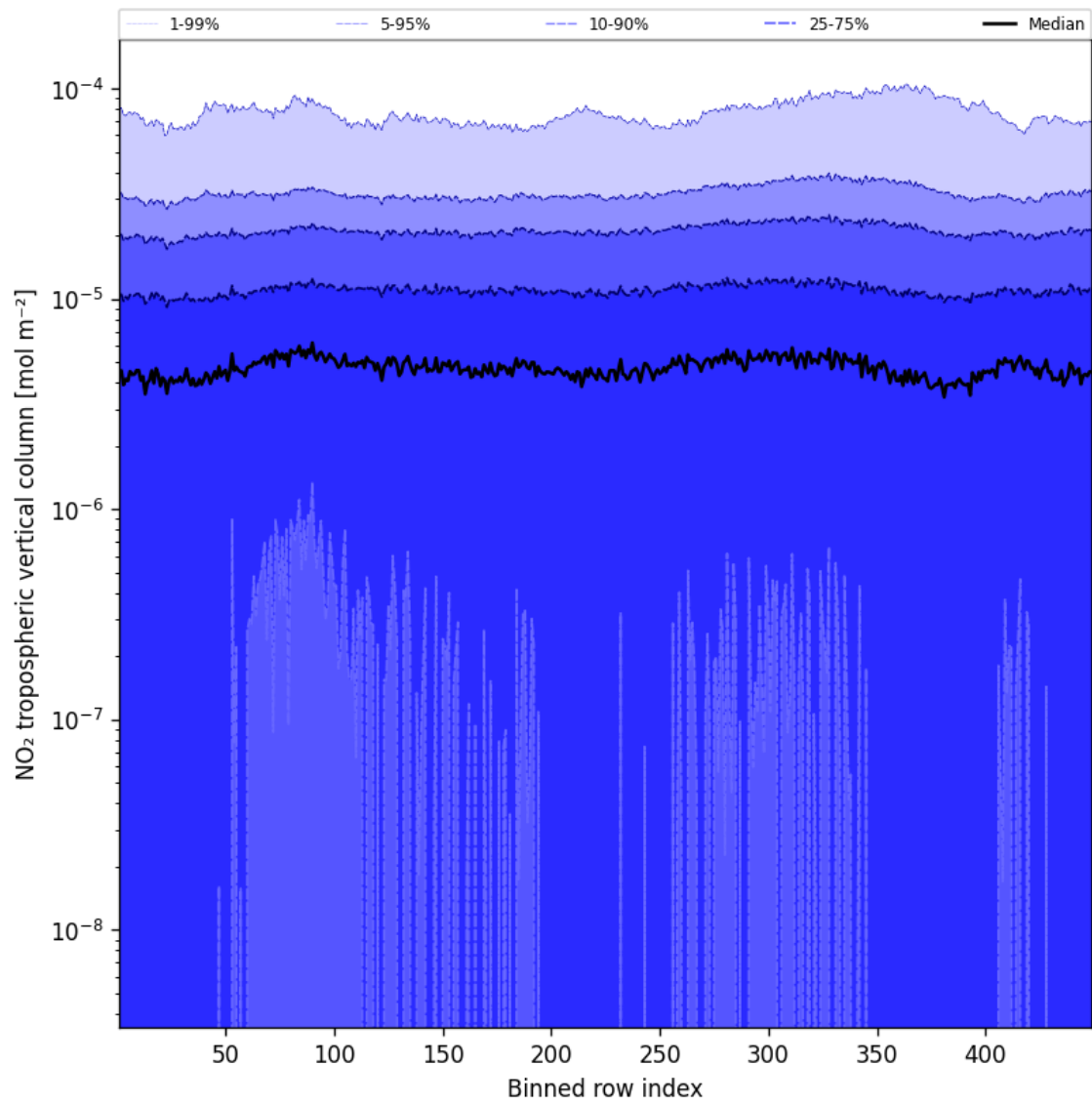
Figure 44: Along track statistics of “NO 2 tropospheric vertical column” for 2025-03-02 to 2025-03-03
