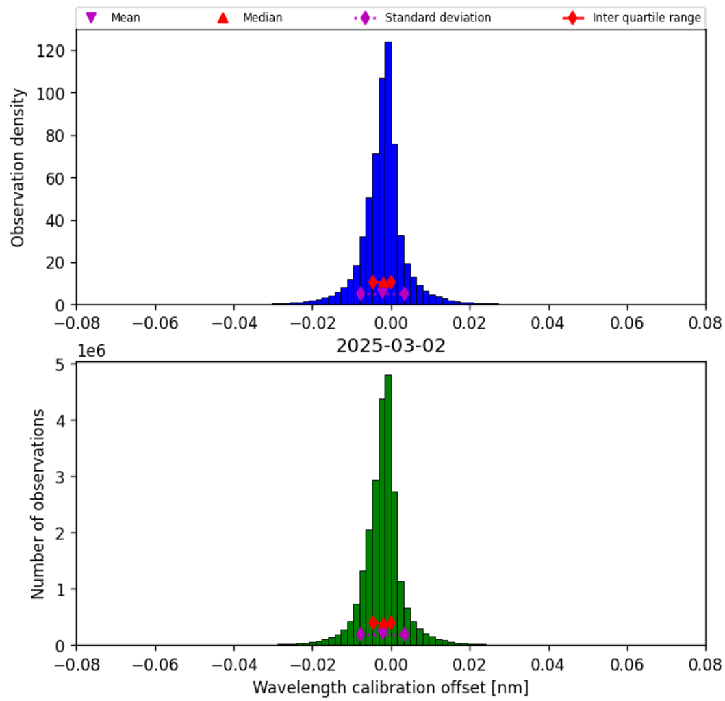
Figure 33: Histogram of “Wavelength calibration offset” for 2025-03-02 to 2025-03-03
