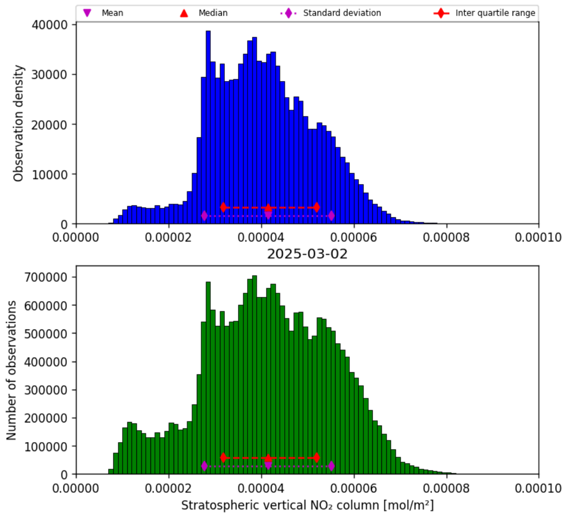
Figure 34: Histogram of “Stratospheric vertical NO 2 column” for 2025-03-02 to 2025-03-03
