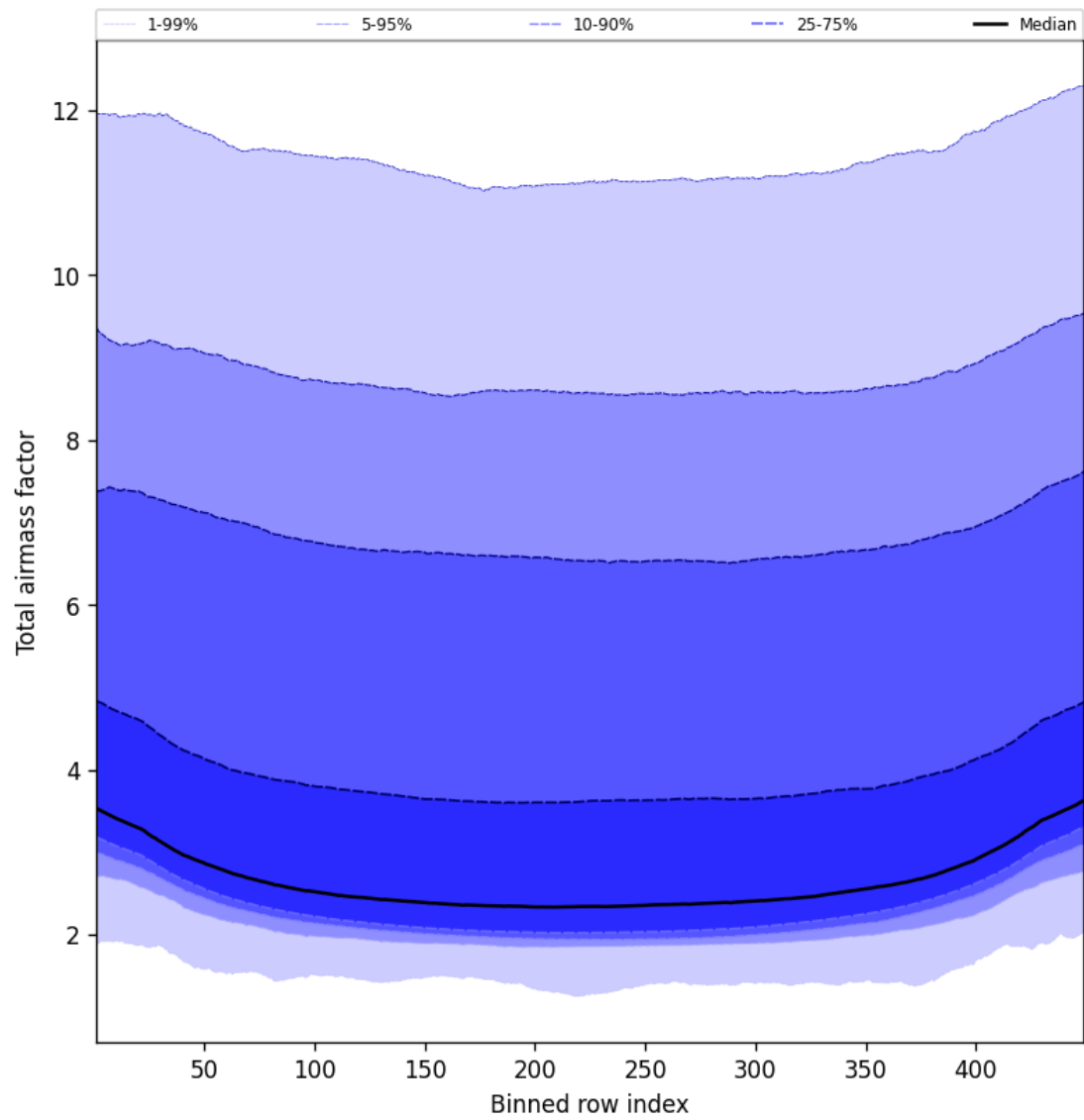
Figure 47: Along track statistics of “Total airmass factor” for 2025-03-02 to 2025-03-03
