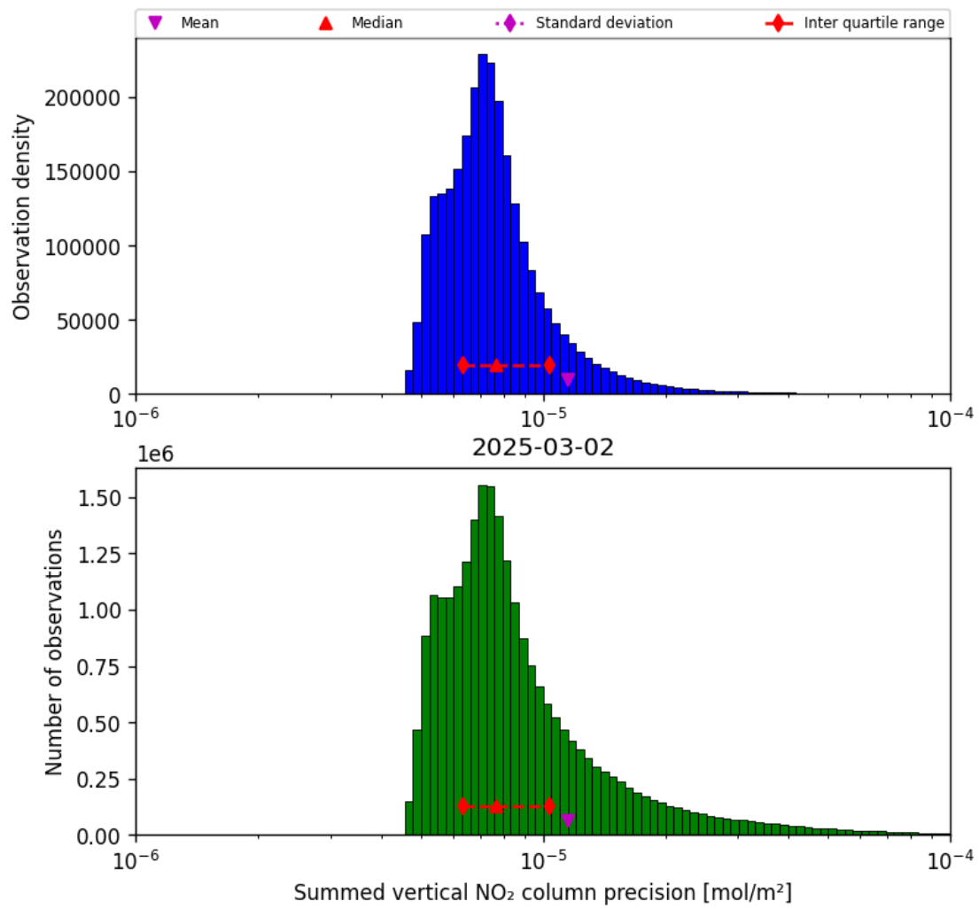
Figure 39: Histogram of “Summed vertical NO 2 column precision” for 2025-03-02 to 2025-03-03
