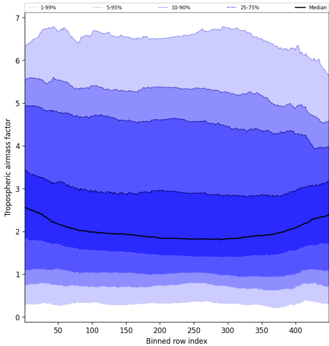
Figure 46: Along track statistics of “Tropospheric air mass factor” for 2025-03-02 to 2025-03-03
