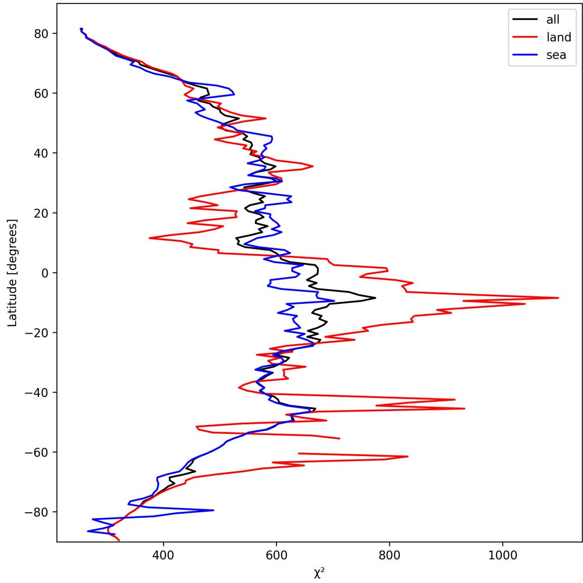
Figure 23: Zonal average of “ \chi^2 ” for 2025-03-02 to 2025-03-03.
