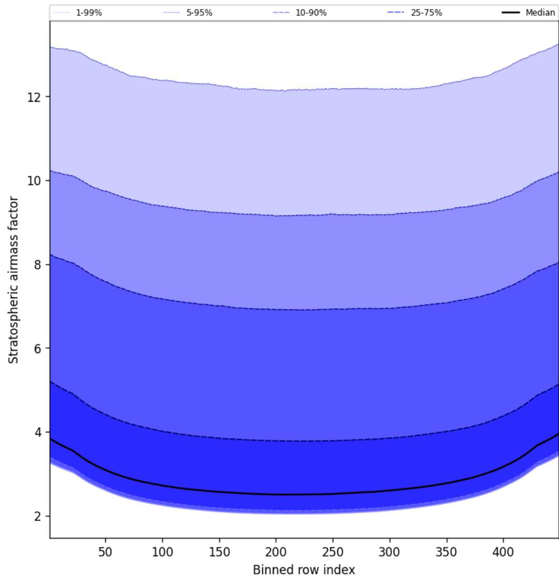
Figure 59: Along track statistics of “Stratospheric airmass factor” for 2025-03-02 to 2025-03-03
