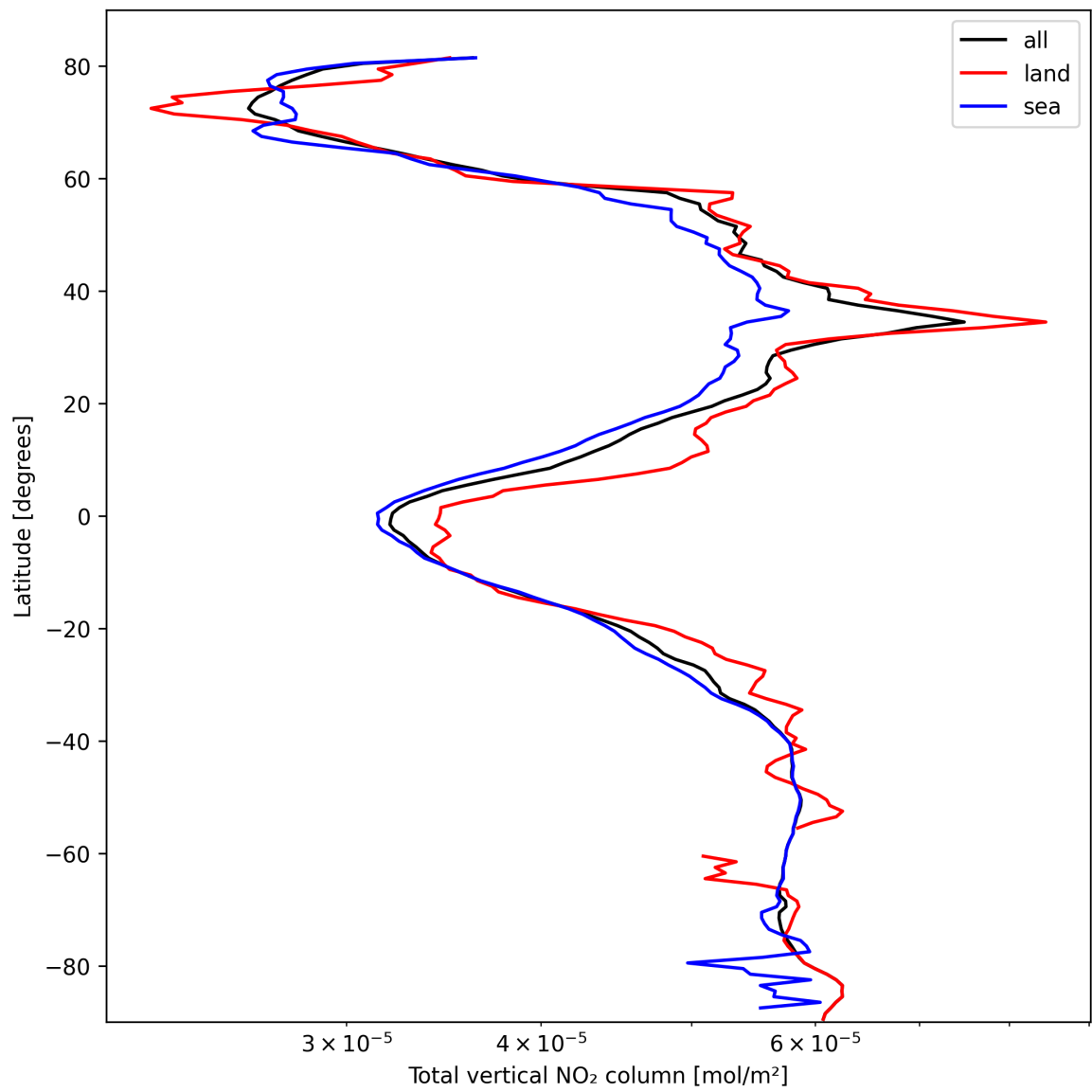
Figure 19: Zonal average of “Total vertical NO 2 column” for 2025-03-02 to 2025-03-03.
