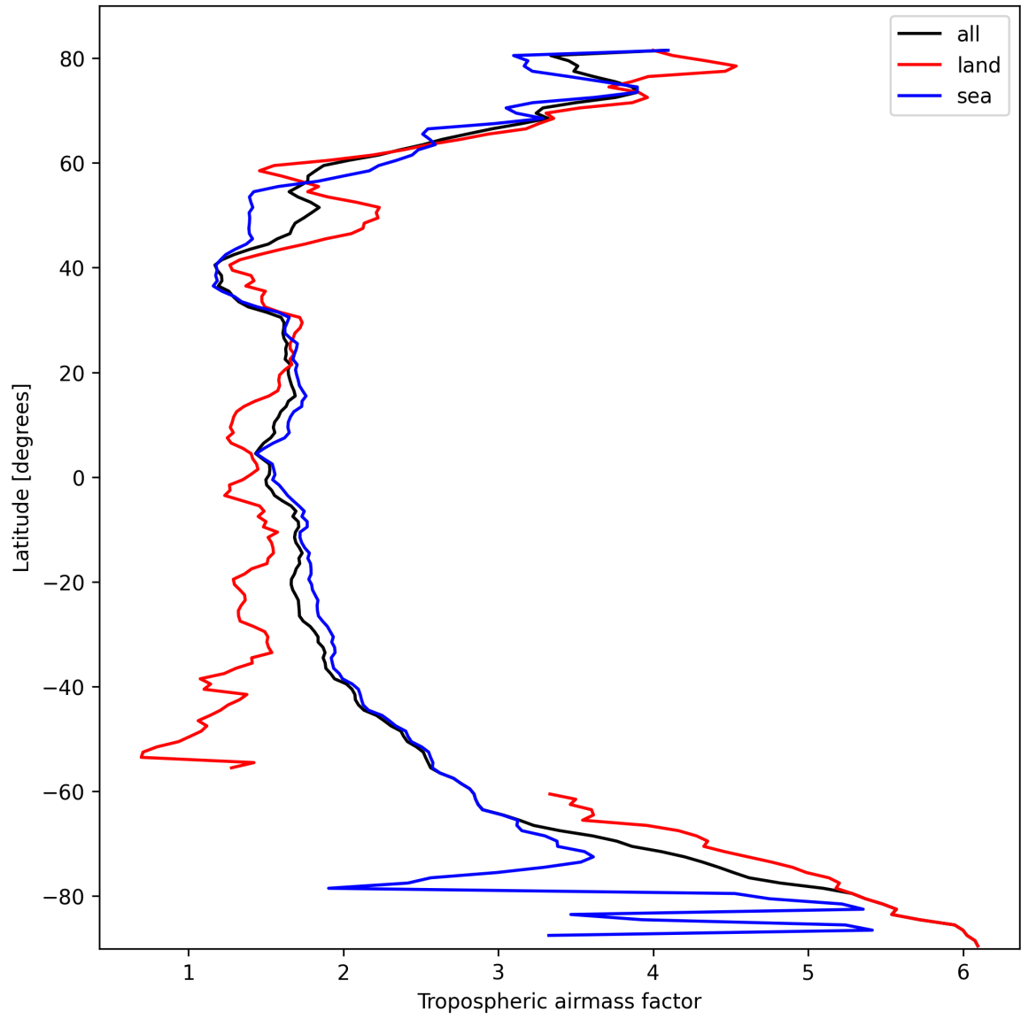
Figure 12: Zonal average of “Tropospheric air mass factor” for 2025-03-02 to 2025-03-03.
