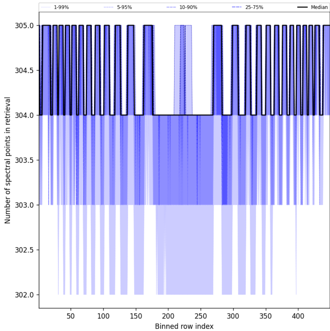
Figure 48: Along track statistics of “Number of spectral points in retrieval” for 2025-03-02 to 2025-03-03
