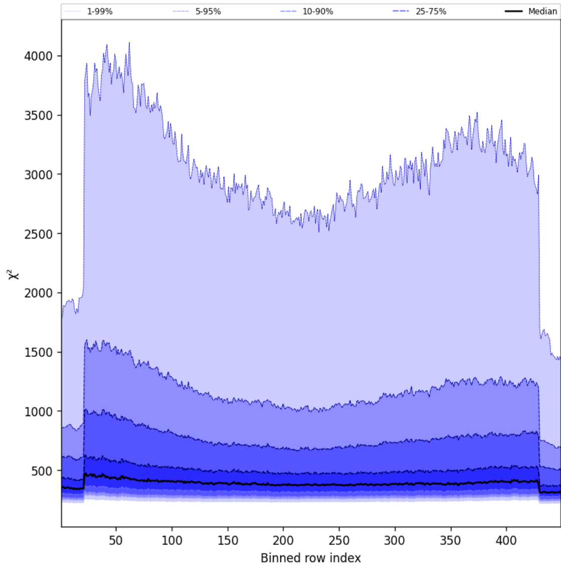
Figure 57: Along track statistics of “ \chi^2 ” for 2025-03-02 to 2025-03-03
