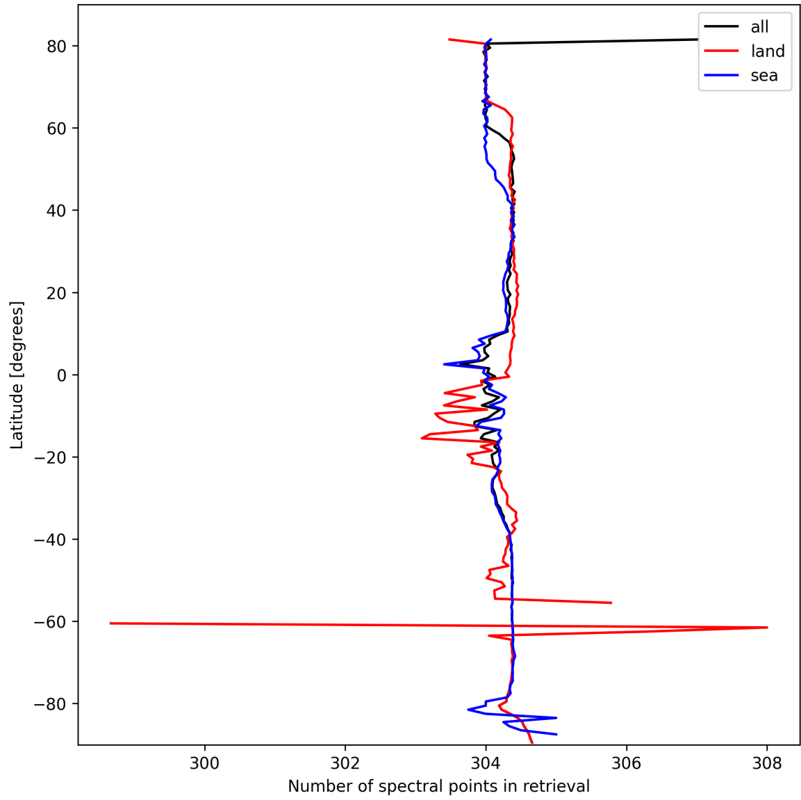
Figure 14: Zonal average of “Number of spectral points in retrieval” for 2025-03-02 to 2025-03-03.
