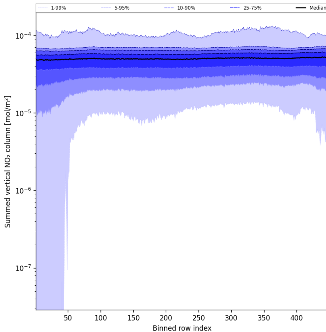
Figure 55: Along track statistics of “Summed vertical NO 2 column” for 2025-03-02 to 2025-03-03
