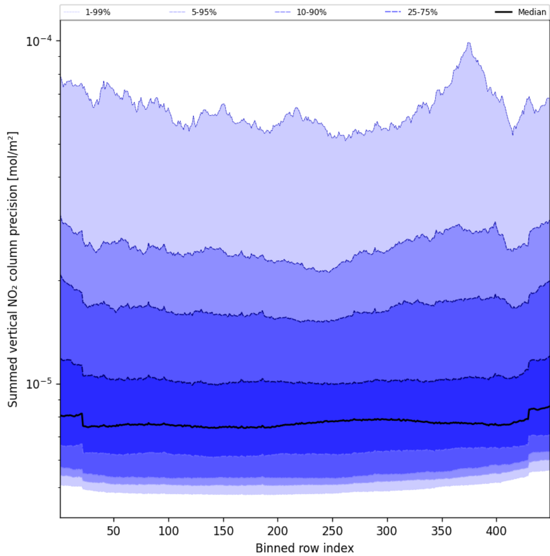
Figure 56: Along track statistics of “Summed vertical NO 2 column precision” for 2025-03-02 to 2025-03-03
