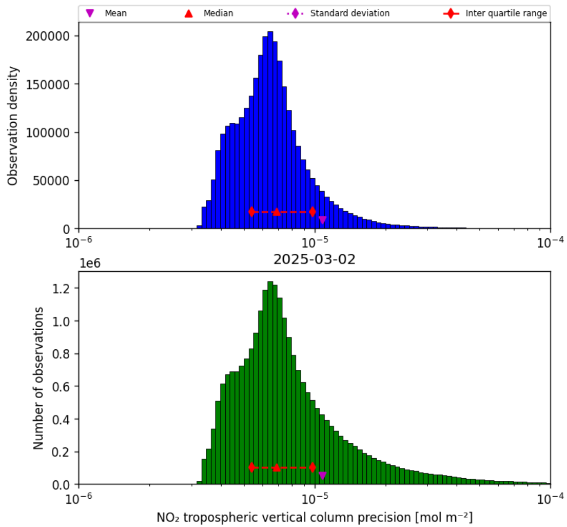
Figure 28: Histogram of “NO 2 tropospheric vertical column precision” for 2025-03-02 to 2025-03-03
