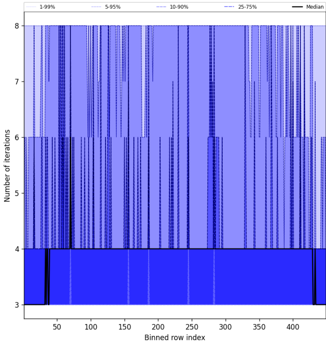
Figure 49: Along track statistics of “Number of iterations” for 2025-03-02 to 2025-03-03
