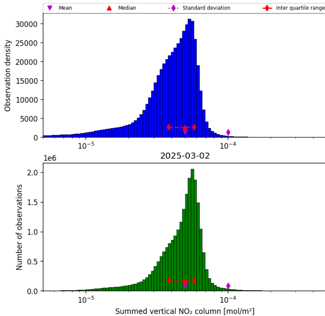
Figure 38: Histogram of “Summed vertical NO 2 column” for 2025-03-02 to 2025-03-03
