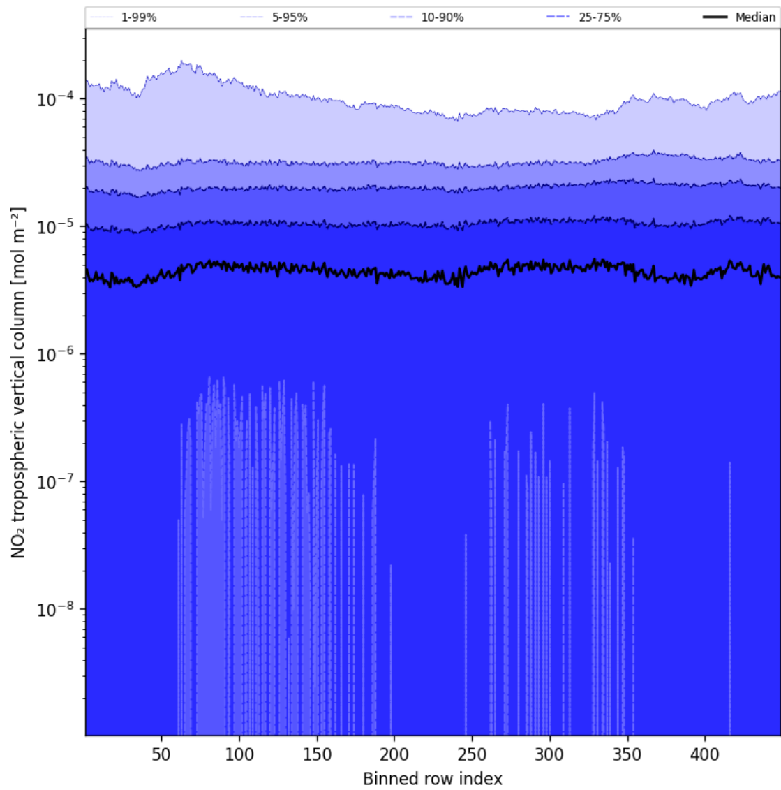
Figure 44: Along track statistics of “NO 2 tropospheric vertical column” for 2025-03-04 to 2025-03-04
