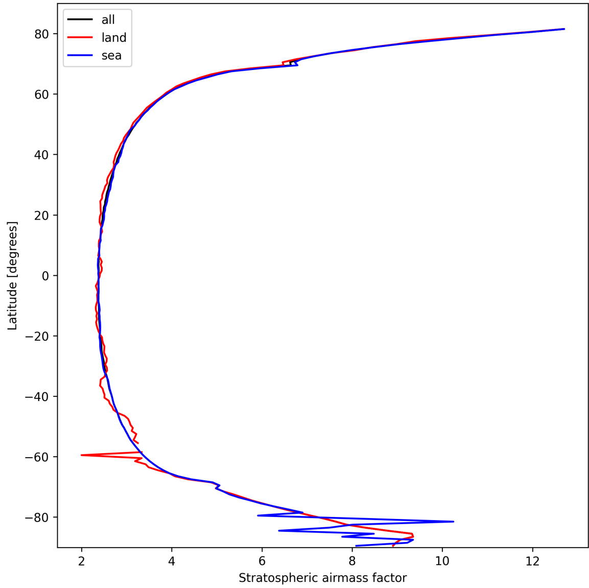
Figure 25: Zonal average of “Stratospheric air mass factor” for 2025-03-04 to 2025-03-04.
