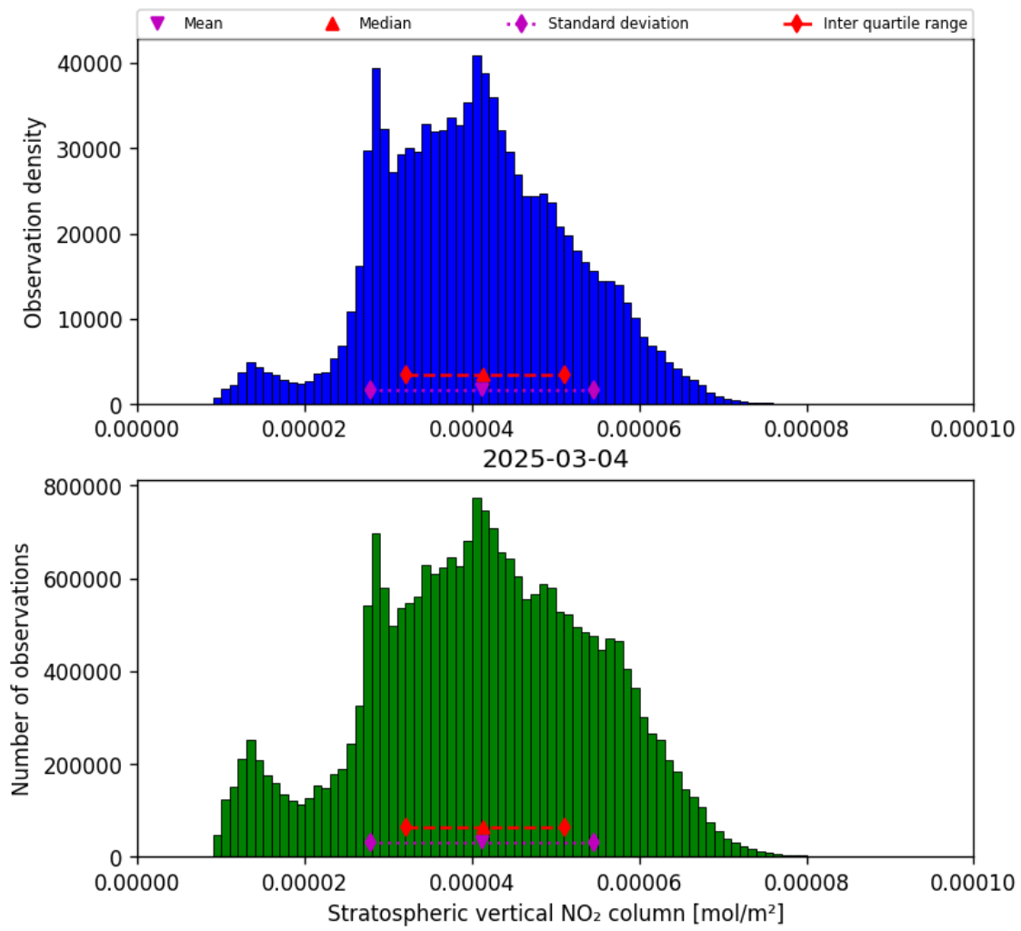
Figure 34: Histogram of “Stratospheric vertical NO 2 column” for 2025-03-04 to 2025-03-04
