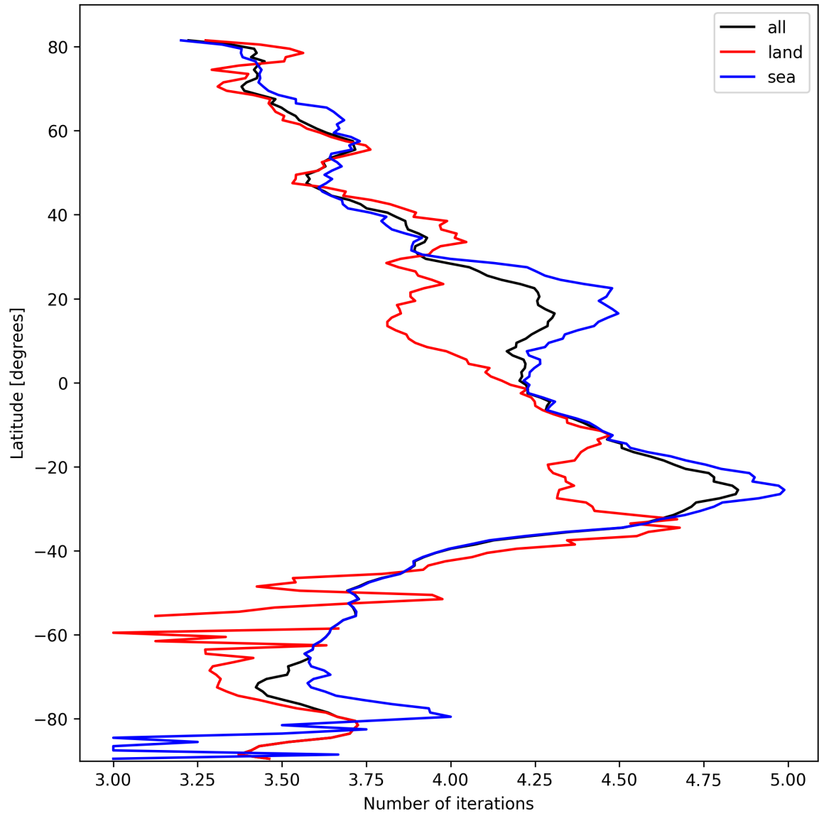
Figure 15: Zonal average of “Number of iterations” for 2025-03-04 to 2025-03-04.
