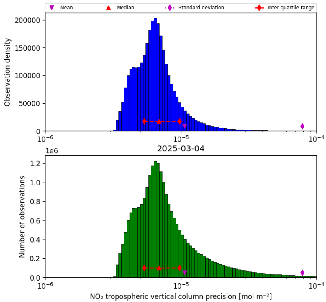
Figure 28: Histogram of “NO 2 tropospheric vertical column precision” for 2025-03-04 to 2025-03-04
