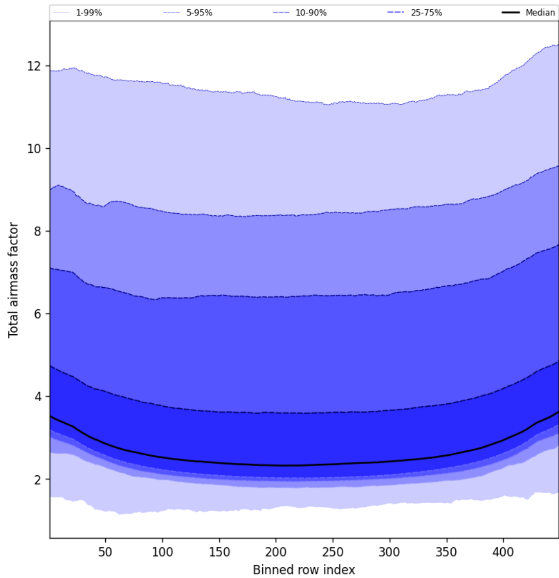
Figure 47: Along track statistics of “Total airmass factor” for 2025-03-04 to 2025-03-04
