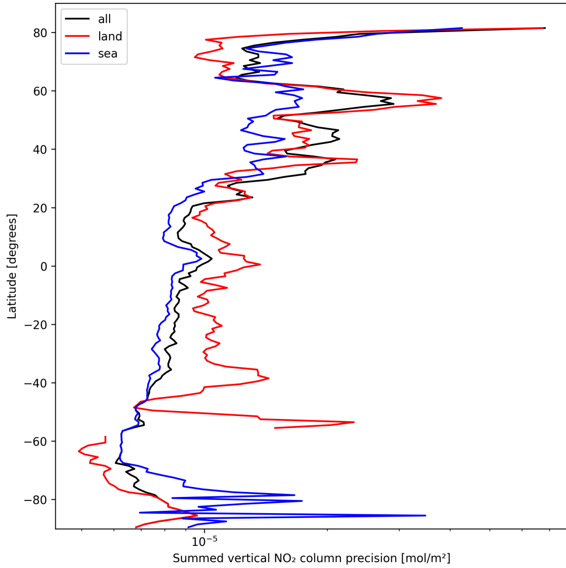
Figure 22: Zonal average of “Summed vertical NO 2 column precision” for 2025-03-04 to 2025-03-04.
