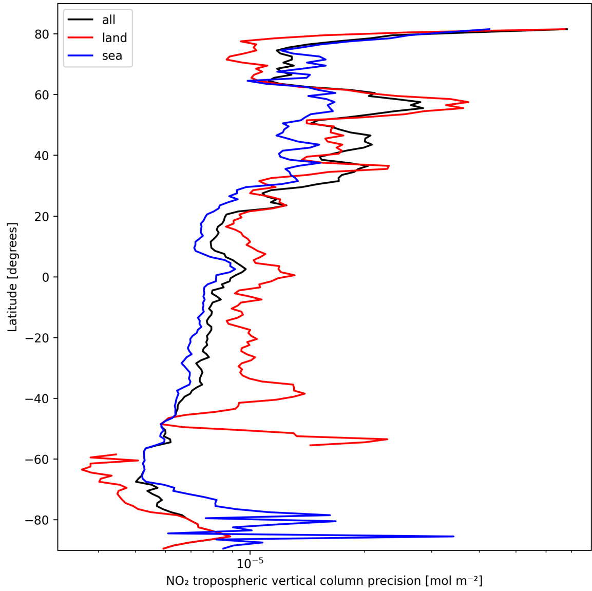
Figure 11: Zonal average of “NO 2 tropospheric vertical column precision” for 2025-03-04 to 2025-03-04.
