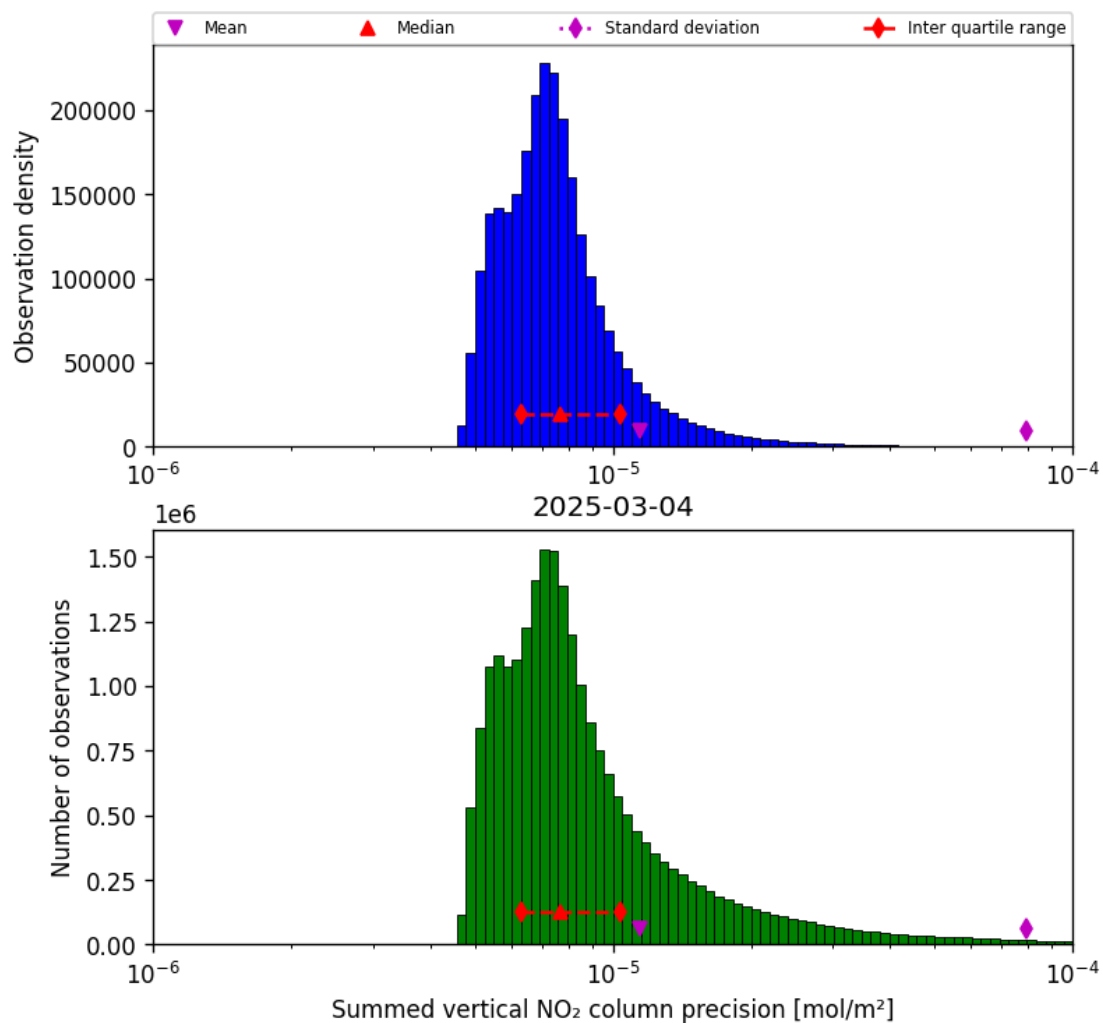
Figure 39: Histogram of "Summed vertical NO 2 column precision" for 2025-03-04 to 2025-03-04
