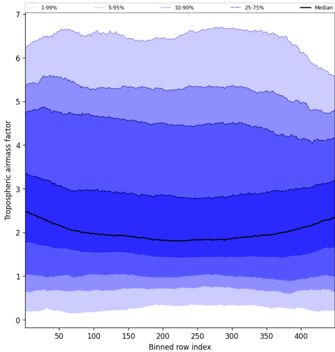
Figure 46: Along track statistics of “Tropospheric airmass factor” for 2025-03-04 to 2025-03-04
