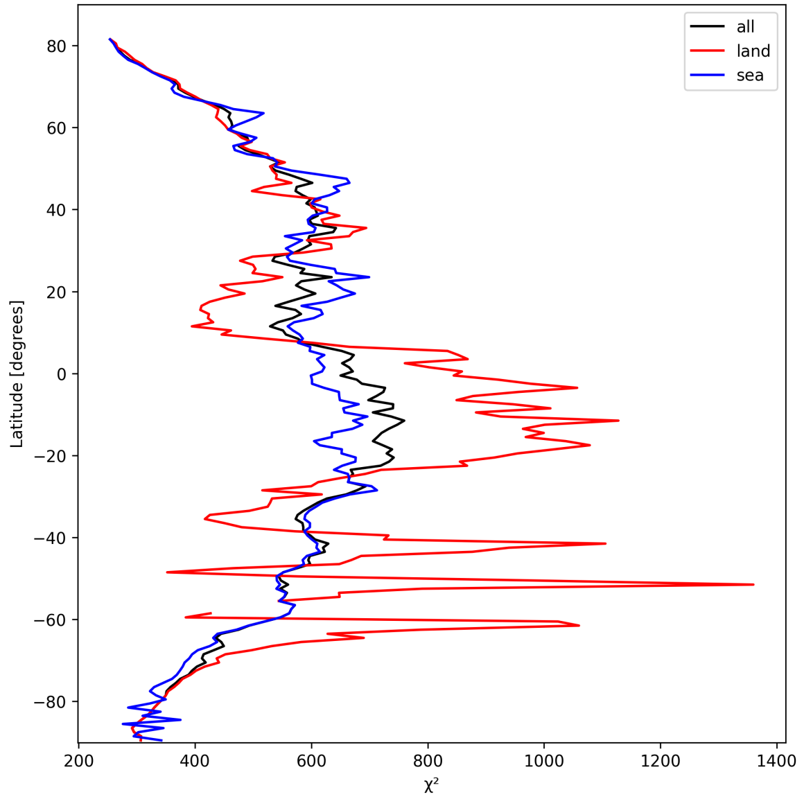
Figure 23: Zonal average of “ \chi^2 ” for 2025-03-04 to 2025-03-04.
