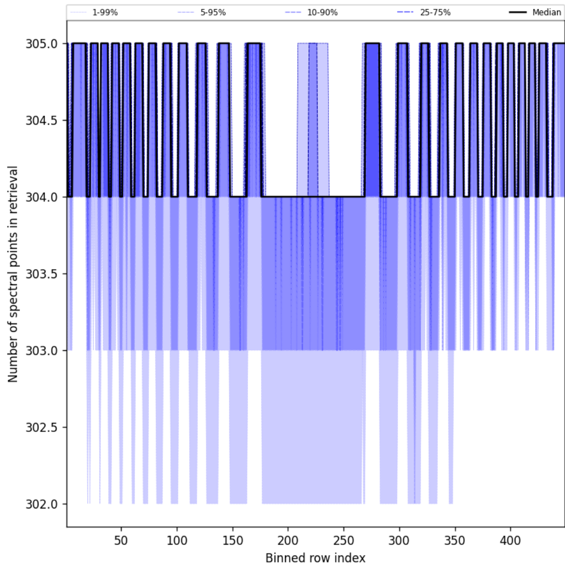
Figure 48: Along track statistics of “Number of spectral points in retrieval” for 2025-03-04 to 2025-03-04
