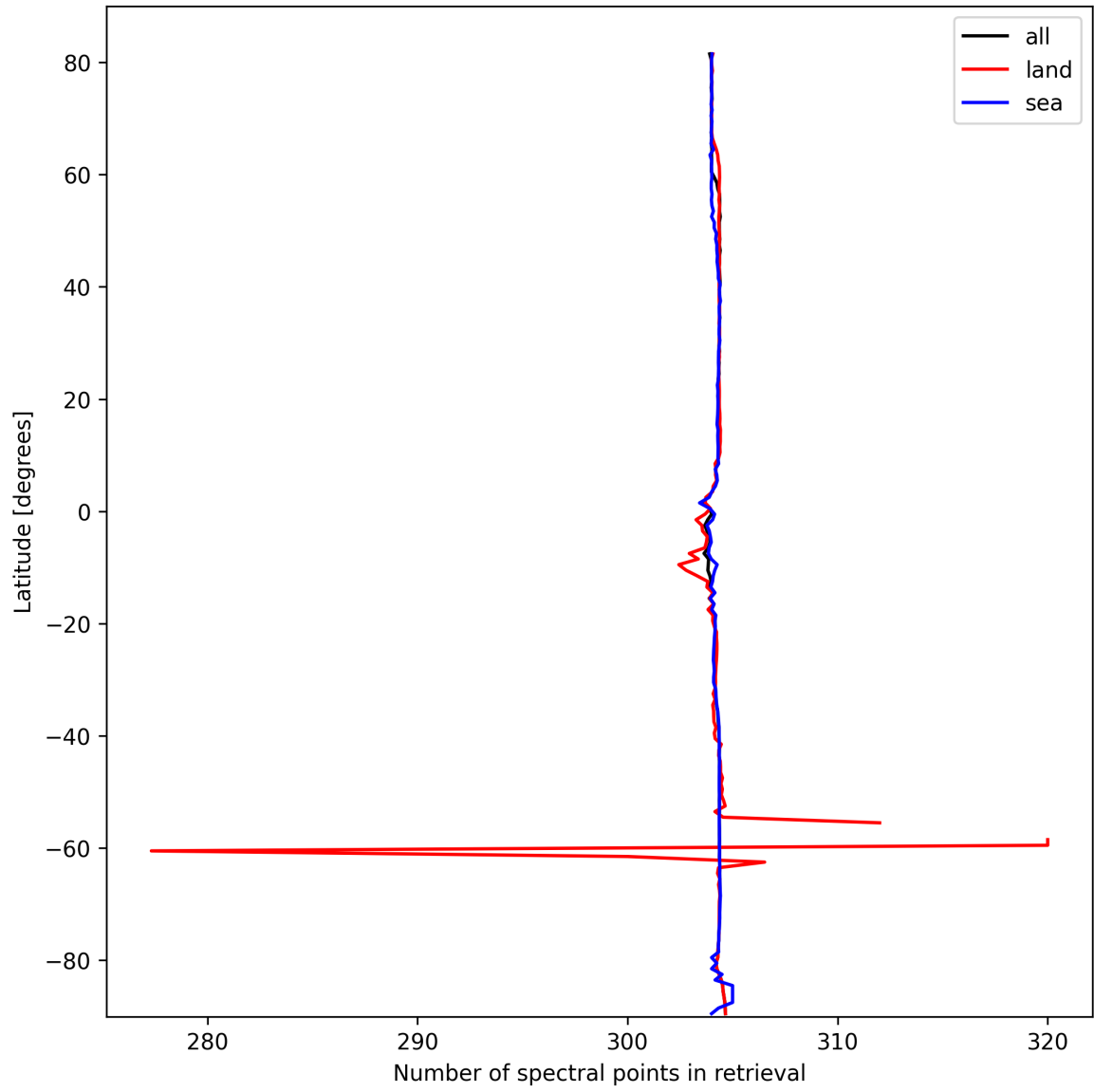
Figure 14: Zonal average of “Number of spectral points in retrieval” for 2025-03-04 to 2025-03-04.
