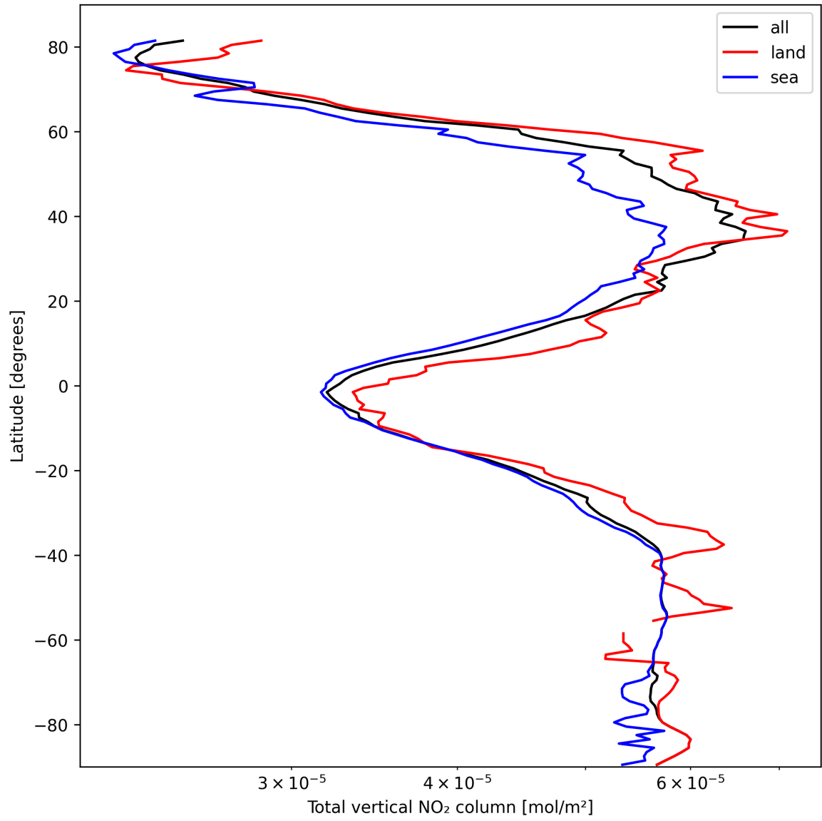
Figure 19: Zonal average of “Total vertical NO 2 column” for 2025-03-04 to 2025-03-04.
