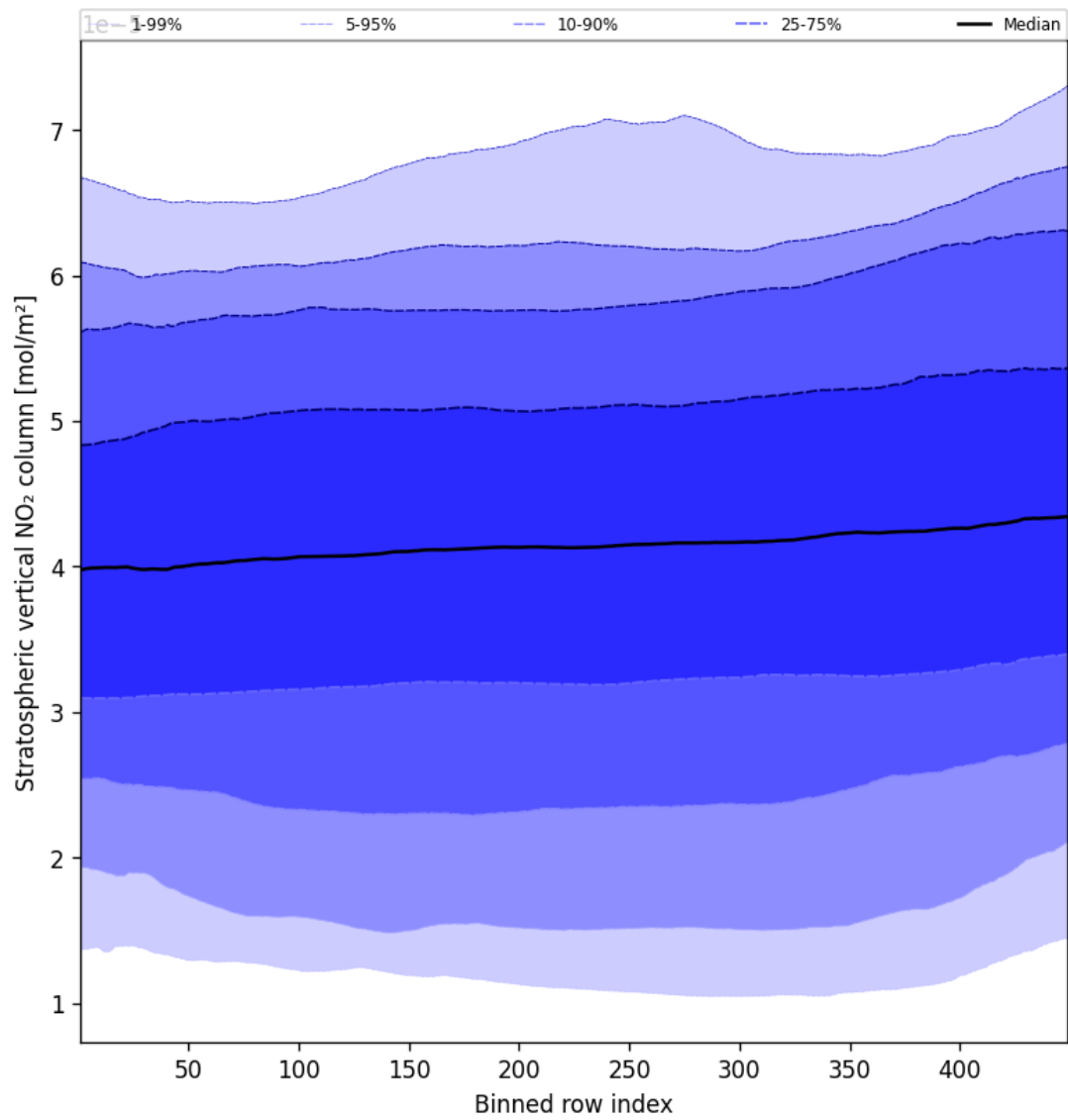
Figure 51: Along track statistics of “Stratospheric vertical NO 2 column” for 2025-03-04 to 2025-03-04
