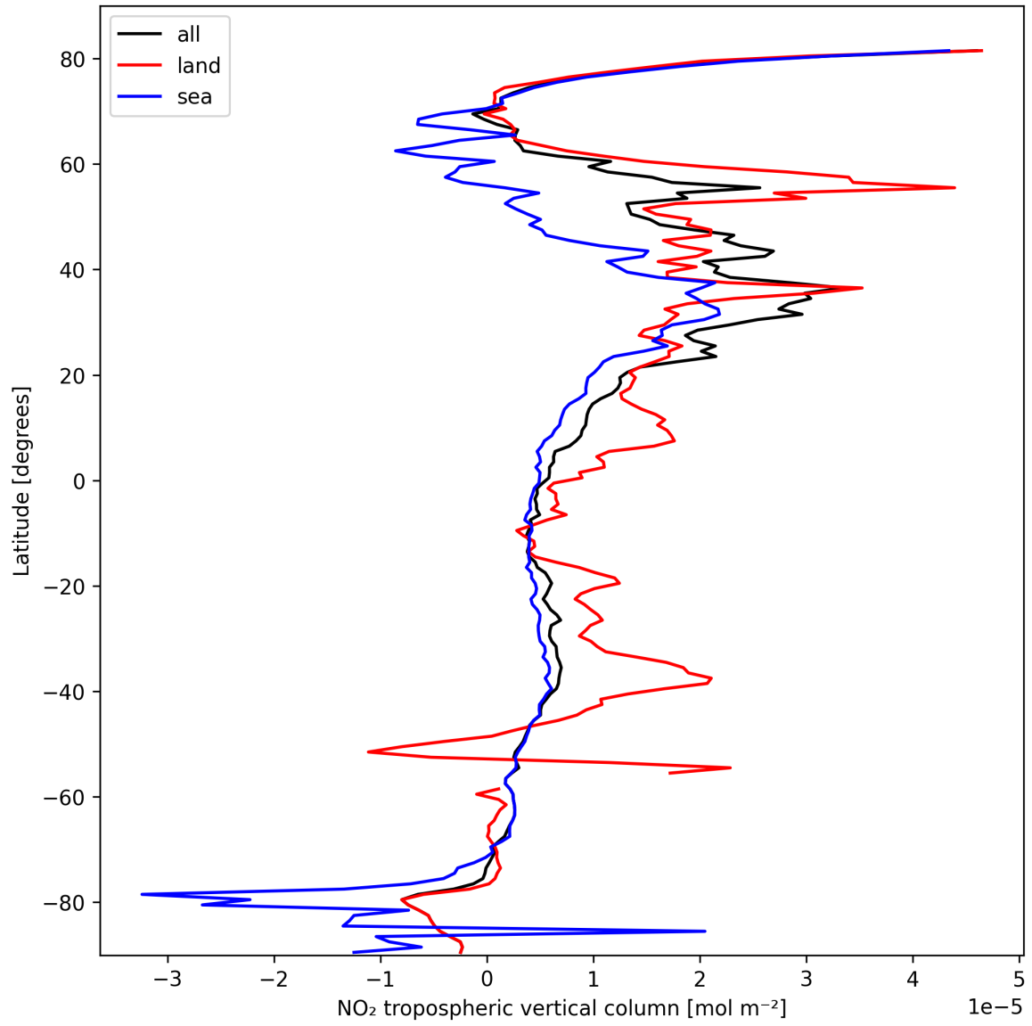
Figure 10: Zonal average of “NO 2 tropospheric vertical column” for 2025-03-04 to 2025-03-04.
