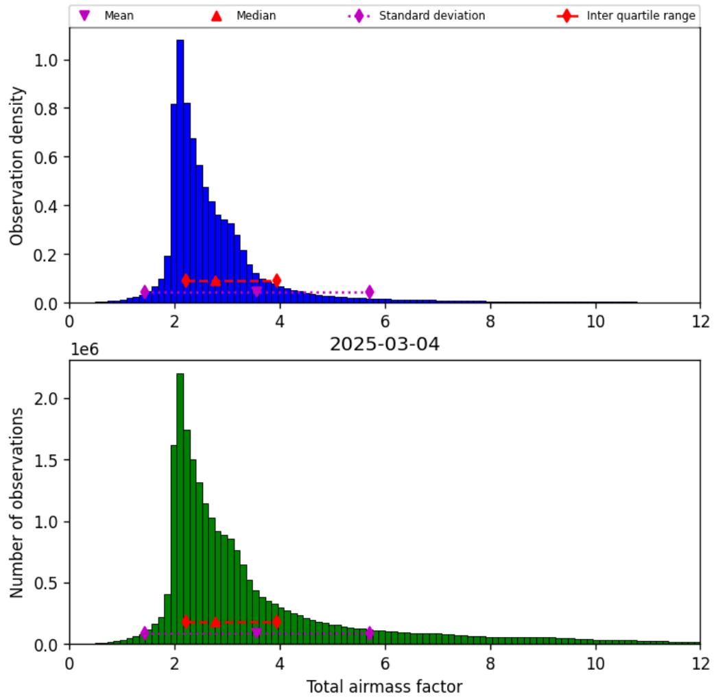
Figure 30: Histogram of “Total airmass factor” for 2025-03-04 to 2025-03-04
