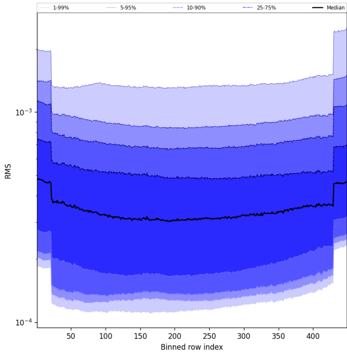
Figure 58: Along track statistics of “RMS” for 2025-03-04 to 2025-03-04
