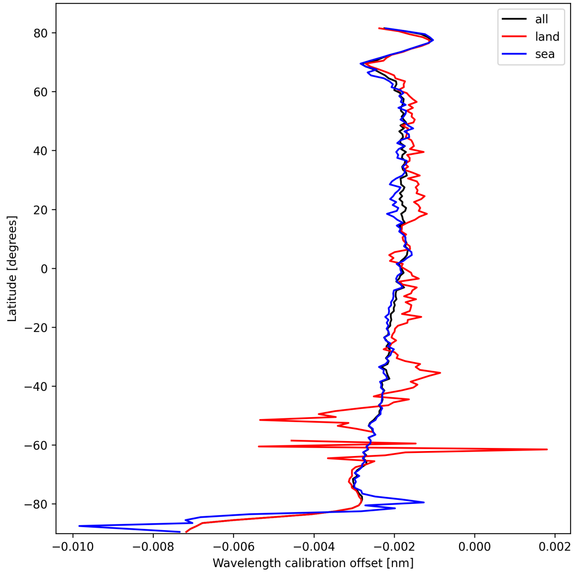
Figure 16: Zonal average of “Wavelength calibration offset” for 2025-03-04 to 2025-03-04.
