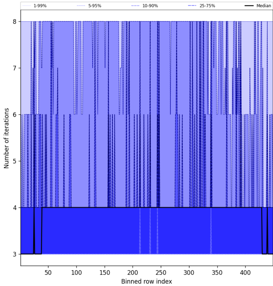
Figure 49: Along track statistics of “Number of iterations” for 2025-03-04 to 2025-03-04
