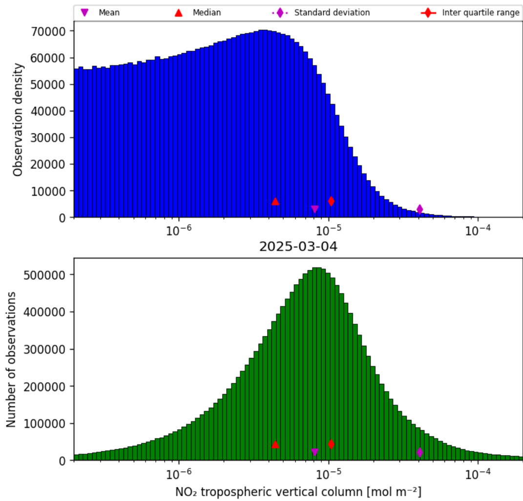
Figure 27: Histogram of “NO 2 tropospheric vertical column” for 2025-03-04 to 2025-03-04
