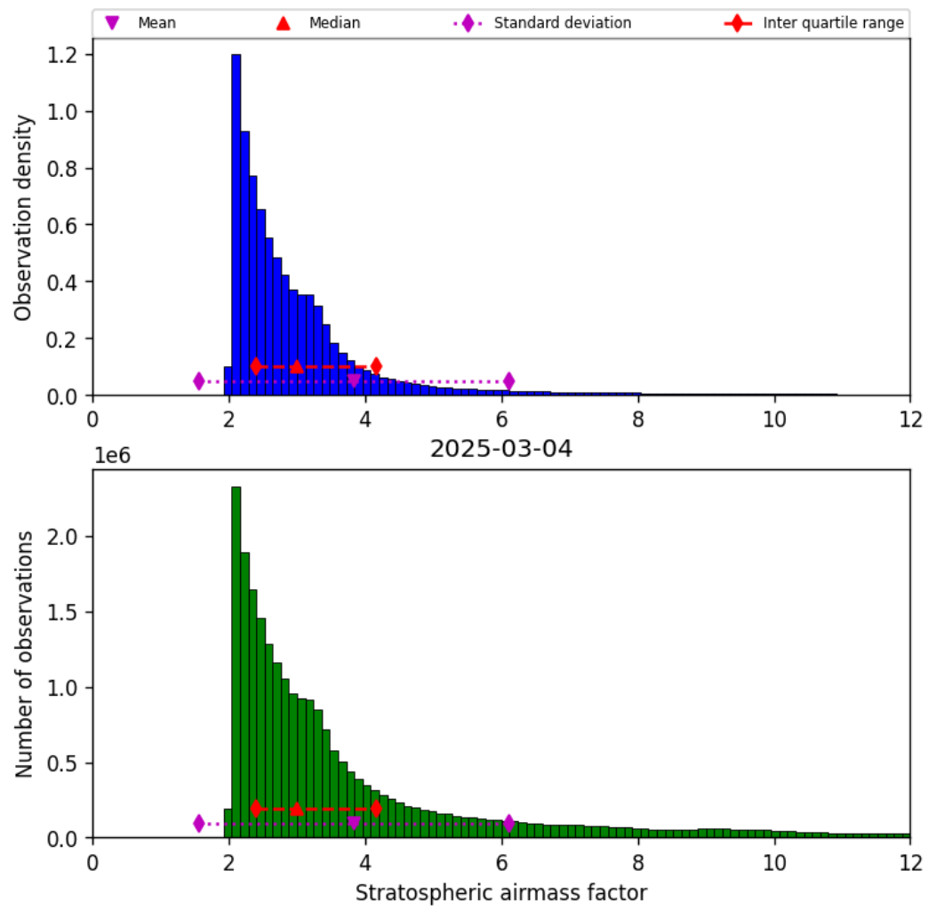
Figure 42: Histogram of “Stratospheric airmass factor” for 2025-03-04 to 2025-03-04
