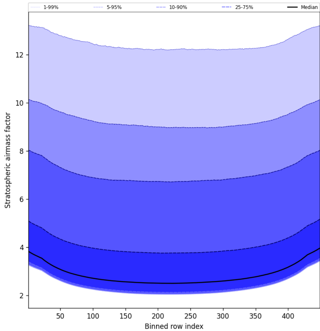
Figure 59: Along track statistics of “Stratospheric airmass factor” for 2025-03-04 to 2025-03-04
