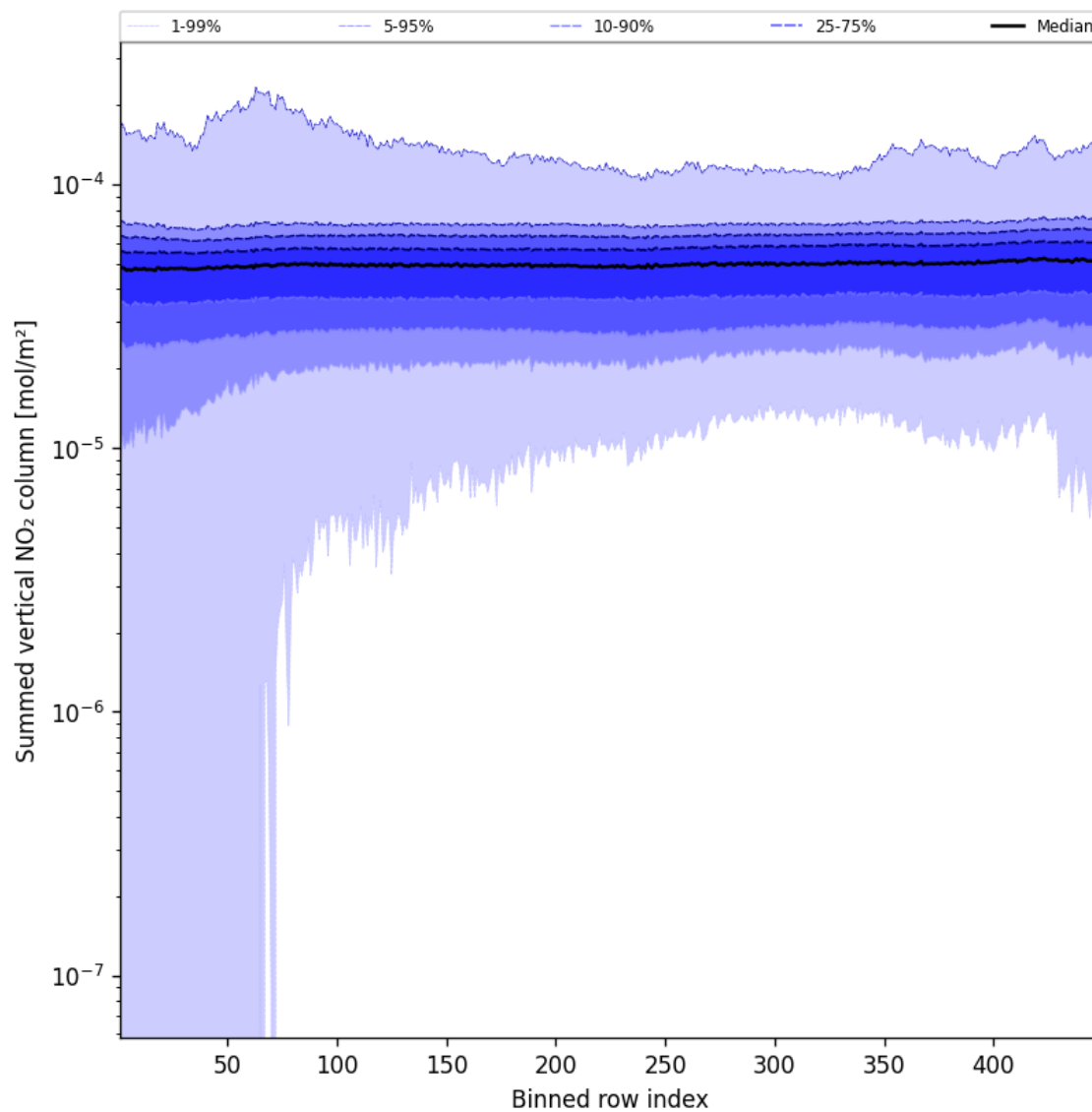
Figure 55: Along track statistics of “Summed vertical NO 2 column” for 2025-03-04 to 2025-03-04
