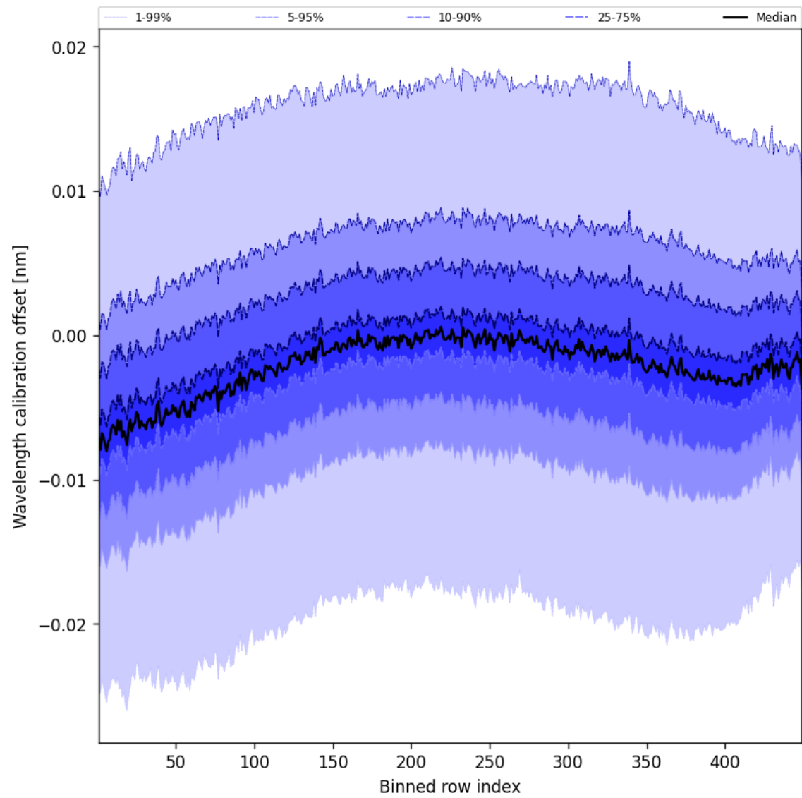
Figure 50: Along track statistics of “Wavelength calibration offset” for 2025-03-04 to 2025-03-04
