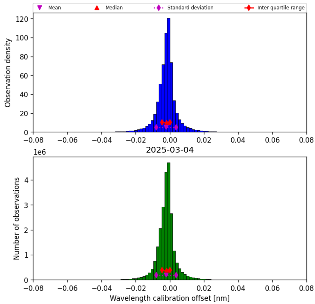
Figure 33: Histogram of “Wavelength calibration offset” for 2025-03-04 to 2025-03-04
