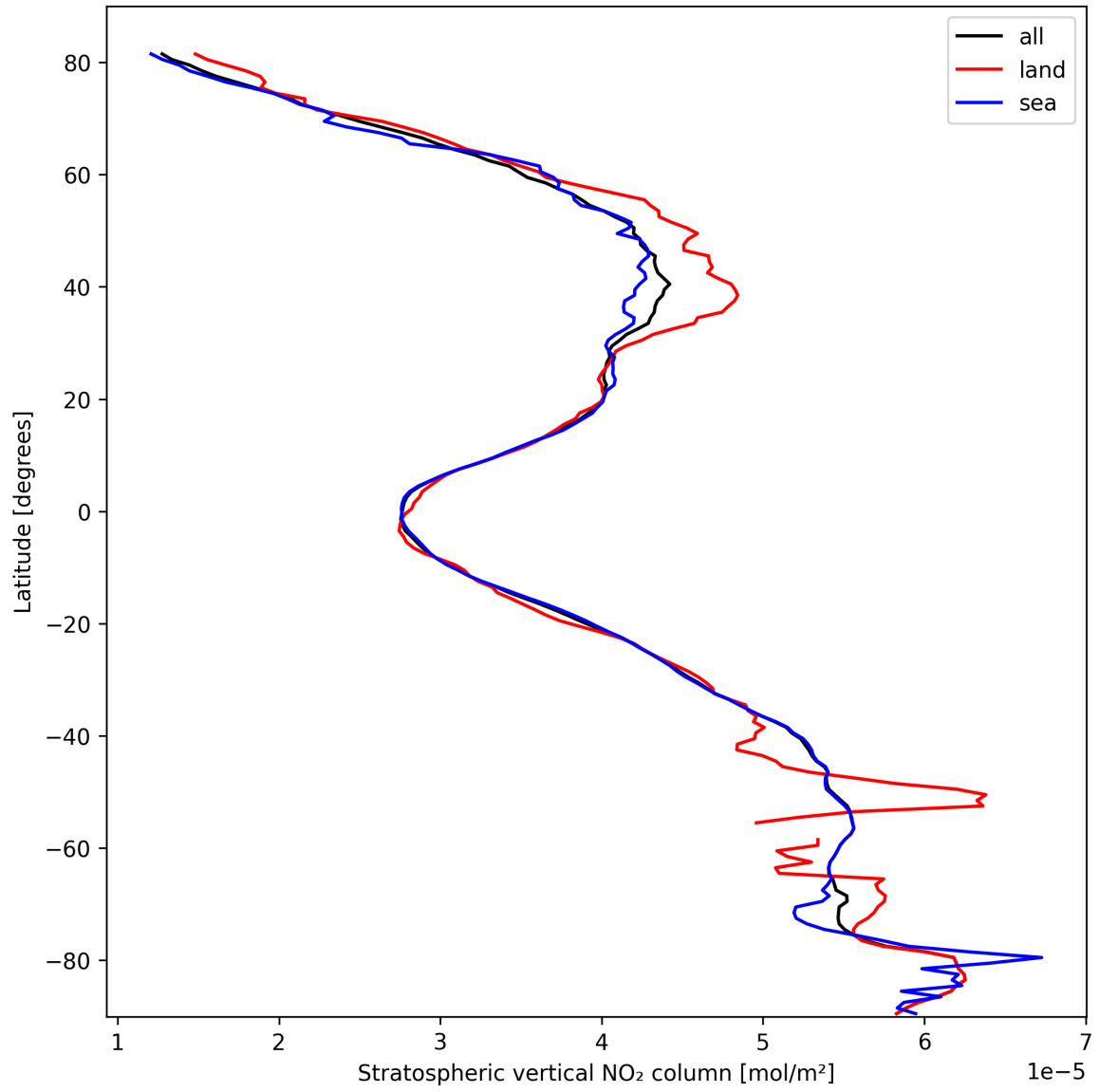
Figure 17: Zonal average of “Stratospheric vertical NO 2 column” for 2025-03-04 to 2025-03-04.
