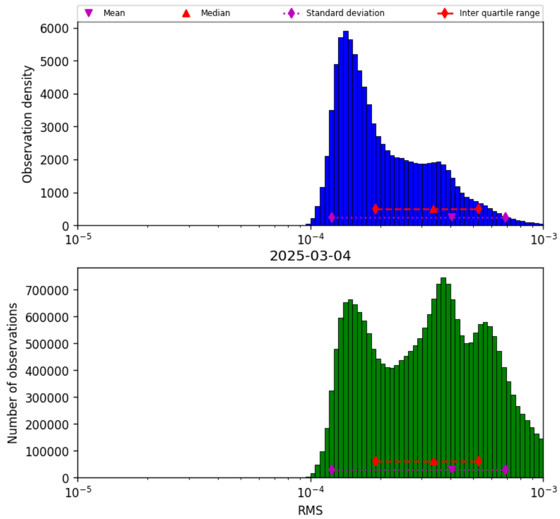
Figure 41: Histogram of “RMS” for 2025-03-04 to 2025-03-04
