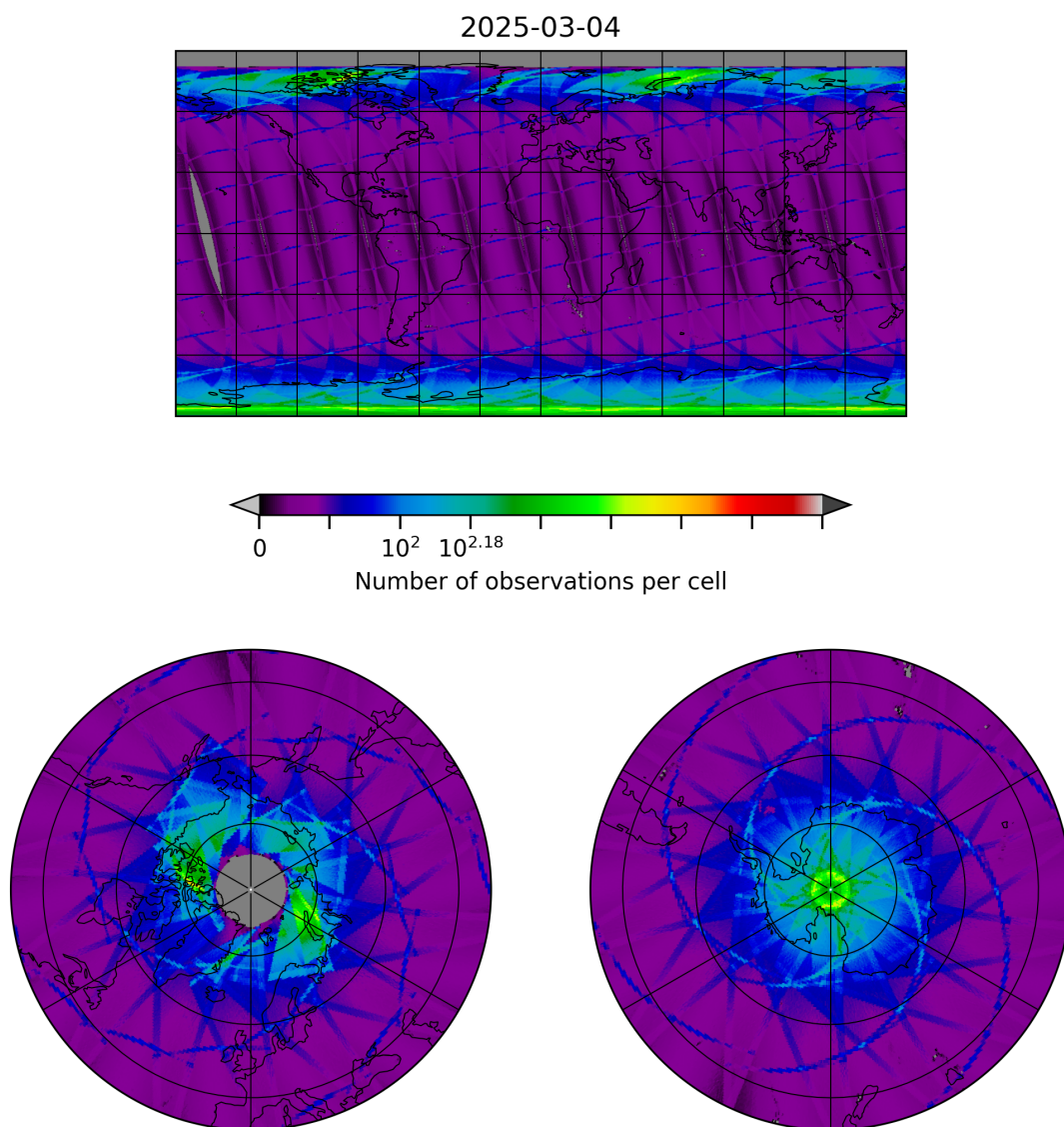
Figure 8: Map of the number of observations for 2025-03-04 to 2025-03-04
