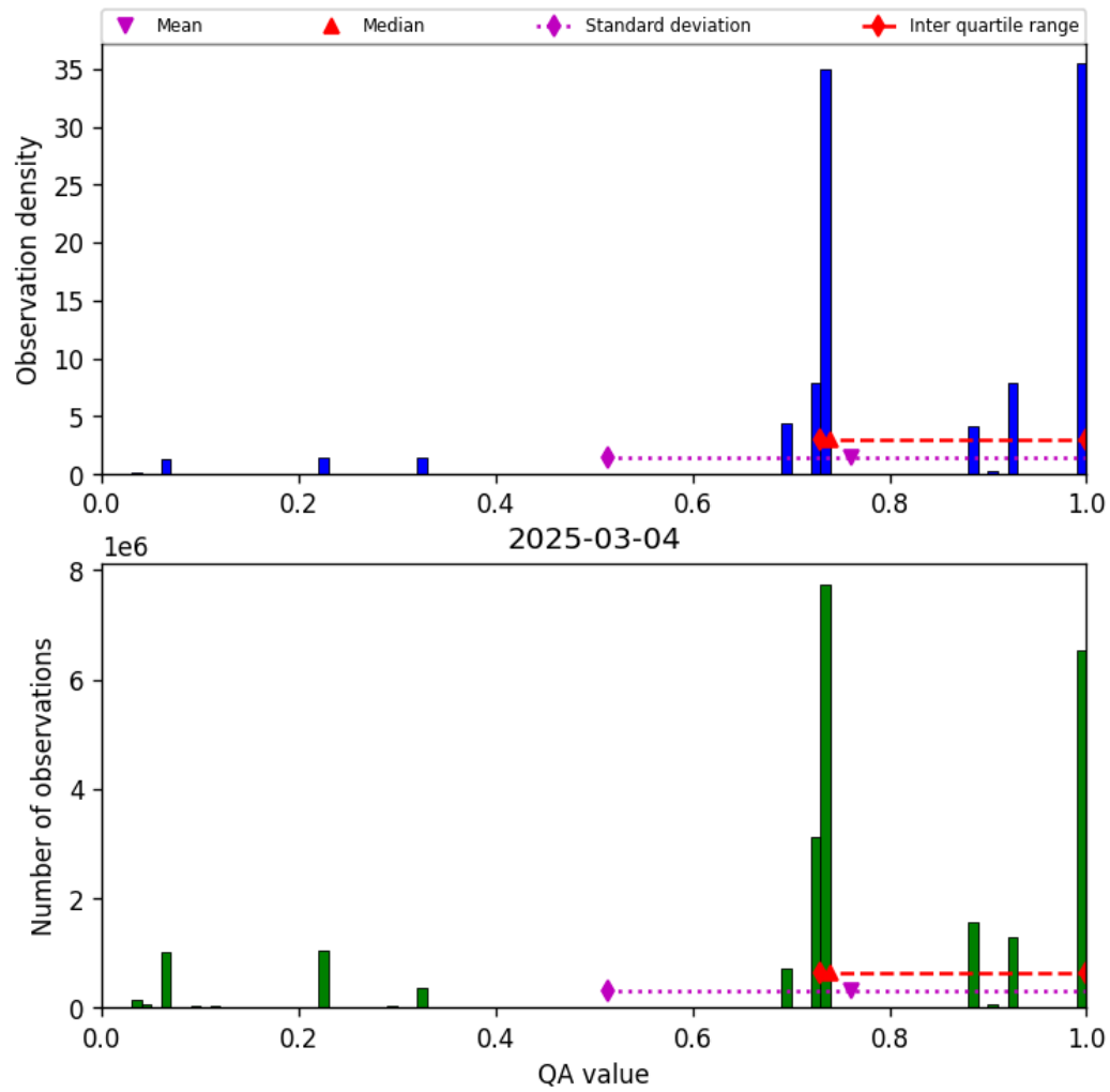
Figure 26: Histogram of “QA value” for 2025-03-04 to 2025-03-04
