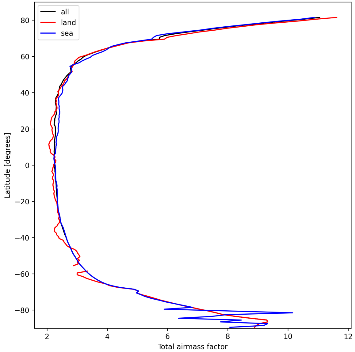
Figure 13: Zonal average of “Total airmass factor” for 2025-03-04 to 2025-03-04.
