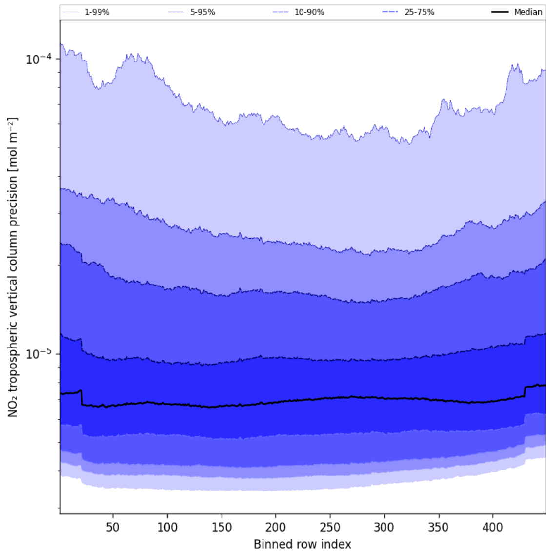
Figure 45: Along track statistics of “NO 2 tropospheric vertical column precision” for 2025-03-04 to 2025-03-04
