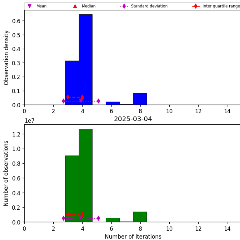
Figure 32: Histogram of “Number of iterations” for 2025-03-04 to 2025-03-04
