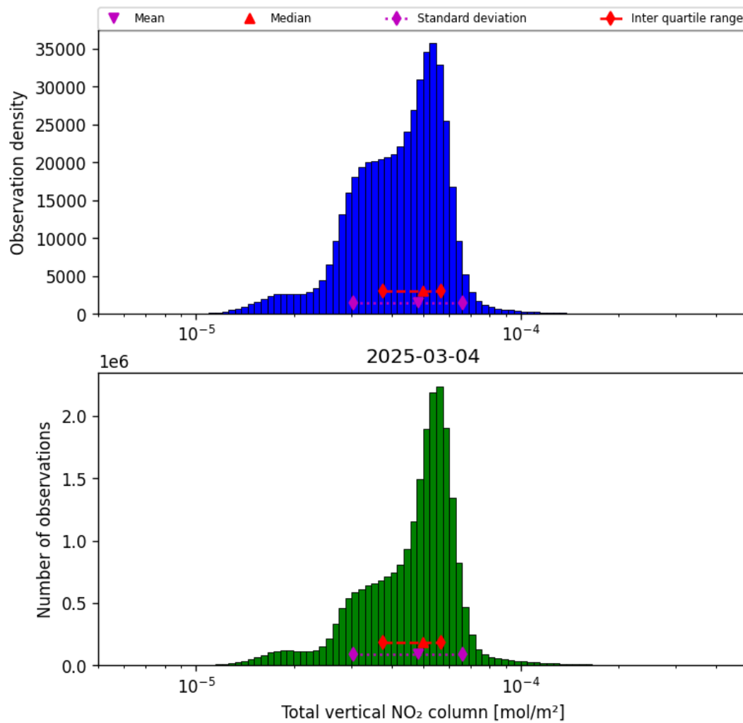
Figure 36: Histogram of “Total vertical NO 2 column” for 2025-03-04 to 2025-03-04
