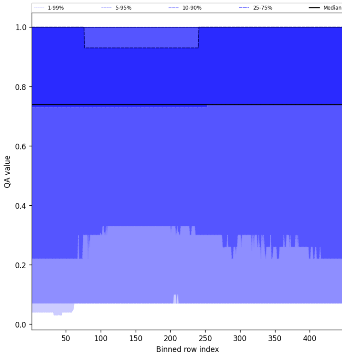
Figure 43: Along track statistics of “QA value” for 2025-03-04 to 2025-03-04
