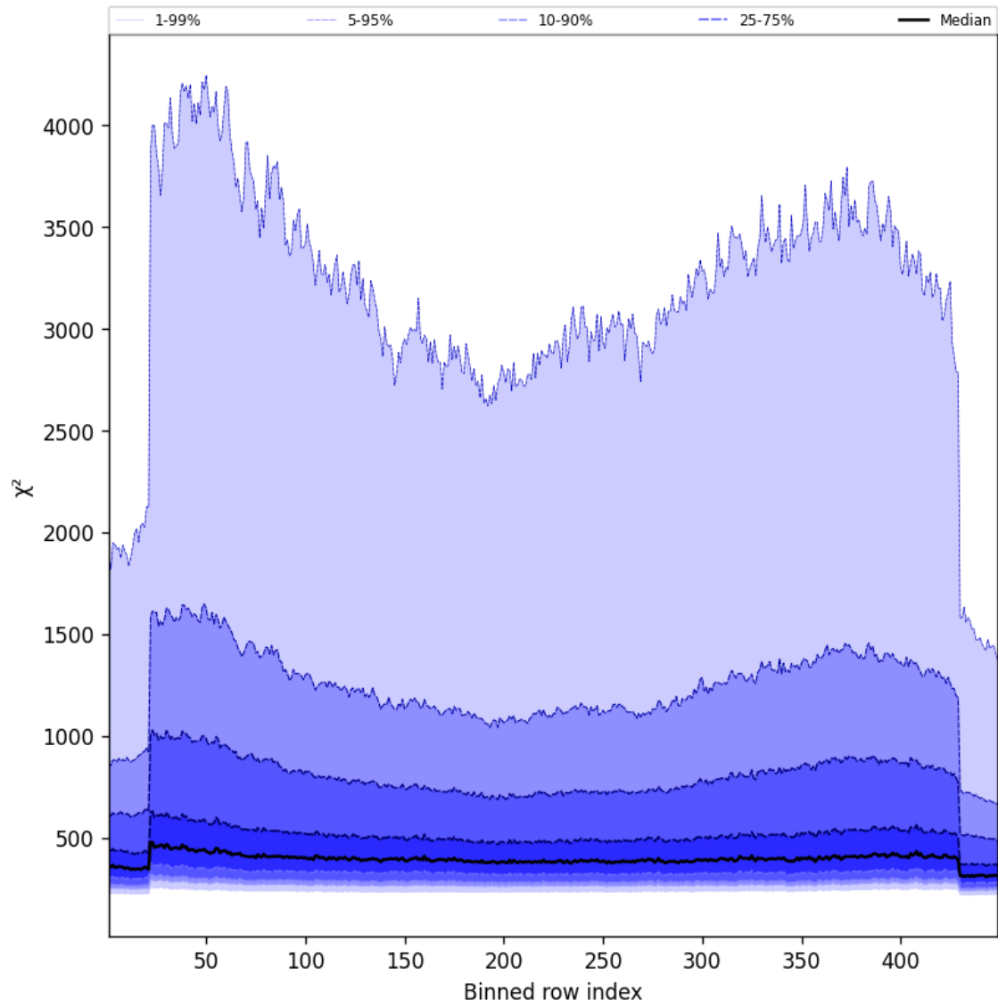
Figure 57: Along track statistics of “ \chi^2 ” for 2025-03-04 to 2025-03-04
