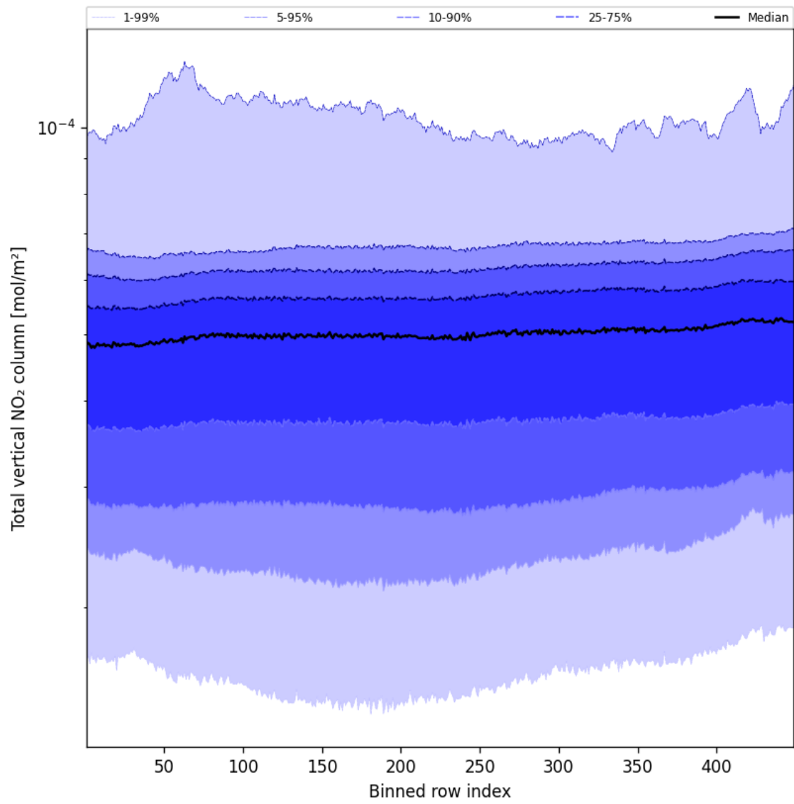
Figure 53: Along track statistics of “Total vertical NO 2 column” for 2025-03-04 to 2025-03-04
