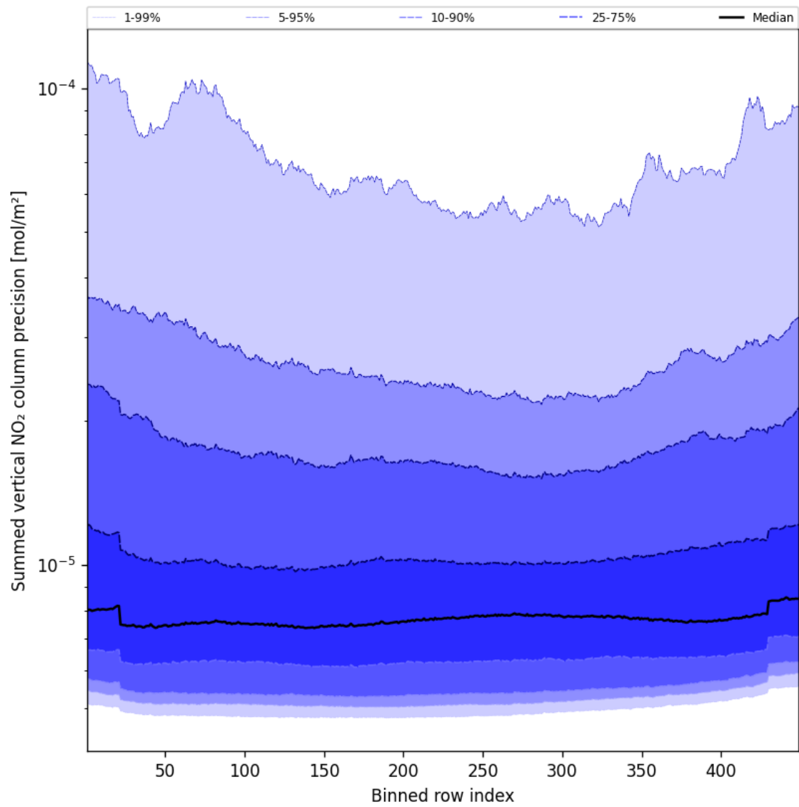
Figure 56: Along track statistics of “Summed vertical NO 2 column precision” for 2025-03-04 to 2025-03-04
