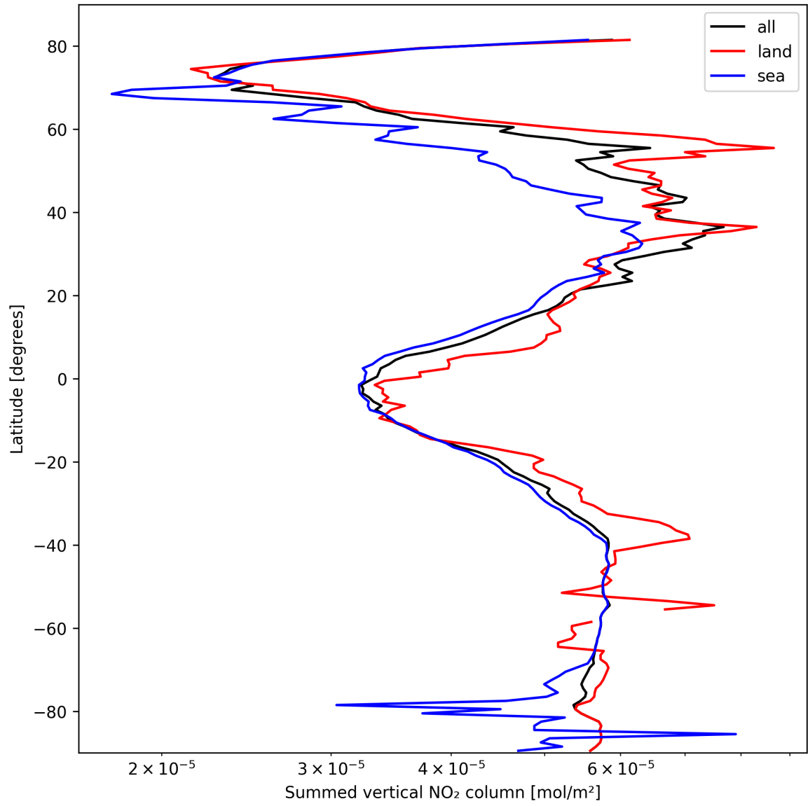
Figure 21: Zonal average of “Summed vertical NO 2 column” for 2025-03-04 to 2025-03-04.
