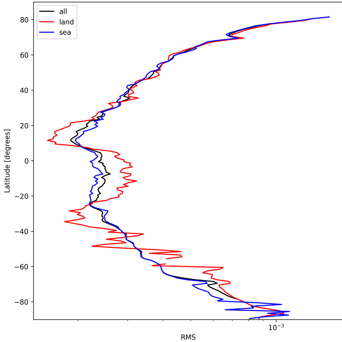
Figure 24: Zonal average of “RMS” for 2025-03-04 to 2025-03-04.
