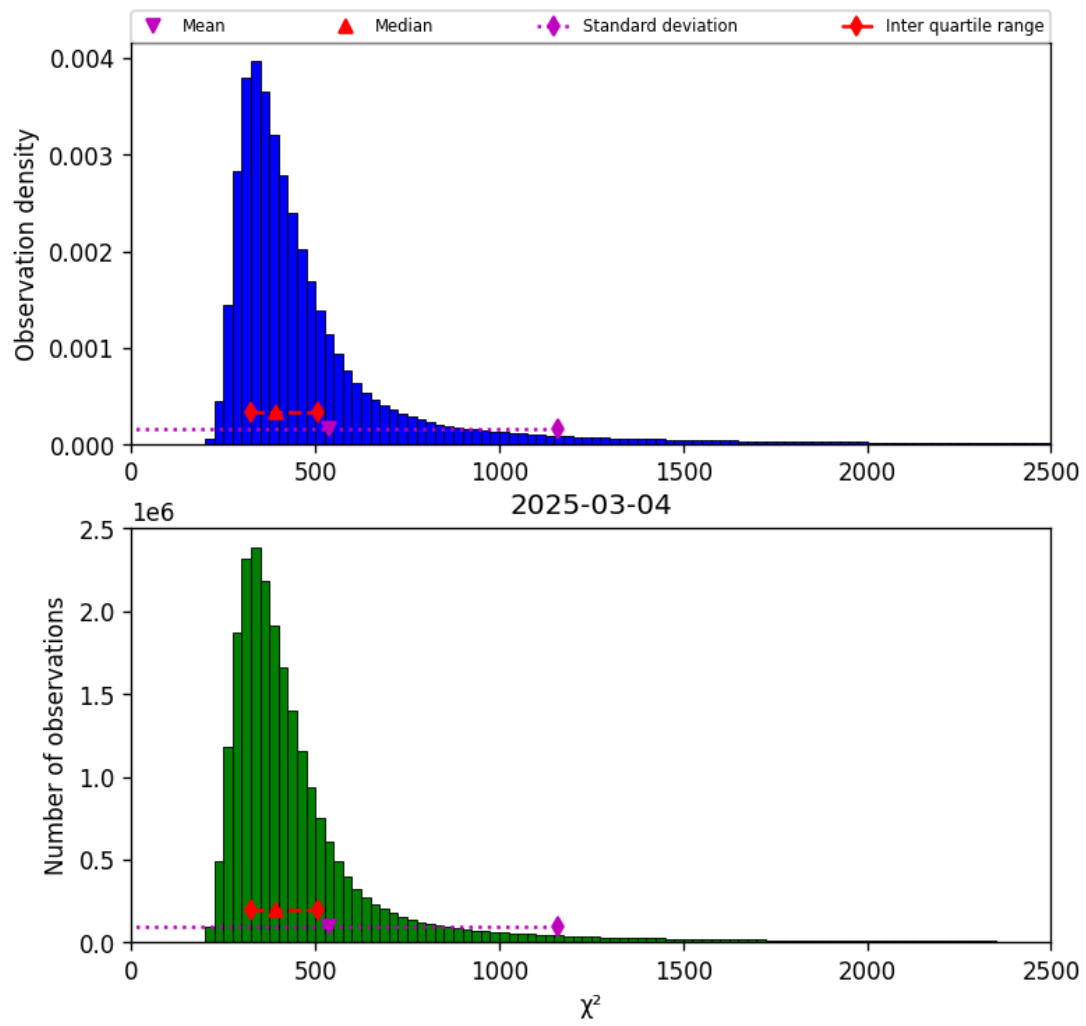
Figure 40: Histogram of “ \chi^2 ” for 2025-03-04 to 2025-03-04
