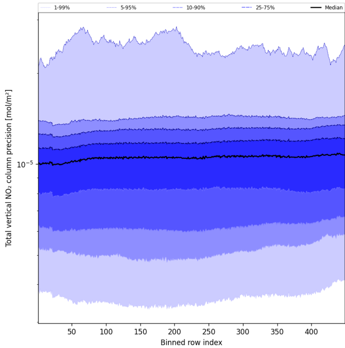
Figure 54: Along track statistics of “Total vertical NO 2 column precision” for 2025-03-04 to 2025-03-04
