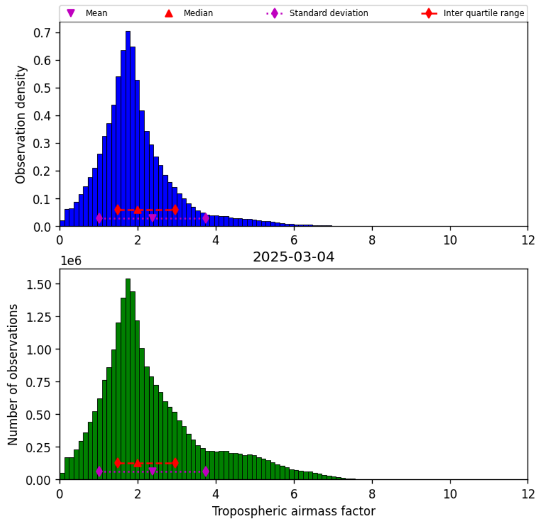
Figure 29: Histogram of “Tropospheric airmass factor” for 2025-03-04 to 2025-03-04
