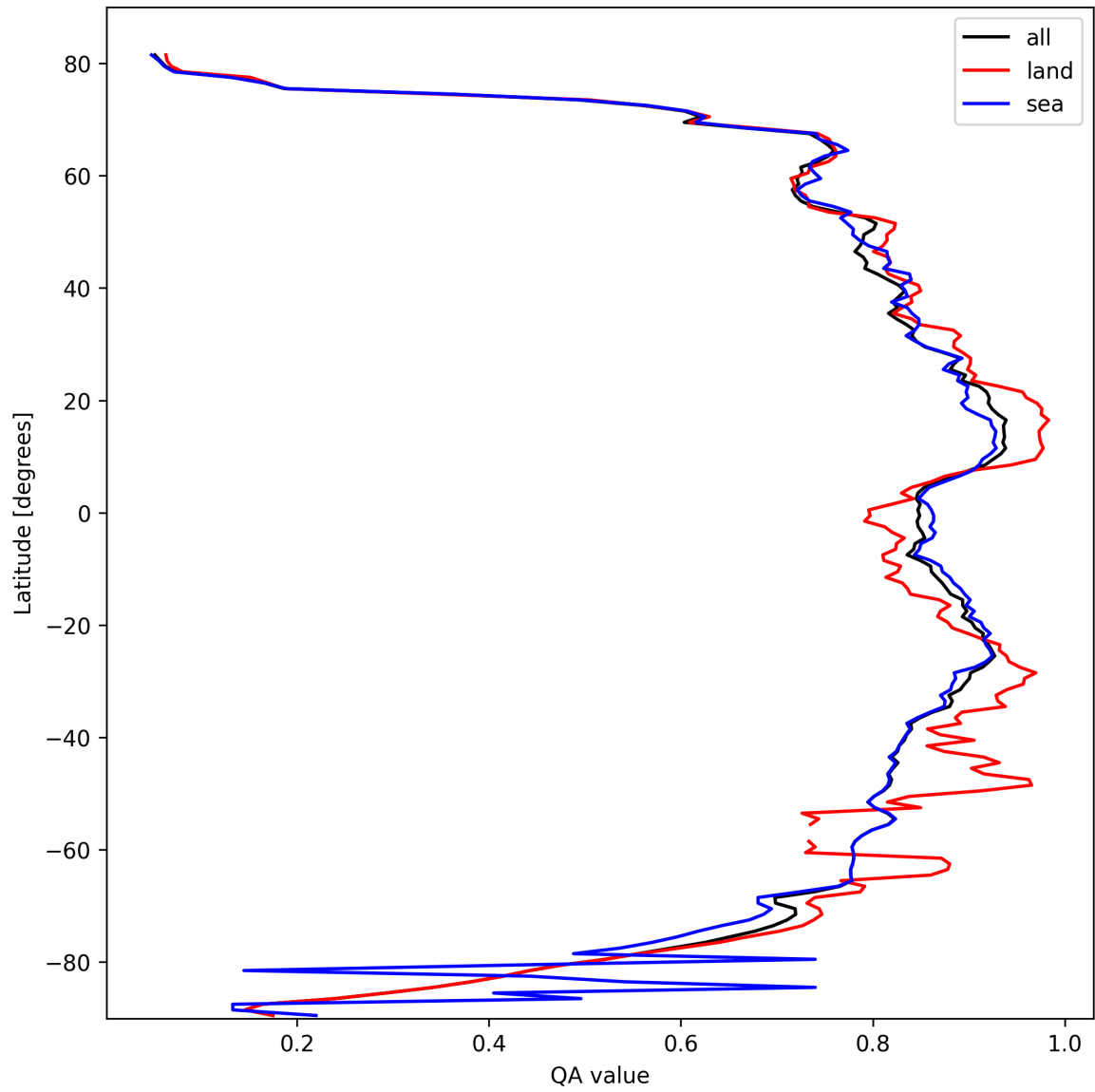
Figure 9: Zonal average of “QA value” for 2025-03-04 to 2025-03-04.
