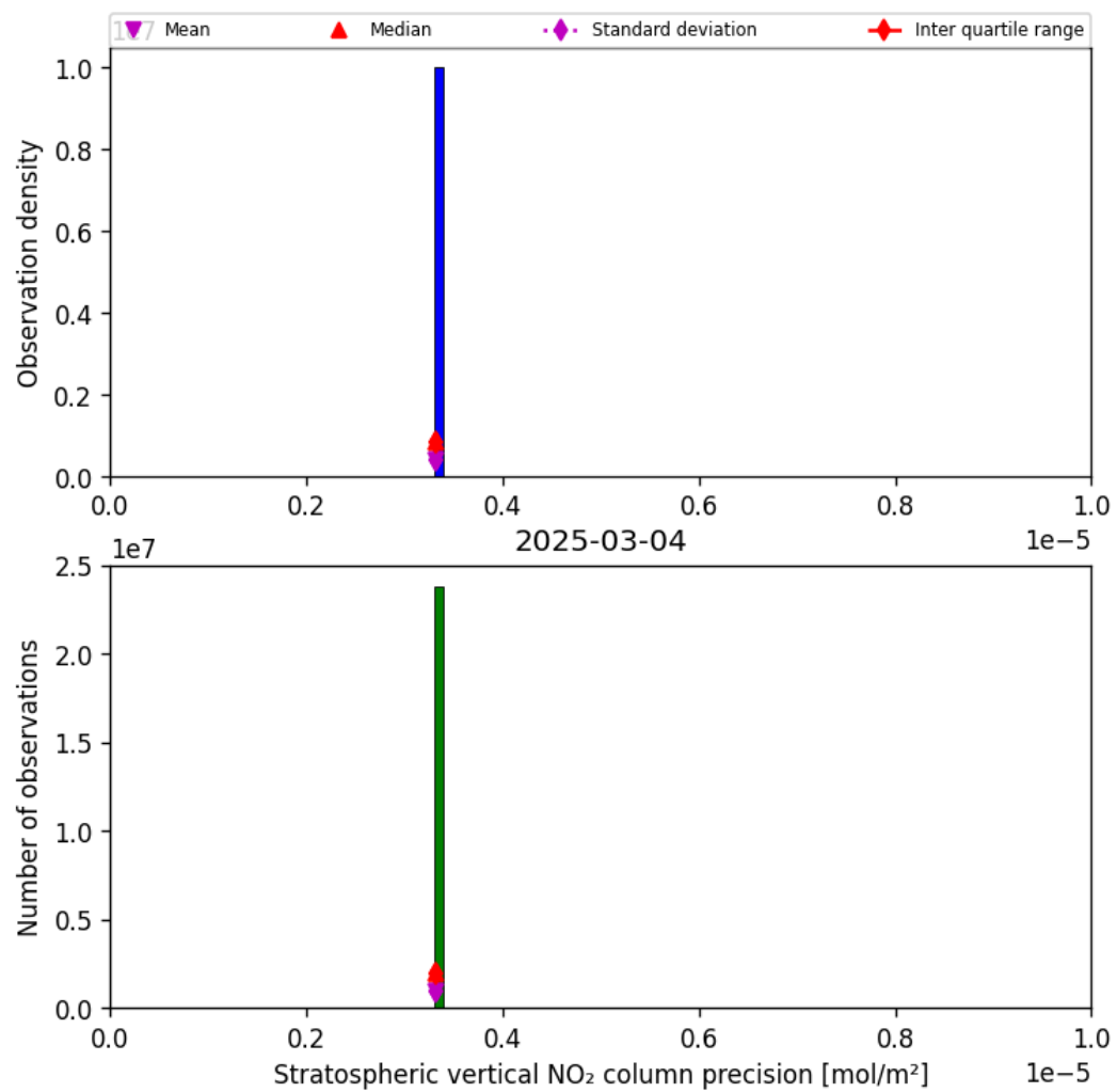
Figure 35: Histogram of “Stratospheric vertical NO 2 column precision” for 2025-03-04 to 2025-03-04
