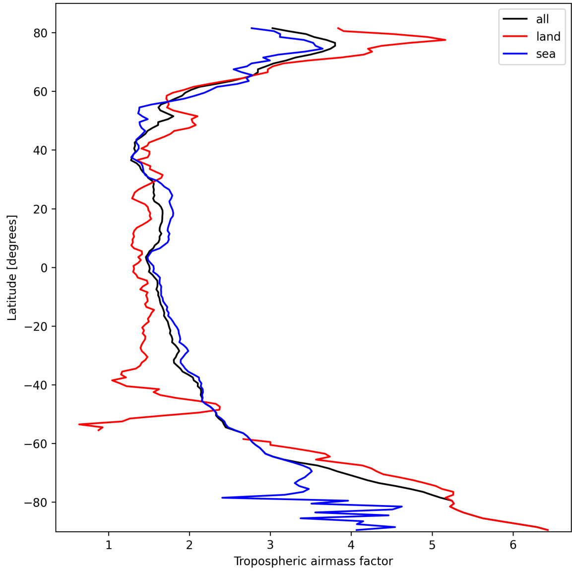
Figure 12: Zonal average of “Tropospheric air mass factor” for 2025-03-04 to 2025-03-04.
