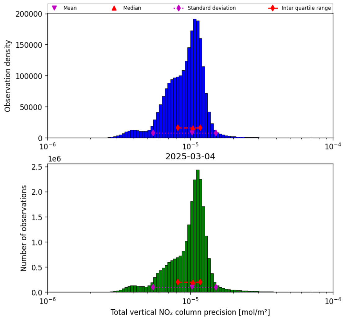
Figure 37: Histogram of “Total vertical NO 2 column precision” for 2025-03-04 to 2025-03-04
