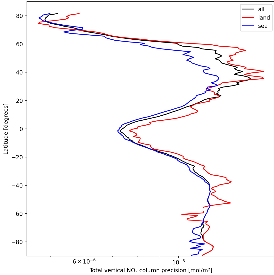
Figure 20: Zonal average of “Total vertical NO 2 column precision” for 2025-03-04 to 2025-03-04.
