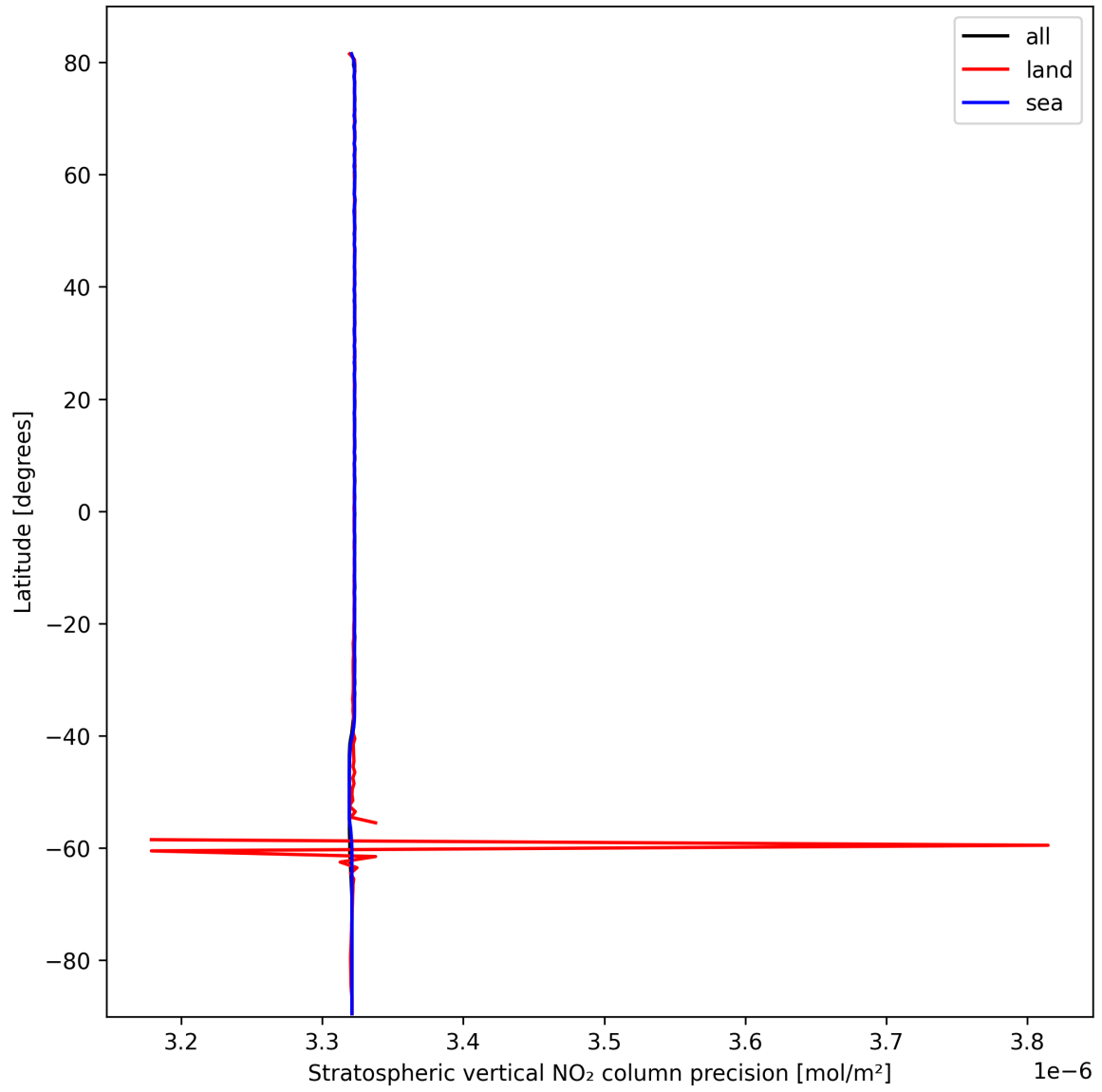
Figure 18: Zonal average of “Stratospheric vertical NO 2 column precision” for 2025-03-04 to 2025-03-04.
