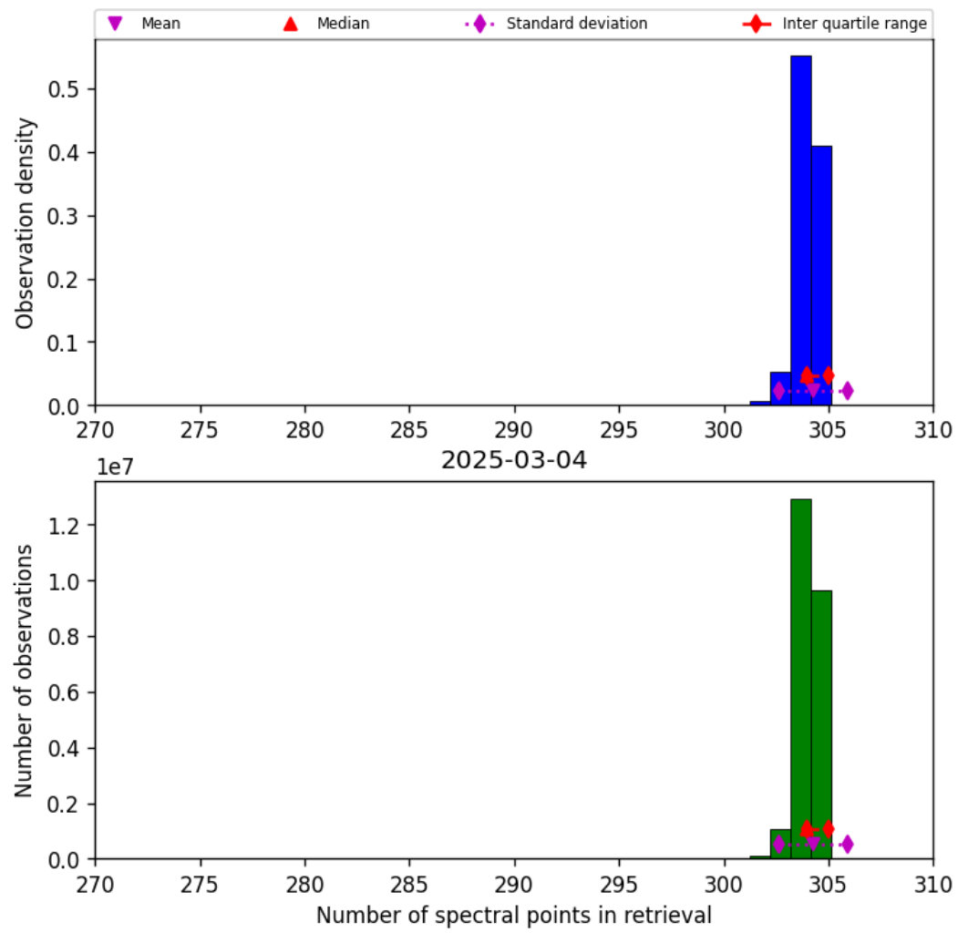
Figure 31: Histogram of “Number of spectral points in retrieval” for 2025-03-04 to 2025-03-04
