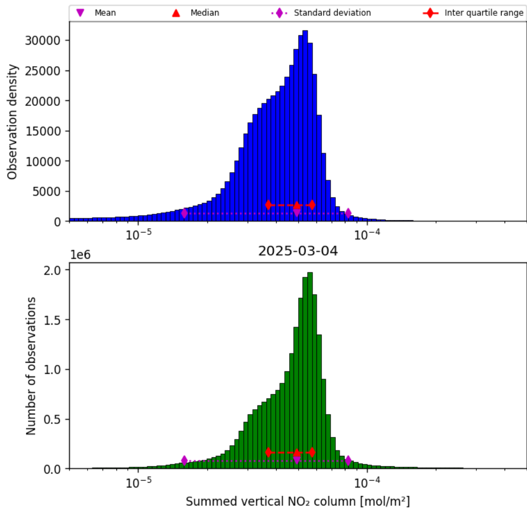
Figure 38: Histogram of “Summed vertical NO 2 column” for 2025-03-04 to 2025-03-04
