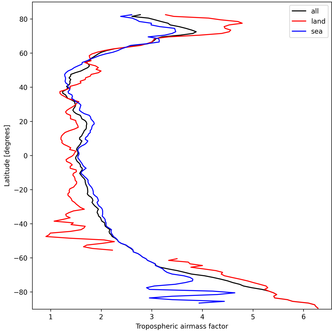
Figure 12: Zonal average of “Tropospheric airmass factor” for 2025-03-05 to 2025-03-05.
