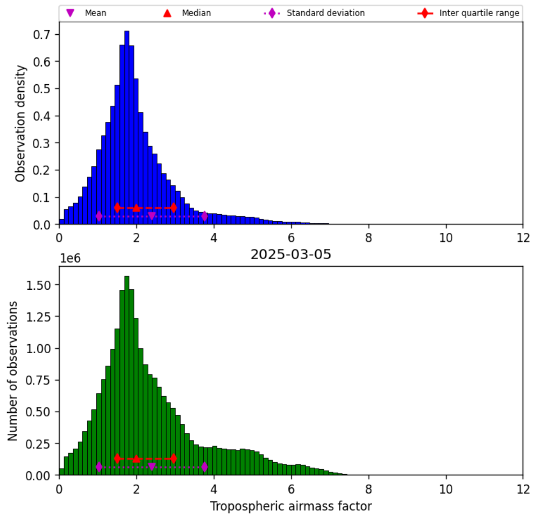
Figure 29: Histogram of “Tropospheric airmass factor” for 2025-03-05 to 2025-03-05
