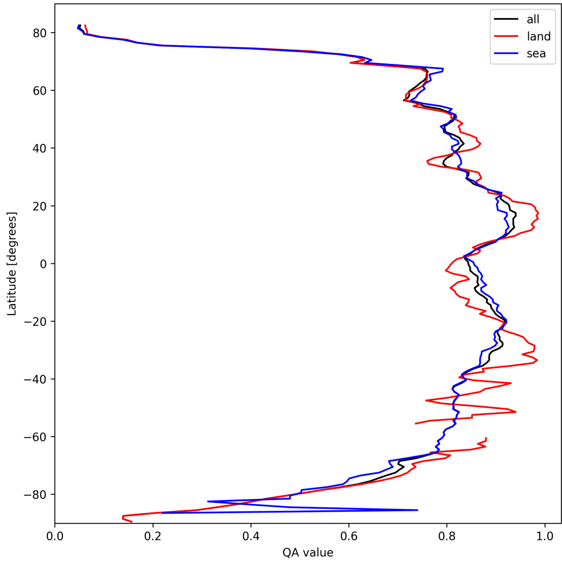
Figure 9: Zonal average of “QA value” for 2025-03-05 to 2025-03-05.
