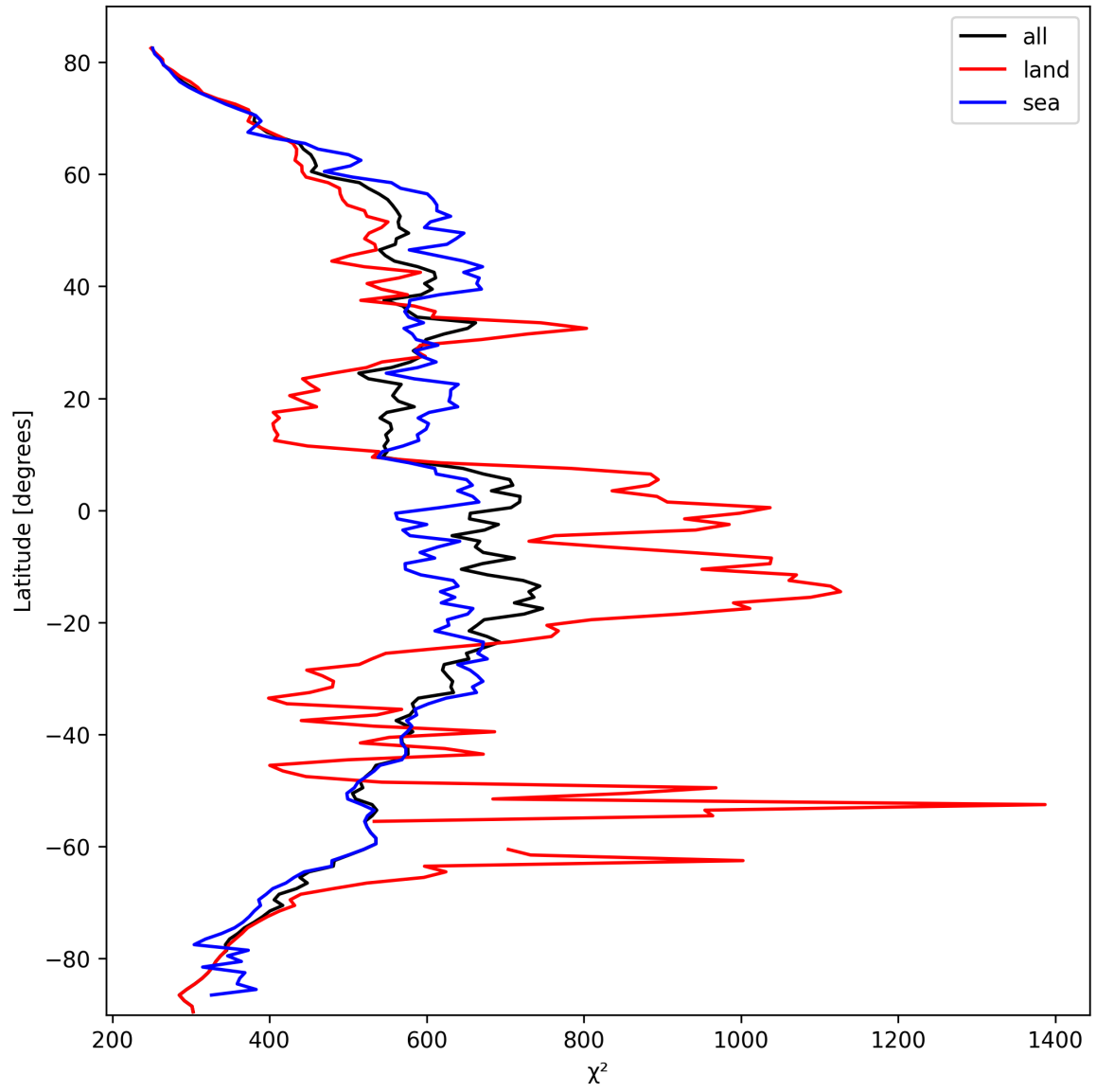
Figure 23: Zonal average of “ \chi^2 ” for 2025-03-05 to 2025-03-05.
