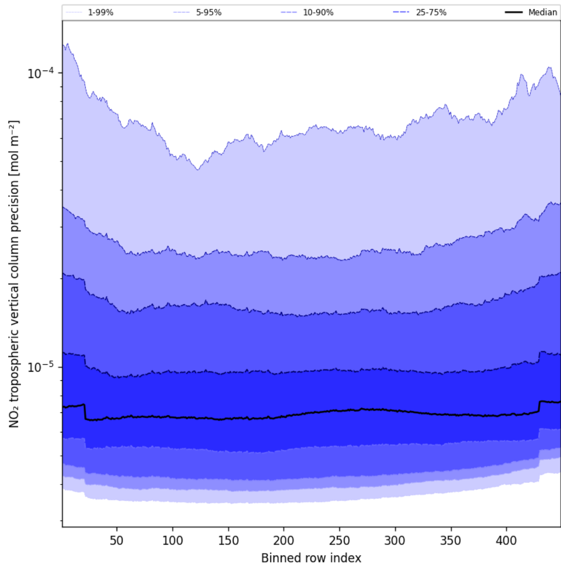
Figure 45: Along track statistics of “NO 2 tropospheric vertical column precision” for 2025-03-05 to 2025-03-05
