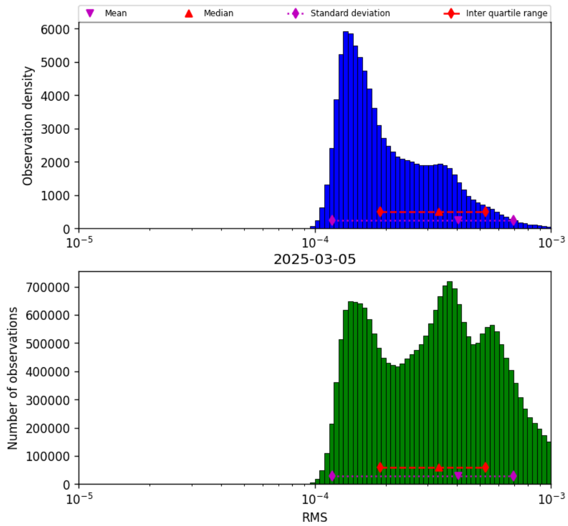
Figure 41: Histogram of “RMS” for 2025-03-05 to 2025-03-05
