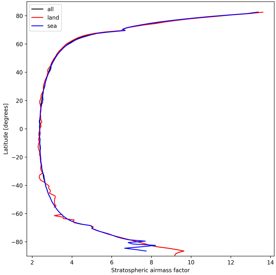
Figure 25: Zonal average of “Stratospheric airmass factor” for 2025-03-05 to 2025-03-05.
