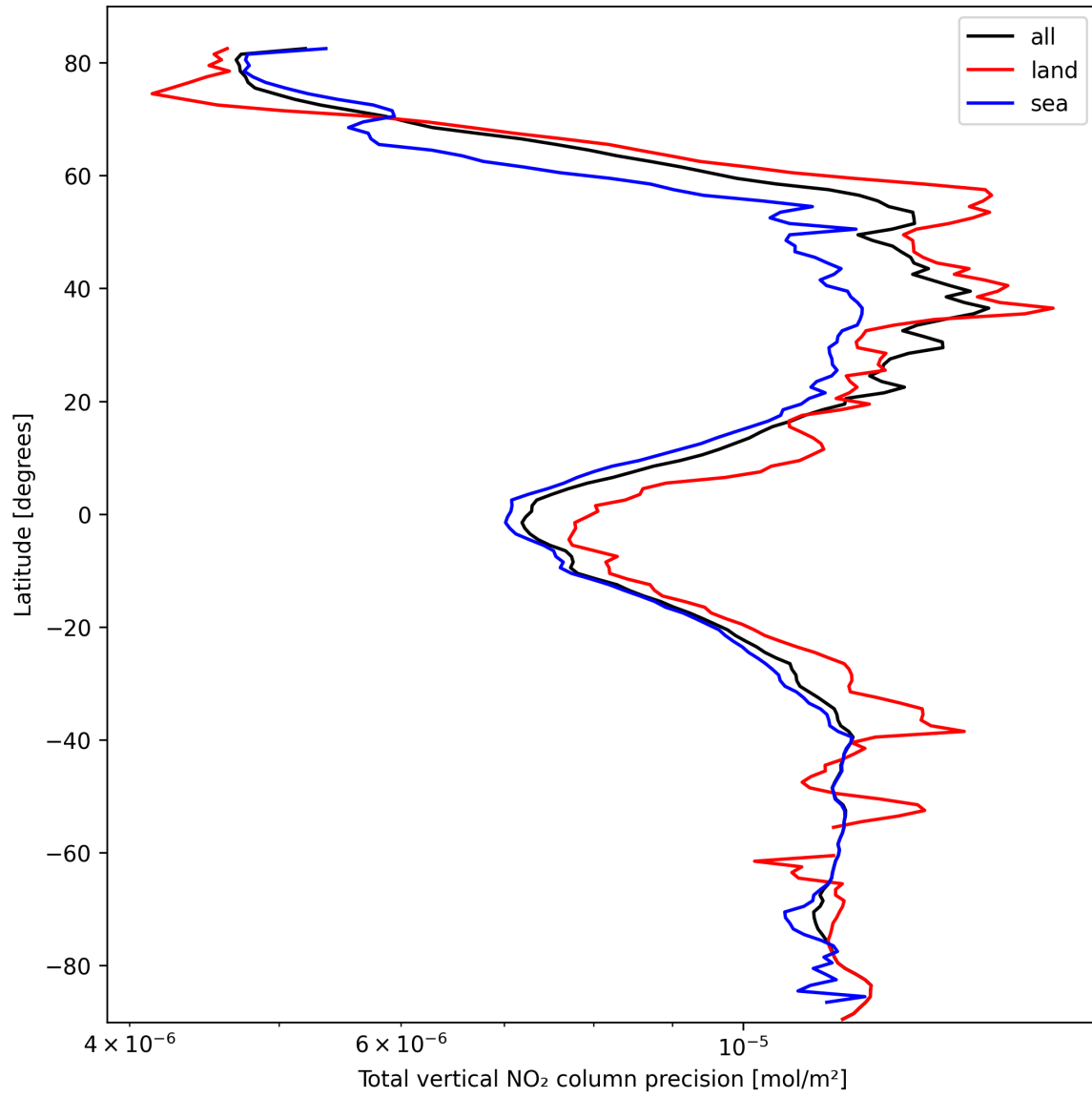
Figure 20: Zonal average of “Total vertical NO 2 column precision” for 2025-03-05 to 2025-03-05.
