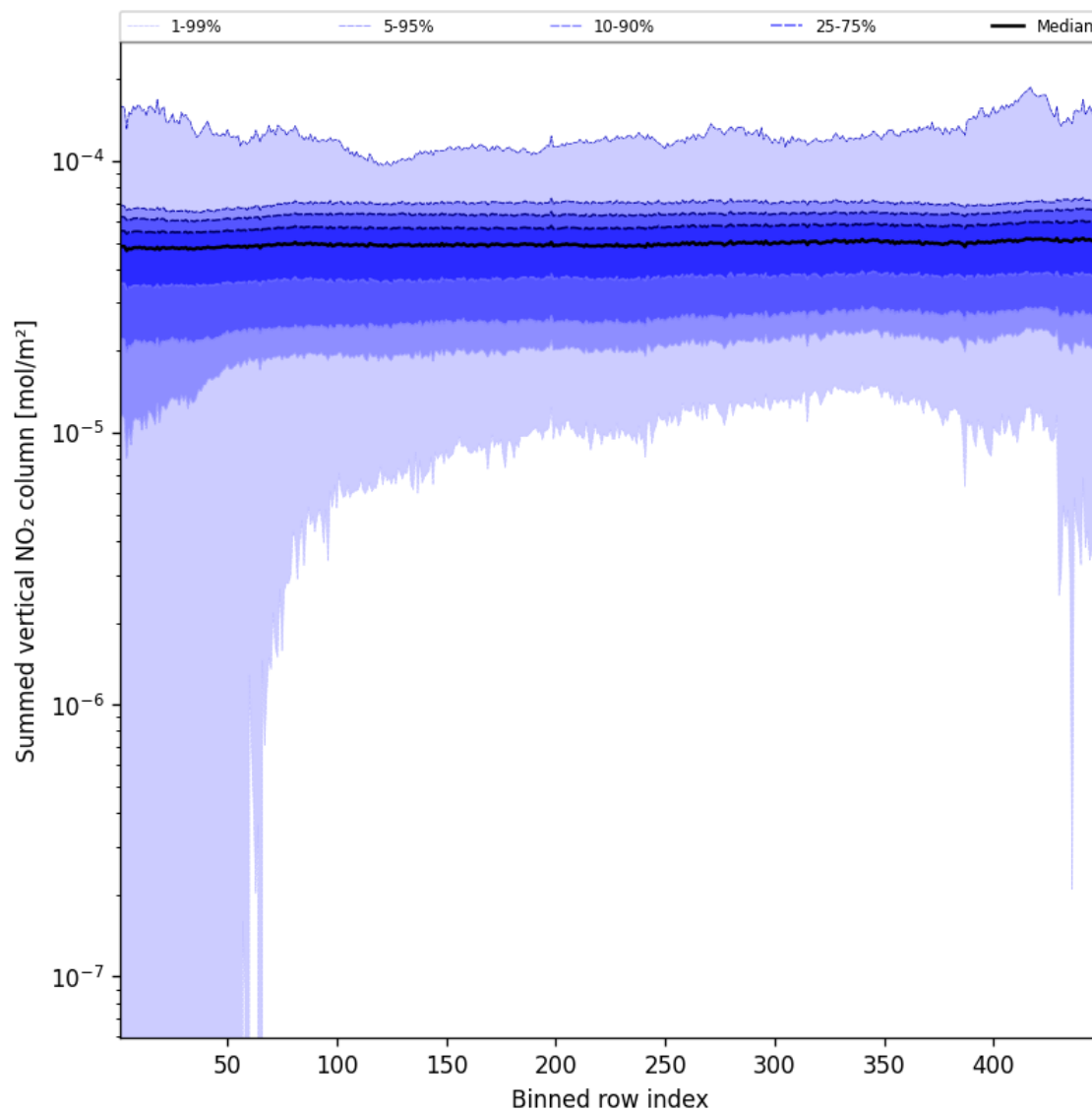
Figure 55: Along track statistics of “Summed vertical NO 2 column” for 2025-03-05 to 2025-03-05
