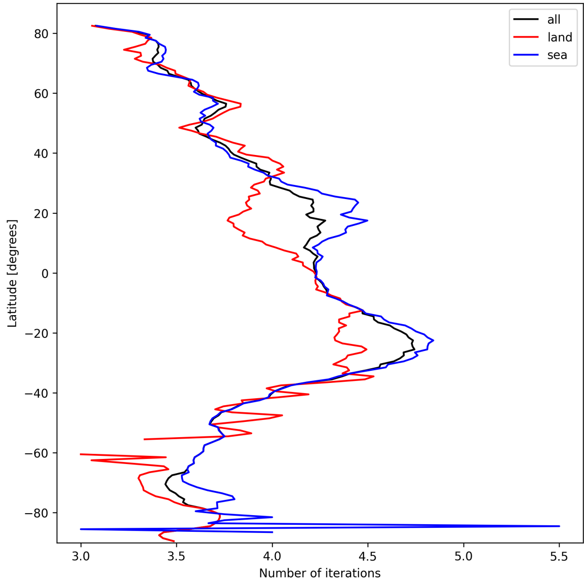
Figure 15: Zonal average of “Number of iterations” for 2025-03-05 to 2025-03-05.
