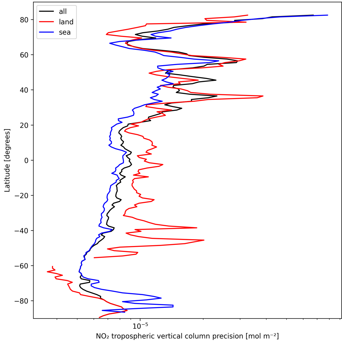
Figure 11: Zonal average of "NO 2 tropospheric vertical column precision" for 2025-03-05 to 2025-03-05.
