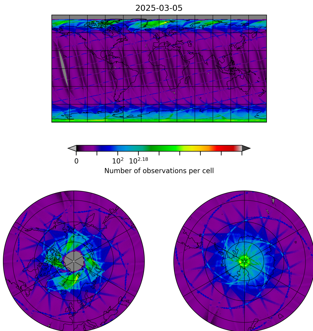
Figure 8: Map of the number of observations for 2025-03-05 to 2025-03-05
