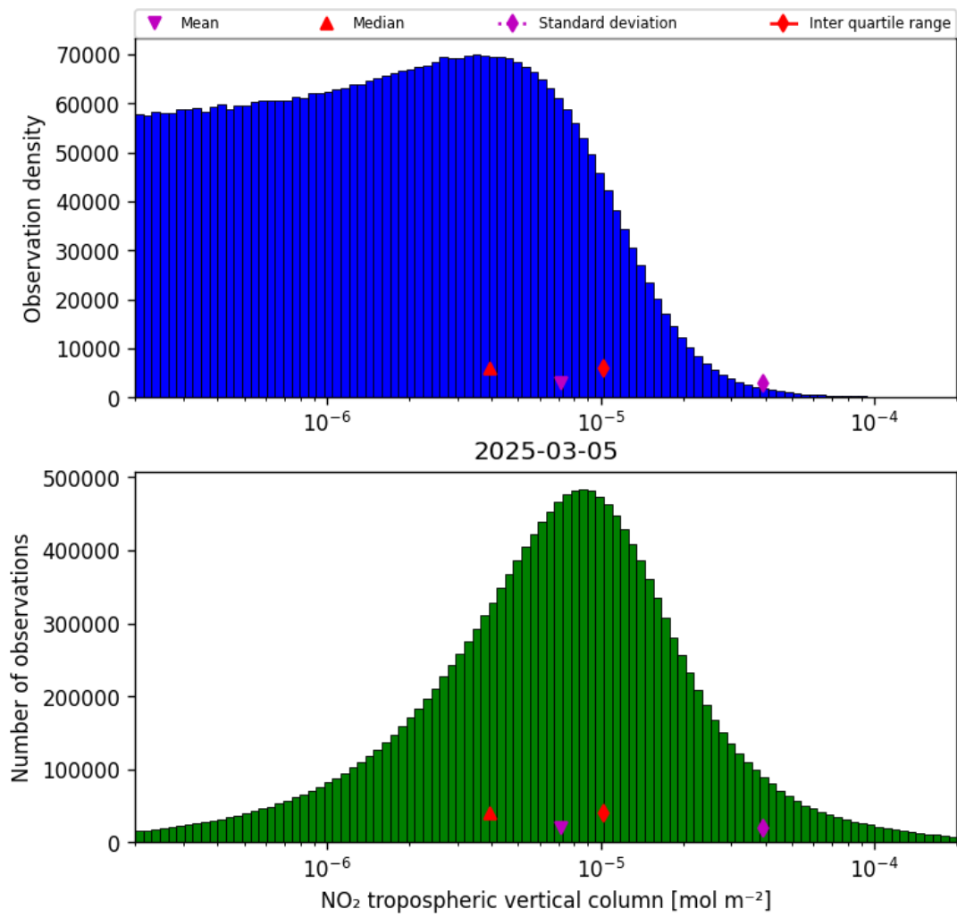
Figure 27: Histogram of “NO 2 tropospheric vertical column” for 2025-03-05 to 2025-03-05
