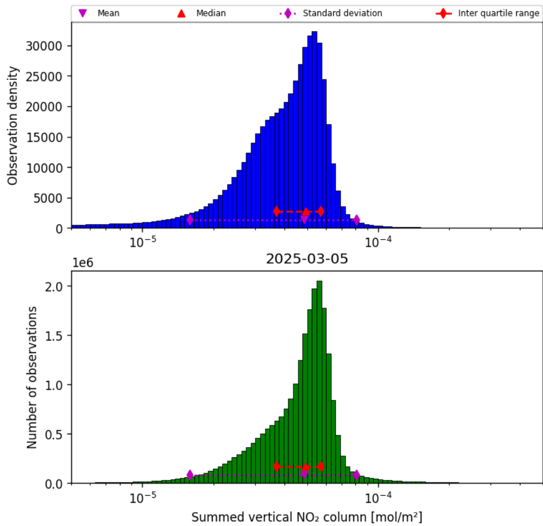
Figure 38: Histogram of “Summed vertical NO 2 column” for 2025-03-05 to 2025-03-05
