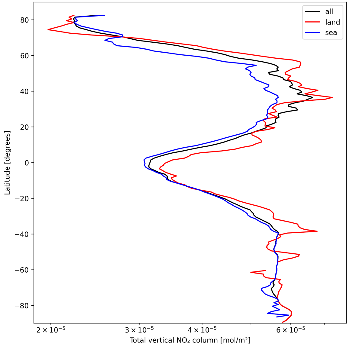
Figure 19: Zonal average of “Total vertical NO 2 column” for 2025-03-05 to 2025-03-05.
