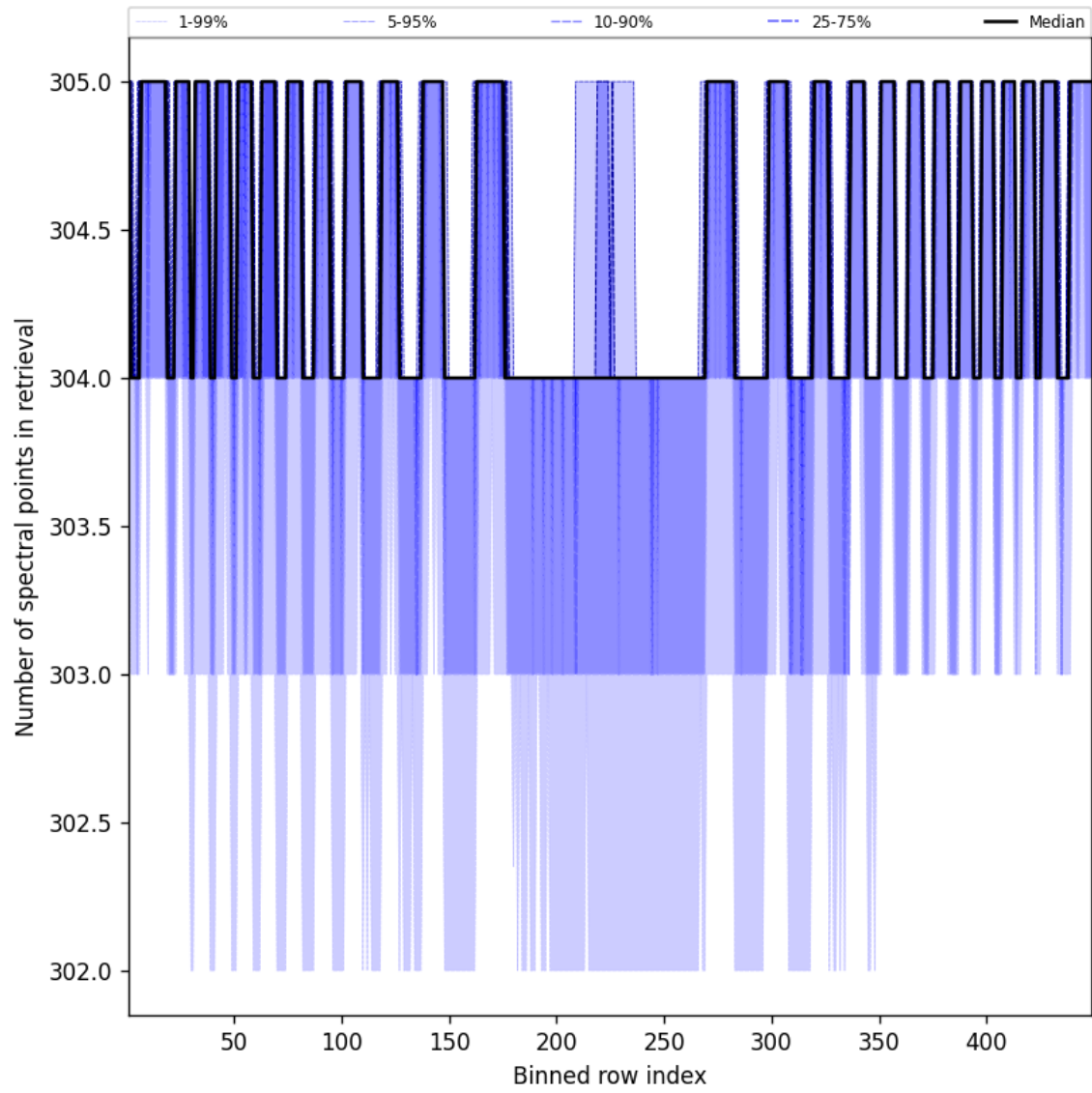
Figure 48: Along track statistics of “Number of spectral points in retrieval” for 2025-03-05 to 2025-03-05
