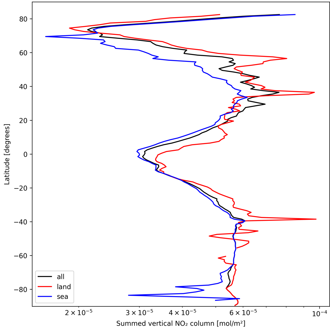
Figure 21: Zonal average of “Summed vertical NO 2 column” for 2025-03-05 to 2025-03-05.
