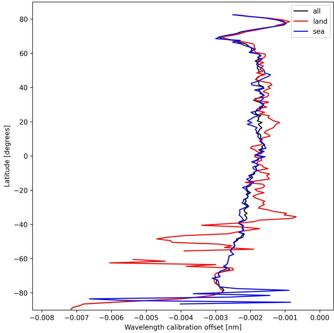
Figure 16: Zonal average of “Wavelength calibration offset” for 2025-03-05 to 2025-03-05.
