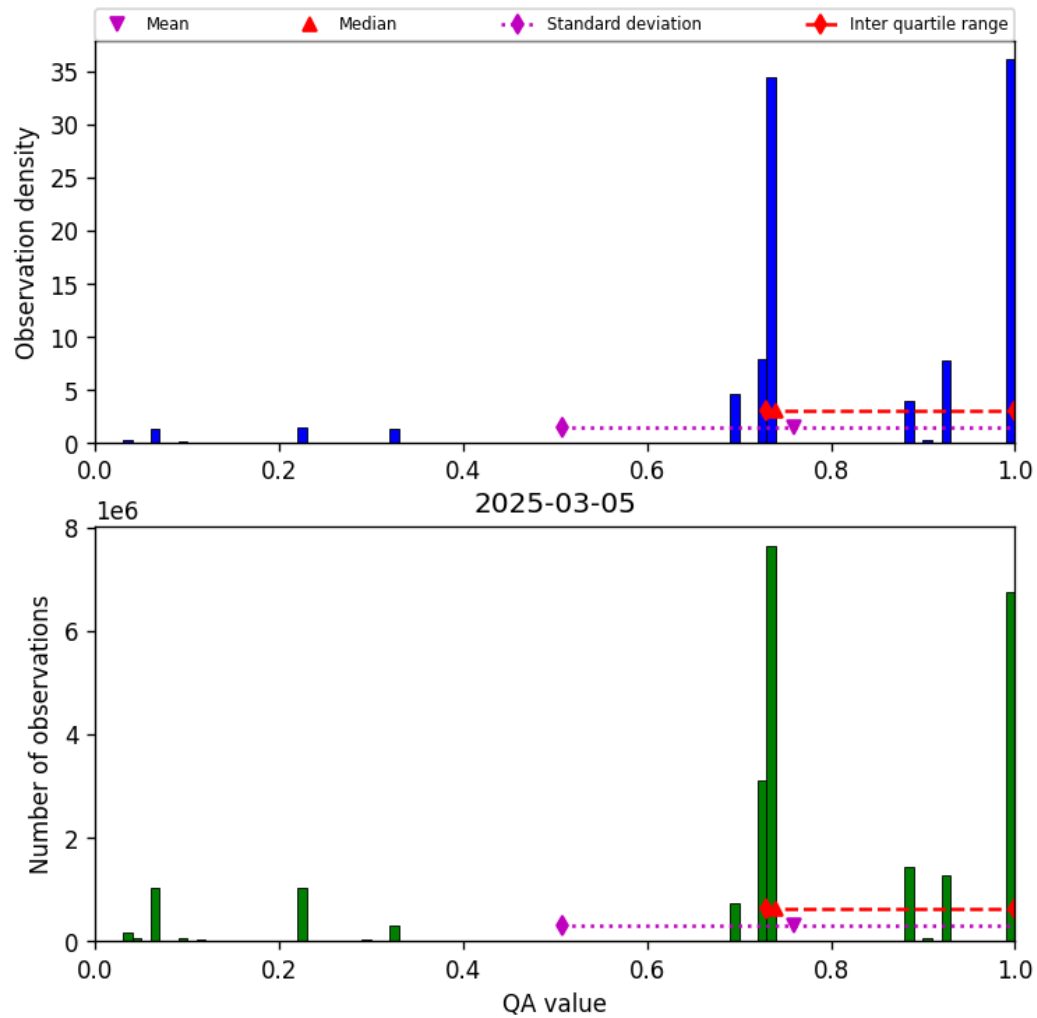
Figure 26: Histogram of “QA value” for 2025-03-05 to 2025-03-05
