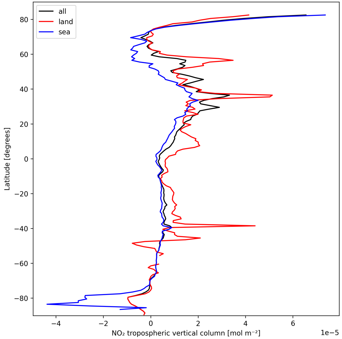
Figure 10: Zonal average of “NO 2 tropospheric vertical column” for 2025-03-05 to 2025-03-05.
