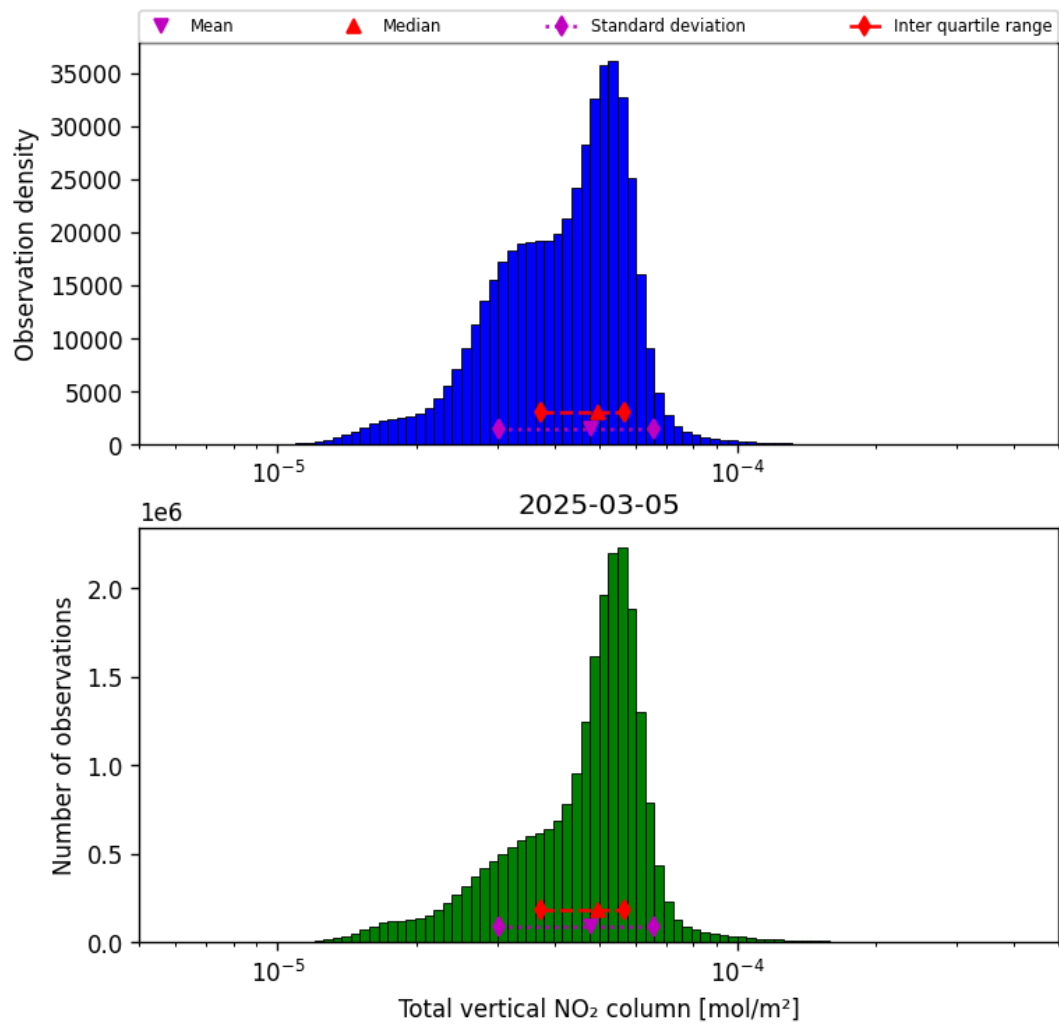
Figure 36: Histogram of “Total vertical NO 2 column” for 2025-03-05 to 2025-03-05
