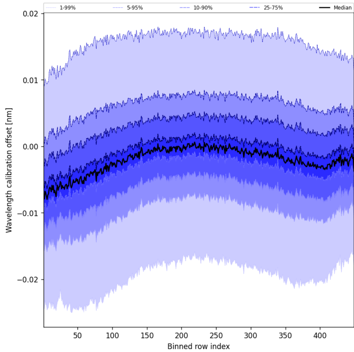
Figure 50: Along track statistics of “Wavelength calibration offset” for 2025-03-05 to 2025-03-05
