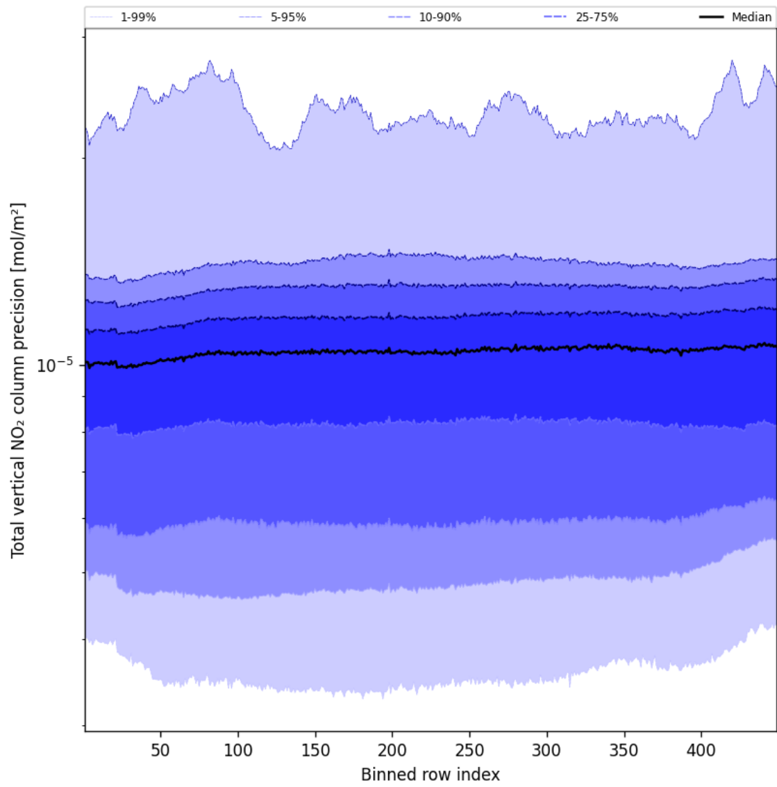
Figure 54: Along track statistics of “Total vertical NO 2 column precision” for 2025-03-05 to 2025-03-05
