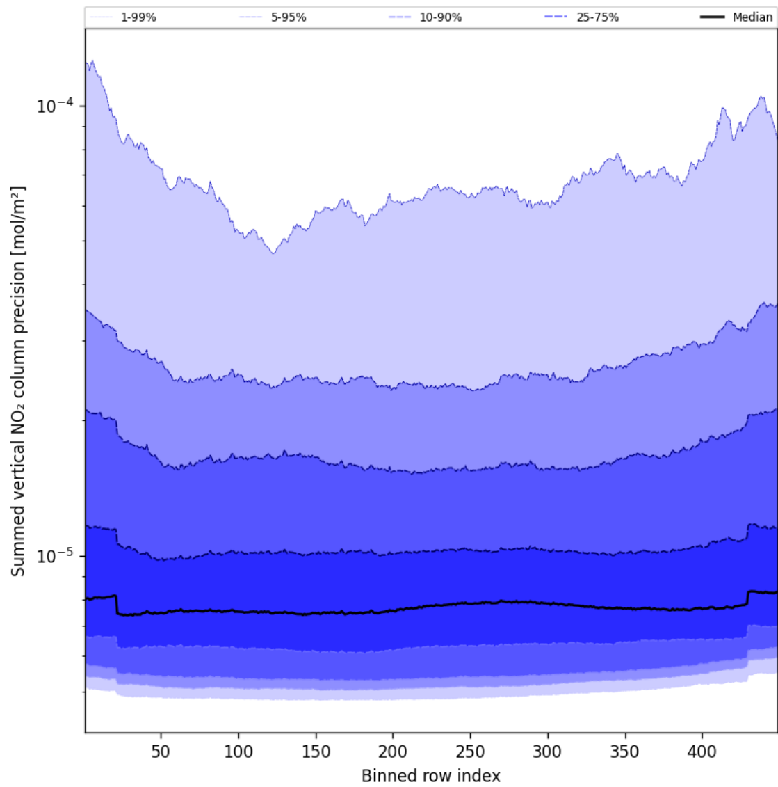
Figure 56: Along track statistics of “Summed vertical NO 2 column precision” for 2025-03-05 to 2025-03-05
