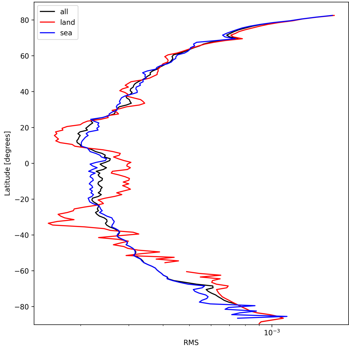
Figure 24: Zonal average of “RMS” for 2025-03-05 to 2025-03-05.
