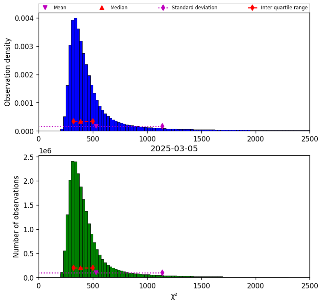
Figure 40: Histogram of “ \chi^2 ” for 2025-03-05 to 2025-03-05
