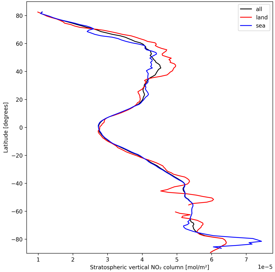
Figure 17: Zonal average of “Stratospheric vertical NO 2 column” for 2025-03-05 to 2025-03-05.
