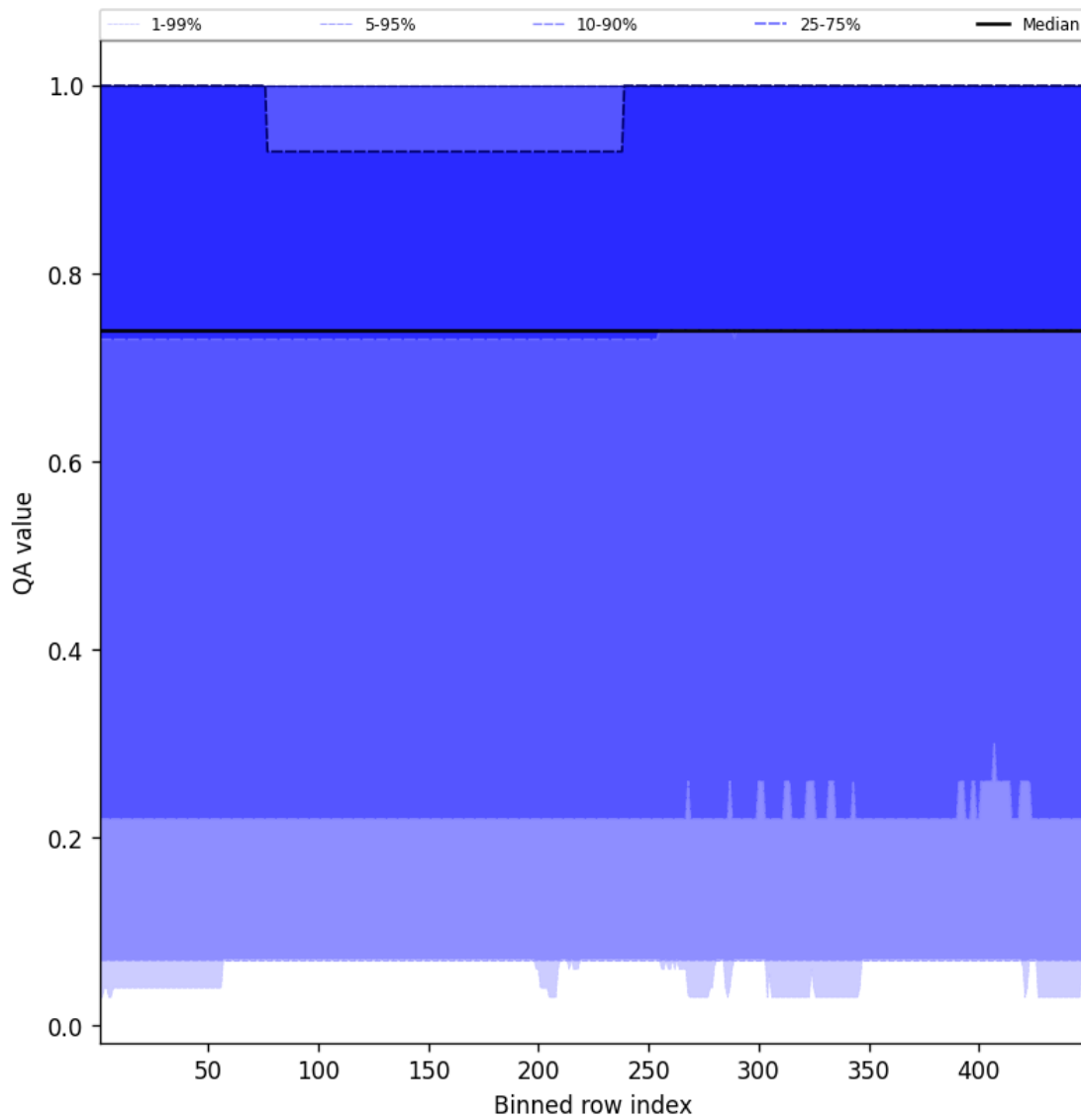
Figure 43: Along track statistics of “QA value” for 2025-03-05 to 2025-03-05
