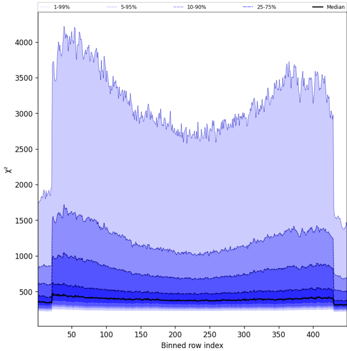
Figure 57: Along track statistics of “ \chi^2 ” for 2025-03-05 to 2025-03-05
