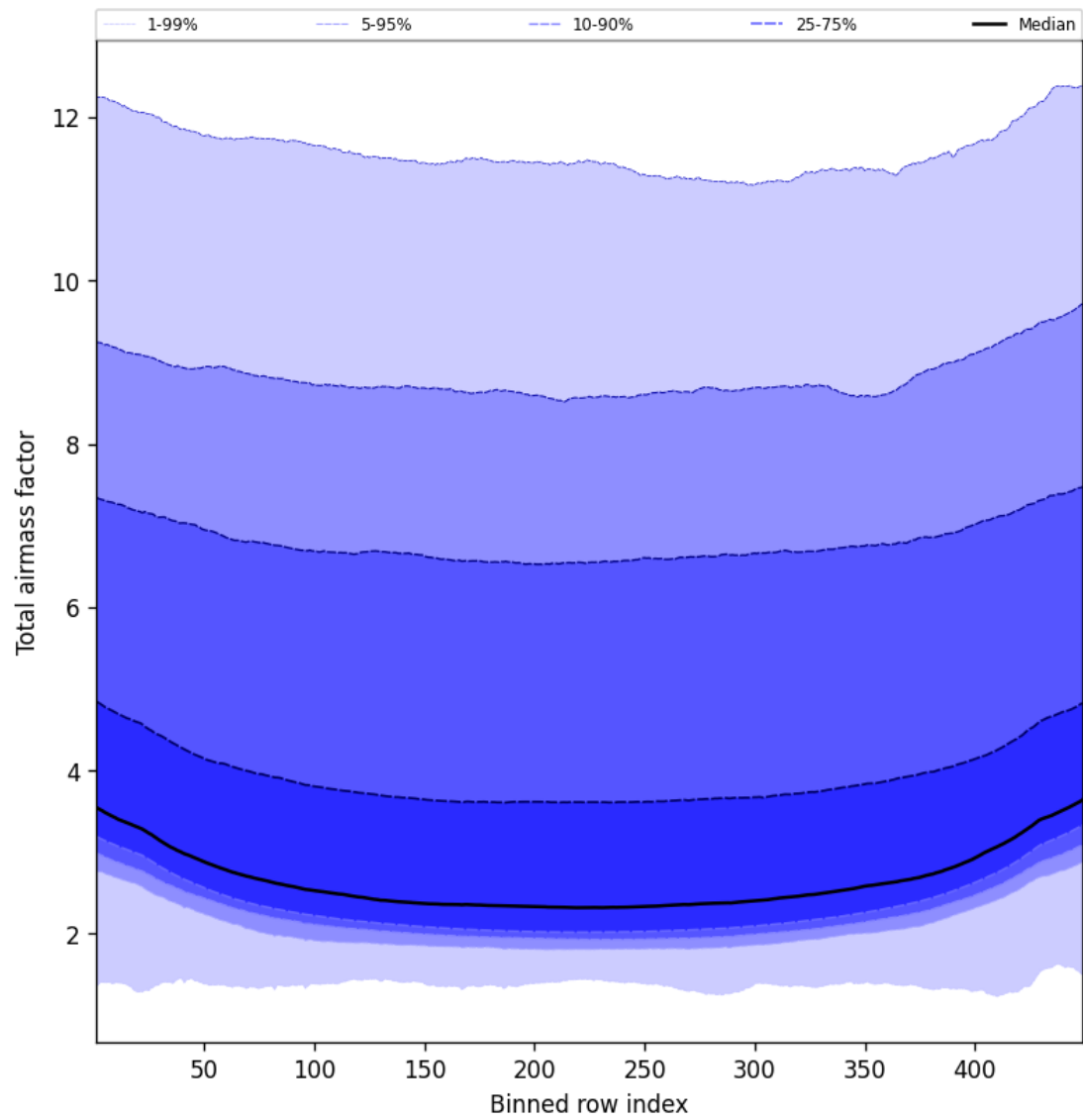
Figure 47: Along track statistics of “Total airmass factor” for 2025-03-05 to 2025-03-05
