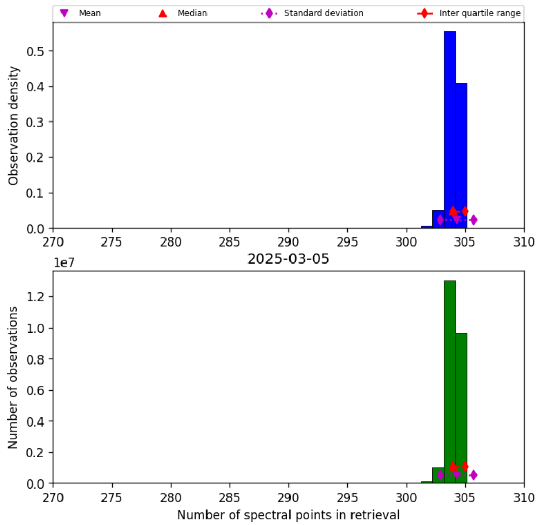
Figure 31: Histogram of “Number of spectral points in retrieval” for 2025-03-05 to 2025-03-05
