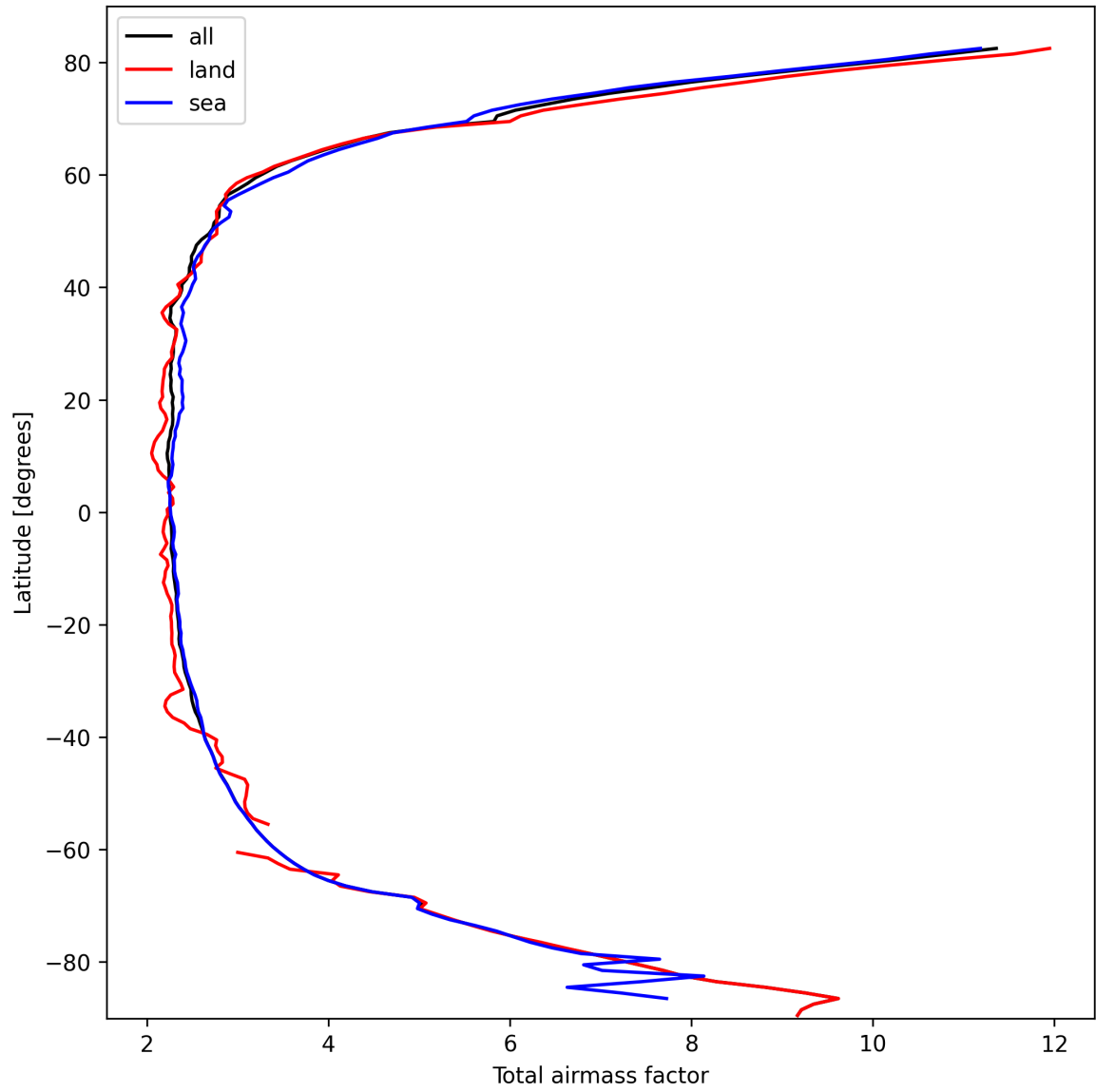
Figure 13: Zonal average of “Total airmass factor” for 2025-03-05 to 2025-03-05.
