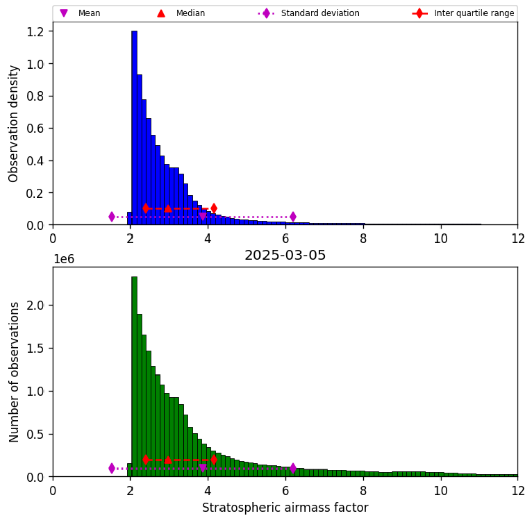
Figure 42: Histogram of “Stratospheric airmass factor” for 2025-03-05 to 2025-03-05
