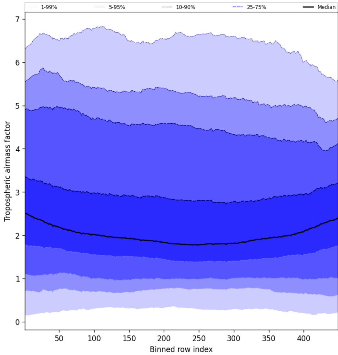
Figure 46: Along track statistics of “Tropospheric airmass factor” for 2025-03-05 to 2025-03-05
