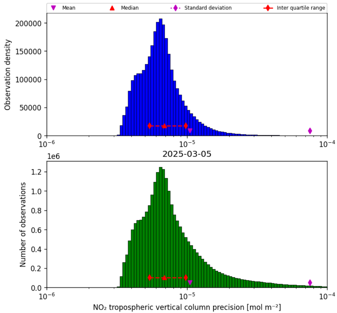
Figure 28: Histogram of “NO 2 tropospheric vertical column precision” for 2025-03-05 to 2025-03-05
