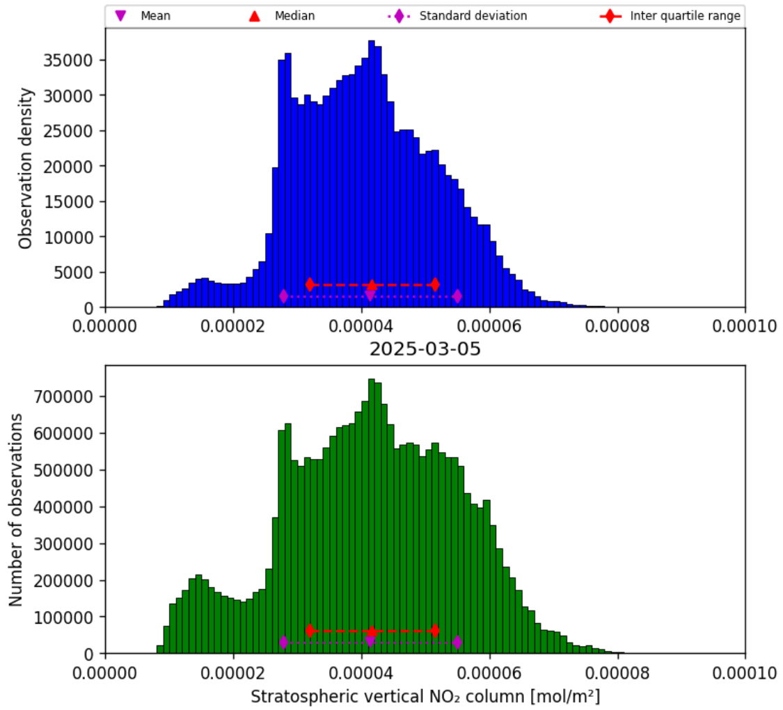
Figure 34: Histogram of “Stratospheric vertical NO 2 column” for 2025-03-05 to 2025-03-05
