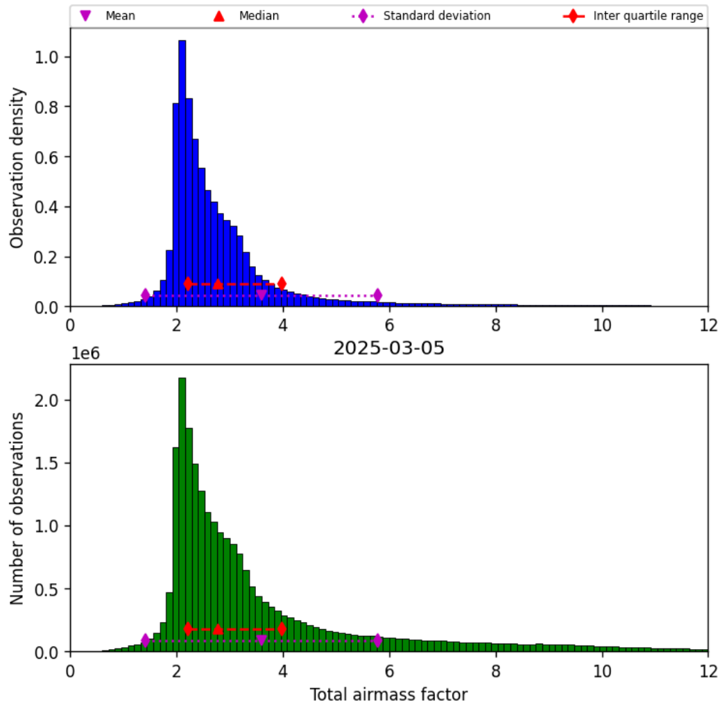
Figure 30: Histogram of “Total airmass factor” for 2025-03-05 to 2025-03-05
