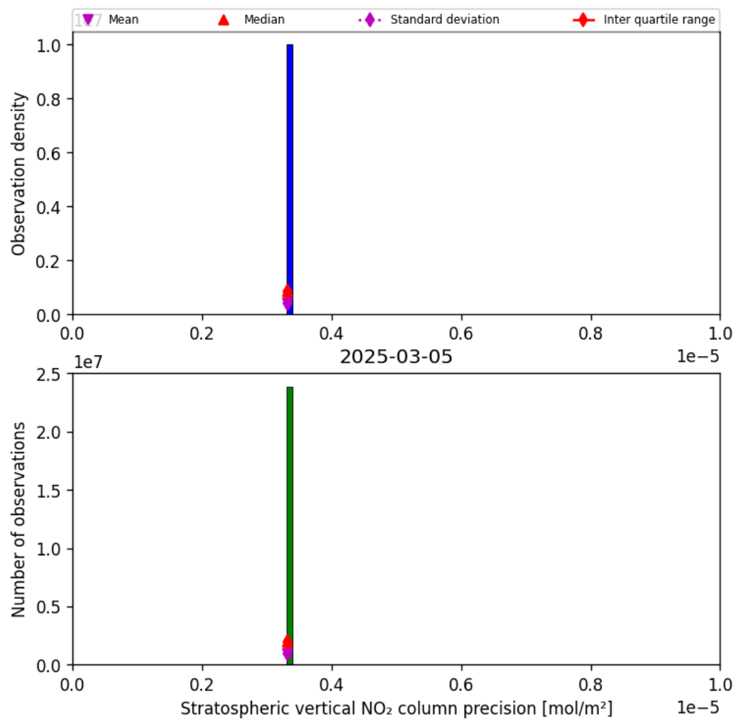
Figure 35: Histogram of “Stratospheric vertical NO 2 column precision” for 2025-03-05 to 2025-03-05
