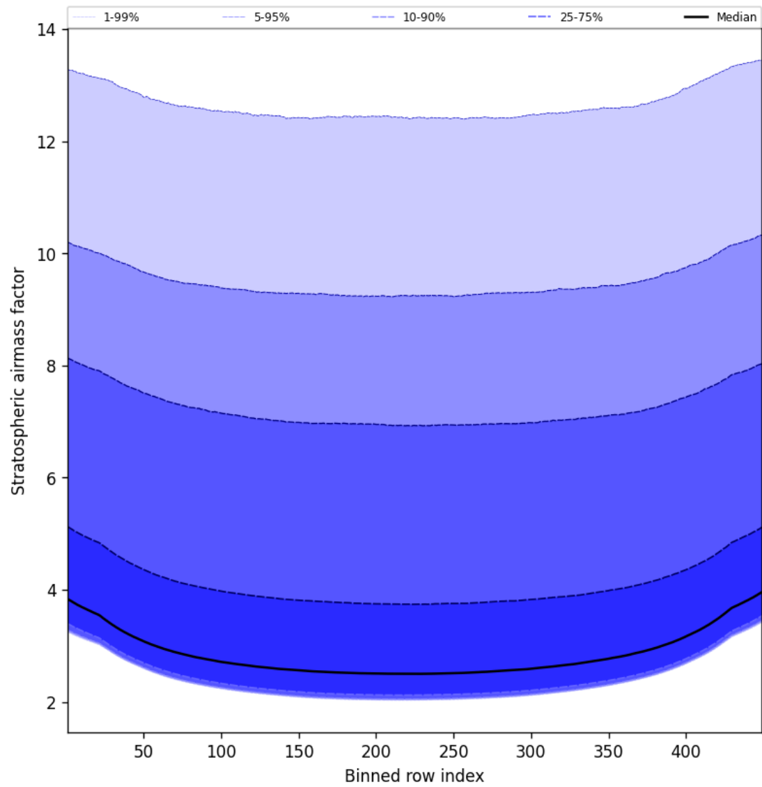
Figure 59: Along track statistics of “Stratospheric airmass factor” for 2025-03-05 to 2025-03-05
