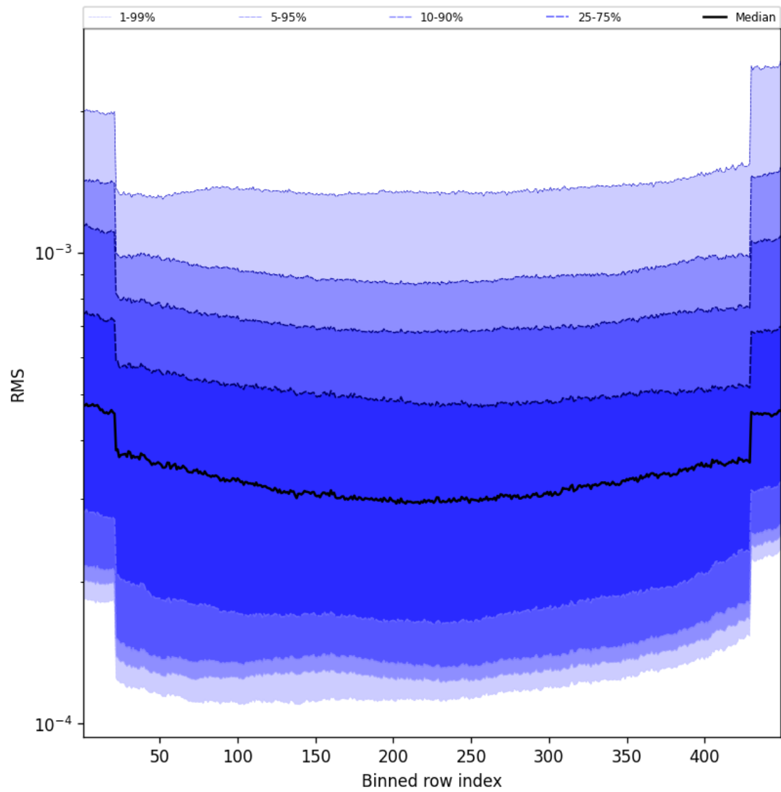
Figure 58: Along track statistics of “RMS” for 2025-03-05 to 2025-03-05
