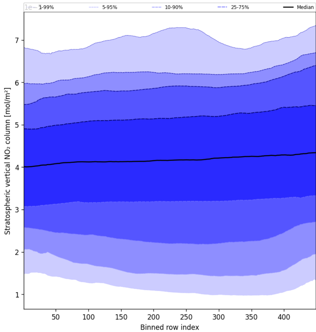
Figure 51: Along track statistics of “Stratospheric vertical NO 2 column” for 2025-03-05 to 2025-03-05
