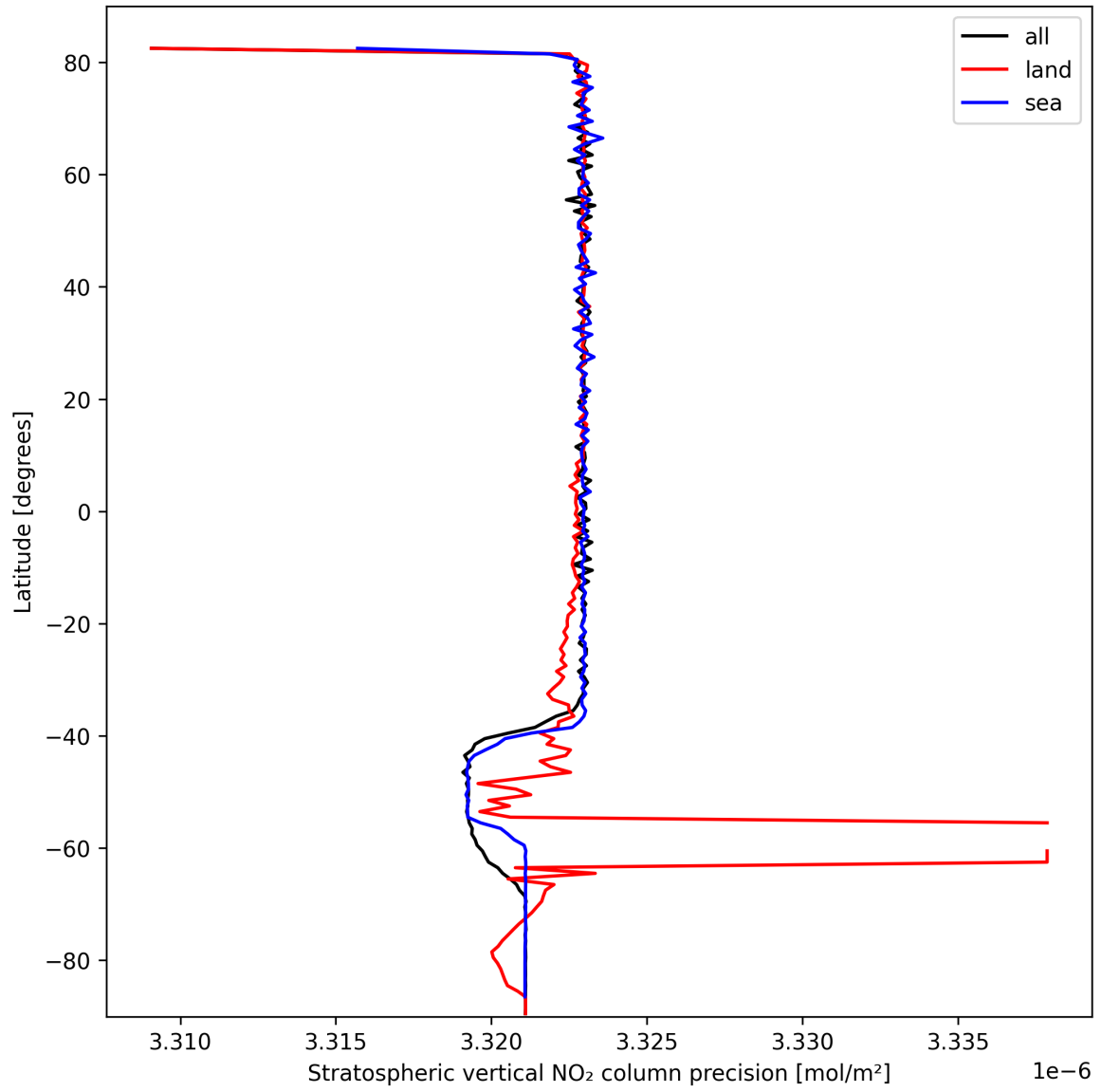
Figure 18: Zonal average of “Stratospheric vertical NO 2 column precision” for 2025-03-05 to 2025-03-05.
