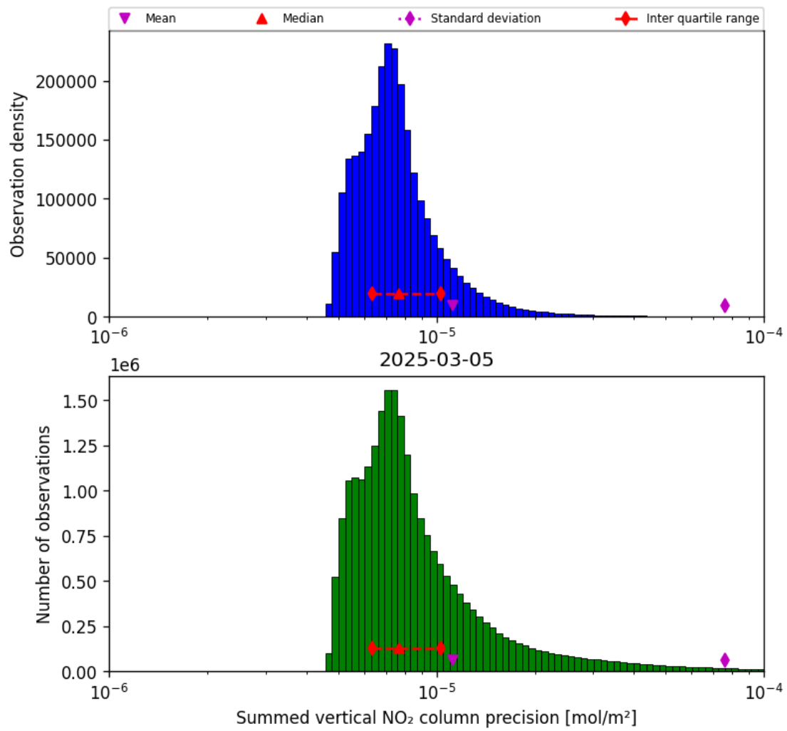
Figure 39: Histogram of "Summed vertical NO 2 column precision" for 2025-03-05 to 2025-03-05
