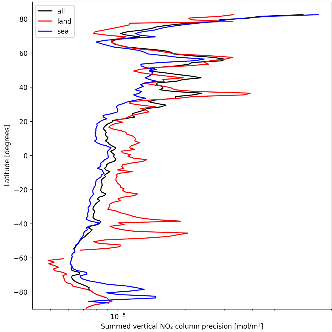
Figure 22: Zonal average of “Summed vertical NO 2 column precision” for 2025-03-05 to 2025-03-05.
