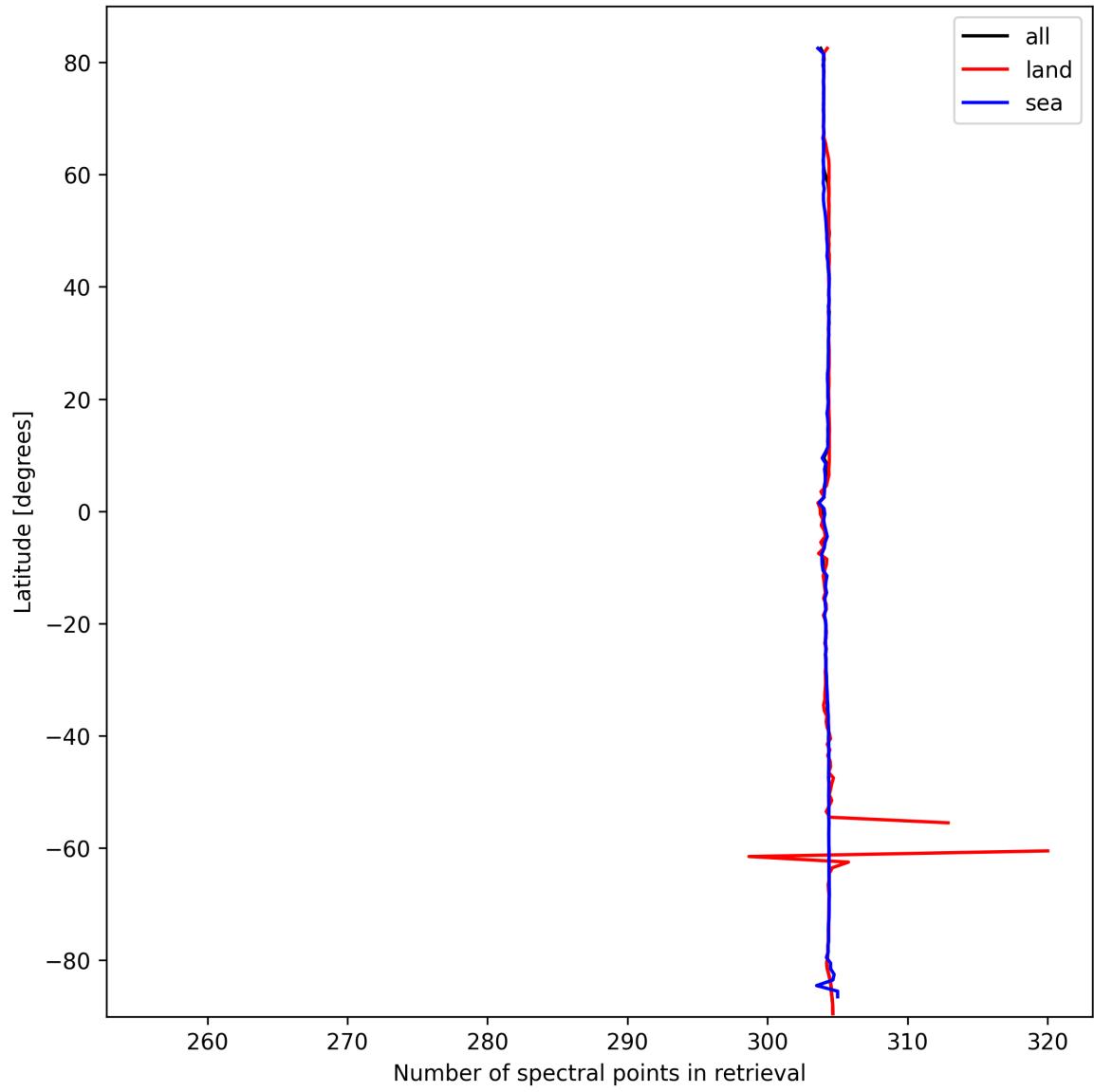
Figure 14: Zonal average of “Number of spectral points in retrieval” for 2025-03-05 to 2025-03-05.
