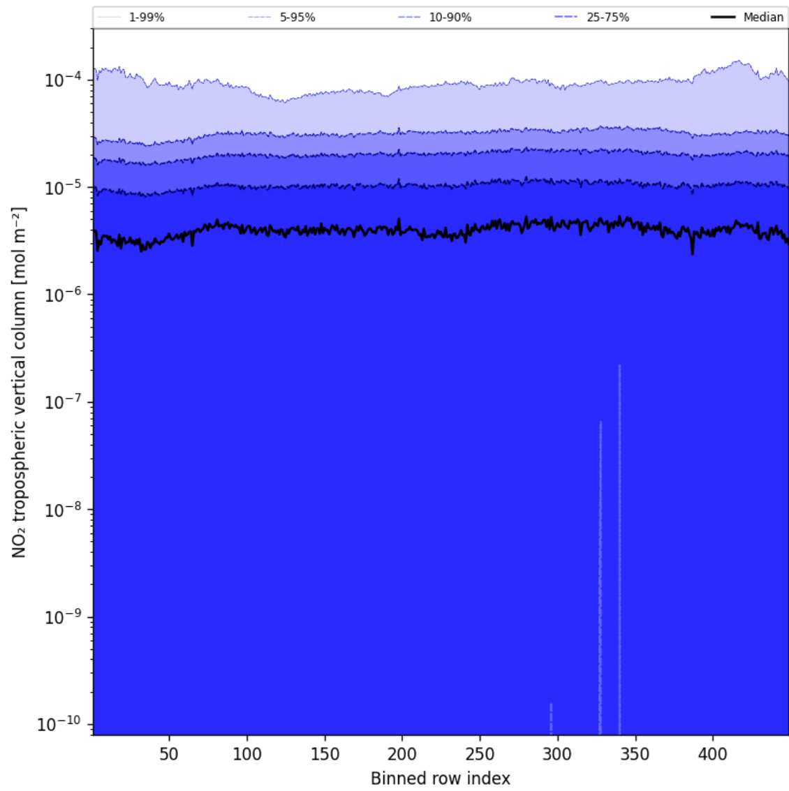
Figure 44: Along track statistics of “NO 2 tropospheric vertical column” for 2025-03-05 to 2025-03-05
