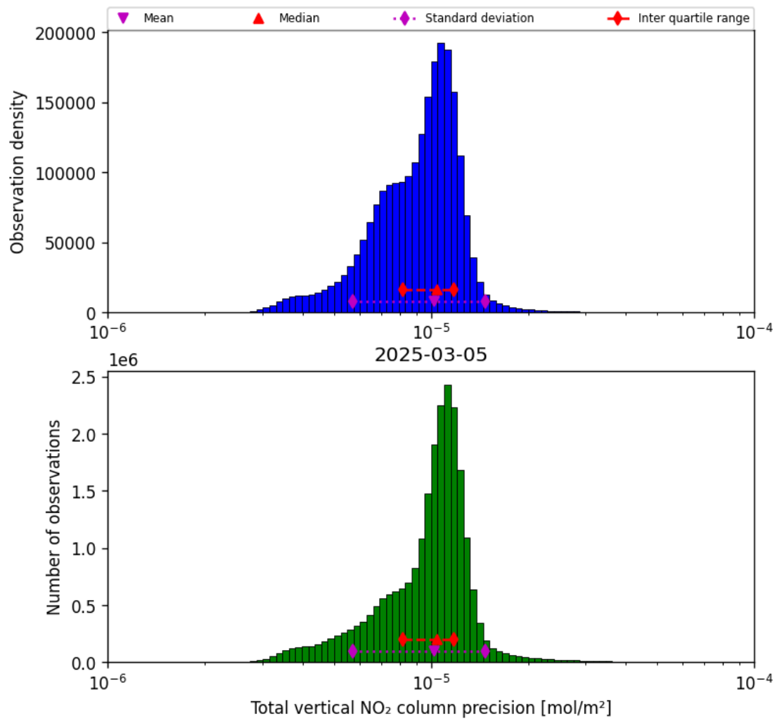
Figure 37: Histogram of "Total vertical NO 2 column precision" for 2025-03-05 to 2025-03-05
