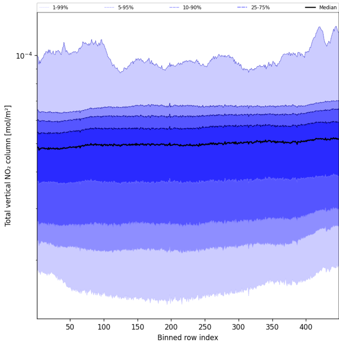
Figure 53: Along track statistics of “Total vertical NO 2 column” for 2025-03-05 to 2025-03-05
