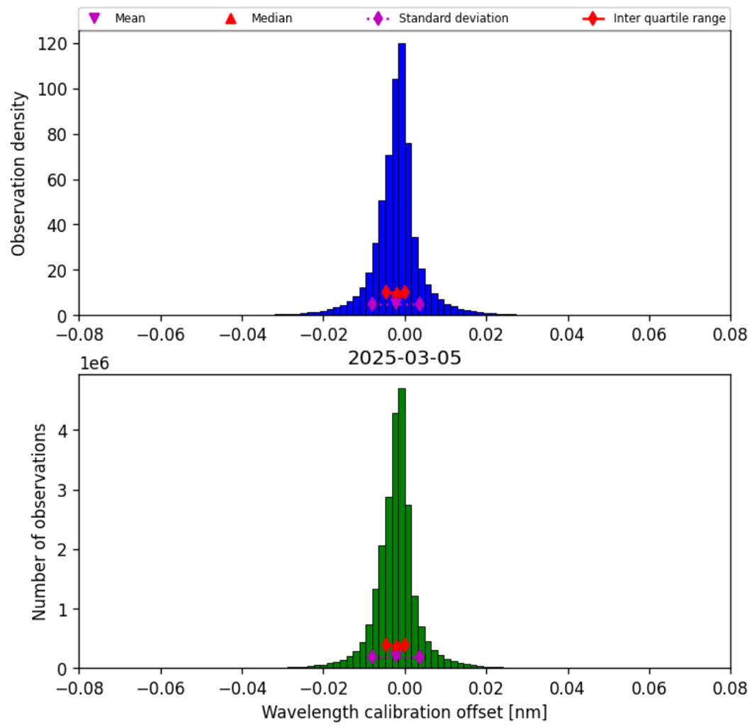
Figure 33: Histogram of “Wavelength calibration offset” for 2025-03-05 to 2025-03-05
