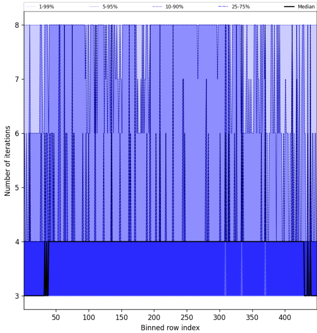
Figure 49: Along track statistics of “Number of iterations” for 2025-03-05 to 2025-03-05
