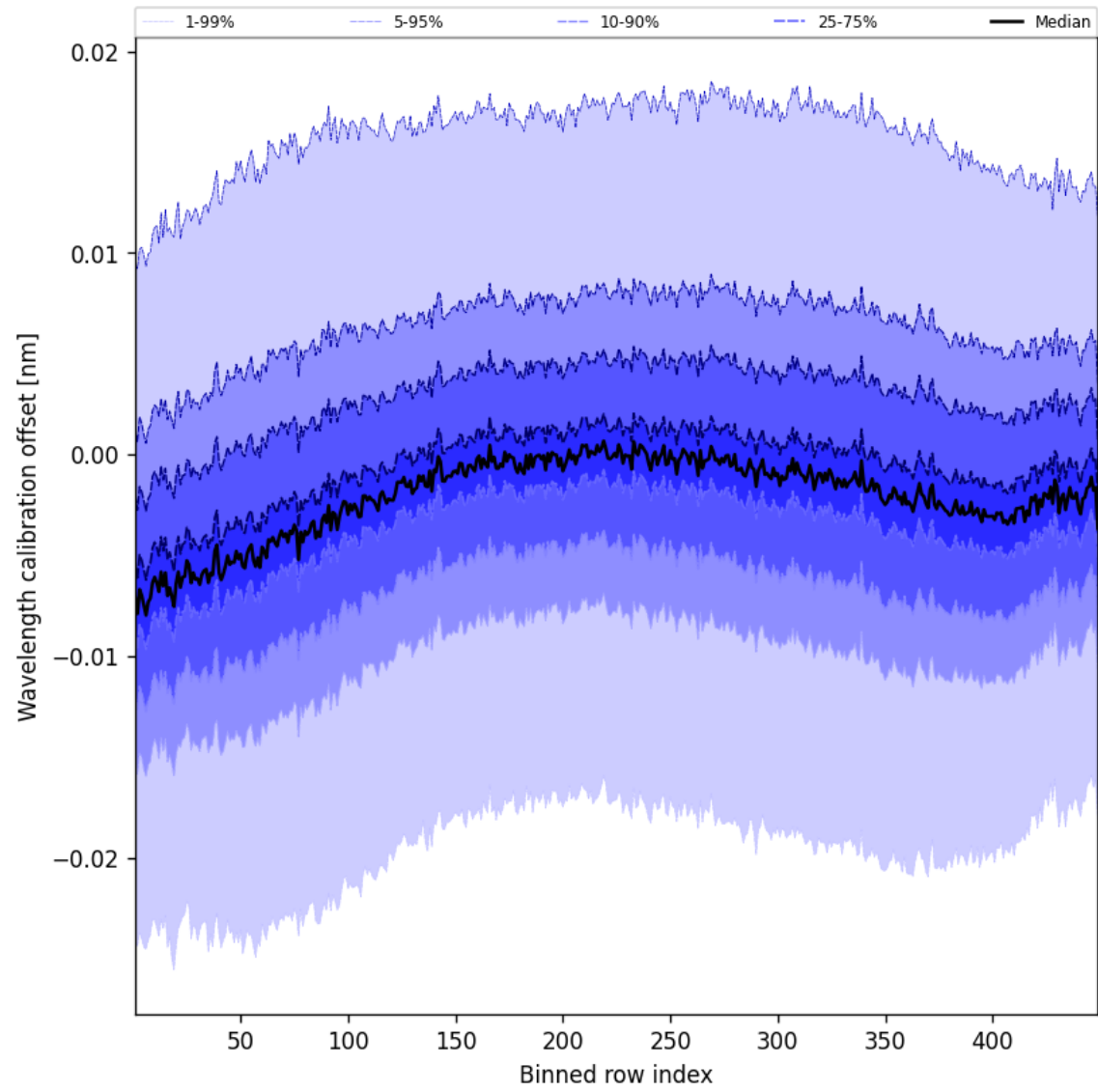
Figure 50: Along track statistics of “Wavelength calibration offset” for 2025-03-06 to 2025-03-07
