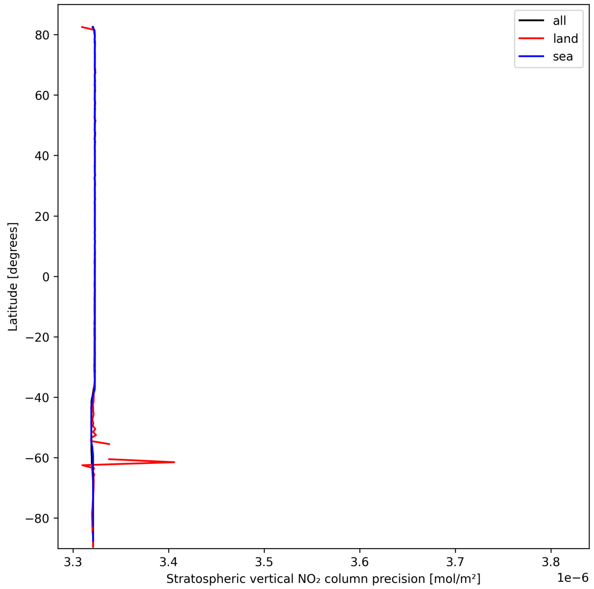
Figure 18: Zonal average of “Stratospheric vertical NO 2 column precision” for 2025-03-06 to 2025-03-07.
