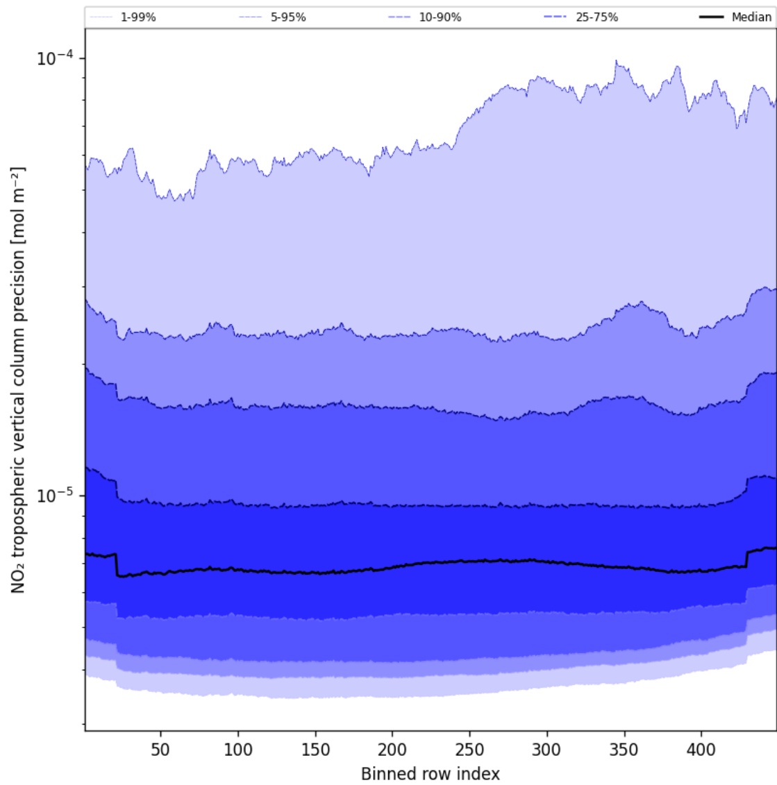
Figure 45: Along track statistics of “NO 2 tropospheric vertical column precision” for 2025-03-06 to 2025-03-07
