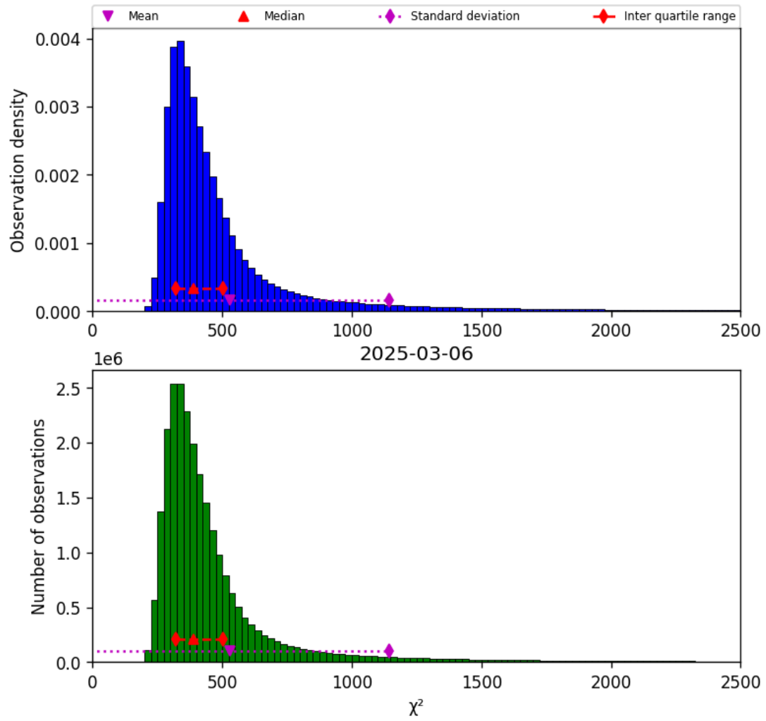
Figure 40: Histogram of “ \chi^2 ” for 2025-03-06 to 2025-03-07
