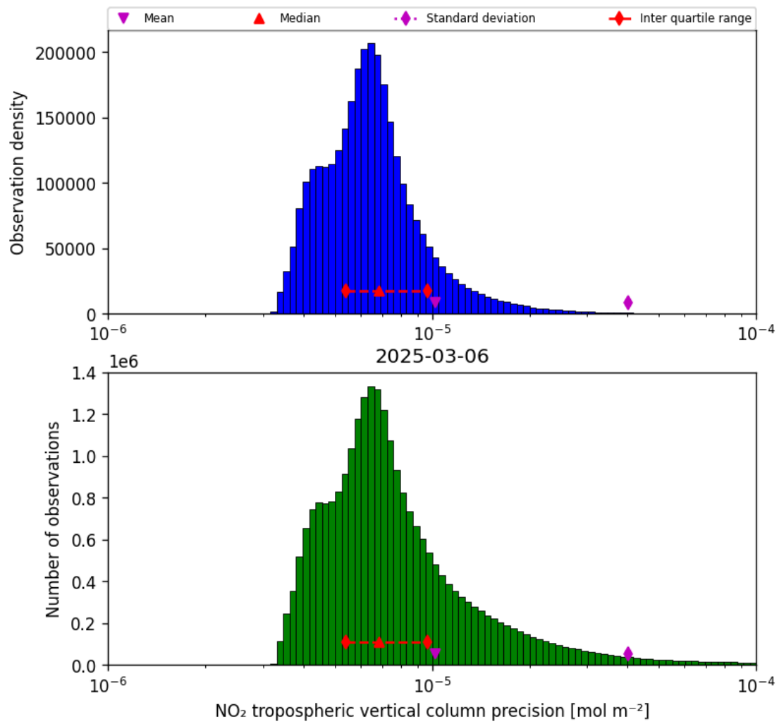
Figure 28: Histogram of “NO 2 tropospheric vertical column precision” for 2025-03-06 to 2025-03-07
