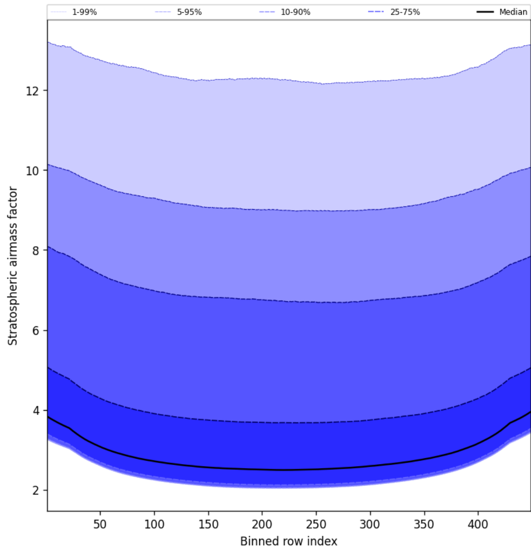
Figure 59: Along track statistics of “Stratospheric airmass factor” for 2025-03-06 to 2025-03-07
