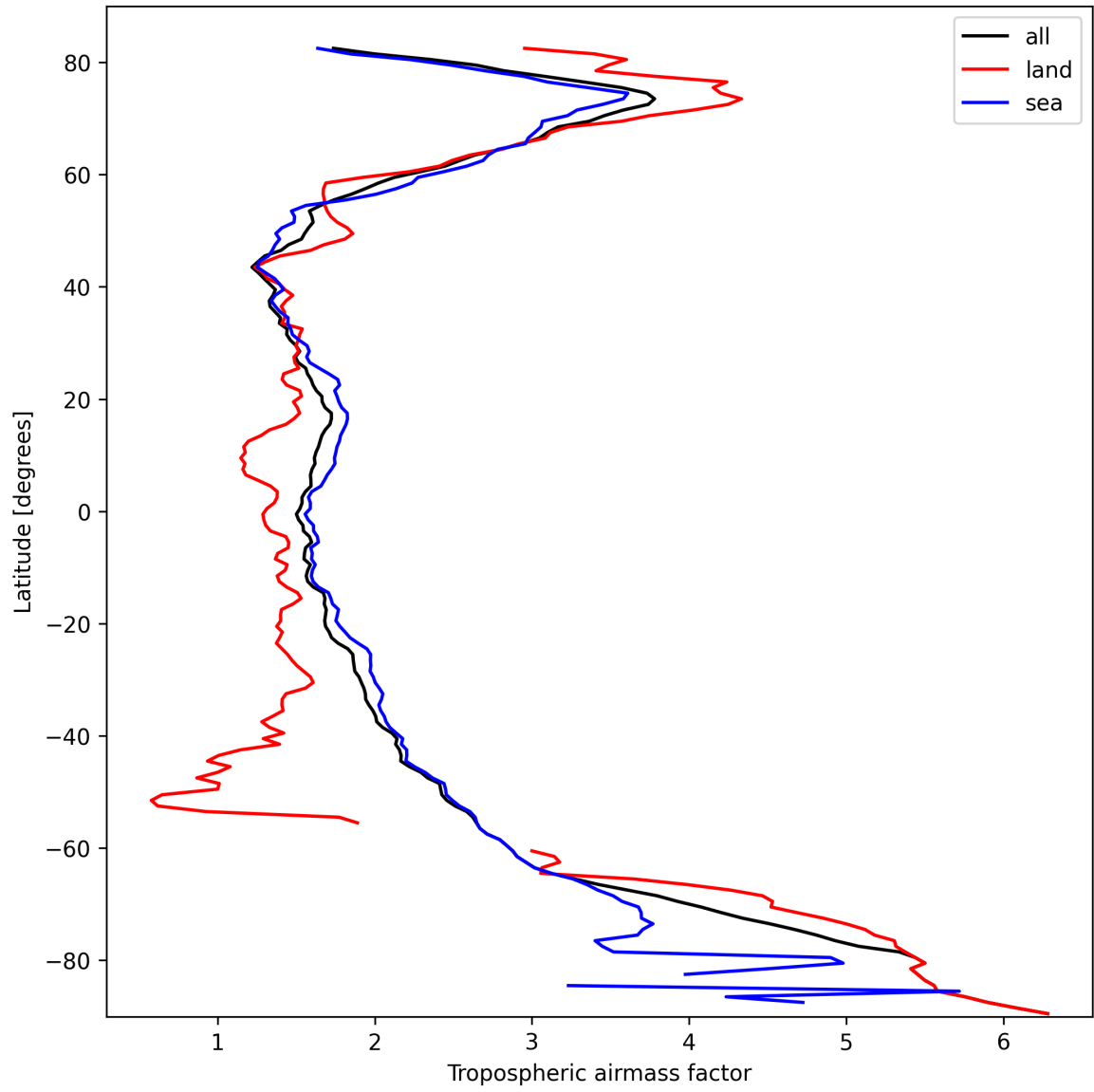
Figure 12: Zonal average of “Tropospheric air mass factor” for 2025-03-06 to 2025-03-07.
