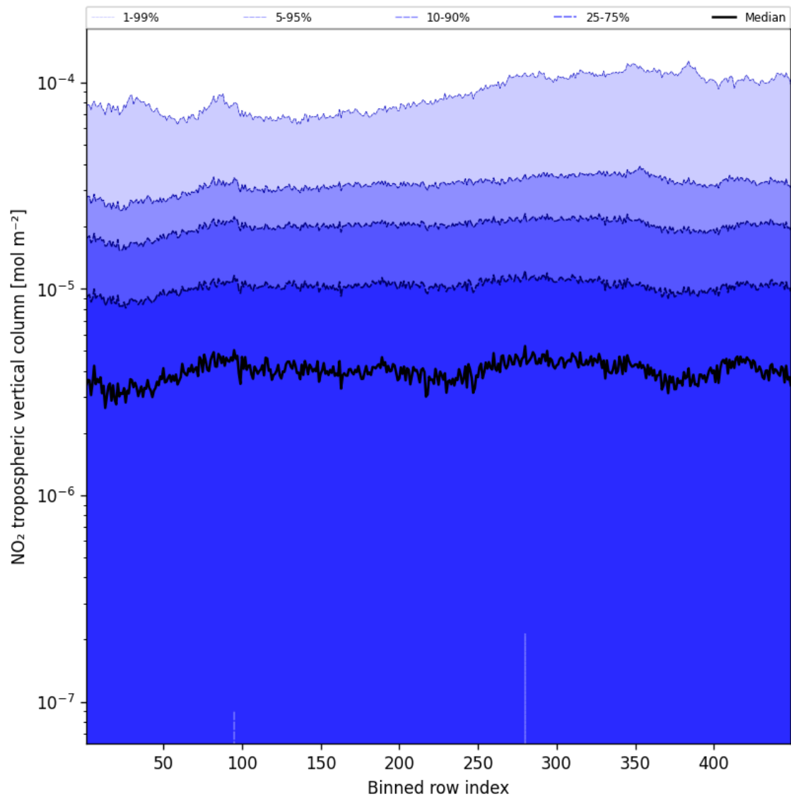
Figure 44: Along track statistics of “NO 2 tropospheric vertical column” for 2025-03-06 to 2025-03-07
