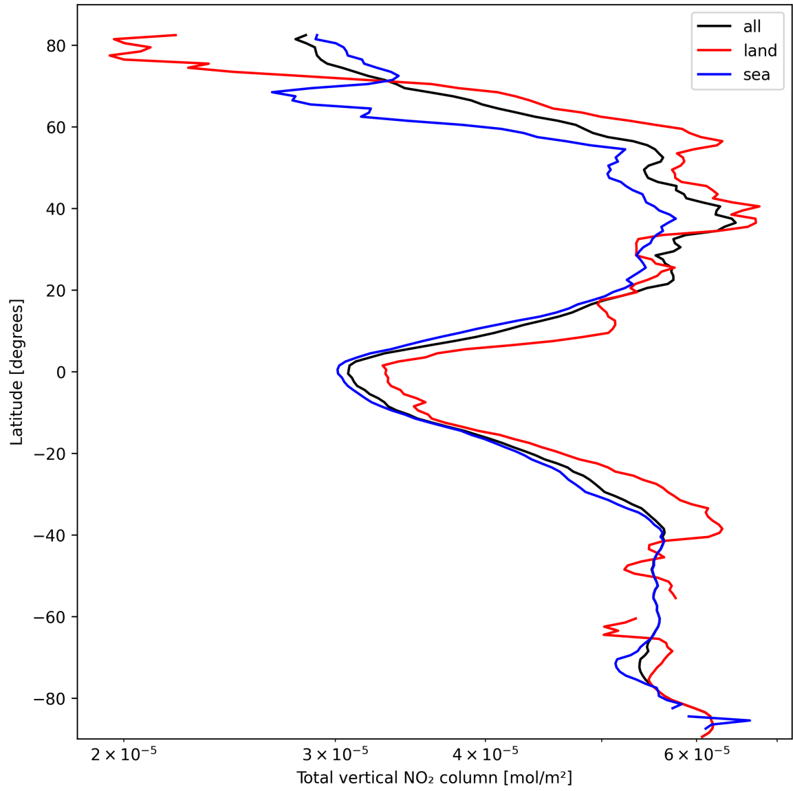
Figure 19: Zonal average of “Total vertical NO 2 column” for 2025-03-06 to 2025-03-07.
