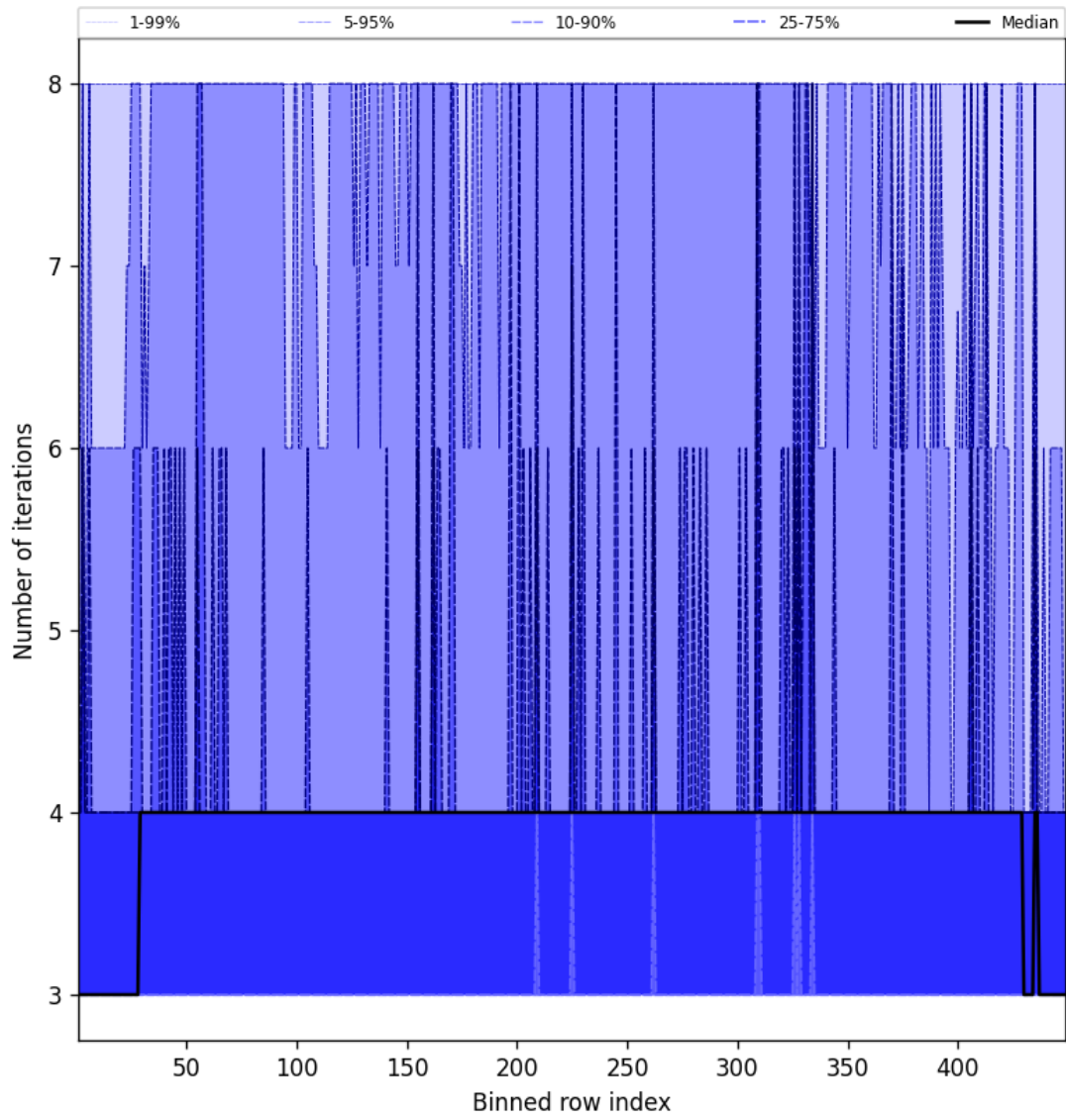
Figure 49: Along track statistics of “Number of iterations” for 2025-03-06 to 2025-03-07
