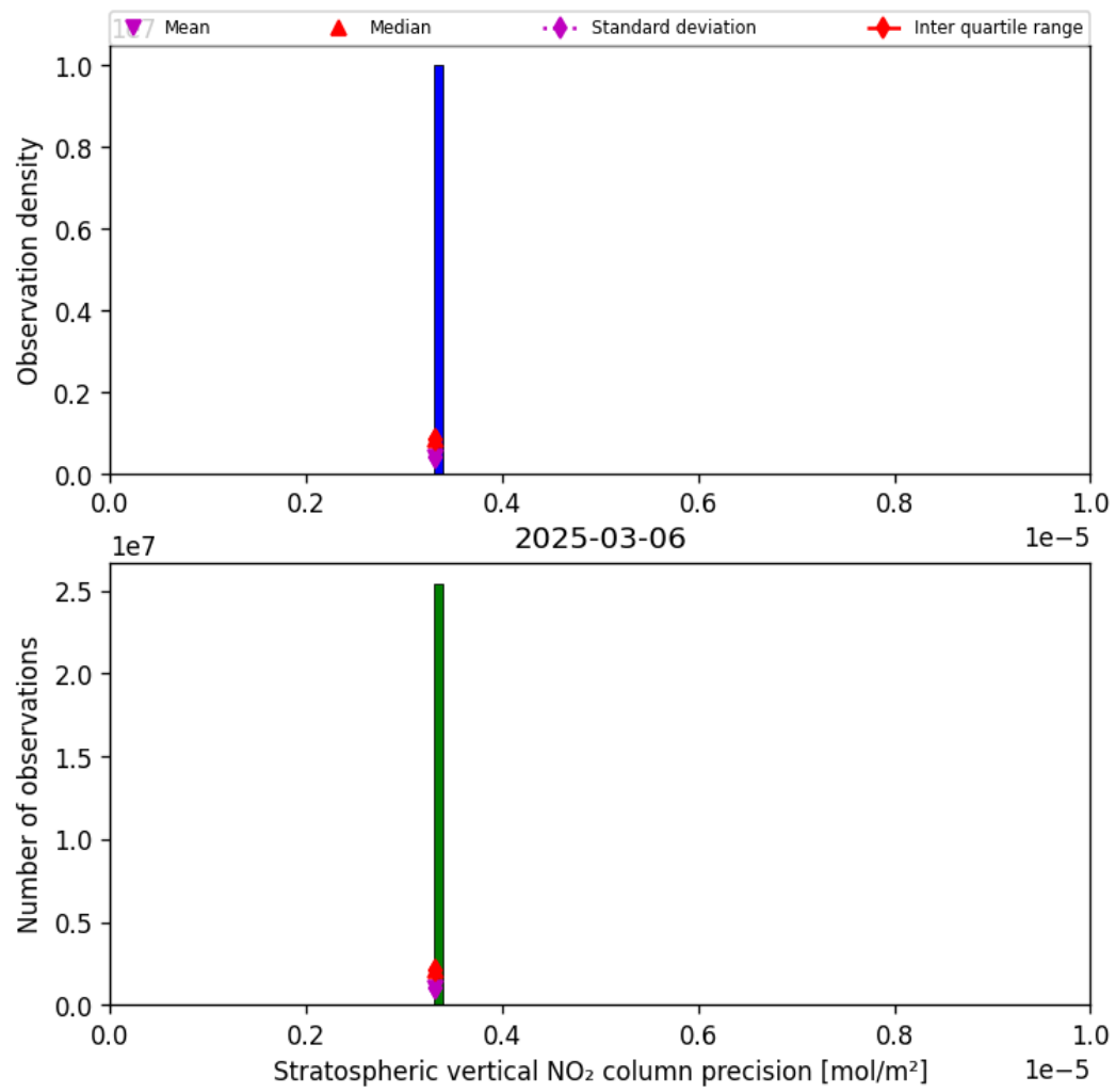
Figure 35: Histogram of “Stratospheric vertical NO 2 column precision” for 2025-03-06 to 2025-03-07
