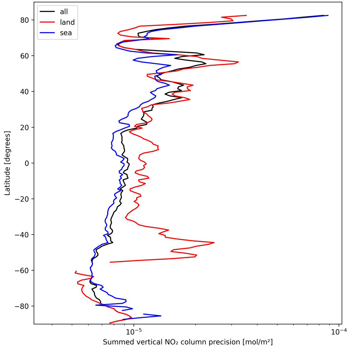
Figure 22: Zonal average of “Summed vertical NO 2 column precision” for 2025-03-06 to 2025-03-07.
