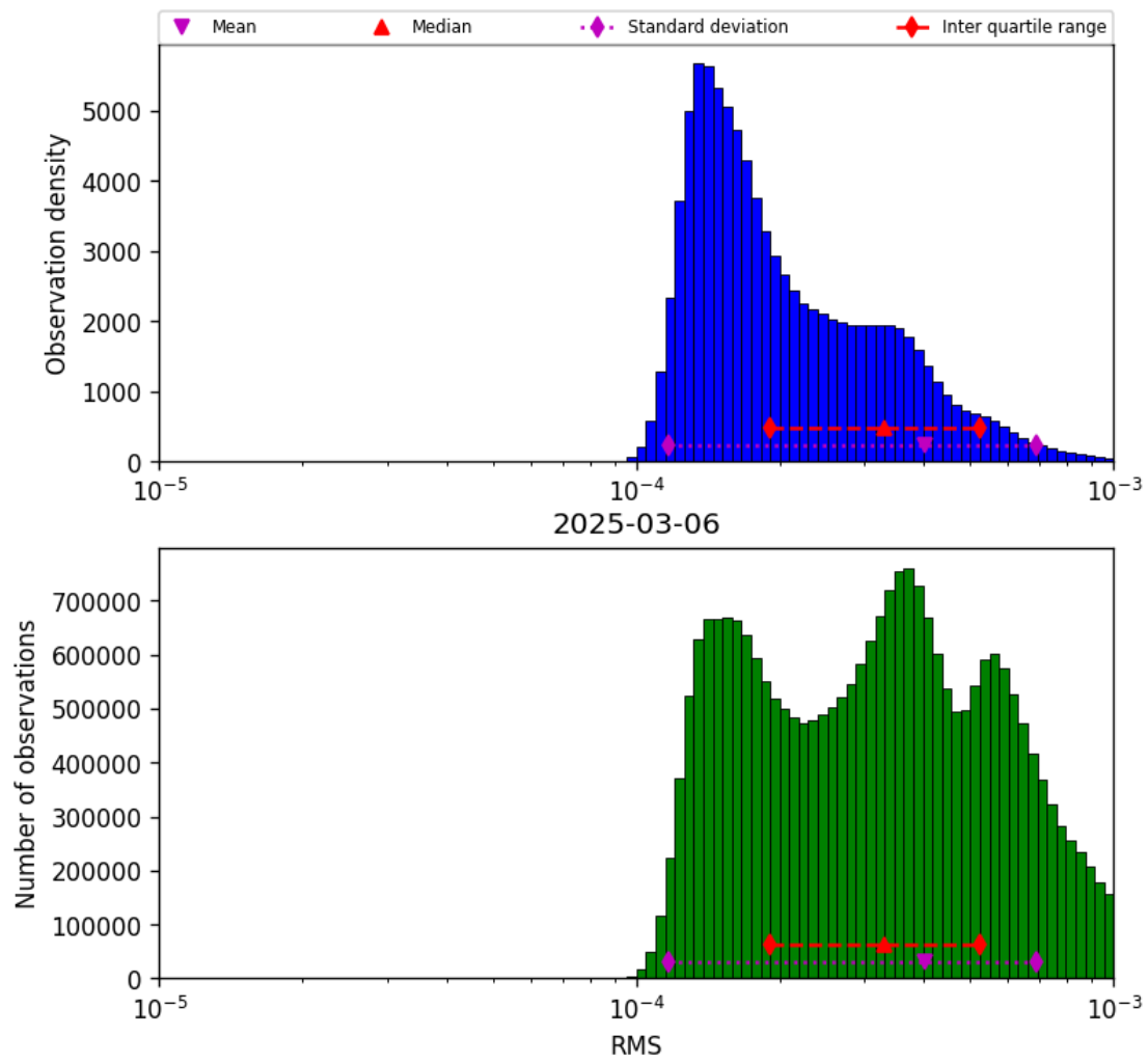
Figure 41: Histogram of “RMS” for 2025-03-06 to 2025-03-07
