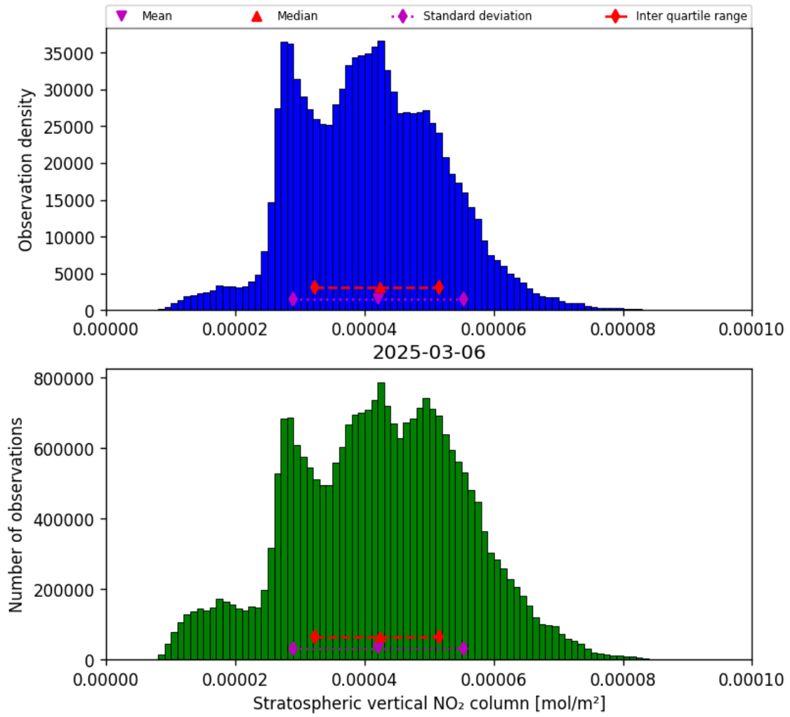
Figure 34: Histogram of “Stratospheric vertical NO 2 column” for 2025-03-06 to 2025-03-07
