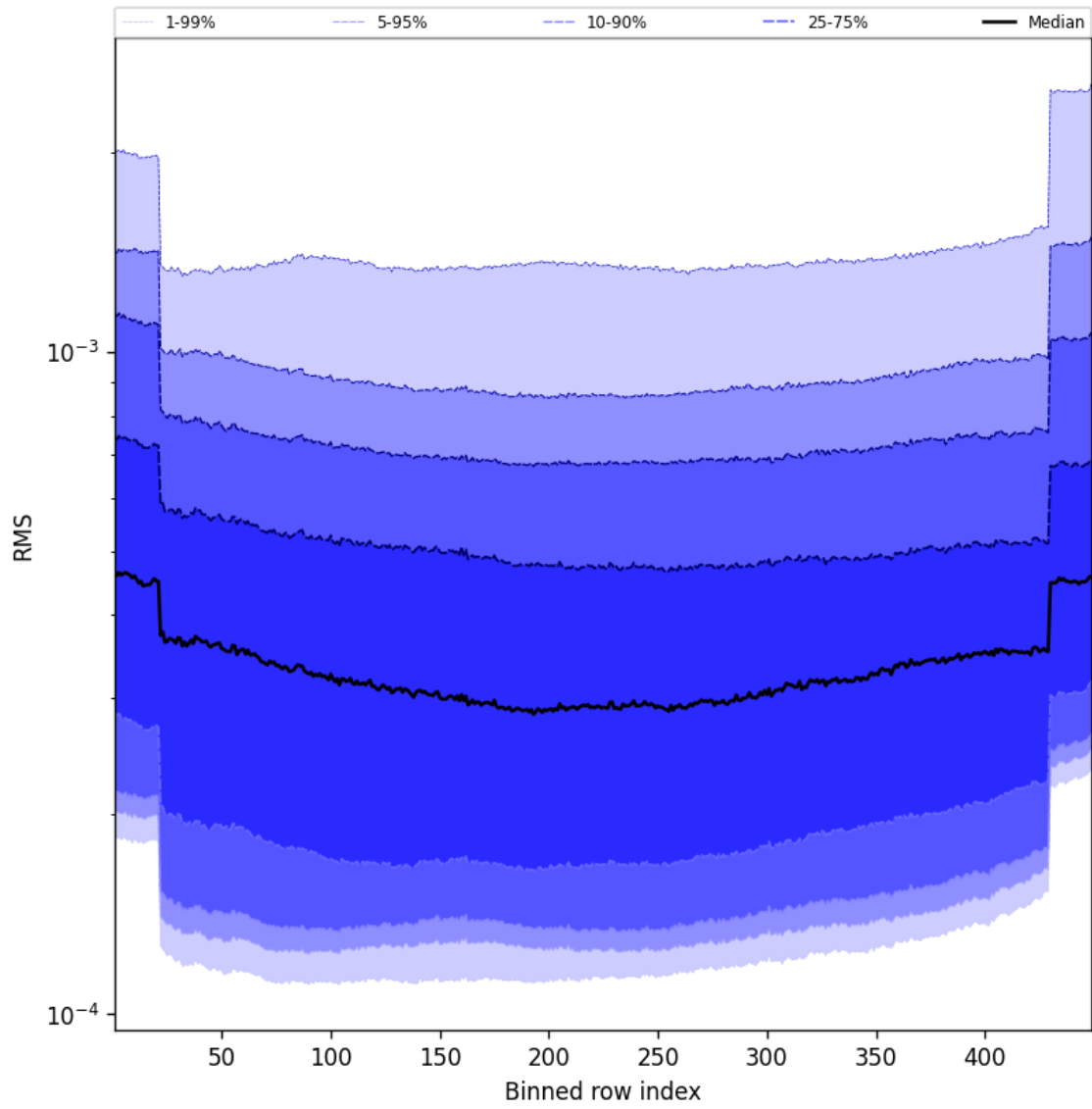
Figure 58: Along track statistics of “RMS” for 2025-03-06 to 2025-03-07
