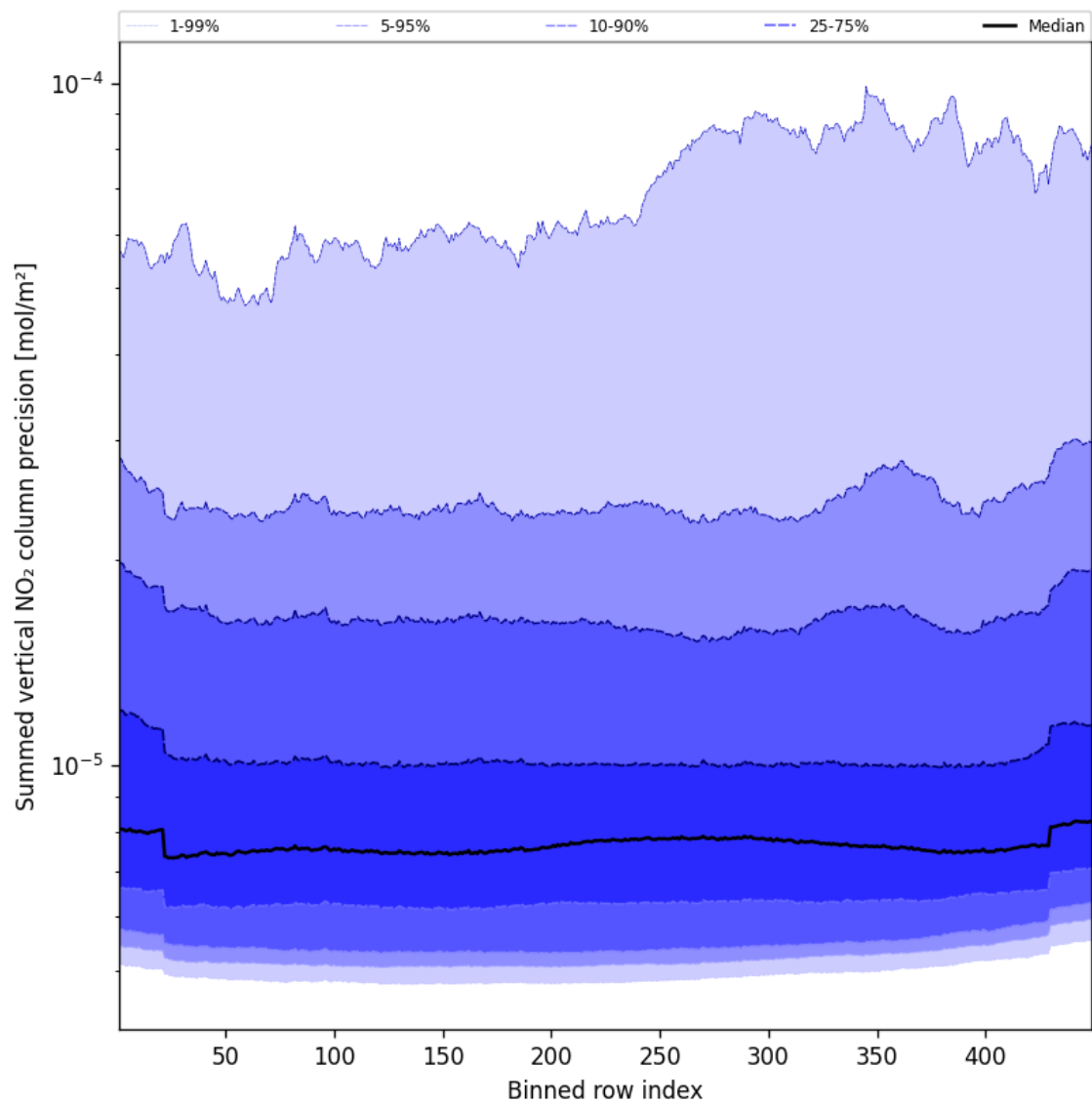
Figure 56: Along track statistics of “Summed vertical NO 2 column precision” for 2025-03-06 to 2025-03-07
