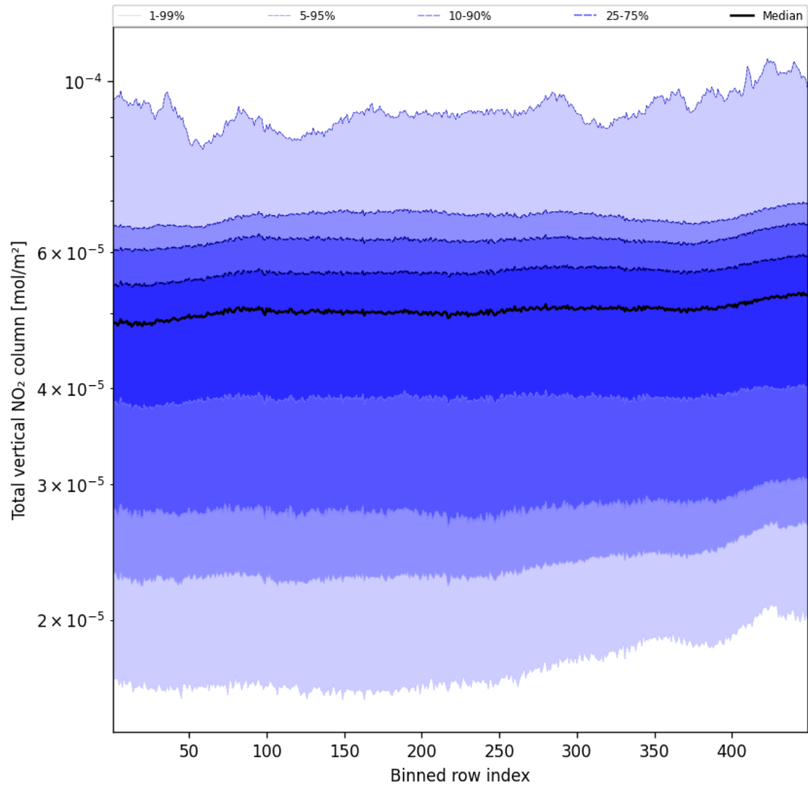
Figure 53: Along track statistics of “Total vertical NO 2 column” for 2025-03-06 to 2025-03-07
