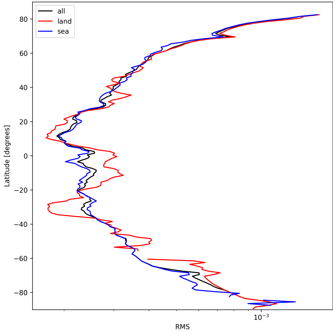
Figure 24: Zonal average of “RMS” for 2025-03-06 to 2025-03-07.
