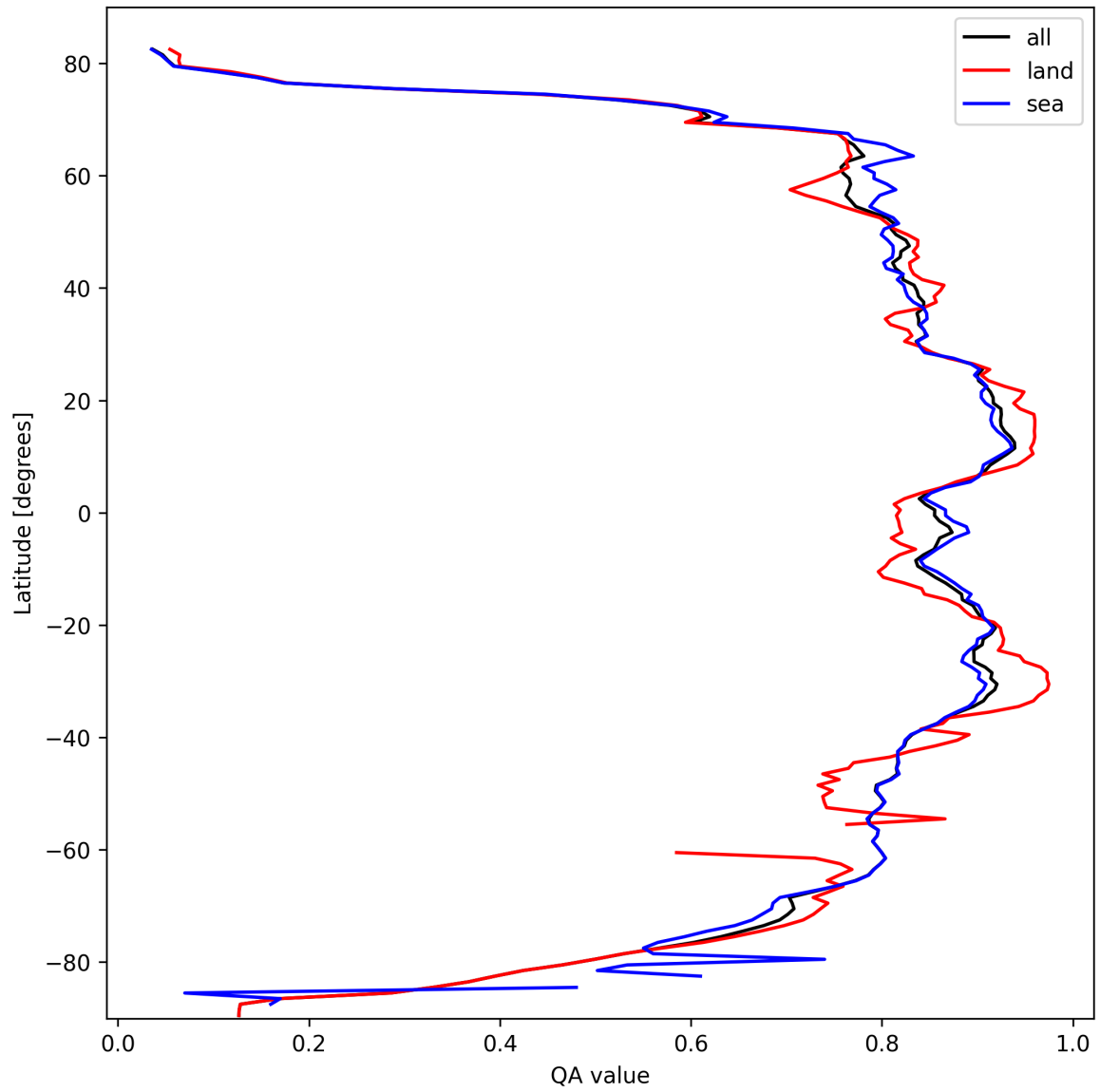
Figure 9: Zonal average of “QA value” for 2025-03-06 to 2025-03-07.
