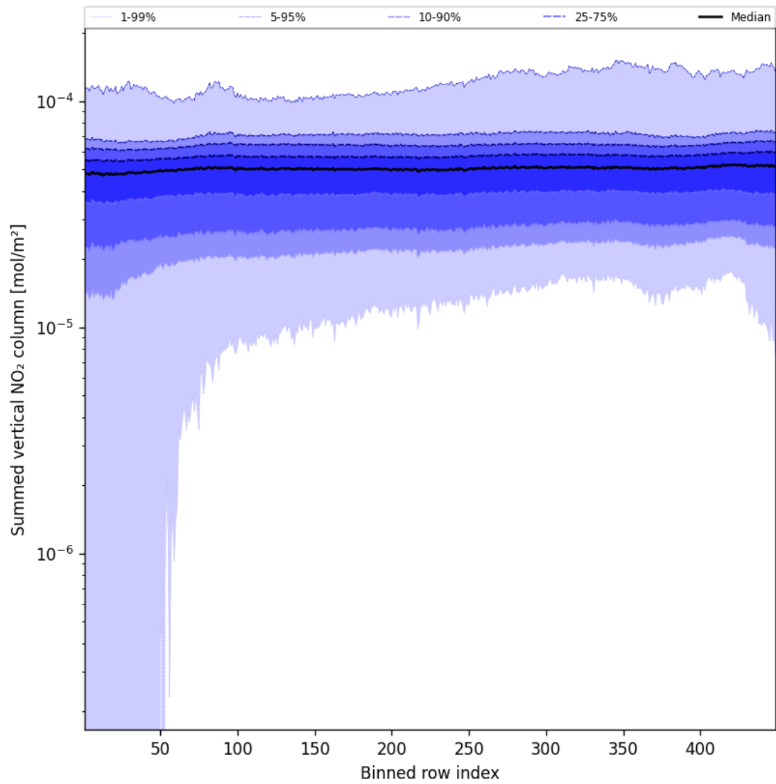
Figure 55: Along track statistics of “Summed vertical NO 2 column” for 2025-03-06 to 2025-03-07
