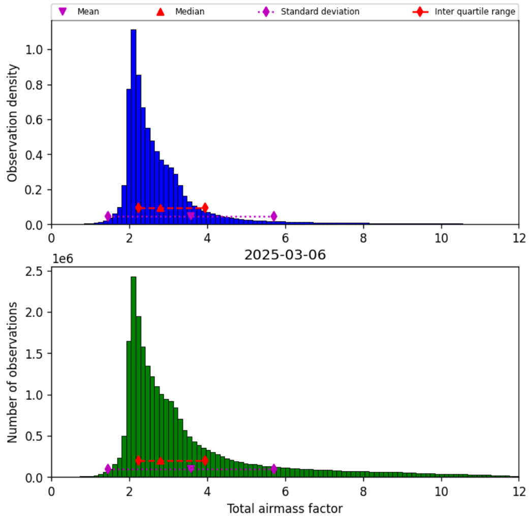
Figure 30: Histogram of “Total airmass factor” for 2025-03-06 to 2025-03-07
