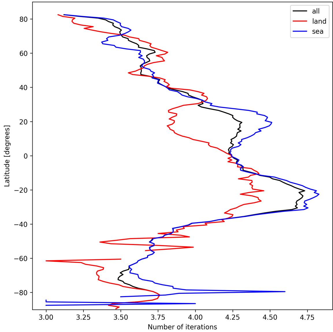
Figure 15: Zonal average of “Number of iterations” for 2025-03-06 to 2025-03-07.
