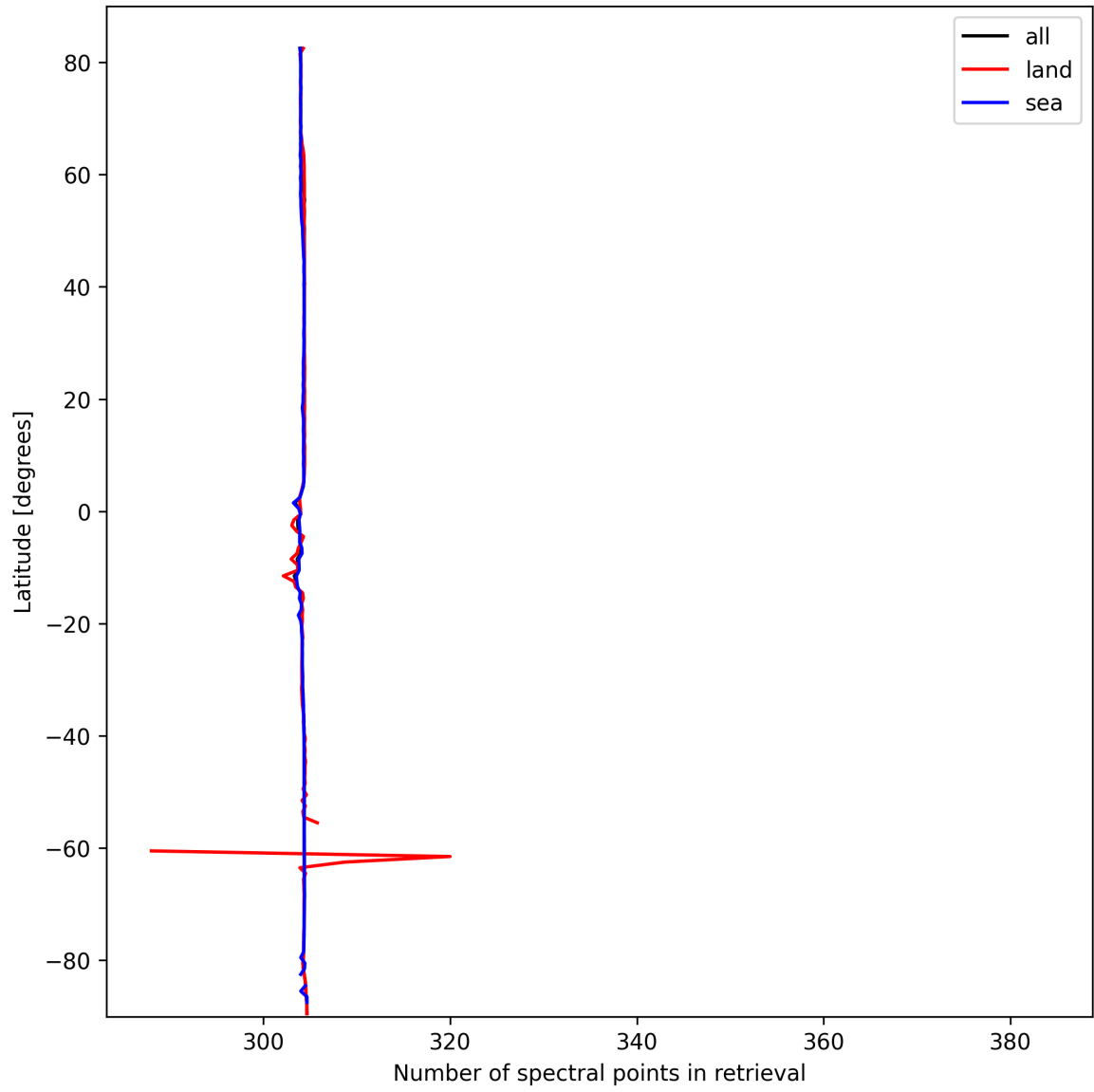
Figure 14: Zonal average of “Number of spectral points in retrieval” for 2025-03-06 to 2025-03-07.
