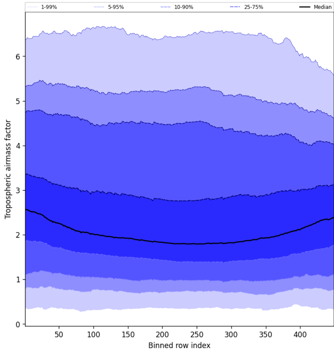
Figure 46: Along track statistics of “Tropospheric airmass factor” for 2025-03-06 to 2025-03-07
