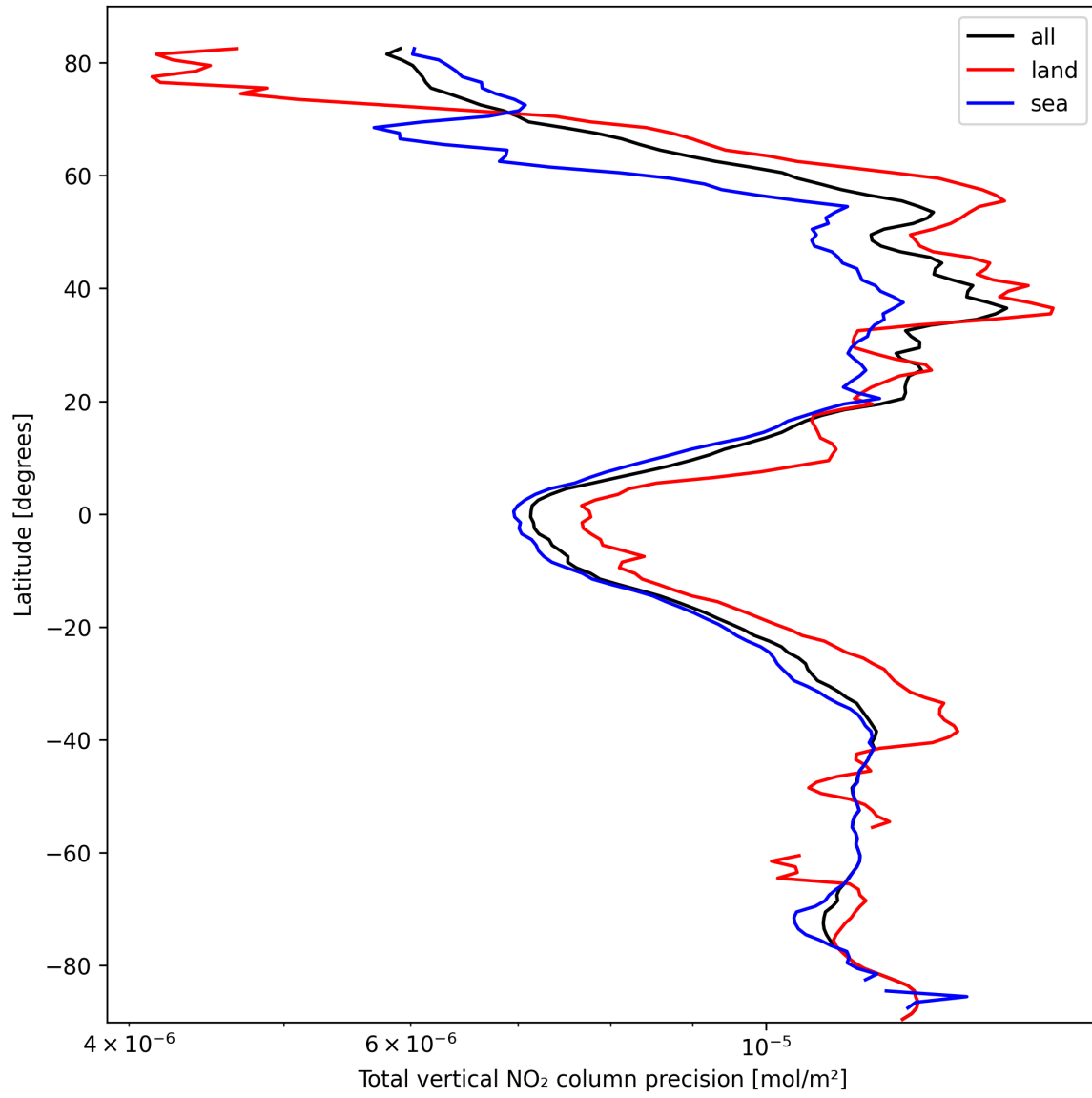
Figure 20: Zonal average of “Total vertical NO 2 column precision” for 2025-03-06 to 2025-03-07.
