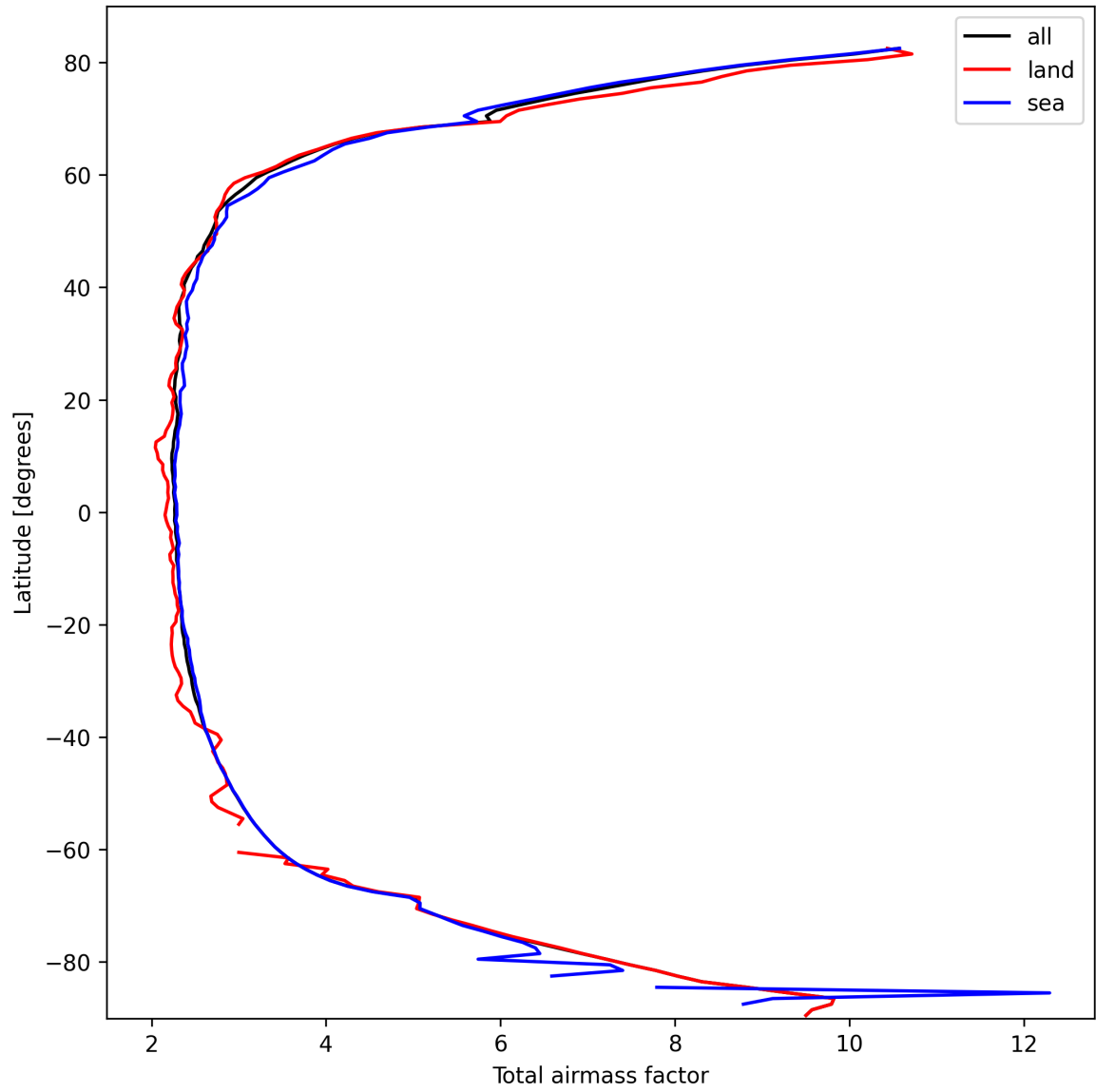
Figure 13: Zonal average of “Total airmass factor” for 2025-03-06 to 2025-03-07.
