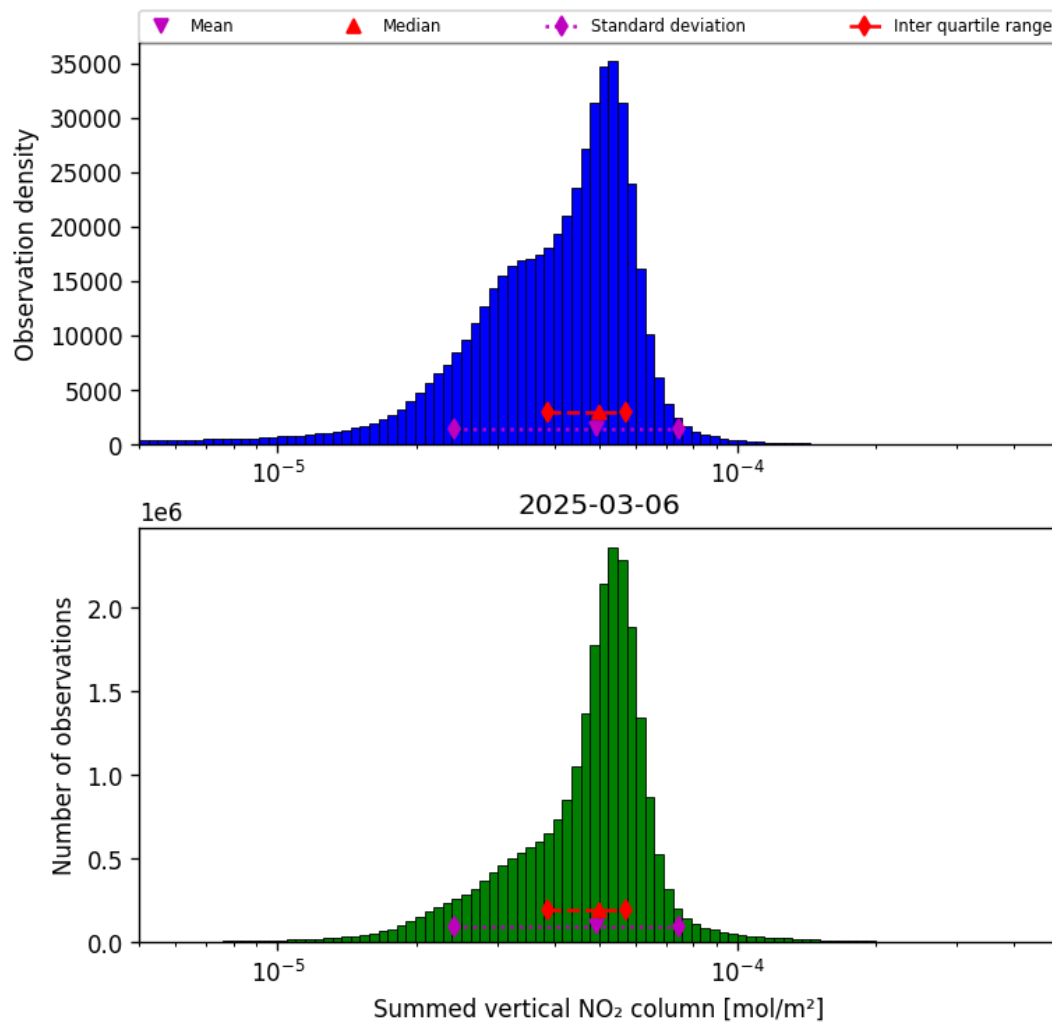
Figure 38: Histogram of “Summed vertical NO 2 column” for 2025-03-06 to 2025-03-07
