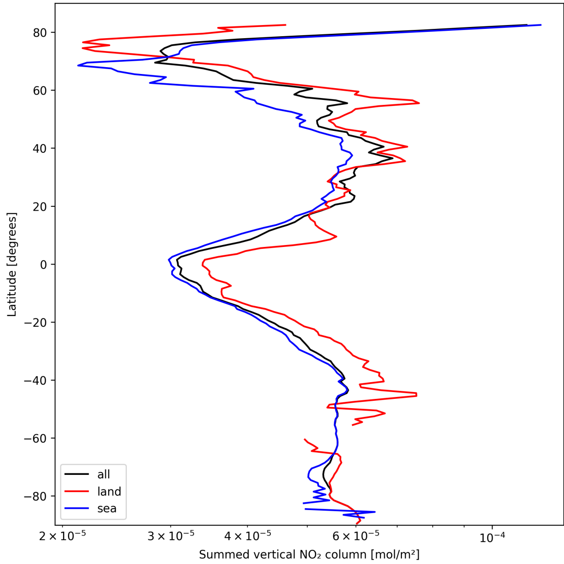
Figure 21: Zonal average of “Summed vertical NO 2 column” for 2025-03-06 to 2025-03-07.
