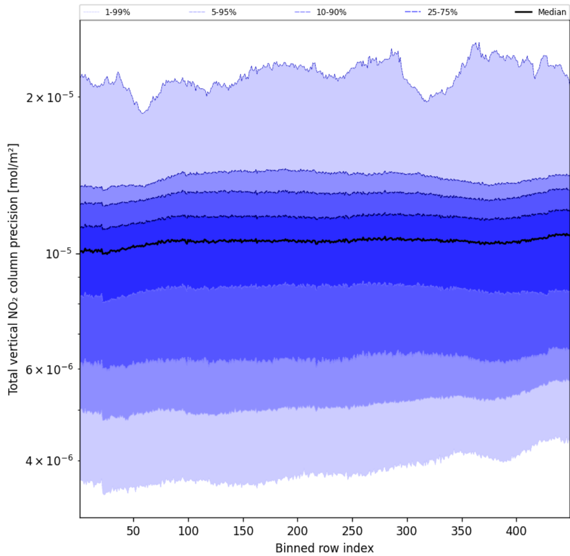
Figure 54: Along track statistics of “Total vertical NO 2 column precision” for 2025-03-06 to 2025-03-07
