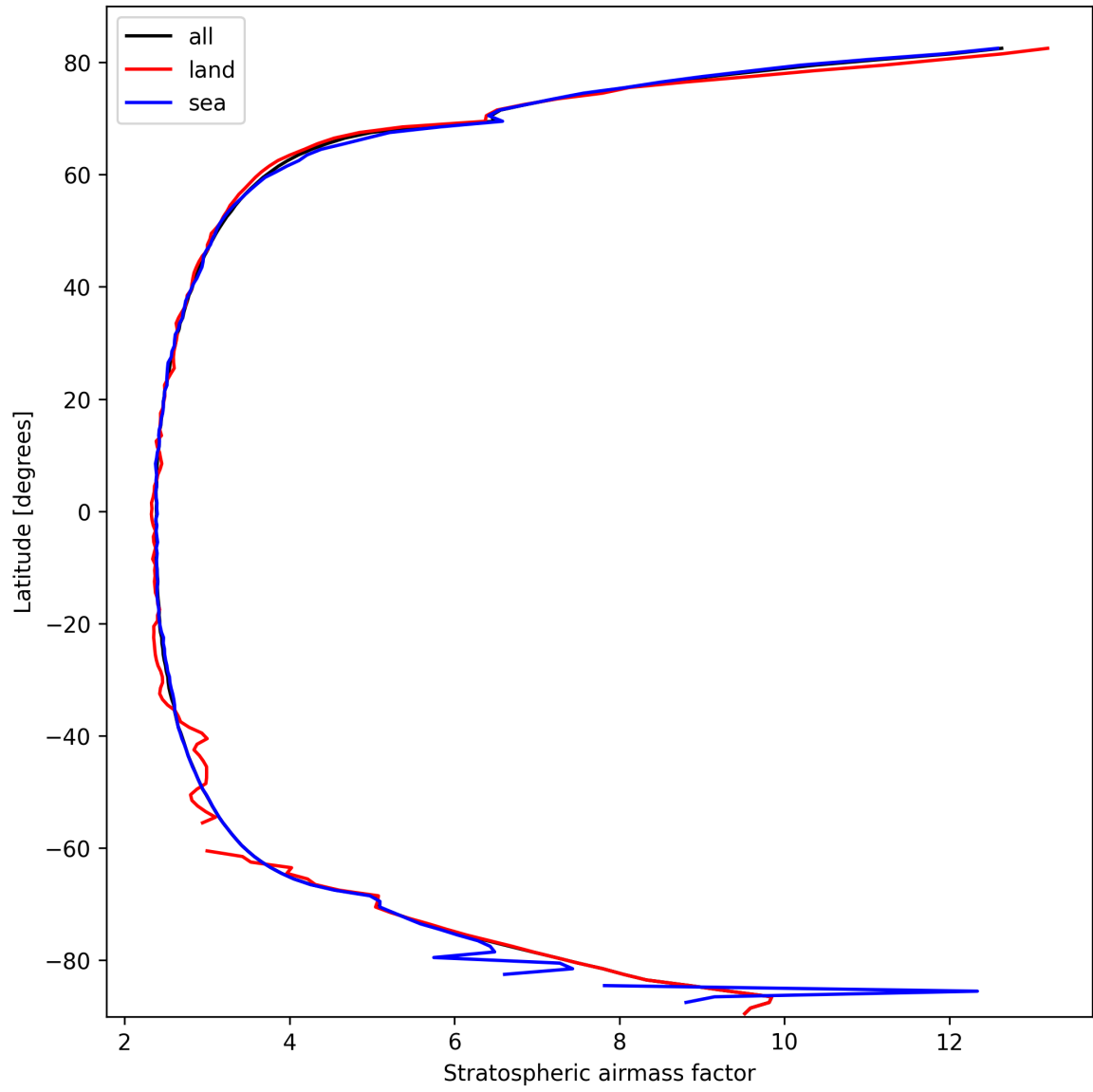
Figure 25: Zonal average of “Stratospheric air mass factor” for 2025-03-06 to 2025-03-07.
