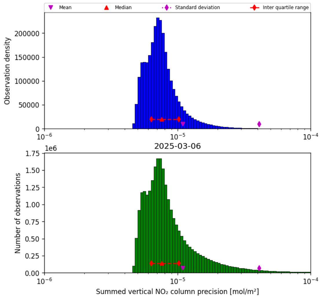
Figure 39: Histogram of “Summed vertical NO 2 column precision” for 2025-03-06 to 2025-03-07
