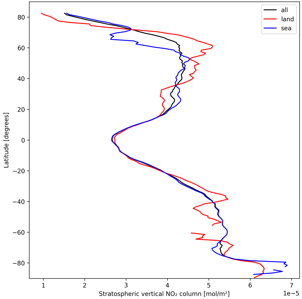
Figure 17: Zonal average of “Stratospheric vertical NO 2 column” for 2025-03-06 to 2025-03-07.
