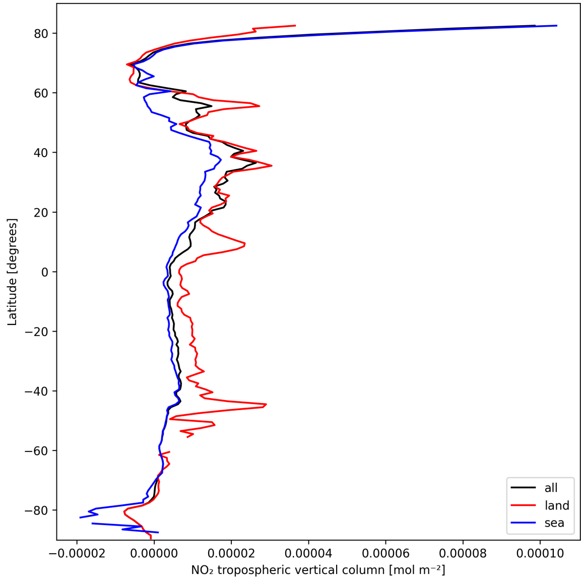
Figure 10: Zonal average of “NO 2 tropospheric vertical column” for 2025-03-06 to 2025-03-07.
