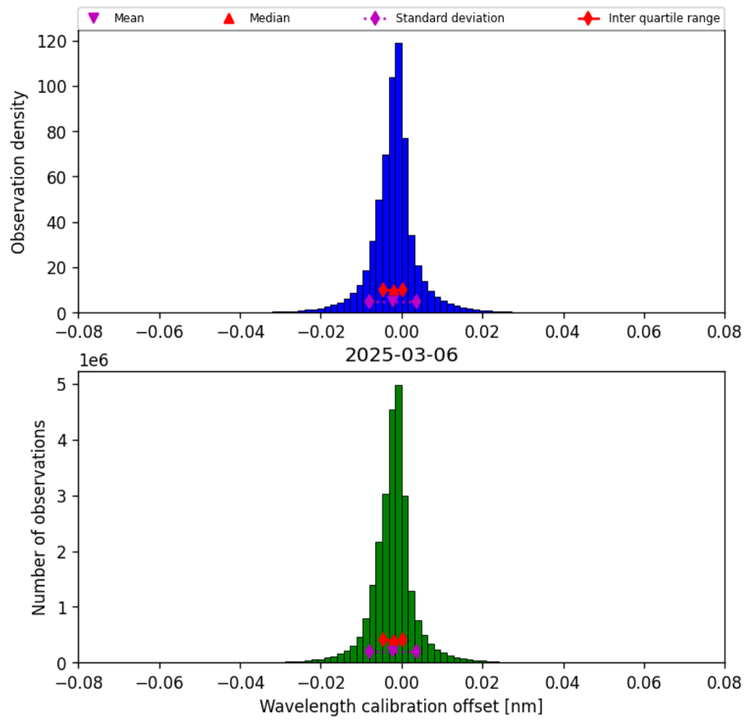
Figure 33: Histogram of “Wavelength calibration offset” for 2025-03-06 to 2025-03-07
