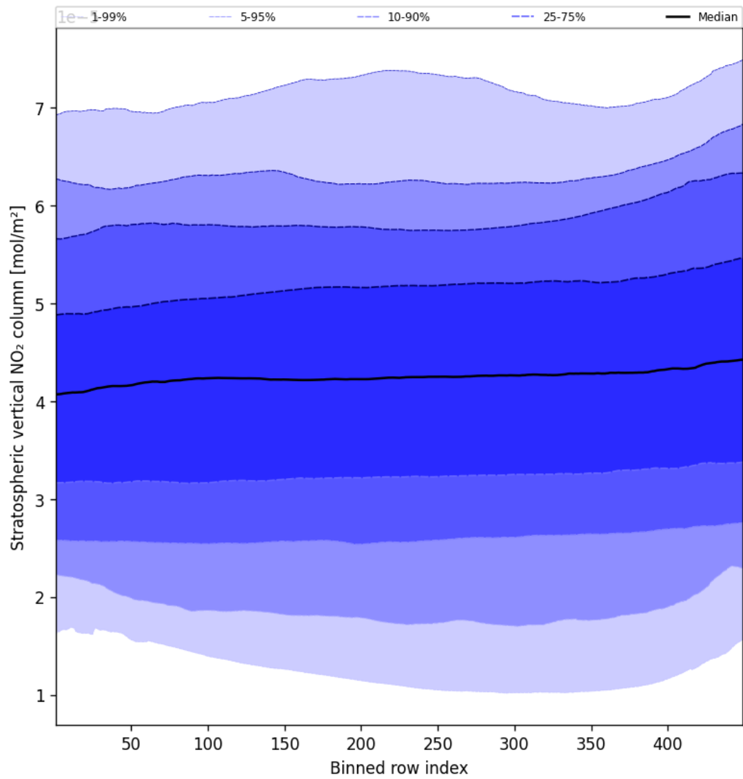
Figure 51: Along track statistics of “Stratospheric vertical NO 2 column” for 2025-03-06 to 2025-03-07
