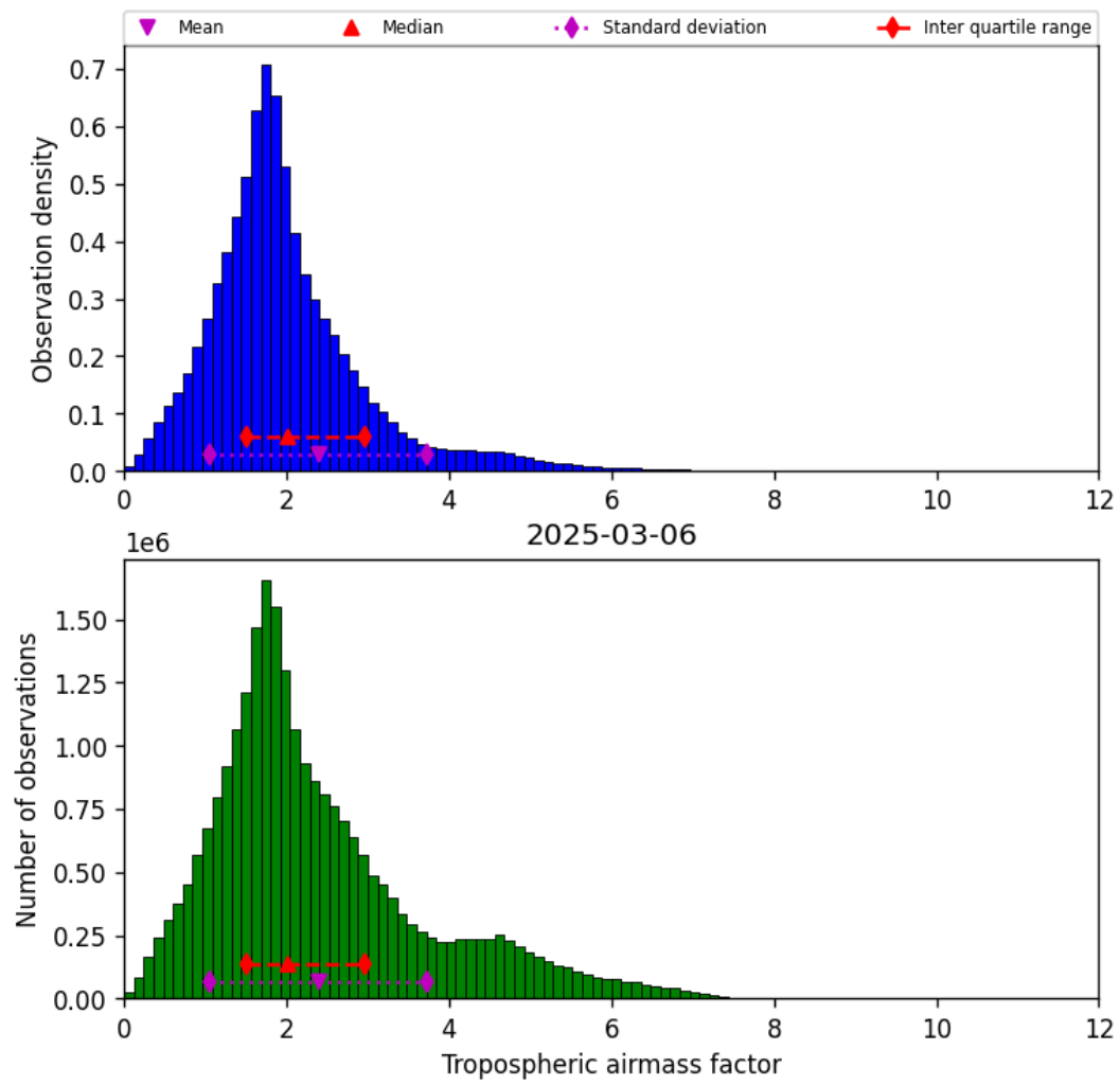
Figure 29: Histogram of “Tropospheric airmass factor” for 2025-03-06 to 2025-03-07
