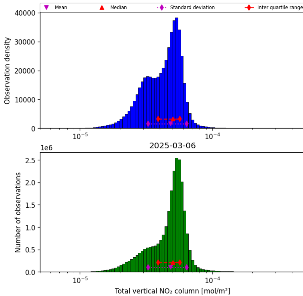
Figure 36: Histogram of “Total vertical NO 2 column” for 2025-03-06 to 2025-03-07
