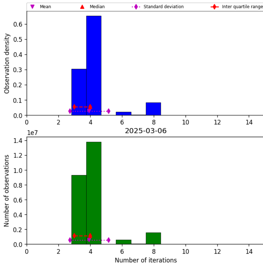
Figure 32: Histogram of “Number of iterations” for 2025-03-06 to 2025-03-07
