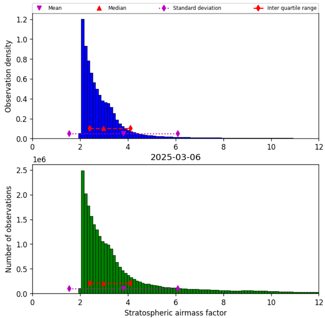
Figure 42: Histogram of “Stratospheric airmass factor” for 2025-03-06 to 2025-03-07
