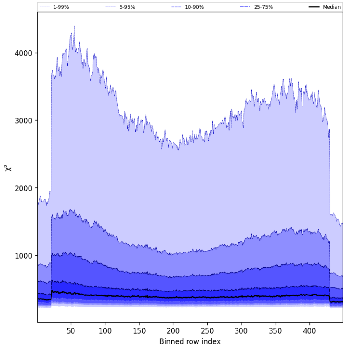
Figure 57: Along track statistics of “ \chi^2 ” for 2025-03-06 to 2025-03-07
