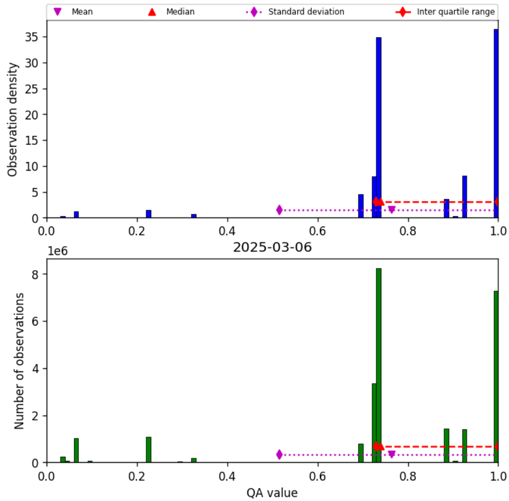
Figure 26: Histogram of “QA value” for 2025-03-06 to 2025-03-07
