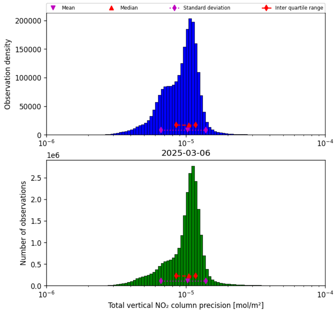
Figure 37: Histogram of "Total vertical NO 2 column precision" for 2025-03-06 to 2025-03-07
