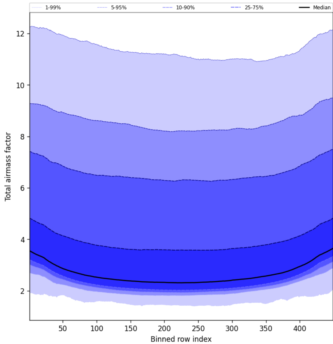
Figure 47: Along track statistics of “Total airmass factor” for 2025-03-06 to 2025-03-07
