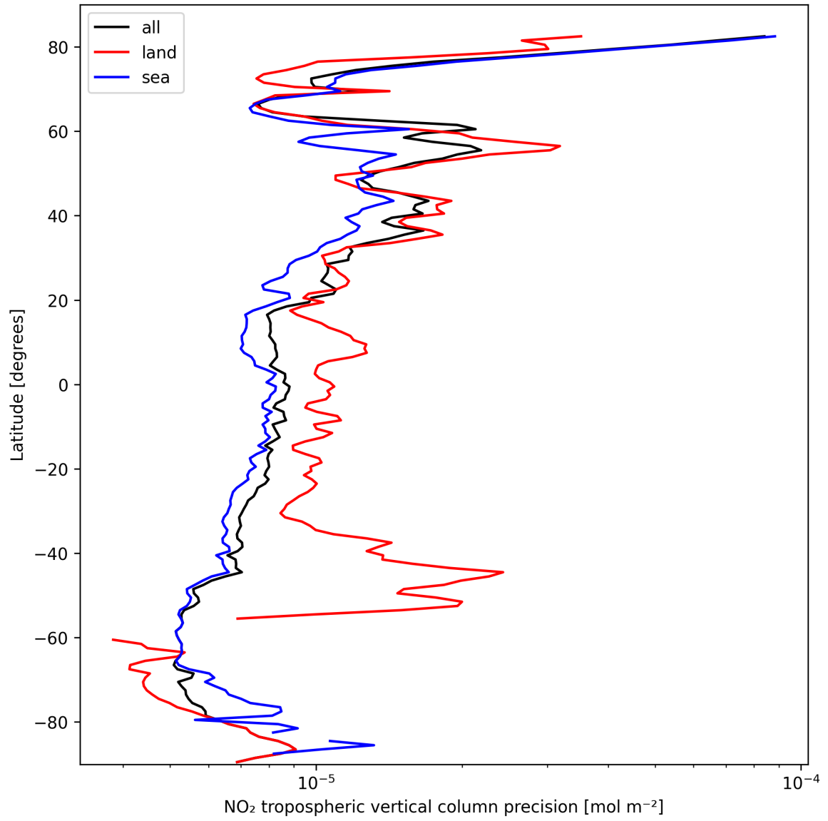
Figure 11: Zonal average of “NO 2 tropospheric vertical column precision” for 2025-03-06 to 2025-03-07.
