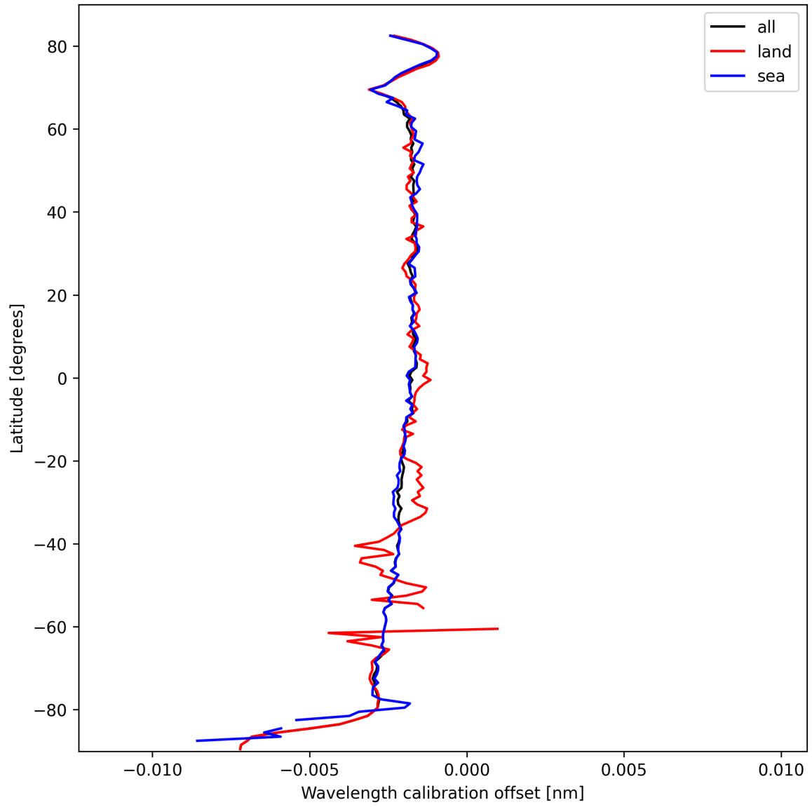
Figure 16: Zonal average of “Wavelength calibration offset” for 2025-03-06 to 2025-03-07.
