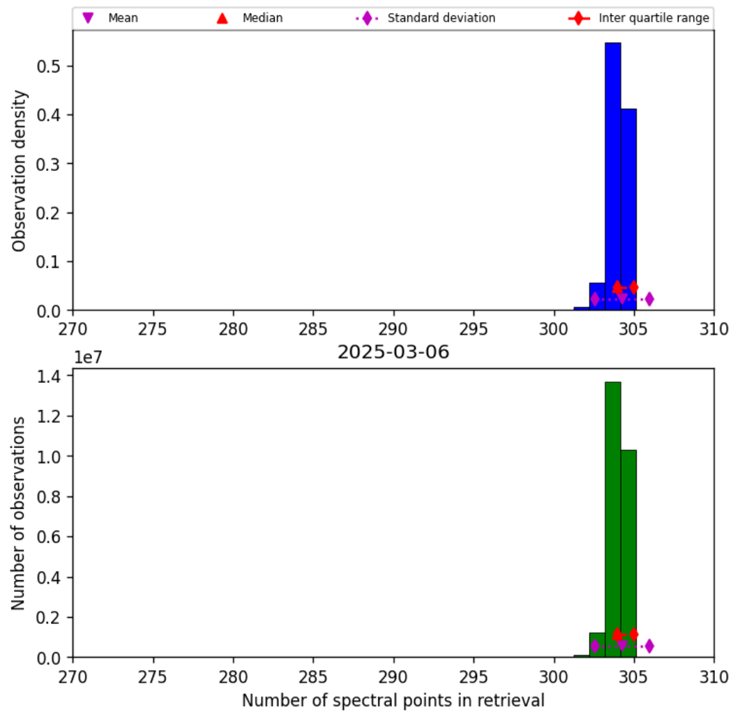
Figure 31: Histogram of “Number of spectral points in retrieval” for 2025-03-06 to 2025-03-07
