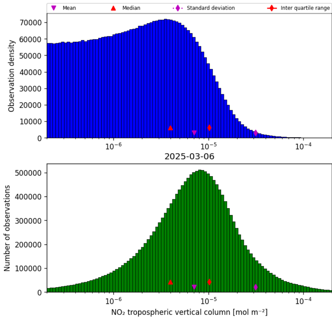
Figure 27: Histogram of “NO 2 tropospheric vertical column” for 2025-03-06 to 2025-03-07
