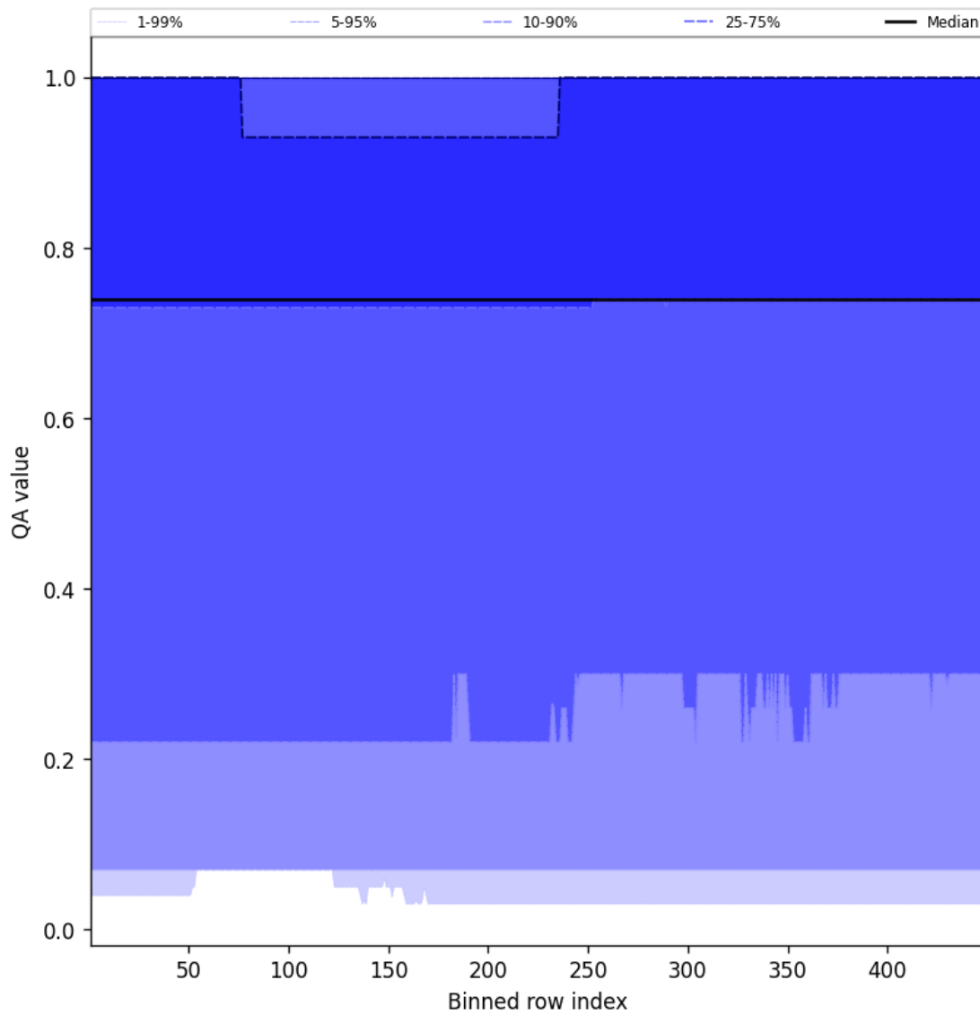
Figure 43: Along track statistics of “QA value” for 2025-03-06 to 2025-03-07
