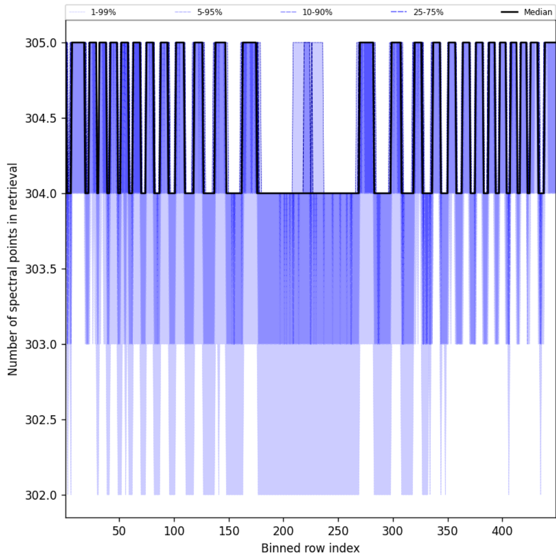
Figure 48: Along track statistics of “Number of spectral points in retrieval” for 2025-03-06 to 2025-03-07
