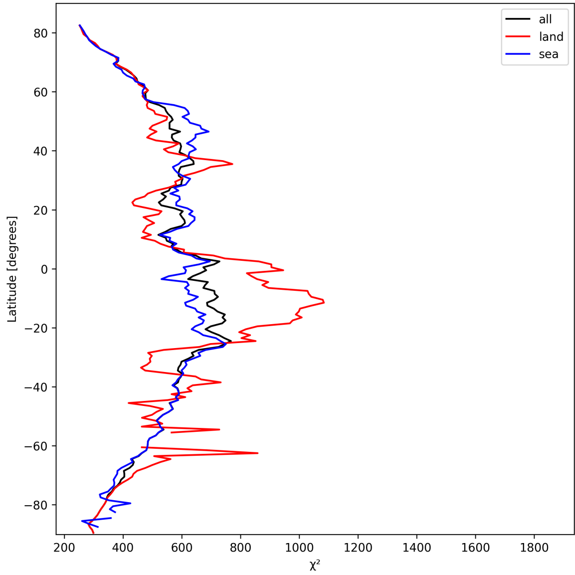
Figure 23: Zonal average of “ \chi^2 ” for 2025-03-06 to 2025-03-07.
