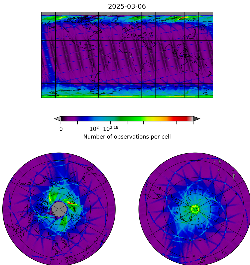
Figure 8: Map of the number of observations for 2025-03-06 to 2025-03-07
