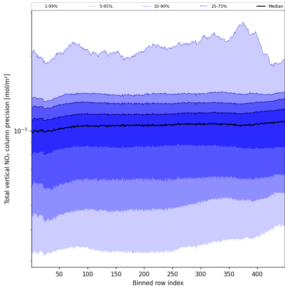
Figure 54: Along track statistics of “Total vertical NO 2 column precision” for 2025-03-07 to 2025-03-08
