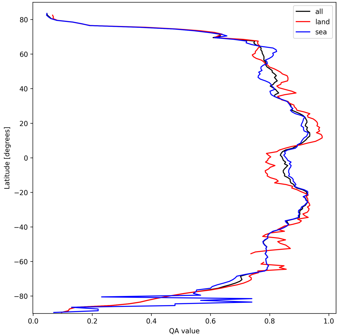
Figure 9: Zonal average of “QA value” for 2025-03-07 to 2025-03-08.
