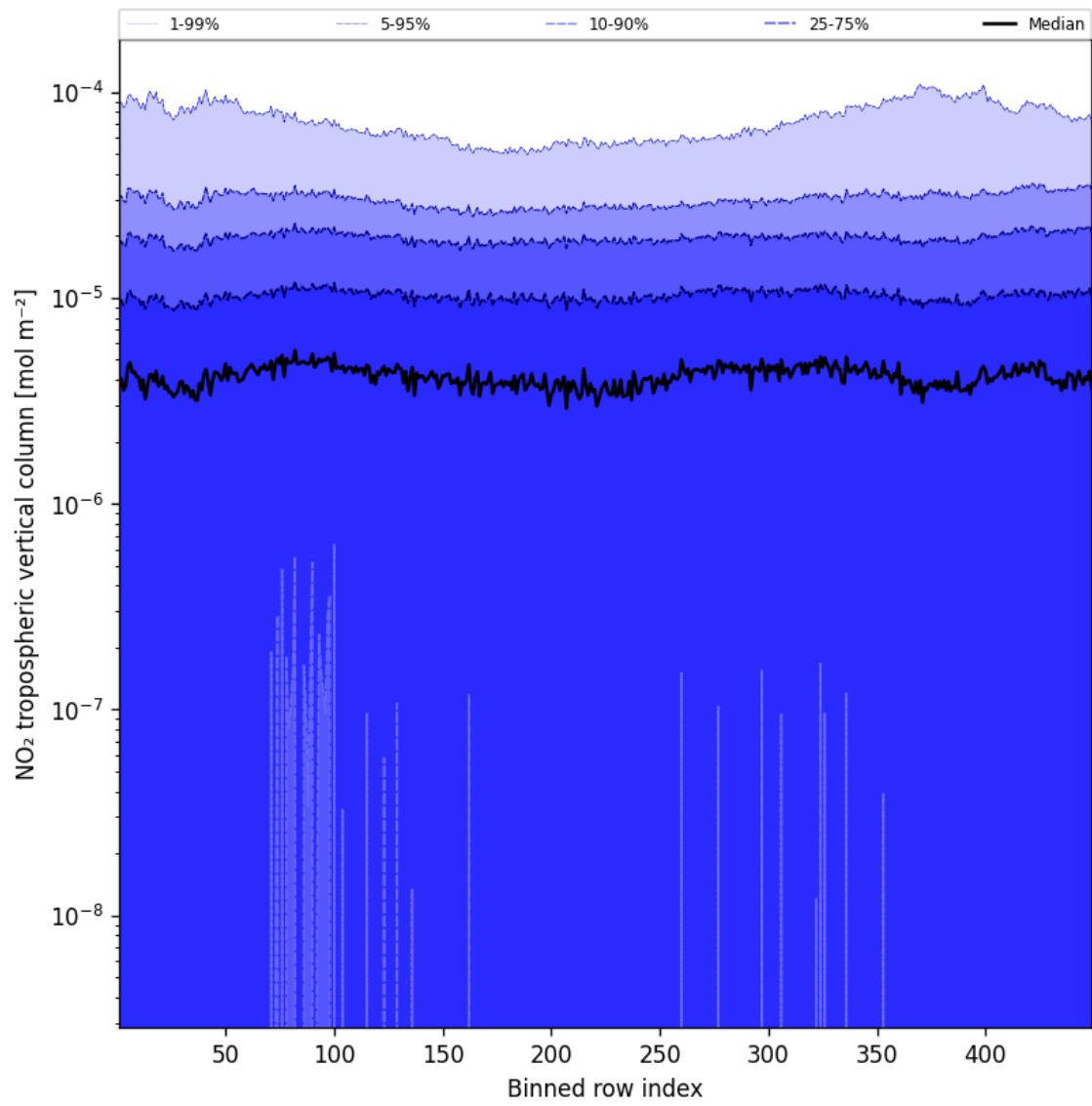
Figure 44: Along track statistics of “NO 2 tropospheric vertical column” for 2025-03-07 to 2025-03-08
