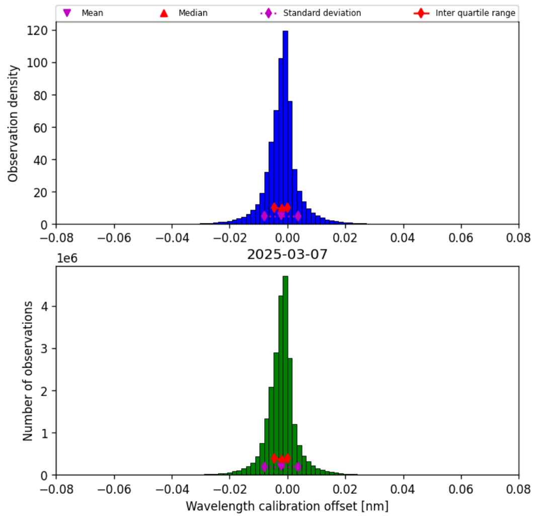
Figure 33: Histogram of “Wavelength calibration offset” for 2025-03-07 to 2025-03-08
