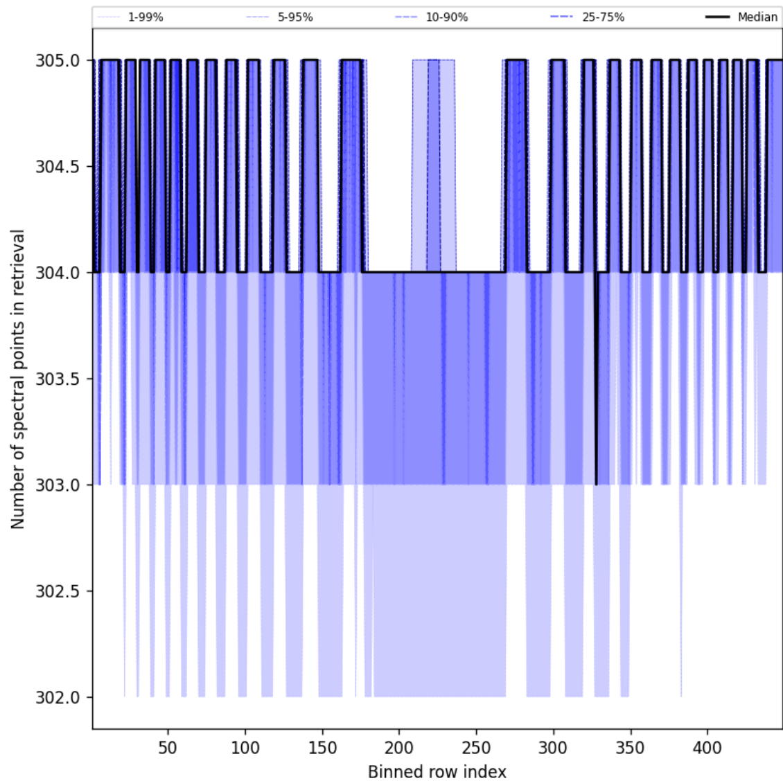
Figure 48: Along track statistics of “Number of spectral points in retrieval” for 2025-03-07 to 2025-03-08
