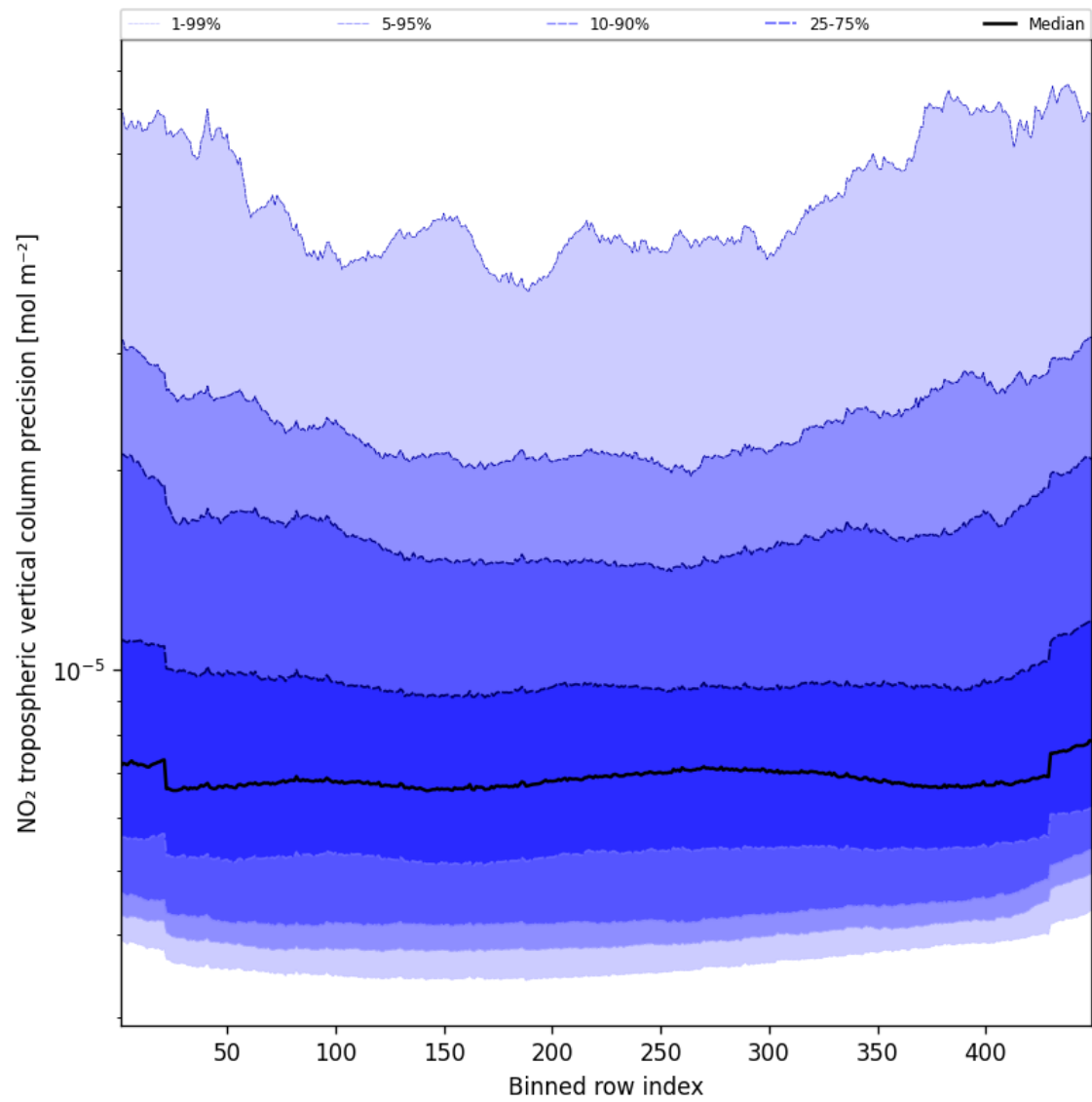
Figure 45: Along track statistics of “NO 2 tropospheric vertical column precision” for 2025-03-07 to 2025-03-08
