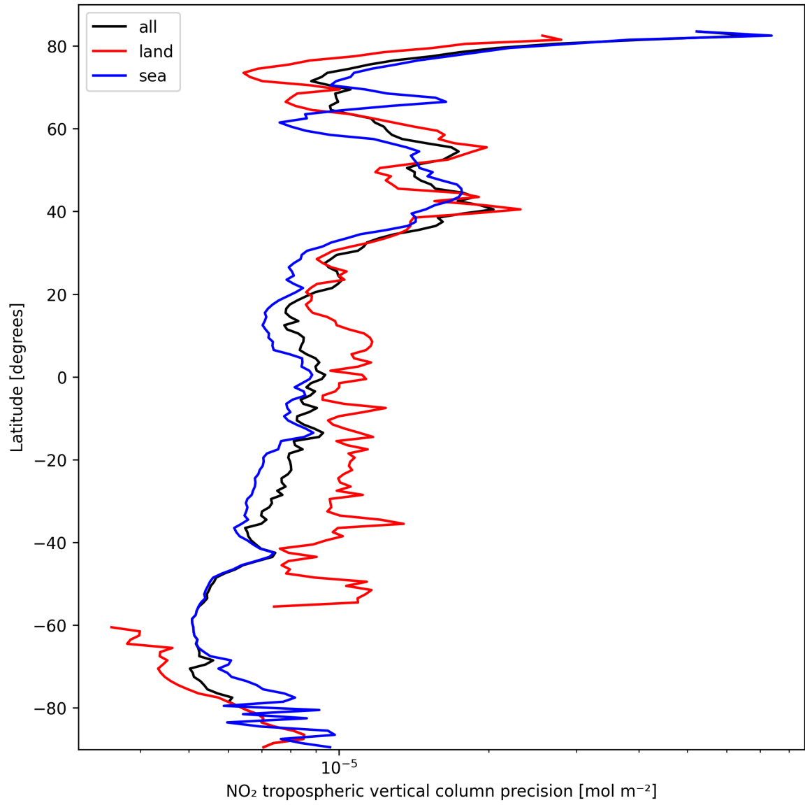
Figure 11: Zonal average of “NO 2 tropospheric vertical column precision” for 2025-03-07 to 2025-03-08.
