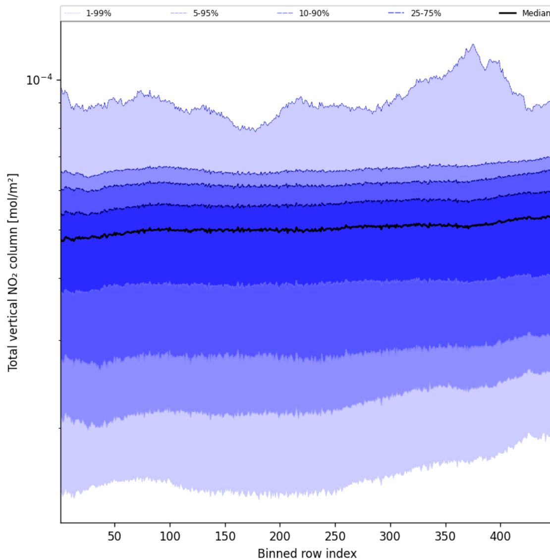
Figure 53: Along track statistics of “Total vertical NO 2 column” for 2025-03-07 to 2025-03-08
