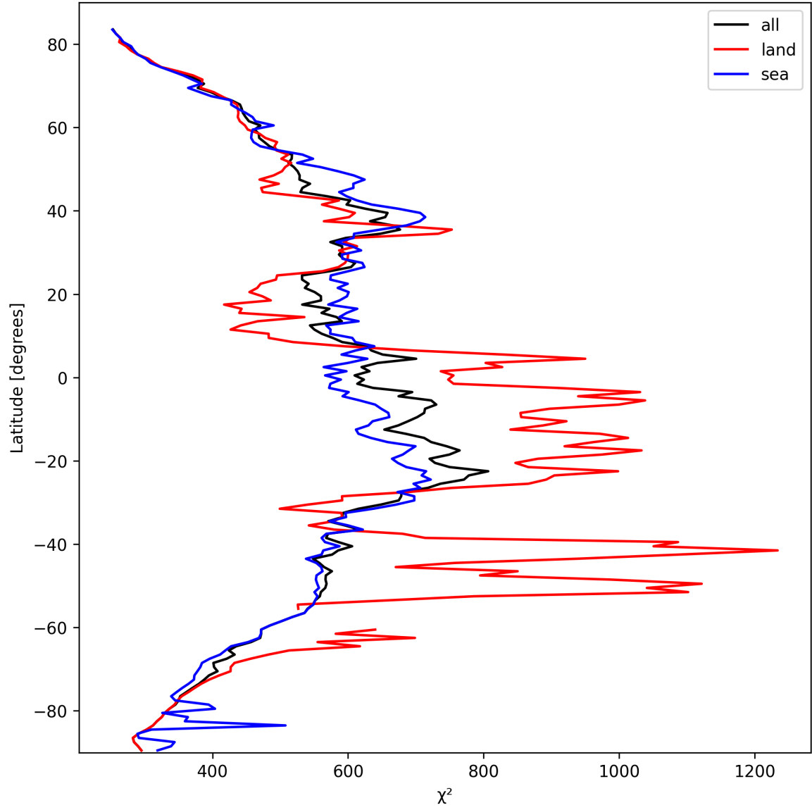
Figure 23: Zonal average of “ \chi^2 ” for 2025-03-07 to 2025-03-08.
