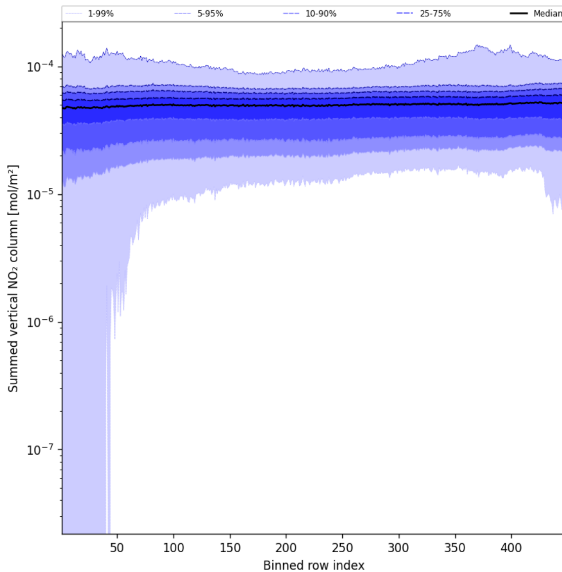
Figure 55: Along track statistics of “Summed vertical NO 2 column” for 2025-03-07 to 2025-03-08
