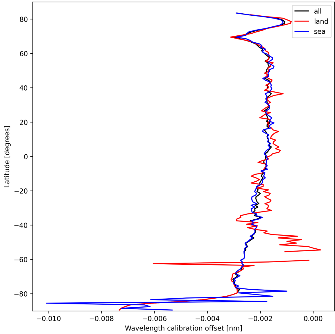
Figure 16: Zonal average of “Wavelength calibration offset” for 2025-03-07 to 2025-03-08.
