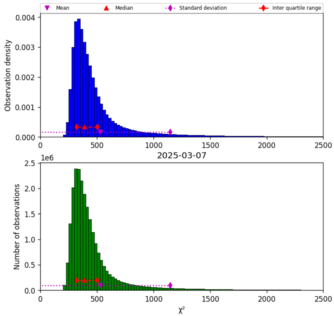
Figure 40: Histogram of “ \chi^2 ” for 2025-03-07 to 2025-03-08
