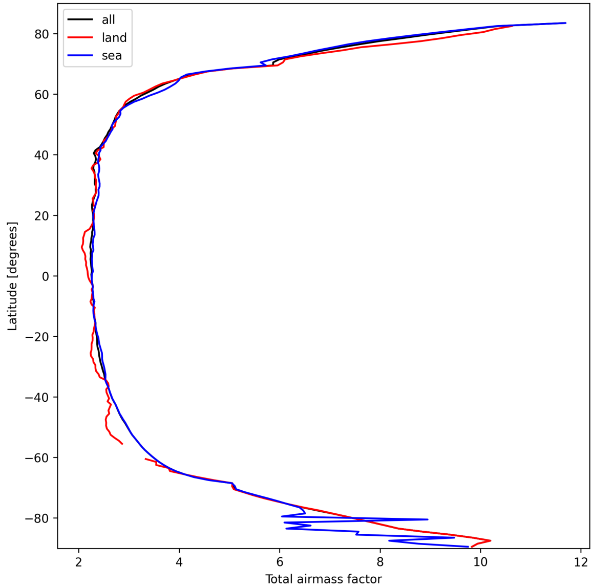
Figure 13: Zonal average of “Total airmass factor” for 2025-03-07 to 2025-03-08.
