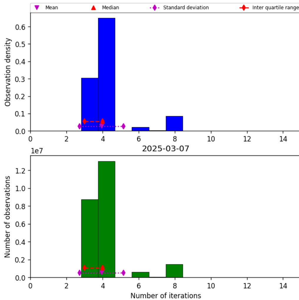
Figure 32: Histogram of “Number of iterations” for 2025-03-07 to 2025-03-08
