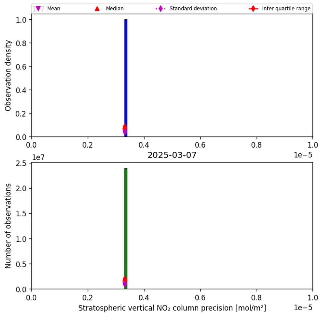
Figure 35: Histogram of “Stratospheric vertical NO 2 column precision” for 2025-03-07 to 2025-03-08
