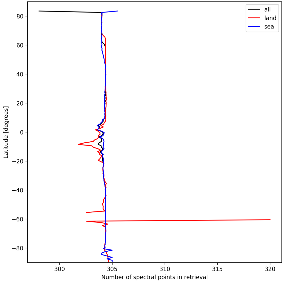
Figure 14: Zonal average of “Number of spectral points in retrieval” for 2025-03-07 to 2025-03-08.
