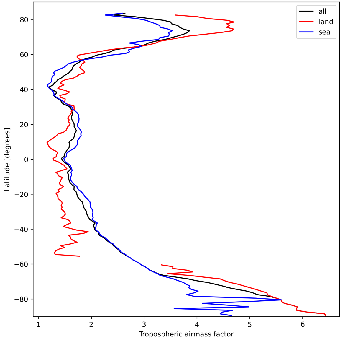
Figure 12: Zonal average of “Tropospheric air mass factor” for 2025-03-07 to 2025-03-08.
