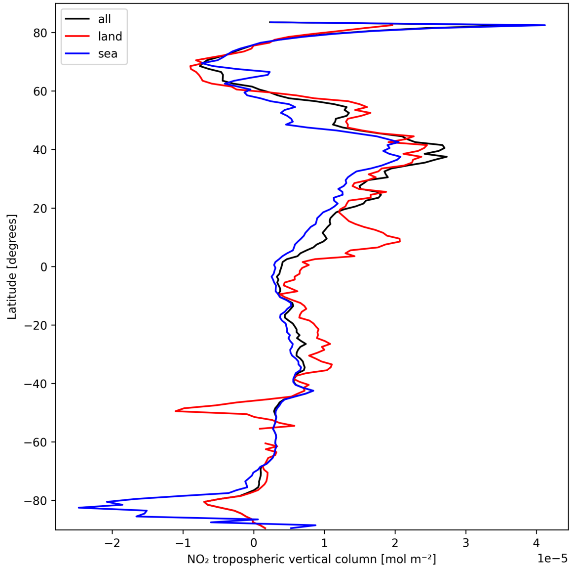
Figure 10: Zonal average of “NO 2 tropospheric vertical column” for 2025-03-07 to 2025-03-08.
