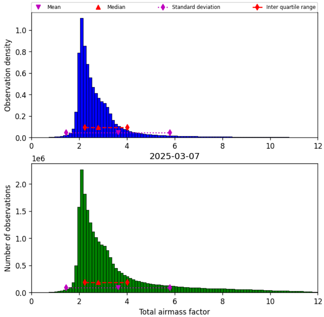
Figure 30: Histogram of “Total airmass factor” for 2025-03-07 to 2025-03-08
