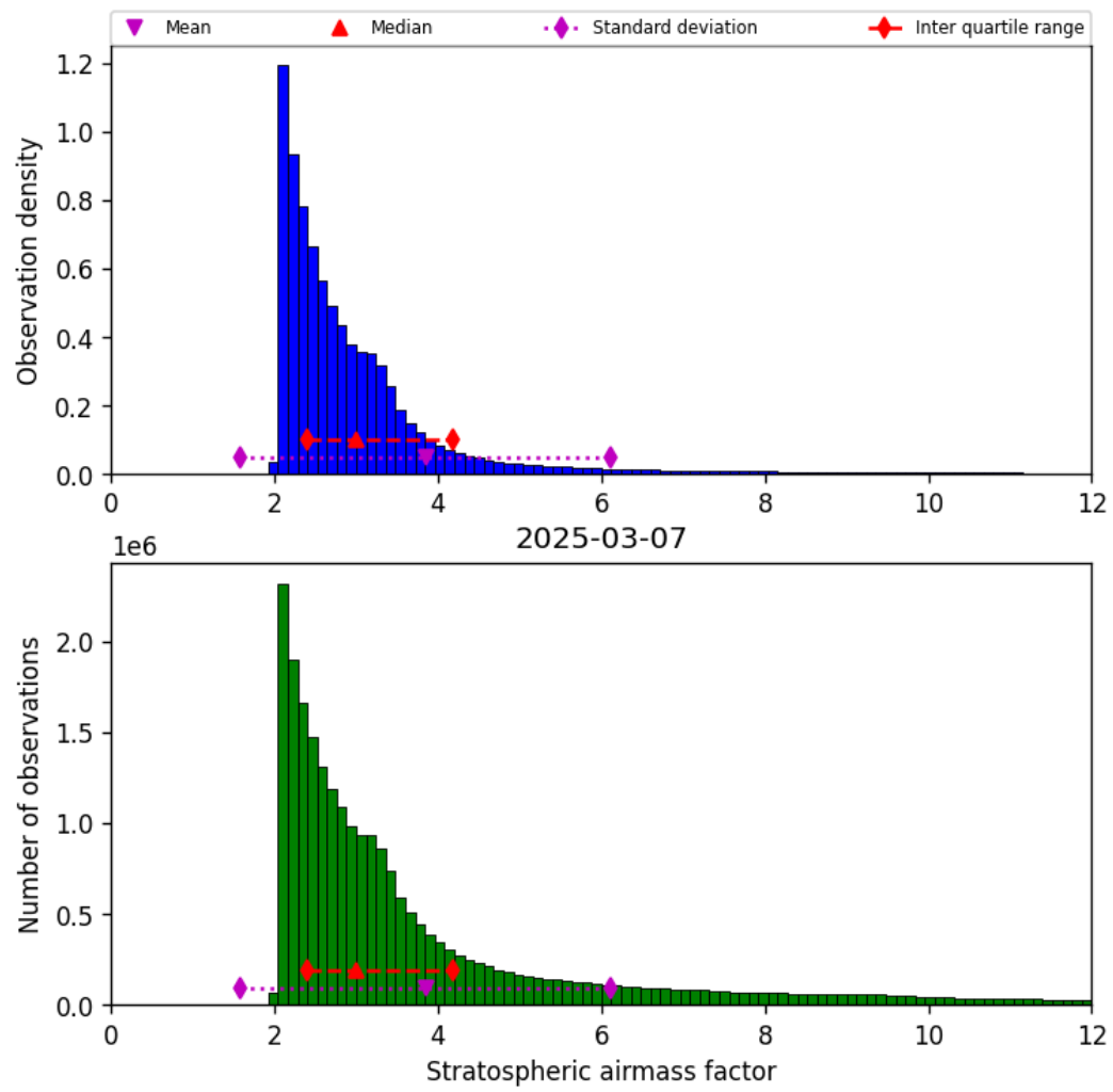
Figure 42: Histogram of “Stratospheric airmass factor” for 2025-03-07 to 2025-03-08
