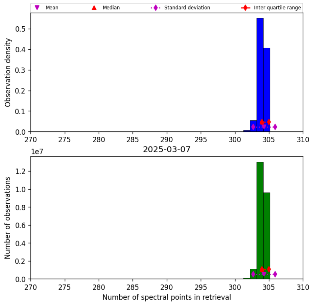
Figure 31: Histogram of “Number of spectral points in retrieval” for 2025-03-07 to 2025-03-08
