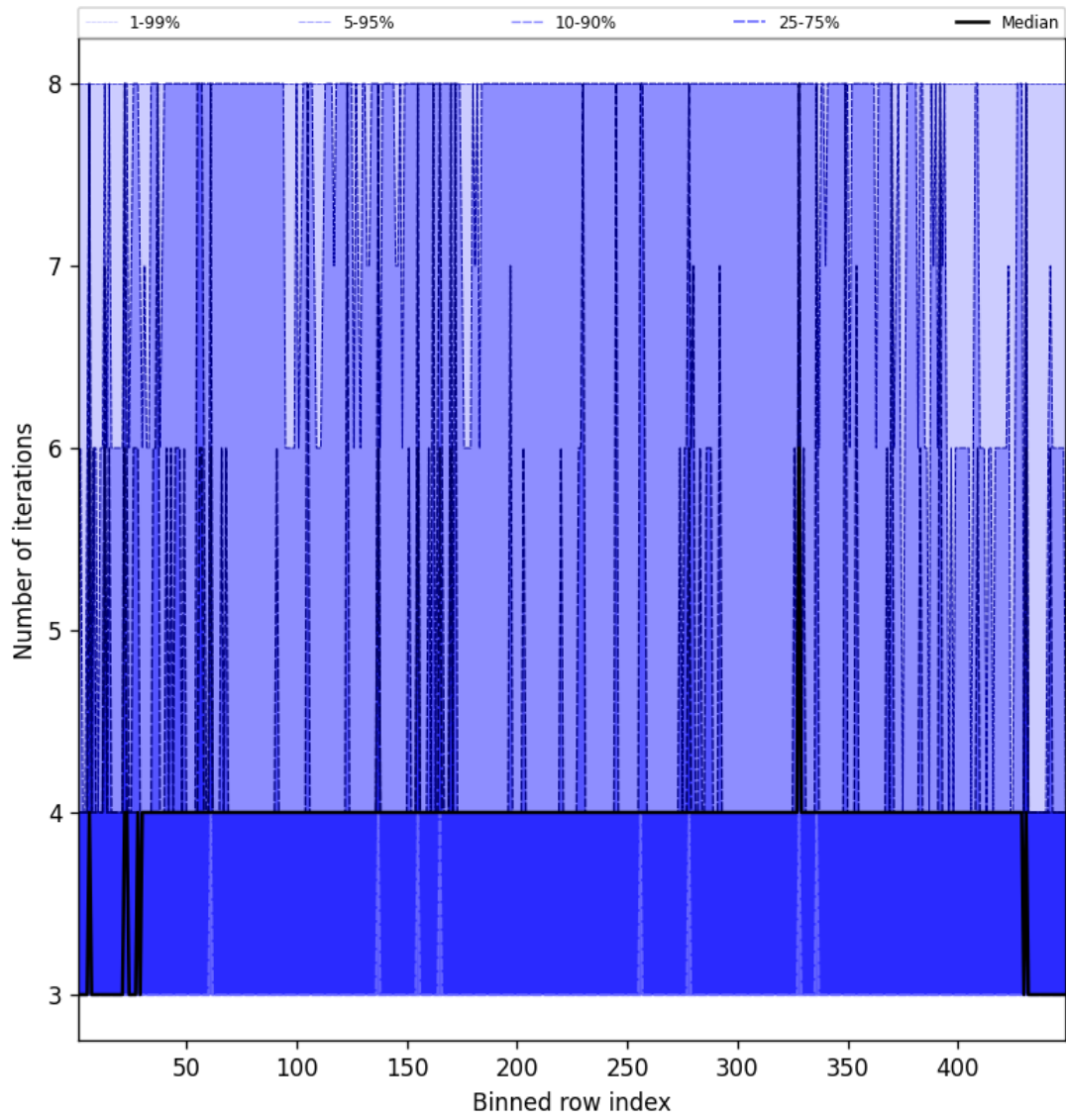
Figure 49: Along track statistics of “Number of iterations” for 2025-03-07 to 2025-03-08
