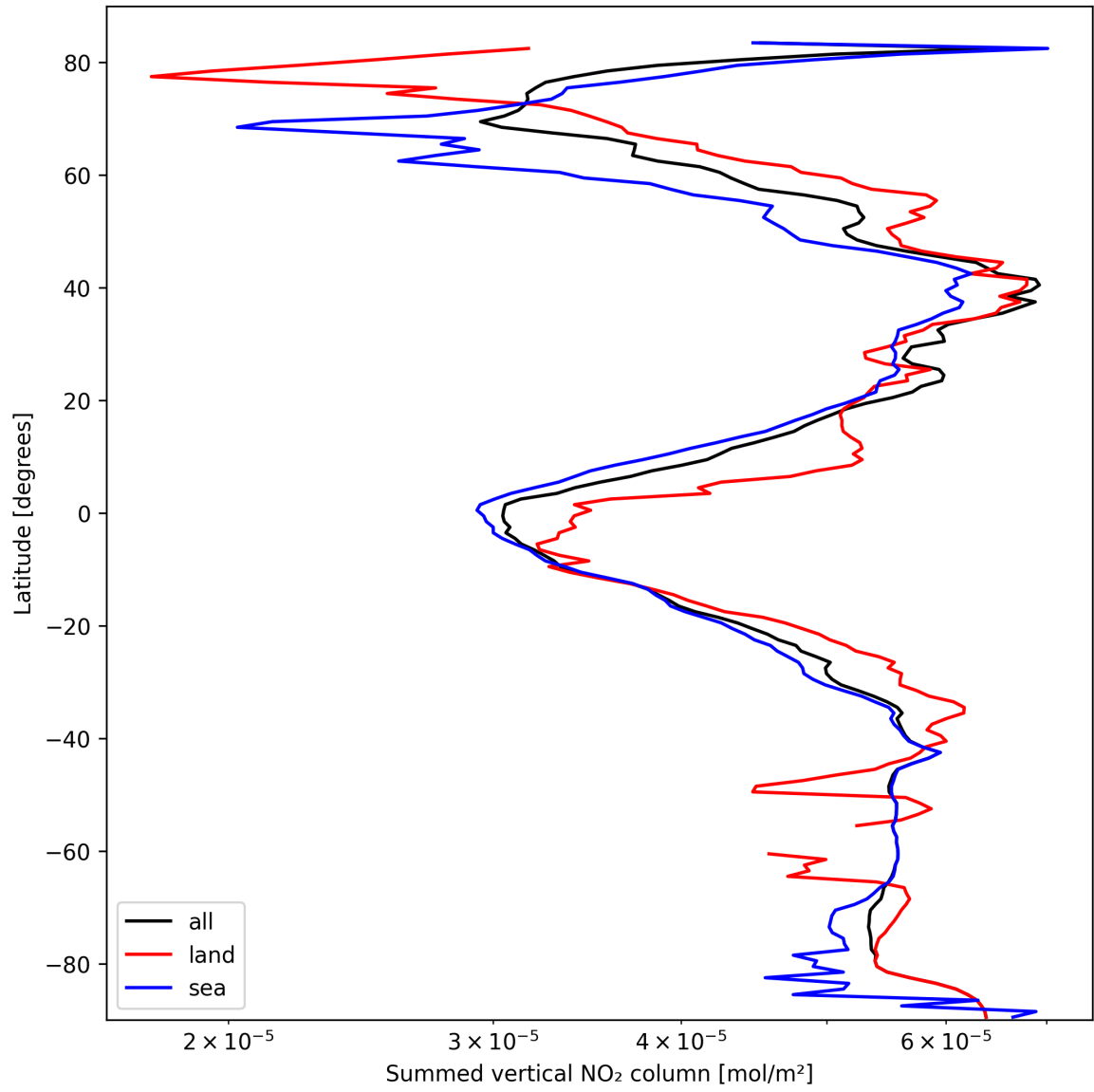
Figure 21: Zonal average of “Summed vertical NO 2 column” for 2025-03-07 to 2025-03-08.
