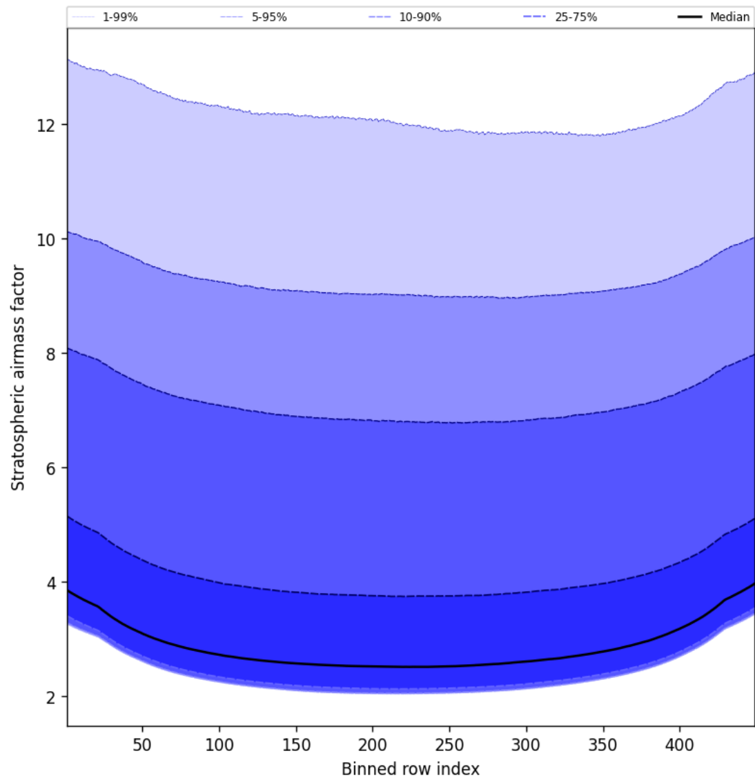
Figure 59: Along track statistics of “Stratospheric airmass factor” for 2025-03-07 to 2025-03-08
