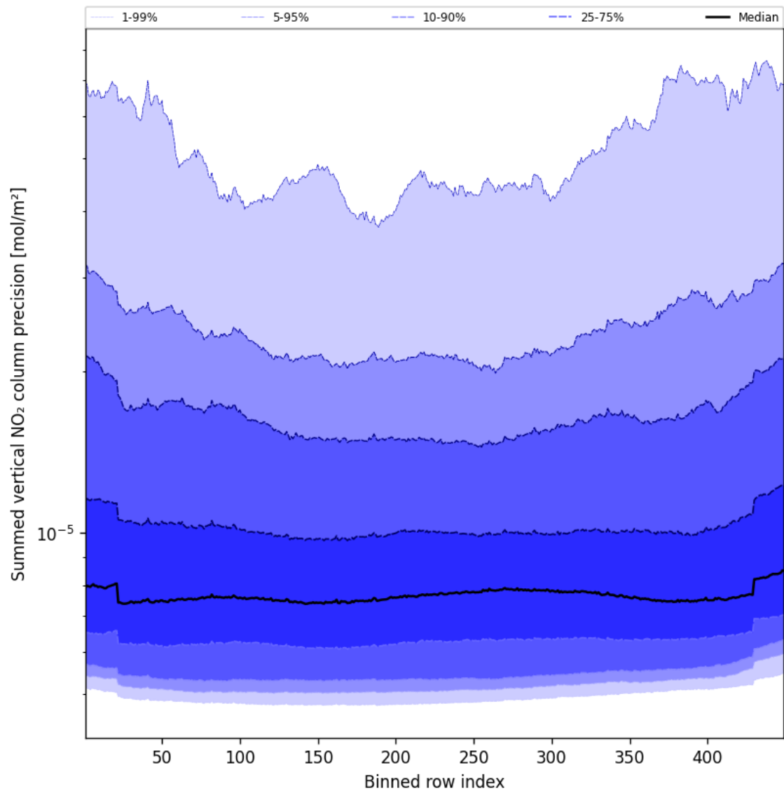
Figure 56: Along track statistics of “Summed vertical NO 2 column precision” for 2025-03-07 to 2025-03-08
