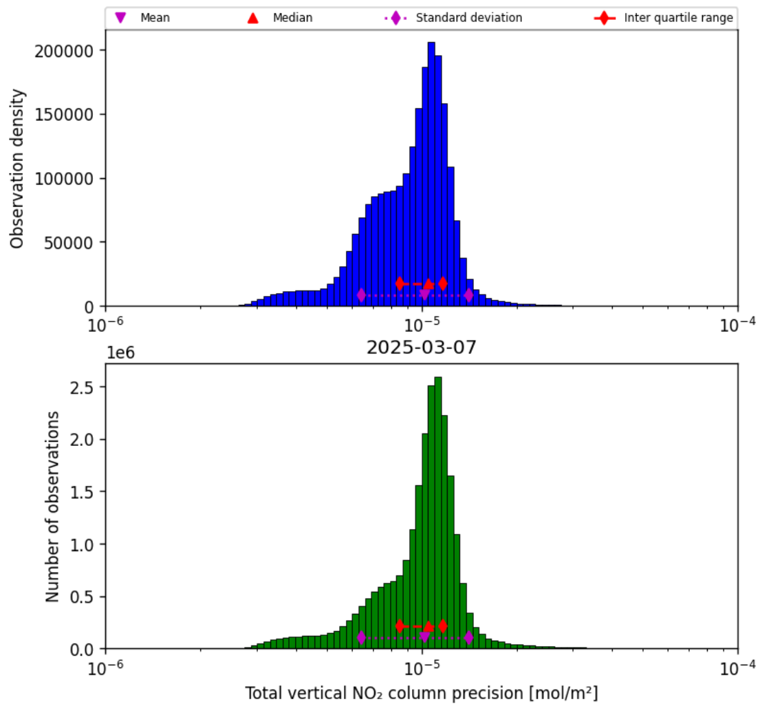
Figure 37: Histogram of "Total vertical NO 2 column precision" for 2025-03-07 to 2025-03-08
