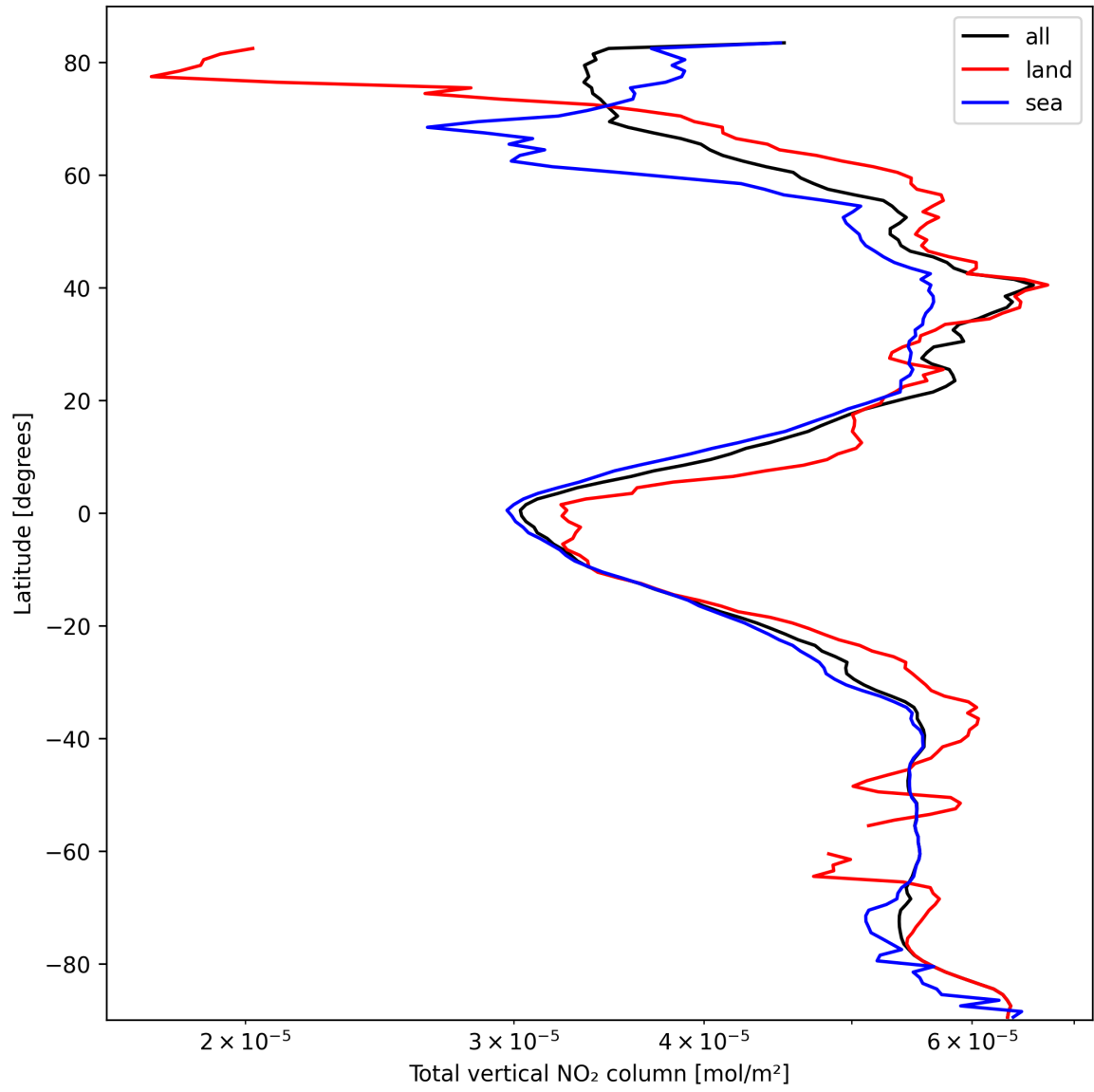
Figure 19: Zonal average of “Total vertical NO 2 column” for 2025-03-07 to 2025-03-08.
