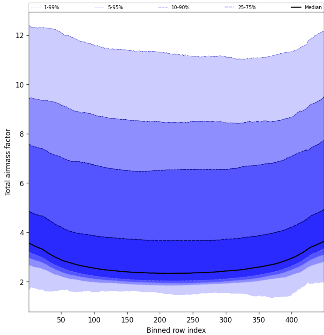
Figure 47: Along track statistics of “Total airmass factor” for 2025-03-07 to 2025-03-08
