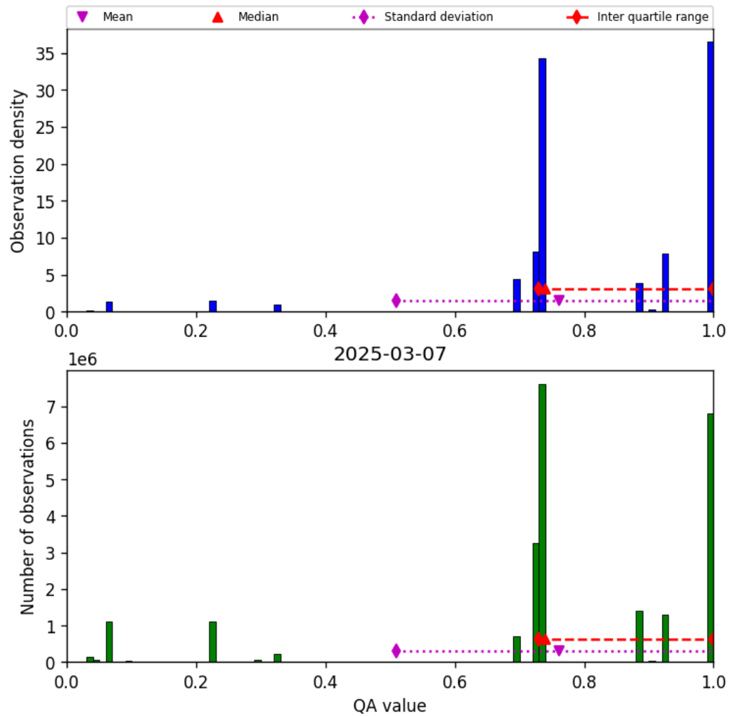
Figure 26: Histogram of “QA value” for 2025-03-07 to 2025-03-08
