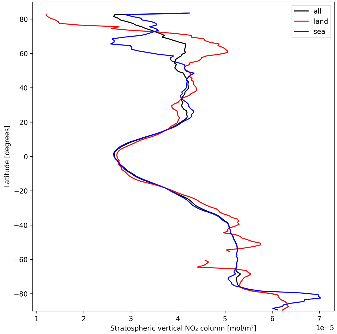
Figure 17: Zonal average of “Stratospheric vertical NO 2 column” for 2025-03-07 to 2025-03-08.
