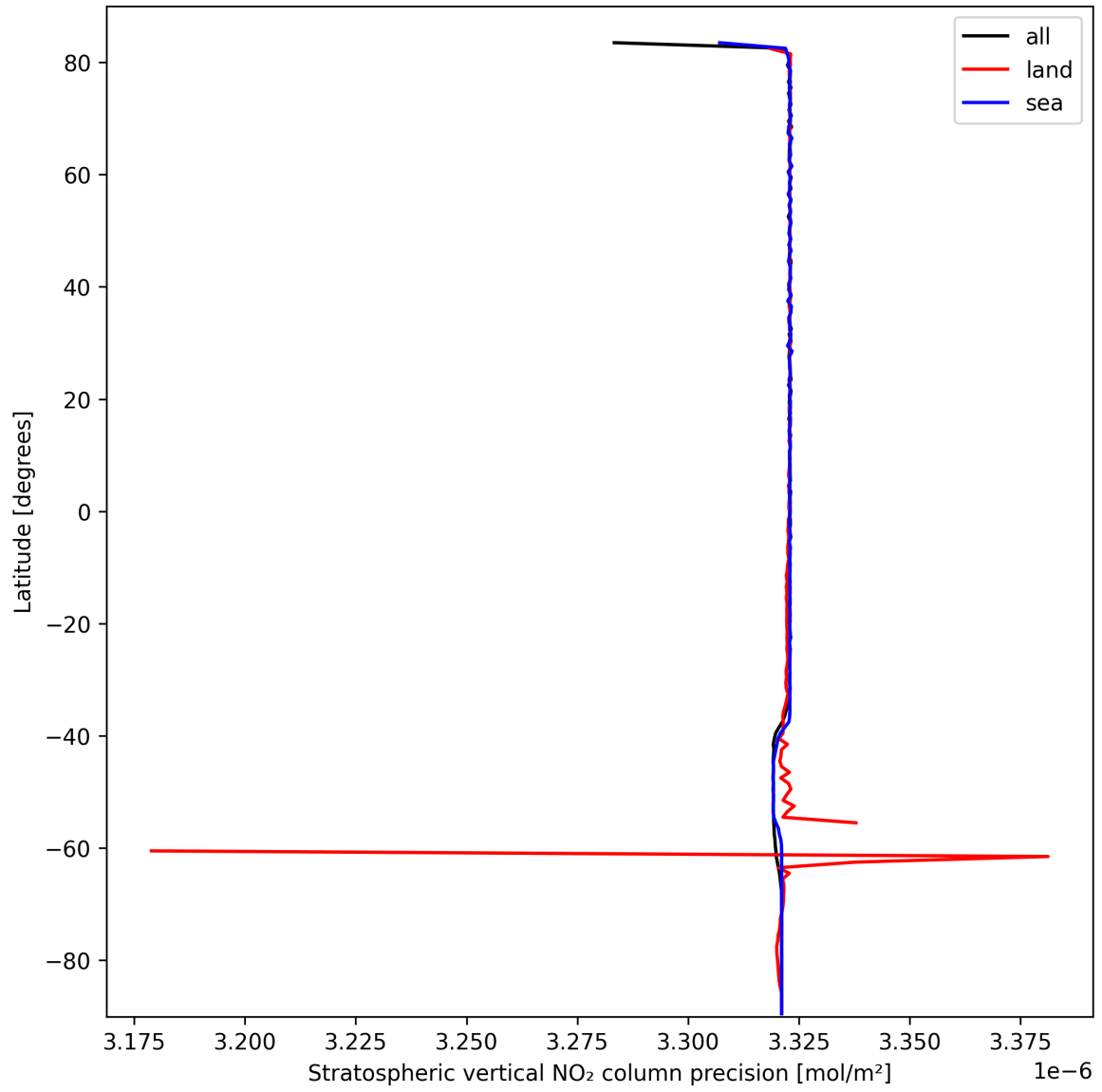
Figure 18: Zonal average of “Stratospheric vertical NO 2 column precision” for 2025-03-07 to 2025-03-08.
