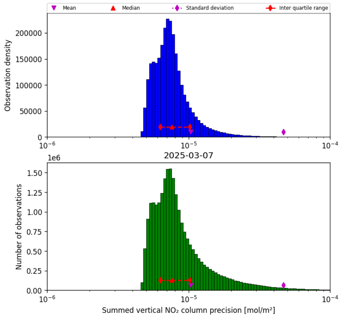
Figure 39: Histogram of "Summed vertical NO 2 column precision" for 2025-03-07 to 2025-03-08
