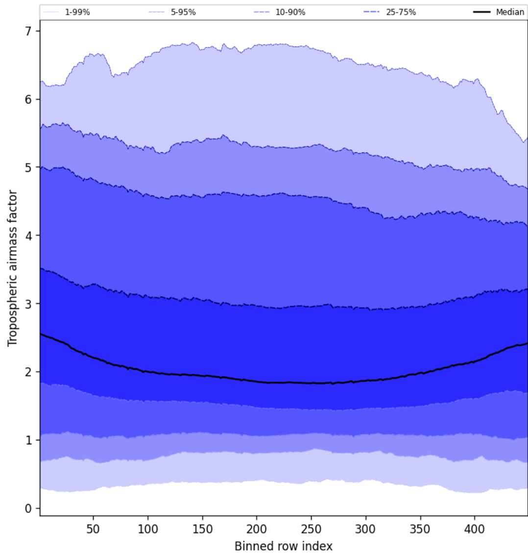
Figure 46: Along track statistics of “Tropospheric airmass factor” for 2025-03-07 to 2025-03-08
