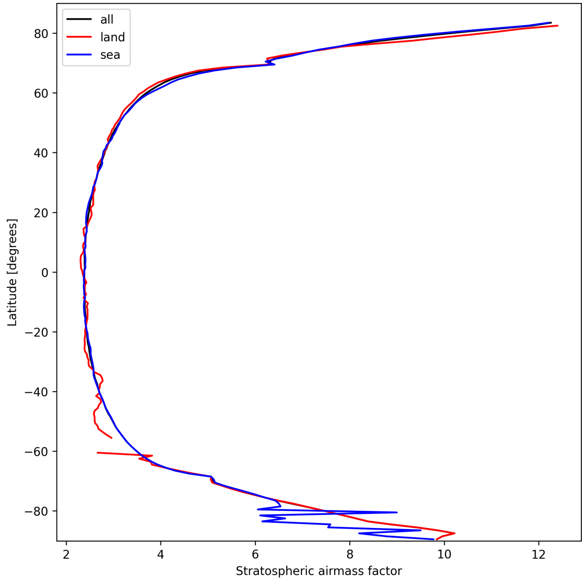
Figure 25: Zonal average of “Stratospheric airmass factor” for 2025-03-07 to 2025-03-08.
