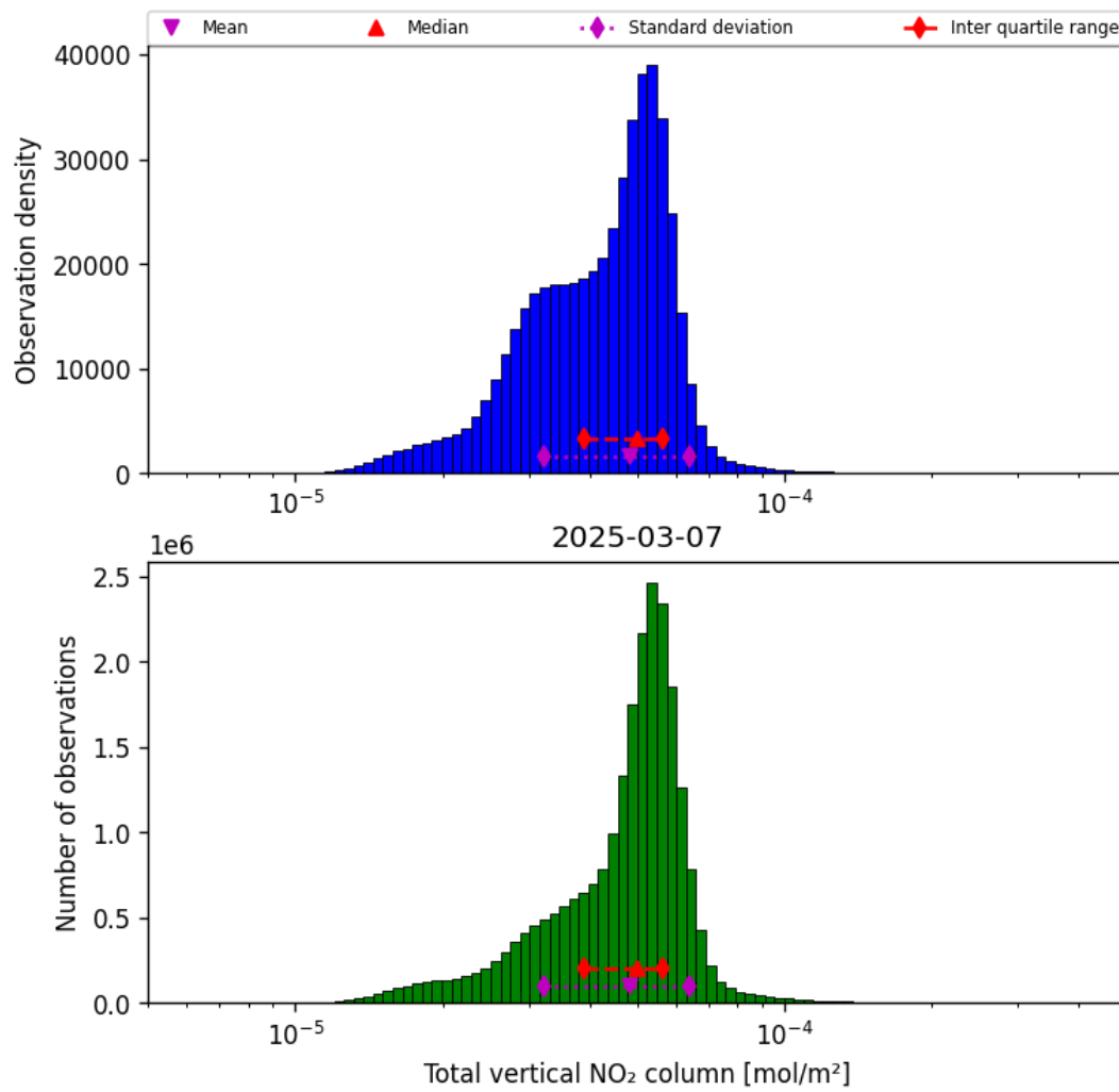
Figure 36: Histogram of “Total vertical NO 2 column” for 2025-03-07 to 2025-03-08
