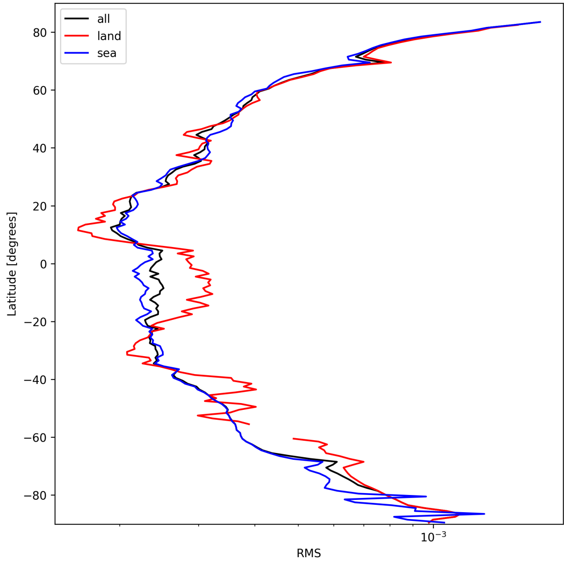
Figure 24: Zonal average of “RMS” for 2025-03-07 to 2025-03-08.
