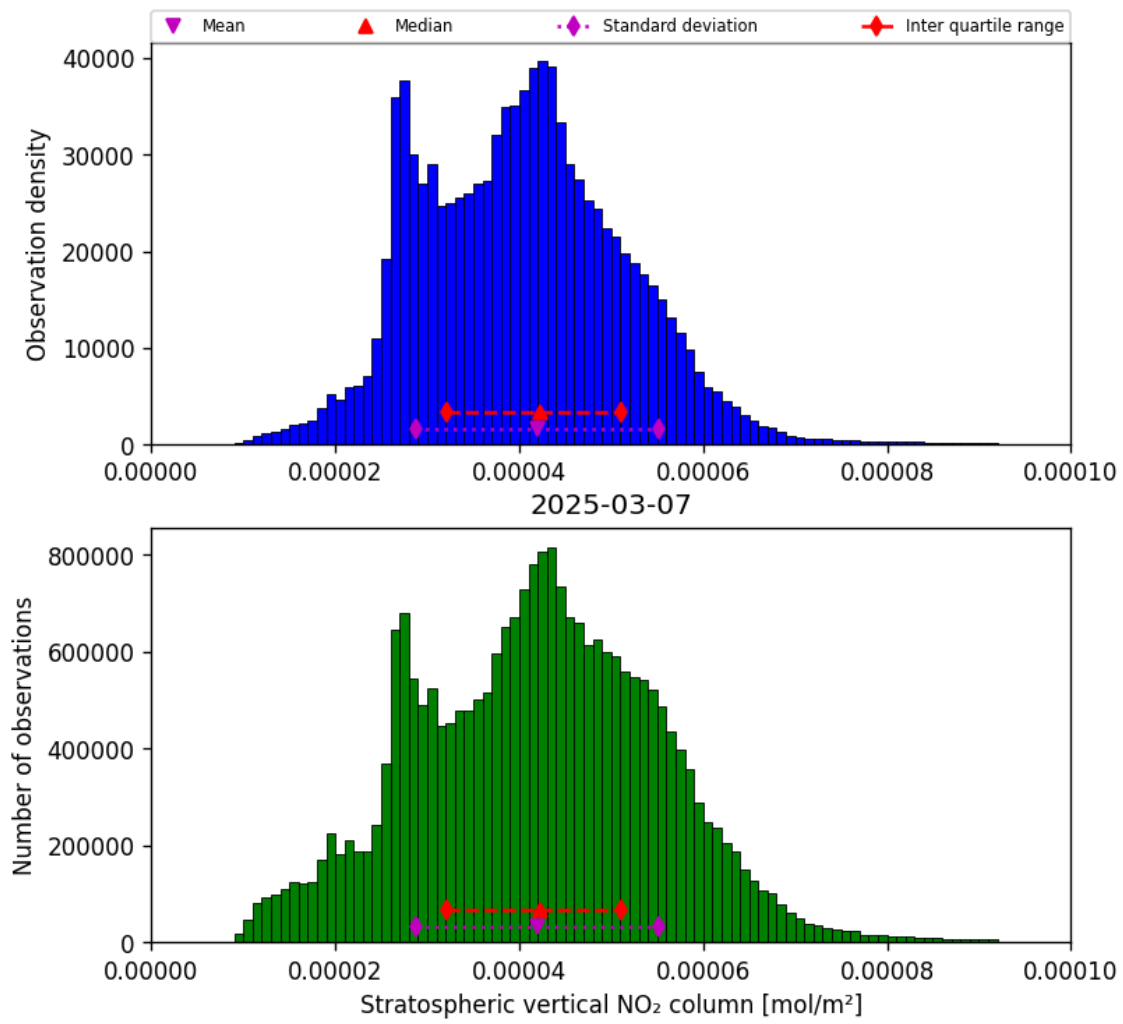
Figure 34: Histogram of “Stratospheric vertical NO 2 column” for 2025-03-07 to 2025-03-08
