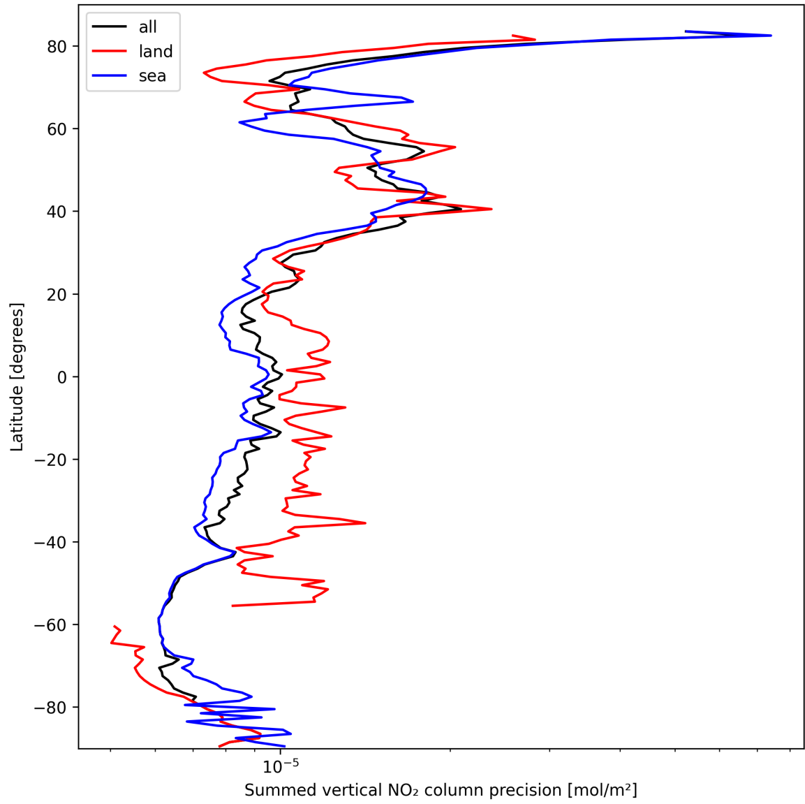
Figure 22: Zonal average of “Summed vertical NO 2 column precision” for 2025-03-07 to 2025-03-08.
