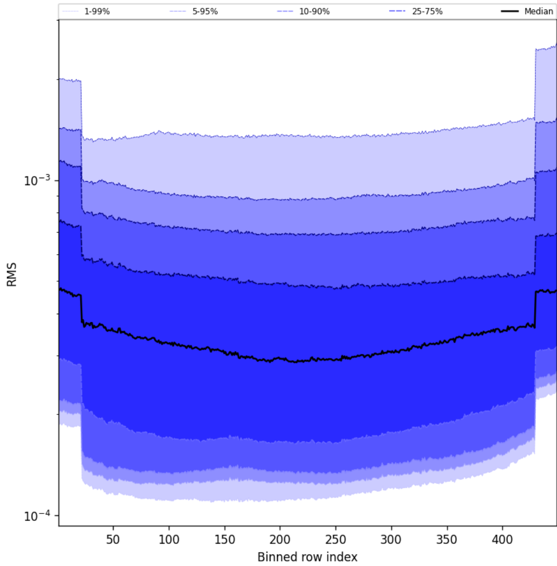
Figure 58: Along track statistics of “RMS” for 2025-03-07 to 2025-03-08
