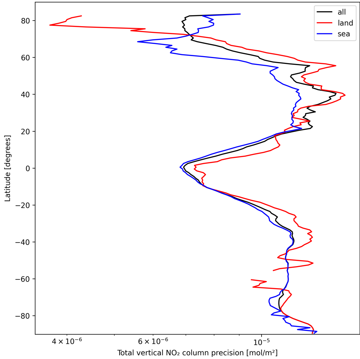
Figure 20: Zonal average of “Total vertical NO 2 column precision” for 2025-03-07 to 2025-03-08.
