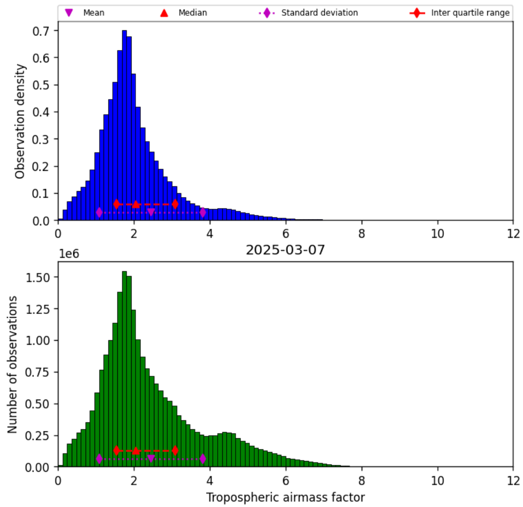
Figure 29: Histogram of “Tropospheric airmass factor” for 2025-03-07 to 2025-03-08
