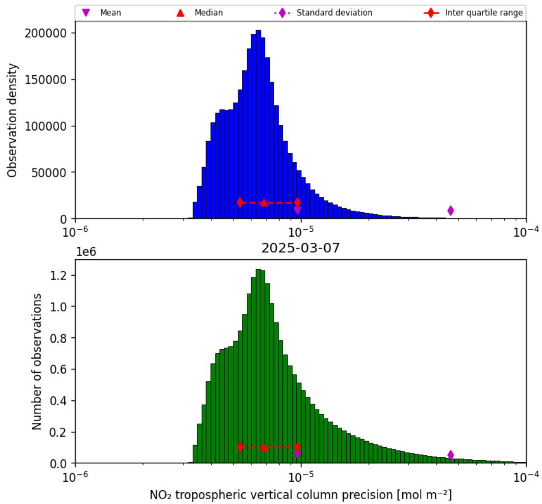
Figure 28: Histogram of “NO 2 tropospheric vertical column precision” for 2025-03-07 to 2025-03-08
