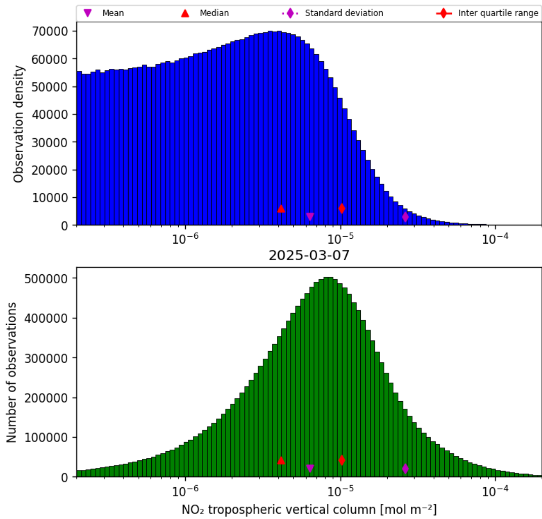
Figure 27: Histogram of “NO 2 tropospheric vertical column” for 2025-03-07 to 2025-03-08
