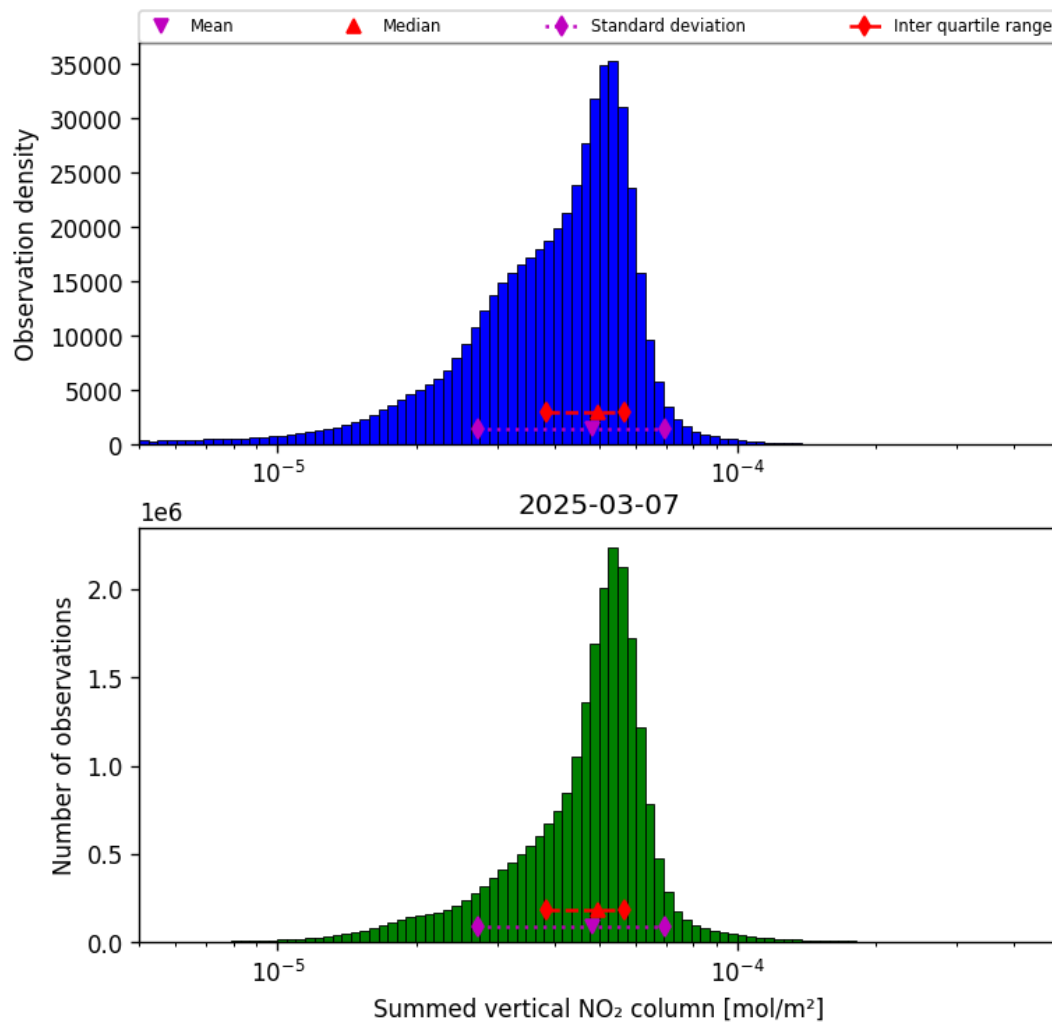
Figure 38: Histogram of “Summed vertical NO 2 column” for 2025-03-07 to 2025-03-08
