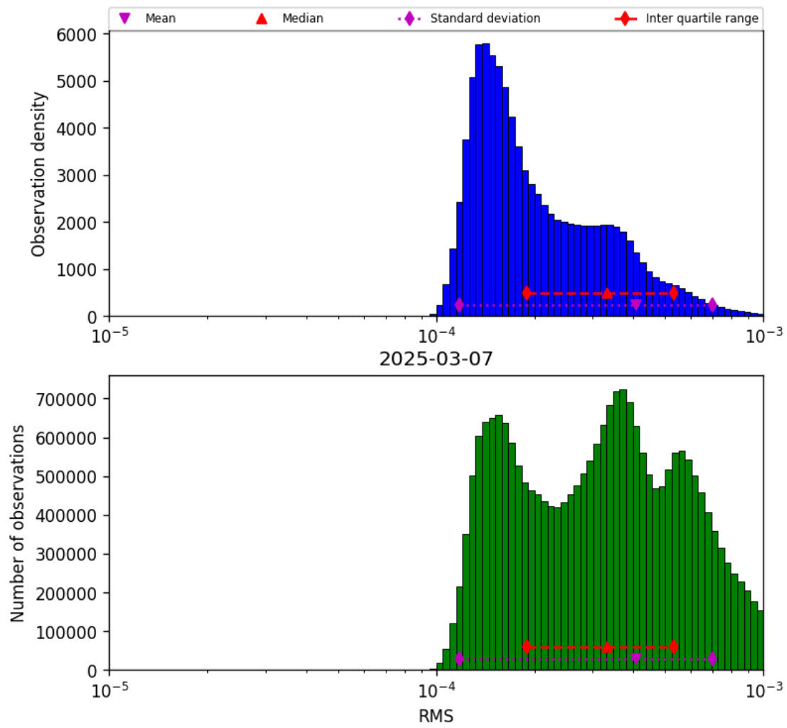
Figure 41: Histogram of “RMS” for 2025-03-07 to 2025-03-08
