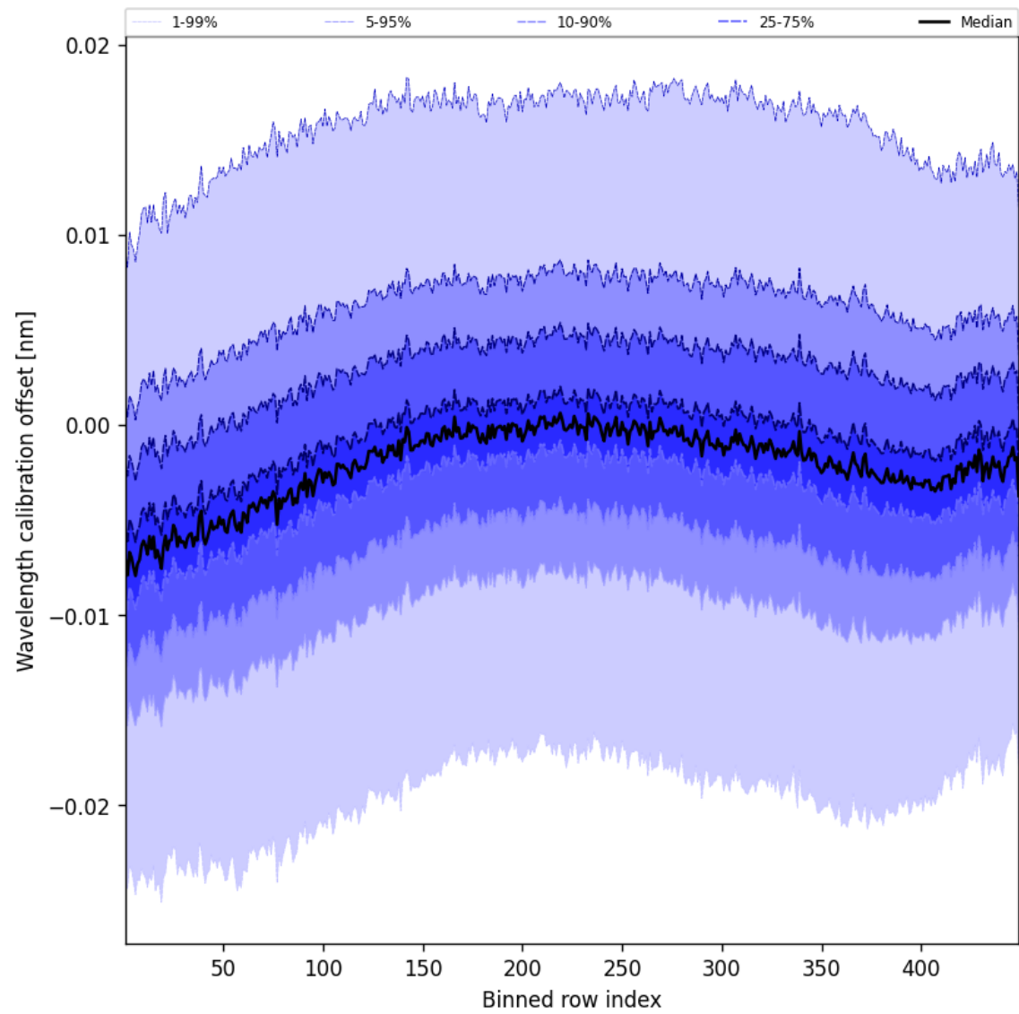
Figure 50: Along track statistics of “Wavelength calibration offset” for 2025-03-07 to 2025-03-08
