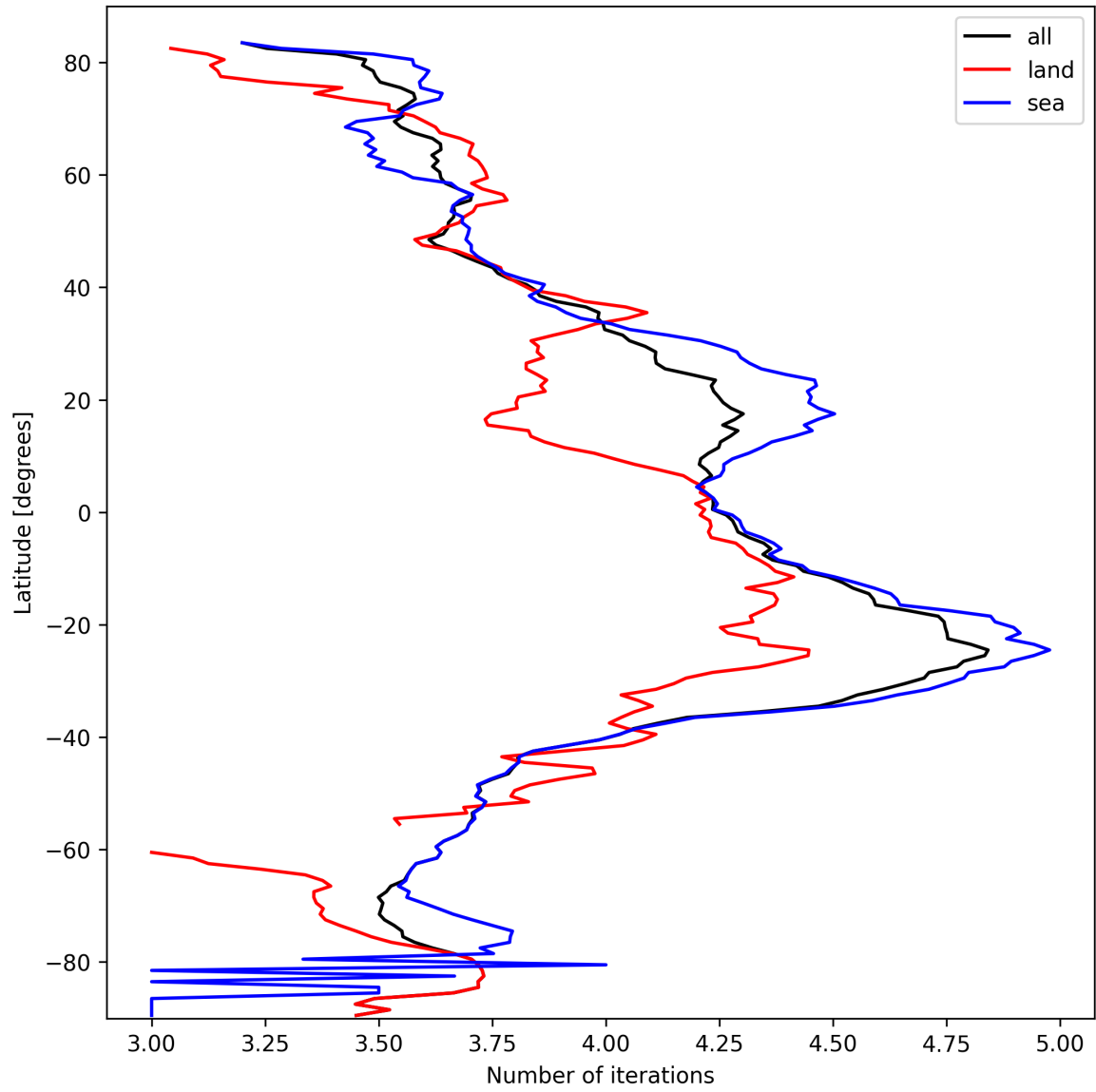
Figure 15: Zonal average of “Number of iterations” for 2025-03-07 to 2025-03-08.
