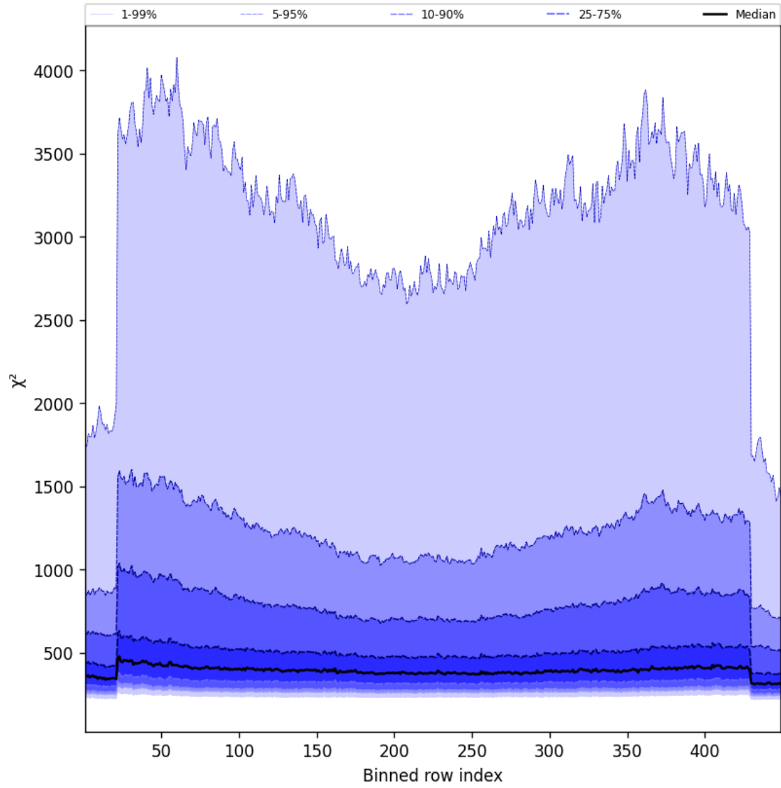
Figure 57: Along track statistics of “ \chi^2 ” for 2025-03-07 to 2025-03-08
