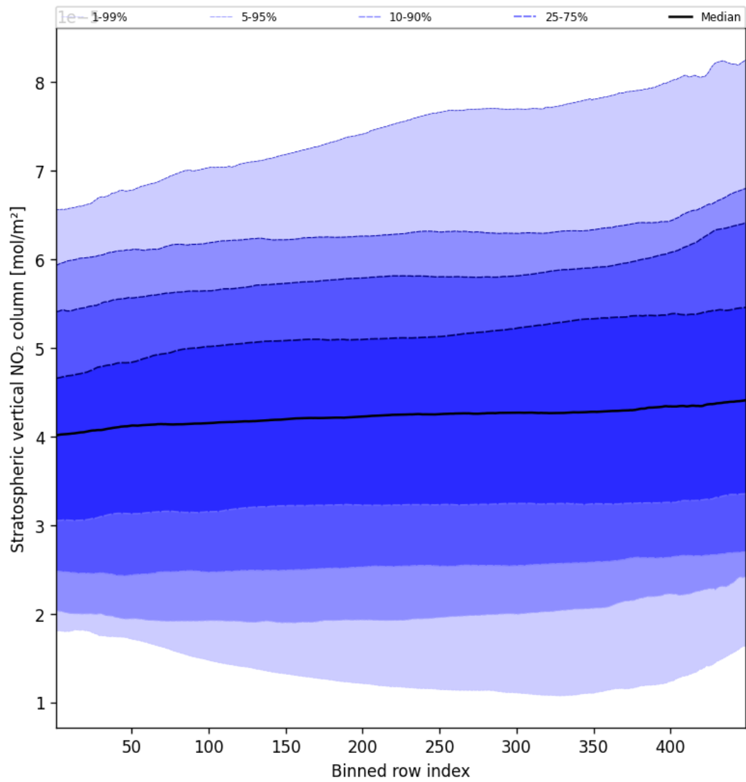
Figure 51: Along track statistics of “Stratospheric vertical NO 2 column” for 2025-03-07 to 2025-03-08
