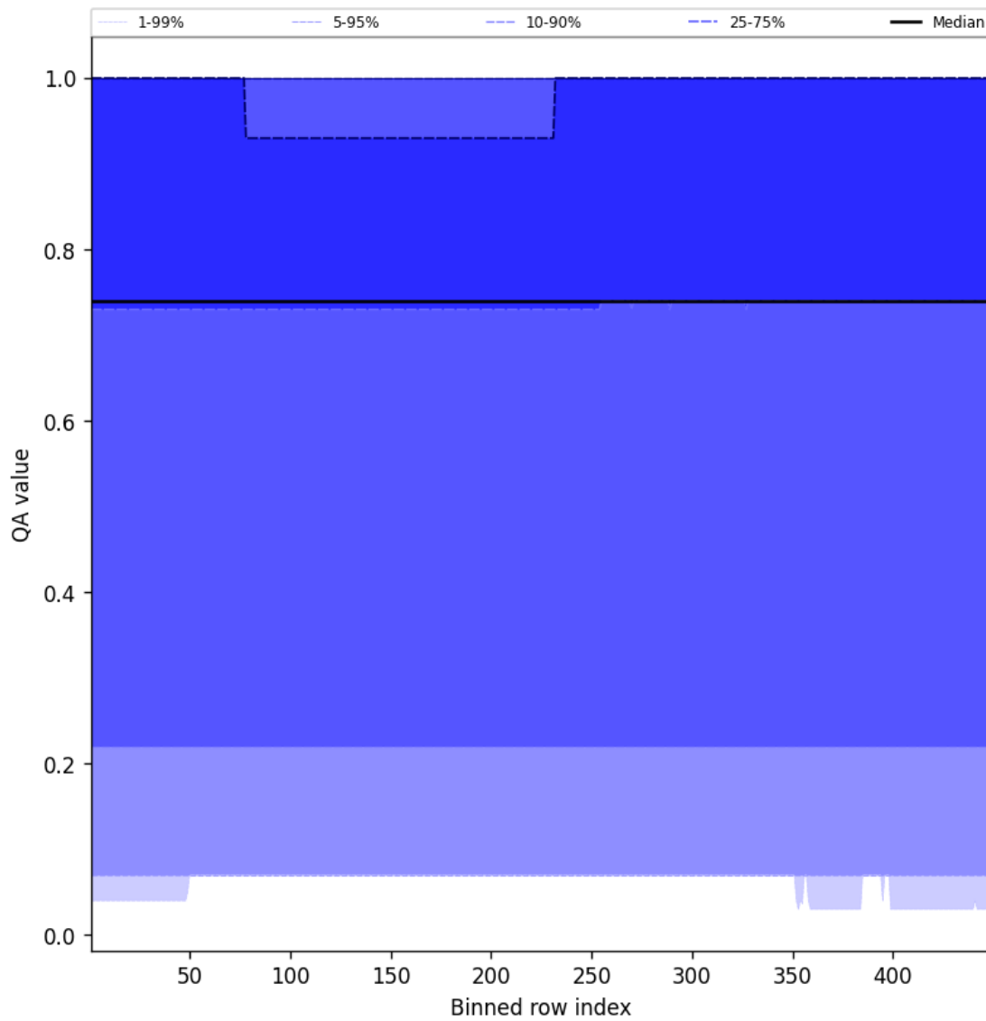
Figure 43: Along track statistics of “QA value” for 2025-03-07 to 2025-03-08
