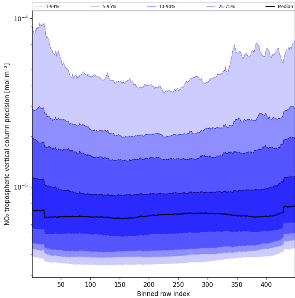
Figure 45: Along track statistics of “NO 2 tropospheric vertical column precision” for 2025-03-08 to 2025-03-09
