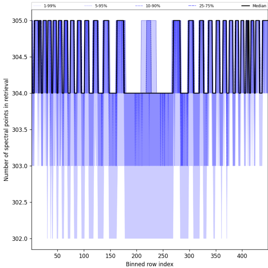
Figure 48: Along track statistics of “Number of spectral points in retrieval” for 2025-03-08 to 2025-03-09
