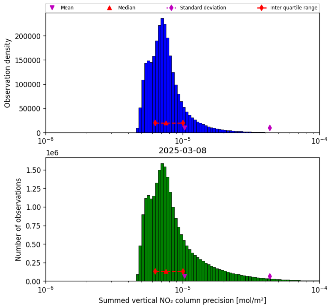
Figure 39: Histogram of “Summed vertical NO 2 column precision” for 2025-03-08 to 2025-03-09
