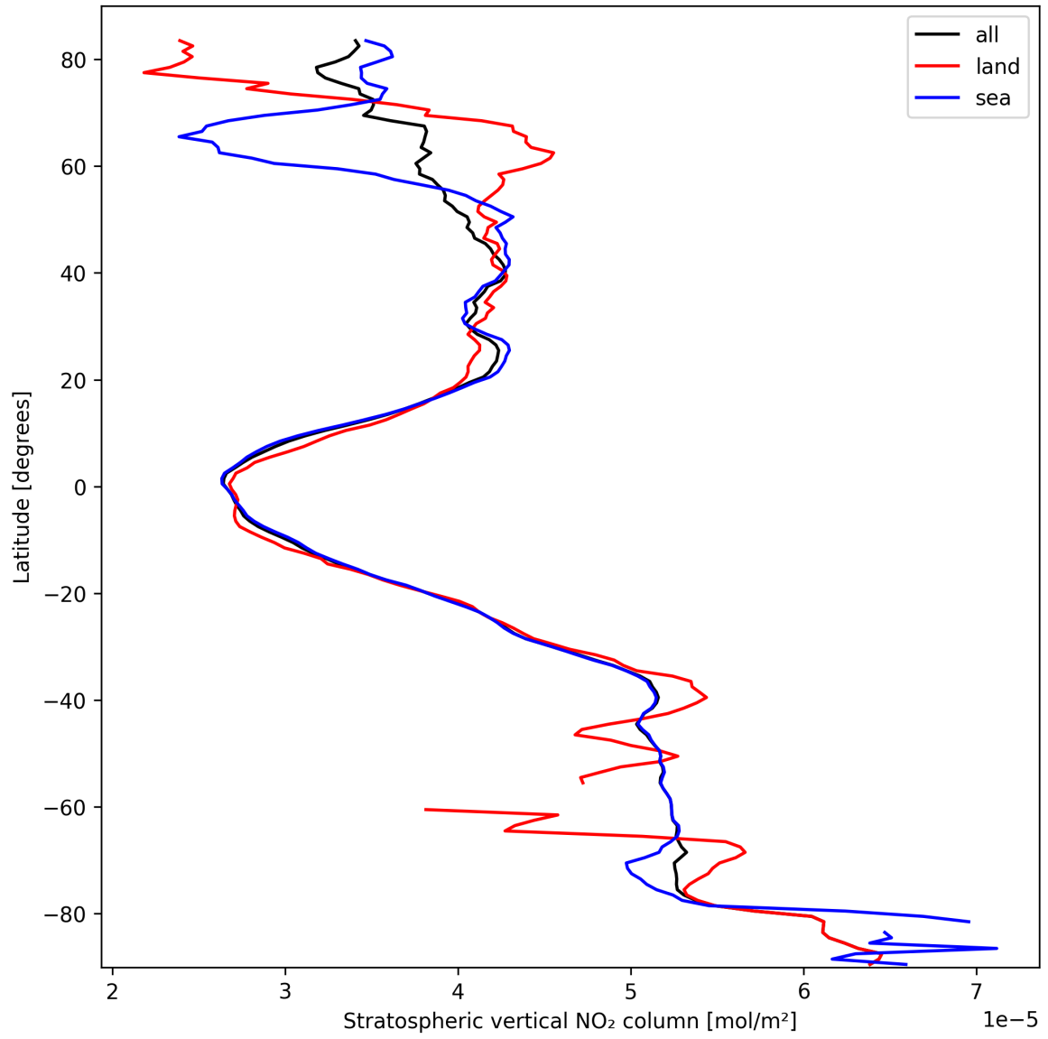
Figure 17: Zonal average of “Stratospheric vertical NO 2 column” for 2025-03-08 to 2025-03-09.
