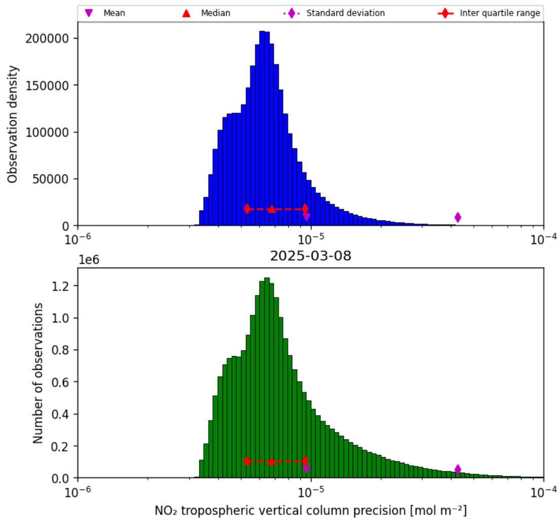
Figure 28: Histogram of “NO 2 tropospheric vertical column precision” for 2025-03-08 to 2025-03-09
