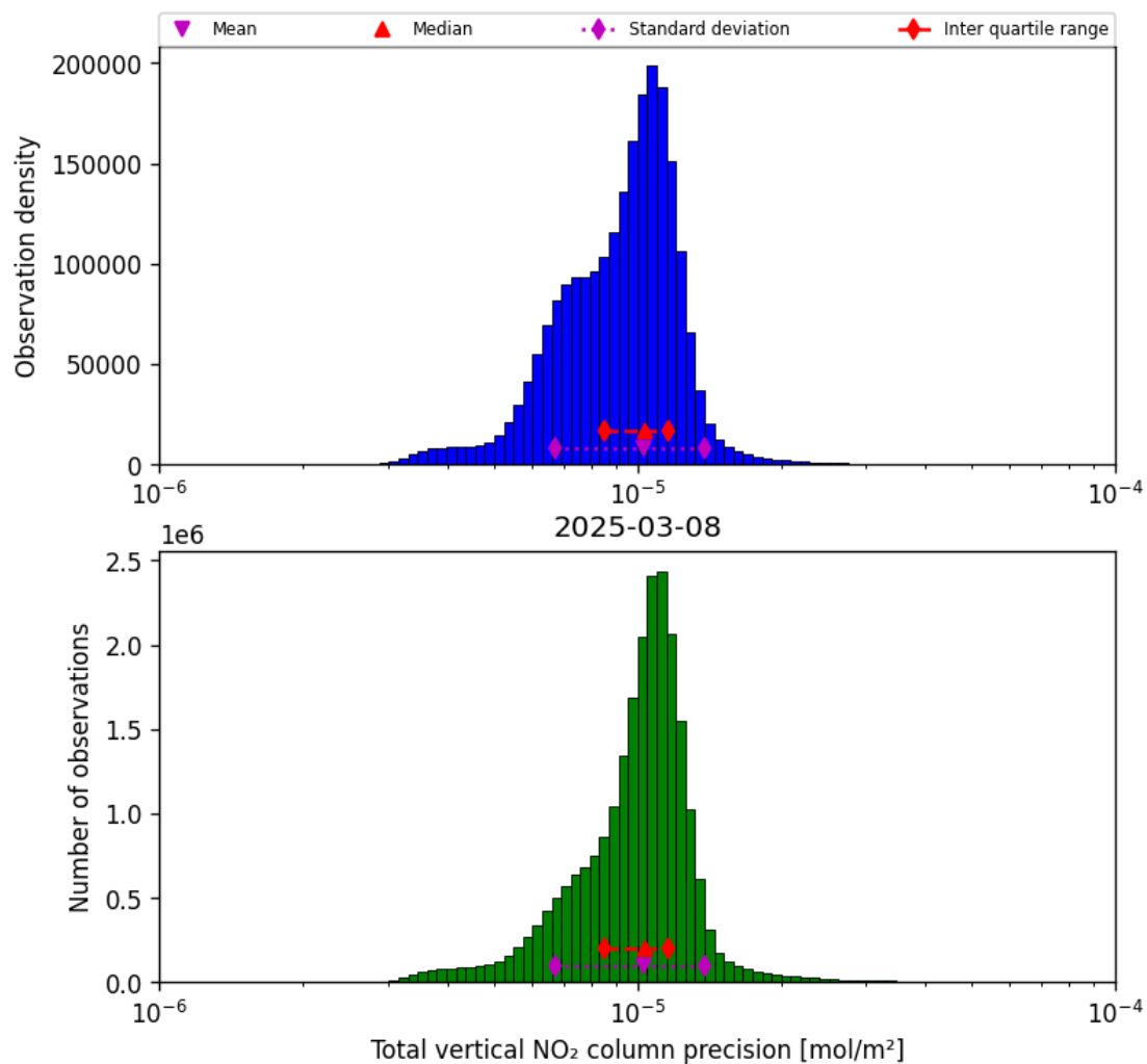
Figure 37: Histogram of “Total vertical NO 2 column precision” for 2025-03-08 to 2025-03-09
