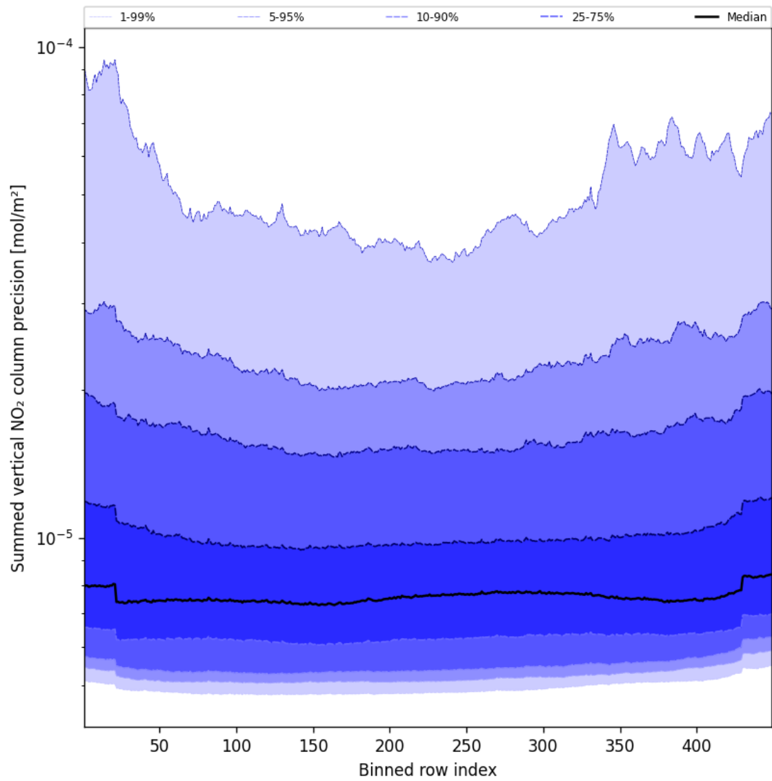
Figure 56: Along track statistics of “Summed vertical NO 2 column precision” for 2025-03-08 to 2025-03-09
