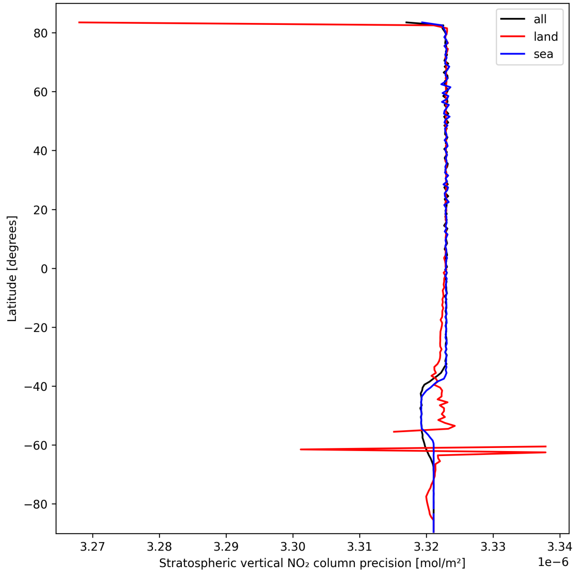
Figure 18: Zonal average of “Stratospheric vertical NO 2 column precision” for 2025-03-08 to 2025-03-09.
