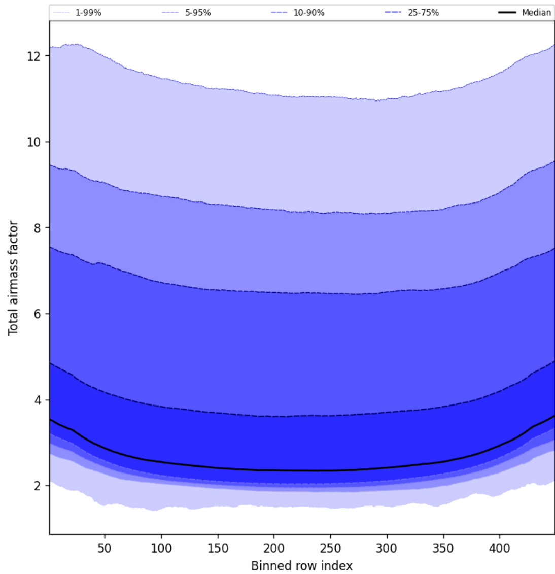
Figure 47: Along track statistics of “Total airmass factor” for 2025-03-08 to 2025-03-09
