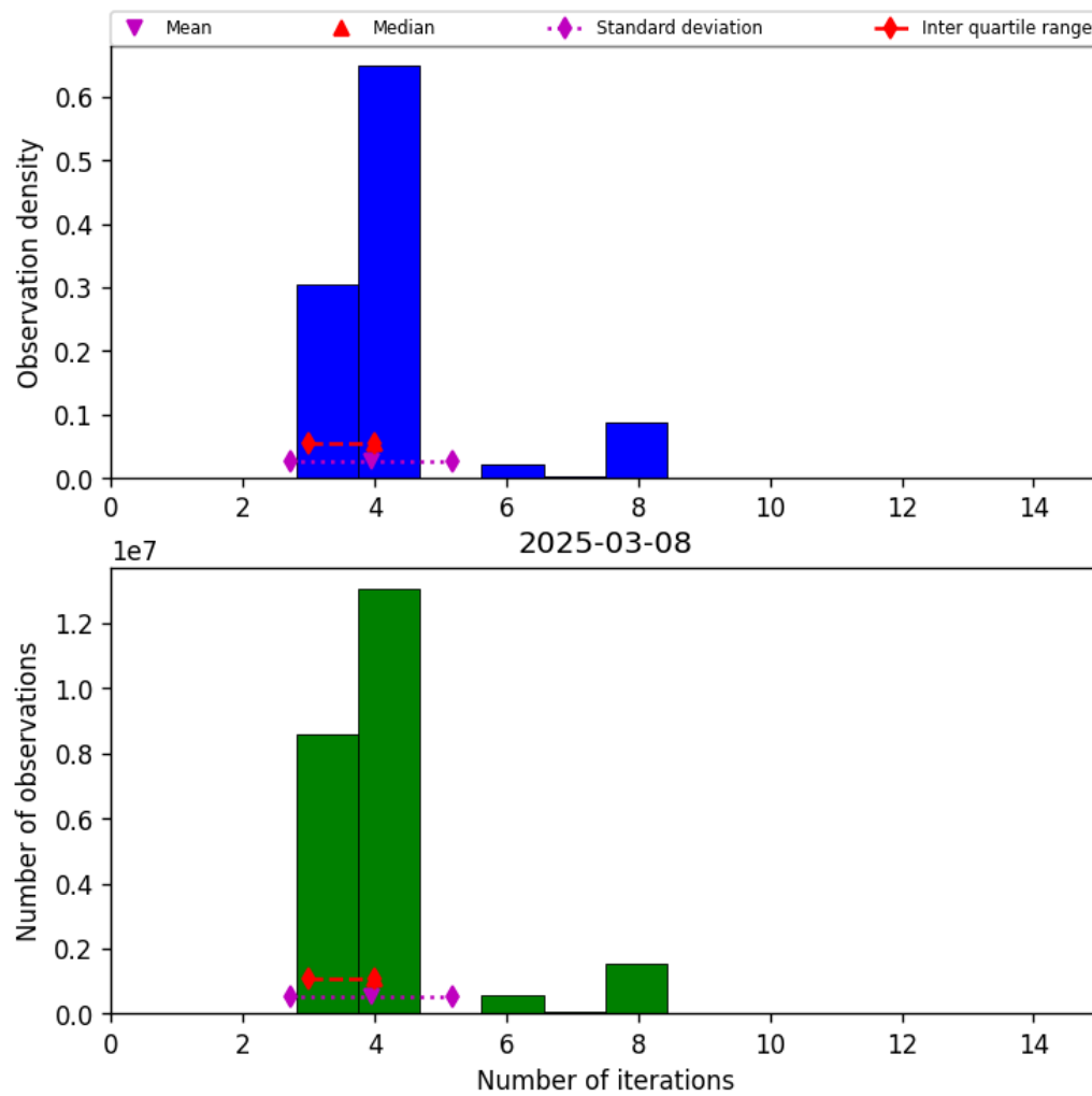
Figure 32: Histogram of “Number of iterations” for 2025-03-08 to 2025-03-09
