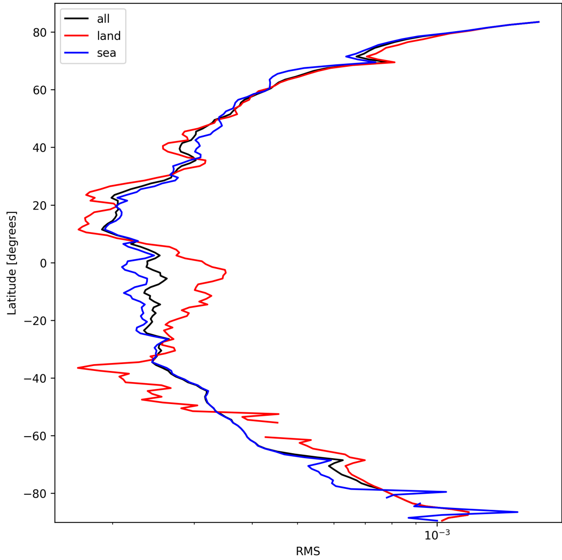
Figure 24: Zonal average of “RMS” for 2025-03-08 to 2025-03-09.
