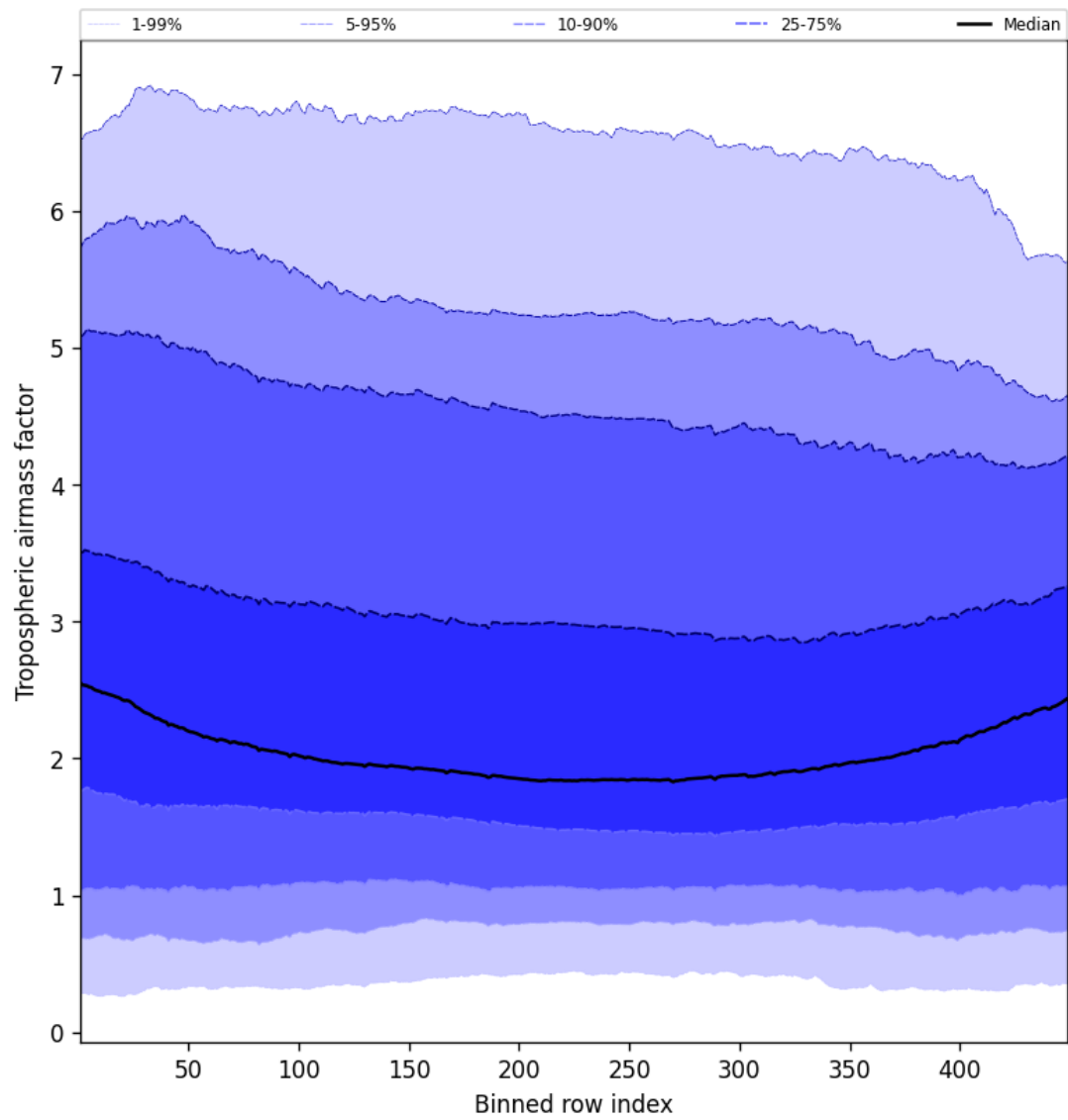
Figure 46: Along track statistics of “Tropospheric air mass factor” for 2025-03-08 to 2025-03-09
