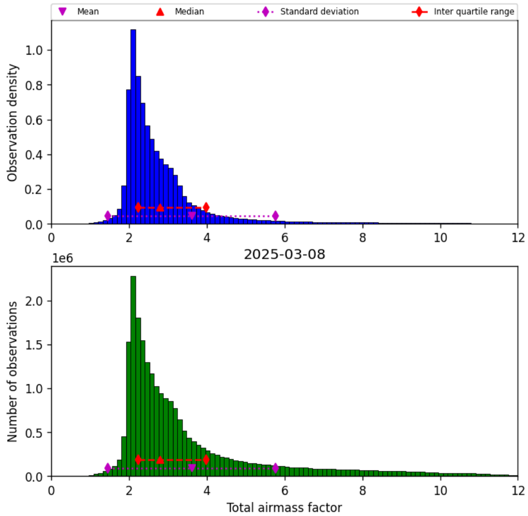
Figure 30: Histogram of “Total airmass factor” for 2025-03-08 to 2025-03-09
