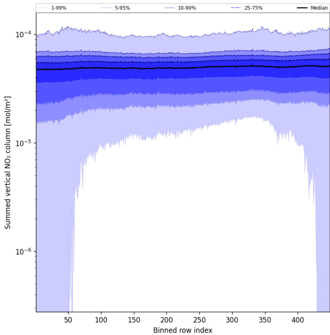
Figure 55: Along track statistics of “Summed vertical NO 2 column” for 2025-03-08 to 2025-03-09
