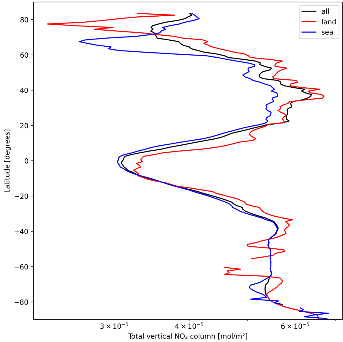
Figure 19: Zonal average of “Total vertical NO 2 column” for 2025-03-08 to 2025-03-09.
