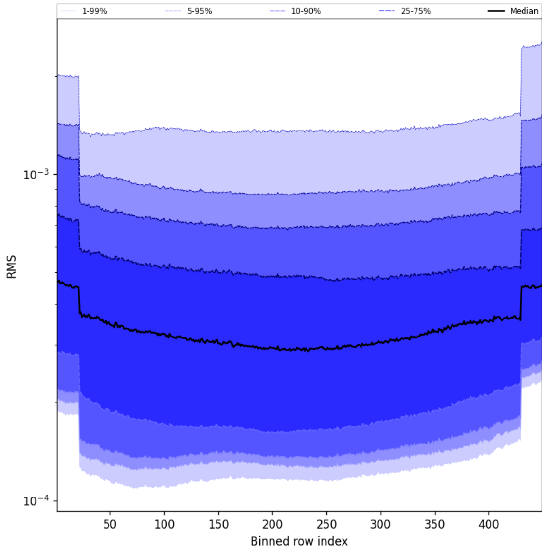
Figure 58: Along track statistics of “RMS” for 2025-03-08 to 2025-03-09
