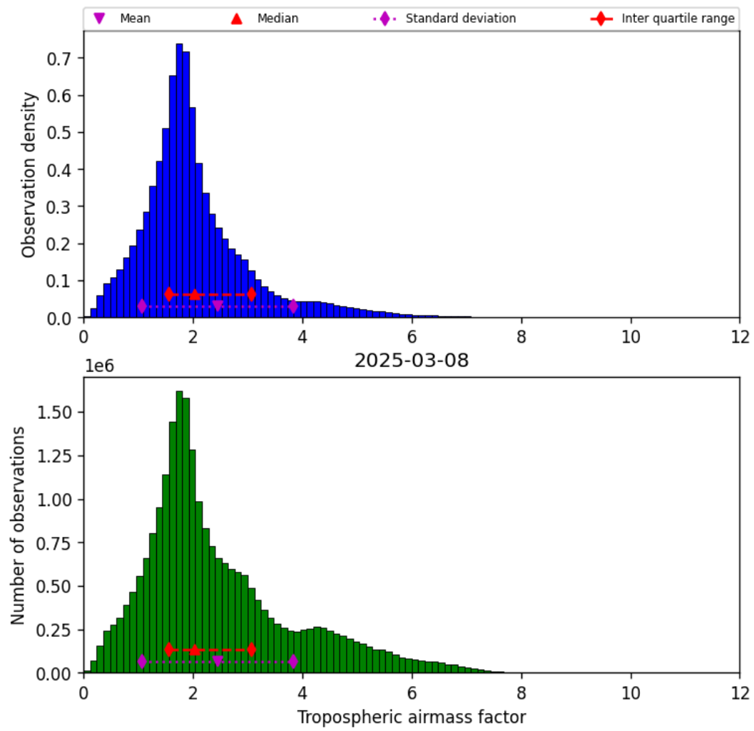
Figure 29: Histogram of “Tropospheric airmass factor” for 2025-03-08 to 2025-03-09
