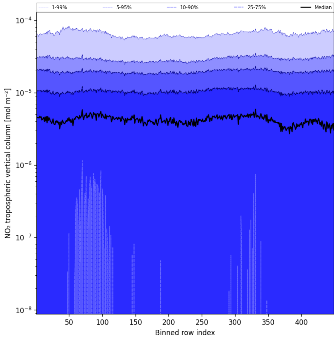
Figure 44: Along track statistics of “NO 2 tropospheric vertical column” for 2025-03-08 to 2025-03-09
