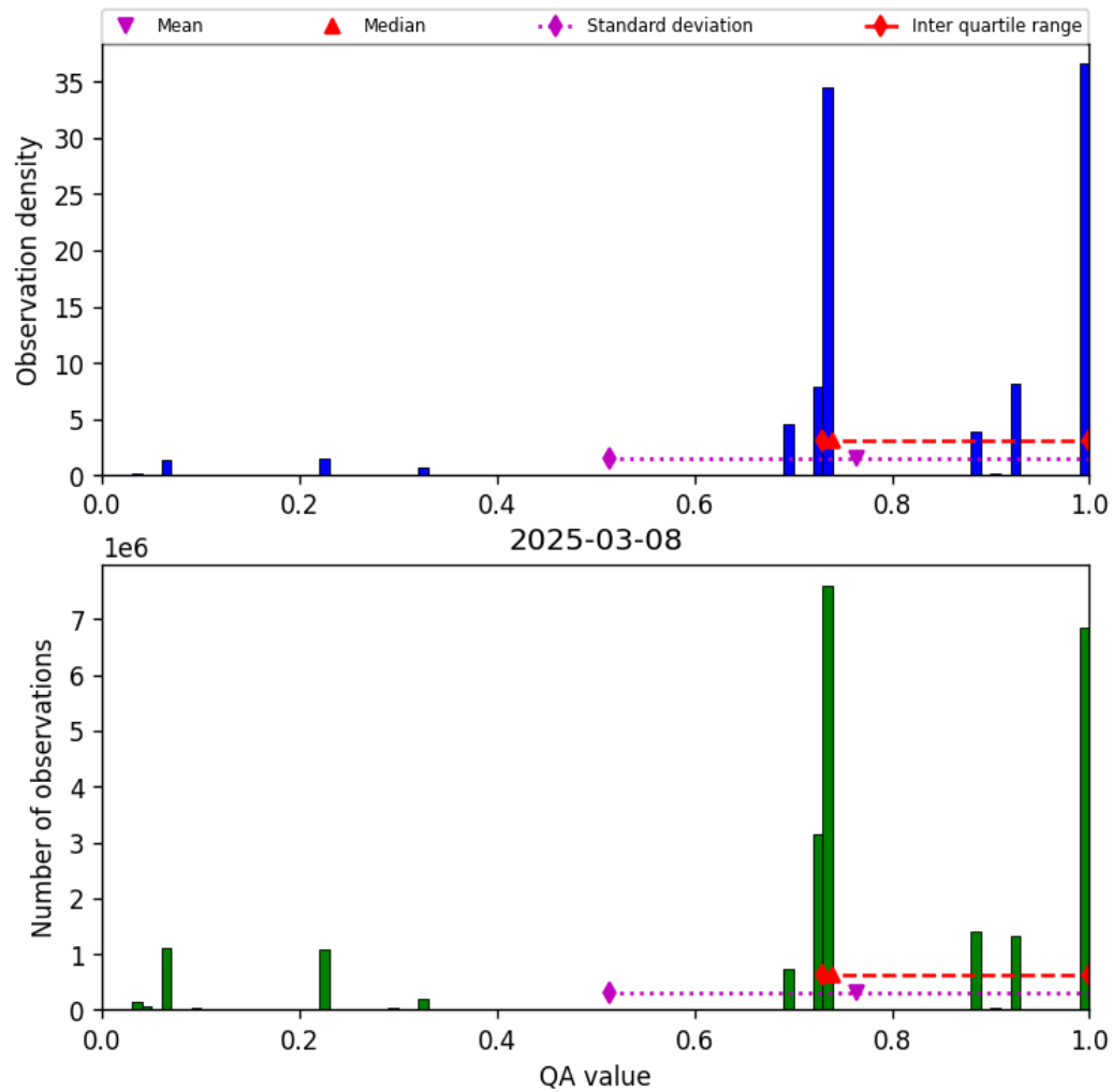
Figure 26: Histogram of “QA value” for 2025-03-08 to 2025-03-09
