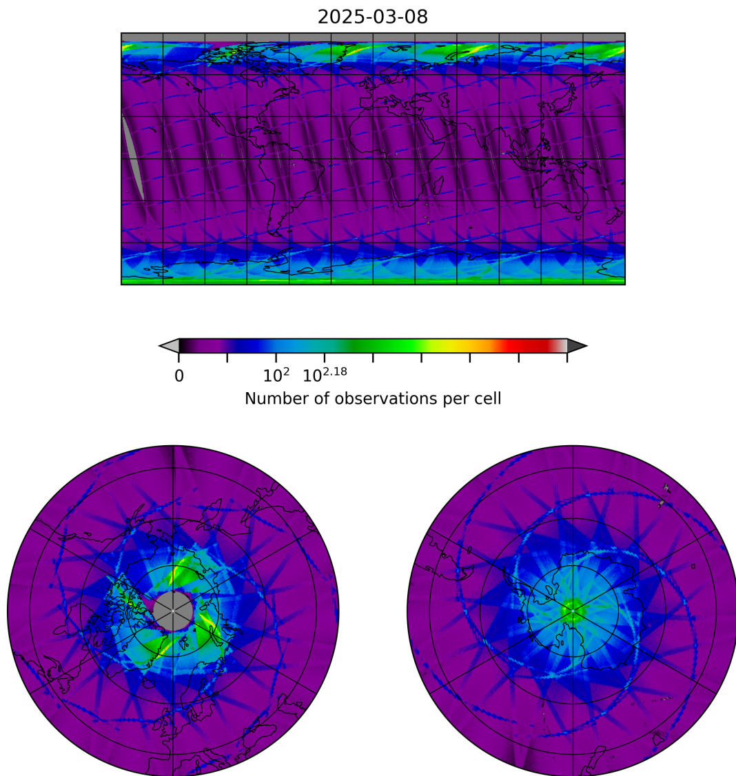
Figure 8: Map of the number of observations for 2025-03-08 to 2025-03-09
