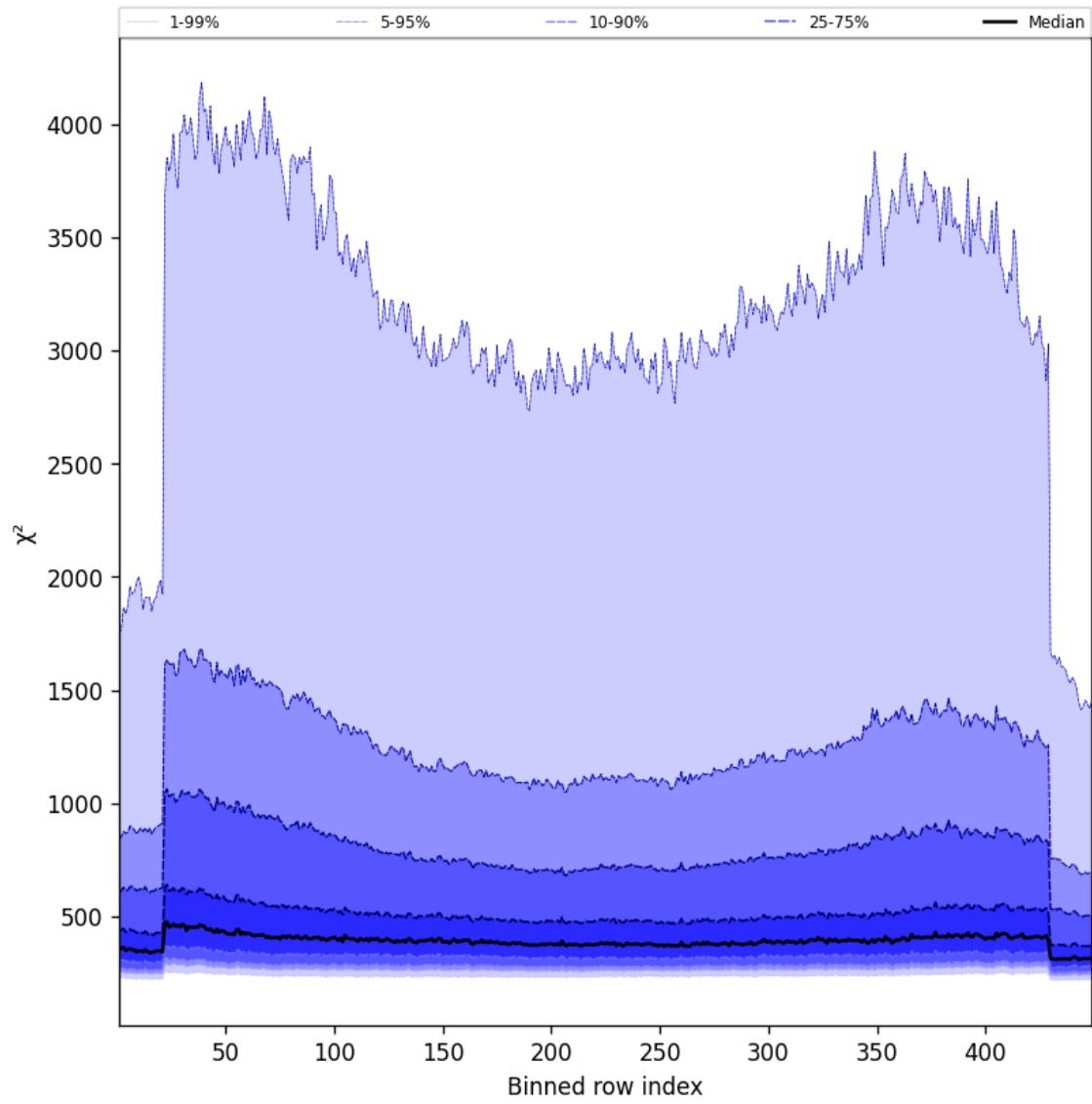
Figure 57: Along track statistics of “ \chi^2 ” for 2025-03-08 to 2025-03-09
