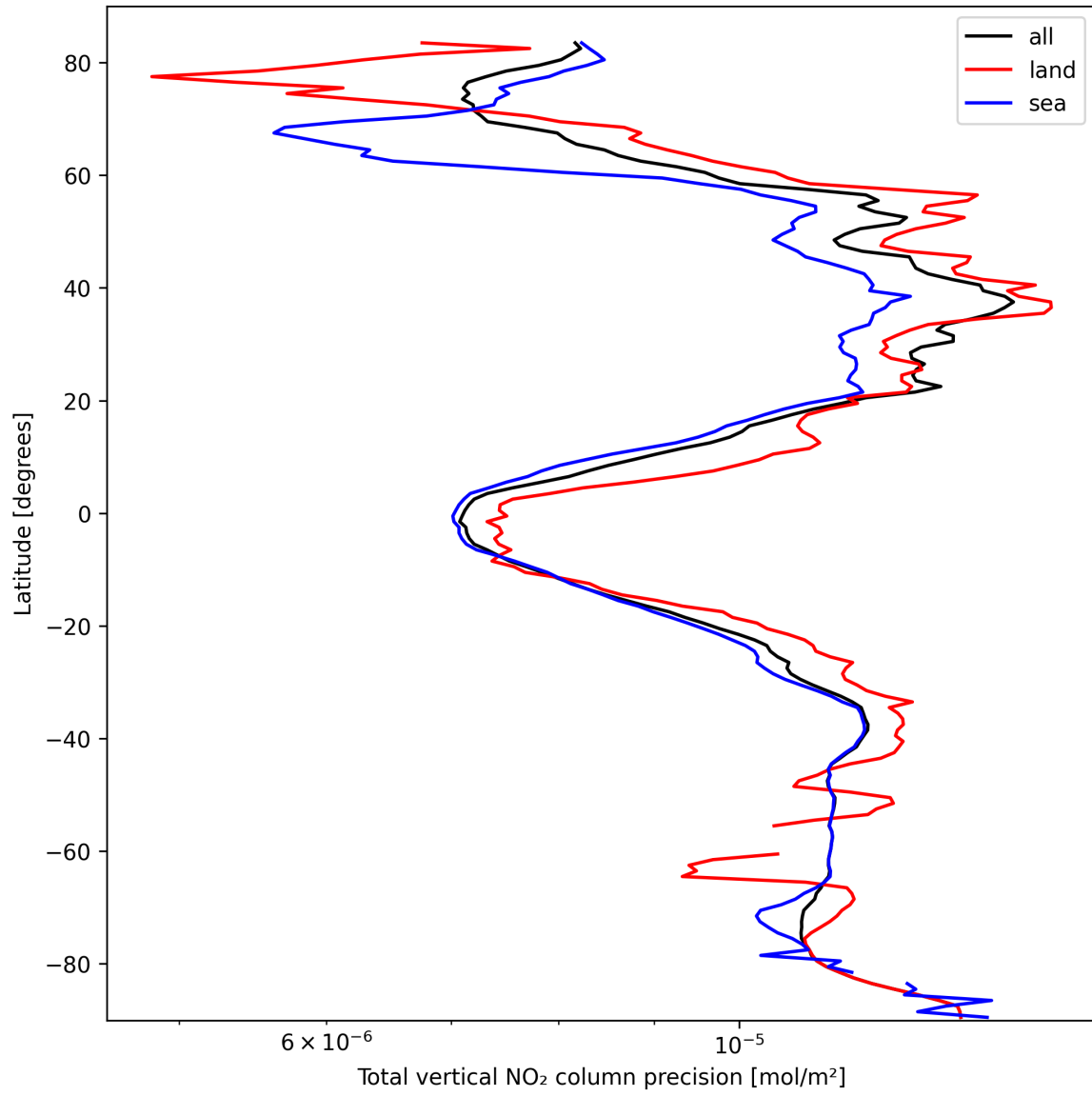
Figure 20: Zonal average of “Total vertical NO 2 column precision” for 2025-03-08 to 2025-03-09.
