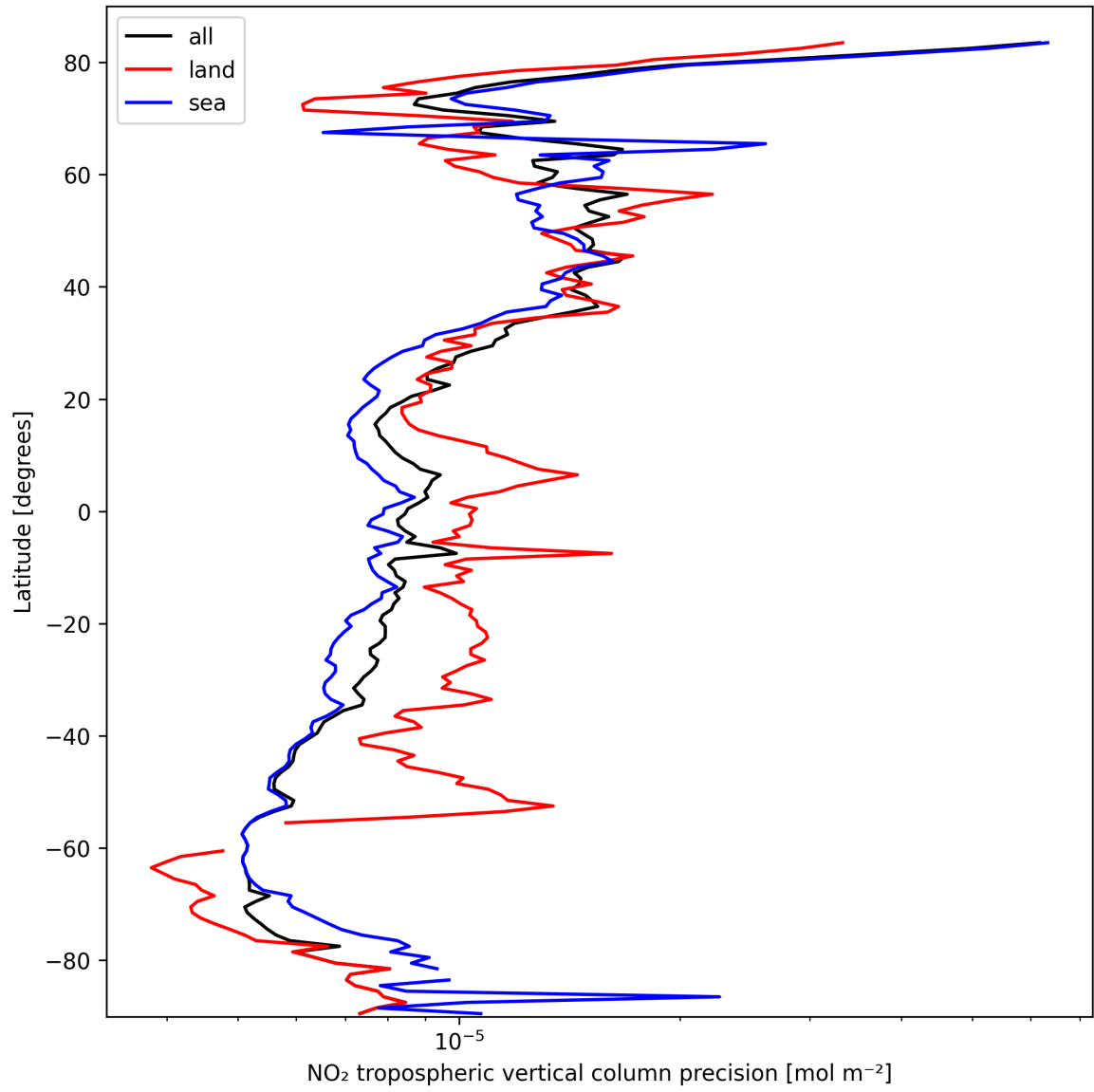
Figure 11: Zonal average of “NO 2 tropospheric vertical column precision” for 2025-03-08 to 2025-03-09.
