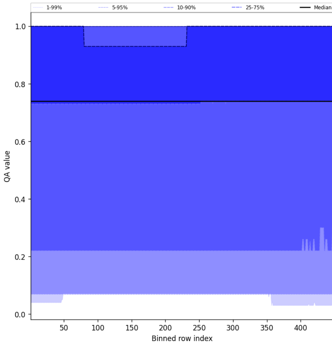
Figure 43: Along track statistics of “QA value” for 2025-03-08 to 2025-03-09
