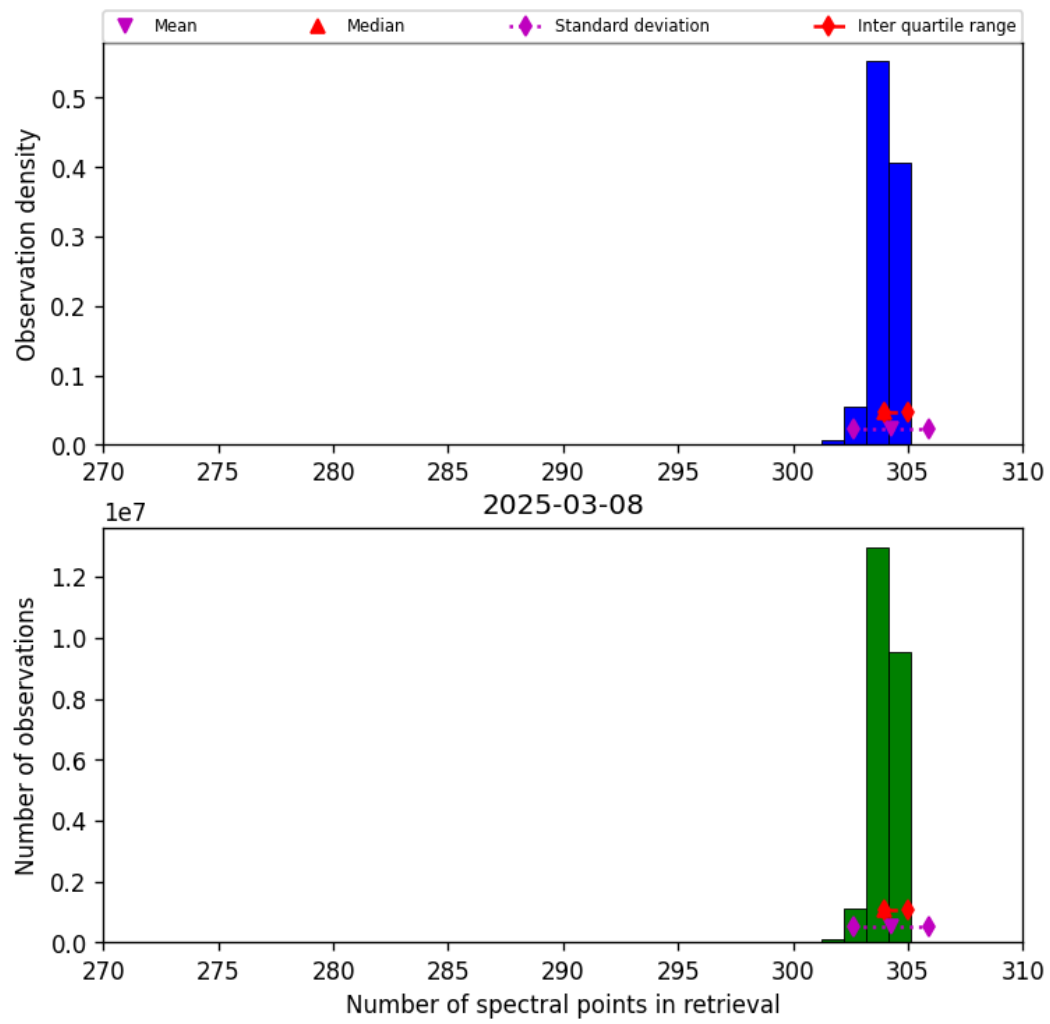
Figure 31: Histogram of “Number of spectral points in retrieval” for 2025-03-08 to 2025-03-09
