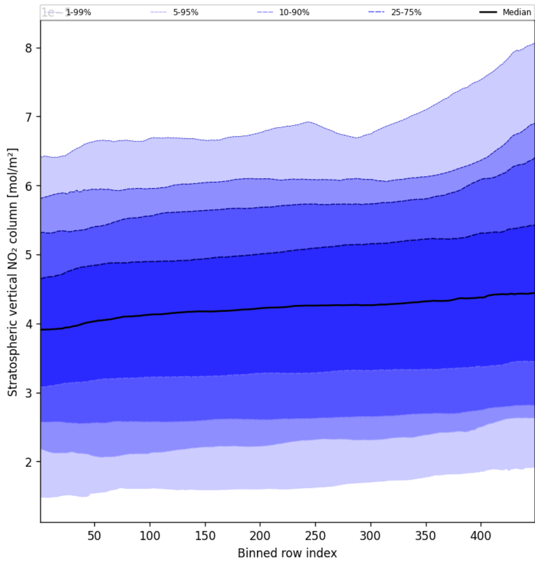
Figure 51: Along track statistics of “Stratospheric vertical NO 2 column” for 2025-03-08 to 2025-03-09
