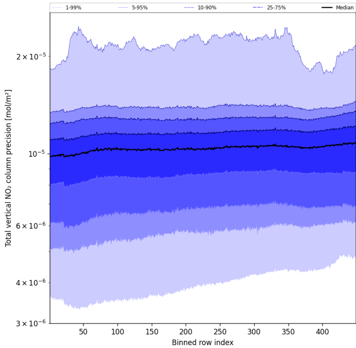
Figure 54: Along track statistics of "Total vertical NO 2 column precision" for 2025-03-08 to 2025-03-09
