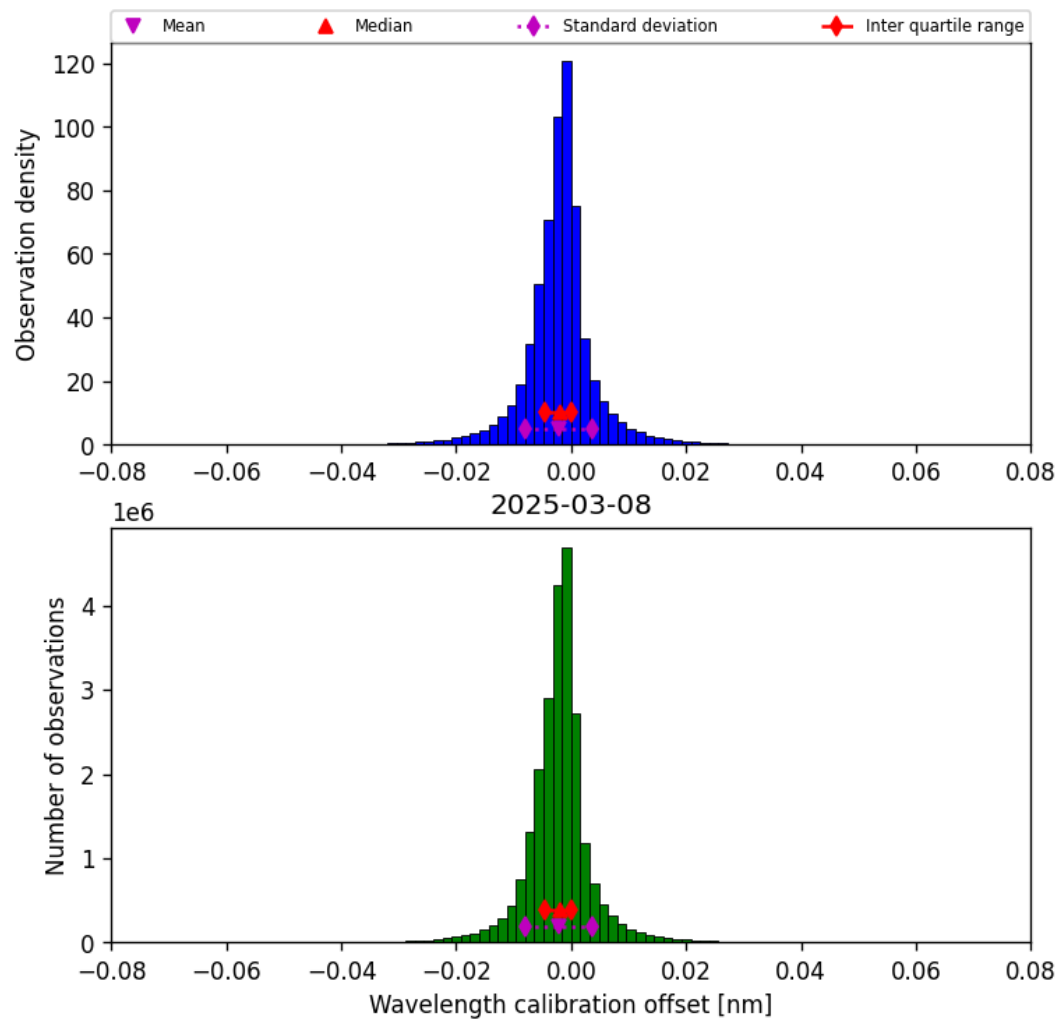
Figure 33: Histogram of “Wavelength calibration offset” for 2025-03-08 to 2025-03-09
