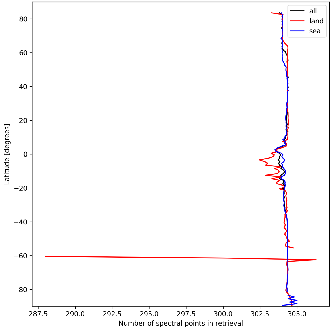
Figure 14: Zonal average of “Number of spectral points in retrieval” for 2025-03-08 to 2025-03-09.
