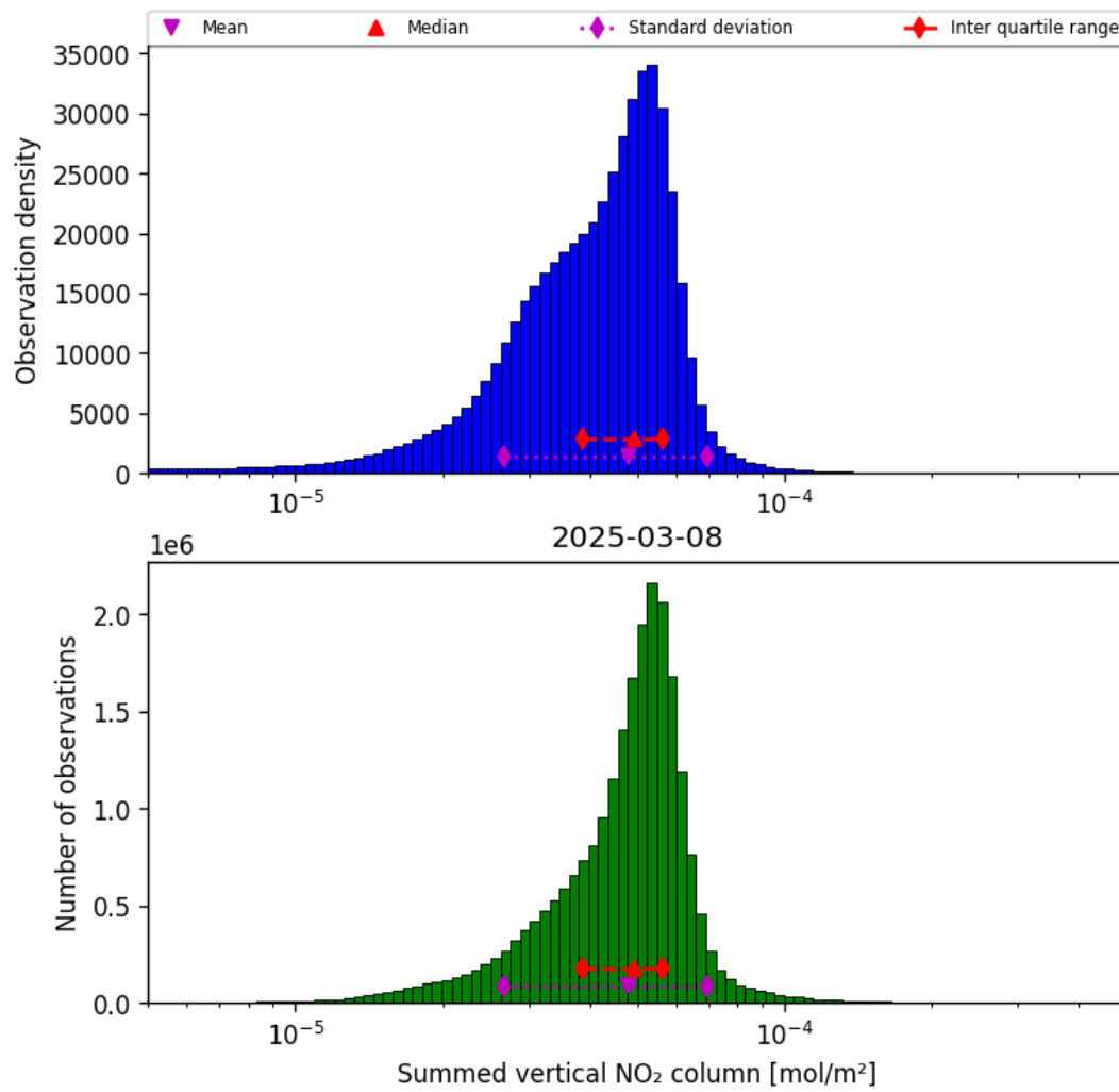
Figure 38: Histogram of “Summed vertical NO 2 column” for 2025-03-08 to 2025-03-09
