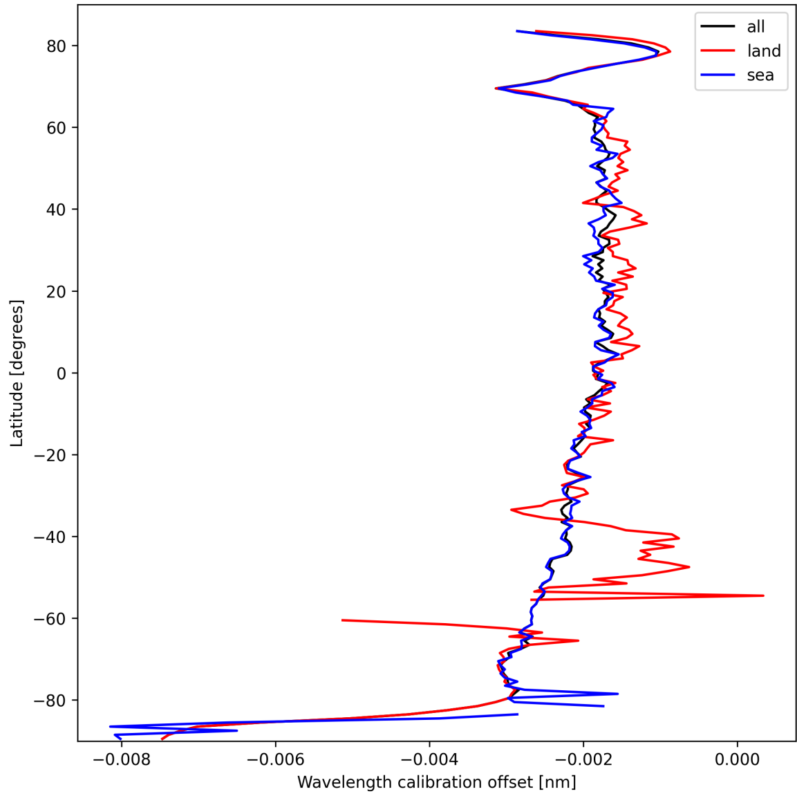
Figure 16: Zonal average of “Wavelength calibration offset” for 2025-03-08 to 2025-03-09.
