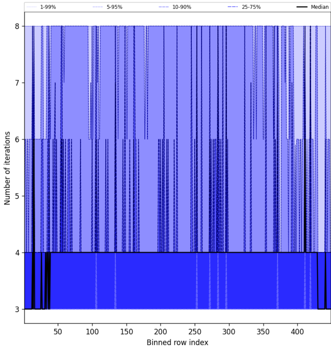
Figure 49: Along track statistics of “Number of iterations” for 2025-03-08 to 2025-03-09
