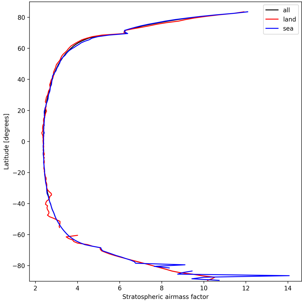
Figure 25: Zonal average of “Stratospheric airmass factor” for 2025-03-08 to 2025-03-09.
