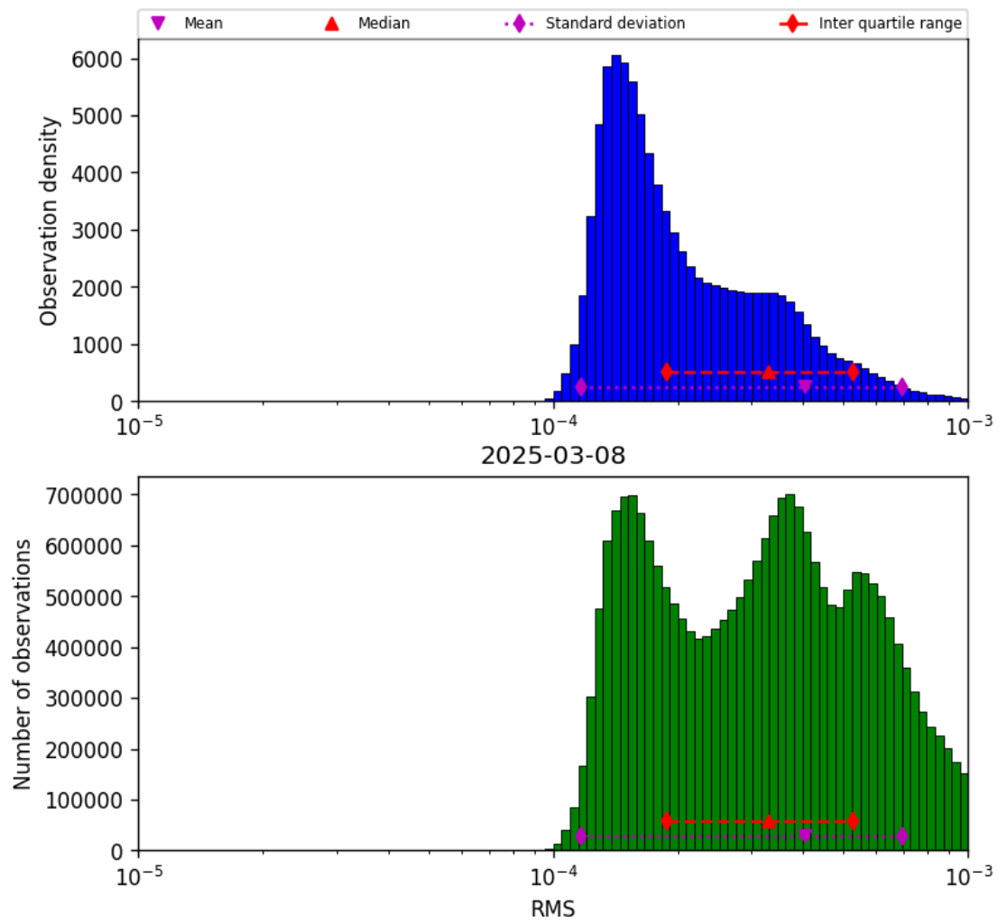
Figure 41: Histogram of “RMS” for 2025-03-08 to 2025-03-09
