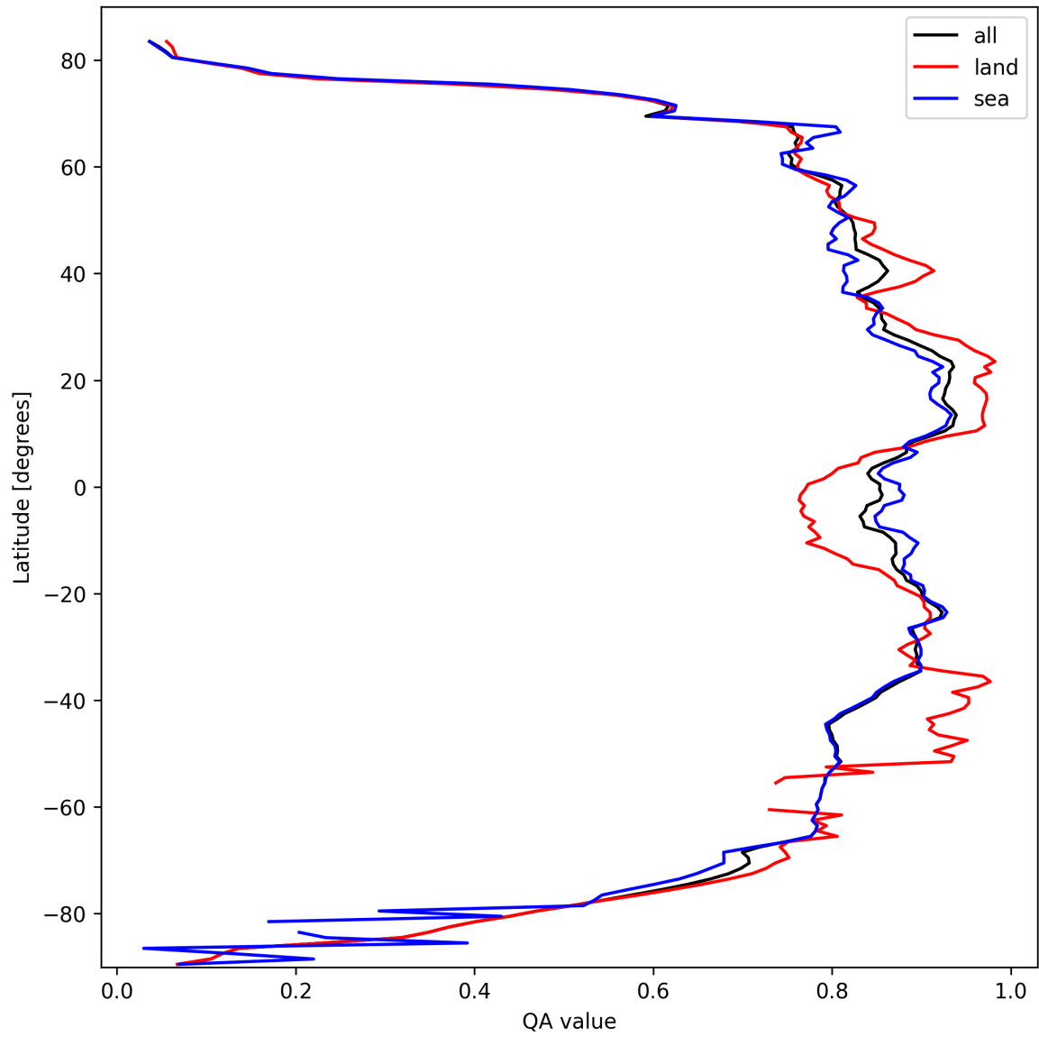
Figure 9: Zonal average of “QA value” for 2025-03-08 to 2025-03-09.
