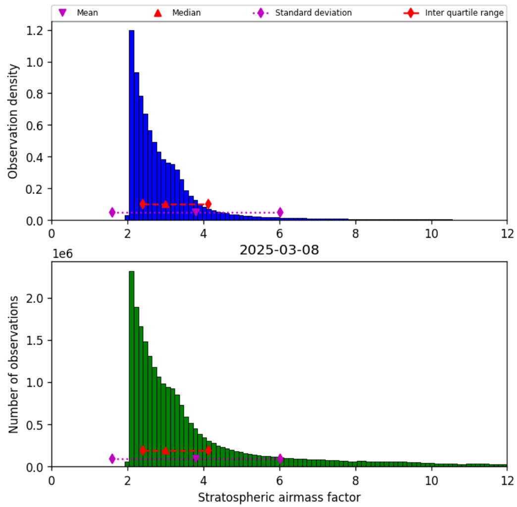
Figure 42: Histogram of “Stratospheric airmass factor” for 2025-03-08 to 2025-03-09
