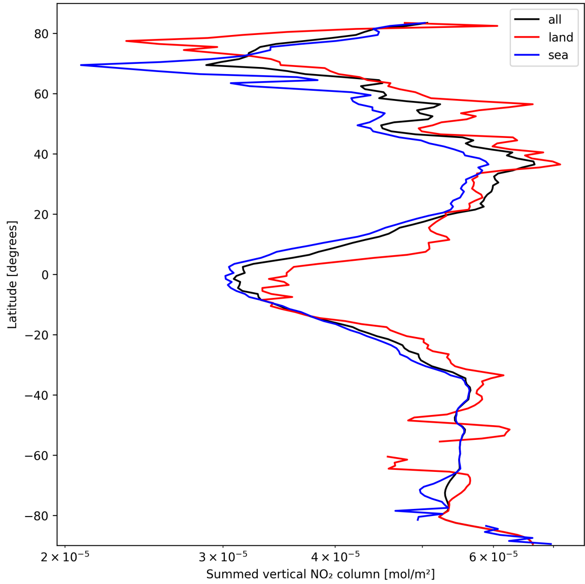
Figure 21: Zonal average of “Summed vertical NO 2 column” for 2025-03-08 to 2025-03-09.
