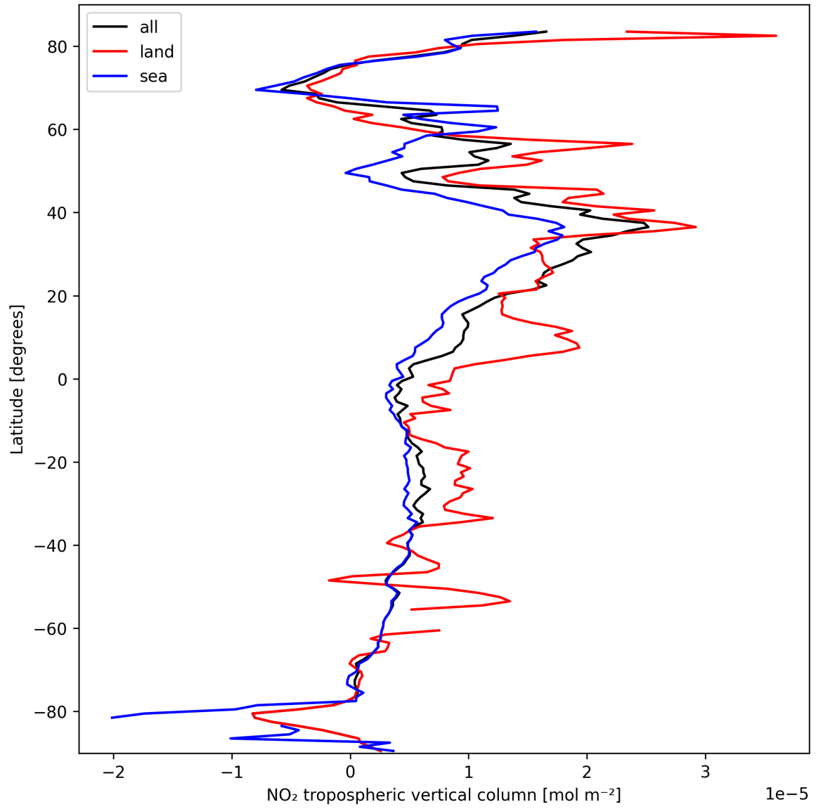
Figure 10: Zonal average of “NO 2 tropospheric vertical column” for 2025-03-08 to 2025-03-09.
