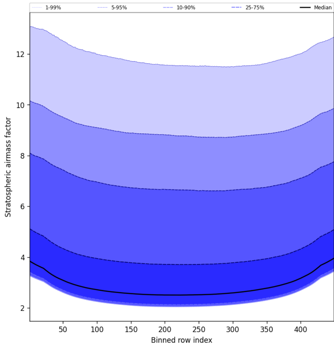
Figure 59: Along track statistics of “Stratospheric airmass factor” for 2025-03-08 to 2025-03-09
