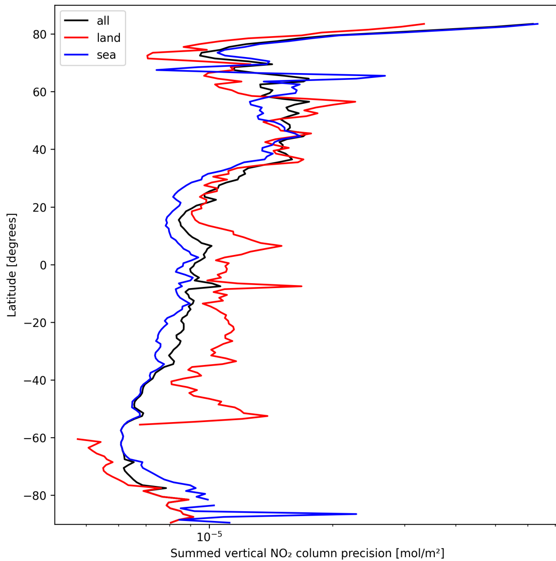
Figure 22: Zonal average of “Summed vertical NO 2 column precision” for 2025-03-08 to 2025-03-09.
