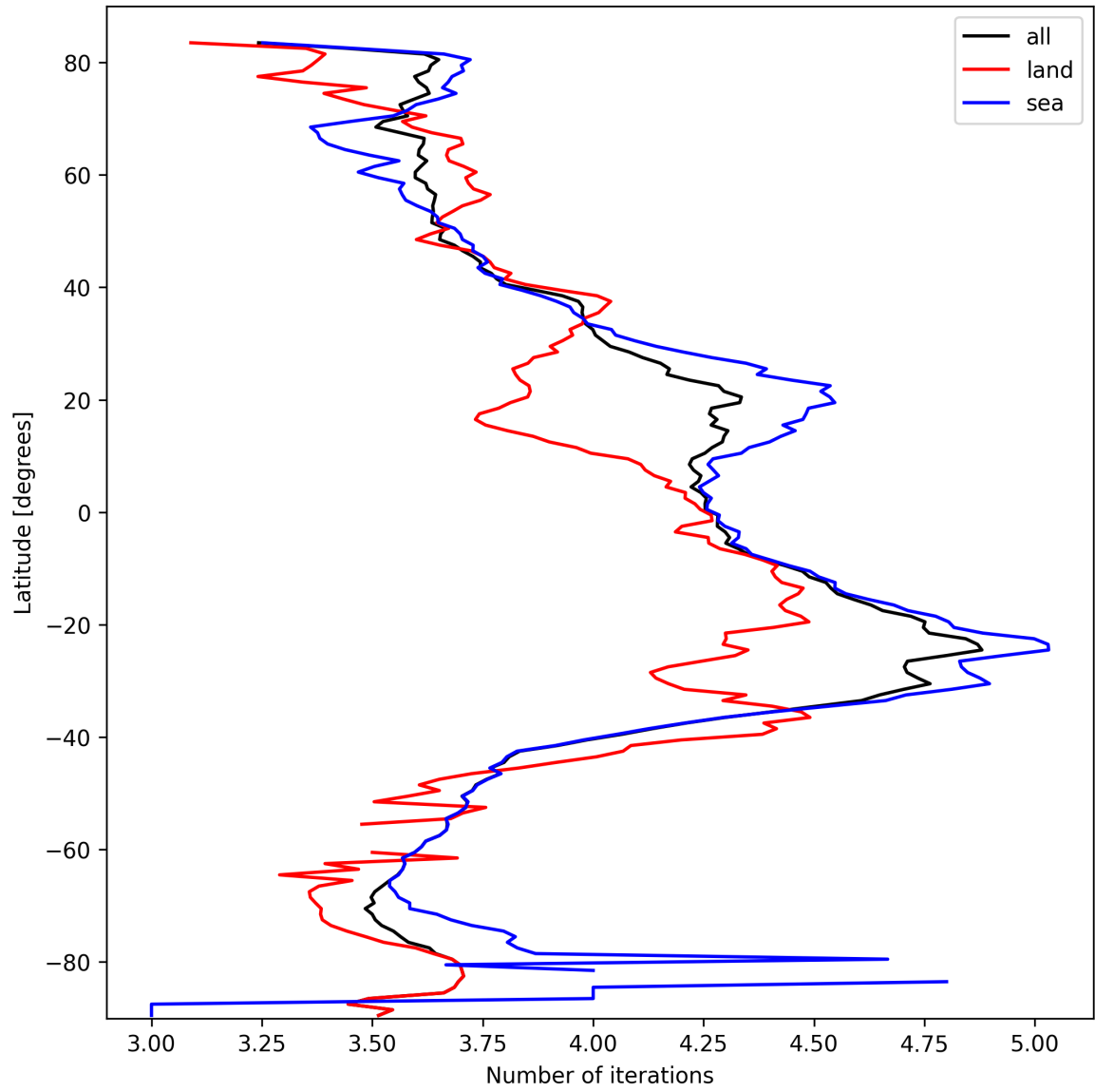
Figure 15: Zonal average of “Number of iterations” for 2025-03-08 to 2025-03-09.
