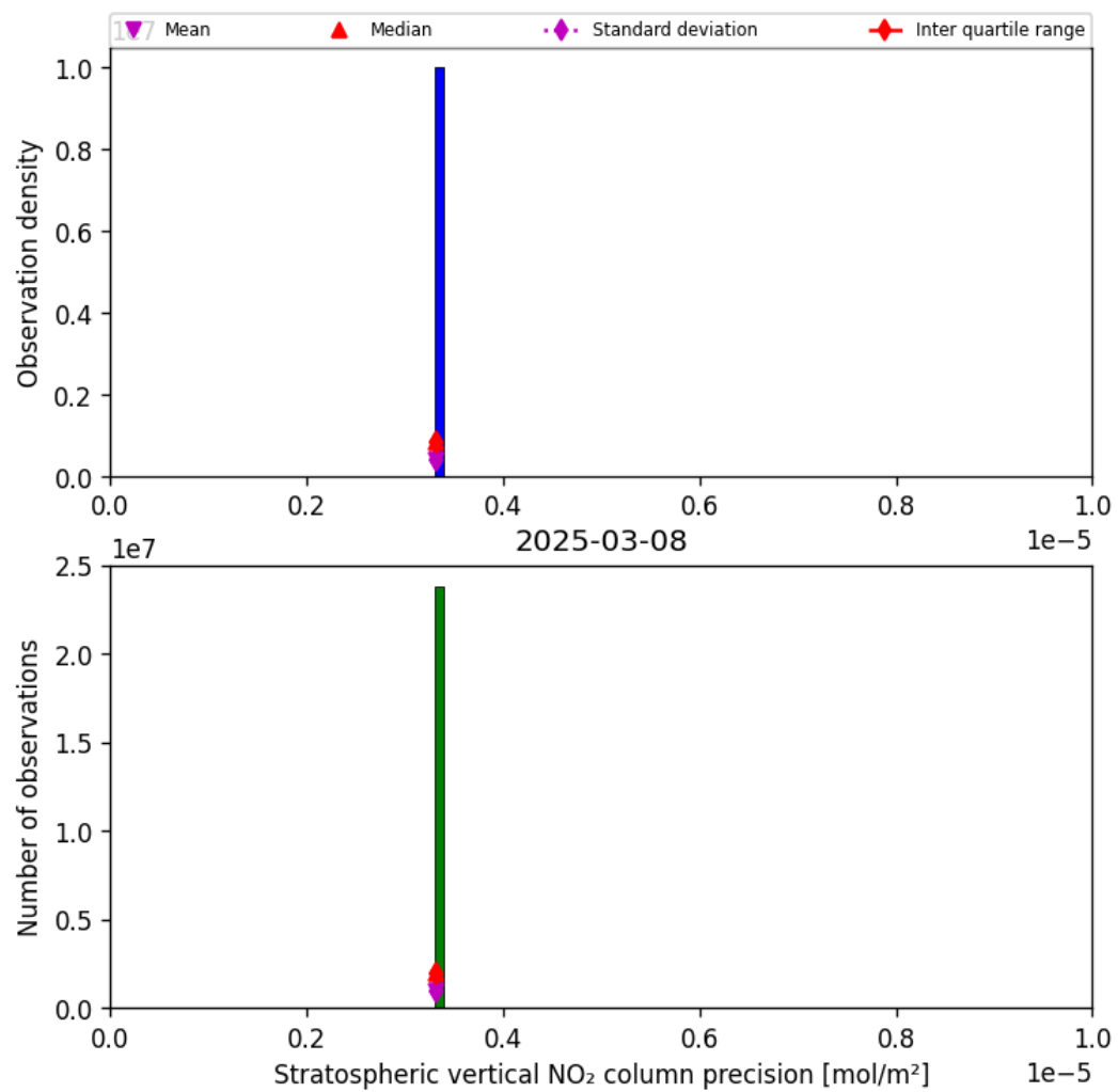
Figure 35: Histogram of “Stratospheric vertical NO 2 column precision” for 2025-03-08 to 2025-03-09
