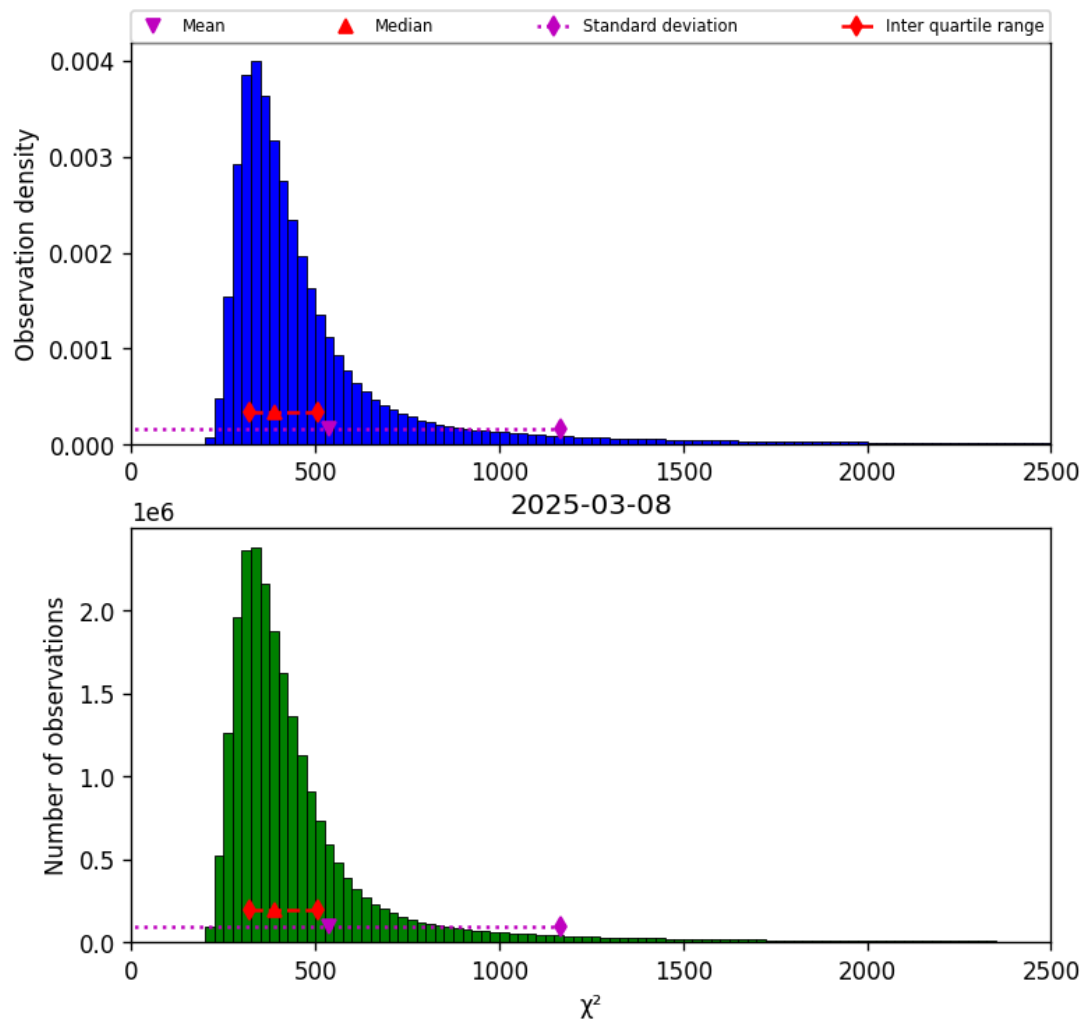
Figure 40: Histogram of “ \chi^2 ” for 2025-03-08 to 2025-03-09
