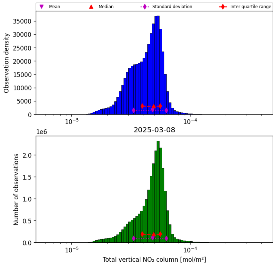
Figure 36: Histogram of “Total vertical NO 2 column” for 2025-03-08 to 2025-03-09
