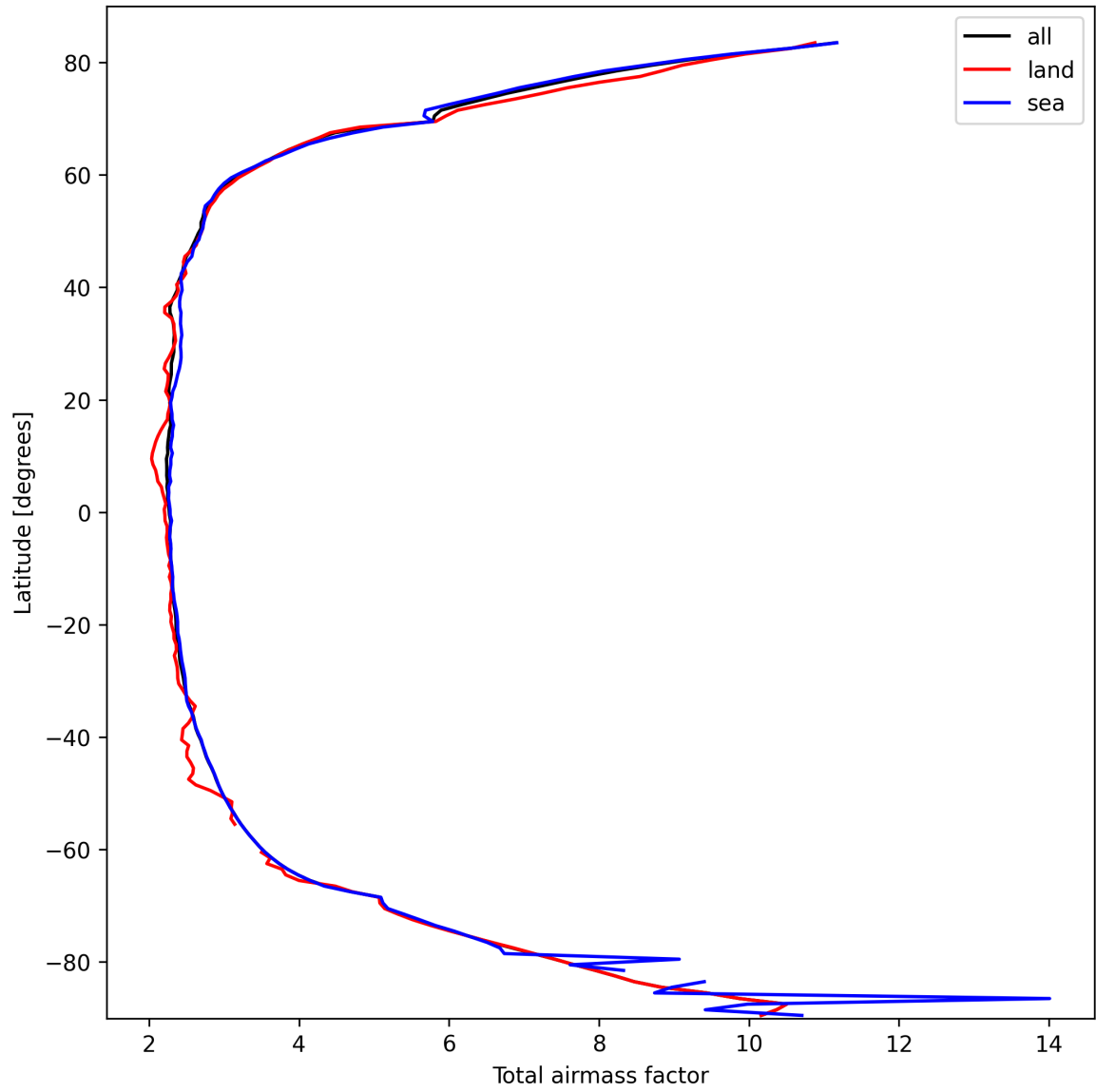
Figure 13: Zonal average of “Total airmass factor” for 2025-03-08 to 2025-03-09.
