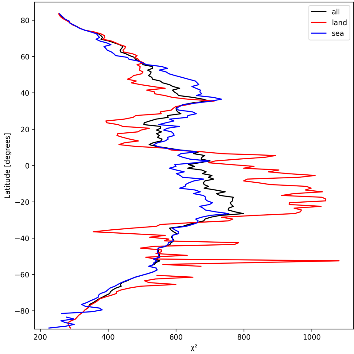
Figure 23: Zonal average of “ \chi^2 ” for 2025-03-08 to 2025-03-09.
