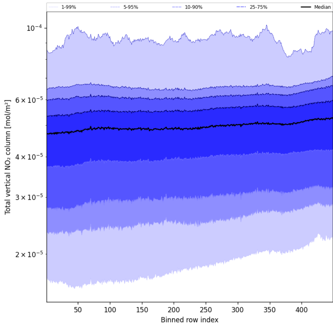
Figure 53: Along track statistics of “Total vertical NO 2 column” for 2025-03-08 to 2025-03-09
