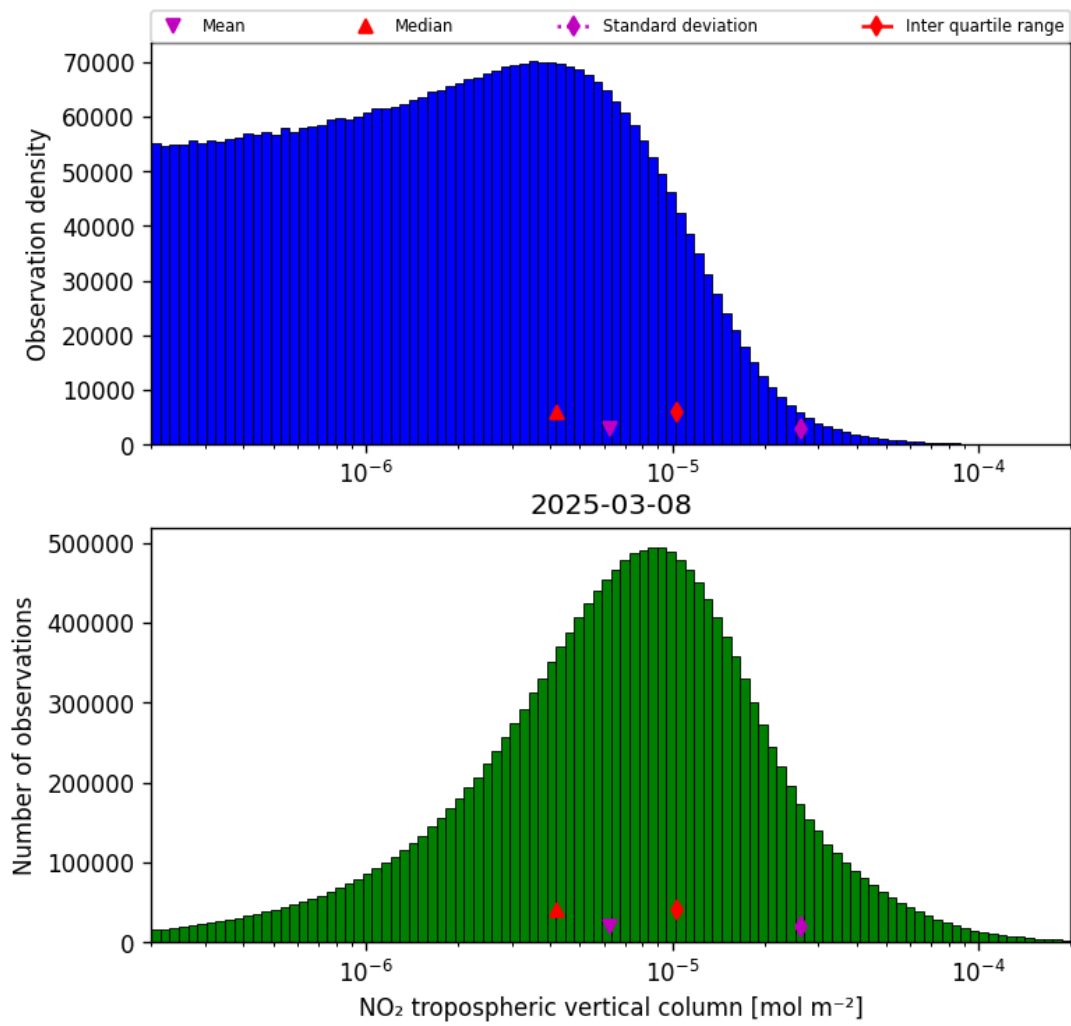
Figure 27: Histogram of “NO 2 tropospheric vertical column” for 2025-03-08 to 2025-03-09
