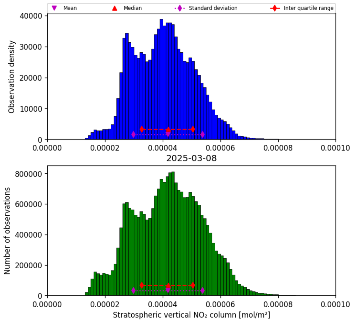
Figure 34: Histogram of “Stratospheric vertical NO 2 column” for 2025-03-08 to 2025-03-09
