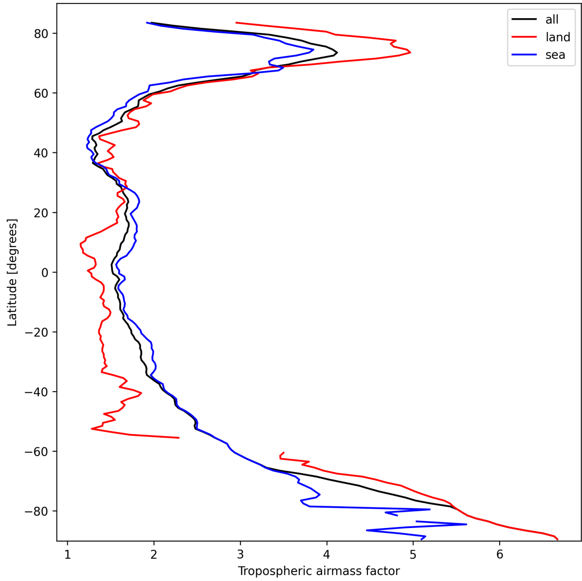
Figure 12: Zonal average of “Tropospheric air mass factor” for 2025-03-08 to 2025-03-09.
