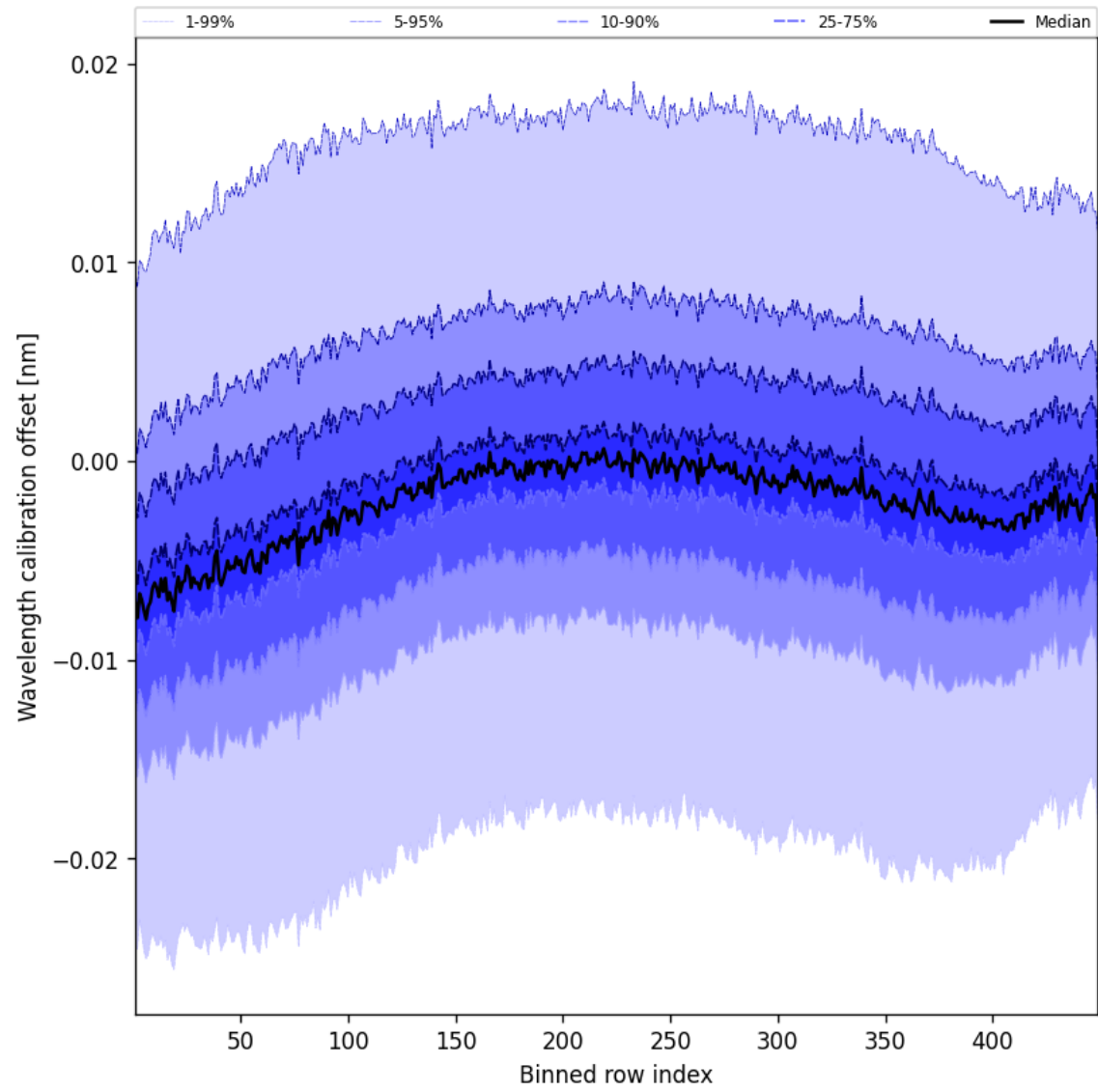
Figure 50: Along track statistics of “Wavelength calibration offset” for 2025-03-08 to 2025-03-09
