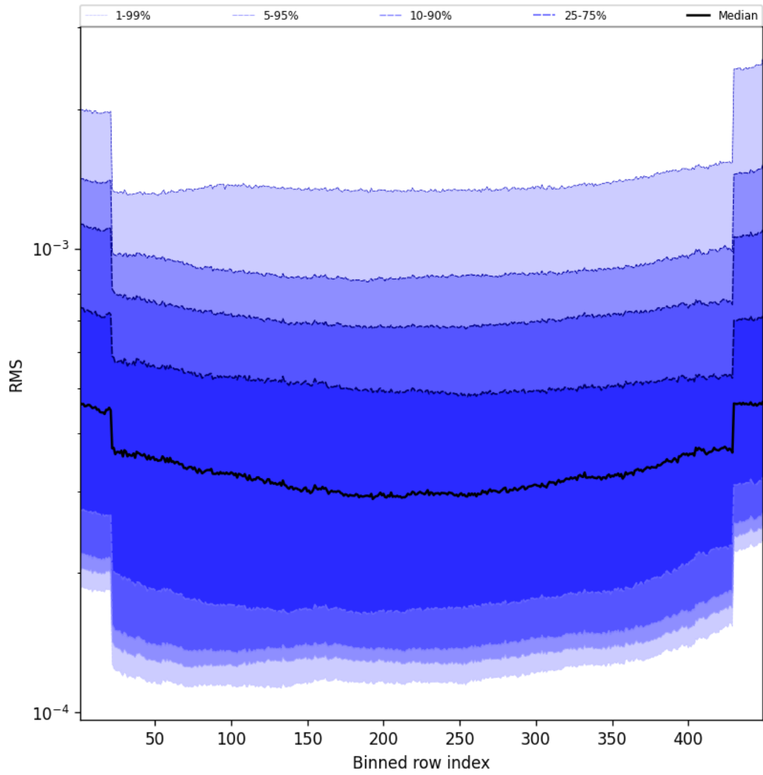
Figure 58: Along track statistics of “RMS” for 2025-03-09 to 2025-03-10
