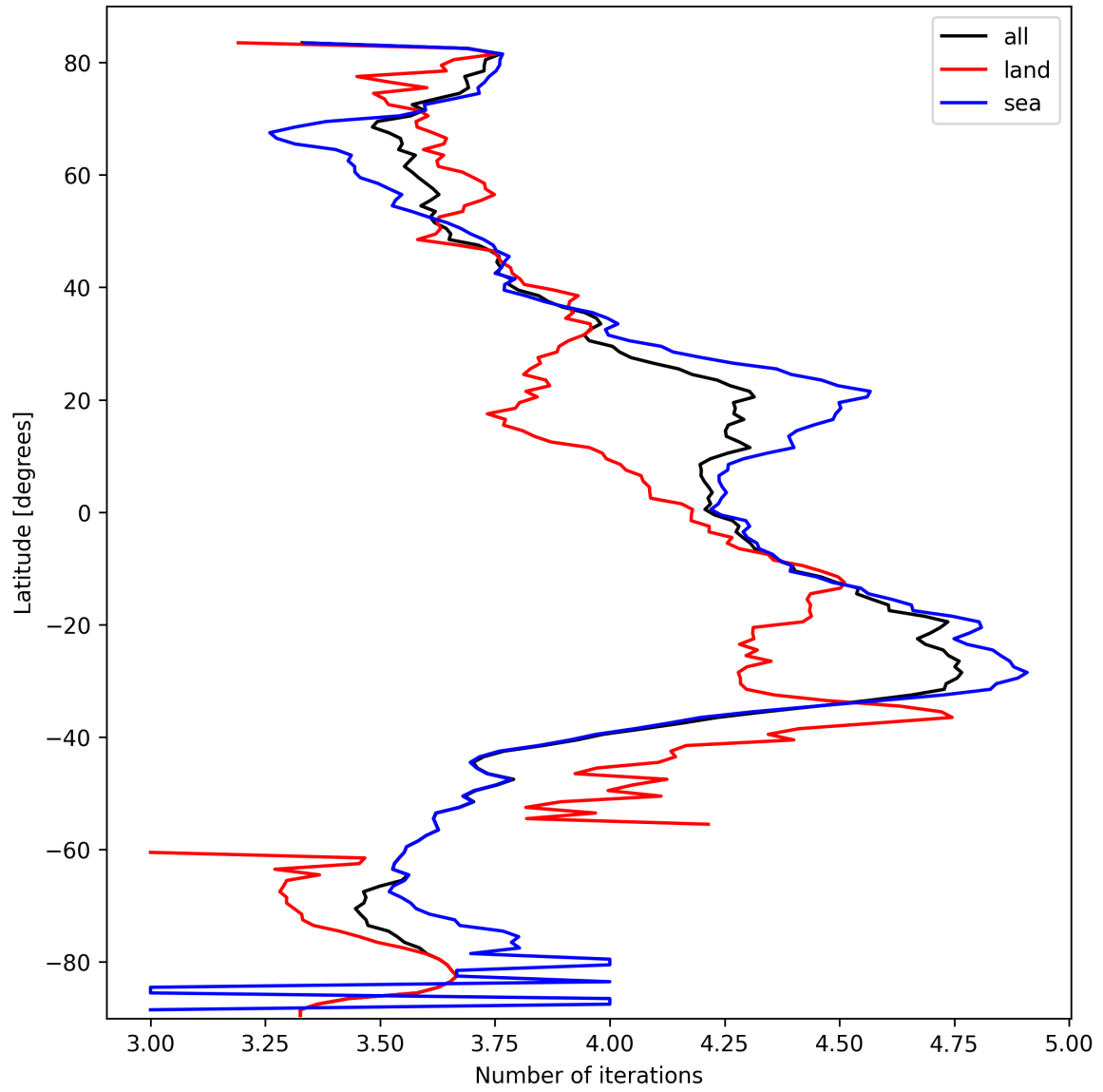
Figure 15: Zonal average of “Number of iterations” for 2025-03-09 to 2025-03-10.
