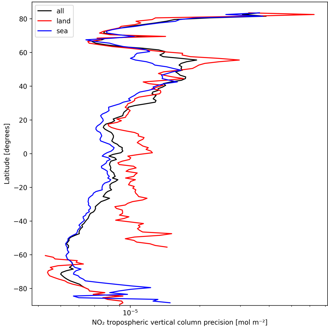
Figure 11: Zonal average of “NO 2 tropospheric vertical column precision” for 2025-03-09 to 2025-03-10.
