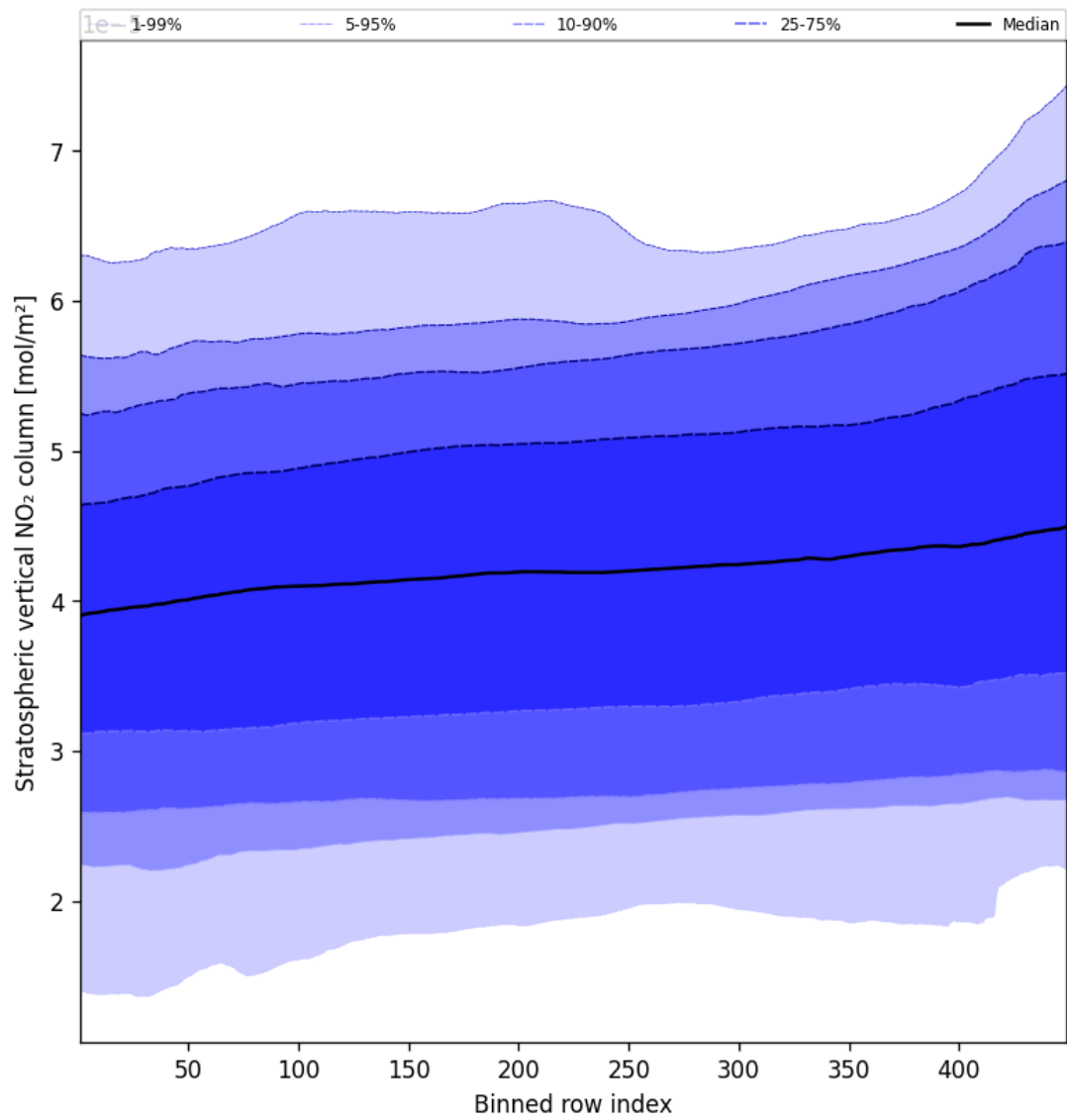
Figure 51: Along track statistics of “Stratospheric vertical NO 2 column” for 2025-03-09 to 2025-03-10
