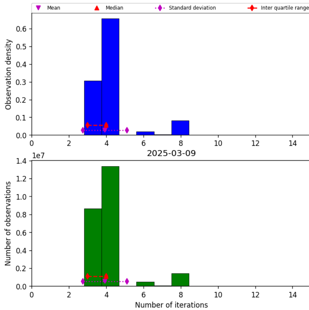
Figure 32: Histogram of “Number of iterations” for 2025-03-09 to 2025-03-10
