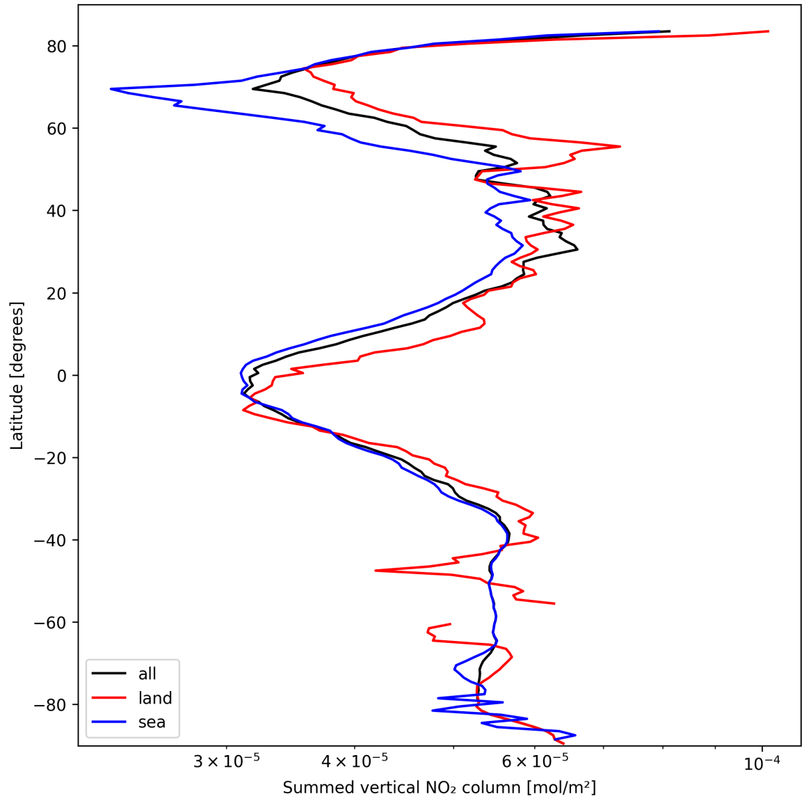
Figure 21: Zonal average of “Summed vertical NO 2 column” for 2025-03-09 to 2025-03-10.
