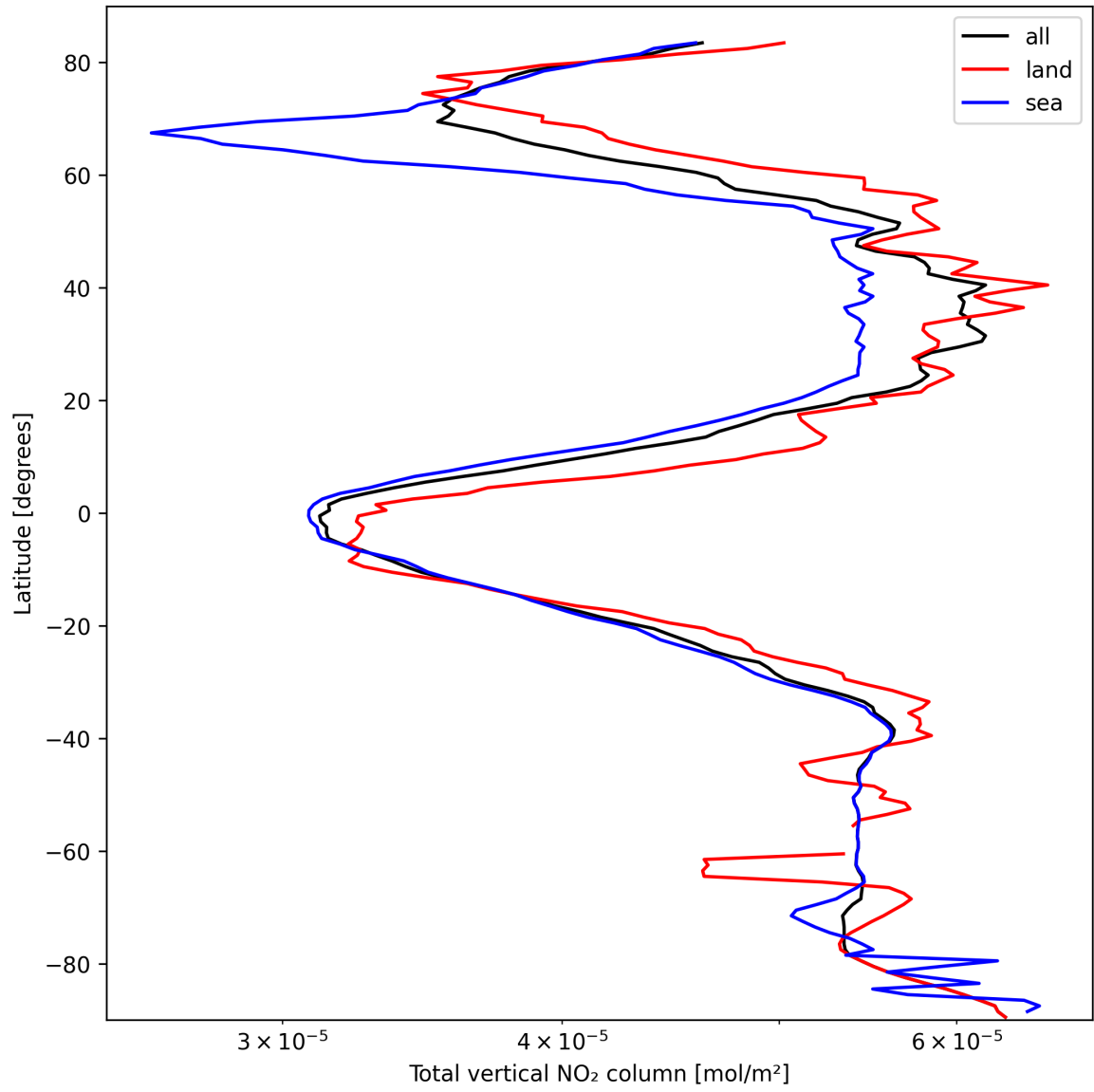
Figure 19: Zonal average of “Total vertical NO 2 column” for 2025-03-09 to 2025-03-10.
