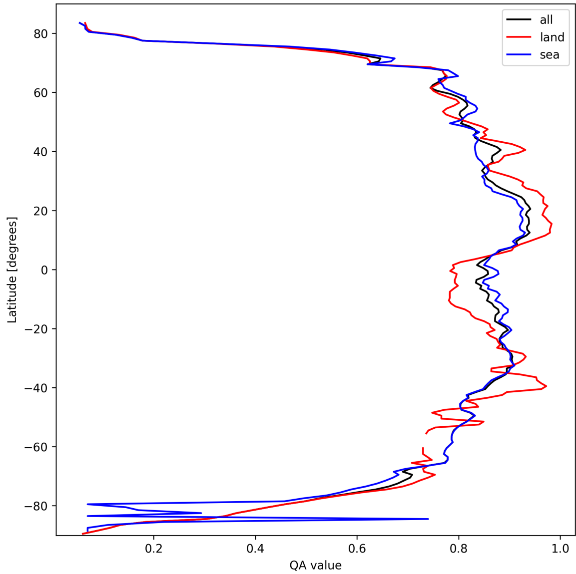
Figure 9: Zonal average of “QA value” for 2025-03-09 to 2025-03-10.
