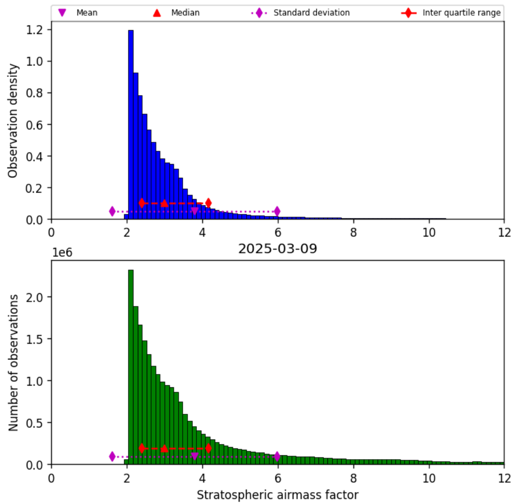
Figure 42: Histogram of “Stratospheric airmass factor” for 2025-03-09 to 2025-03-10
