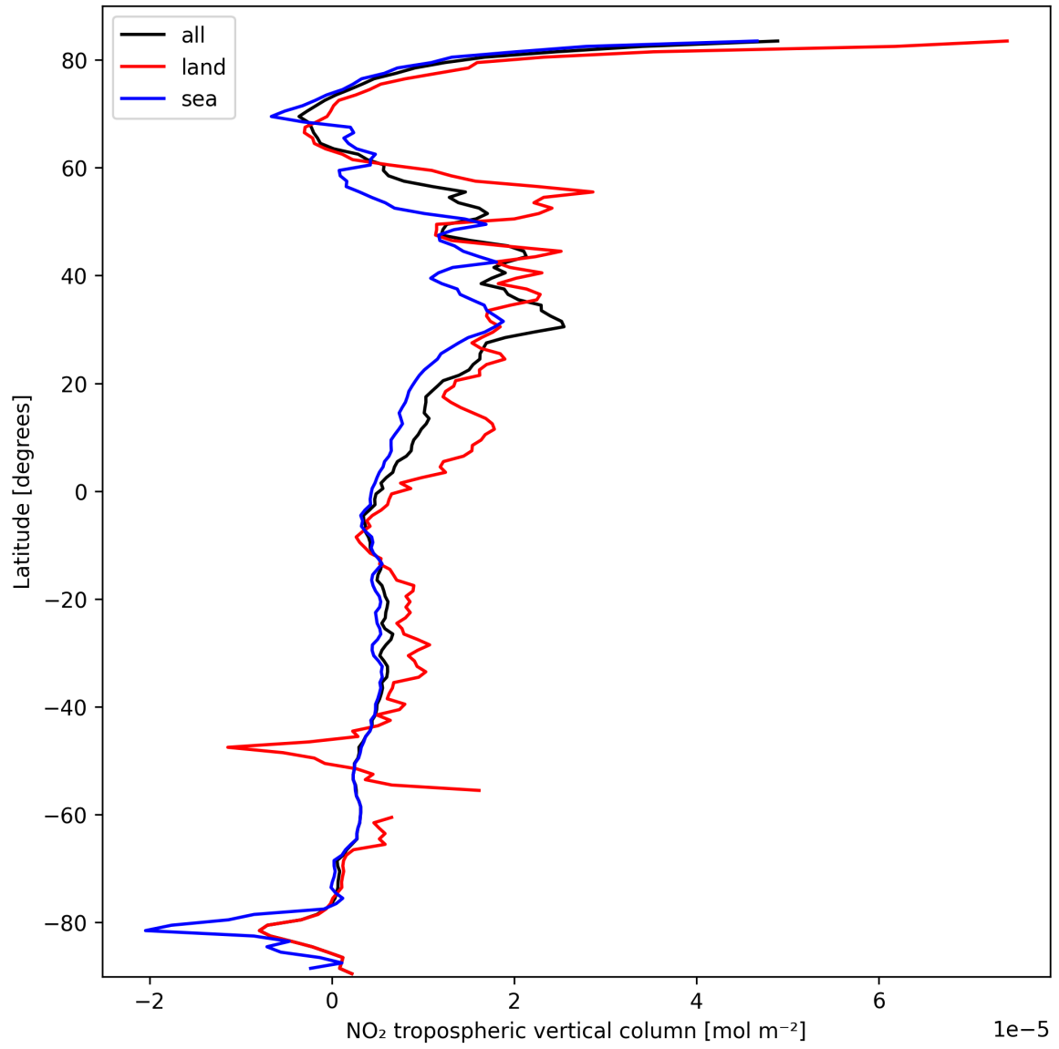
Figure 10: Zonal average of “NO 2 tropospheric vertical column” for 2025-03-09 to 2025-03-10.
