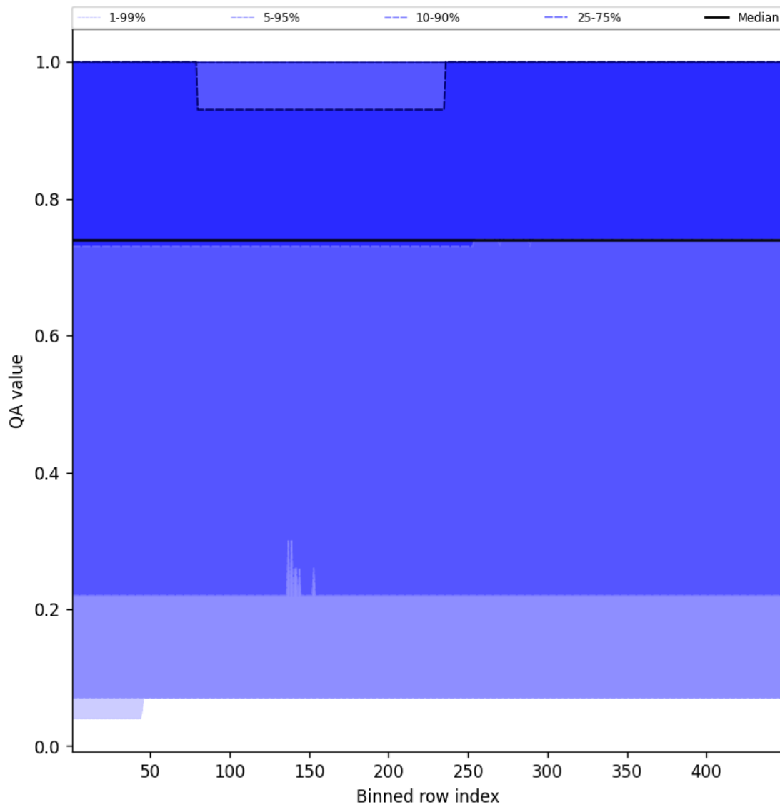
Figure 43: Along track statistics of “QA value” for 2025-03-09 to 2025-03-10
