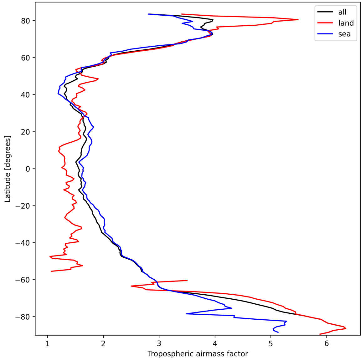
Figure 12: Zonal average of “Tropospheric airmass factor” for 2025-03-09 to 2025-03-10.
