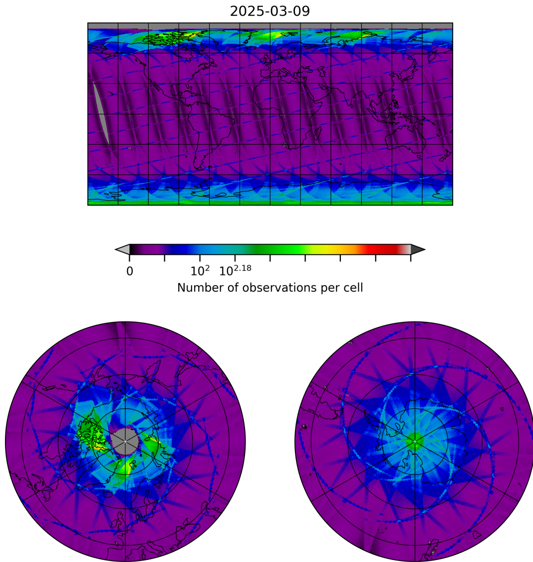
Figure 8: Map of the number of observations for 2025-03-09 to 2025-03-10
