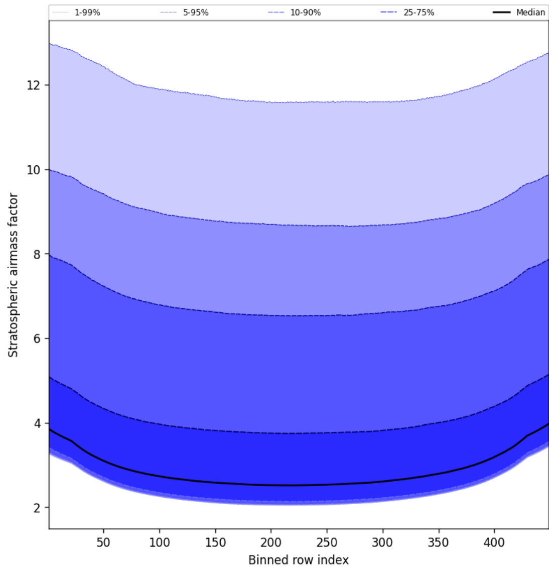
Figure 59: Along track statistics of “Stratospheric airmass factor” for 2025-03-09 to 2025-03-10
