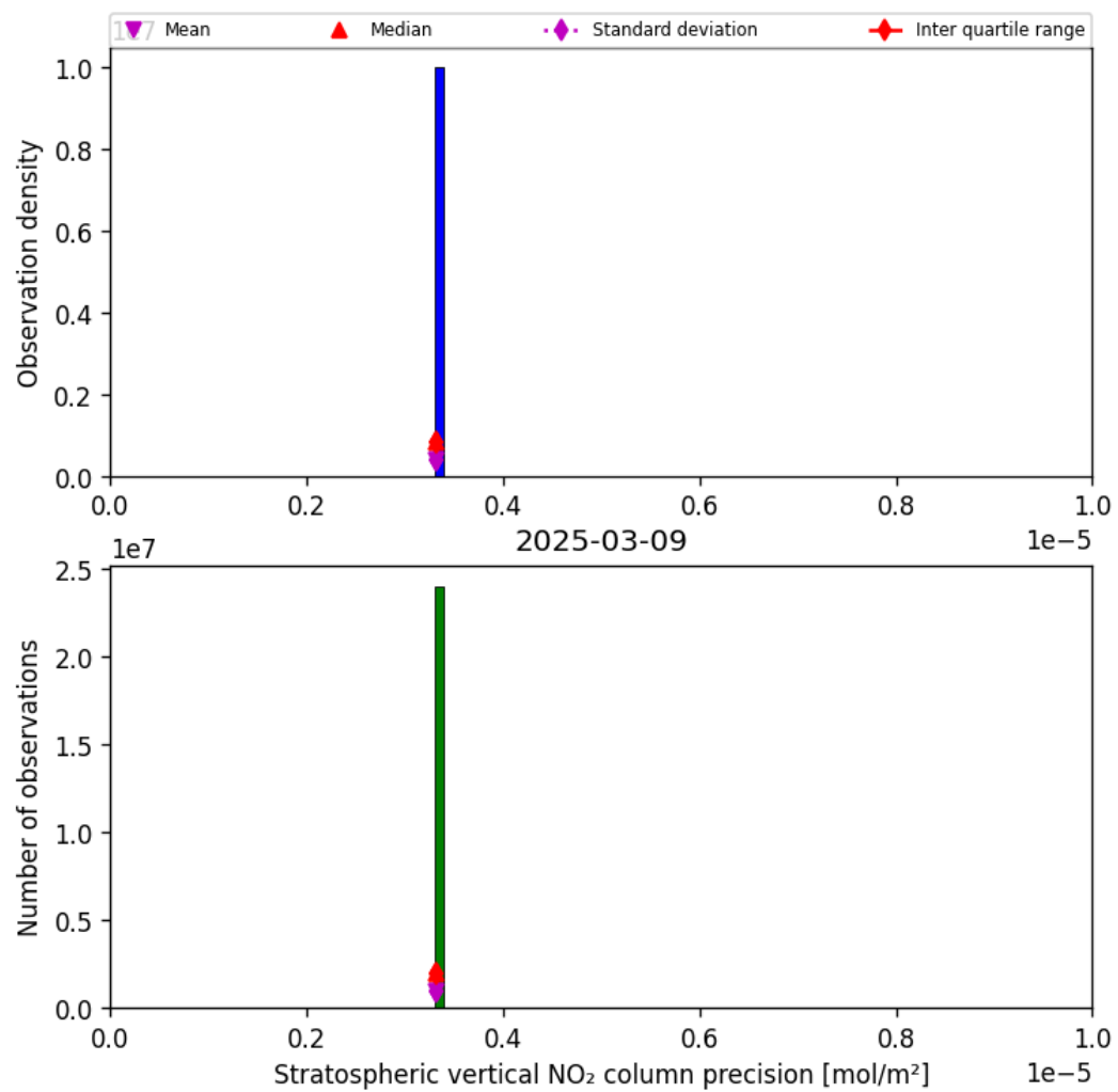
Figure 35: Histogram of “Stratospheric vertical NO 2 column precision” for 2025-03-09 to 2025-03-10
