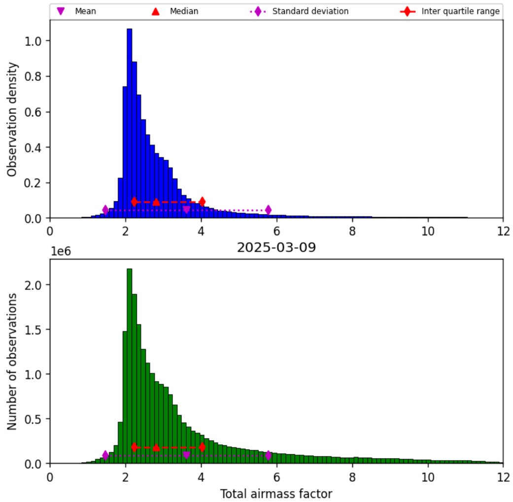
Figure 30: Histogram of “Total airmass factor” for 2025-03-09 to 2025-03-10
