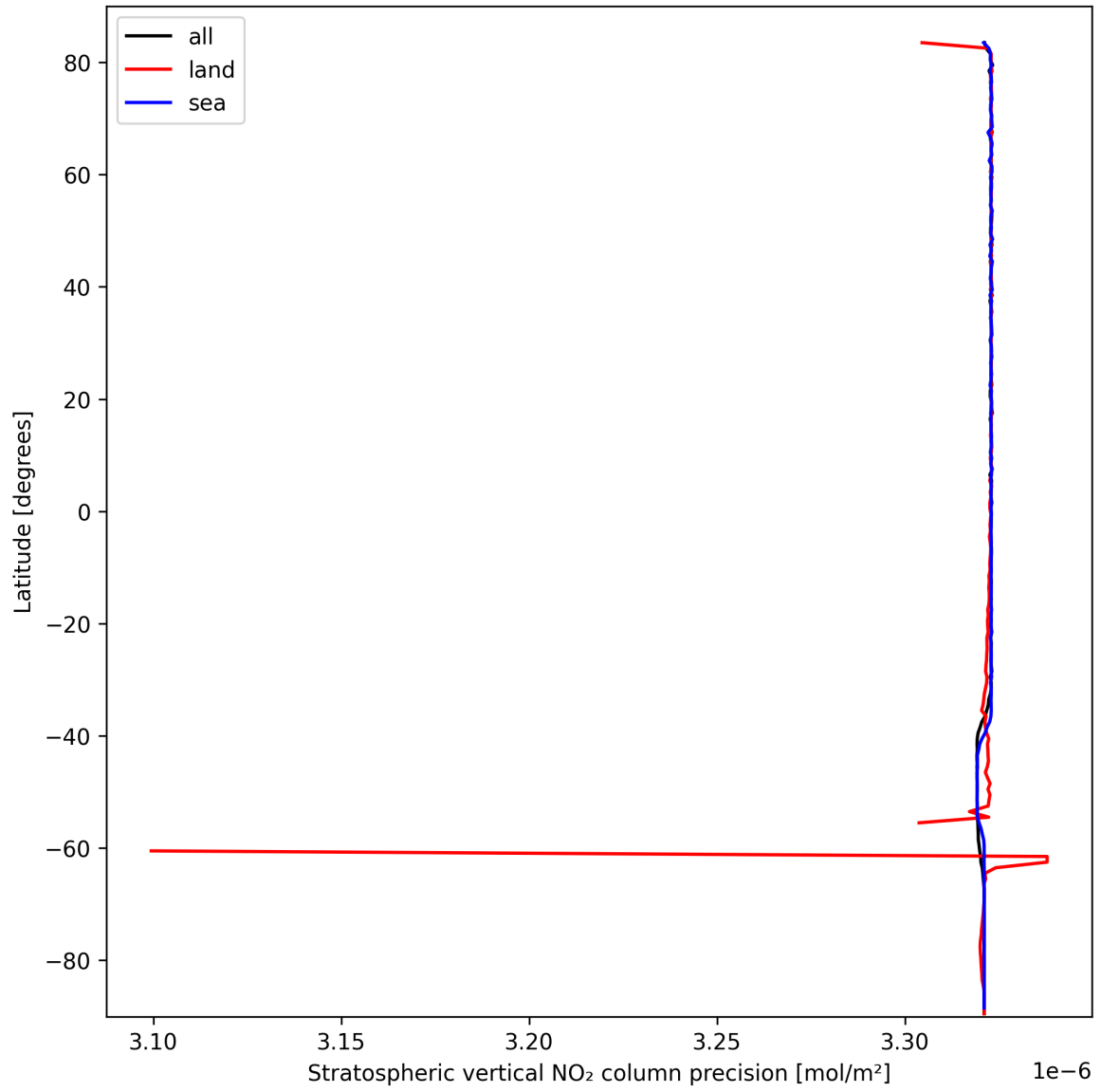
Figure 18: Zonal average of “Stratospheric vertical NO 2 column precision” for 2025-03-09 to 2025-03-10.
