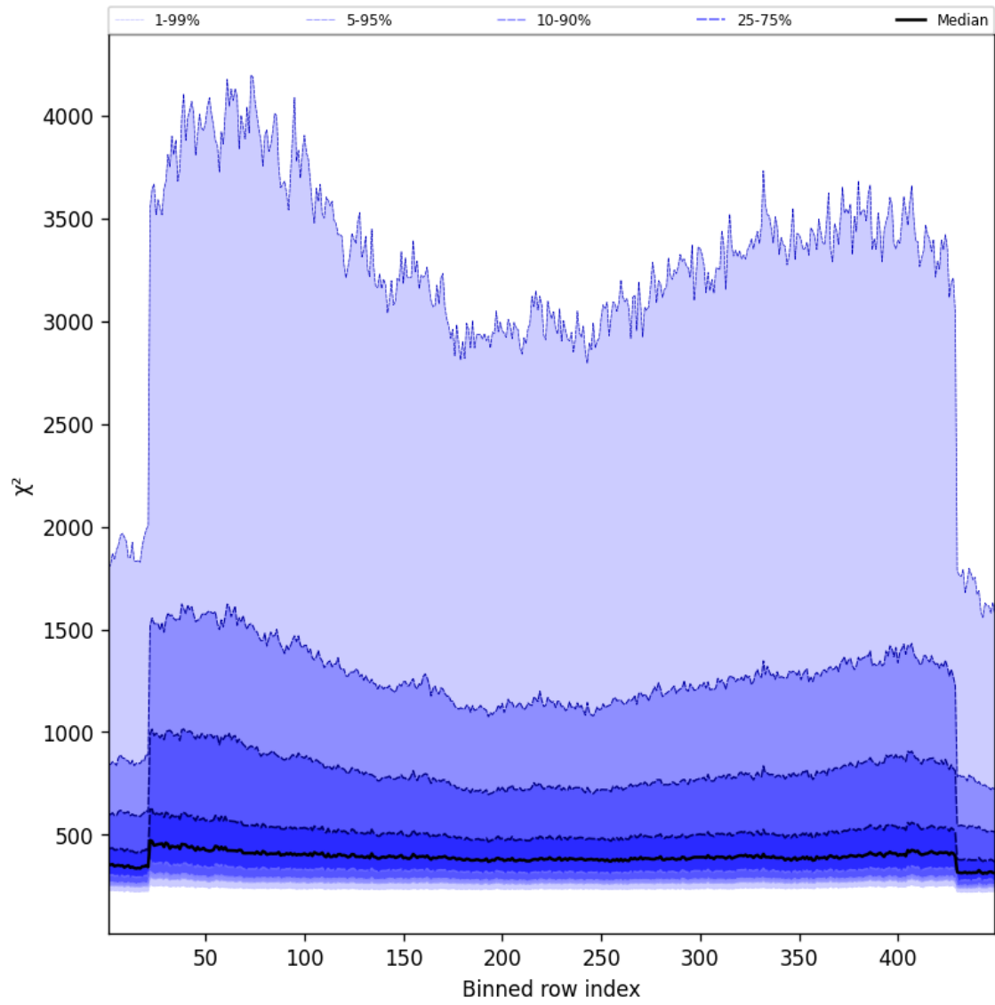
Figure 57: Along track statistics of “ \chi^2 ” for 2025-03-09 to 2025-03-10
