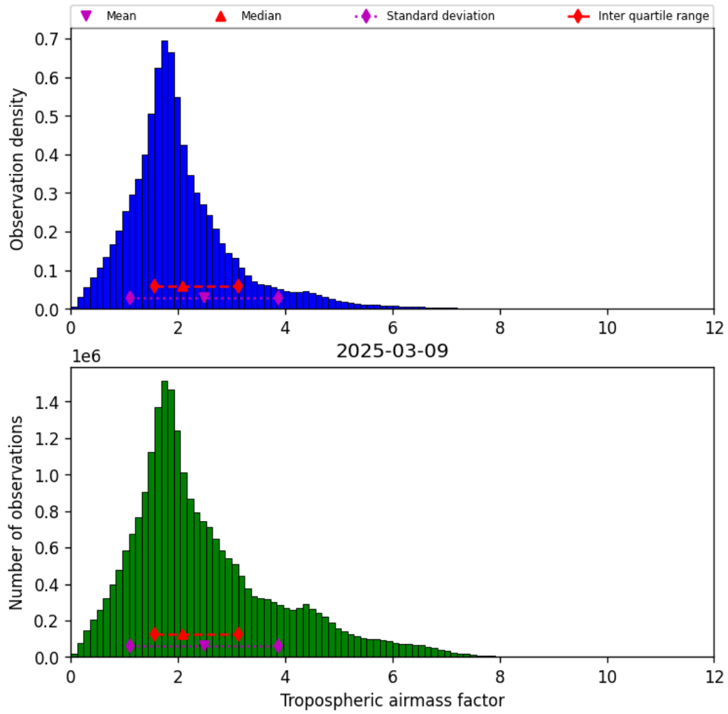
Figure 29: Histogram of “Tropospheric airmass factor” for 2025-03-09 to 2025-03-10
