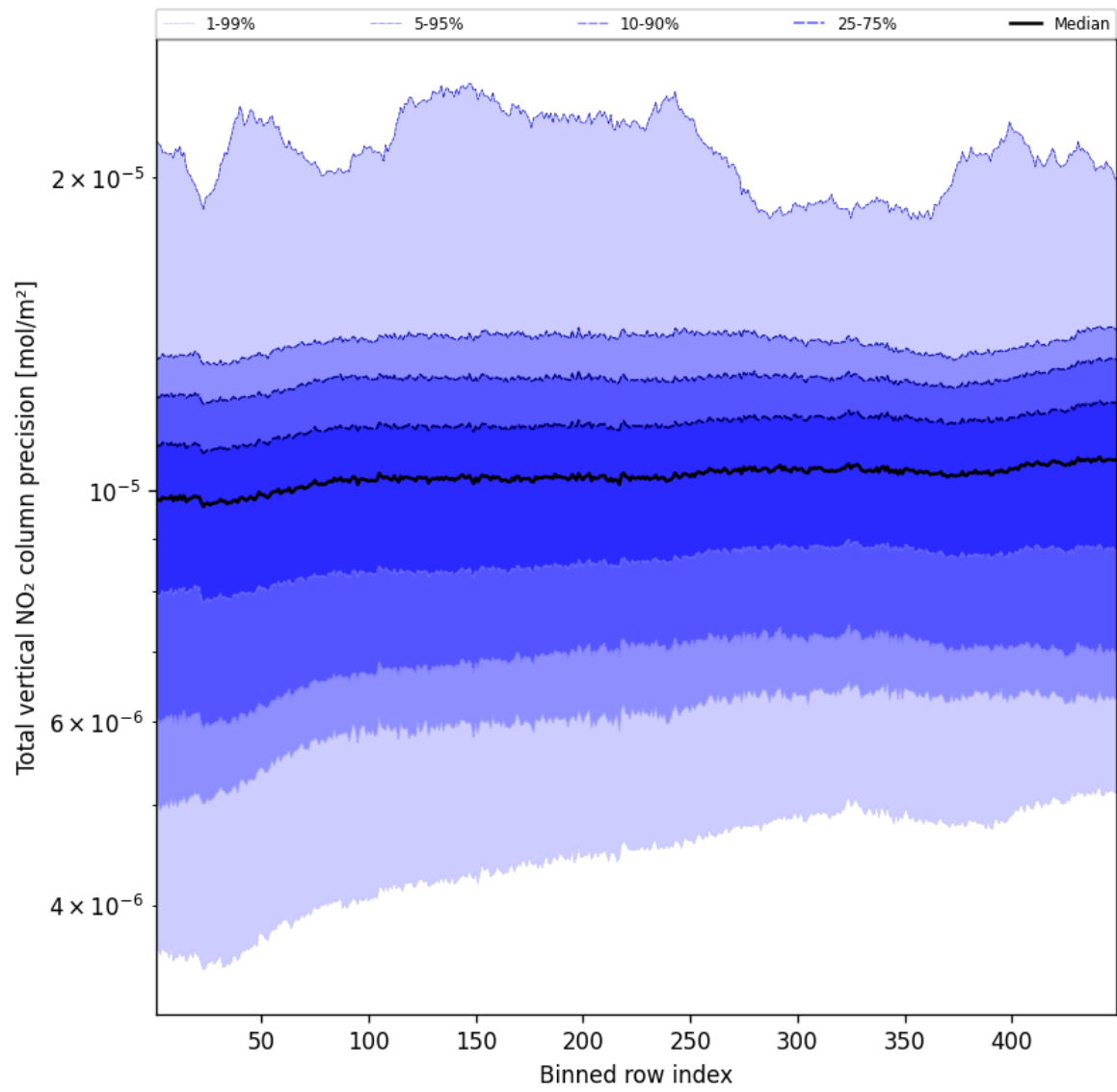
Figure 54: Along track statistics of “Total vertical NO 2 column precision” for 2025-03-09 to 2025-03-10
