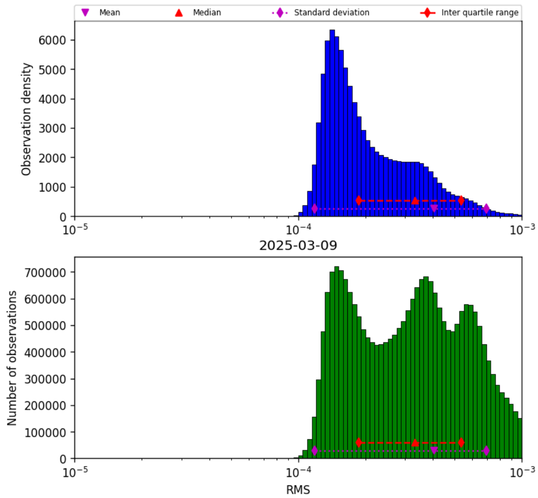
Figure 41: Histogram of “RMS” for 2025-03-09 to 2025-03-10
