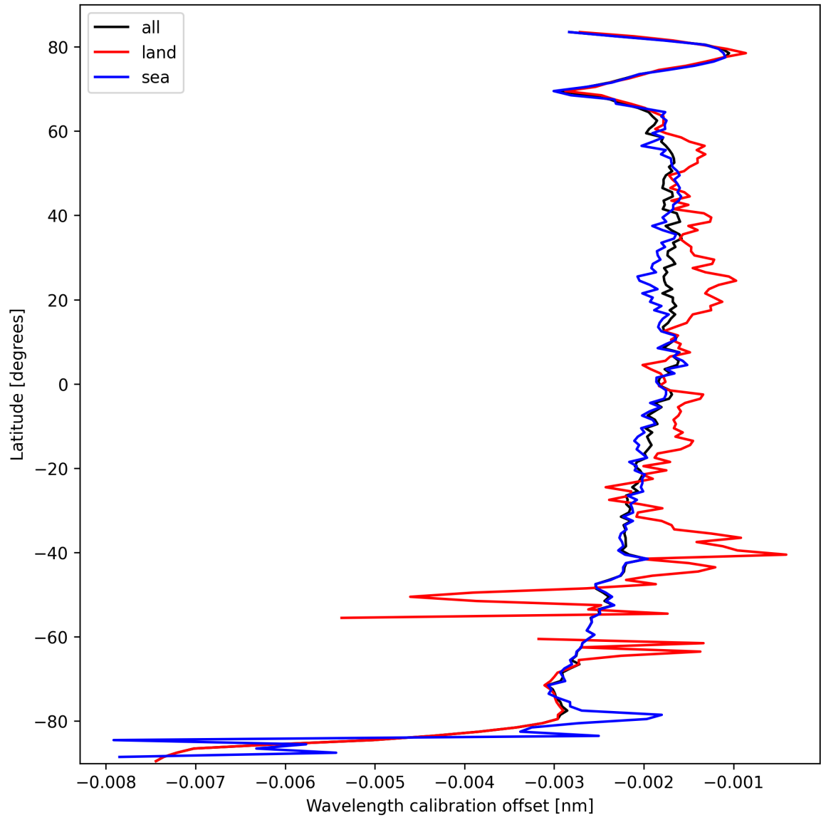
Figure 16: Zonal average of “Wavelength calibration offset” for 2025-03-09 to 2025-03-10.
