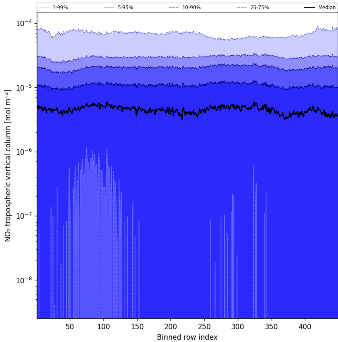
Figure 44: Along track statistics of “NO 2 tropospheric vertical column” for 2025-03-09 to 2025-03-10
