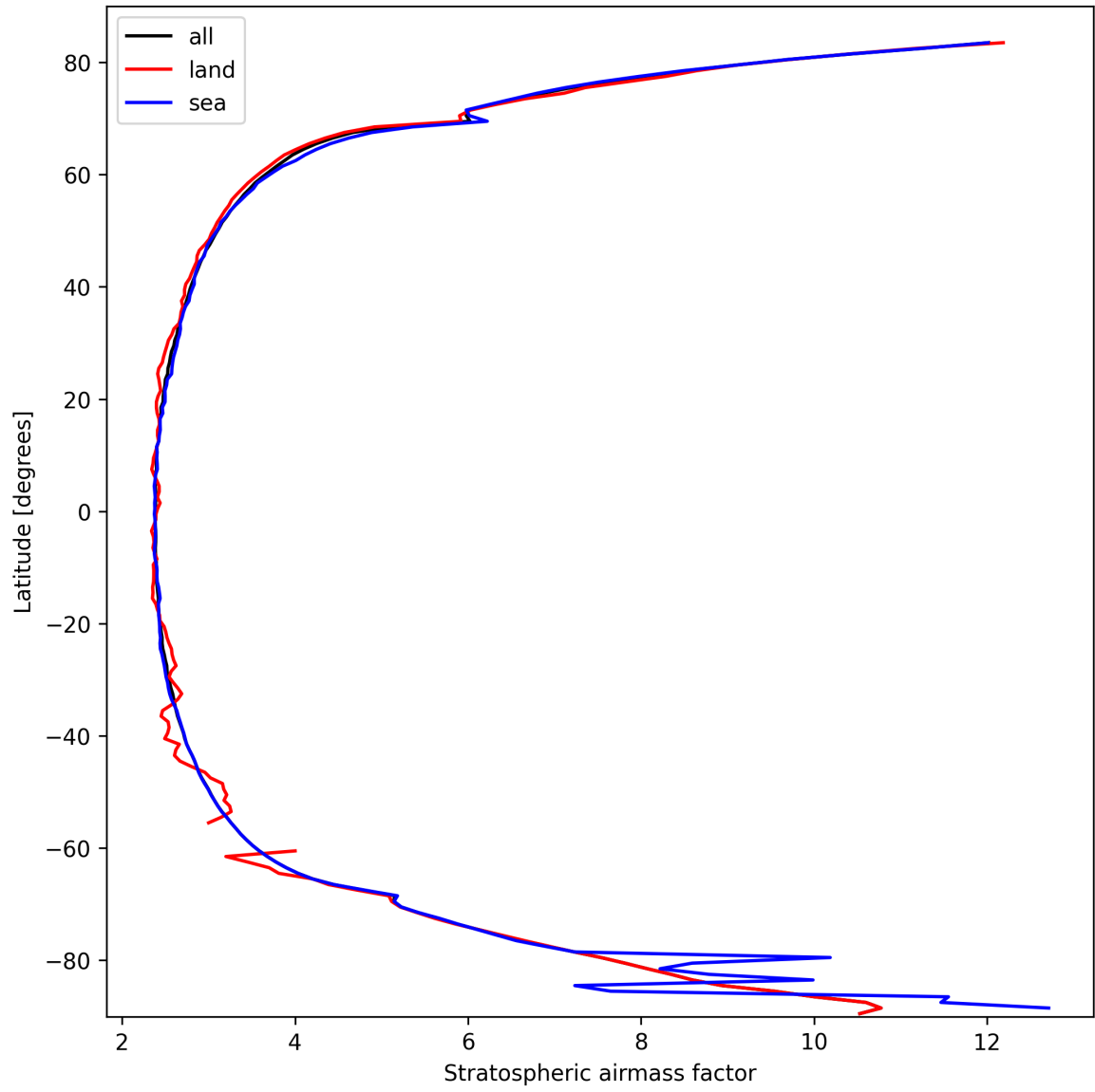
Figure 25: Zonal average of “Stratospheric air mass factor” for 2025-03-09 to 2025-03-10.
