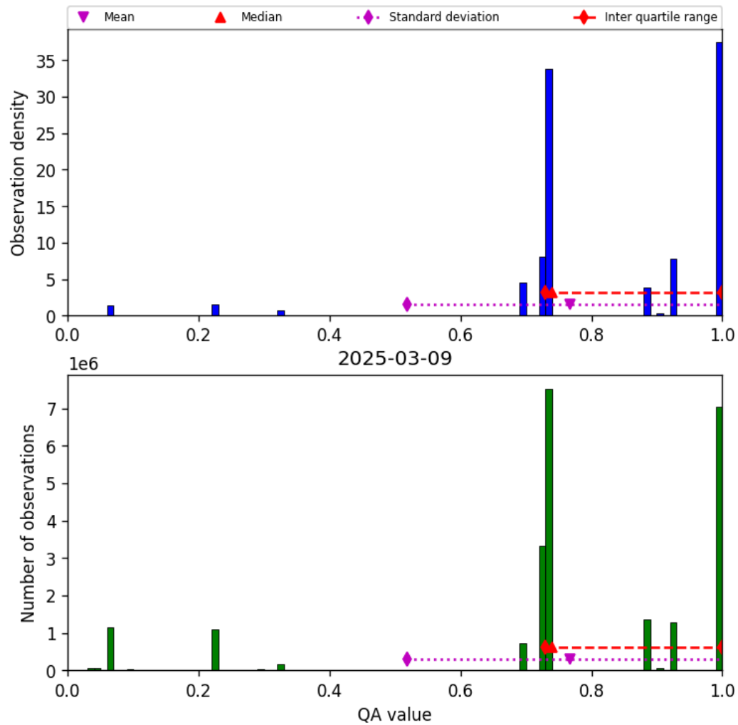
Figure 26: Histogram of “QA value” for 2025-03-09 to 2025-03-10
