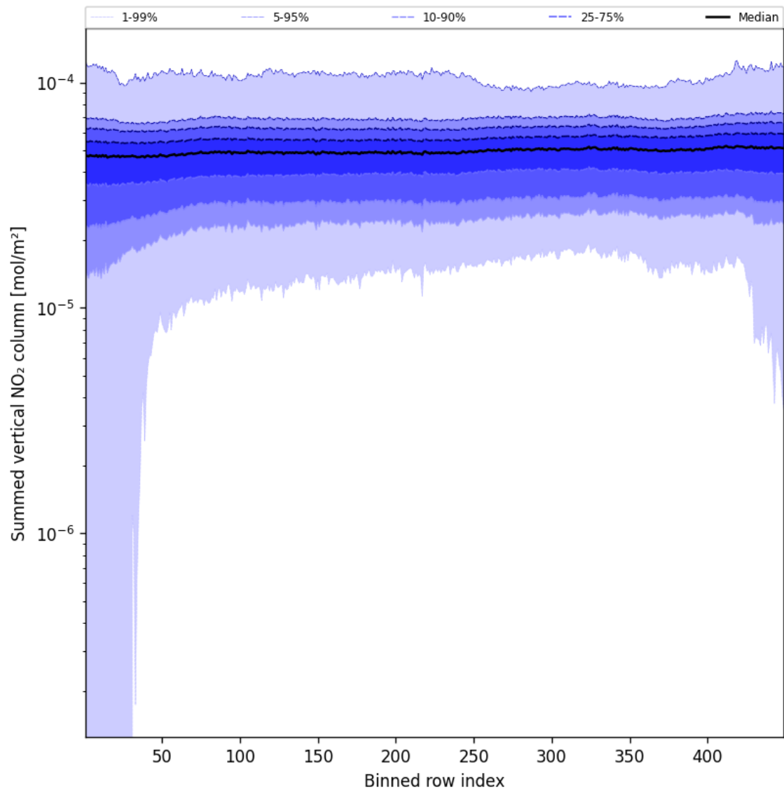
Figure 55: Along track statistics of “Summed vertical NO 2 column” for 2025-03-09 to 2025-03-10
