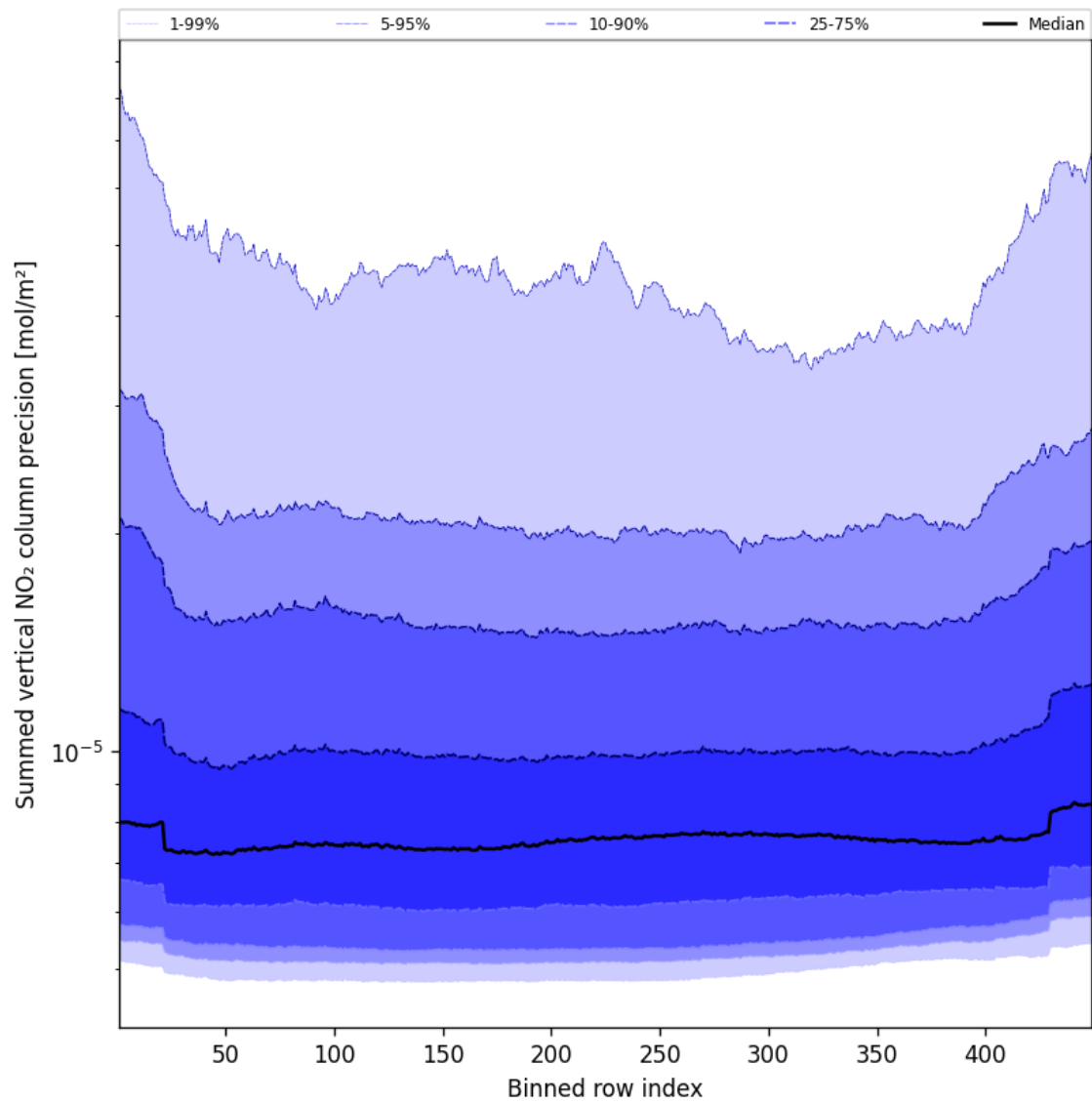
Figure 56: Along track statistics of “Summed vertical NO 2 column precision” for 2025-03-09 to 2025-03-10
