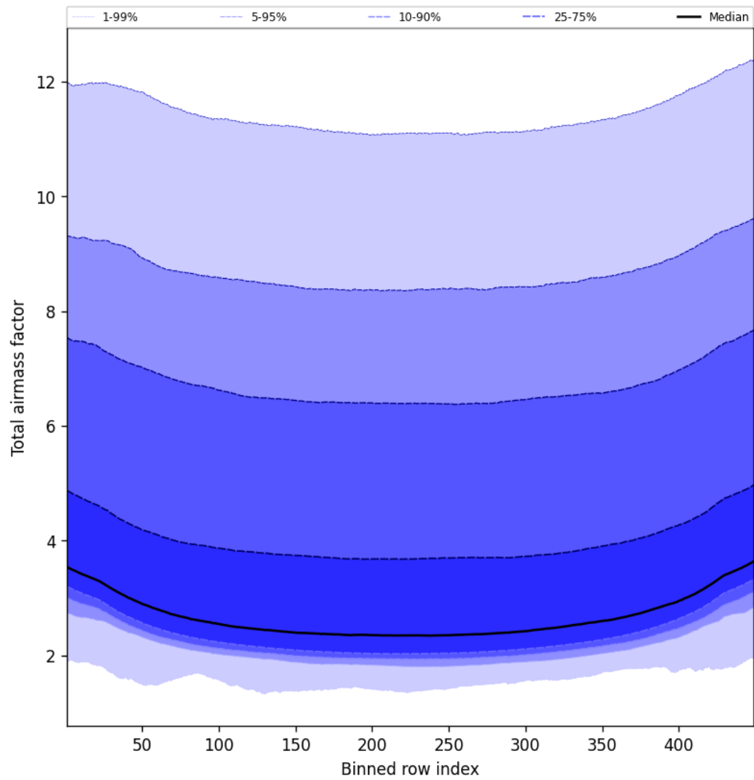
Figure 47: Along track statistics of “Total airmass factor” for 2025-03-09 to 2025-03-10
