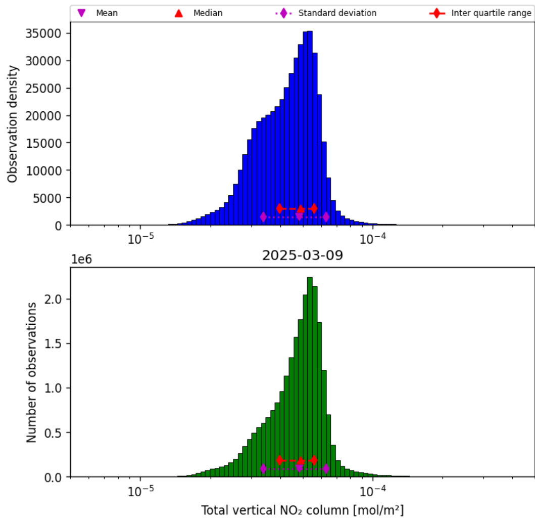
Figure 36: Histogram of “Total vertical NO 2 column” for 2025-03-09 to 2025-03-10
