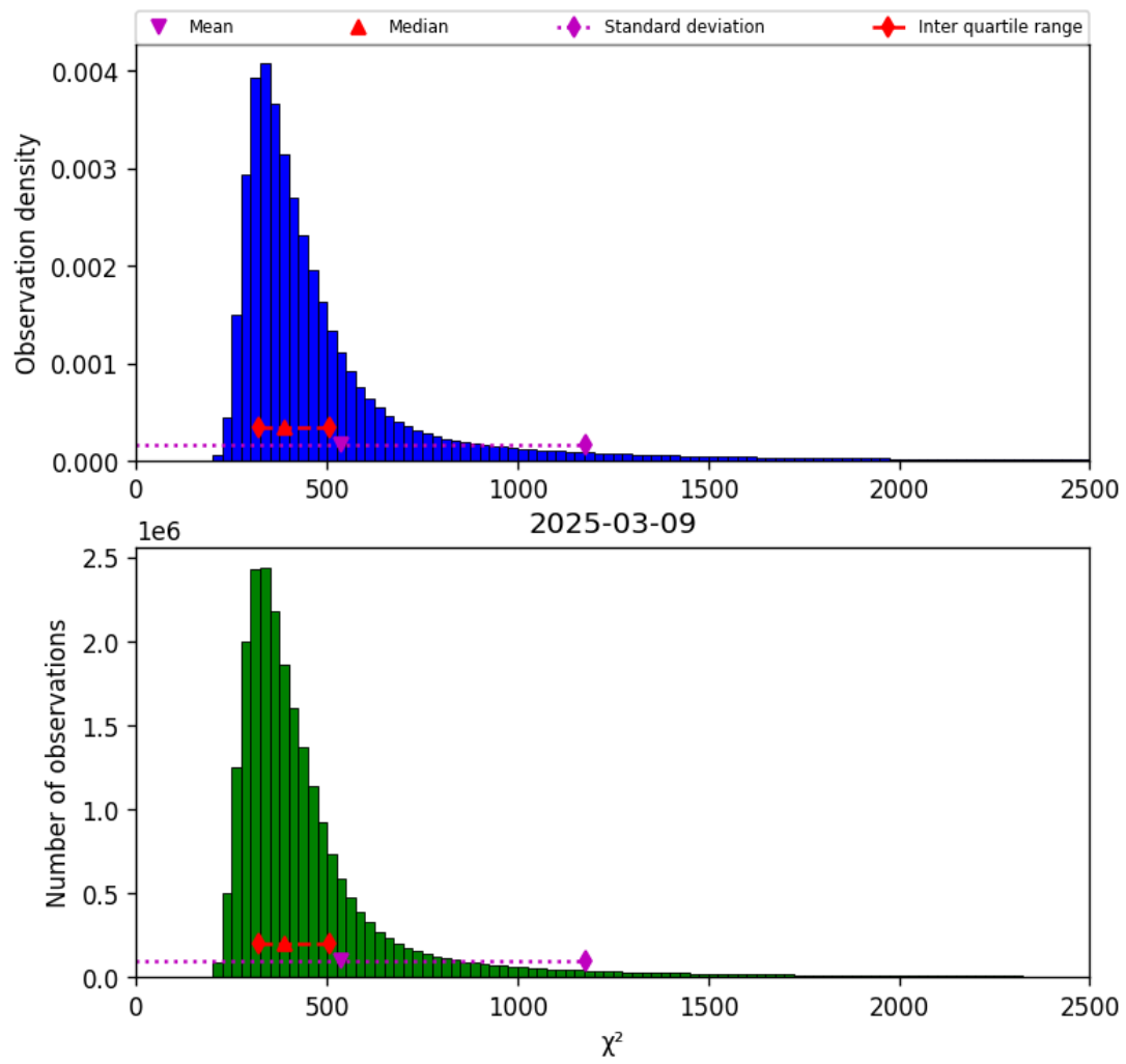
Figure 40: Histogram of “ \chi^2 ” for 2025-03-09 to 2025-03-10
