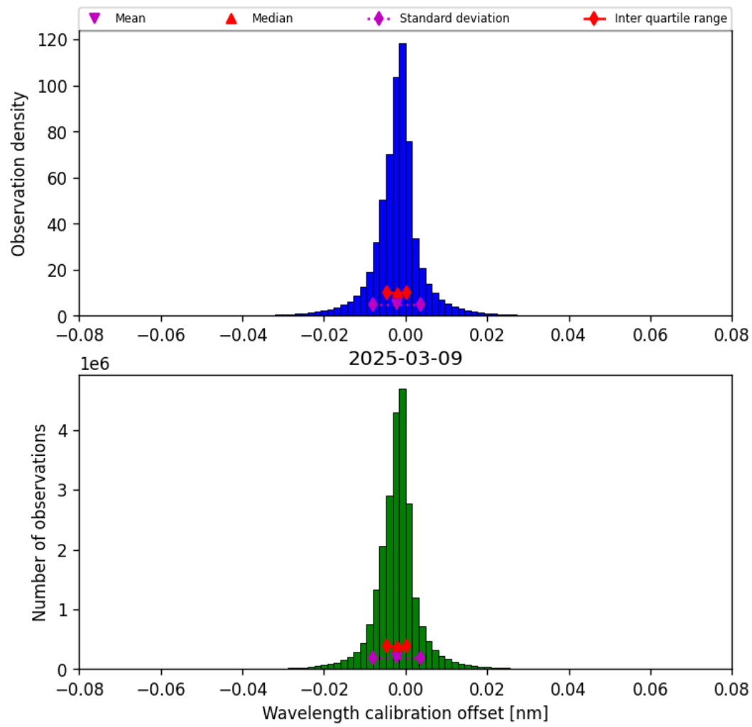
Figure 33: Histogram of “Wavelength calibration offset” for 2025-03-09 to 2025-03-10
