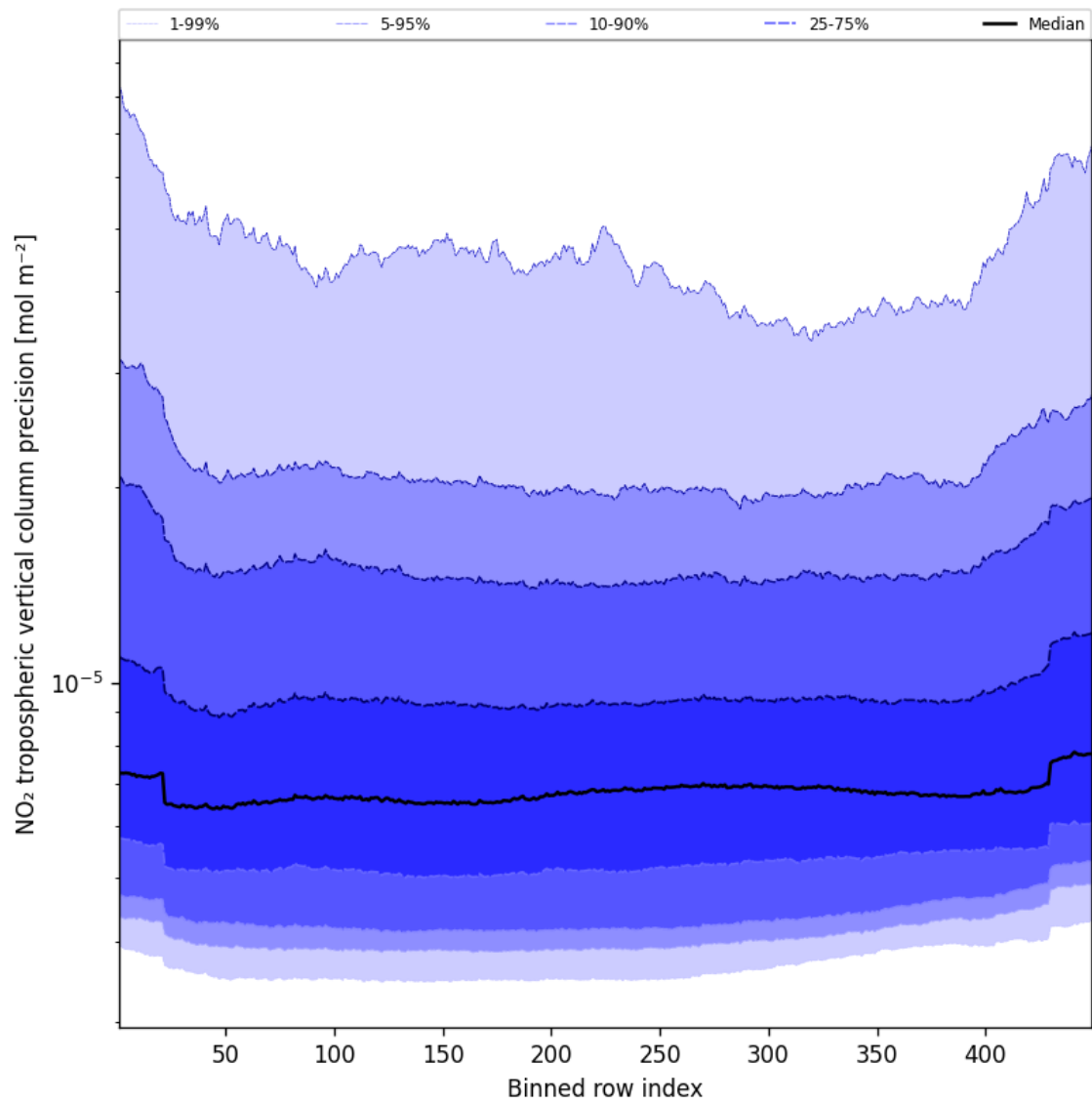
Figure 45: Along track statistics of “NO 2 tropospheric vertical column precision” for 2025-03-09 to 2025-03-10
