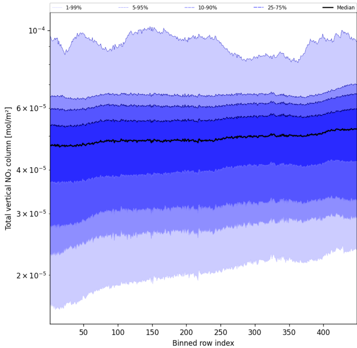
Figure 53: Along track statistics of “Total vertical NO 2 column” for 2025-03-09 to 2025-03-10
