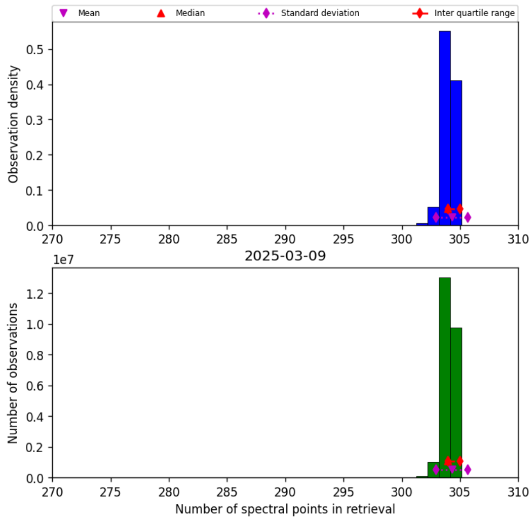
Figure 31: Histogram of “Number of spectral points in retrieval” for 2025-03-09 to 2025-03-10
