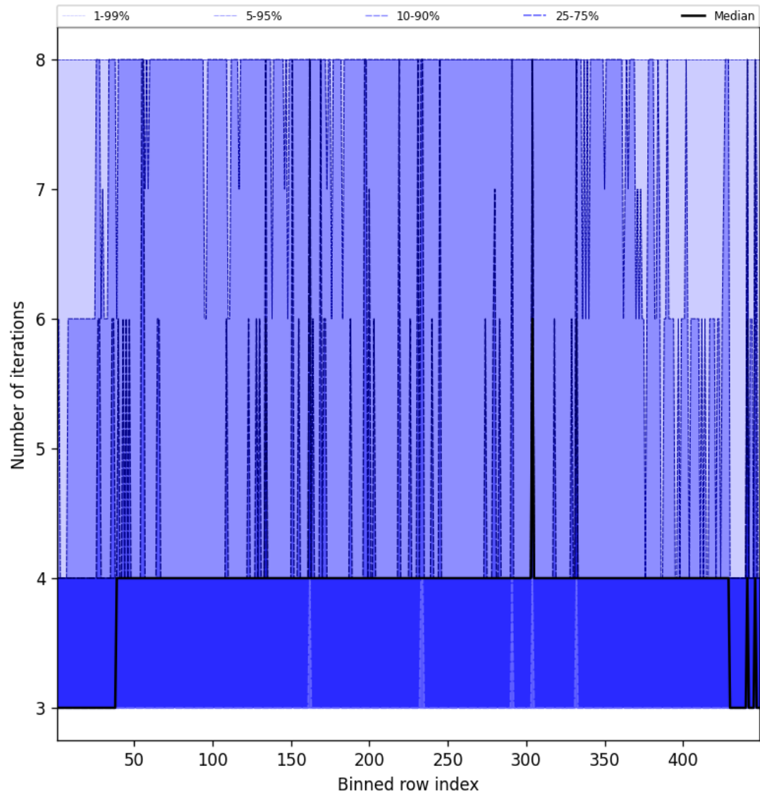
Figure 49: Along track statistics of “Number of iterations” for 2025-03-09 to 2025-03-10
