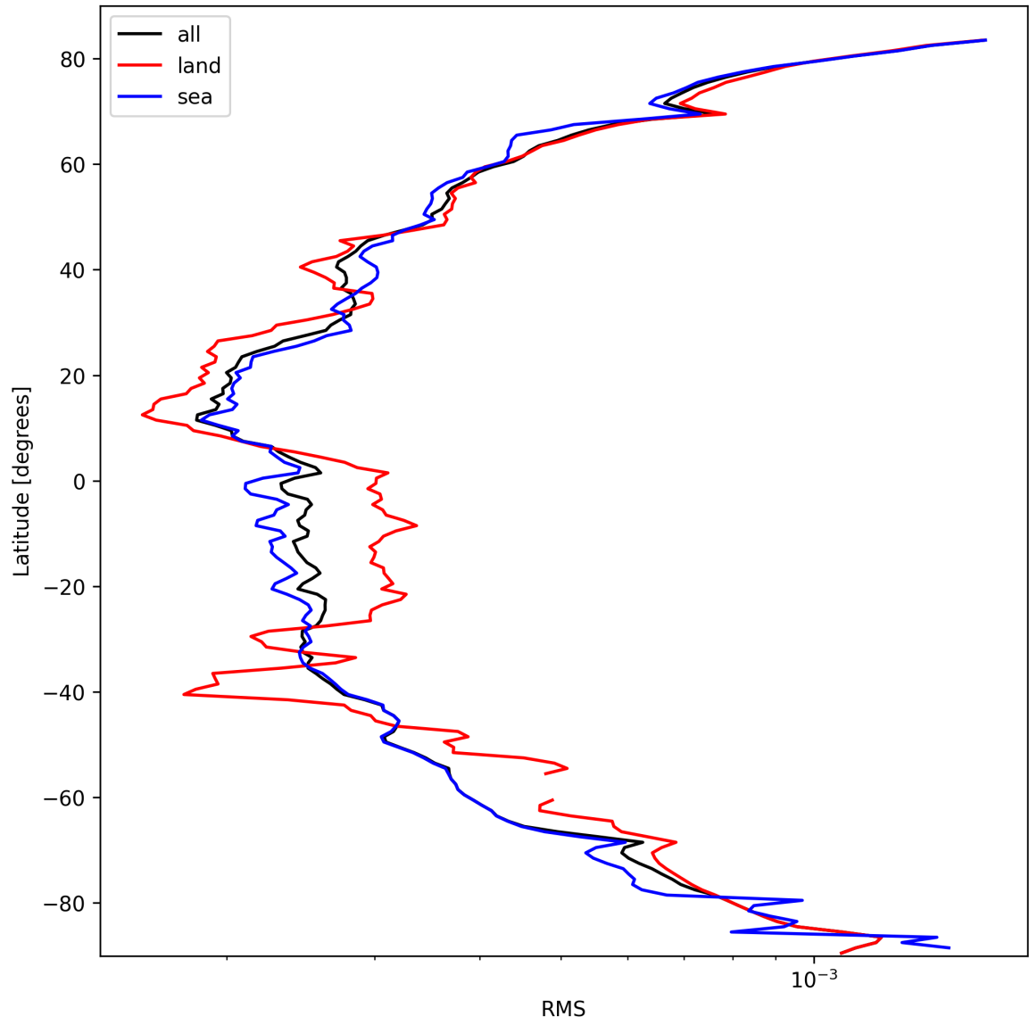
Figure 24: Zonal average of “RMS” for 2025-03-09 to 2025-03-10.
