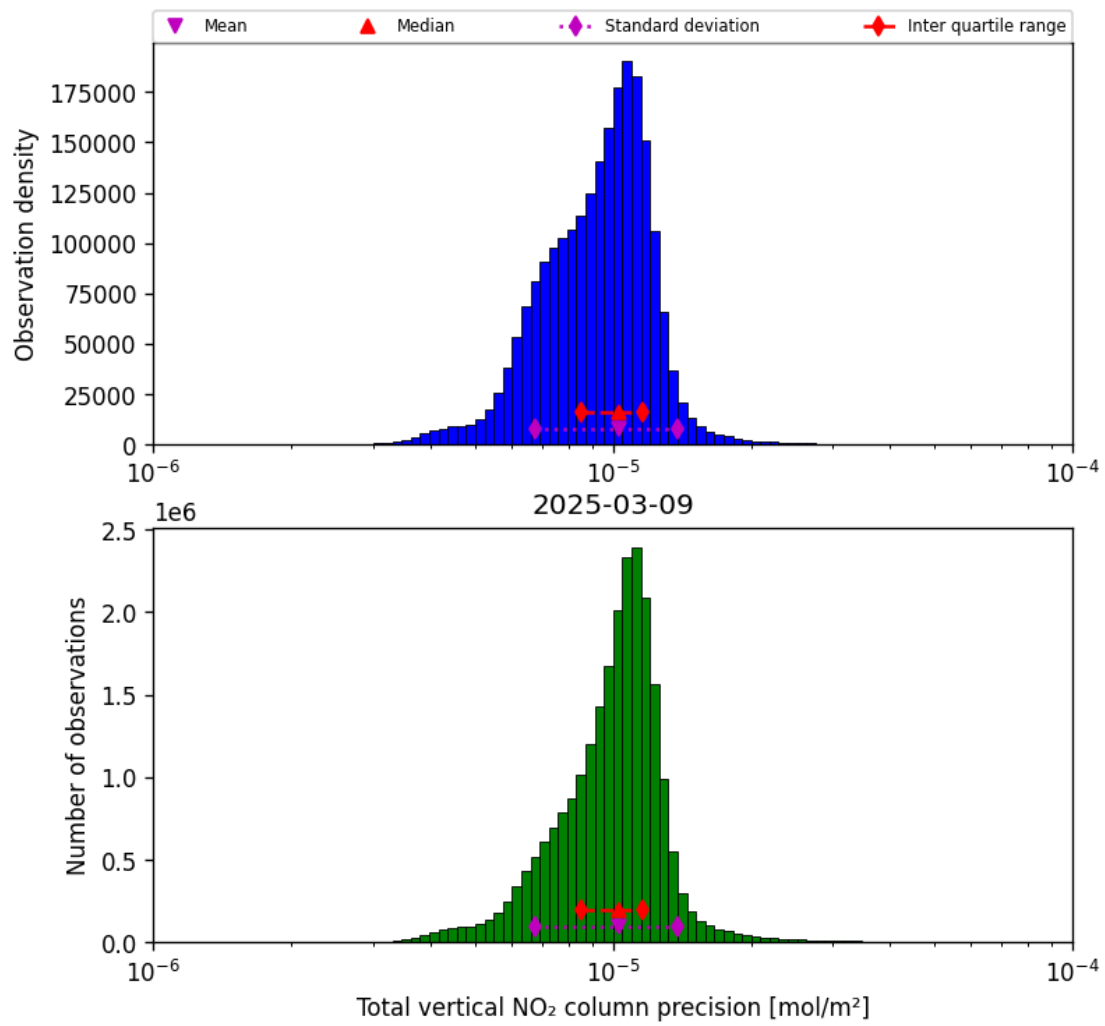
Figure 37: Histogram of “Total vertical NO 2 column precision” for 2025-03-09 to 2025-03-10
