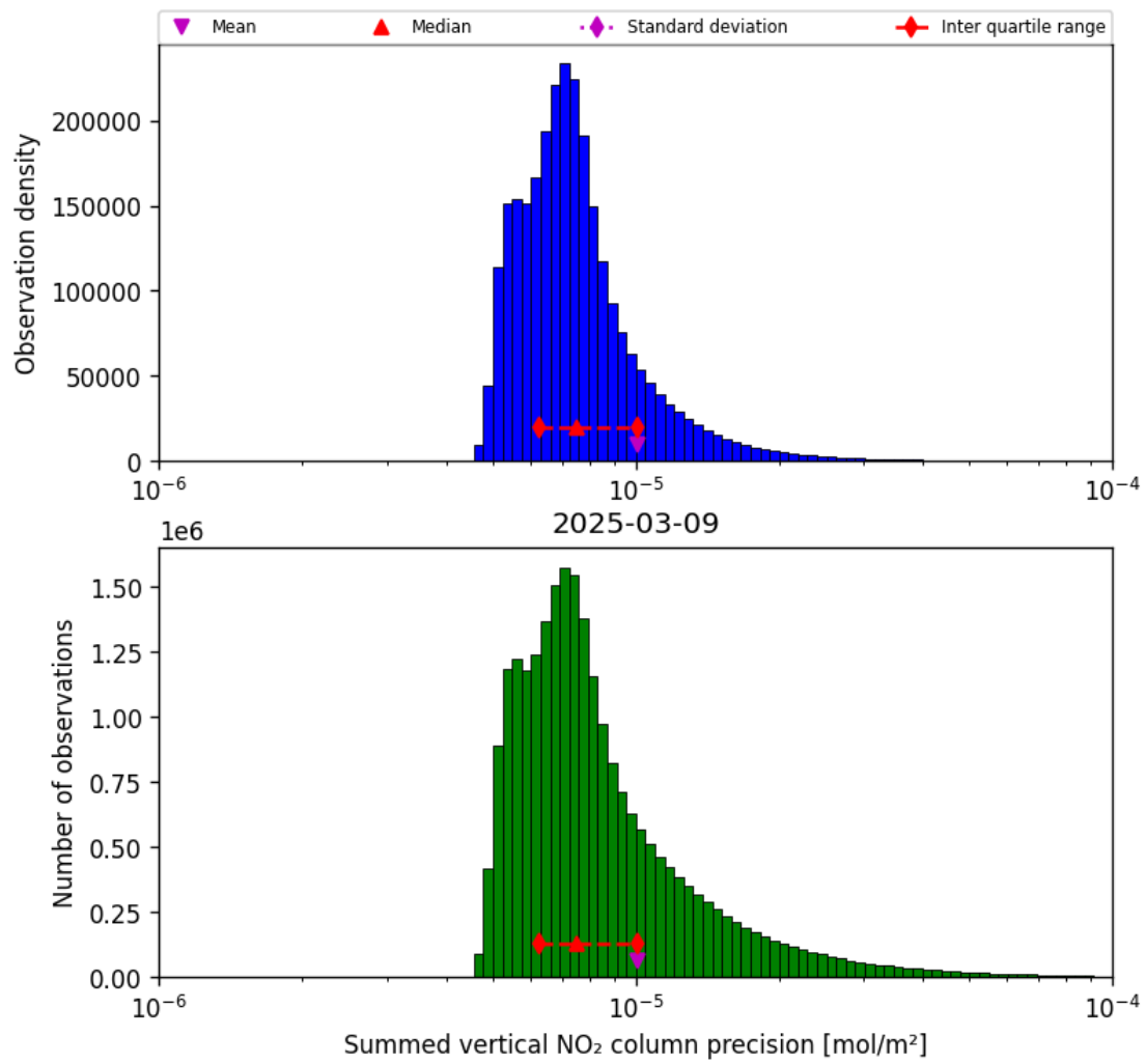
Figure 39: Histogram of “Summed vertical NO 2 column precision” for 2025-03-09 to 2025-03-10
