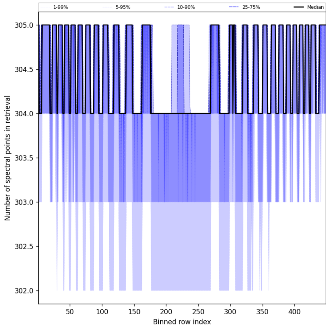
Figure 48: Along track statistics of “Number of spectral points in retrieval” for 2025-03-09 to 2025-03-10
