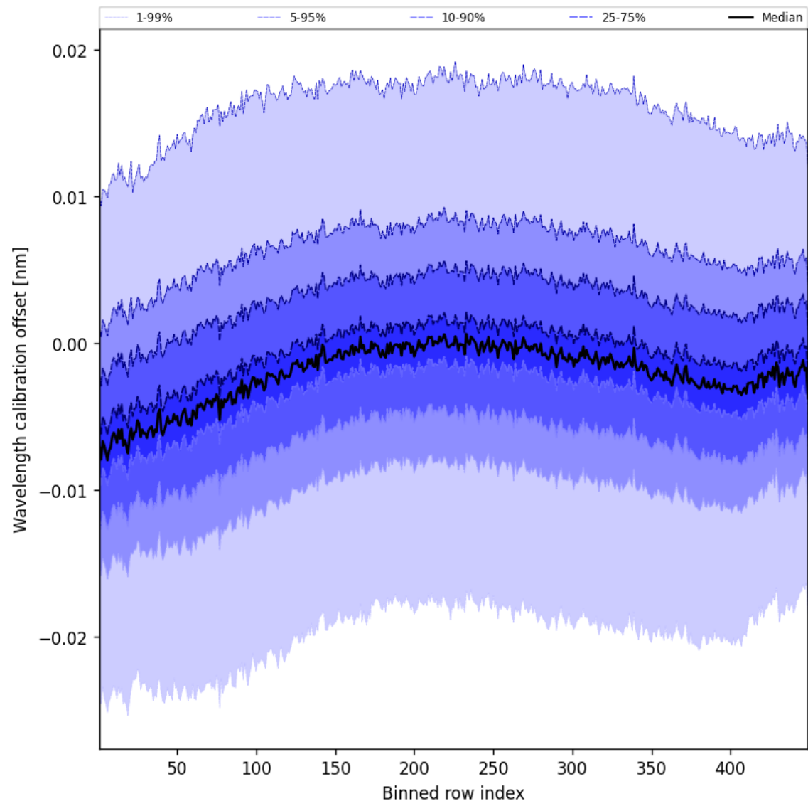
Figure 50: Along track statistics of “Wavelength calibration offset” for 2025-03-09 to 2025-03-10
