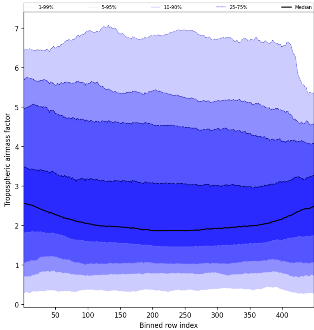
Figure 46: Along track statistics of “Tropospheric air mass factor” for 2025-03-09 to 2025-03-10
