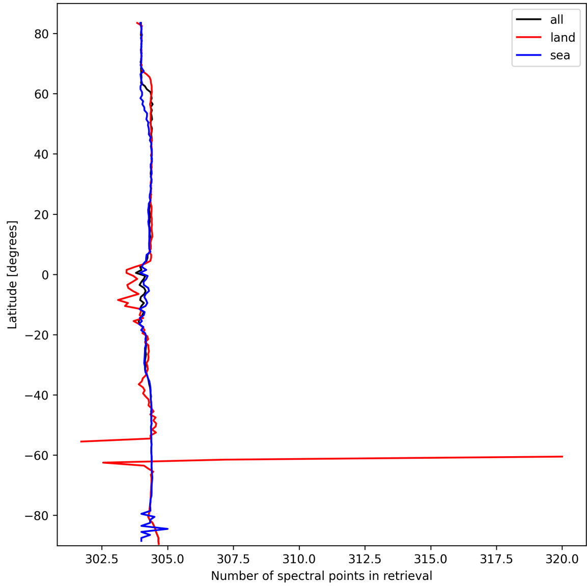
Figure 14: Zonal average of “Number of spectral points in retrieval” for 2025-03-09 to 2025-03-10.
