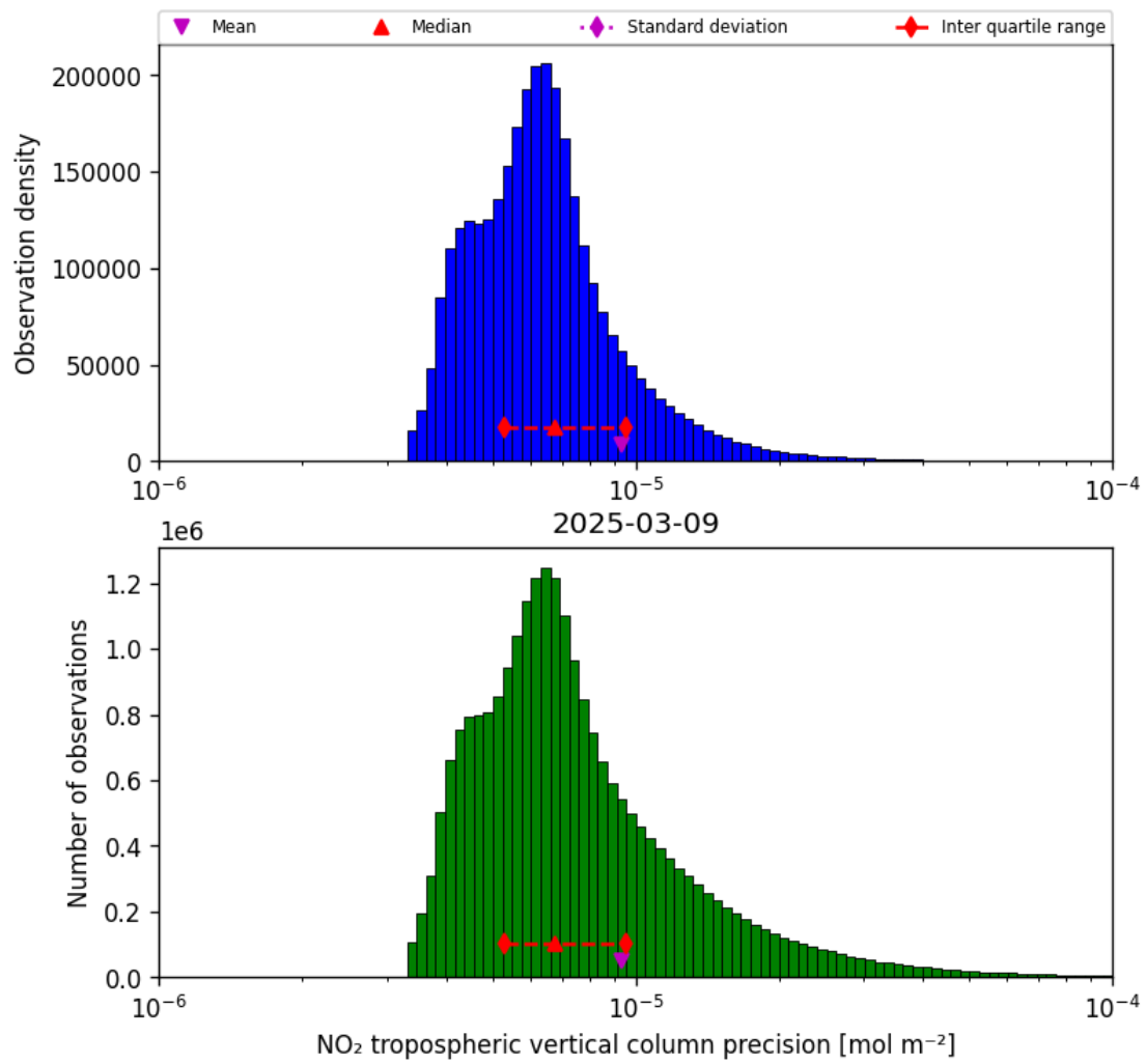
Figure 28: Histogram of “NO 2 tropospheric vertical column precision” for 2025-03-09 to 2025-03-10
