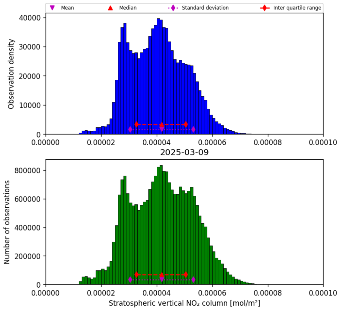
Figure 34: Histogram of “Stratospheric vertical NO 2 column” for 2025-03-09 to 2025-03-10
