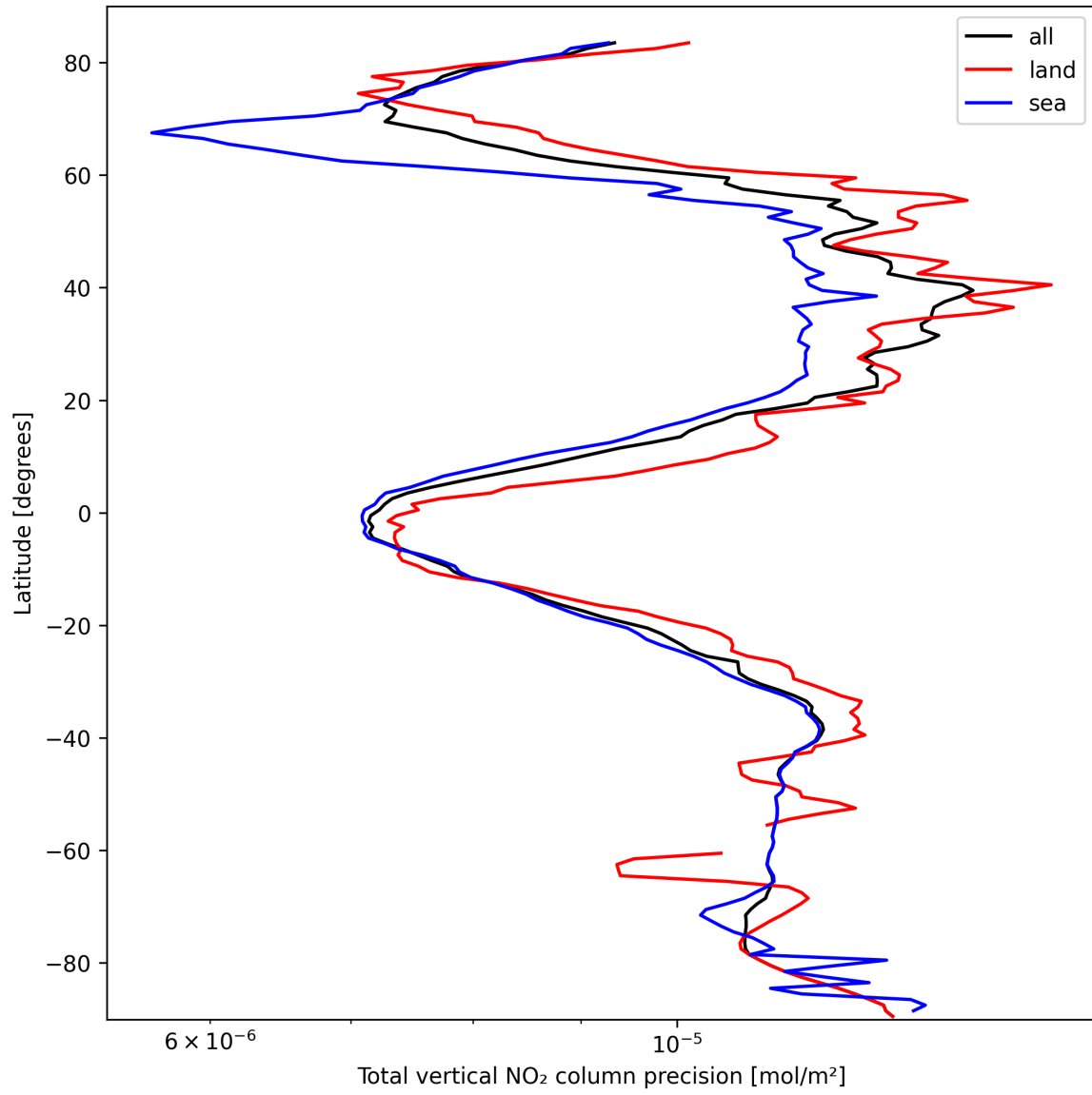
Figure 20: Zonal average of “Total vertical NO 2 column precision” for 2025-03-09 to 2025-03-10.
