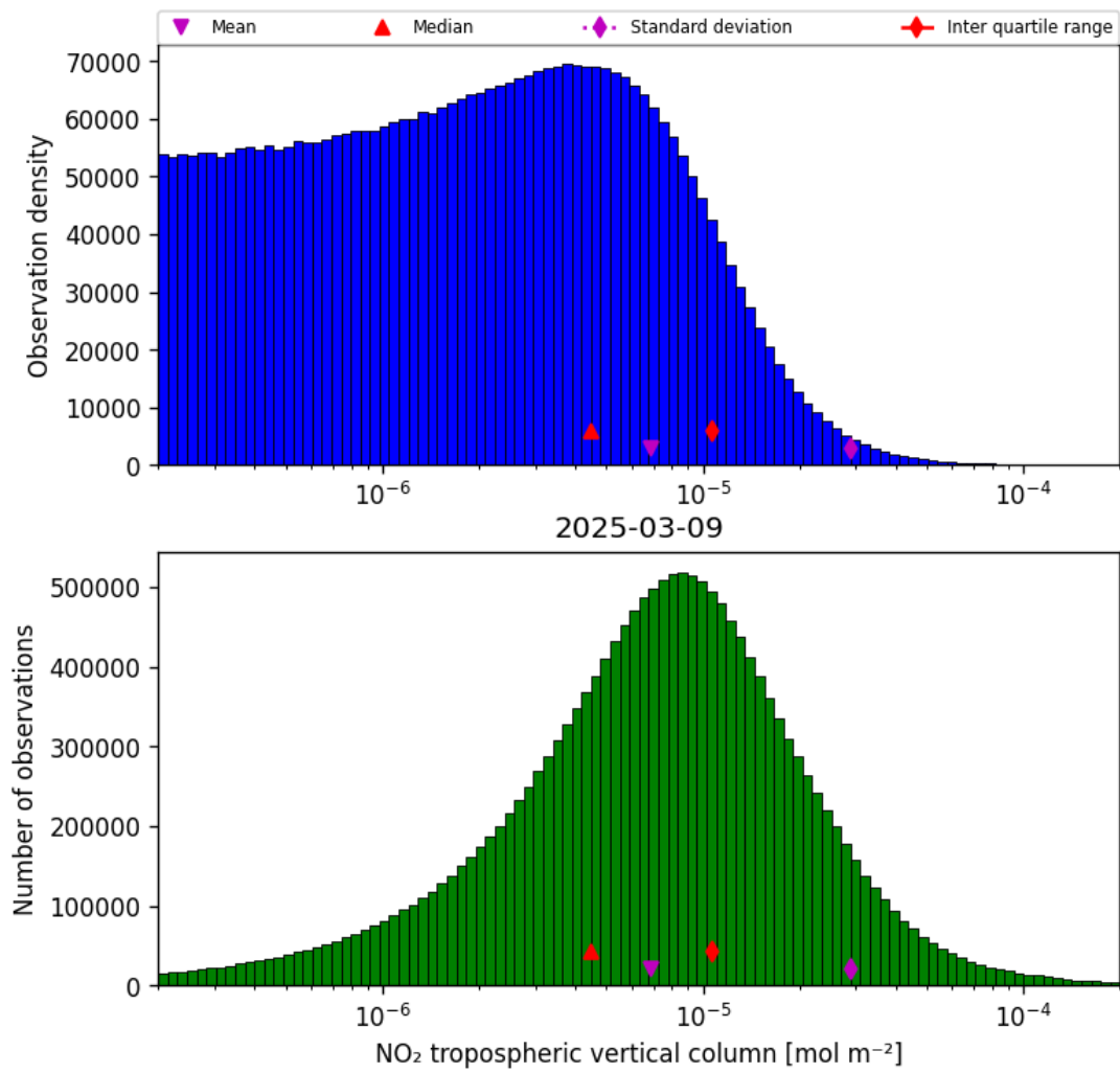
Figure 27: Histogram of “NO 2 tropospheric vertical column” for 2025-03-09 to 2025-03-10
