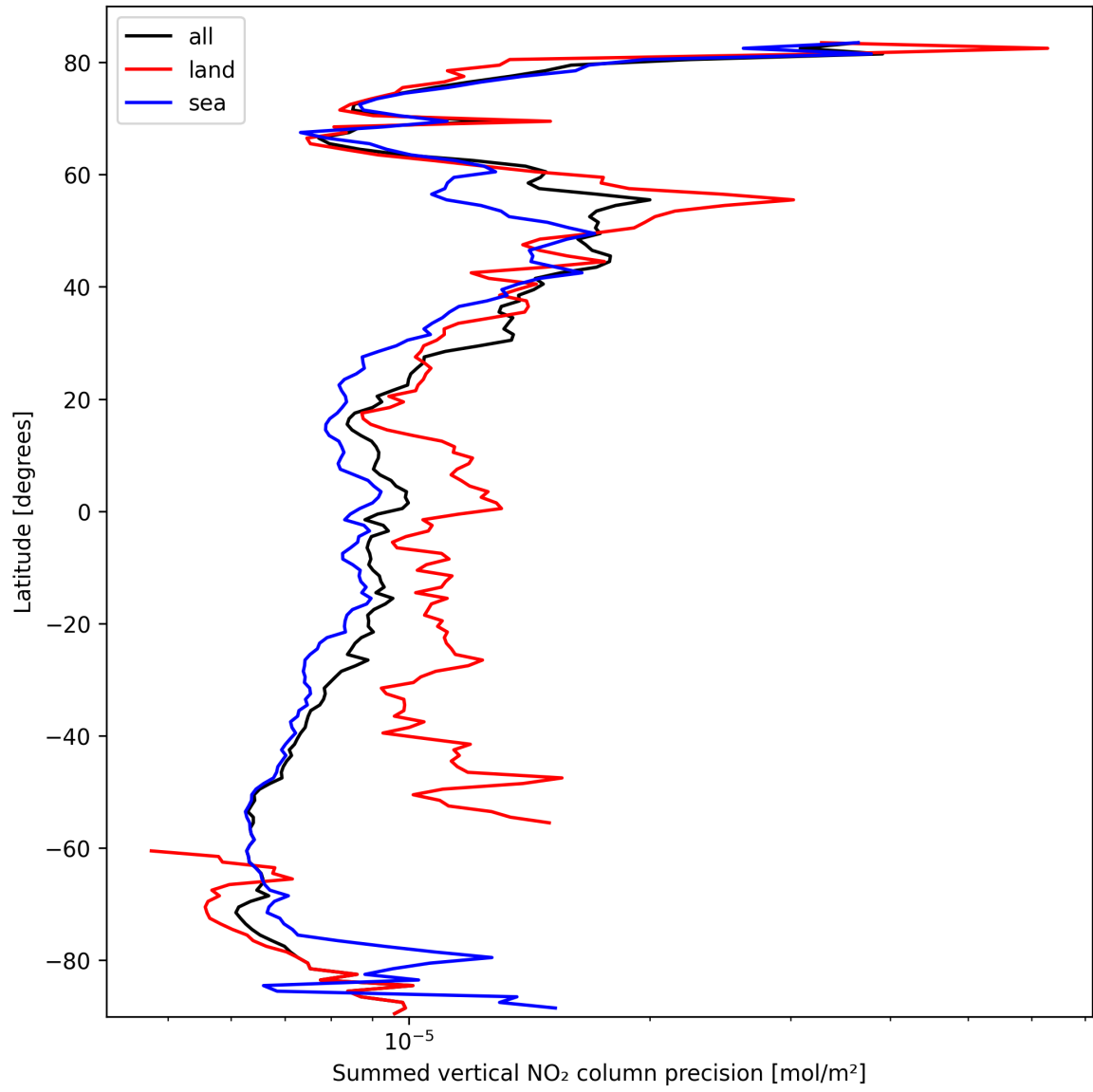
Figure 22: Zonal average of “Summed vertical NO 2 column precision” for 2025-03-09 to 2025-03-10.
