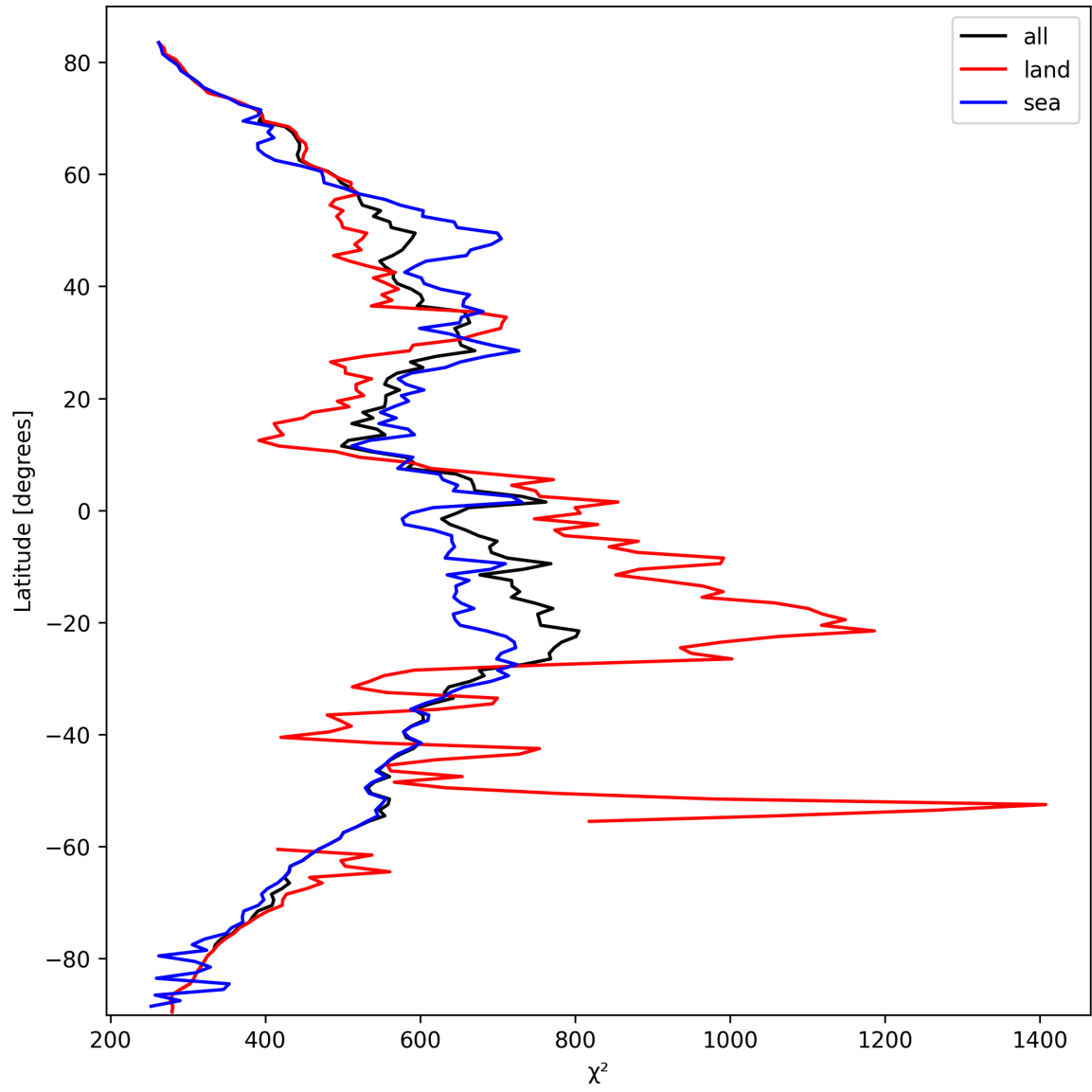
Figure 23: Zonal average of “ \chi^2 ” for 2025-03-09 to 2025-03-10.
