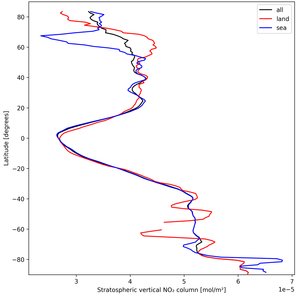
Figure 17: Zonal average of “Stratospheric vertical NO 2 column” for 2025-03-09 to 2025-03-10.
