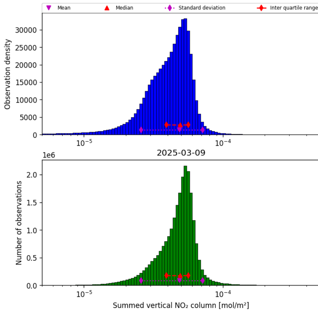
Figure 38: Histogram of “Summed vertical NO 2 column” for 2025-03-09 to 2025-03-10
