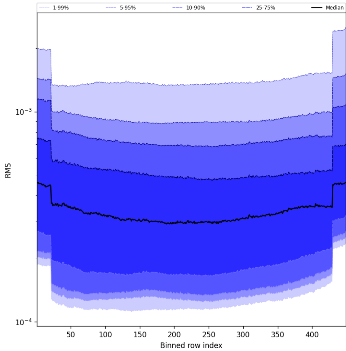
Figure 58: Along track statistics of “RMS” for 2025-03-10 to 2025-03-10
