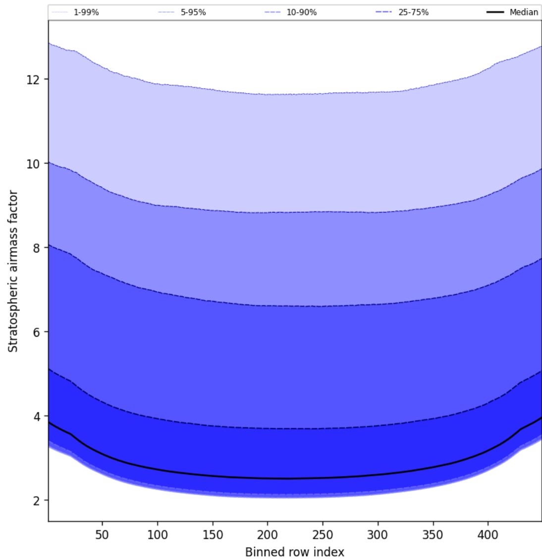
Figure 59: Along track statistics of “Stratospheric airmass factor” for 2025-03-10 to 2025-03-10
