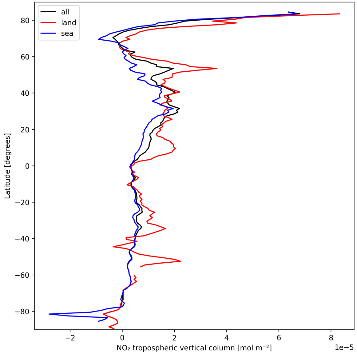
Figure 10: Zonal average of “NO 2 tropospheric vertical column” for 2025-03-10 to 2025-03-10.
