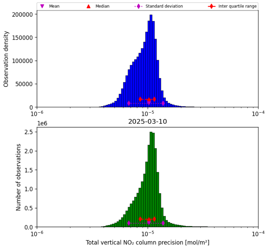
Figure 37: Histogram of "Total vertical NO 2 column precision" for 2025-03-10 to 2025-03-10
