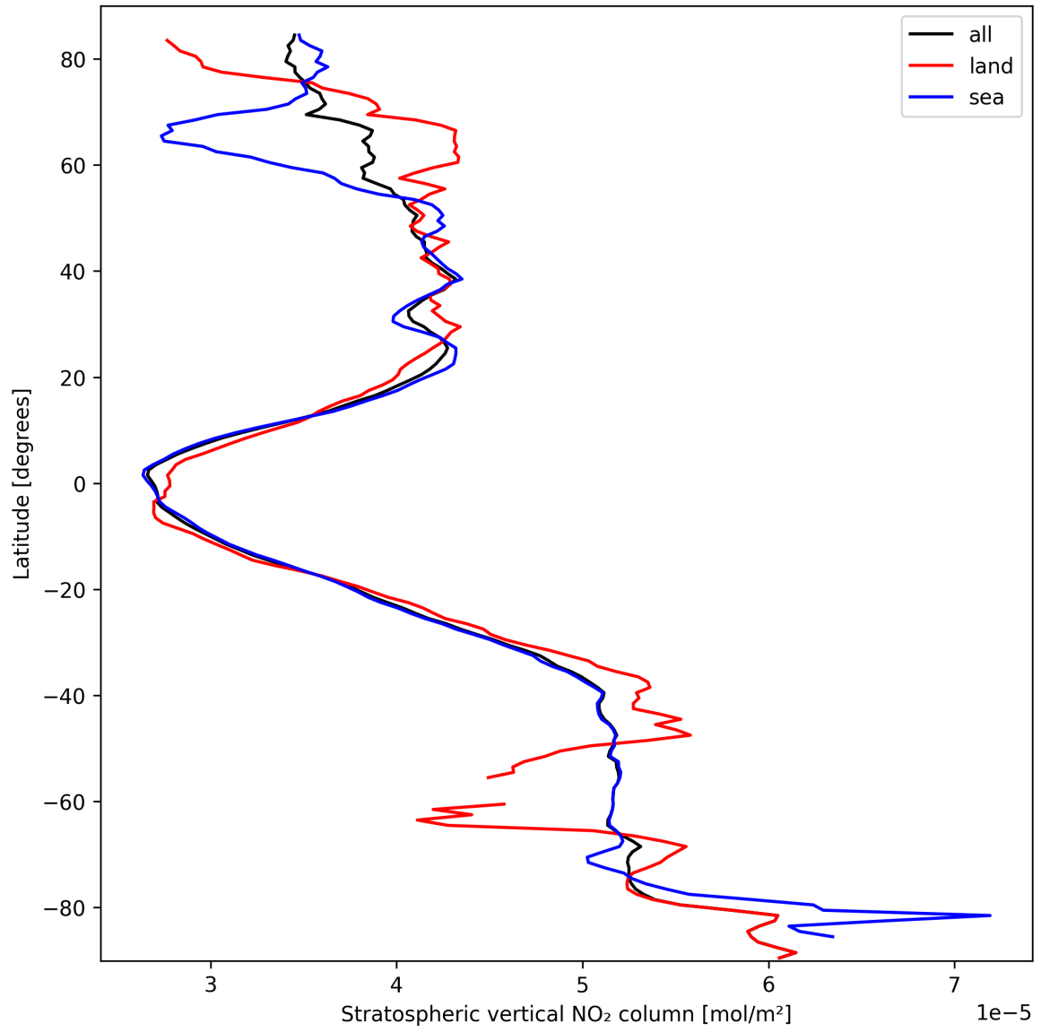
Figure 17: Zonal average of “Stratospheric vertical NO 2 column” for 2025-03-10 to 2025-03-10.
