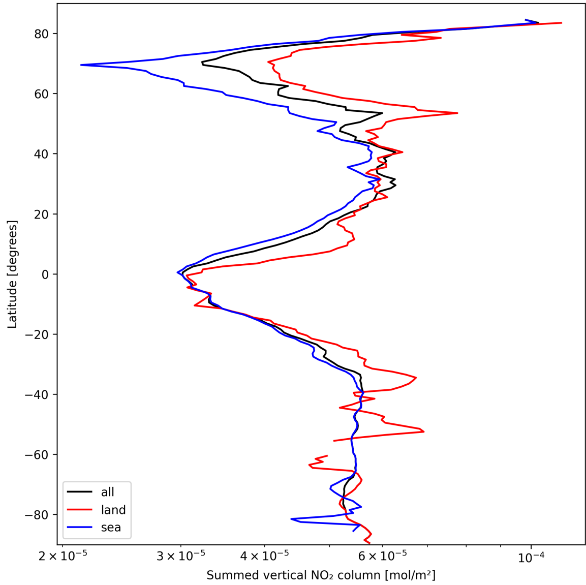
Figure 21: Zonal average of “Summed vertical NO 2 column” for 2025-03-10 to 2025-03-10.
