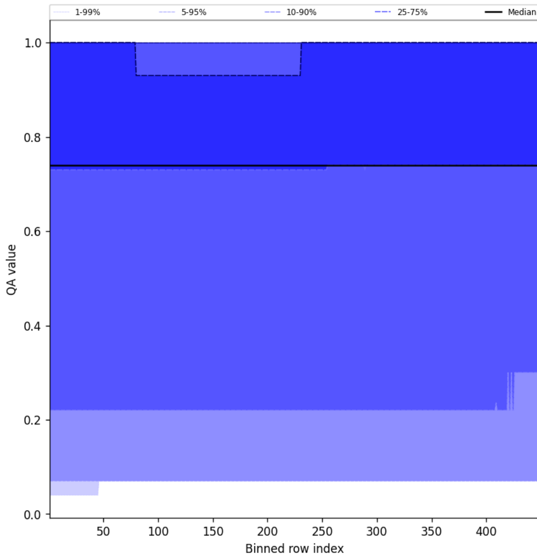
Figure 43: Along track statistics of “QA value” for 2025-03-10 to 2025-03-10
