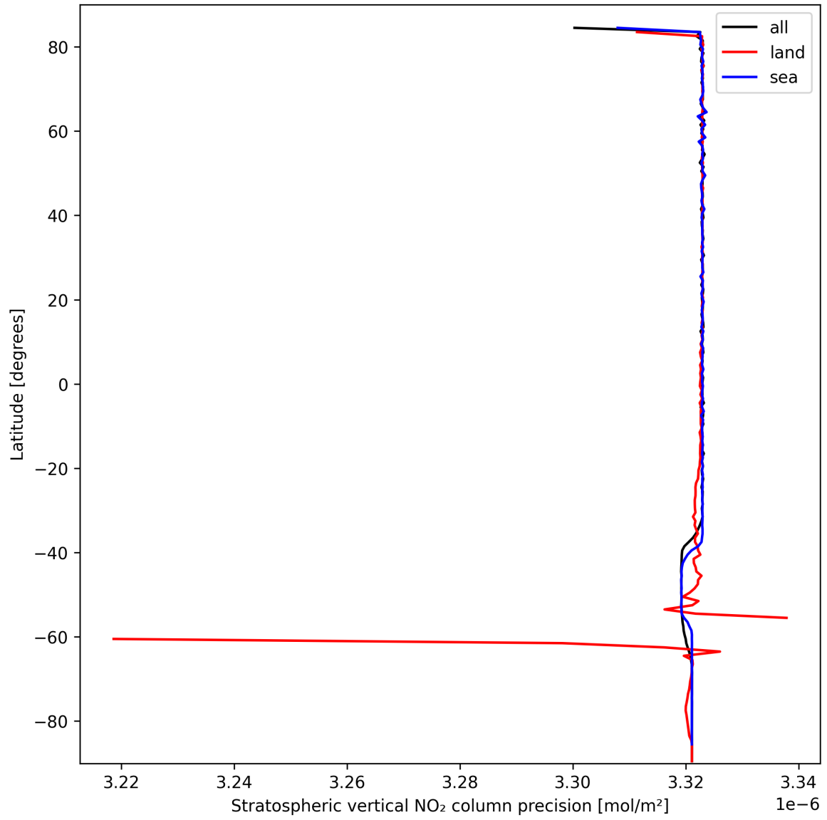
Figure 18: Zonal average of “Stratospheric vertical NO 2 column precision” for 2025-03-10 to 2025-03-10.
