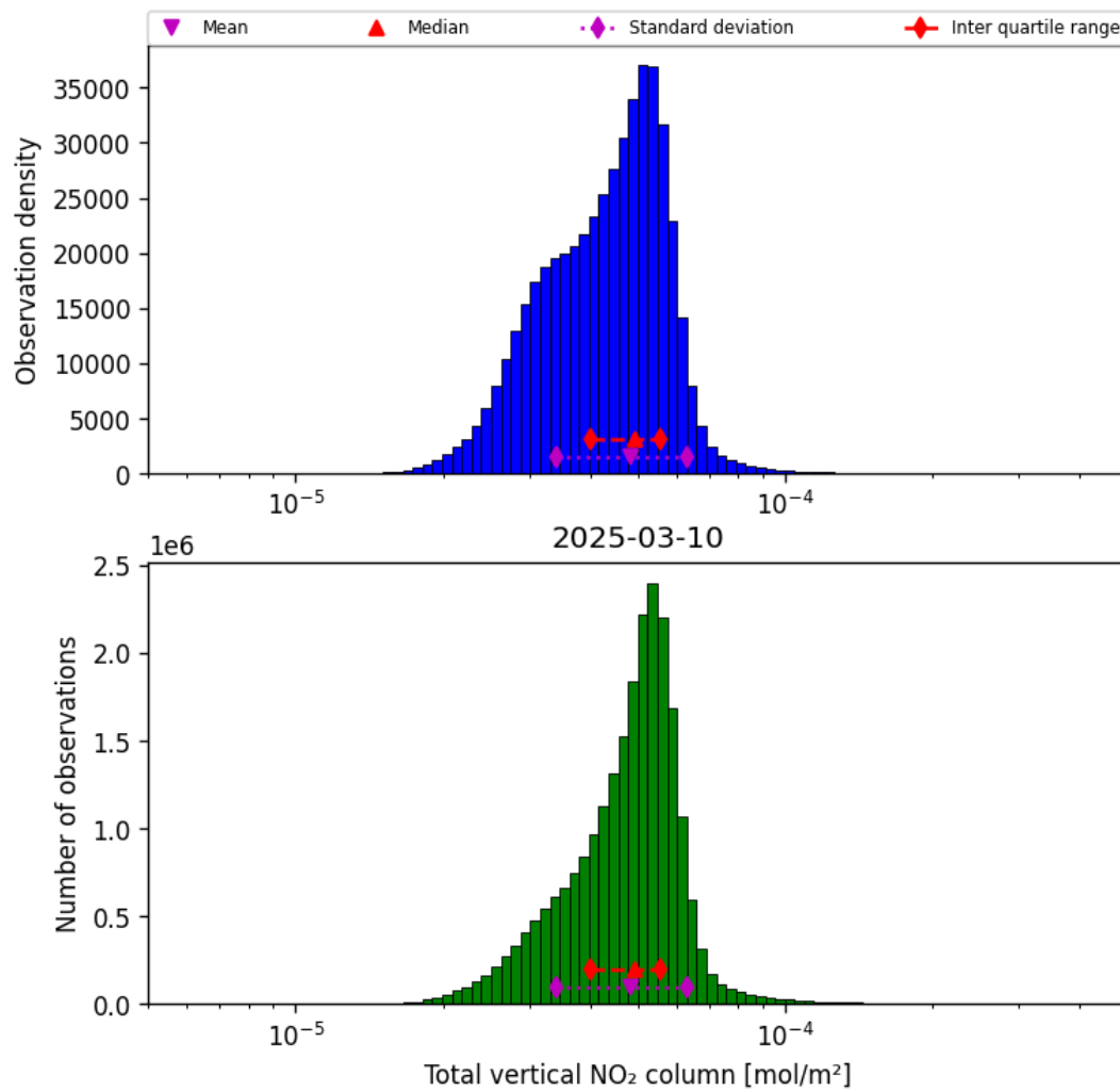
Figure 36: Histogram of “Total vertical NO 2 column” for 2025-03-10 to 2025-03-10
