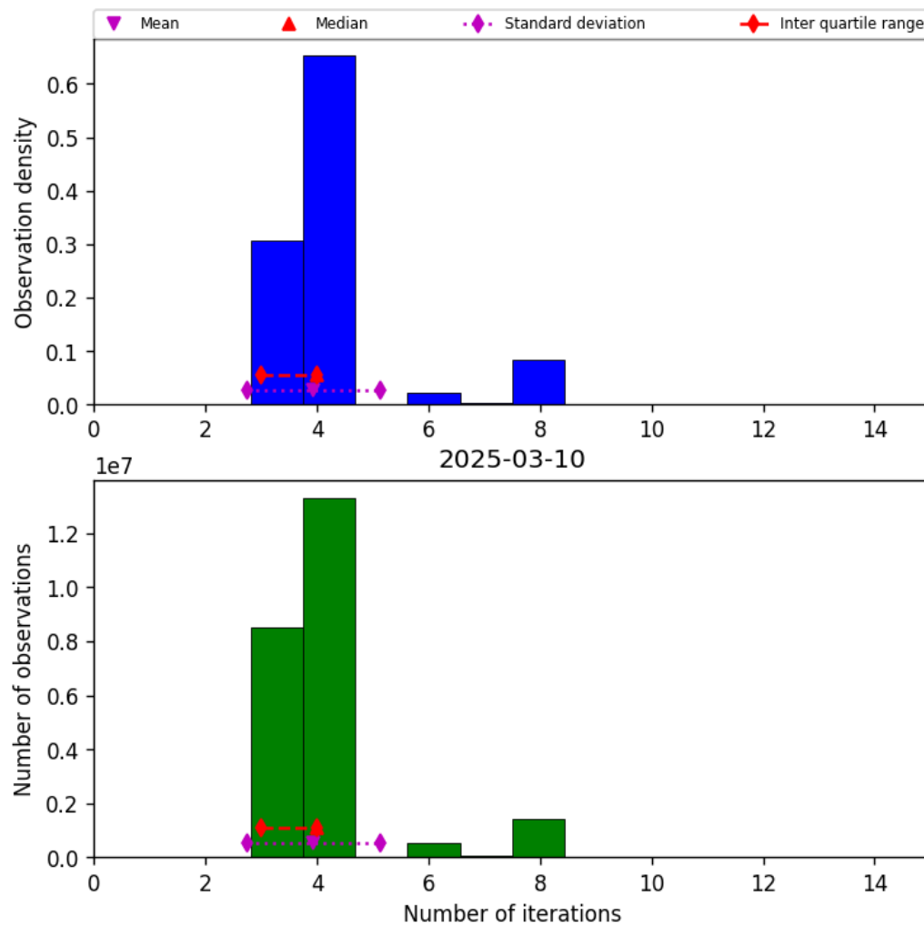
Figure 32: Histogram of “Number of iterations” for 2025-03-10 to 2025-03-10
