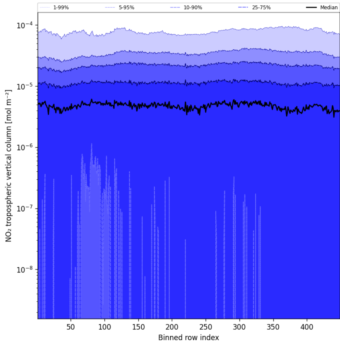
Figure 44: Along track statistics of “NO 2 tropospheric vertical column” for 2025-03-10 to 2025-03-10
