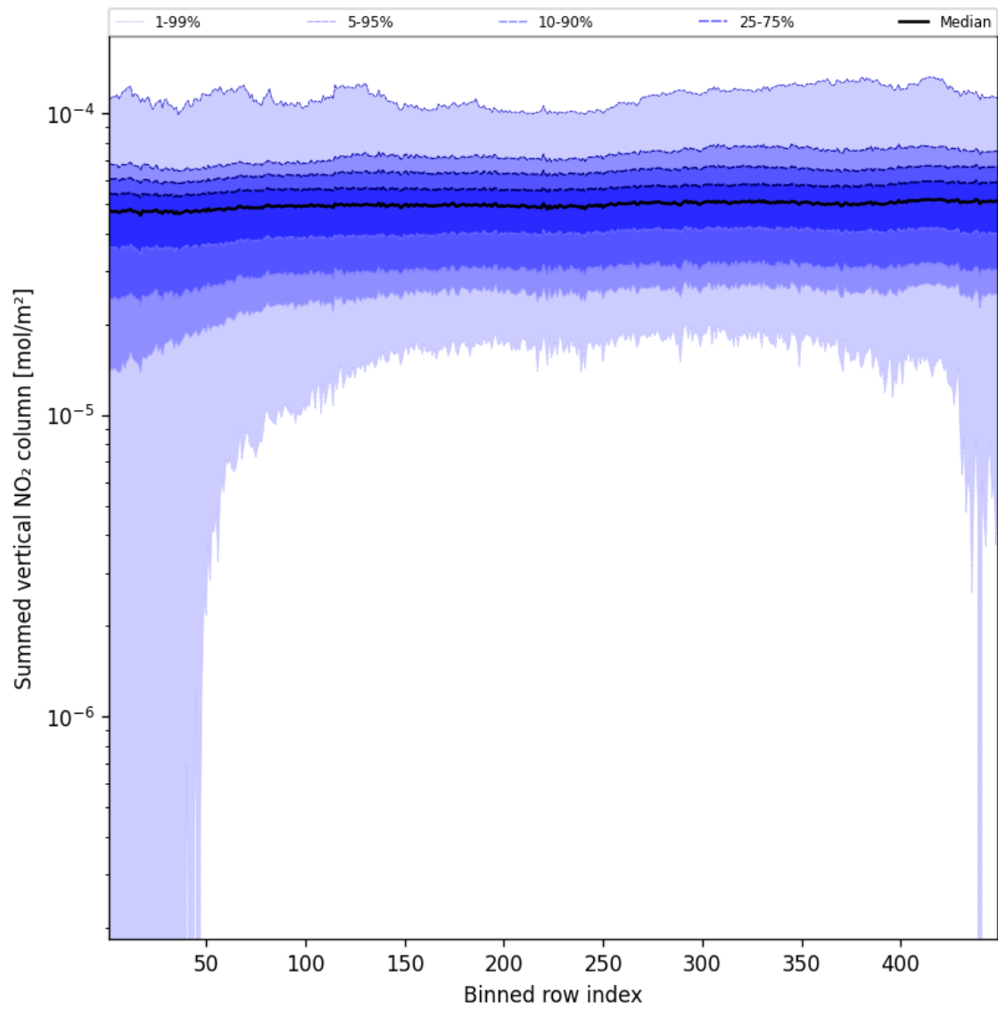
Figure 55: Along track statistics of “Summed vertical NO 2 column” for 2025-03-10 to 2025-03-10
