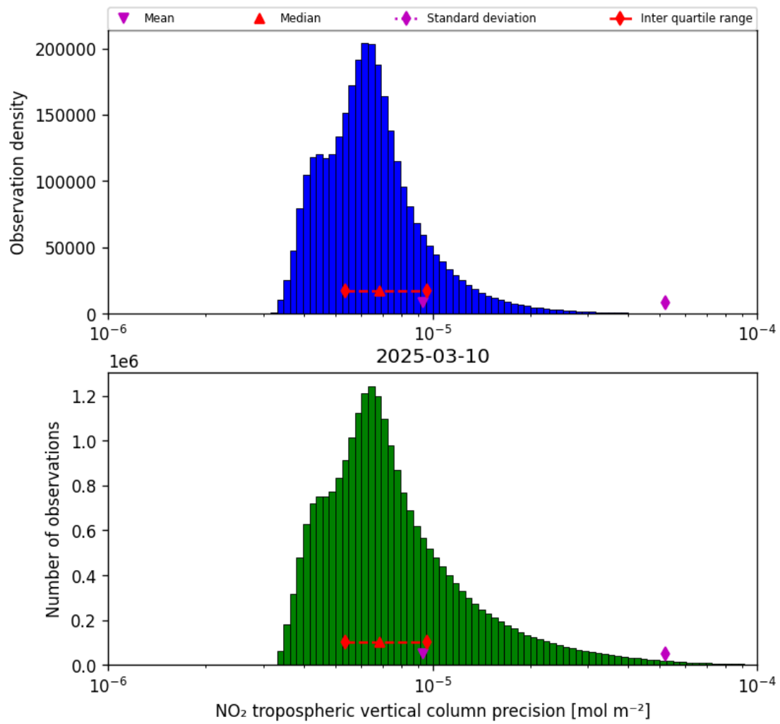
Figure 28: Histogram of “NO 2 tropospheric vertical column precision” for 2025-03-10 to 2025-03-10
