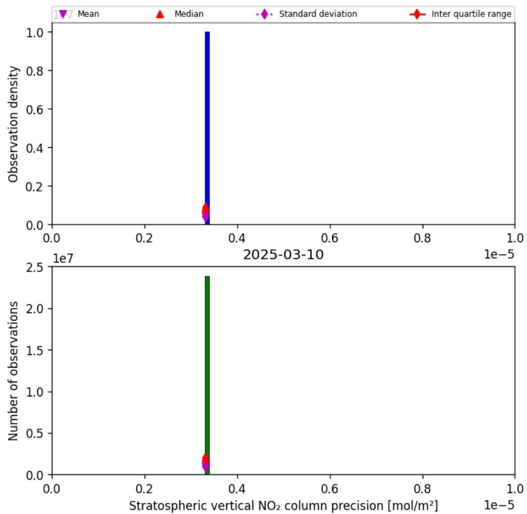
Figure 35: Histogram of “Stratospheric vertical NO 2 column precision” for 2025-03-10 to 2025-03-10
