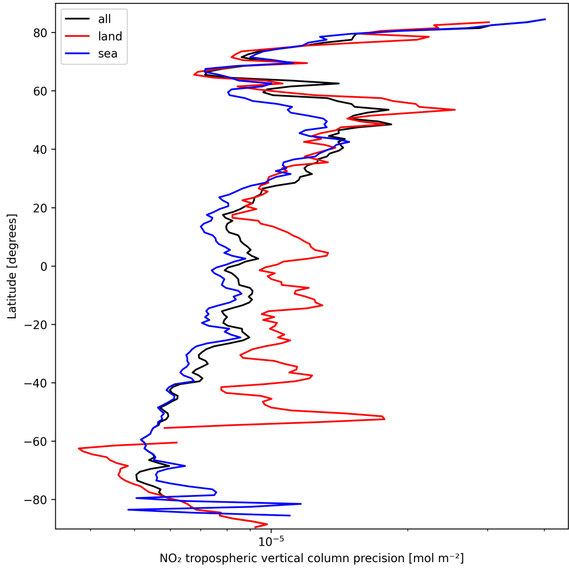
Figure 11: Zonal average of “NO 2 tropospheric vertical column precision” for 2025-03-10 to 2025-03-10.
