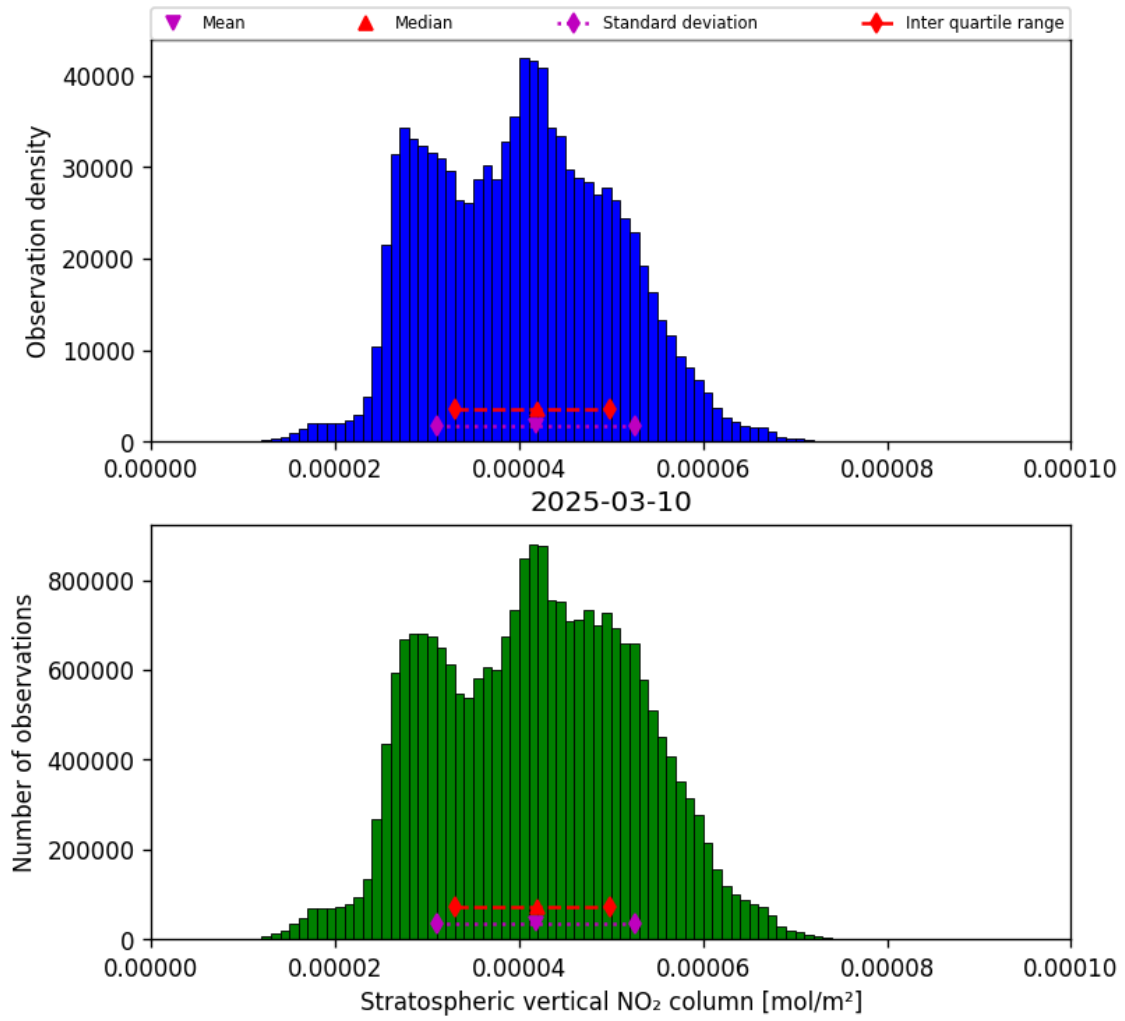
Figure 34: Histogram of “Stratospheric vertical NO 2 column” for 2025-03-10 to 2025-03-10
