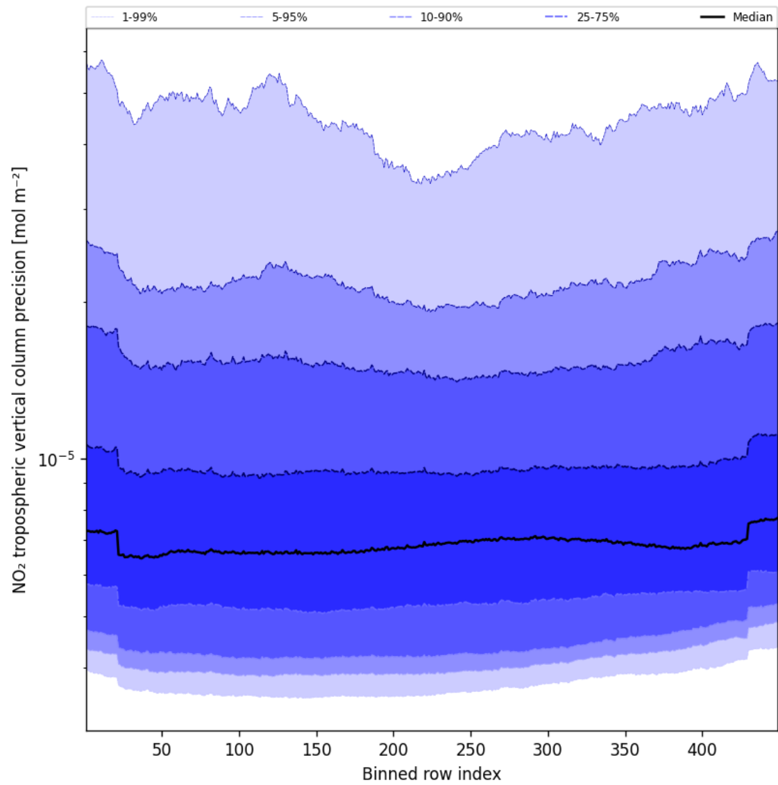
Figure 45: Along track statistics of “NO 2 tropospheric vertical column precision” for 2025-03-10 to 2025-03-10
