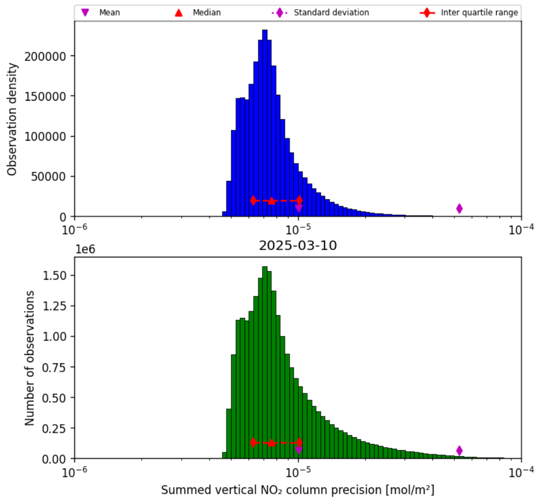
Figure 39: Histogram of "Summed vertical NO 2 column precision" for 2025-03-10 to 2025-03-10
