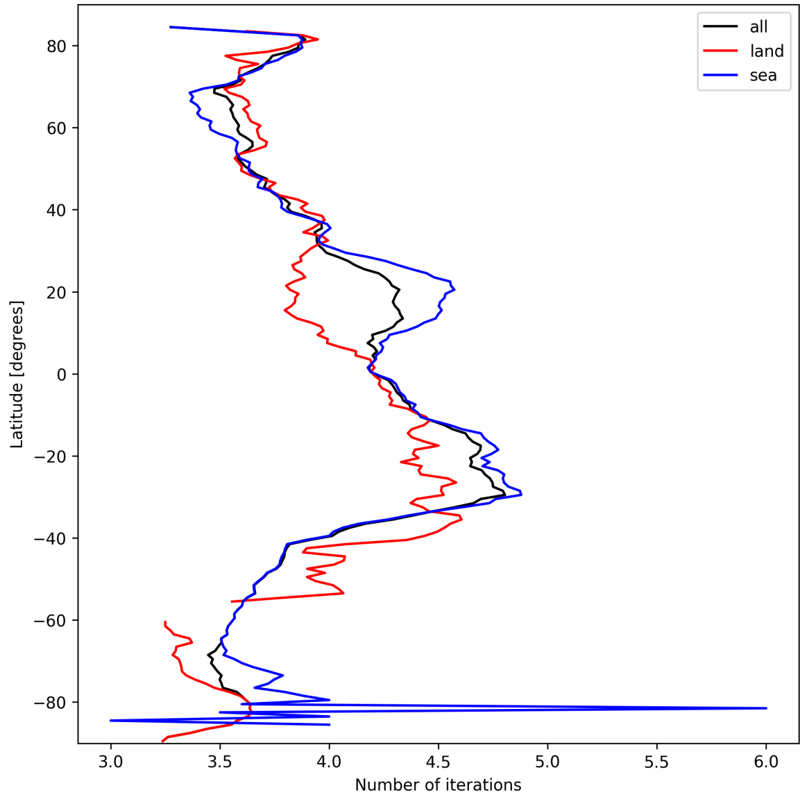
Figure 15: Zonal average of “Number of iterations” for 2025-03-10 to 2025-03-10.
