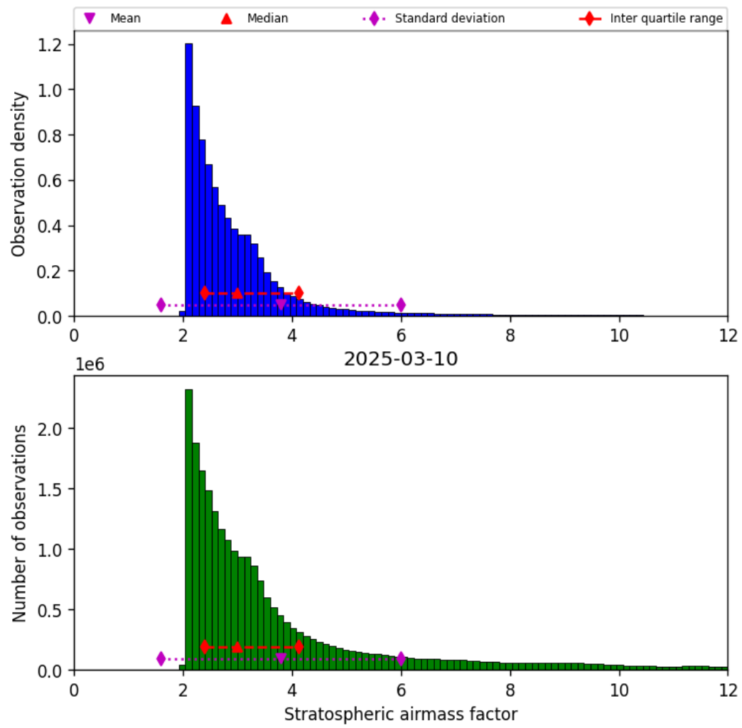
Figure 42: Histogram of “Stratospheric airmass factor” for 2025-03-10 to 2025-03-10
