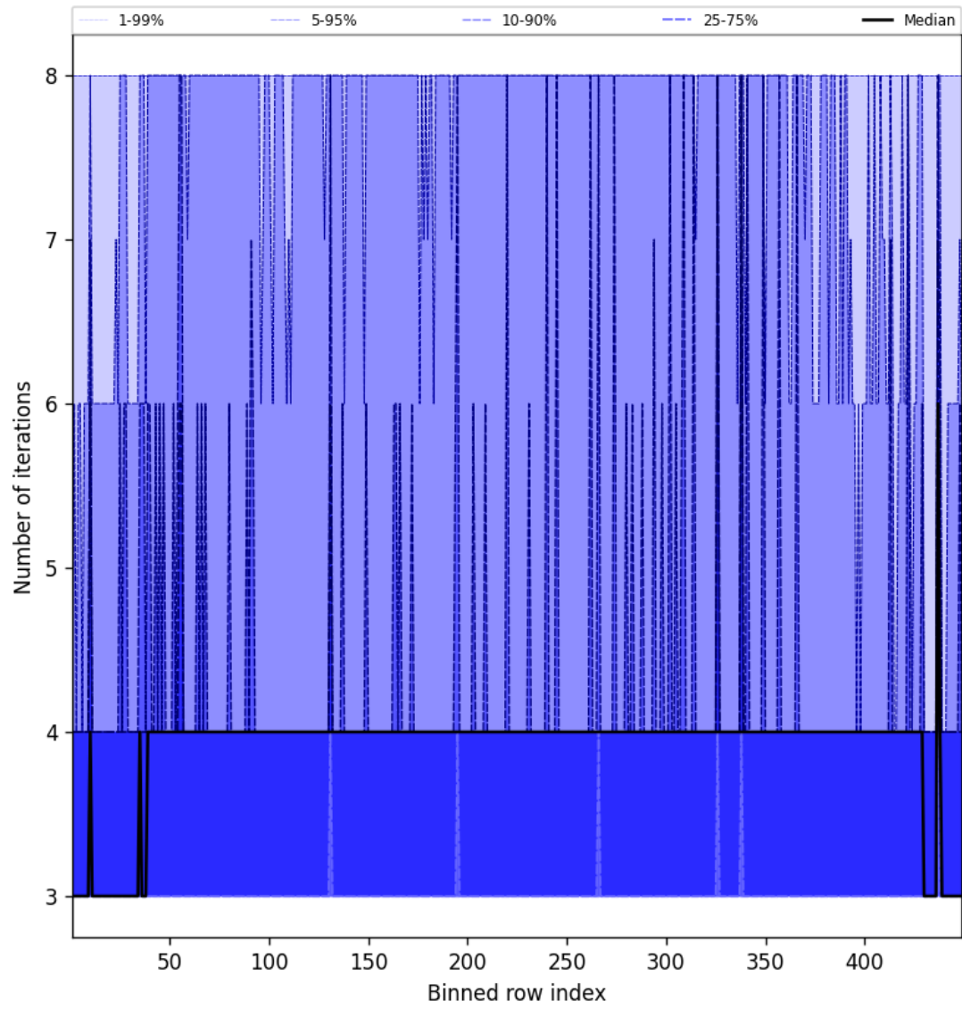
Figure 49: Along track statistics of “Number of iterations” for 2025-03-10 to 2025-03-10
