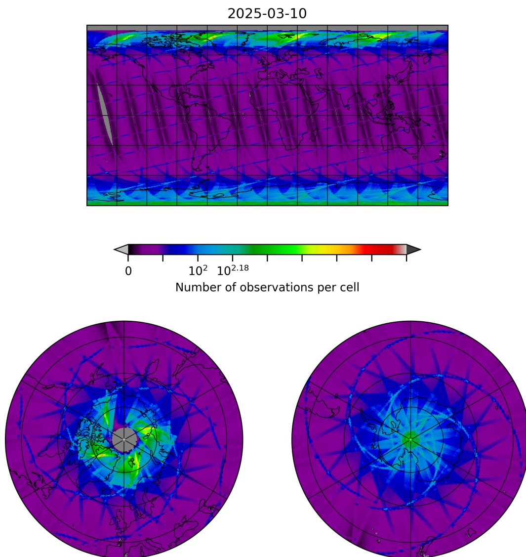
Figure 8: Map of the number of observations for 2025-03-10 to 2025-03-10
