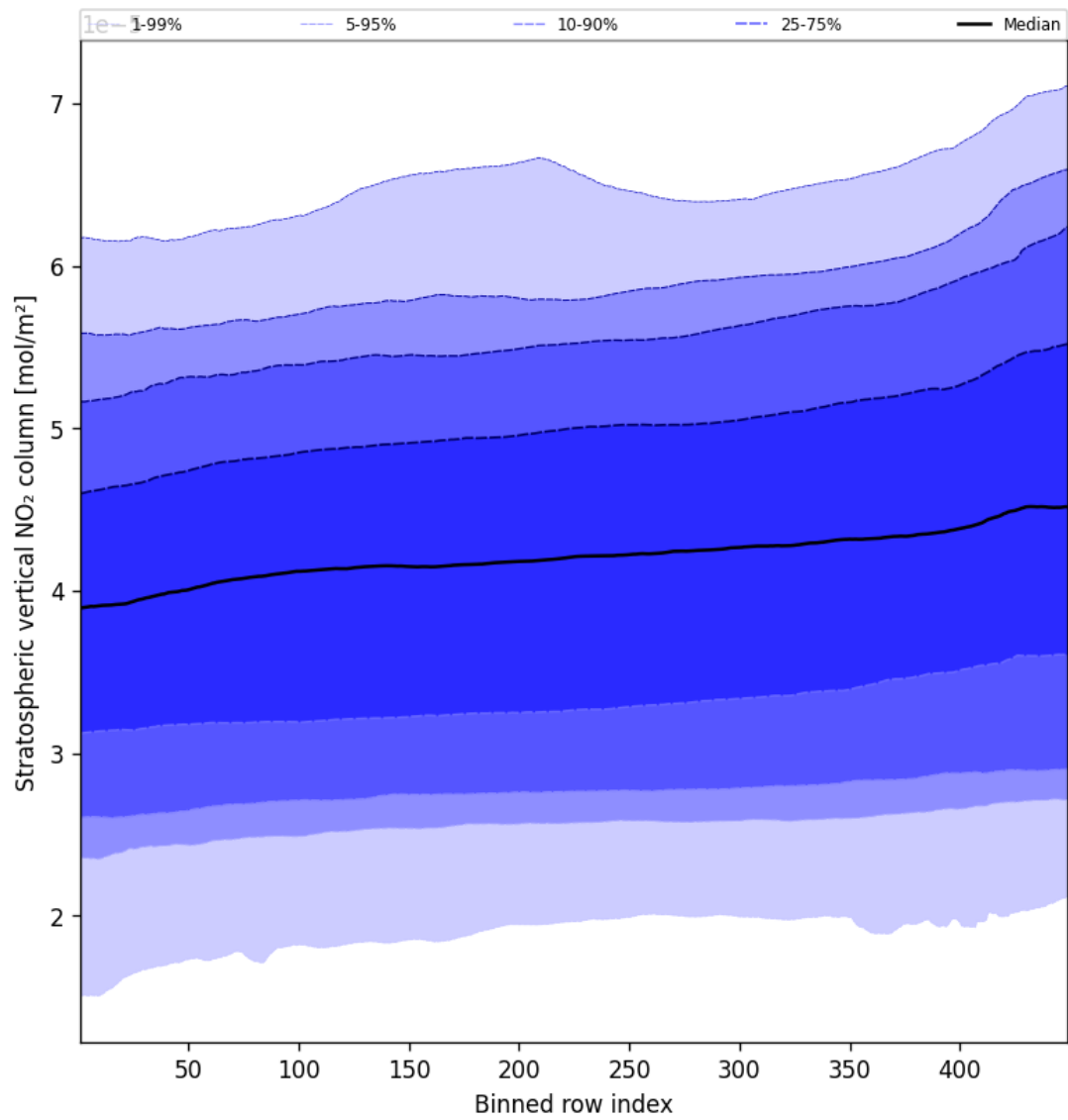
Figure 51: Along track statistics of “Stratospheric vertical NO 2 column” for 2025-03-10 to 2025-03-10
