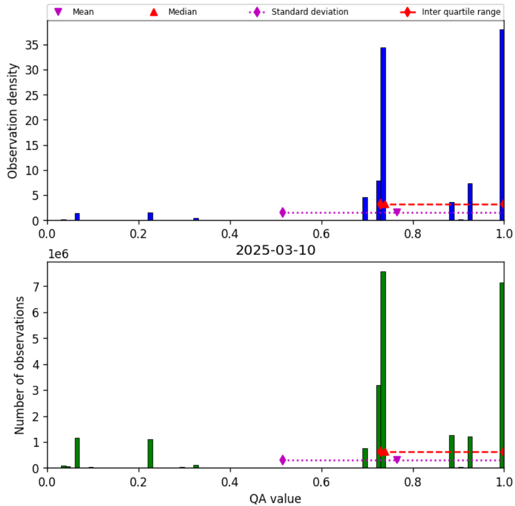
Figure 26: Histogram of “QA value” for 2025-03-10 to 2025-03-10
