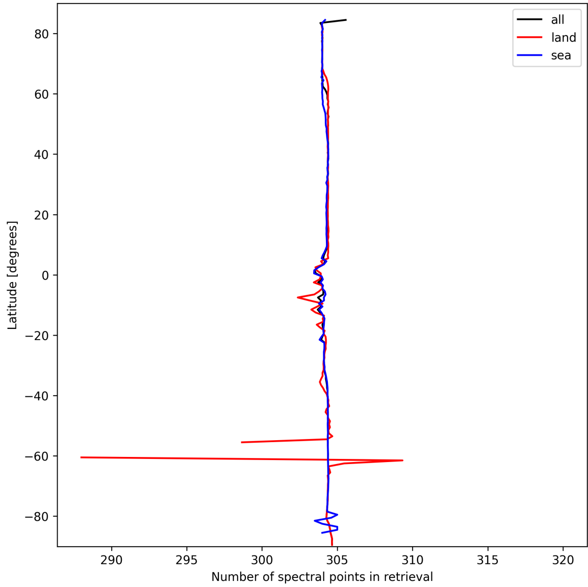
Figure 14: Zonal average of “Number of spectral points in retrieval” for 2025-03-10 to 2025-03-10.
