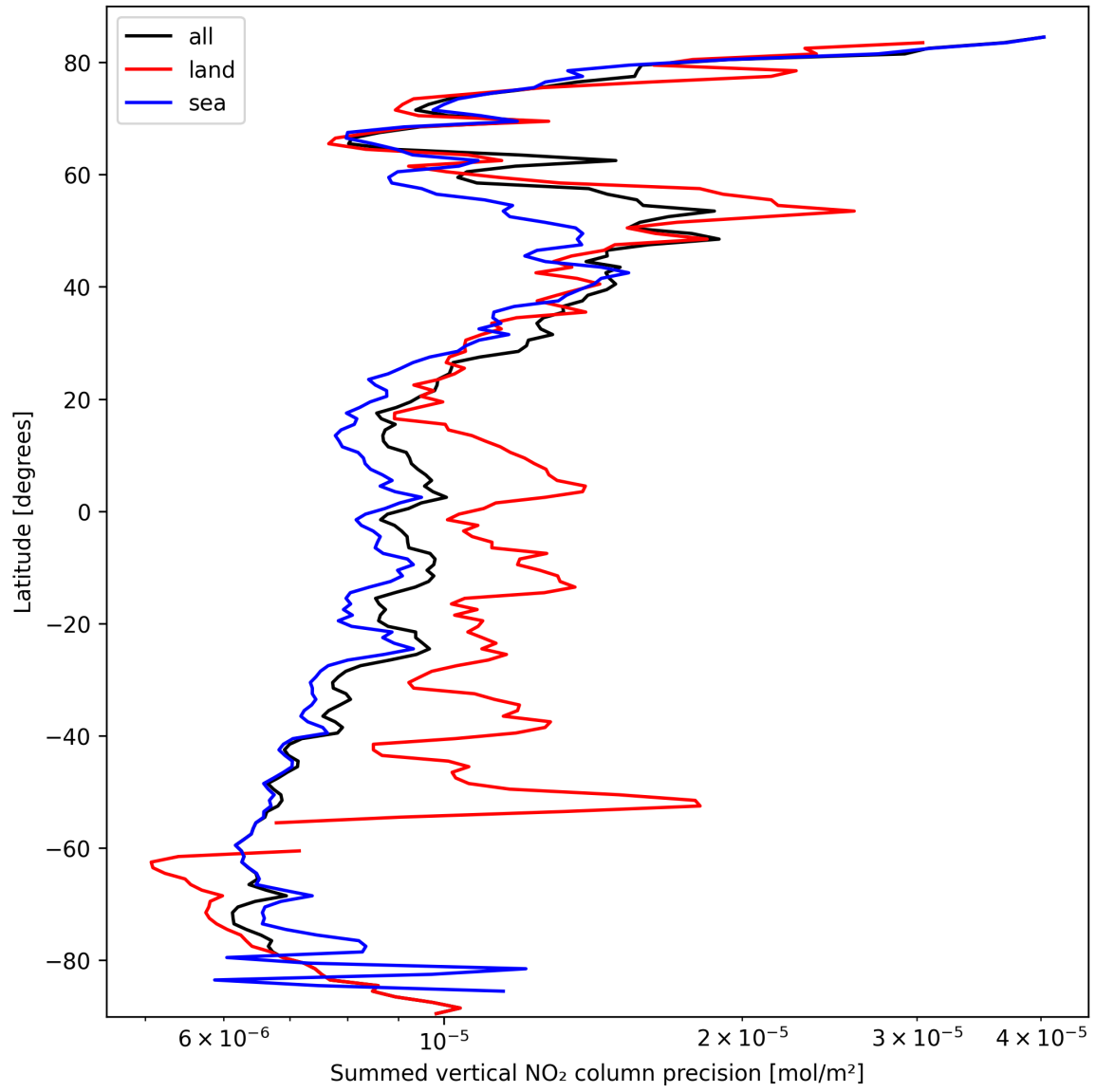
Figure 22: Zonal average of “Summed vertical NO 2 column precision” for 2025-03-10 to 2025-03-10.
