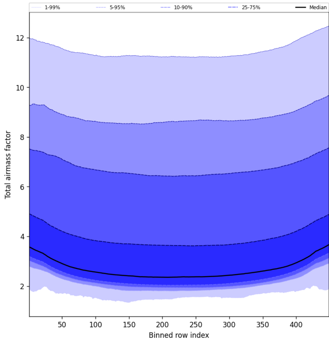
Figure 47: Along track statistics of “Total airmass factor” for 2025-03-10 to 2025-03-10
