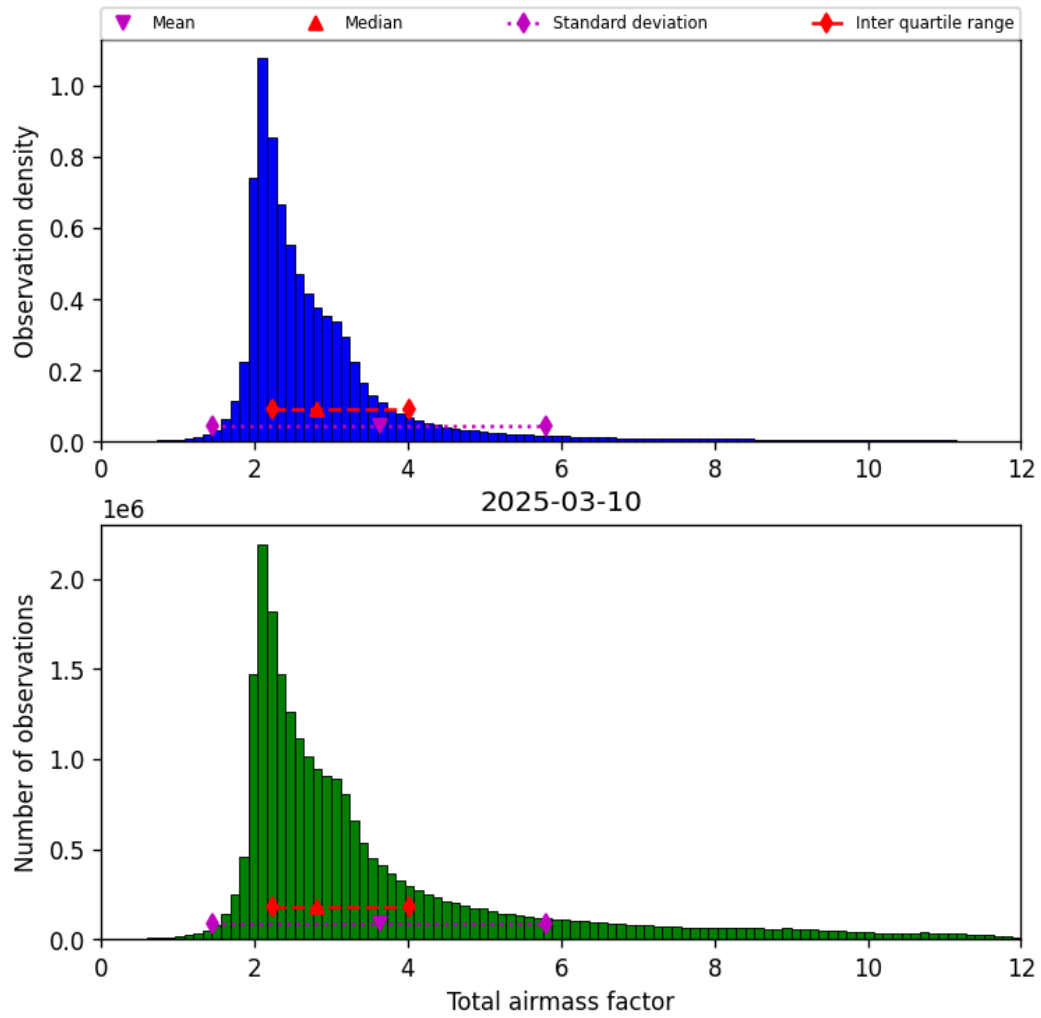
Figure 30: Histogram of “Total airmass factor” for 2025-03-10 to 2025-03-10
