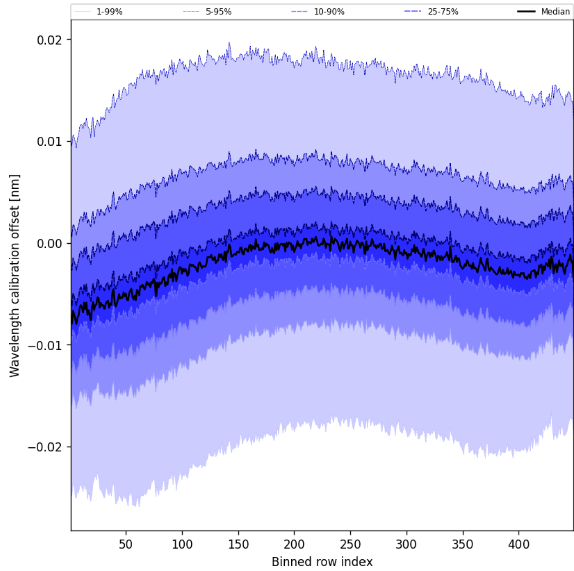
Figure 50: Along track statistics of “Wavelength calibration offset” for 2025-03-10 to 2025-03-10
