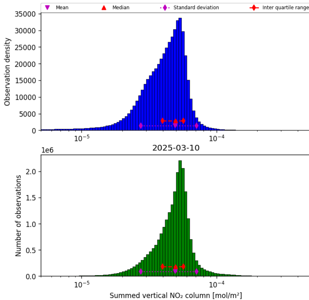
Figure 38: Histogram of “Summed vertical NO 2 column” for 2025-03-10 to 2025-03-10
