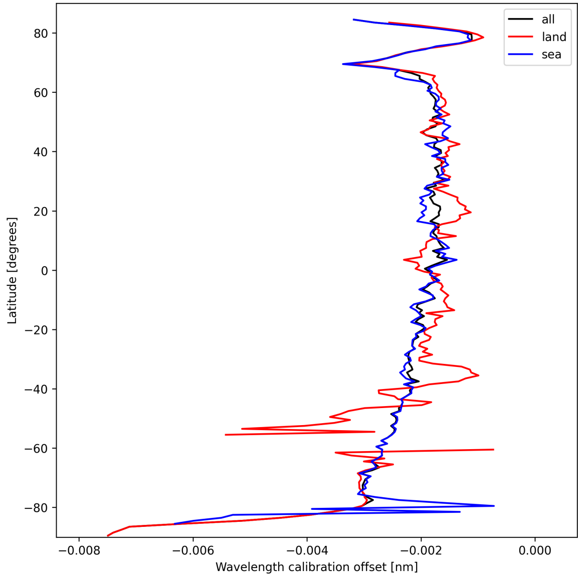
Figure 16: Zonal average of “Wavelength calibration offset” for 2025-03-10 to 2025-03-10.
