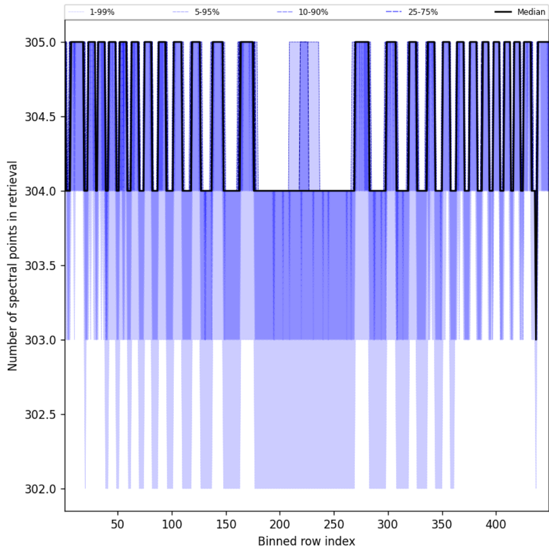
Figure 48: Along track statistics of “Number of spectral points in retrieval” for 2025-03-10 to 2025-03-10
