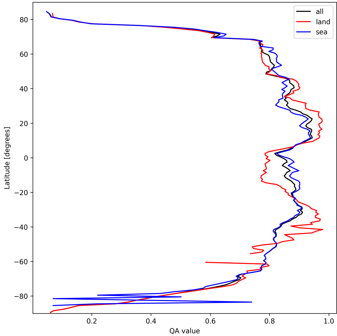
Figure 9: Zonal average of “QA value” for 2025-03-10 to 2025-03-10.
