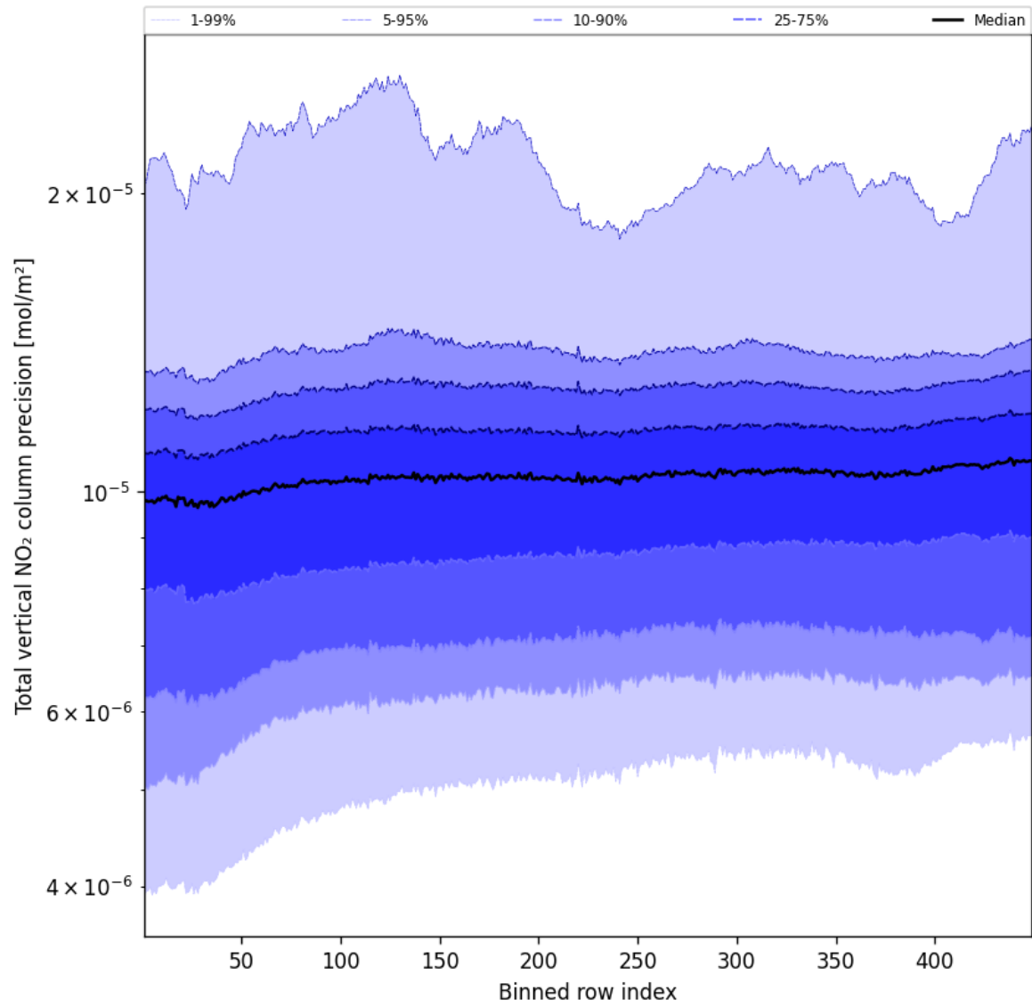
Figure 54: Along track statistics of “Total vertical NO 2 column precision” for 2025-03-10 to 2025-03-10
