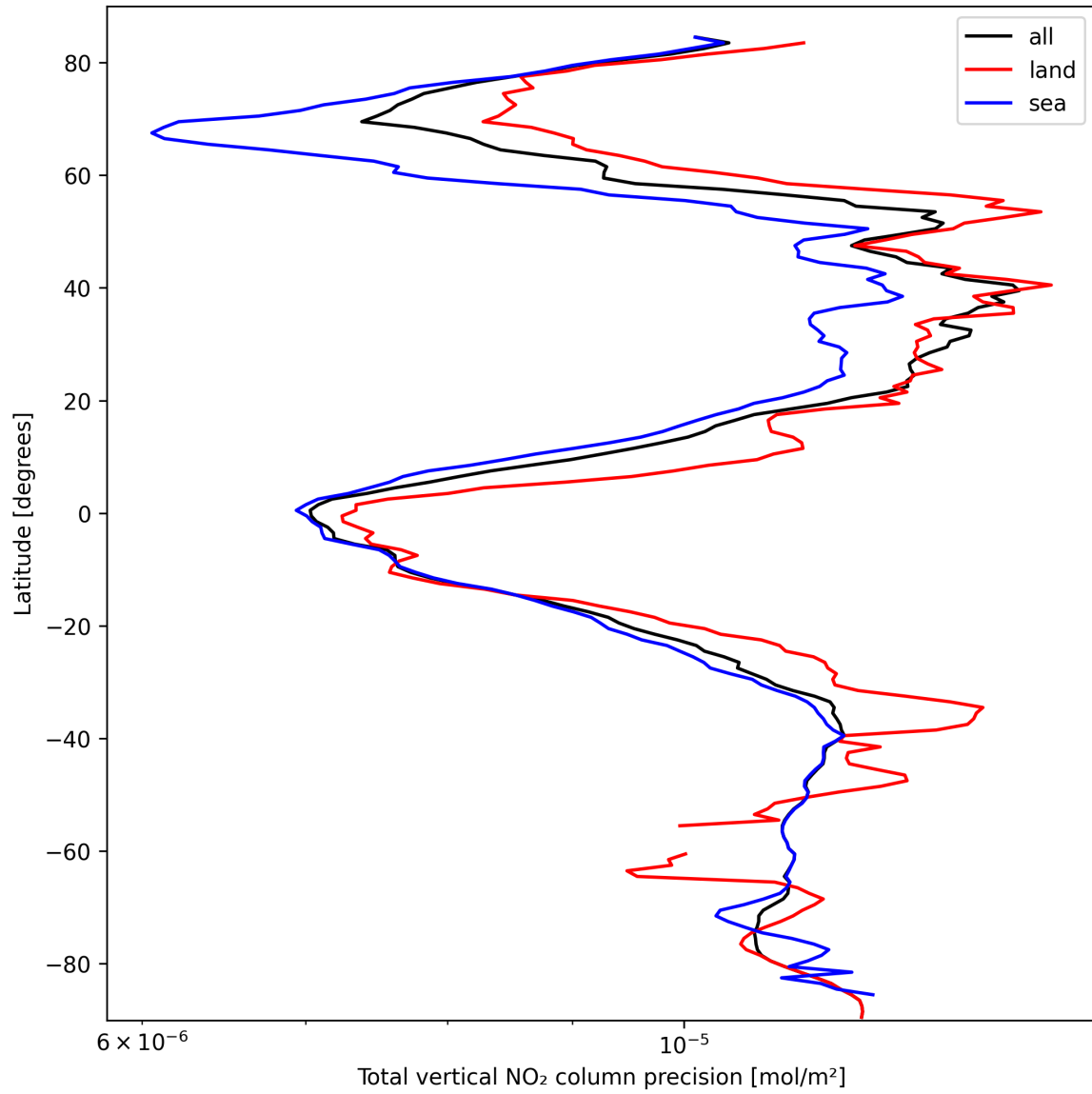
Figure 20: Zonal average of “Total vertical NO 2 column precision” for 2025-03-10 to 2025-03-10.
