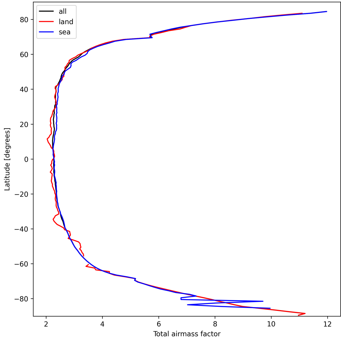
Figure 13: Zonal average of “Total airmass factor” for 2025-03-10 to 2025-03-10.
