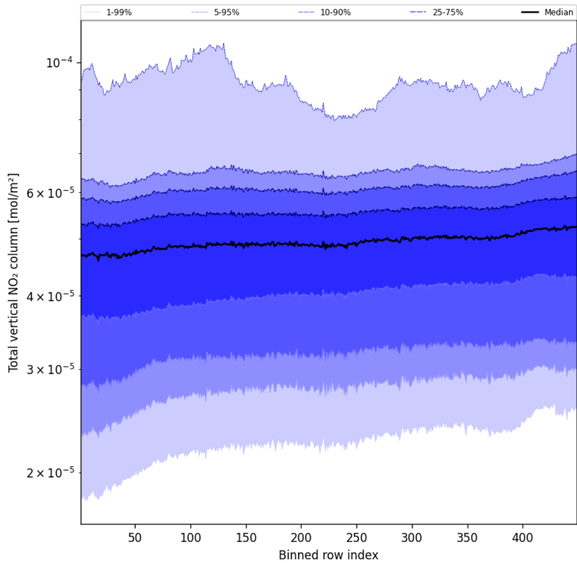
Figure 53: Along track statistics of “Total vertical NO 2 column” for 2025-03-10 to 2025-03-10
