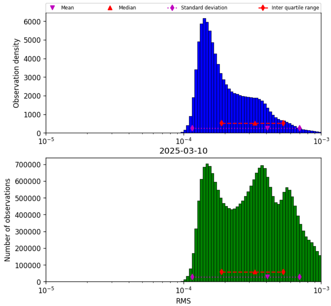
Figure 41: Histogram of “RMS” for 2025-03-10 to 2025-03-10
