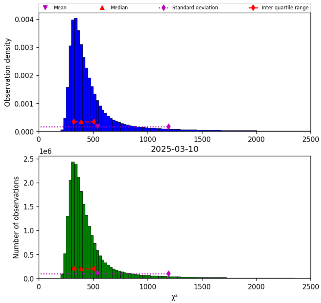
Figure 40: Histogram of “ \chi^2 ” for 2025-03-10 to 2025-03-10
