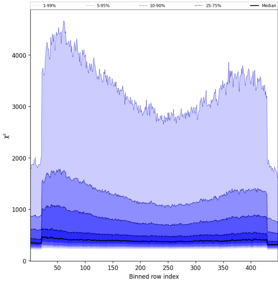
Figure 57: Along track statistics of “ \chi^2 ” for 2025-03-10 to 2025-03-10
