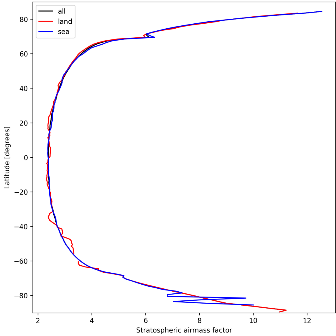
Figure 25: Zonal average of “Stratospheric air mass factor” for 2025-03-10 to 2025-03-10.
