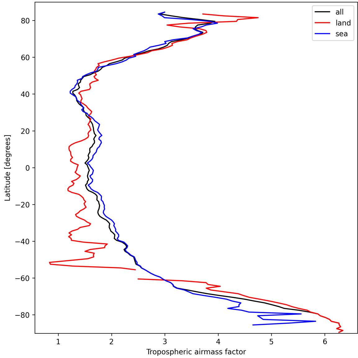
Figure 12: Zonal average of “Tropospheric airmass factor” for 2025-03-10 to 2025-03-10.
