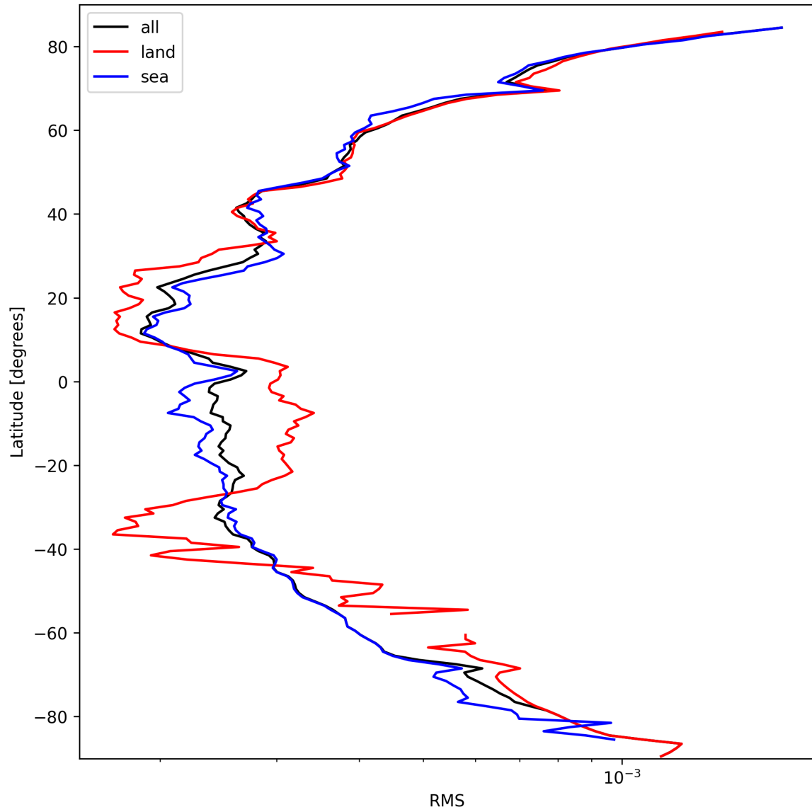
Figure 24: Zonal average of “RMS” for 2025-03-10 to 2025-03-10.
