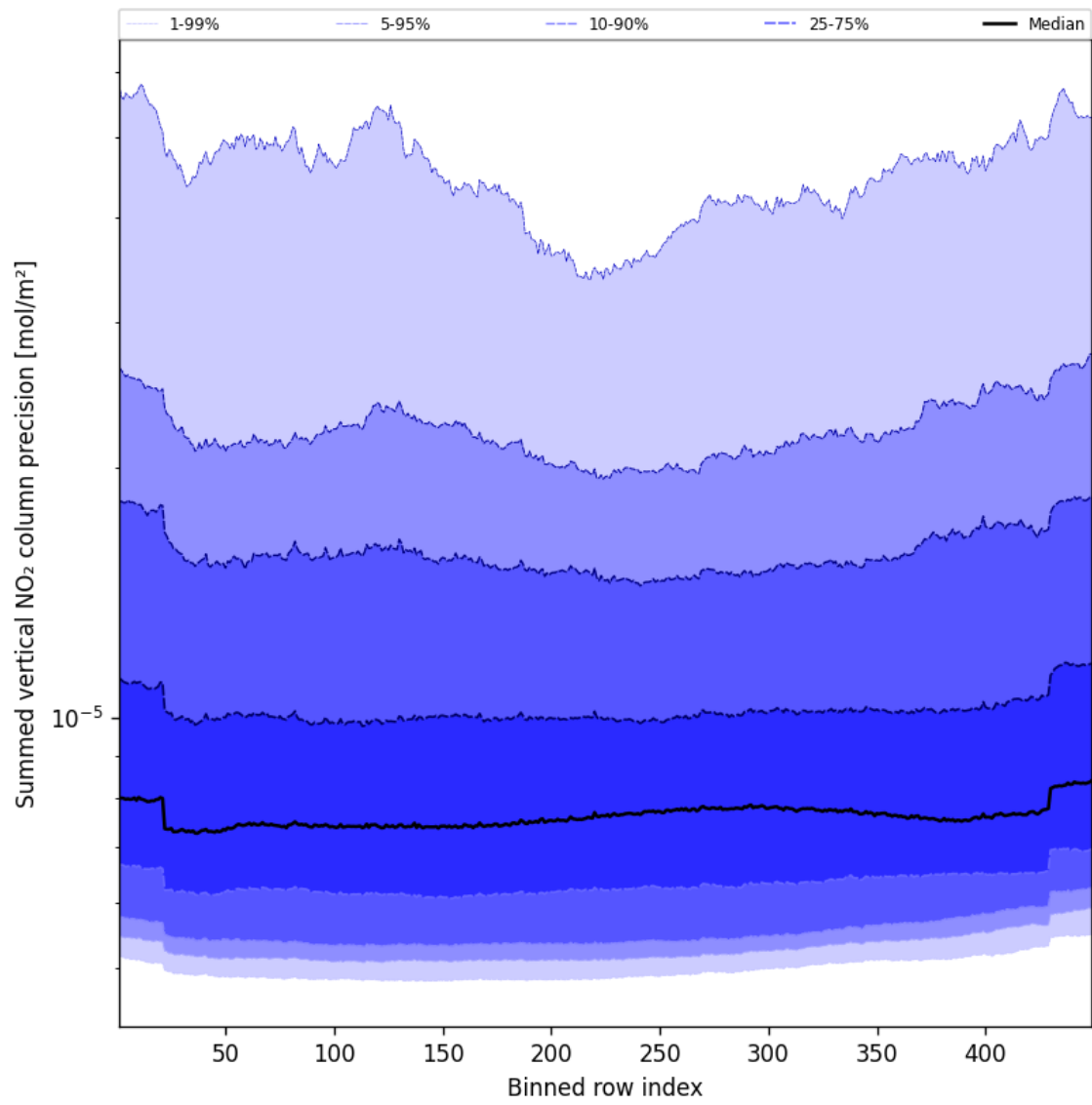
Figure 56: Along track statistics of “Summed vertical NO 2 column precision” for 2025-03-10 to 2025-03-10
