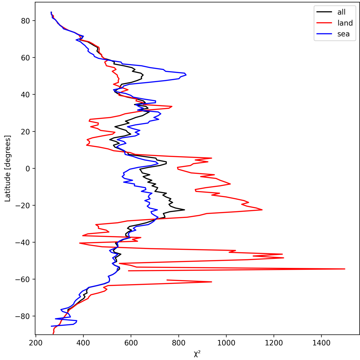
Figure 23: Zonal average of “ \chi^2 ” for 2025-03-10 to 2025-03-10.
