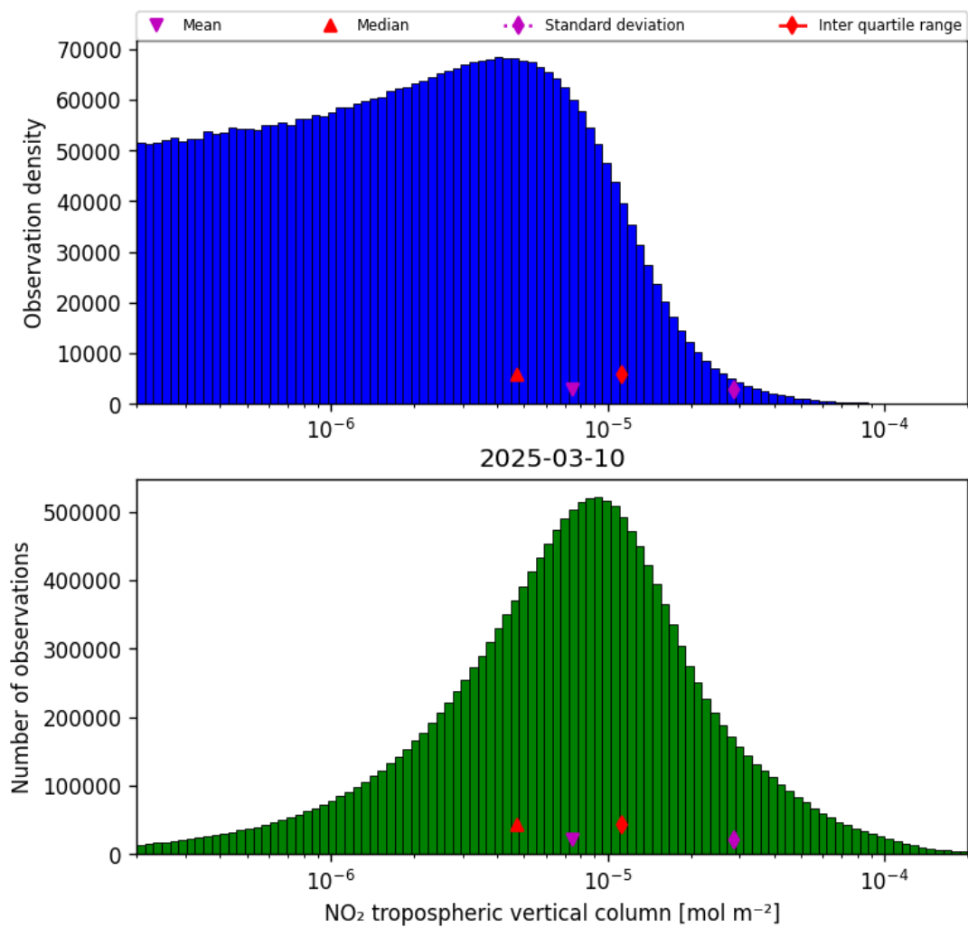
Figure 27: Histogram of “NO 2 tropospheric vertical column” for 2025-03-10 to 2025-03-10
