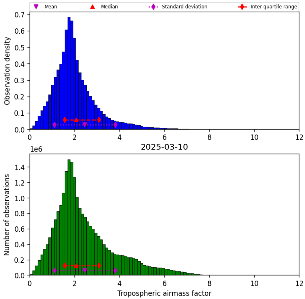
Figure 29: Histogram of “Tropospheric airmass factor” for 2025-03-10 to 2025-03-10
