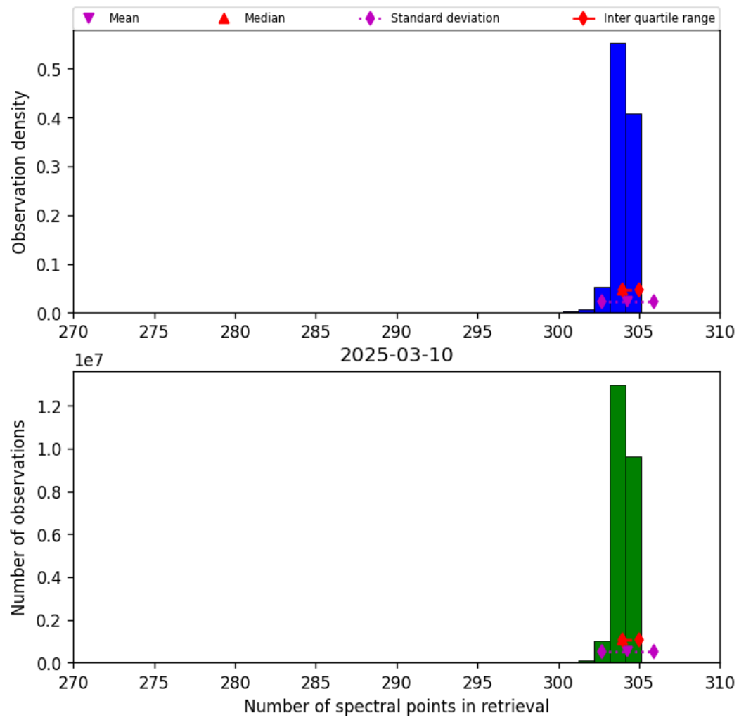
Figure 31: Histogram of “Number of spectral points in retrieval” for 2025-03-10 to 2025-03-10
