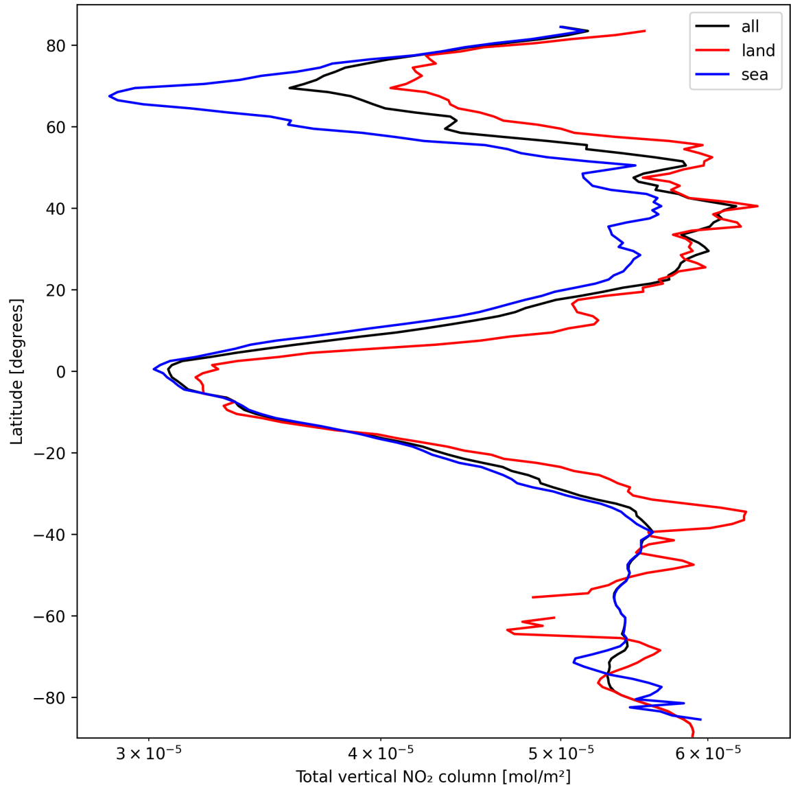
Figure 19: Zonal average of “Total vertical NO 2 column” for 2025-03-10 to 2025-03-10.
