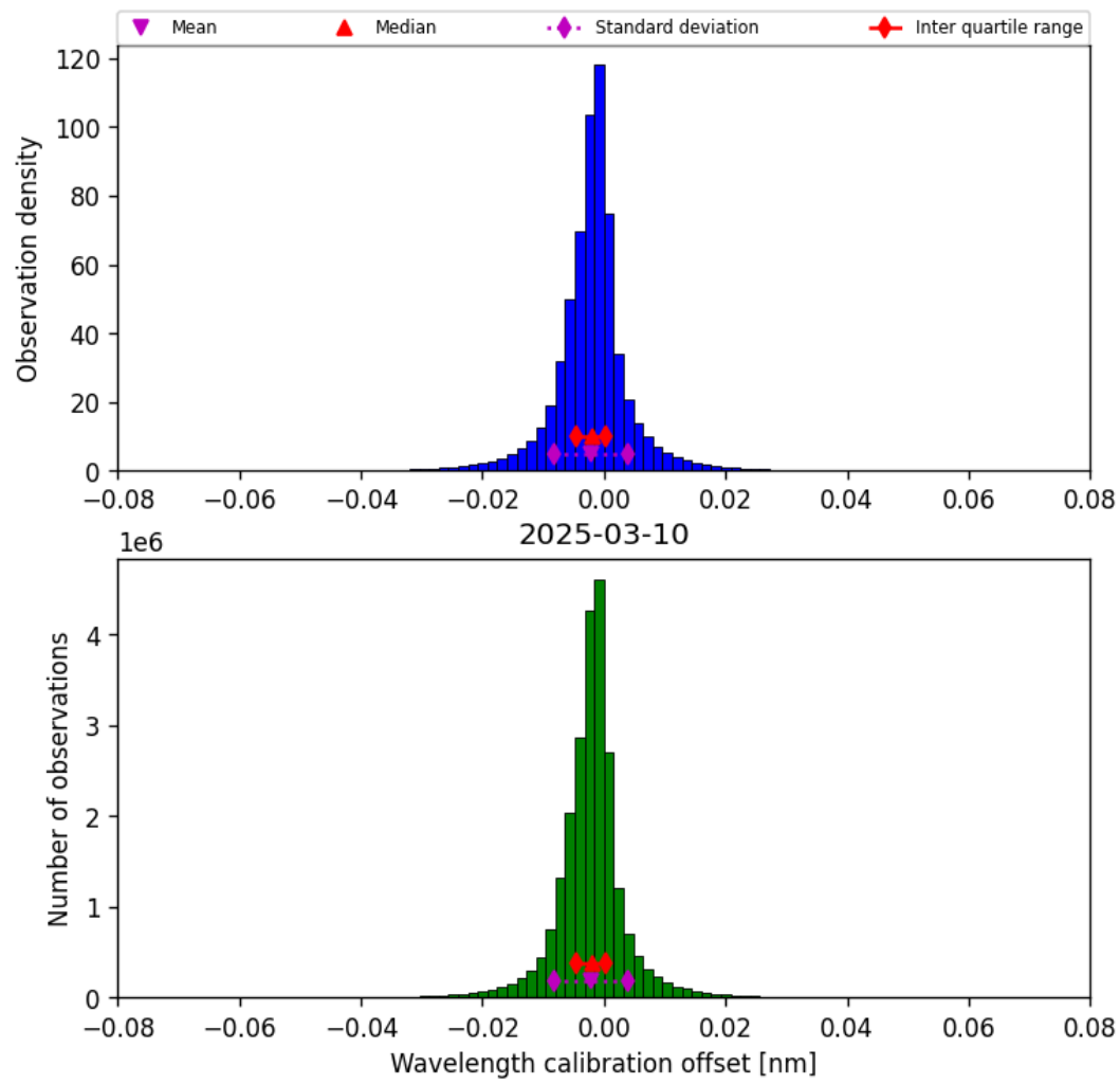
Figure 33: Histogram of “Wavelength calibration offset” for 2025-03-10 to 2025-03-10
