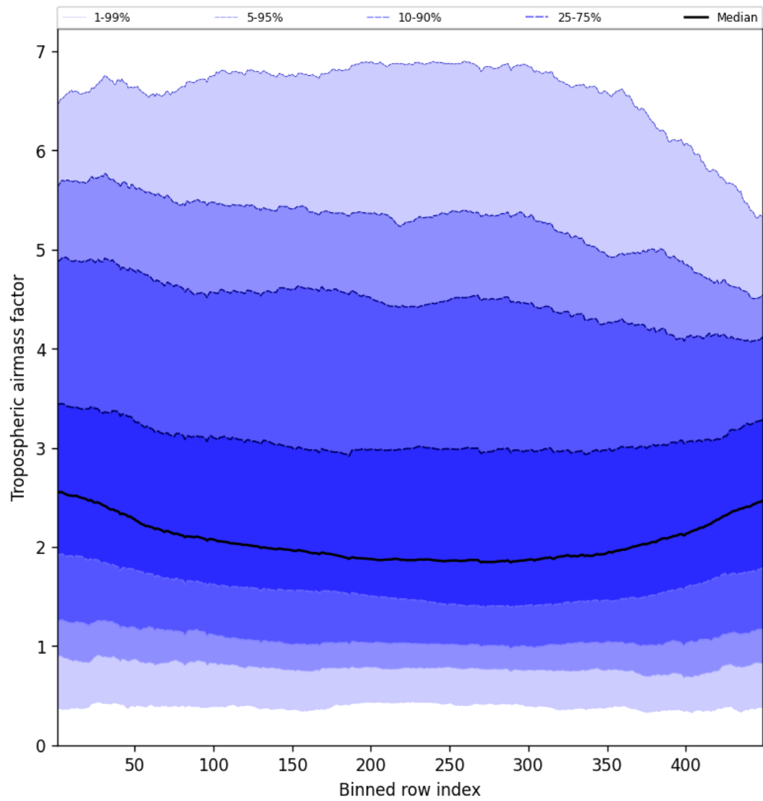
Figure 46: Along track statistics of “Tropospheric airmass factor” for 2025-03-10 to 2025-03-10
