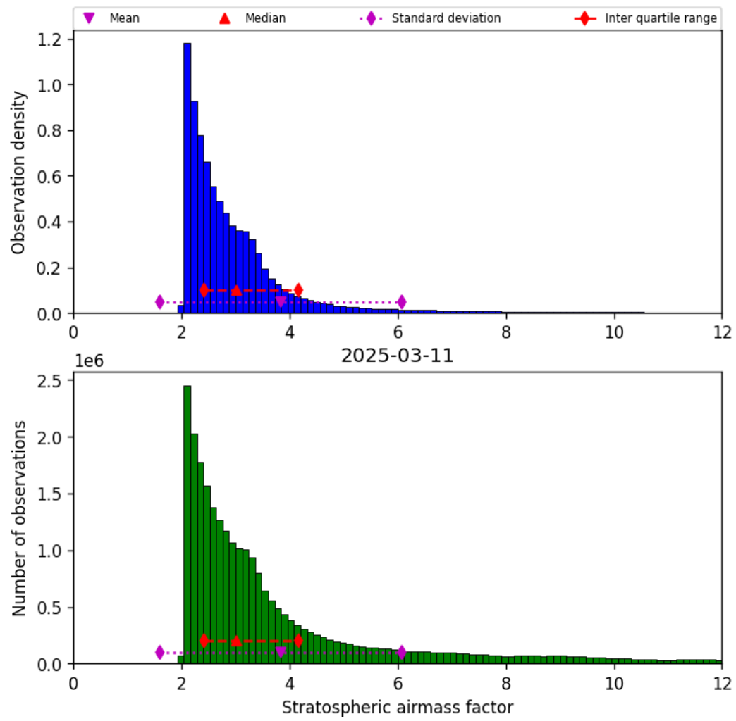
Figure 42: Histogram of “Stratospheric airmass factor” for 2025-03-11 to 2025-03-12
