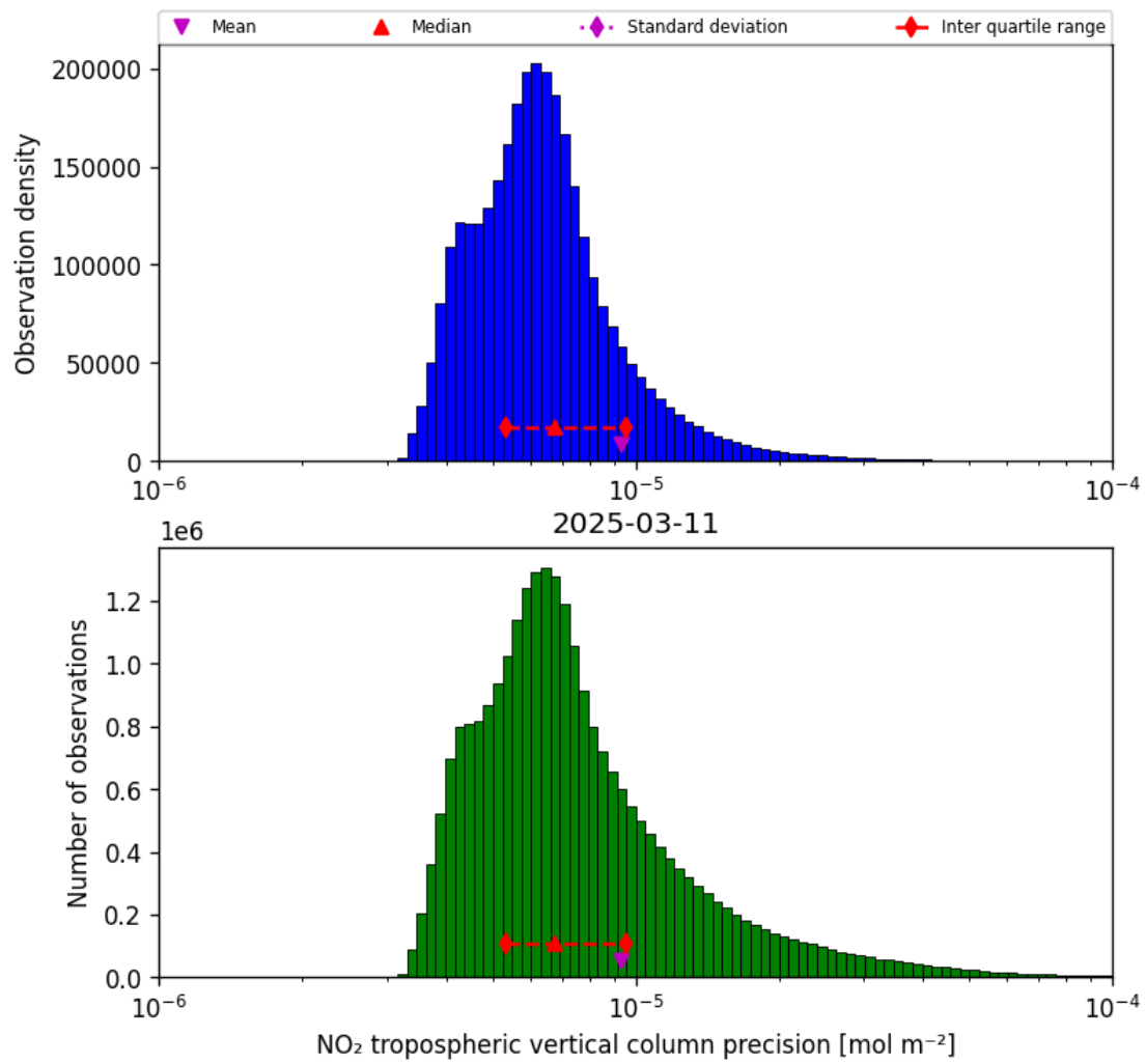
Figure 28: Histogram of “NO 2 tropospheric vertical column precision” for 2025-03-11 to 2025-03-12
