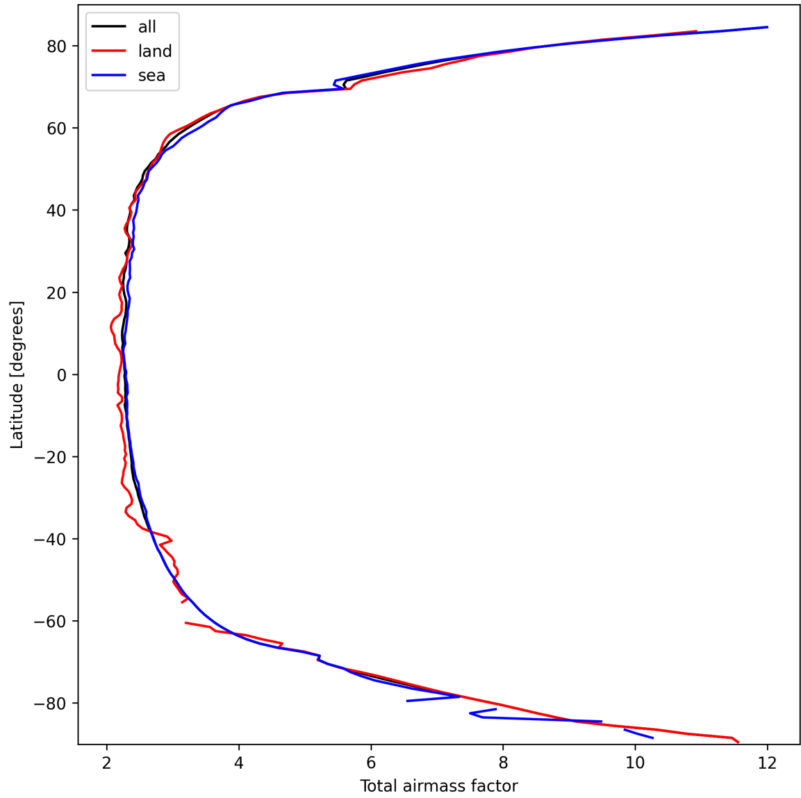
Figure 13: Zonal average of “Total airmass factor” for 2025-03-11 to 2025-03-12.
