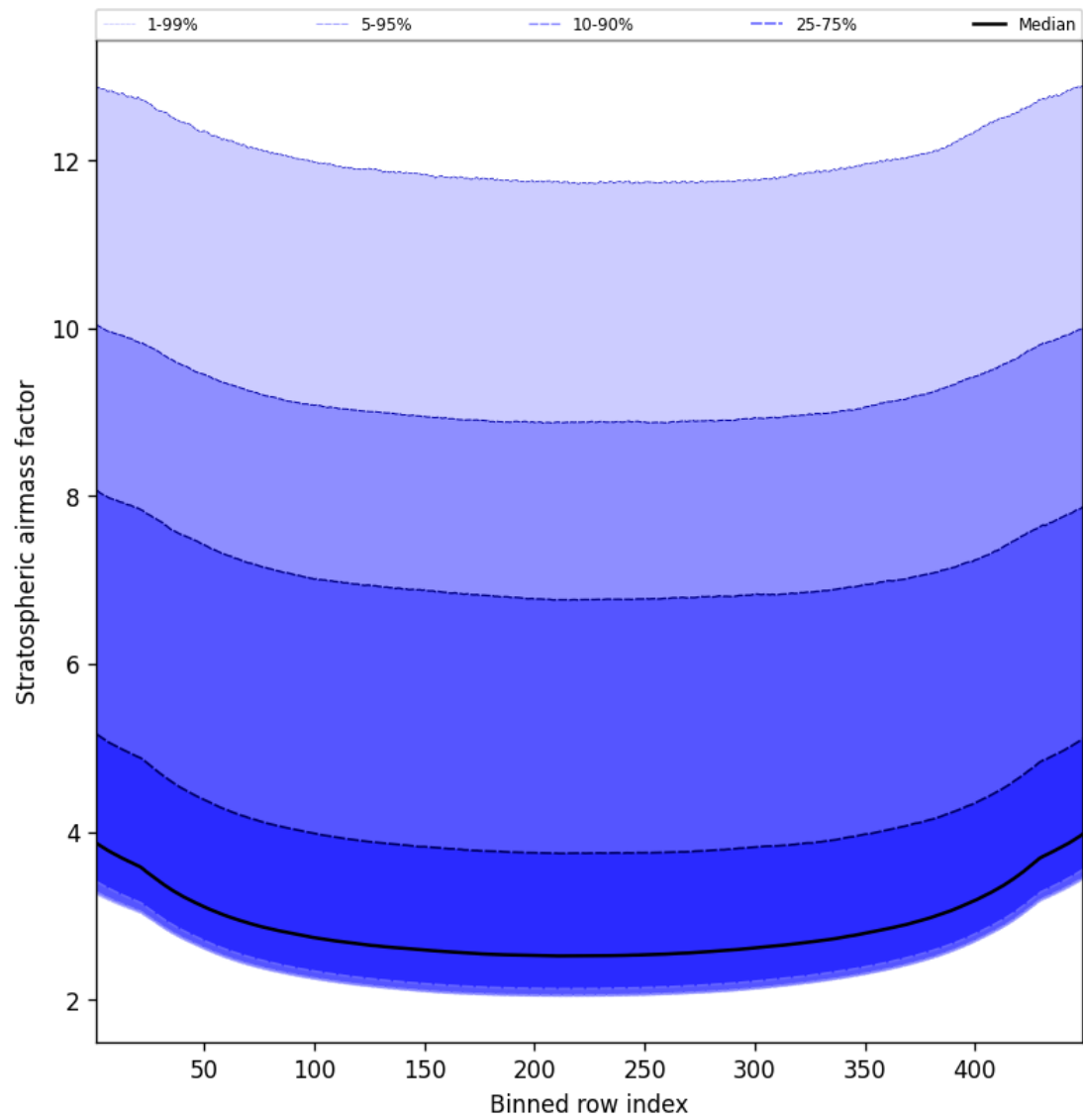
Figure 59: Along track statistics of “Stratospheric airmass factor” for 2025-03-11 to 2025-03-12
