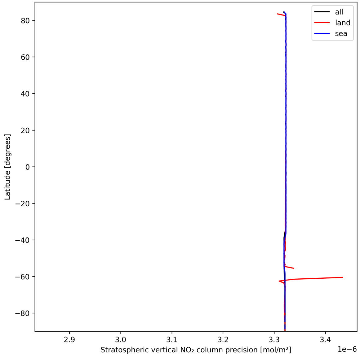
Figure 18: Zonal average of “Stratospheric vertical NO 2 column precision” for 2025-03-11 to 2025-03-12.
