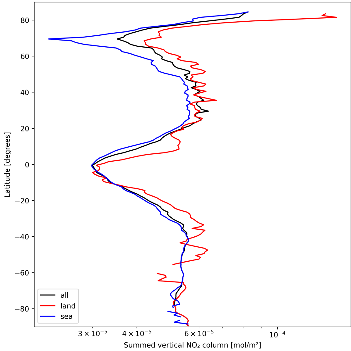
Figure 21: Zonal average of “Summed vertical NO 2 column” for 2025-03-11 to 2025-03-12.
