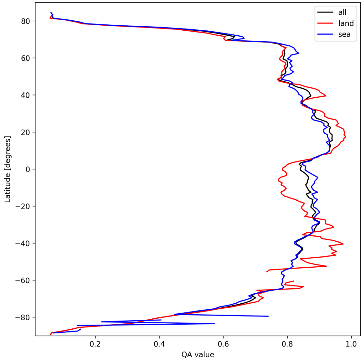
Figure 9: Zonal average of “QA value” for 2025-03-11 to 2025-03-12.
