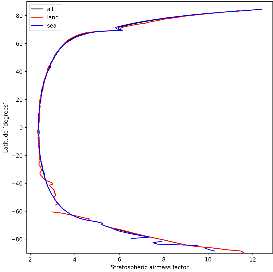
Figure 25: Zonal average of “Stratospheric airmass factor” for 2025-03-11 to 2025-03-12.
