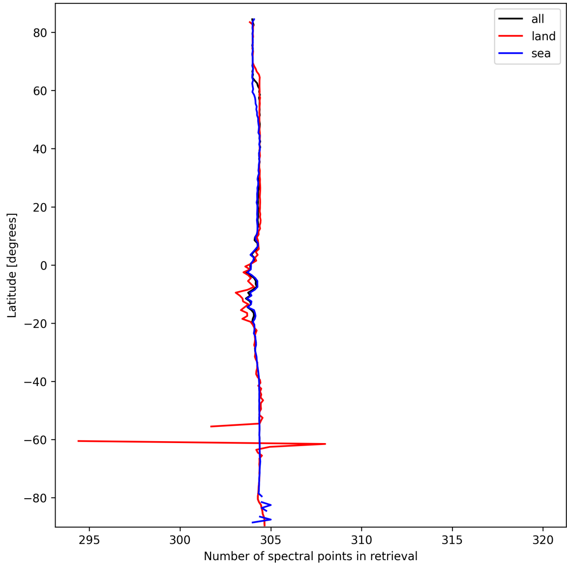
Figure 14: Zonal average of “Number of spectral points in retrieval” for 2025-03-11 to 2025-03-12.
