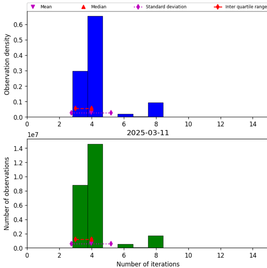
Figure 32: Histogram of “Number of iterations” for 2025-03-11 to 2025-03-12
