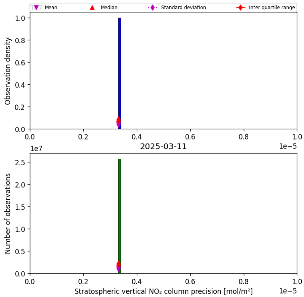
Figure 35: Histogram of “Stratospheric vertical NO 2 column precision” for 2025-03-11 to 2025-03-12
