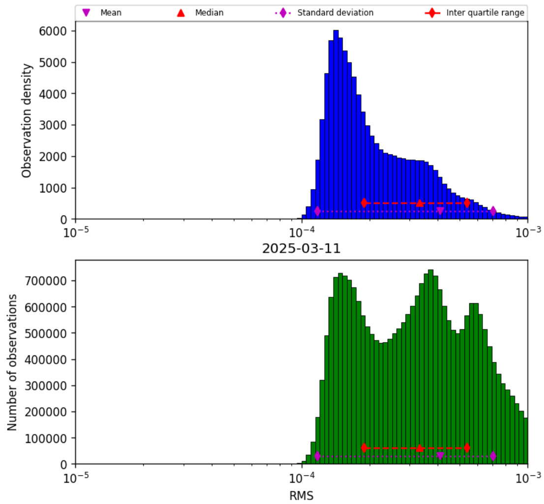
Figure 41: Histogram of “RMS” for 2025-03-11 to 2025-03-12
