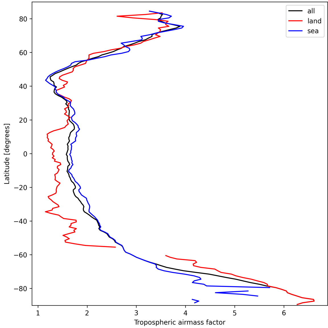
Figure 12: Zonal average of “Tropospheric air mass factor” for 2025-03-11 to 2025-03-12.
