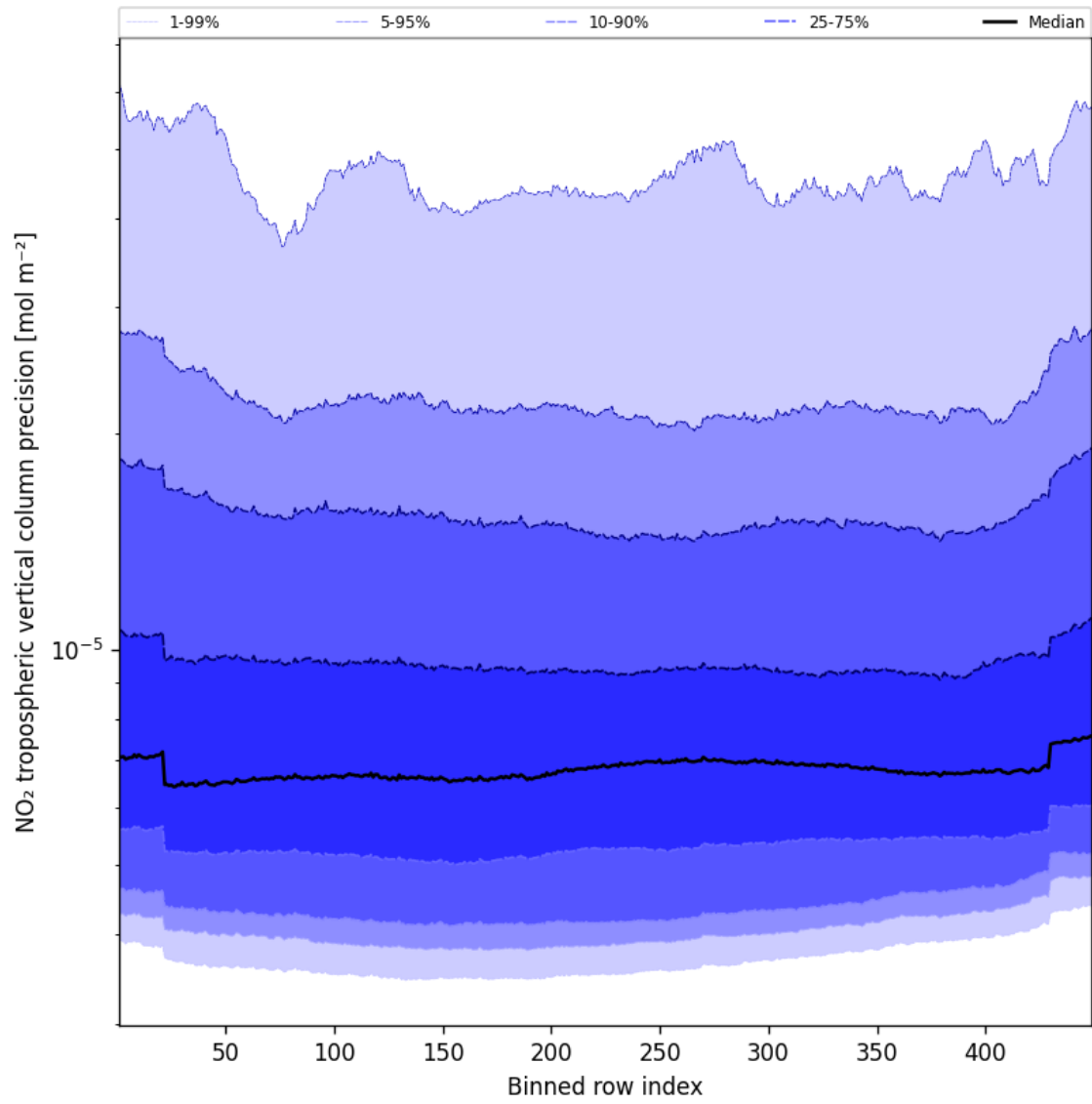
Figure 45: Along track statistics of “NO 2 tropospheric vertical column precision” for 2025-03-11 to 2025-03-12
