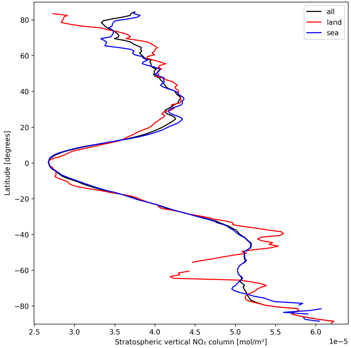
Figure 17: Zonal average of “Stratospheric vertical NO 2 column” for 2025-03-11 to 2025-03-12.
