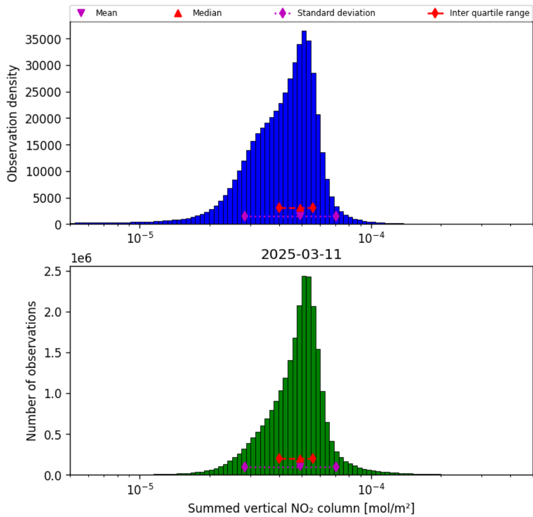
Figure 38: Histogram of “Summed vertical NO 2 column” for 2025-03-11 to 2025-03-12
