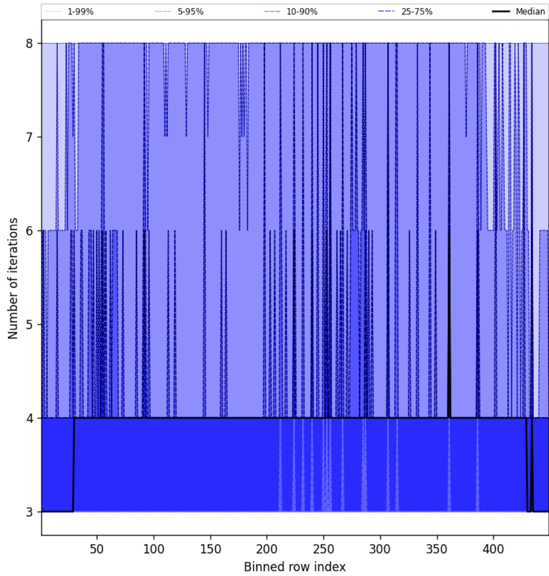
Figure 49: Along track statistics of “Number of iterations” for 2025-03-11 to 2025-03-12
