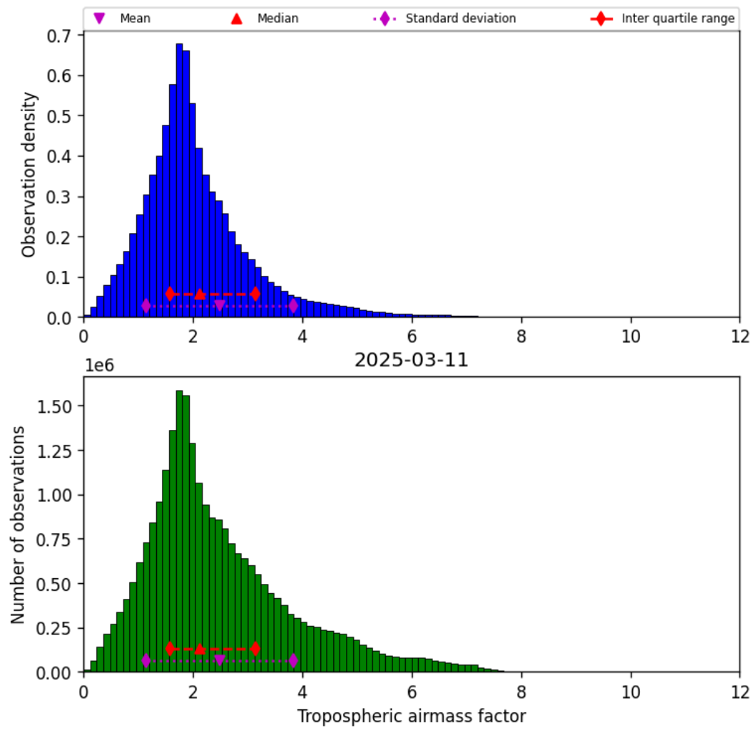
Figure 29: Histogram of “Tropospheric airmass factor” for 2025-03-11 to 2025-03-12
