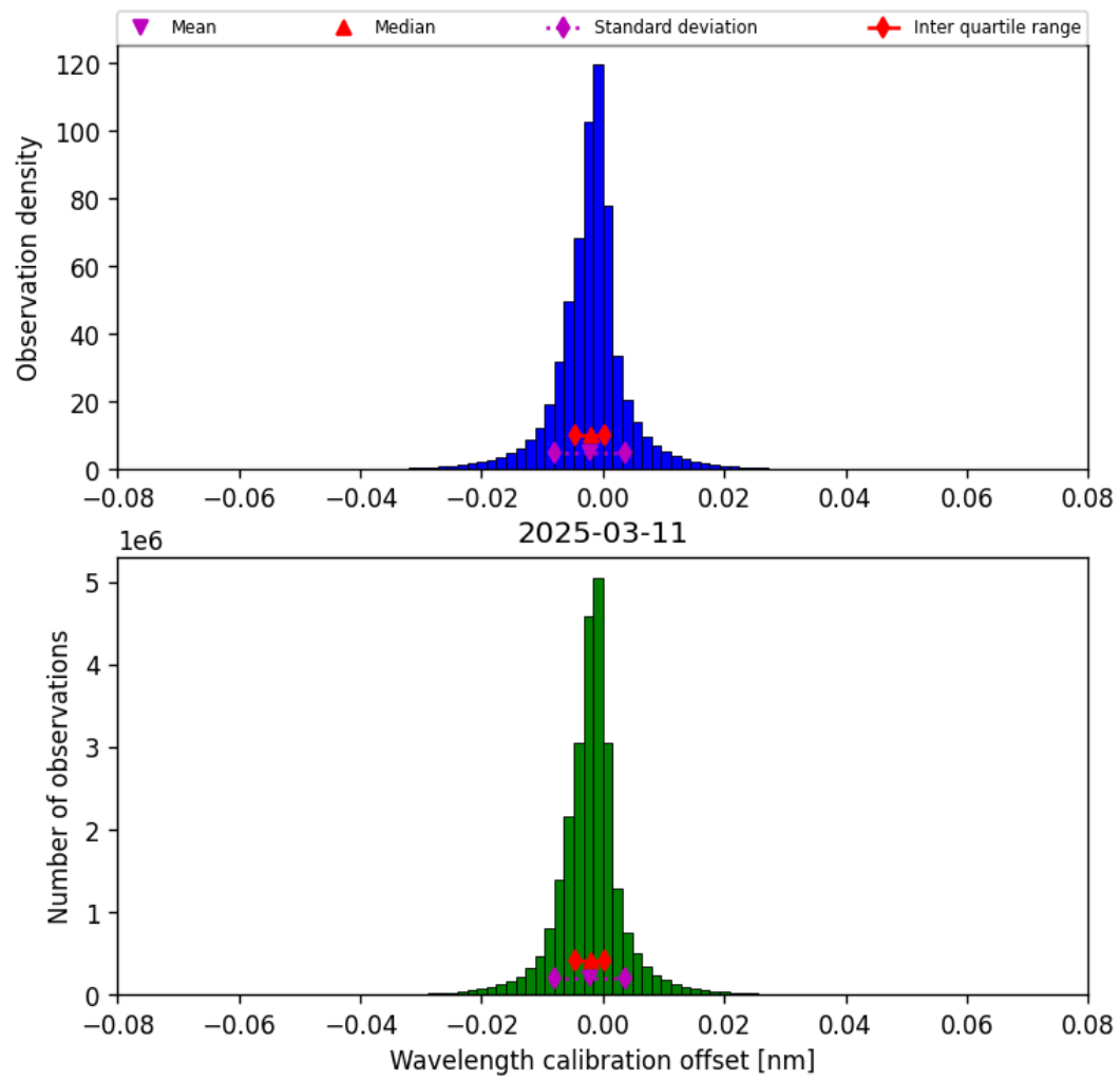
Figure 33: Histogram of “Wavelength calibration offset” for 2025-03-11 to 2025-03-12
