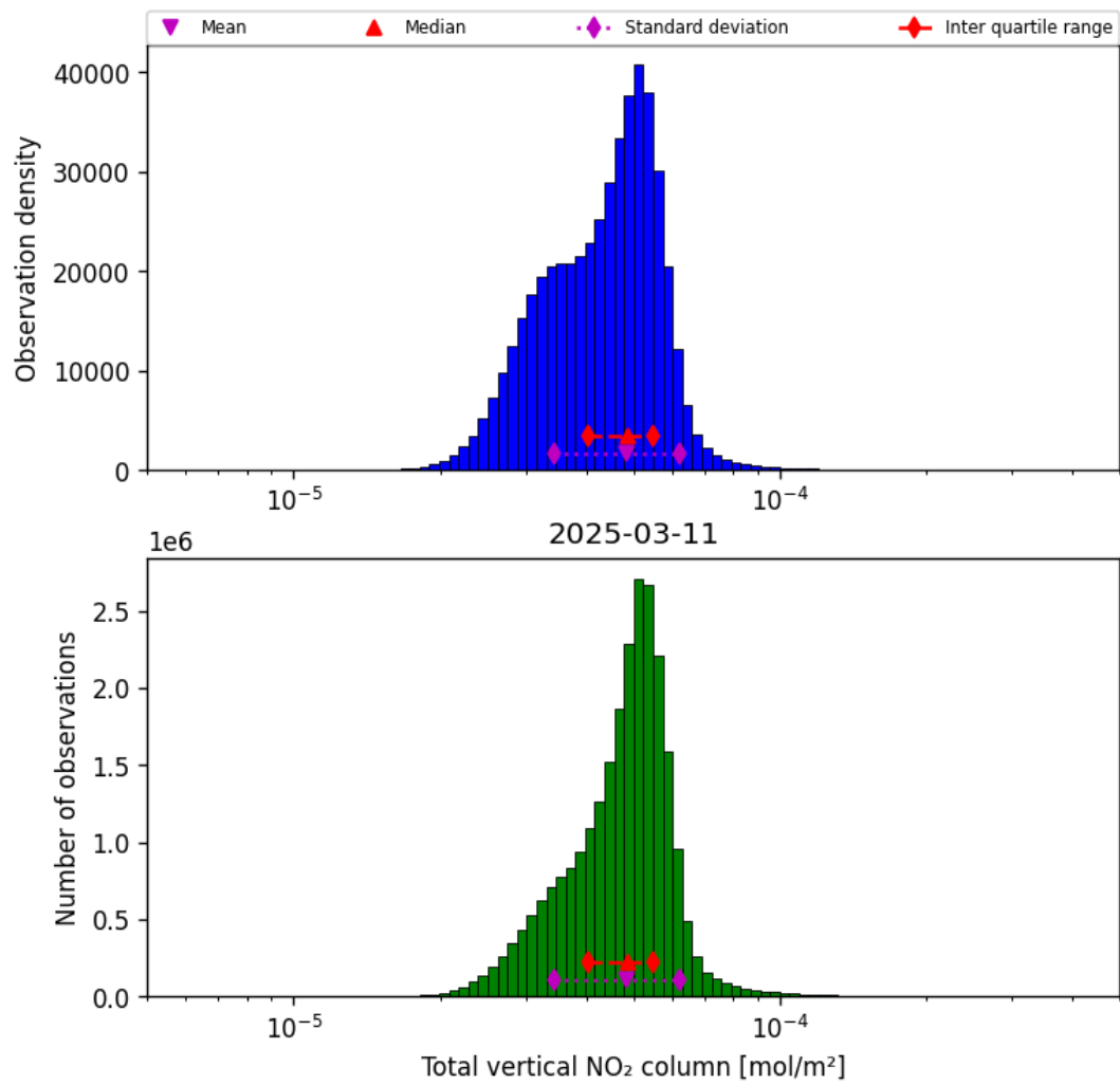
Figure 36: Histogram of “Total vertical NO 2 column” for 2025-03-11 to 2025-03-12
