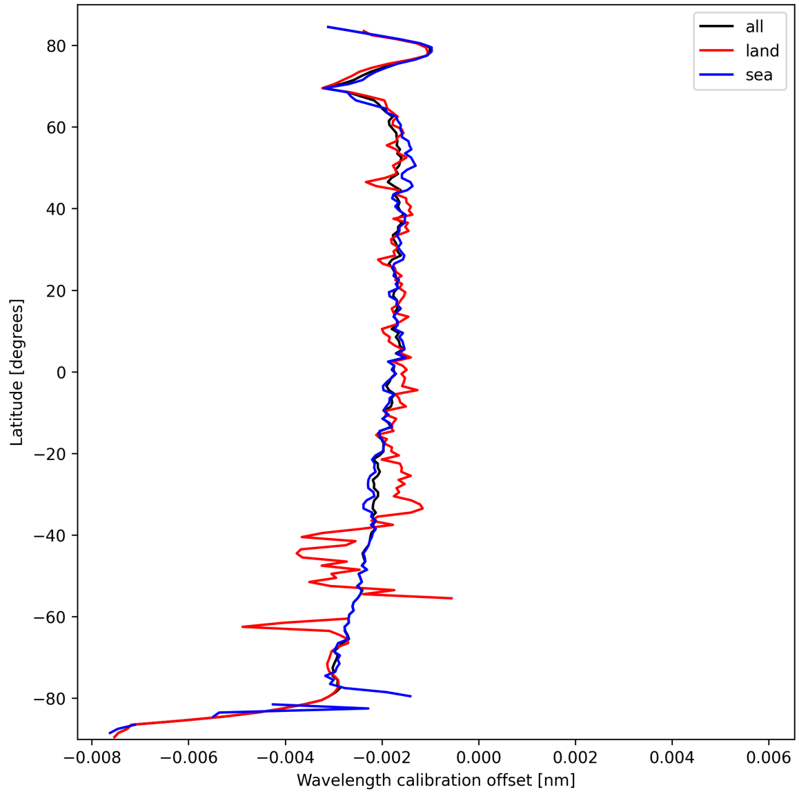
Figure 16: Zonal average of “Wavelength calibration offset” for 2025-03-11 to 2025-03-12.
