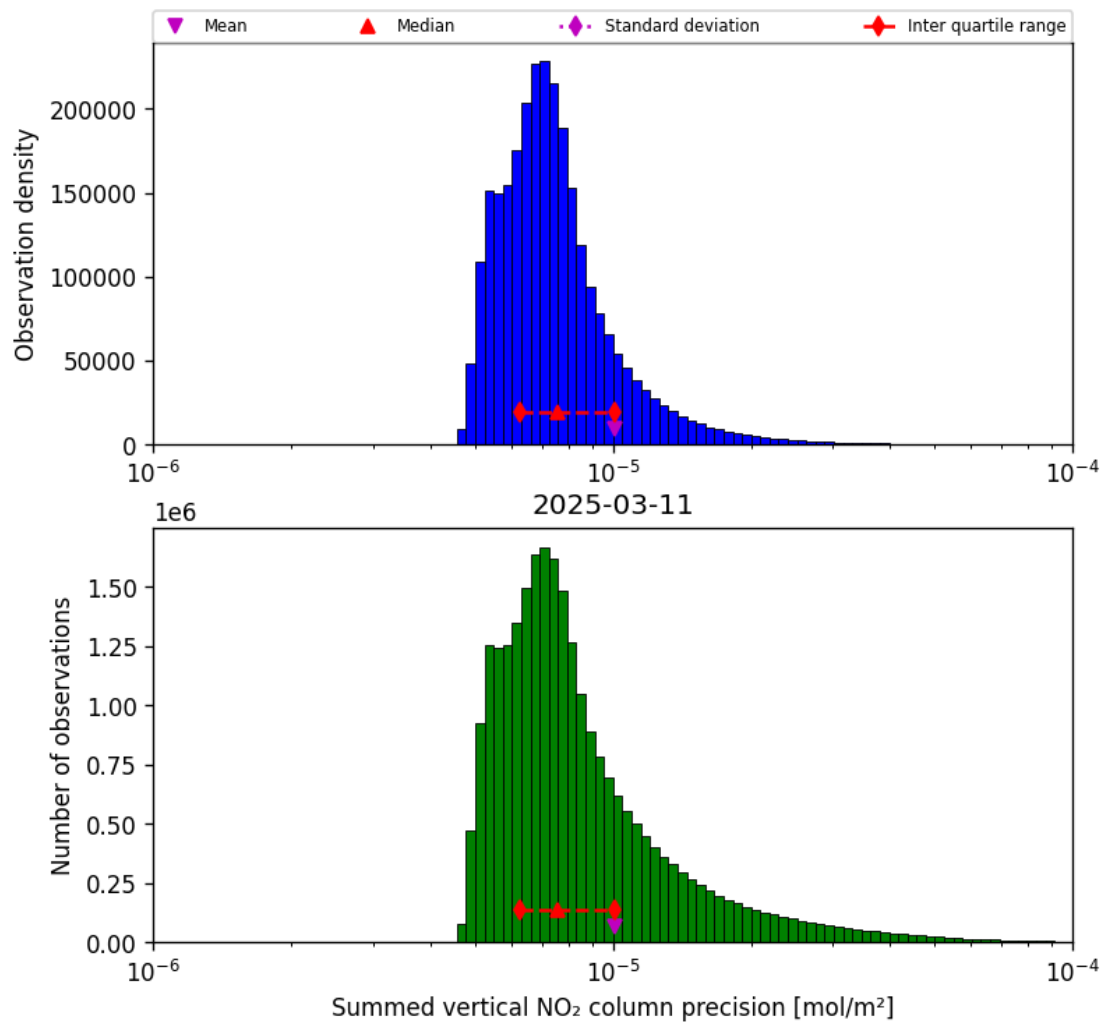
Figure 39: Histogram of “Summed vertical NO 2 column precision” for 2025-03-11 to 2025-03-12
