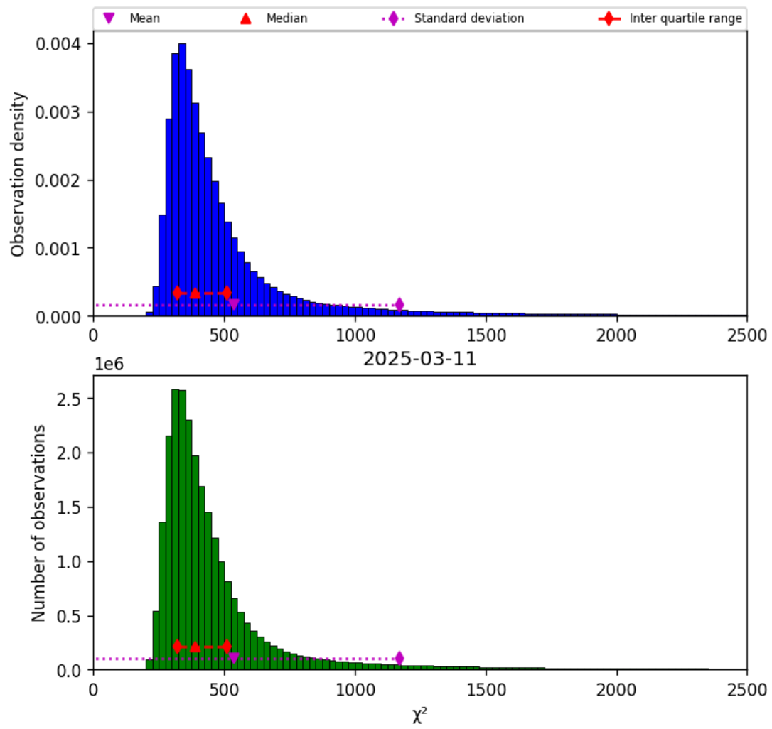
Figure 40: Histogram of “ \chi^2 ” for 2025-03-11 to 2025-03-12
