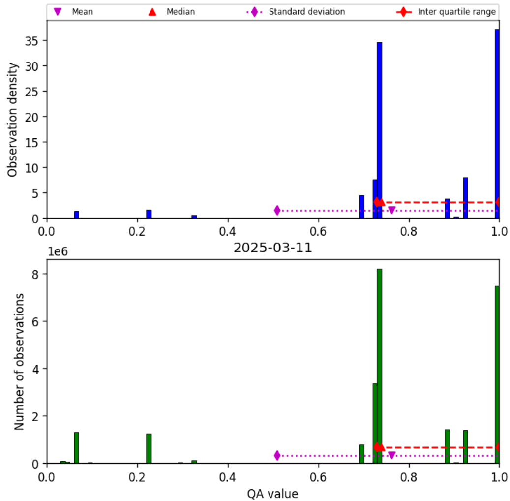
Figure 26: Histogram of “QA value” for 2025-03-11 to 2025-03-12
