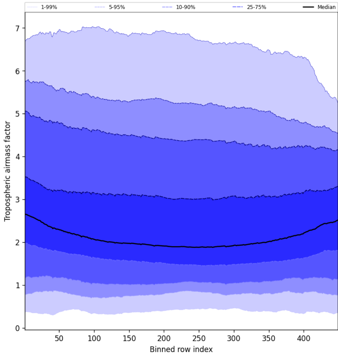
Figure 46: Along track statistics of “Tropospheric airmass factor” for 2025-03-11 to 2025-03-12
