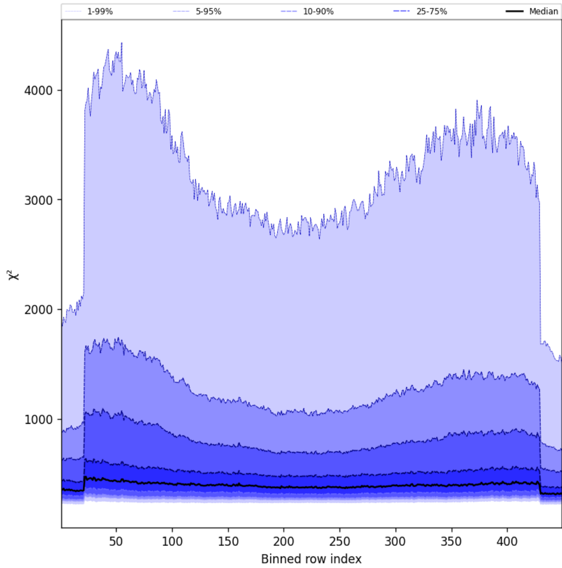
Figure 57: Along track statistics of “ \chi^2 ” for 2025-03-11 to 2025-03-12
