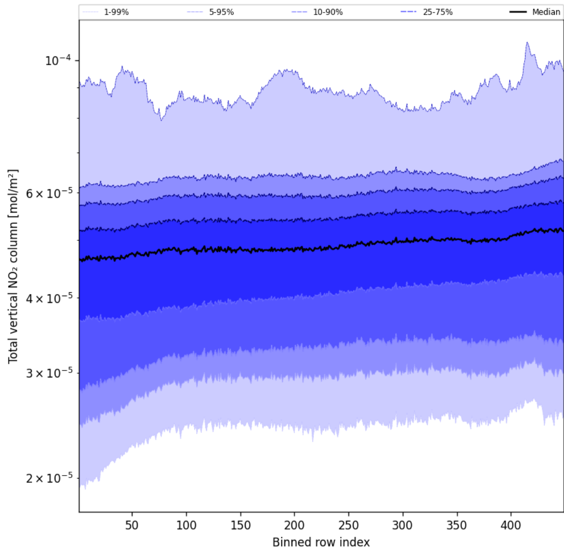
Figure 53: Along track statistics of “Total vertical NO 2 column” for 2025-03-11 to 2025-03-12
