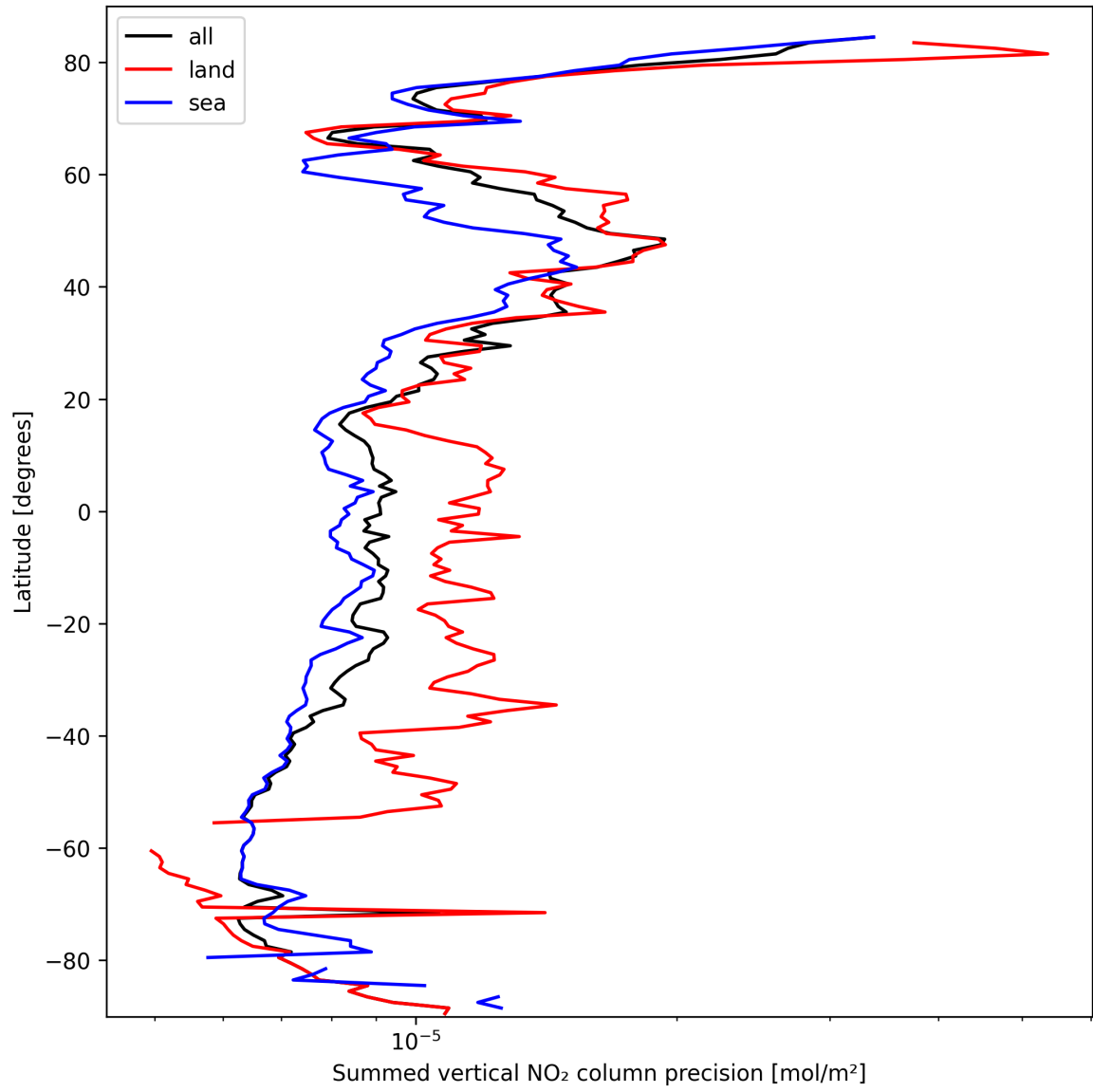
Figure 22: Zonal average of “Summed vertical NO 2 column precision” for 2025-03-11 to 2025-03-12.
