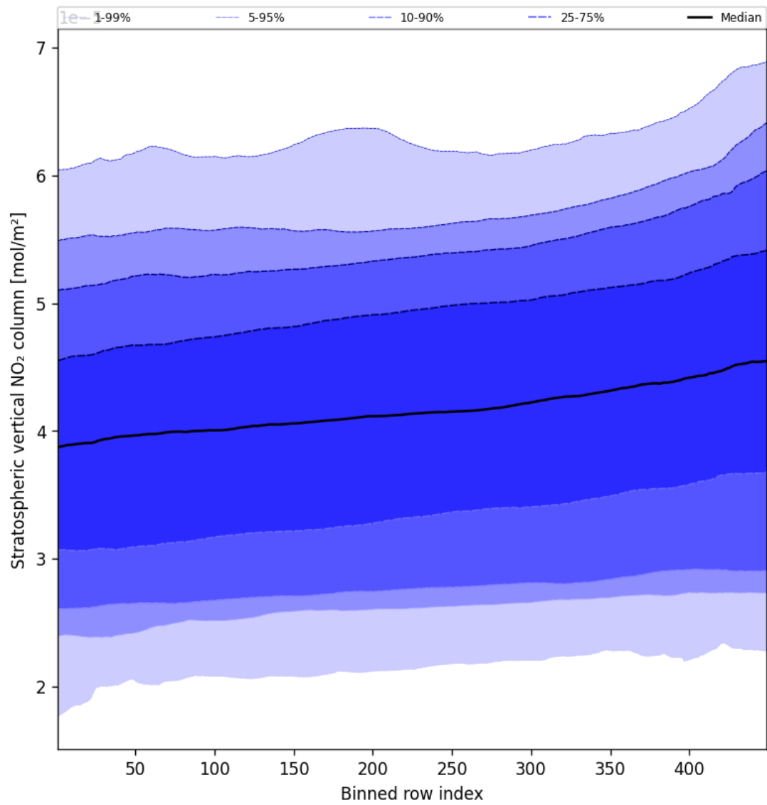
Figure 51: Along track statistics of “Stratospheric vertical NO 2 column” for 2025-03-11 to 2025-03-12
