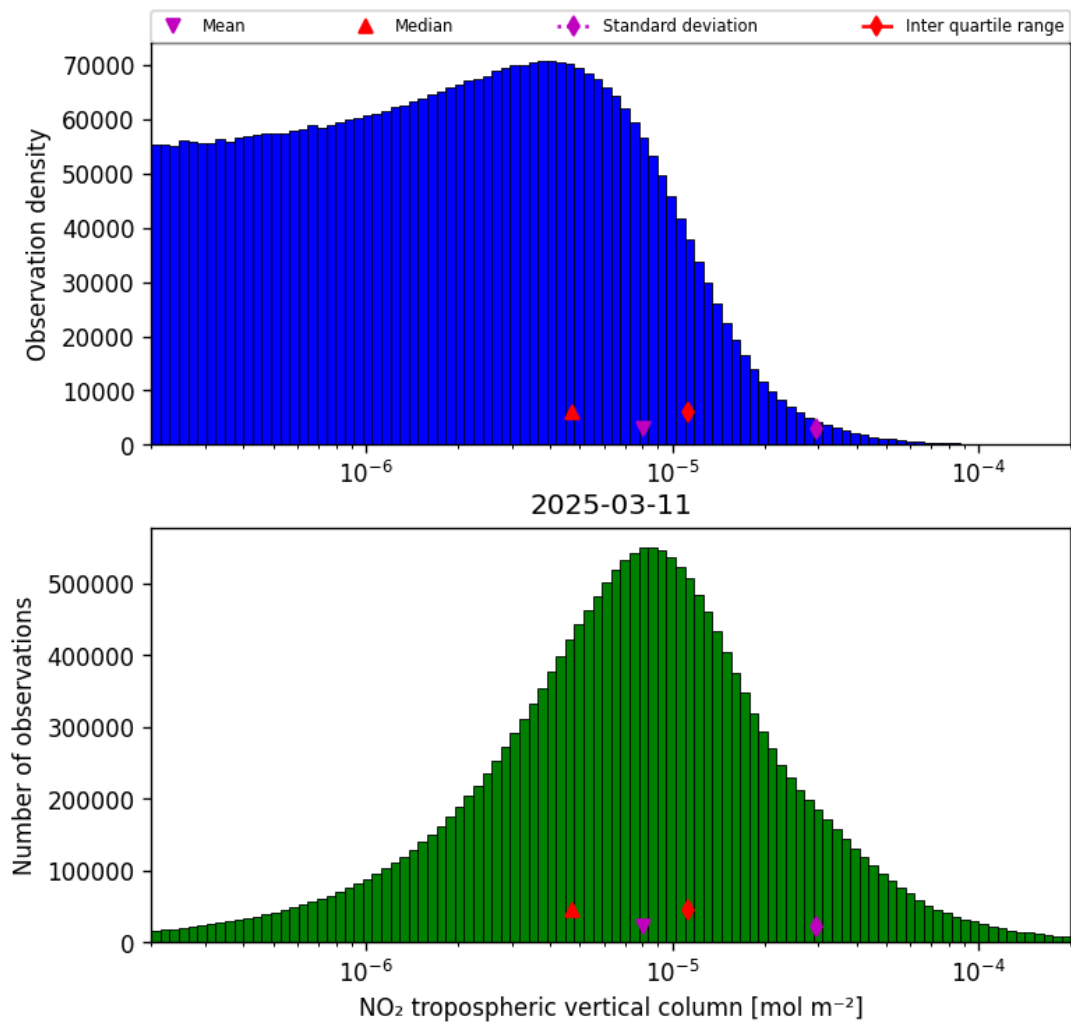
Figure 27: Histogram of “NO 2 tropospheric vertical column” for 2025-03-11 to 2025-03-12
