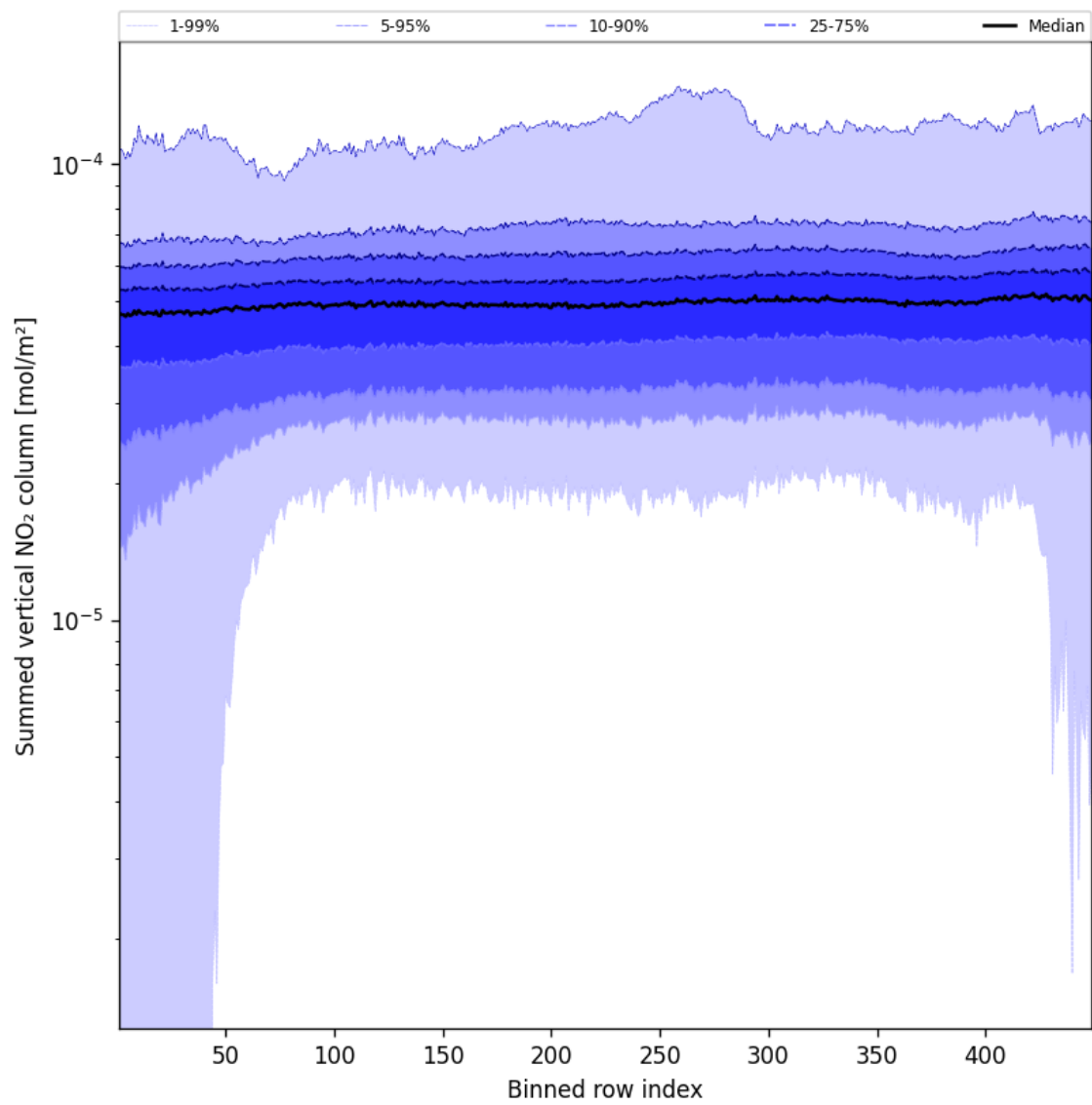
Figure 55: Along track statistics of “Summed vertical NO 2 column” for 2025-03-11 to 2025-03-12
