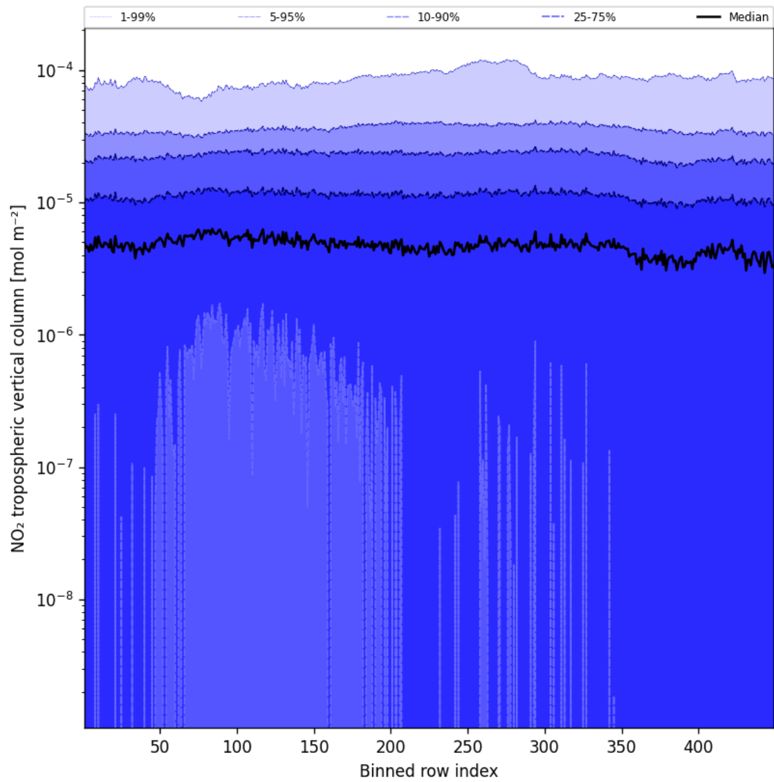
Figure 44: Along track statistics of “NO 2 tropospheric vertical column” for 2025-03-11 to 2025-03-12
