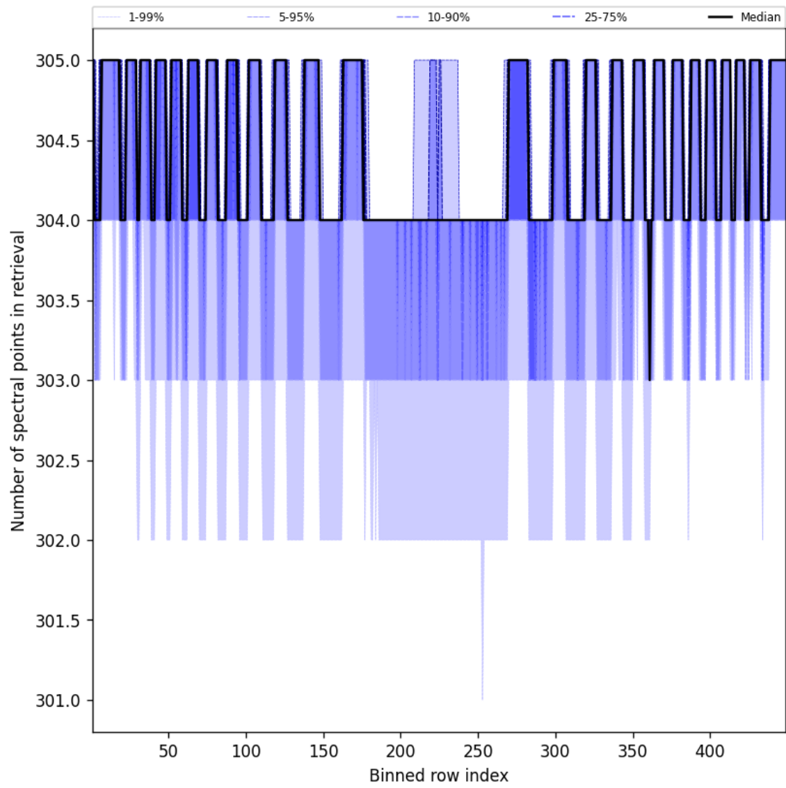
Figure 48: Along track statistics of “Number of spectral points in retrieval” for 2025-03-11 to 2025-03-12
