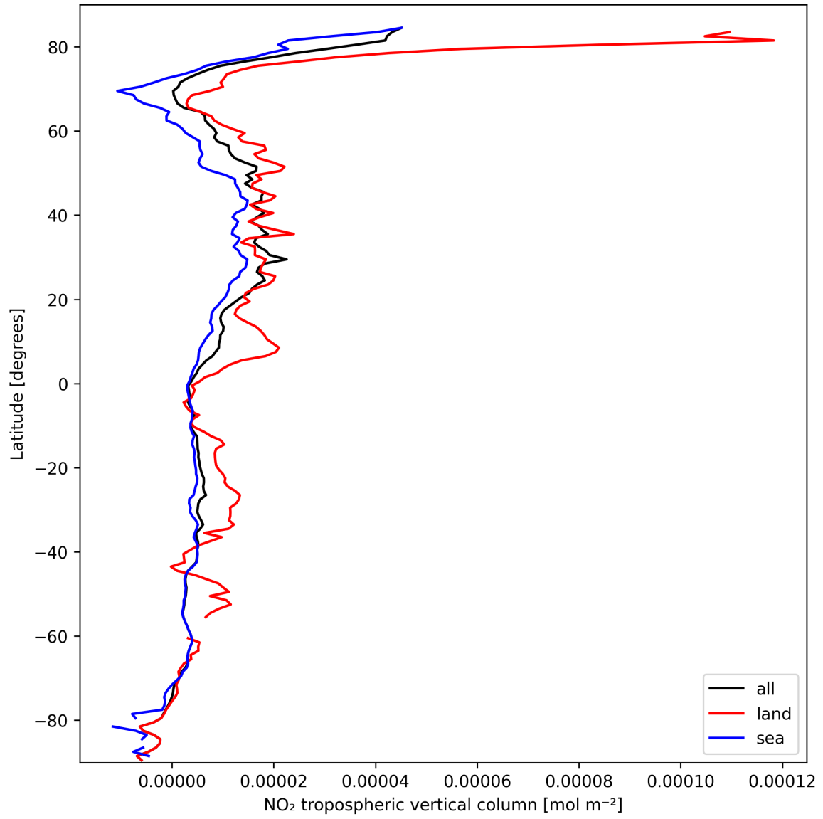
Figure 10: Zonal average of “NO 2 tropospheric vertical column” for 2025-03-11 to 2025-03-12.
