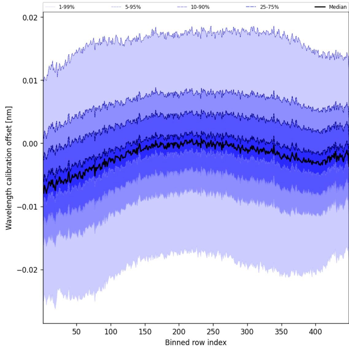
Figure 50: Along track statistics of “Wavelength calibration offset” for 2025-03-11 to 2025-03-12
