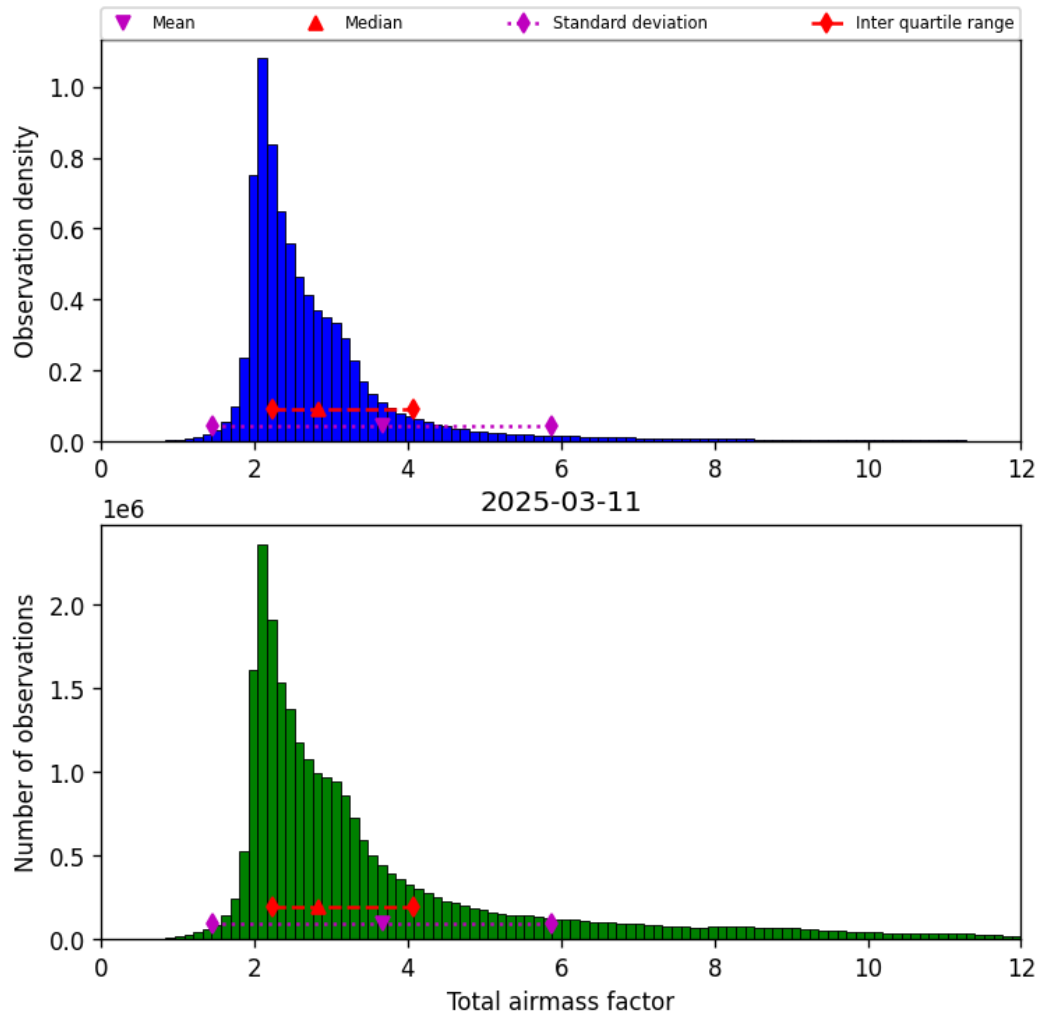
Figure 30: Histogram of “Total airmass factor” for 2025-03-11 to 2025-03-12
