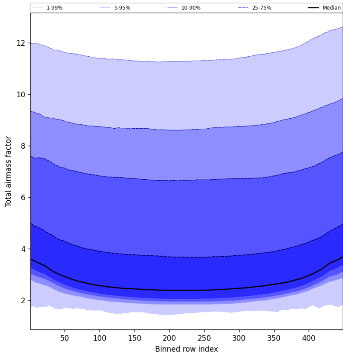
Figure 47: Along track statistics of “Total airmass factor” for 2025-03-11 to 2025-03-12
