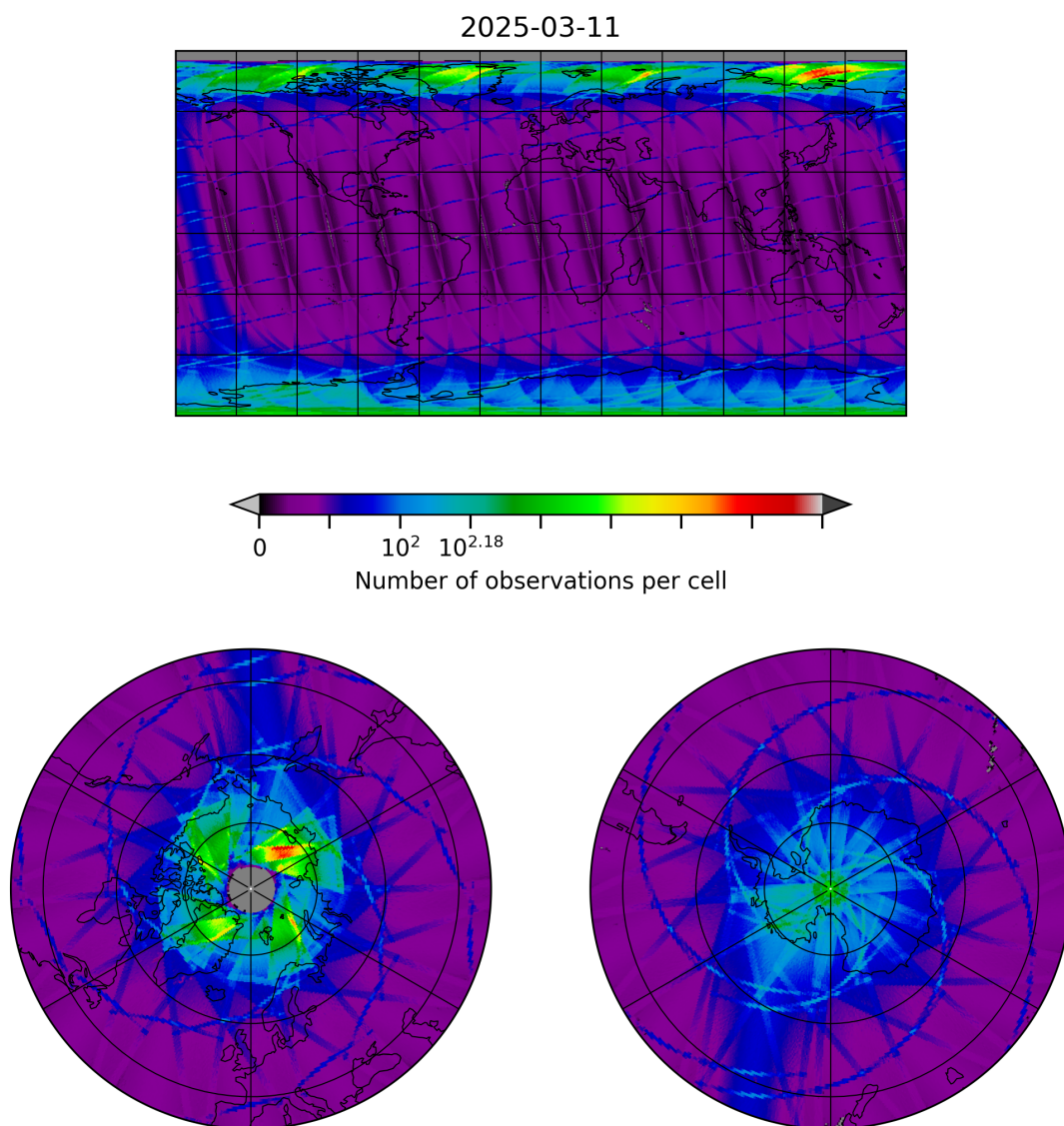
Figure 8: Map of the number of observations for 2025-03-11 to 2025-03-12
