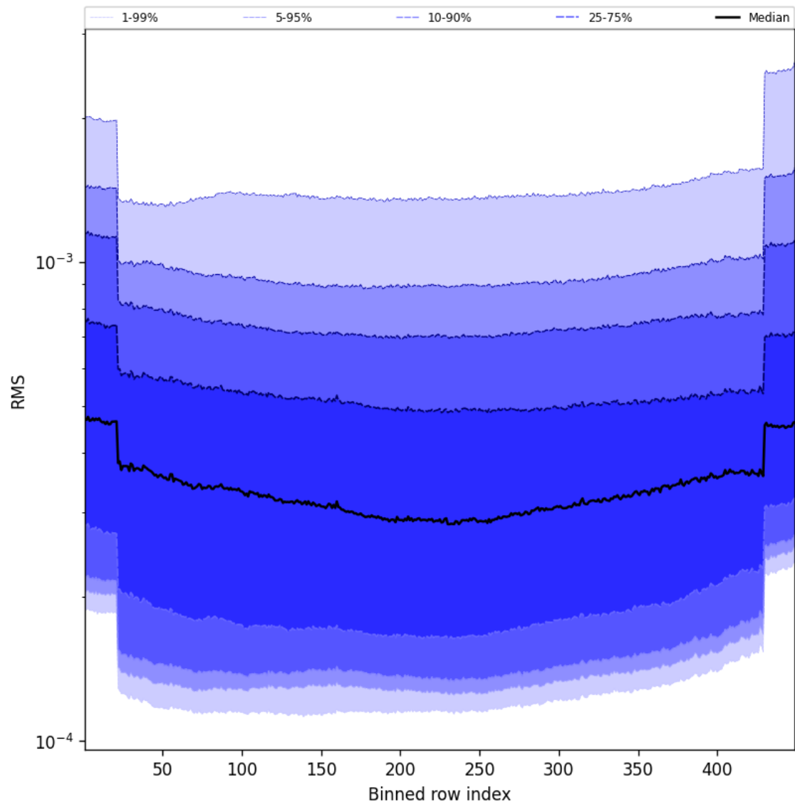
Figure 58: Along track statistics of “RMS” for 2025-03-11 to 2025-03-12
