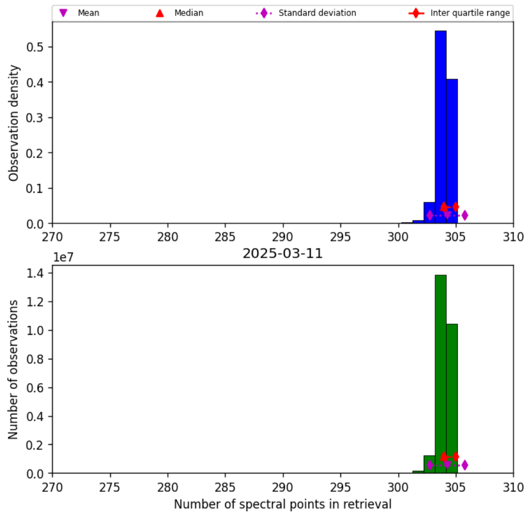
Figure 31: Histogram of “Number of spectral points in retrieval” for 2025-03-11 to 2025-03-12
