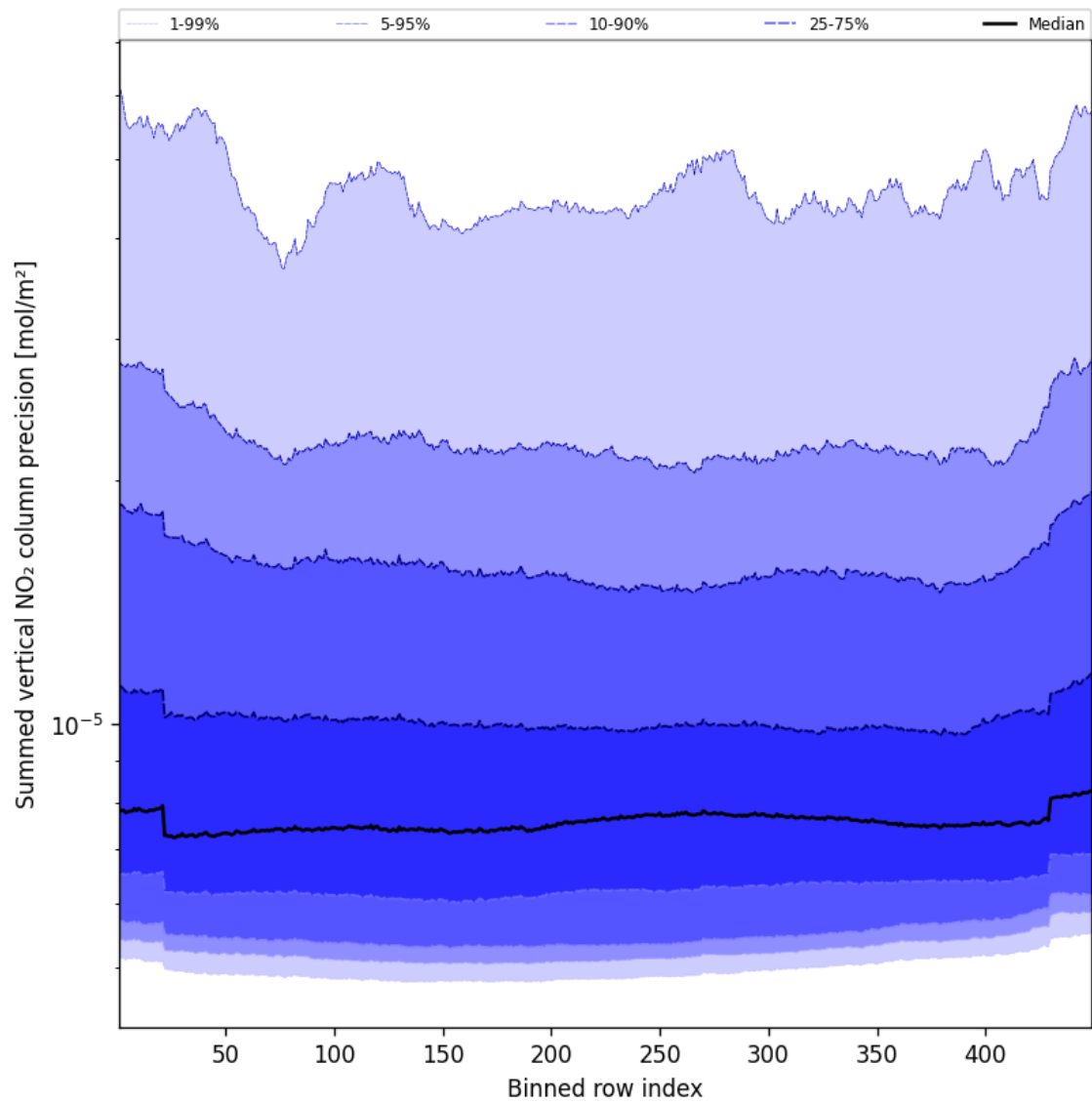
Figure 56: Along track statistics of “Summed vertical NO 2 column precision” for 2025-03-11 to 2025-03-12
