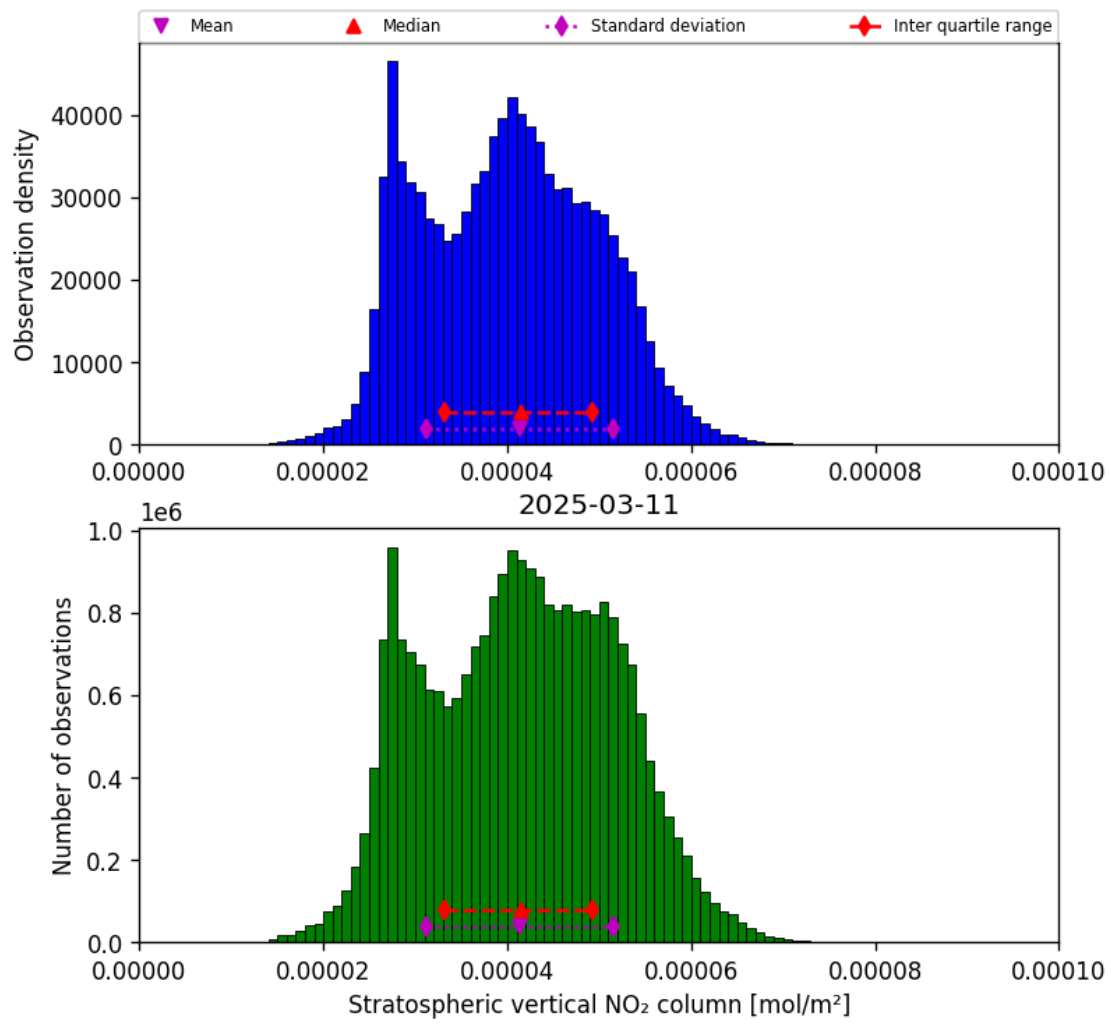
Figure 34: Histogram of “Stratospheric vertical NO 2 column” for 2025-03-11 to 2025-03-12
