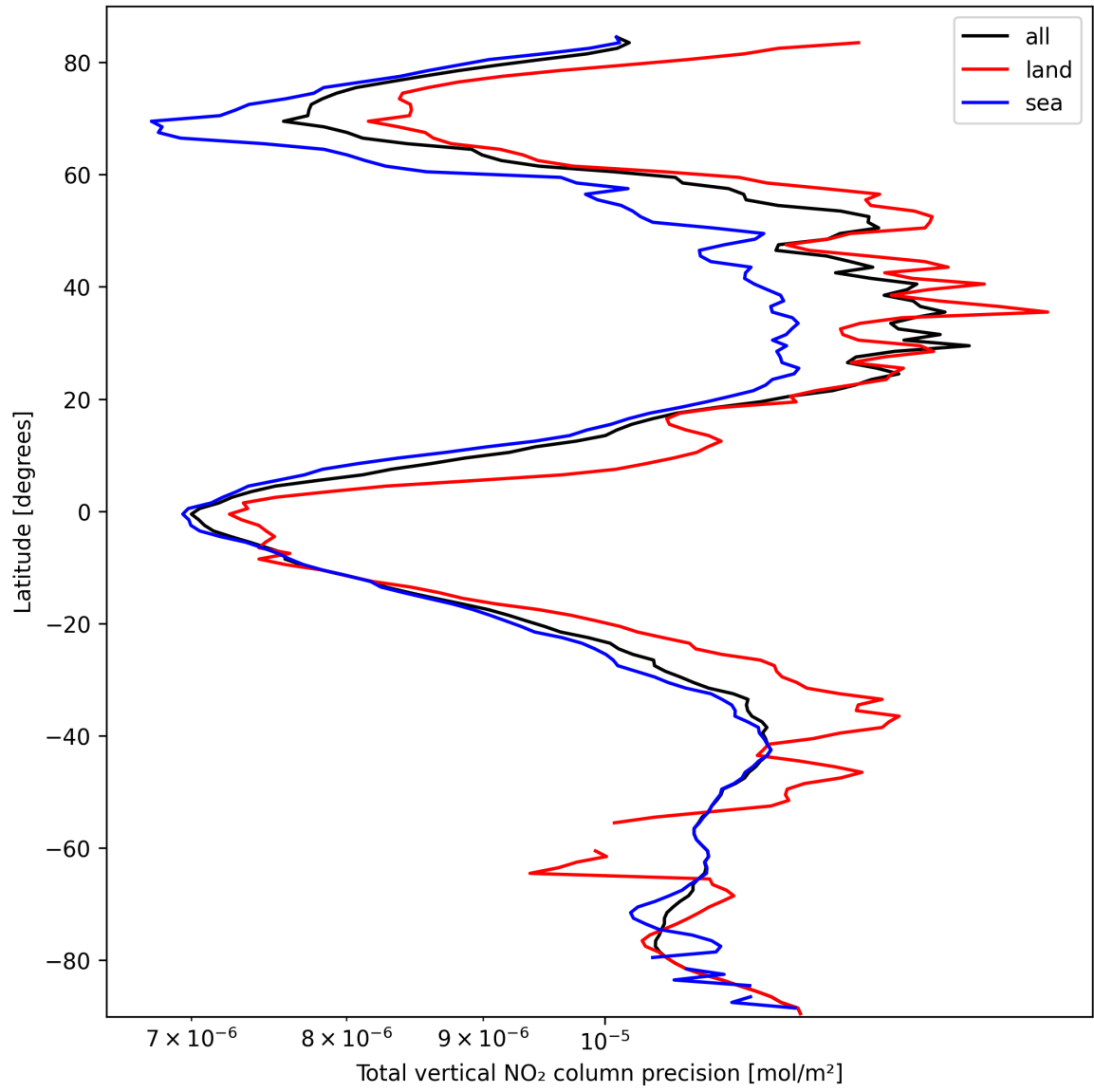
Figure 20: Zonal average of “Total vertical NO 2 column precision” for 2025-03-11 to 2025-03-12.
