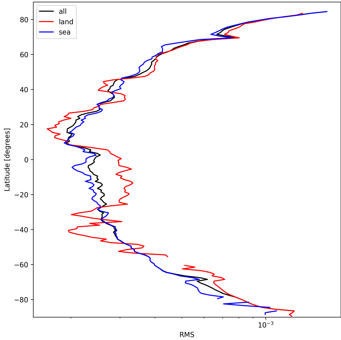
Figure 24: Zonal average of “RMS” for 2025-03-11 to 2025-03-12.
