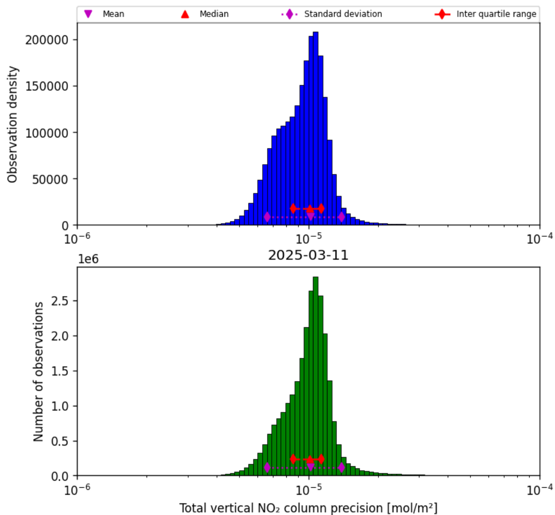
Figure 37: Histogram of “Total vertical NO 2 column precision” for 2025-03-11 to 2025-03-12
