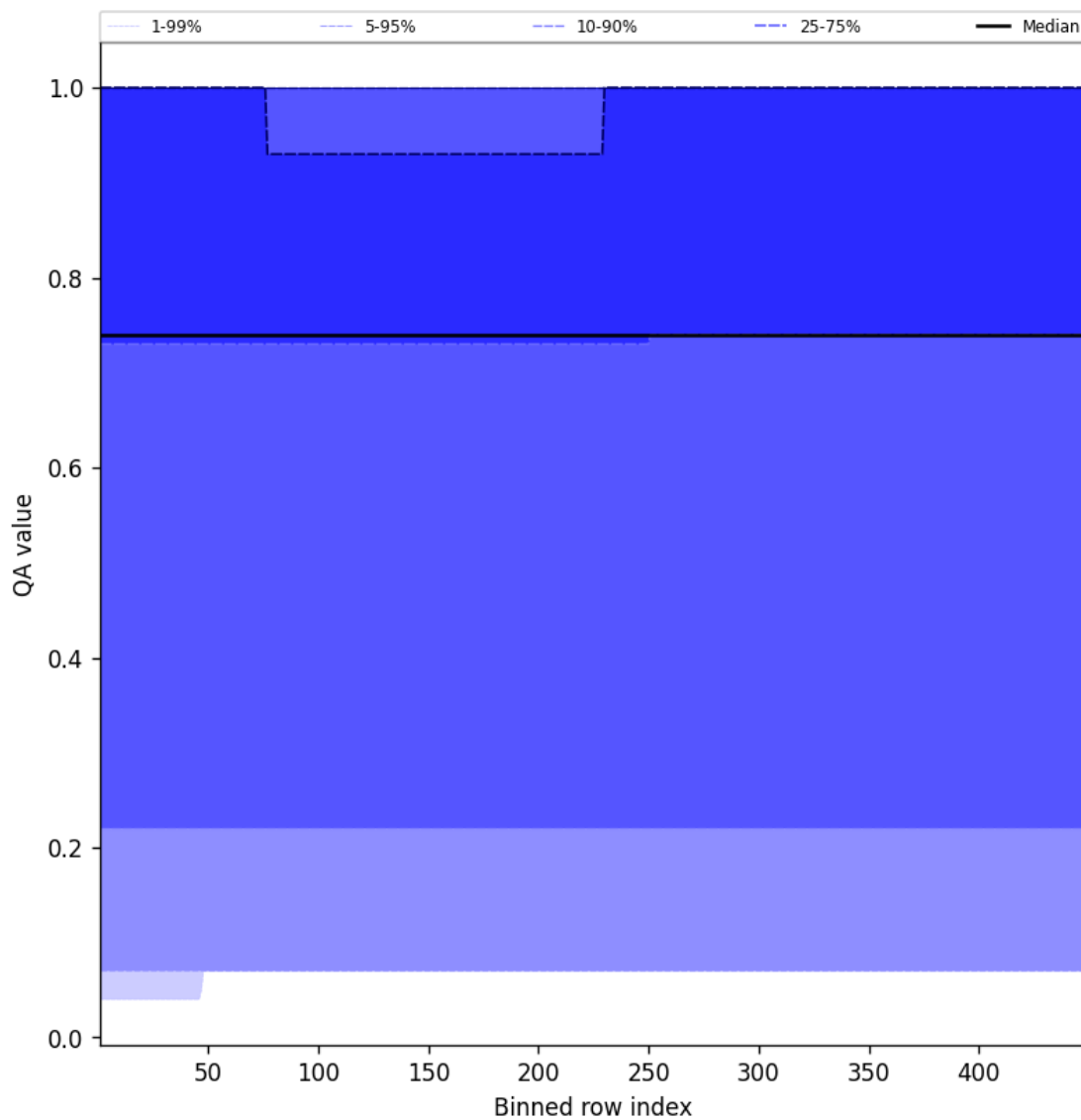
Figure 43: Along track statistics of “QA value” for 2025-03-11 to 2025-03-12
