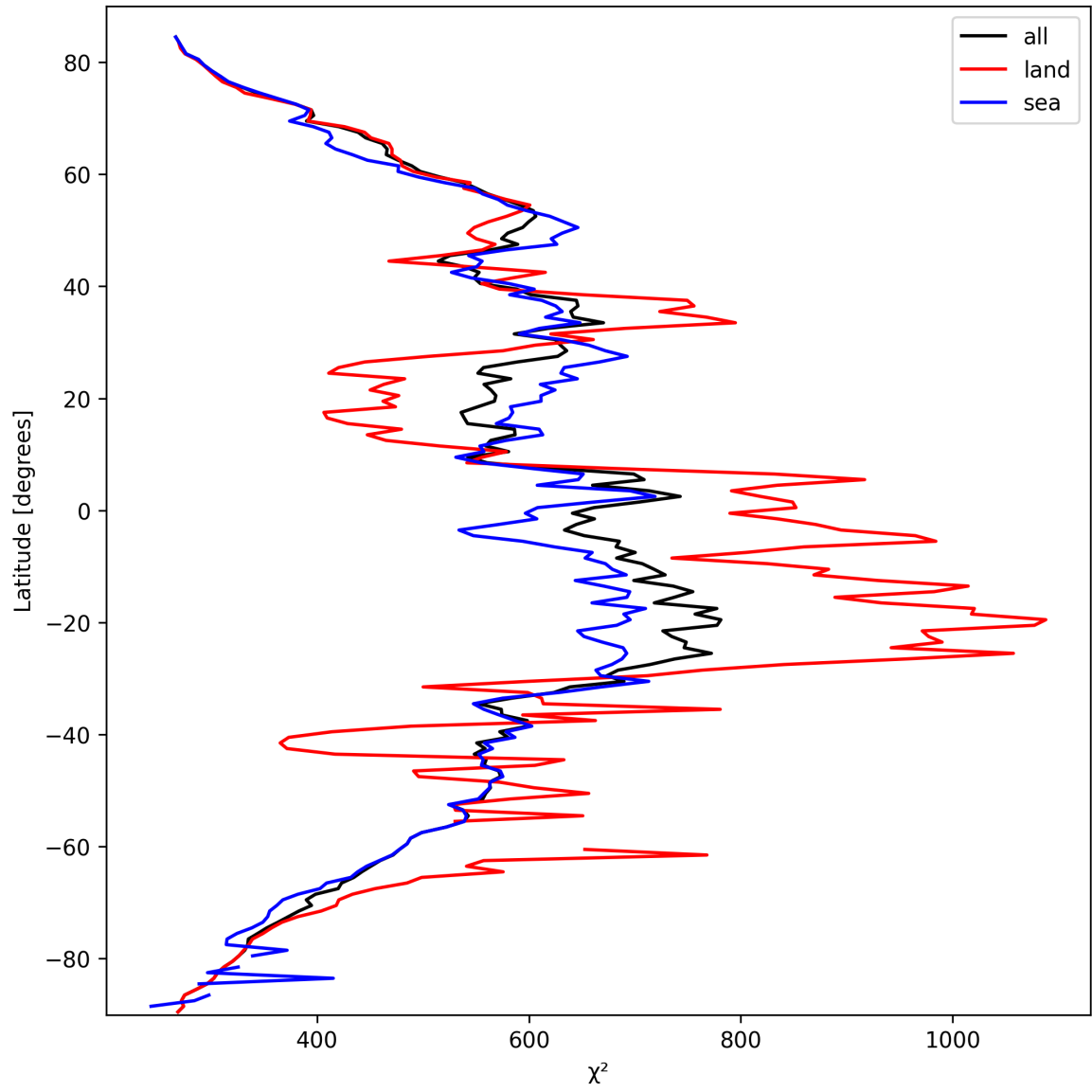
Figure 23: Zonal average of “ \chi^2 ” for 2025-03-11 to 2025-03-12.
