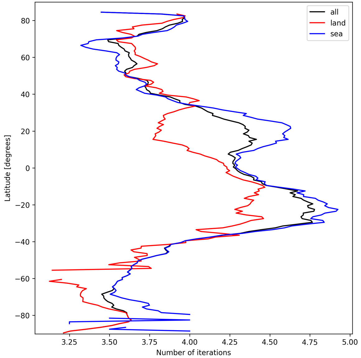
Figure 15: Zonal average of “Number of iterations” for 2025-03-11 to 2025-03-12.
