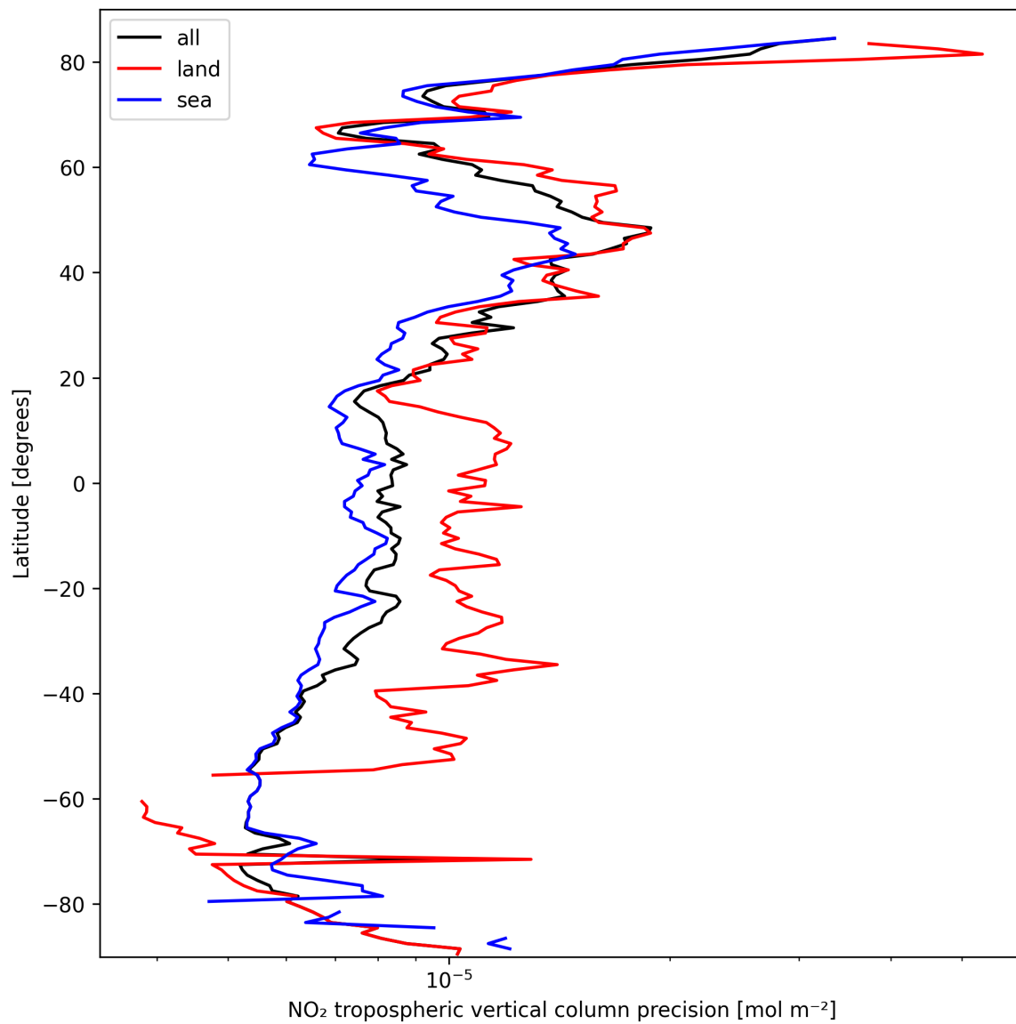
Figure 11: Zonal average of “NO 2 tropospheric vertical column precision” for 2025-03-11 to 2025-03-12.
