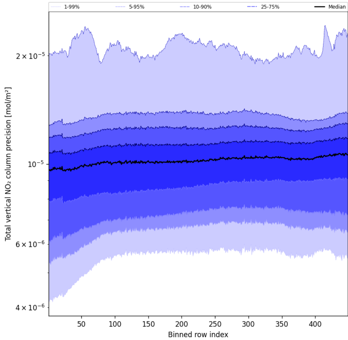
Figure 54: Along track statistics of “Total vertical NO 2 column precision” for 2025-03-11 to 2025-03-12
