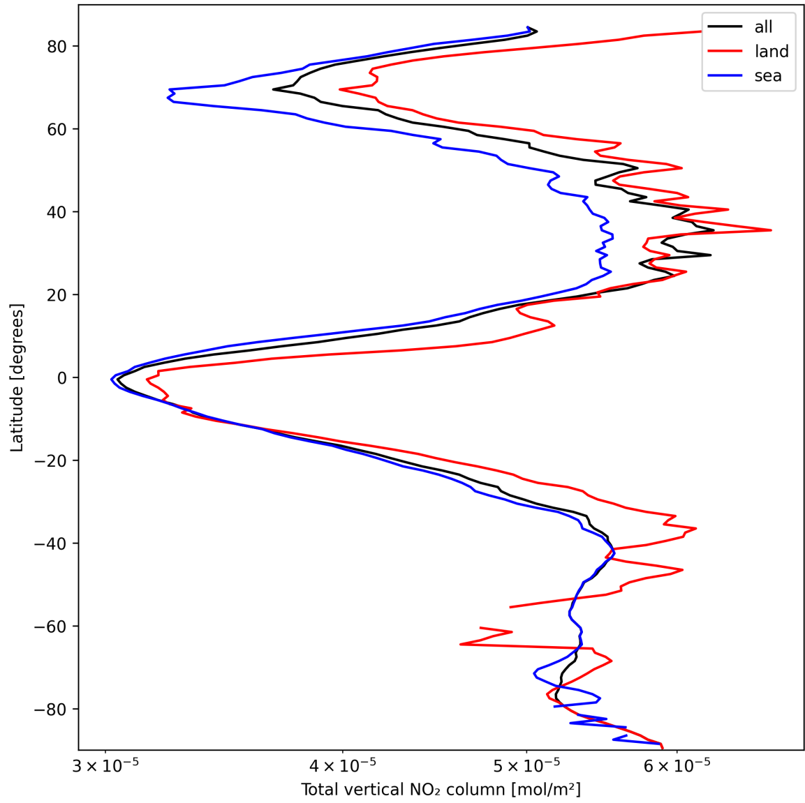
Figure 19: Zonal average of “Total vertical NO 2 column” for 2025-03-11 to 2025-03-12.
