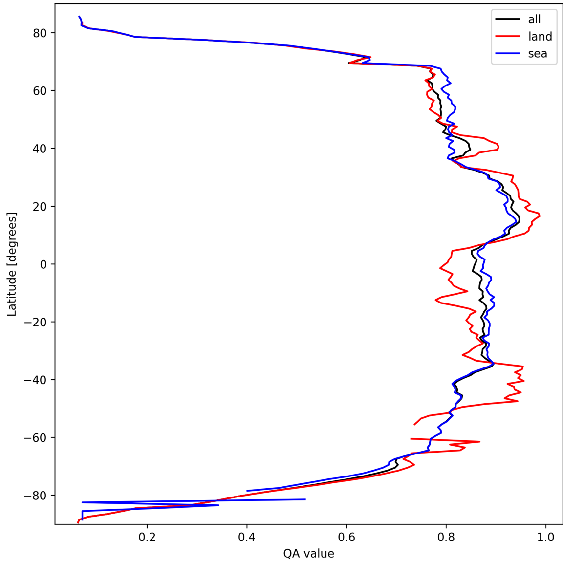
Figure 9: Zonal average of “QA value” for 2025-03-12 to 2025-03-13.
