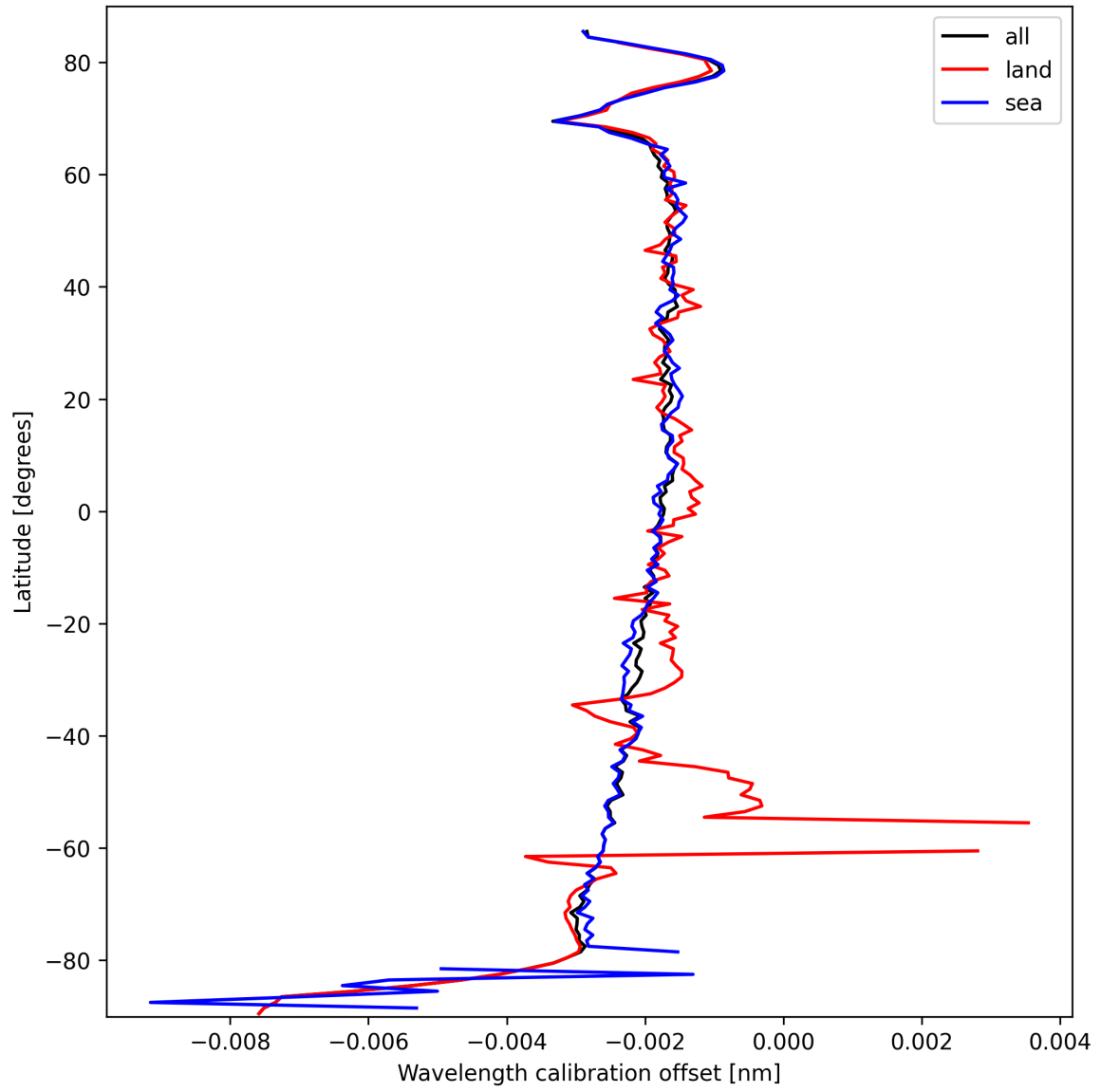
Figure 16: Zonal average of “Wavelength calibration offset” for 2025-03-12 to 2025-03-13.
