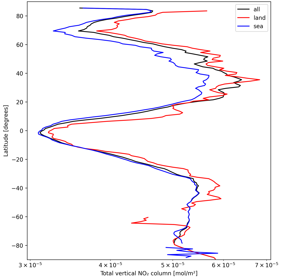
Figure 19: Zonal average of “Total vertical NO 2 column” for 2025-03-12 to 2025-03-13.
