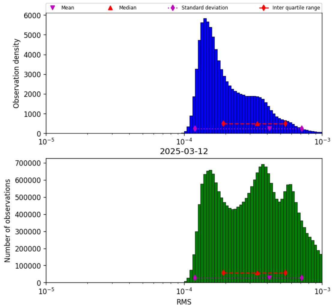
Figure 41: Histogram of “RMS” for 2025-03-12 to 2025-03-13
