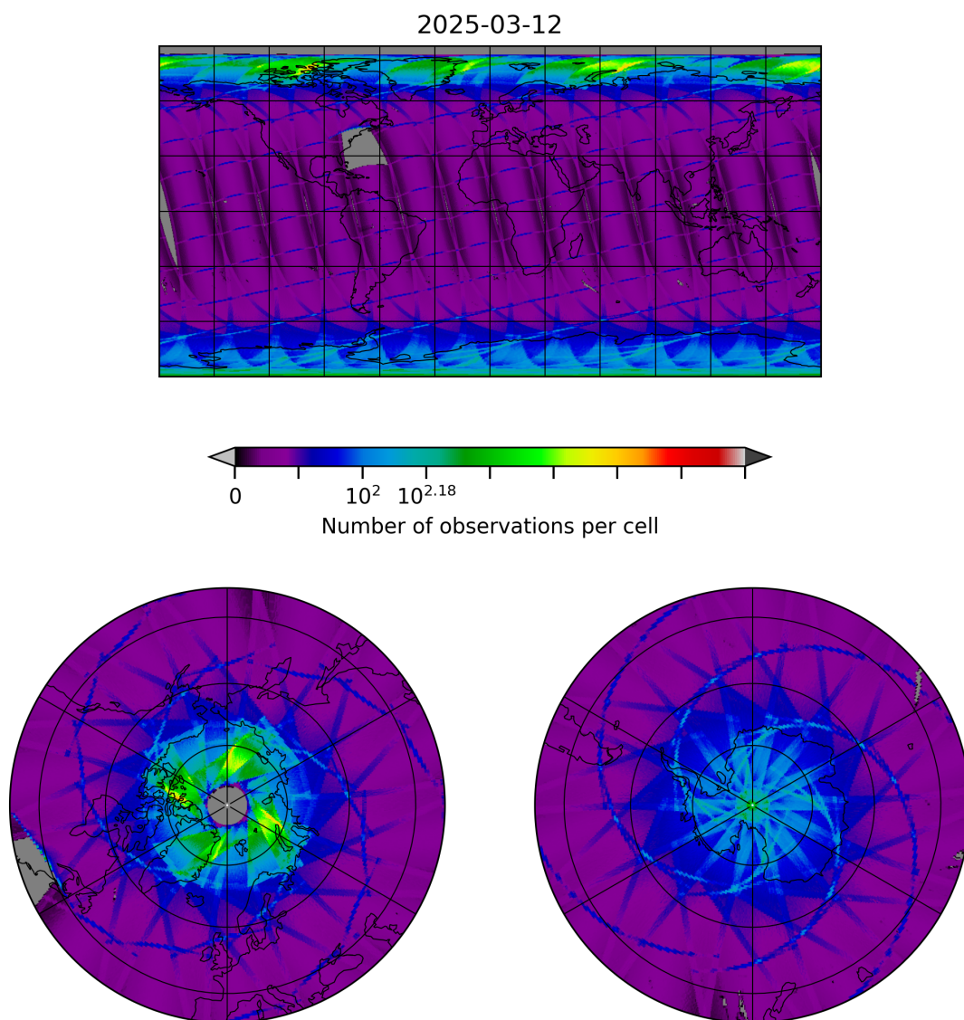
Figure 8: Map of the number of observations for 2025-03-12 to 2025-03-13
