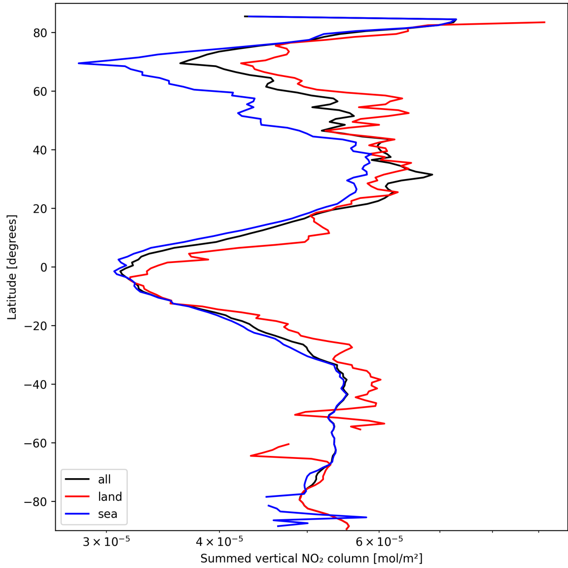
Figure 21: Zonal average of “Summed vertical NO 2 column” for 2025-03-12 to 2025-03-13.
