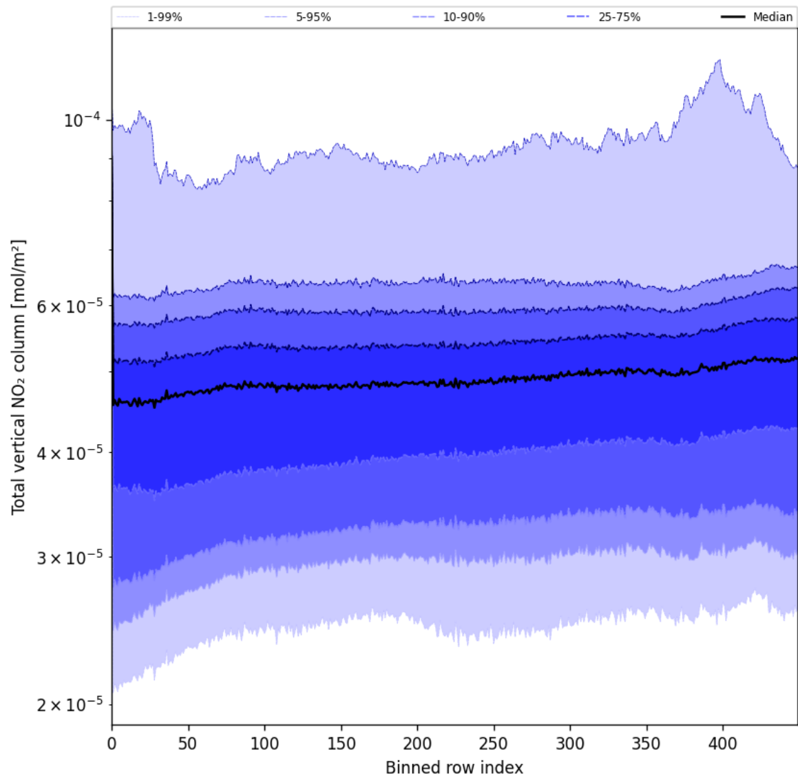
Figure 53: Along track statistics of “Total vertical NO 2 column” for 2025-03-12 to 2025-03-13
