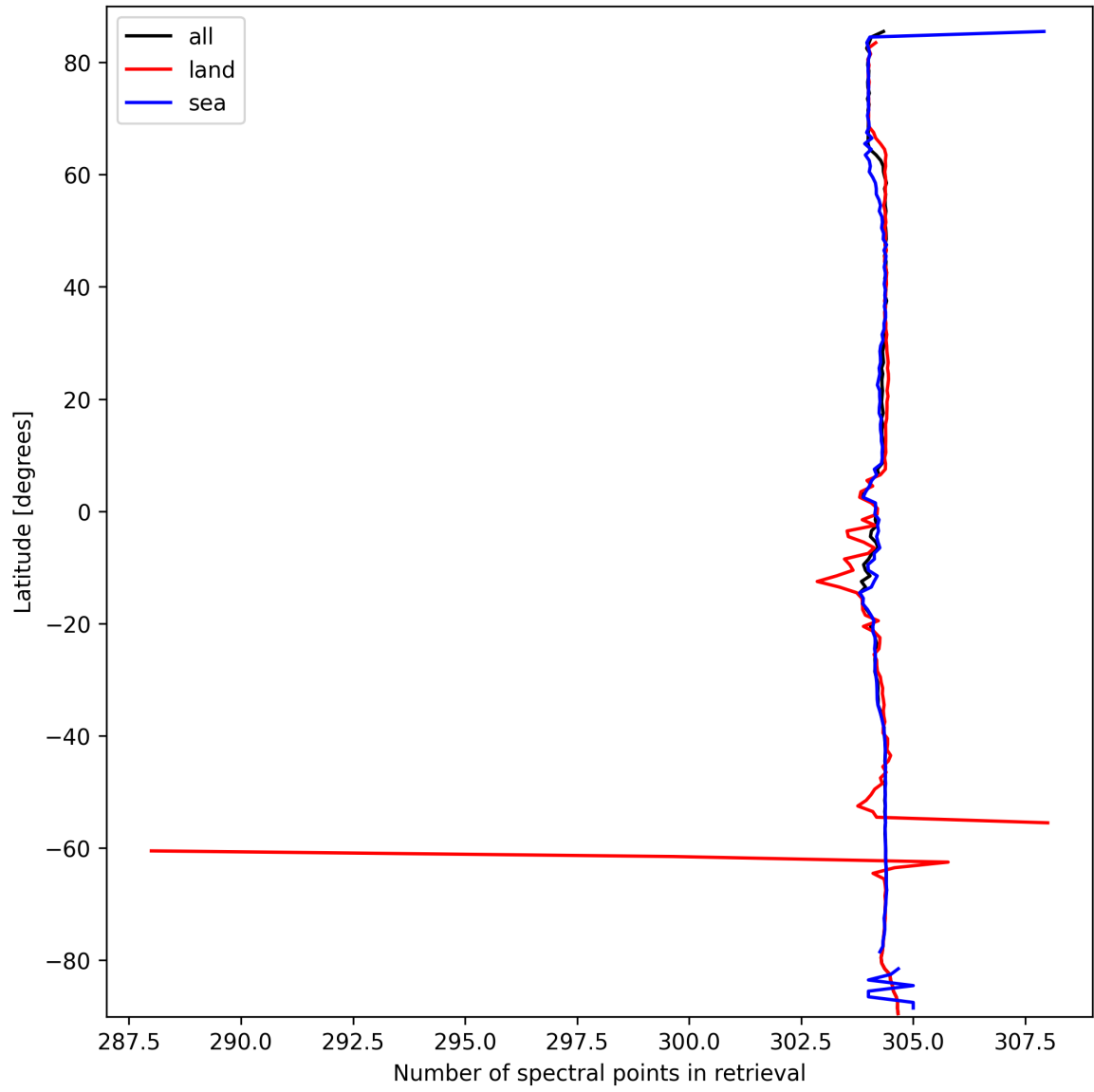
Figure 14: Zonal average of “Number of spectral points in retrieval” for 2025-03-12 to 2025-03-13.
