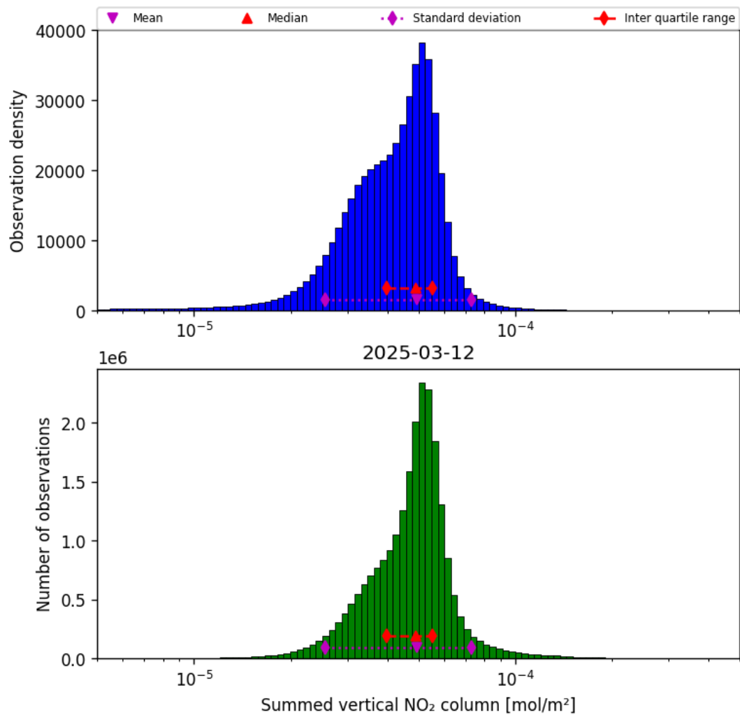
Figure 38: Histogram of “Summed vertical NO 2 column” for 2025-03-12 to 2025-03-13
