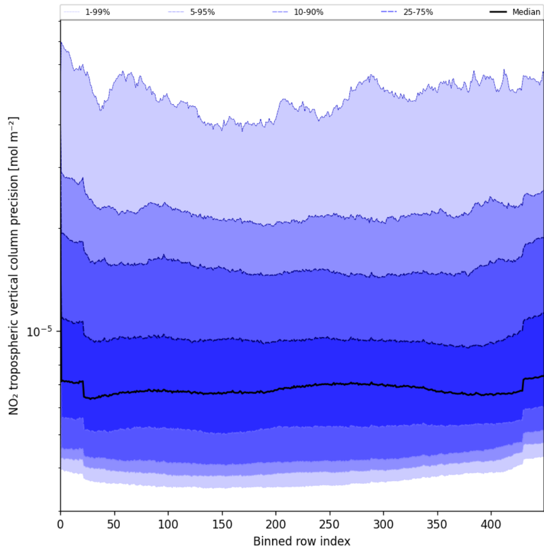
Figure 45: Along track statistics of “NO 2 tropospheric vertical column precision” for 2025-03-12 to 2025-03-13
