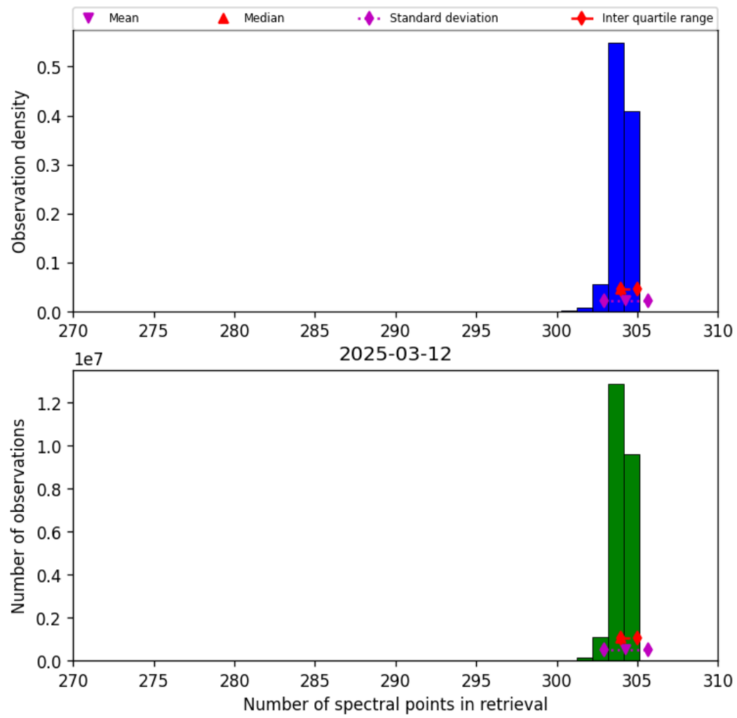
Figure 31: Histogram of “Number of spectral points in retrieval” for 2025-03-12 to 2025-03-13
