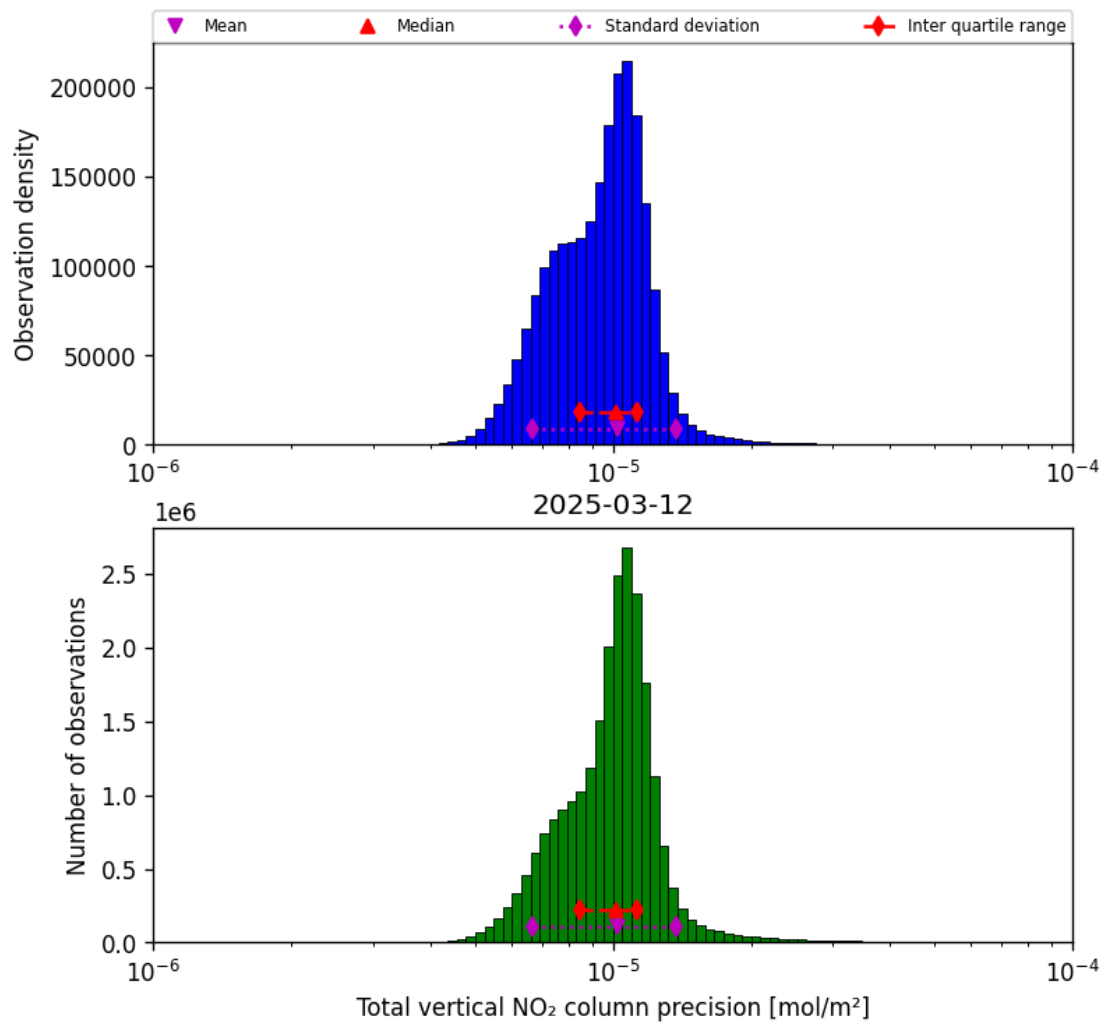
Figure 37: Histogram of “Total vertical NO 2 column precision” for 2025-03-12 to 2025-03-13
