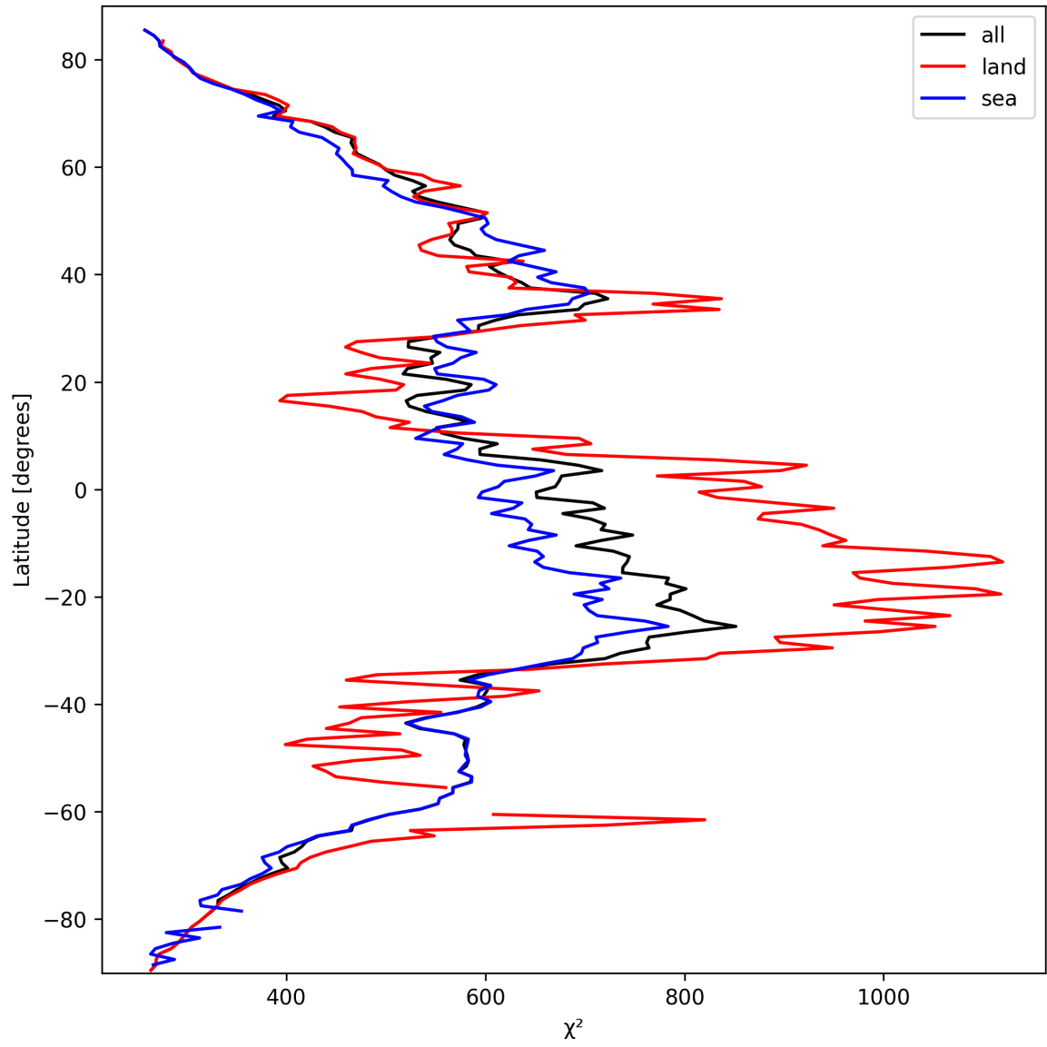
Figure 23: Zonal average of “ \chi^2 ” for 2025-03-12 to 2025-03-13.
