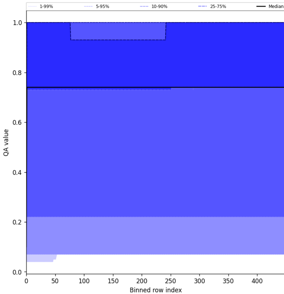
Figure 43: Along track statistics of “QA value” for 2025-03-12 to 2025-03-13
