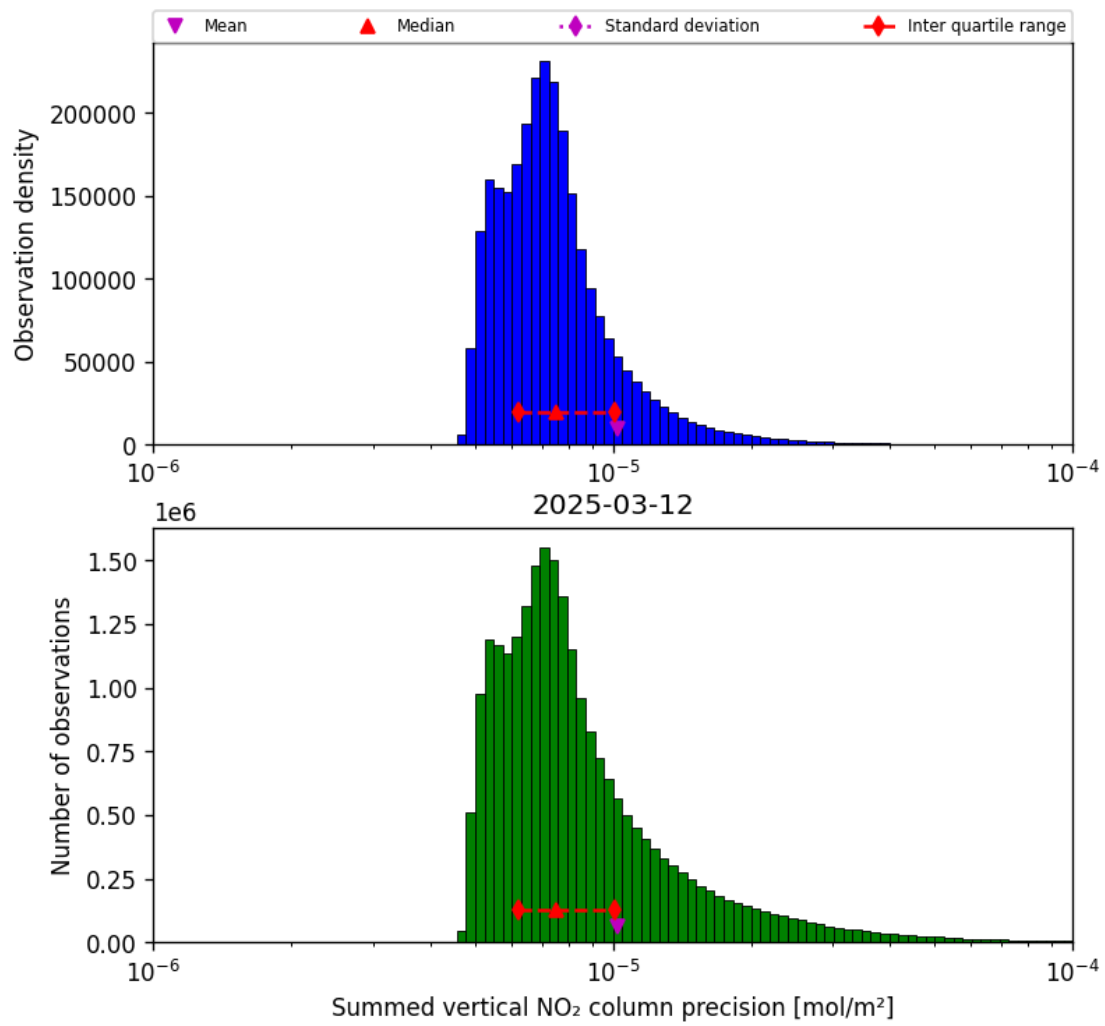
Figure 39: Histogram of “Summed vertical NO 2 column precision” for 2025-03-12 to 2025-03-13
