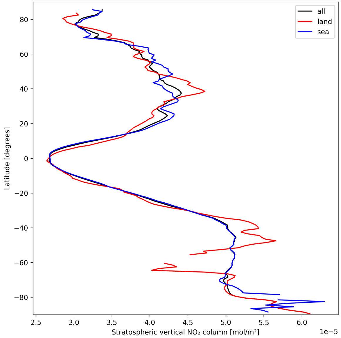
Figure 17: Zonal average of “Stratospheric vertical NO 2 column” for 2025-03-12 to 2025-03-13.
