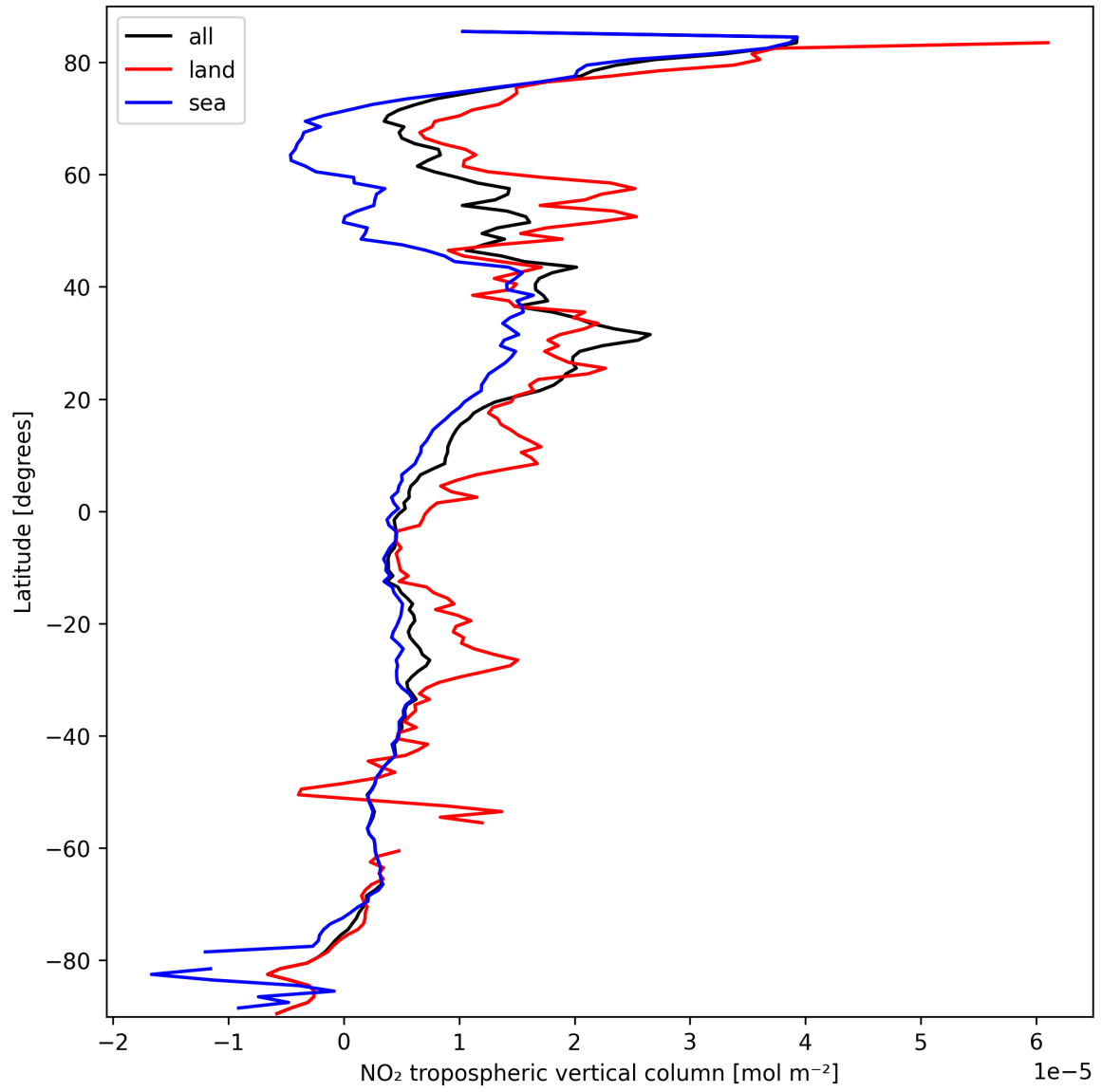
Figure 10: Zonal average of “NO 2 tropospheric vertical column” for 2025-03-12 to 2025-03-13.
