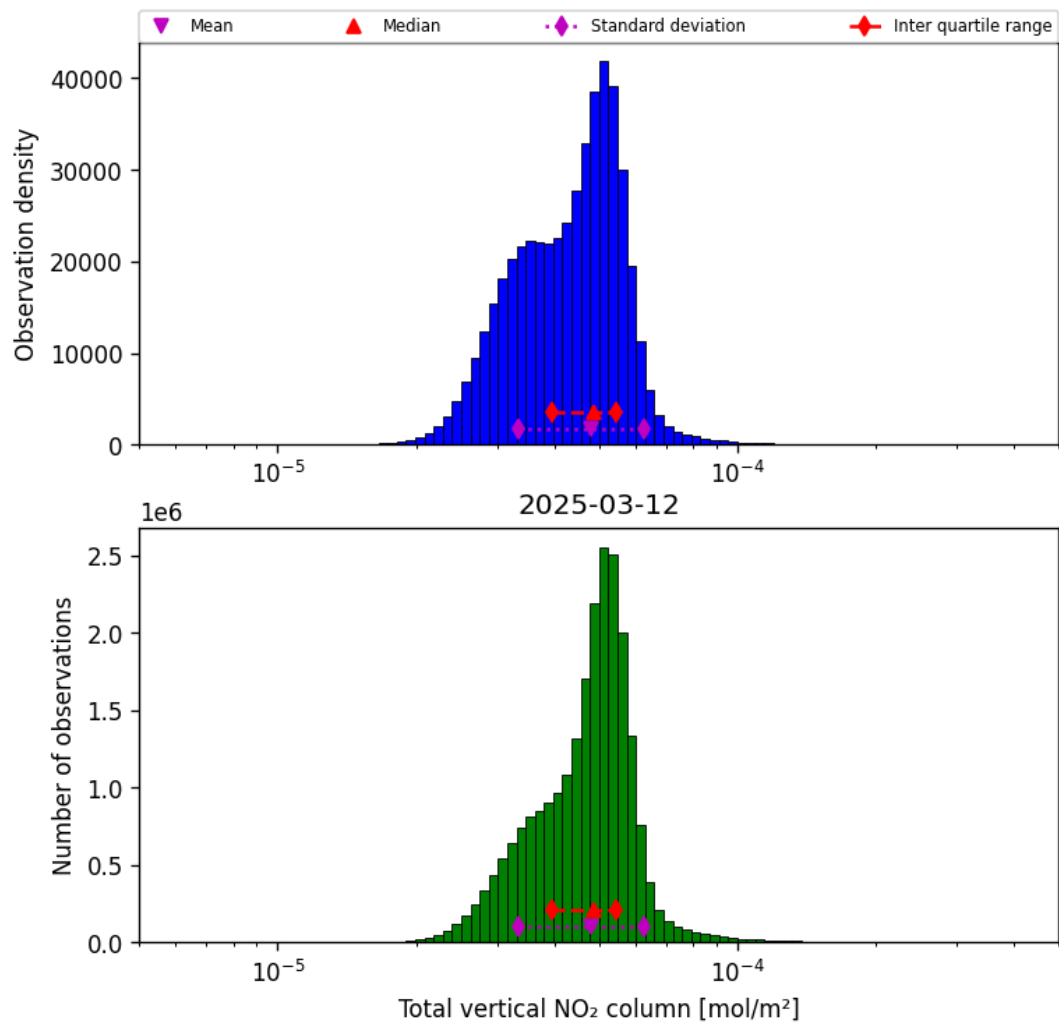
Figure 36: Histogram of “Total vertical NO 2 column” for 2025-03-12 to 2025-03-13
