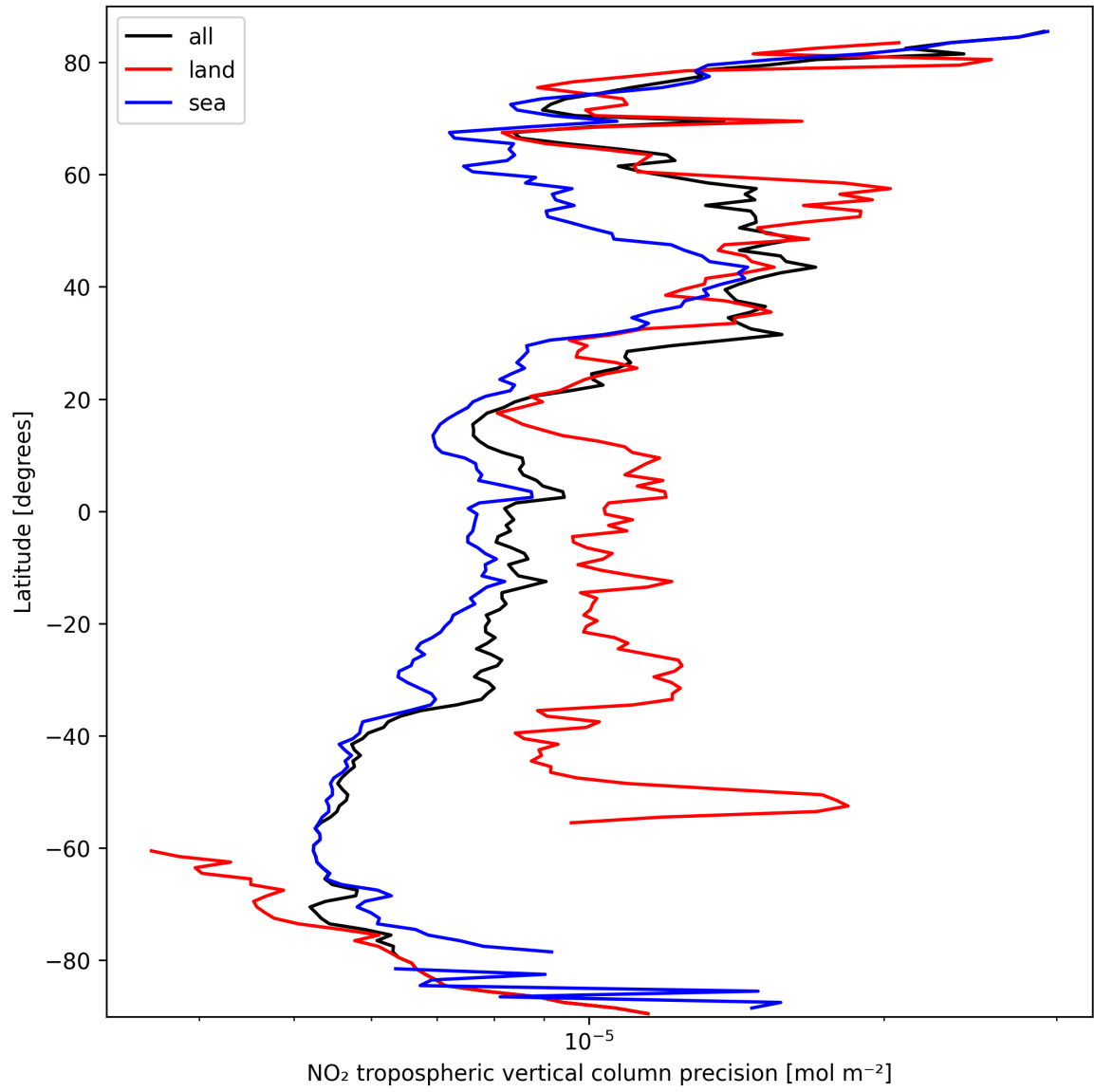
Figure 11: Zonal average of “NO 2 tropospheric vertical column precision” for 2025-03-12 to 2025-03-13.
