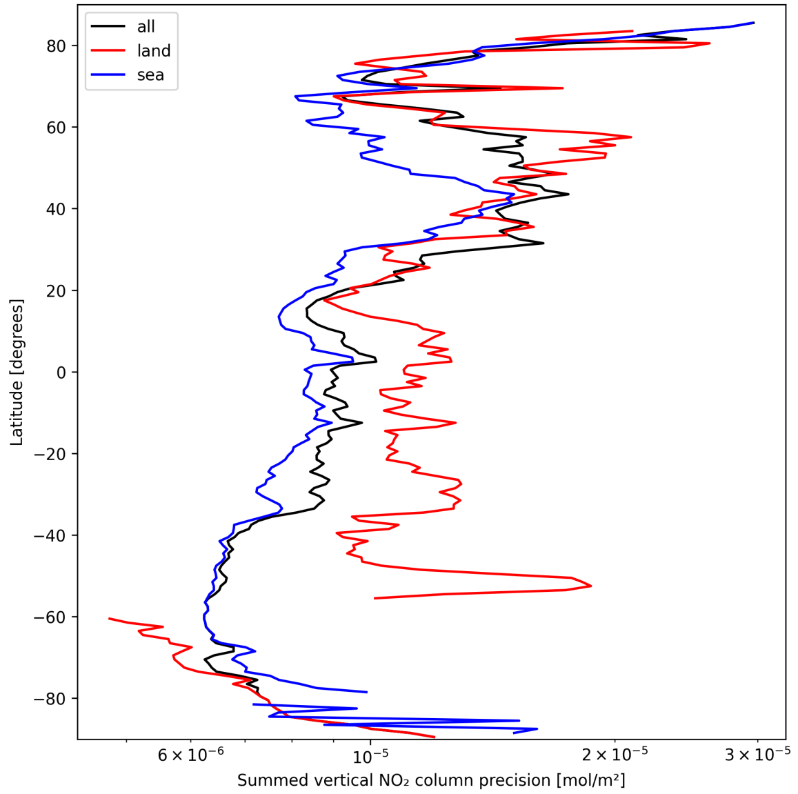
Figure 22: Zonal average of “Summed vertical NO 2 column precision” for 2025-03-12 to 2025-03-13.
