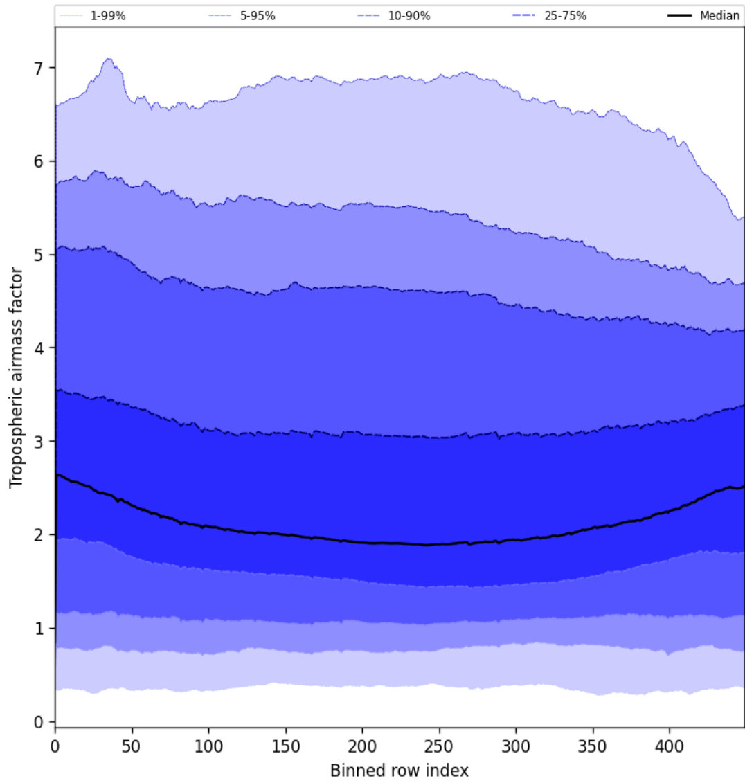
Figure 46: Along track statistics of “Tropospheric air mass factor” for 2025-03-12 to 2025-03-13
