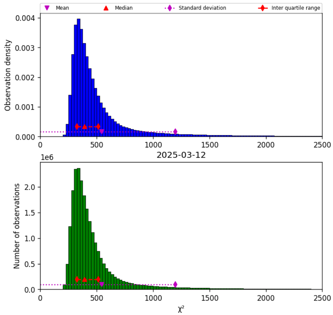
Figure 40: Histogram of “ \chi^2 ” for 2025-03-12 to 2025-03-13
