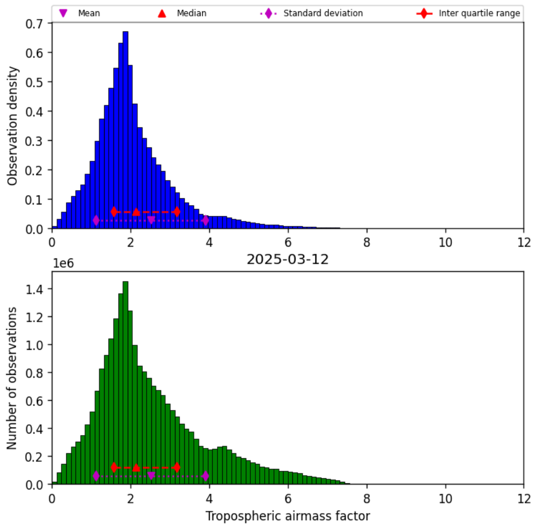
Figure 29: Histogram of “Tropospheric airmass factor” for 2025-03-12 to 2025-03-13
