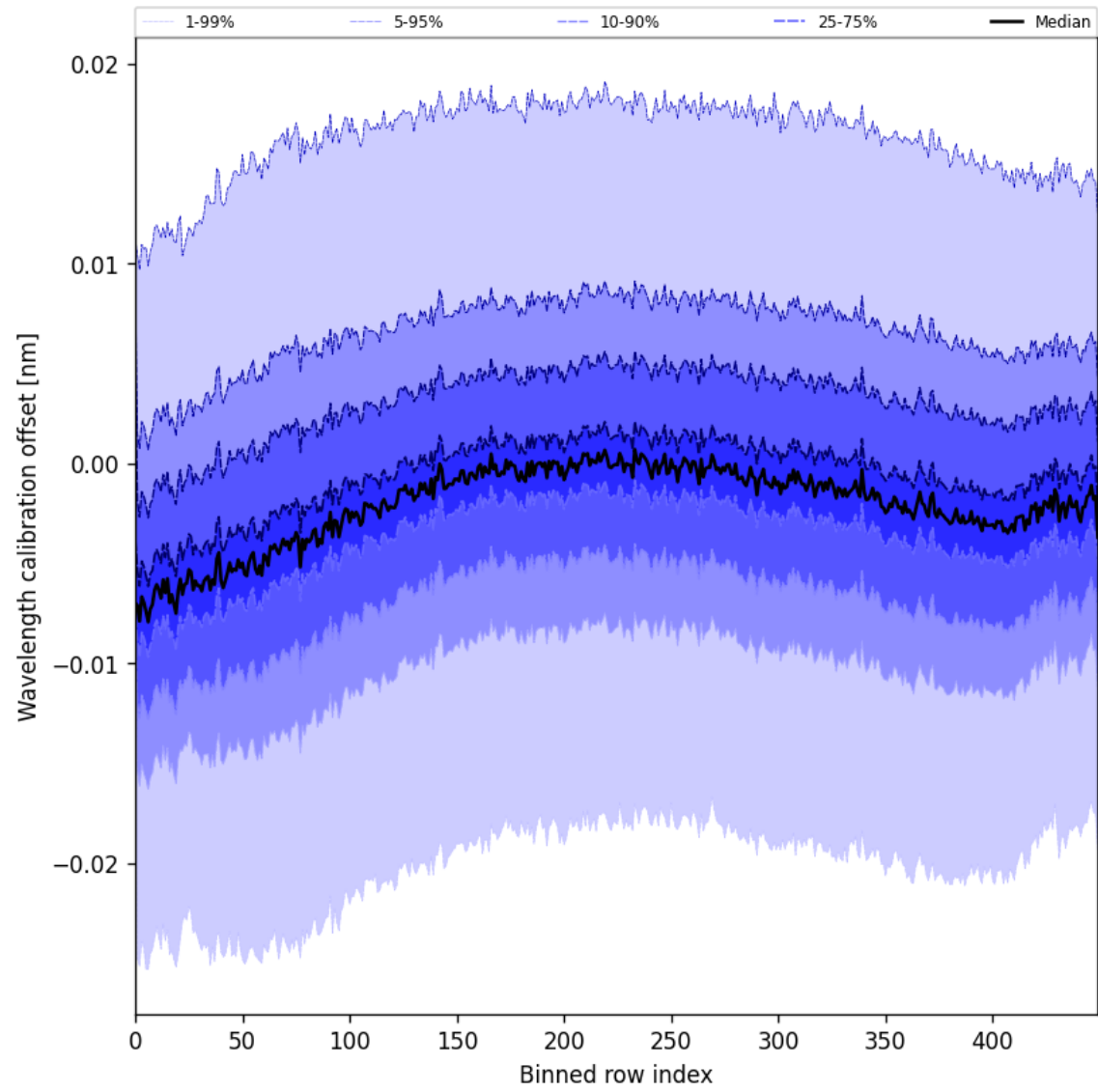
Figure 50: Along track statistics of “Wavelength calibration offset” for 2025-03-12 to 2025-03-13
