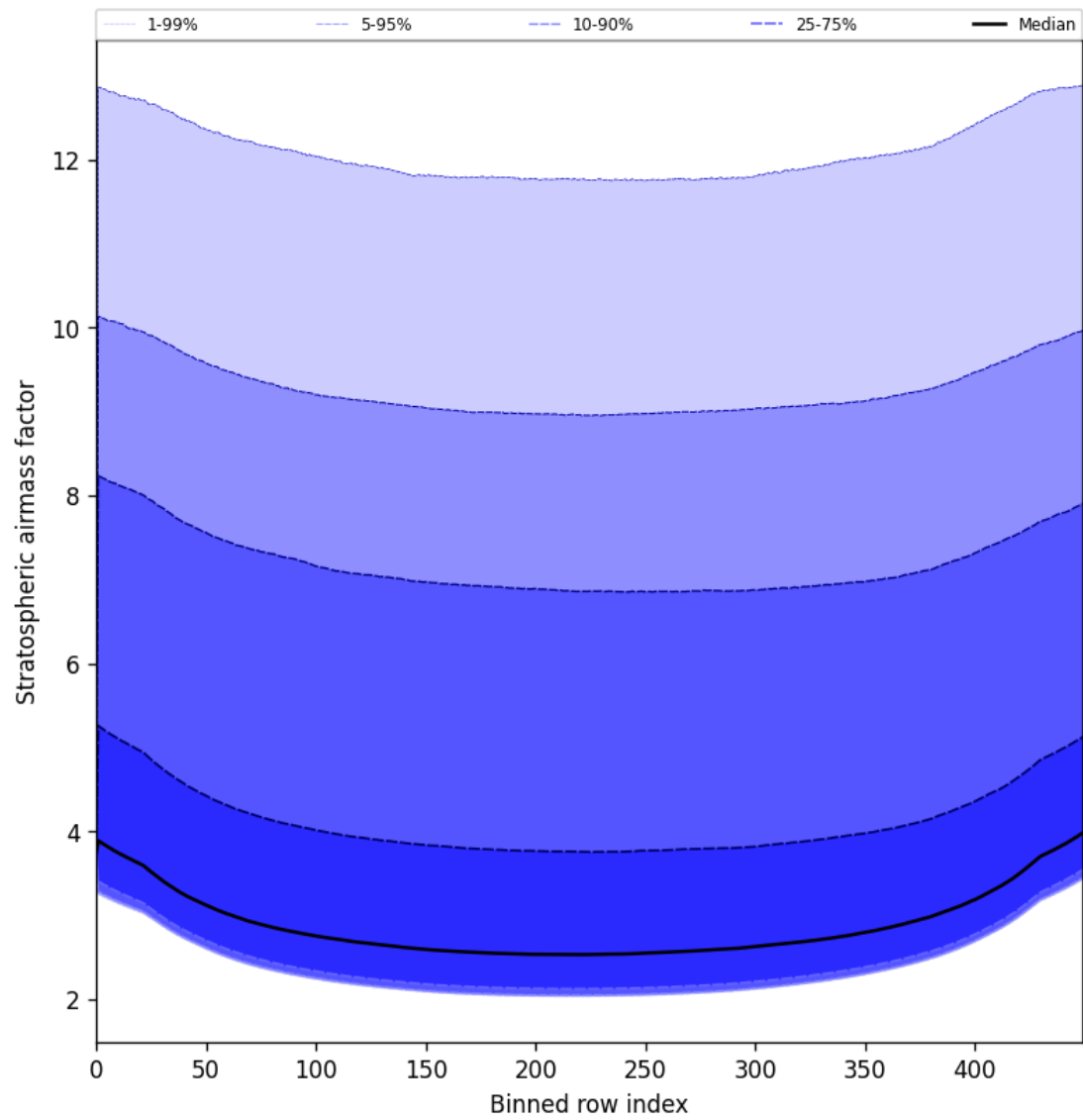
Figure 59: Along track statistics of “Stratospheric airmass factor” for 2025-03-12 to 2025-03-13
