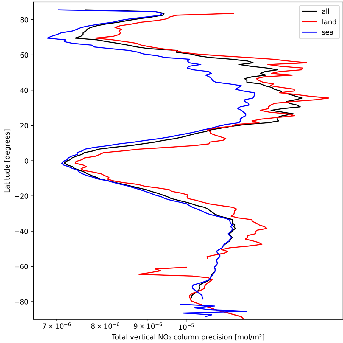
Figure 20: Zonal average of “Total vertical NO 2 column precision” for 2025-03-12 to 2025-03-13.
