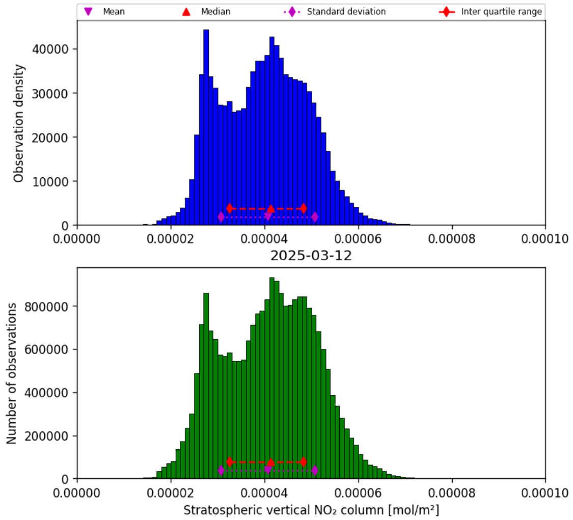
Figure 34: Histogram of “Stratospheric vertical NO 2 column” for 2025-03-12 to 2025-03-13
