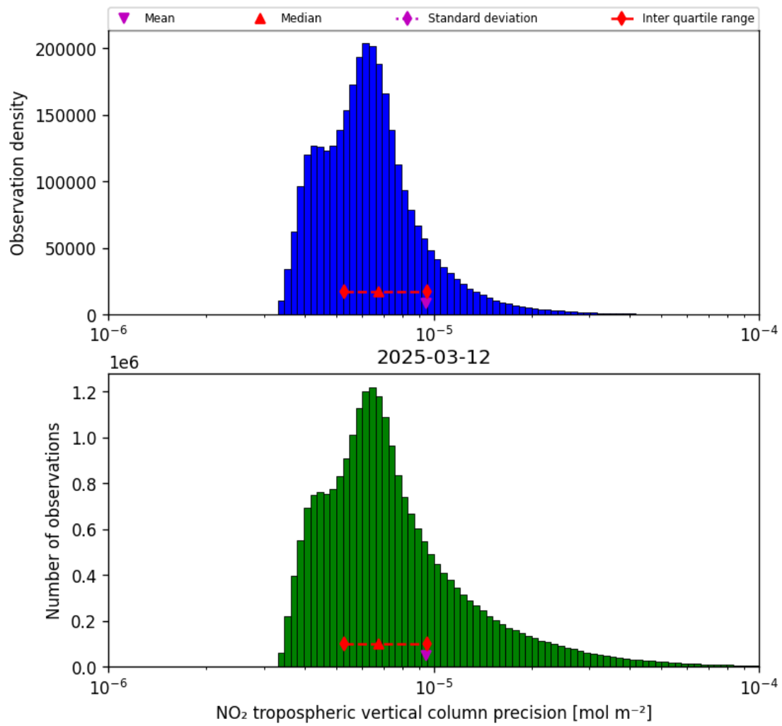
Figure 28: Histogram of “NO 2 tropospheric vertical column precision” for 2025-03-12 to 2025-03-13
