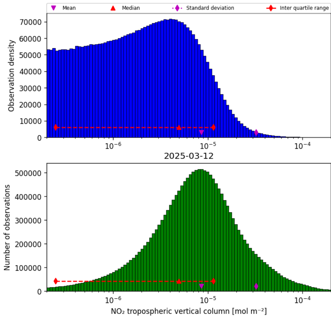
Figure 27: Histogram of “NO 2 tropospheric vertical column” for 2025-03-12 to 2025-03-13
