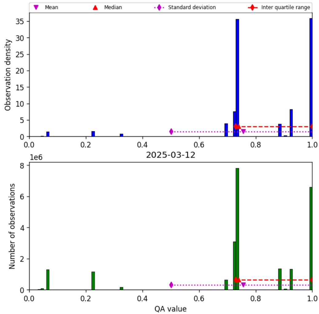
Figure 26: Histogram of “QA value” for 2025-03-12 to 2025-03-13
