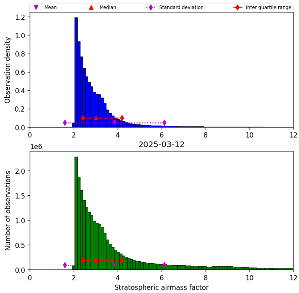
Figure 42: Histogram of “Stratospheric airmass factor” for 2025-03-12 to 2025-03-13
