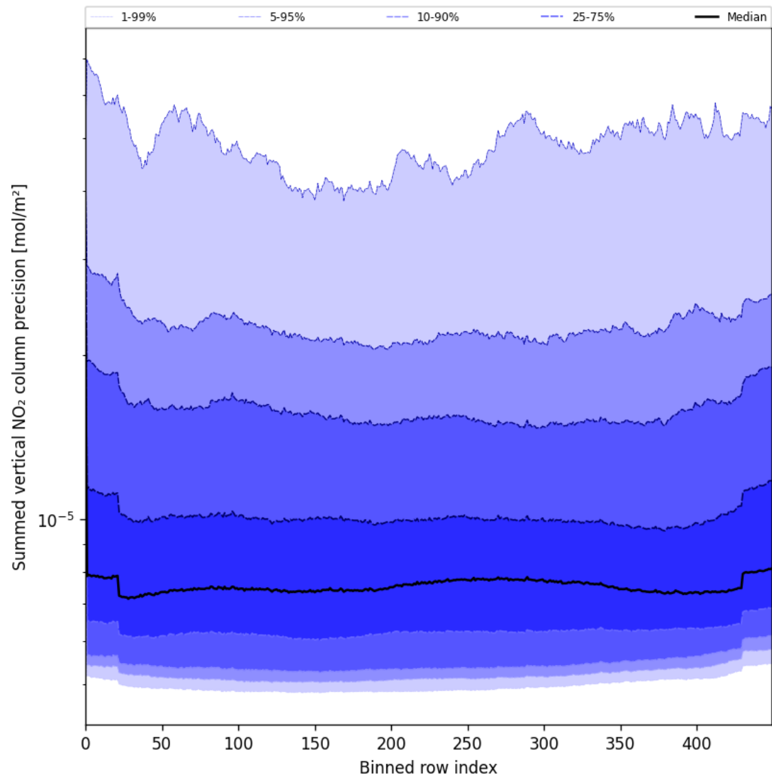
Figure 56: Along track statistics of “Summed vertical NO 2 column precision” for 2025-03-12 to 2025-03-13
