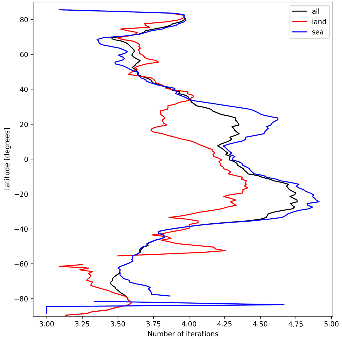
Figure 15: Zonal average of “Number of iterations” for 2025-03-12 to 2025-03-13.
