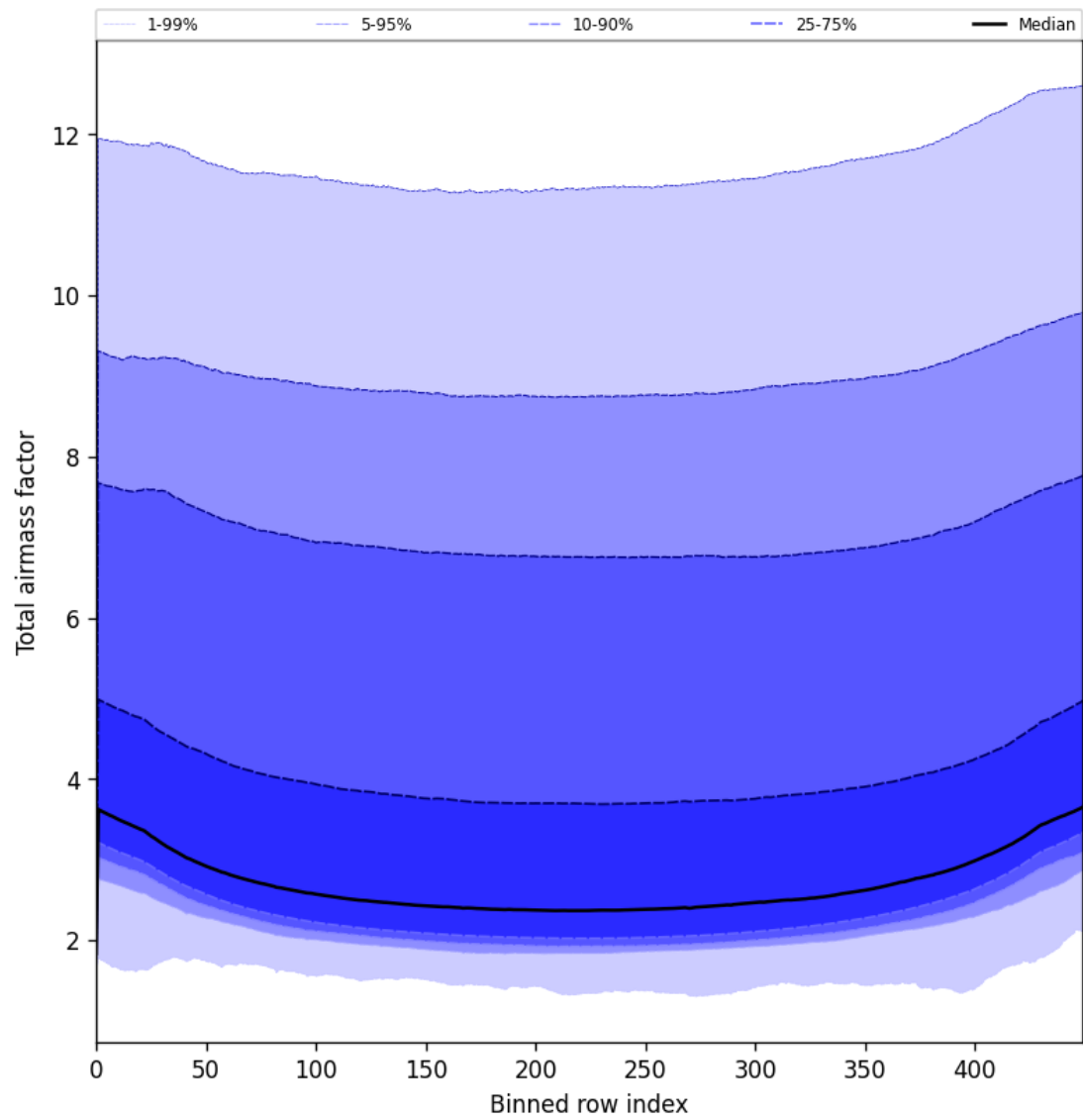
Figure 47: Along track statistics of “Total airmass factor” for 2025-03-12 to 2025-03-13
