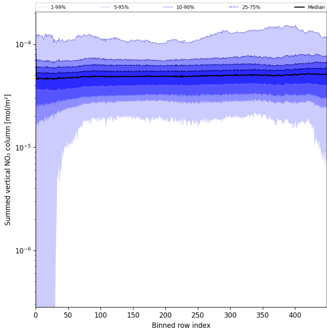
Figure 55: Along track statistics of “Summed vertical NO 2 column” for 2025-03-12 to 2025-03-13
