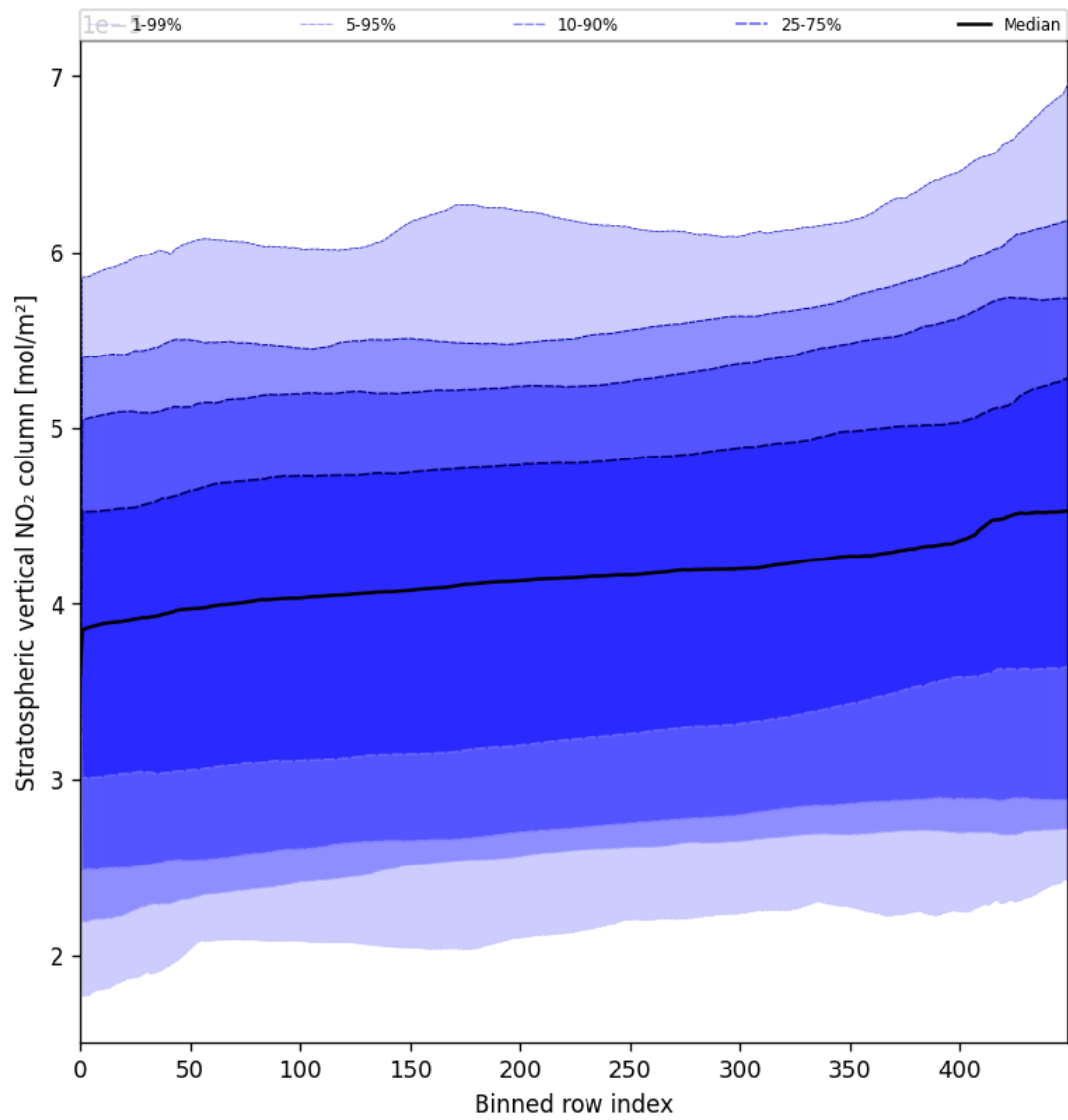
Figure 51: Along track statistics of “Stratospheric vertical NO 2 column” for 2025-03-12 to 2025-03-13
