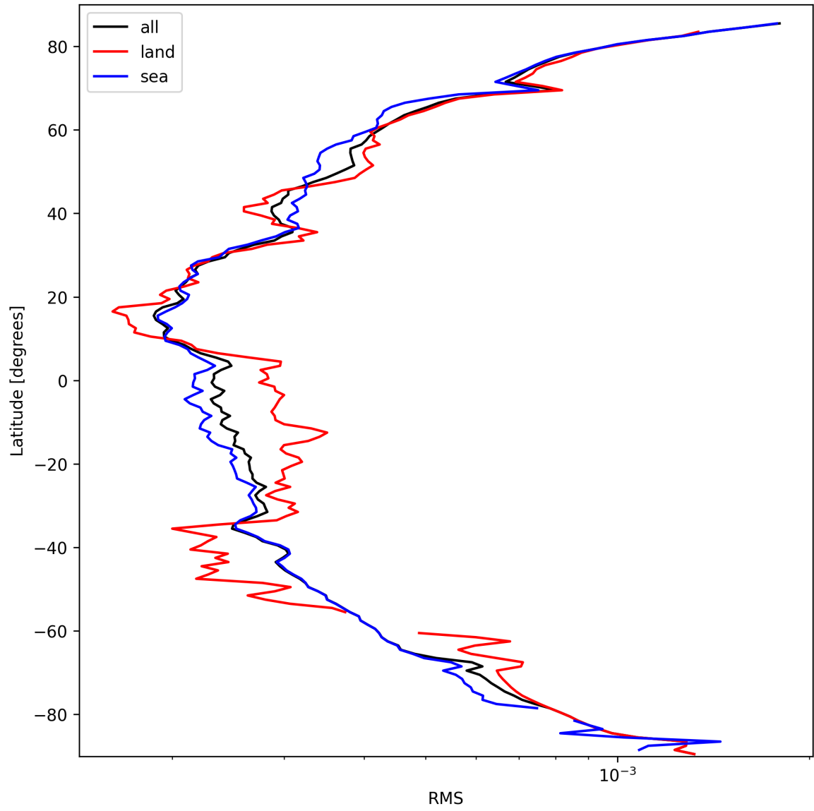
Figure 24: Zonal average of “RMS” for 2025-03-12 to 2025-03-13.
