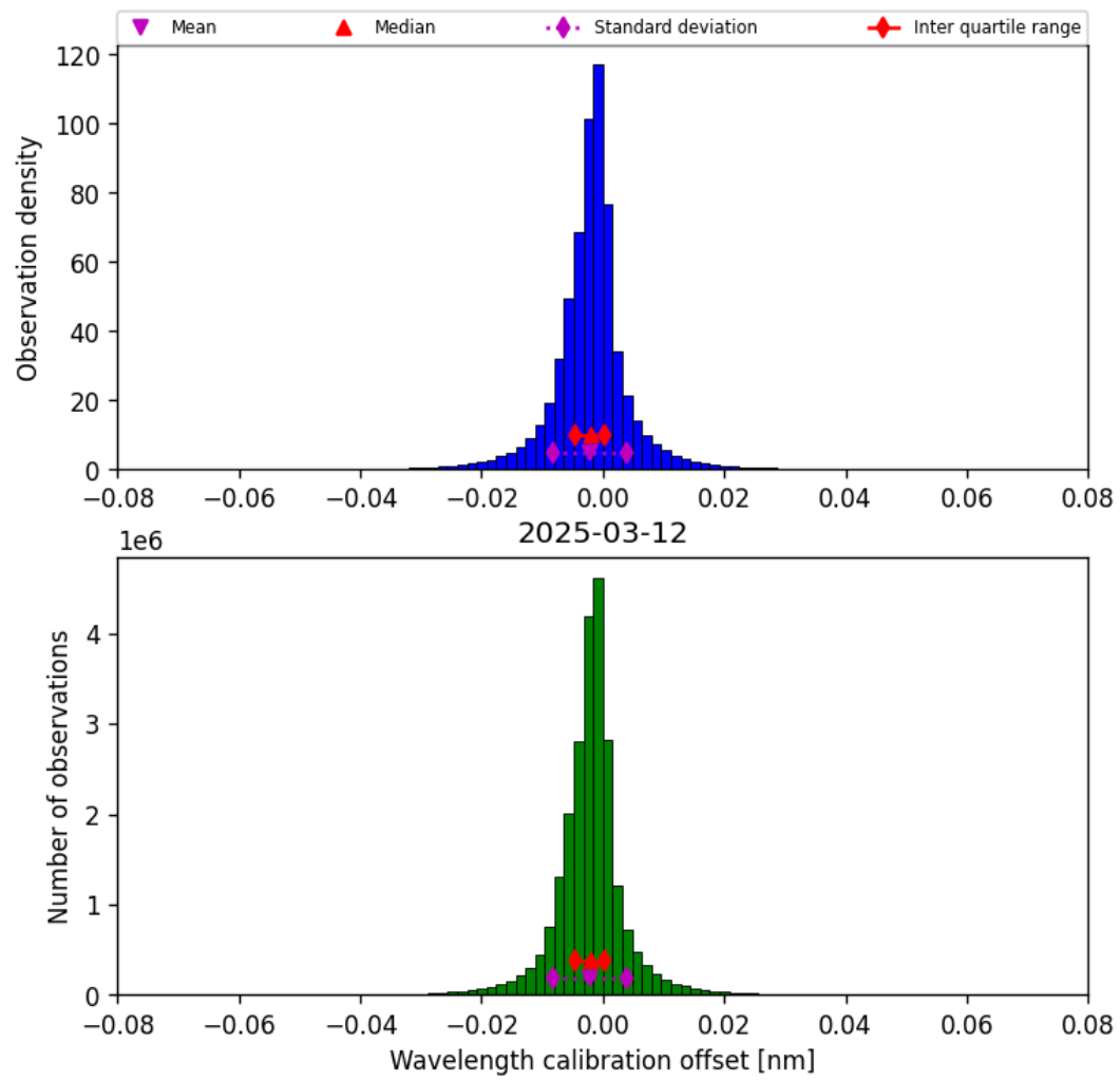
Figure 33: Histogram of “Wavelength calibration offset” for 2025-03-12 to 2025-03-13
