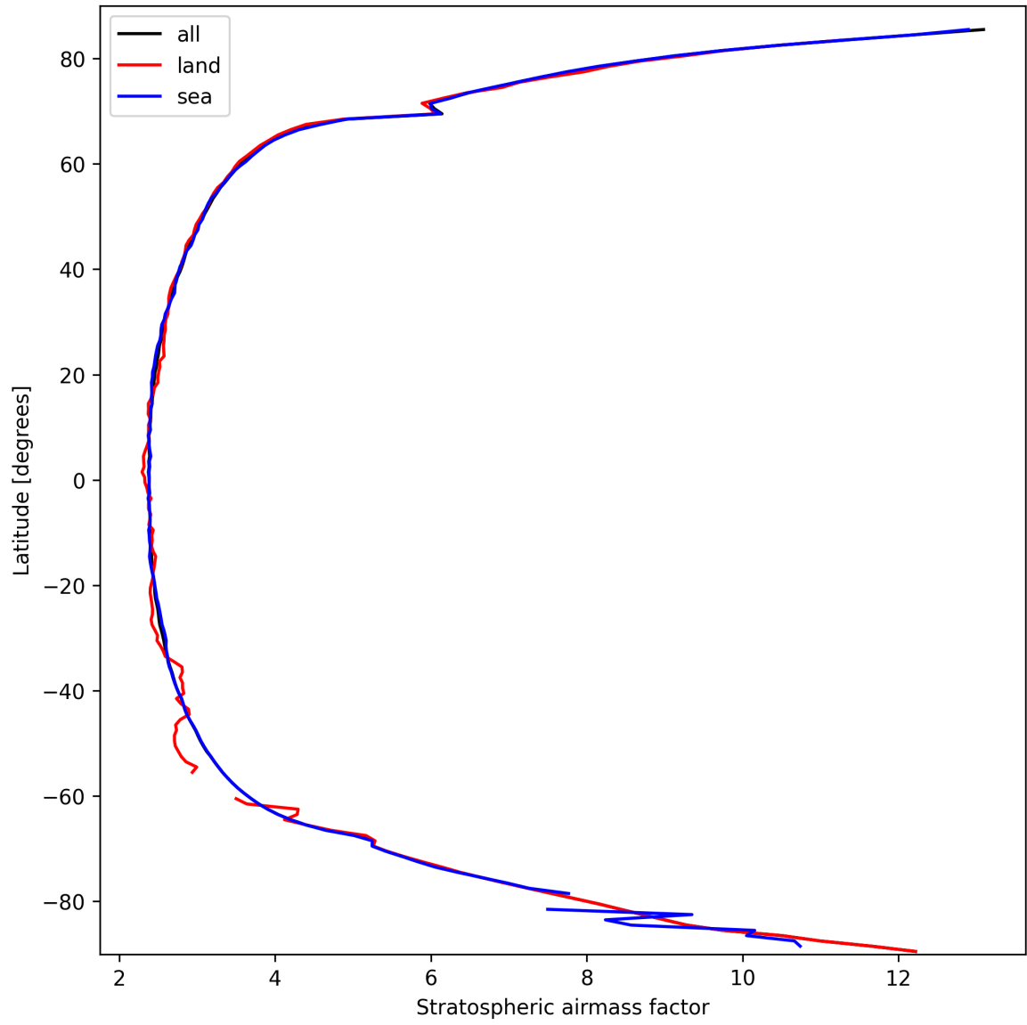
Figure 25: Zonal average of “Stratospheric airmass factor” for 2025-03-12 to 2025-03-13.
