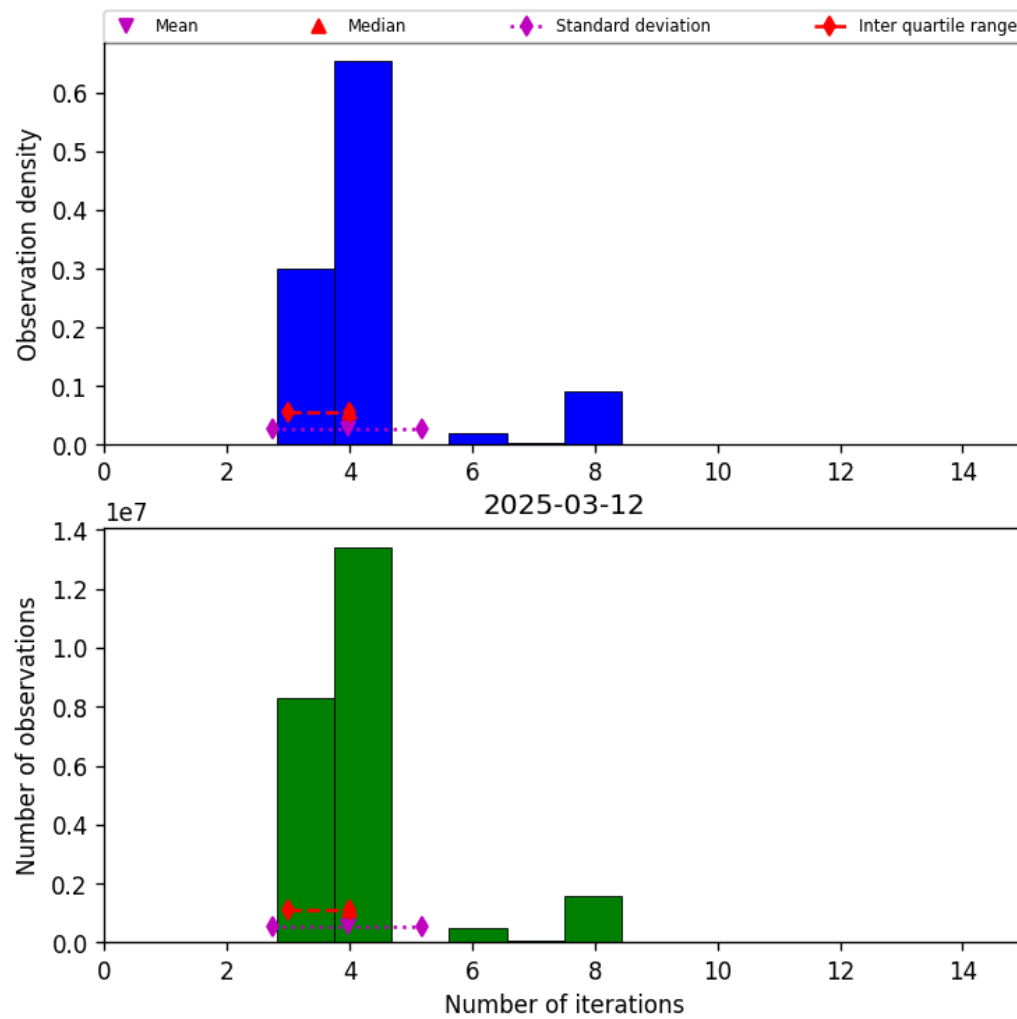
Figure 32: Histogram of “Number of iterations” for 2025-03-12 to 2025-03-13
