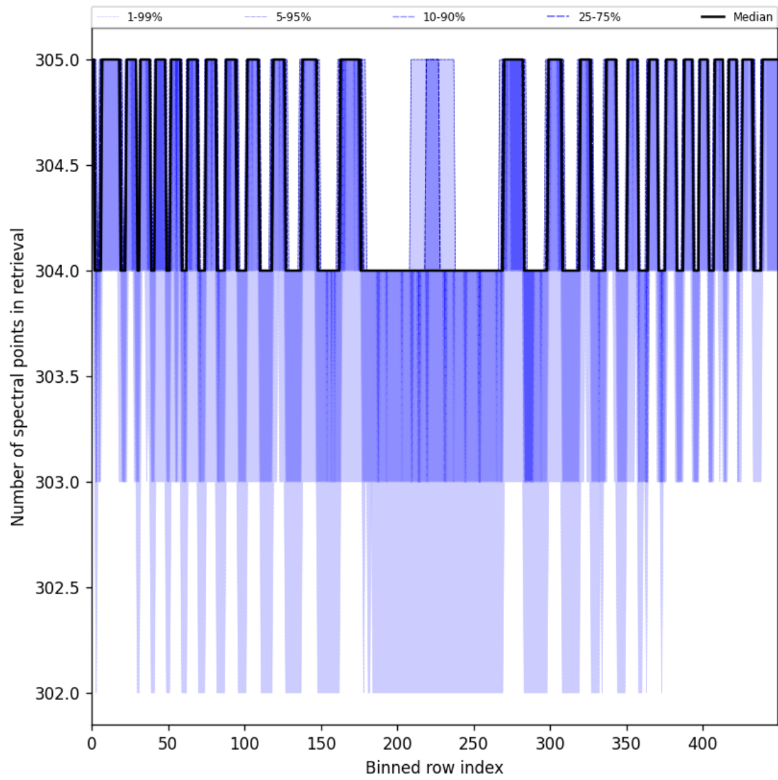
Figure 48: Along track statistics of “Number of spectral points in retrieval” for 2025-03-12 to 2025-03-13
