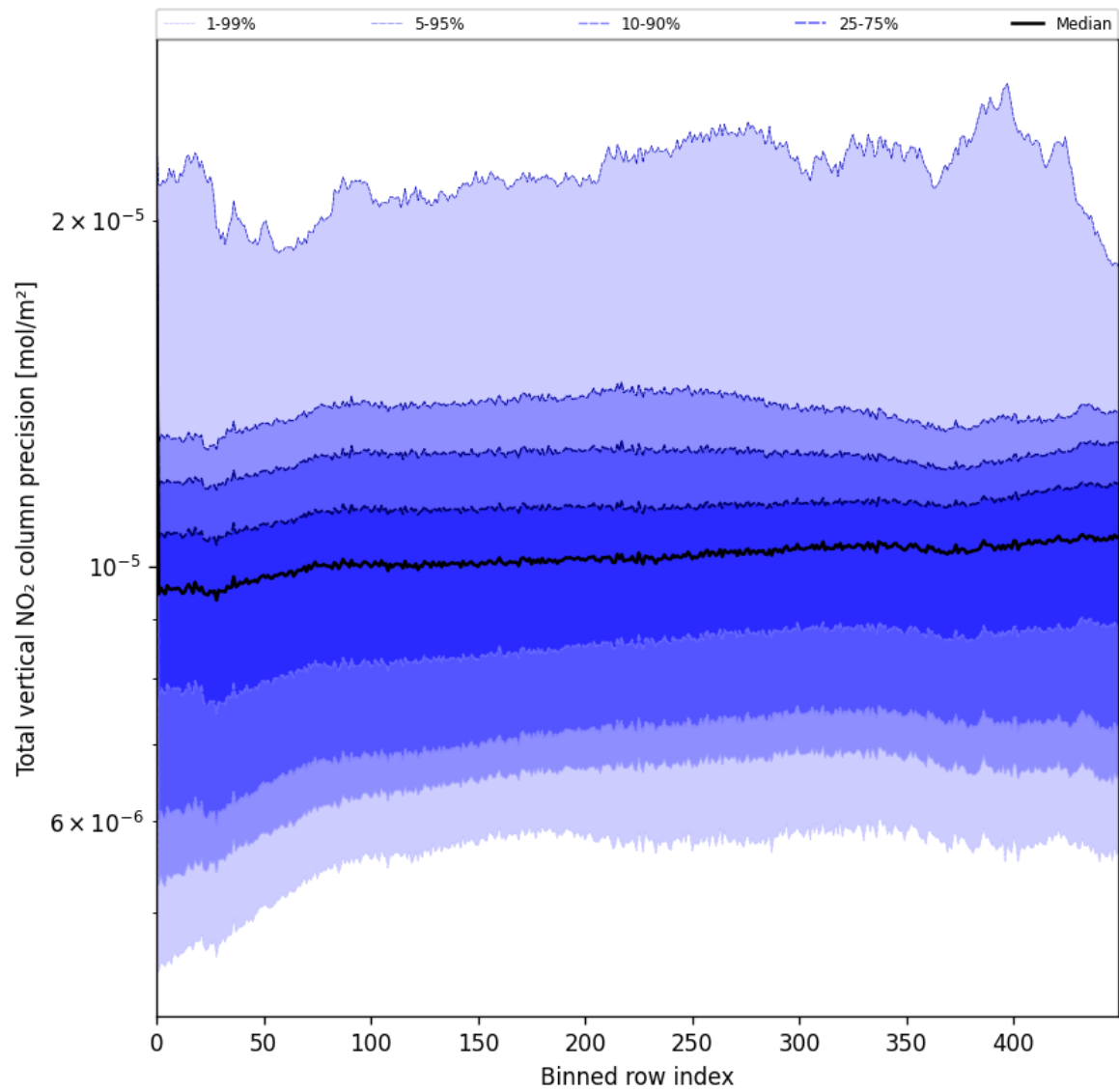
Figure 54: Along track statistics of “Total vertical NO 2 column precision” for 2025-03-12 to 2025-03-13
