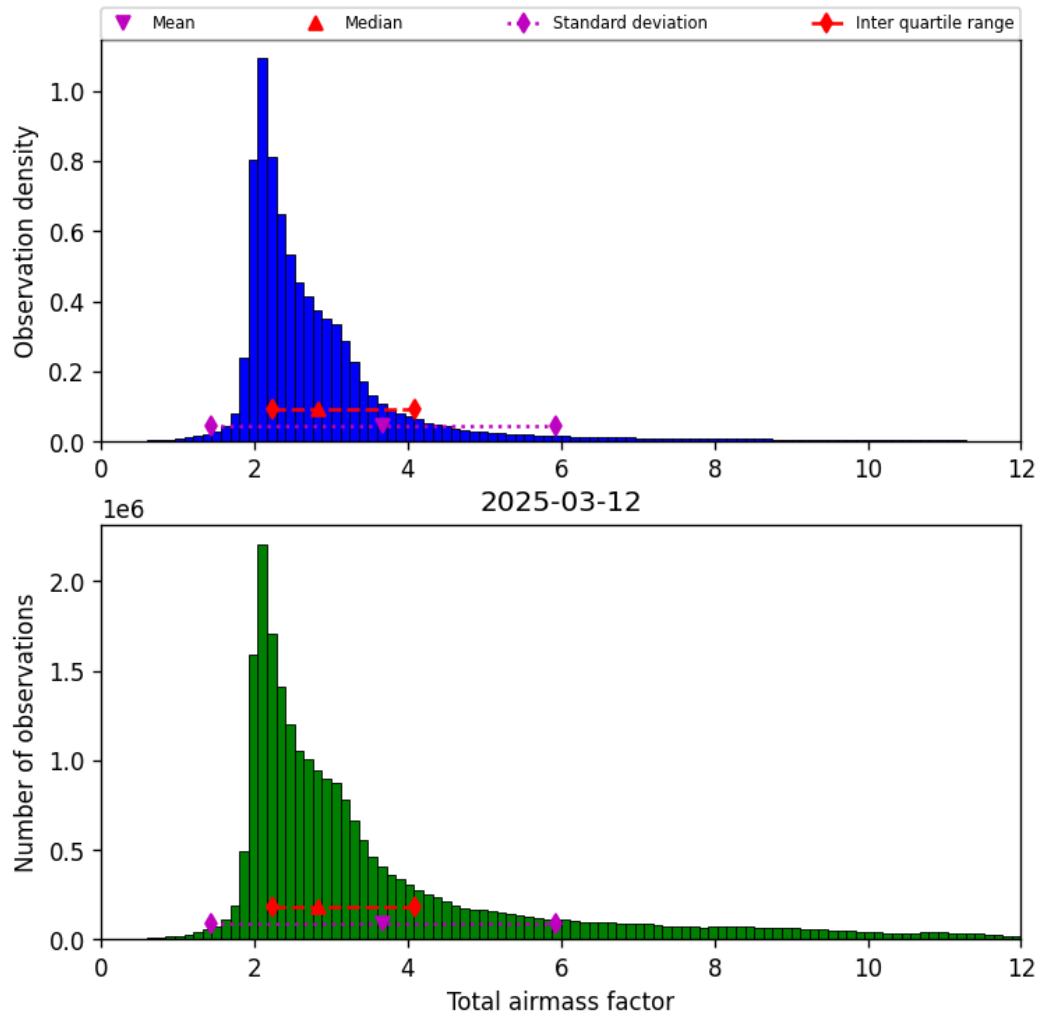
Figure 30: Histogram of “Total airmass factor” for 2025-03-12 to 2025-03-13
