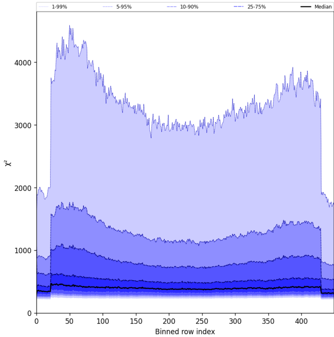
Figure 57: Along track statistics of “ \chi^2 ” for 2025-03-12 to 2025-03-13
