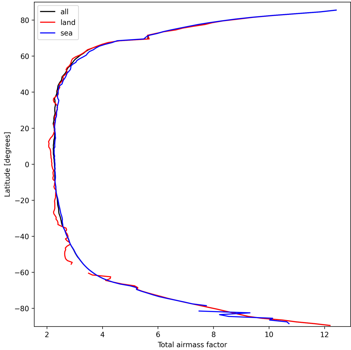
Figure 13: Zonal average of “Total airmass factor” for 2025-03-12 to 2025-03-13.
