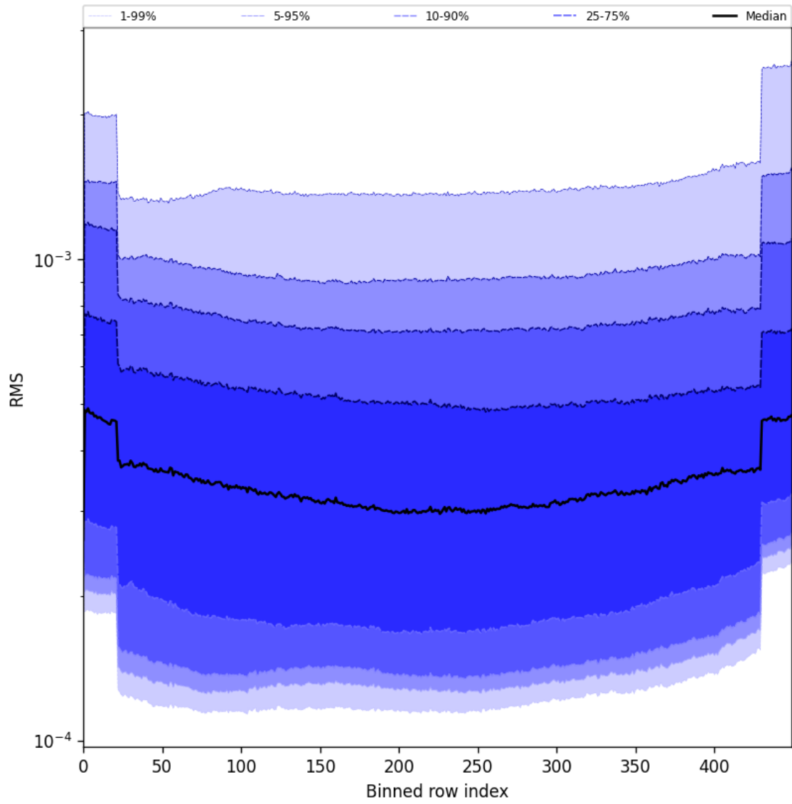
Figure 58: Along track statistics of “RMS” for 2025-03-12 to 2025-03-13
