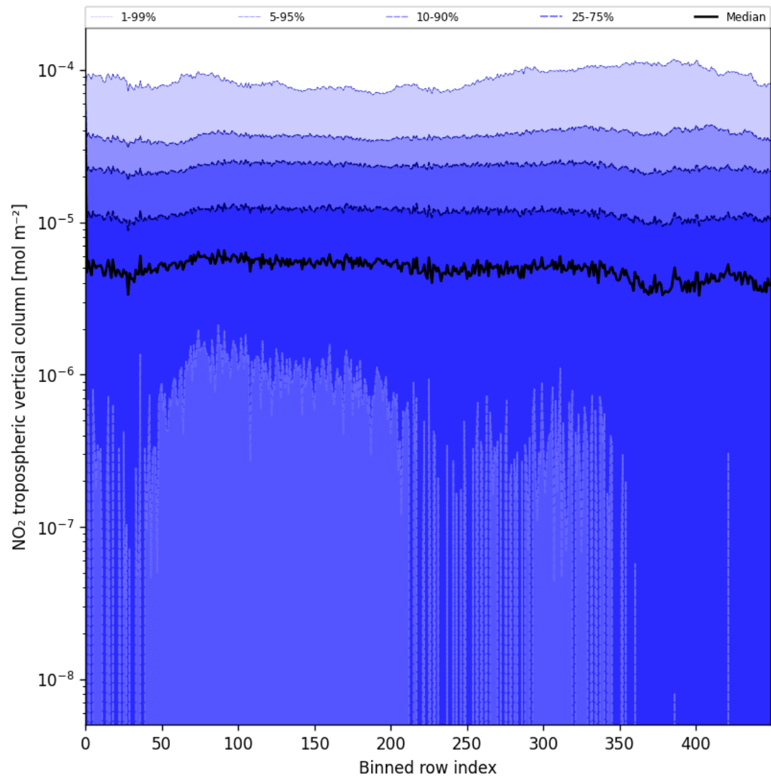
Figure 44: Along track statistics of “NO 2 tropospheric vertical column” for 2025-03-12 to 2025-03-13
