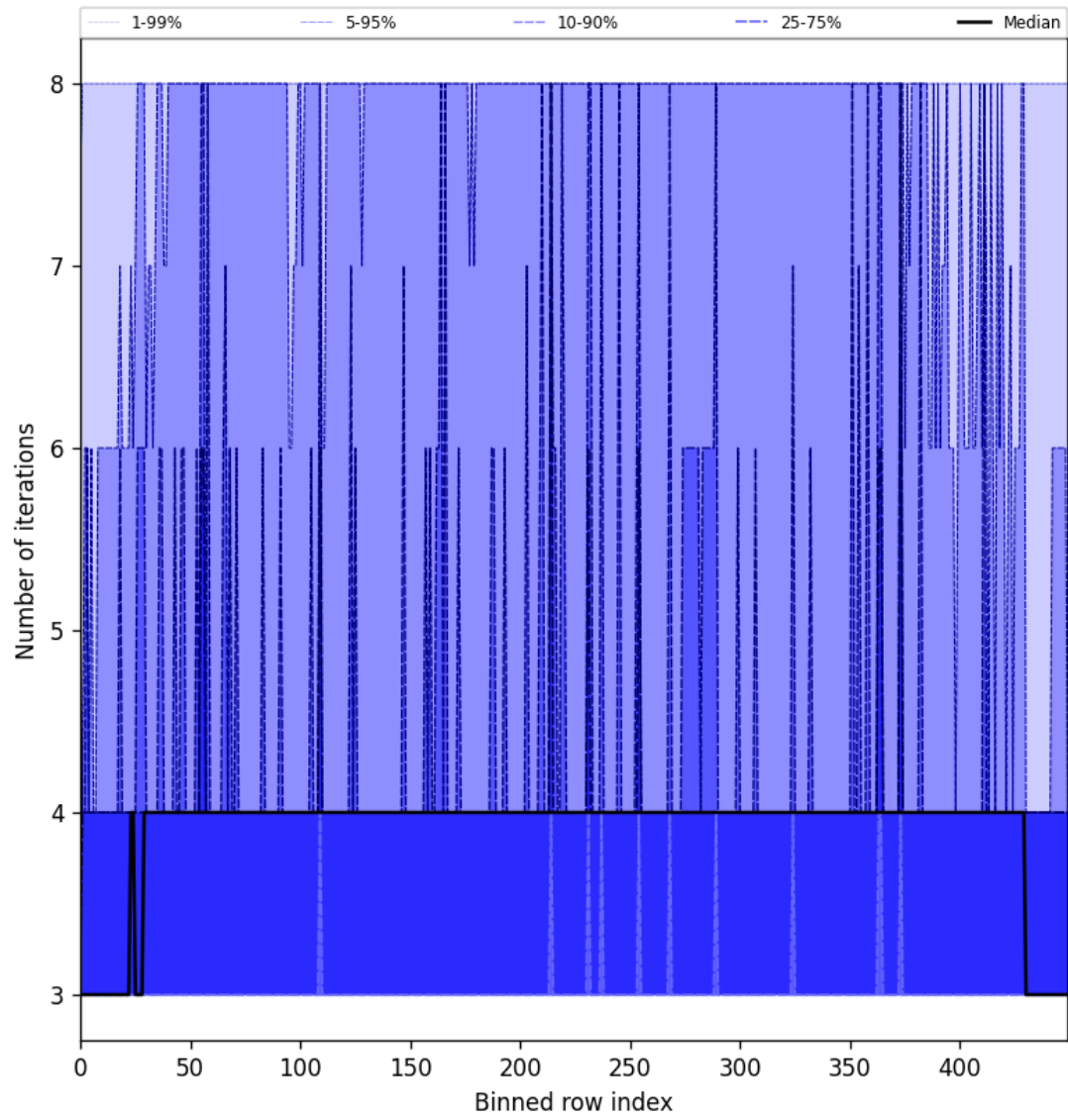
Figure 49: Along track statistics of “Number of iterations” for 2025-03-12 to 2025-03-13
