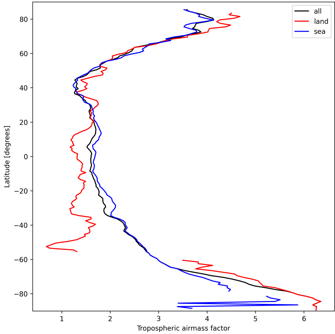
Figure 12: Zonal average of “Tropospheric airmass factor” for 2025-03-12 to 2025-03-13.
