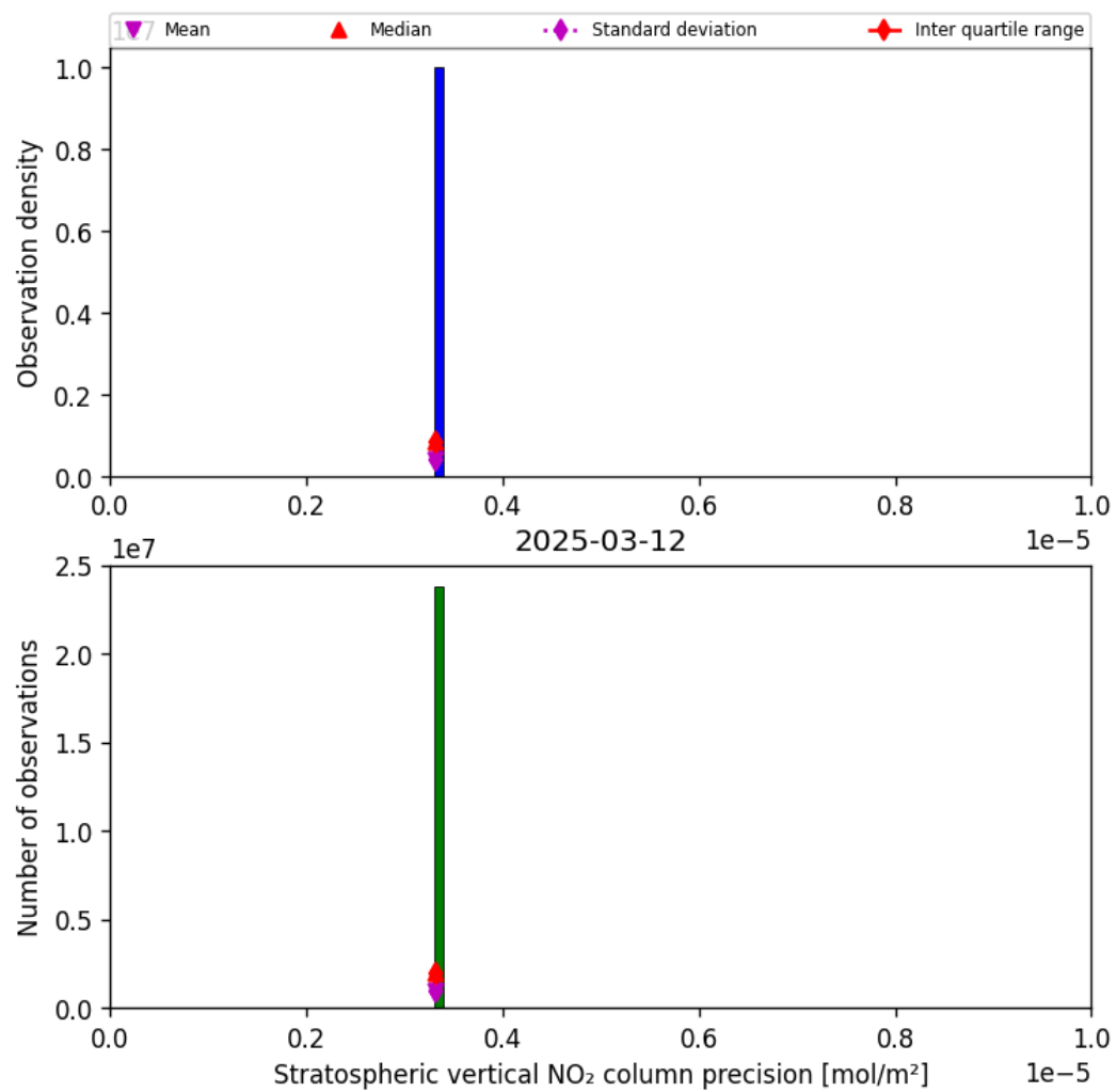
Figure 35: Histogram of “Stratospheric vertical NO 2 column precision” for 2025-03-12 to 2025-03-13
