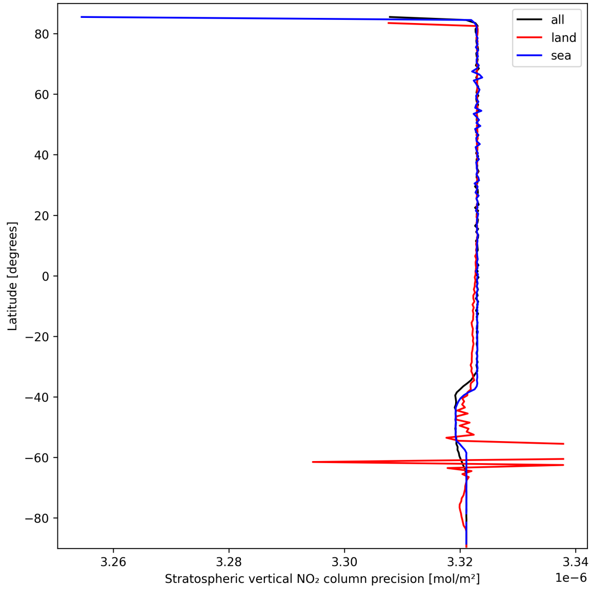
Figure 18: Zonal average of "Stratospheric vertical NO 2 column precision" for 2025-03-12 to 2025-03-13.
