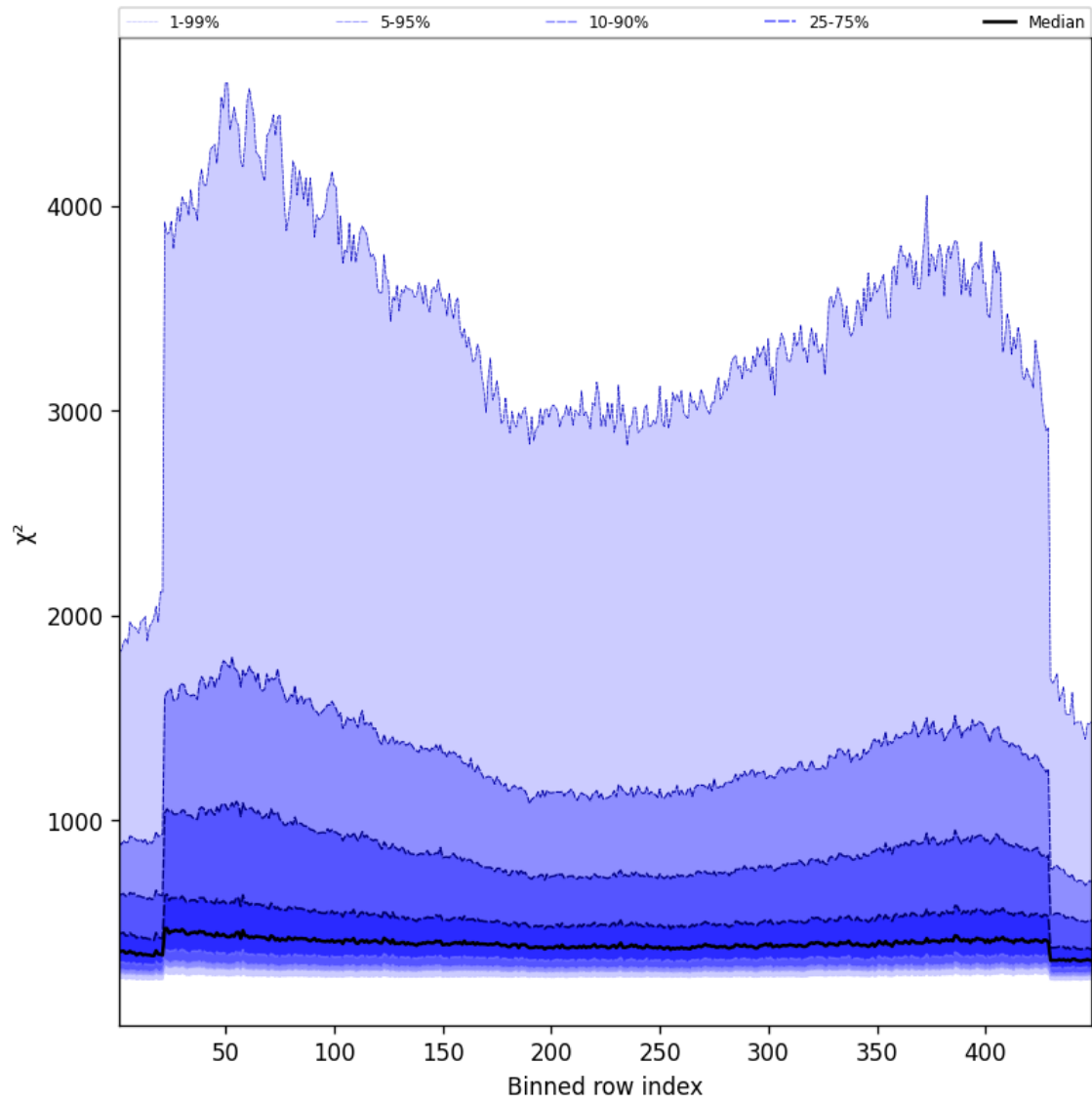
Figure 57: Along track statistics of “ \chi^2 ” for 2025-03-13 to 2025-03-14
