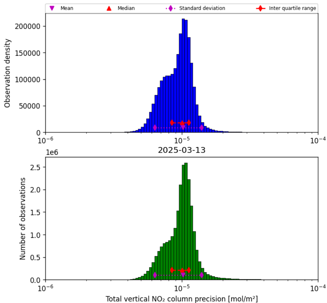
Figure 37: Histogram of “Total vertical NO 2 column precision” for 2025-03-13 to 2025-03-14
