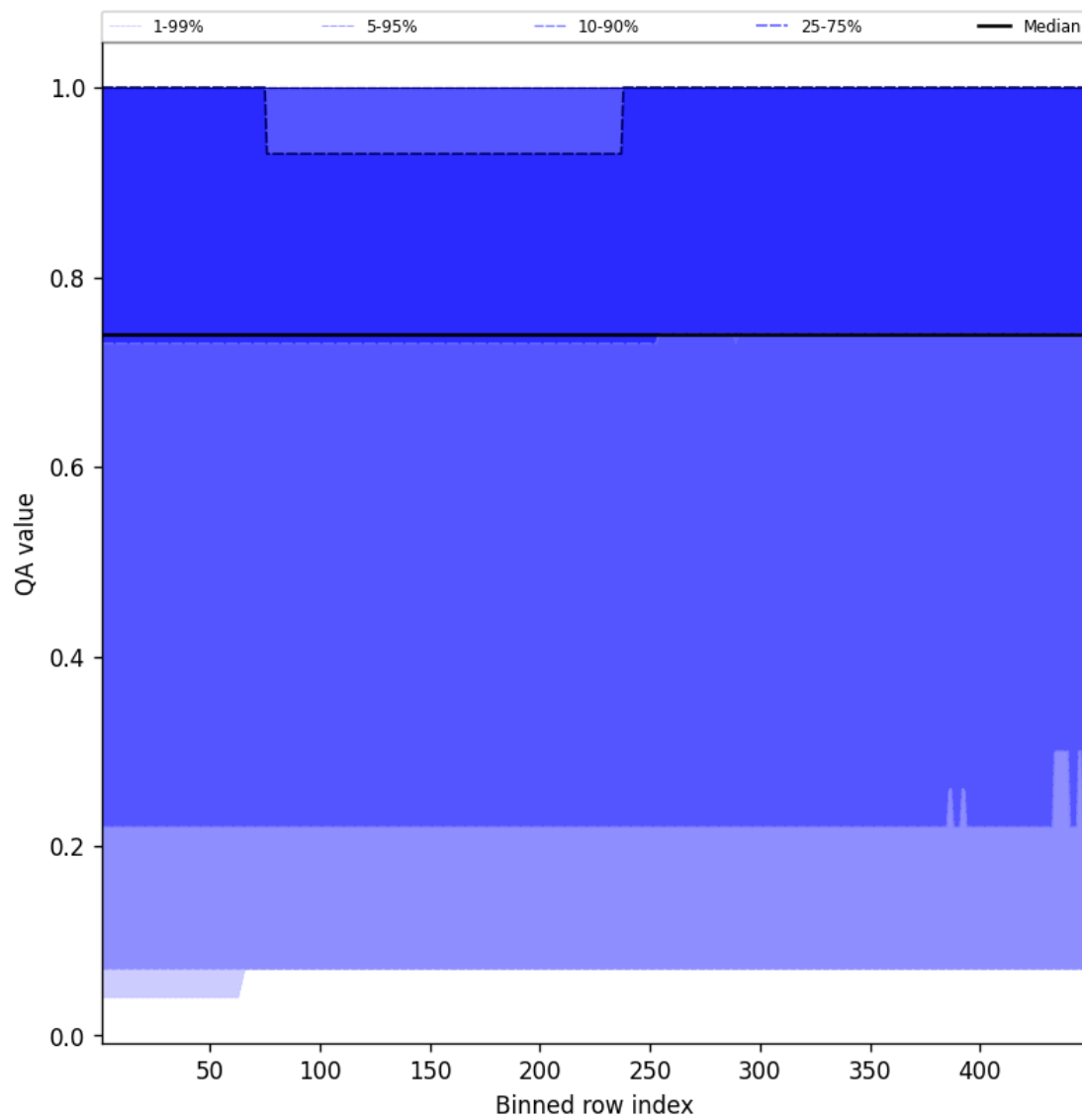
Figure 43: Along track statistics of “QA value” for 2025-03-13 to 2025-03-14
