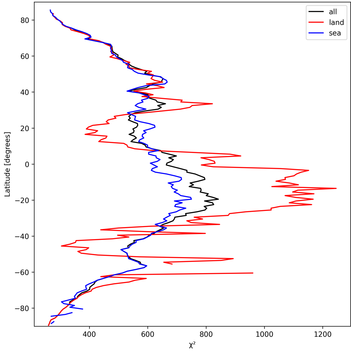
Figure 23: Zonal average of “ \chi^2 ” for 2025-03-13 to 2025-03-14.
