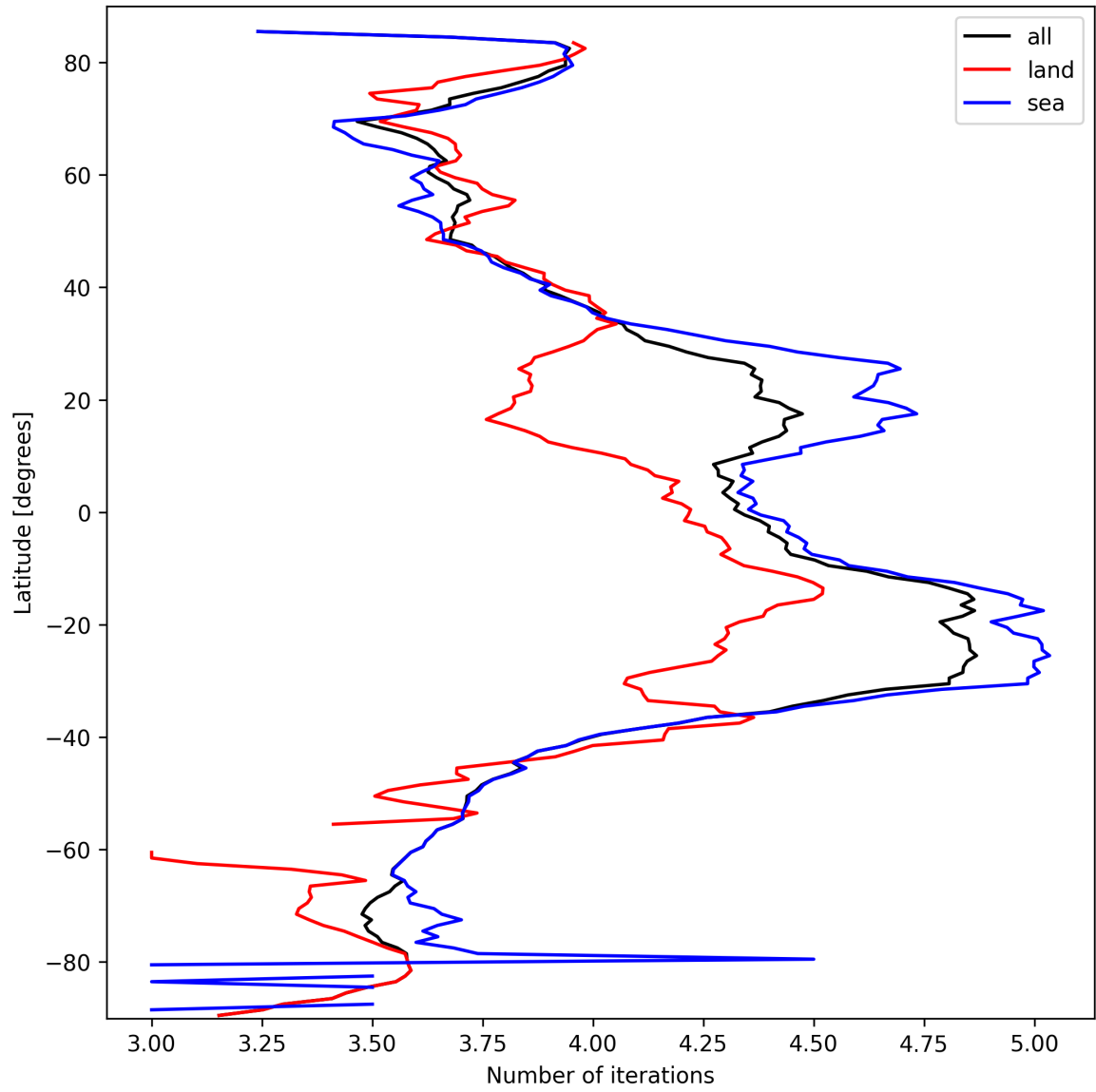
Figure 15: Zonal average of “Number of iterations” for 2025-03-13 to 2025-03-14.
