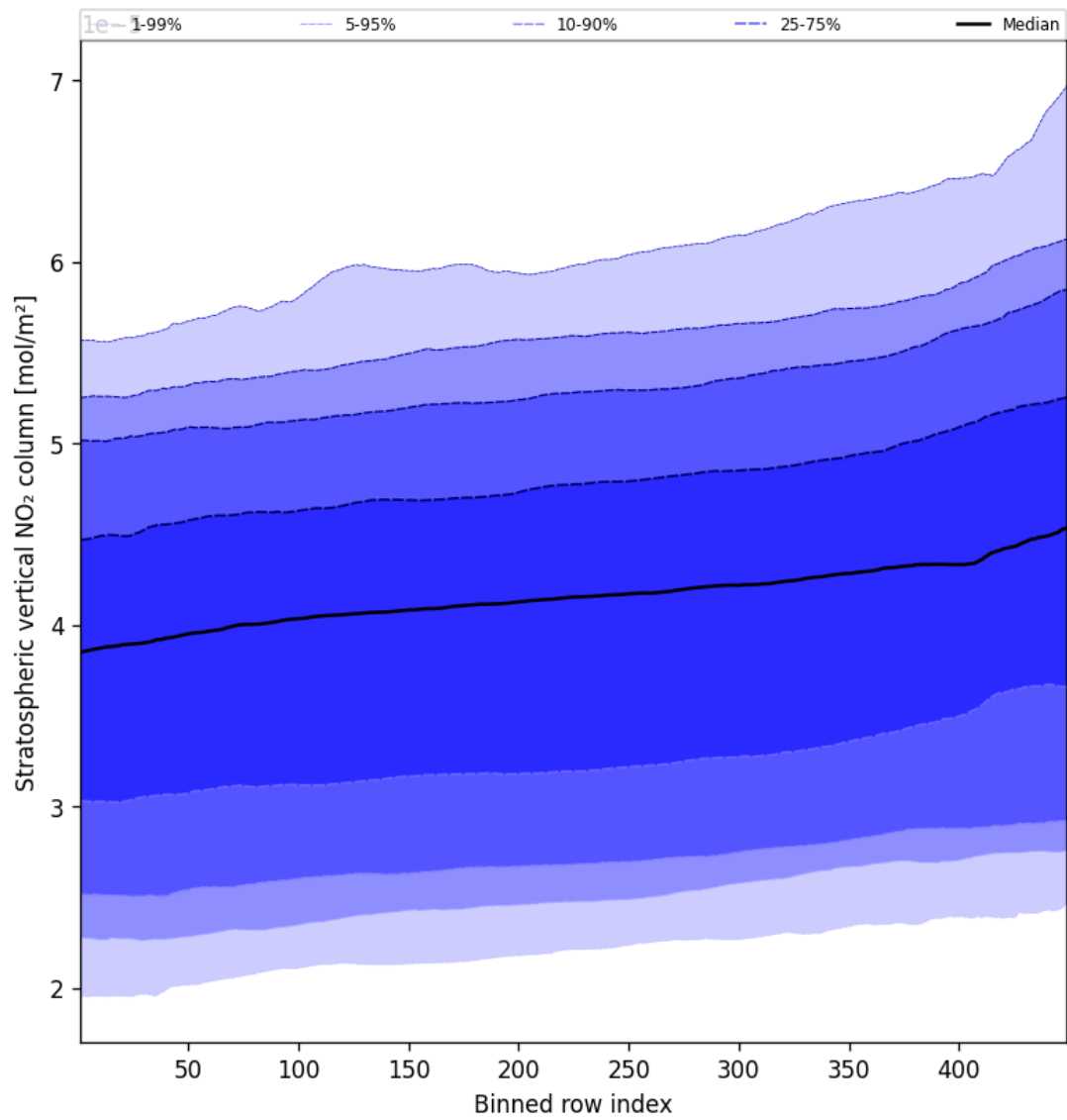
Figure 51: Along track statistics of “Stratospheric vertical NO 2 column” for 2025-03-13 to 2025-03-14
