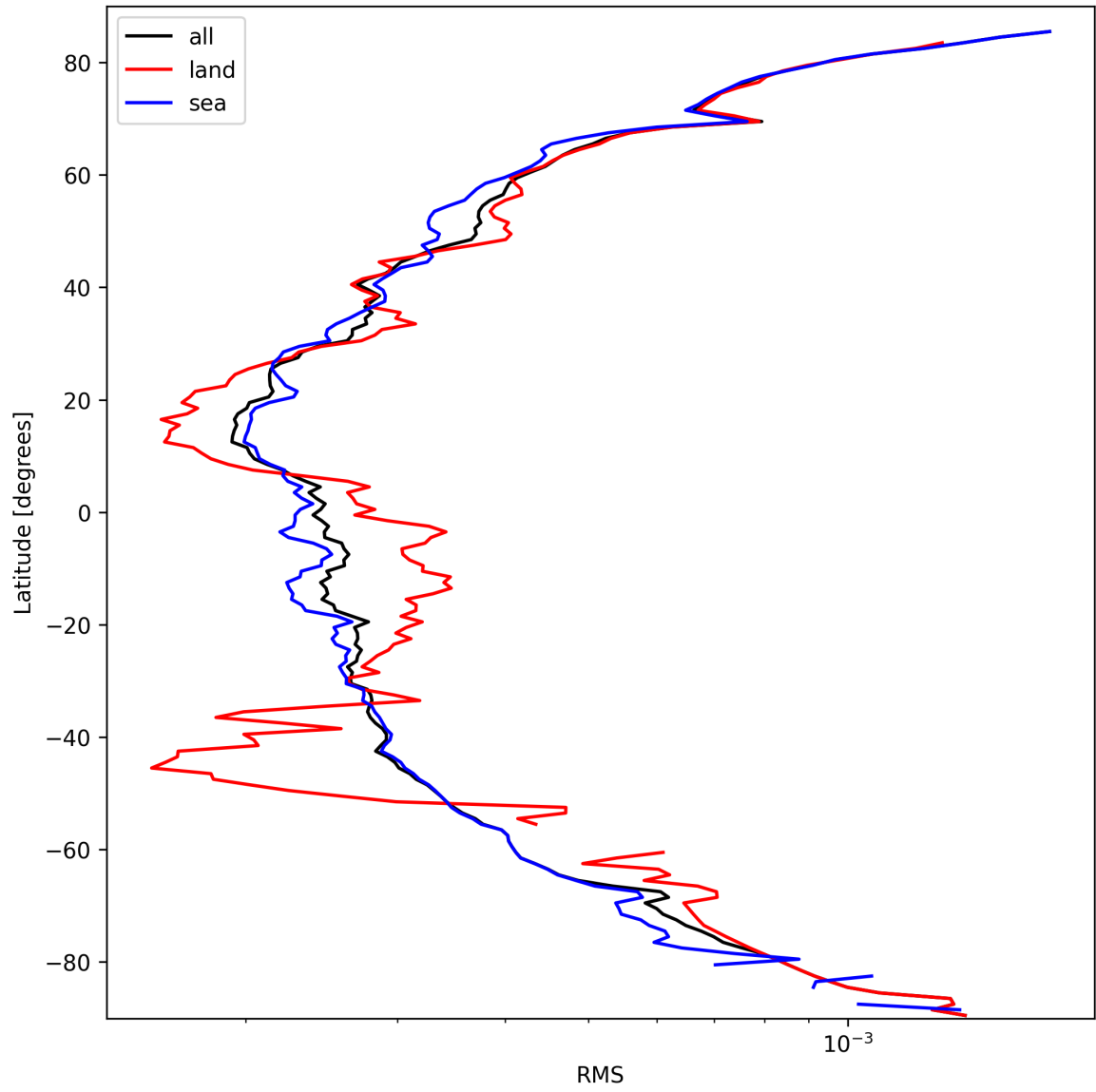
Figure 24: Zonal average of “RMS” for 2025-03-13 to 2025-03-14.
