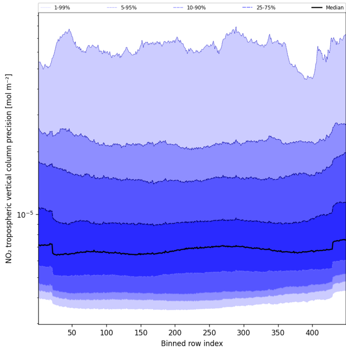
Figure 45: Along track statistics of “NO 2 tropospheric vertical column precision” for 2025-03-13 to 2025-03-14
