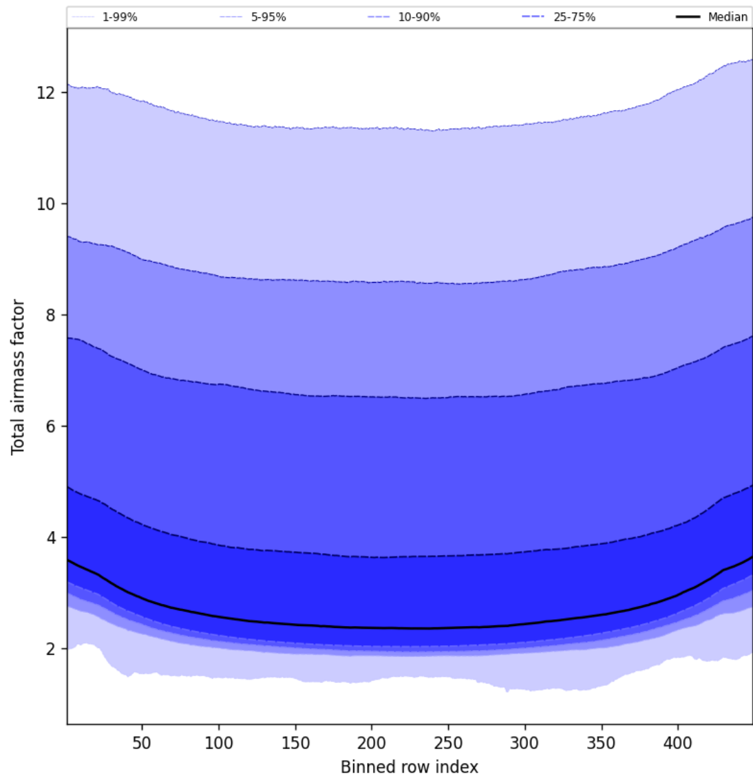
Figure 47: Along track statistics of “Total airmass factor” for 2025-03-13 to 2025-03-14
