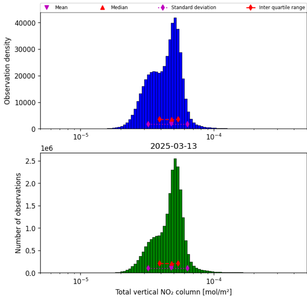
Figure 36: Histogram of “Total vertical NO 2 column” for 2025-03-13 to 2025-03-14
