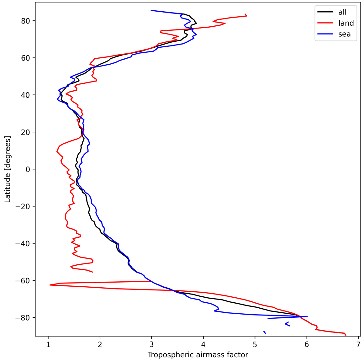
Figure 12: Zonal average of “Tropospheric airmass factor” for 2025-03-13 to 2025-03-14.
