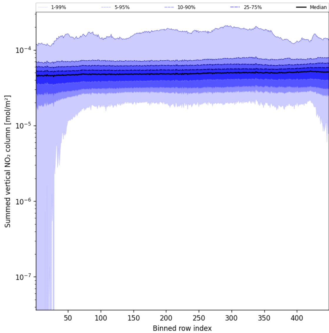
Figure 55: Along track statistics of “Summed vertical NO 2 column” for 2025-03-13 to 2025-03-14
