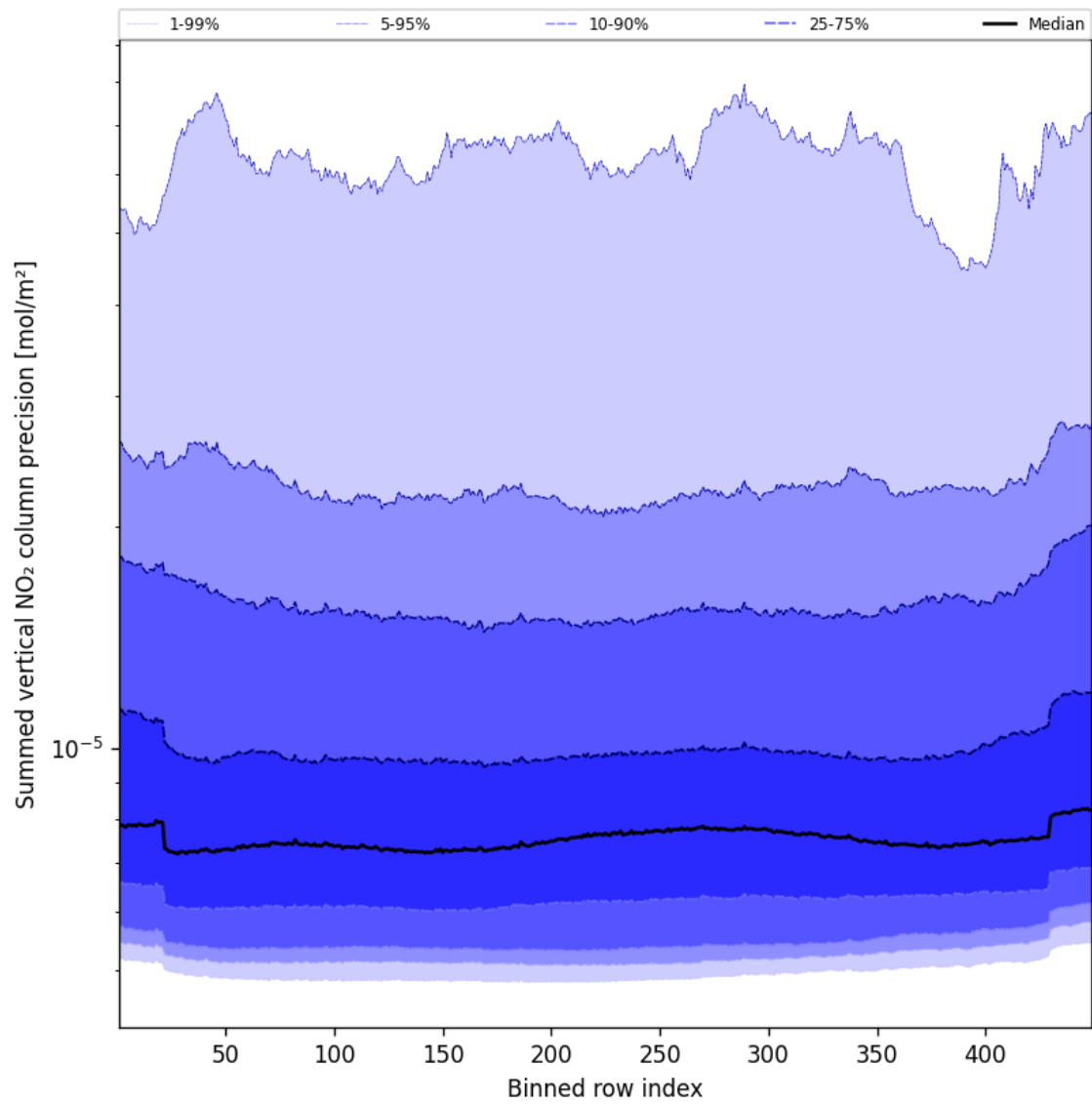
Figure 56: Along track statistics of “Summed vertical NO 2 column precision” for 2025-03-13 to 2025-03-14
