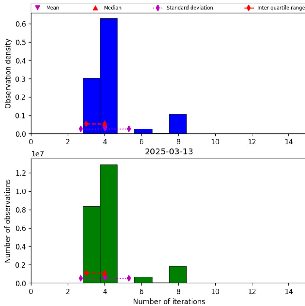
Figure 32: Histogram of “Number of iterations” for 2025-03-13 to 2025-03-14
