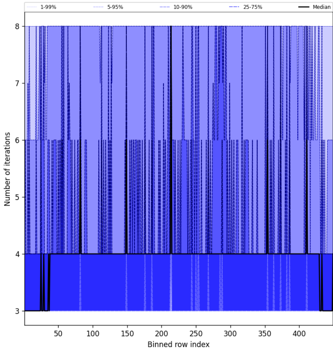
Figure 49: Along track statistics of “Number of iterations” for 2025-03-13 to 2025-03-14
