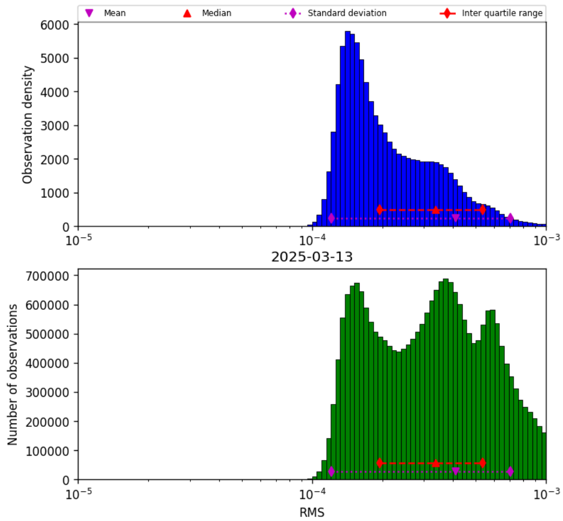
Figure 41: Histogram of “RMS” for 2025-03-13 to 2025-03-14
