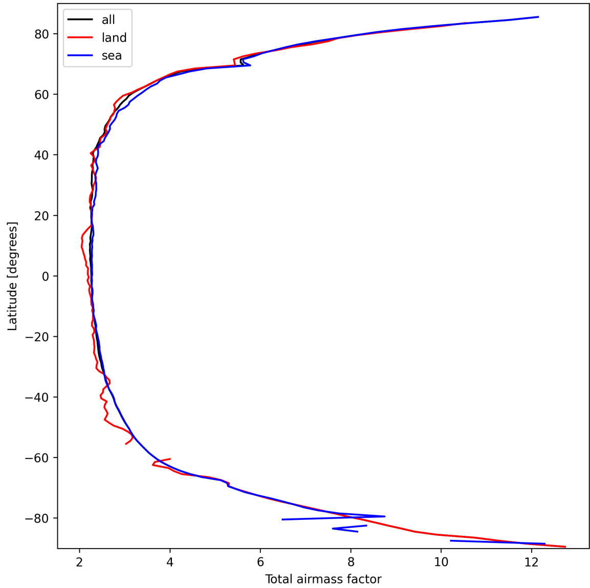
Figure 13: Zonal average of “Total airmass factor” for 2025-03-13 to 2025-03-14.
