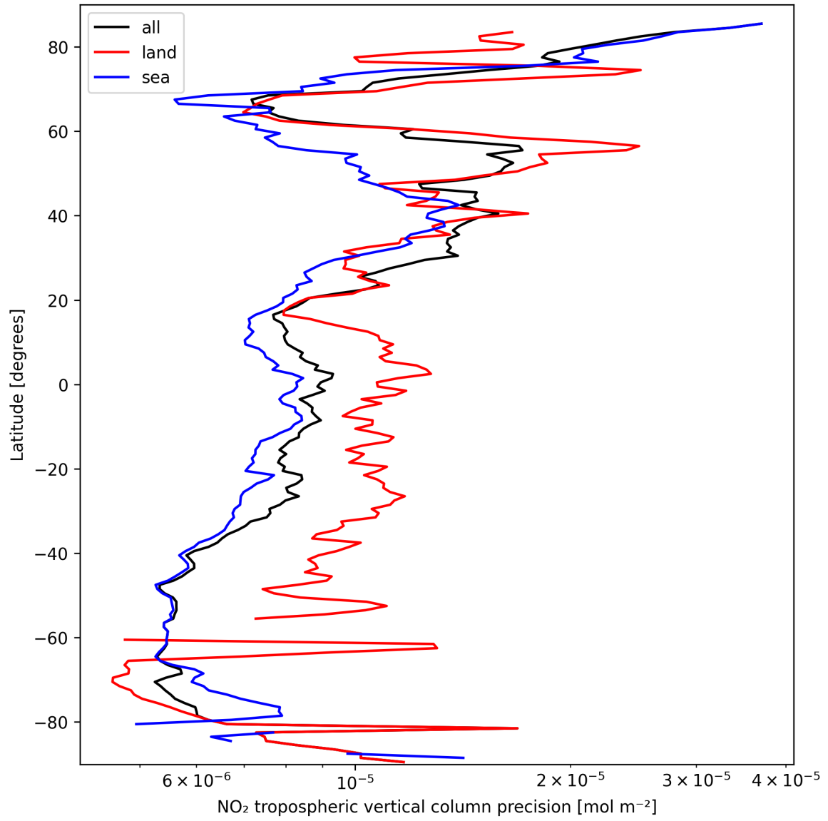
Figure 11: Zonal average of “NO 2 tropospheric vertical column precision” for 2025-03-13 to 2025-03-14.
