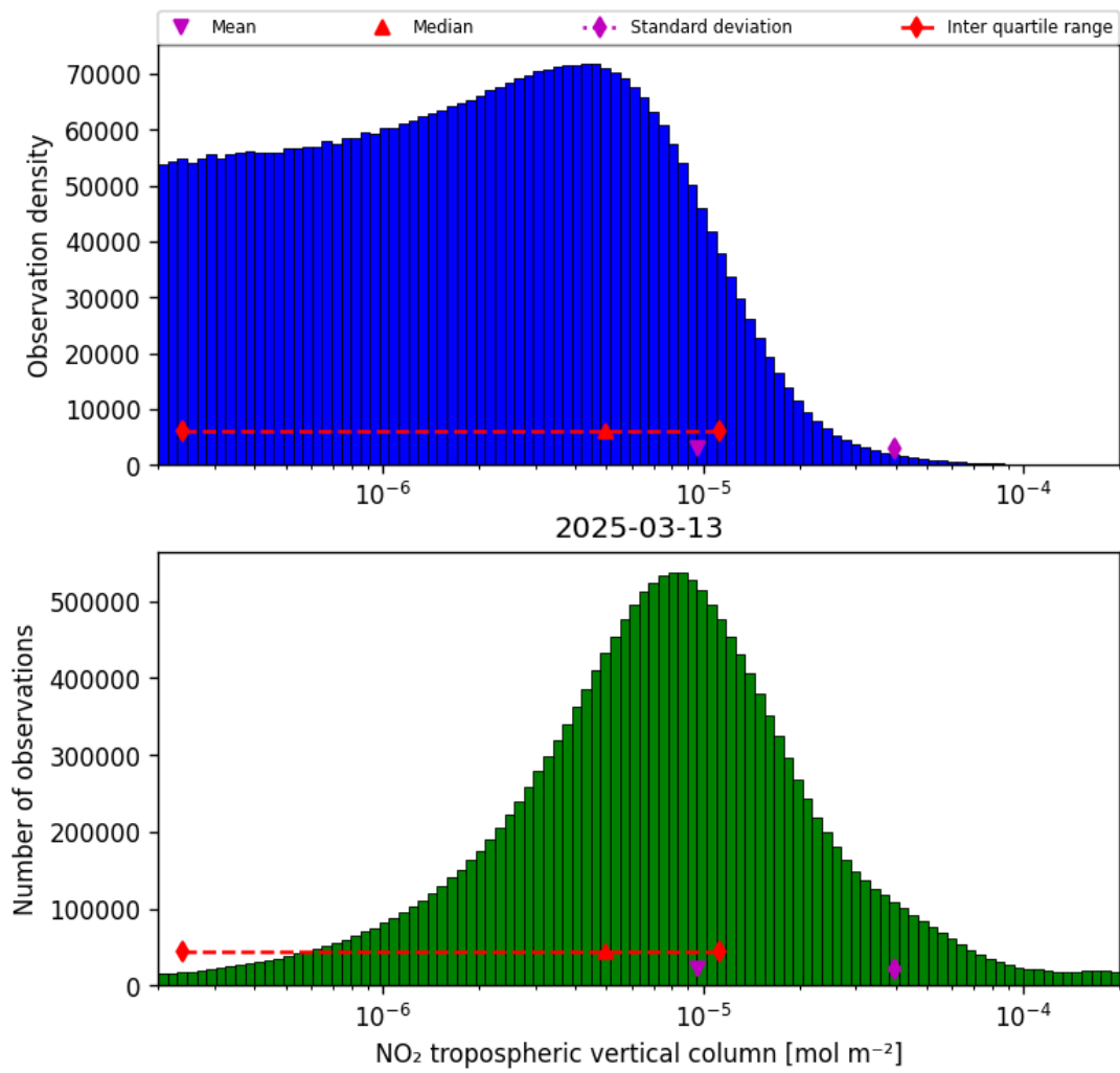
Figure 27: Histogram of “NO 2 tropospheric vertical column” for 2025-03-13 to 2025-03-14
