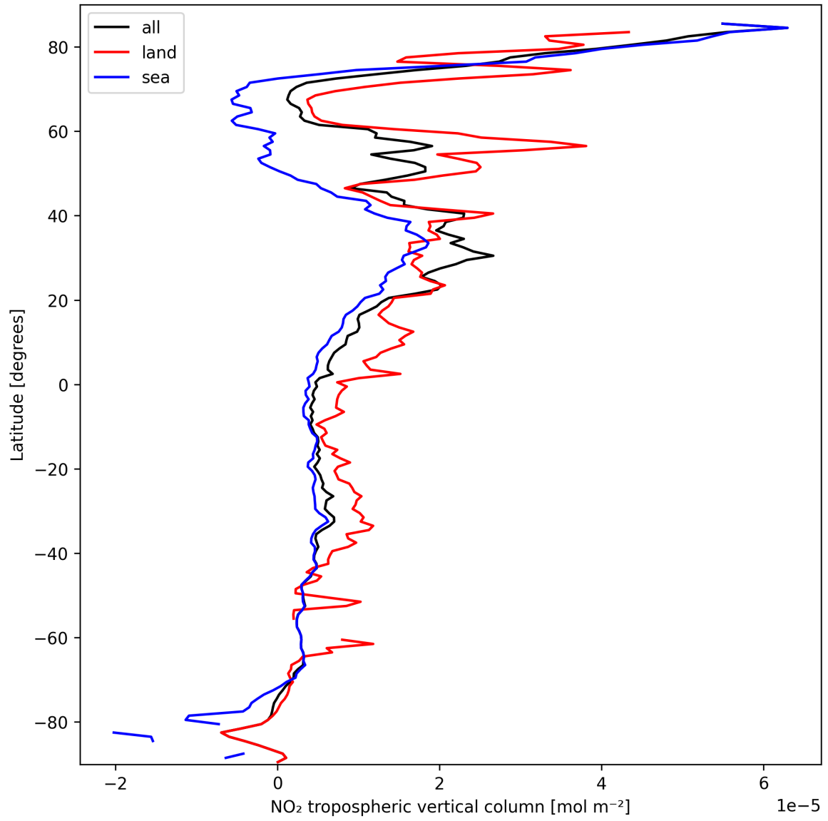
Figure 10: Zonal average of “NO 2 tropospheric vertical column” for 2025-03-13 to 2025-03-14.
