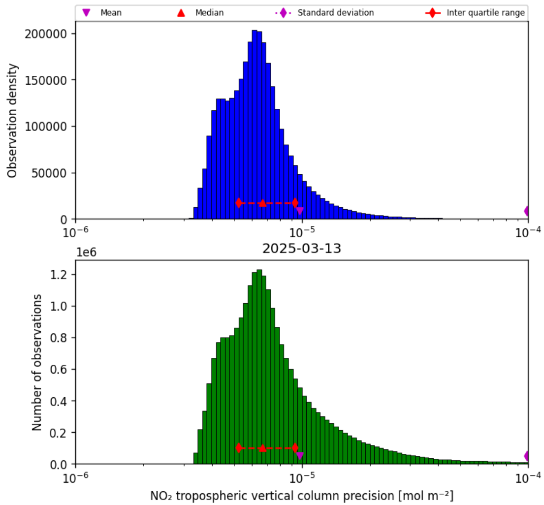
Figure 28: Histogram of “NO 2 tropospheric vertical column precision” for 2025-03-13 to 2025-03-14
