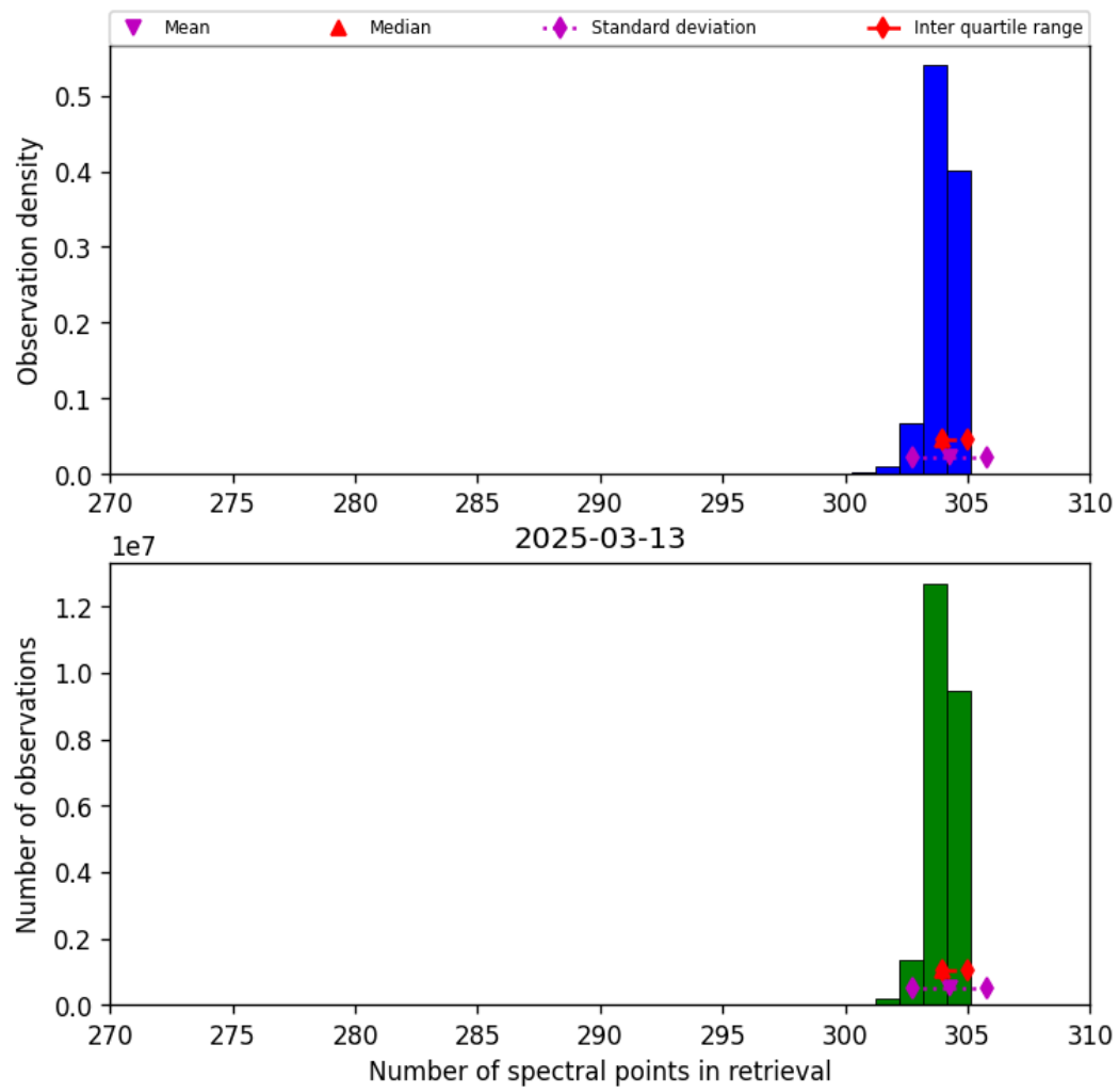
Figure 31: Histogram of “Number of spectral points in retrieval” for 2025-03-13 to 2025-03-14
