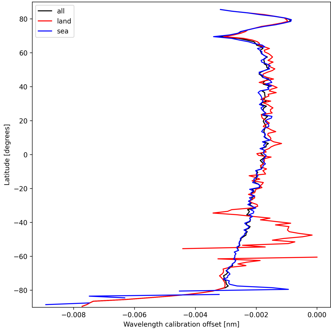
Figure 16: Zonal average of “Wavelength calibration offset” for 2025-03-13 to 2025-03-14.
