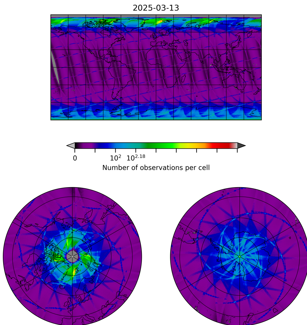
Figure 8: Map of the number of observations for 2025-03-13 to 2025-03-14
