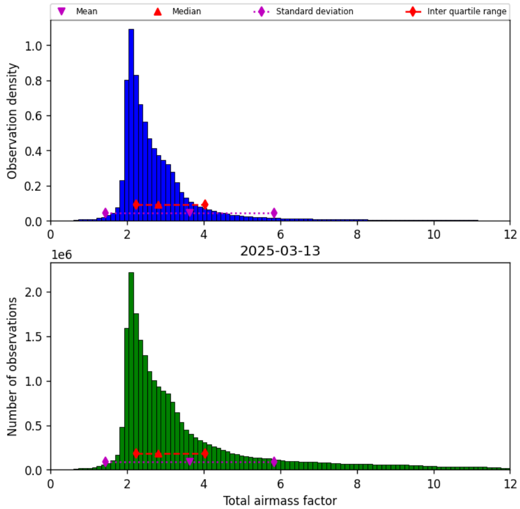
Figure 30: Histogram of “Total airmass factor” for 2025-03-13 to 2025-03-14
