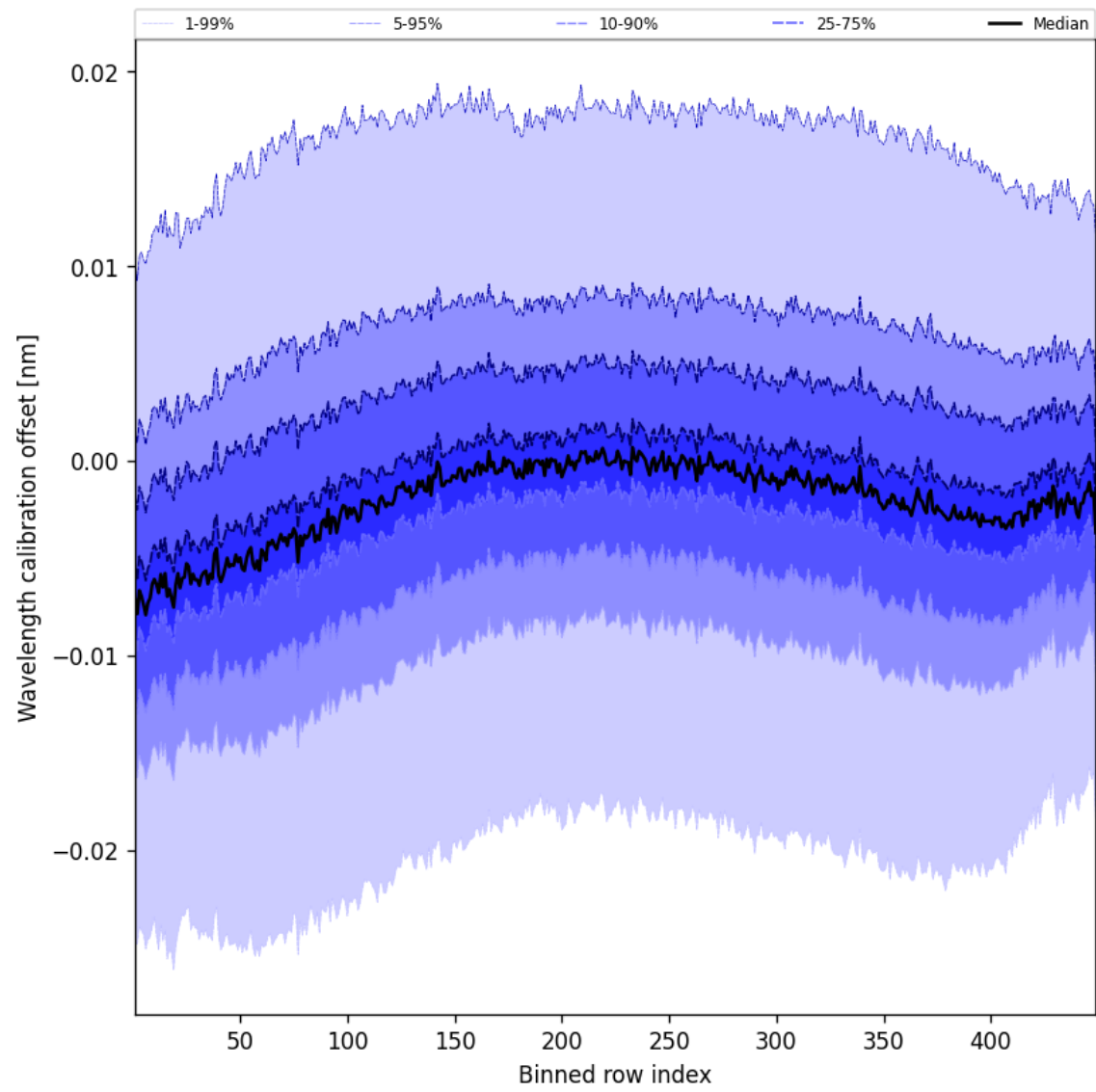
Figure 50: Along track statistics of “Wavelength calibration offset” for 2025-03-13 to 2025-03-14
