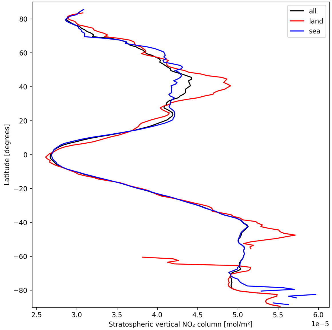
Figure 17: Zonal average of “Stratospheric vertical NO 2 column” for 2025-03-13 to 2025-03-14.
