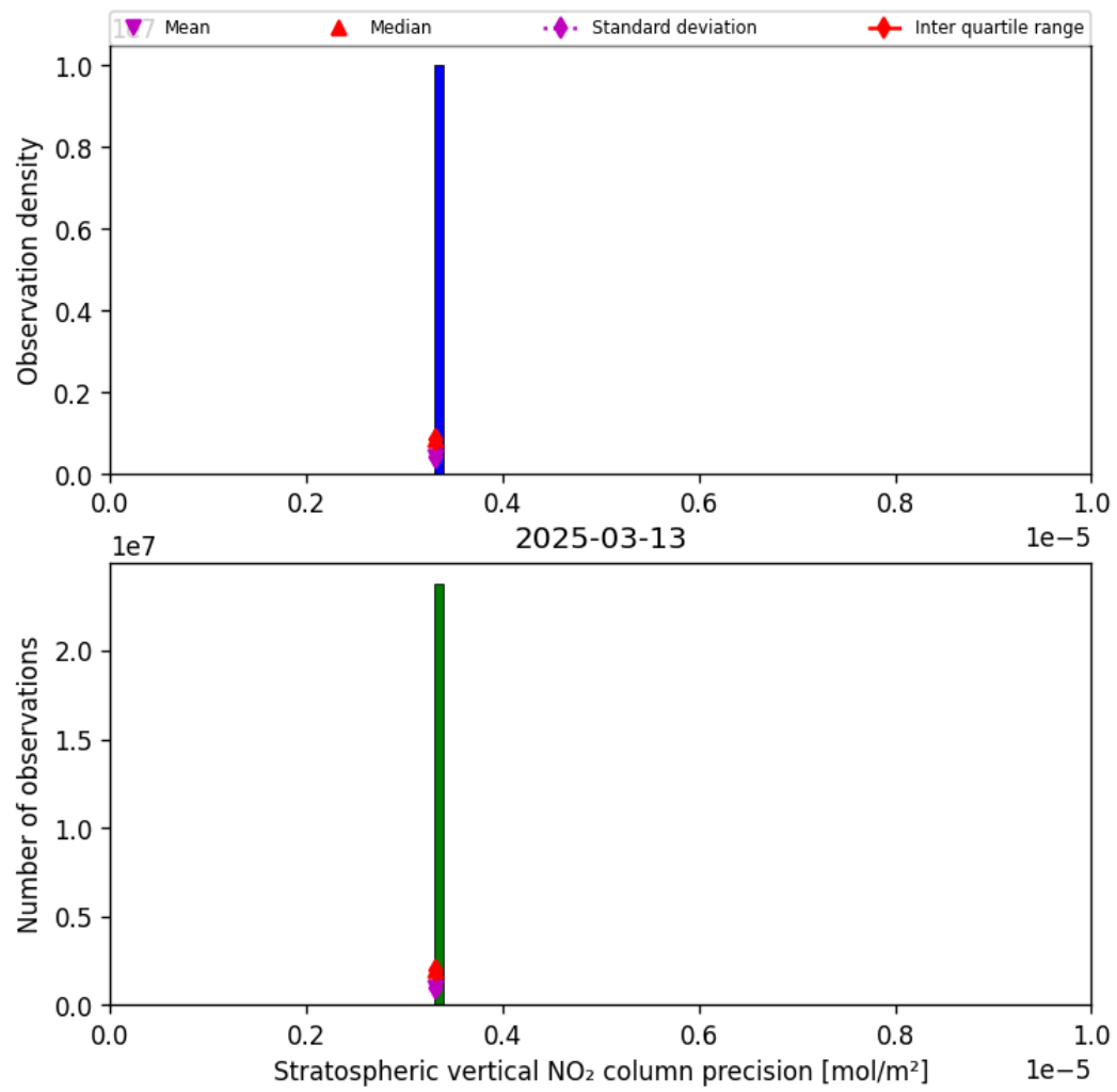
Figure 35: Histogram of “Stratospheric vertical NO 2 column precision” for 2025-03-13 to 2025-03-14
