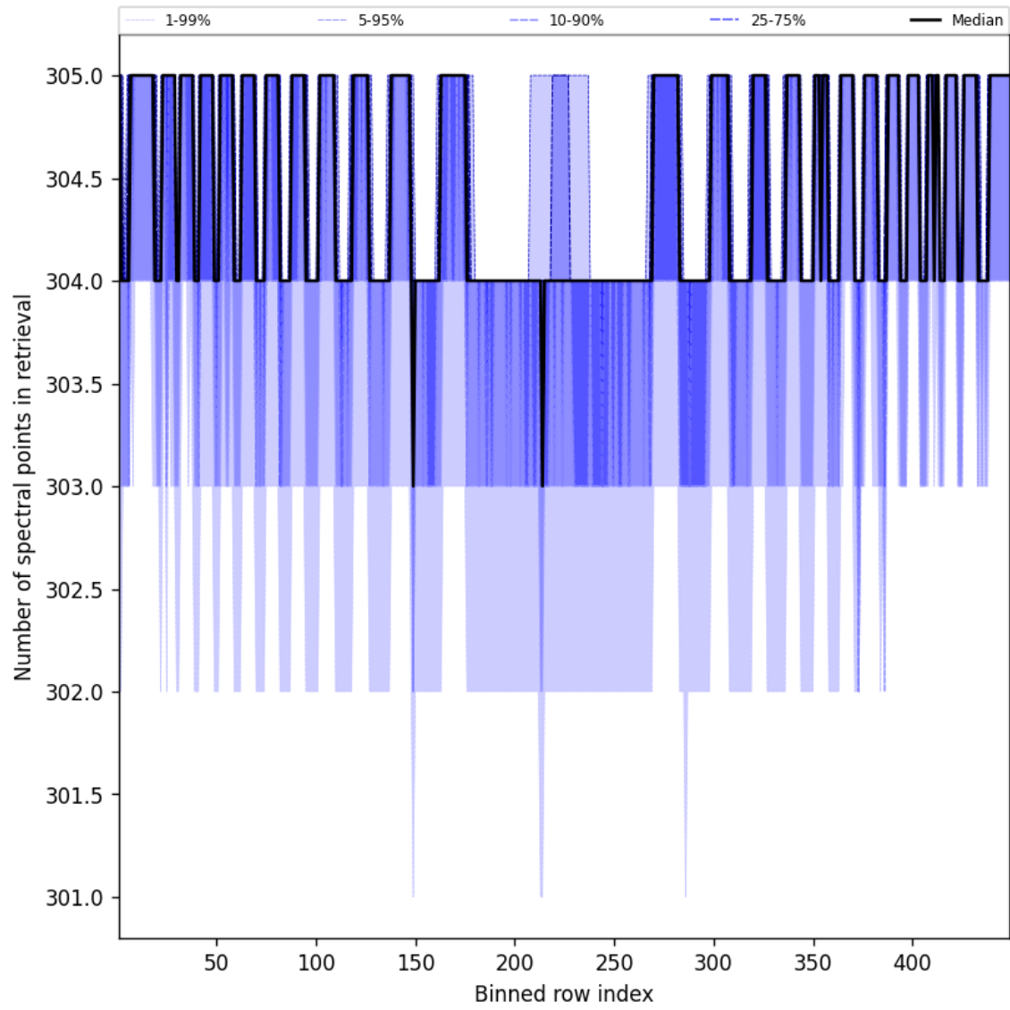
Figure 48: Along track statistics of “Number of spectral points in retrieval” for 2025-03-13 to 2025-03-14
