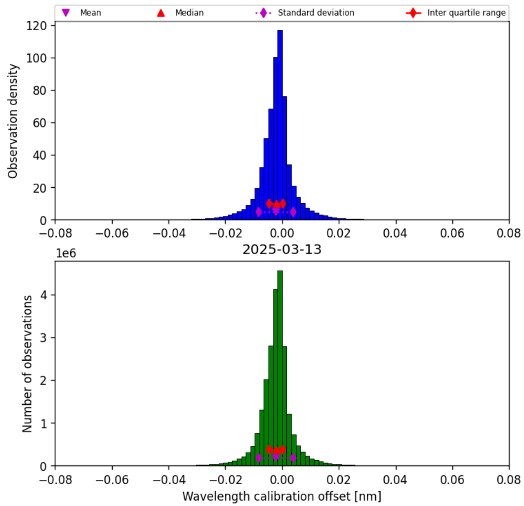
Figure 33: Histogram of “Wavelength calibration offset” for 2025-03-13 to 2025-03-14
