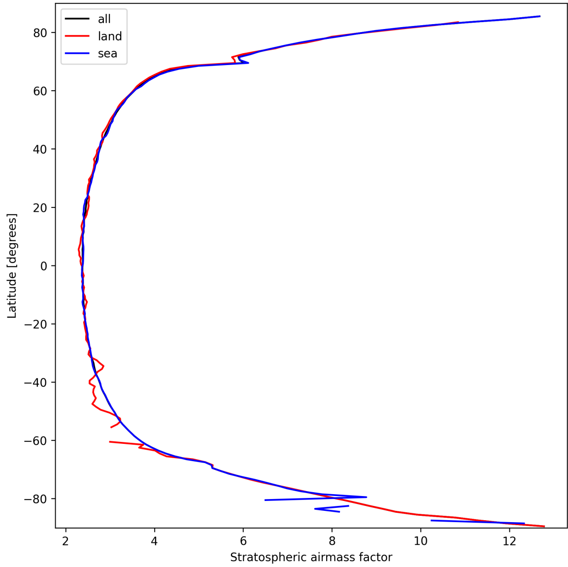
Figure 25: Zonal average of “Stratospheric airmass factor” for 2025-03-13 to 2025-03-14.
