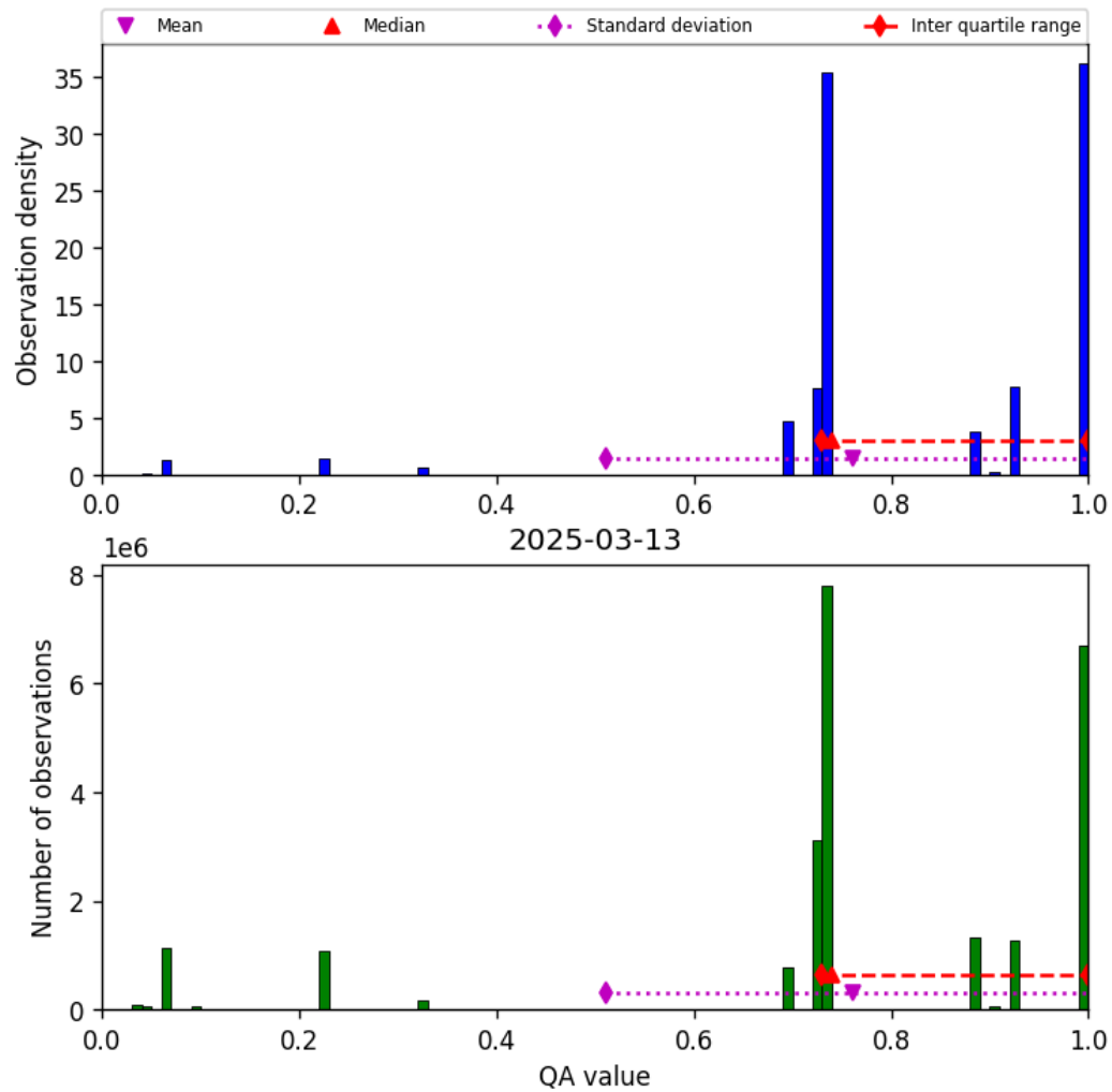
Figure 26: Histogram of “QA value” for 2025-03-13 to 2025-03-14
