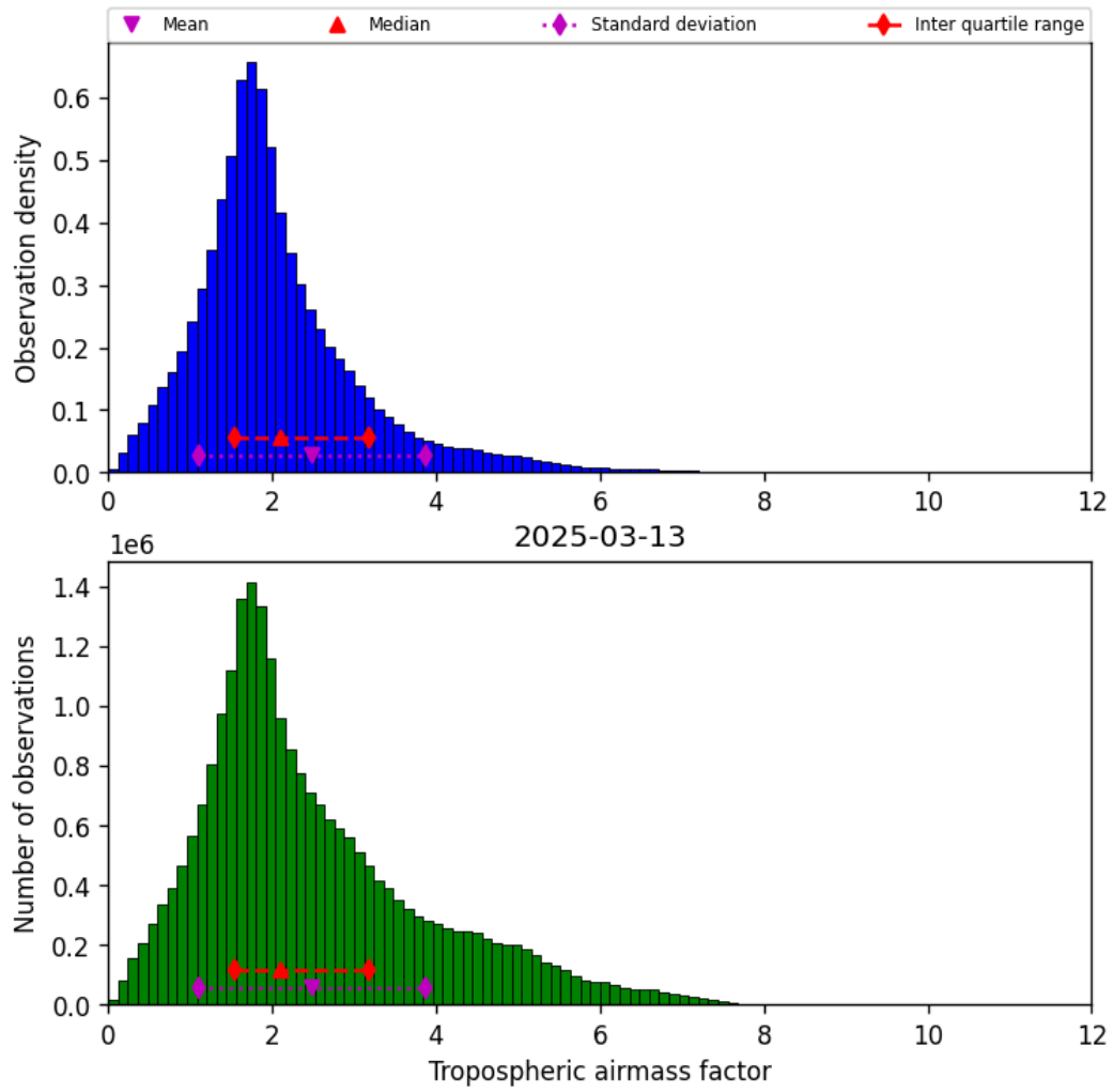
Figure 29: Histogram of “Tropospheric airmass factor” for 2025-03-13 to 2025-03-14
