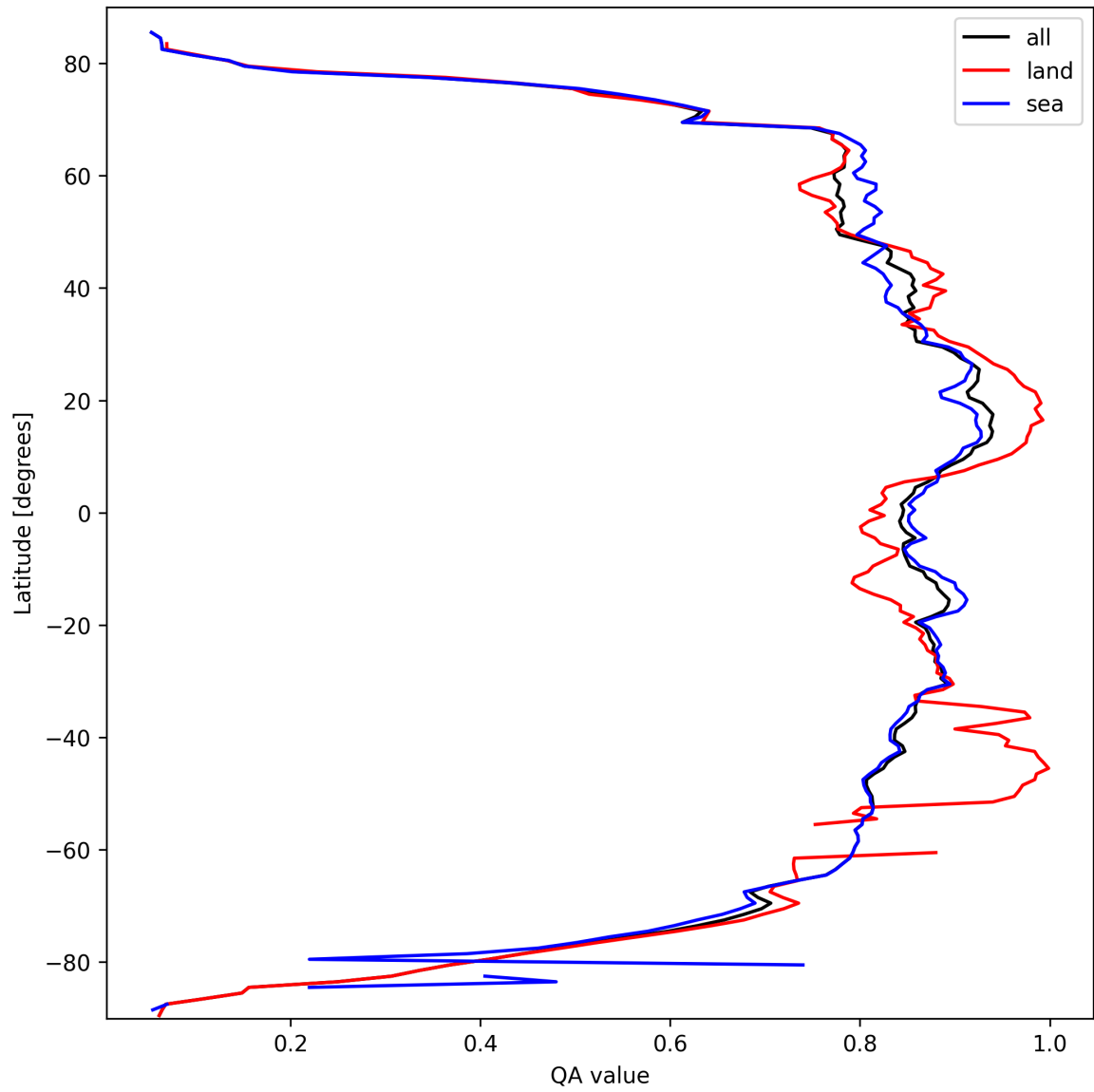
Figure 9: Zonal average of “QA value” for 2025-03-13 to 2025-03-14.
