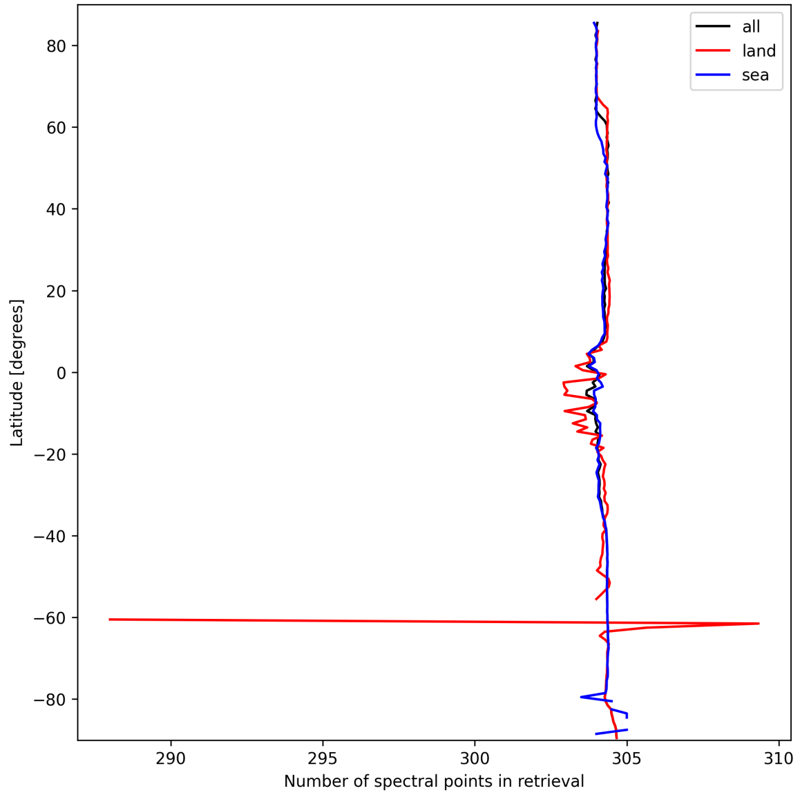
Figure 14: Zonal average of “Number of spectral points in retrieval” for 2025-03-13 to 2025-03-14.
