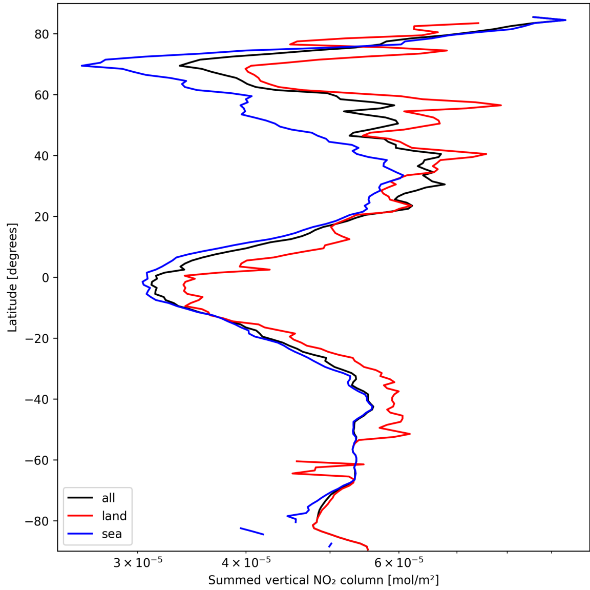
Figure 21: Zonal average of “Summed vertical NO 2 column” for 2025-03-13 to 2025-03-14.
