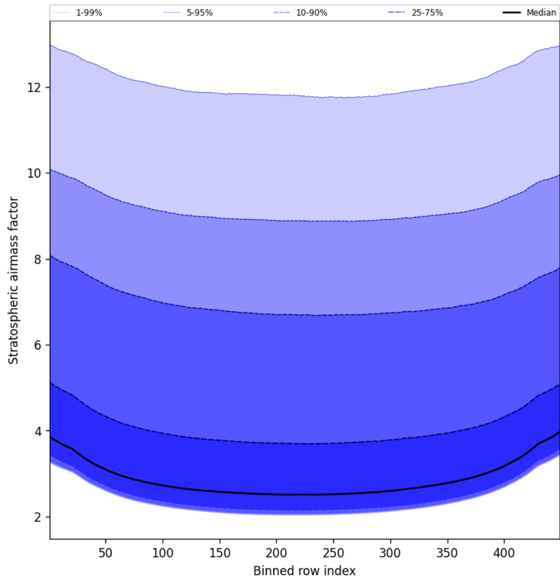
Figure 59: Along track statistics of “Stratospheric airmass factor” for 2025-03-13 to 2025-03-14
