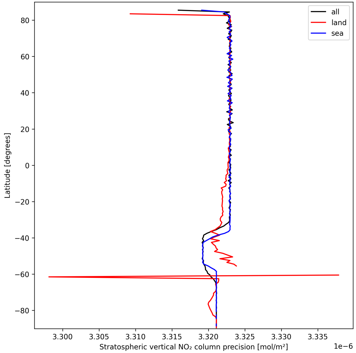
Figure 18: Zonal average of “Stratospheric vertical NO 2 column precision” for 2025-03-13 to 2025-03-14.
