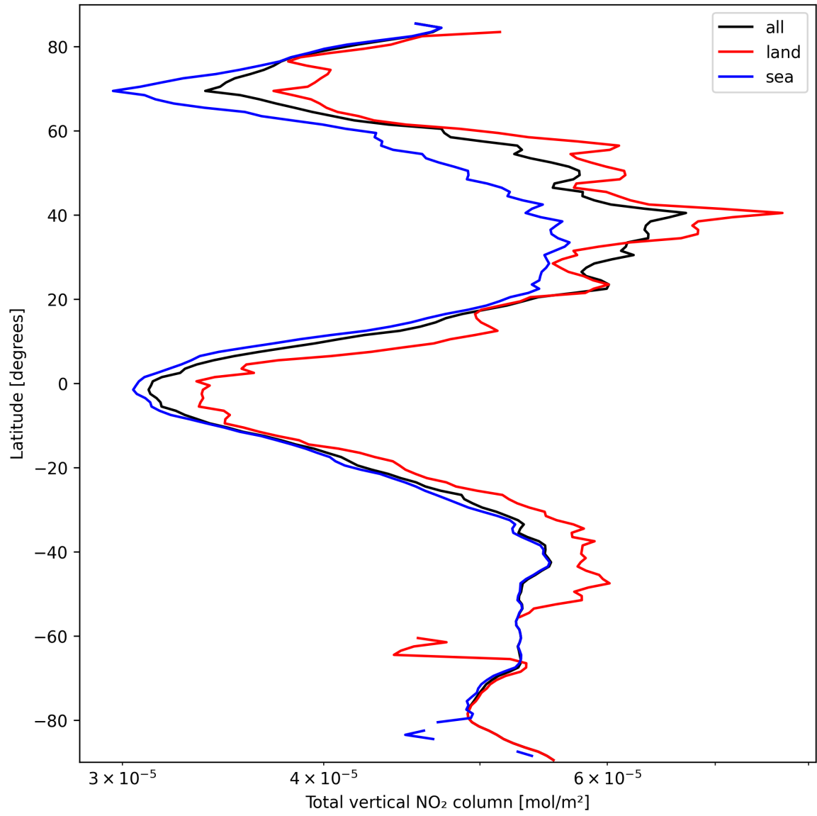
Figure 19: Zonal average of “Total vertical NO 2 column” for 2025-03-13 to 2025-03-14.
