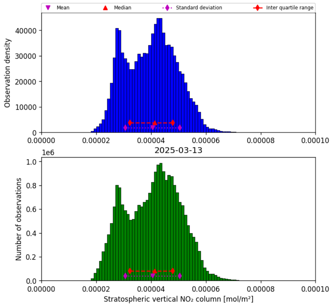
Figure 34: Histogram of “Stratospheric vertical NO 2 column” for 2025-03-13 to 2025-03-14
