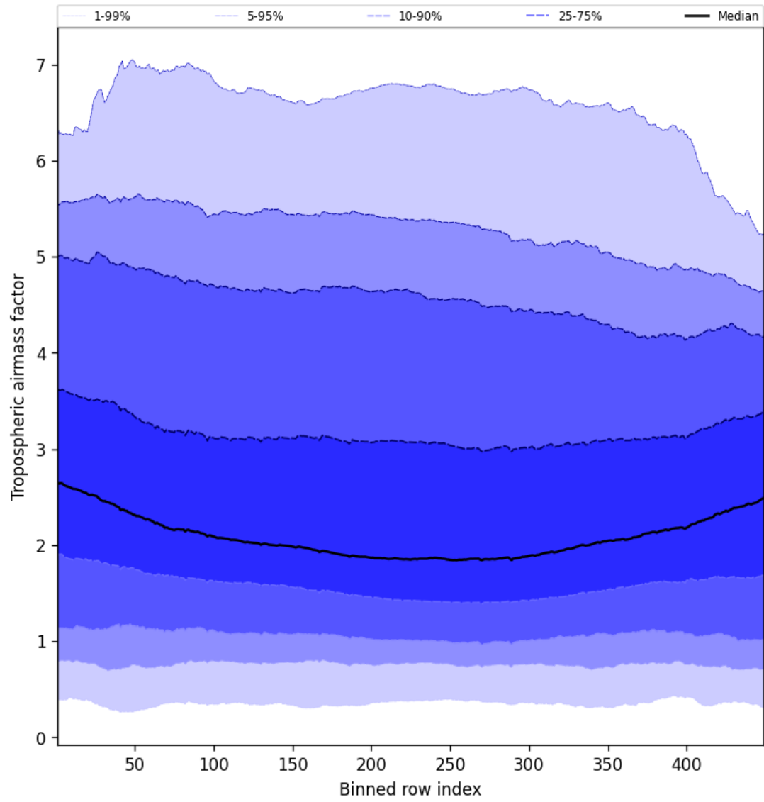
Figure 46: Along track statistics of “Tropospheric air mass factor” for 2025-03-13 to 2025-03-14
