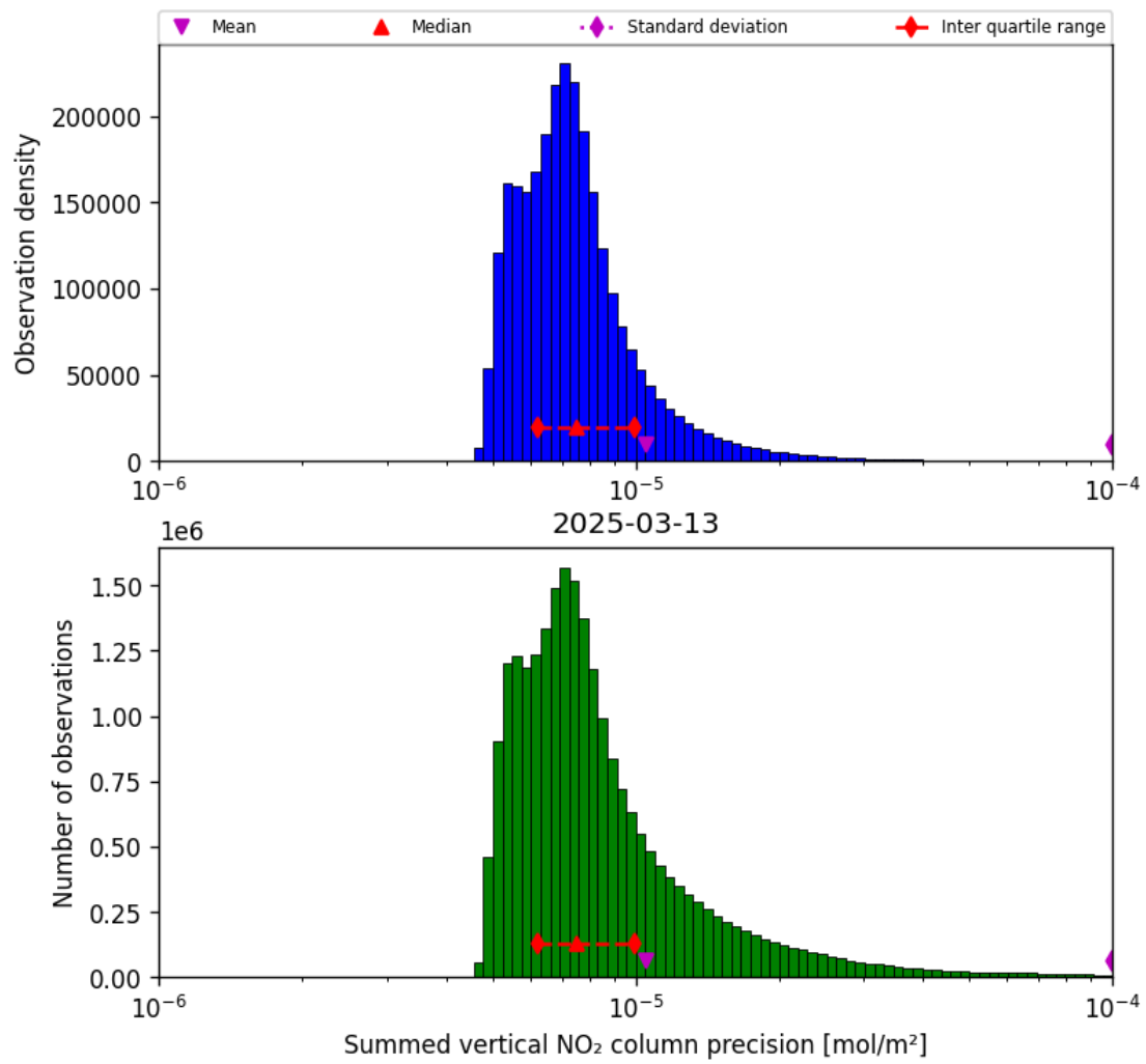
Figure 39: Histogram of "Summed vertical NO 2 column precision" for 2025-03-13 to 2025-03-14
