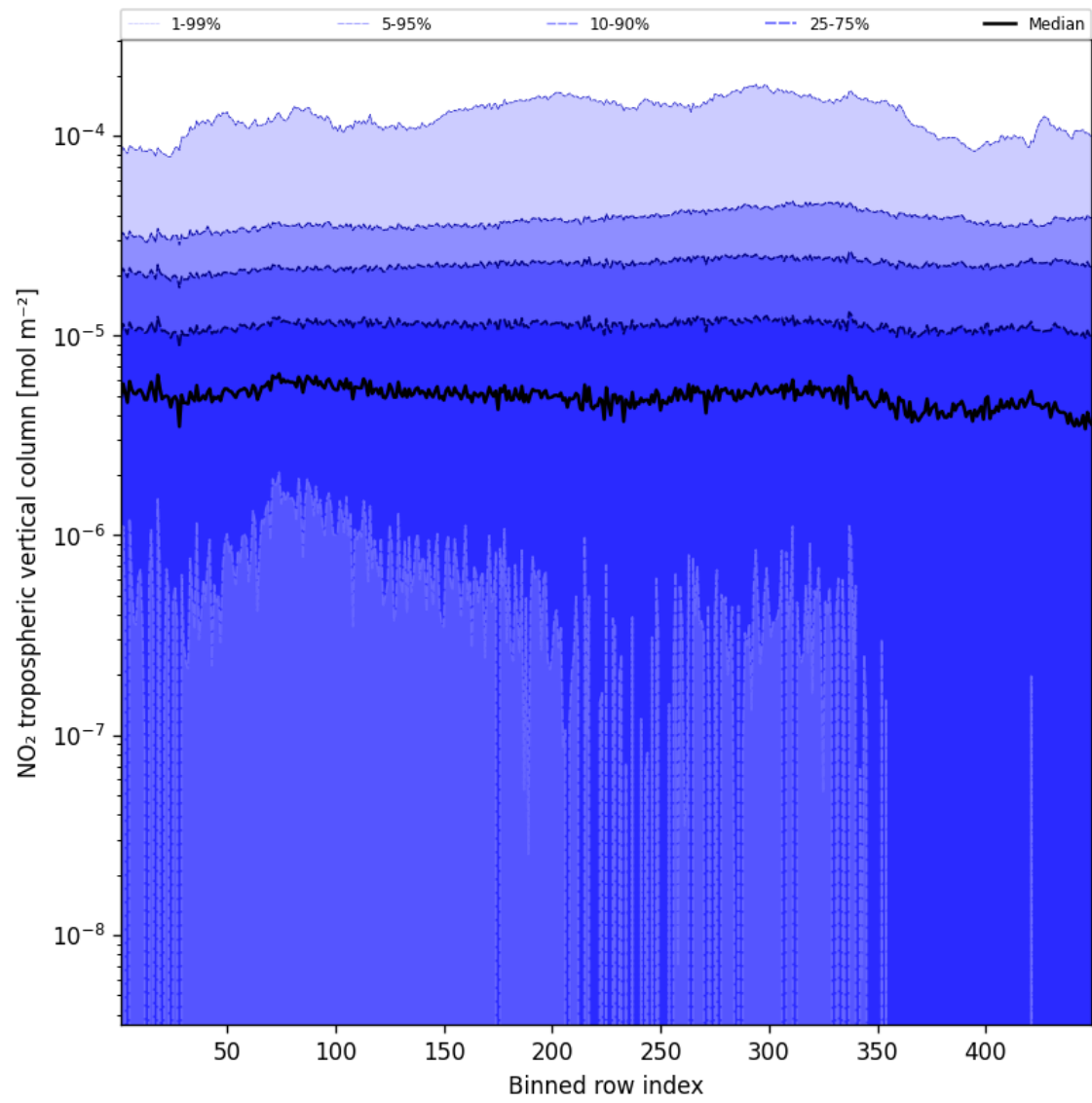
Figure 44: Along track statistics of “NO 2 tropospheric vertical column” for 2025-03-13 to 2025-03-14
