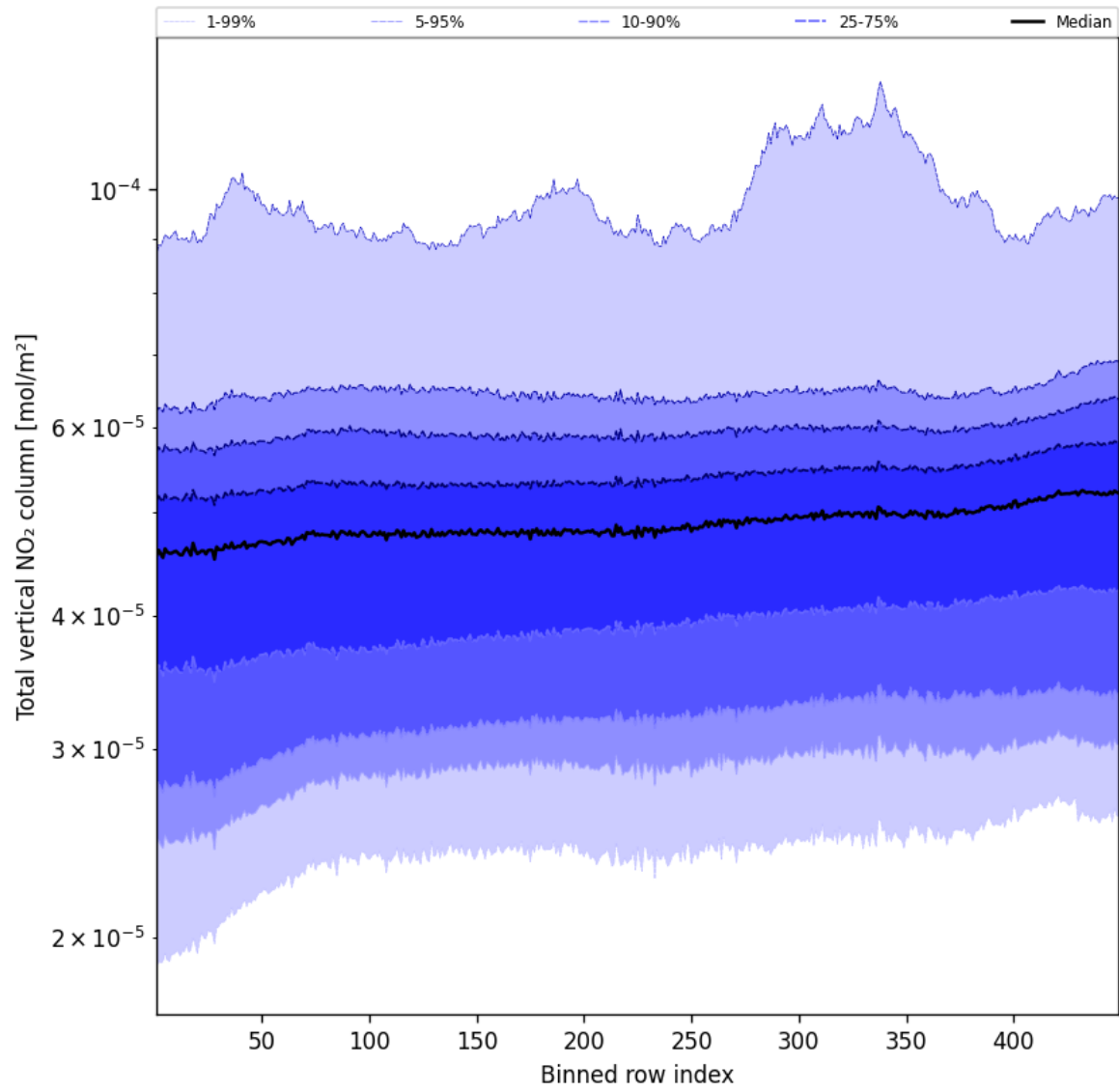
Figure 53: Along track statistics of “Total vertical NO 2 column” for 2025-03-13 to 2025-03-14
