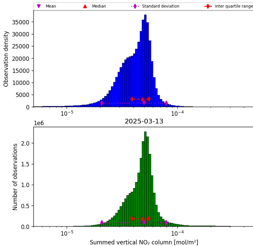
Figure 38: Histogram of “Summed vertical NO 2 column” for 2025-03-13 to 2025-03-14
