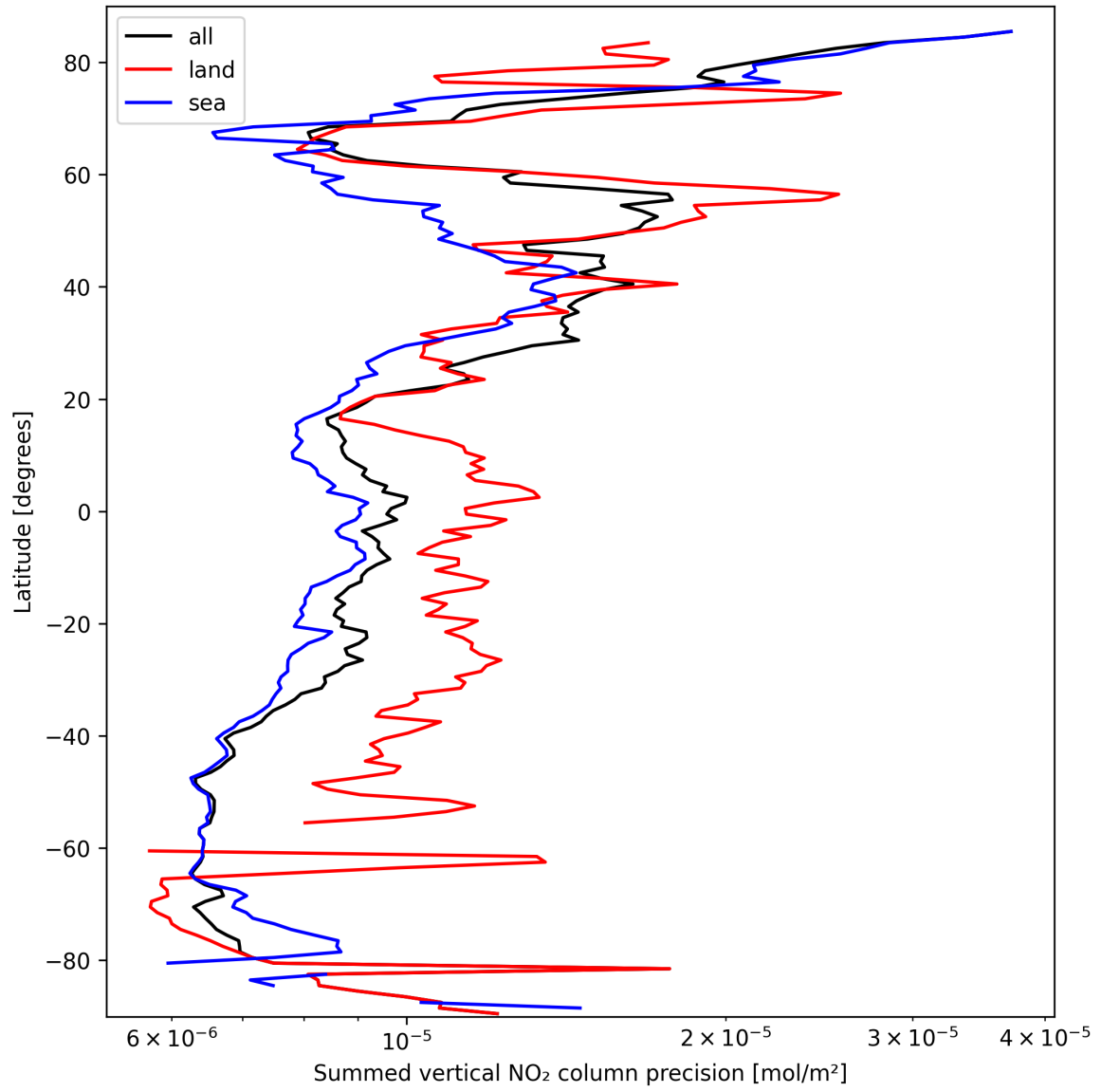
Figure 22: Zonal average of “Summed vertical NO 2 column precision” for 2025-03-13 to 2025-03-14.
