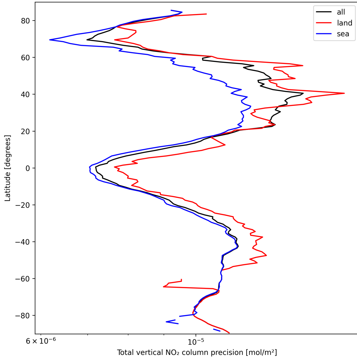
Figure 20: Zonal average of “Total vertical NO 2 column precision” for 2025-03-13 to 2025-03-14.
