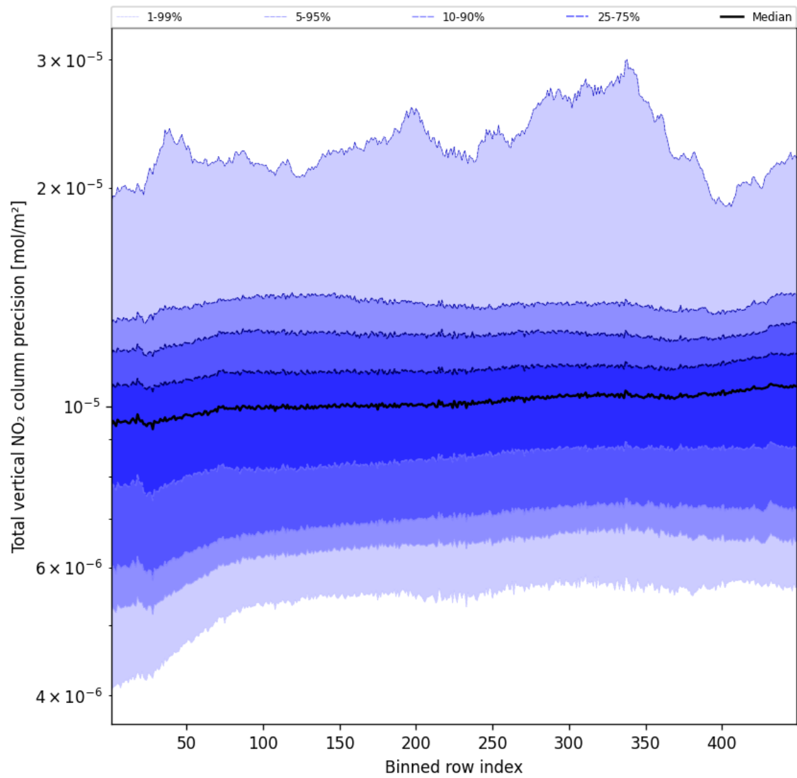
Figure 54: Along track statistics of “Total vertical NO 2 column precision” for 2025-03-13 to 2025-03-14
