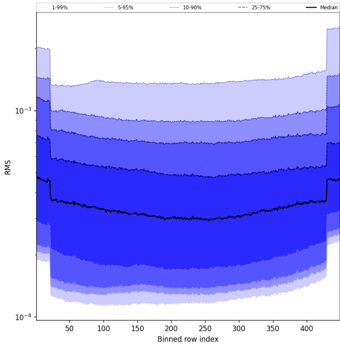
Figure 58: Along track statistics of “RMS” for 2025-03-13 to 2025-03-14
