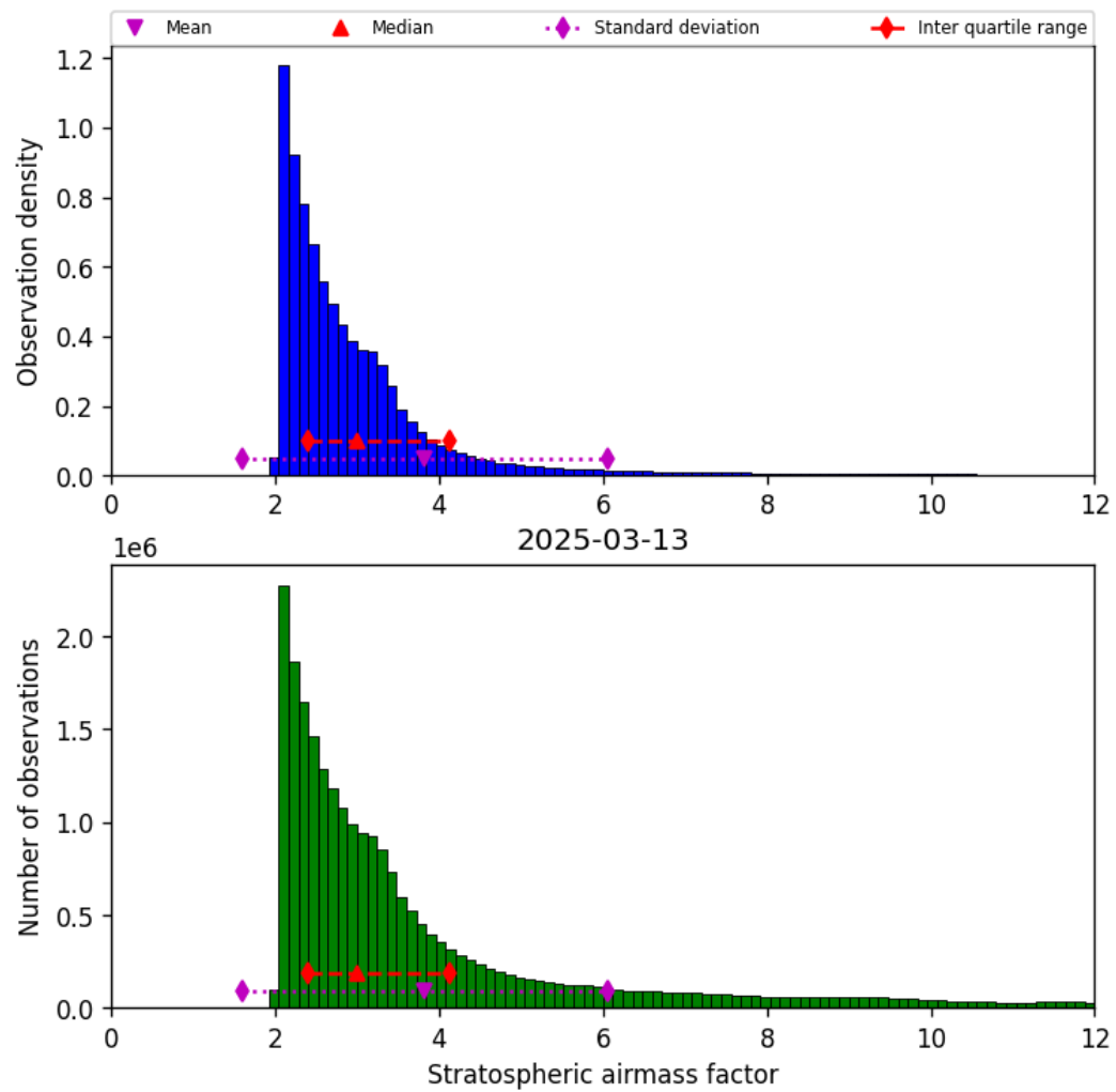
Figure 42: Histogram of “Stratospheric airmass factor” for 2025-03-13 to 2025-03-14
