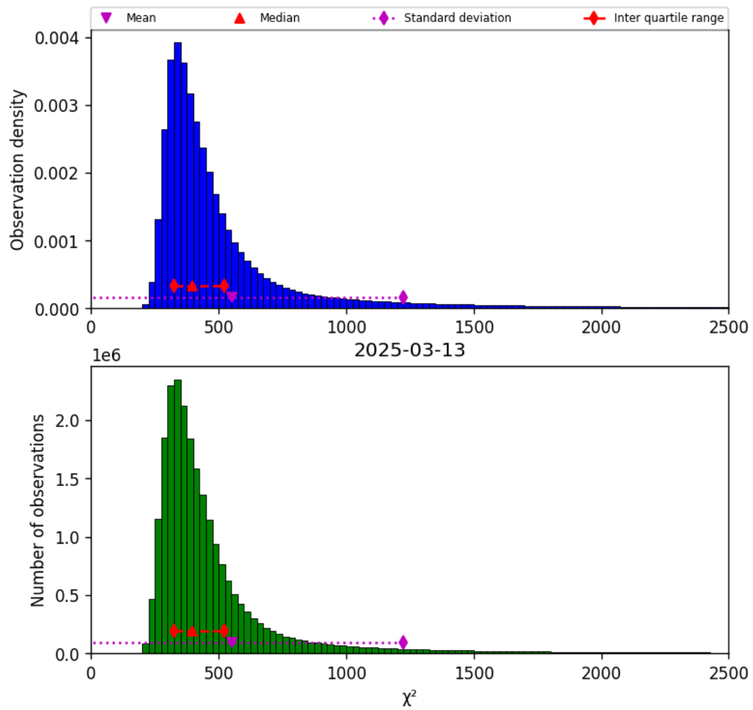
Figure 40: Histogram of “ \chi^2 ” for 2025-03-13 to 2025-03-14
