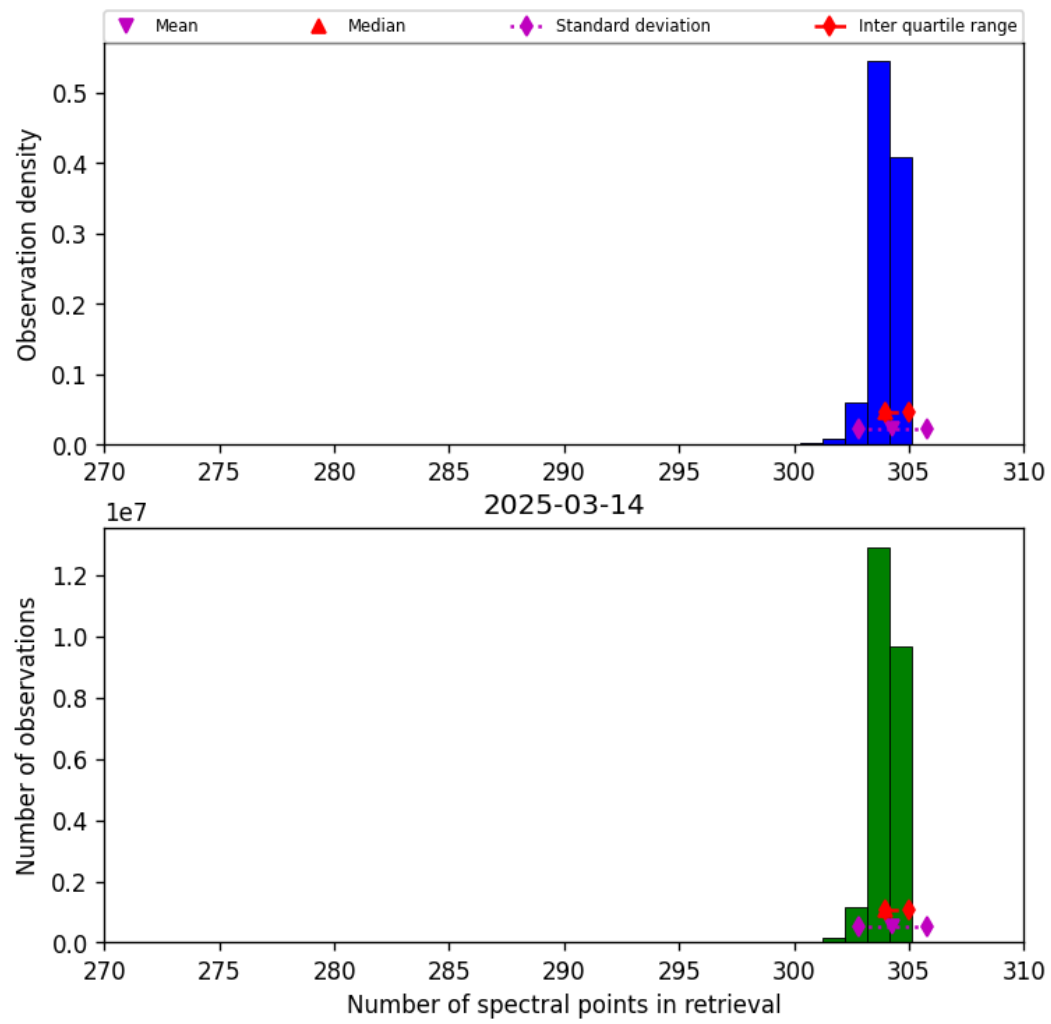
Figure 31: Histogram of “Number of spectral points in retrieval” for 2025-03-14 to 2025-03-15
