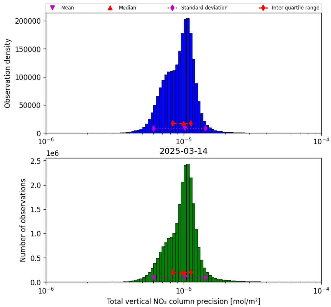
Figure 37: Histogram of “Total vertical NO 2 column precision” for 2025-03-14 to 2025-03-15
