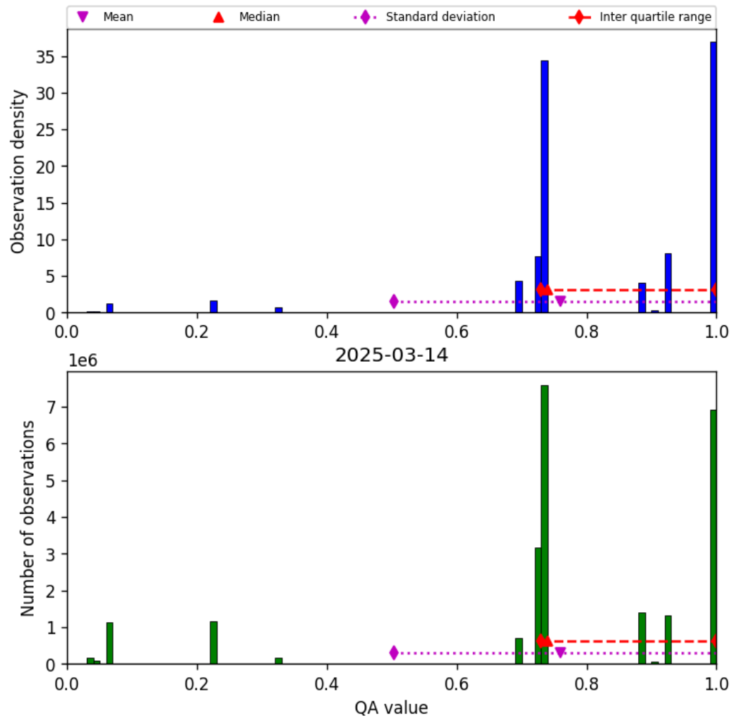
Figure 26: Histogram of “QA value” for 2025-03-14 to 2025-03-15
