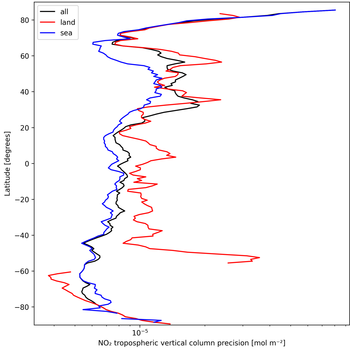
Figure 11: Zonal average of “NO 2 tropospheric vertical column precision” for 2025-03-14 to 2025-03-15.
