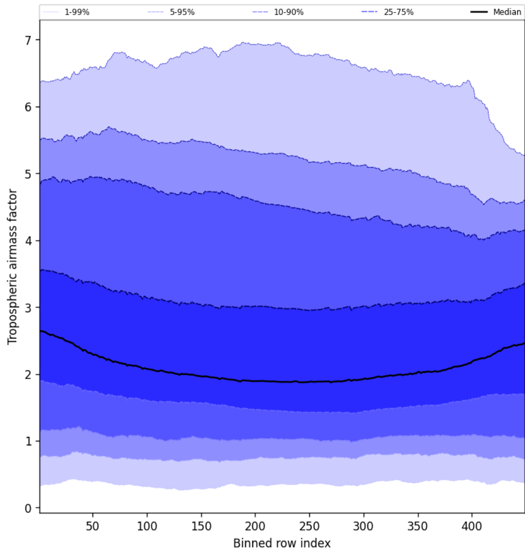
Figure 46: Along track statistics of “Tropospheric air mass factor” for 2025-03-14 to 2025-03-15
