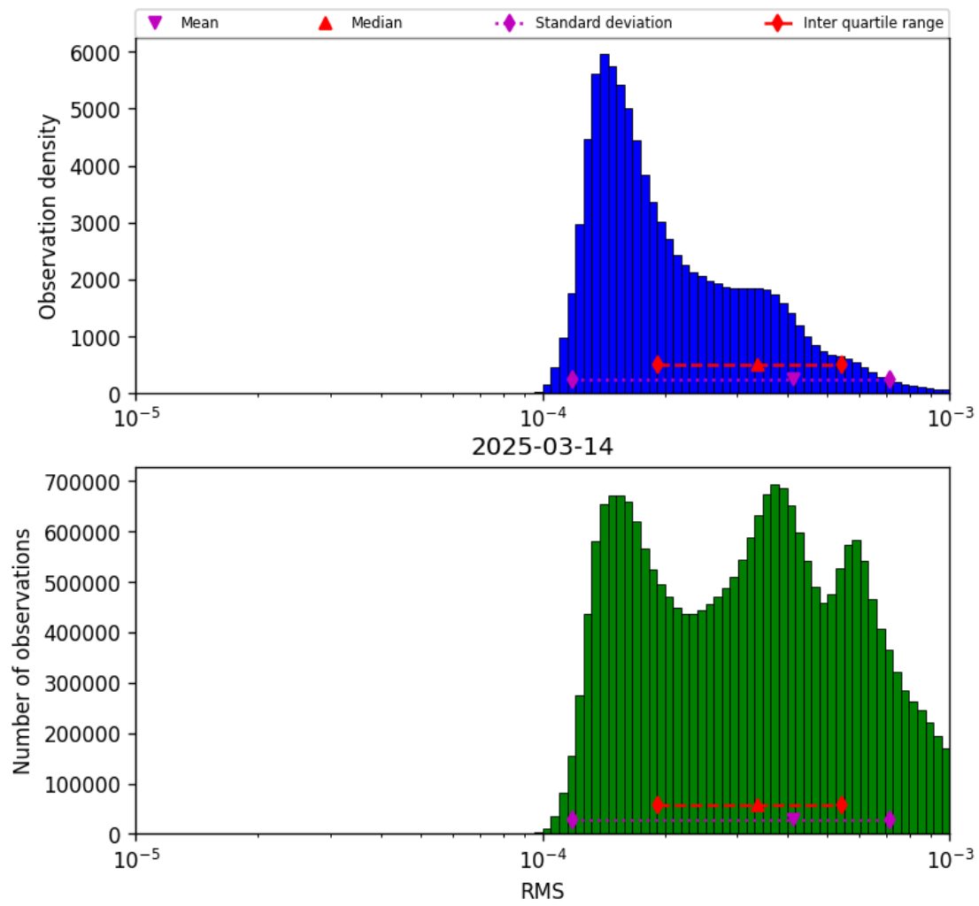
Figure 41: Histogram of “RMS” for 2025-03-14 to 2025-03-15
