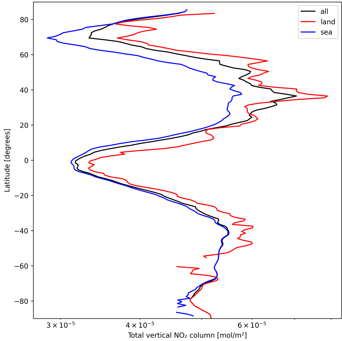
Figure 19: Zonal average of “Total vertical NO 2 column” for 2025-03-14 to 2025-03-15.
