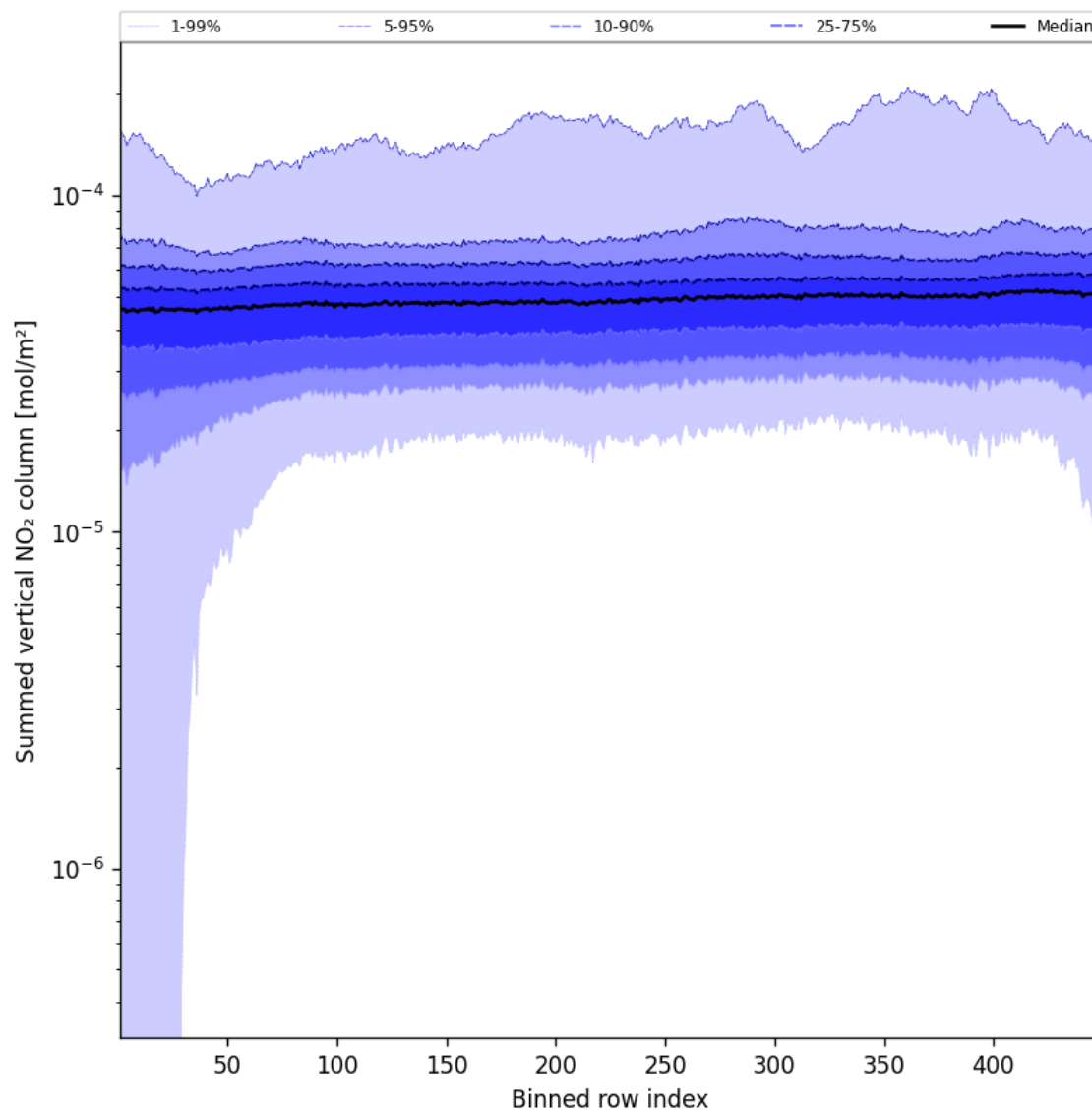
Figure 55: Along track statistics of “Summed vertical NO 2 column” for 2025-03-14 to 2025-03-15
