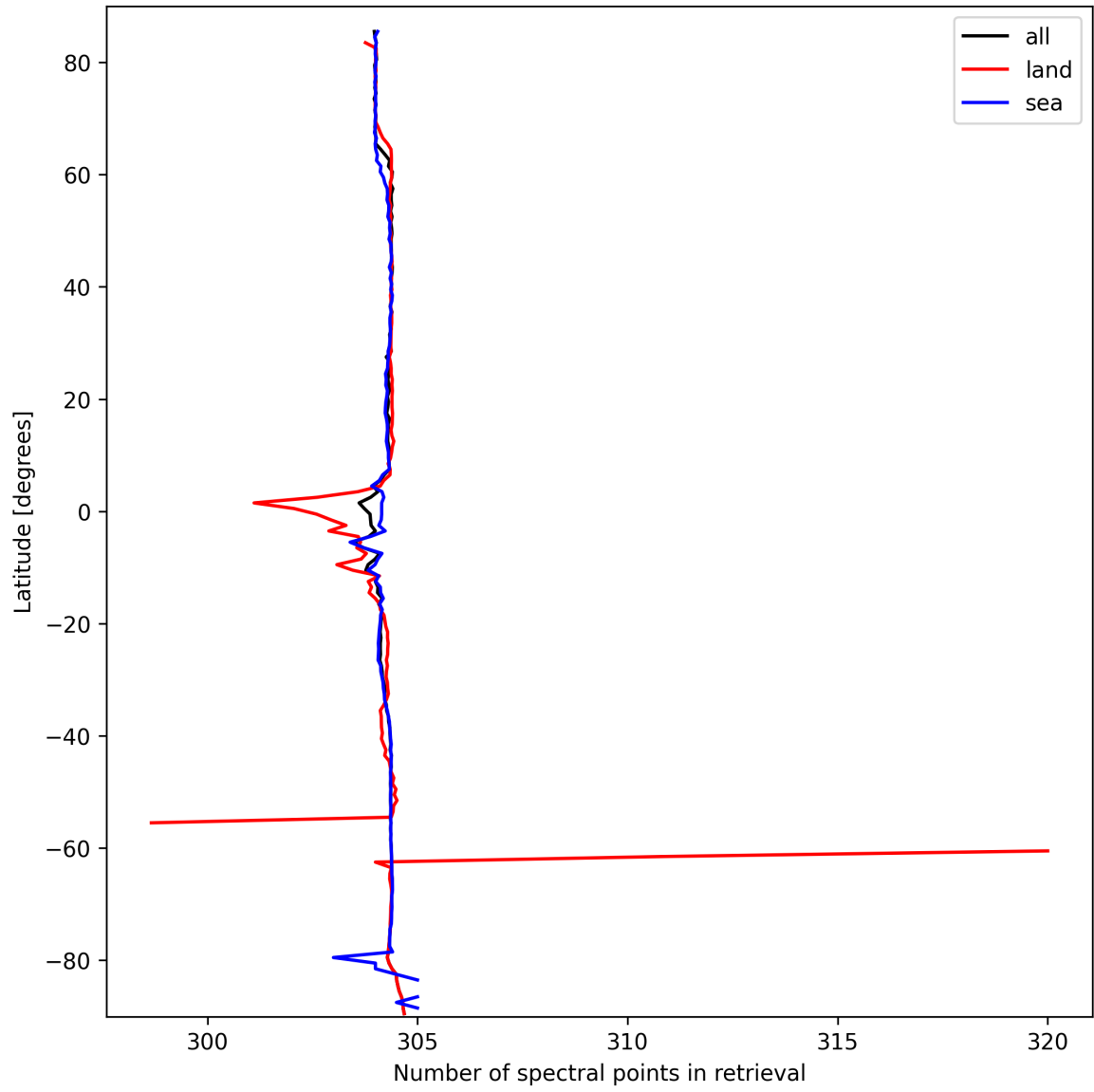
Figure 14: Zonal average of “Number of spectral points in retrieval” for 2025-03-14 to 2025-03-15.
