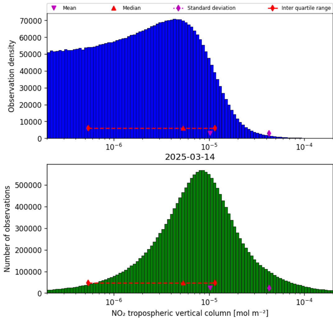
Figure 27: Histogram of “NO 2 tropospheric vertical column” for 2025-03-14 to 2025-03-15
