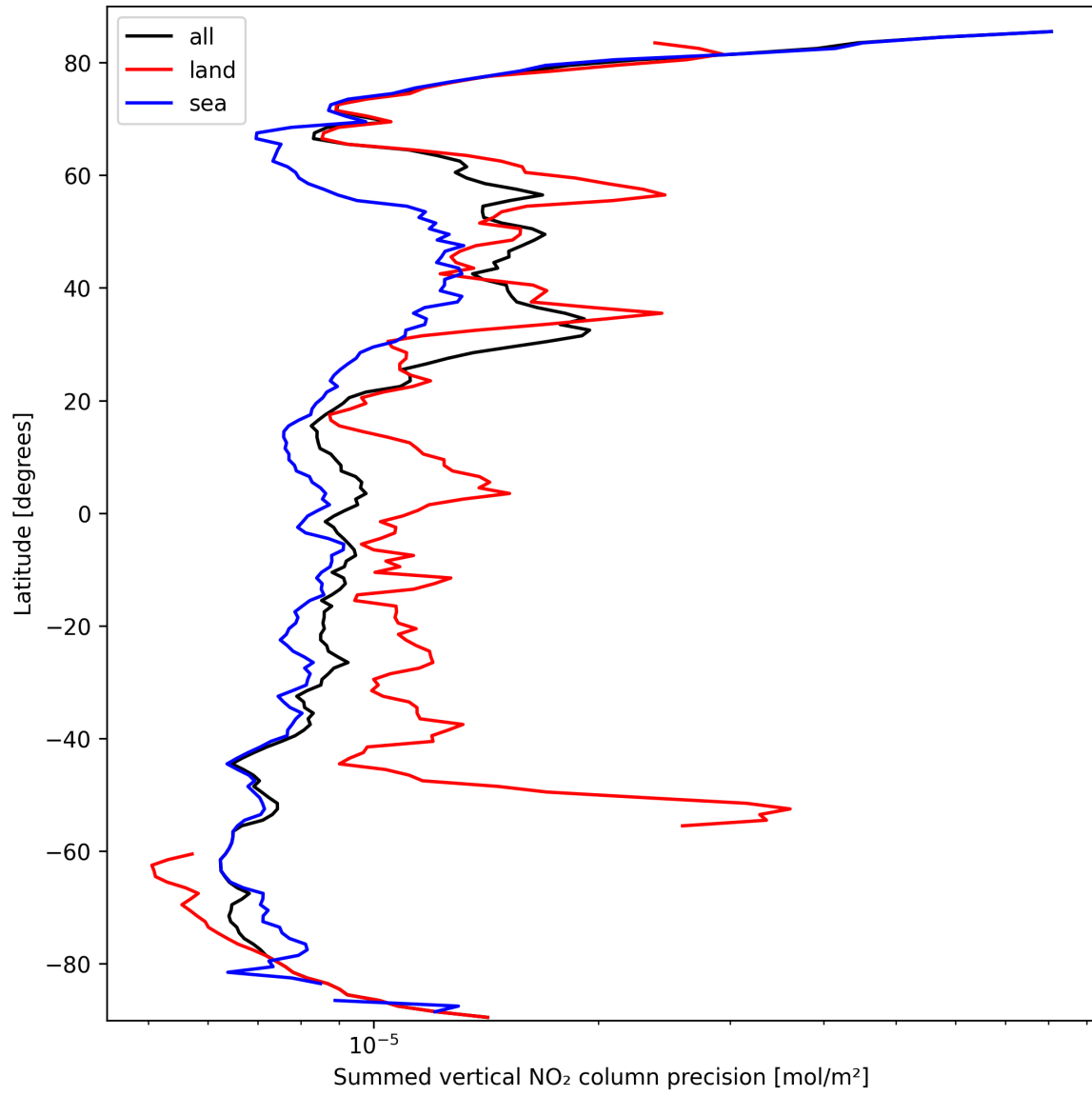
Figure 22: Zonal average of “Summed vertical NO 2 column precision” for 2025-03-14 to 2025-03-15.
