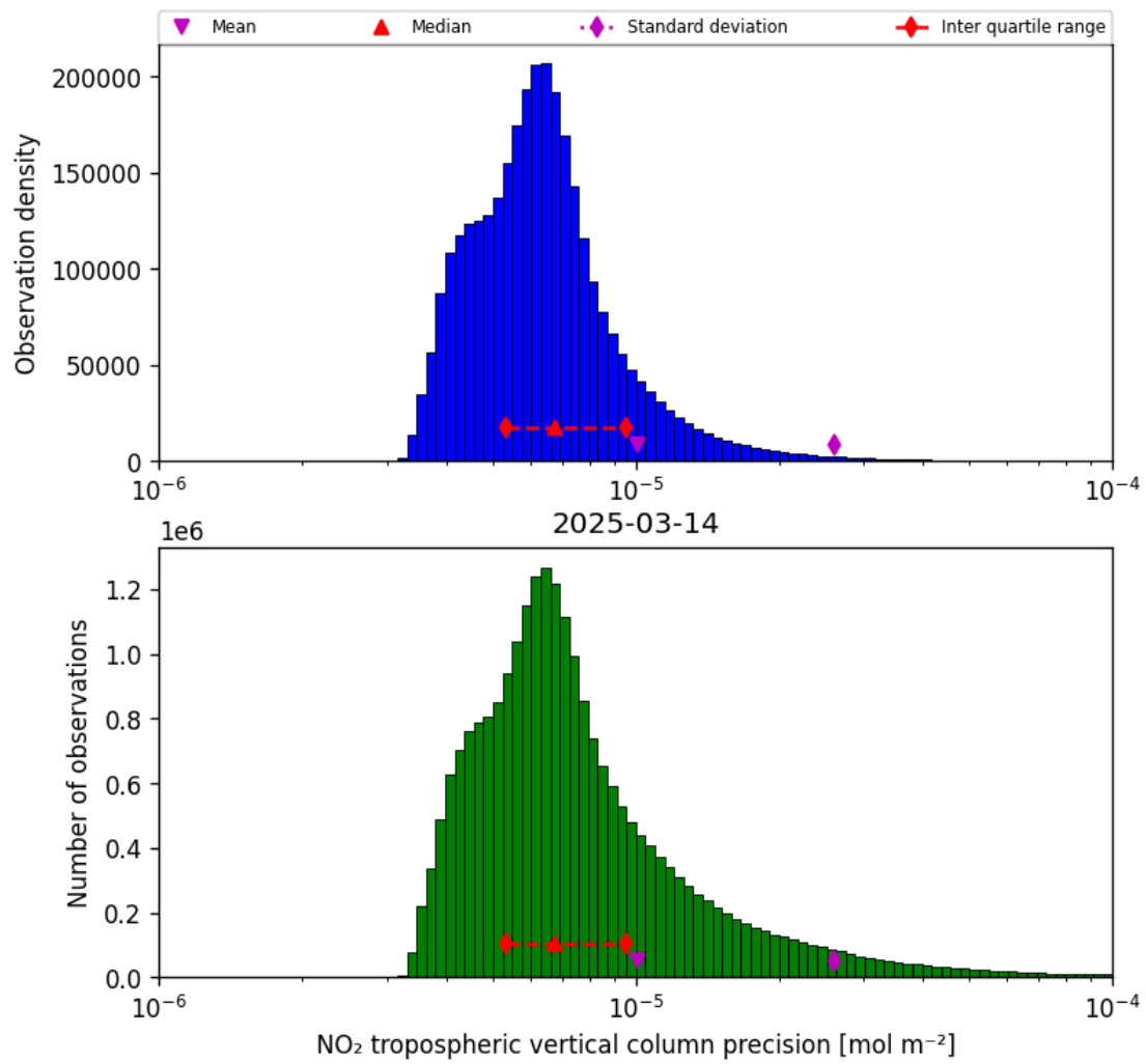
Figure 28: Histogram of “NO 2 tropospheric vertical column precision” for 2025-03-14 to 2025-03-15
