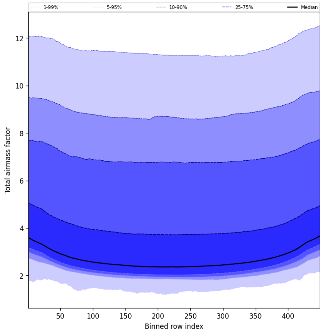
Figure 47: Along track statistics of “Total airmass factor” for 2025-03-14 to 2025-03-15
