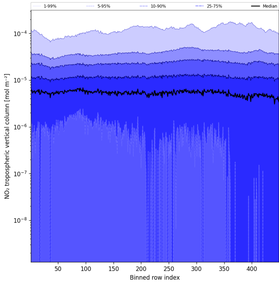
Figure 44: Along track statistics of “NO 2 tropospheric vertical column” for 2025-03-14 to 2025-03-15
