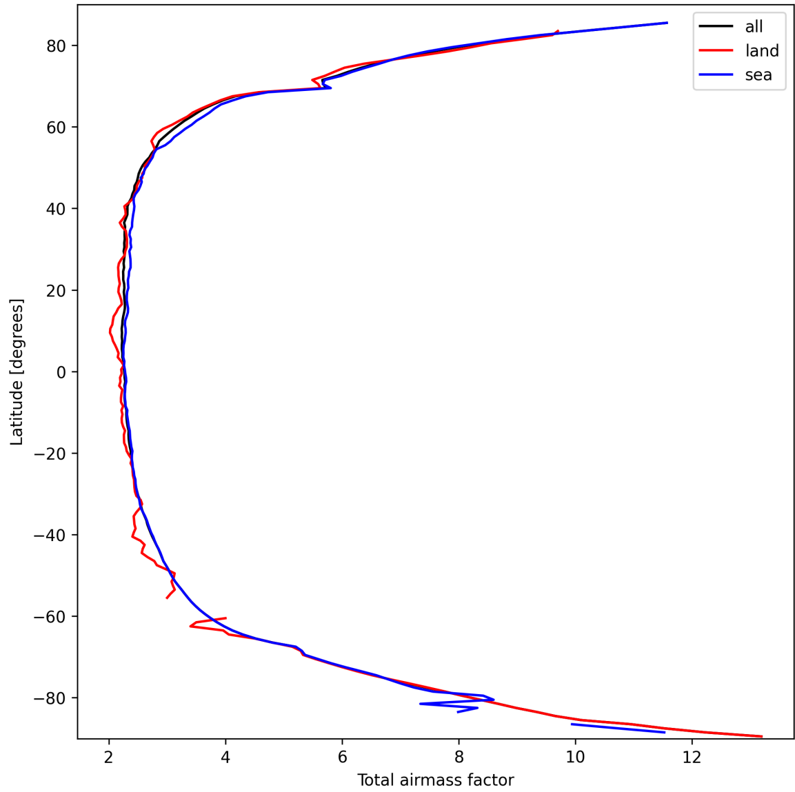
Figure 13: Zonal average of “Total airmass factor” for 2025-03-14 to 2025-03-15.
