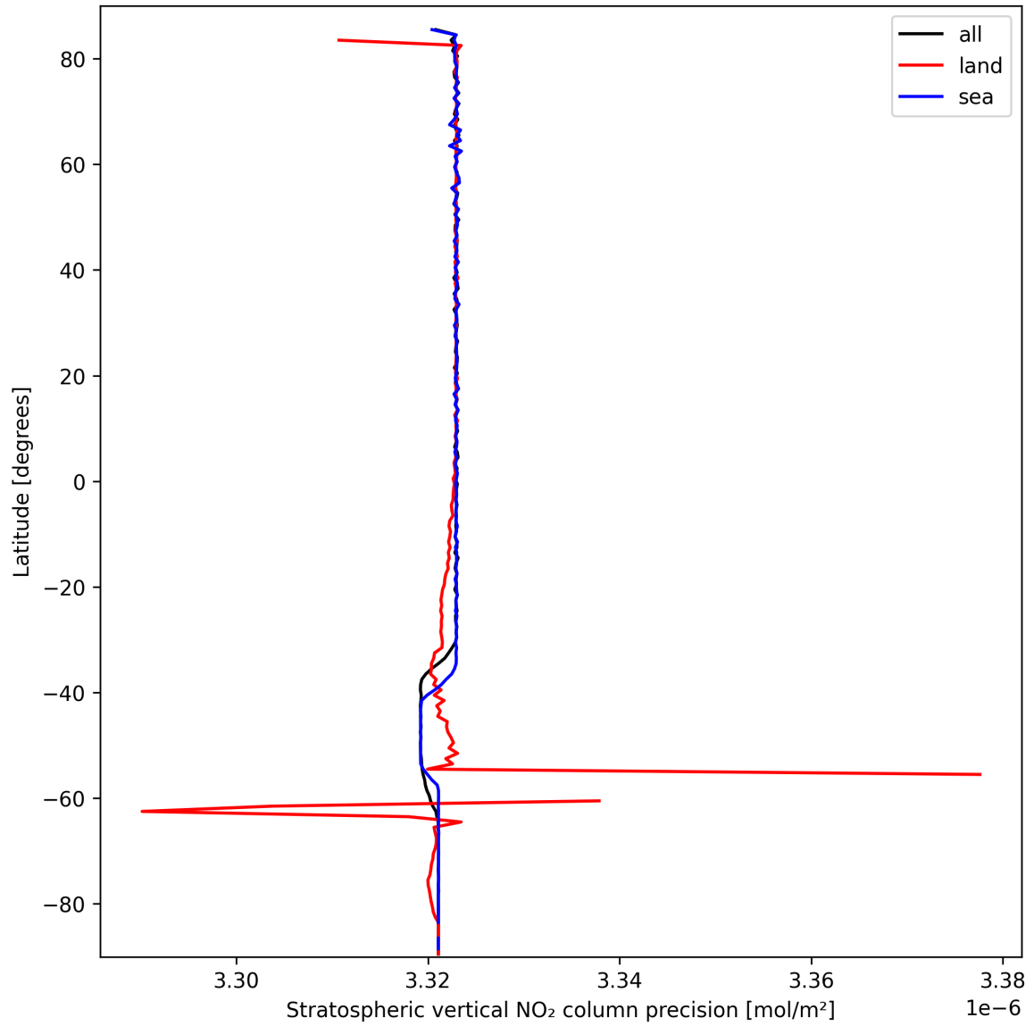
Figure 18: Zonal average of “Stratospheric vertical NO 2 column precision” for 2025-03-14 to 2025-03-15.
