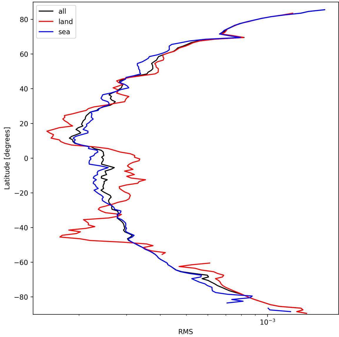
Figure 24: Zonal average of “RMS” for 2025-03-14 to 2025-03-15.
