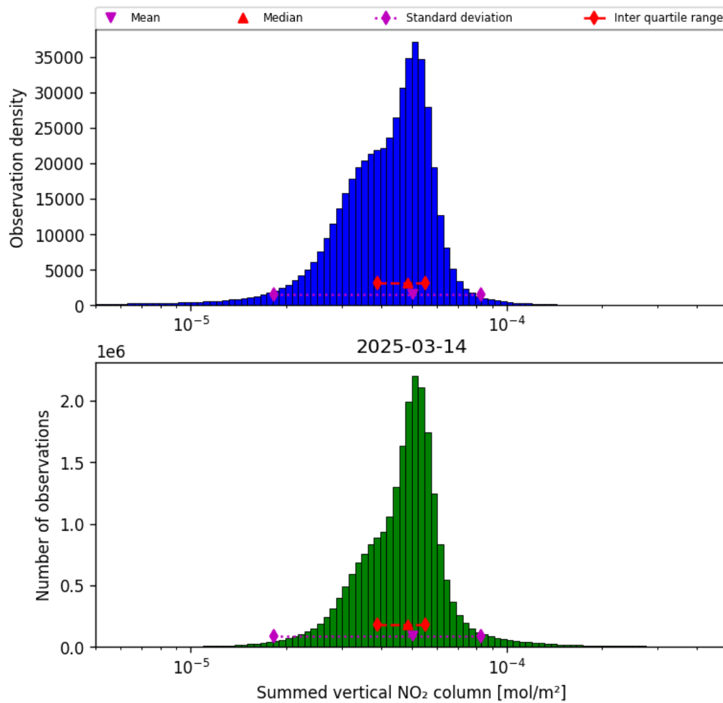
Figure 38: Histogram of “Summed vertical NO 2 column” for 2025-03-14 to 2025-03-15
