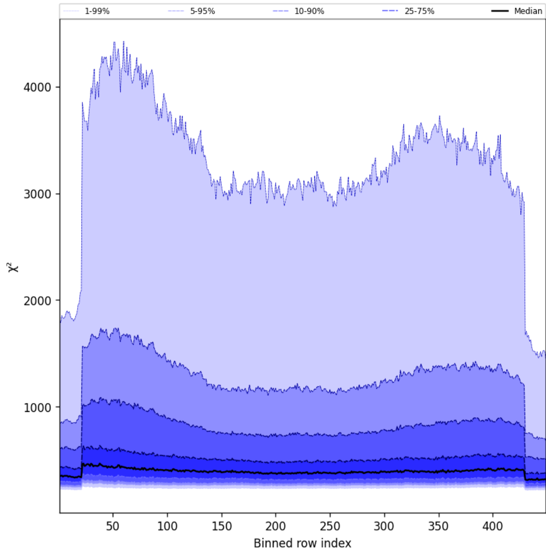
Figure 57: Along track statistics of “ \chi^2 ” for 2025-03-14 to 2025-03-15
