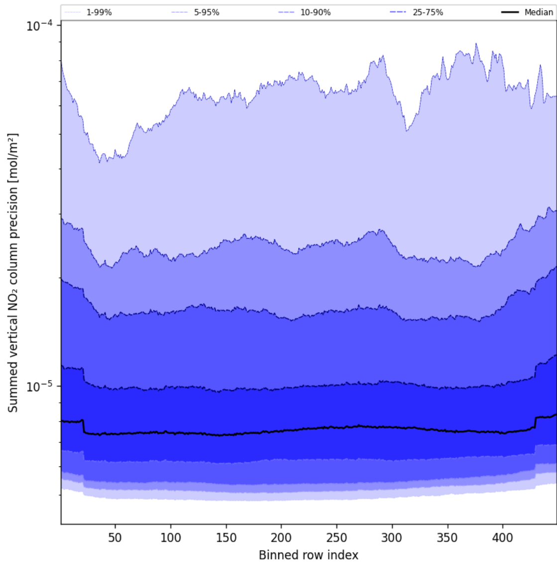
Figure 56: Along track statistics of “Summed vertical NO 2 column precision” for 2025-03-14 to 2025-03-15
