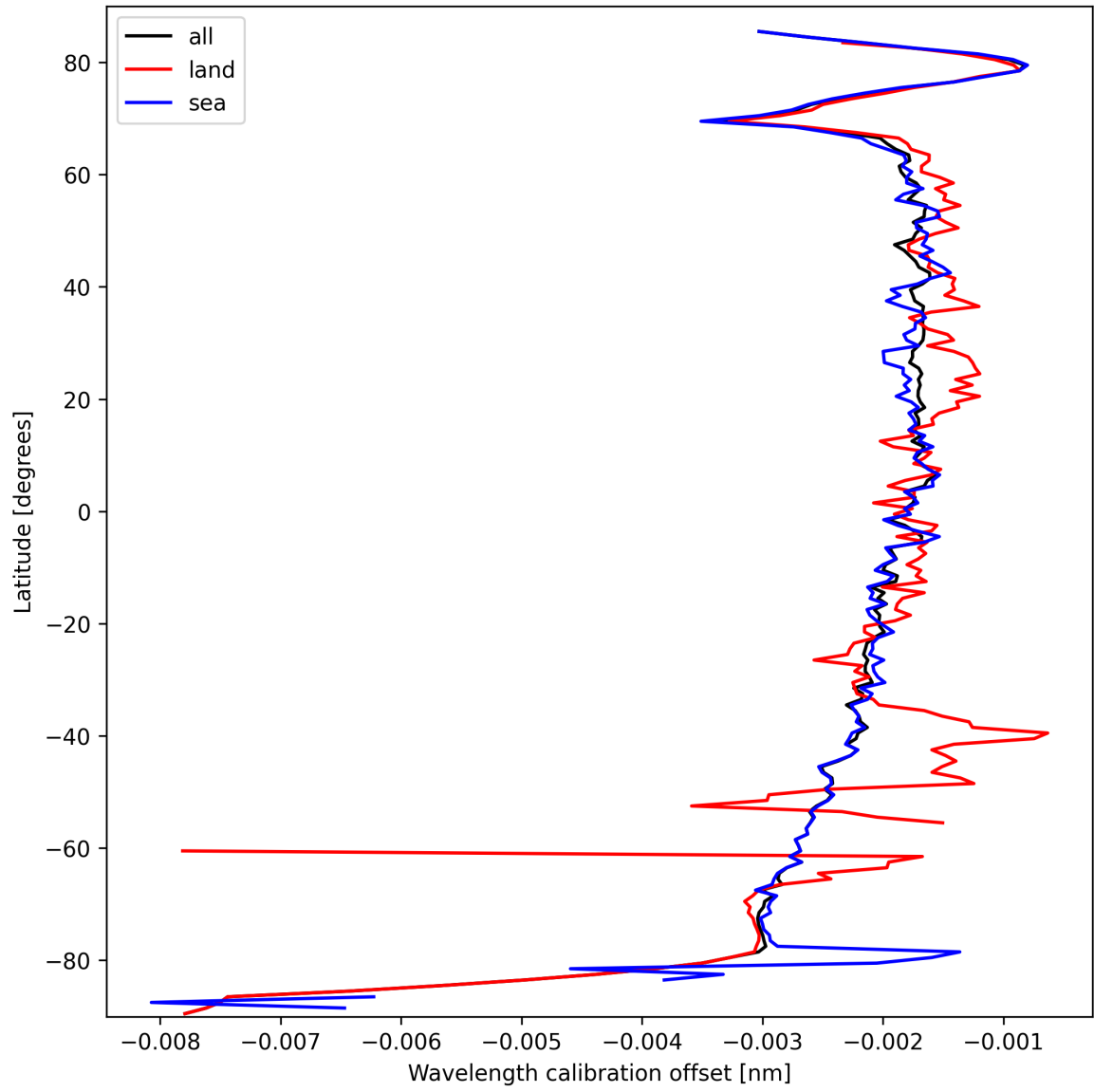
Figure 16: Zonal average of “Wavelength calibration offset” for 2025-03-14 to 2025-03-15.
