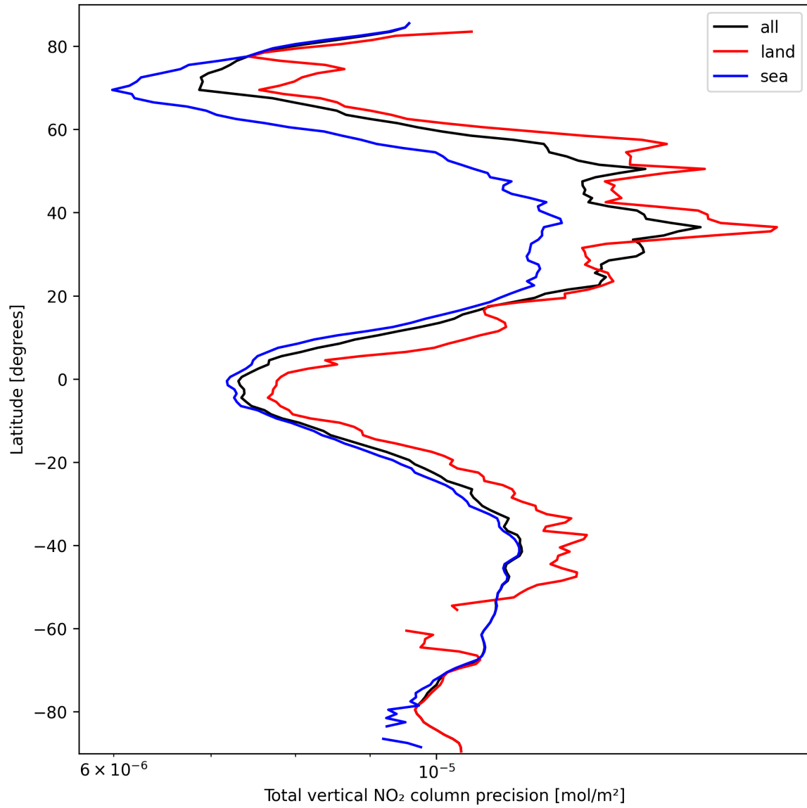
Figure 20: Zonal average of “Total vertical NO 2 column precision” for 2025-03-14 to 2025-03-15.
