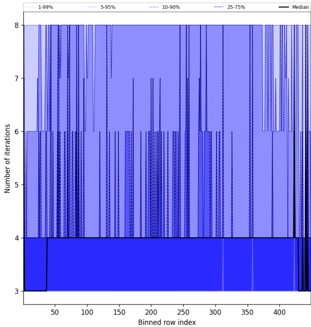
Figure 49: Along track statistics of “Number of iterations” for 2025-03-14 to 2025-03-15
