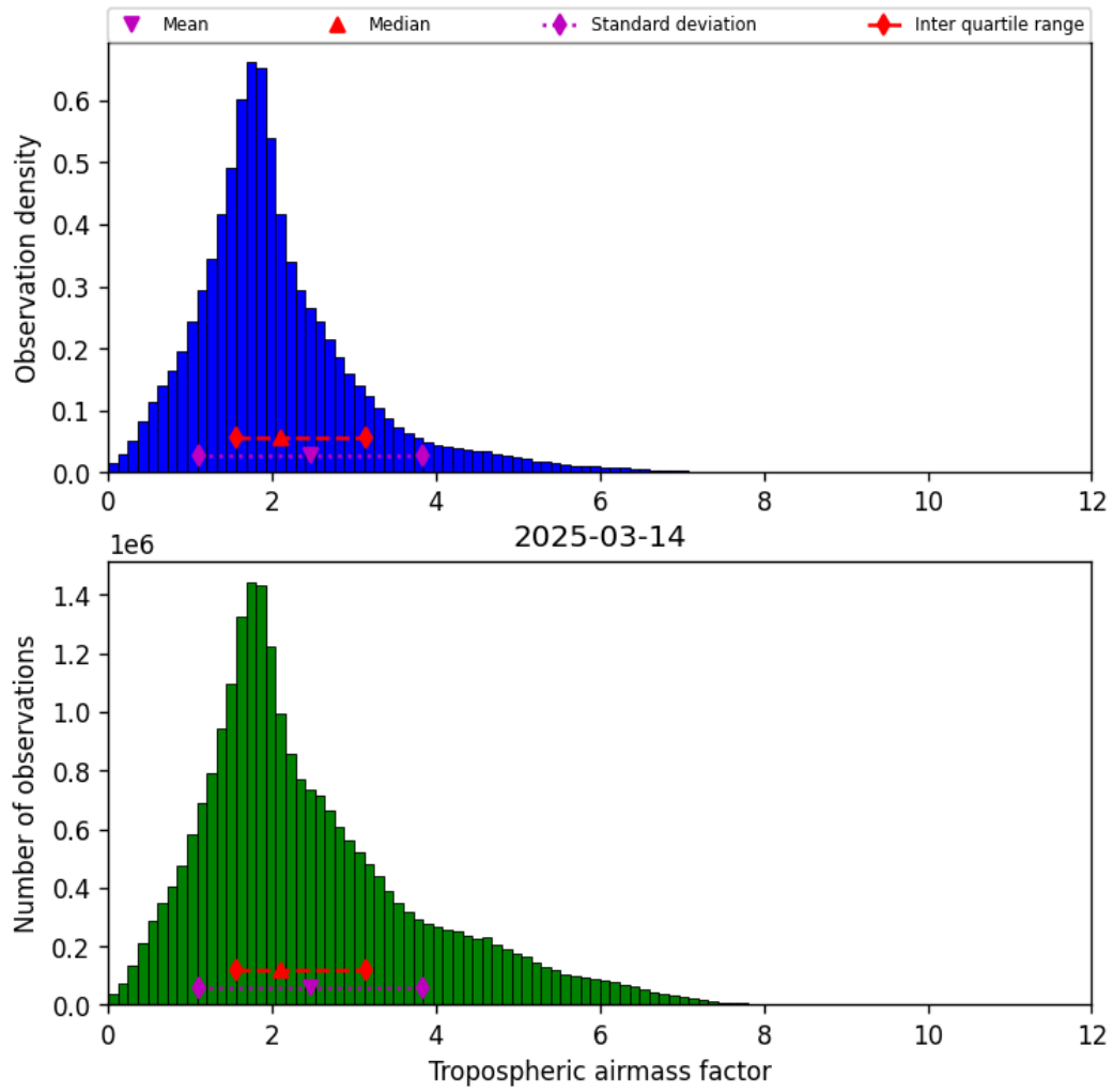
Figure 29: Histogram of “Tropospheric airmass factor” for 2025-03-14 to 2025-03-15
