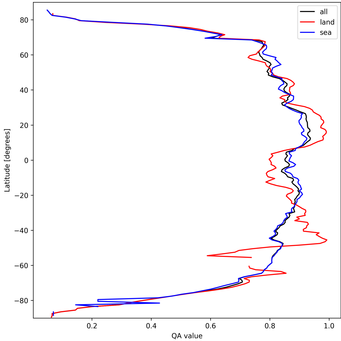
Figure 9: Zonal average of “QA value” for 2025-03-14 to 2025-03-15.
