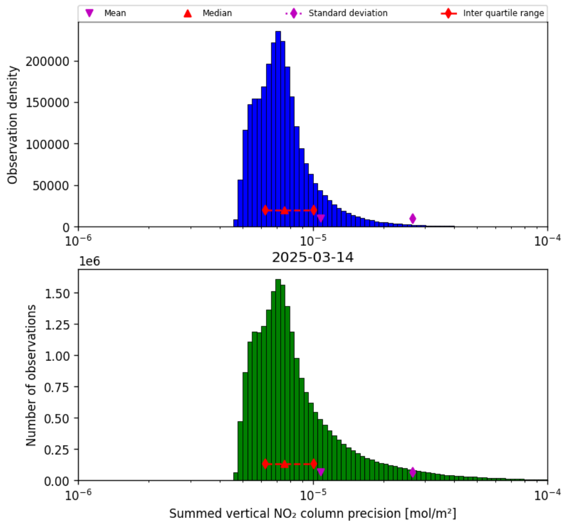
Figure 39: Histogram of “Summed vertical NO 2 column precision” for 2025-03-14 to 2025-03-15
