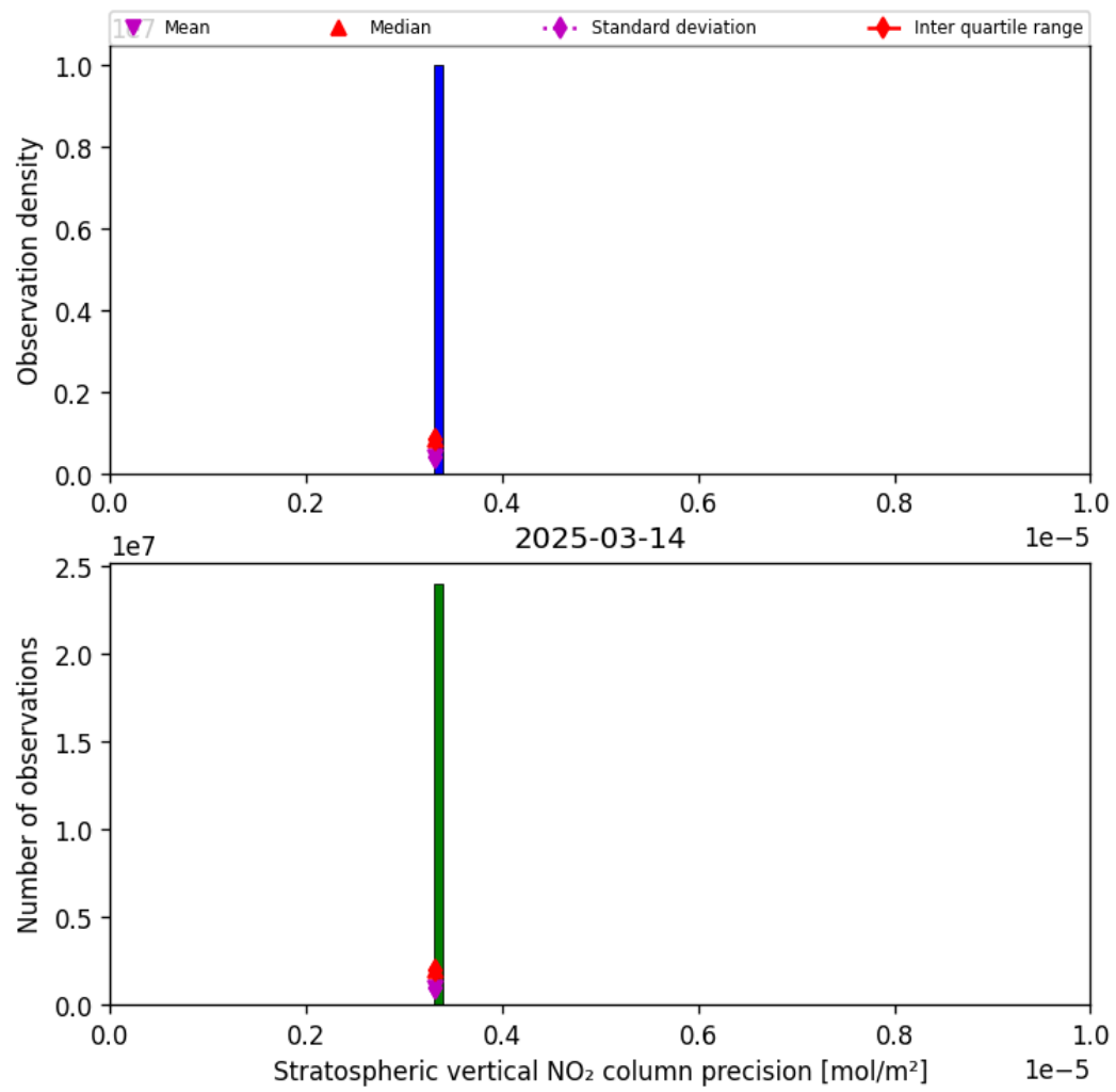
Figure 35: Histogram of “Stratospheric vertical NO 2 column precision” for 2025-03-14 to 2025-03-15
