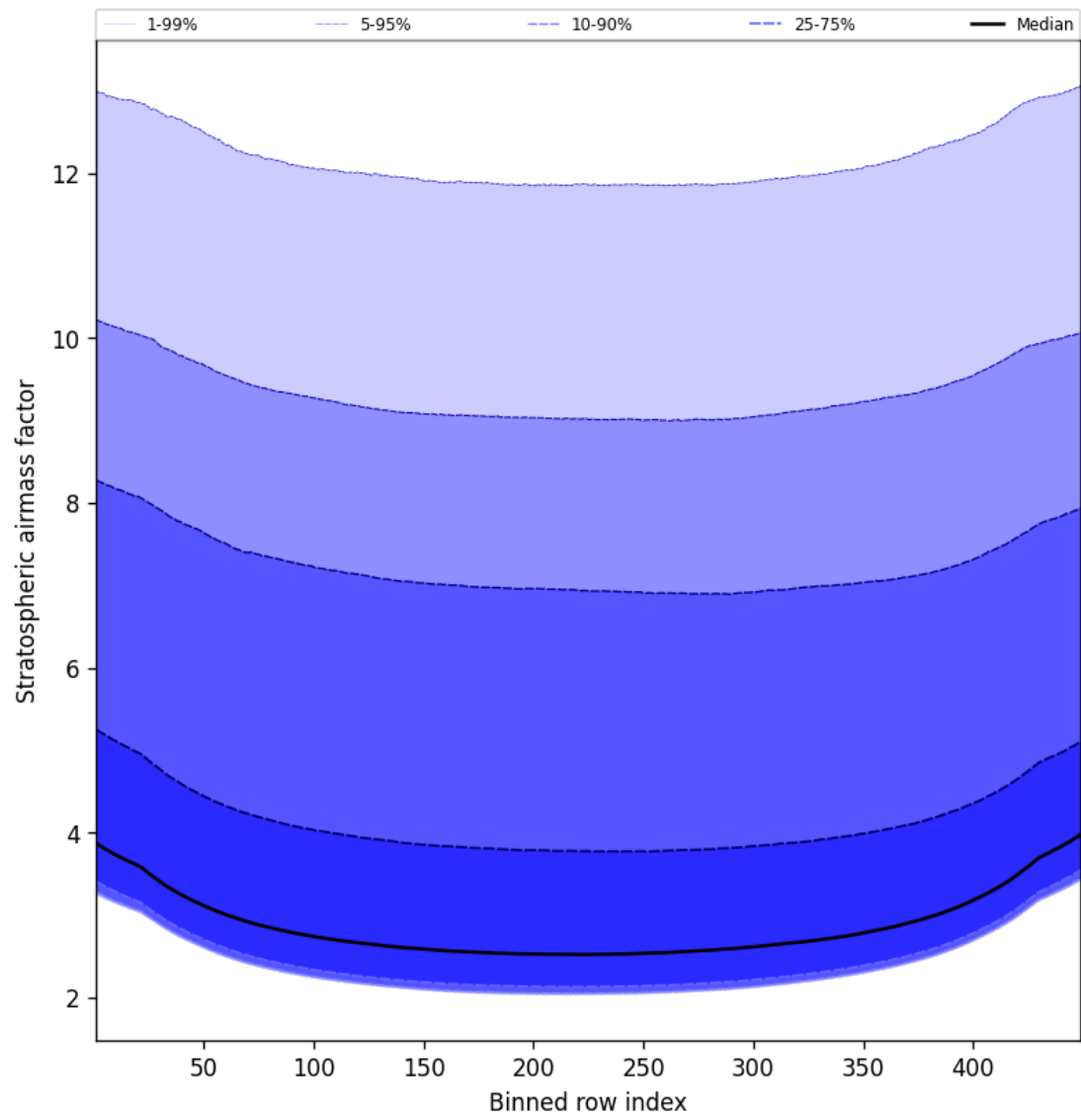
Figure 59: Along track statistics of “Stratospheric airmass factor” for 2025-03-14 to 2025-03-15
