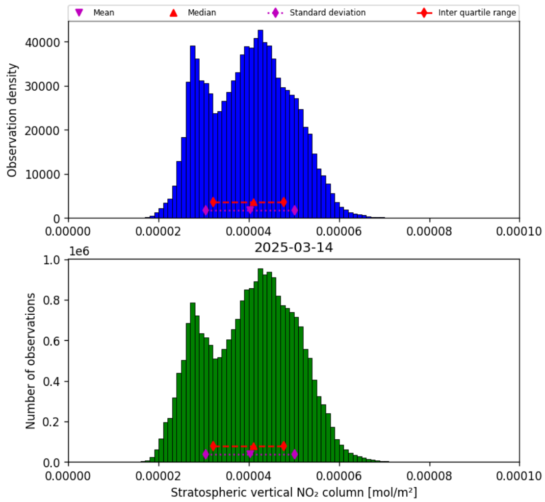
Figure 34: Histogram of “Stratospheric vertical NO 2 column” for 2025-03-14 to 2025-03-15
