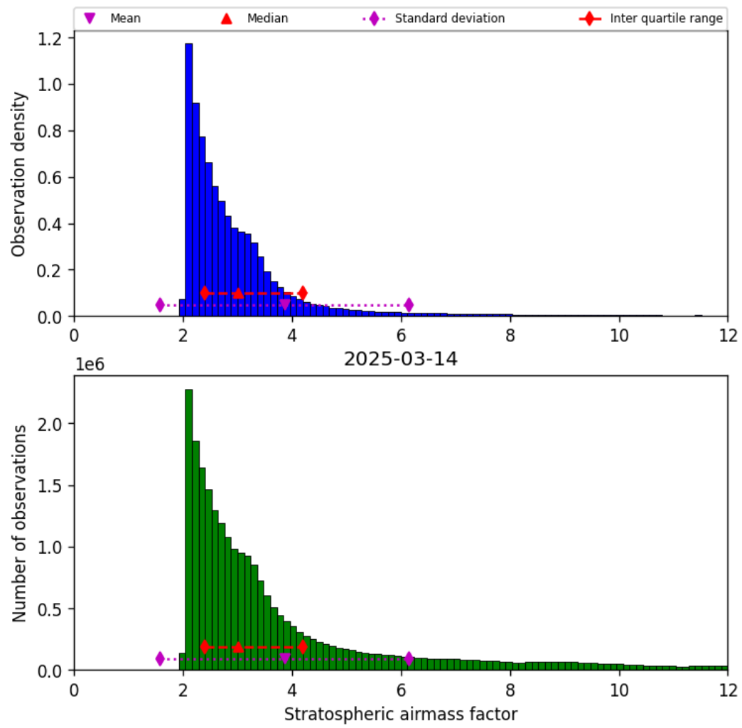
Figure 42: Histogram of “Stratospheric airmass factor” for 2025-03-14 to 2025-03-15
