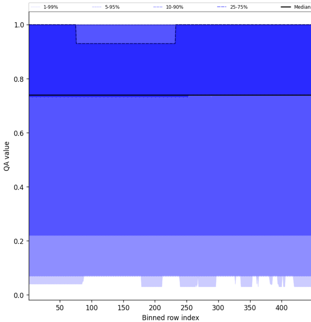
Figure 43: Along track statistics of “QA value” for 2025-03-14 to 2025-03-15
