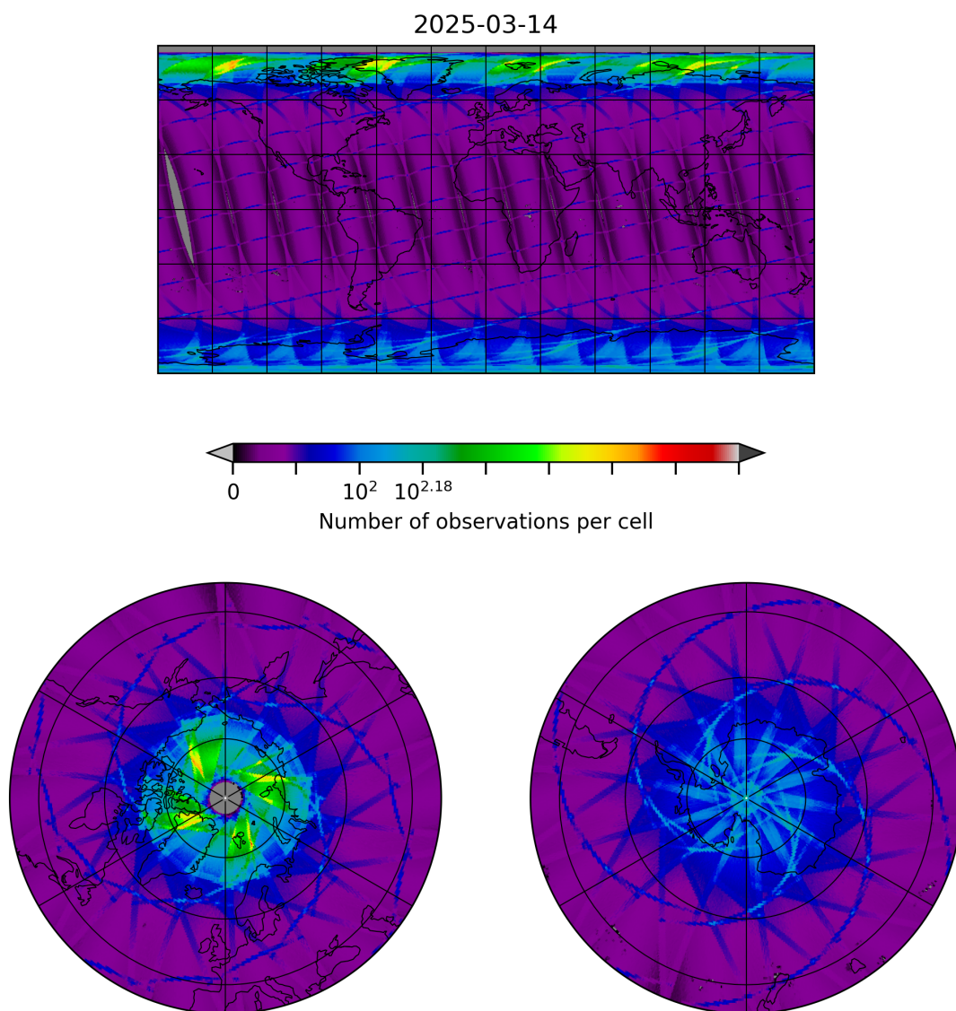
Figure 8: Map of the number of observations for 2025-03-14 to 2025-03-15
