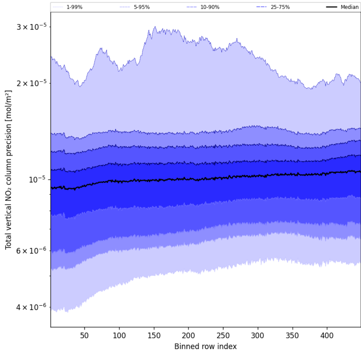
Figure 54: Along track statistics of “Total vertical NO 2 column precision” for 2025-03-14 to 2025-03-15
