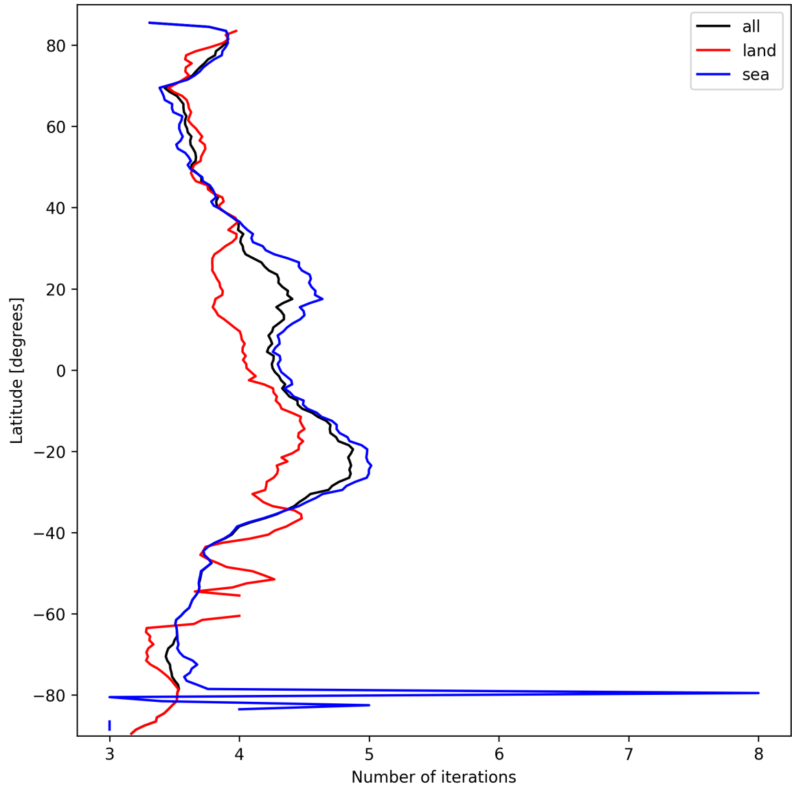
Figure 15: Zonal average of “Number of iterations” for 2025-03-14 to 2025-03-15.
