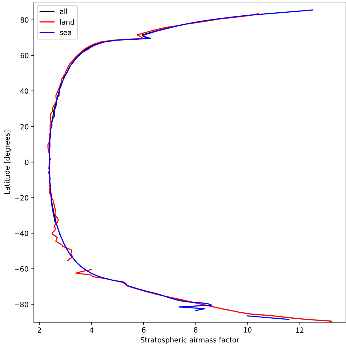
Figure 25: Zonal average of “Stratospheric airmass factor” for 2025-03-14 to 2025-03-15.
