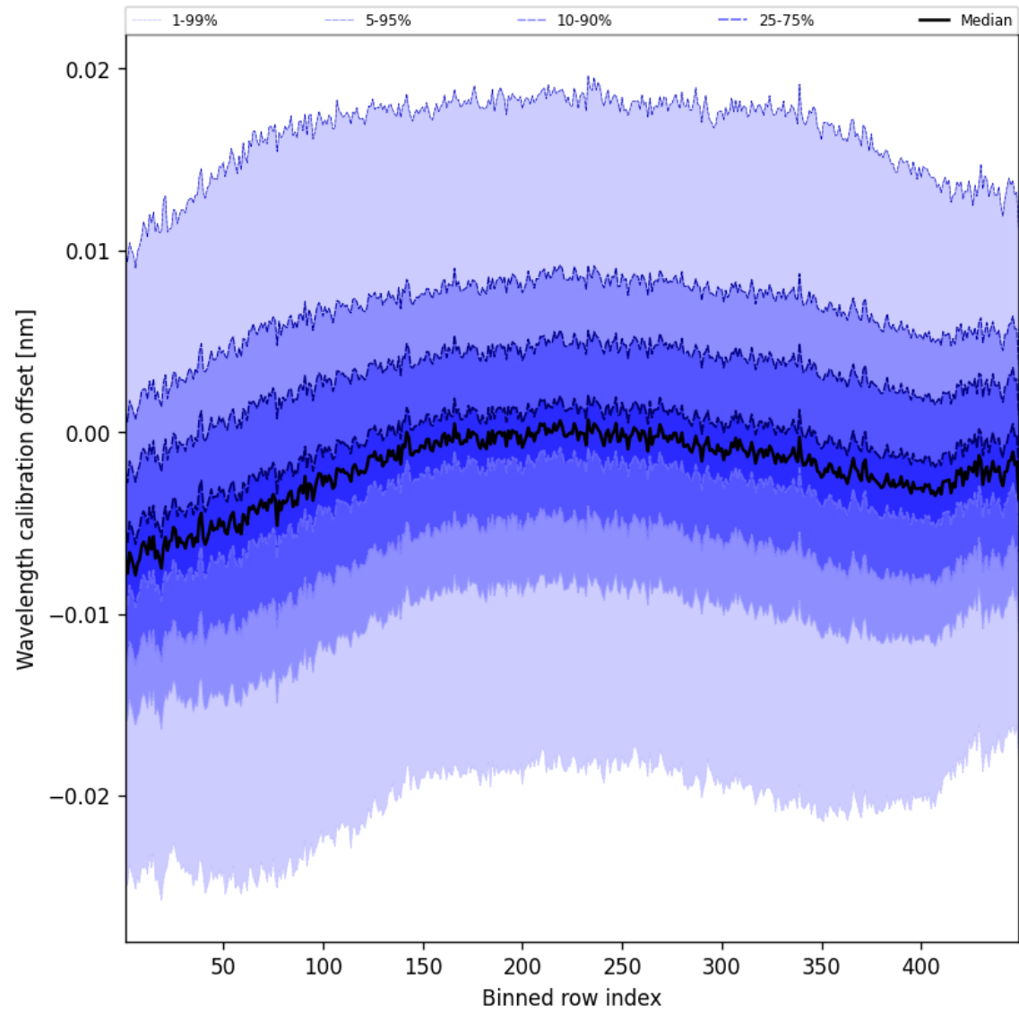
Figure 50: Along track statistics of “Wavelength calibration offset” for 2025-03-14 to 2025-03-15
