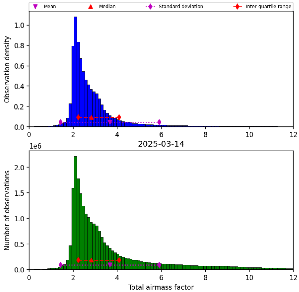
Figure 30: Histogram of “Total airmass factor” for 2025-03-14 to 2025-03-15
