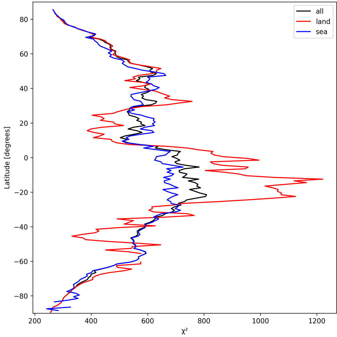
Figure 23: Zonal average of “ \chi^2 ” for 2025-03-14 to 2025-03-15.
