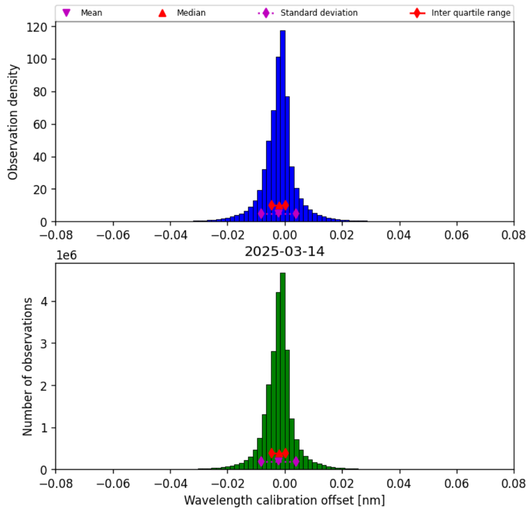
Figure 33: Histogram of “Wavelength calibration offset” for 2025-03-14 to 2025-03-15
