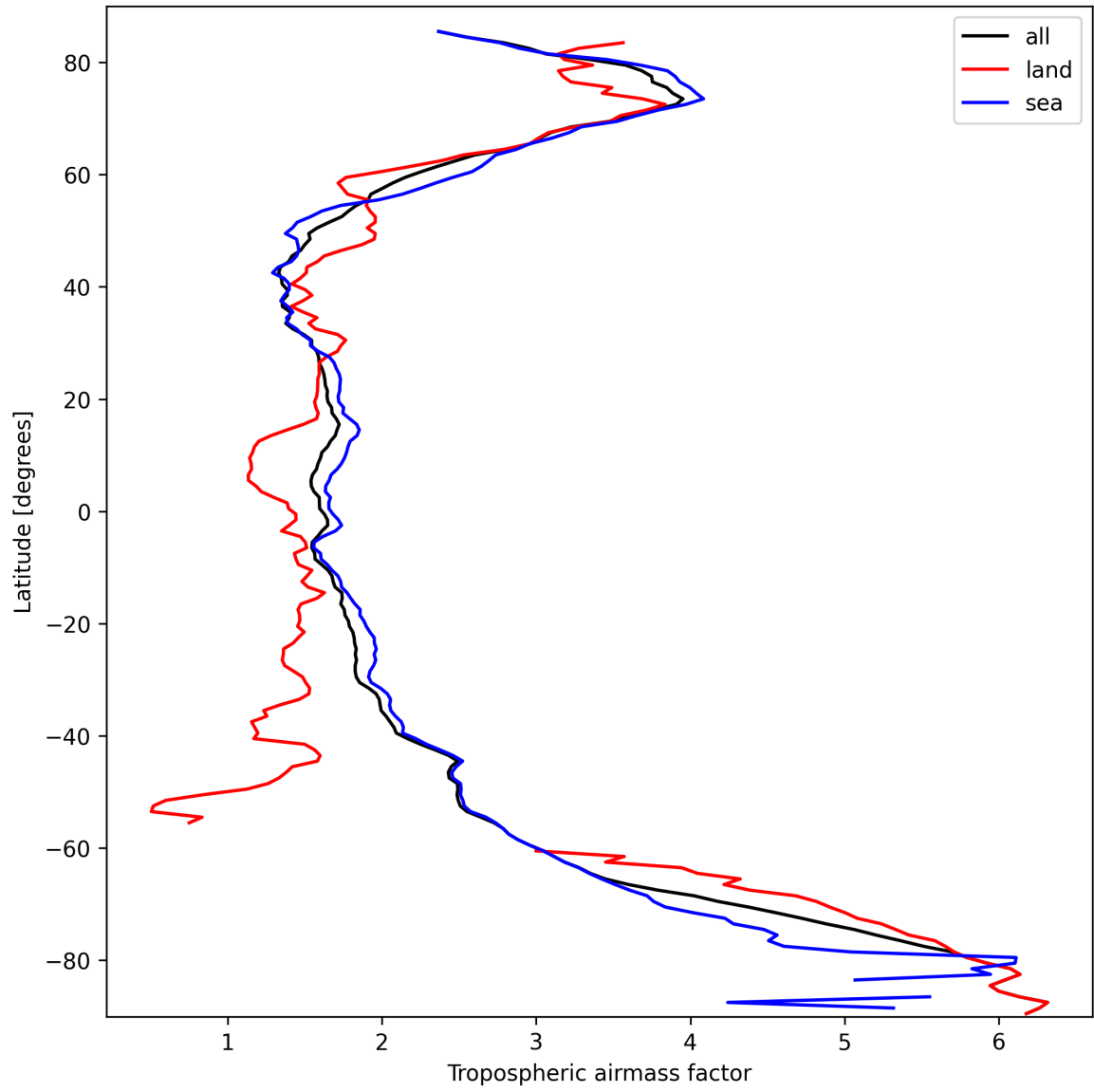
Figure 12: Zonal average of “Tropospheric air mass factor” for 2025-03-14 to 2025-03-15.
