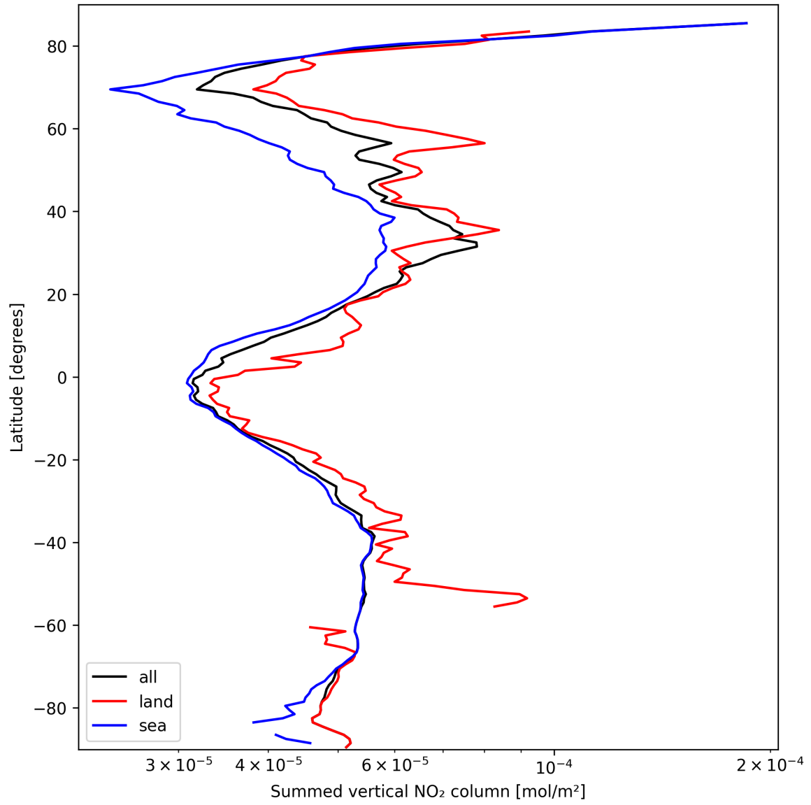
Figure 21: Zonal average of “Summed vertical NO 2 column” for 2025-03-14 to 2025-03-15.
