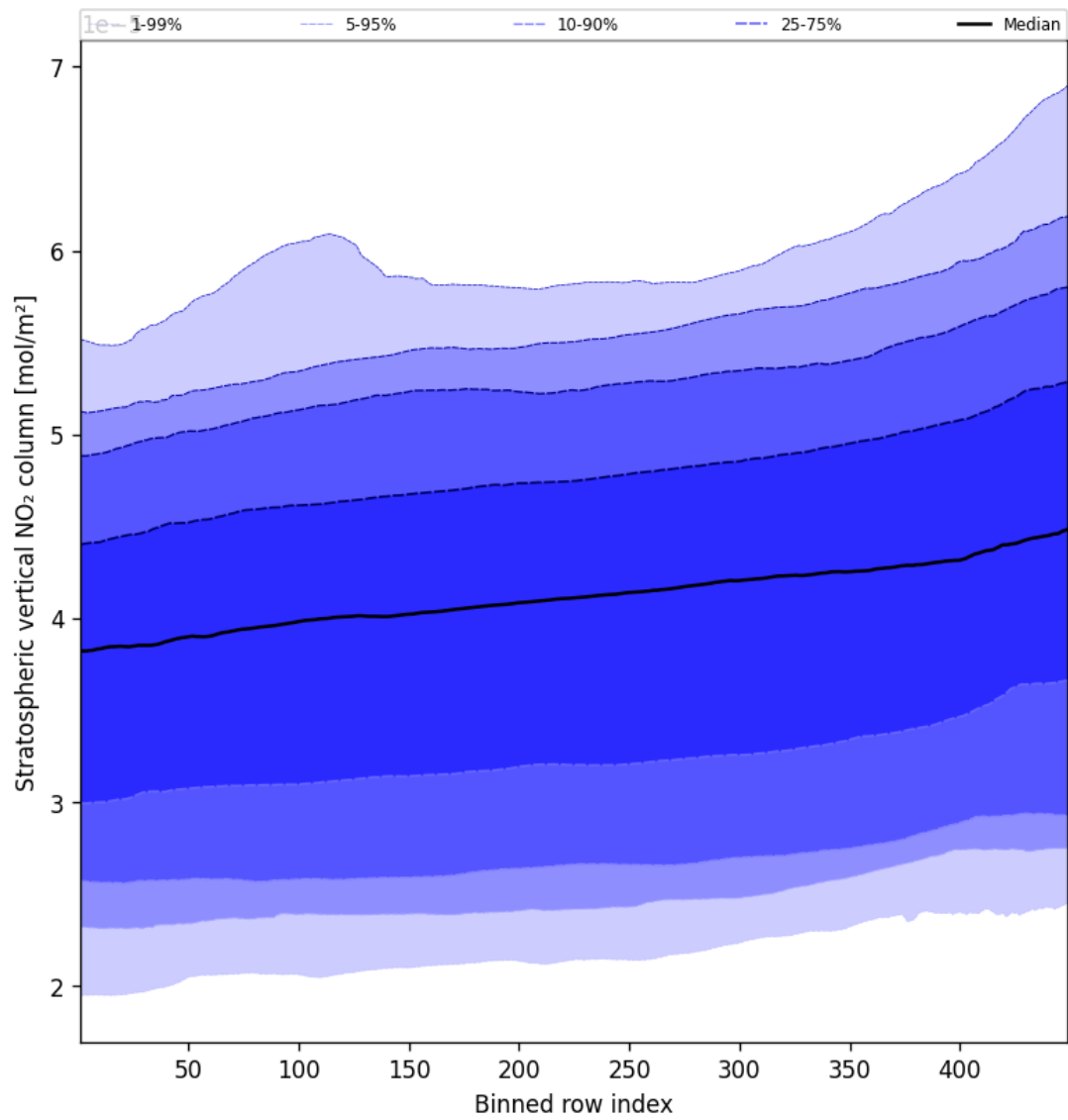
Figure 51: Along track statistics of “Stratospheric vertical NO 2 column” for 2025-03-14 to 2025-03-15
