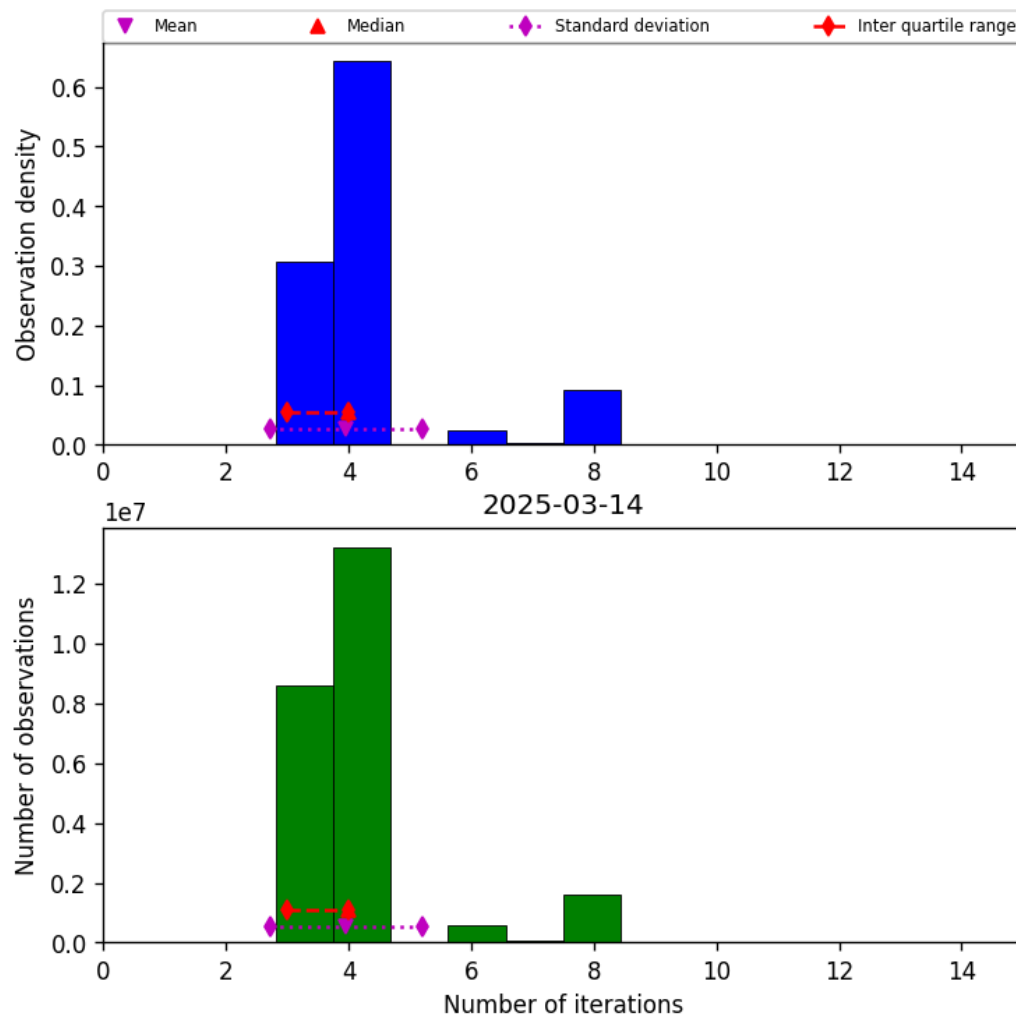
Figure 32: Histogram of “Number of iterations” for 2025-03-14 to 2025-03-15
