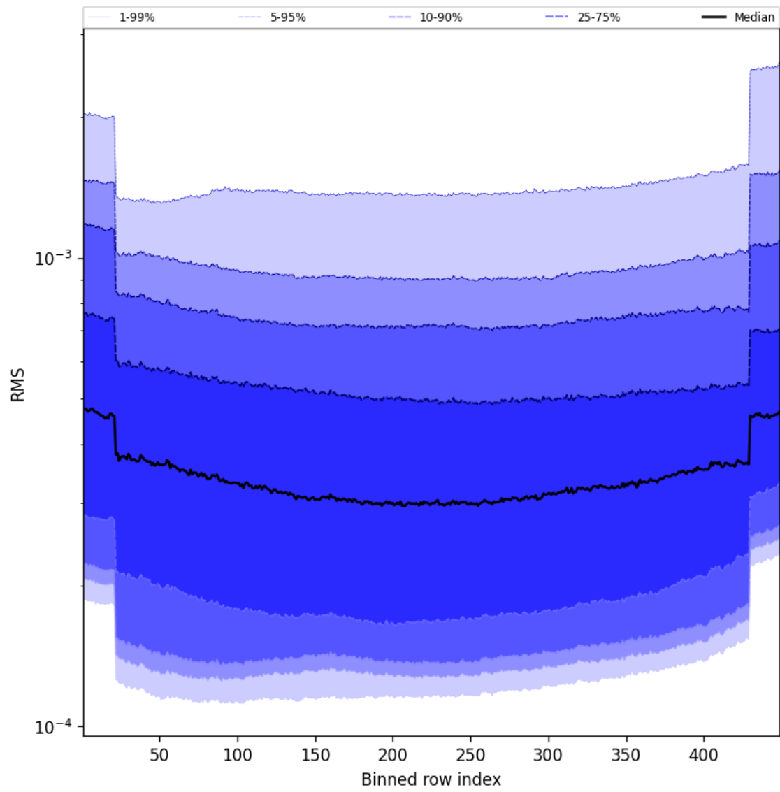
Figure 58: Along track statistics of “RMS” for 2025-03-14 to 2025-03-15
