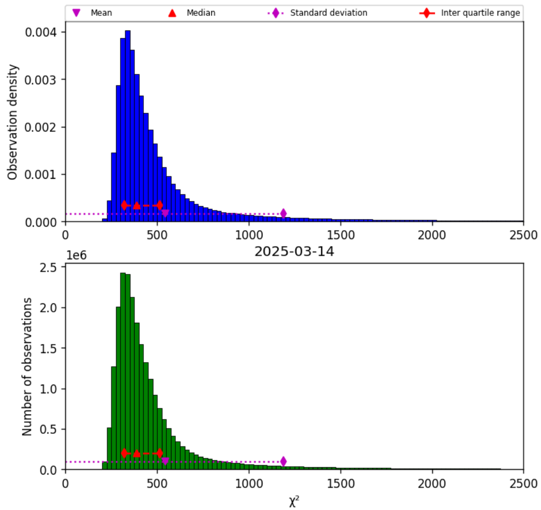
Figure 40: Histogram of “ \chi^2 ” for 2025-03-14 to 2025-03-15
