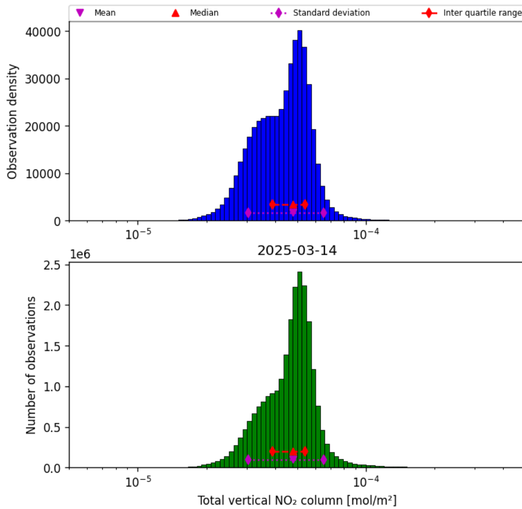
Figure 36: Histogram of “Total vertical NO 2 column” for 2025-03-14 to 2025-03-15
