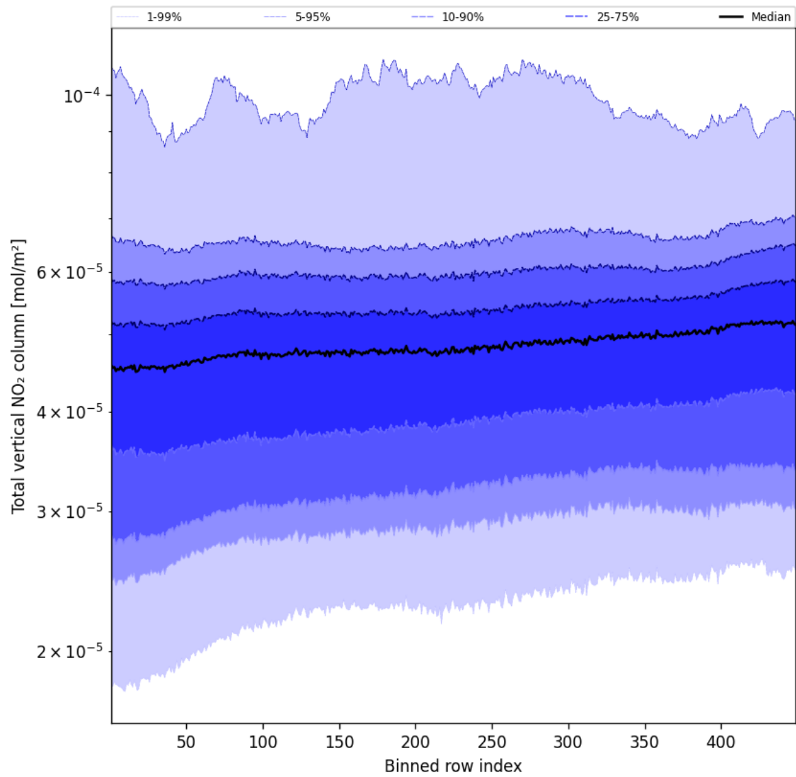
Figure 53: Along track statistics of “Total vertical NO 2 column” for 2025-03-14 to 2025-03-15
