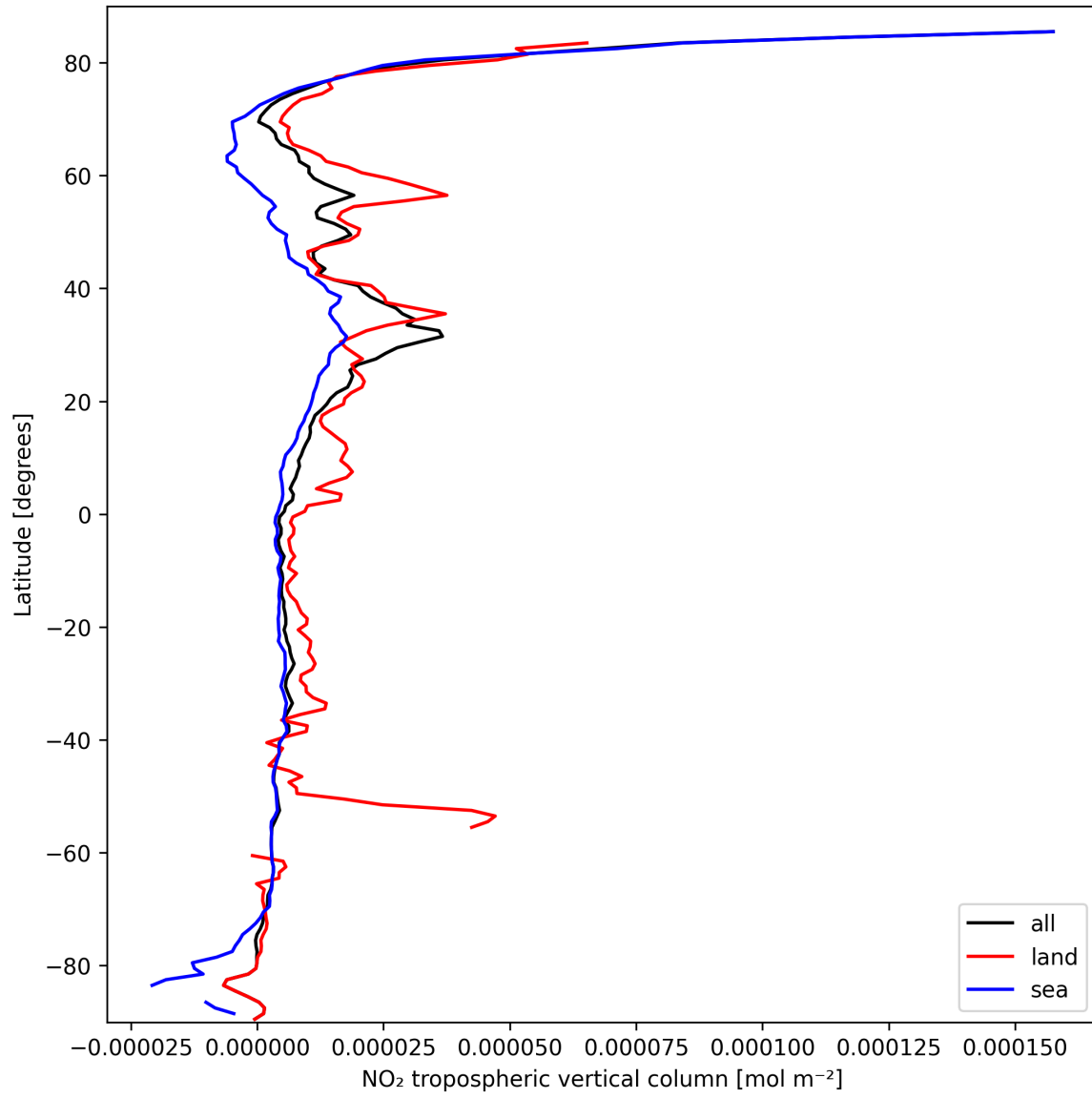
Figure 10: Zonal average of “NO 2 tropospheric vertical column” for 2025-03-14 to 2025-03-15.
