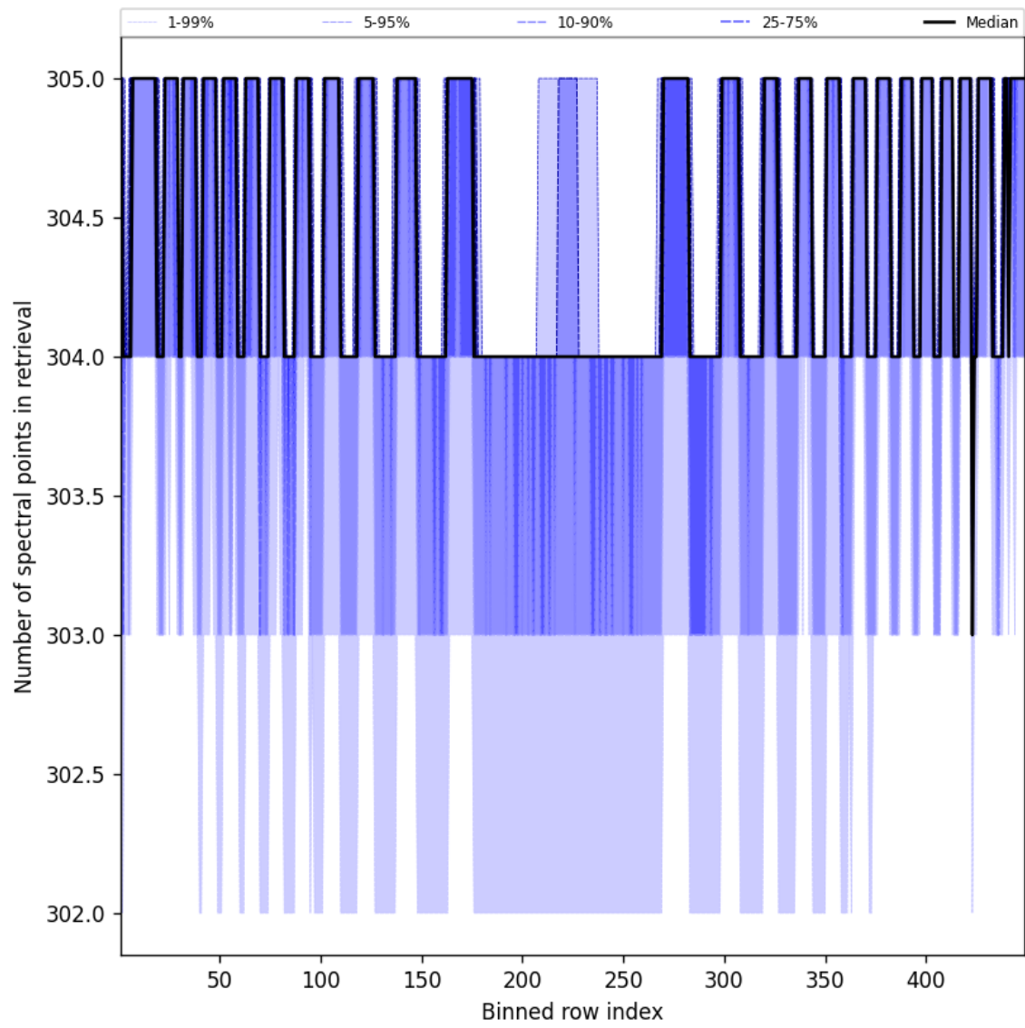
Figure 48: Along track statistics of “Number of spectral points in retrieval” for 2025-03-14 to 2025-03-15
