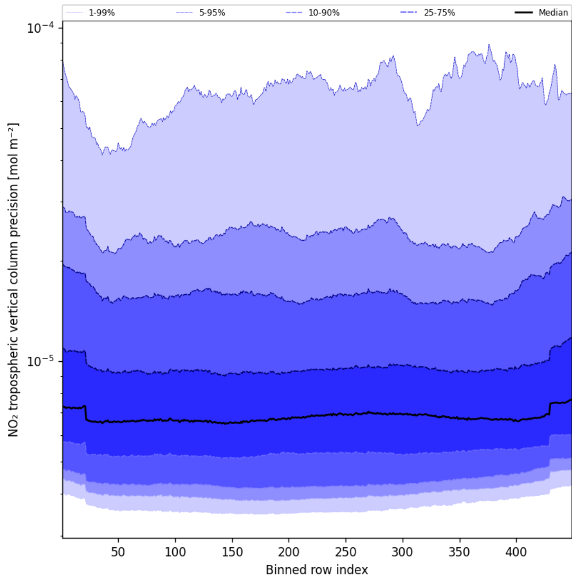
Figure 45: Along track statistics of “NO 2 tropospheric vertical column precision” for 2025-03-14 to 2025-03-15
