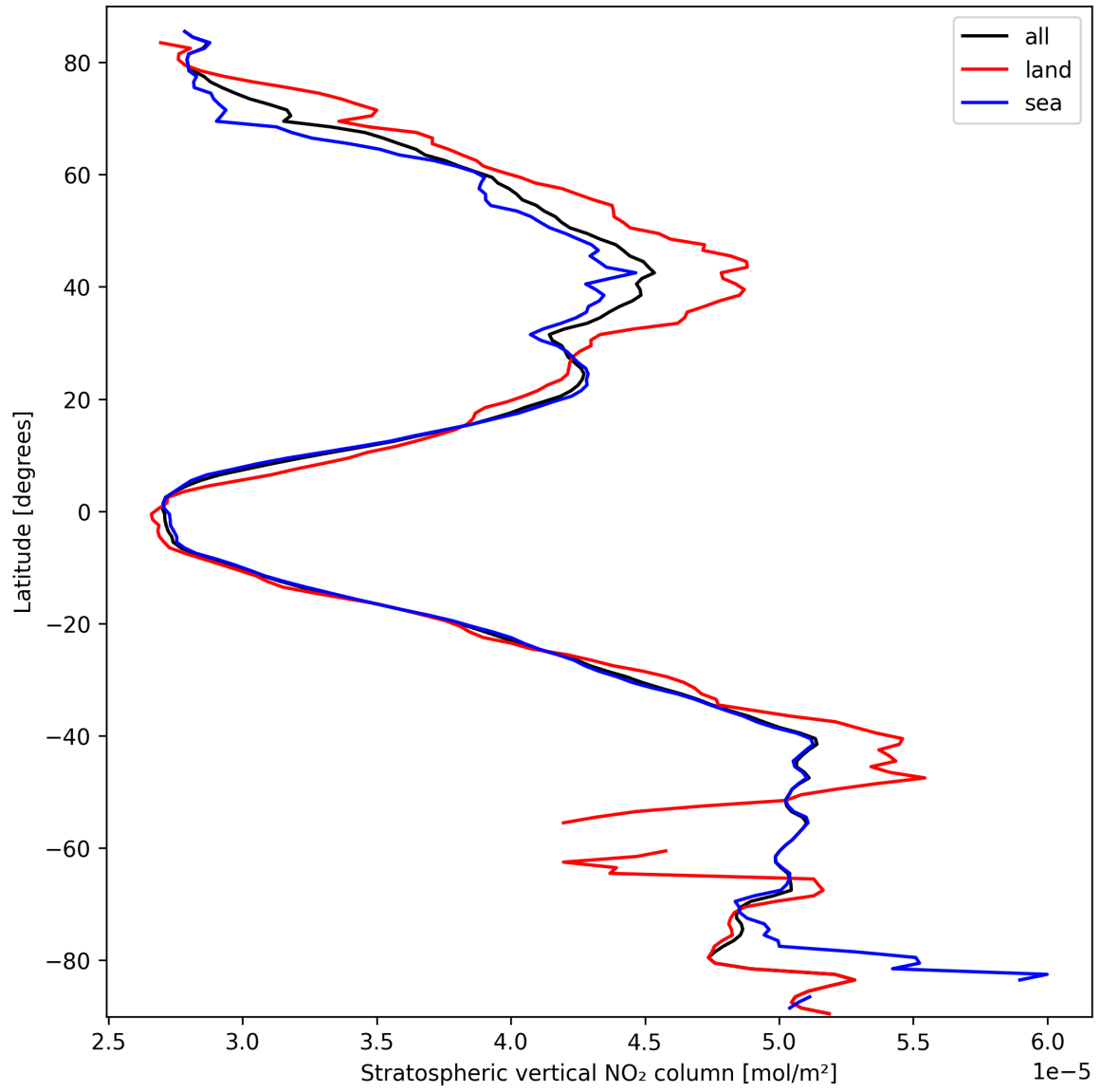
Figure 17: Zonal average of “Stratospheric vertical NO 2 column” for 2025-03-14 to 2025-03-15.
