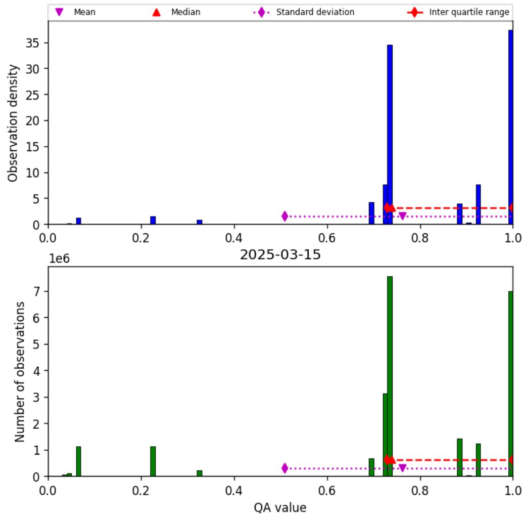
Figure 26: Histogram of “QA value” for 2025-03-15 to 2025-03-15
