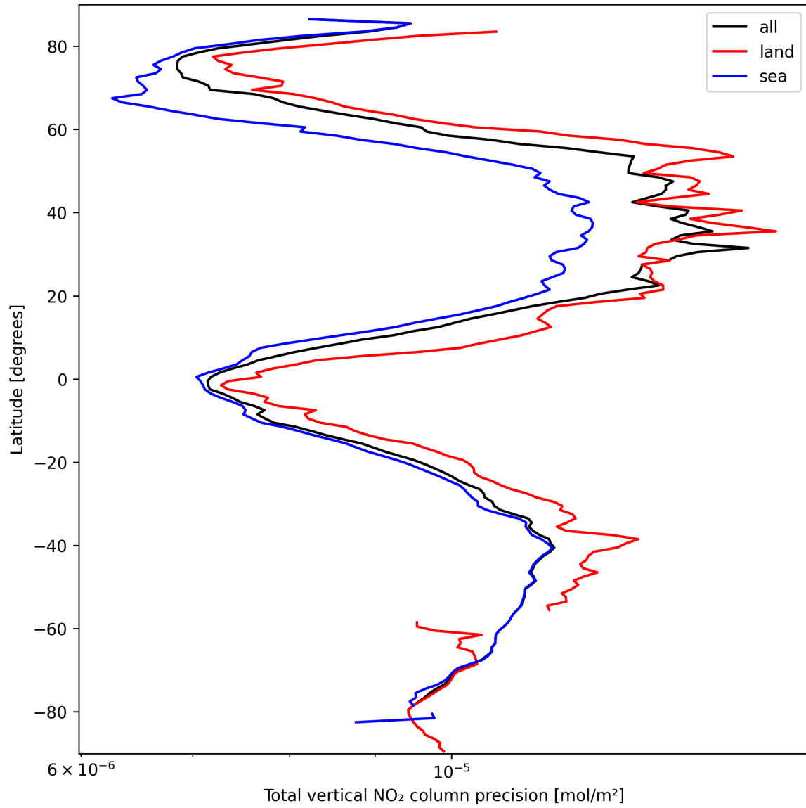
Figure 20: Zonal average of “Total vertical NO 2 column precision” for 2025-03-15 to 2025-03-15.
