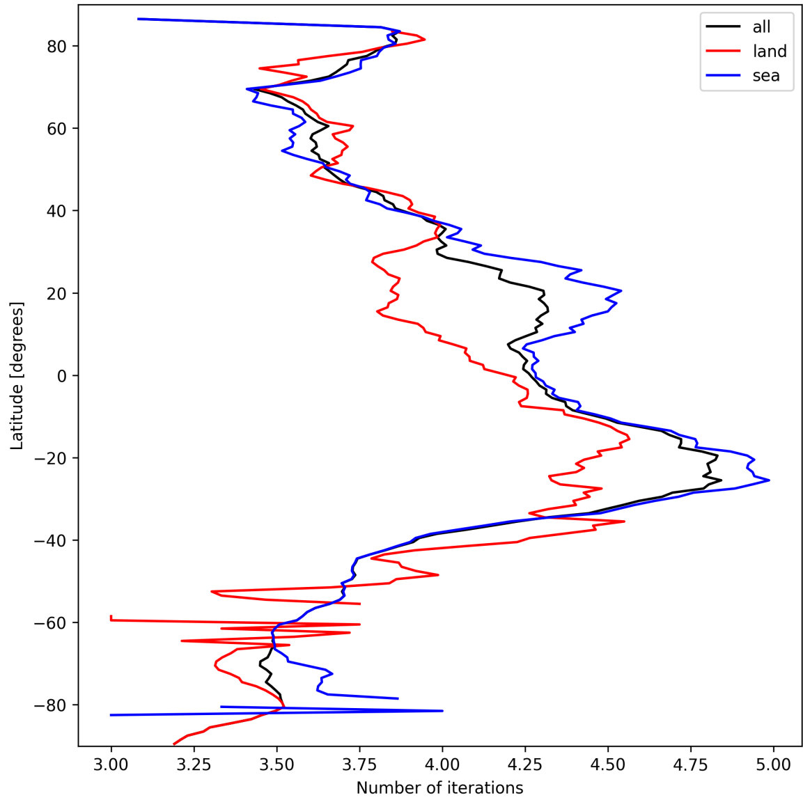
Figure 15: Zonal average of “Number of iterations” for 2025-03-15 to 2025-03-15.
