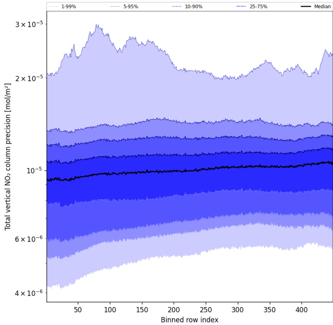
Figure 54: Along track statistics of “Total vertical NO 2 column precision” for 2025-03-15 to 2025-03-15
