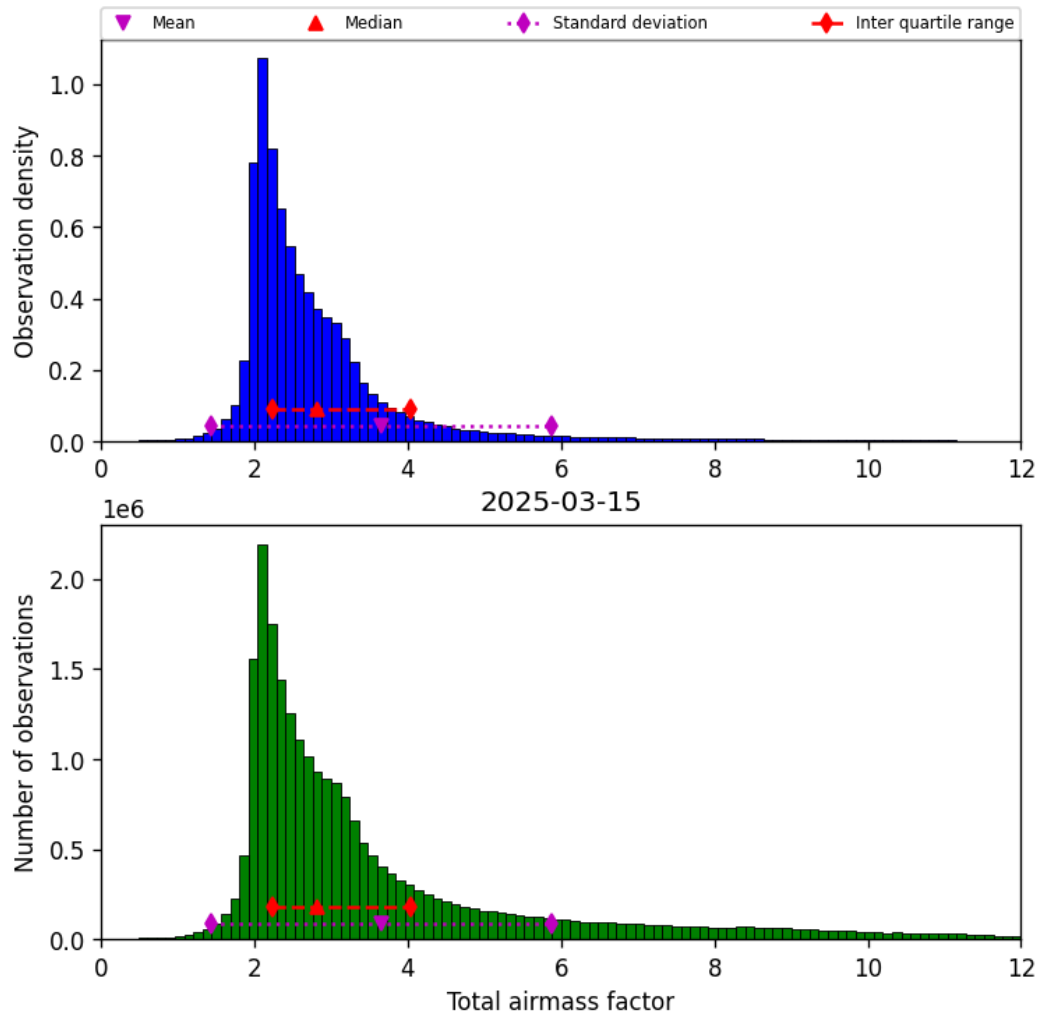
Figure 30: Histogram of “Total airmass factor” for 2025-03-15 to 2025-03-15
