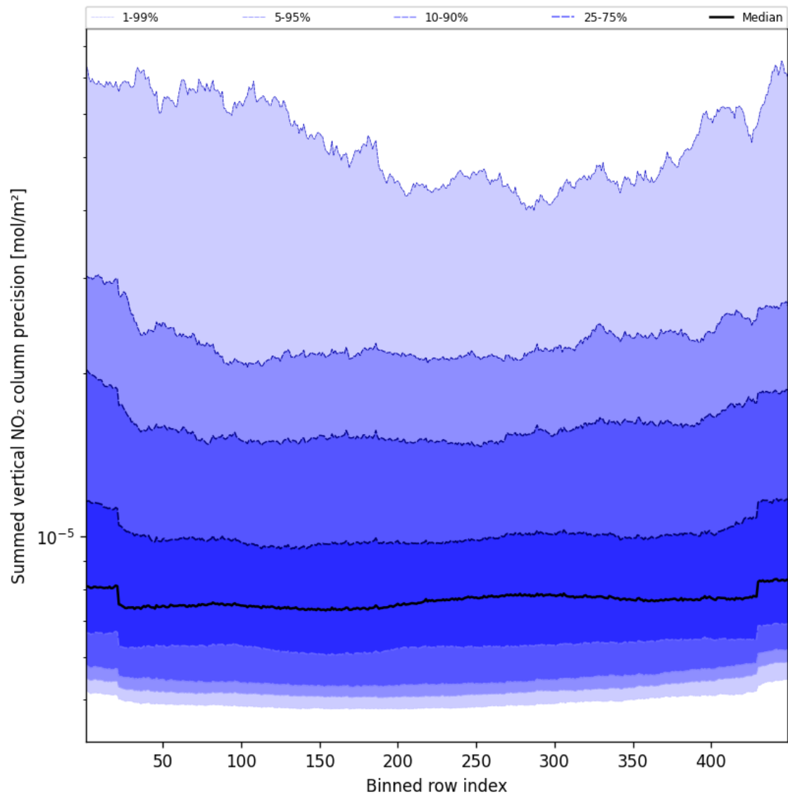
Figure 56: Along track statistics of “Summed vertical NO 2 column precision” for 2025-03-15 to 2025-03-15
