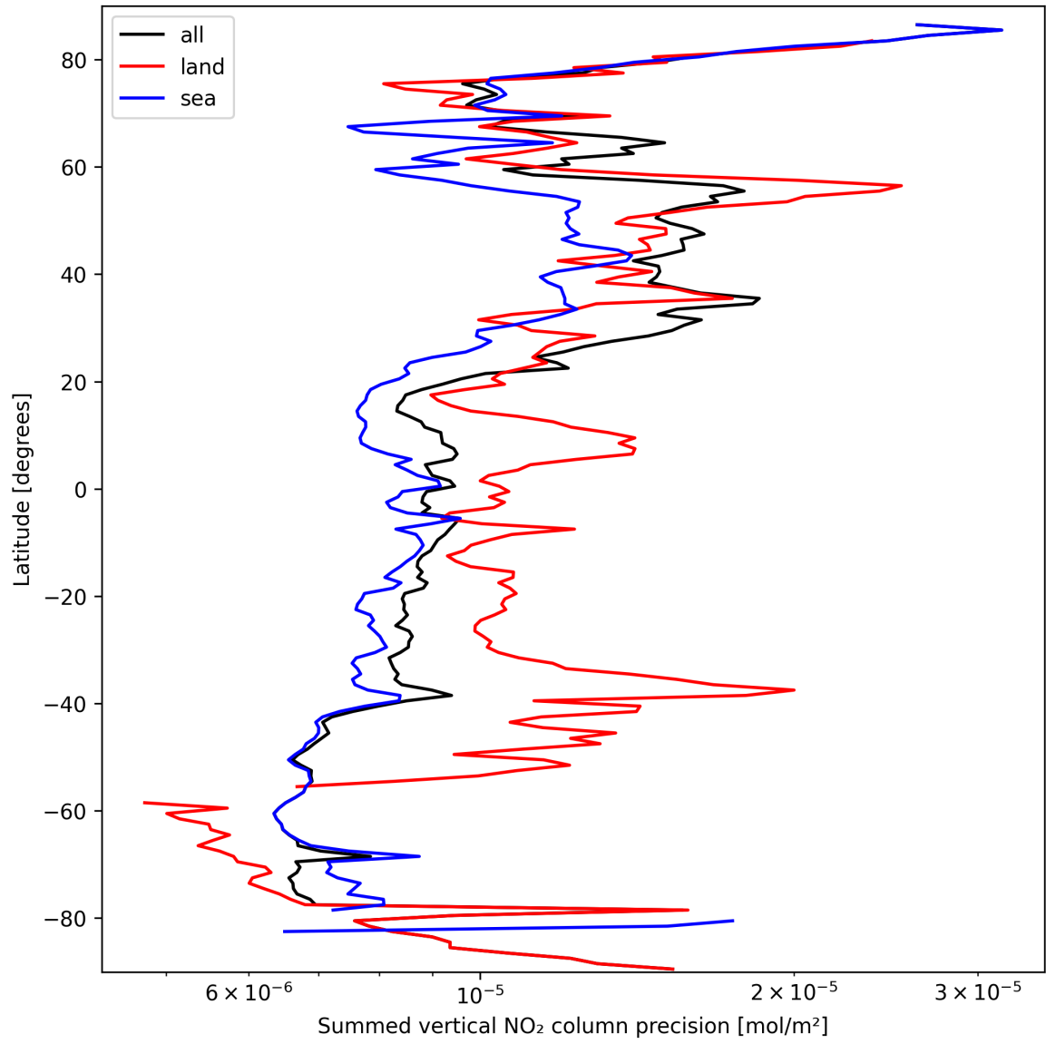
Figure 22: Zonal average of “Summed vertical NO 2 column precision” for 2025-03-15 to 2025-03-15.
