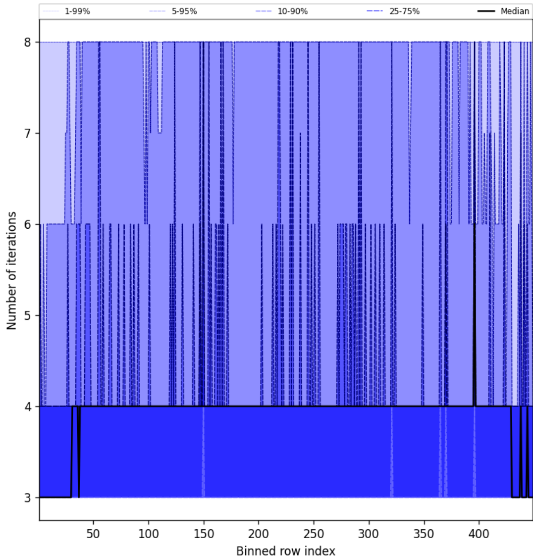
Figure 49: Along track statistics of “Number of iterations” for 2025-03-15 to 2025-03-15
