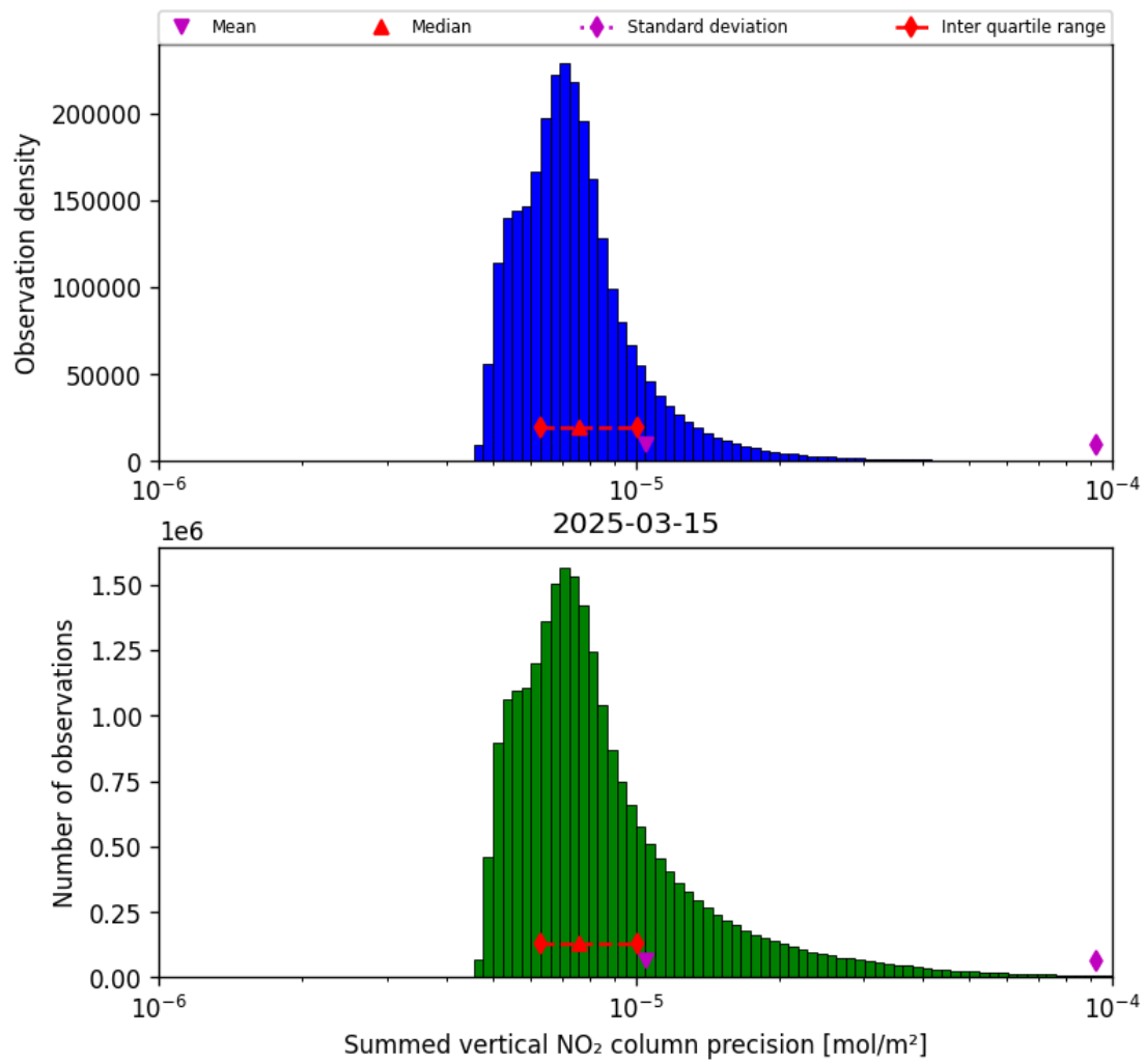
Figure 39: Histogram of "Summed vertical NO 2 column precision" for 2025-03-15 to 2025-03-15
