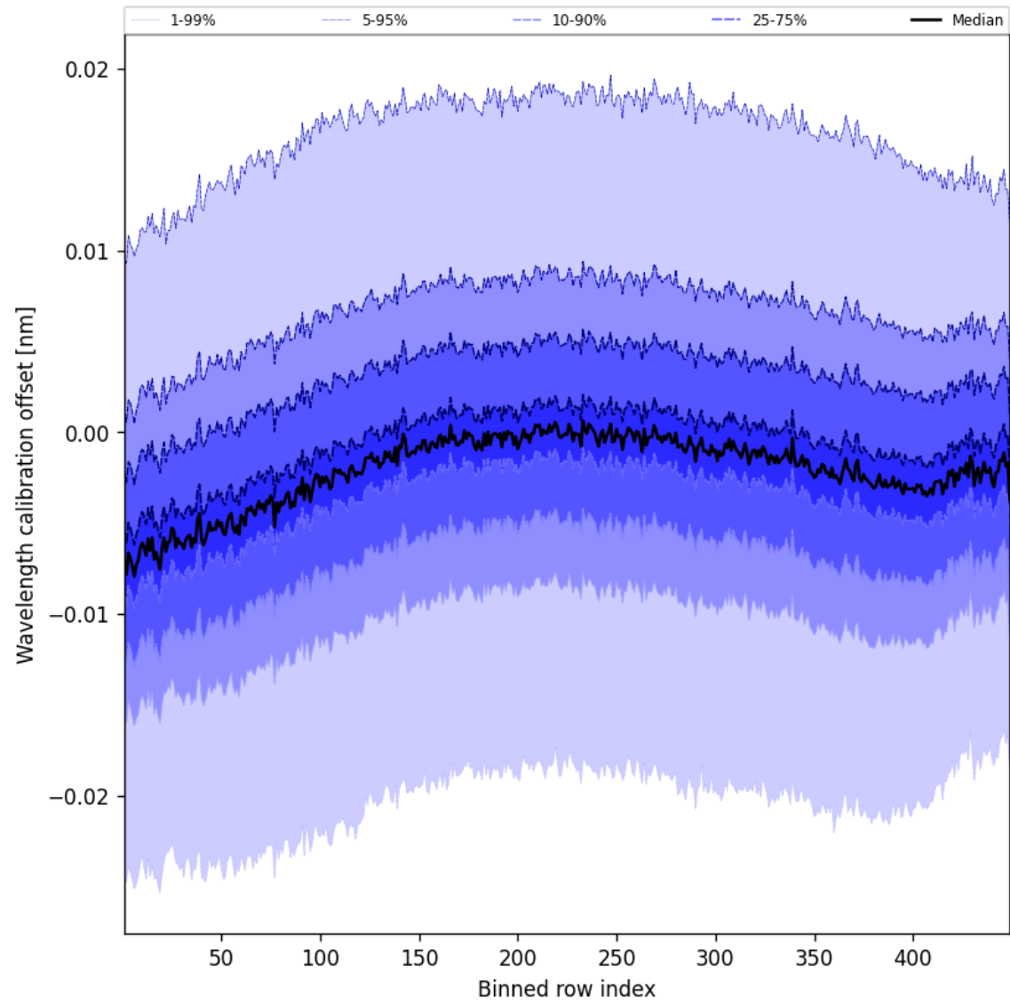
Figure 50: Along track statistics of “Wavelength calibration offset” for 2025-03-15 to 2025-03-15
