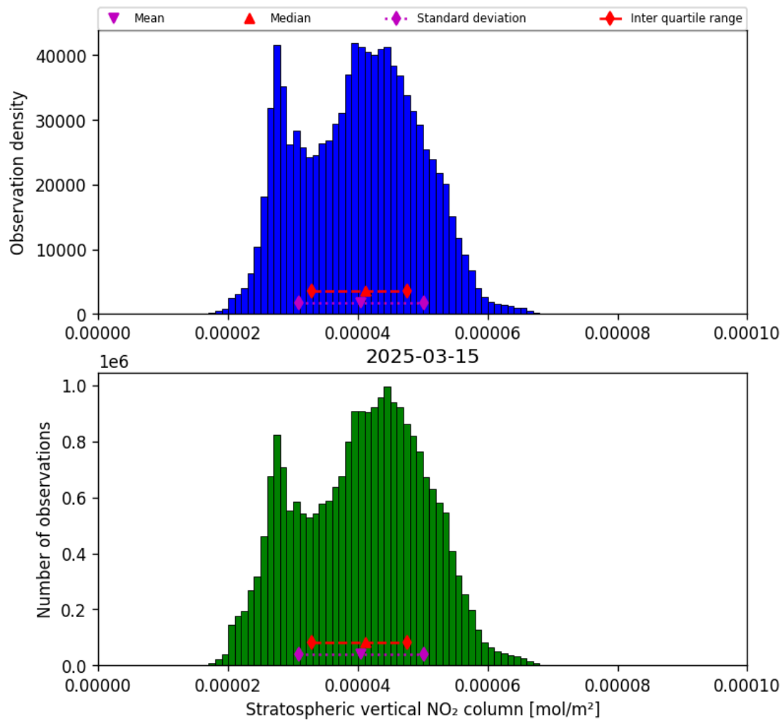
Figure 34: Histogram of “Stratospheric vertical NO 2 column” for 2025-03-15 to 2025-03-15
