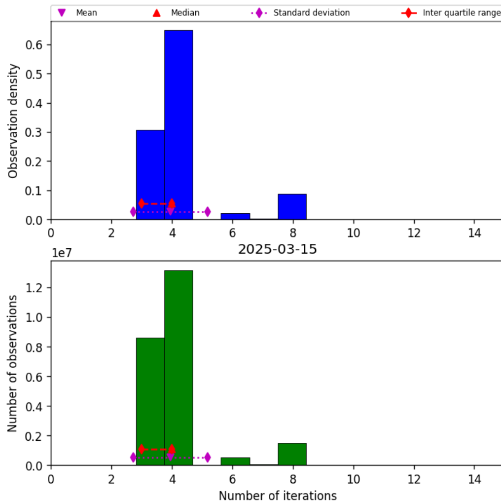
Figure 32: Histogram of “Number of iterations” for 2025-03-15 to 2025-03-15
