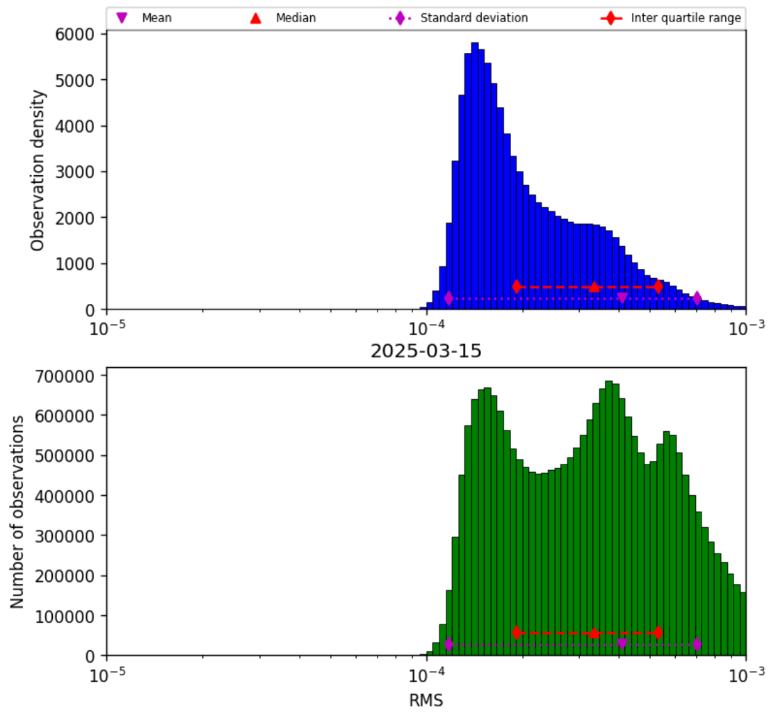
Figure 41: Histogram of “RMS” for 2025-03-15 to 2025-03-15
