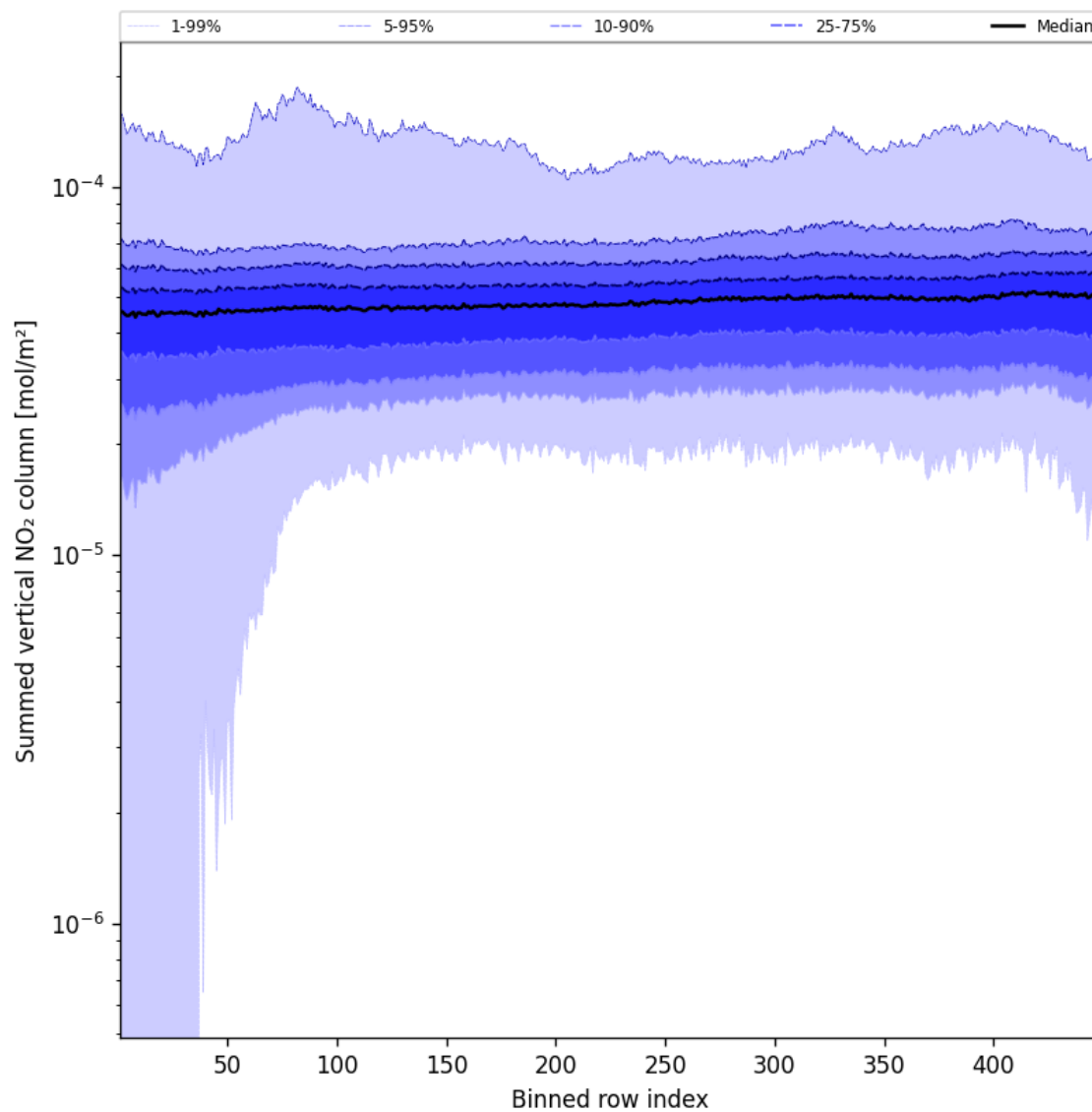
Figure 55: Along track statistics of “Summed vertical NO 2 column” for 2025-03-15 to 2025-03-15
