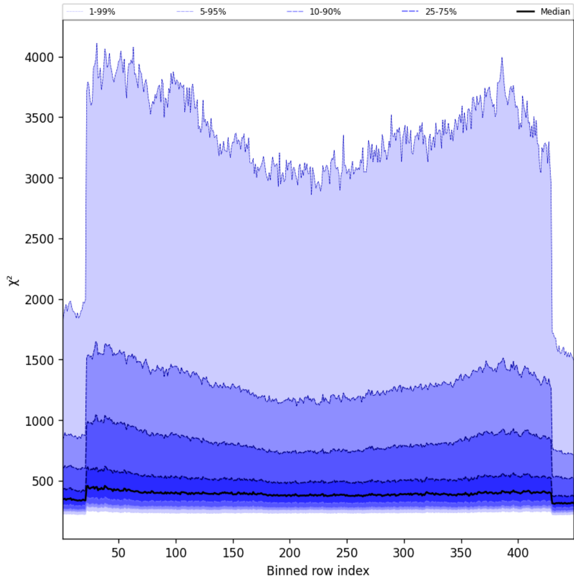
Figure 57: Along track statistics of “ \chi^2 ” for 2025-03-15 to 2025-03-15
