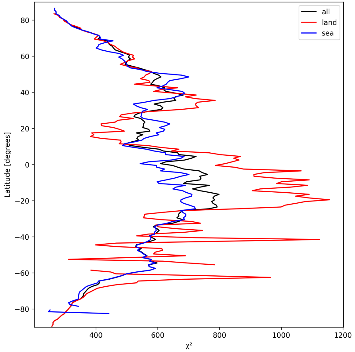
Figure 23: Zonal average of “ \chi^2 ” for 2025-03-15 to 2025-03-15.
