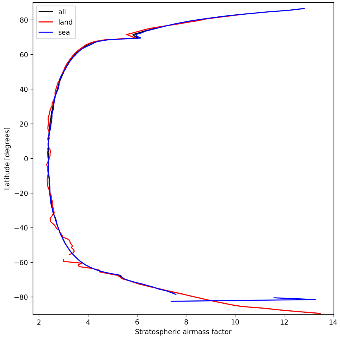
Figure 25: Zonal average of “Stratospheric airmass factor” for 2025-03-15 to 2025-03-15.
