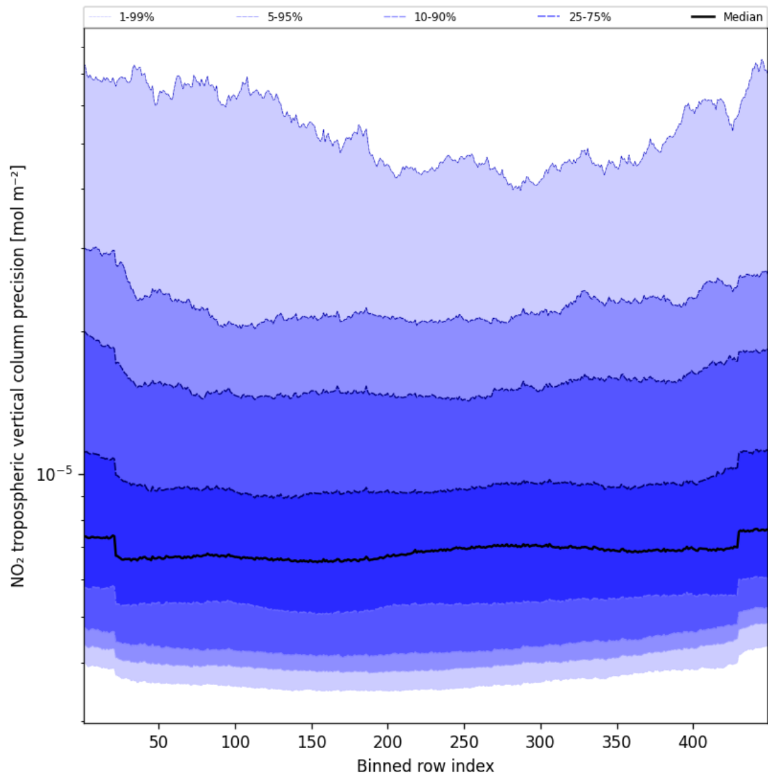
Figure 45: Along track statistics of “NO 2 tropospheric vertical column precision” for 2025-03-15 to 2025-03-15
