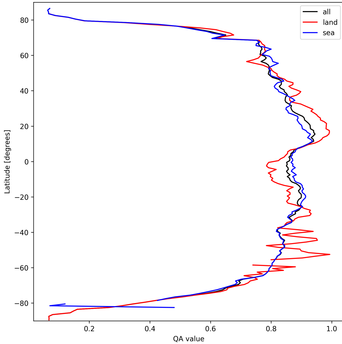
Figure 9: Zonal average of “QA value” for 2025-03-15 to 2025-03-15.
