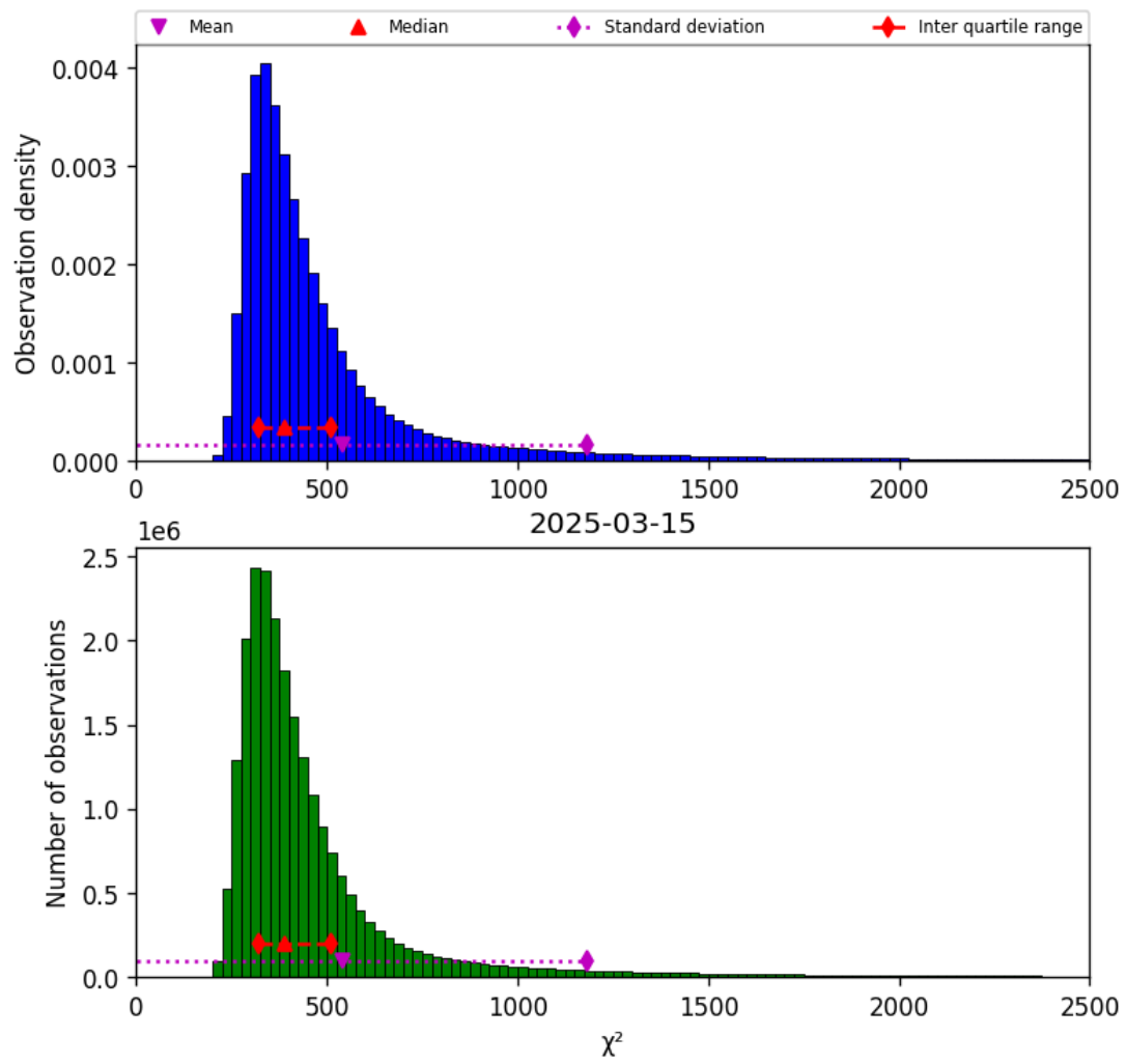
Figure 40: Histogram of “ \chi^2 ” for 2025-03-15 to 2025-03-15
