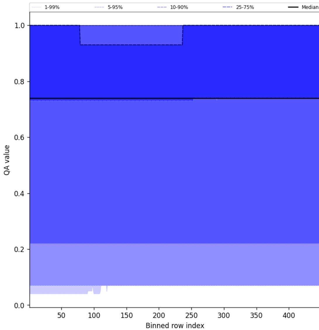
Figure 43: Along track statistics of “QA value” for 2025-03-15 to 2025-03-15
