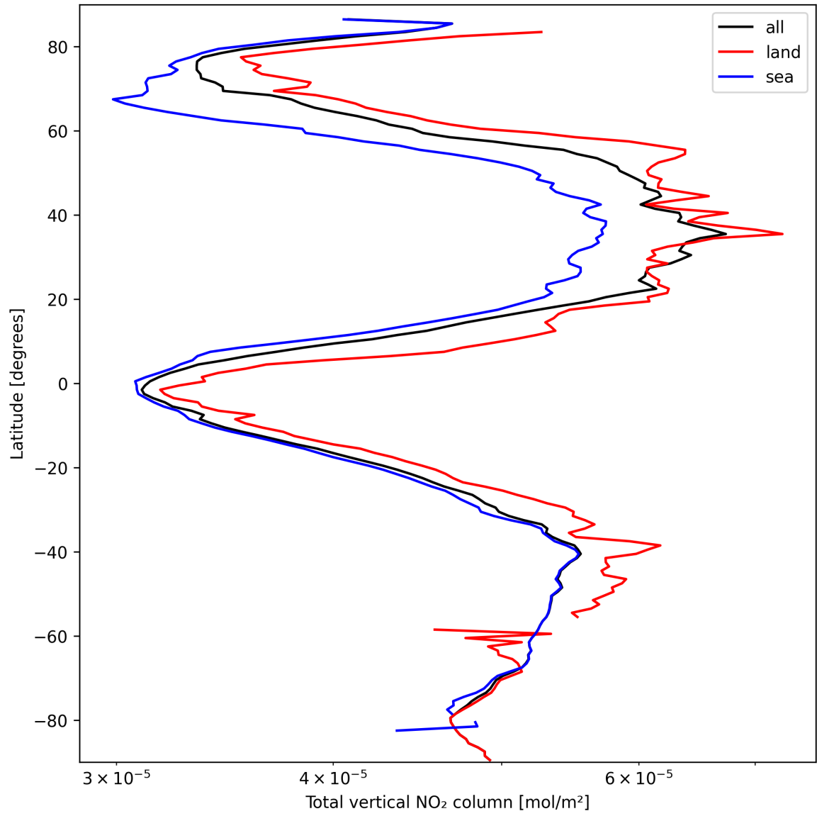
Figure 19: Zonal average of “Total vertical NO 2 column” for 2025-03-15 to 2025-03-15.
