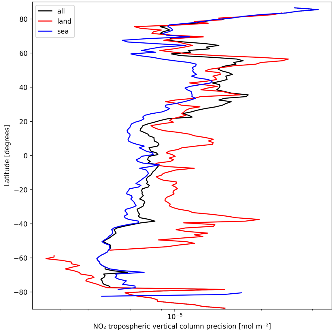
Figure 11: Zonal average of “NO 2 tropospheric vertical column precision” for 2025-03-15 to 2025-03-15.
