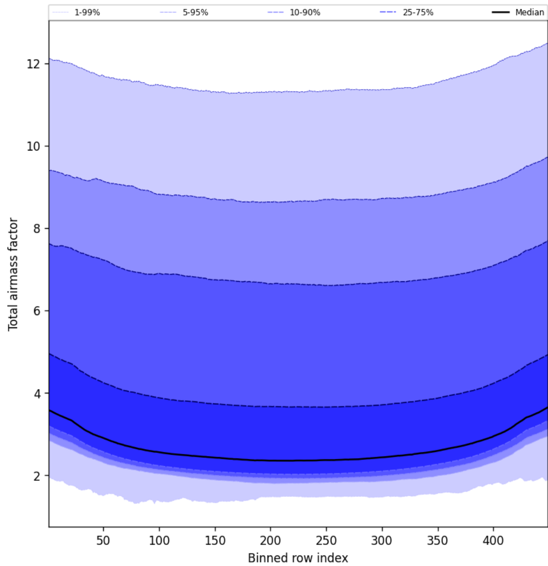
Figure 47: Along track statistics of “Total airmass factor” for 2025-03-15 to 2025-03-15
