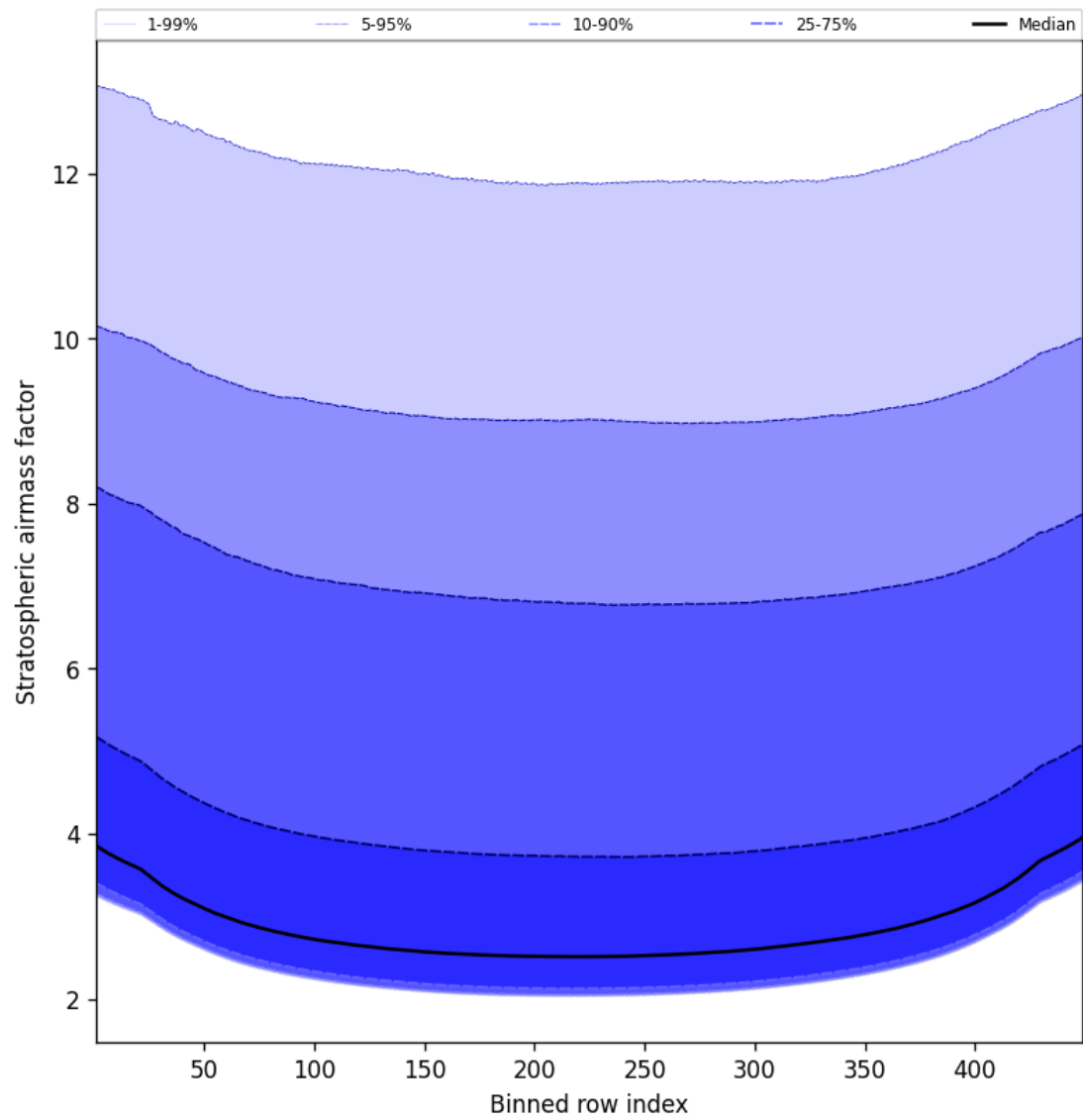
Figure 59: Along track statistics of “Stratospheric airmass factor” for 2025-03-15 to 2025-03-15
