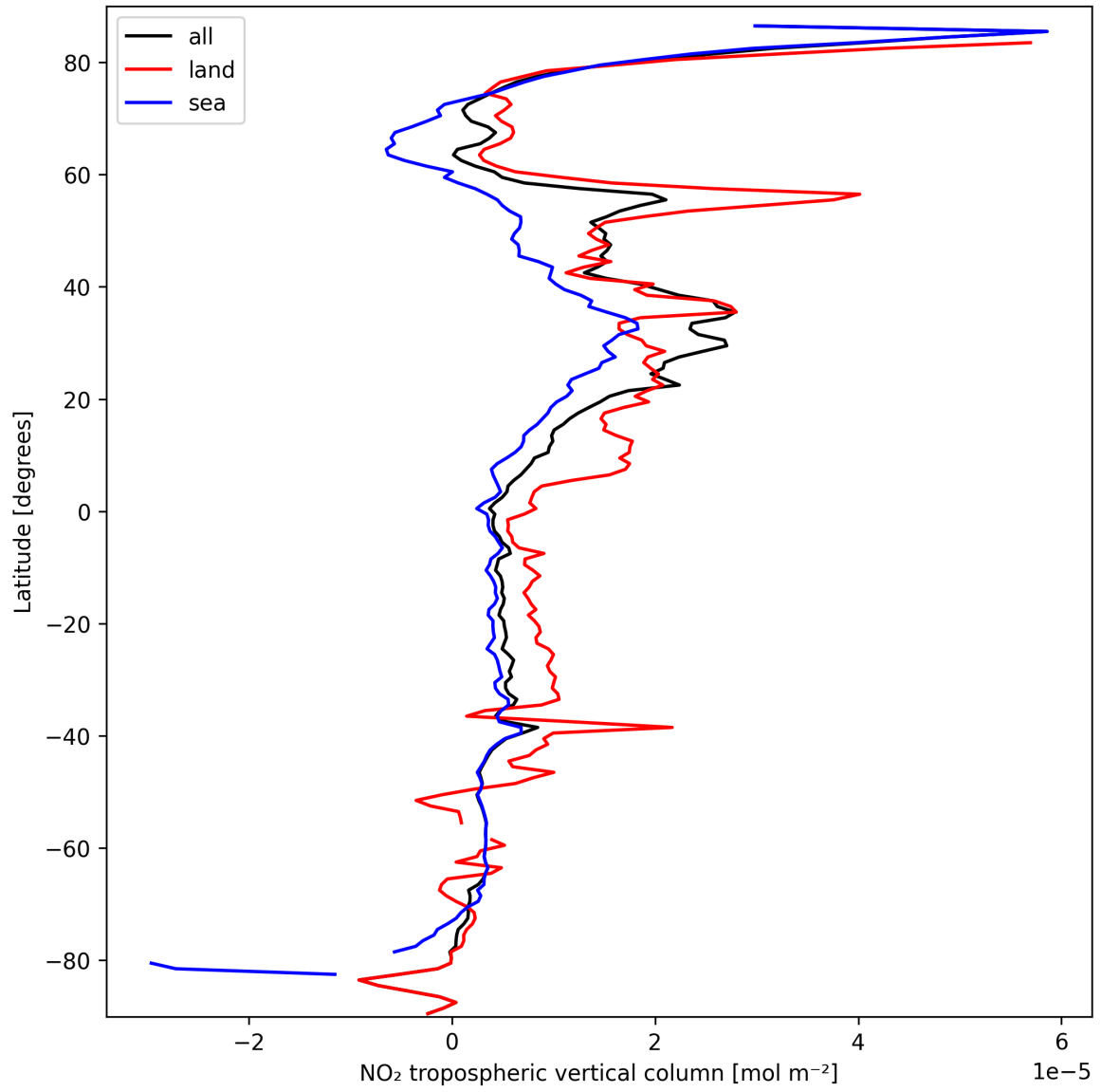
Figure 10: Zonal average of “NO 2 tropospheric vertical column” for 2025-03-15 to 2025-03-15.
