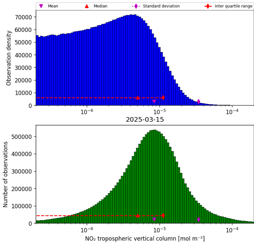
Figure 27: Histogram of “NO 2 tropospheric vertical column” for 2025-03-15 to 2025-03-15
