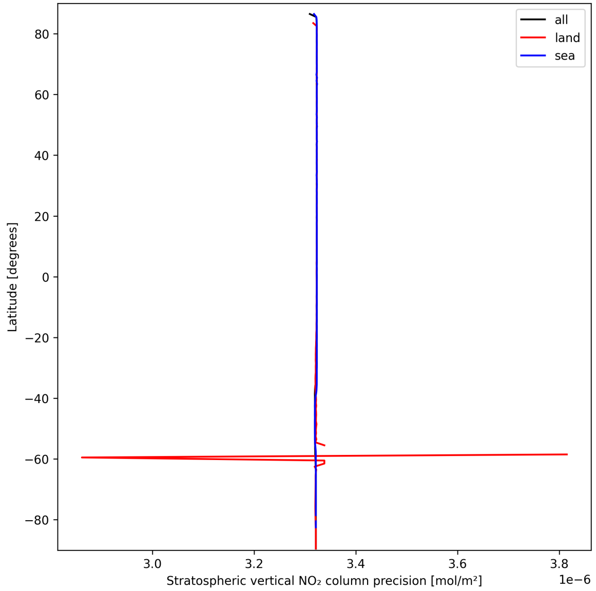
Figure 18: Zonal average of “Stratospheric vertical NO 2 column precision” for 2025-03-15 to 2025-03-15.
