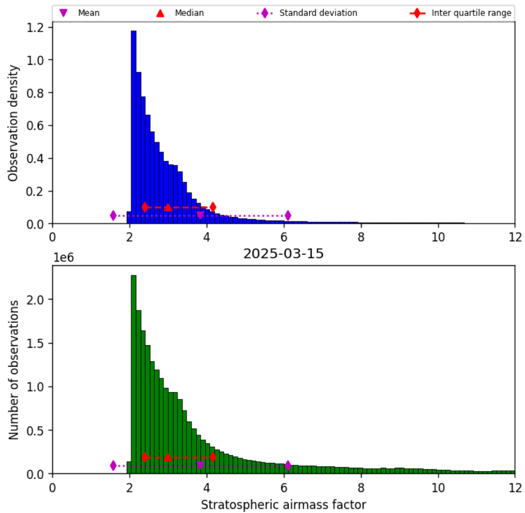
Figure 42: Histogram of “Stratospheric airmass factor” for 2025-03-15 to 2025-03-15
