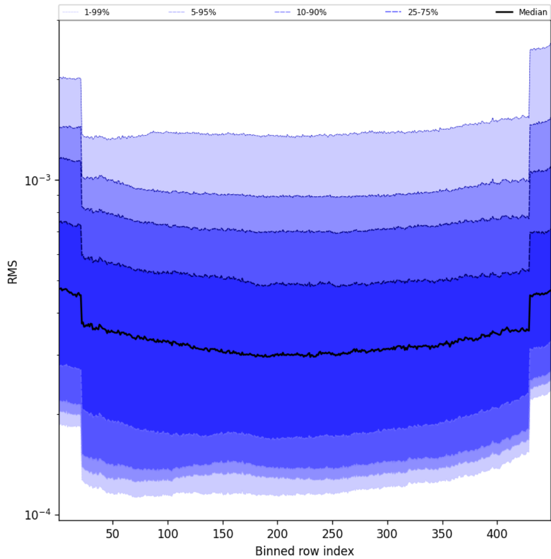
Figure 58: Along track statistics of “RMS” for 2025-03-15 to 2025-03-15
