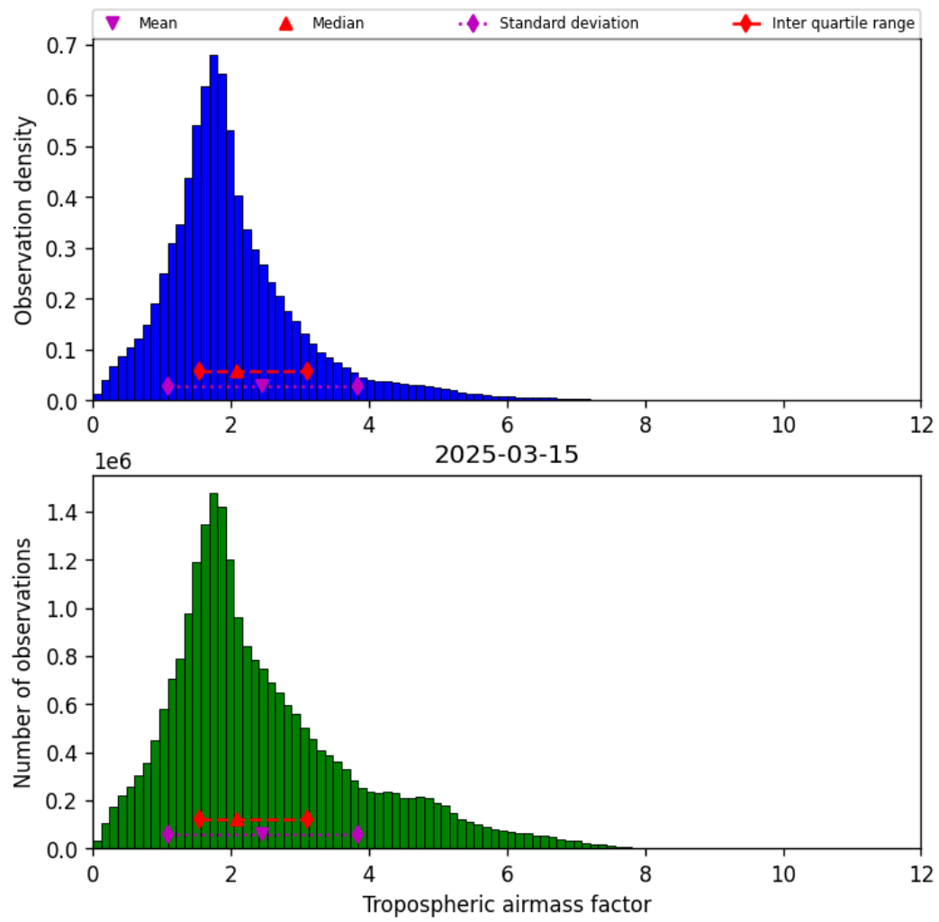
Figure 29: Histogram of “Tropospheric airmass factor” for 2025-03-15 to 2025-03-15
