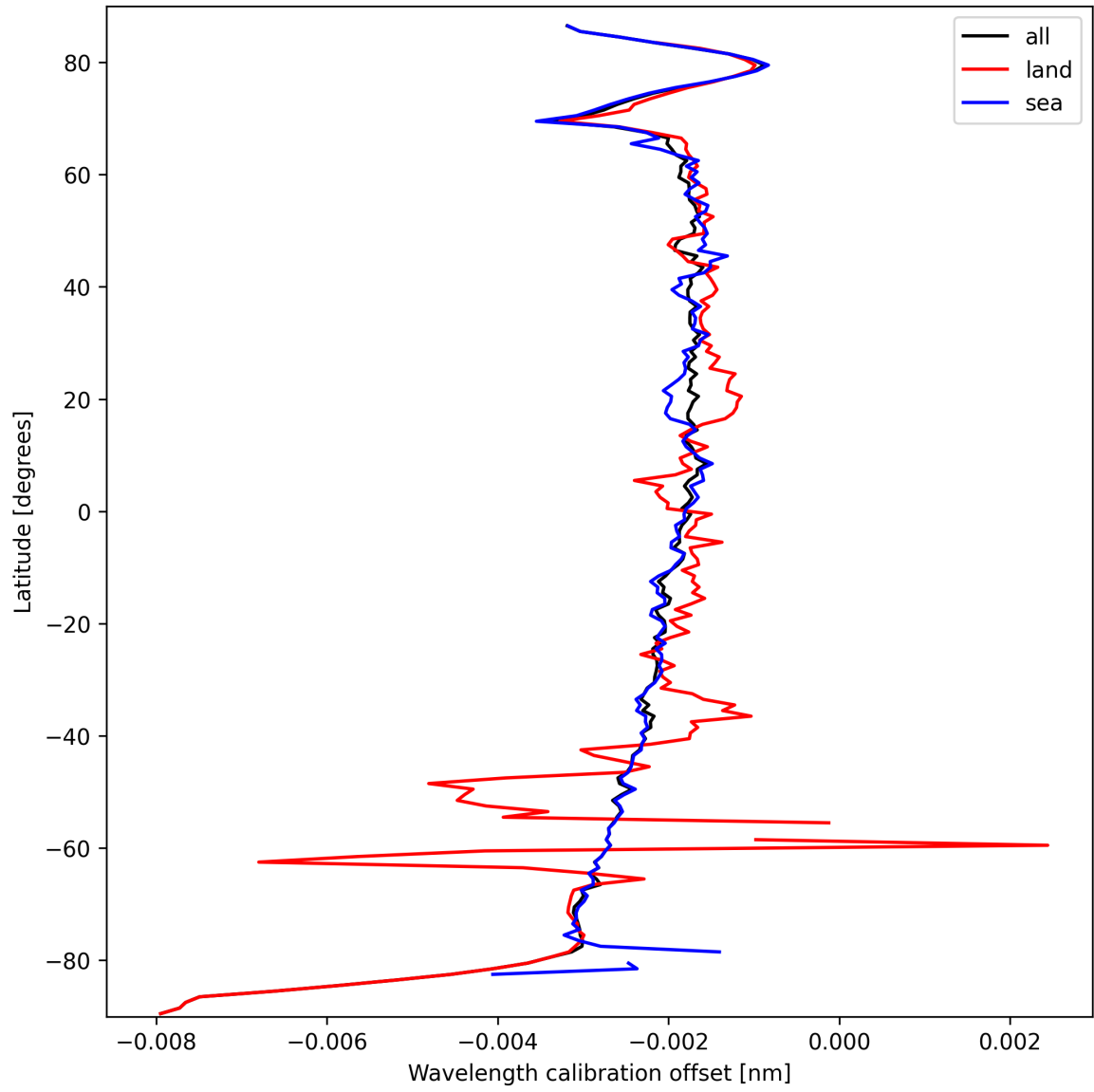
Figure 16: Zonal average of “Wavelength calibration offset” for 2025-03-15 to 2025-03-15.
