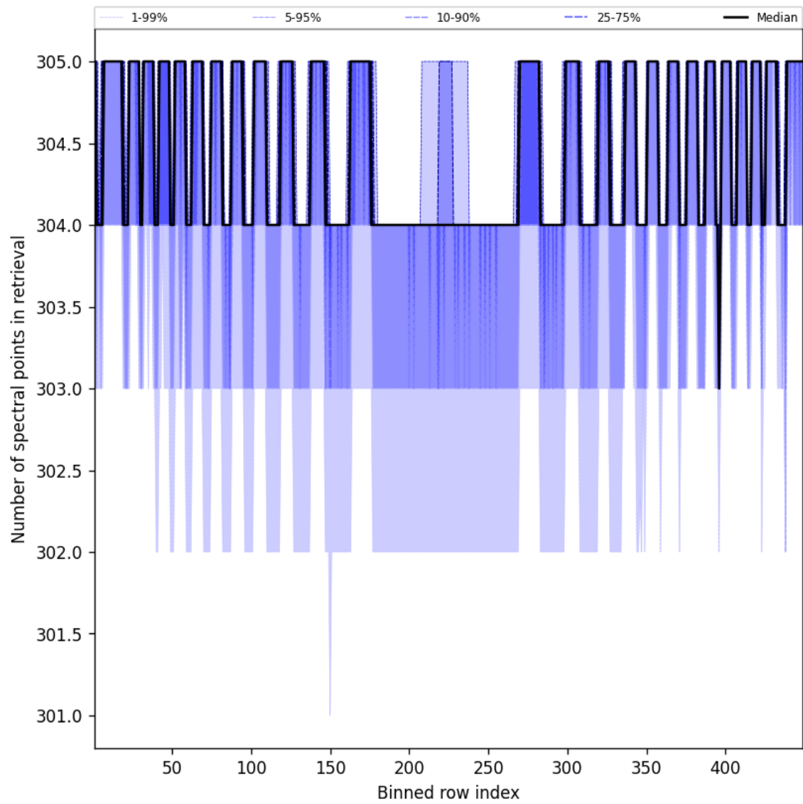
Figure 48: Along track statistics of “Number of spectral points in retrieval” for 2025-03-15 to 2025-03-15
