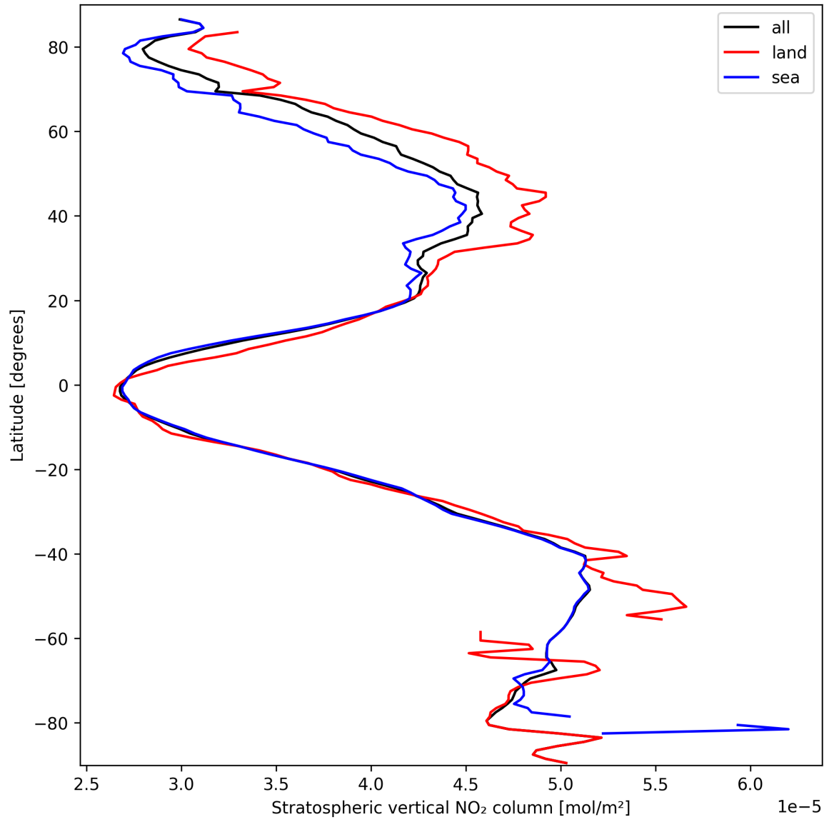
Figure 17: Zonal average of “Stratospheric vertical NO 2 column” for 2025-03-15 to 2025-03-15.
