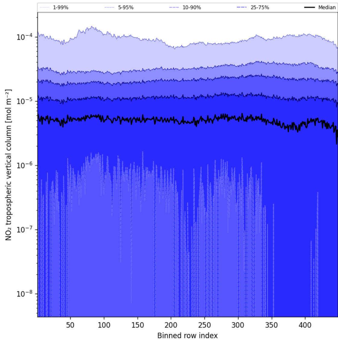
Figure 44: Along track statistics of “NO 2 tropospheric vertical column” for 2025-03-15 to 2025-03-15
