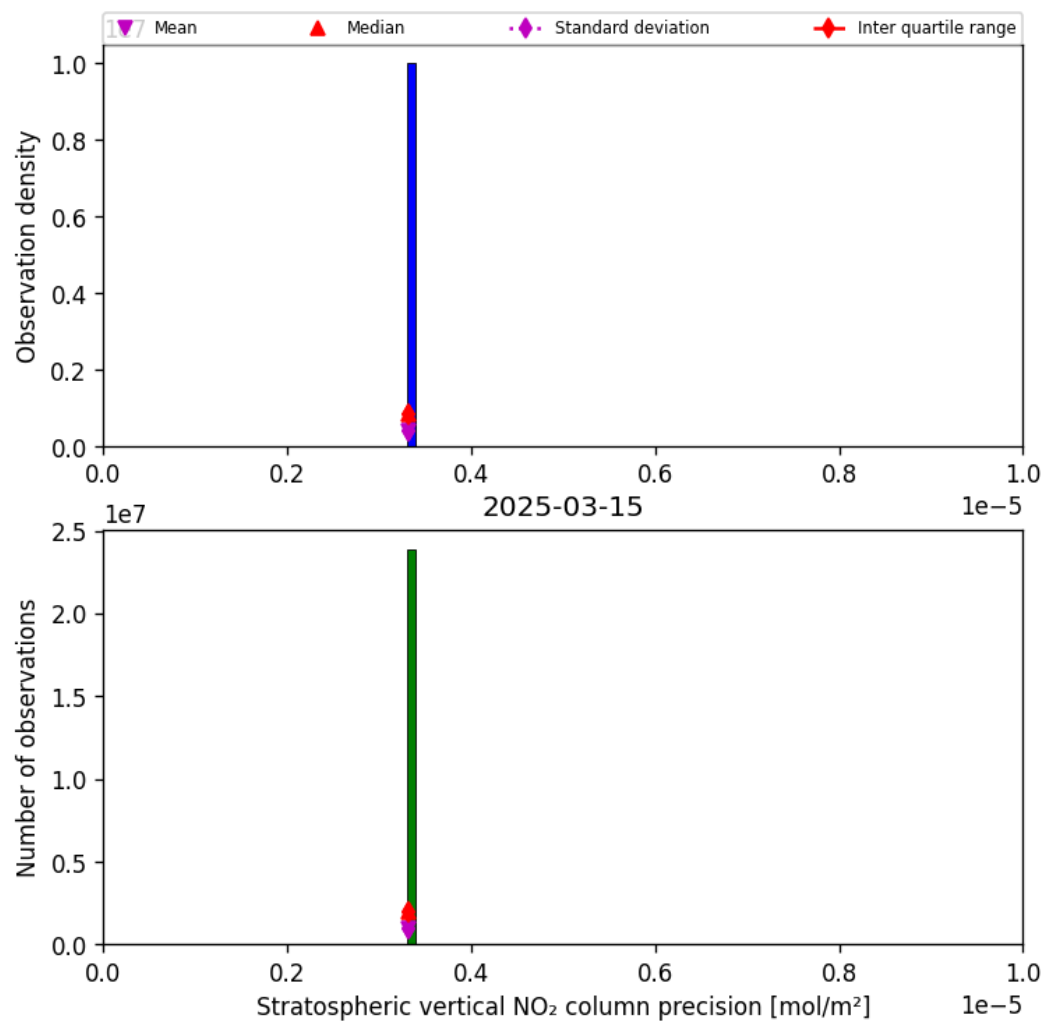
Figure 35: Histogram of “Stratospheric vertical NO 2 column precision” for 2025-03-15 to 2025-03-15
