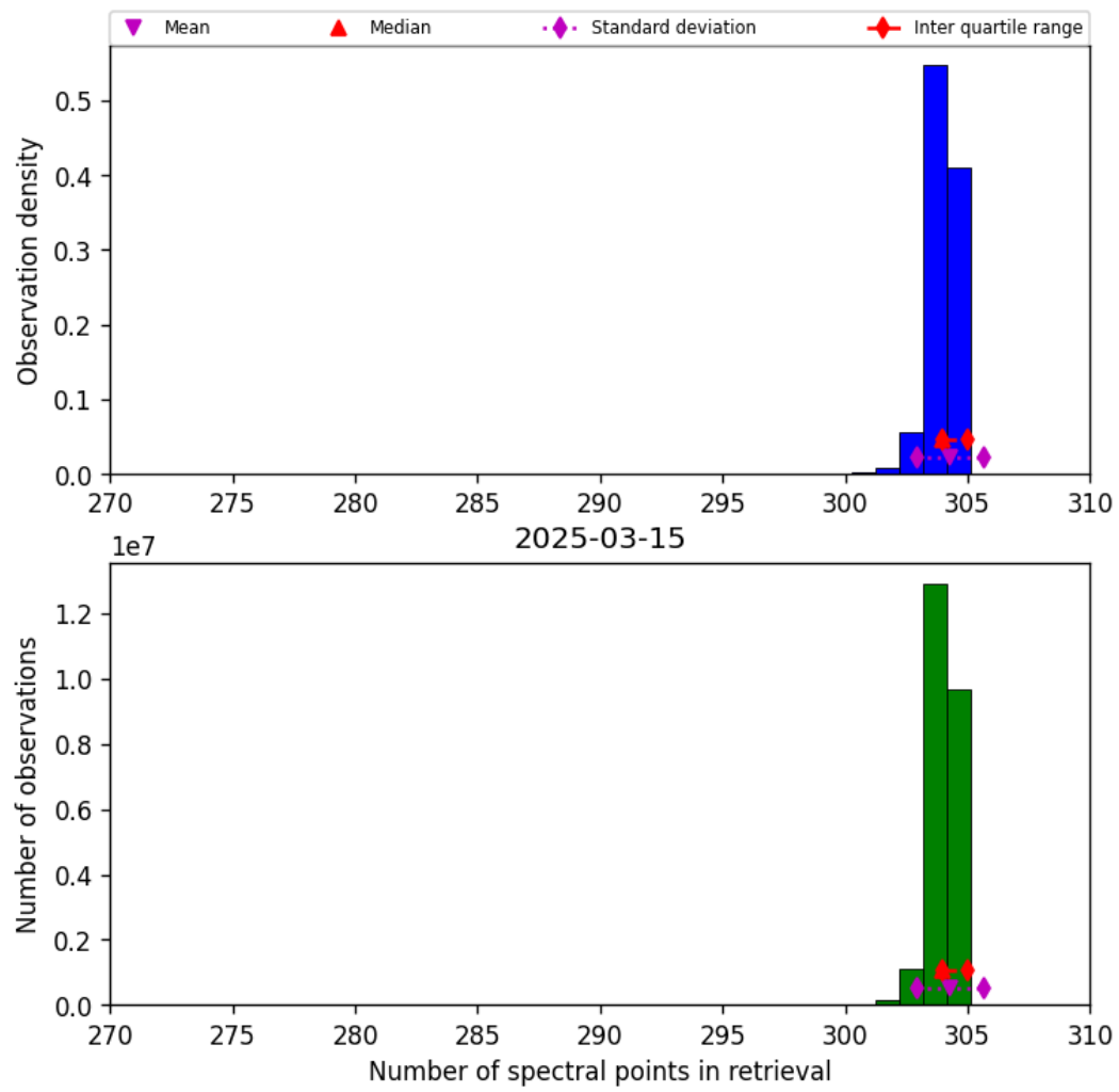
Figure 31: Histogram of “Number of spectral points in retrieval” for 2025-03-15 to 2025-03-15
