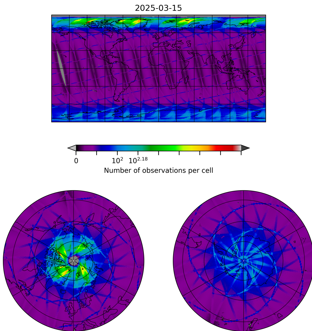
Figure 8: Map of the number of observations for 2025-03-15 to 2025-03-15
