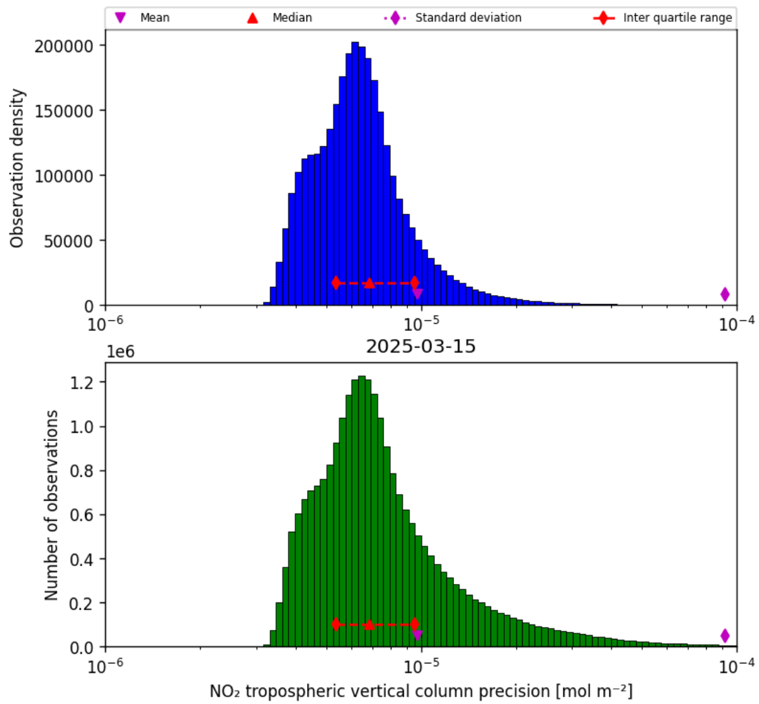
Figure 28: Histogram of “NO 2 tropospheric vertical column precision” for 2025-03-15 to 2025-03-15
