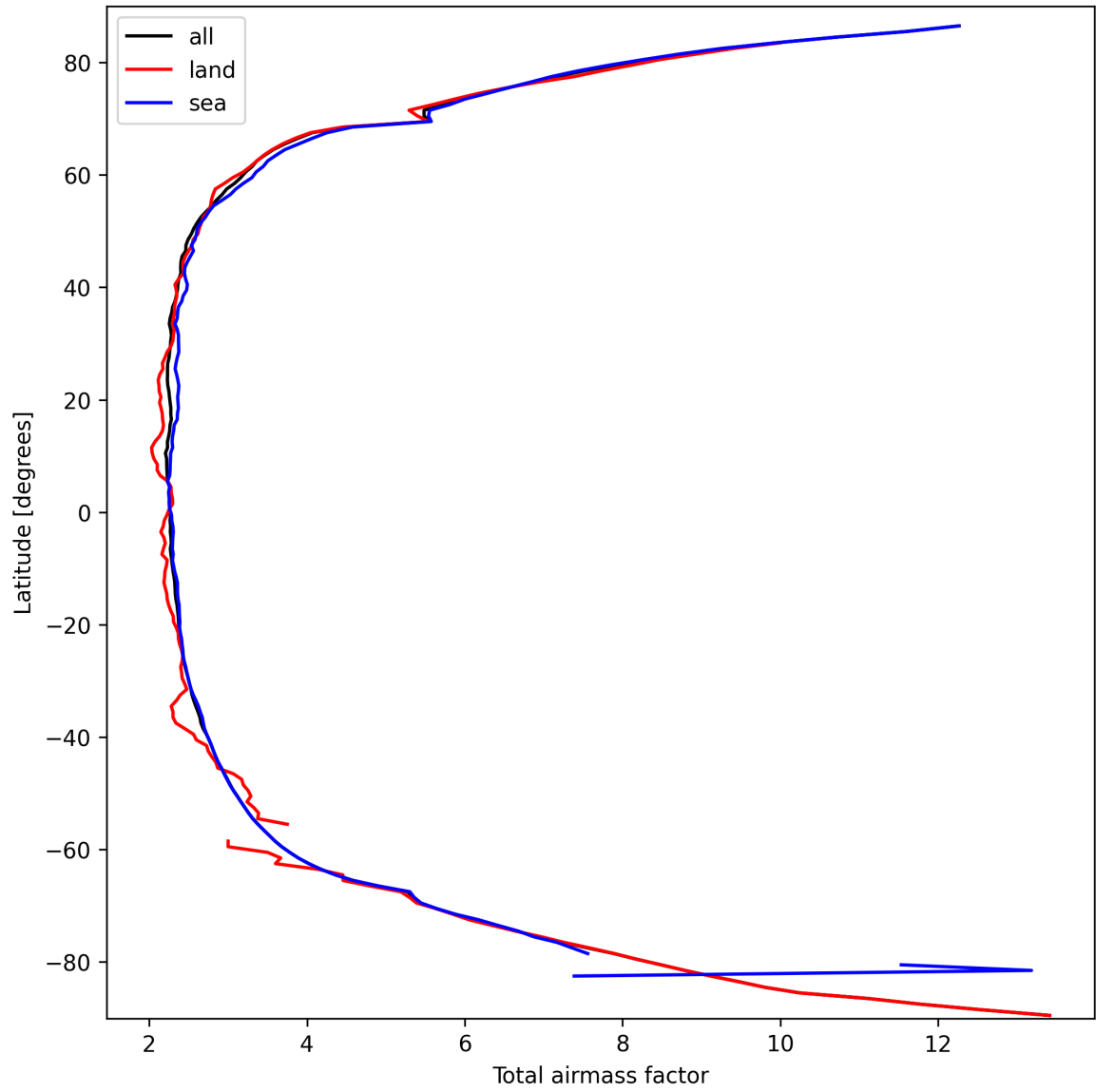
Figure 13: Zonal average of “Total airmass factor” for 2025-03-15 to 2025-03-15.
