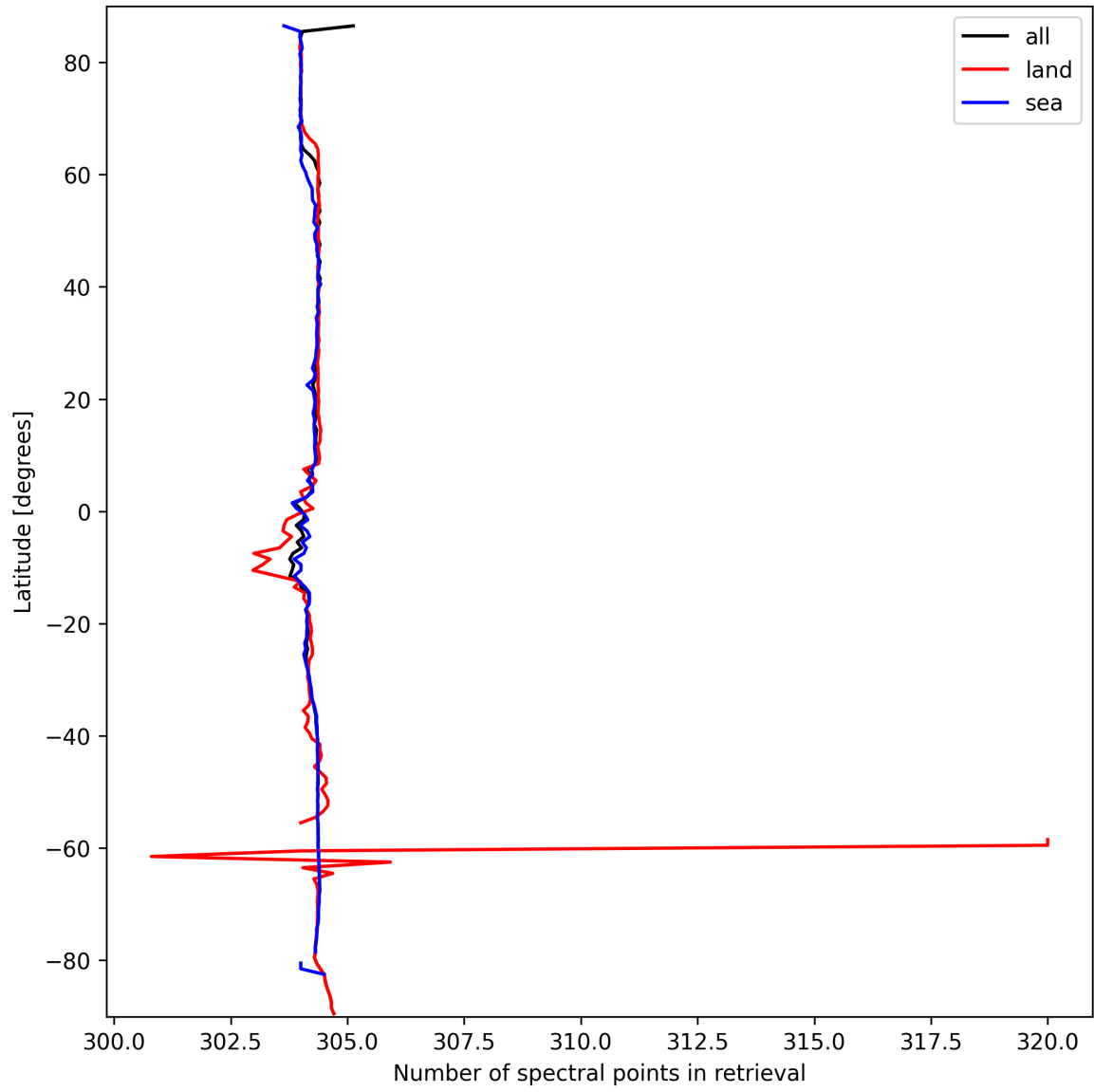
Figure 14: Zonal average of “Number of spectral points in retrieval” for 2025-03-15 to 2025-03-15.
