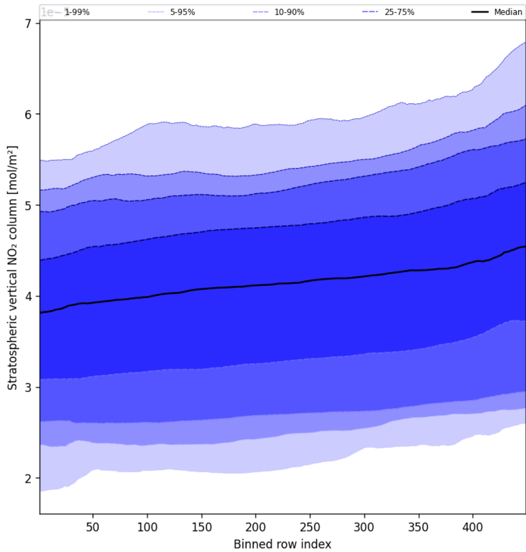
Figure 51: Along track statistics of “Stratospheric vertical NO 2 column” for 2025-03-15 to 2025-03-15
