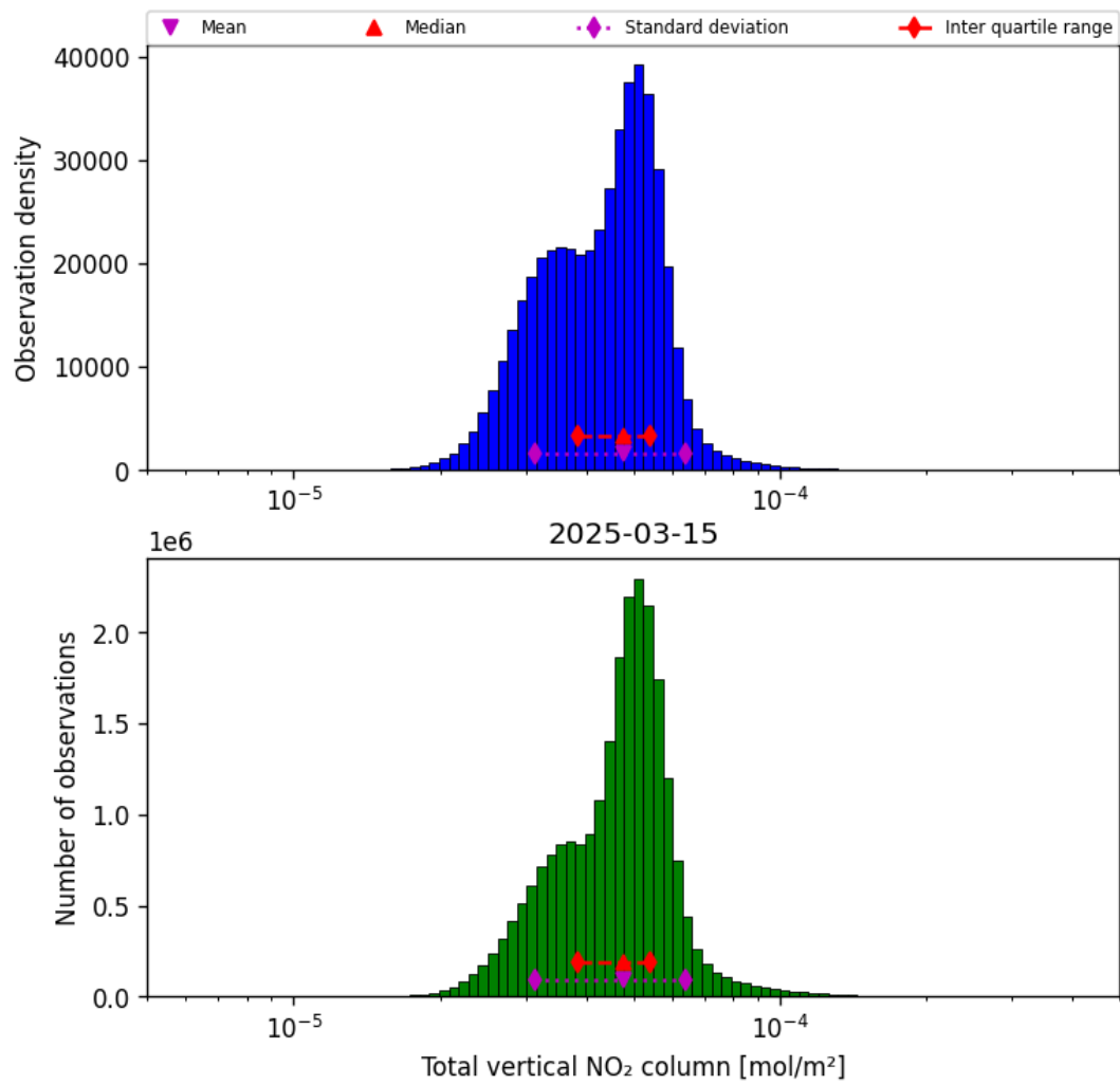
Figure 36: Histogram of "Total vertical NO 2 column" for 2025-03-15 to 2025-03-15
