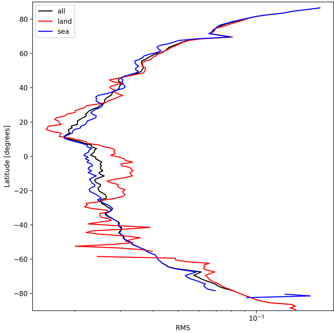
Figure 24: Zonal average of “RMS” for 2025-03-15 to 2025-03-15.
