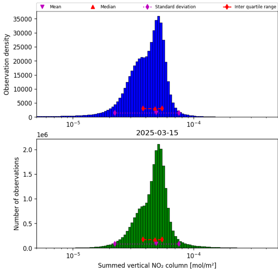
Figure 38: Histogram of “Summed vertical NO 2 column” for 2025-03-15 to 2025-03-15
