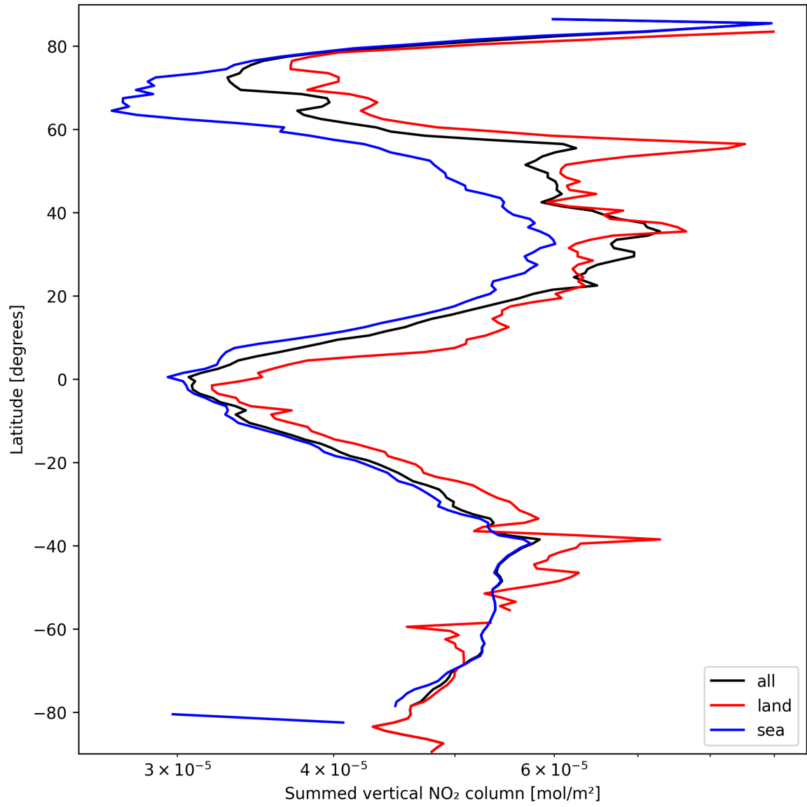
Figure 21: Zonal average of “Summed vertical NO 2 column” for 2025-03-15 to 2025-03-15.
