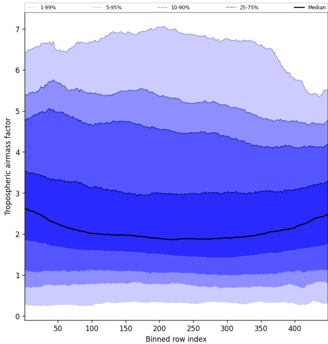
Figure 46: Along track statistics of “Tropospheric air mass factor” for 2025-03-15 to 2025-03-15
