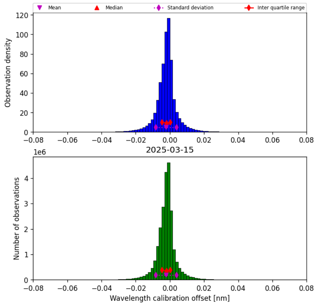
Figure 33: Histogram of “Wavelength calibration offset” for 2025-03-15 to 2025-03-15
