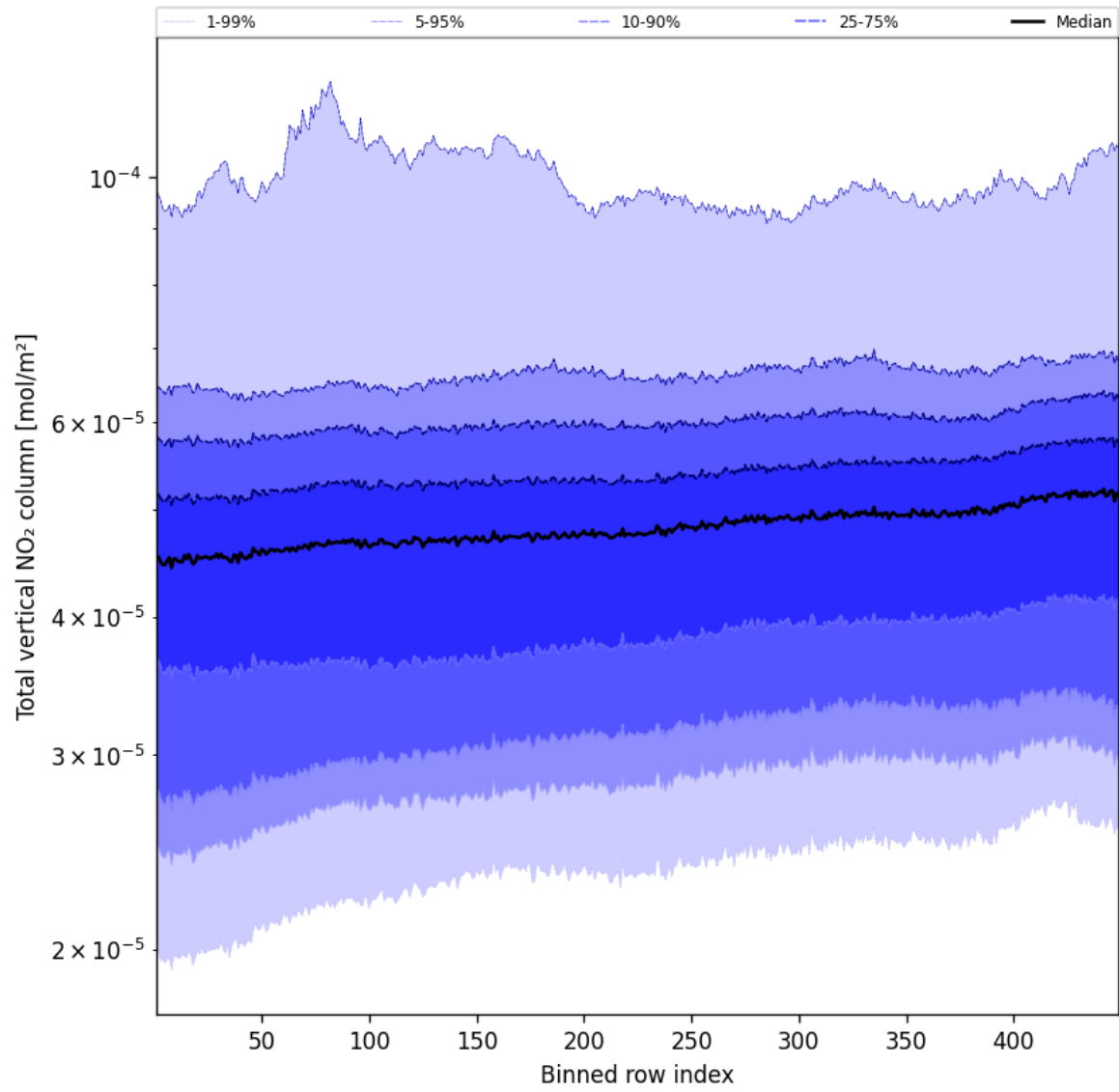
Figure 53: Along track statistics of “Total vertical NO 2 column” for 2025-03-15 to 2025-03-15
