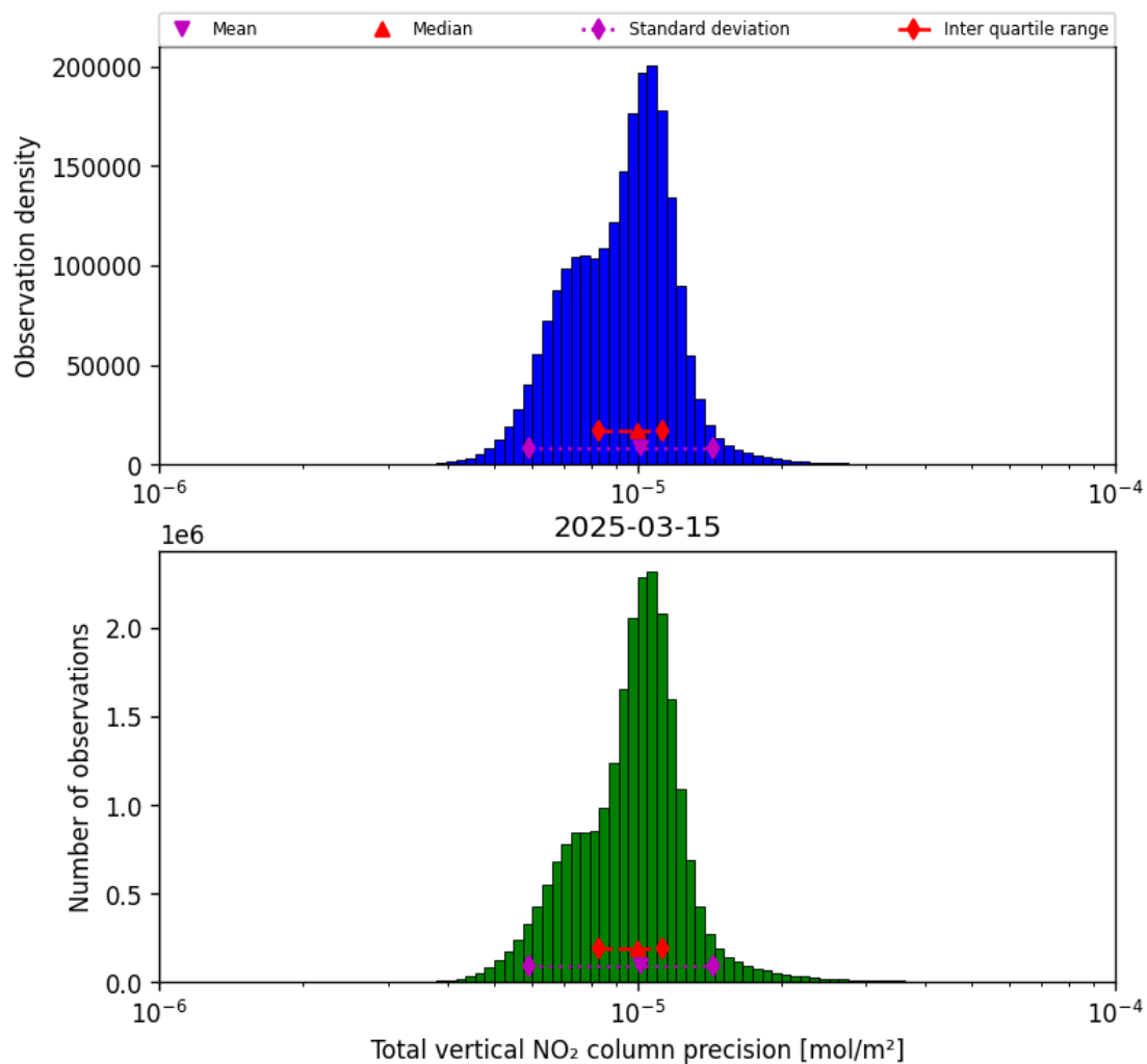
Figure 37: Histogram of “Total vertical NO 2 column precision” for 2025-03-15 to 2025-03-15
