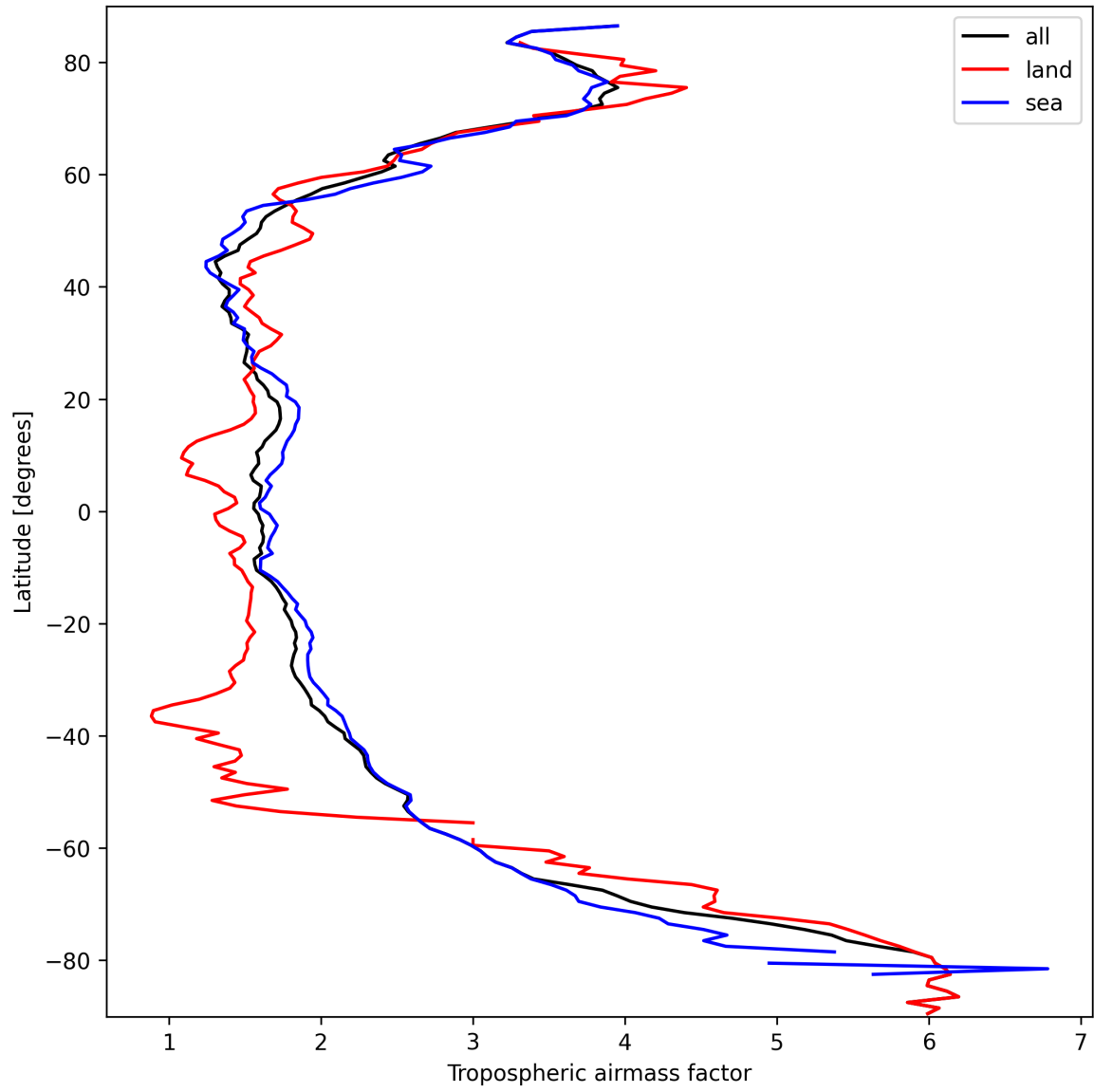
Figure 12: Zonal average of “Tropospheric air mass factor” for 2025-03-15 to 2025-03-15.
