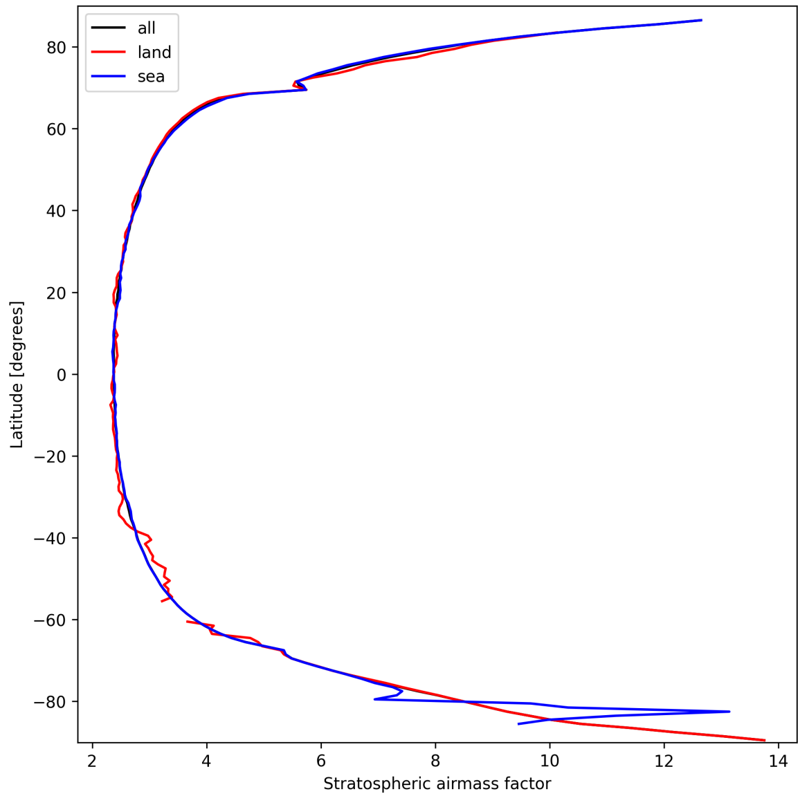
Figure 25: Zonal average of “Stratospheric airmass factor” for 2025-03-16 to 2025-03-17.
