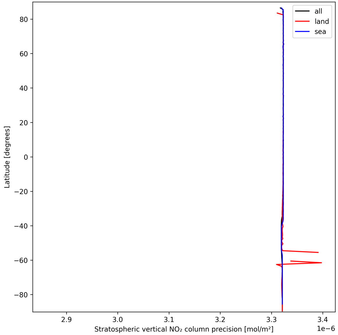
Figure 18: Zonal average of “Stratospheric vertical NO 2 column precision” for 2025-03-16 to 2025-03-17.
