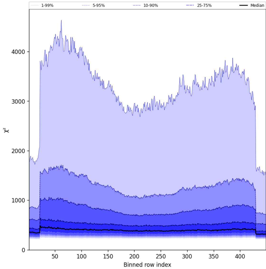
Figure 57: Along track statistics of “ \chi^2 ” for 2025-03-16 to 2025-03-17
