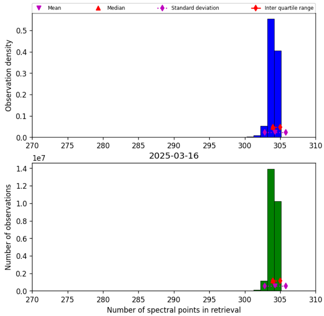
Figure 31: Histogram of “Number of spectral points in retrieval” for 2025-03-16 to 2025-03-17
