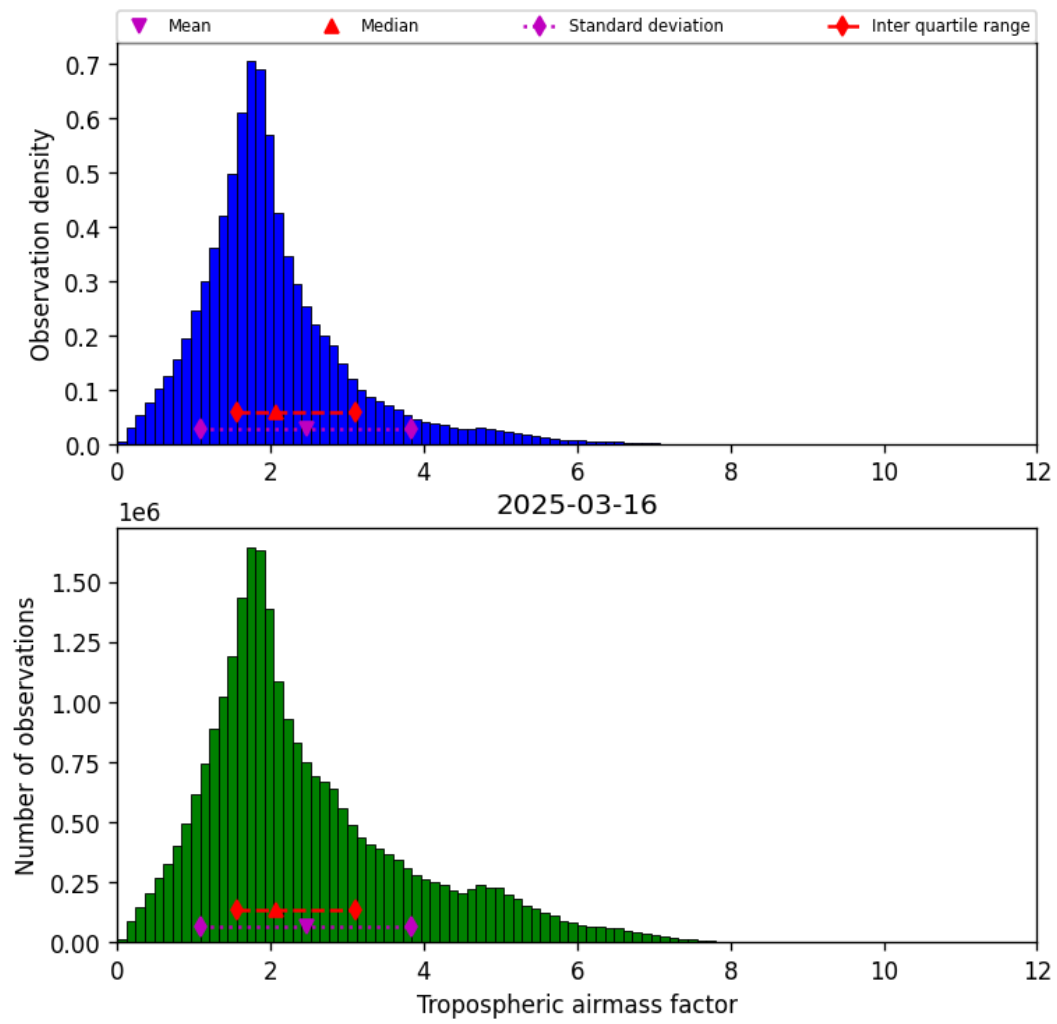
Figure 29: Histogram of “Tropospheric airmass factor” for 2025-03-16 to 2025-03-17
