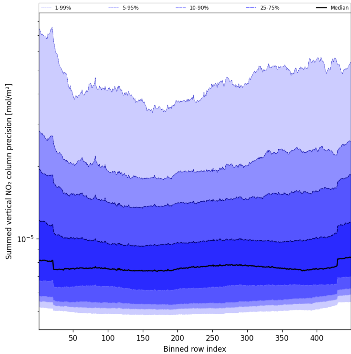
Figure 56: Along track statistics of “Summed vertical NO 2 column precision” for 2025-03-16 to 2025-03-17
