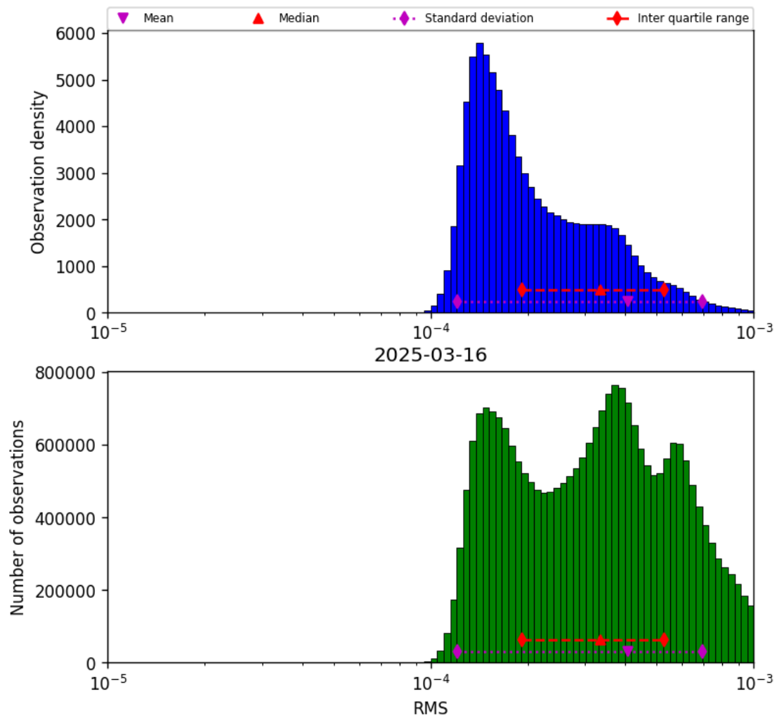
Figure 41: Histogram of “RMS” for 2025-03-16 to 2025-03-17
