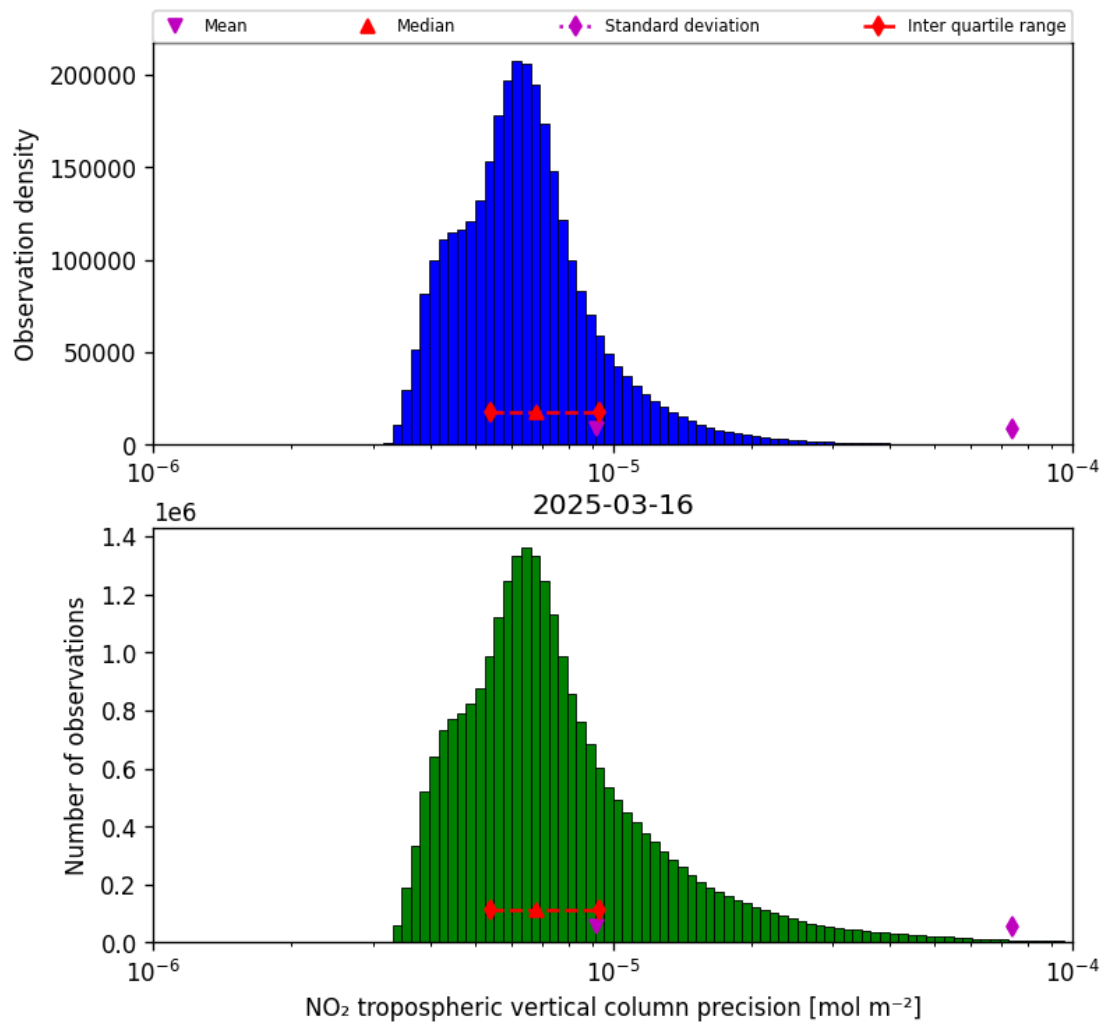
Figure 28: Histogram of “NO 2 tropospheric vertical column precision” for 2025-03-16 to 2025-03-17
