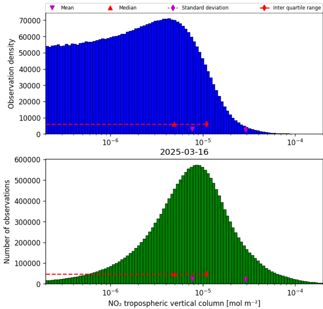
Figure 27: Histogram of “NO 2 tropospheric vertical column” for 2025-03-16 to 2025-03-17
