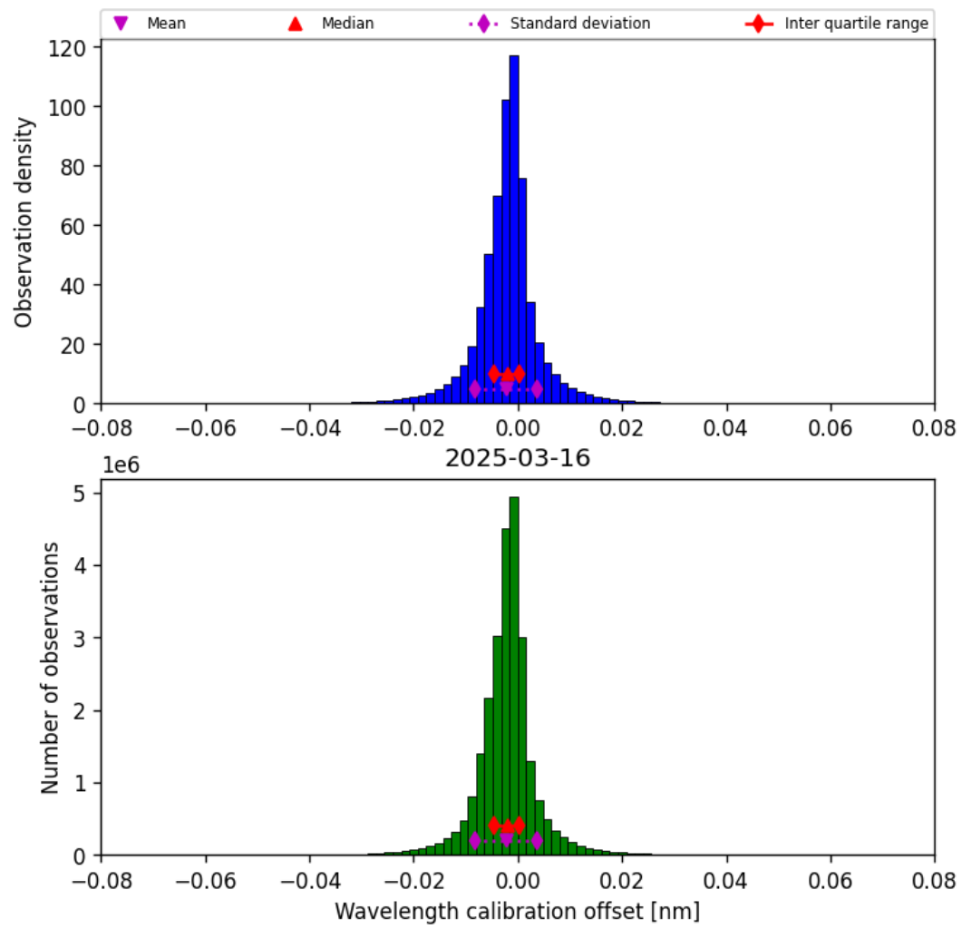
Figure 33: Histogram of “Wavelength calibration offset” for 2025-03-16 to 2025-03-17
