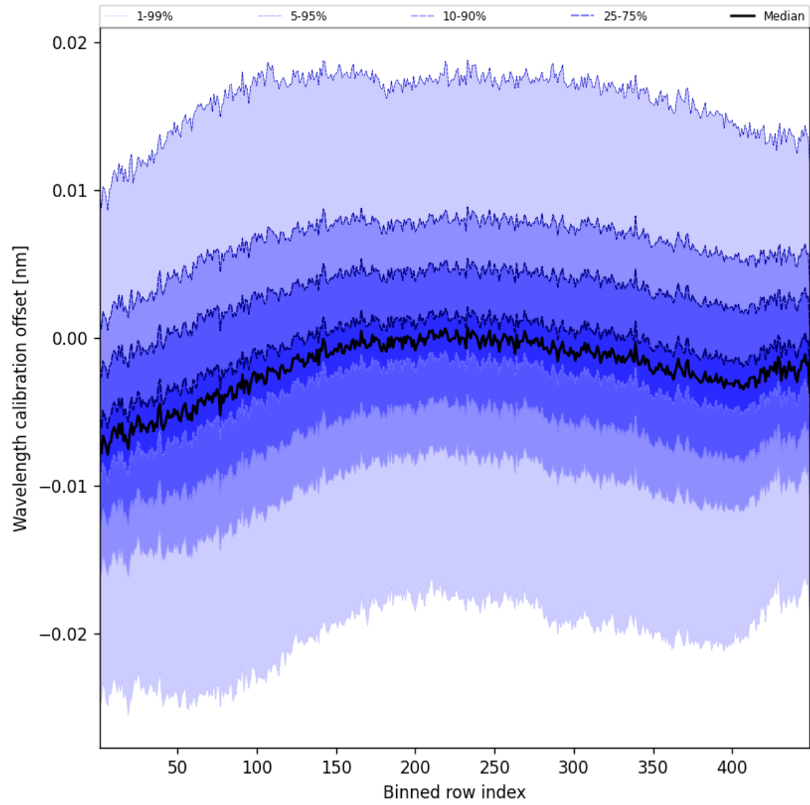
Figure 50: Along track statistics of “Wavelength calibration offset” for 2025-03-16 to 2025-03-17
