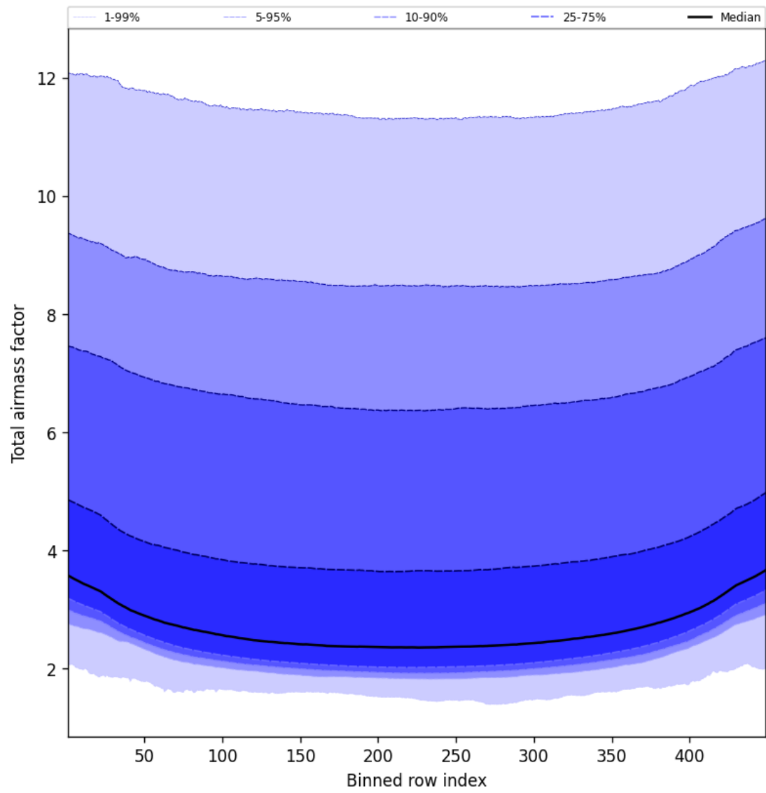
Figure 47: Along track statistics of “Total airmass factor” for 2025-03-16 to 2025-03-17
