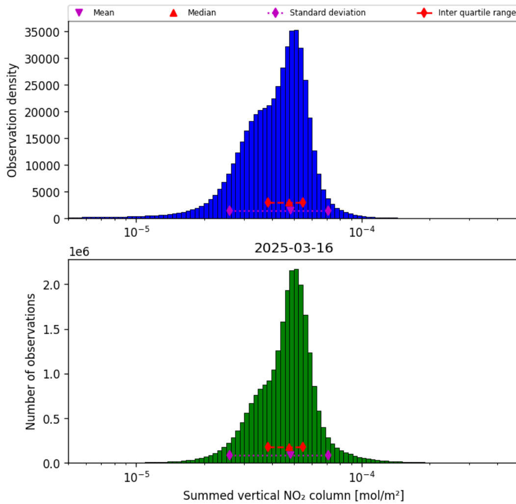
Figure 38: Histogram of “Summed vertical NO 2 column” for 2025-03-16 to 2025-03-17
