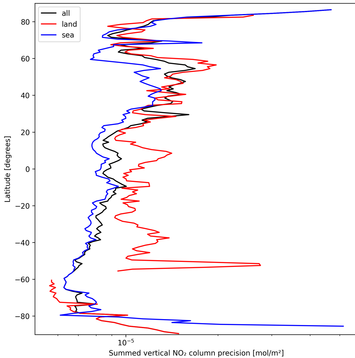
Figure 22: Zonal average of “Summed vertical NO 2 column precision” for 2025-03-16 to 2025-03-17.
