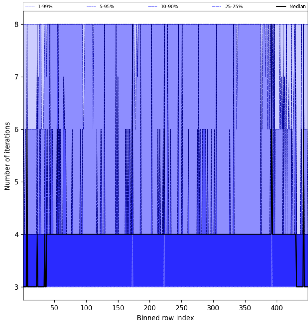
Figure 49: Along track statistics of “Number of iterations” for 2025-03-16 to 2025-03-17
