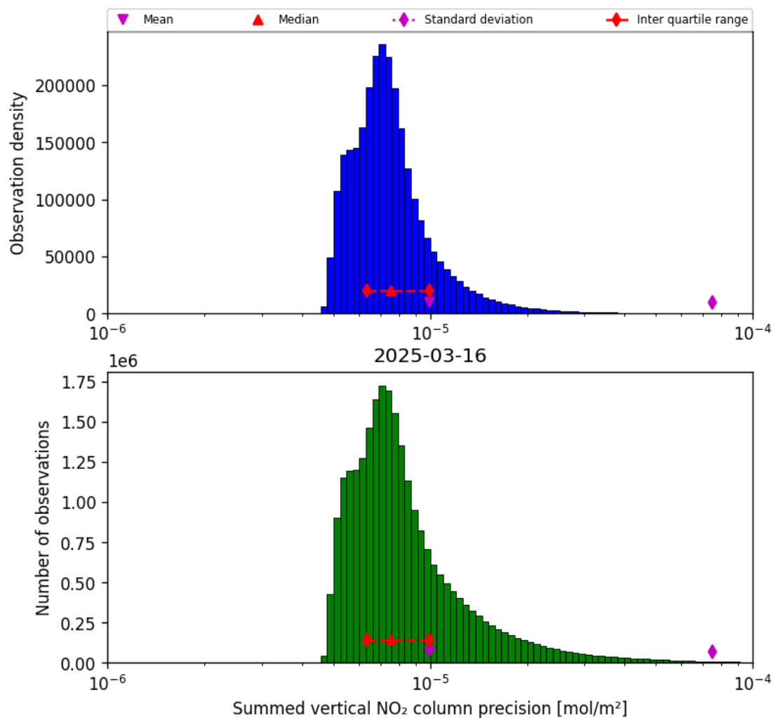
Figure 39: Histogram of “Summed vertical NO 2 column precision” for 2025-03-16 to 2025-03-17
