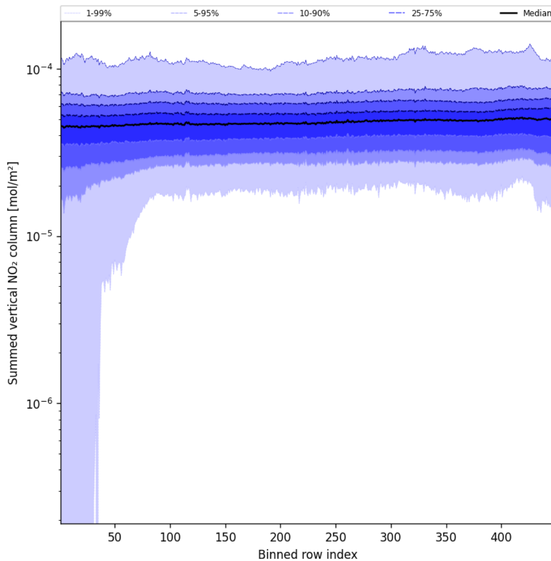
Figure 55: Along track statistics of “Summed vertical NO 2 column” for 2025-03-16 to 2025-03-17
