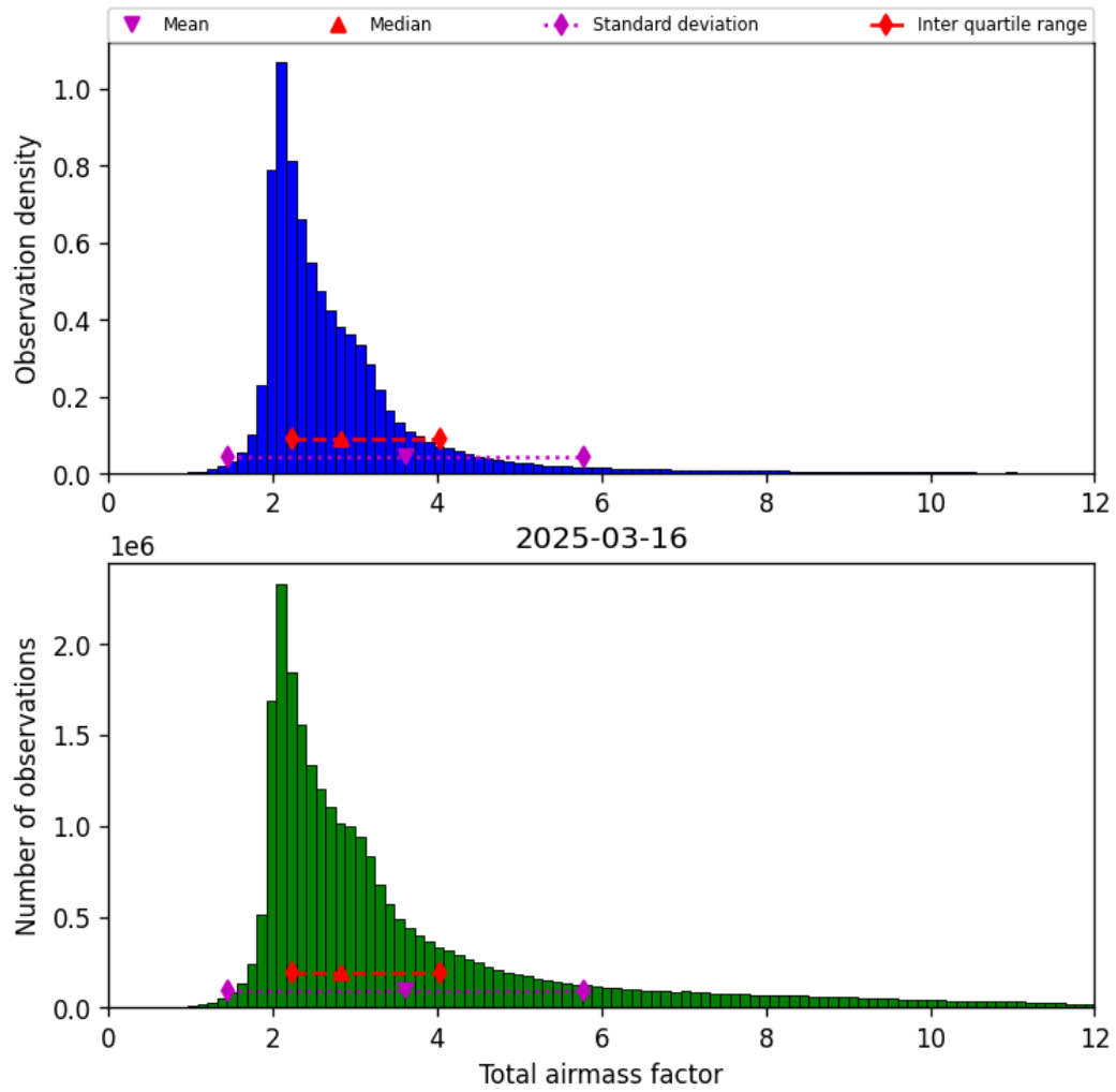
Figure 30: Histogram of “Total airmass factor” for 2025-03-16 to 2025-03-17
