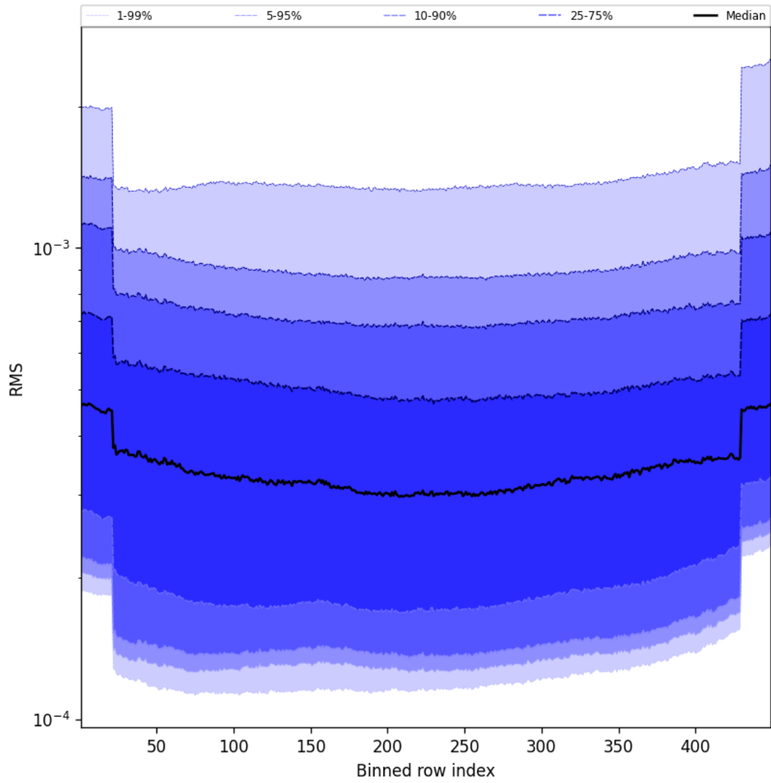
Figure 58: Along track statistics of “RMS” for 2025-03-16 to 2025-03-17
