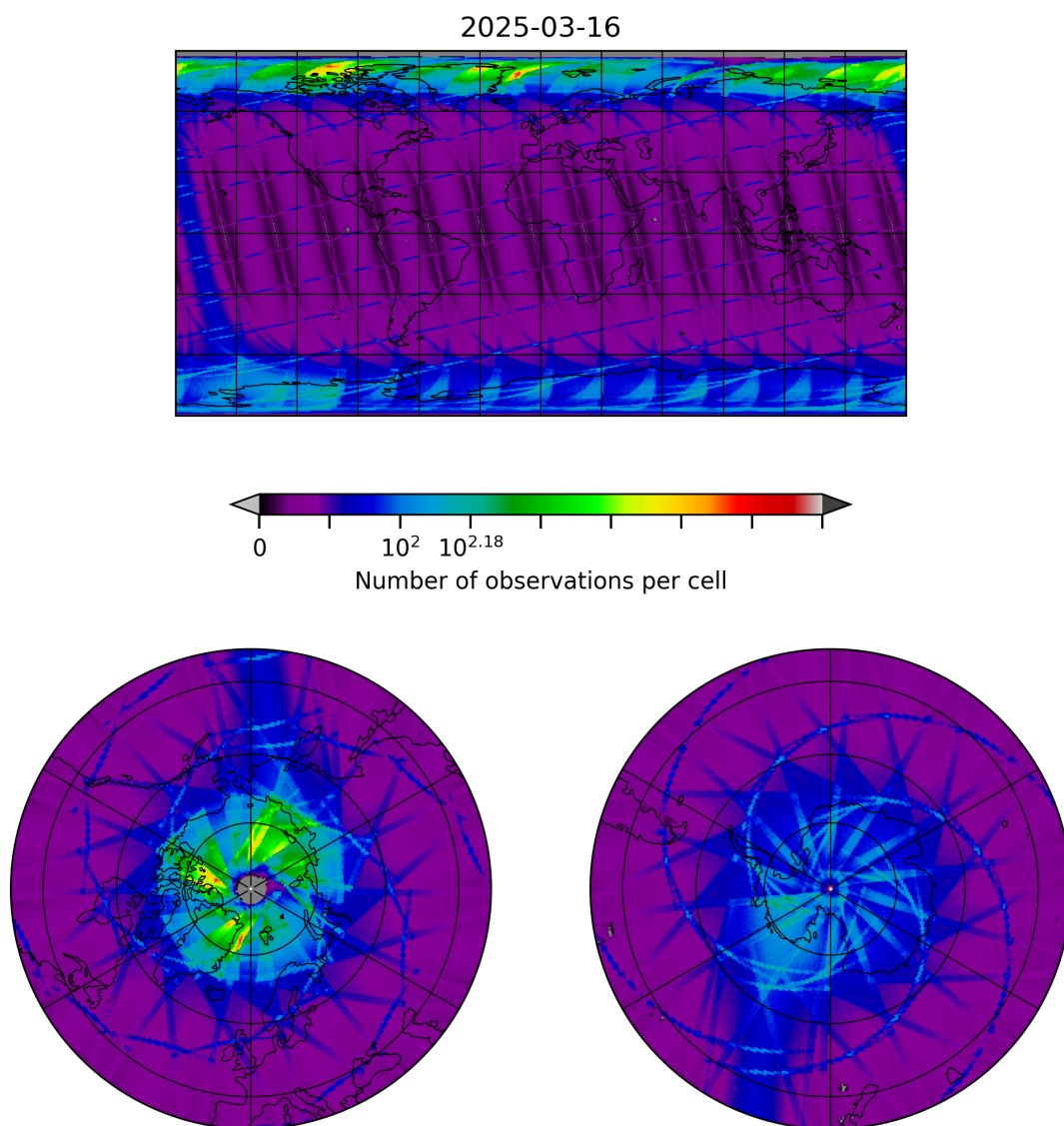
Figure 8: Map of the number of observations for 2025-03-16 to 2025-03-17
