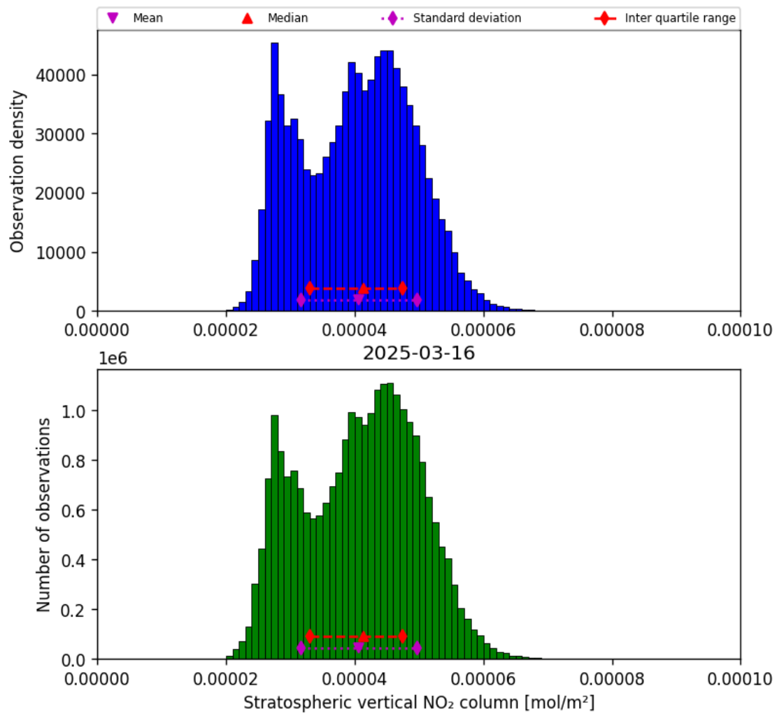
Figure 34: Histogram of “Stratospheric vertical NO 2 column” for 2025-03-16 to 2025-03-17
