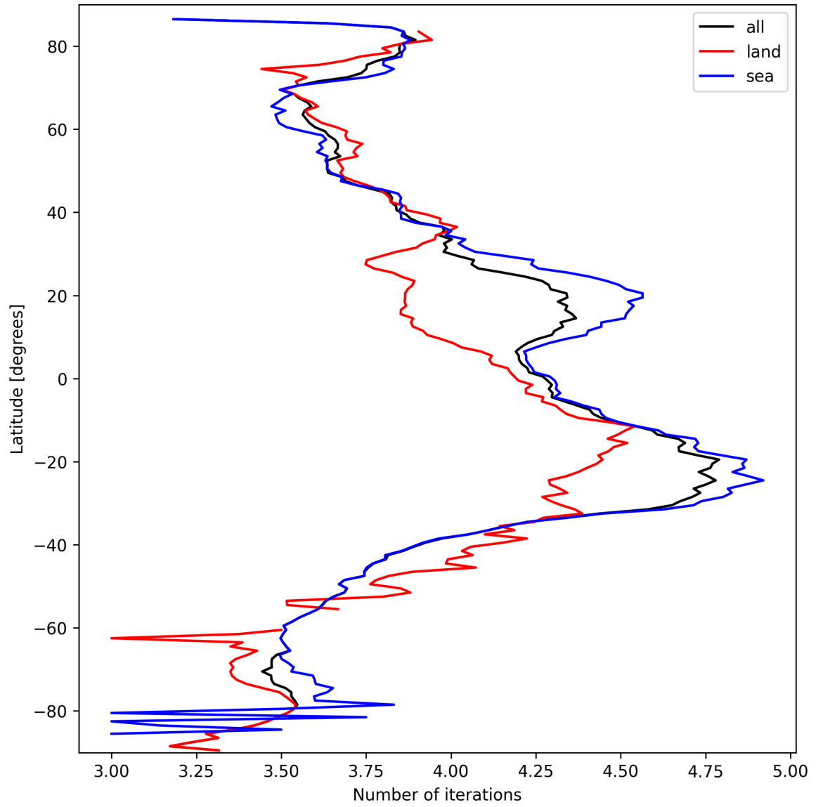
Figure 15: Zonal average of “Number of iterations” for 2025-03-16 to 2025-03-17.
