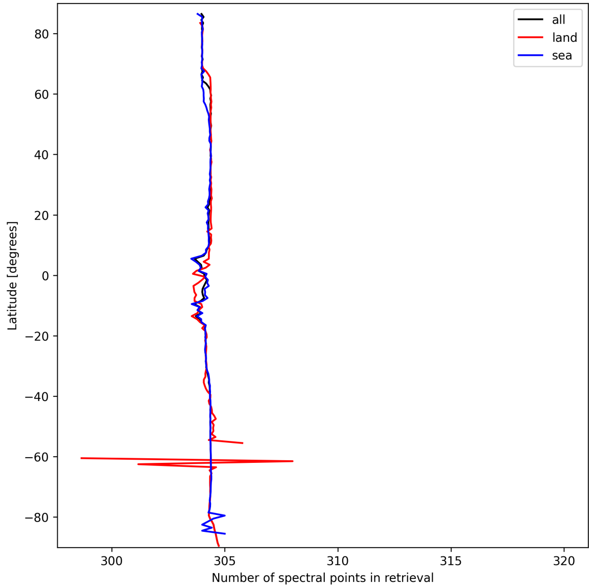
Figure 14: Zonal average of “Number of spectral points in retrieval” for 2025-03-16 to 2025-03-17.
