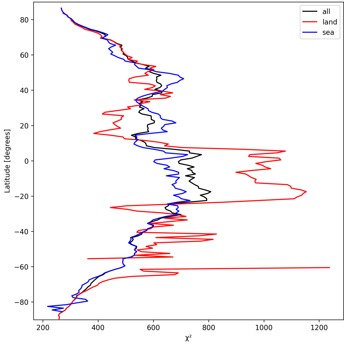
Figure 23: Zonal average of “ \chi^2 ” for 2025-03-16 to 2025-03-17.
