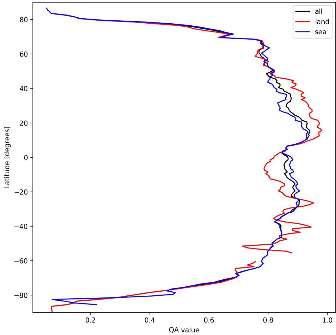
Figure 9: Zonal average of “QA value” for 2025-03-16 to 2025-03-17.
