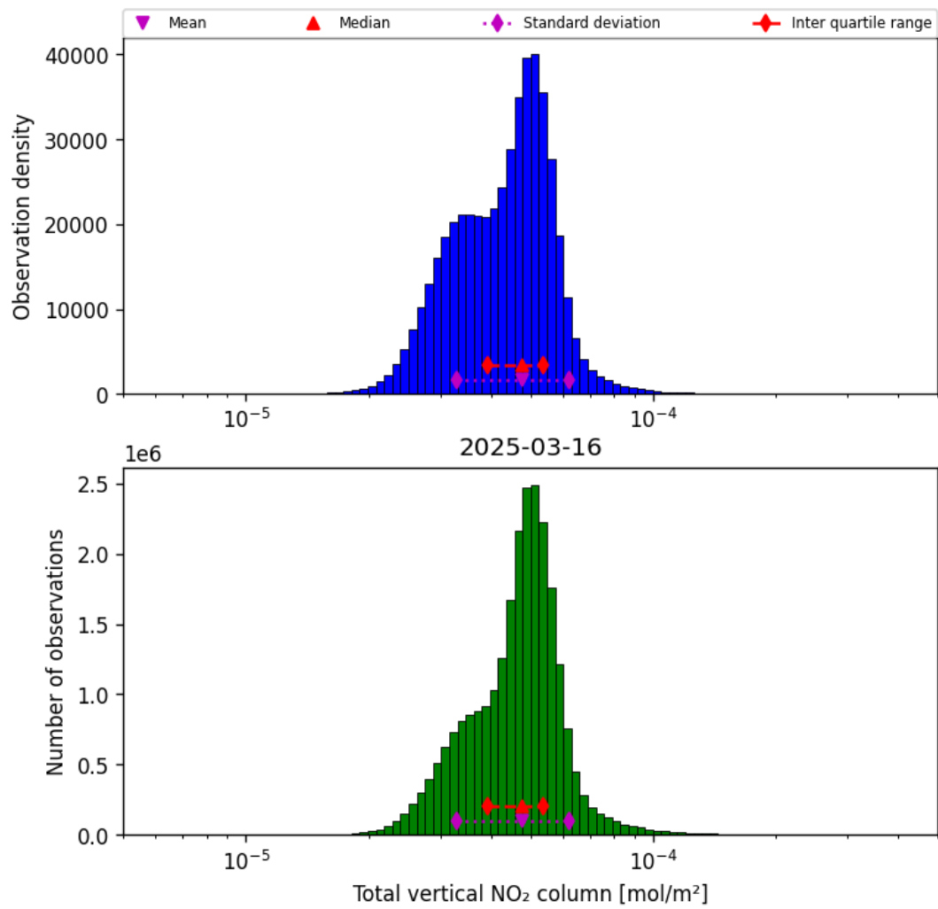
Figure 36: Histogram of “Total vertical NO 2 column” for 2025-03-16 to 2025-03-17
