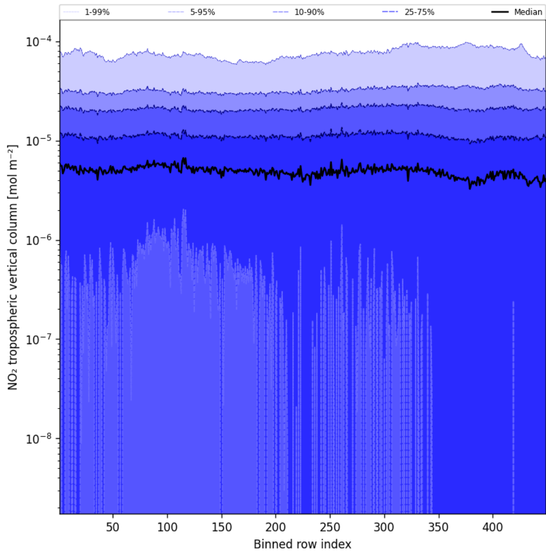
Figure 44: Along track statistics of “NO 2 tropospheric vertical column” for 2025-03-16 to 2025-03-17
