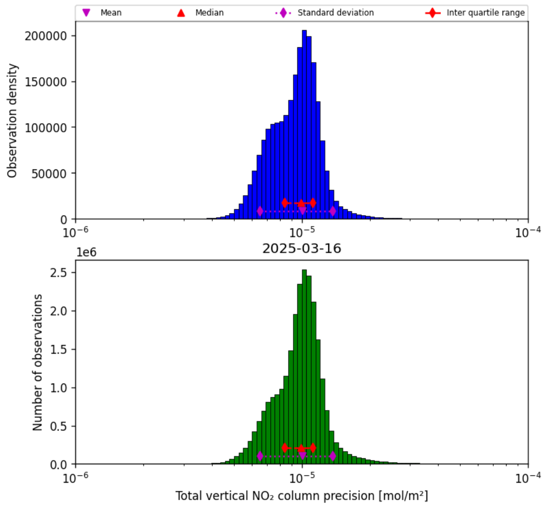
Figure 37: Histogram of “Total vertical NO 2 column precision” for 2025-03-16 to 2025-03-17
