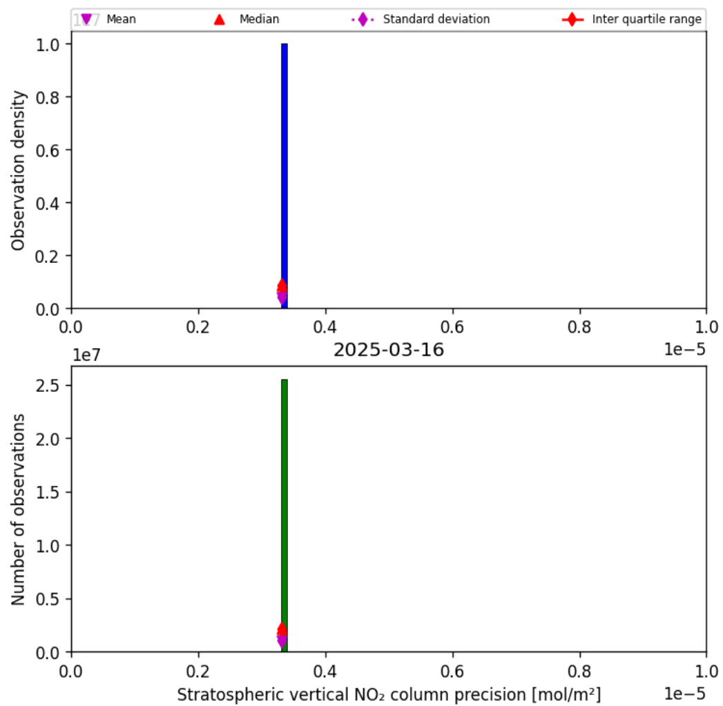
Figure 35: Histogram of “Stratospheric vertical NO 2 column precision” for 2025-03-16 to 2025-03-17
