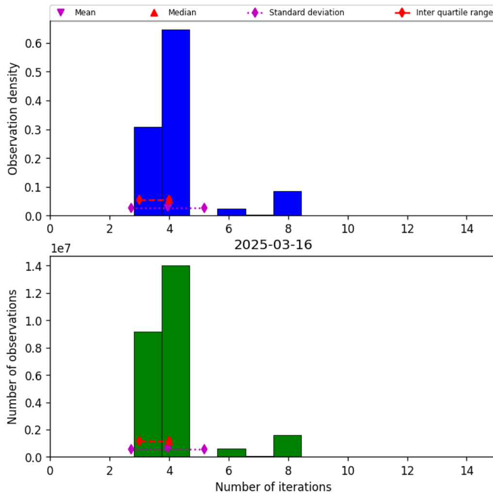
Figure 32: Histogram of “Number of iterations” for 2025-03-16 to 2025-03-17
