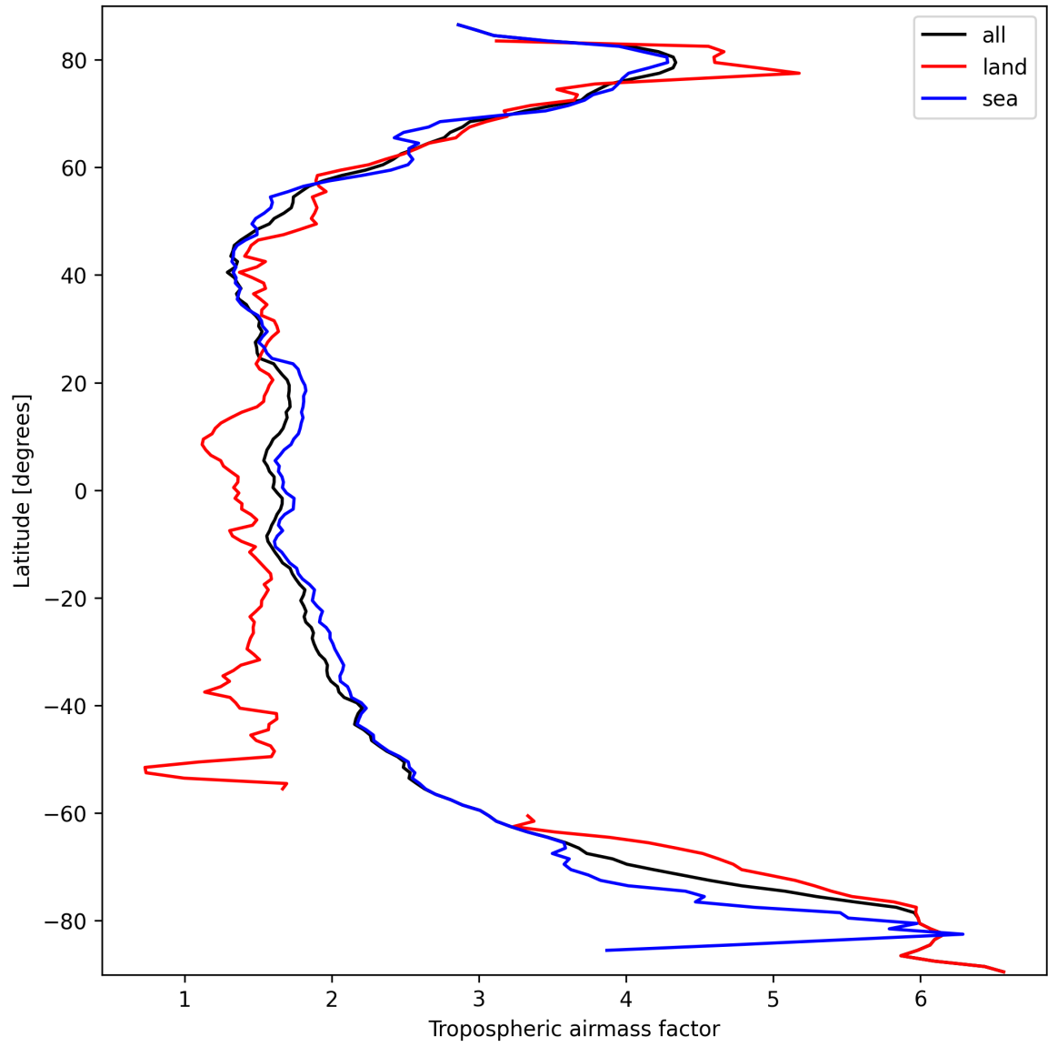
Figure 12: Zonal average of “Tropospheric airmass factor” for 2025-03-16 to 2025-03-17.
