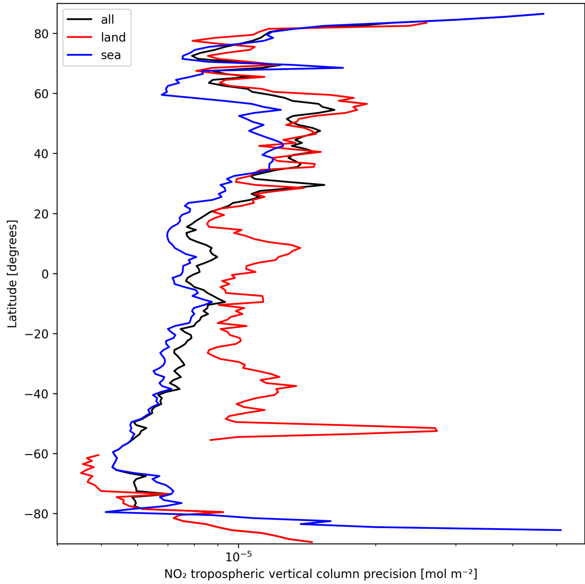
Figure 11: Zonal average of “NO 2 tropospheric vertical column precision” for 2025-03-16 to 2025-03-17.
