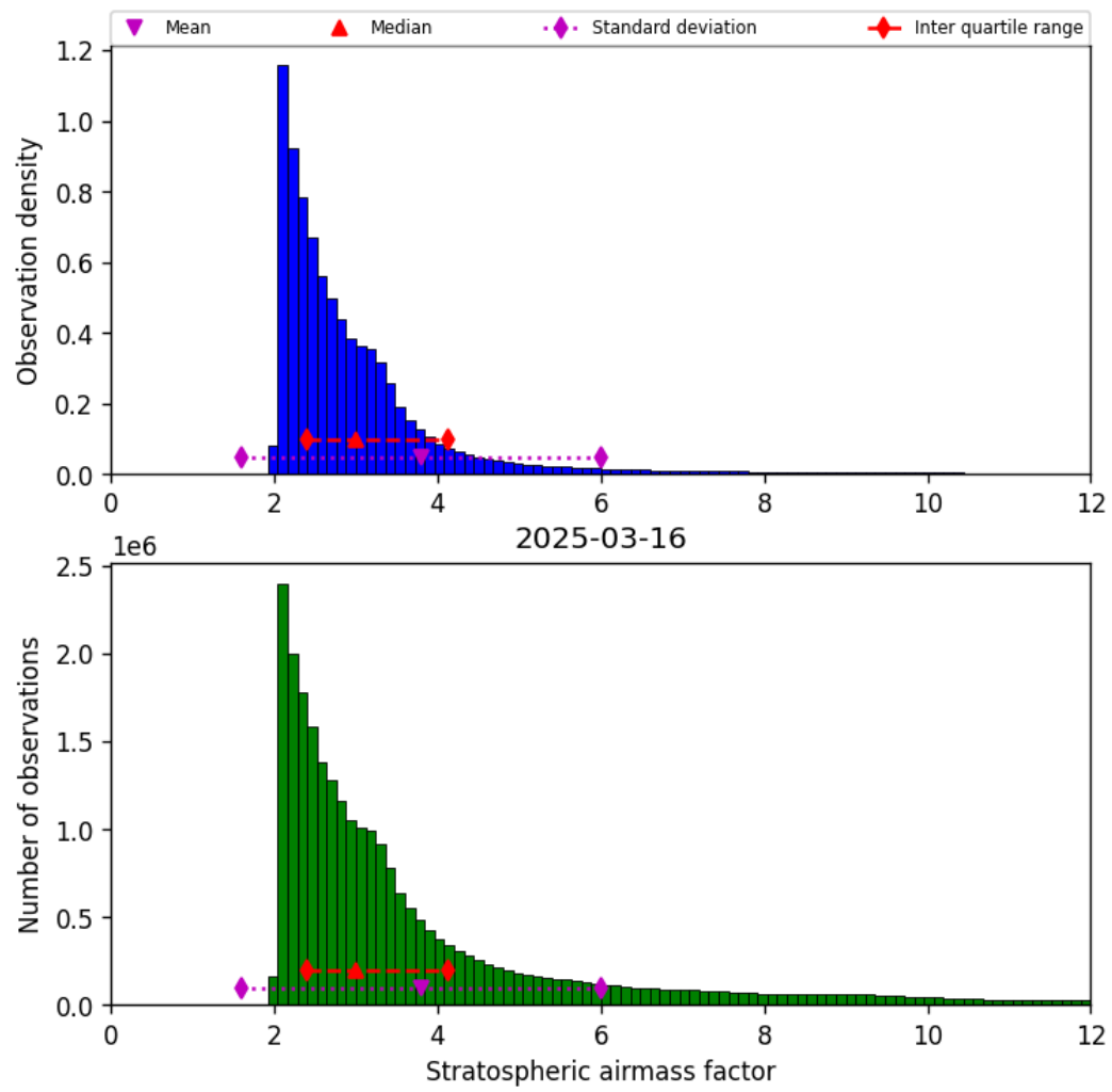
Figure 42: Histogram of “Stratospheric airmass factor” for 2025-03-16 to 2025-03-17
