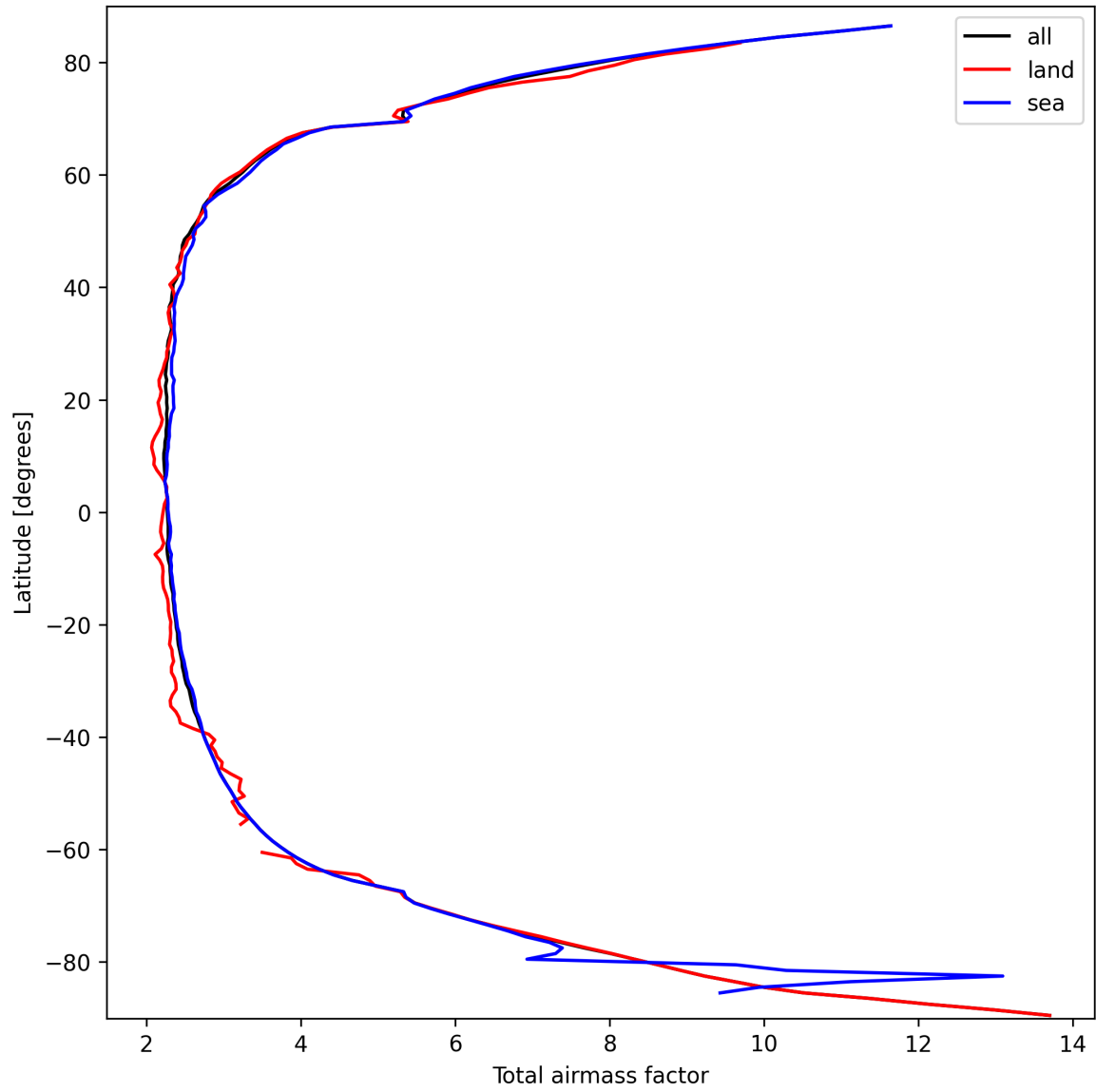
Figure 13: Zonal average of “Total airmass factor” for 2025-03-16 to 2025-03-17.
