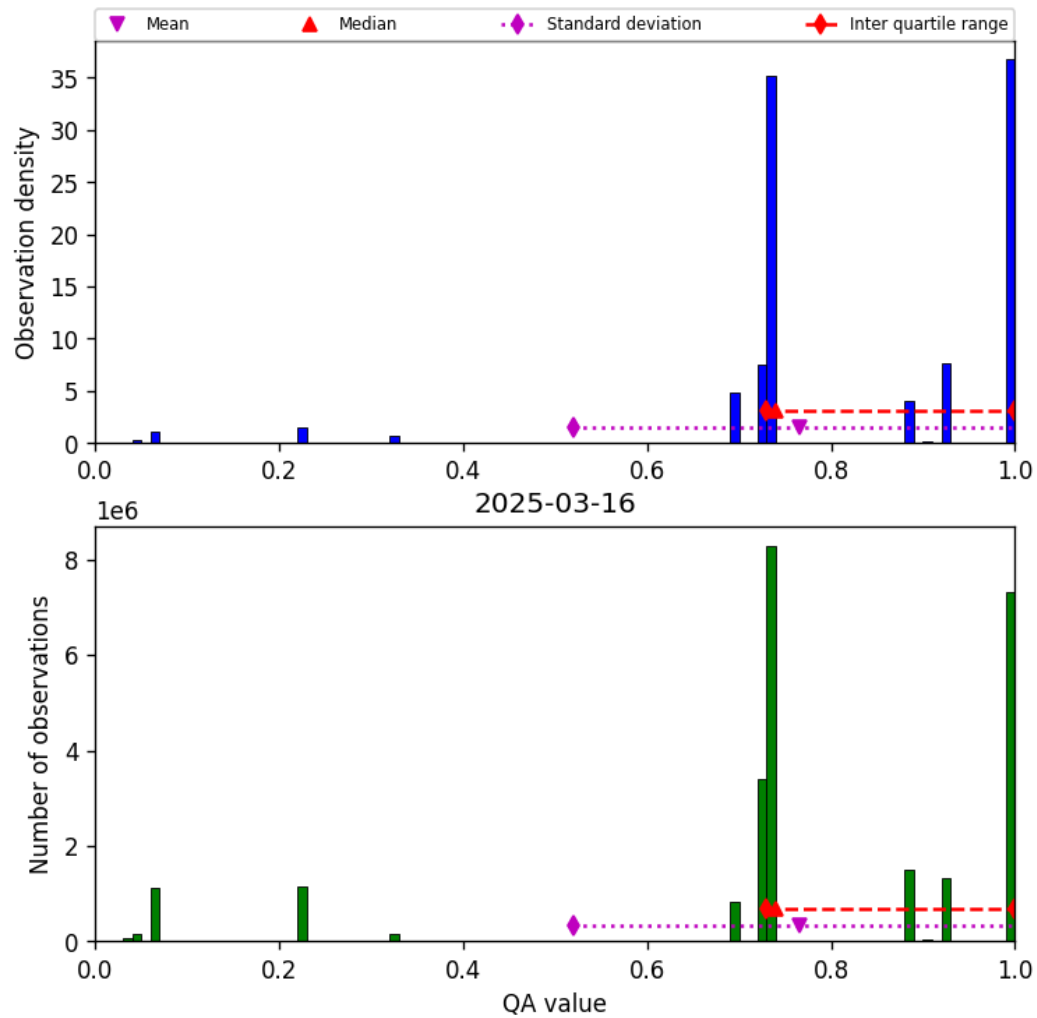
Figure 26: Histogram of “QA value” for 2025-03-16 to 2025-03-17
