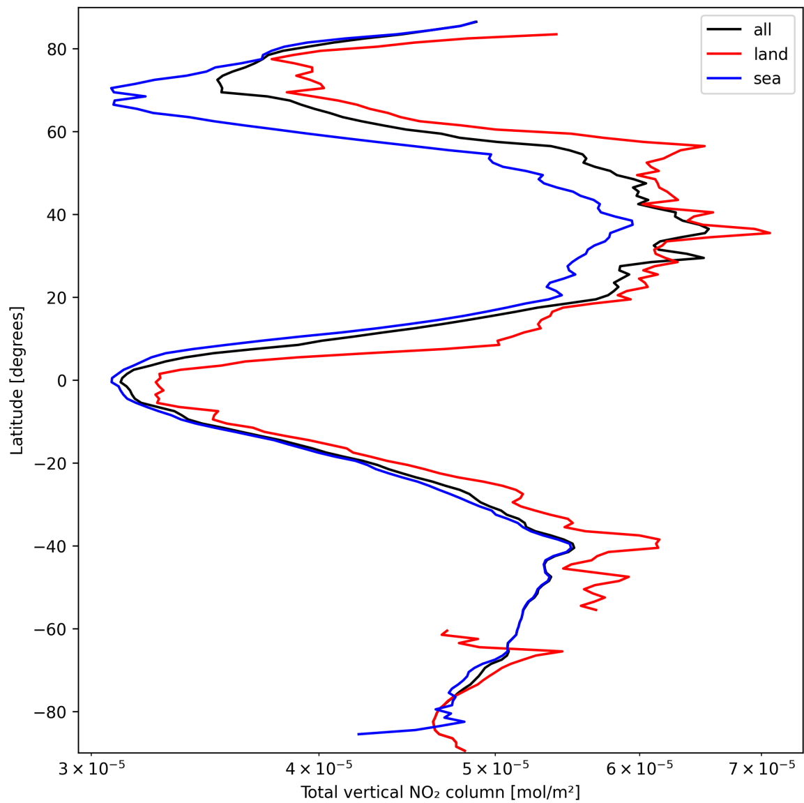
Figure 19: Zonal average of “Total vertical NO 2 column” for 2025-03-16 to 2025-03-17.
