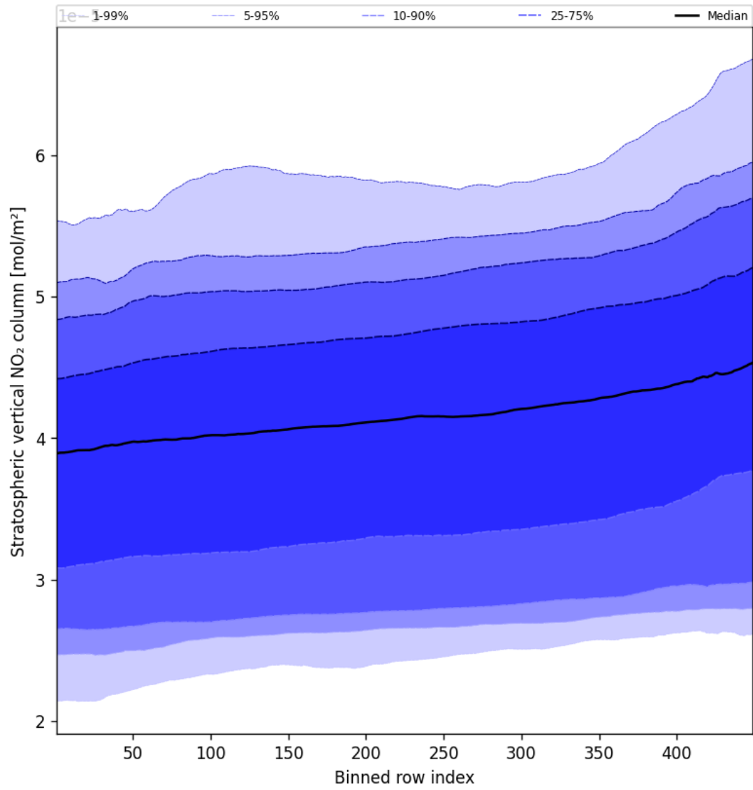
Figure 51: Along track statistics of “Stratospheric vertical NO 2 column” for 2025-03-16 to 2025-03-17
