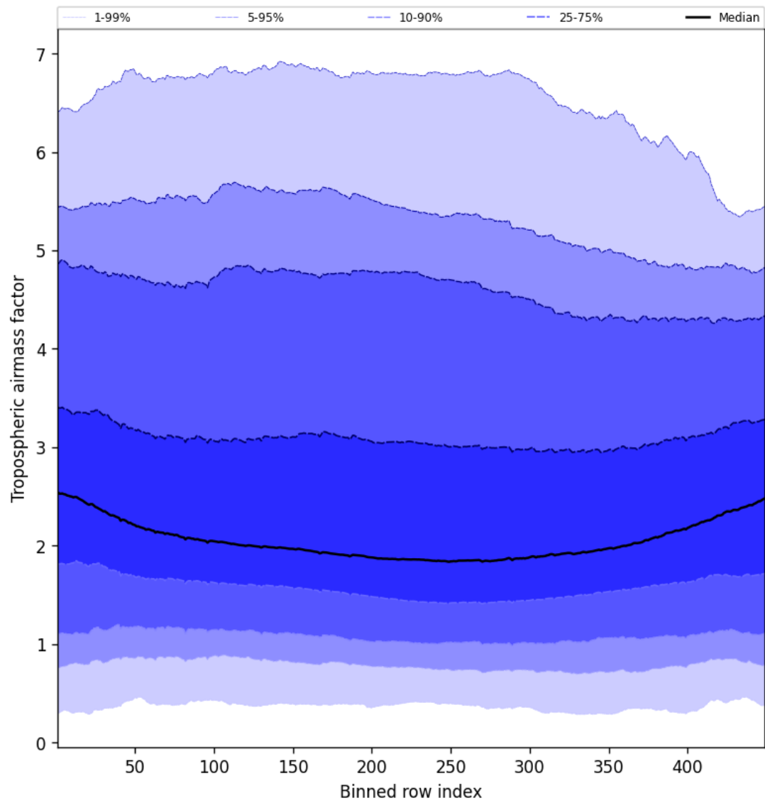
Figure 46: Along track statistics of “Tropospheric air mass factor” for 2025-03-16 to 2025-03-17
