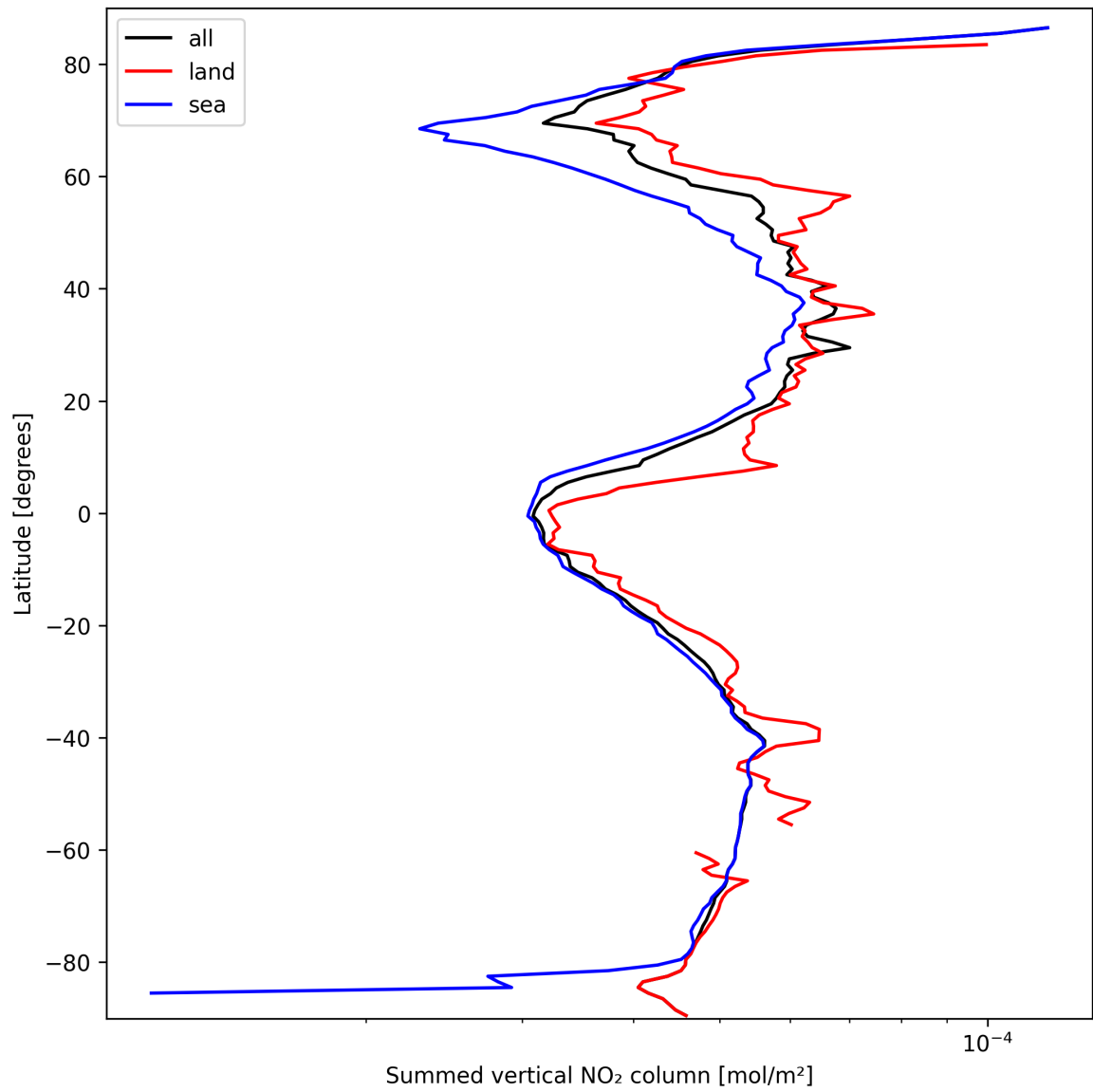
Figure 21: Zonal average of “Summed vertical NO 2 column” for 2025-03-16 to 2025-03-17.
