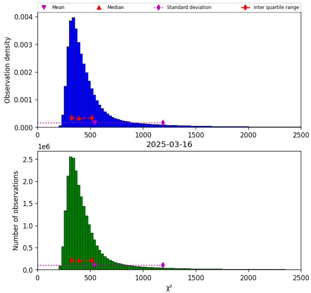
Figure 40: Histogram of “ \chi^2 ” for 2025-03-16 to 2025-03-17
