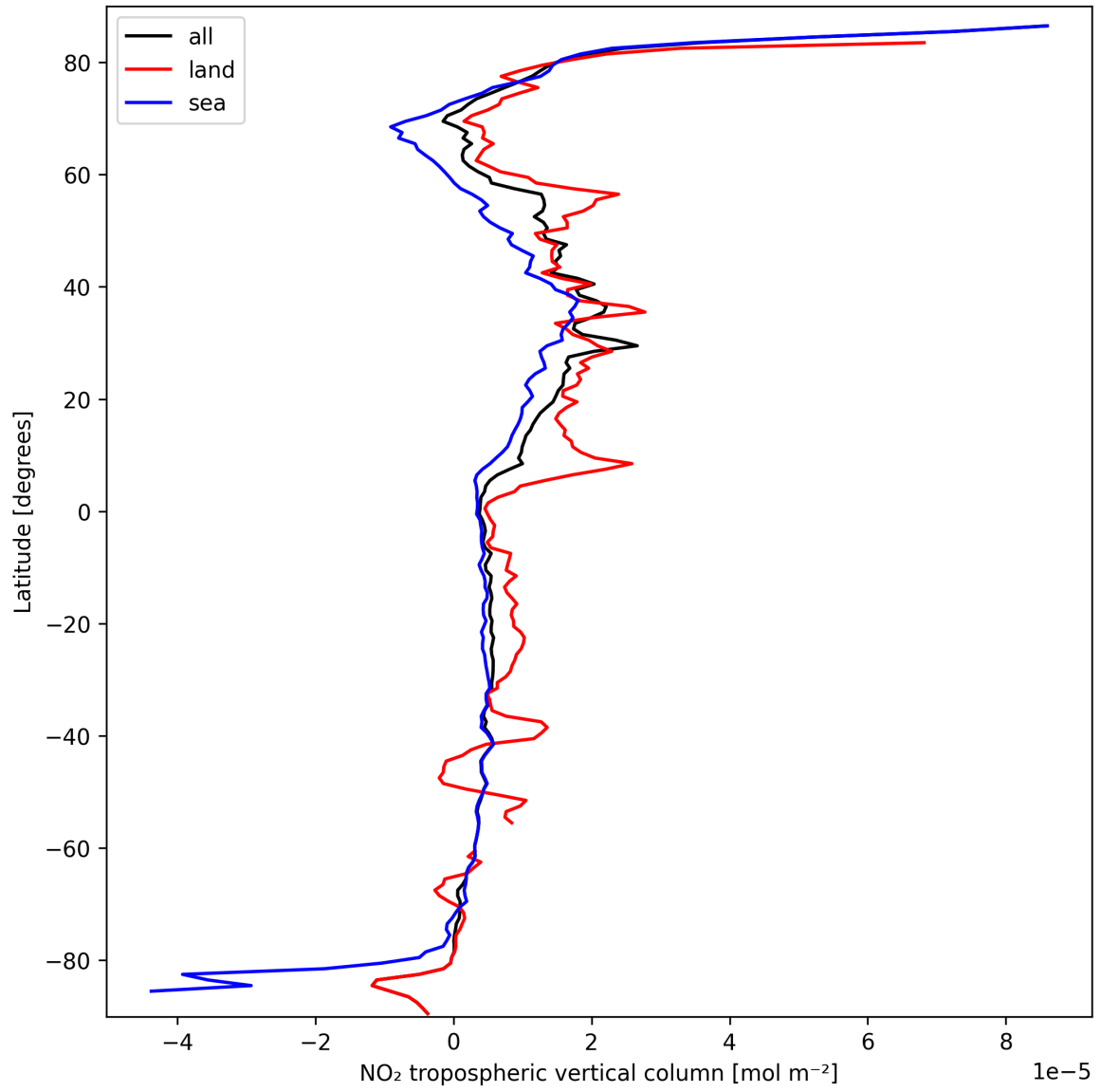
Figure 10: Zonal average of “NO 2 tropospheric vertical column” for 2025-03-16 to 2025-03-17.
