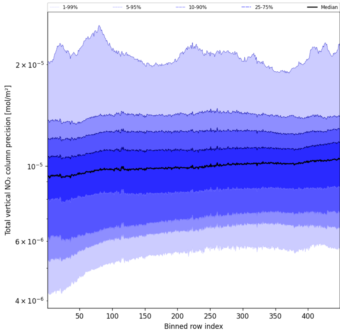
Figure 54: Along track statistics of “Total vertical NO 2 column precision” for 2025-03-16 to 2025-03-17
