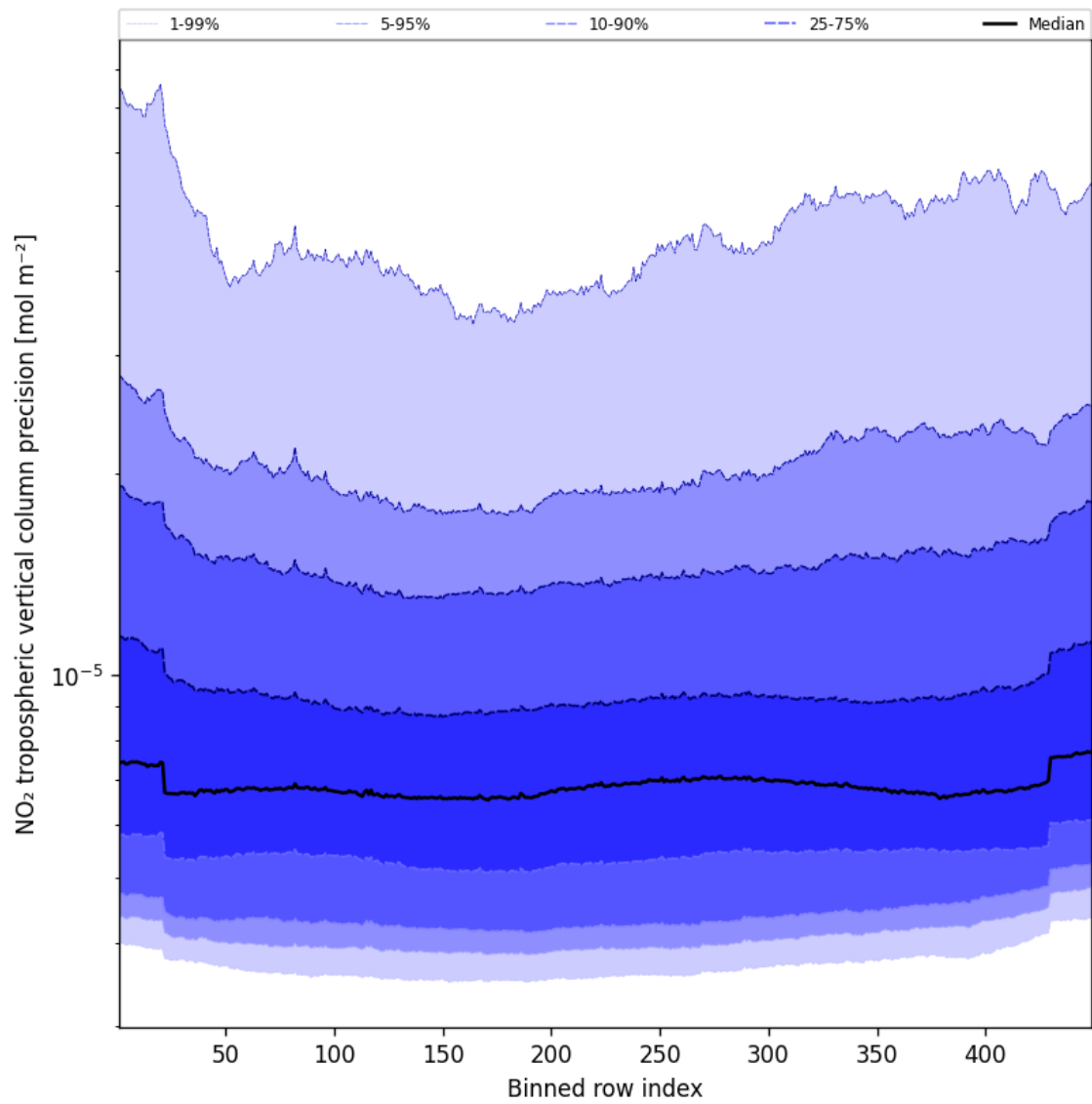
Figure 45: Along track statistics of “NO 2 tropospheric vertical column precision” for 2025-03-16 to 2025-03-17
