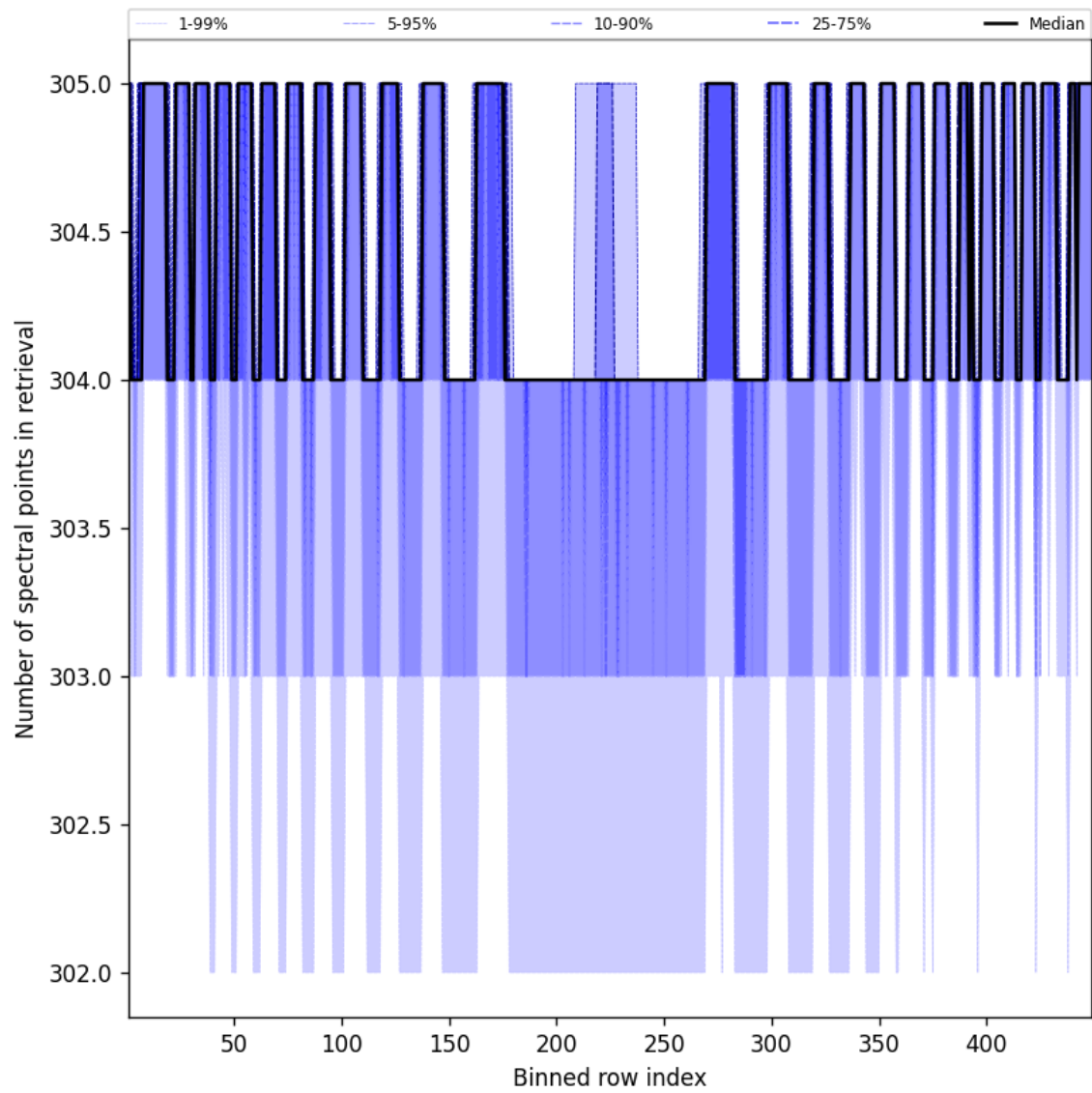
Figure 48: Along track statistics of “Number of spectral points in retrieval” for 2025-03-16 to 2025-03-17
