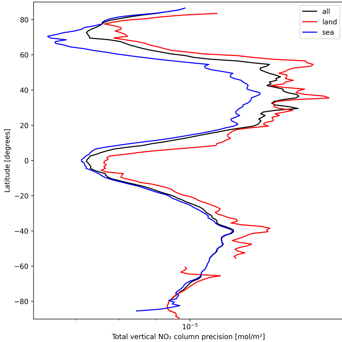
Figure 20: Zonal average of “Total vertical NO 2 column precision” for 2025-03-16 to 2025-03-17.
