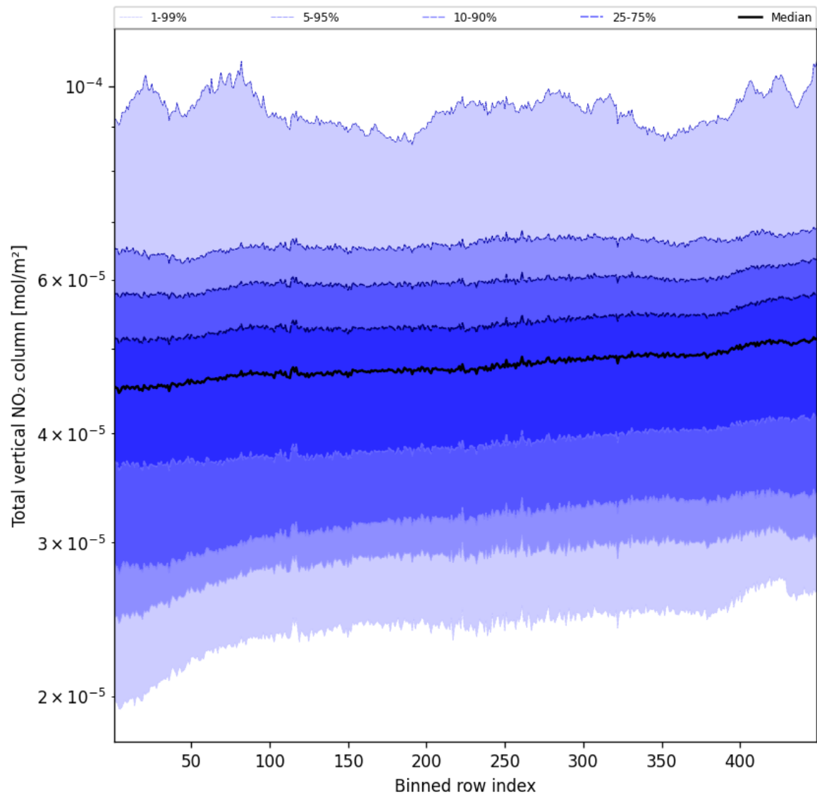
Figure 53: Along track statistics of “Total vertical NO 2 column” for 2025-03-16 to 2025-03-17
