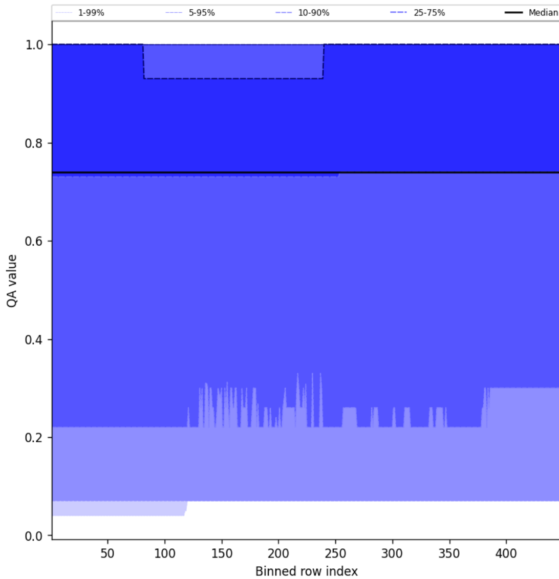
Figure 43: Along track statistics of “QA value” for 2025-03-16 to 2025-03-17
