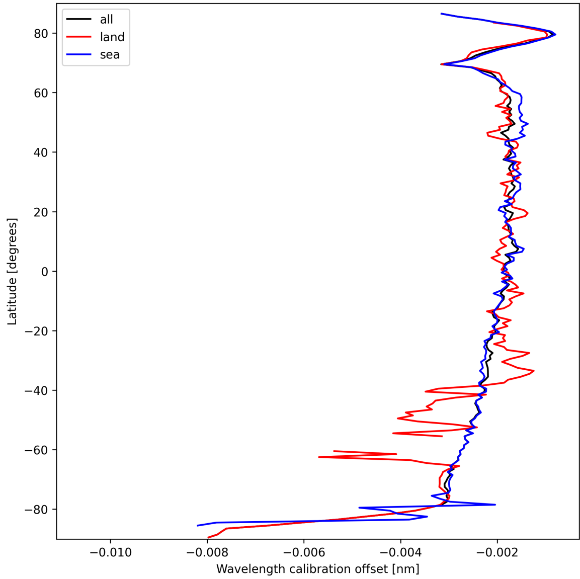
Figure 16: Zonal average of “Wavelength calibration offset” for 2025-03-16 to 2025-03-17.
