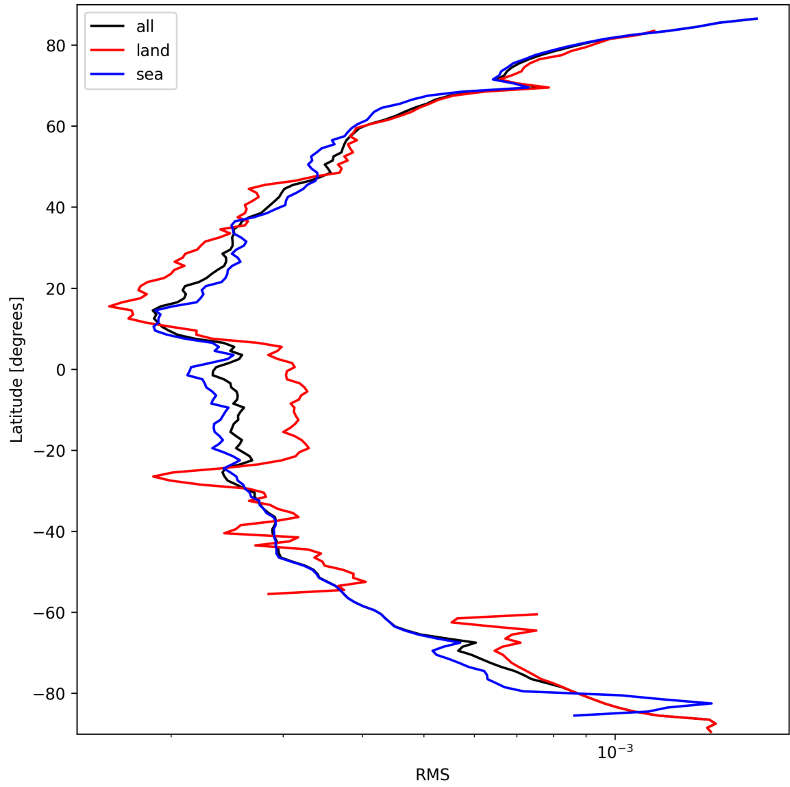
Figure 24: Zonal average of “RMS” for 2025-03-16 to 2025-03-17.
