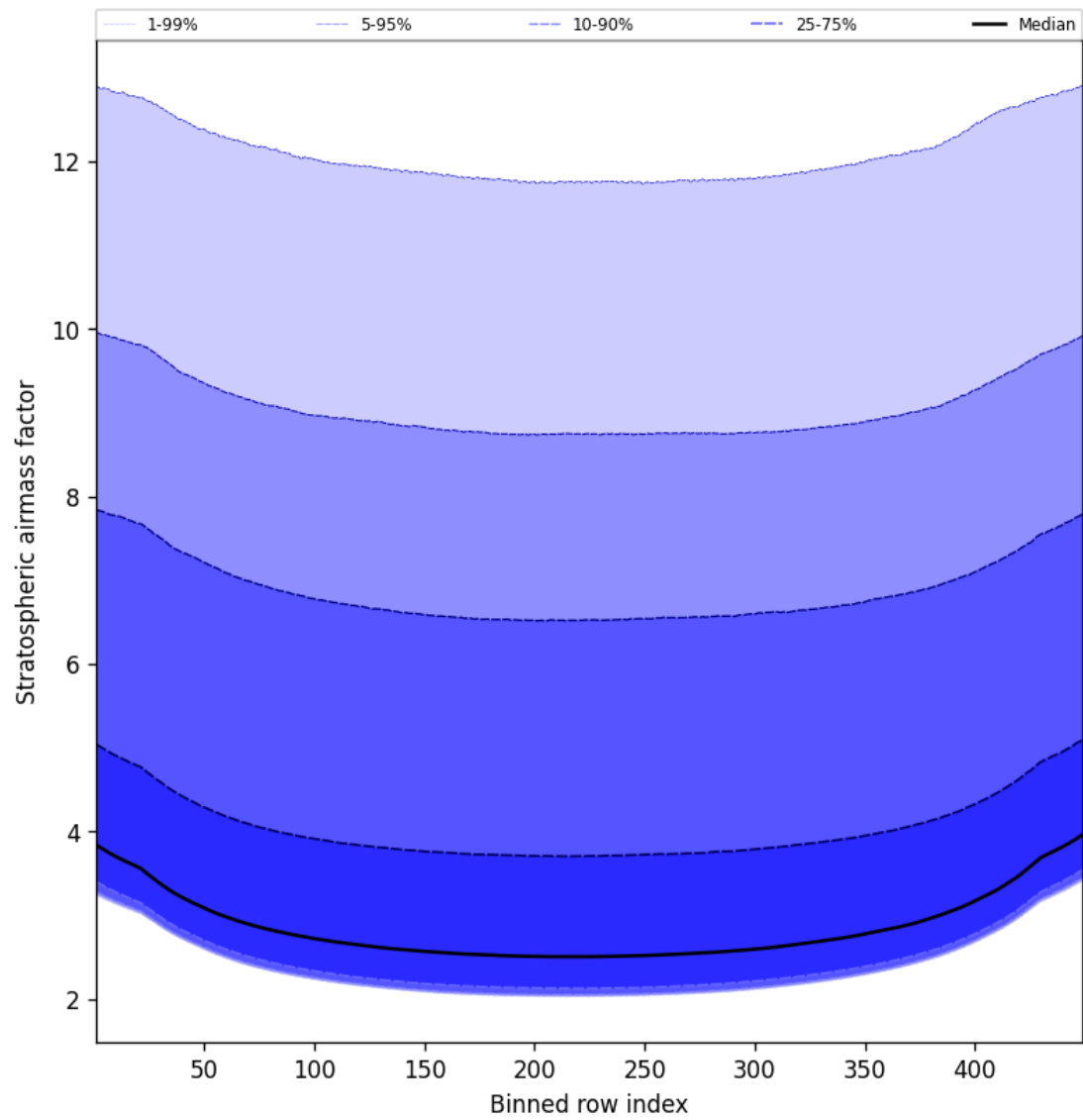
Figure 59: Along track statistics of “Stratospheric airmass factor” for 2025-03-16 to 2025-03-17
