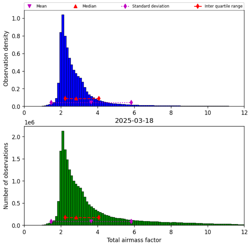
Figure 30: Histogram of “Total airmass factor” for 2025-03-18 to 2025-03-19
