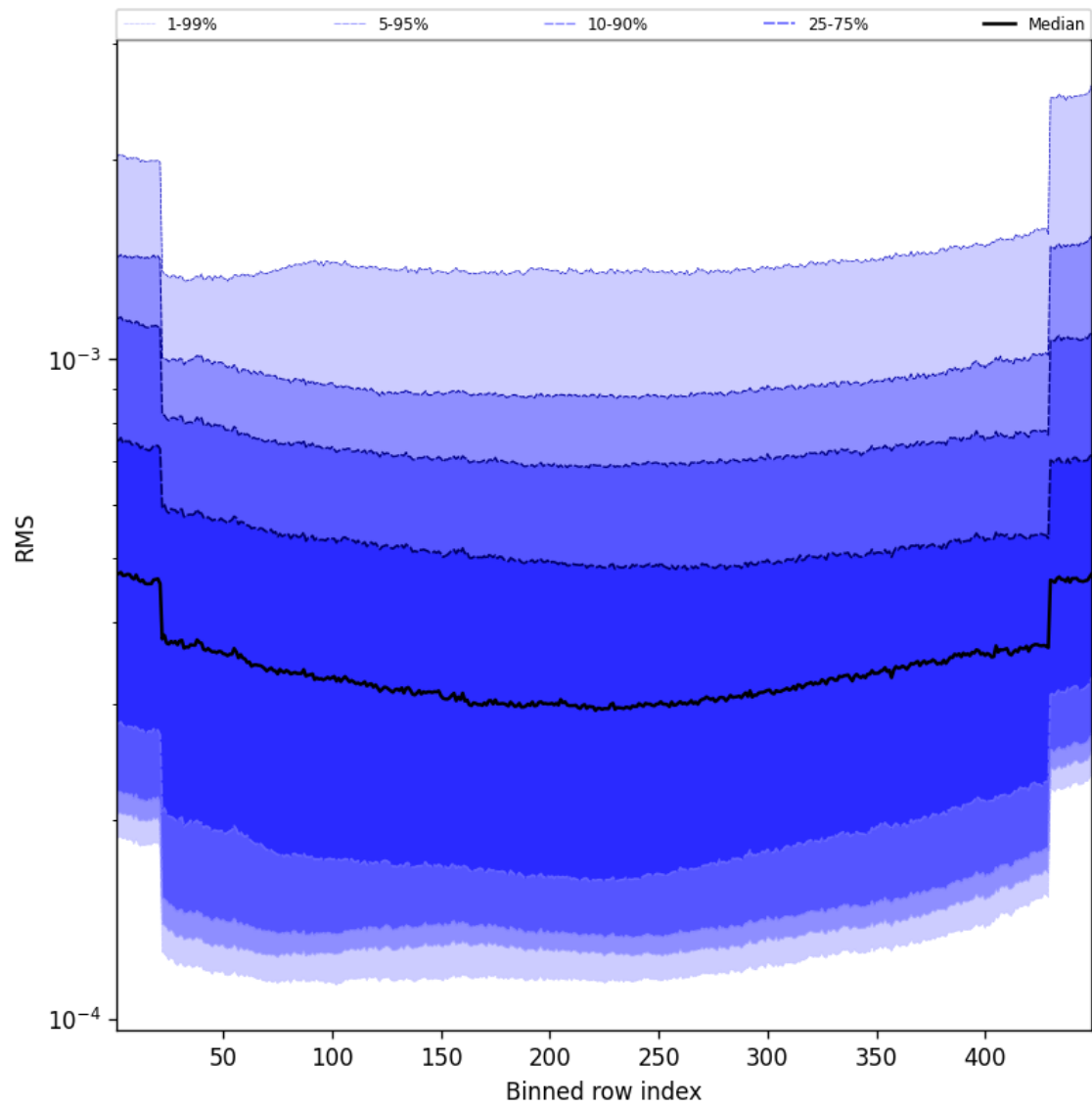
Figure 58: Along track statistics of “RMS” for 2025-03-18 to 2025-03-19
