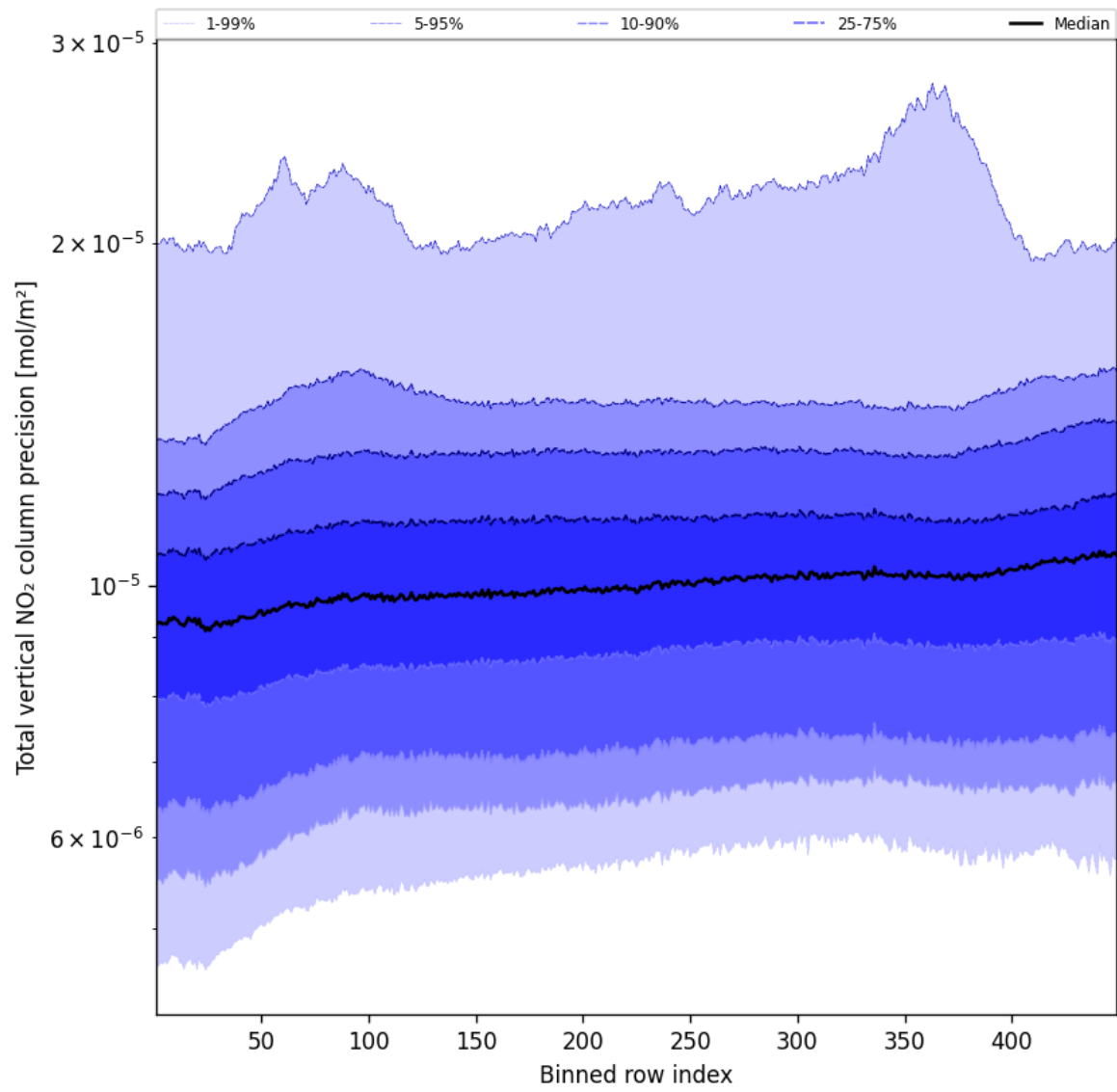
Figure 54: Along track statistics of “Total vertical NO 2 column precision” for 2025-03-18 to 2025-03-19
