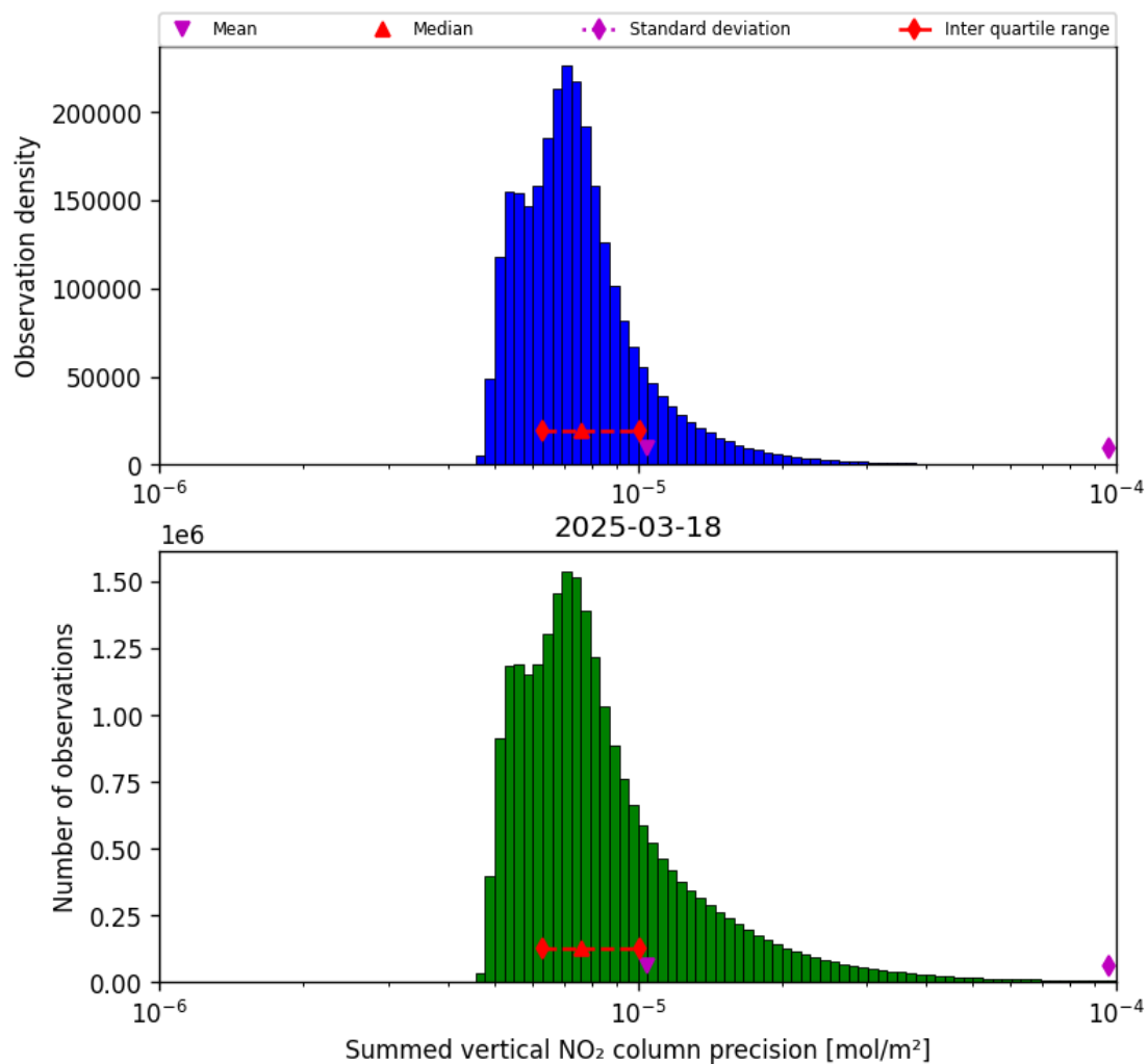
Figure 39: Histogram of “Summed vertical NO 2 column precision” for 2025-03-18 to 2025-03-19
