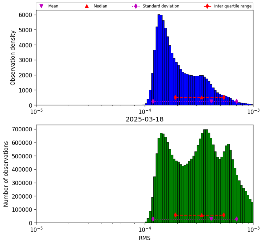
Figure 41: Histogram of “RMS” for 2025-03-18 to 2025-03-19
