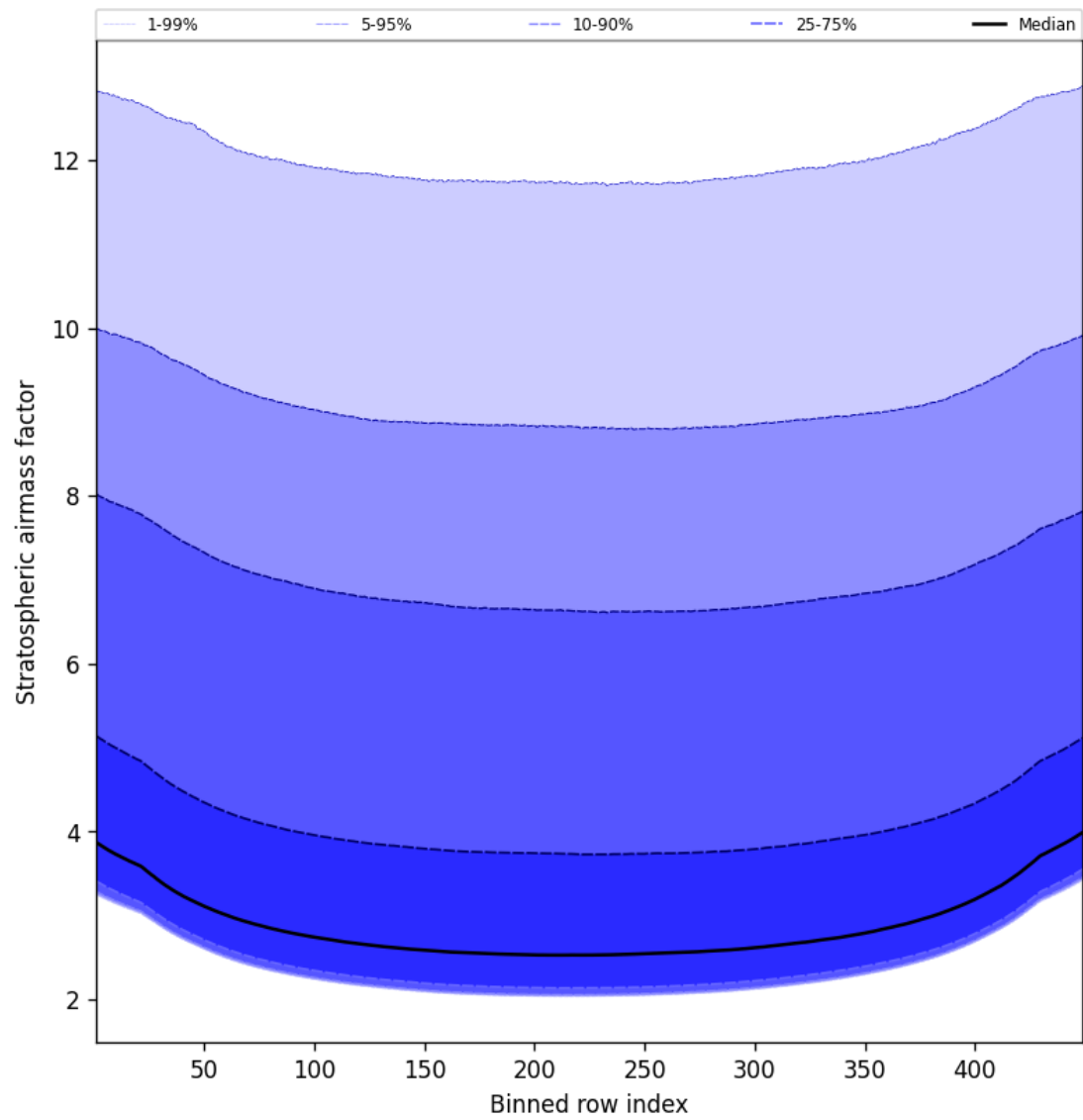
Figure 59: Along track statistics of “Stratospheric airmass factor” for 2025-03-18 to 2025-03-19
