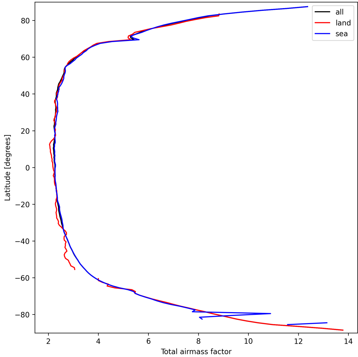
Figure 13: Zonal average of “Total airmass factor” for 2025-03-18 to 2025-03-19.
