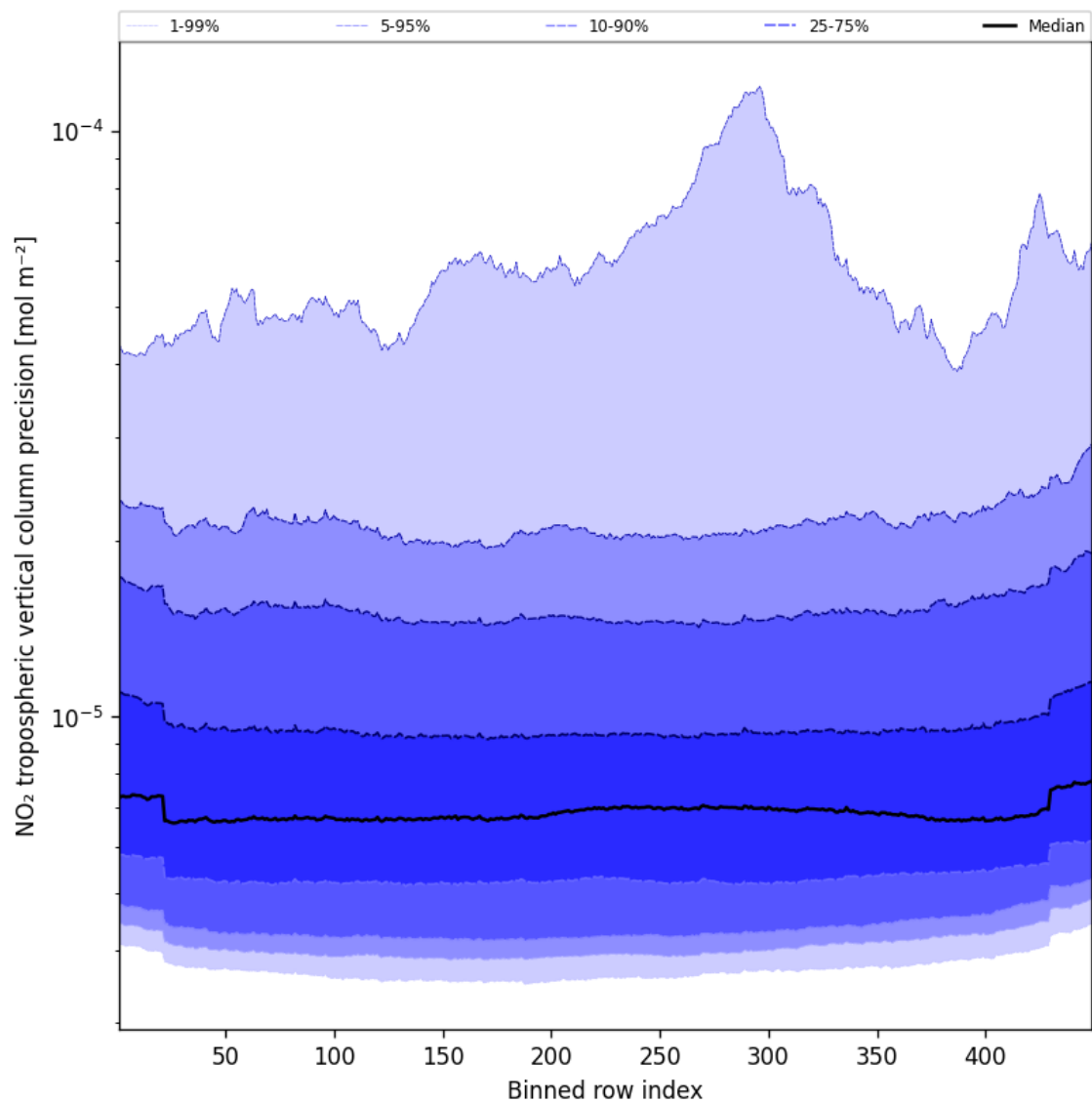
Figure 45: Along track statistics of “NO 2 tropospheric vertical column precision” for 2025-03-18 to 2025-03-19
