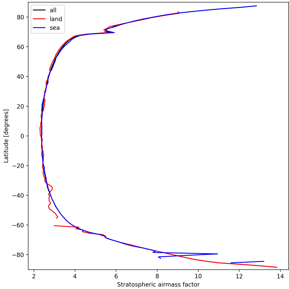
Figure 25: Zonal average of “Stratospheric airmass factor” for 2025-03-18 to 2025-03-19.
