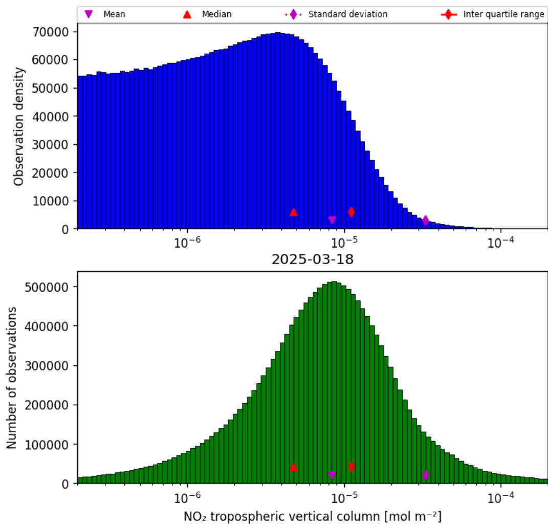
Figure 27: Histogram of “NO 2 tropospheric vertical column” for 2025-03-18 to 2025-03-19
