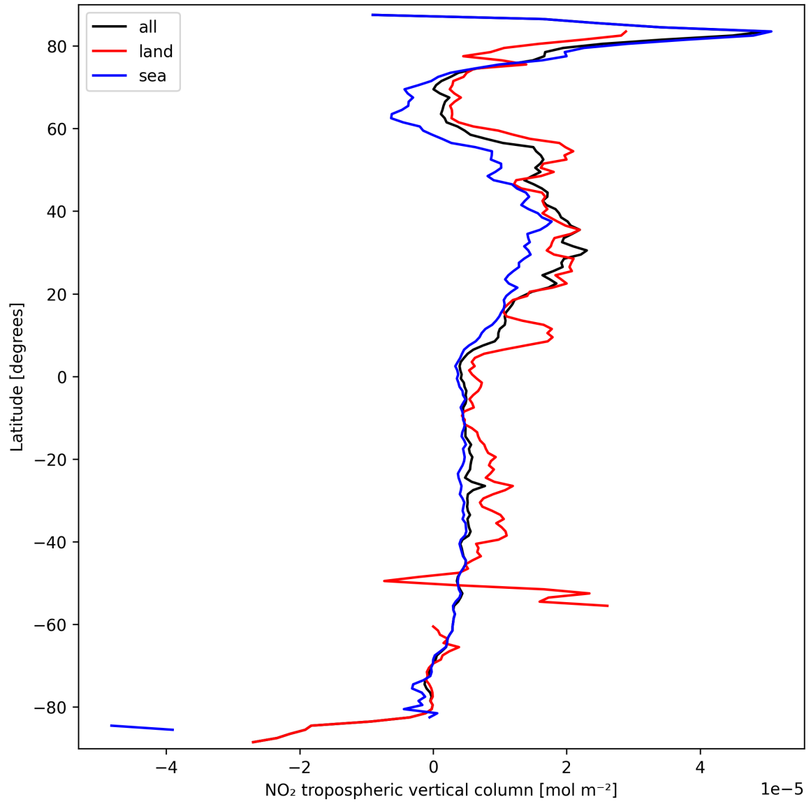
Figure 10: Zonal average of “NO 2 tropospheric vertical column” for 2025-03-18 to 2025-03-19.
