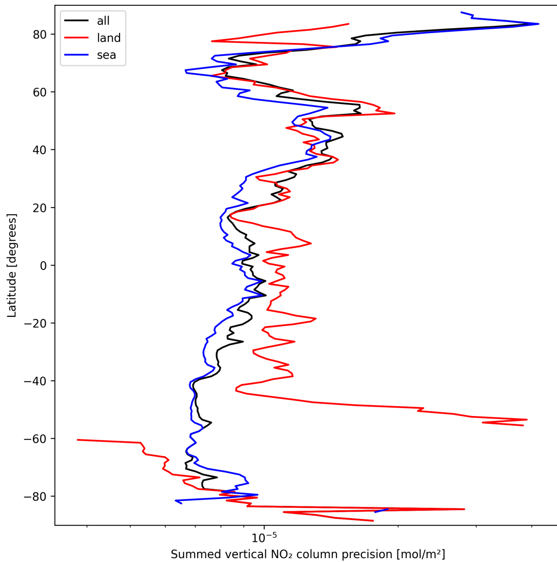
Figure 22: Zonal average of “Summed vertical NO 2 column precision” for 2025-03-18 to 2025-03-19.
