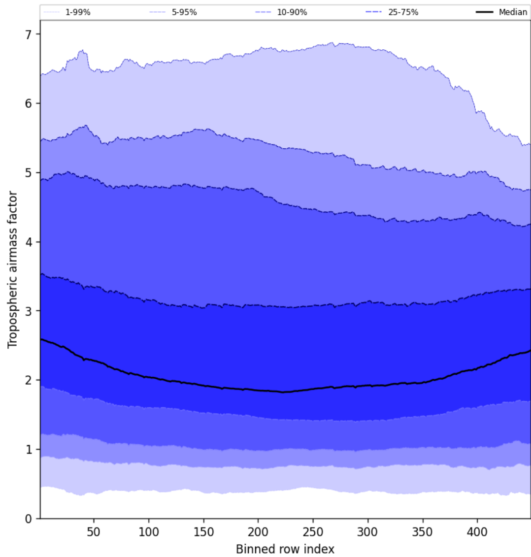
Figure 46: Along track statistics of “Tropospheric air mass factor” for 2025-03-18 to 2025-03-19
