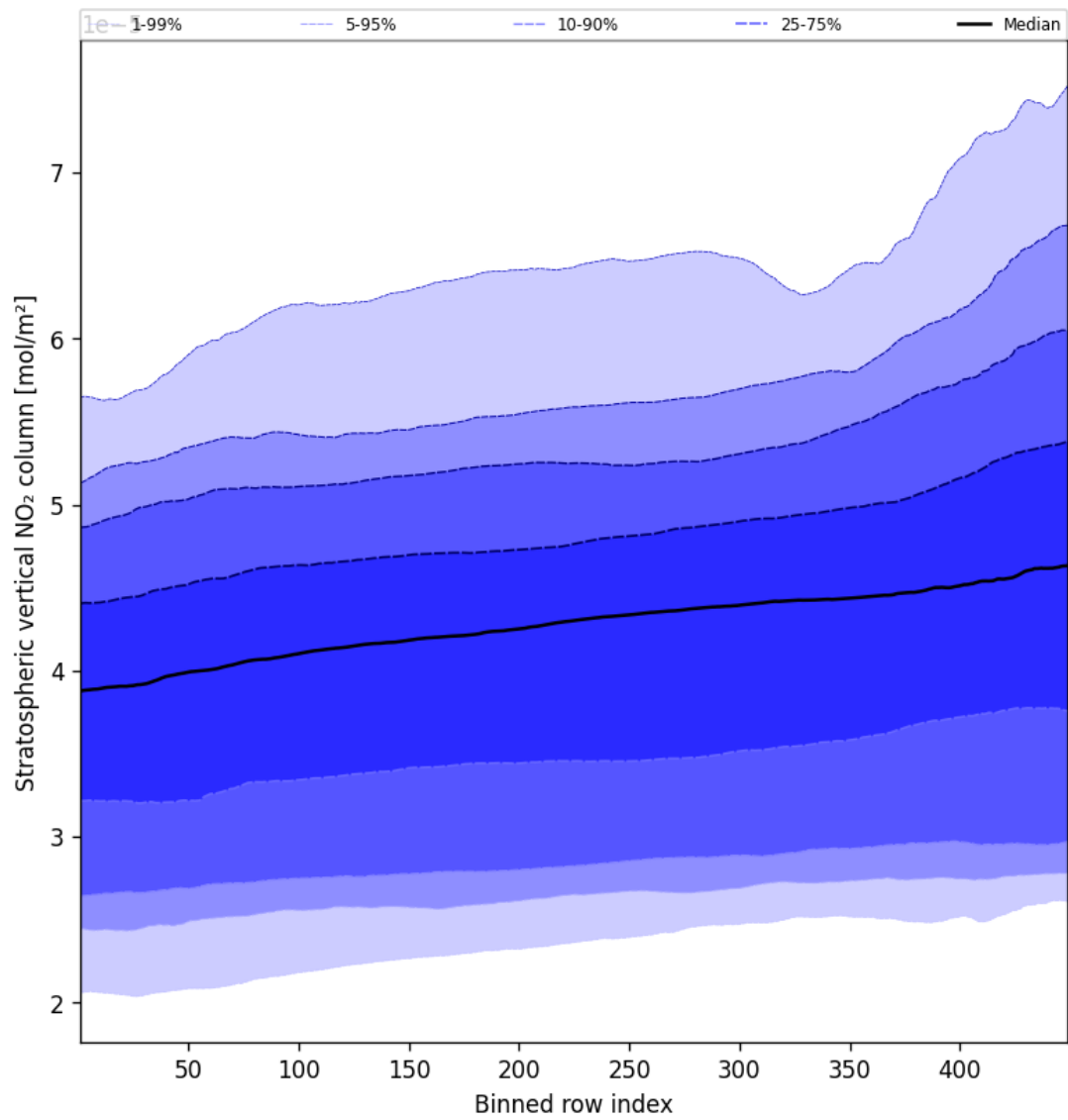
Figure 51: Along track statistics of “Stratospheric vertical NO 2 column” for 2025-03-18 to 2025-03-19
