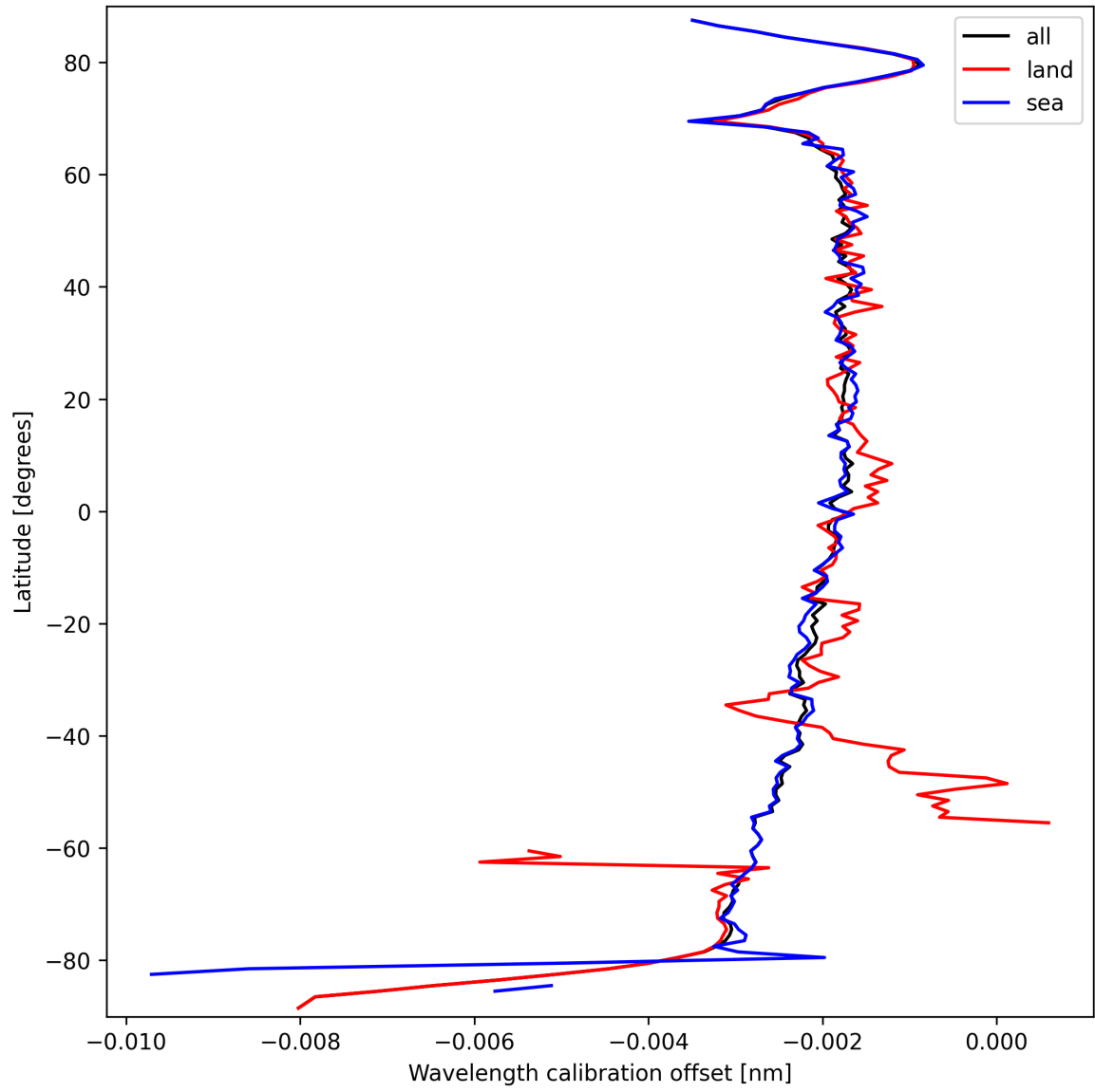
Figure 16: Zonal average of “Wavelength calibration offset” for 2025-03-18 to 2025-03-19.
