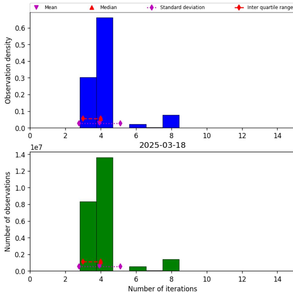
Figure 32: Histogram of “Number of iterations” for 2025-03-18 to 2025-03-19
