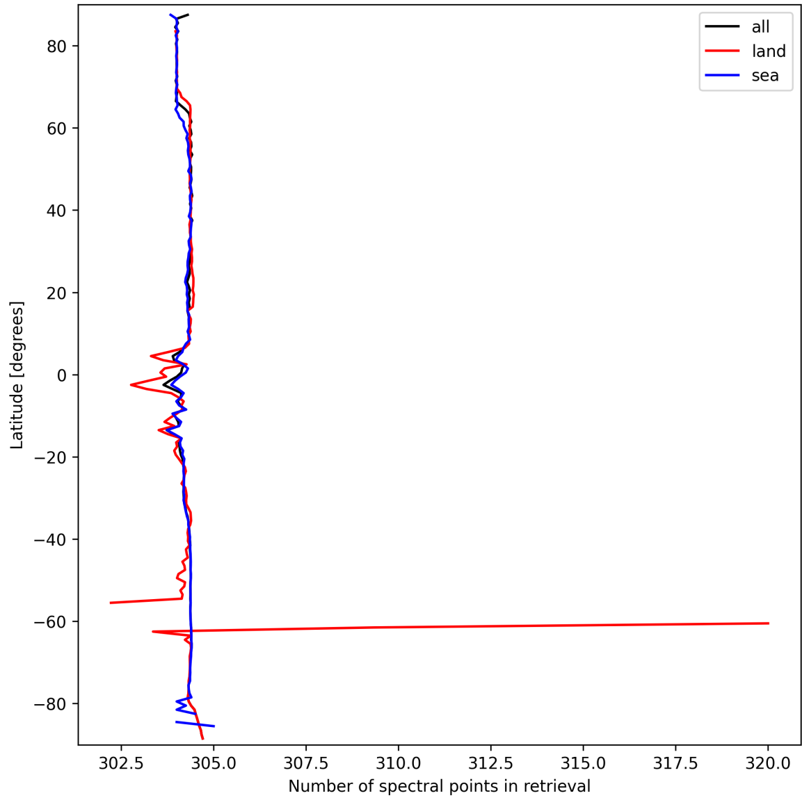
Figure 14: Zonal average of “Number of spectral points in retrieval” for 2025-03-18 to 2025-03-19.
