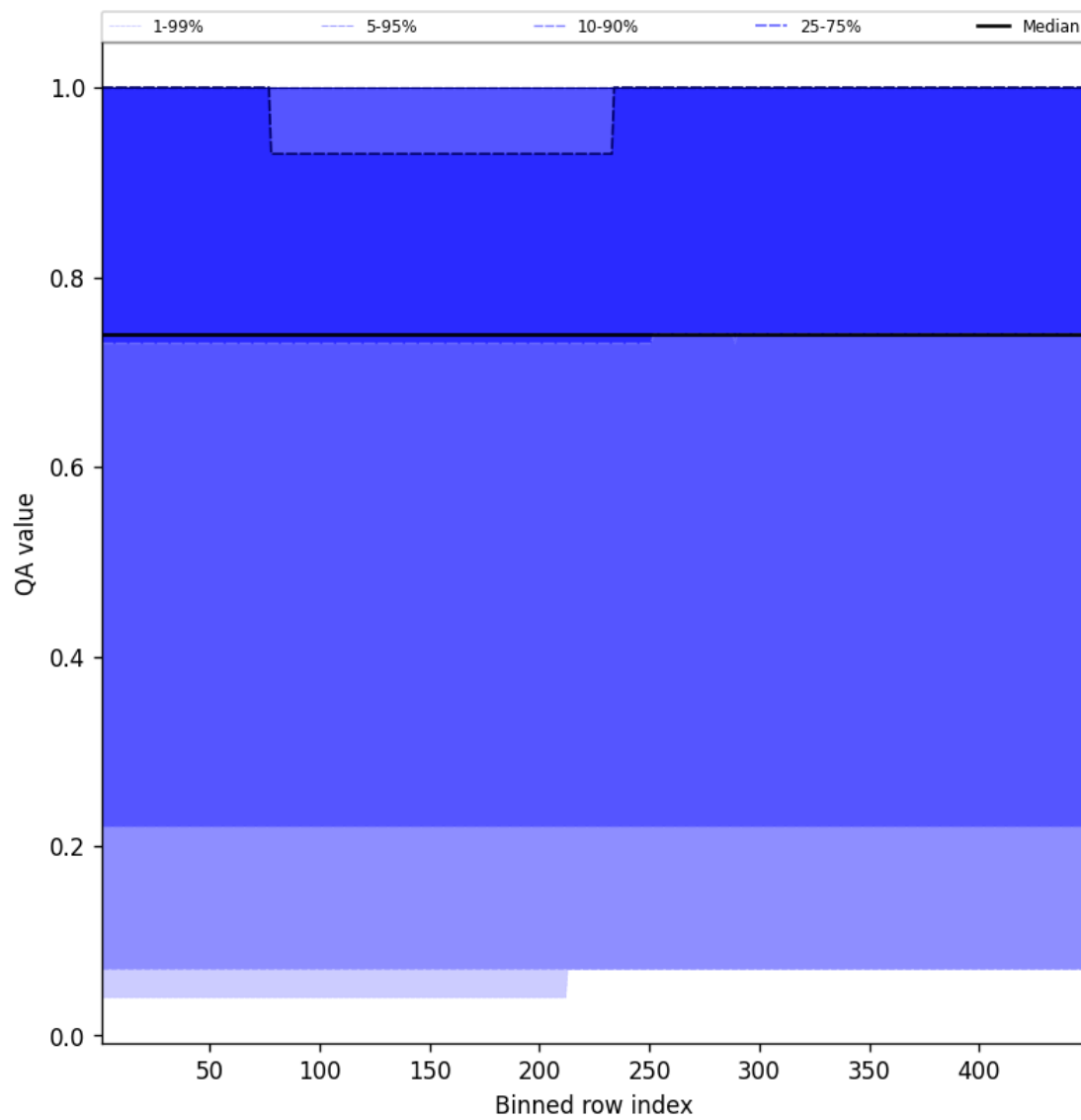
Figure 43: Along track statistics of “QA value” for 2025-03-18 to 2025-03-19
