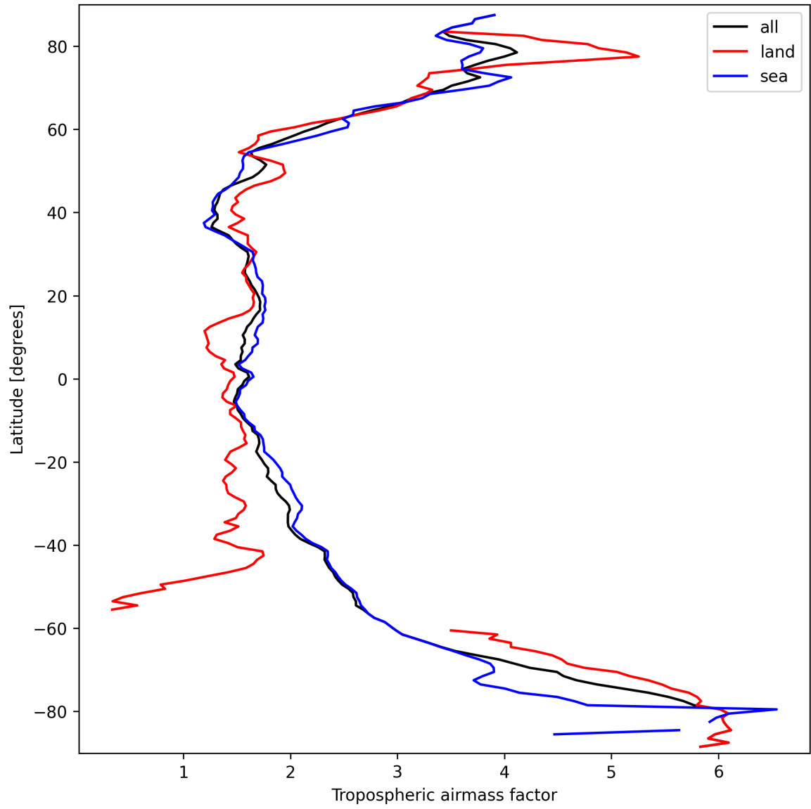
Figure 12: Zonal average of “Tropospheric airmass factor” for 2025-03-18 to 2025-03-19.
