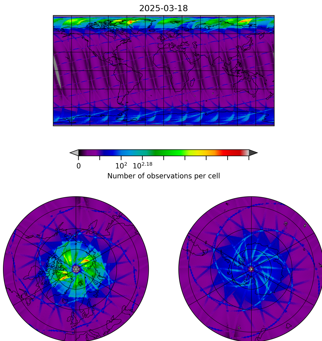
Figure 8: Map of the number of observations for 2025-03-18 to 2025-03-19
