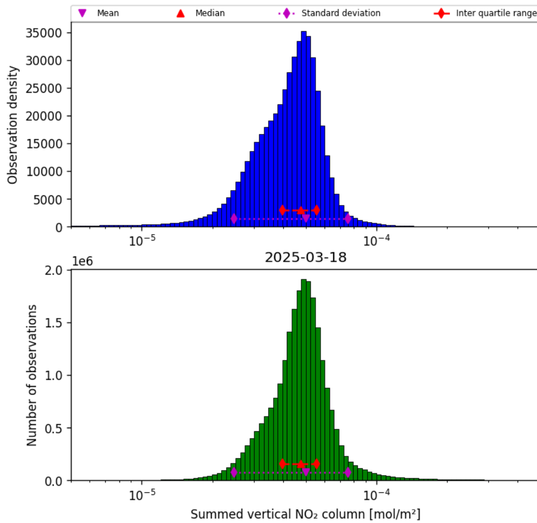
Figure 38: Histogram of “Summed vertical NO 2 column” for 2025-03-18 to 2025-03-19
