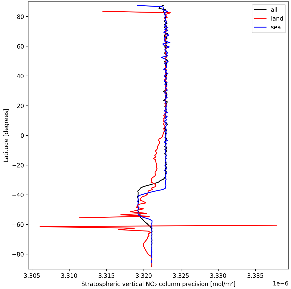
Figure 18: Zonal average of “Stratospheric vertical NO 2 column precision” for 2025-03-18 to 2025-03-19.
