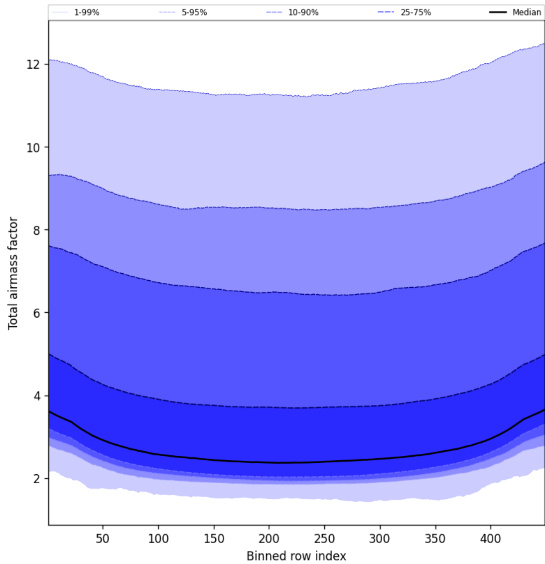
Figure 47: Along track statistics of “Total airmass factor” for 2025-03-18 to 2025-03-19
