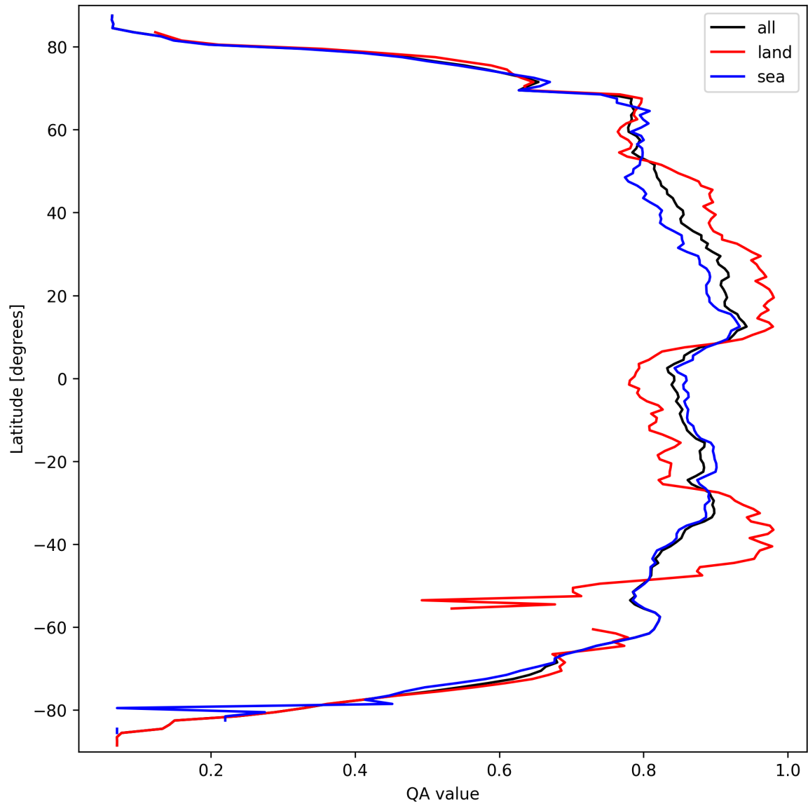
Figure 9: Zonal average of “QA value” for 2025-03-18 to 2025-03-19.
