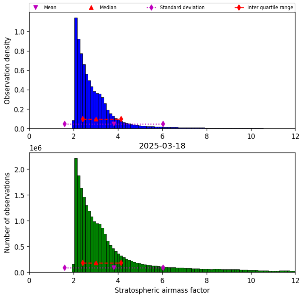
Figure 42: Histogram of “Stratospheric airmass factor” for 2025-03-18 to 2025-03-19
