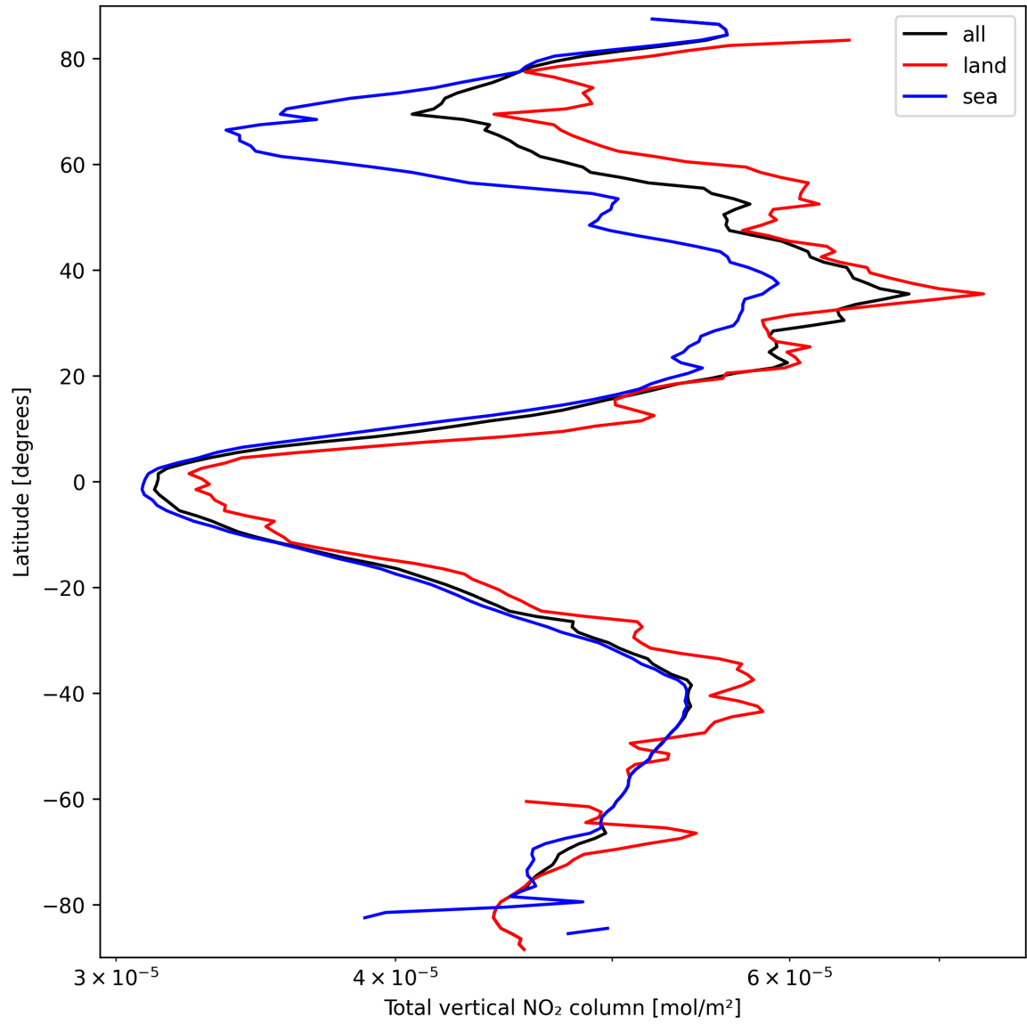
Figure 19: Zonal average of “Total vertical NO 2 column” for 2025-03-18 to 2025-03-19.
