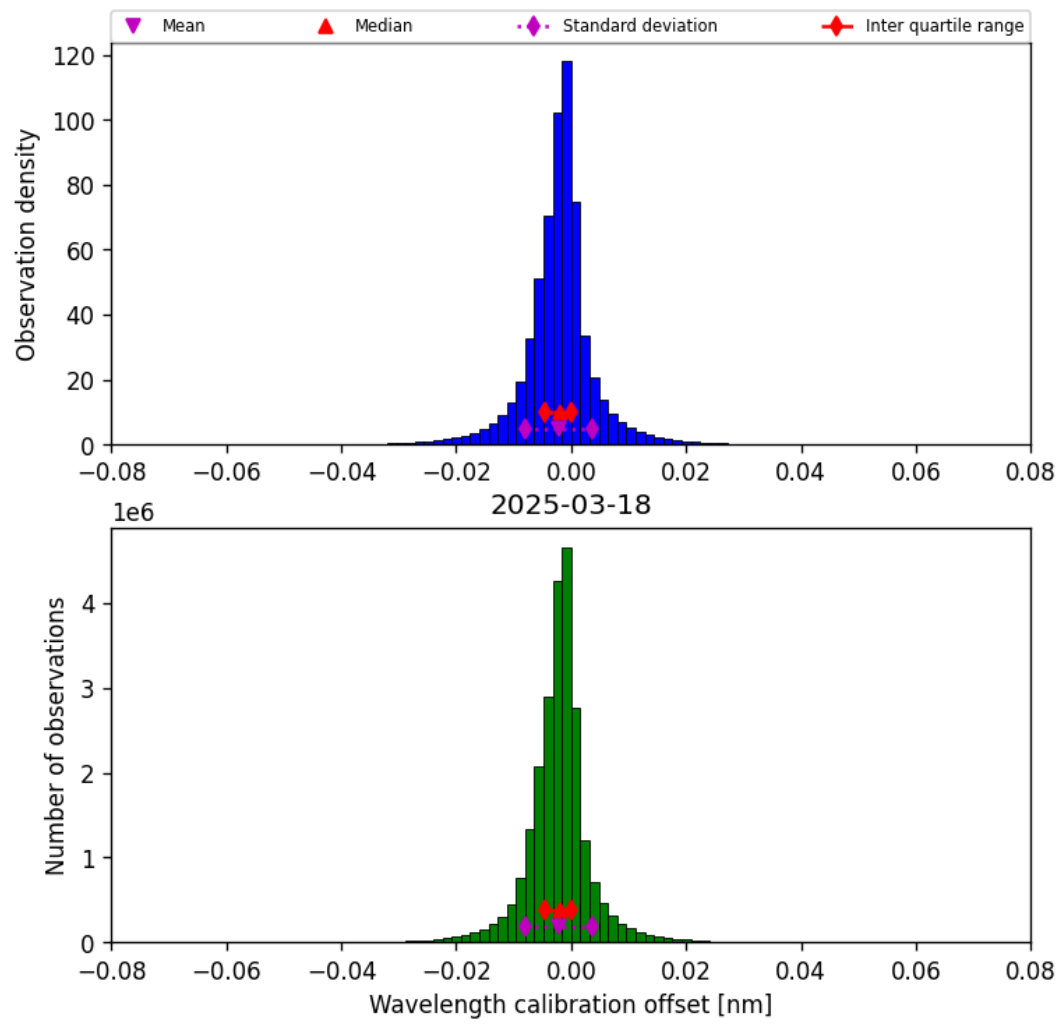
Figure 33: Histogram of “Wavelength calibration offset” for 2025-03-18 to 2025-03-19
