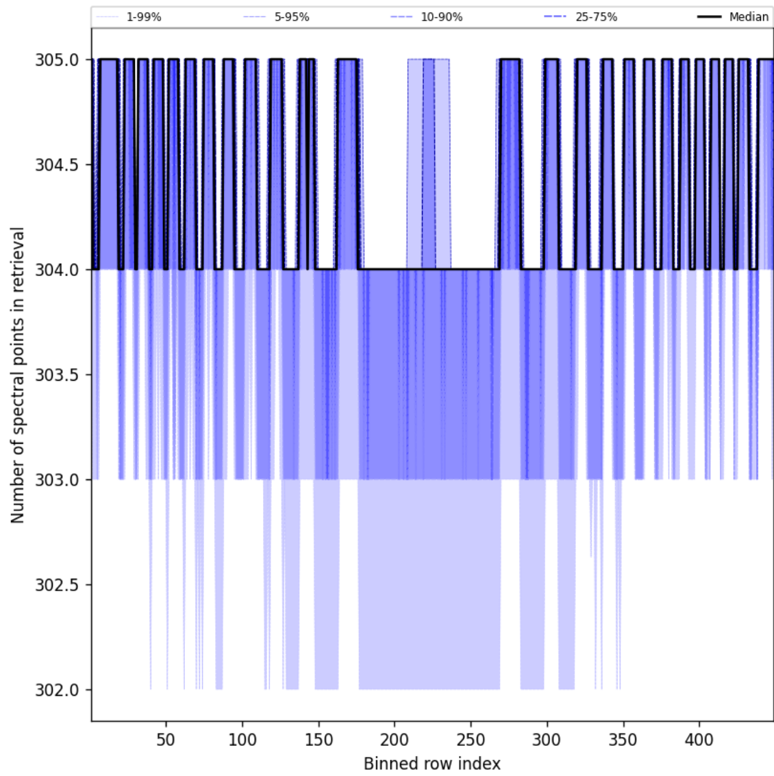
Figure 48: Along track statistics of “Number of spectral points in retrieval” for 2025-03-18 to 2025-03-19
