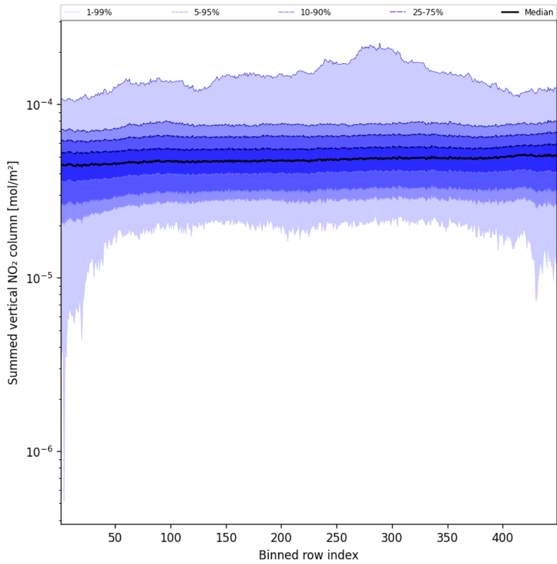
Figure 55: Along track statistics of “Summed vertical NO 2 column” for 2025-03-18 to 2025-03-19
