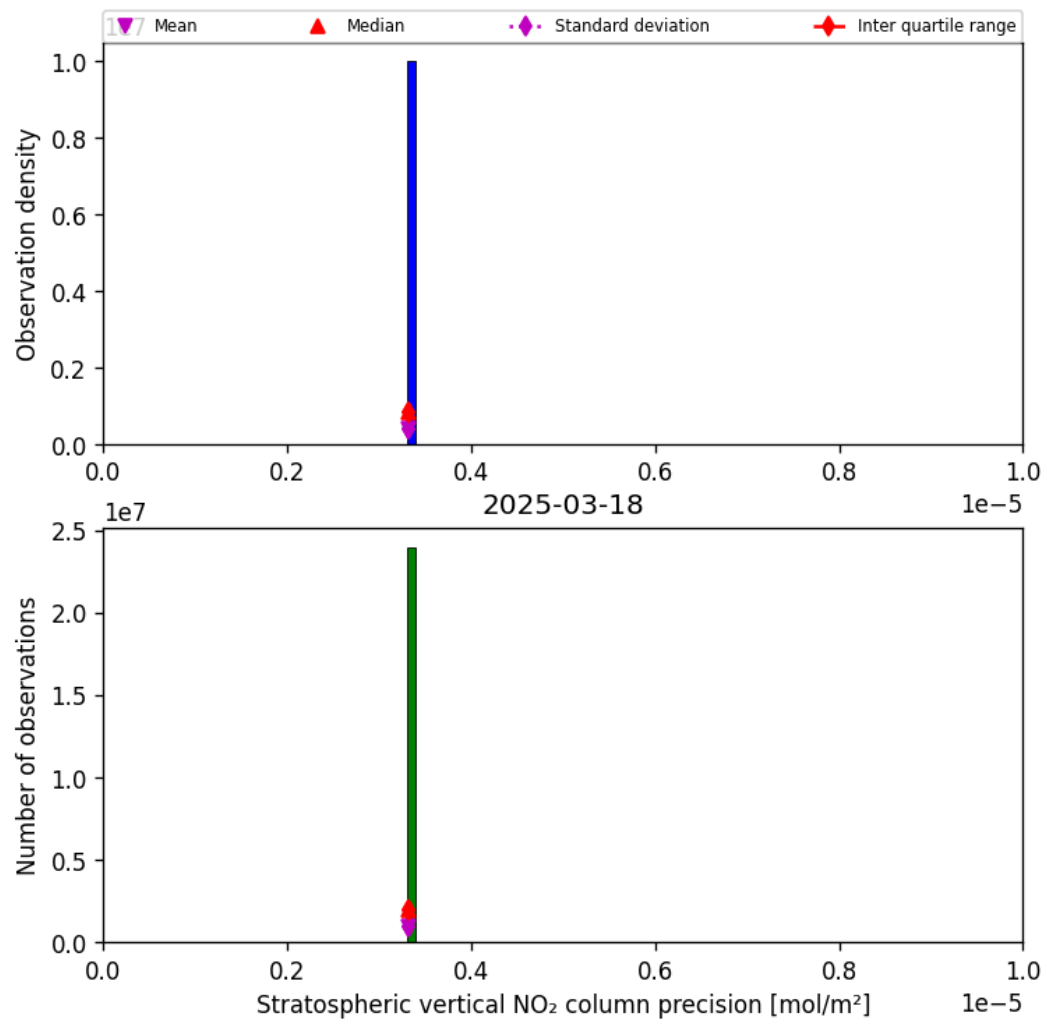
Figure 35: Histogram of “Stratospheric vertical NO 2 column precision” for 2025-03-18 to 2025-03-19
