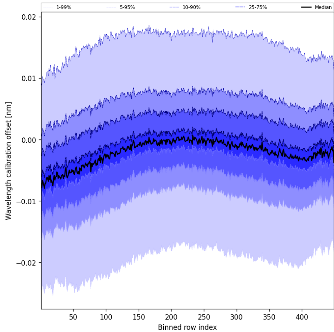
Figure 50: Along track statistics of “Wavelength calibration offset” for 2025-03-18 to 2025-03-19
