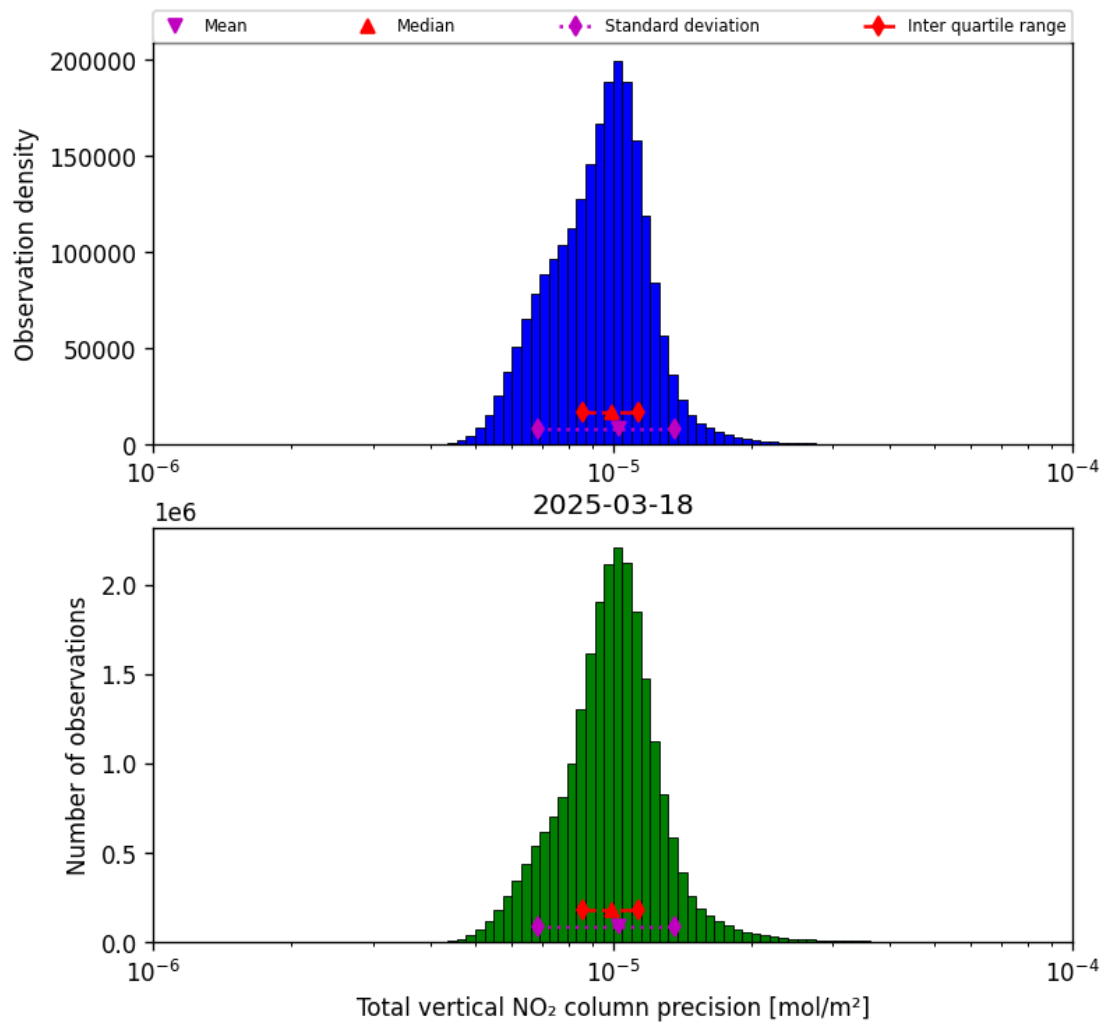
Figure 37: Histogram of “Total vertical NO 2 column precision” for 2025-03-18 to 2025-03-19
