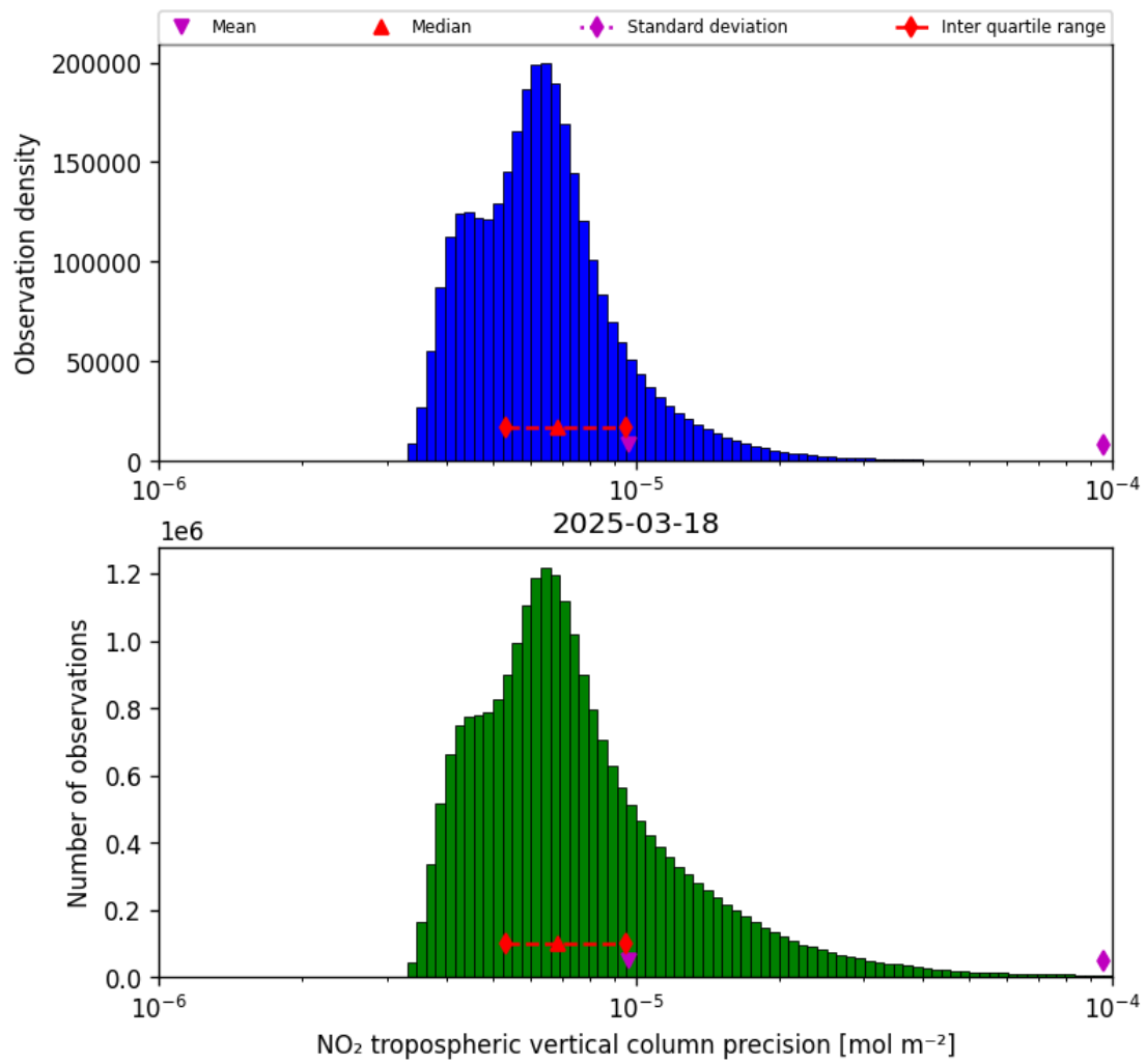
Figure 28: Histogram of “NO 2 tropospheric vertical column precision” for 2025-03-18 to 2025-03-19
