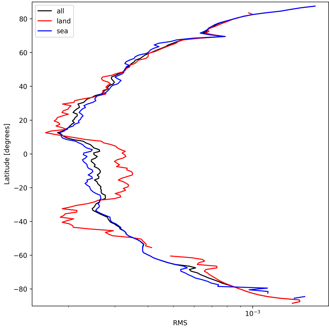
Figure 24: Zonal average of “RMS” for 2025-03-18 to 2025-03-19.
