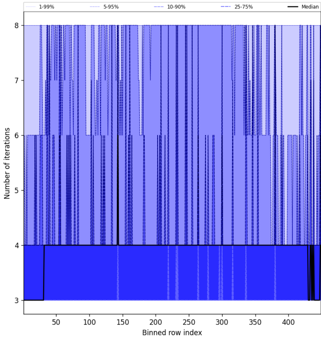
Figure 49: Along track statistics of “Number of iterations” for 2025-03-18 to 2025-03-19
