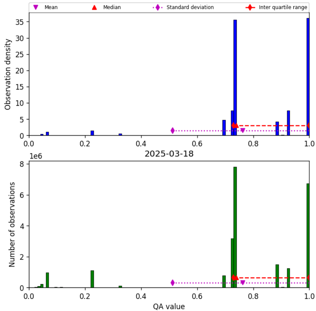
Figure 26: Histogram of “QA value” for 2025-03-18 to 2025-03-19
