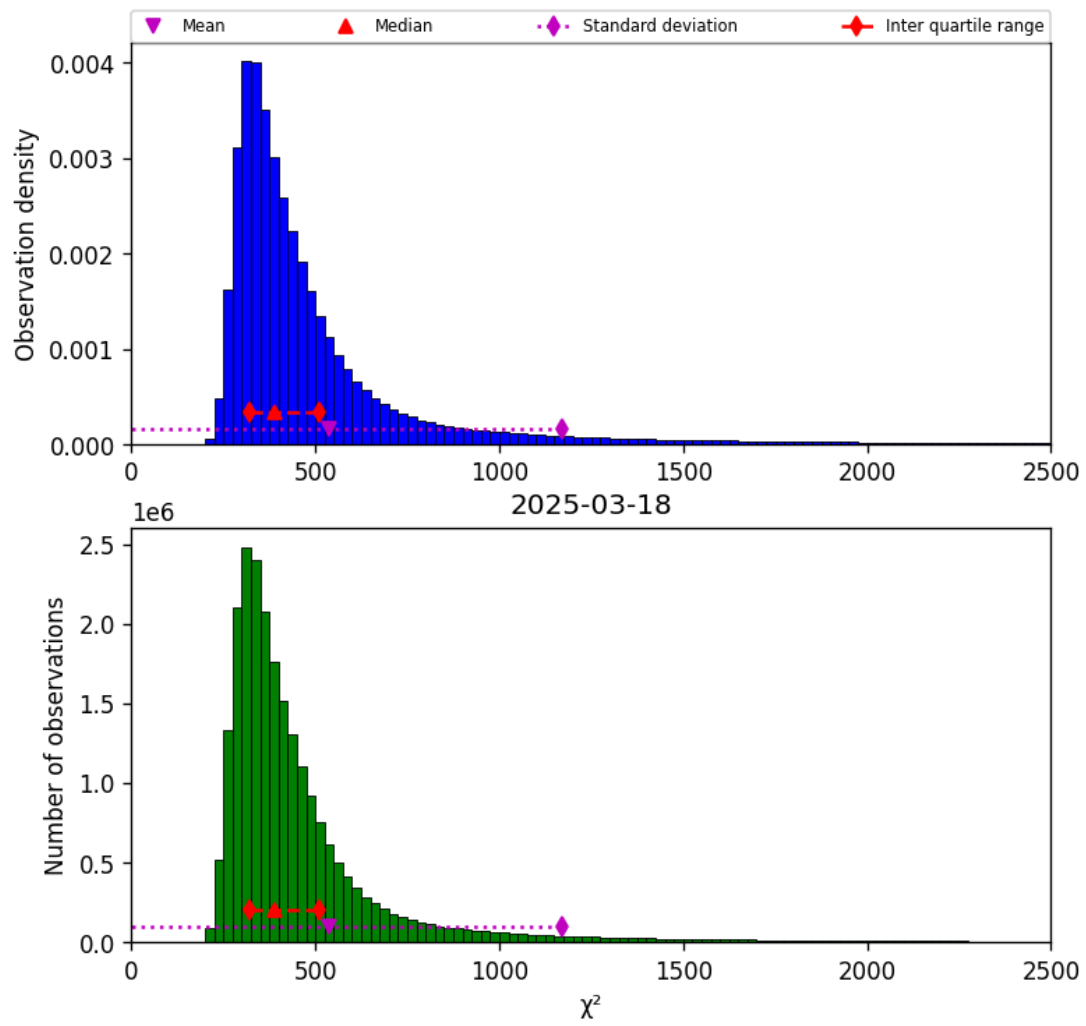
Figure 40: Histogram of “ \chi^2 ” for 2025-03-18 to 2025-03-19
