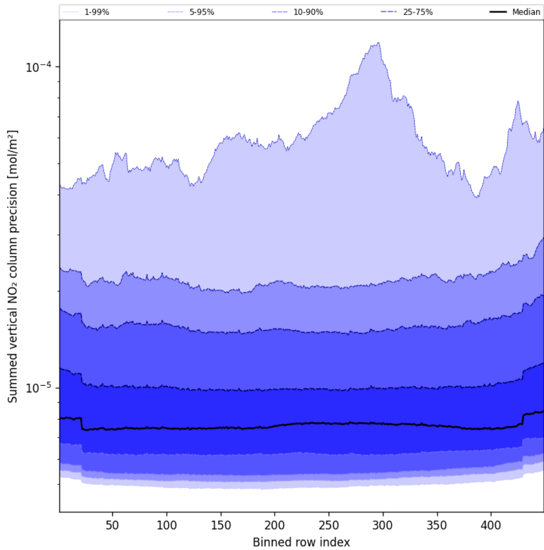
Figure 56: Along track statistics of “Summed vertical NO 2 column precision” for 2025-03-18 to 2025-03-19
