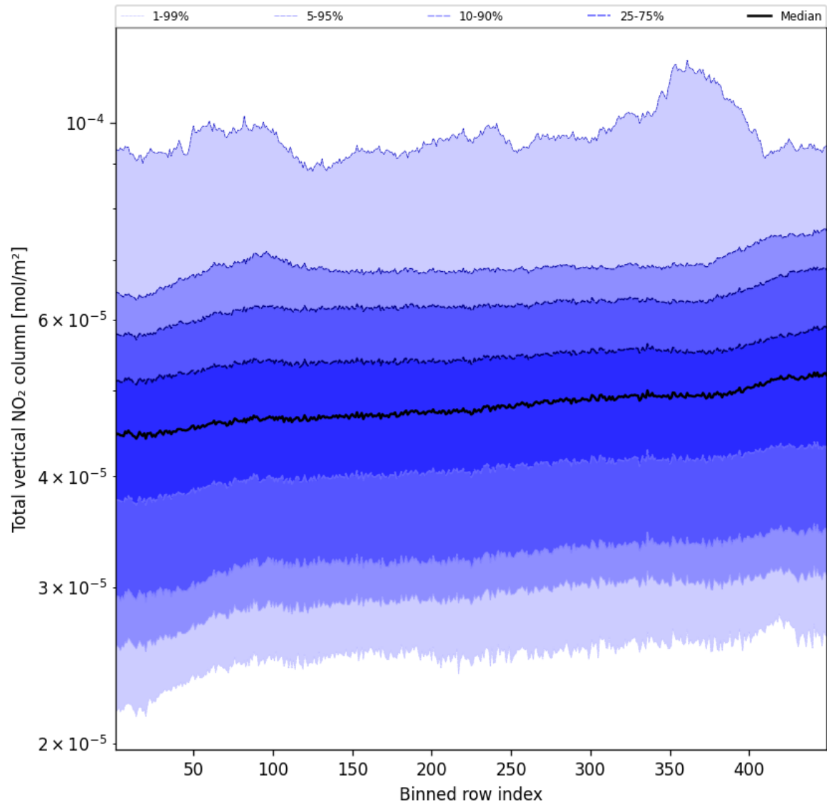
Figure 53: Along track statistics of “Total vertical NO 2 column” for 2025-03-18 to 2025-03-19
