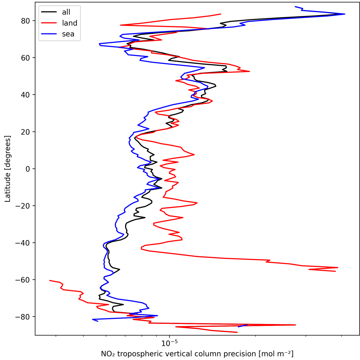
Figure 11: Zonal average of “NO 2 tropospheric vertical column precision” for 2025-03-18 to 2025-03-19.
