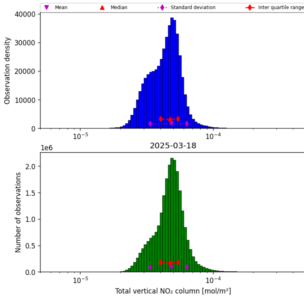
Figure 36: Histogram of "Total vertical NO 2 column" for 2025-03-18 to 2025-03-19
