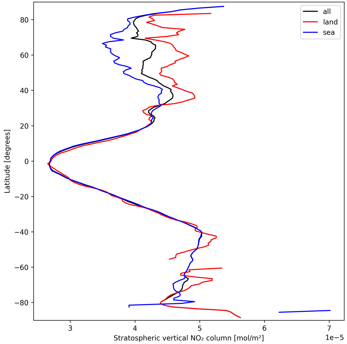
Figure 17: Zonal average of “Stratospheric vertical NO 2 column” for 2025-03-18 to 2025-03-19.
