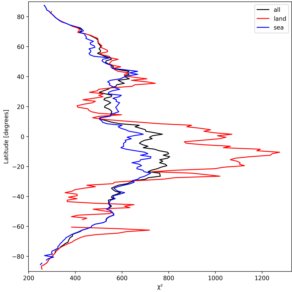
Figure 23: Zonal average of “ \chi^2 ” for 2025-03-18 to 2025-03-19.
