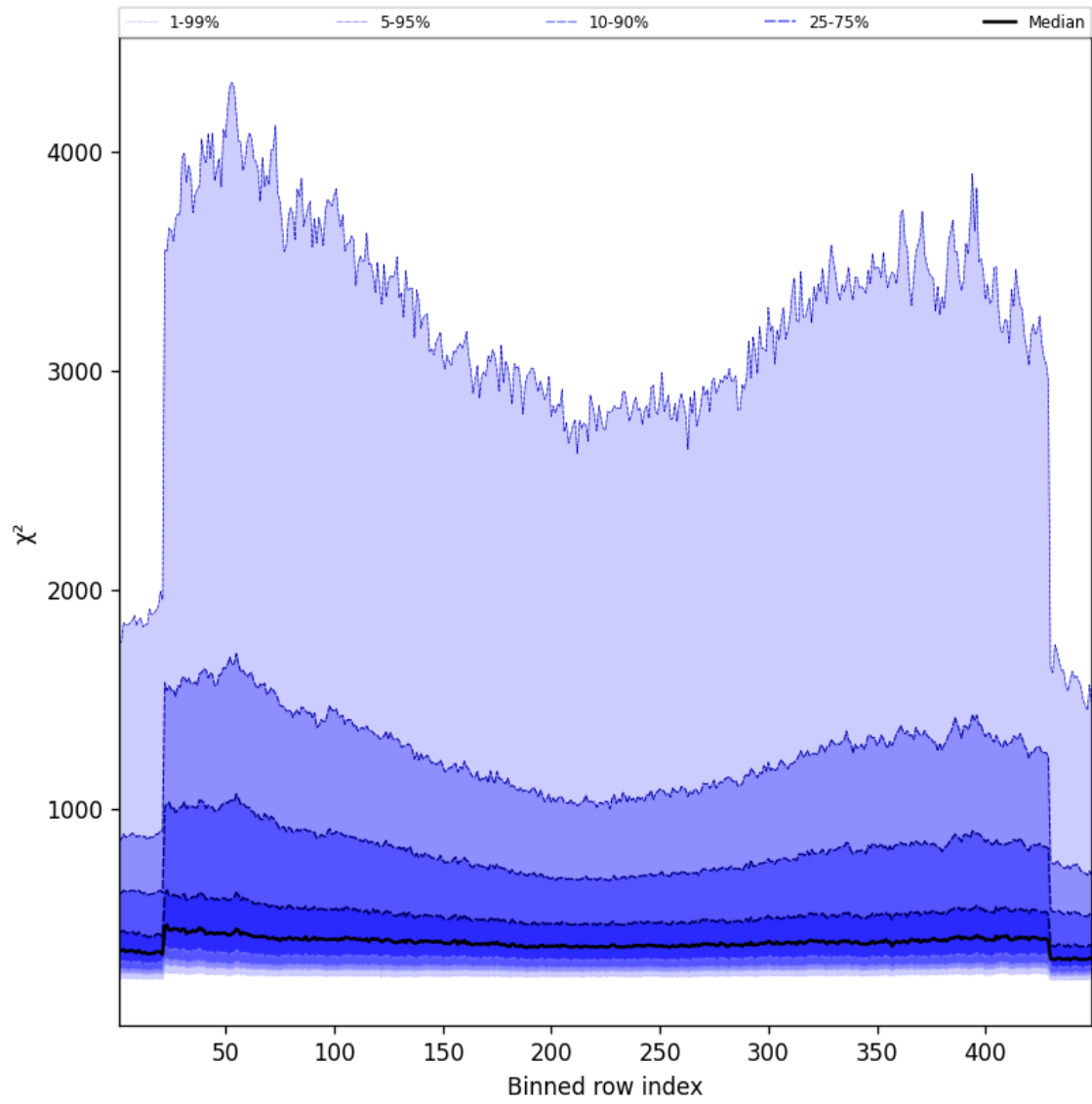
Figure 57: Along track statistics of “ \chi^2 ” for 2025-03-18 to 2025-03-19
