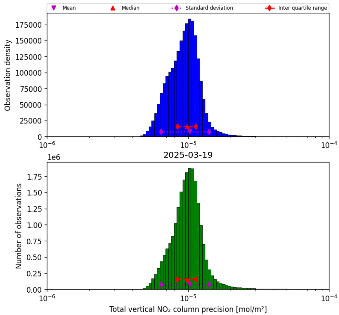
Figure 37: Histogram of "Total vertical NO 2 column precision" for 2025-03-19 to 2025-03-20
