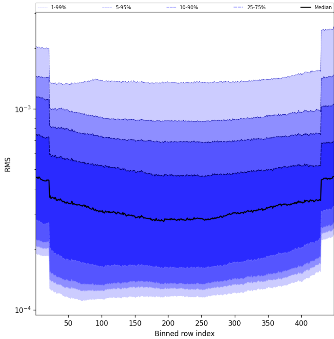
Figure 58: Along track statistics of “RMS” for 2025-03-19 to 2025-03-20
