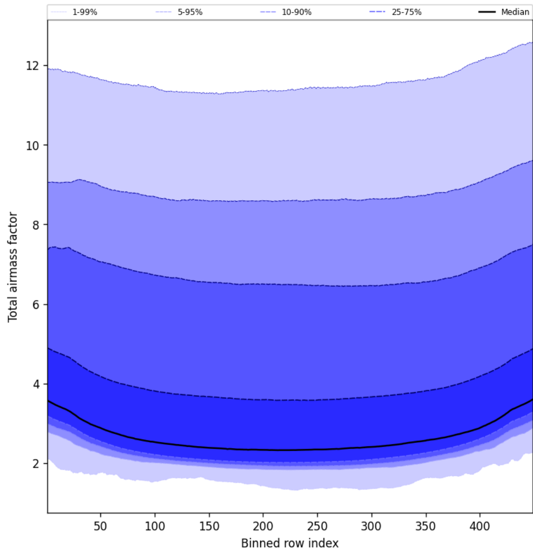
Figure 47: Along track statistics of “Total airmass factor” for 2025-03-19 to 2025-03-20
