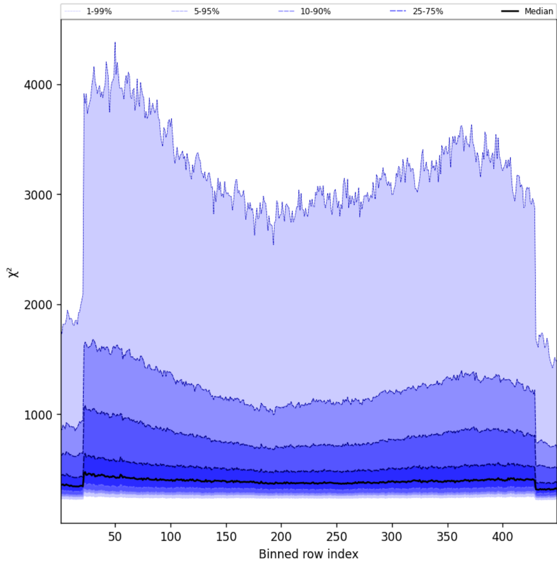
Figure 57: Along track statistics of “ \chi^2 ” for 2025-03-19 to 2025-03-20
