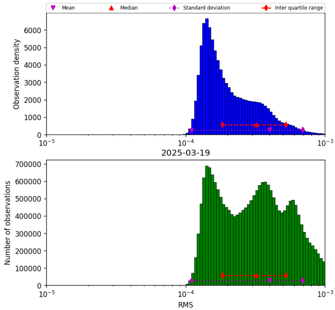
Figure 41: Histogram of “RMS” for 2025-03-19 to 2025-03-20
