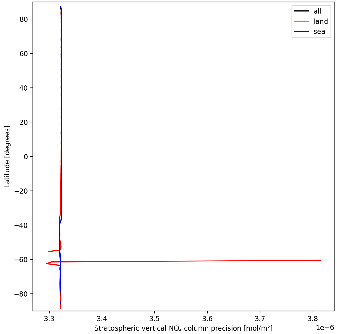
Figure 18: Zonal average of “Stratospheric vertical NO 2 column precision” for 2025-03-19 to 2025-03-20.
