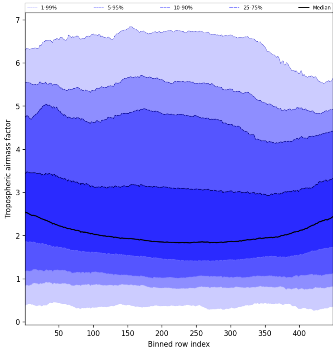
Figure 46: Along track statistics of “Tropospheric airmass factor” for 2025-03-19 to 2025-03-20
