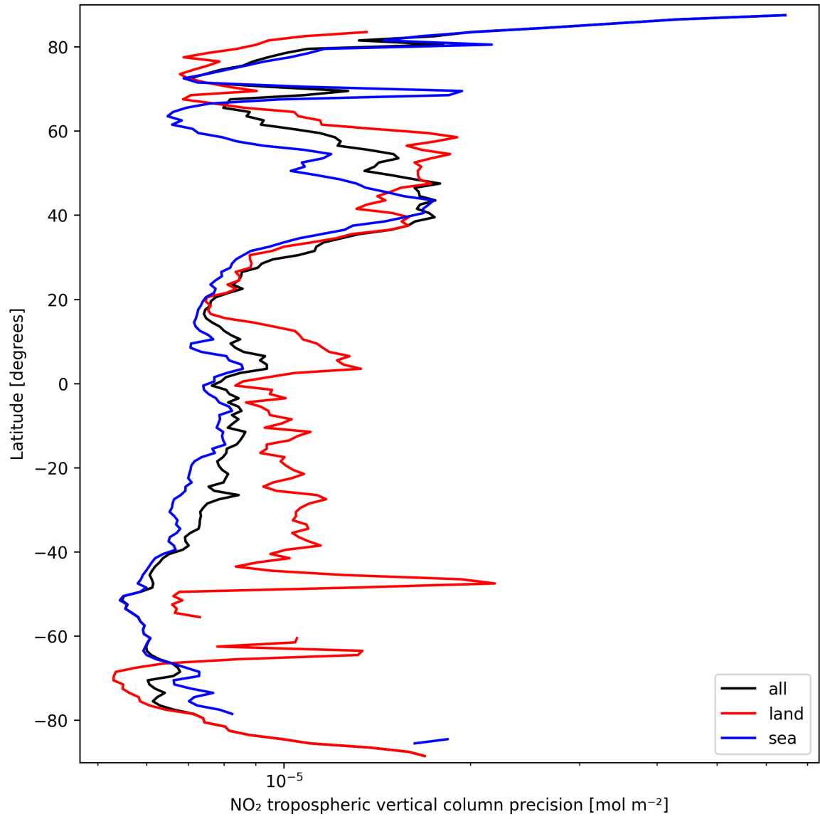
Figure 11: Zonal average of “NO 2 tropospheric vertical column precision” for 2025-03-19 to 2025-03-20.
