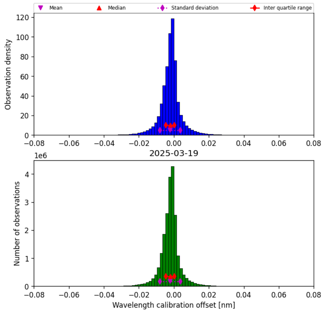
Figure 33: Histogram of “Wavelength calibration offset” for 2025-03-19 to 2025-03-20
