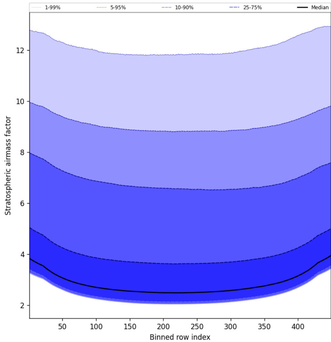
Figure 59: Along track statistics of “Stratospheric airmass factor” for 2025-03-19 to 2025-03-20
