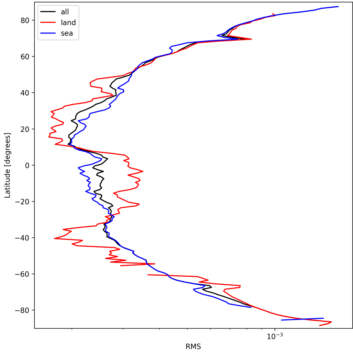
Figure 24: Zonal average of “RMS” for 2025-03-19 to 2025-03-20.
