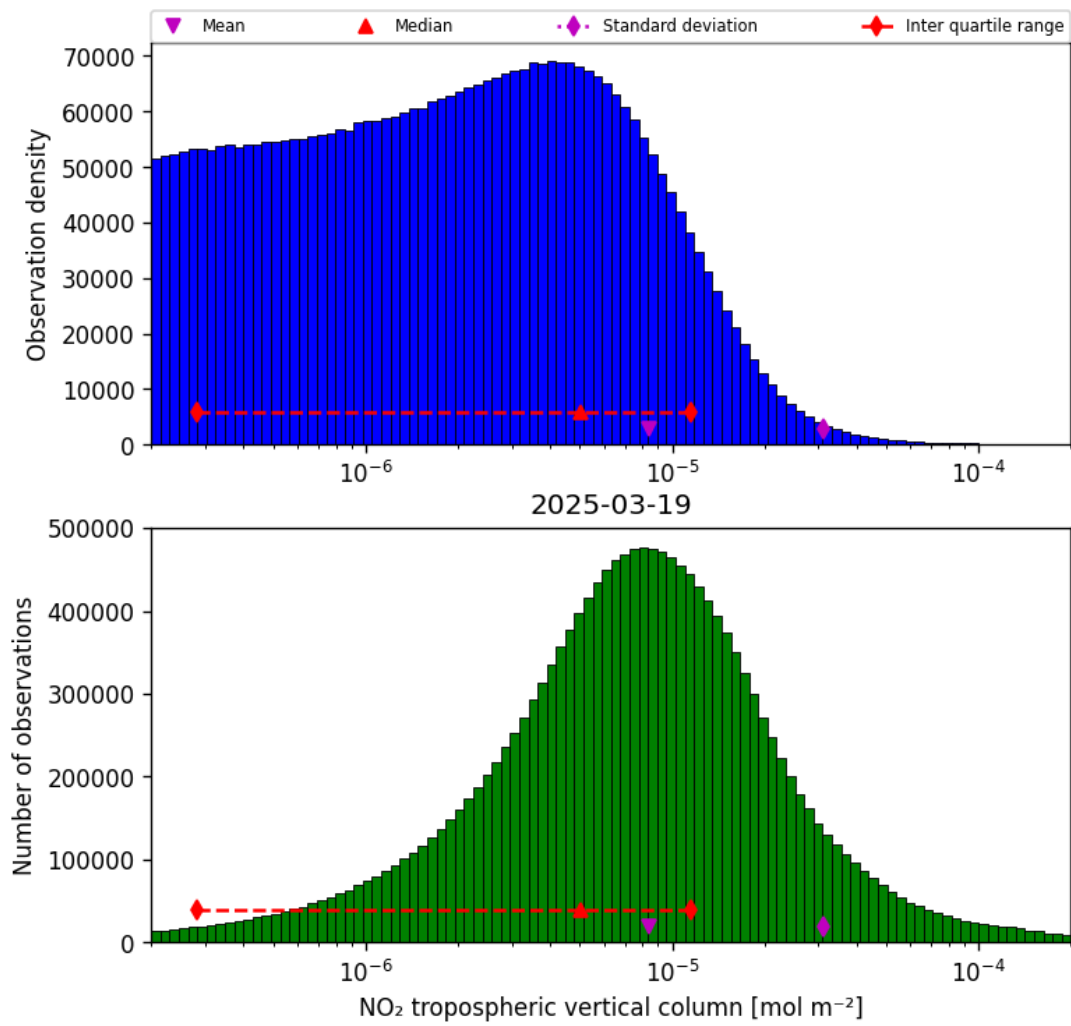
Figure 27: Histogram of “NO 2 tropospheric vertical column” for 2025-03-19 to 2025-03-20
