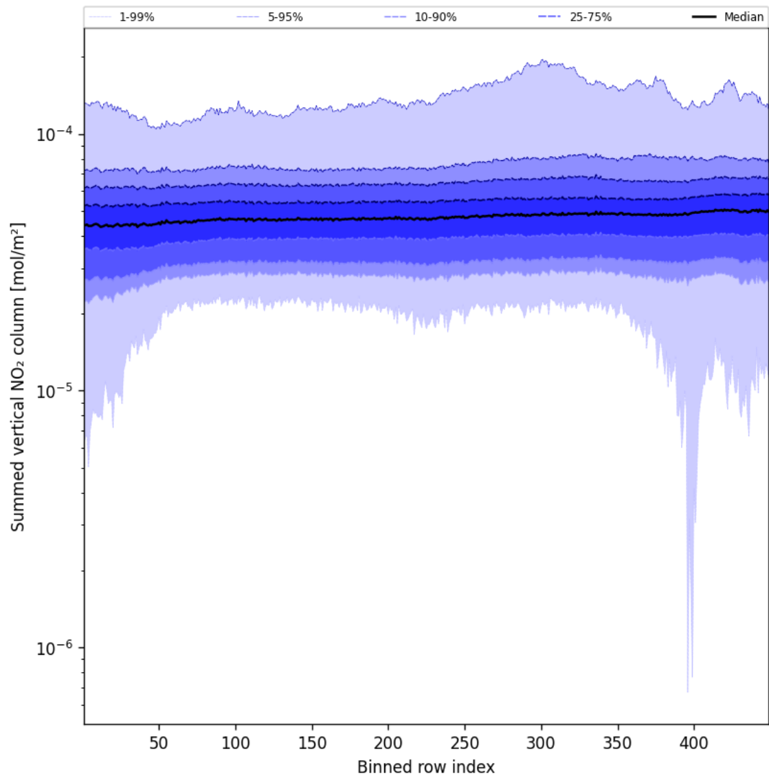
Figure 55: Along track statistics of “Summed vertical NO 2 column” for 2025-03-19 to 2025-03-20
