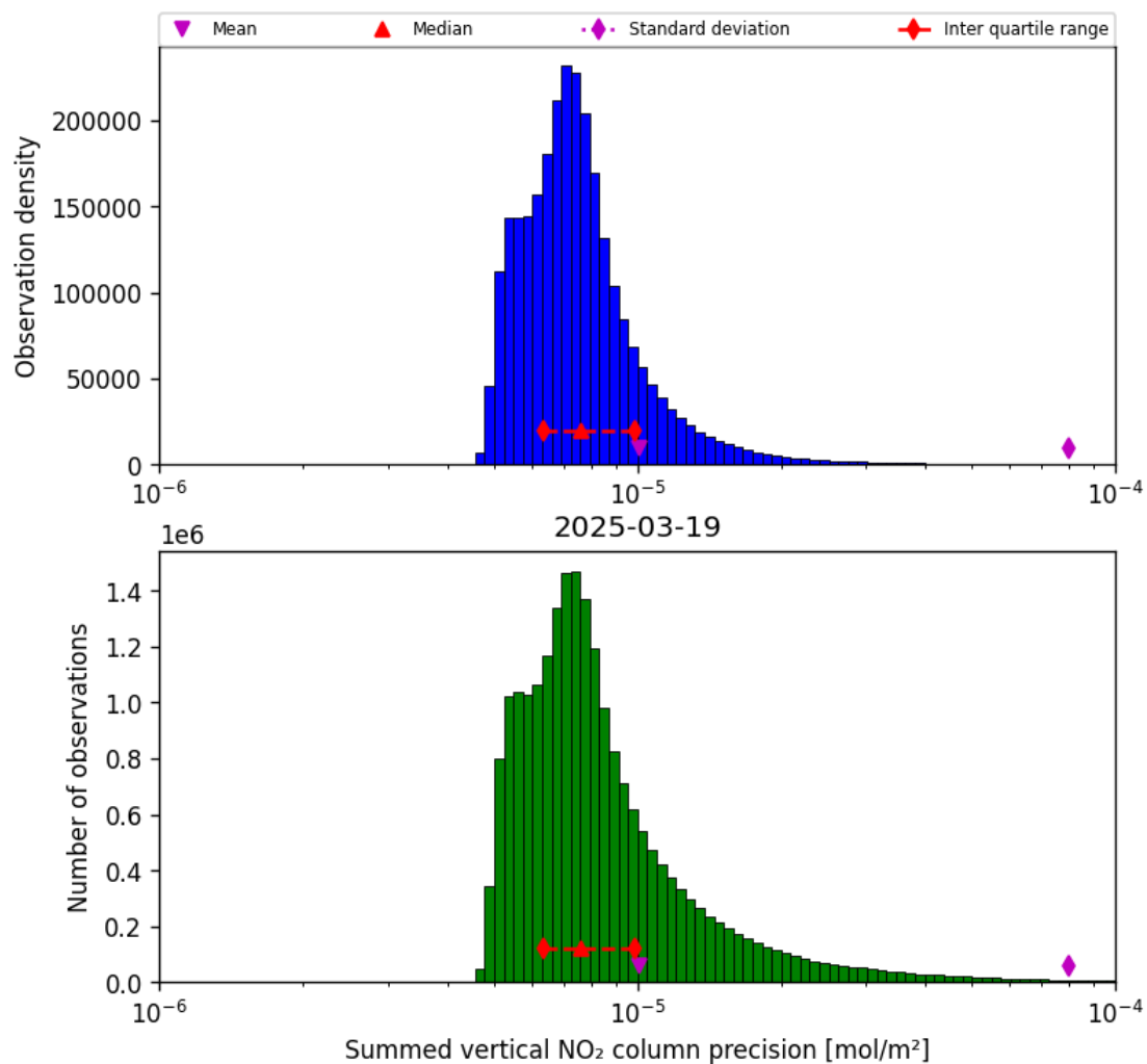
Figure 39: Histogram of "Summed vertical NO 2 column precision" for 2025-03-19 to 2025-03-20
