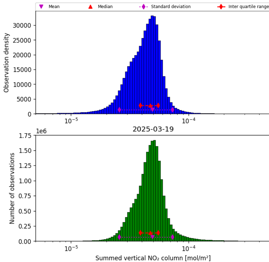
Figure 38: Histogram of “Summed vertical NO 2 column” for 2025-03-19 to 2025-03-20
