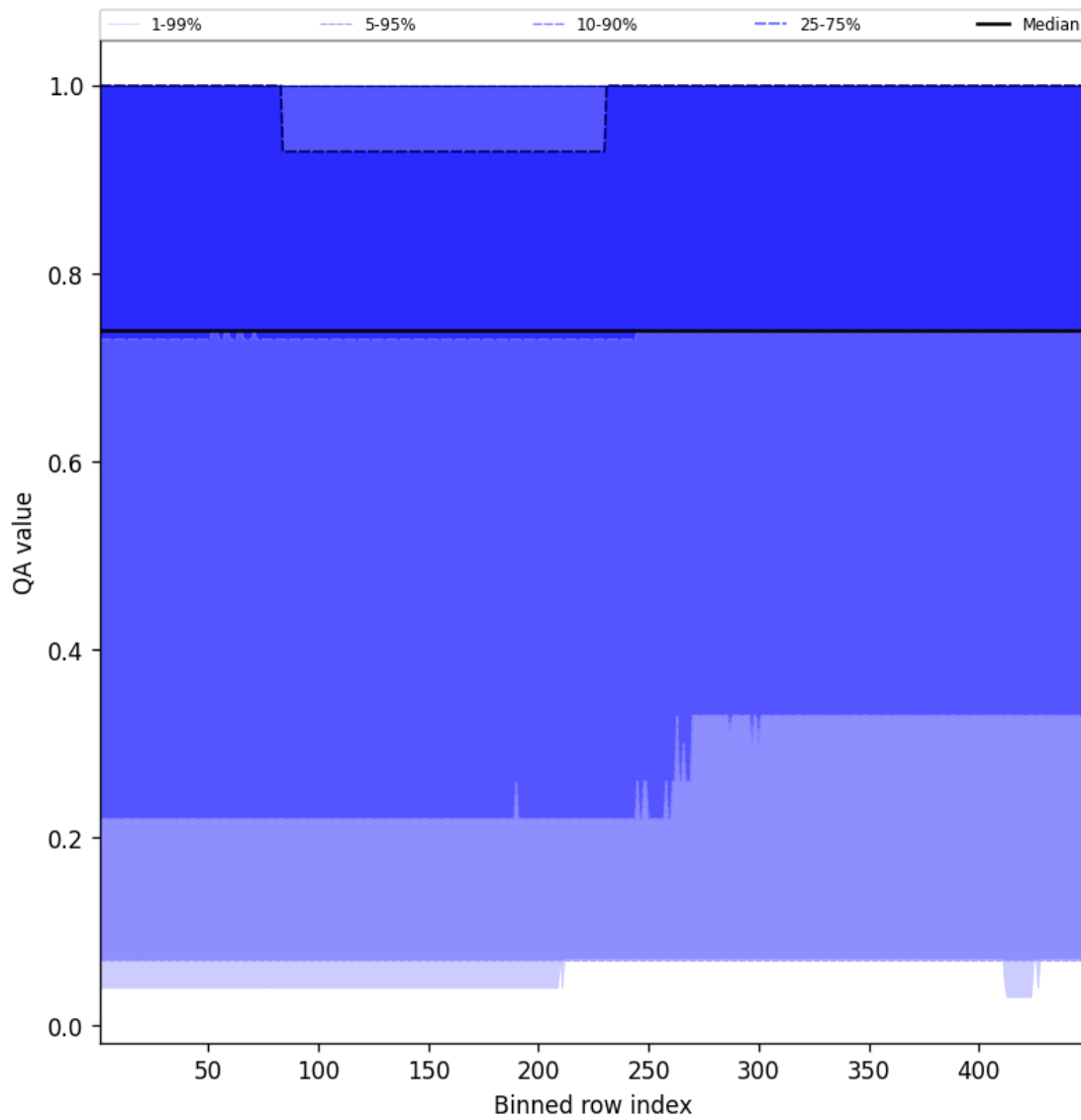
Figure 43: Along track statistics of “QA value” for 2025-03-19 to 2025-03-20
