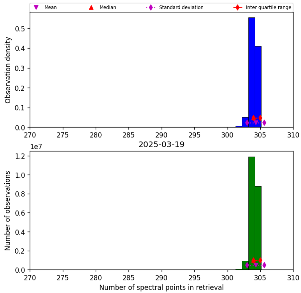
Figure 31: Histogram of “Number of spectral points in retrieval” for 2025-03-19 to 2025-03-20
