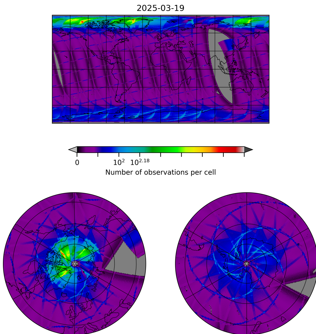
Figure 8: Map of the number of observations for 2025-03-19 to 2025-03-20
