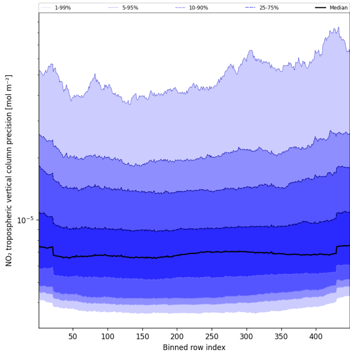
Figure 45: Along track statistics of “NO 2 tropospheric vertical column precision” for 2025-03-19 to 2025-03-20
