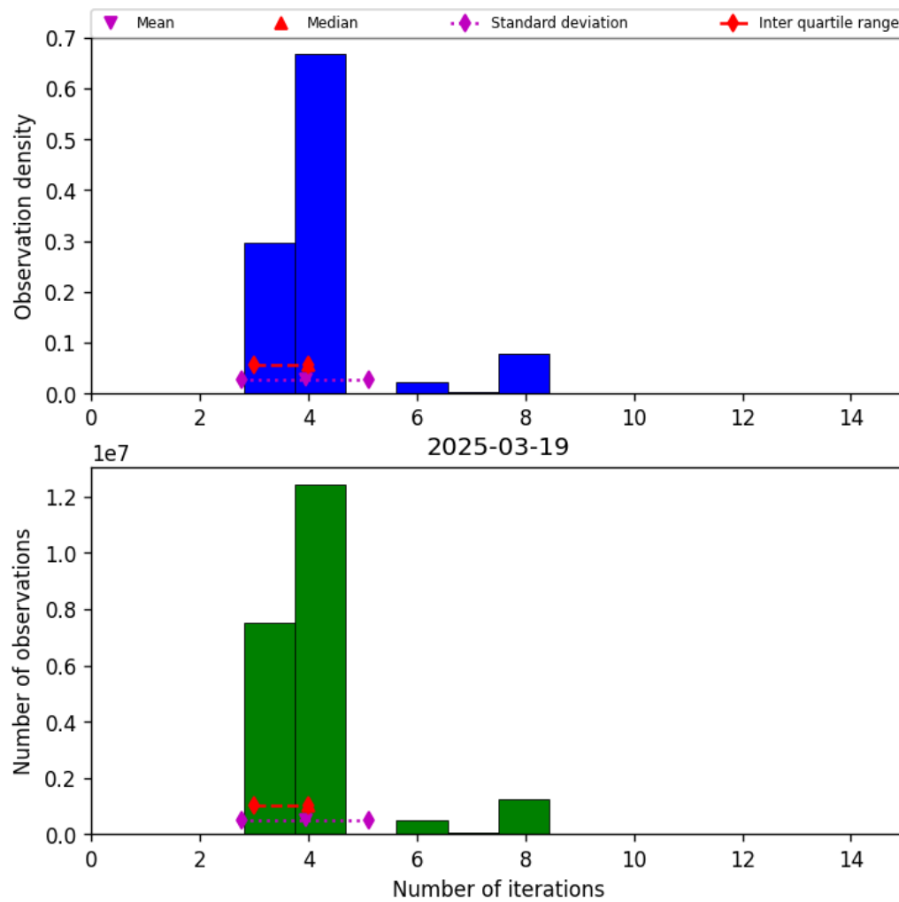
Figure 32: Histogram of “Number of iterations” for 2025-03-19 to 2025-03-20
