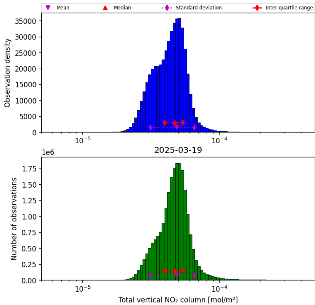
Figure 36: Histogram of “Total vertical NO 2 column” for 2025-03-19 to 2025-03-20
