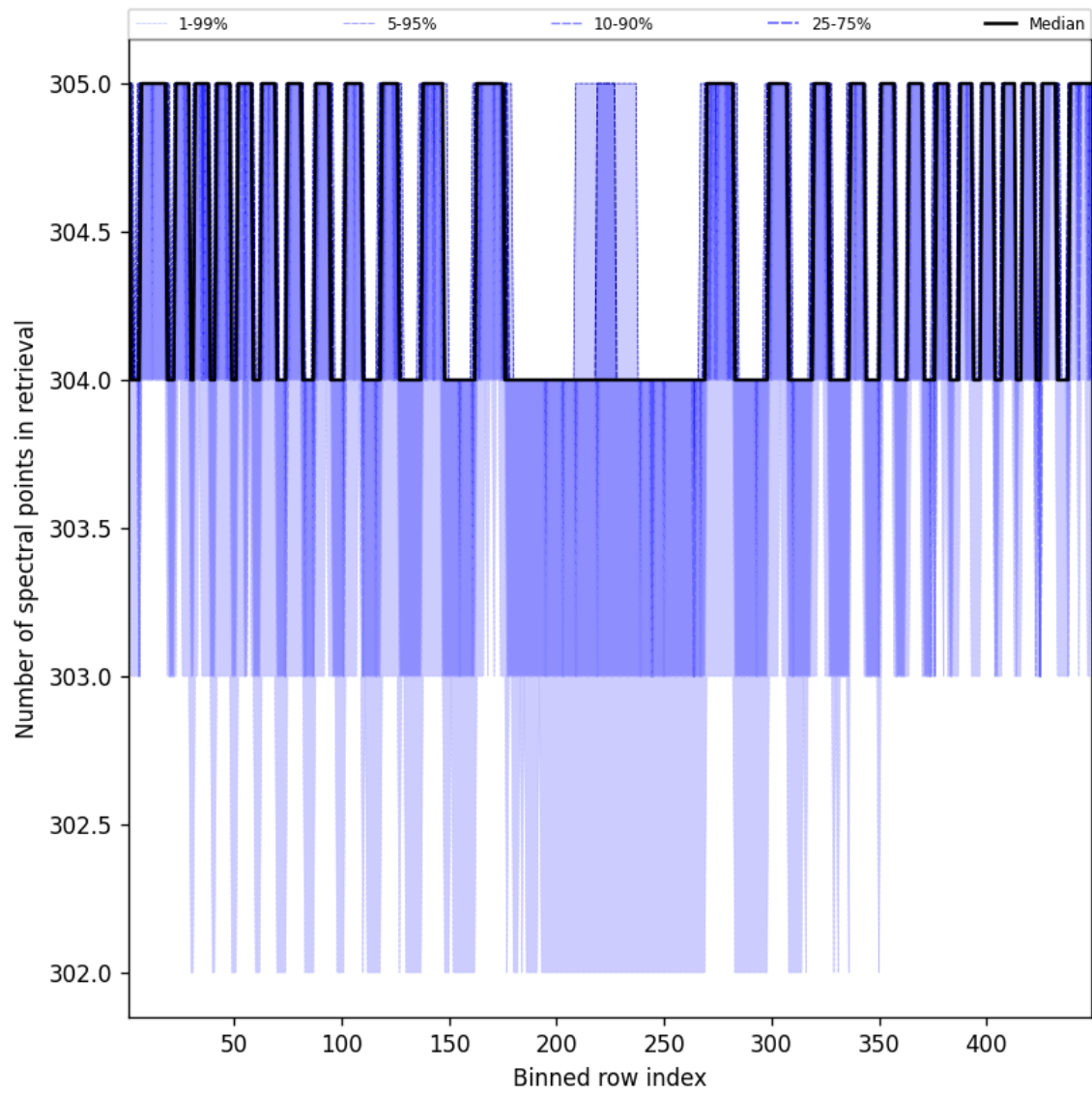
Figure 48: Along track statistics of “Number of spectral points in retrieval” for 2025-03-19 to 2025-03-20
