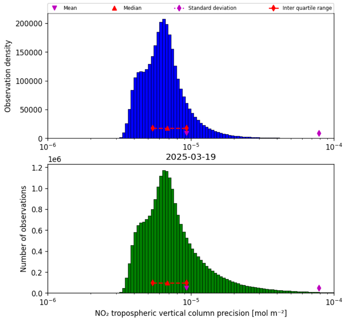
Figure 28: Histogram of “NO 2 tropospheric vertical column precision” for 2025-03-19 to 2025-03-20
