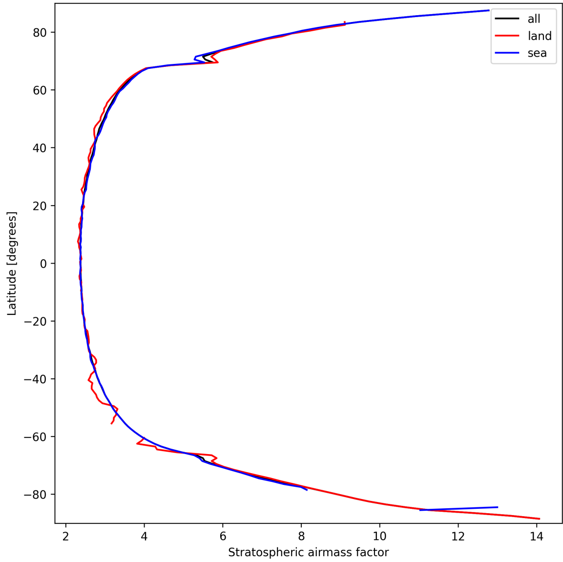
Figure 25: Zonal average of “Stratospheric air mass factor” for 2025-03-19 to 2025-03-20.
