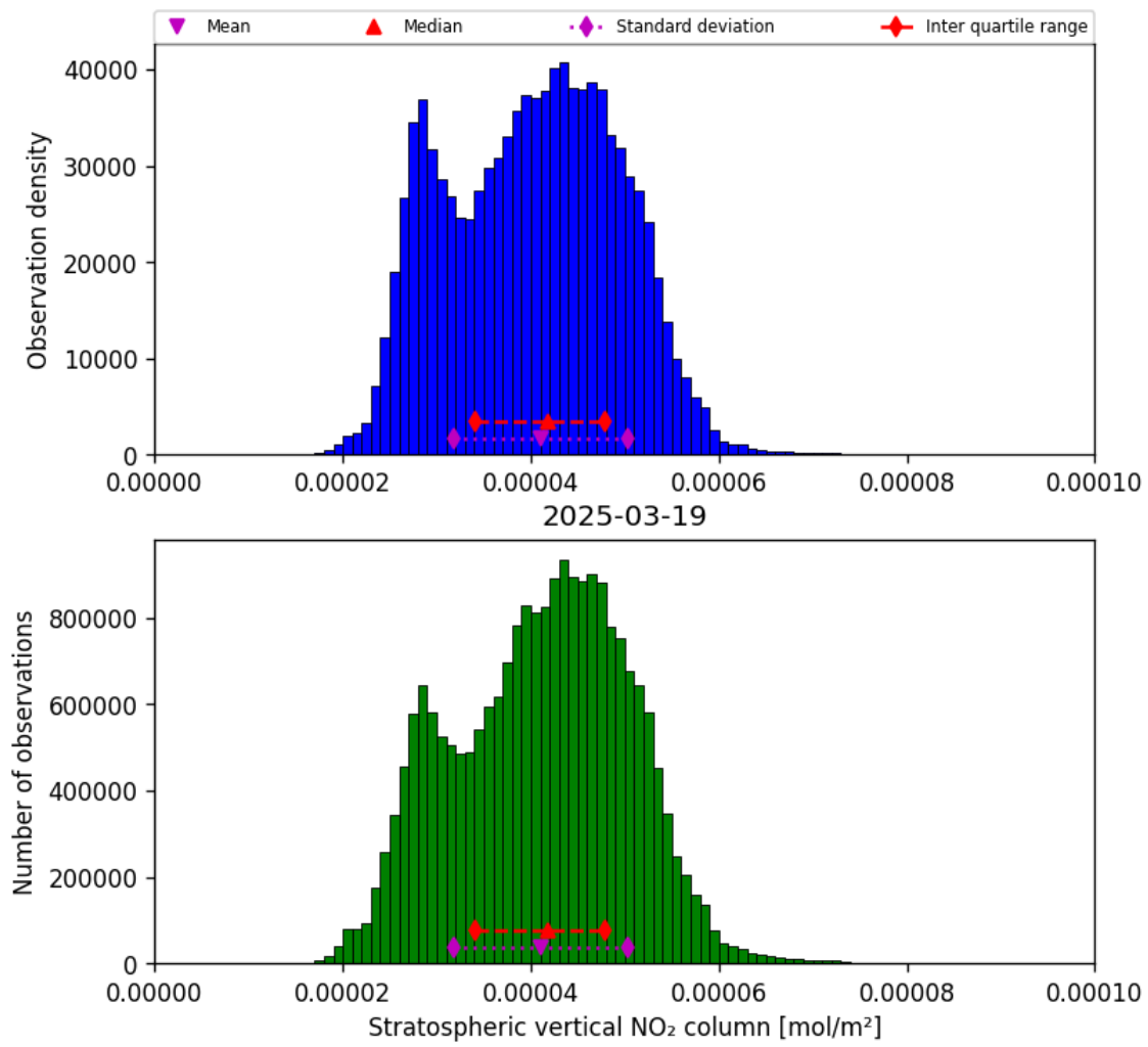
Figure 34: Histogram of “Stratospheric vertical NO 2 column” for 2025-03-19 to 2025-03-20
