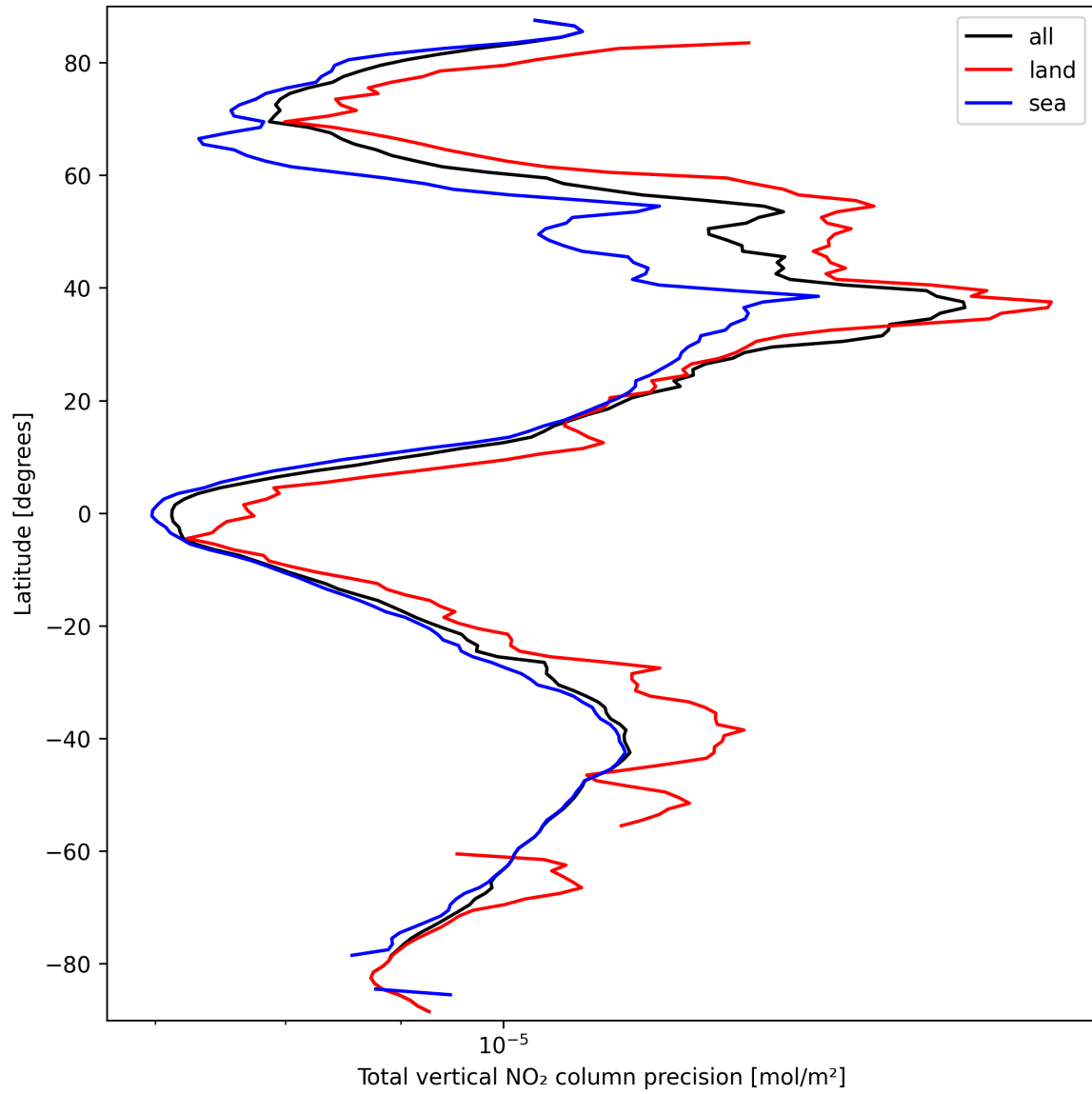
Figure 20: Zonal average of “Total vertical NO 2 column precision” for 2025-03-19 to 2025-03-20.
