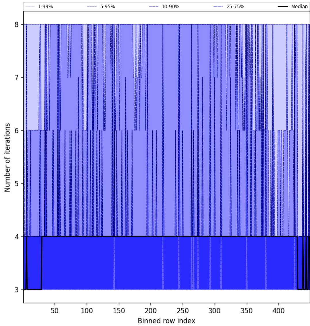
Figure 49: Along track statistics of “Number of iterations” for 2025-03-19 to 2025-03-20
