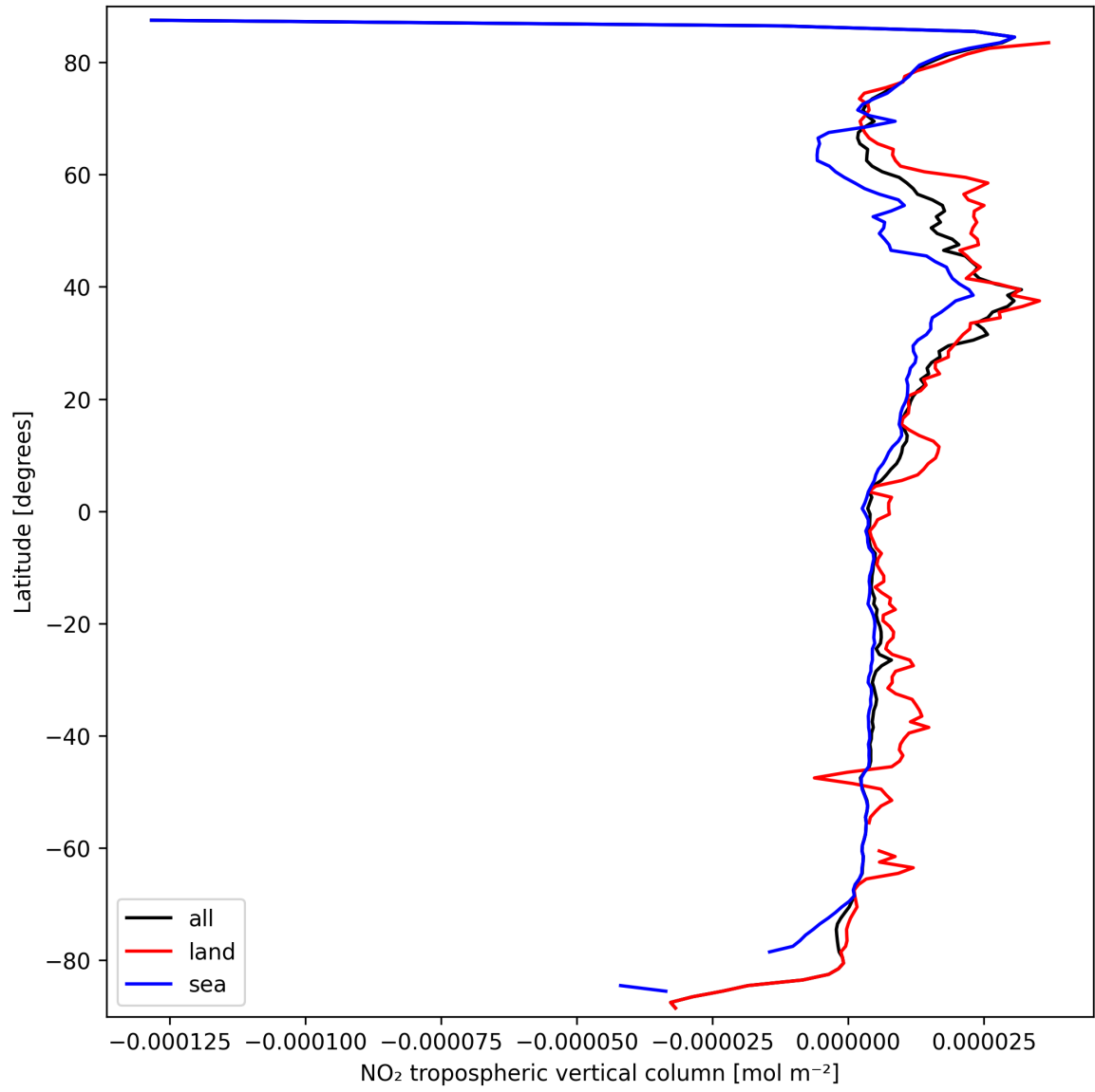
Figure 10: Zonal average of “NO 2 tropospheric vertical column” for 2025-03-19 to 2025-03-20.
