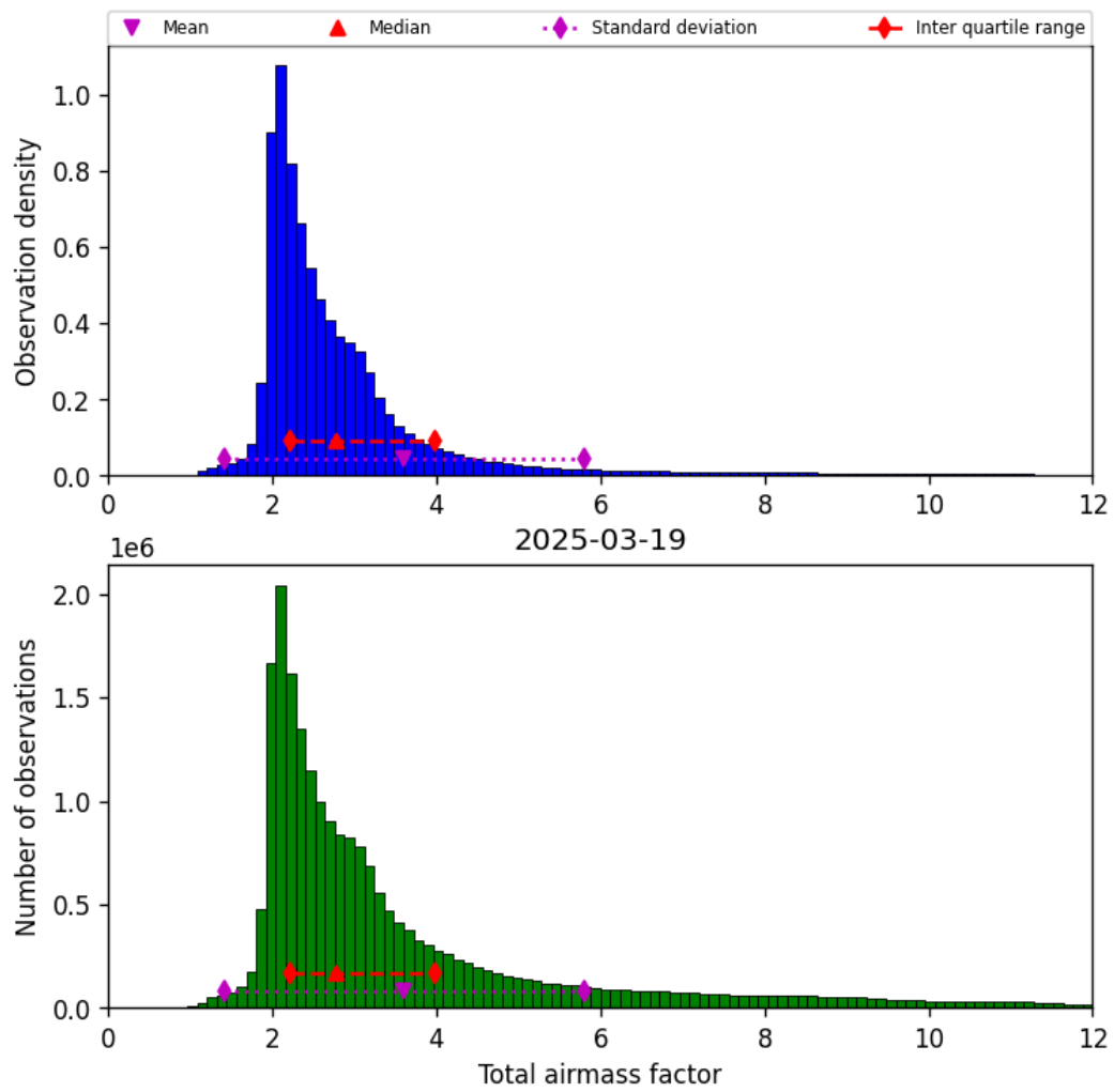
Figure 30: Histogram of “Total airmass factor” for 2025-03-19 to 2025-03-20
