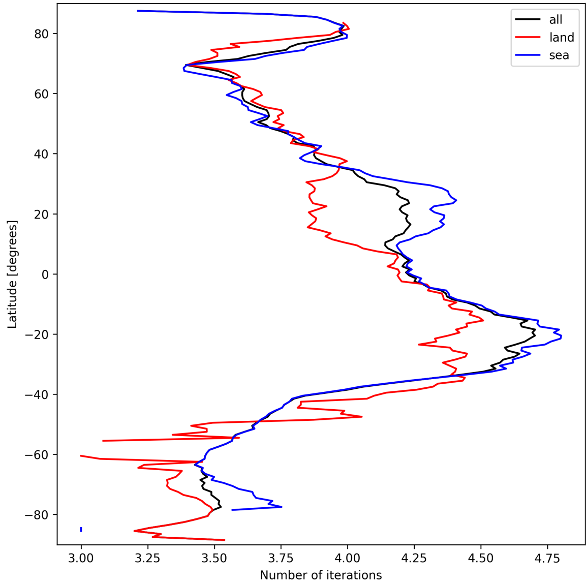
Figure 15: Zonal average of “Number of iterations” for 2025-03-19 to 2025-03-20.
