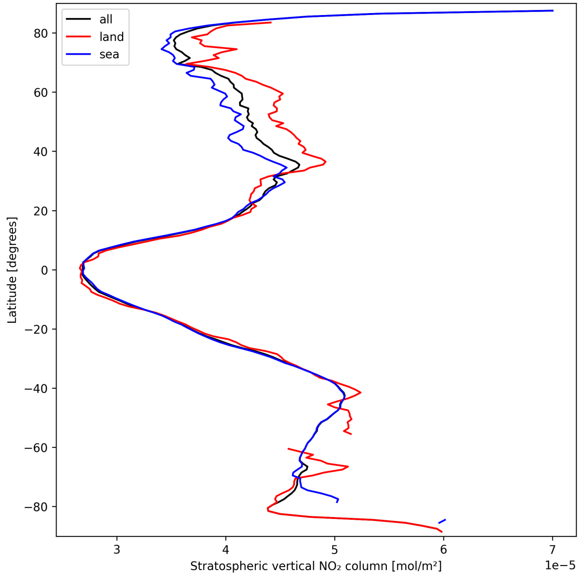
Figure 17: Zonal average of “Stratospheric vertical NO 2 column” for 2025-03-19 to 2025-03-20.
