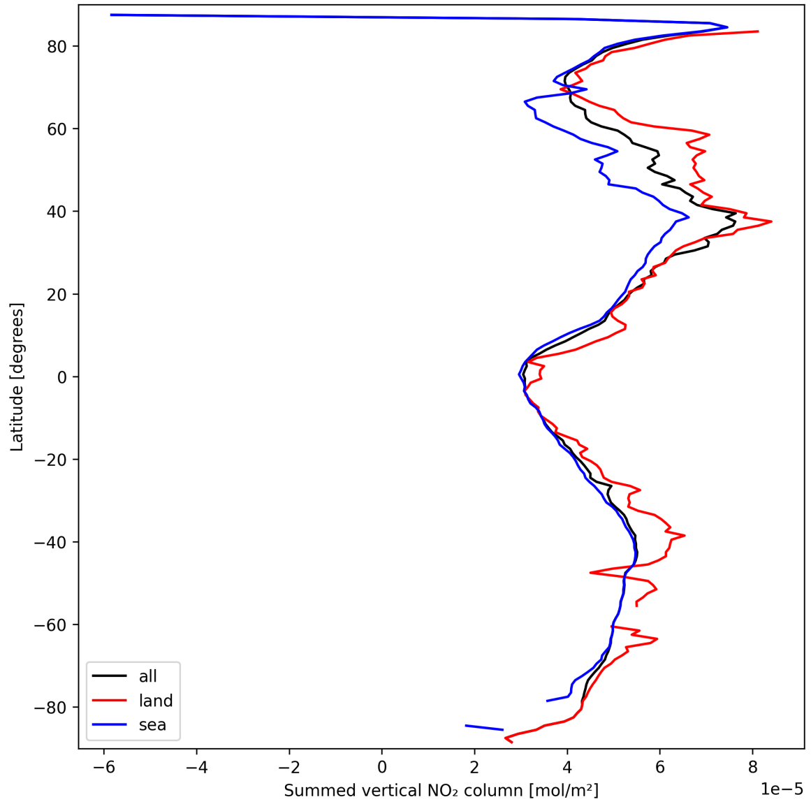
Figure 21: Zonal average of “Summed vertical NO 2 column” for 2025-03-19 to 2025-03-20.
