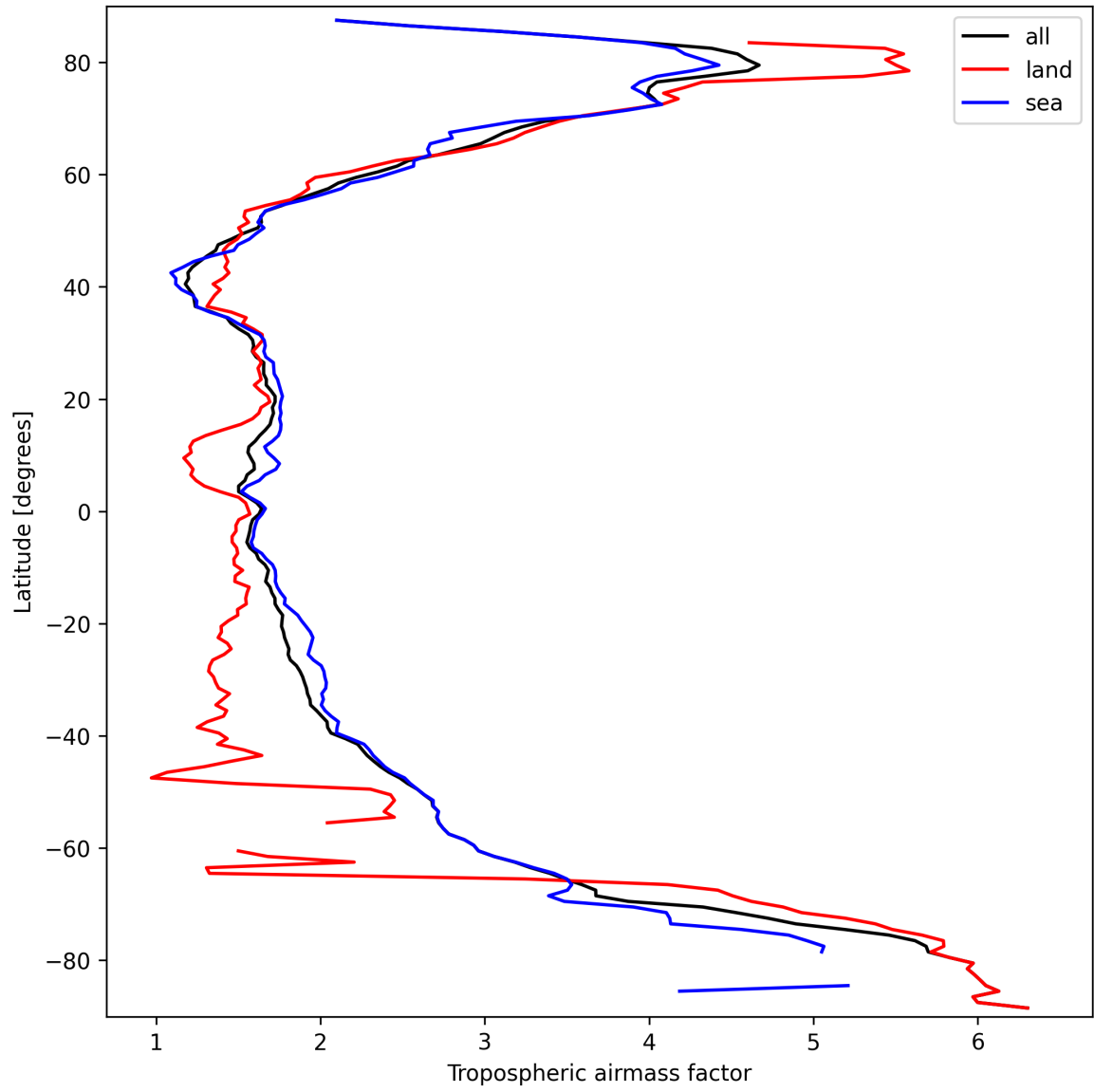
Figure 12: Zonal average of “Tropospheric air mass factor” for 2025-03-19 to 2025-03-20.
