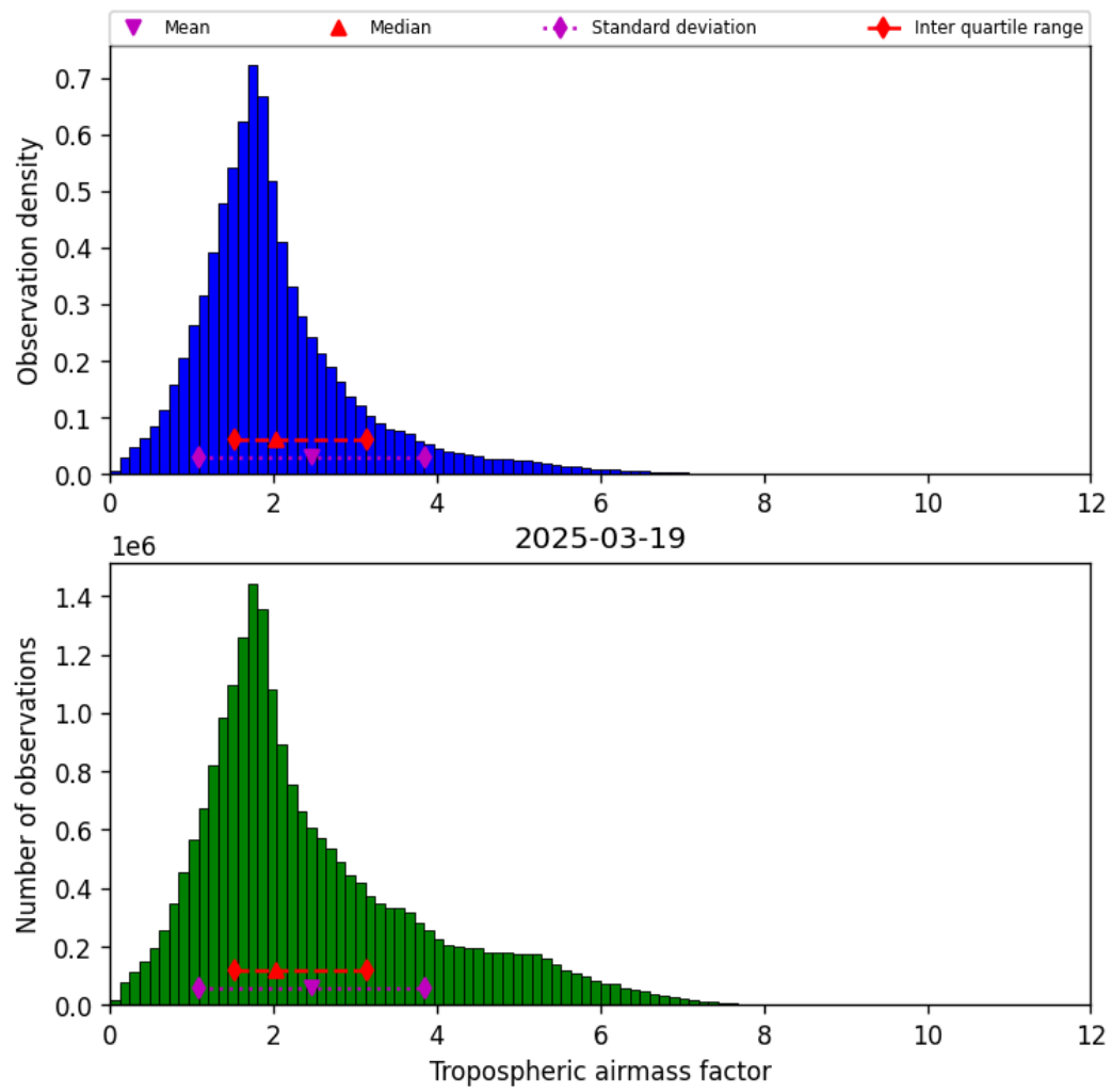
Figure 29: Histogram of “Tropospheric airmass factor” for 2025-03-19 to 2025-03-20
