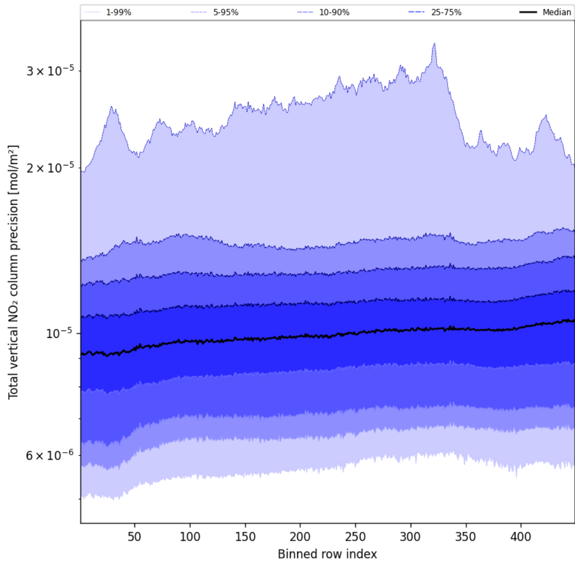
Figure 54: Along track statistics of “Total vertical NO 2 column precision” for 2025-03-19 to 2025-03-20
