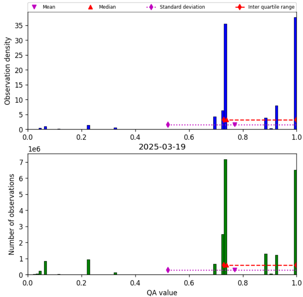
Figure 26: Histogram of “QA value” for 2025-03-19 to 2025-03-20
