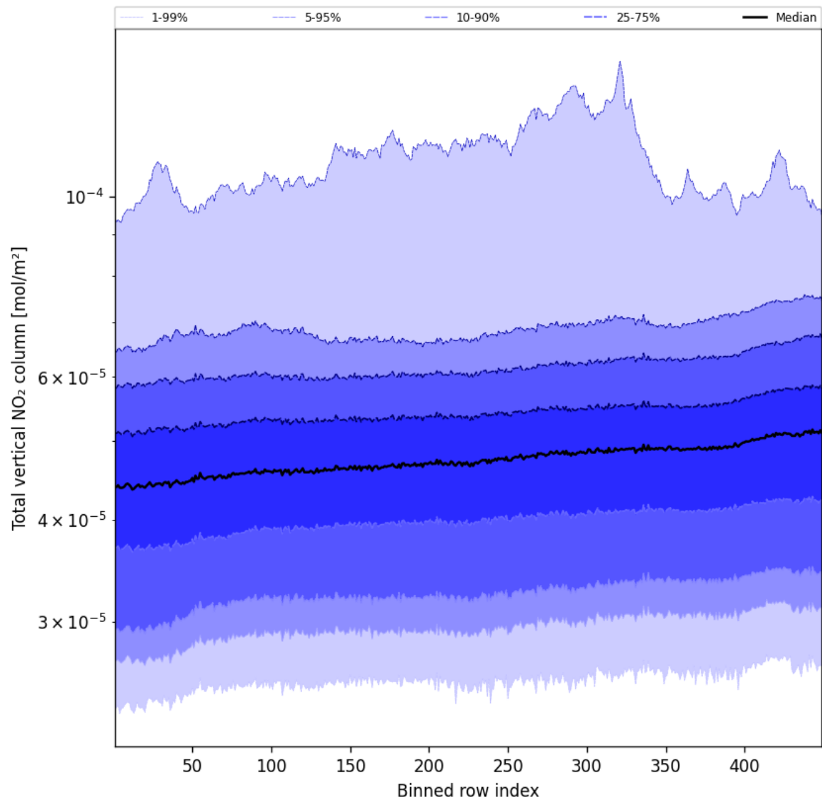
Figure 53: Along track statistics of “Total vertical NO 2 column” for 2025-03-19 to 2025-03-20
