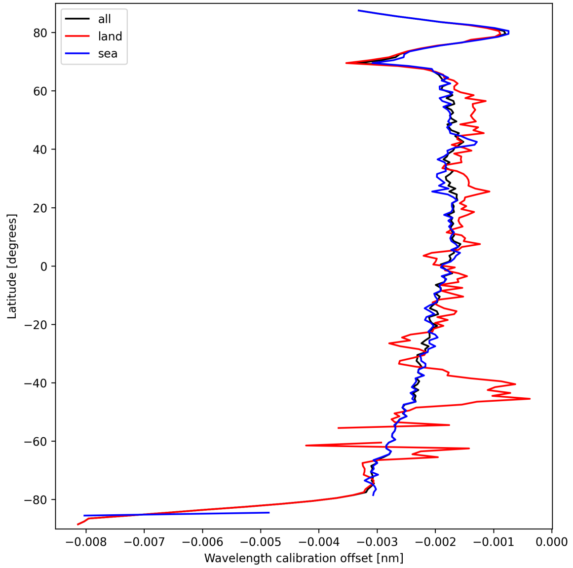
Figure 16: Zonal average of “Wavelength calibration offset” for 2025-03-19 to 2025-03-20.
