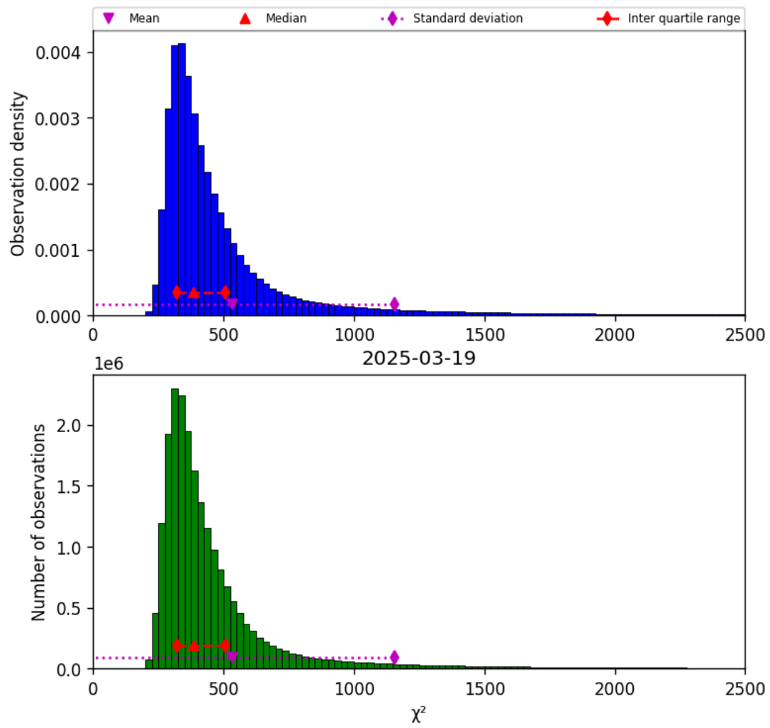
Figure 40: Histogram of “ \chi^2 ” for 2025-03-19 to 2025-03-20
