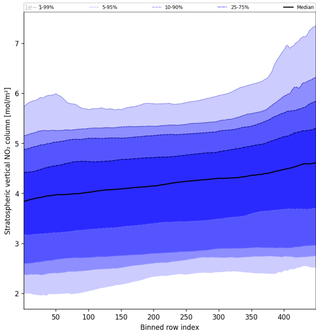
Figure 51: Along track statistics of “Stratospheric vertical NO 2 column” for 2025-03-19 to 2025-03-20
