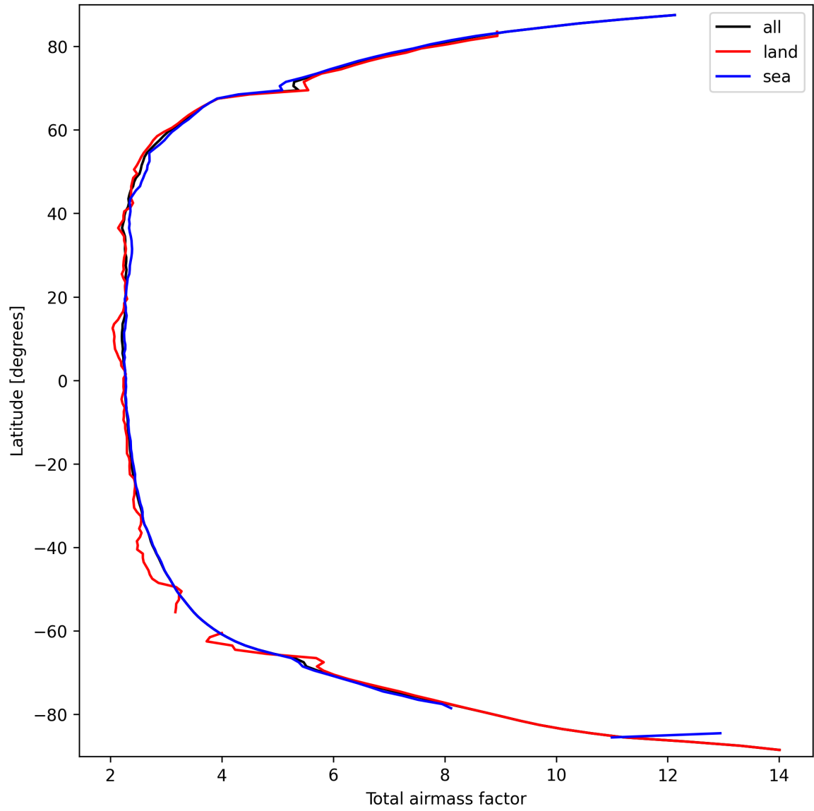
Figure 13: Zonal average of “Total airmass factor” for 2025-03-19 to 2025-03-20.
