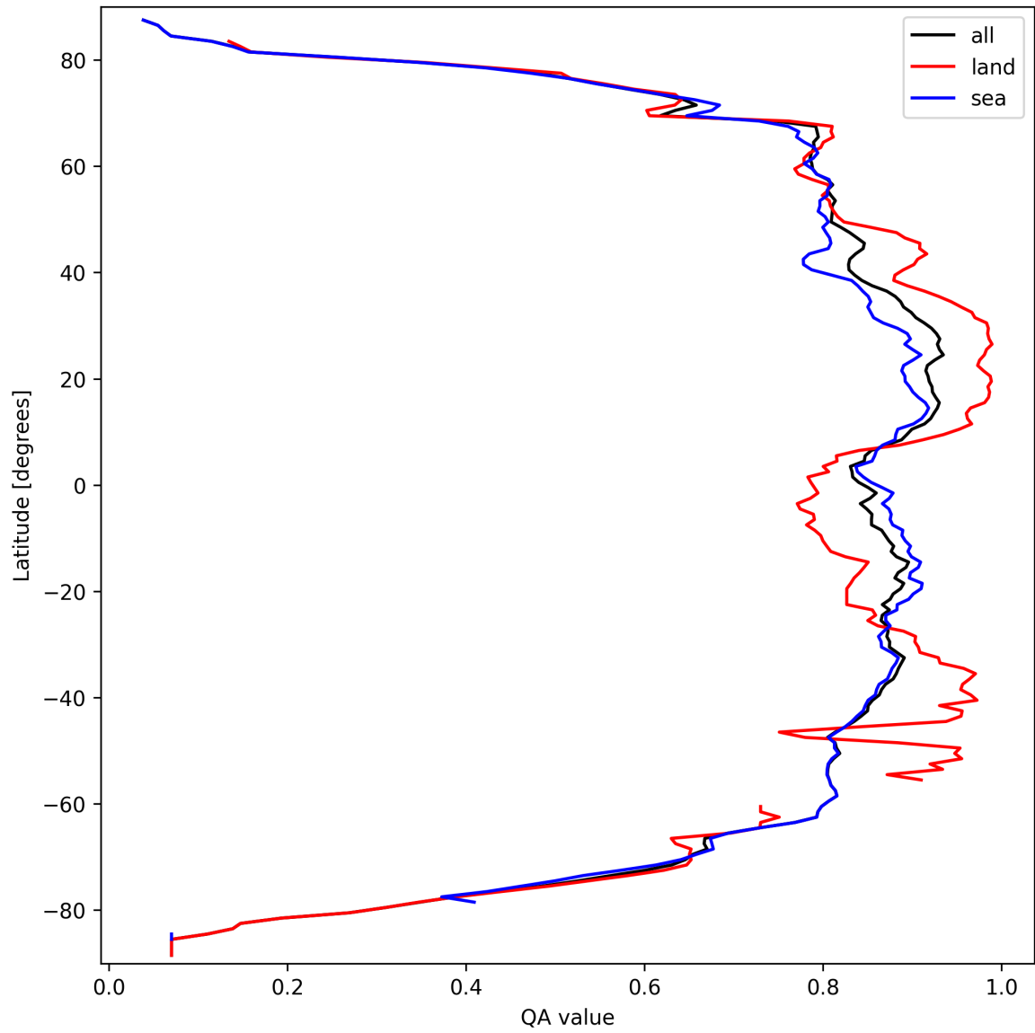
Figure 9: Zonal average of “QA value” for 2025-03-19 to 2025-03-20.
