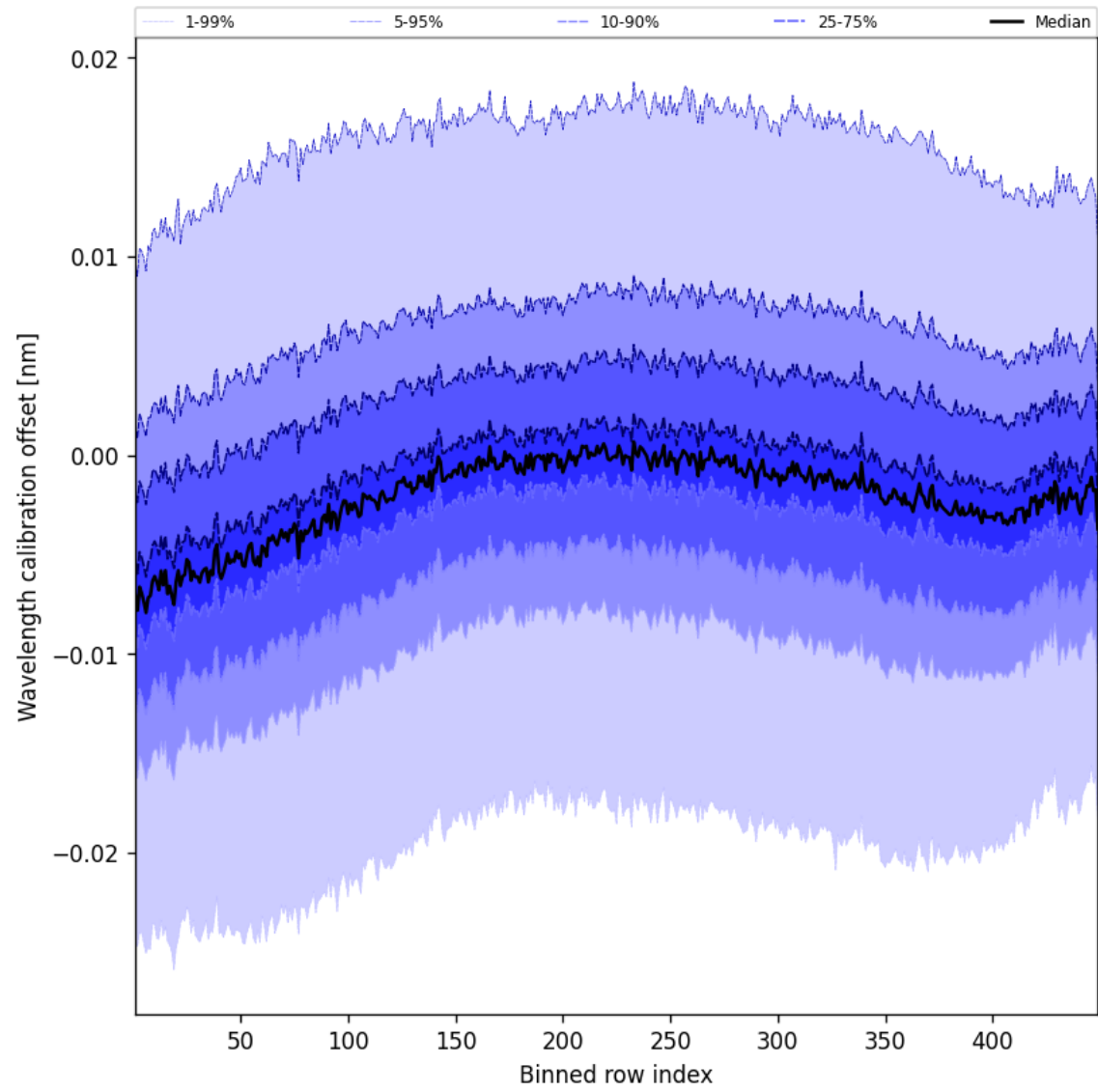
Figure 50: Along track statistics of “Wavelength calibration offset” for 2025-03-19 to 2025-03-20
