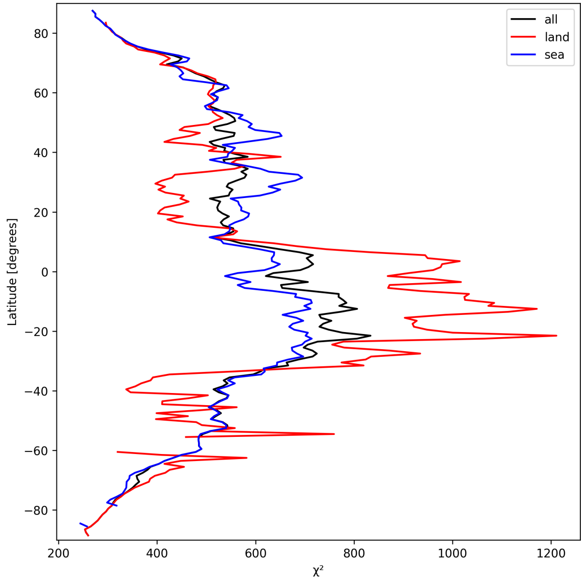
Figure 23: Zonal average of “ \chi^2 ” for 2025-03-19 to 2025-03-20.
