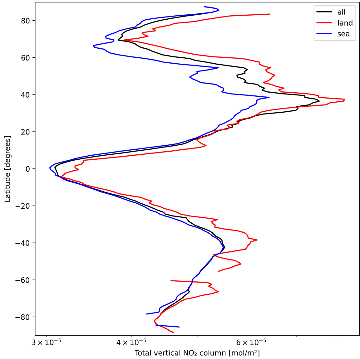
Figure 19: Zonal average of “Total vertical NO 2 column” for 2025-03-19 to 2025-03-20.
