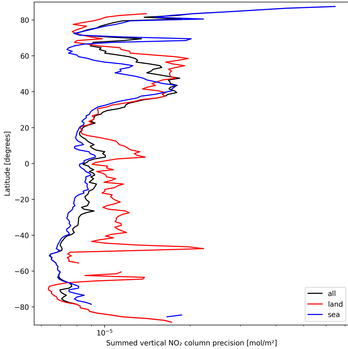
Figure 22: Zonal average of “Summed vertical NO 2 column precision” for 2025-03-19 to 2025-03-20.
