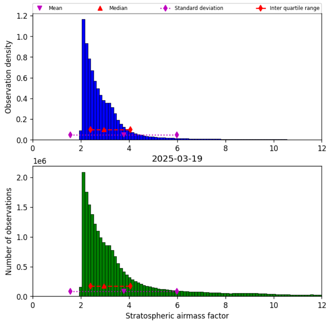
Figure 42: Histogram of “Stratospheric airmass factor” for 2025-03-19 to 2025-03-20
