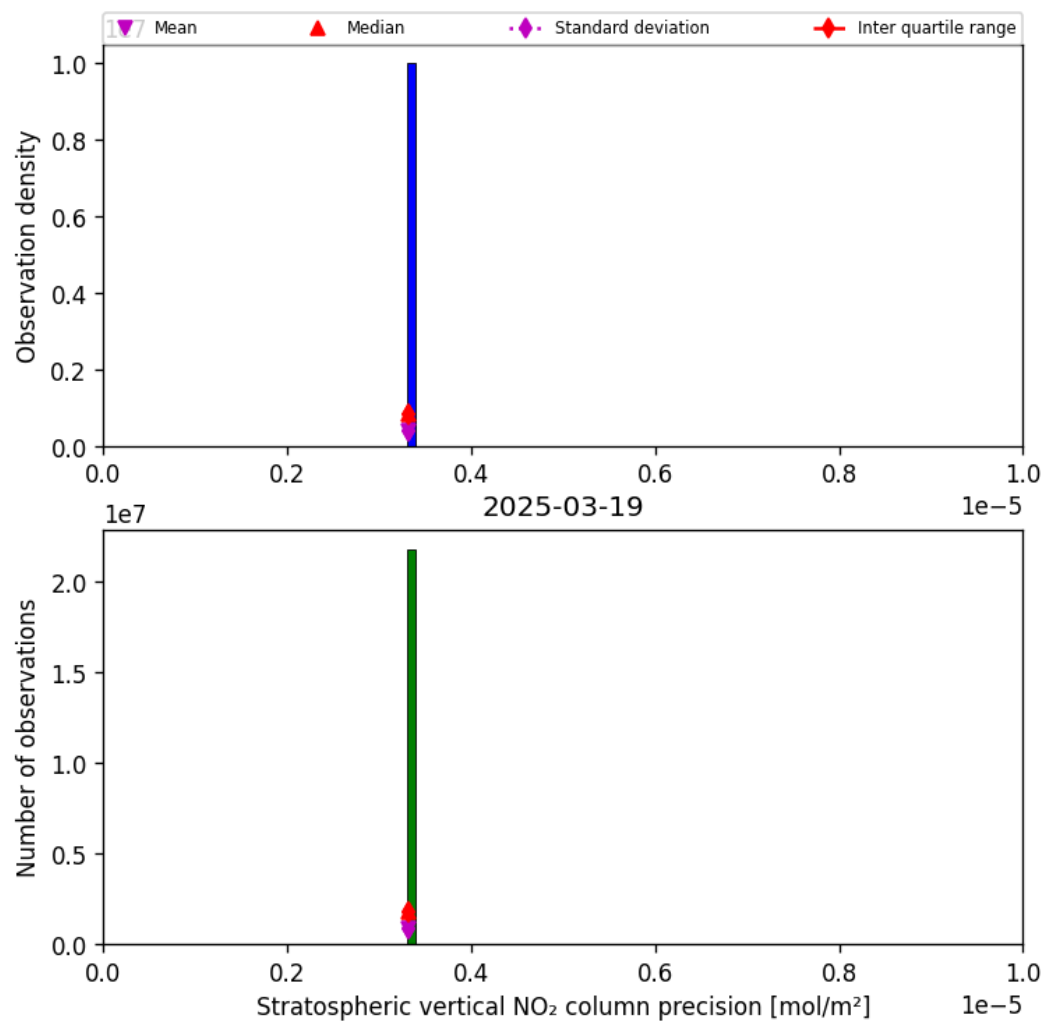
Figure 35: Histogram of “Stratospheric vertical NO 2 column precision” for 2025-03-19 to 2025-03-20
