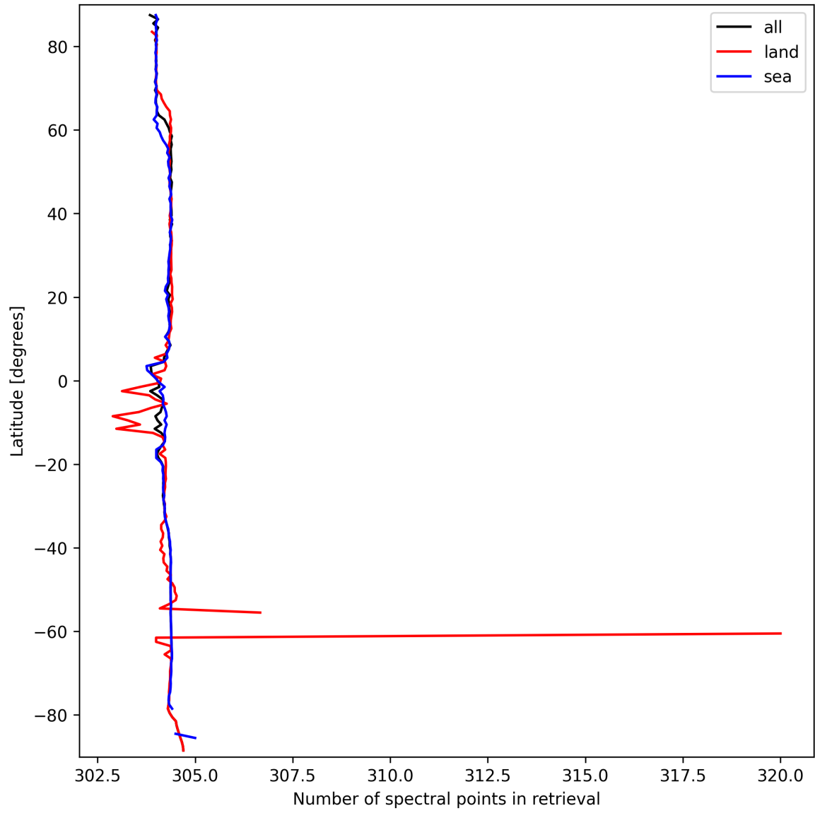
Figure 14: Zonal average of “Number of spectral points in retrieval” for 2025-03-19 to 2025-03-20.
