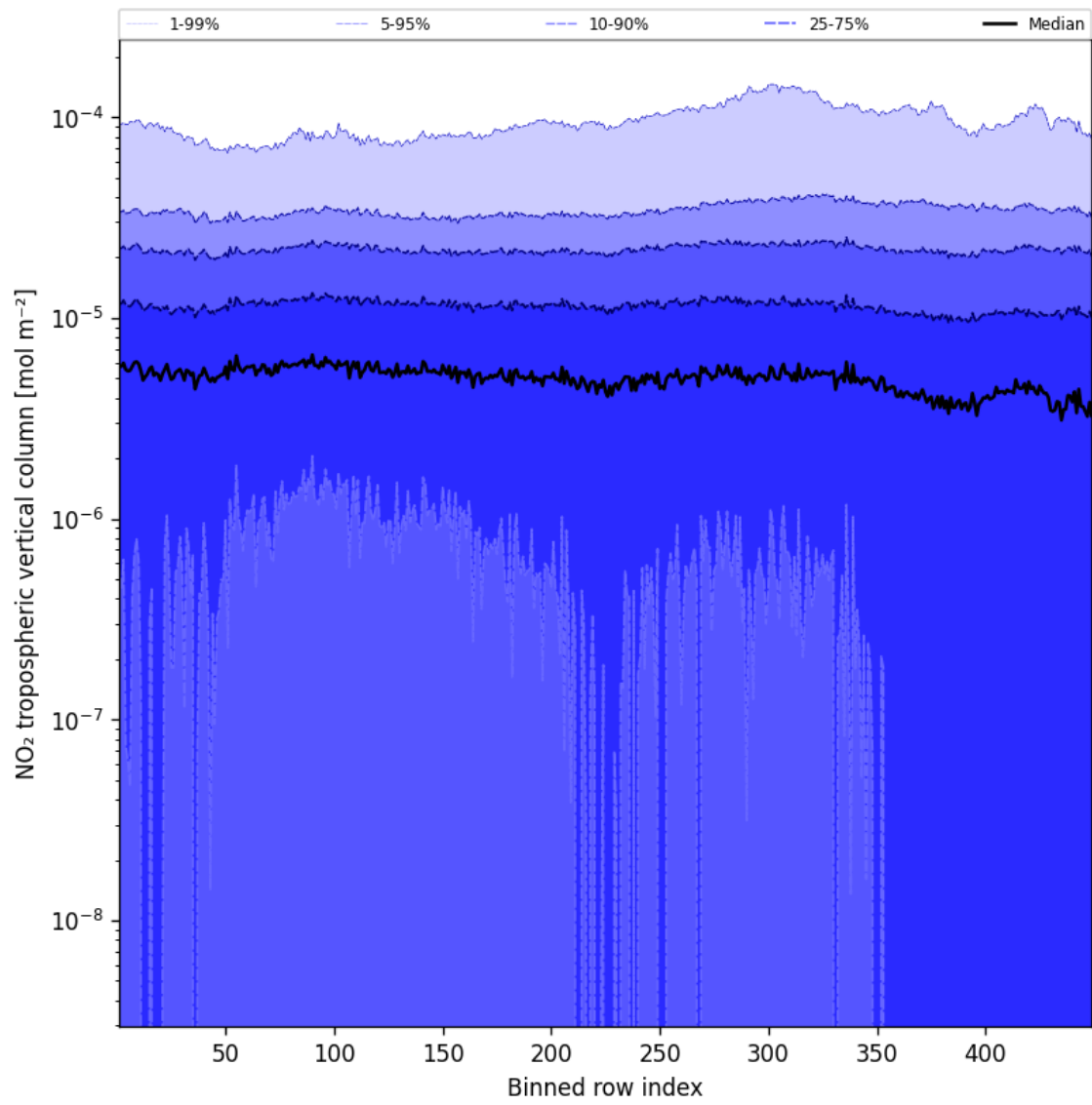
Figure 44: Along track statistics of “NO 2 tropospheric vertical column” for 2025-03-19 to 2025-03-20
