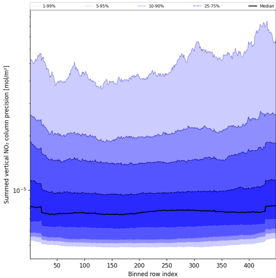
Figure 56: Along track statistics of “Summed vertical NO 2 column precision” for 2025-03-19 to 2025-03-20
