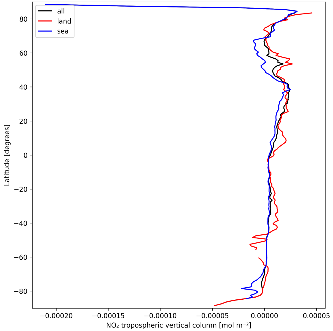
Figure 10: Zonal average of “NO 2 tropospheric vertical column” for 2025-03-20 to 2025-03-21.
