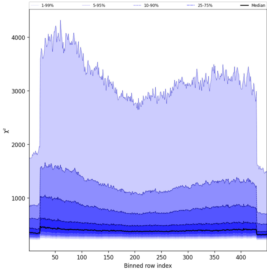
Figure 57: Along track statistics of “ \chi^2 ” for 2025-03-20 to 2025-03-21
