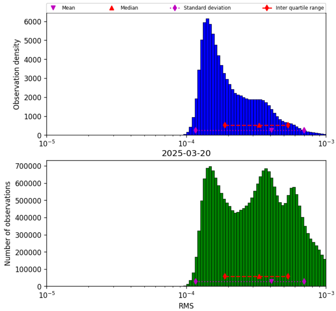
Figure 41: Histogram of “RMS” for 2025-03-20 to 2025-03-21
