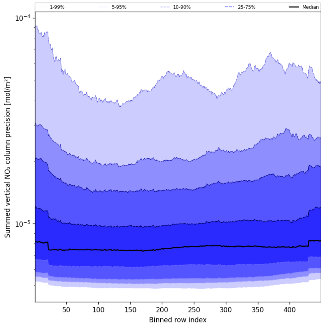
Figure 56: Along track statistics of “Summed vertical NO 2 column precision” for 2025-03-20 to 2025-03-21
