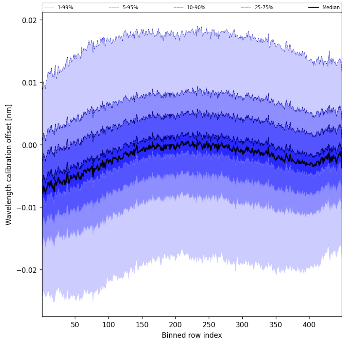
Figure 50: Along track statistics of “Wavelength calibration offset” for 2025-03-20 to 2025-03-21
