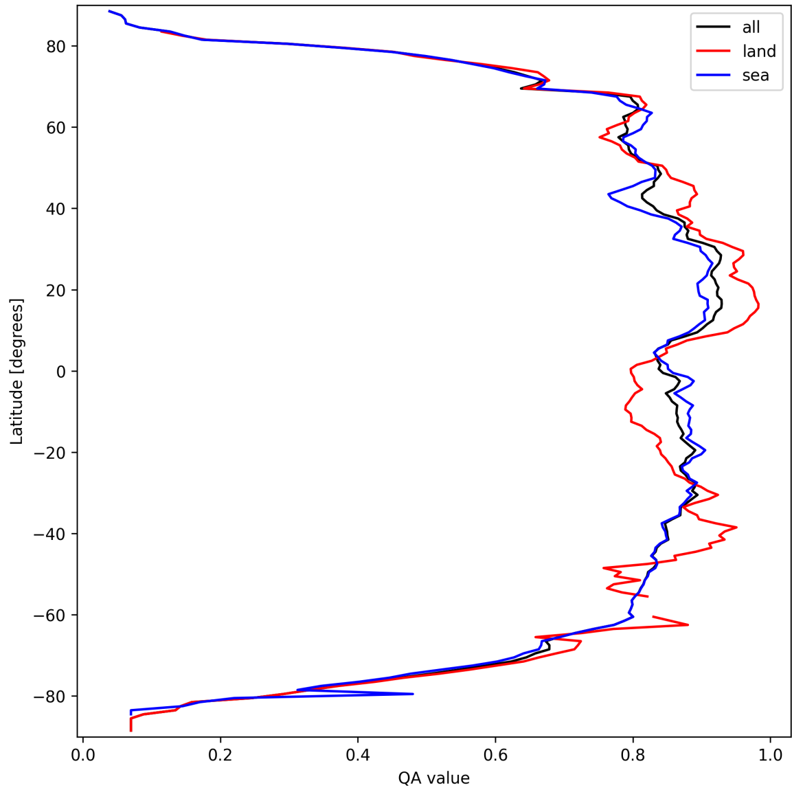
Figure 9: Zonal average of “QA value” for 2025-03-20 to 2025-03-21.
