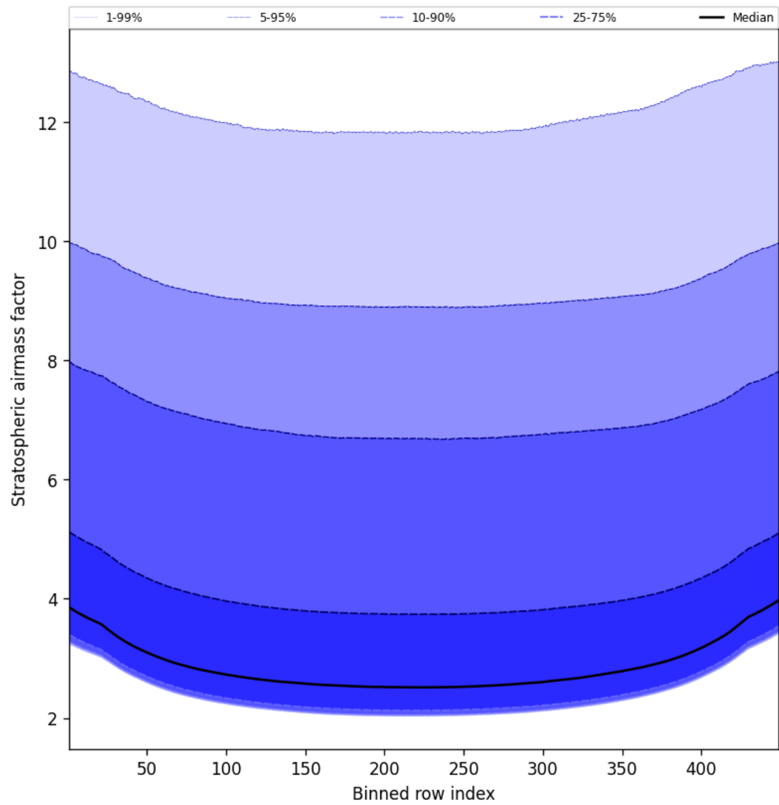
Figure 59: Along track statistics of “Stratospheric airmass factor” for 2025-03-20 to 2025-03-21
