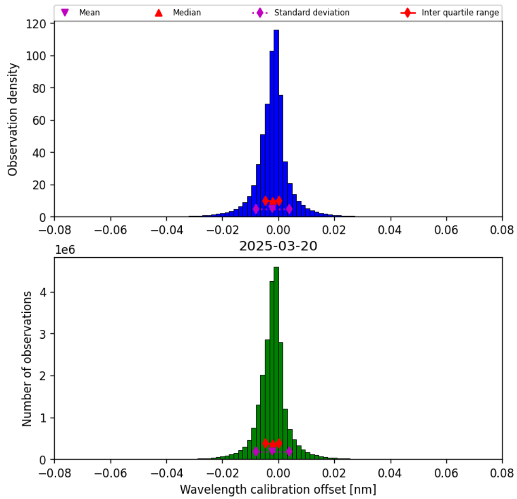
Figure 33: Histogram of “Wavelength calibration offset” for 2025-03-20 to 2025-03-21
