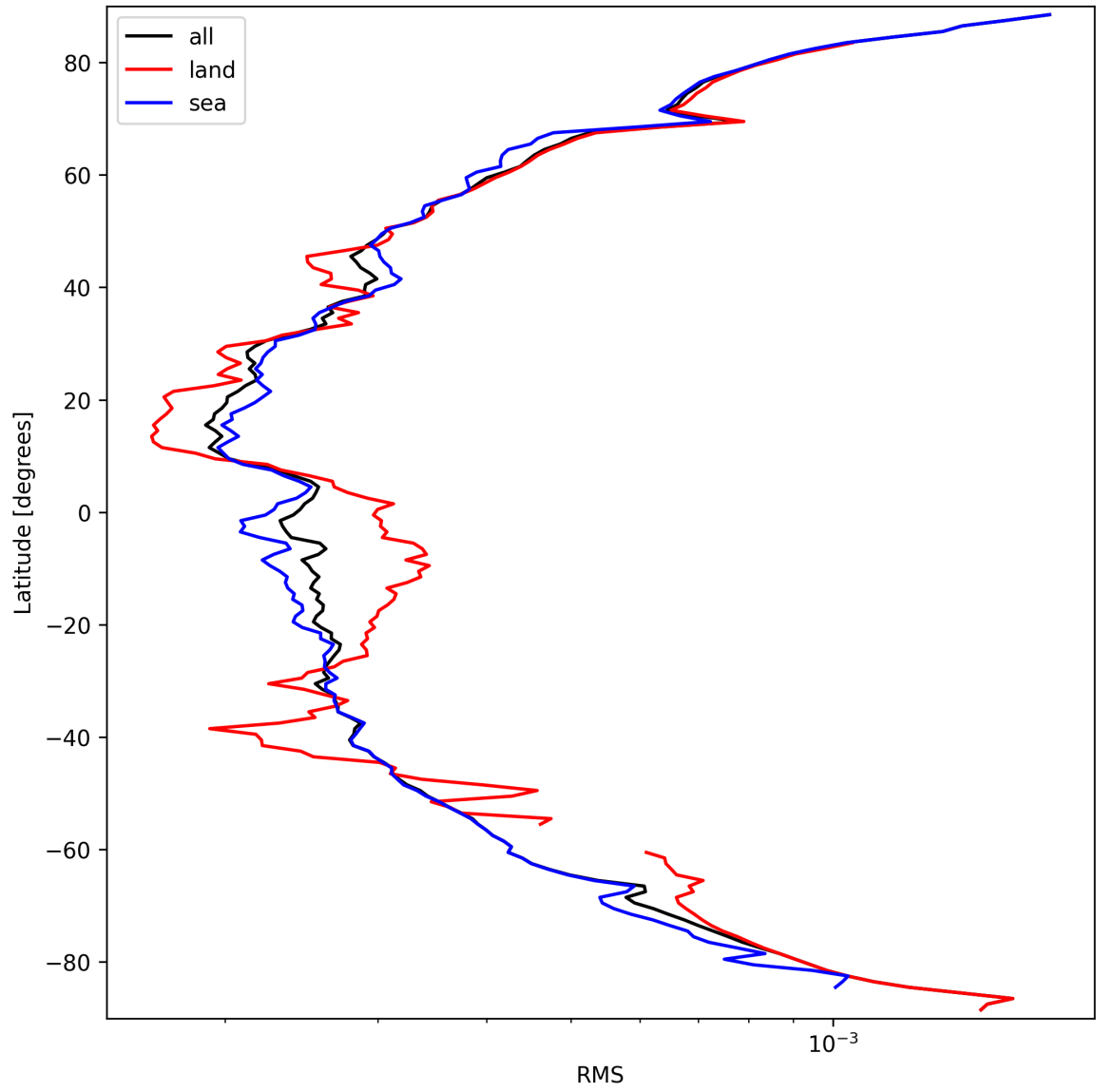
Figure 24: Zonal average of “RMS” for 2025-03-20 to 2025-03-21.
