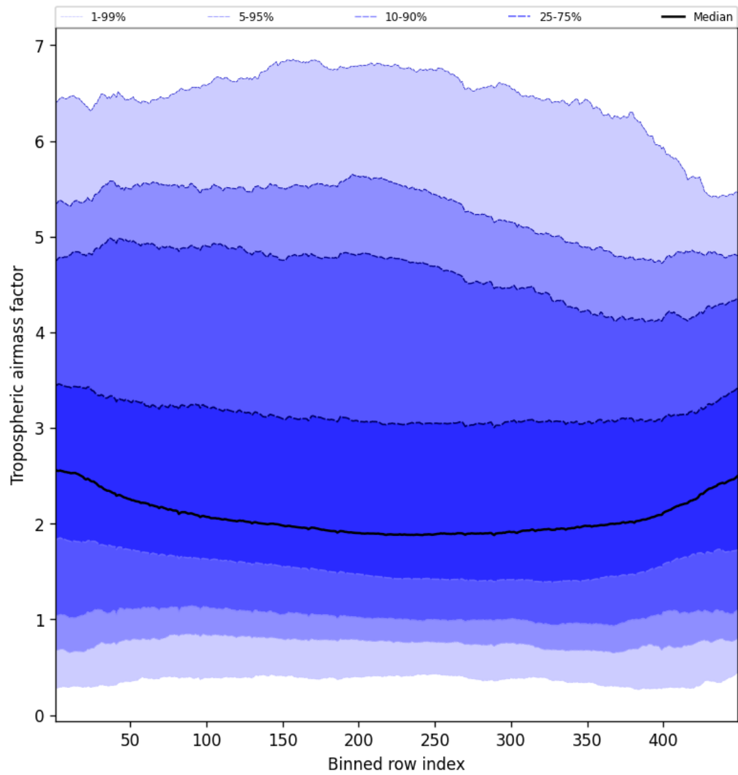
Figure 46: Along track statistics of “Tropospheric airmass factor” for 2025-03-20 to 2025-03-21
