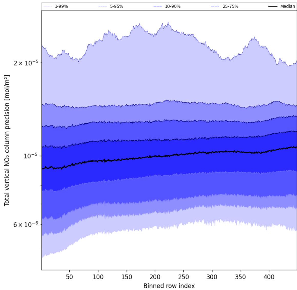
Figure 54: Along track statistics of "Total vertical NO 2 column precision" for 2025-03-20 to 2025-03-21
