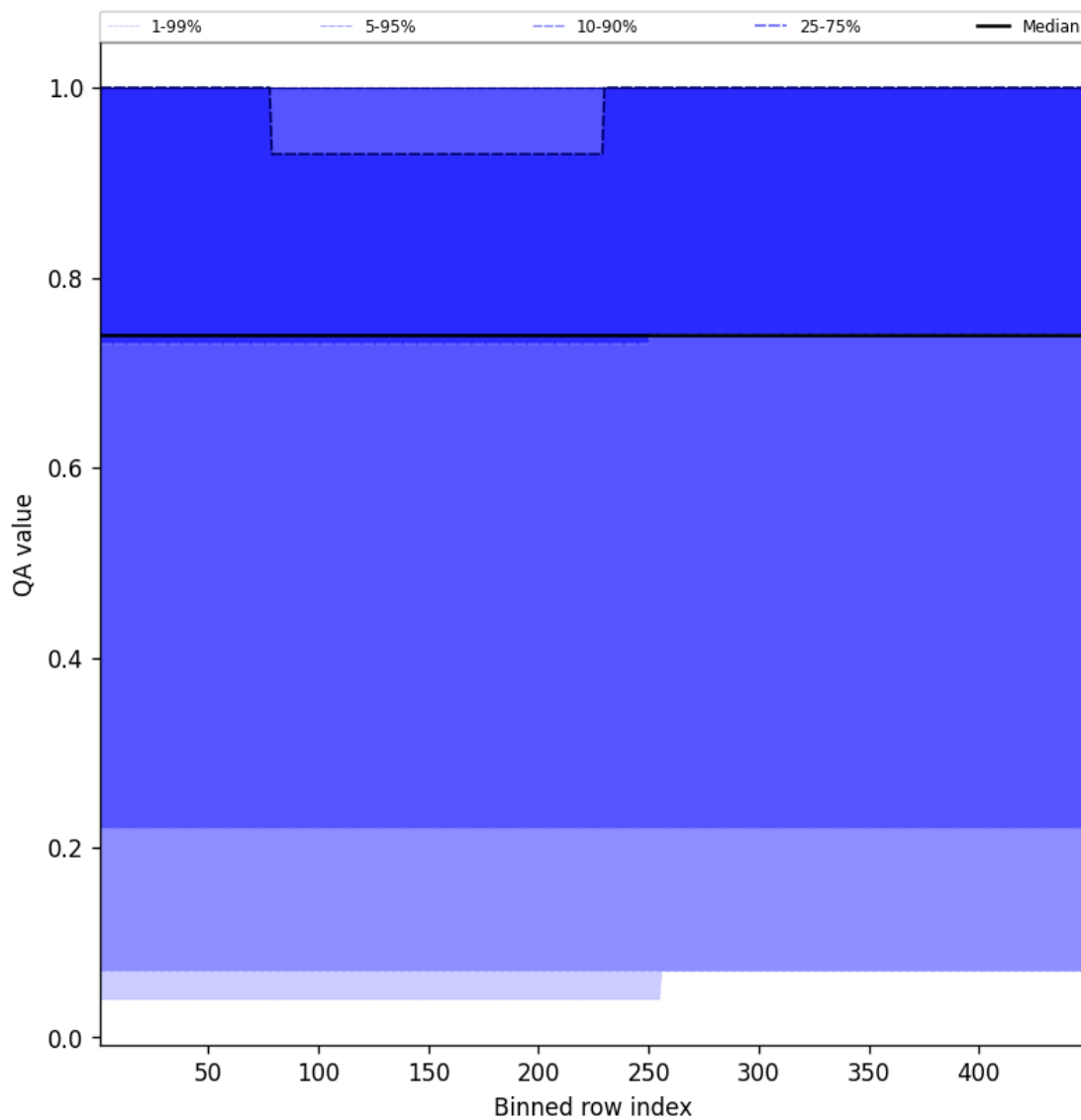
Figure 43: Along track statistics of “QA value” for 2025-03-20 to 2025-03-21
