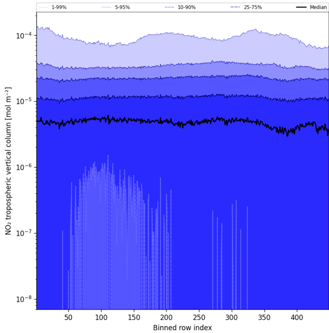
Figure 44: Along track statistics of “NO 2 tropospheric vertical column” for 2025-03-20 to 2025-03-21
