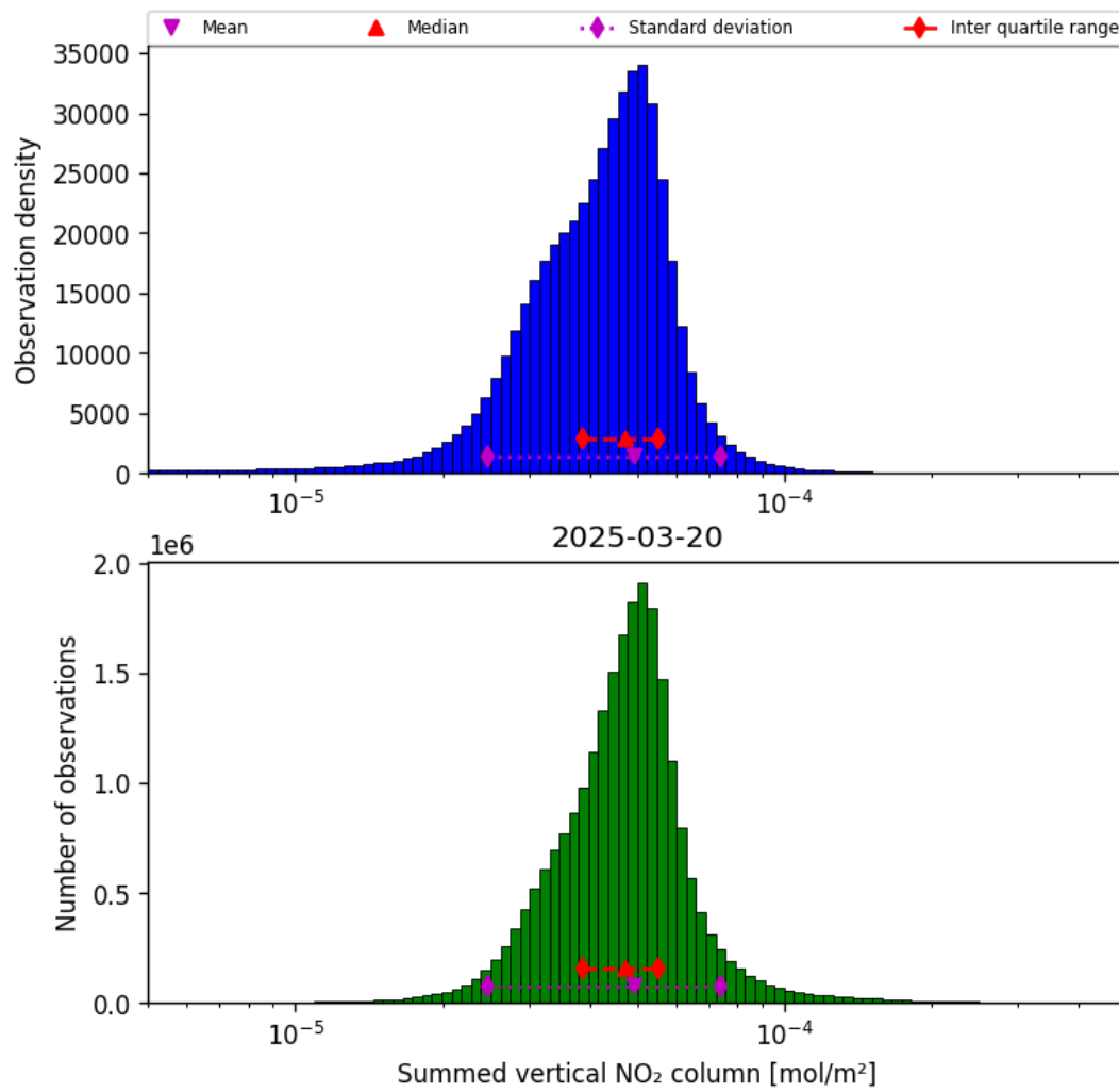
Figure 38: Histogram of “Summed vertical NO 2 column” for 2025-03-20 to 2025-03-21
