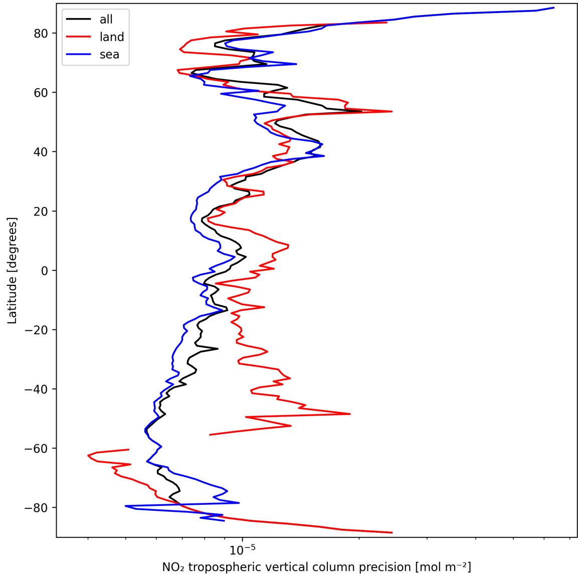
Figure 11: Zonal average of “NO 2 tropospheric vertical column precision” for 2025-03-20 to 2025-03-21.
