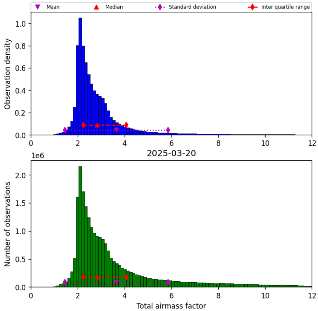
Figure 30: Histogram of “Total airmass factor” for 2025-03-20 to 2025-03-21
