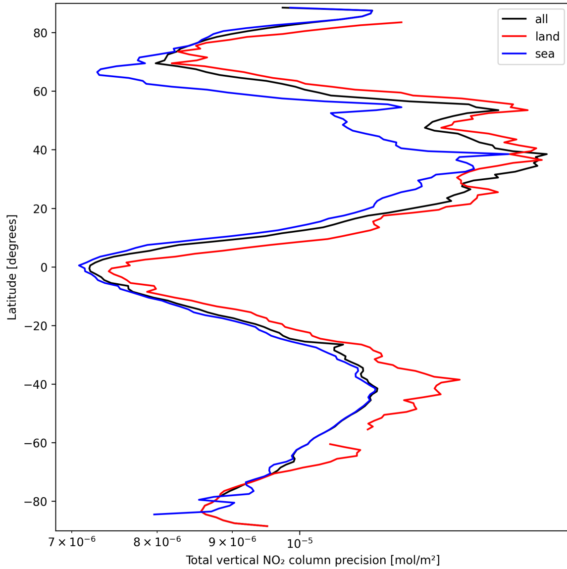
Figure 20: Zonal average of “Total vertical NO 2 column precision” for 2025-03-20 to 2025-03-21.
