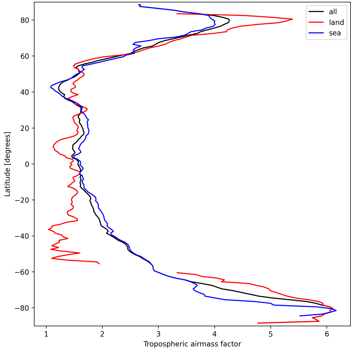
Figure 12: Zonal average of “Tropospheric airmass factor” for 2025-03-20 to 2025-03-21.
