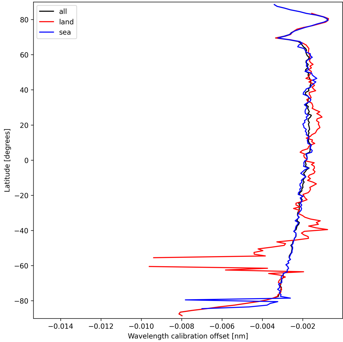
Figure 16: Zonal average of “Wavelength calibration offset” for 2025-03-20 to 2025-03-21.
