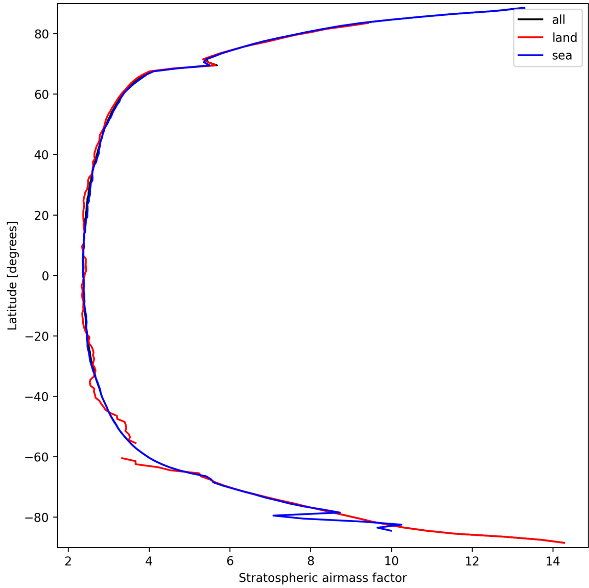
Figure 25: Zonal average of “Stratospheric airmass factor” for 2025-03-20 to 2025-03-21.
