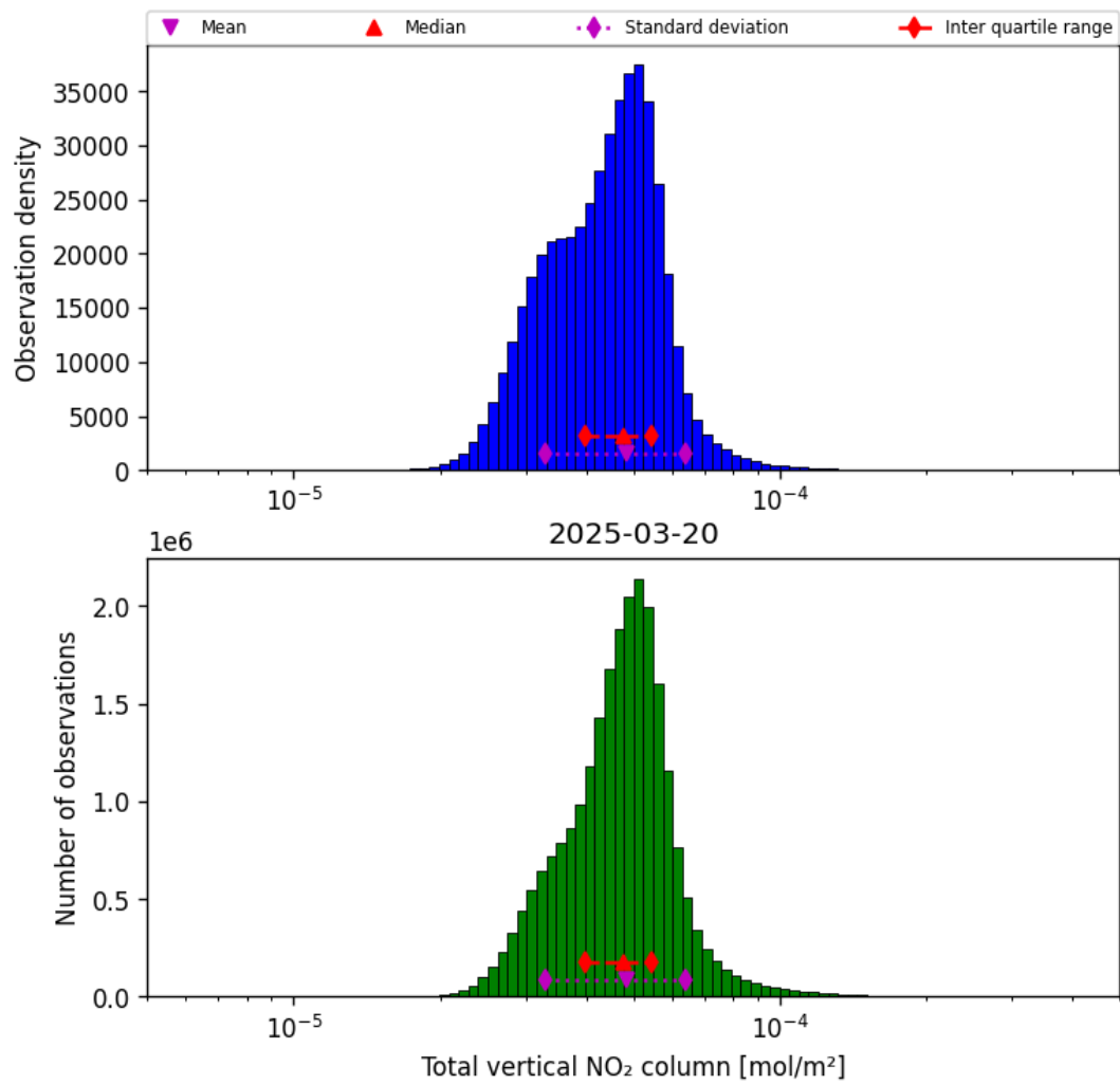
Figure 36: Histogram of “Total vertical NO 2 column” for 2025-03-20 to 2025-03-21
