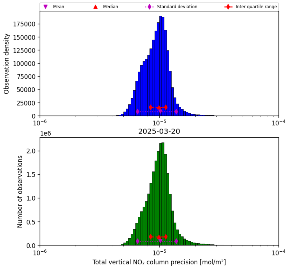
Figure 37: Histogram of "Total vertical NO 2 column precision" for 2025-03-20 to 2025-03-21
