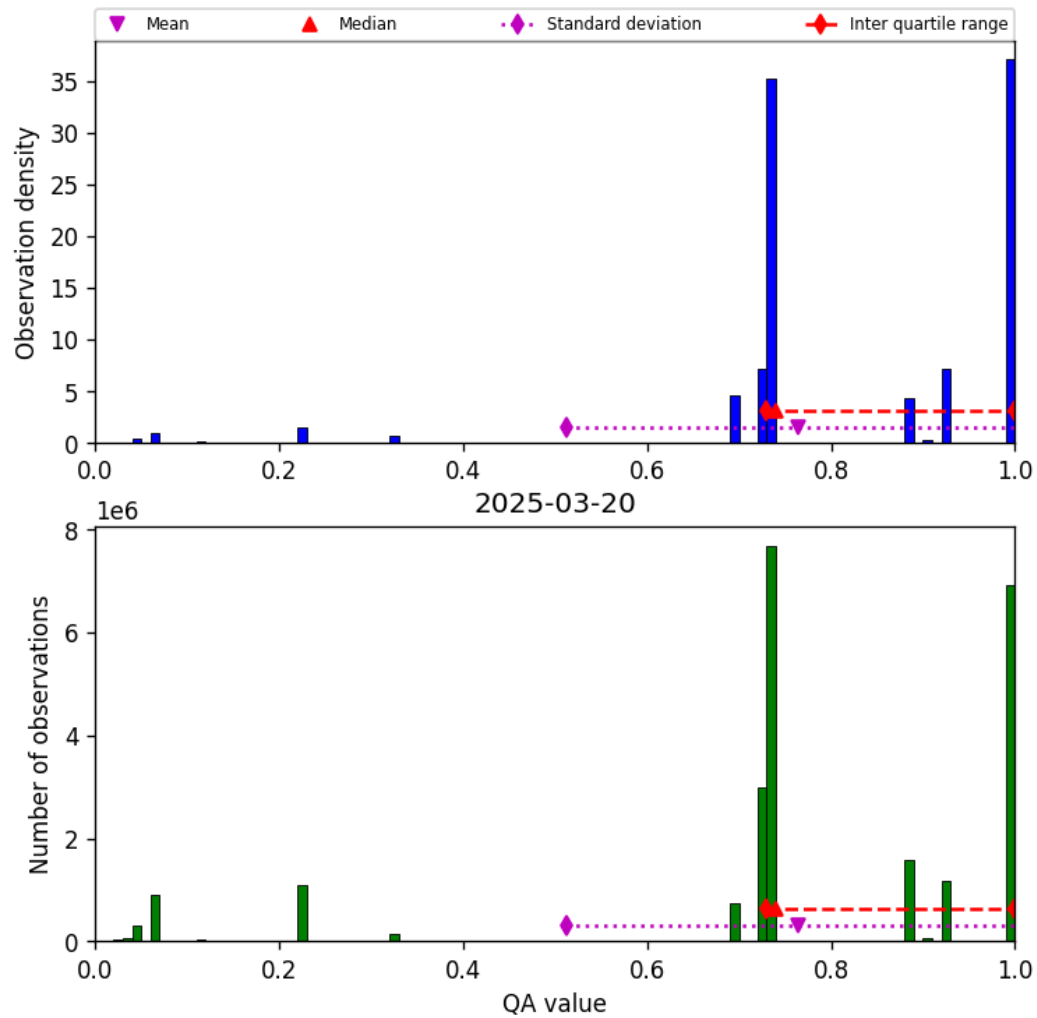
Figure 26: Histogram of “QA value” for 2025-03-20 to 2025-03-21
