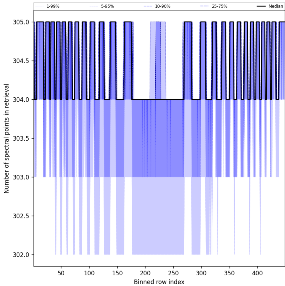
Figure 48: Along track statistics of “Number of spectral points in retrieval” for 2025-03-20 to 2025-03-21
