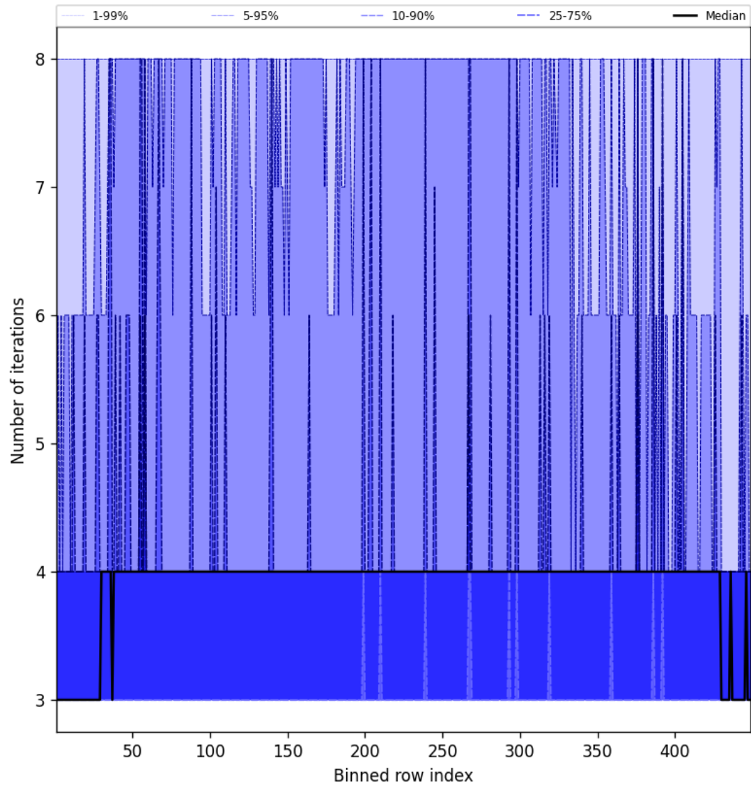
Figure 49: Along track statistics of “Number of iterations” for 2025-03-20 to 2025-03-21
