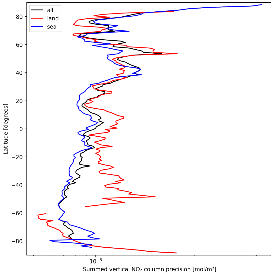
Figure 22: Zonal average of “Summed vertical NO 2 column precision” for 2025-03-20 to 2025-03-21.
