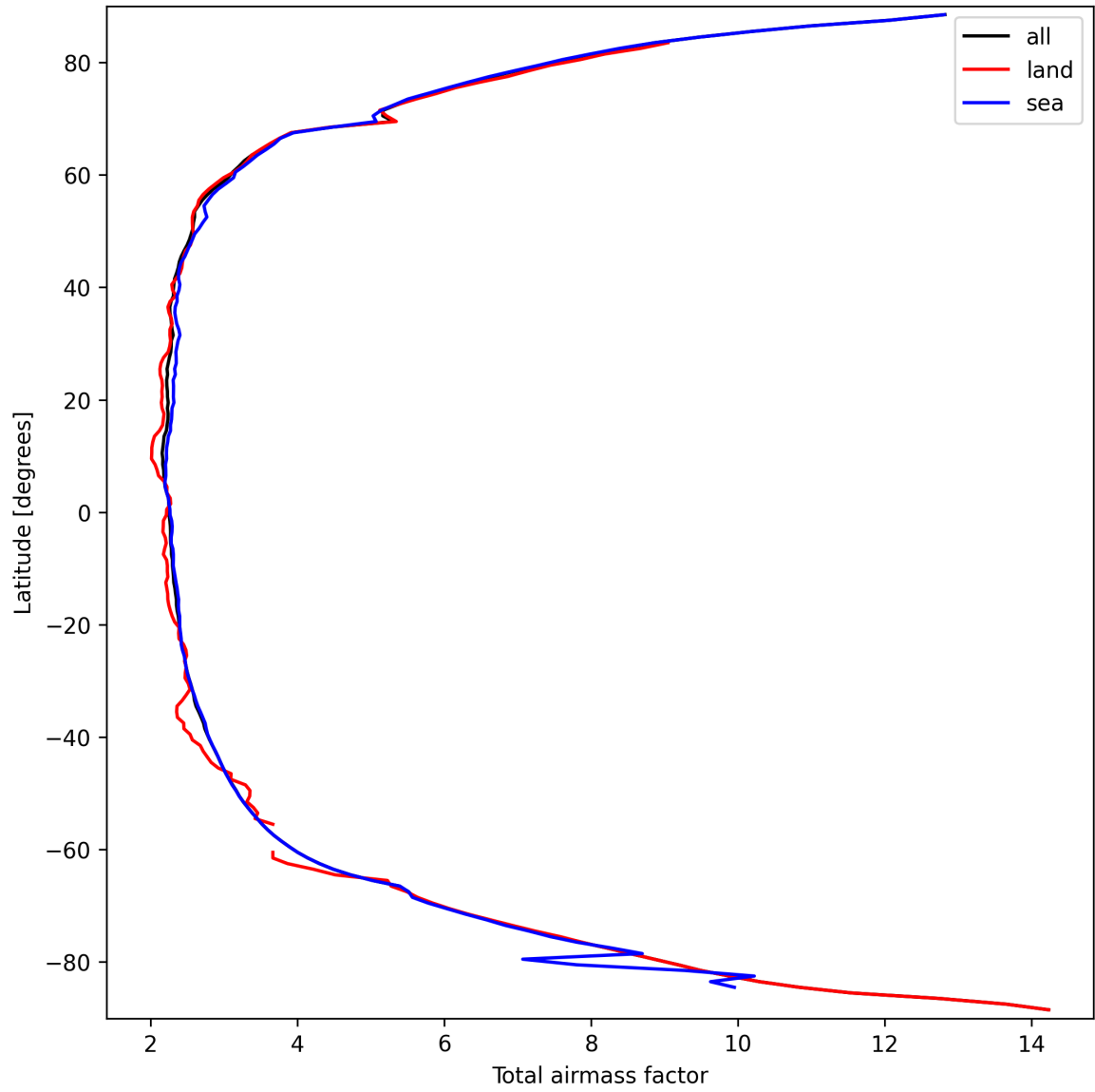
Figure 13: Zonal average of “Total airmass factor” for 2025-03-20 to 2025-03-21.
