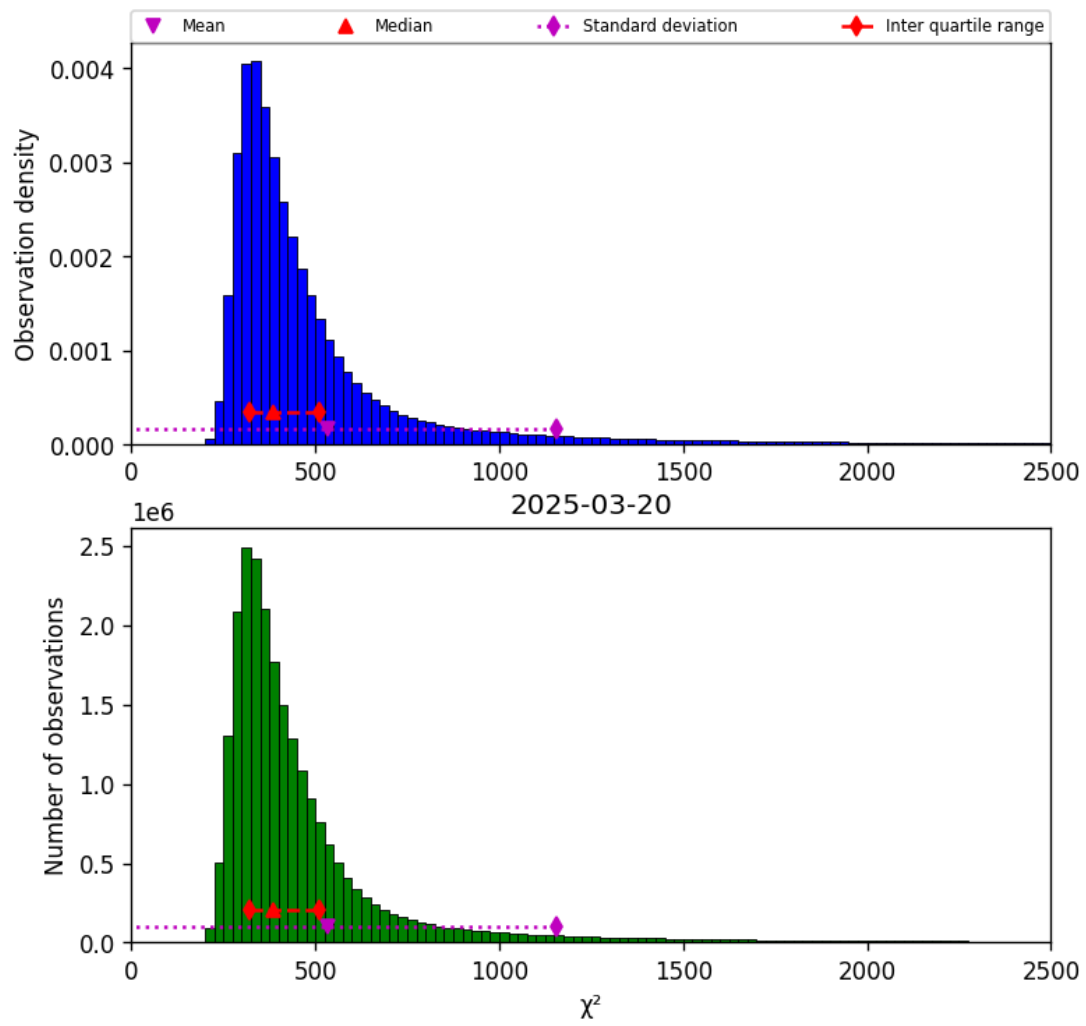
Figure 40: Histogram of “ \chi^2 ” for 2025-03-20 to 2025-03-21
