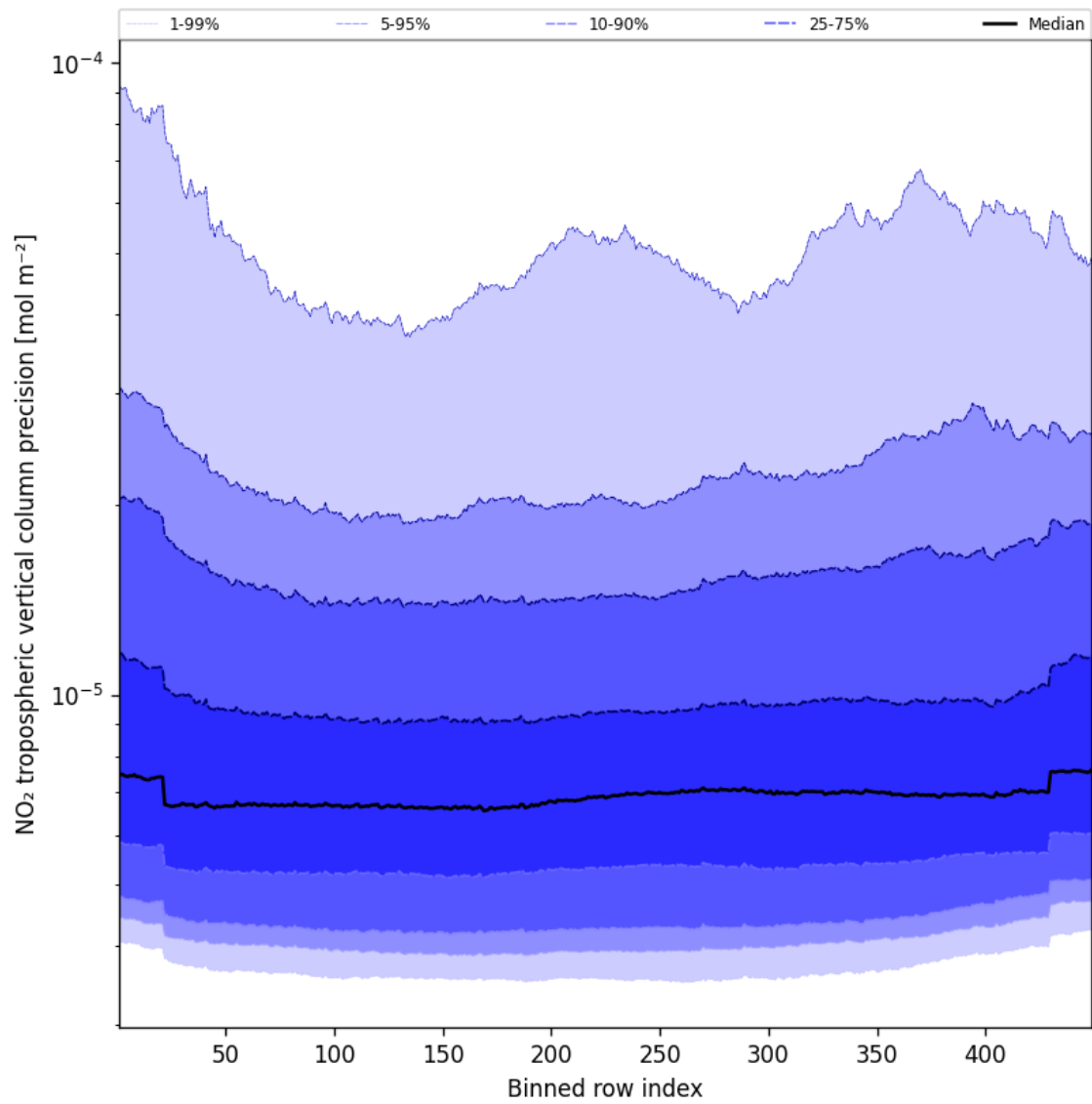
Figure 45: Along track statistics of “NO 2 tropospheric vertical column precision” for 2025-03-20 to 2025-03-21
