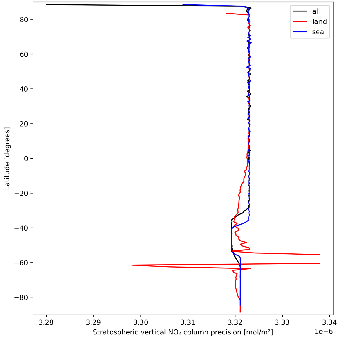
Figure 18: Zonal average of "Stratospheric vertical NO 2 column precision" for 2025-03-20 to 2025-03-21.
