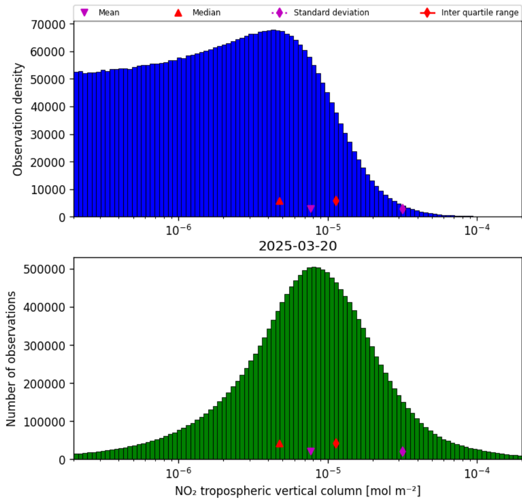
Figure 27: Histogram of “NO 2 tropospheric vertical column” for 2025-03-20 to 2025-03-21
