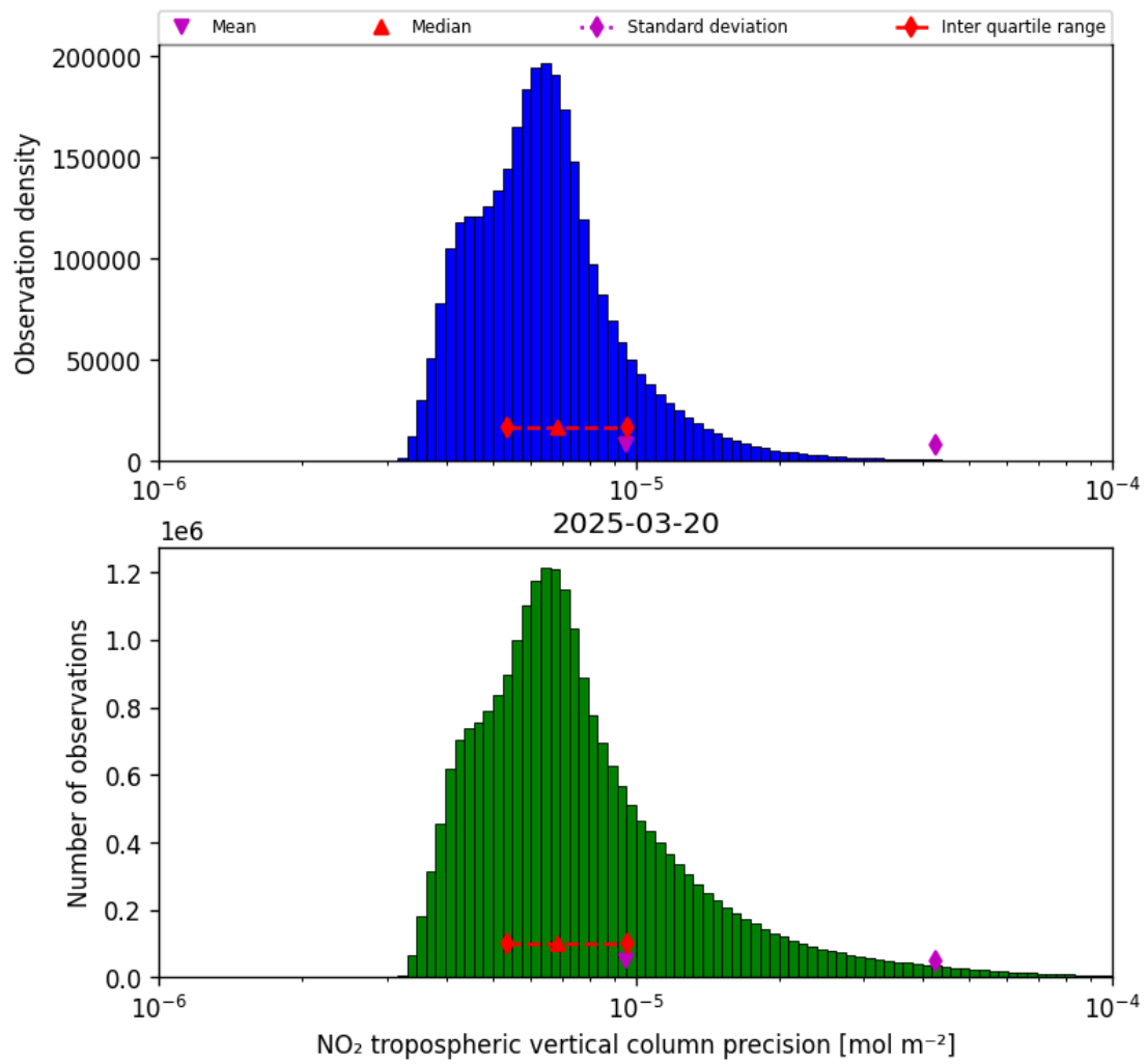
Figure 28: Histogram of “NO 2 tropospheric vertical column precision” for 2025-03-20 to 2025-03-21
