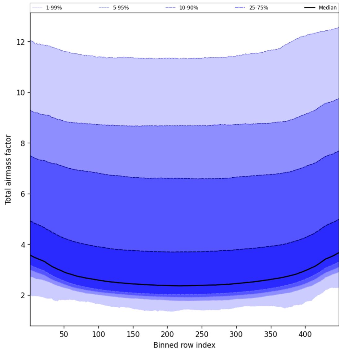
Figure 47: Along track statistics of “Total airmass factor” for 2025-03-20 to 2025-03-21
