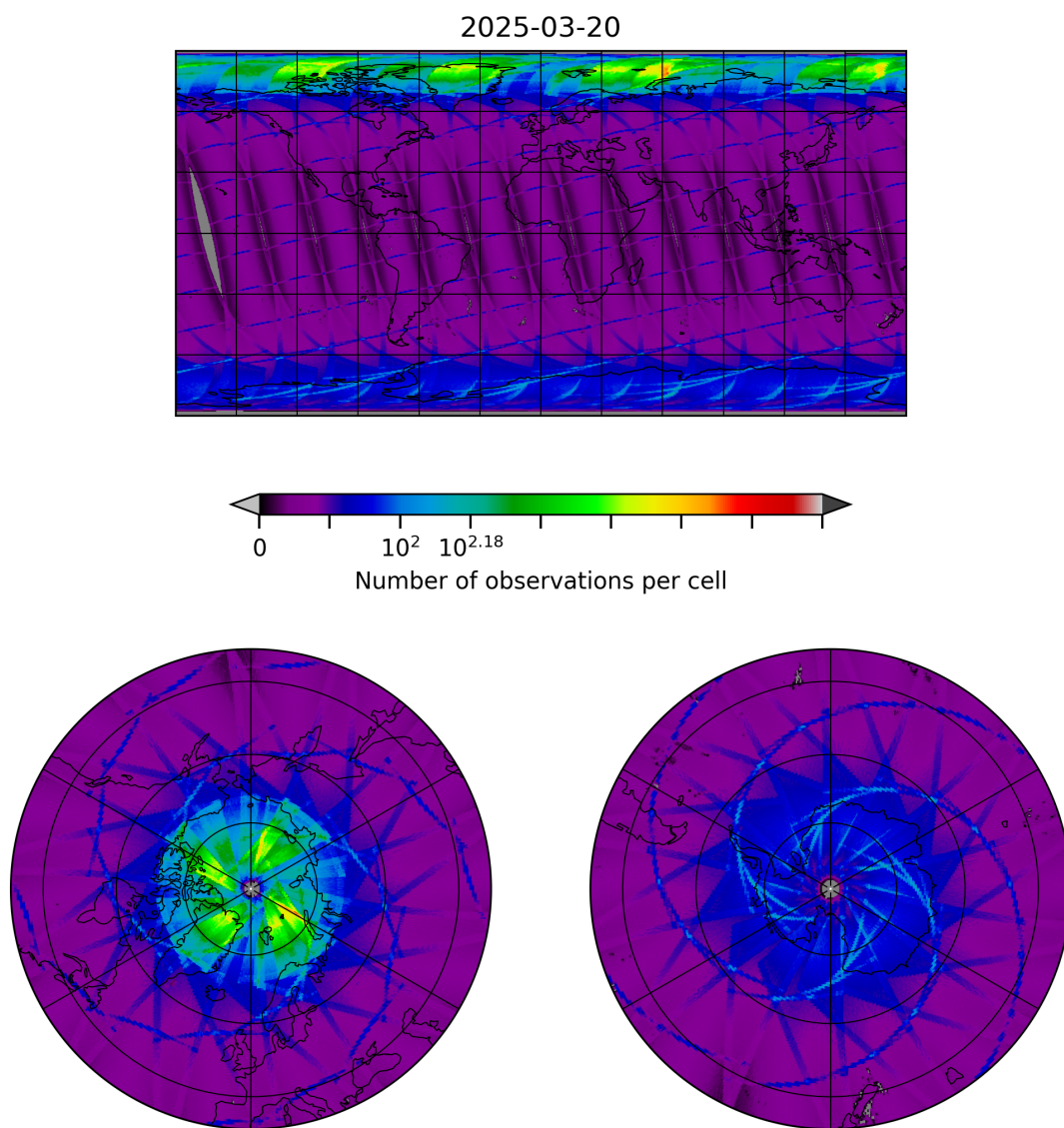
Figure 8: Map of the number of observations for 2025-03-20 to 2025-03-21
