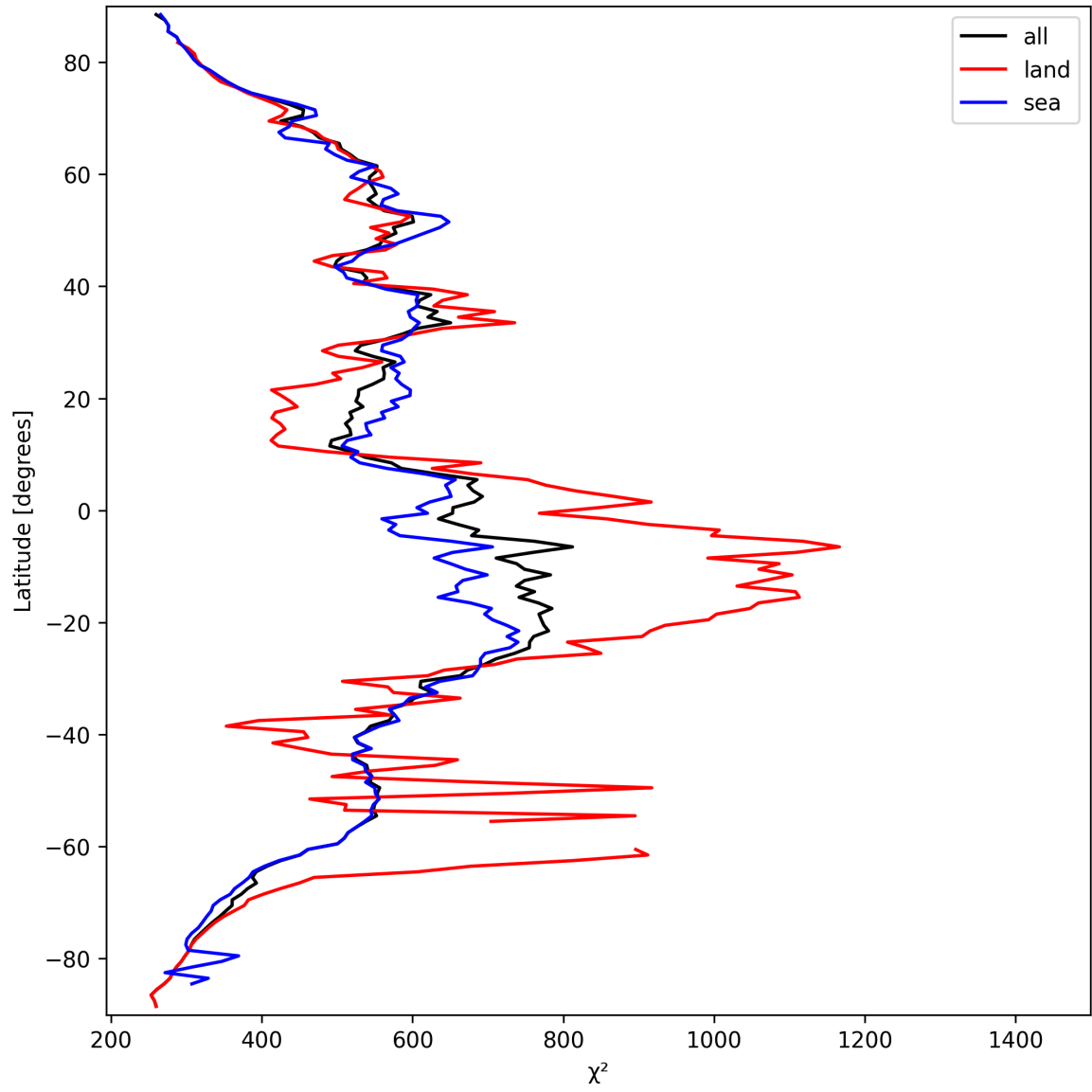
Figure 23: Zonal average of “ \chi^2 ” for 2025-03-20 to 2025-03-21.
