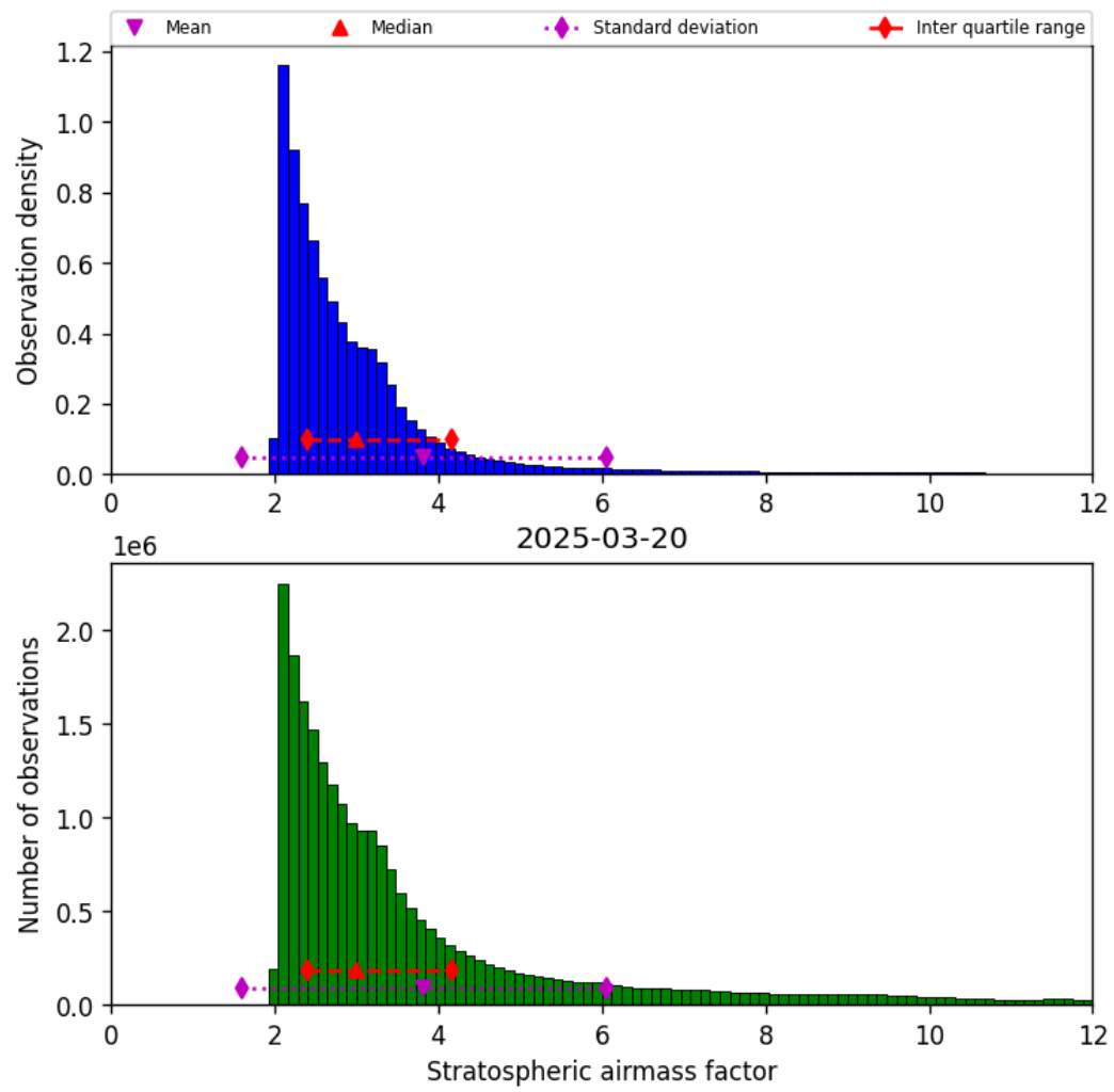
Figure 42: Histogram of “Stratospheric airmass factor” for 2025-03-20 to 2025-03-21
