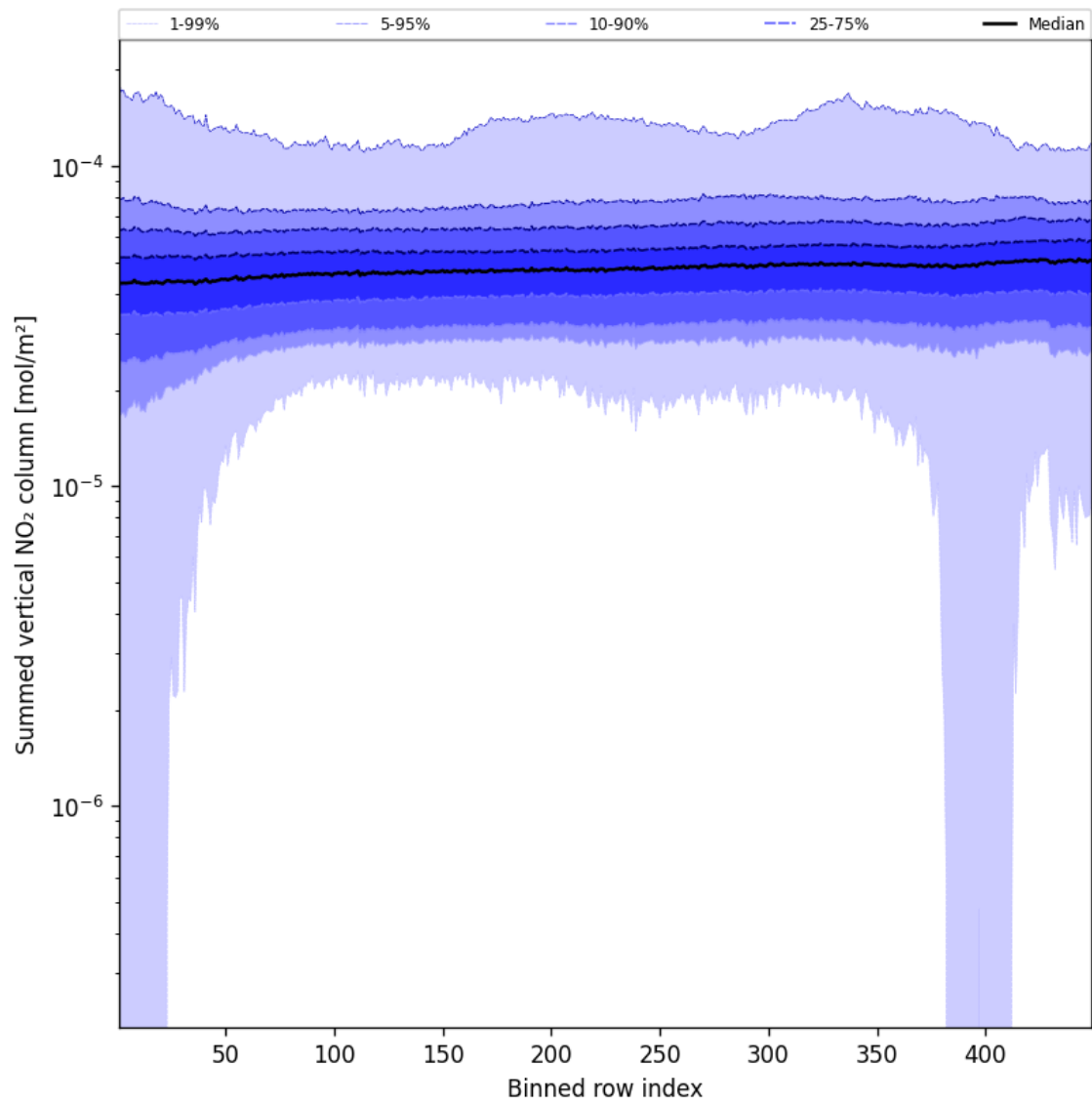
Figure 55: Along track statistics of “Summed vertical NO 2 column” for 2025-03-20 to 2025-03-21
