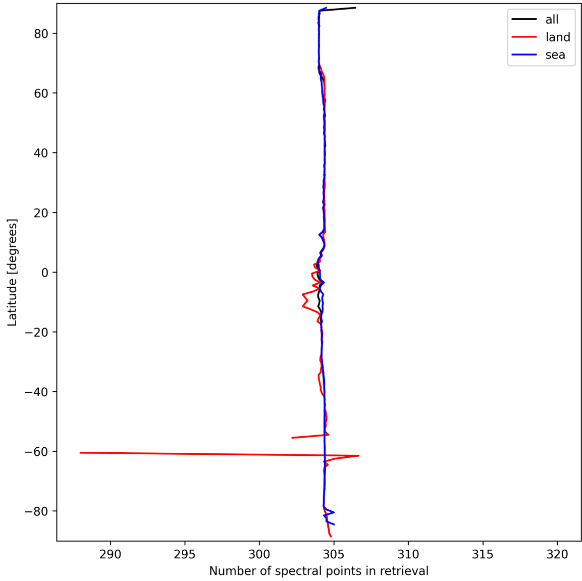
Figure 14: Zonal average of “Number of spectral points in retrieval” for 2025-03-20 to 2025-03-21.
