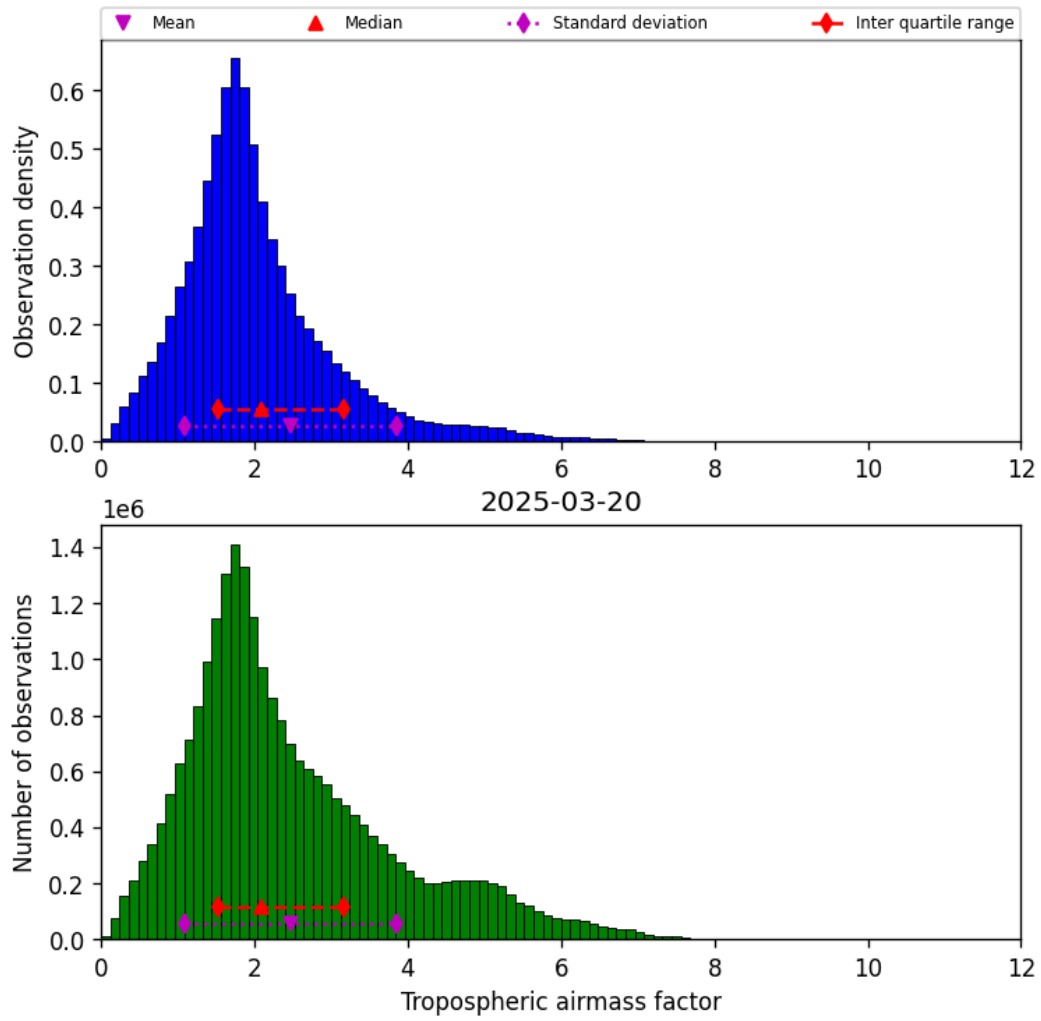
Figure 29: Histogram of “Tropospheric airmass factor” for 2025-03-20 to 2025-03-21
