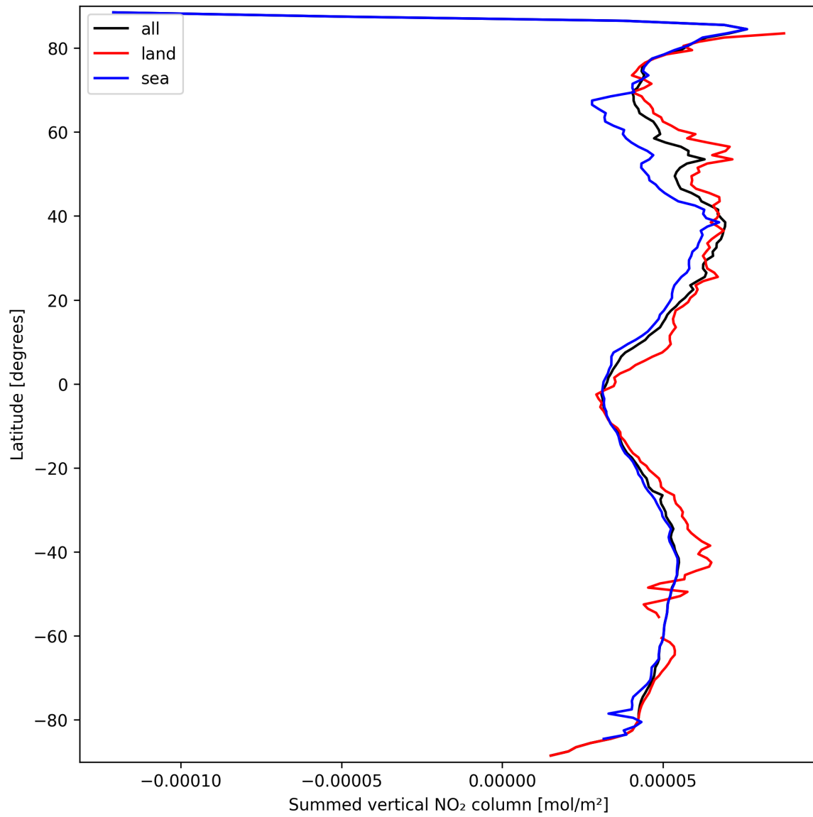
Figure 21: Zonal average of “Summed vertical NO 2 column” for 2025-03-20 to 2025-03-21.
