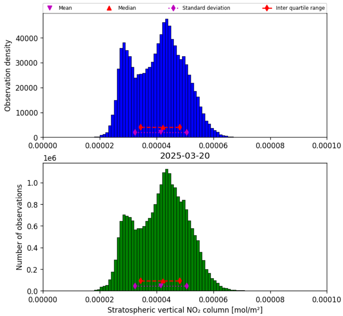
Figure 34: Histogram of “Stratospheric vertical NO 2 column” for 2025-03-20 to 2025-03-21
