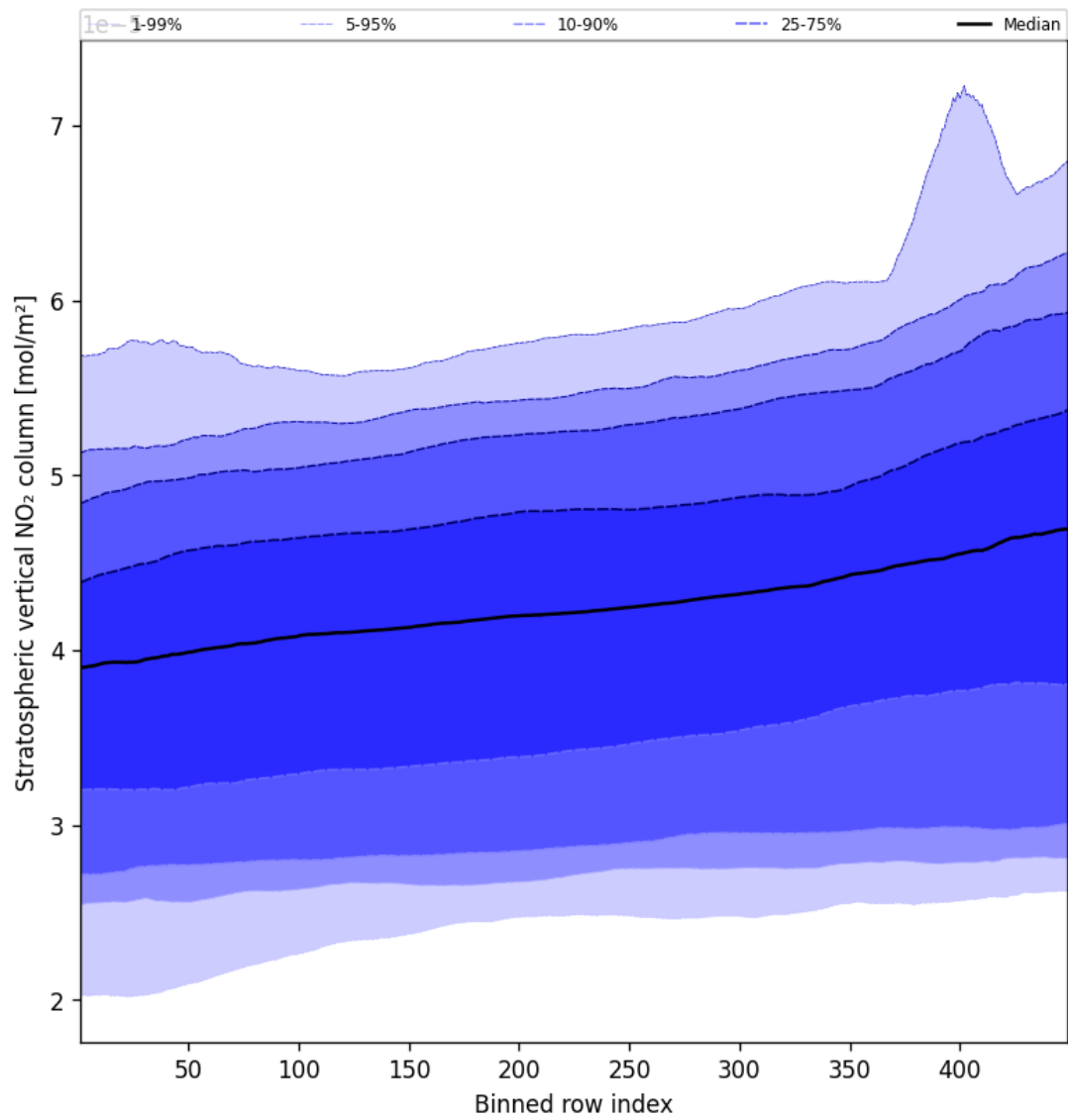
Figure 51: Along track statistics of “Stratospheric vertical NO 2 column” for 2025-03-20 to 2025-03-21
