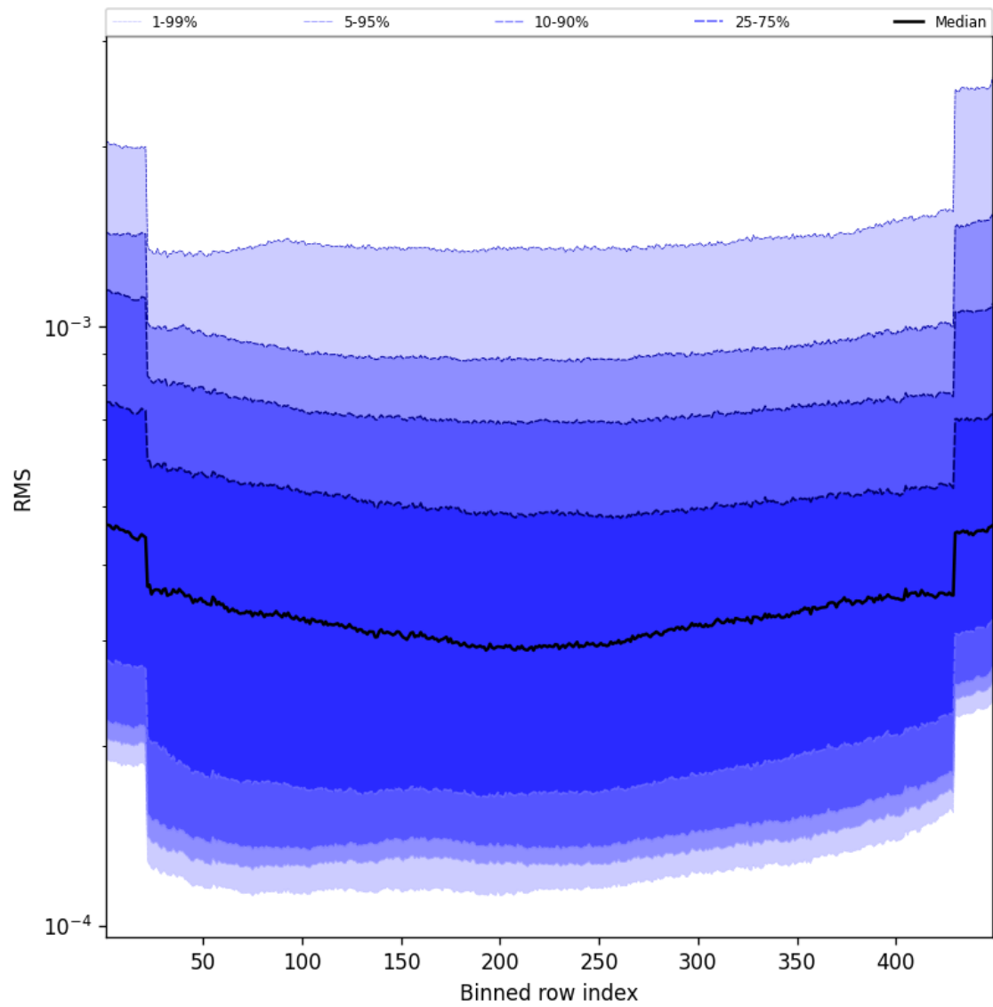
Figure 58: Along track statistics of “RMS” for 2025-03-20 to 2025-03-21
