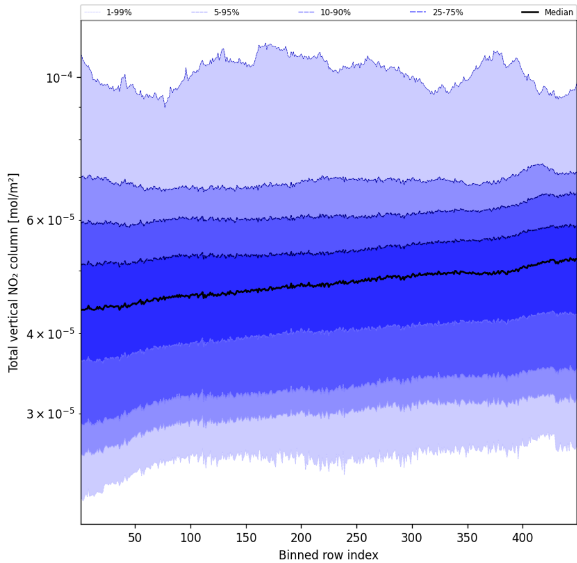
Figure 53: Along track statistics of “Total vertical NO 2 column” for 2025-03-20 to 2025-03-21
