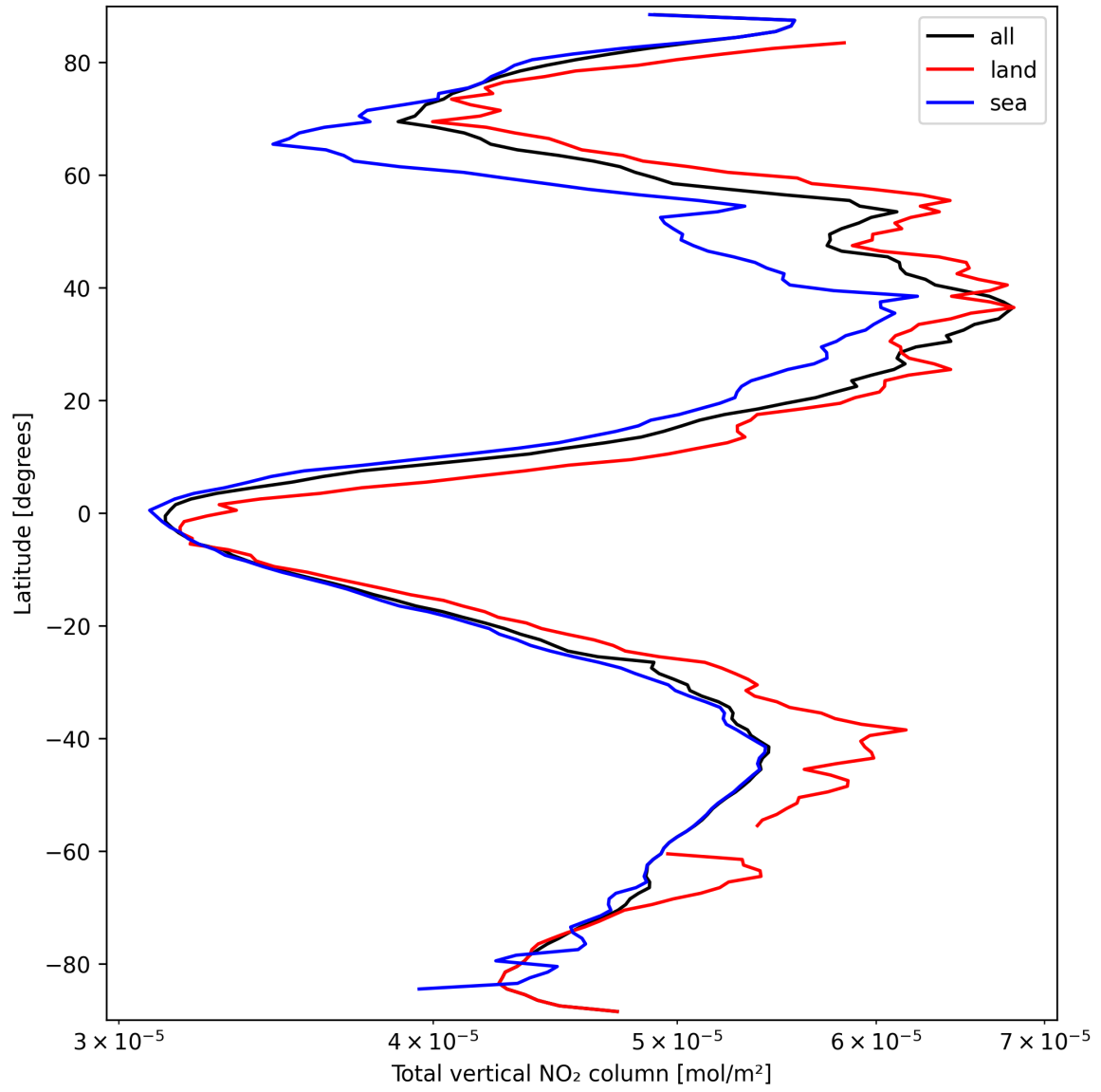
Figure 19: Zonal average of “Total vertical NO 2 column” for 2025-03-20 to 2025-03-21.
