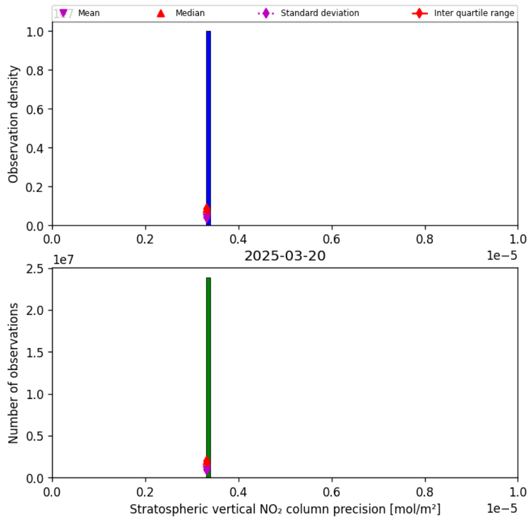
Figure 35: Histogram of “Stratospheric vertical NO 2 column precision” for 2025-03-20 to 2025-03-21
