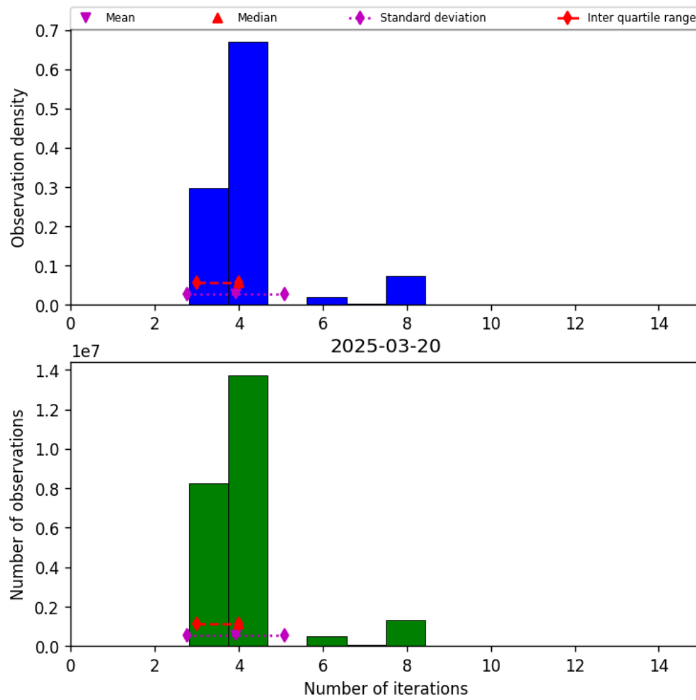
Figure 32: Histogram of “Number of iterations” for 2025-03-20 to 2025-03-21
