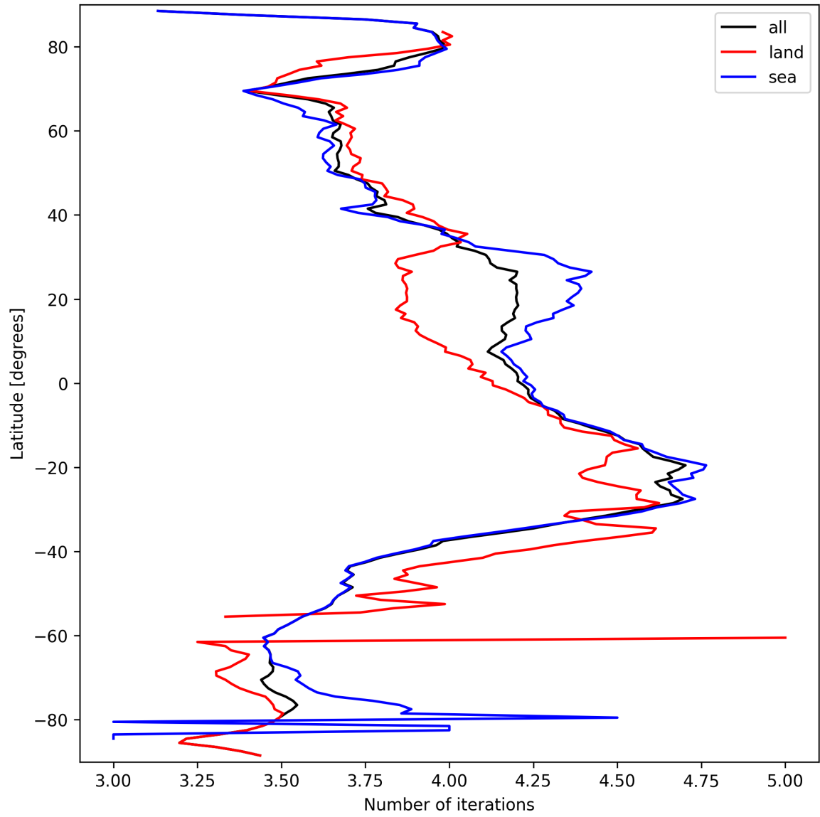
Figure 15: Zonal average of “Number of iterations” for 2025-03-20 to 2025-03-21.
