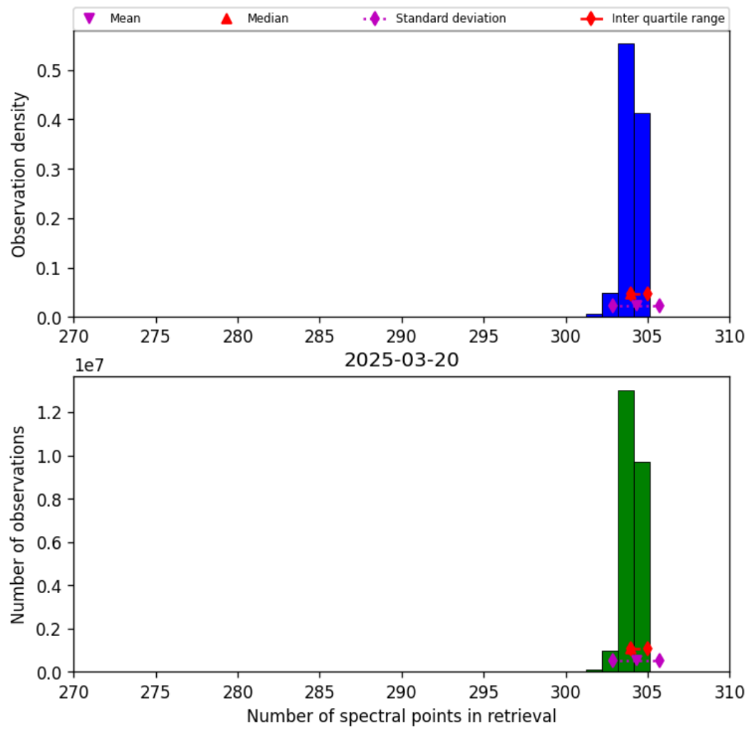
Figure 31: Histogram of “Number of spectral points in retrieval” for 2025-03-20 to 2025-03-21
