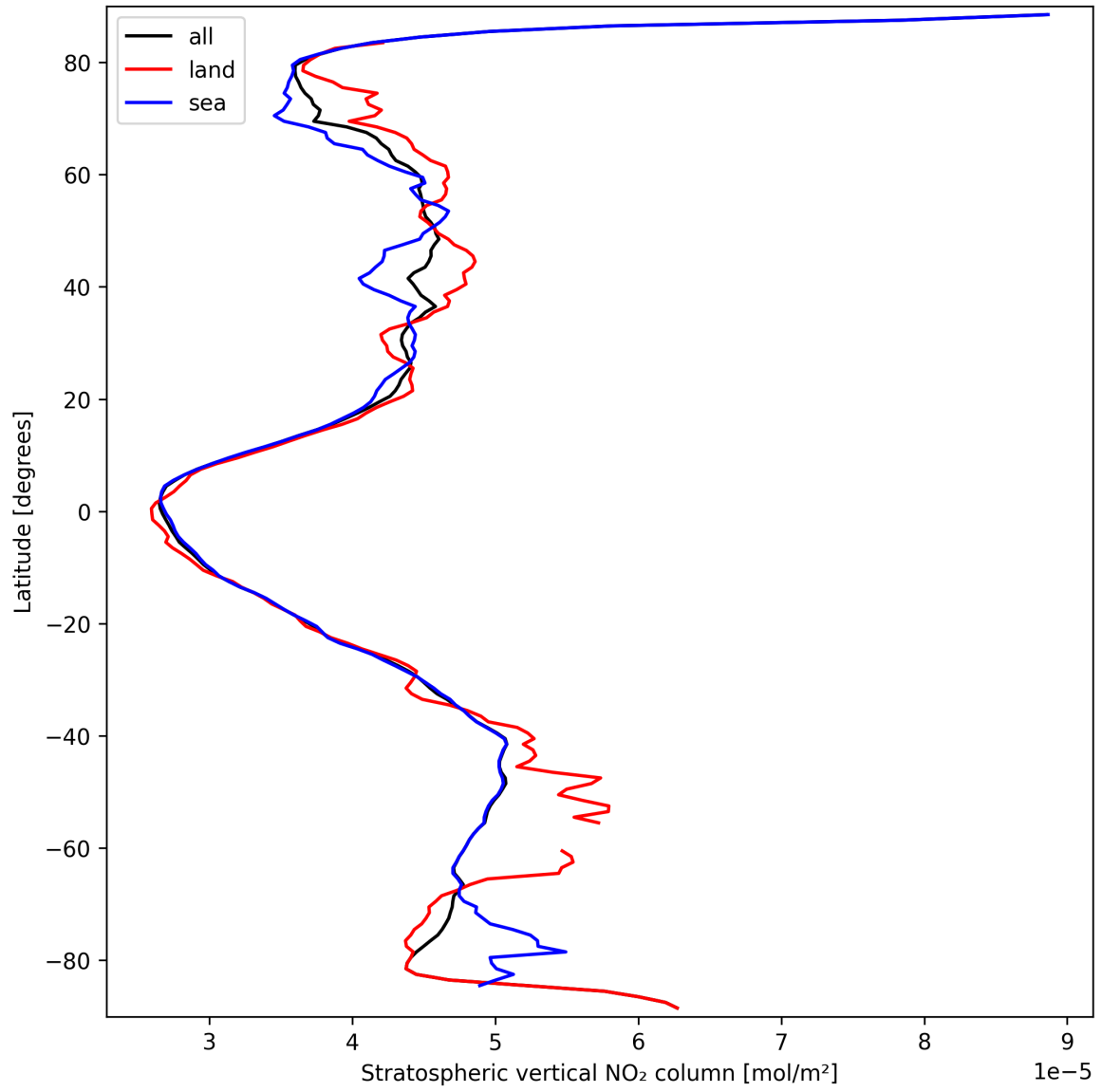
Figure 17: Zonal average of “Stratospheric vertical NO 2 column” for 2025-03-20 to 2025-03-21.
