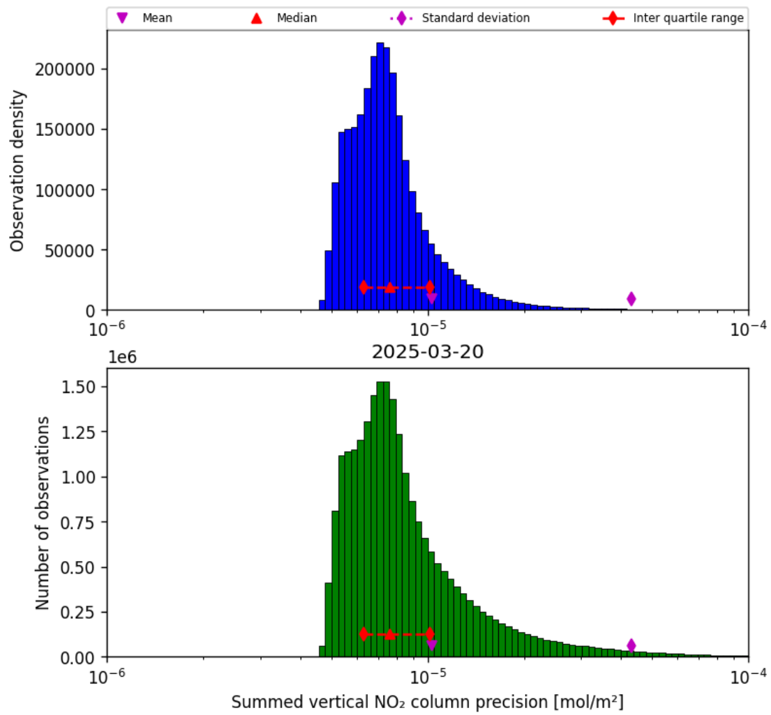
Figure 39: Histogram of “Summed vertical NO 2 column precision” for 2025-03-20 to 2025-03-21
