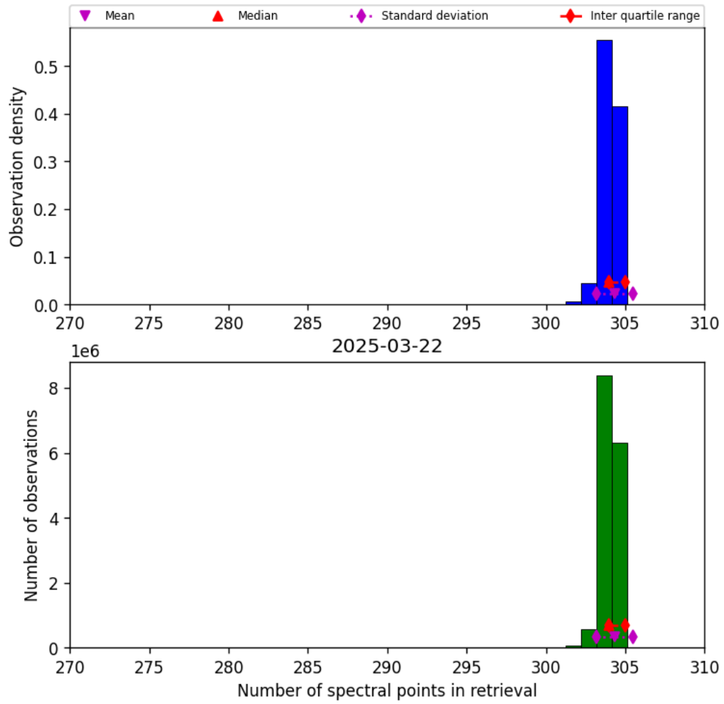
Figure 31: Histogram of “Number of spectral points in retrieval” for 2025-03-22 to 2025-03-22
