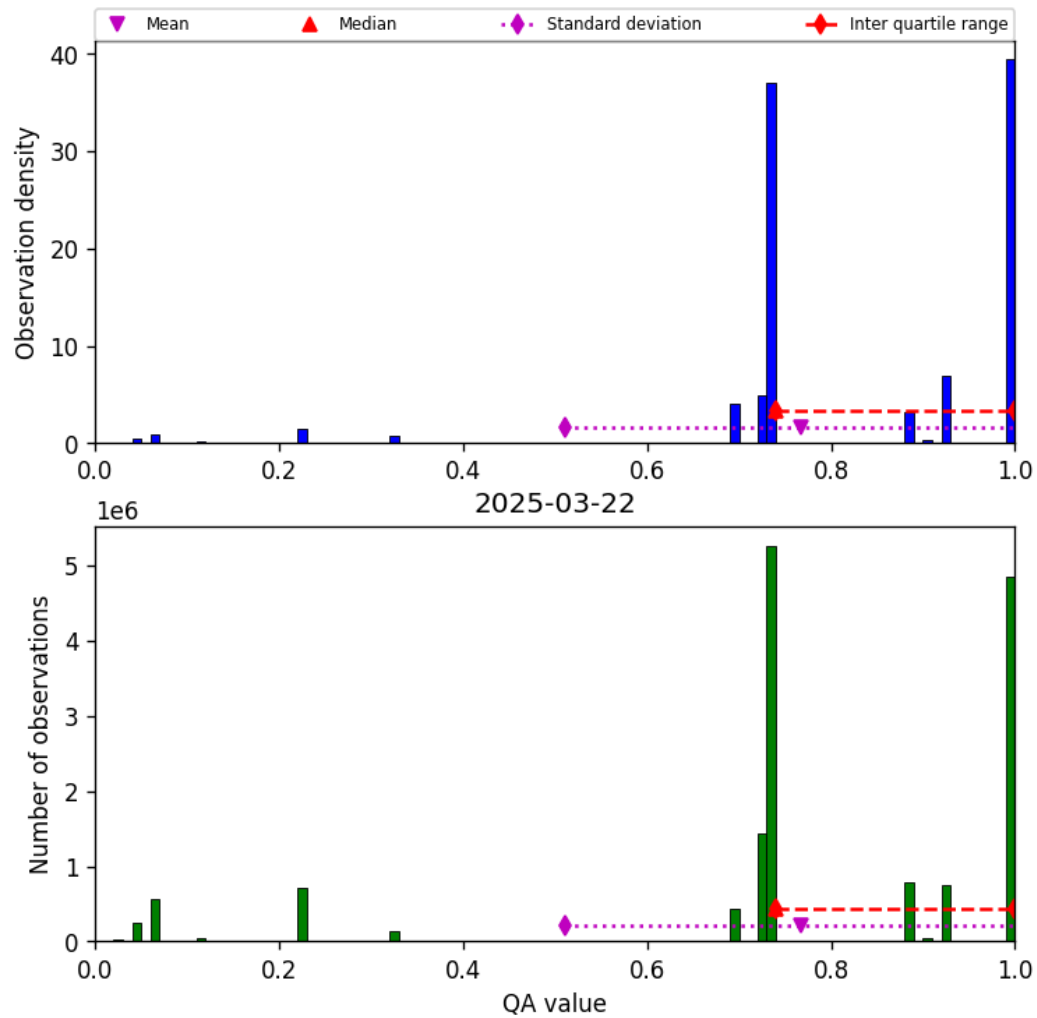
Figure 26: Histogram of “QA value” for 2025-03-22 to 2025-03-22
