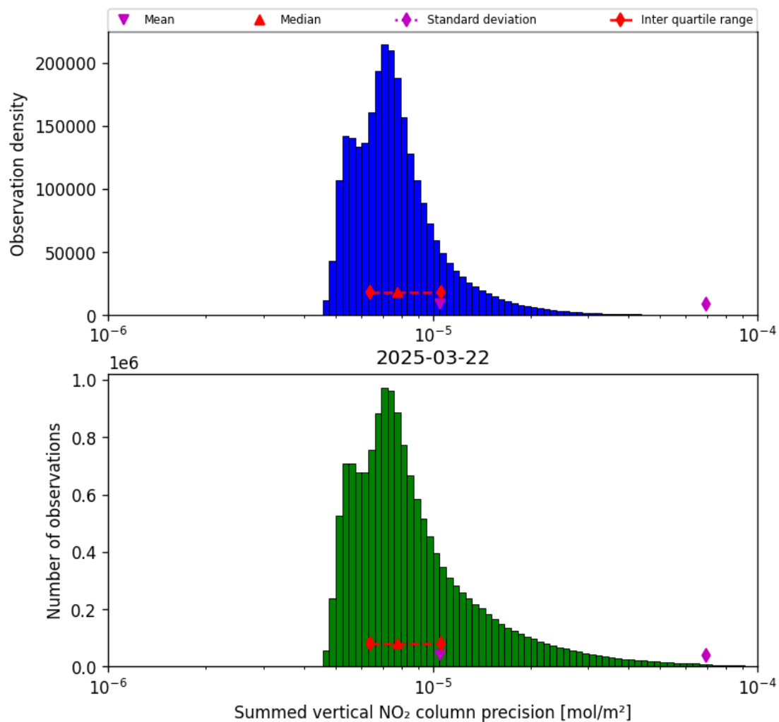
Figure 39: Histogram of "Summed vertical NO 2 column precision" for 2025-03-22 to 2025-03-22
