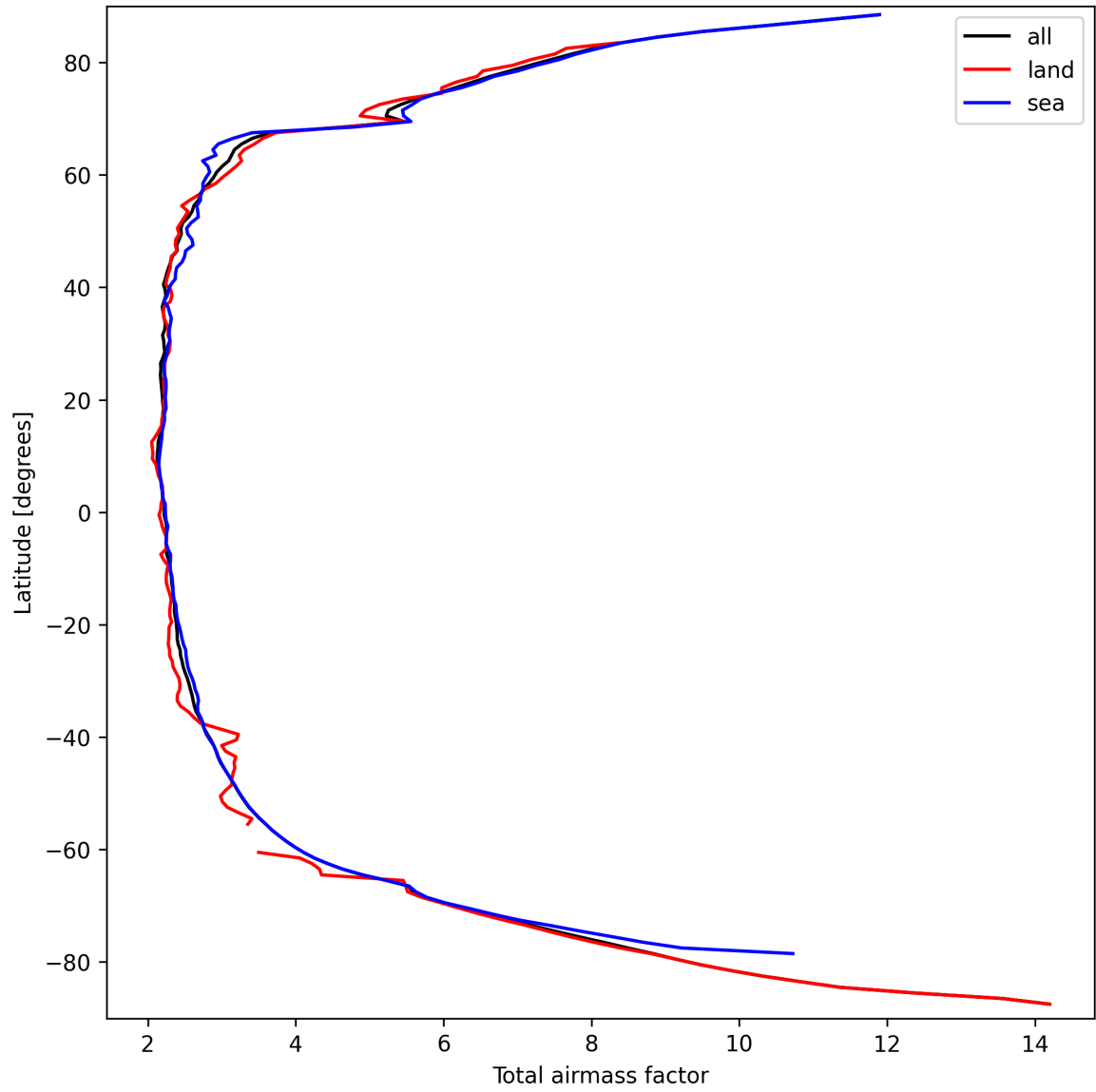
Figure 13: Zonal average of “Total airmass factor” for 2025-03-22 to 2025-03-22.
