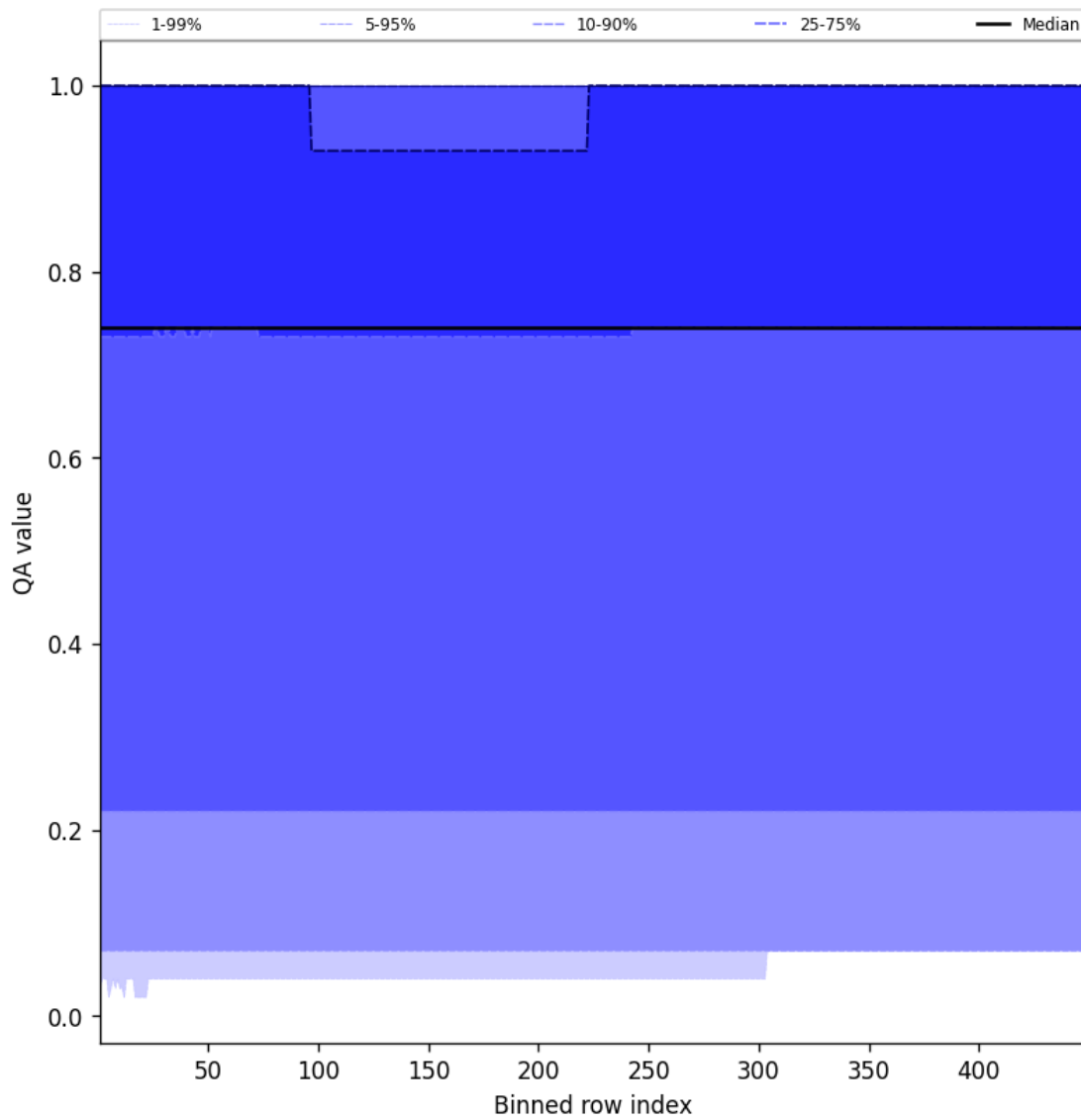
Figure 43: Along track statistics of “QA value” for 2025-03-22 to 2025-03-22
