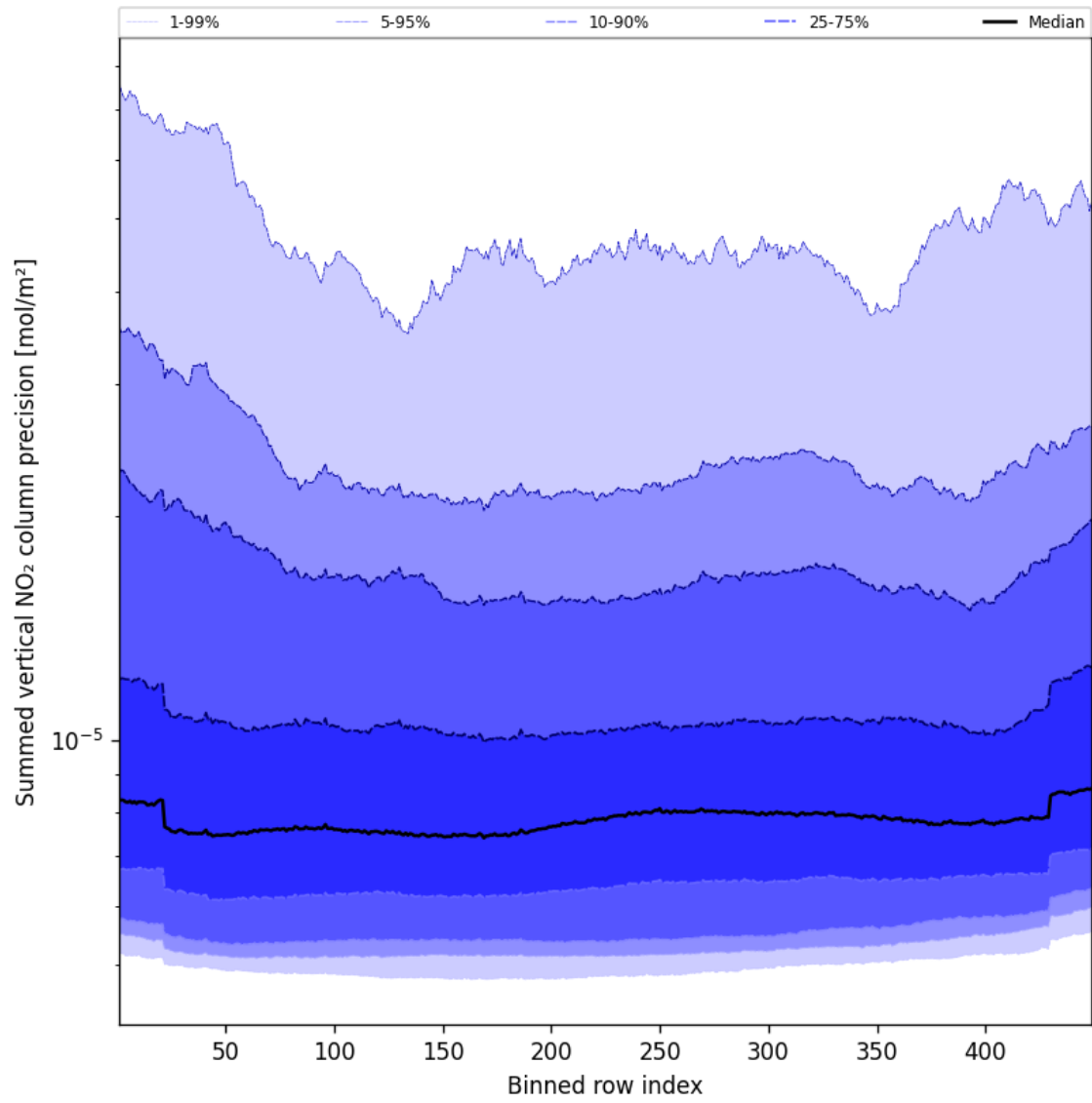
Figure 56: Along track statistics of “Summed vertical NO 2 column precision” for 2025-03-22 to 2025-03-22
