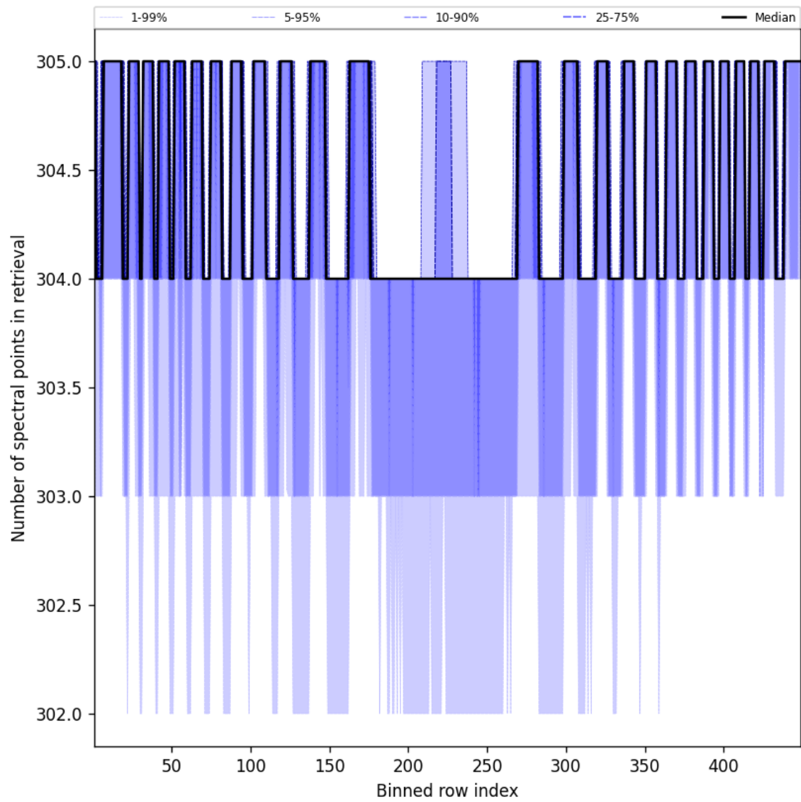
Figure 48: Along track statistics of “Number of spectral points in retrieval” for 2025-03-22 to 2025-03-22
