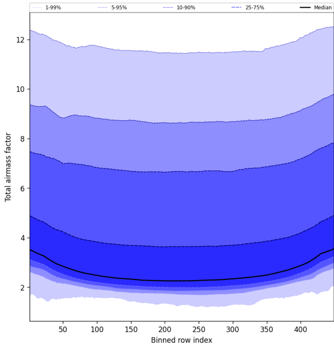
Figure 47: Along track statistics of “Total airmass factor” for 2025-03-22 to 2025-03-22
