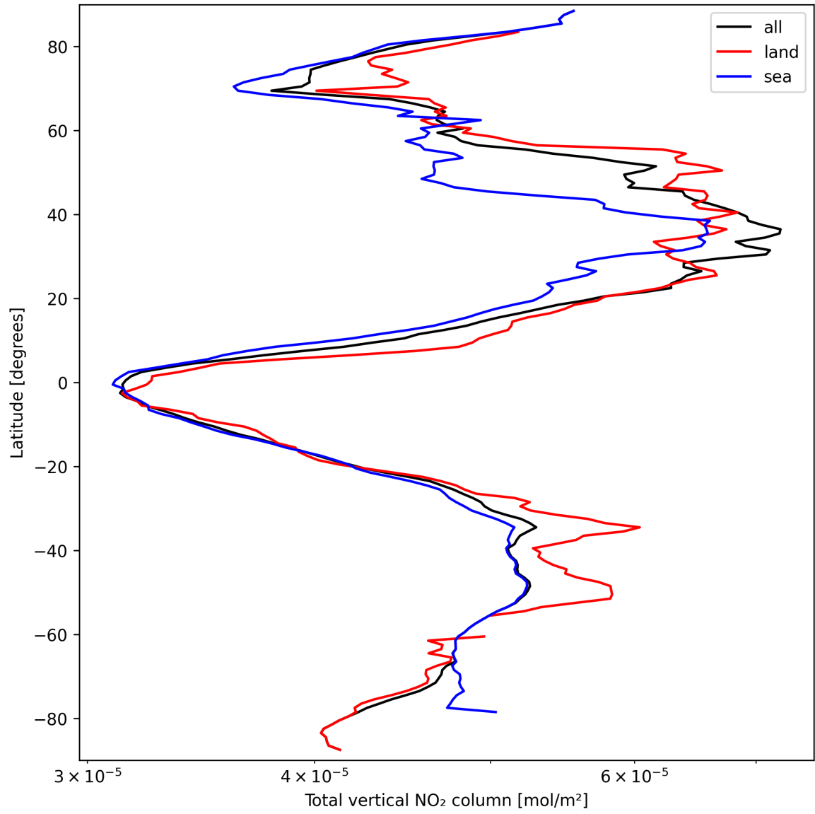
Figure 19: Zonal average of “Total vertical NO 2 column” for 2025-03-22 to 2025-03-22.
