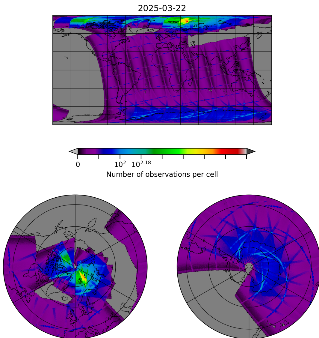
Figure 8: Map of the number of observations for 2025-03-22 to 2025-03-22
