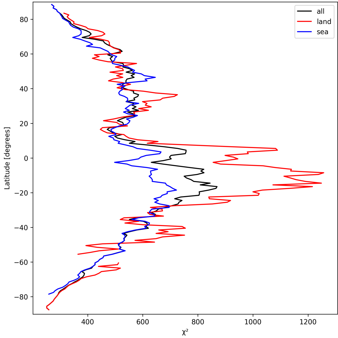
Figure 23: Zonal average of “ \chi^2 ” for 2025-03-22 to 2025-03-22.
