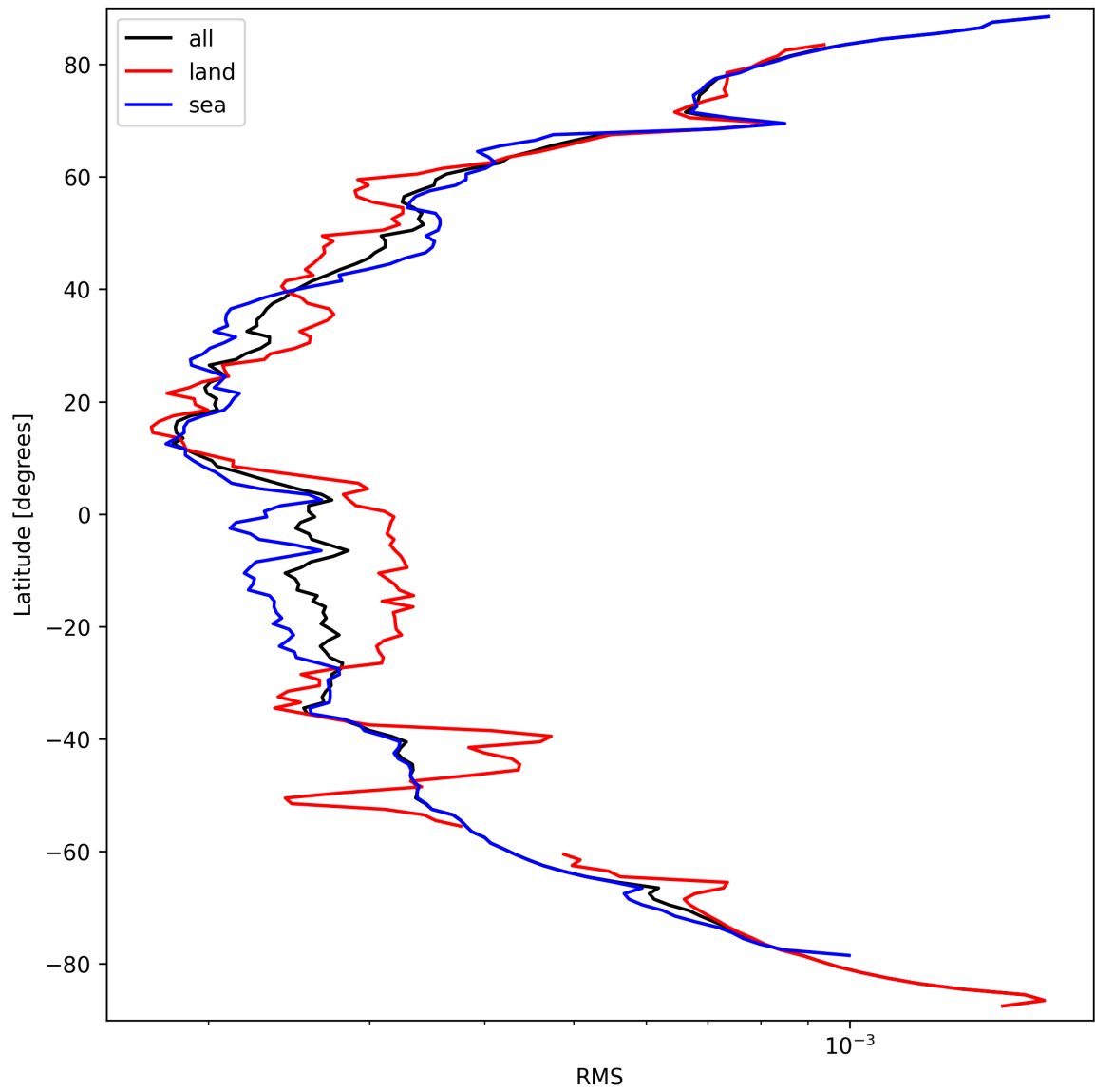
Figure 24: Zonal average of “RMS” for 2025-03-22 to 2025-03-22.
