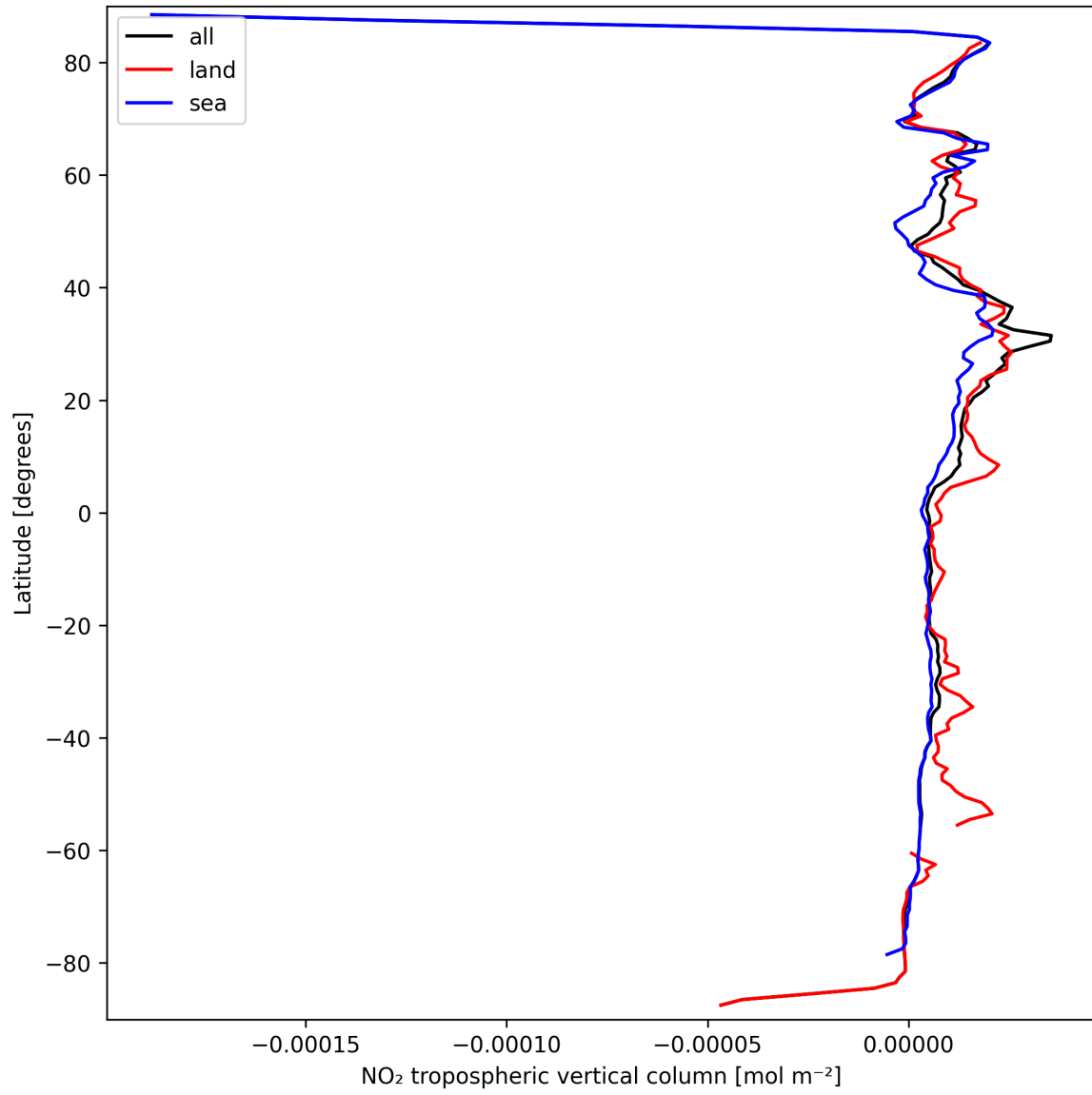
Figure 10: Zonal average of “NO 2 tropospheric vertical column” for 2025-03-22 to 2025-03-22.
