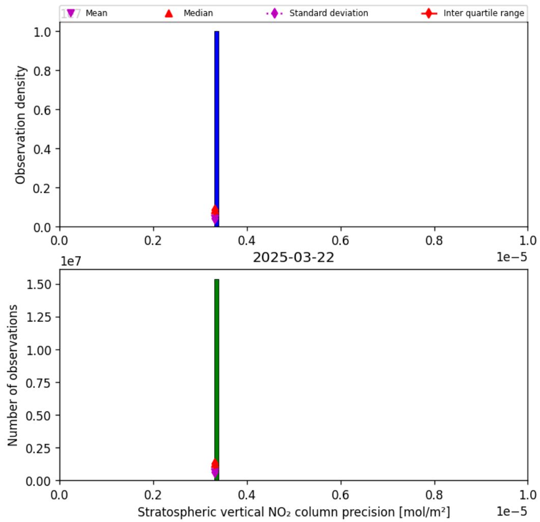
Figure 35: Histogram of “Stratospheric vertical NO 2 column precision” for 2025-03-22 to 2025-03-22
