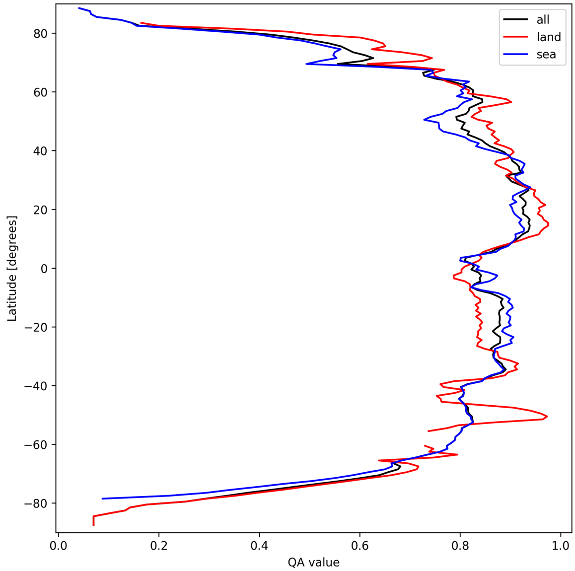
Figure 9: Zonal average of “QA value” for 2025-03-22 to 2025-03-22.
