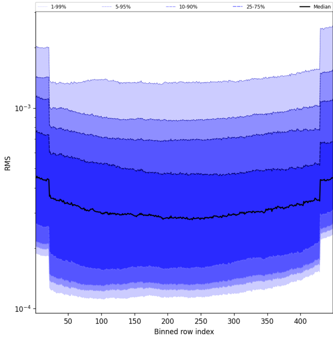
Figure 58: Along track statistics of “RMS” for 2025-03-22 to 2025-03-22
