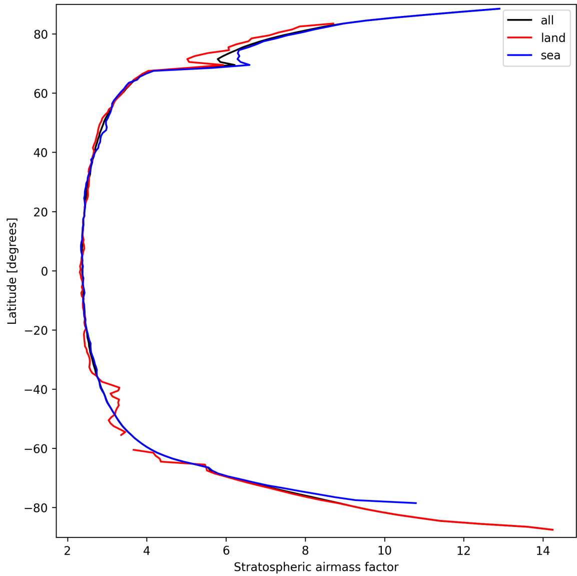
Figure 25: Zonal average of “Stratospheric air mass factor” for 2025-03-22 to 2025-03-22.
