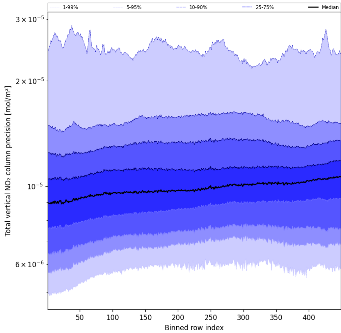
Figure 54: Along track statistics of “Total vertical NO 2 column precision” for 2025-03-22 to 2025-03-22
