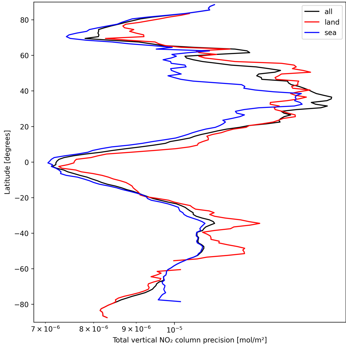
Figure 20: Zonal average of “Total vertical NO 2 column precision” for 2025-03-22 to 2025-03-22.
