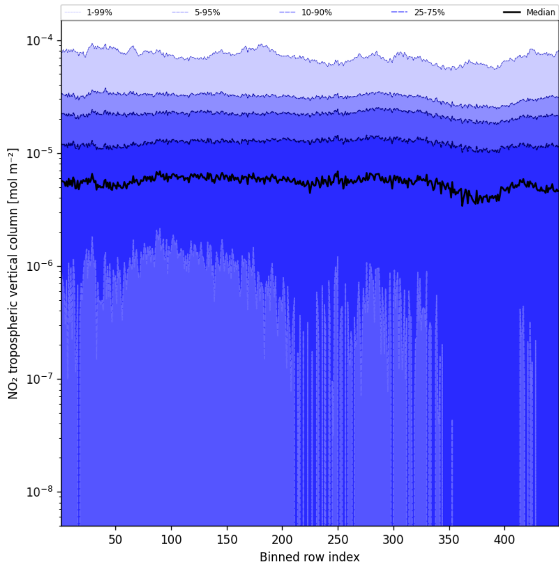
Figure 44: Along track statistics of “NO 2 tropospheric vertical column” for 2025-03-22 to 2025-03-22
