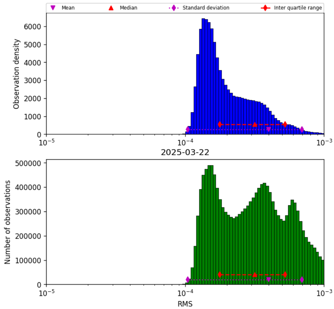
Figure 41: Histogram of “RMS” for 2025-03-22 to 2025-03-22
