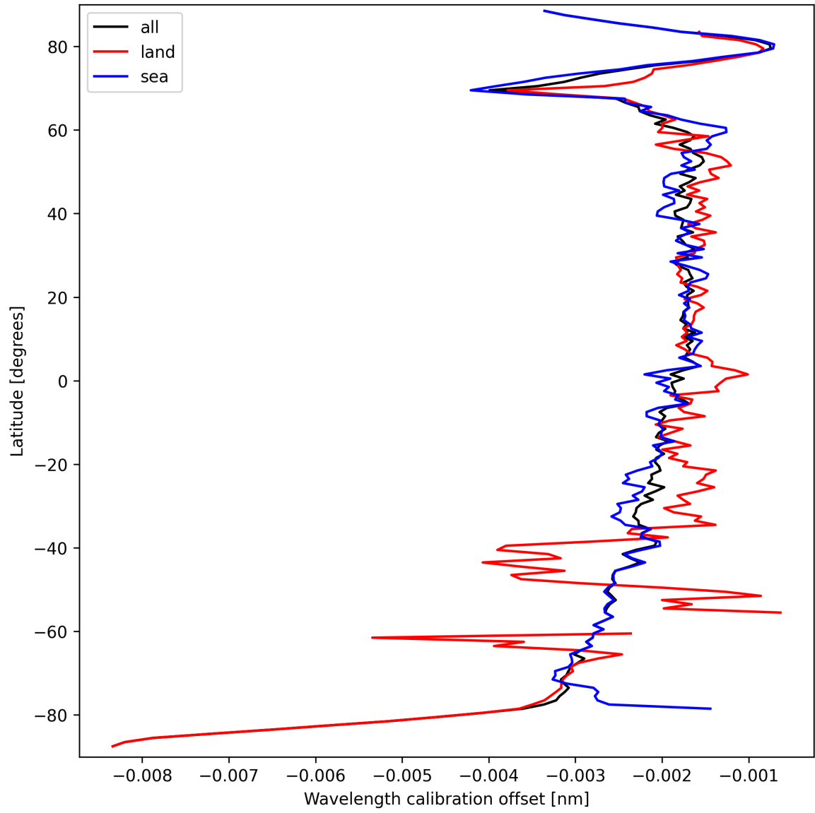
Figure 16: Zonal average of “Wavelength calibration offset” for 2025-03-22 to 2025-03-22.
