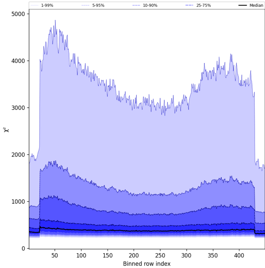
Figure 57: Along track statistics of “ \chi^2 ” for 2025-03-22 to 2025-03-22
