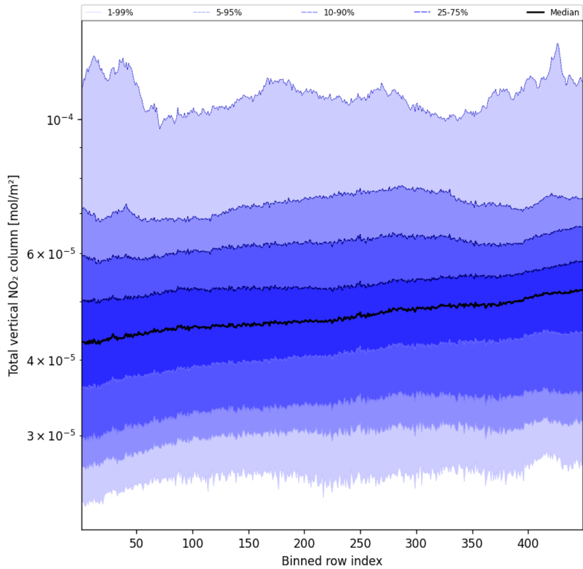
Figure 53: Along track statistics of “Total vertical NO 2 column” for 2025-03-22 to 2025-03-22
