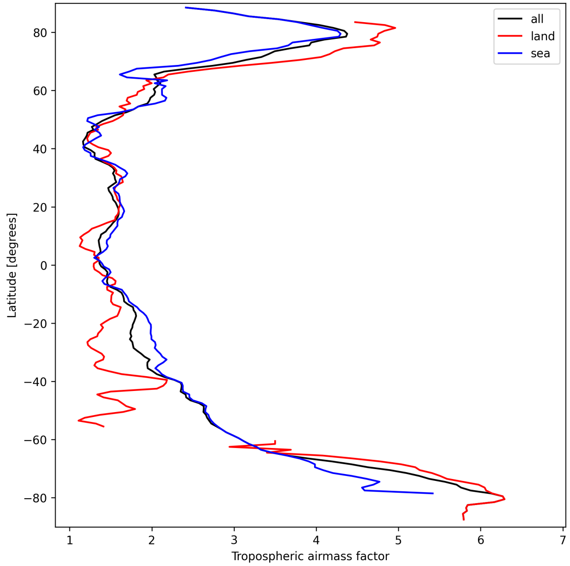
Figure 12: Zonal average of “Tropospheric air mass factor” for 2025-03-22 to 2025-03-22.
