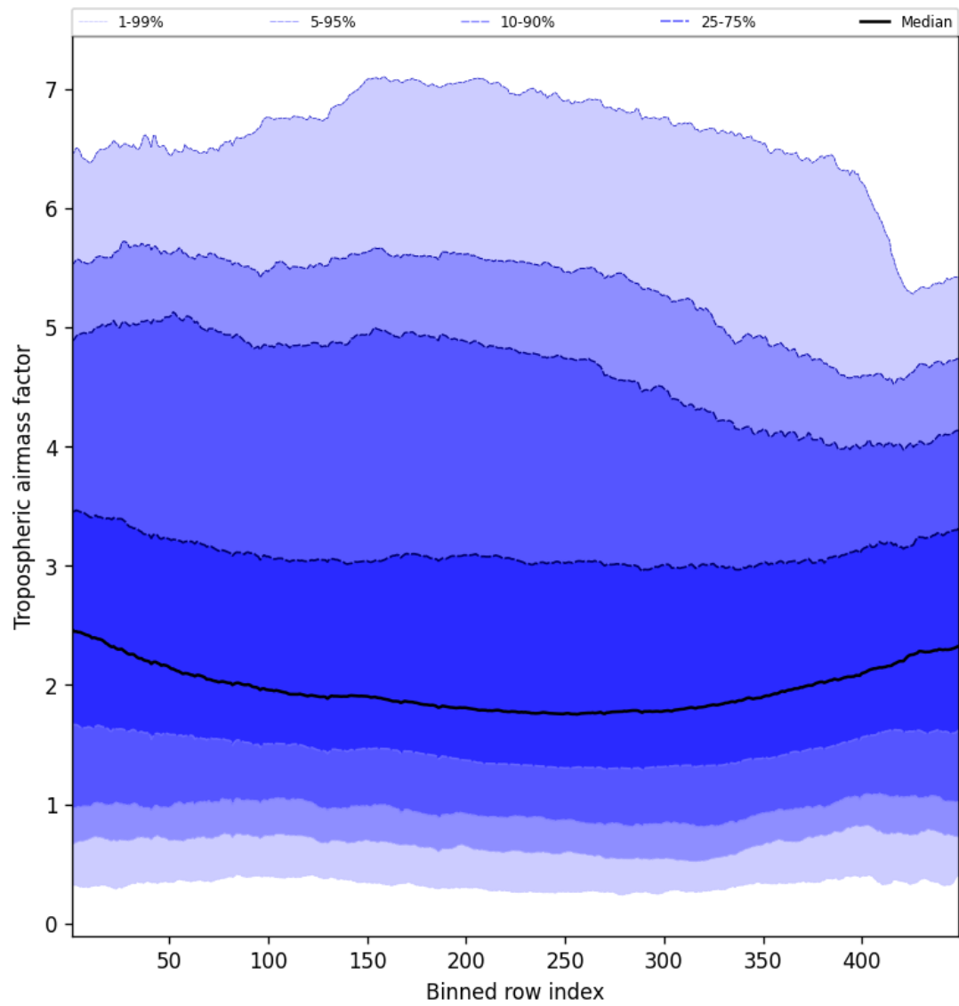
Figure 46: Along track statistics of “Tropospheric airmass factor” for 2025-03-22 to 2025-03-22
