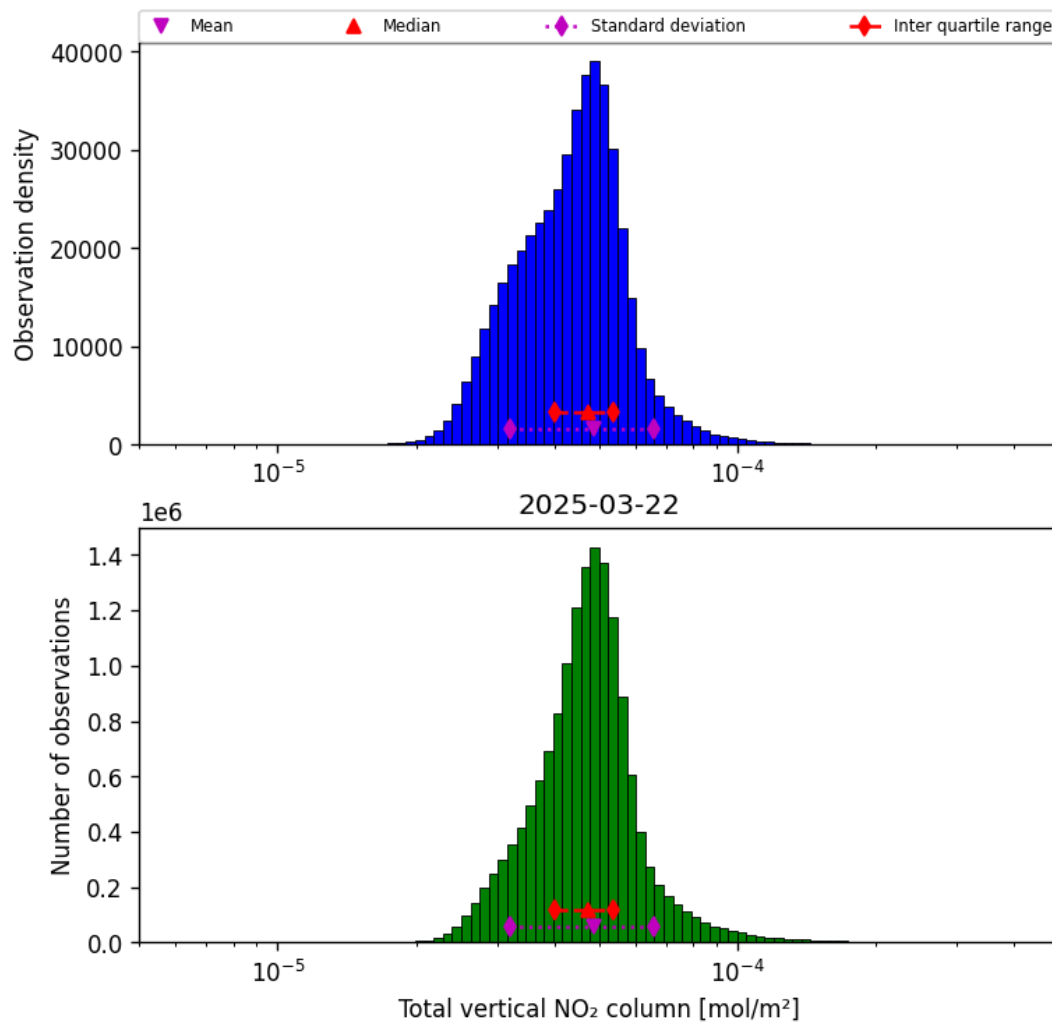
Figure 36: Histogram of “Total vertical NO 2 column” for 2025-03-22 to 2025-03-22
