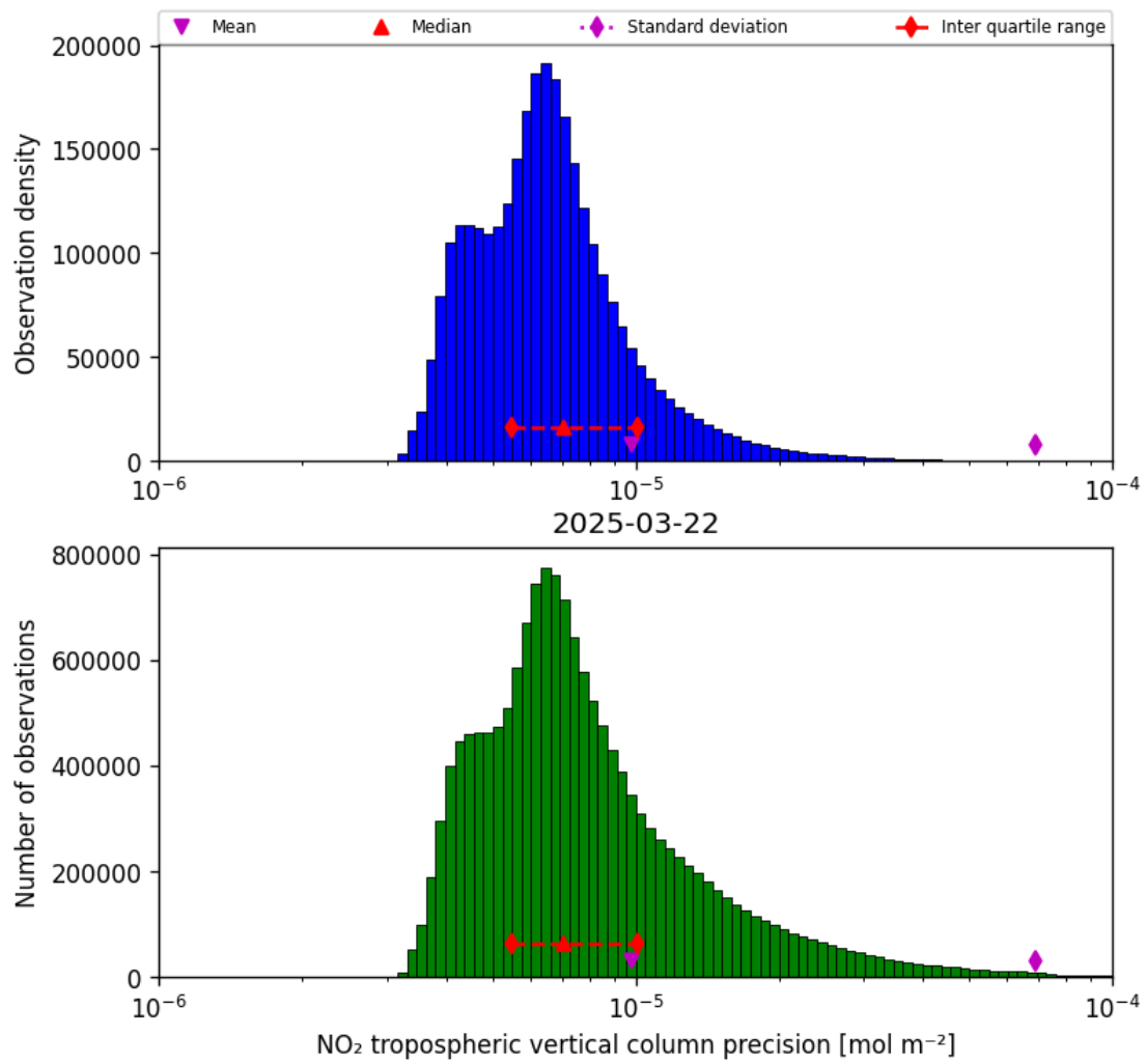
Figure 28: Histogram of “NO 2 tropospheric vertical column precision” for 2025-03-22 to 2025-03-22
