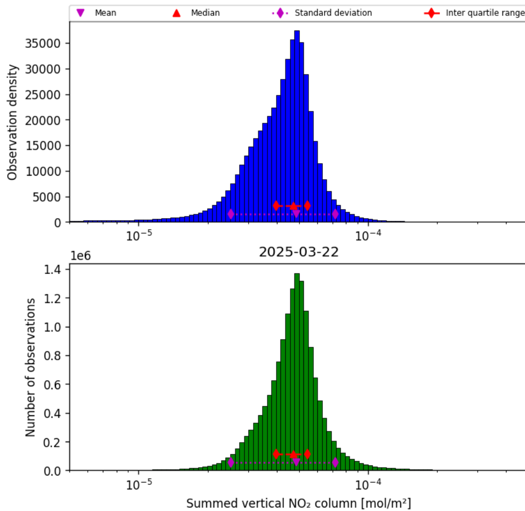
Figure 38: Histogram of “Summed vertical NO 2 column” for 2025-03-22 to 2025-03-22
