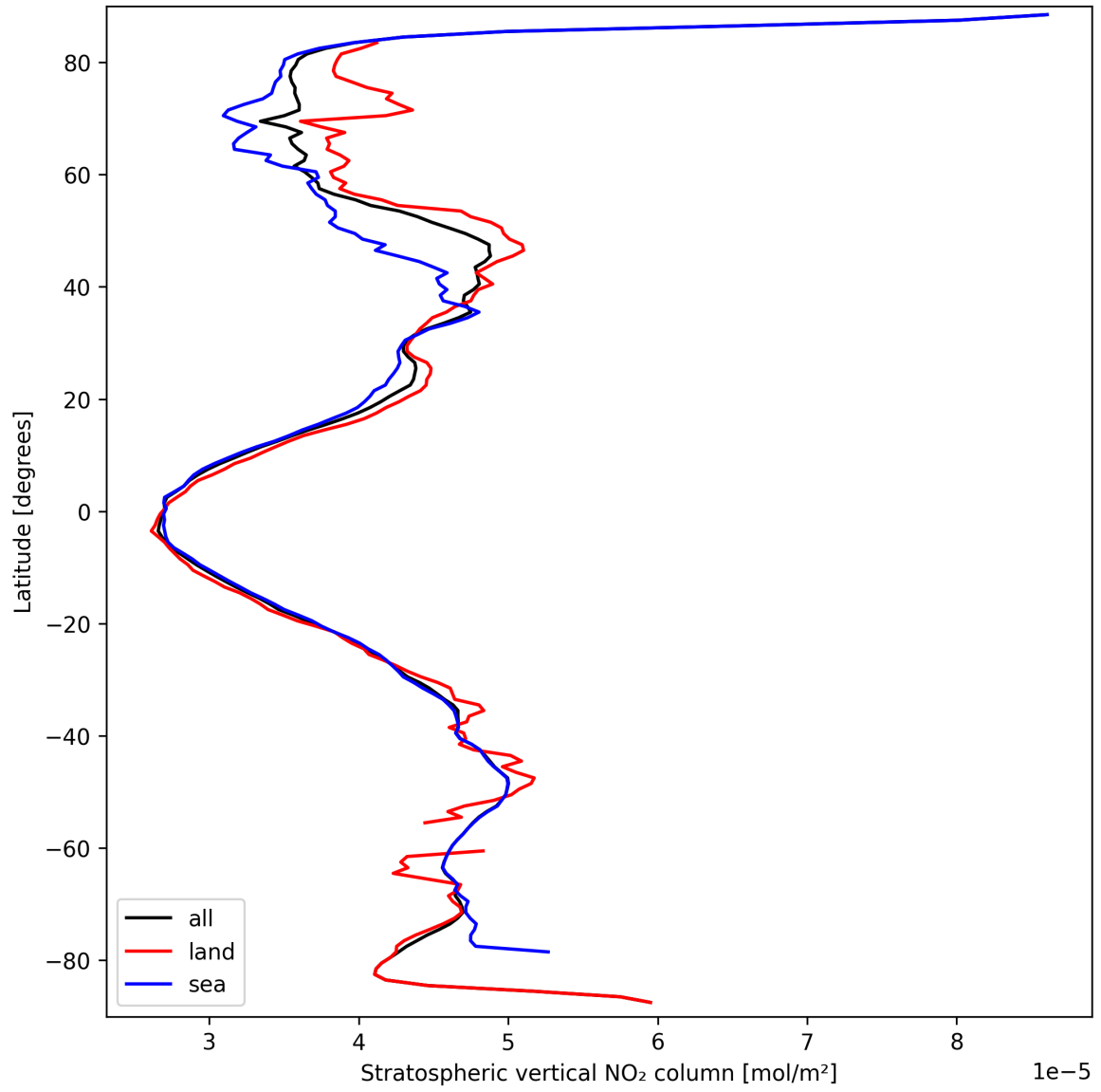
Figure 17: Zonal average of “Stratospheric vertical NO 2 column” for 2025-03-22 to 2025-03-22.
