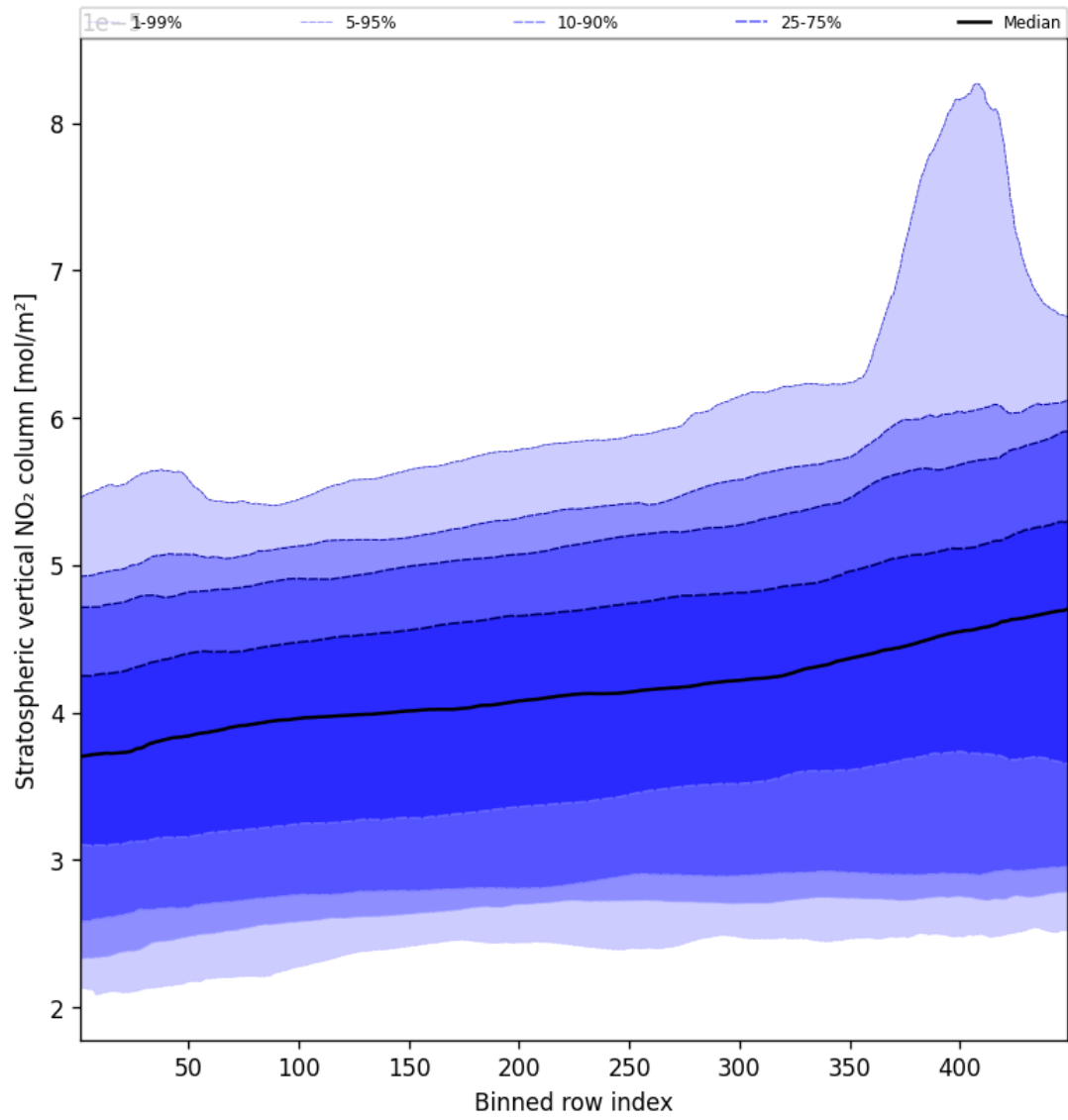
Figure 51: Along track statistics of “Stratospheric vertical NO 2 column” for 2025-03-22 to 2025-03-22
