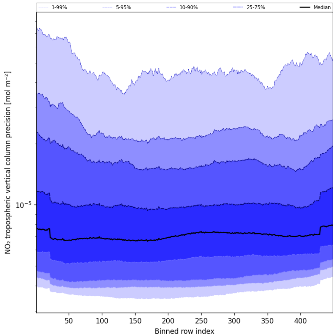
Figure 45: Along track statistics of “NO 2 tropospheric vertical column precision” for 2025-03-22 to 2025-03-22
