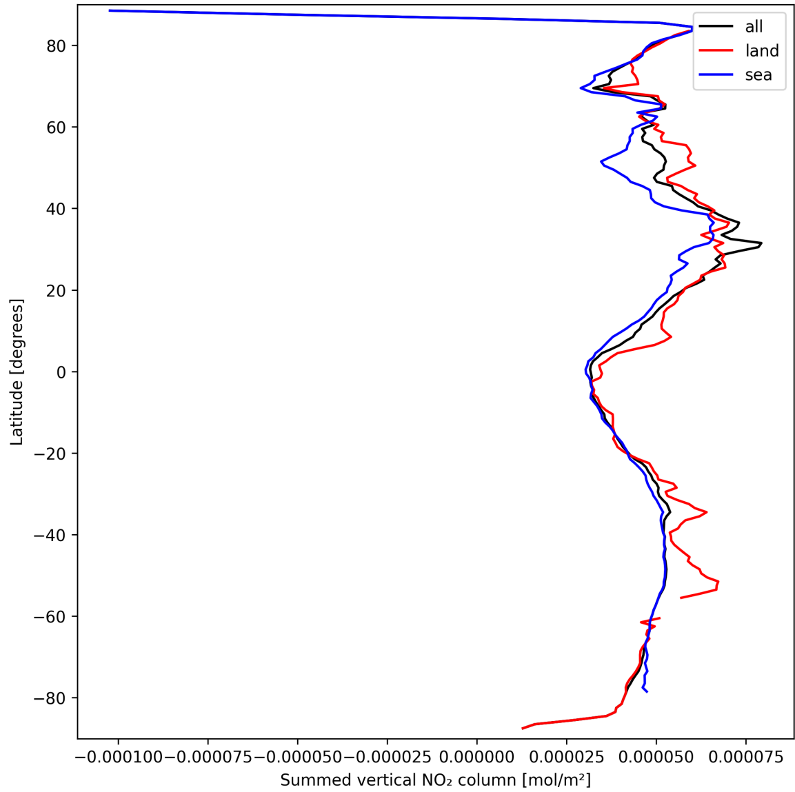
Figure 21: Zonal average of “Summed vertical NO 2 column” for 2025-03-22 to 2025-03-22.
