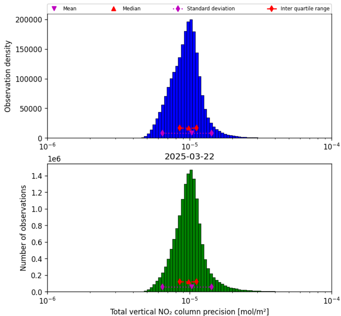
Figure 37: Histogram of "Total vertical NO 2 column precision" for 2025-03-22 to 2025-03-22
