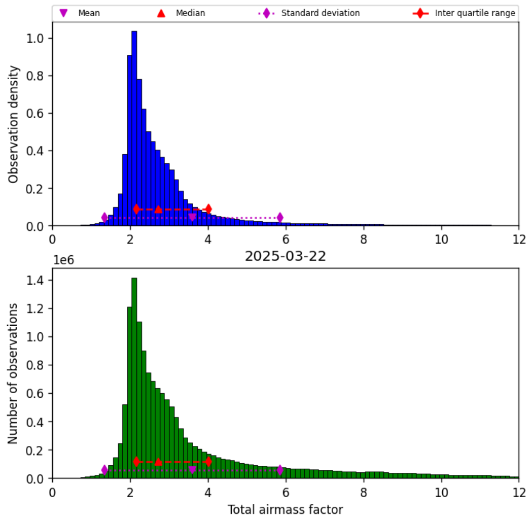
Figure 30: Histogram of “Total airmass factor” for 2025-03-22 to 2025-03-22
