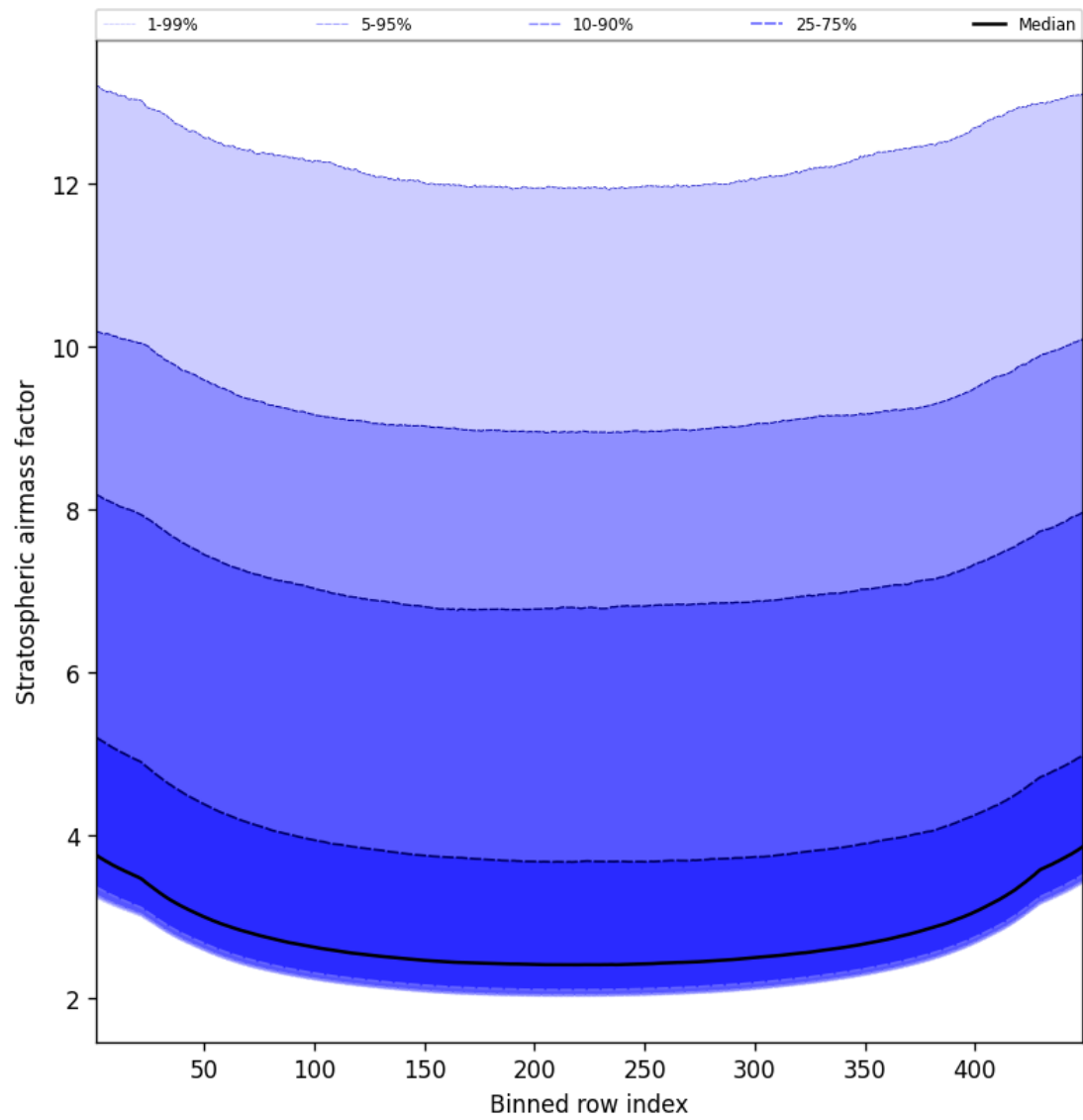
Figure 59: Along track statistics of “Stratospheric airmass factor” for 2025-03-22 to 2025-03-22
