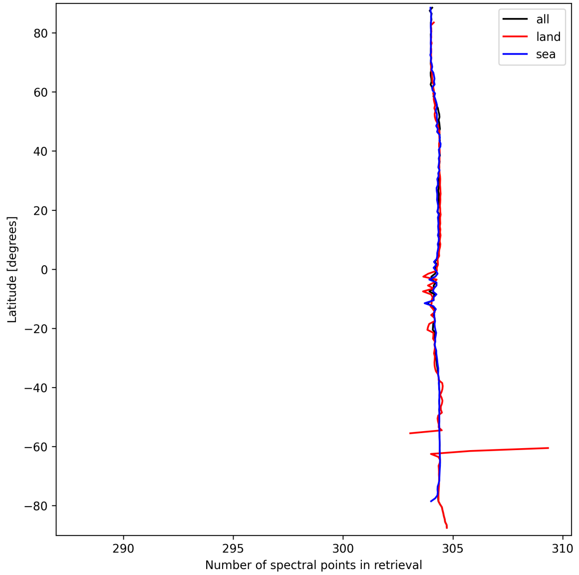
Figure 14: Zonal average of “Number of spectral points in retrieval” for 2025-03-22 to 2025-03-22.
