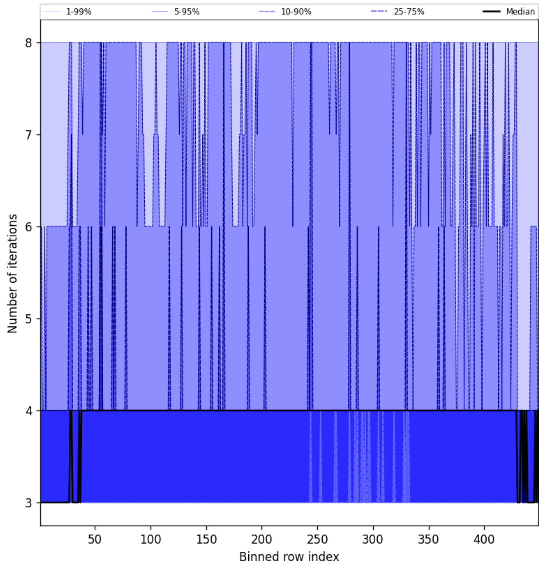
Figure 49: Along track statistics of “Number of iterations” for 2025-03-22 to 2025-03-22
