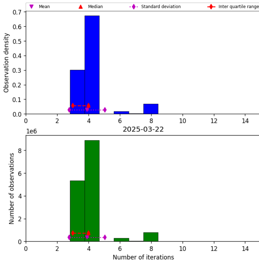
Figure 32: Histogram of “Number of iterations” for 2025-03-22 to 2025-03-22
