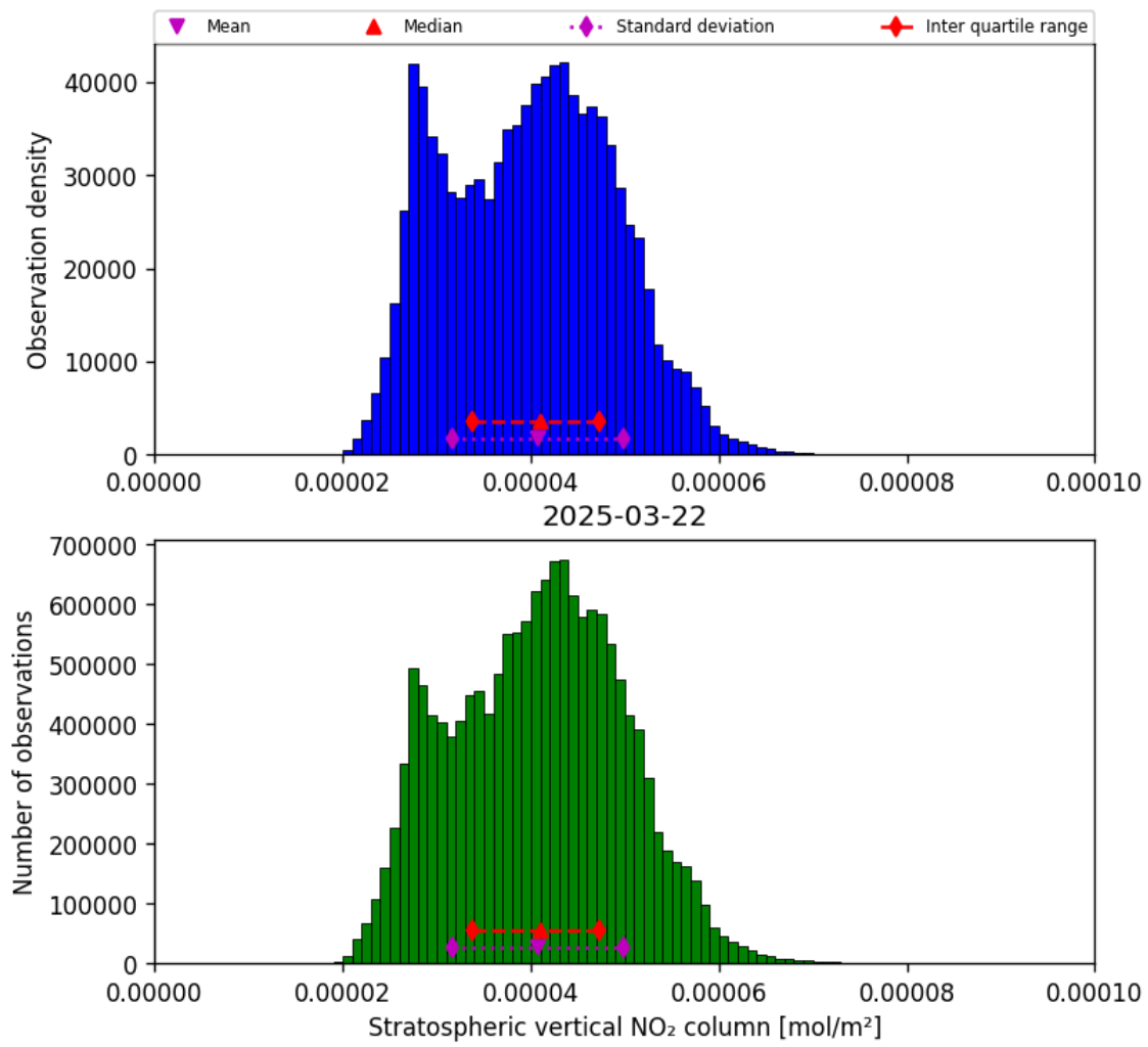
Figure 34: Histogram of “Stratospheric vertical NO 2 column” for 2025-03-22 to 2025-03-22
