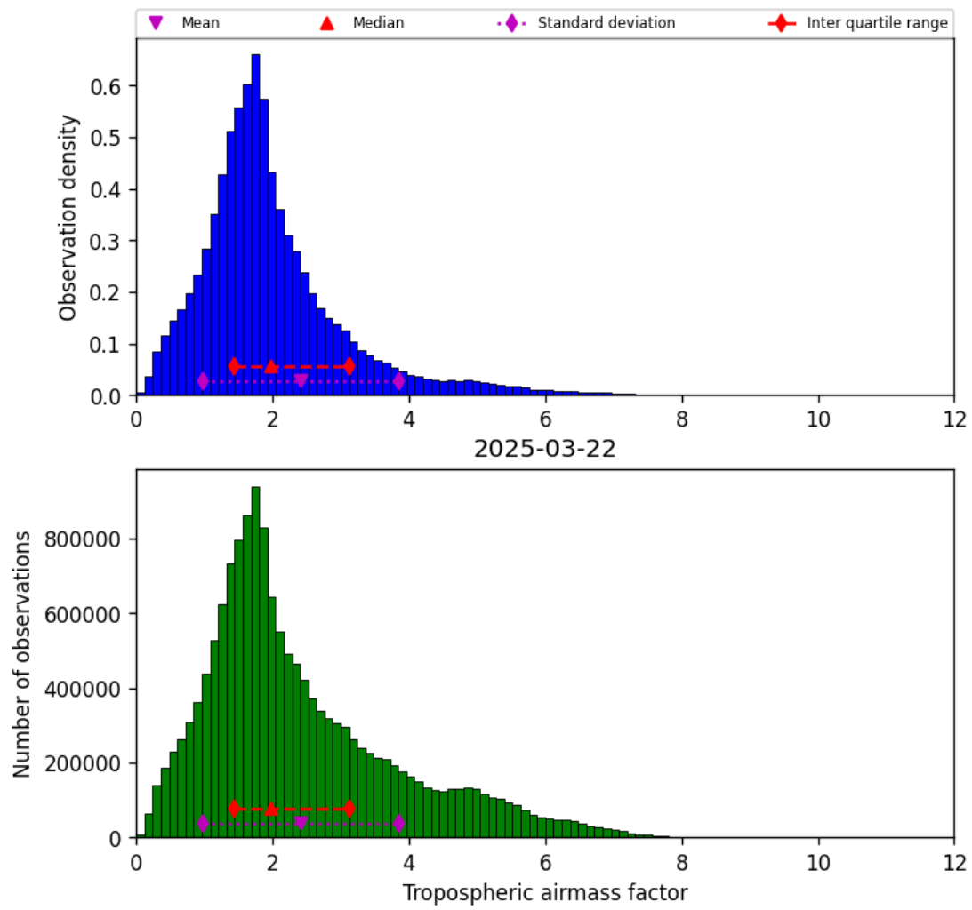
Figure 29: Histogram of “Tropospheric airmass factor” for 2025-03-22 to 2025-03-22
