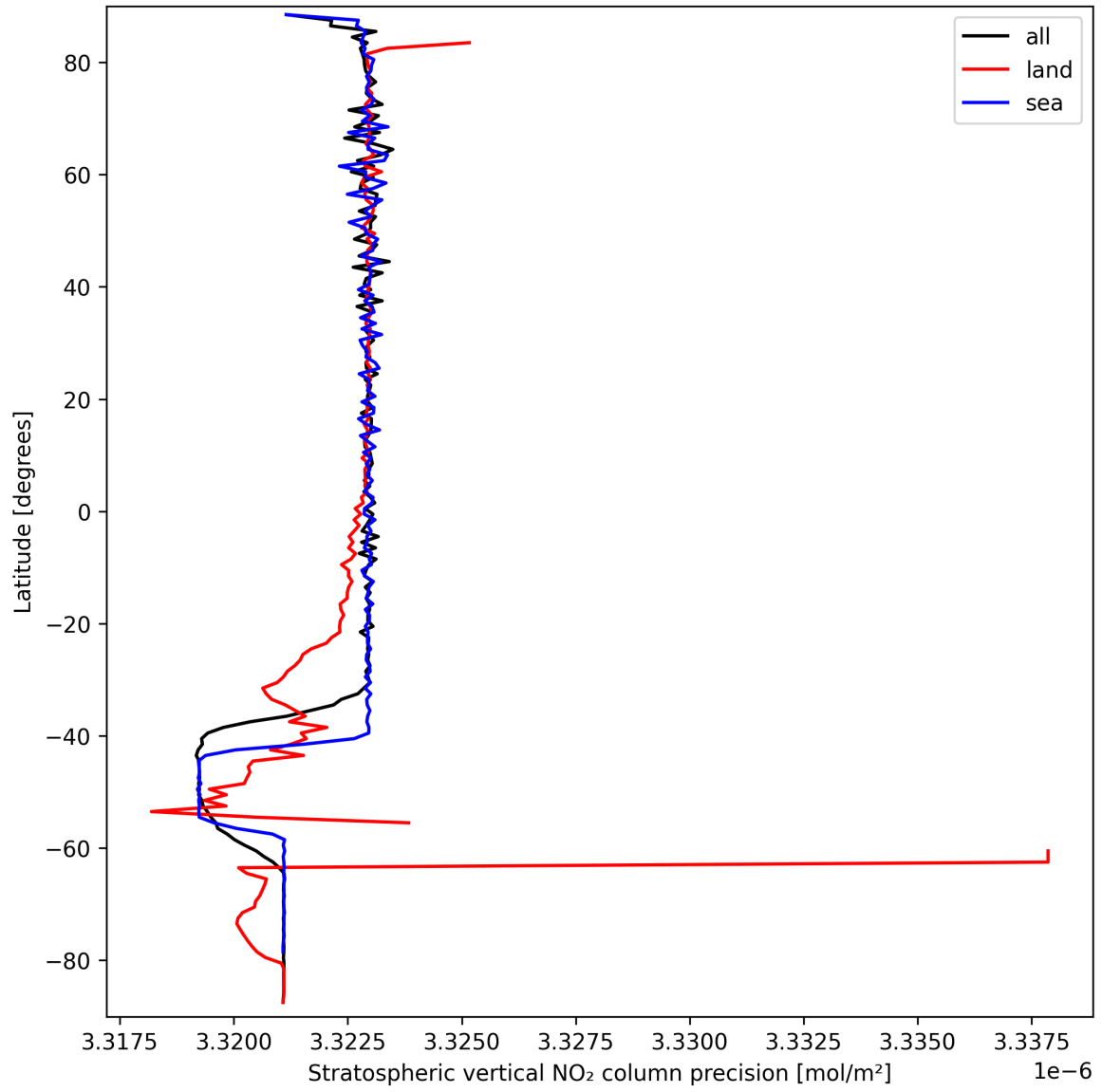
Figure 18: Zonal average of “Stratospheric vertical NO 2 column precision” for 2025-03-22 to 2025-03-22.
