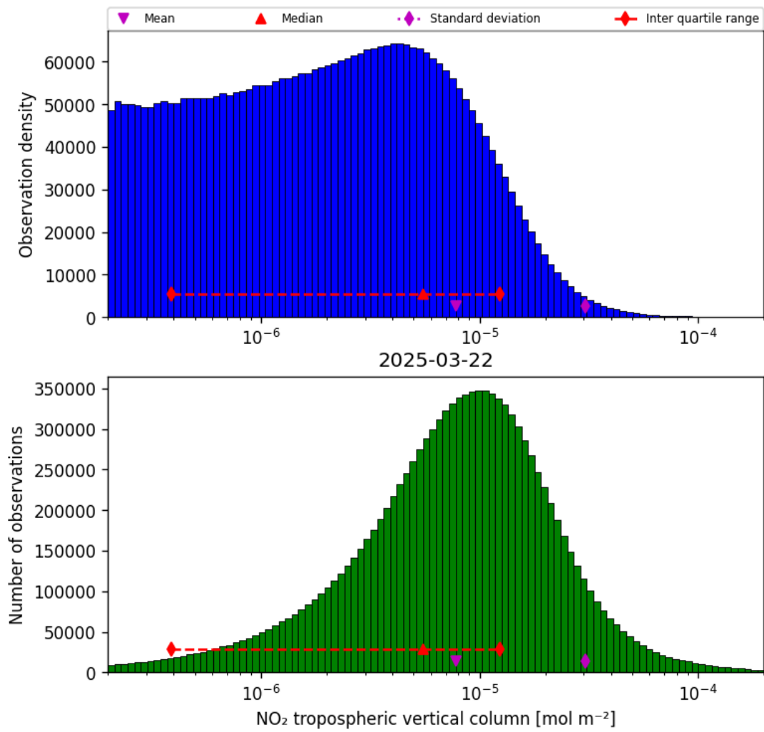
Figure 27: Histogram of “NO 2 tropospheric vertical column” for 2025-03-22 to 2025-03-22
