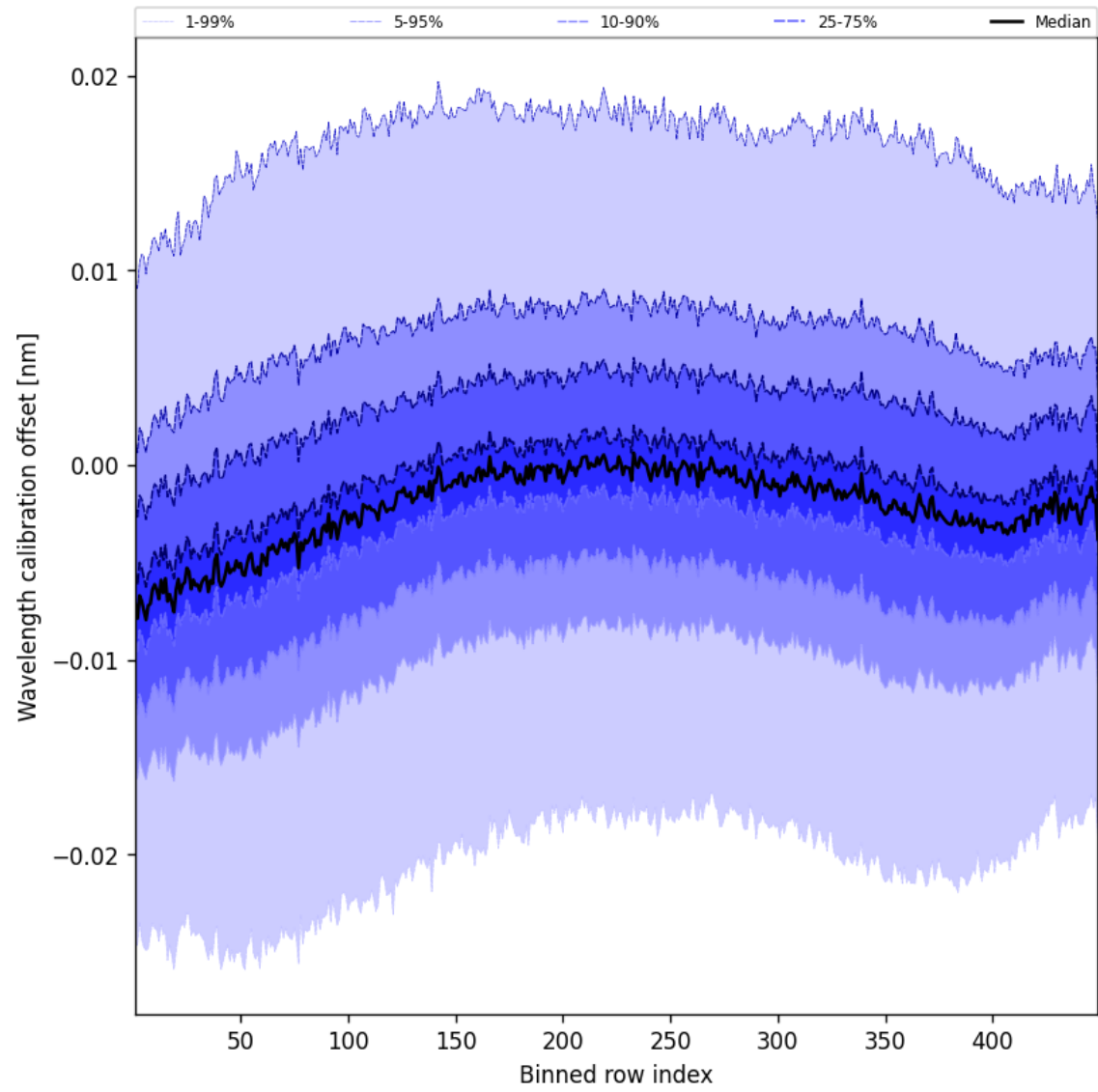
Figure 50: Along track statistics of “Wavelength calibration offset” for 2025-03-22 to 2025-03-22
