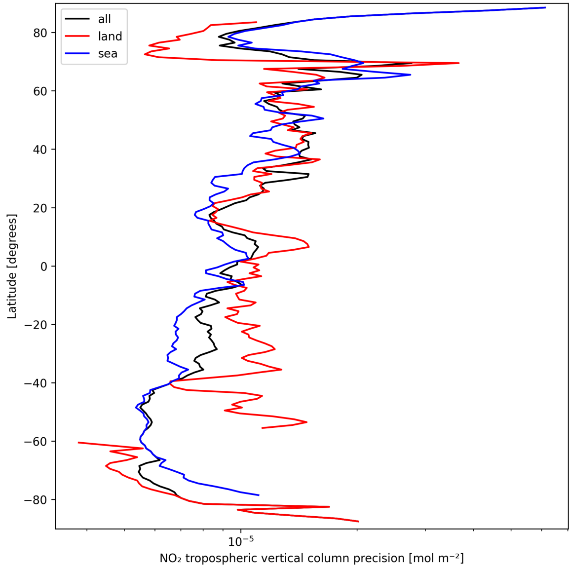
Figure 11: Zonal average of “NO 2 tropospheric vertical column precision” for 2025-03-22 to 2025-03-22.
