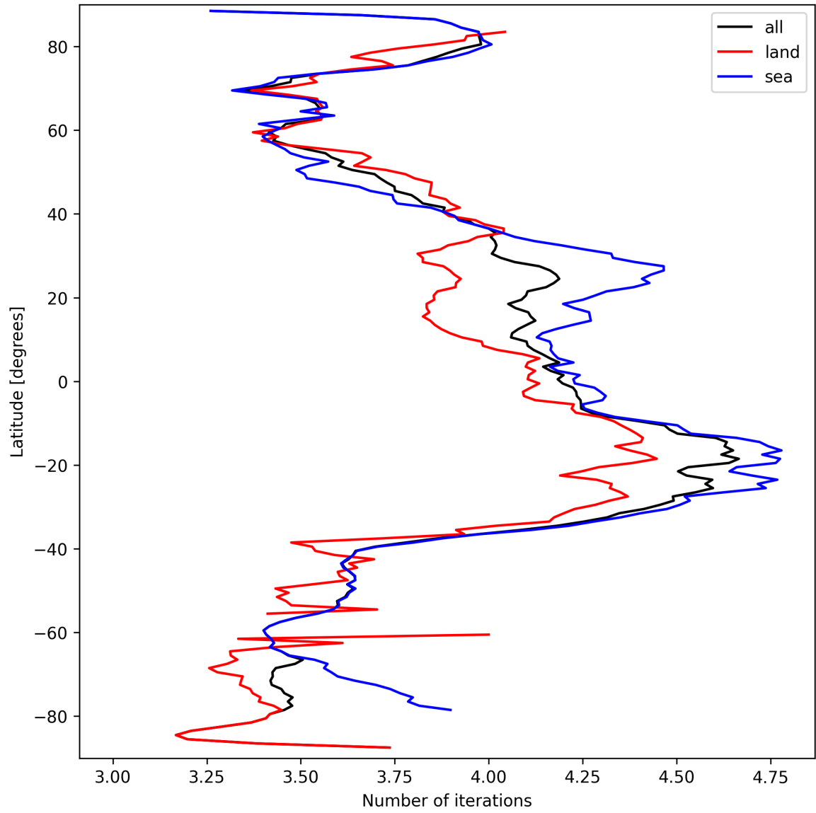
Figure 15: Zonal average of “Number of iterations” for 2025-03-22 to 2025-03-22.
