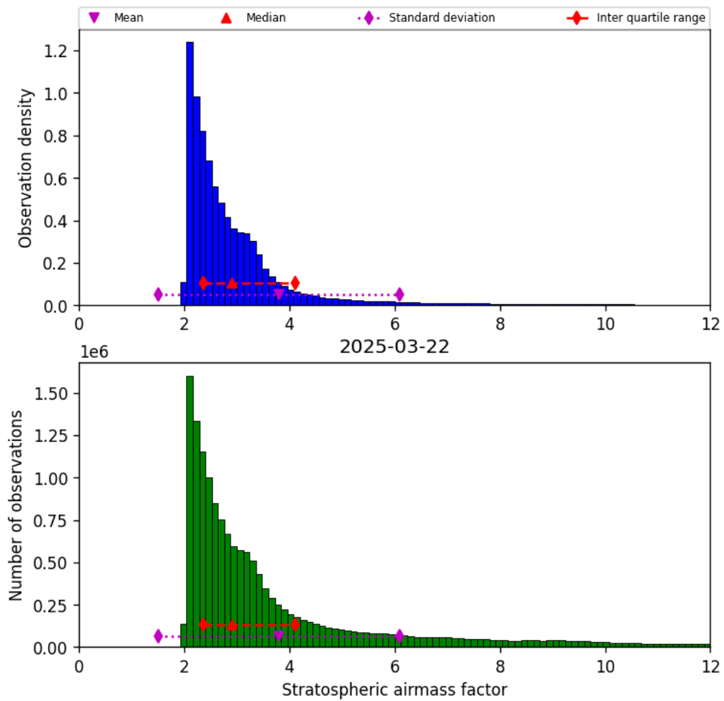
Figure 42: Histogram of “Stratospheric airmass factor” for 2025-03-22 to 2025-03-22
