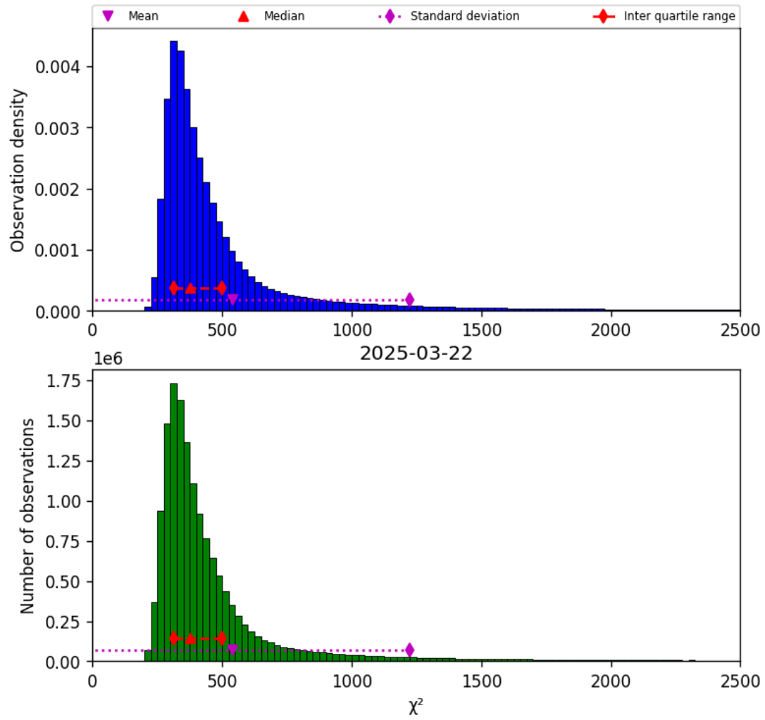
Figure 40: Histogram of " \chi^2 " for 2025-03-22 to 2025-03-22
