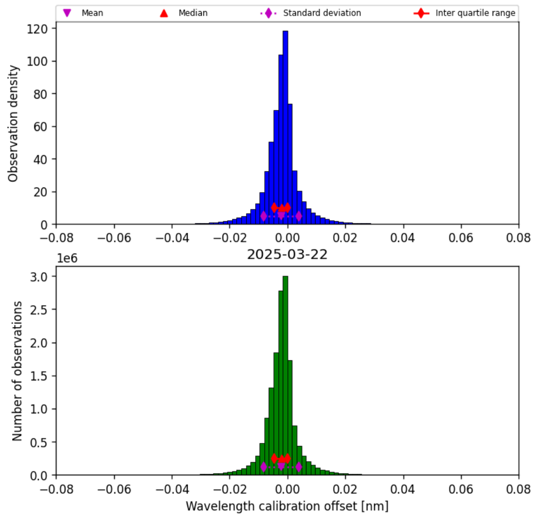
Figure 33: Histogram of “Wavelength calibration offset” for 2025-03-22 to 2025-03-22
