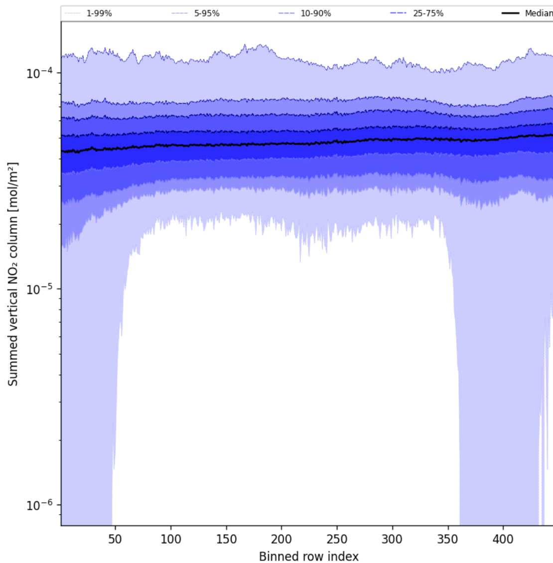
Figure 55: Along track statistics of “Summed vertical NO 2 column” for 2025-03-22 to 2025-03-22
