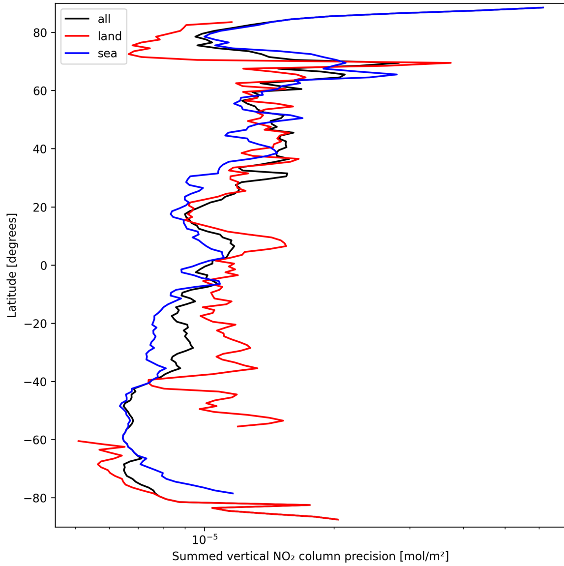
Figure 22: Zonal average of “Summed vertical NO 2 column precision” for 2025-03-22 to 2025-03-22.
