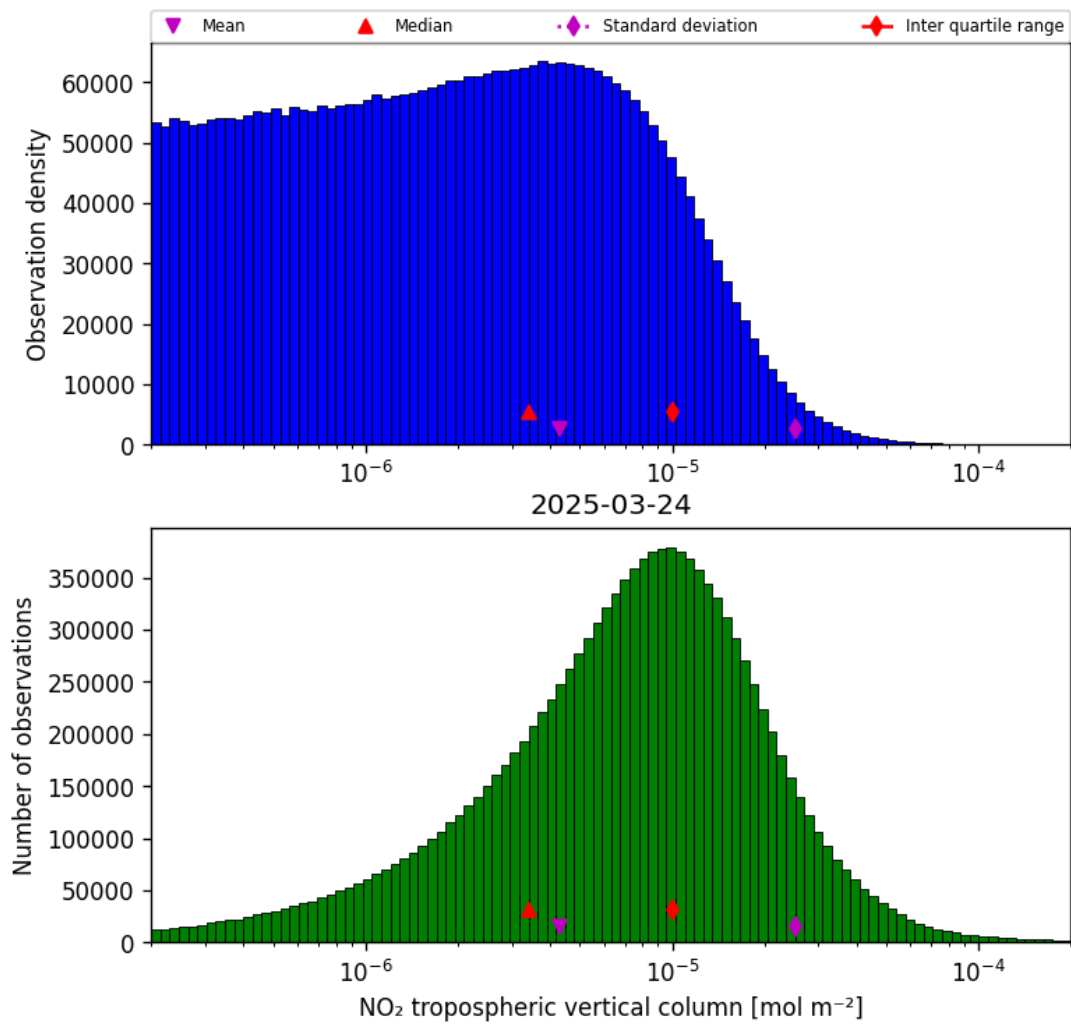
Figure 27: Histogram of “NO 2 tropospheric vertical column” for 2025-03-24 to 2025-03-25
