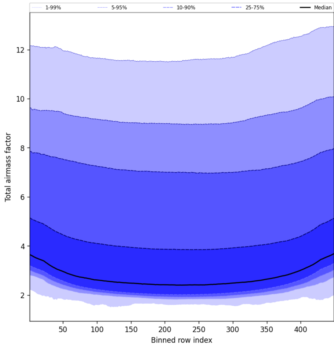
Figure 47: Along track statistics of “Total airmass factor” for 2025-03-24 to 2025-03-25
