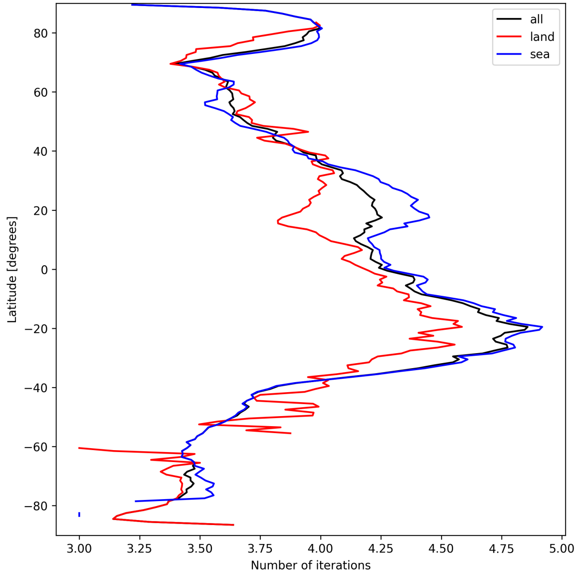
Figure 15: Zonal average of “Number of iterations” for 2025-03-24 to 2025-03-25.
