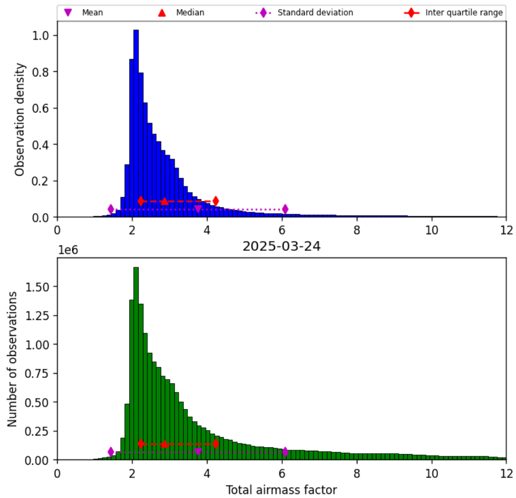
Figure 30: Histogram of “Total airmass factor” for 2025-03-24 to 2025-03-25
