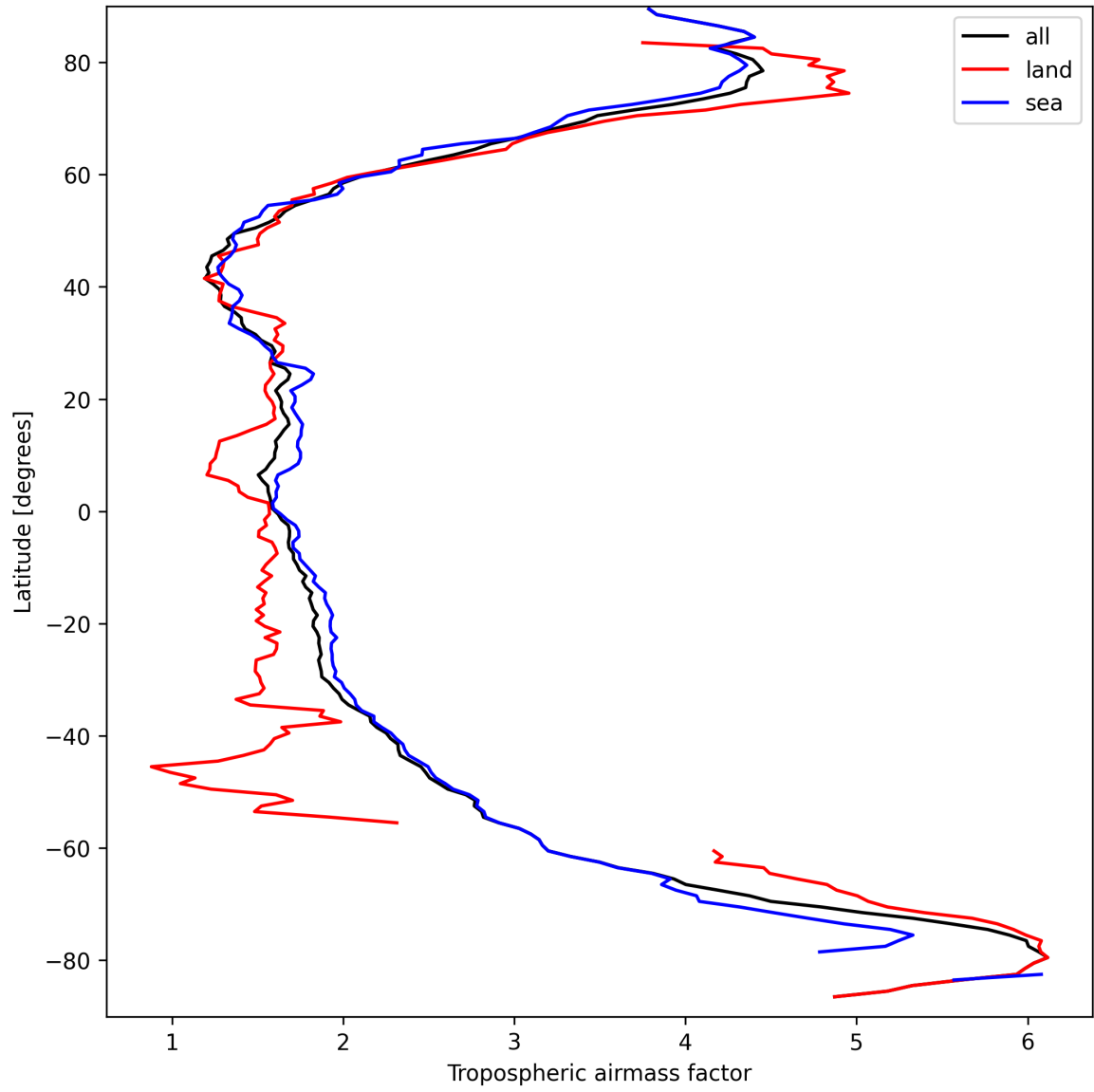
Figure 12: Zonal average of “Tropospheric air mass factor” for 2025-03-24 to 2025-03-25.
