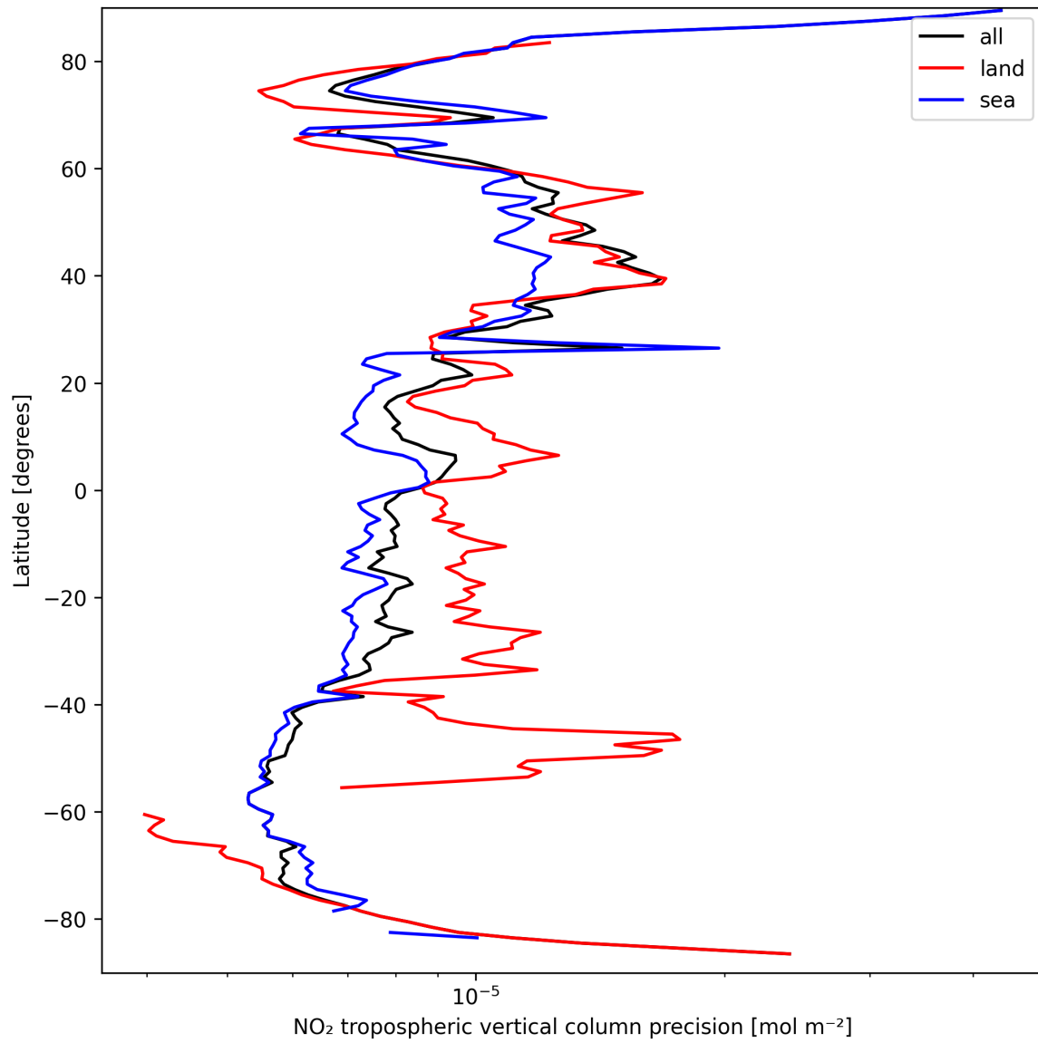
Figure 11: Zonal average of “NO 2 tropospheric vertical column precision” for 2025-03-24 to 2025-03-25.
