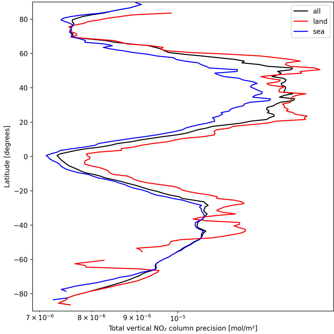
Figure 20: Zonal average of “Total vertical NO 2 column precision” for 2025-03-24 to 2025-03-25.
