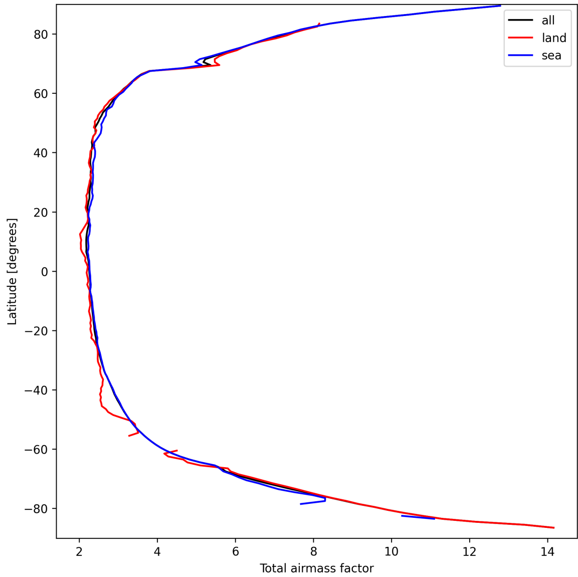
Figure 13: Zonal average of “Total airmass factor” for 2025-03-24 to 2025-03-25.
