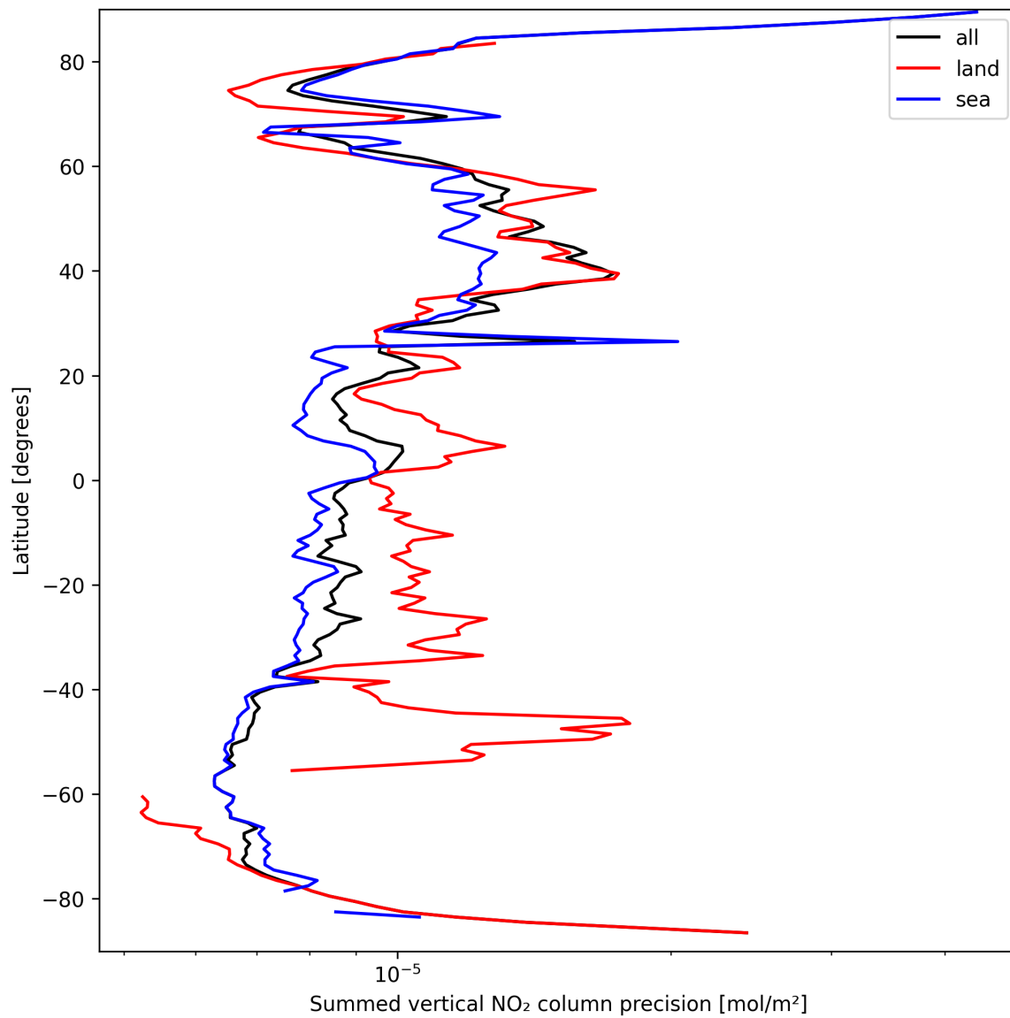
Figure 22: Zonal average of “Summed vertical NO 2 column precision” for 2025-03-24 to 2025-03-25.
