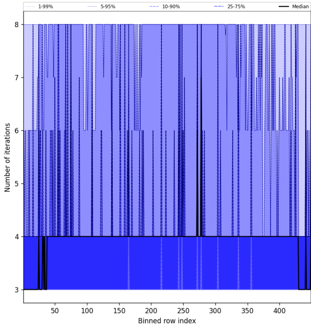
Figure 49: Along track statistics of “Number of iterations” for 2025-03-24 to 2025-03-25
