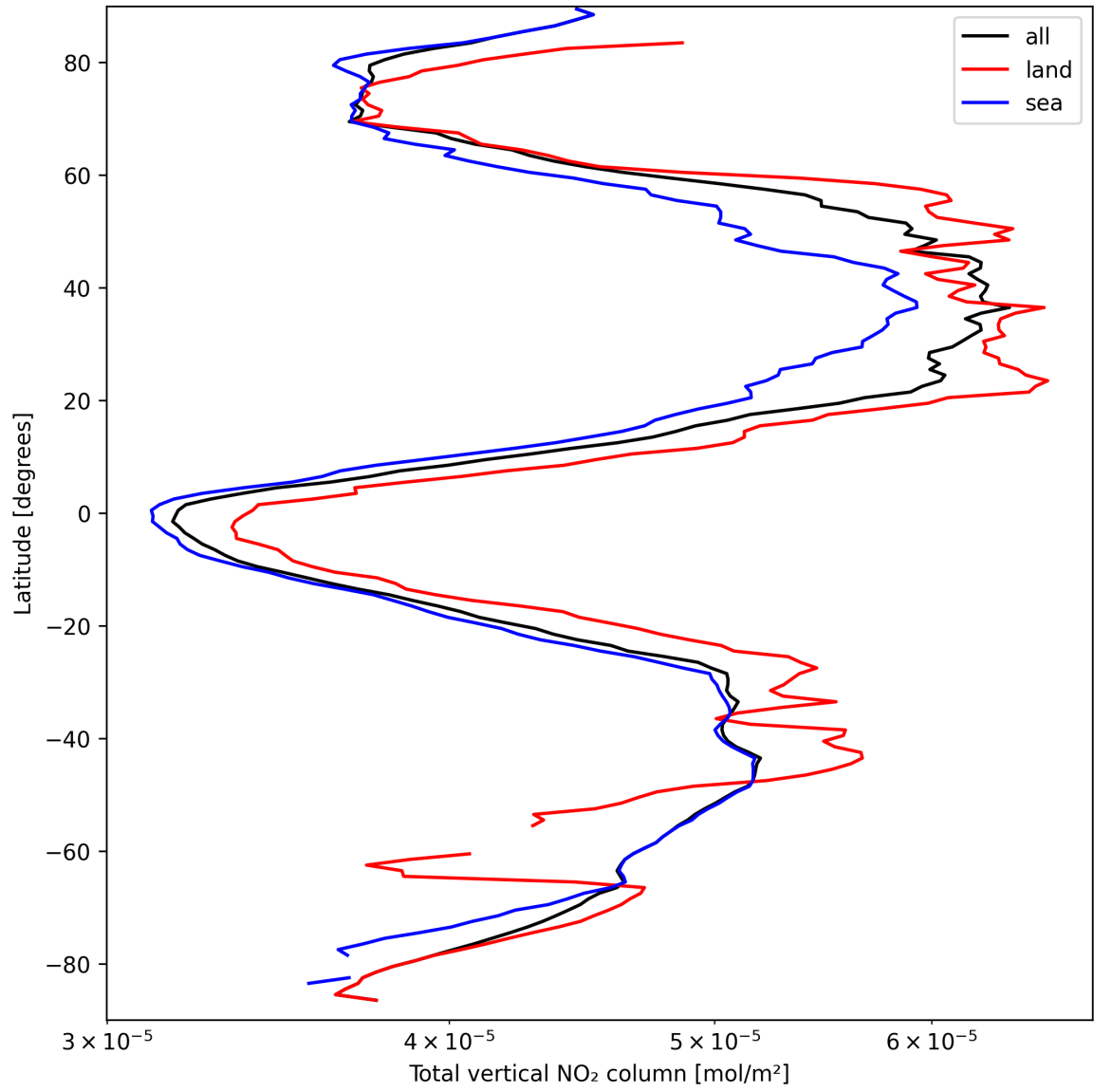
Figure 19: Zonal average of “Total vertical NO 2 column” for 2025-03-24 to 2025-03-25.
