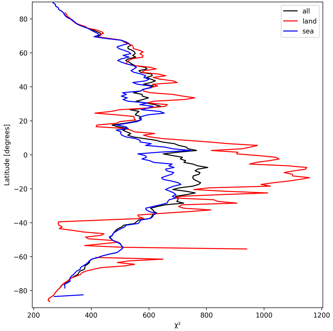
Figure 23: Zonal average of “ \chi^2 ” for 2025-03-24 to 2025-03-25.
