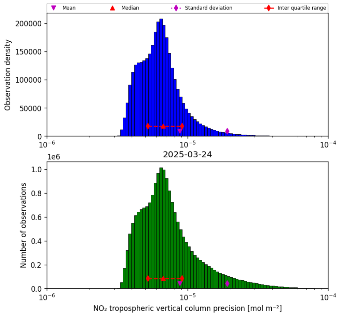
Figure 28: Histogram of “NO 2 tropospheric vertical column precision” for 2025-03-24 to 2025-03-25
