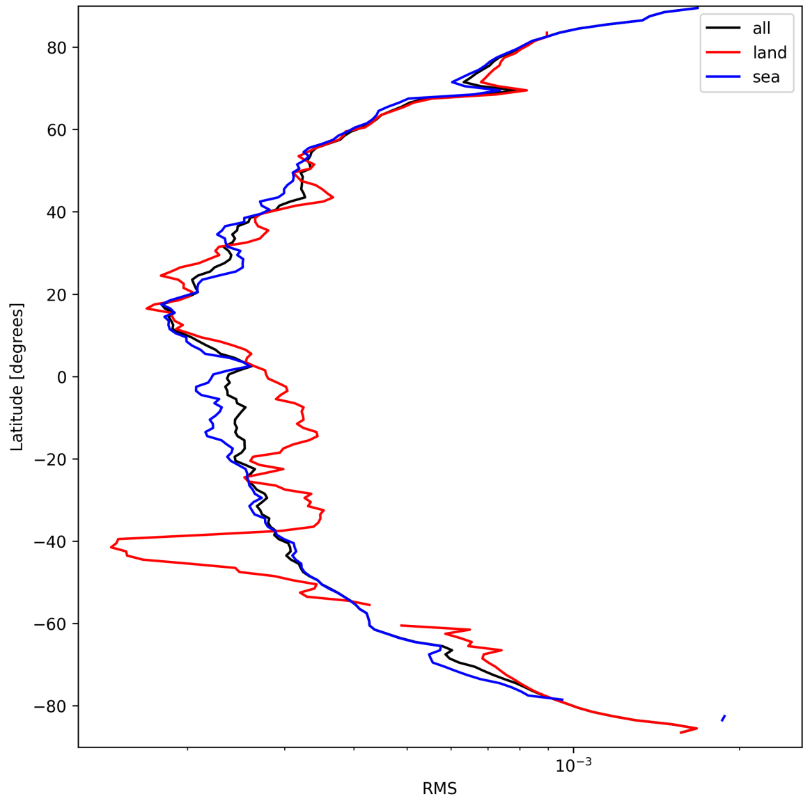
Figure 24: Zonal average of “RMS” for 2025-03-24 to 2025-03-25.
