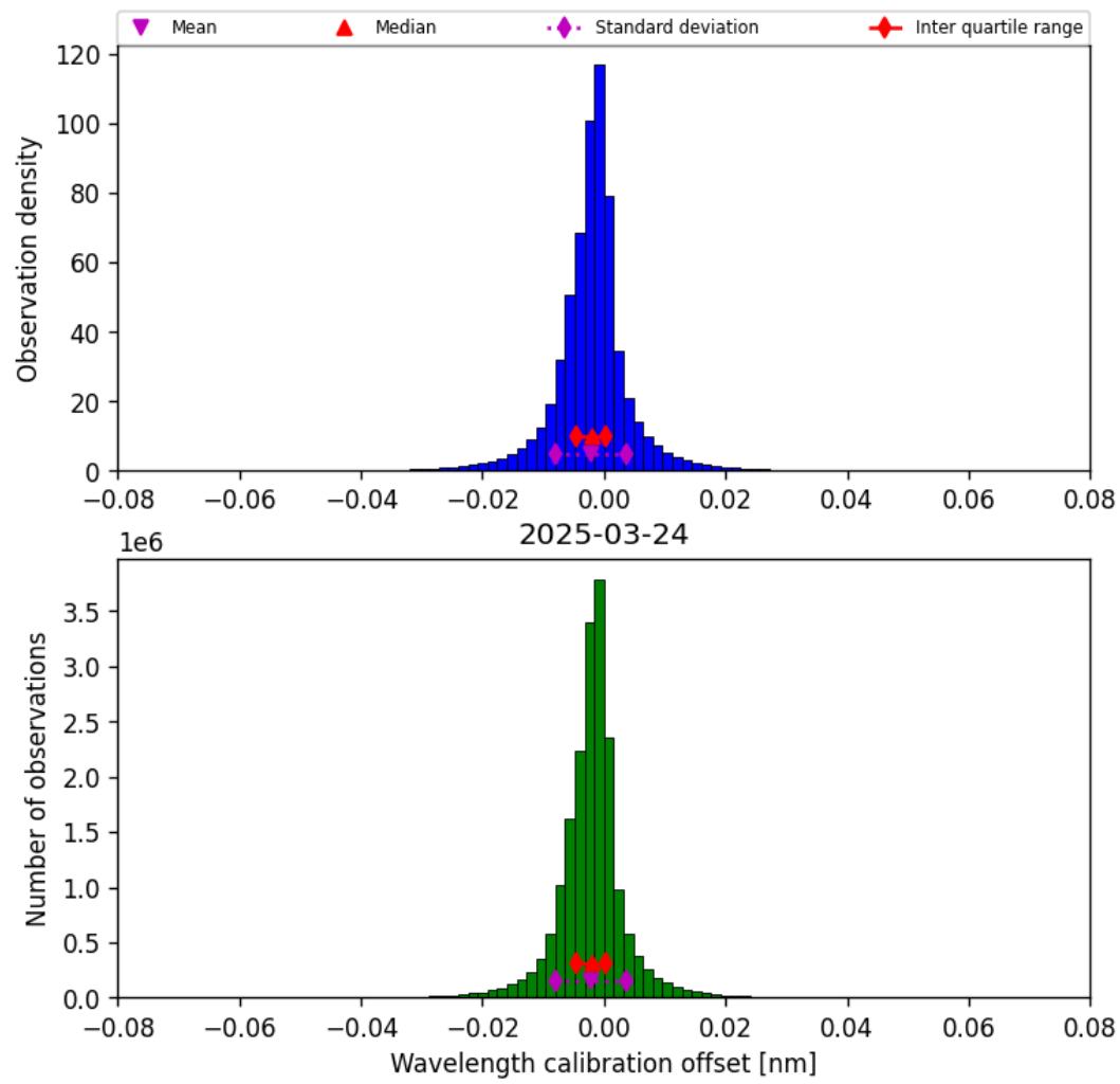
Figure 33: Histogram of “Wavelength calibration offset” for 2025-03-24 to 2025-03-25
