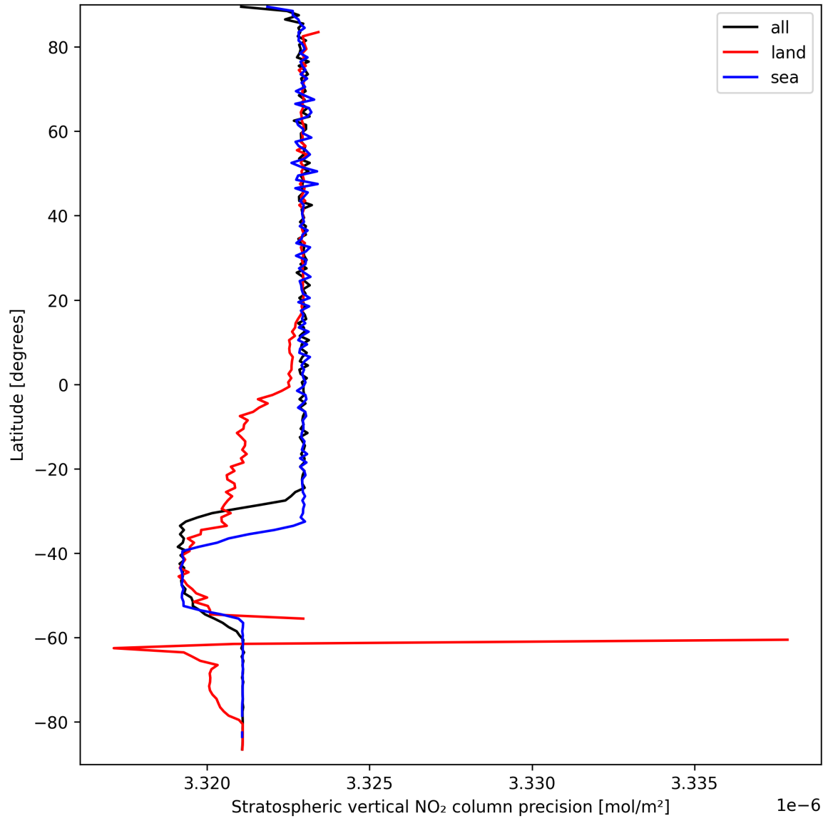
Figure 18: Zonal average of “Stratospheric vertical NO 2 column precision” for 2025-03-24 to 2025-03-25.
