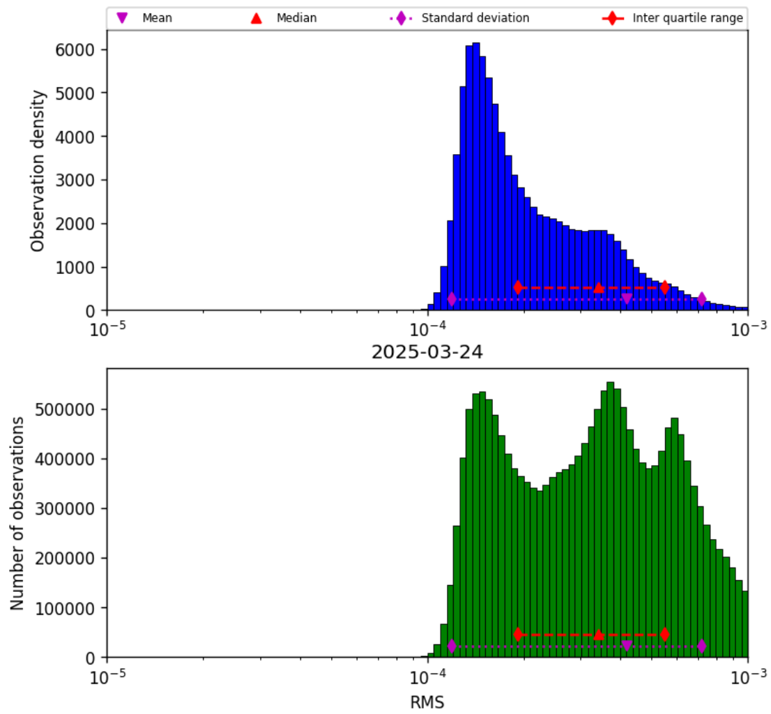
Figure 41: Histogram of “RMS” for 2025-03-24 to 2025-03-25
