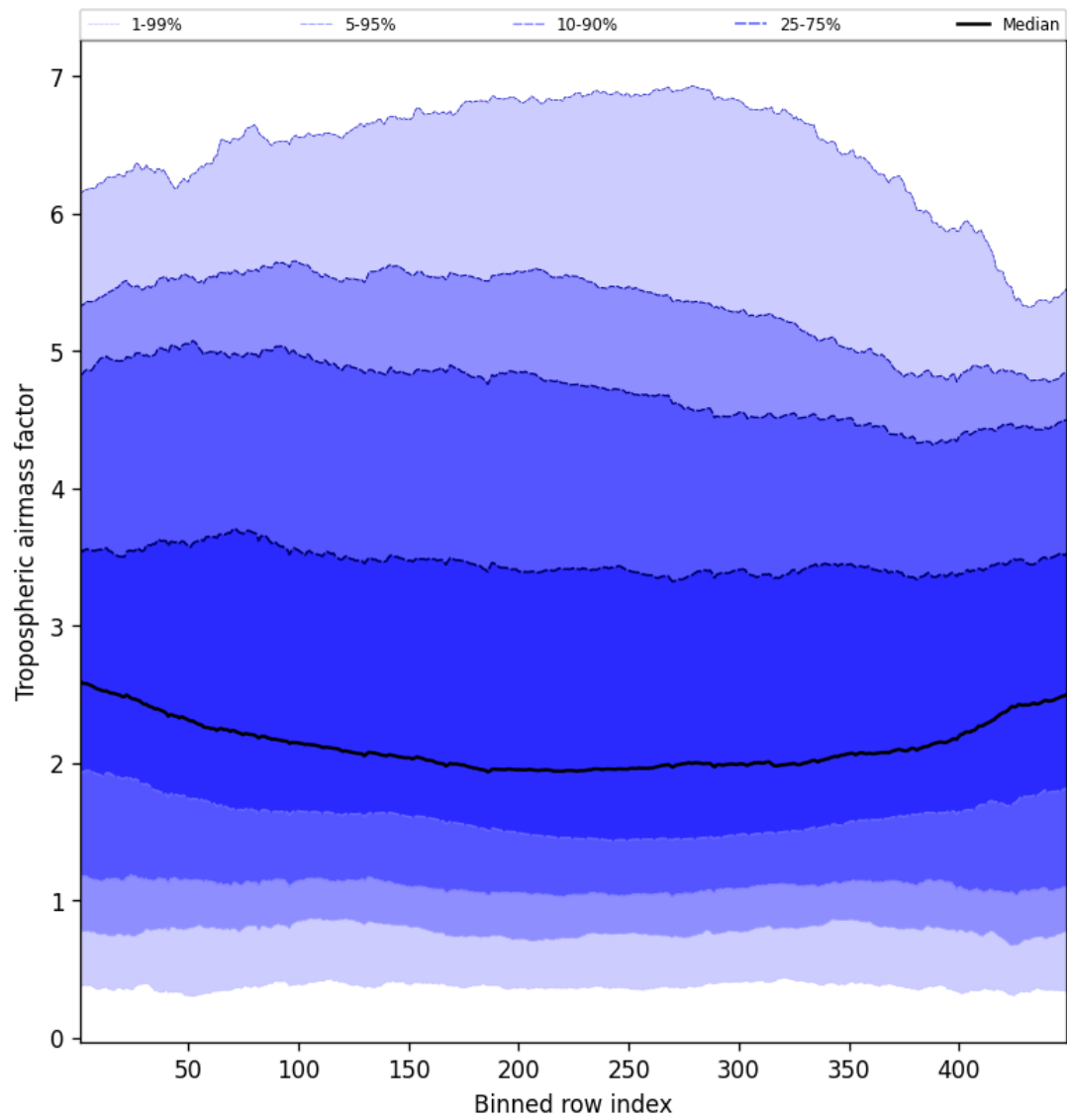
Figure 46: Along track statistics of “Tropospheric airmass factor” for 2025-03-24 to 2025-03-25
