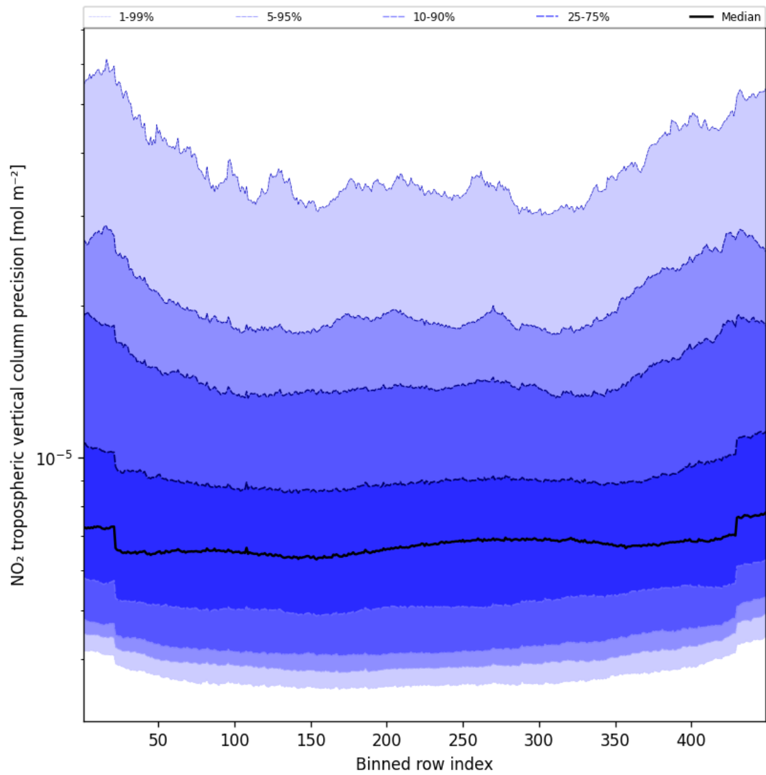
Figure 45: Along track statistics of “NO 2 tropospheric vertical column precision” for 2025-03-24 to 2025-03-25
