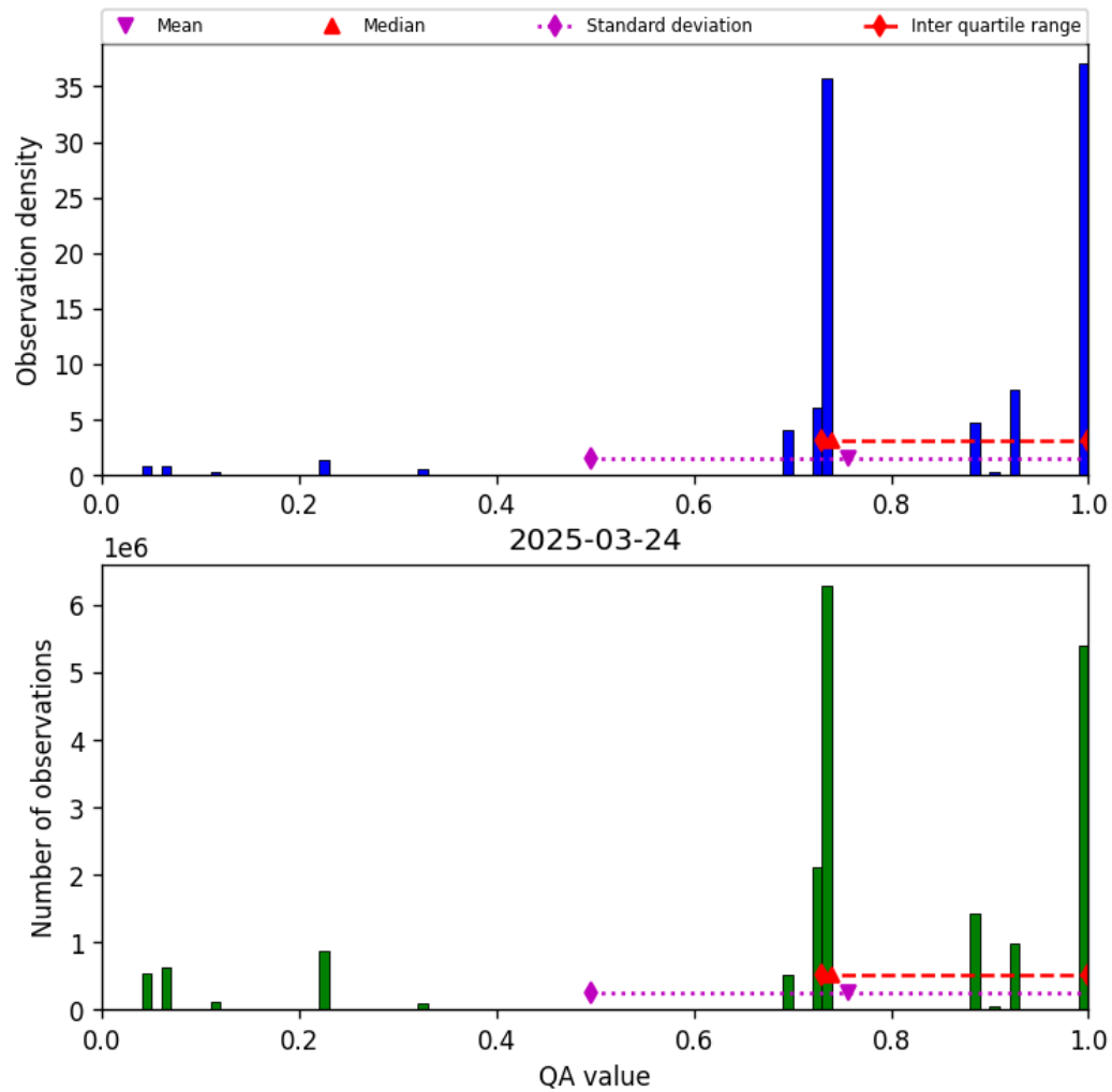
Figure 26: Histogram of “QA value” for 2025-03-24 to 2025-03-25
