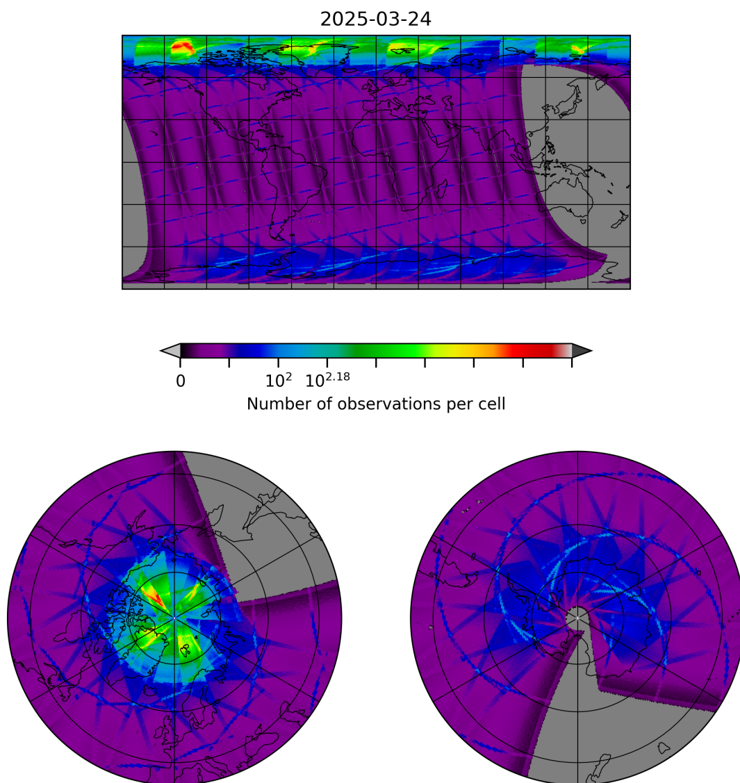
Figure 8: Map of the number of observations for 2025-03-24 to 2025-03-25
