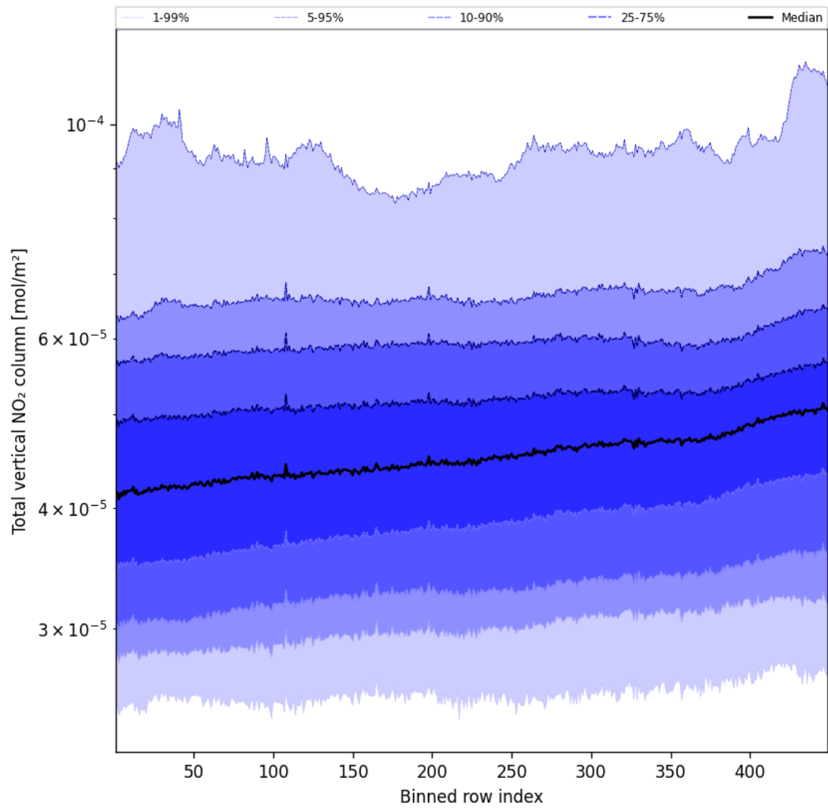
Figure 53: Along track statistics of “Total vertical NO 2 column” for 2025-03-24 to 2025-03-25
