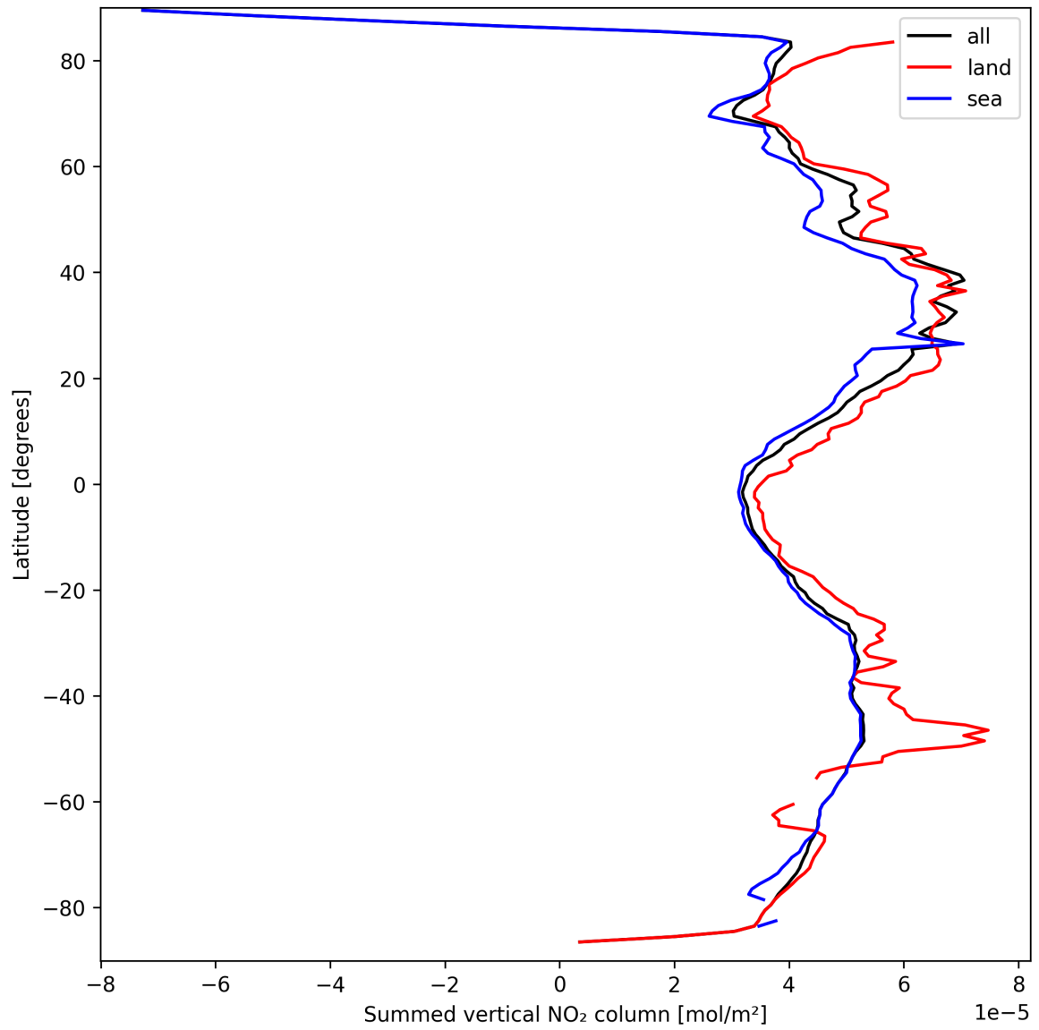
Figure 21: Zonal average of “Summed vertical NO 2 column” for 2025-03-24 to 2025-03-25.
