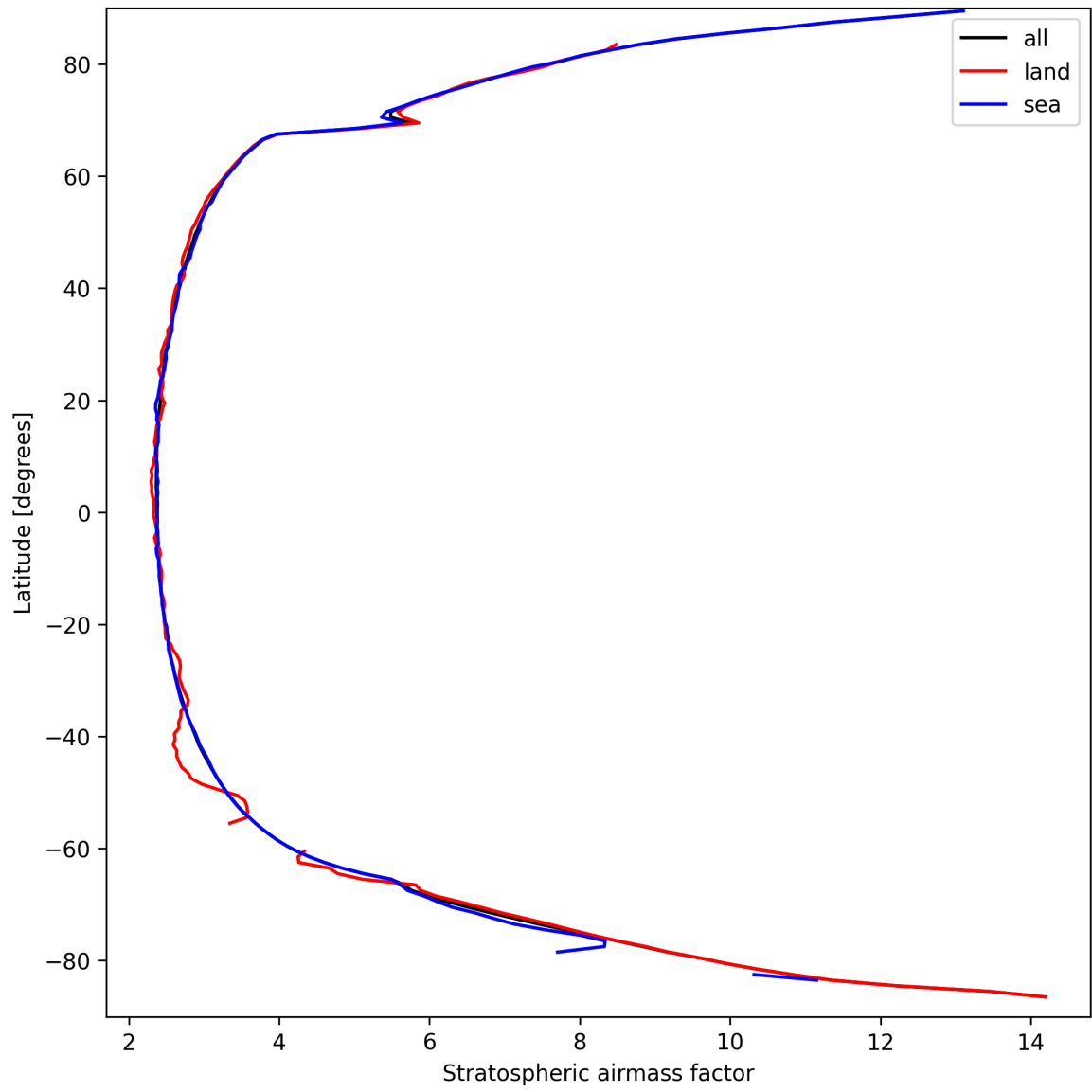
Figure 25: Zonal average of “Stratospheric airmass factor” for 2025-03-24 to 2025-03-25.
