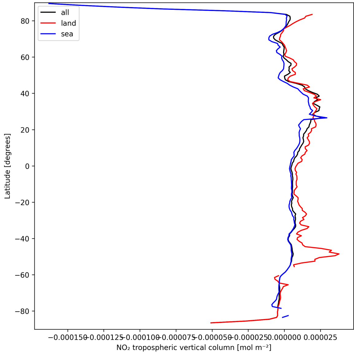
Figure 10: Zonal average of “NO 2 tropospheric vertical column” for 2025-03-24 to 2025-03-25.
