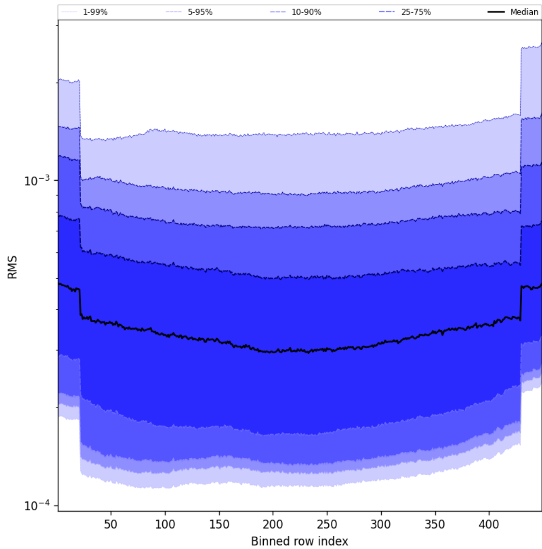
Figure 58: Along track statistics of “RMS” for 2025-03-24 to 2025-03-25
