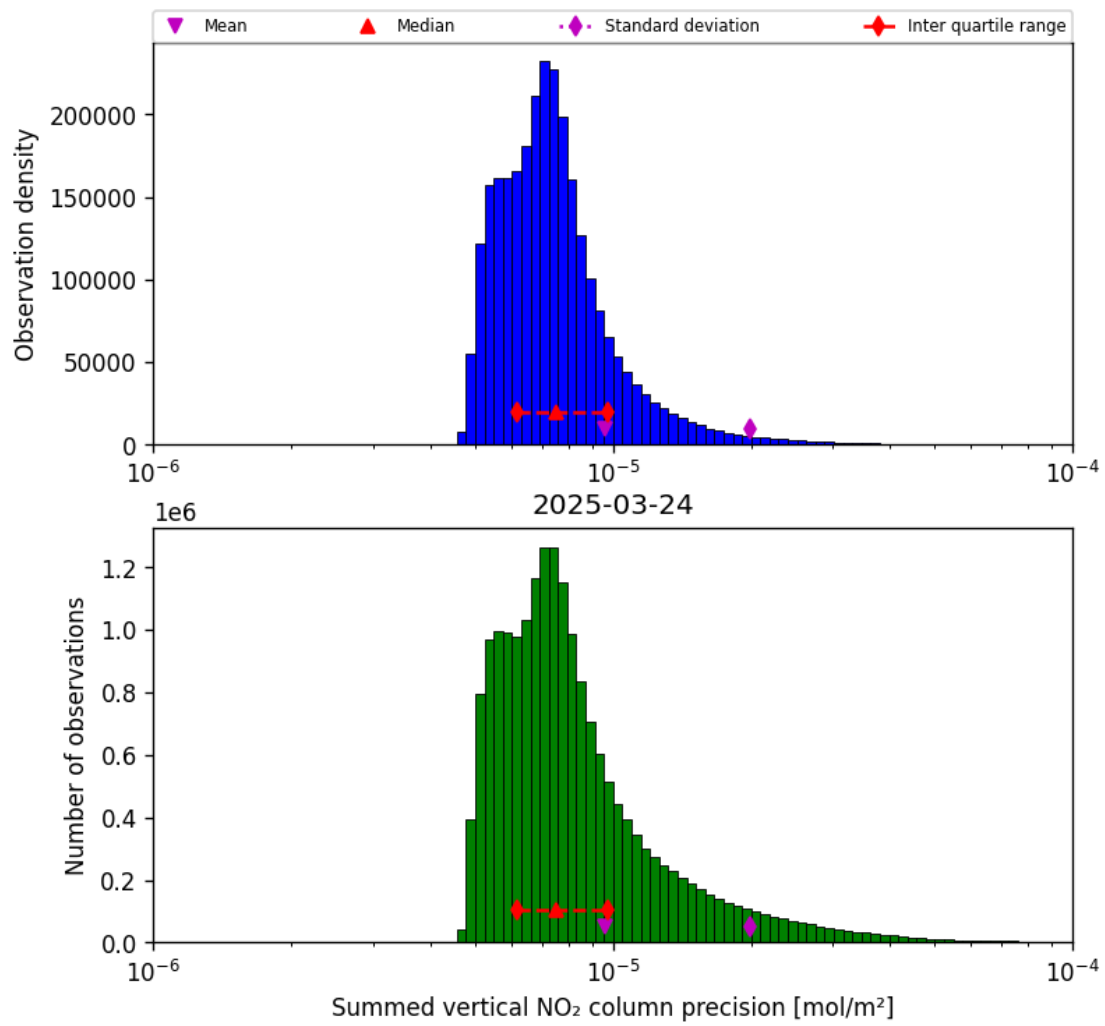
Figure 39: Histogram of “Summed vertical NO 2 column precision” for 2025-03-24 to 2025-03-25
