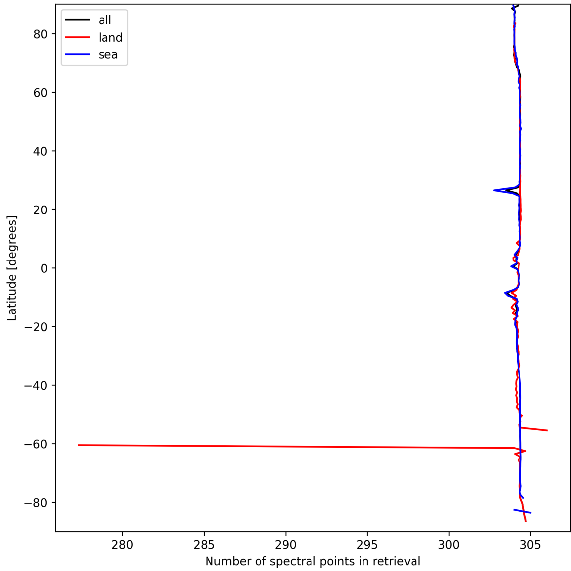
Figure 14: Zonal average of “Number of spectral points in retrieval” for 2025-03-24 to 2025-03-25.
