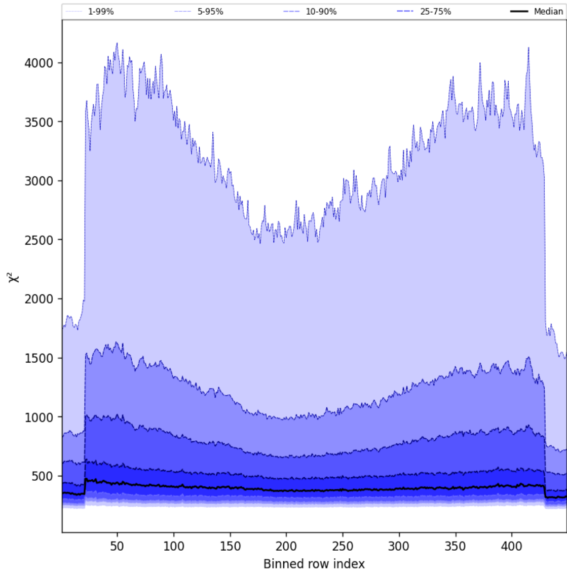
Figure 57: Along track statistics of “ \chi^2 ” for 2025-03-24 to 2025-03-25
