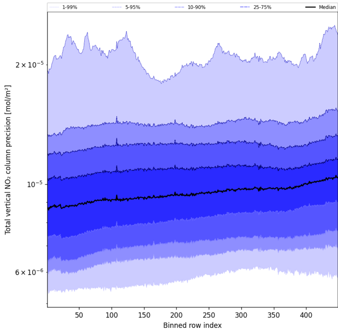
Figure 54: Along track statistics of “Total vertical NO 2 column precision” for 2025-03-24 to 2025-03-25
