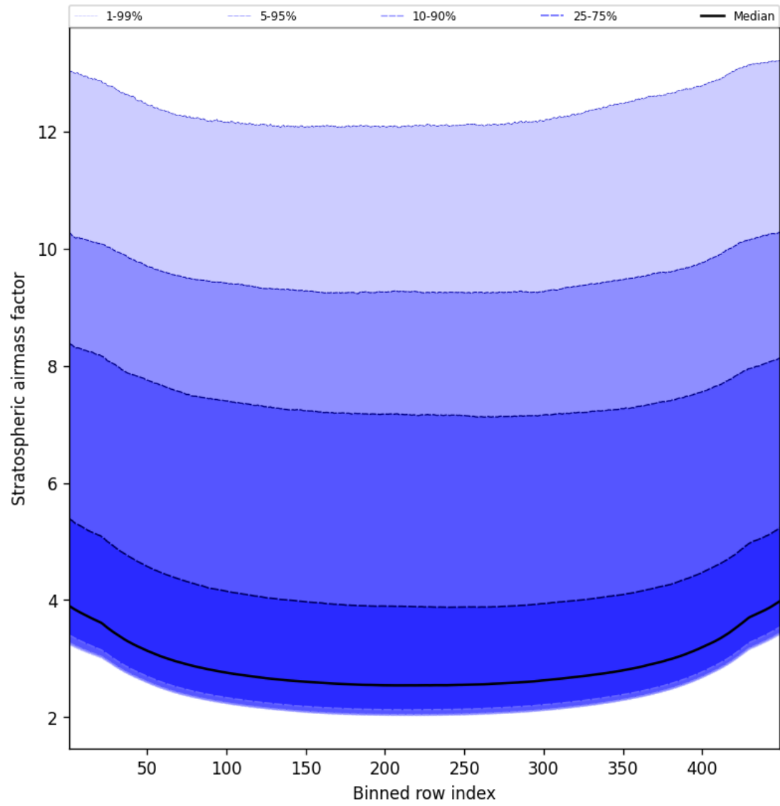
Figure 59: Along track statistics of “Stratospheric airmass factor” for 2025-03-24 to 2025-03-25
