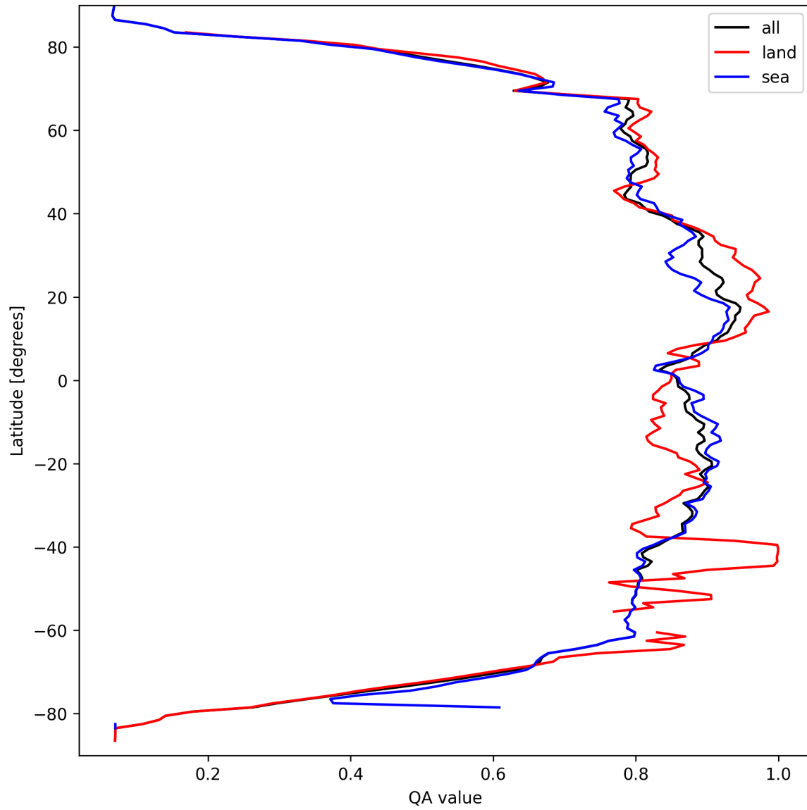
Figure 9: Zonal average of “QA value” for 2025-03-24 to 2025-03-25.
