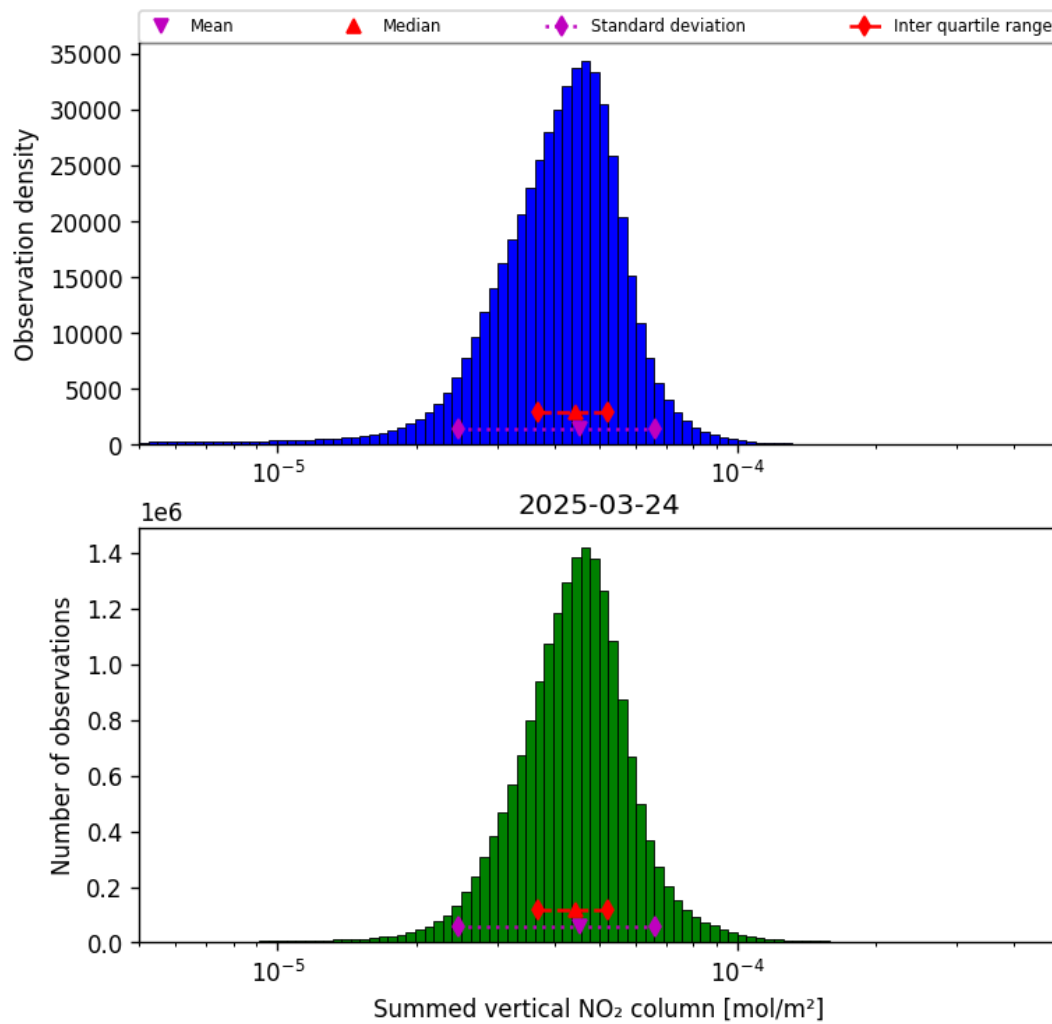
Figure 38: Histogram of "Summed vertical NO 2 column" for 2025-03-24 to 2025-03-25
