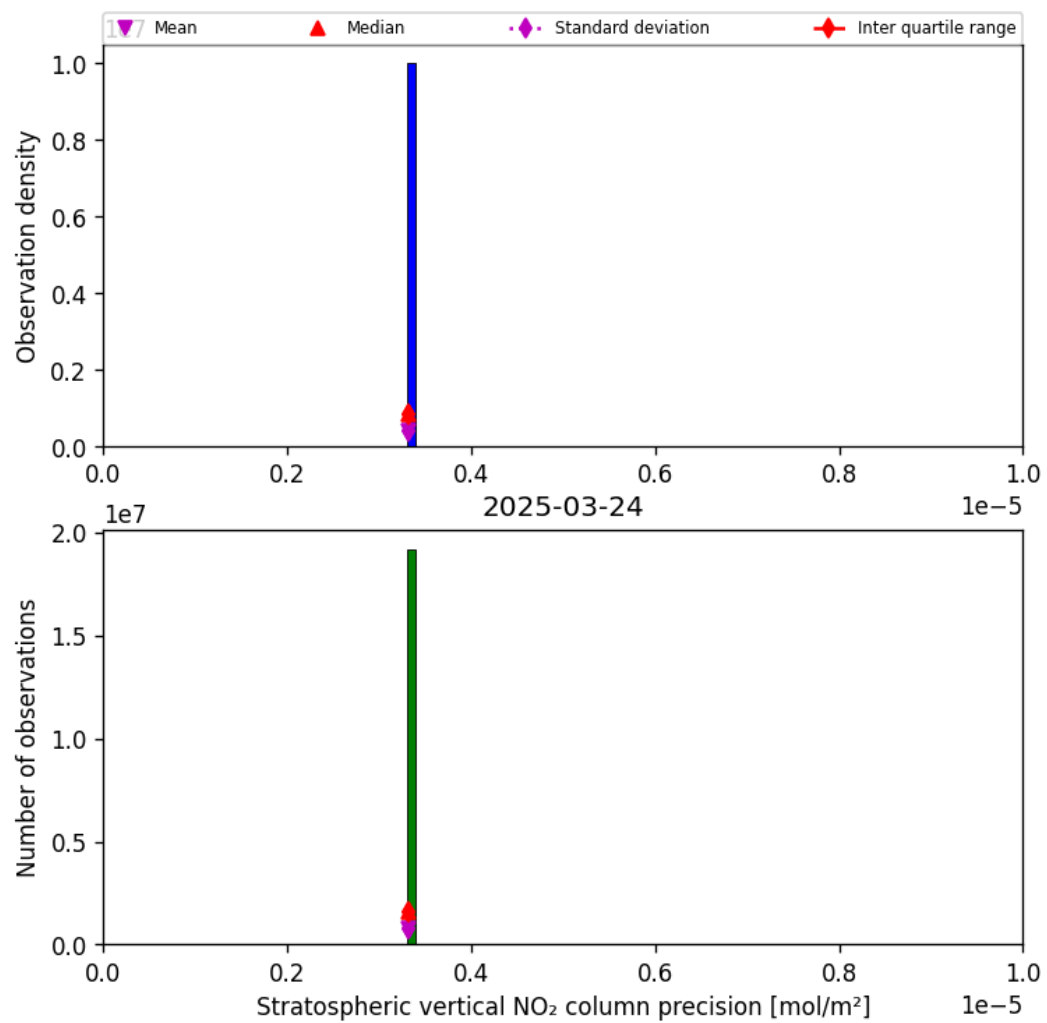
Figure 35: Histogram of “Stratospheric vertical NO 2 column precision” for 2025-03-24 to 2025-03-25
