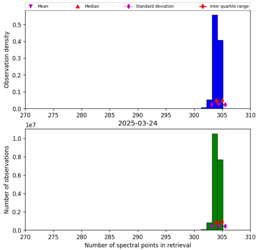
Figure 31: Histogram of “Number of spectral points in retrieval” for 2025-03-24 to 2025-03-25
