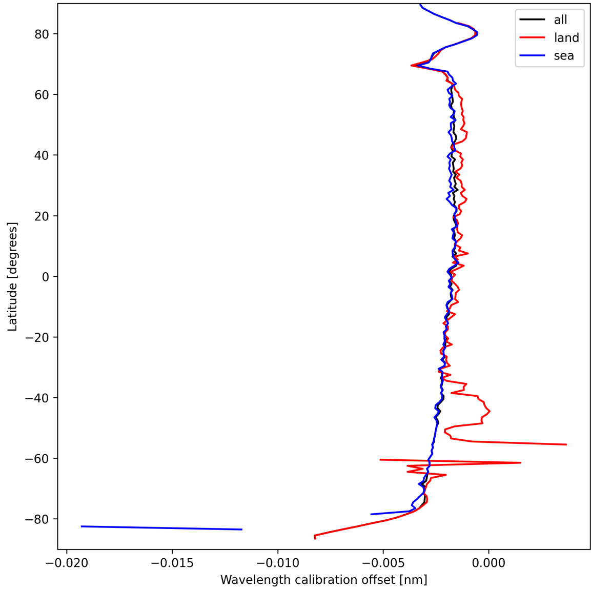
Figure 16: Zonal average of “Wavelength calibration offset” for 2025-03-24 to 2025-03-25.
