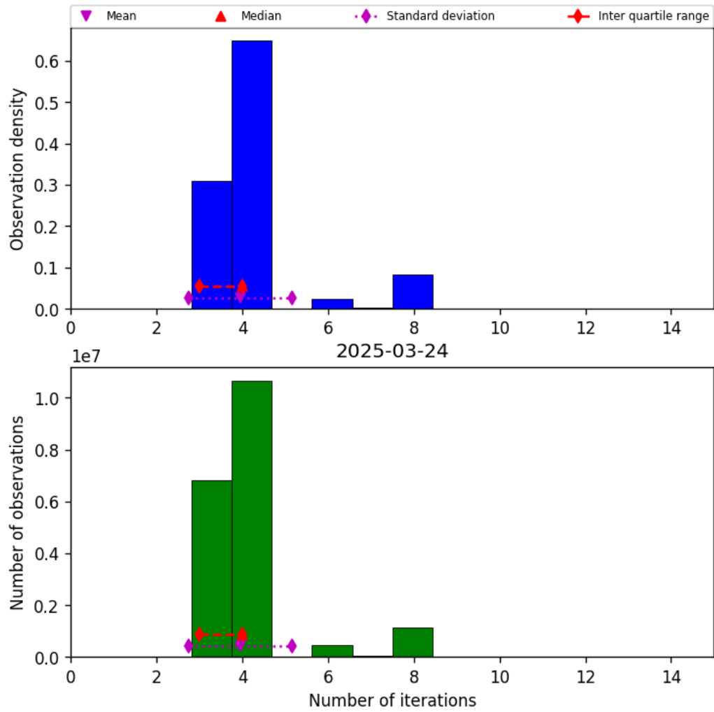
Figure 32: Histogram of “Number of iterations” for 2025-03-24 to 2025-03-25
