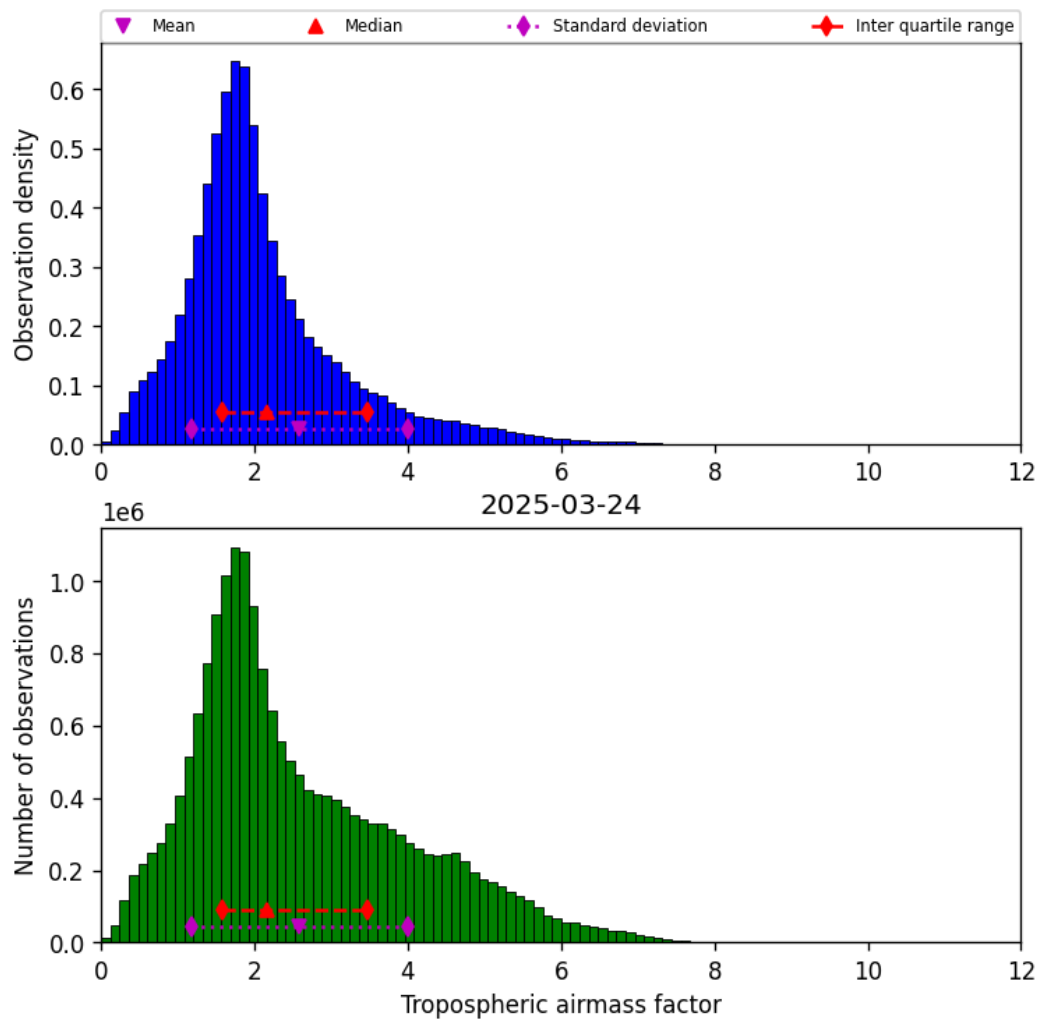
Figure 29: Histogram of “Tropospheric airmass factor” for 2025-03-24 to 2025-03-25
