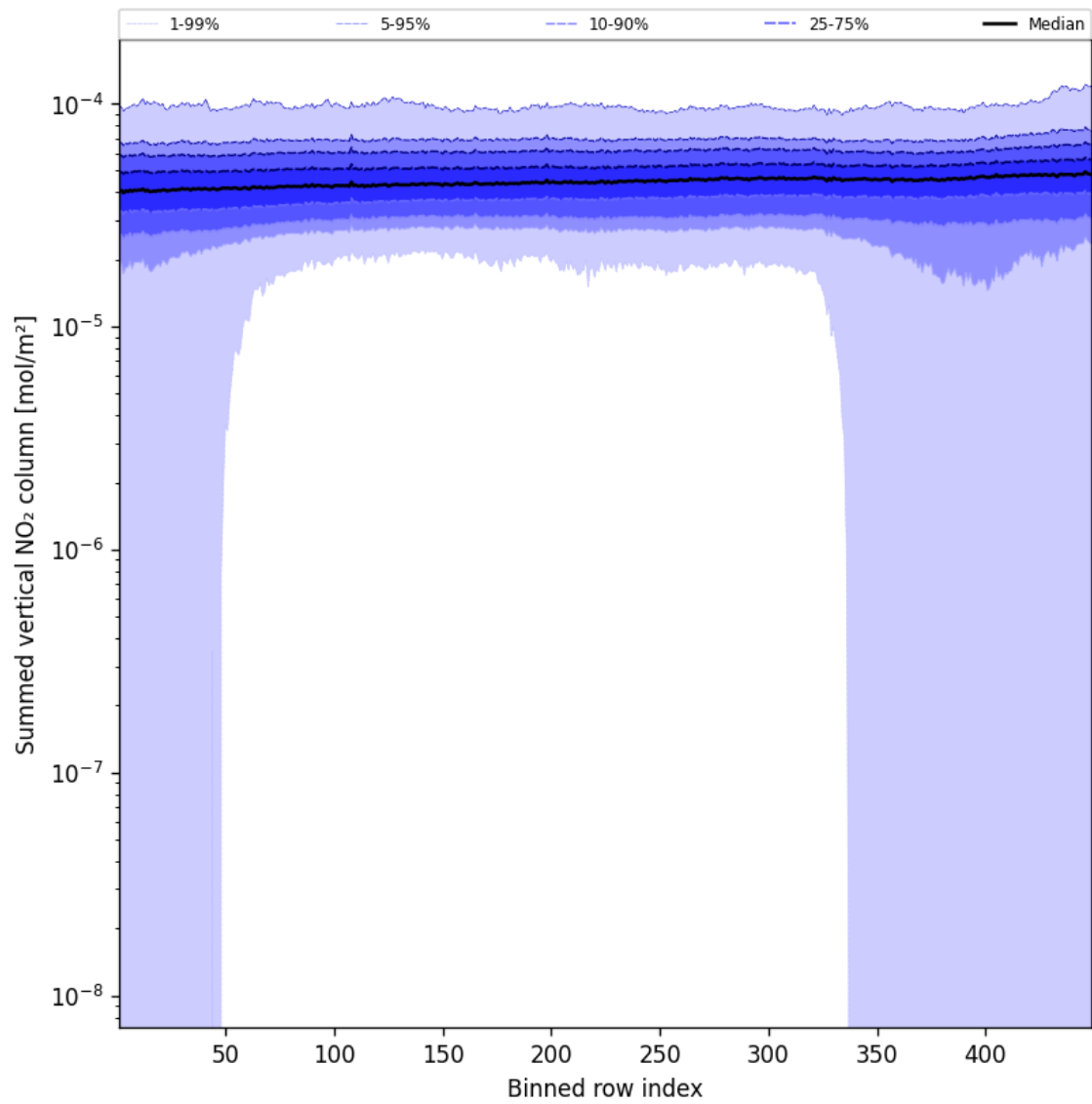
Figure 55: Along track statistics of “Summed vertical NO 2 column” for 2025-03-24 to 2025-03-25
