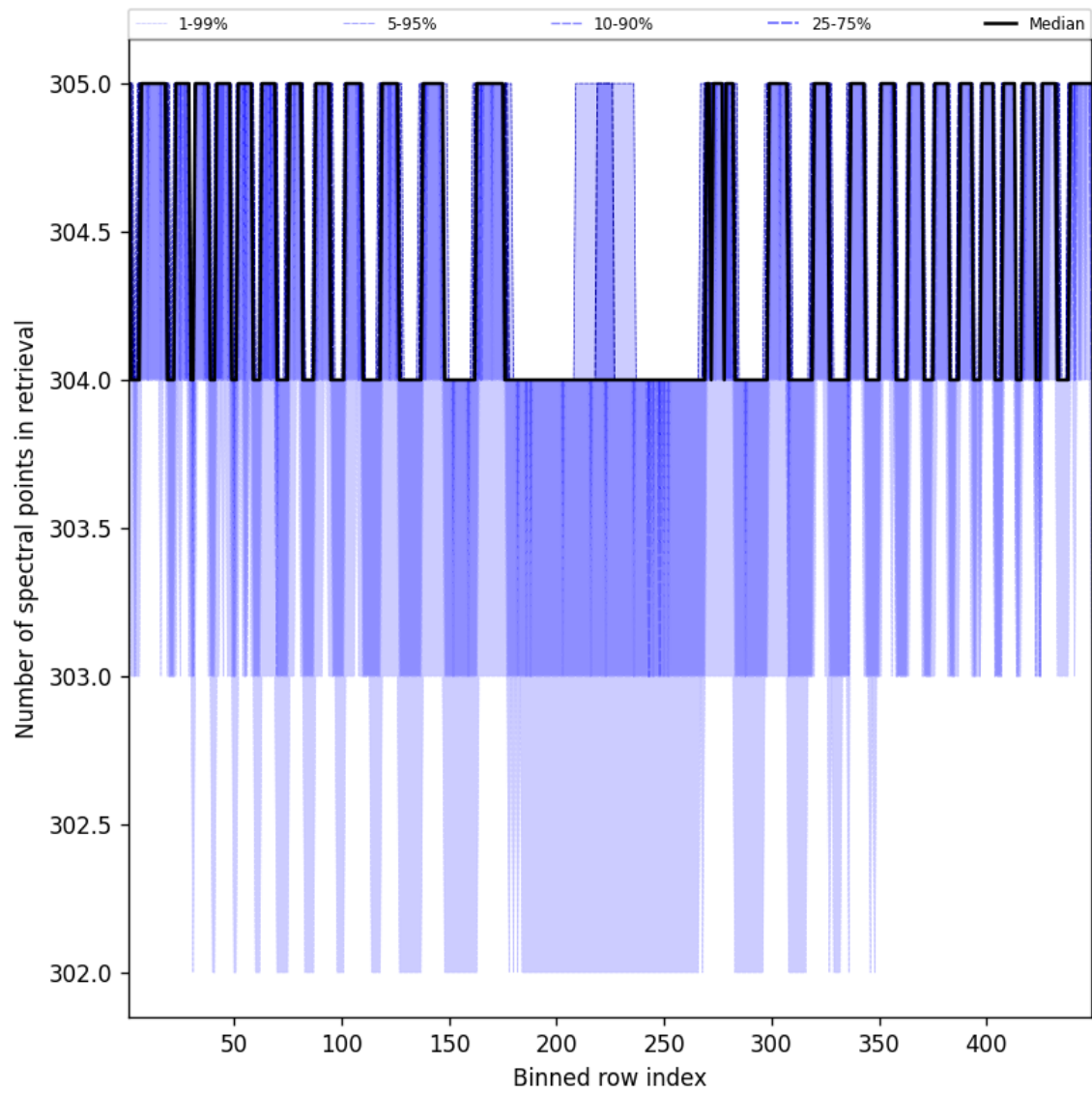
Figure 48: Along track statistics of “Number of spectral points in retrieval” for 2025-03-24 to 2025-03-25
