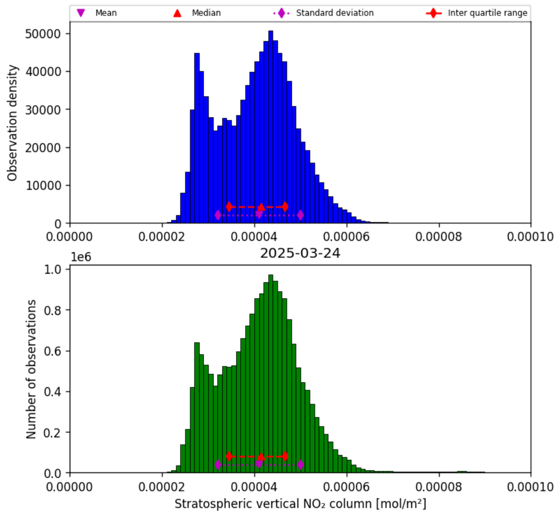
Figure 34: Histogram of “Stratospheric vertical NO 2 column” for 2025-03-24 to 2025-03-25
