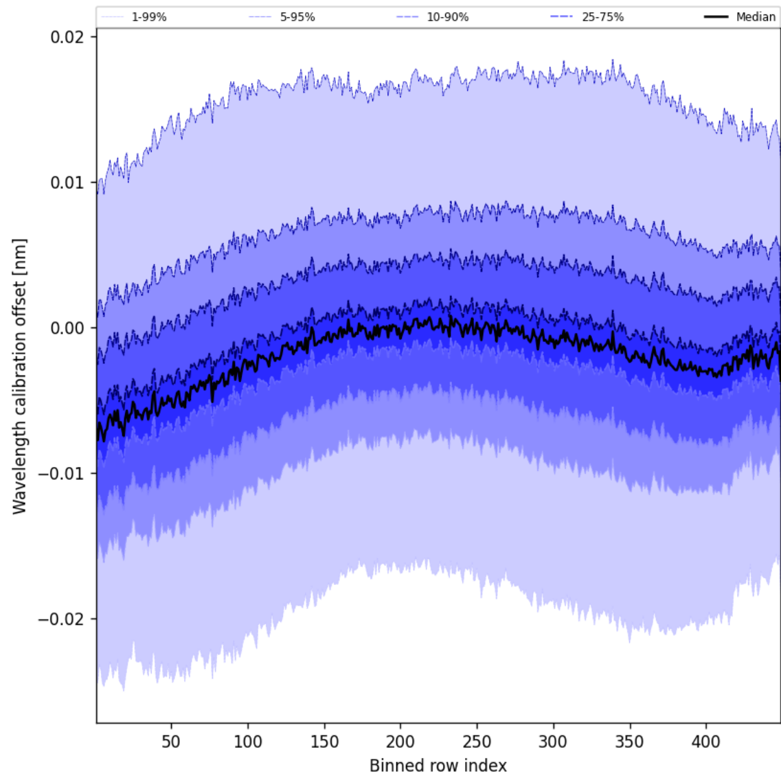
Figure 50: Along track statistics of “Wavelength calibration offset” for 2025-03-24 to 2025-03-25
