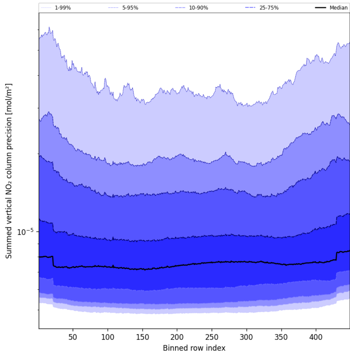
Figure 56: Along track statistics of “Summed vertical NO 2 column precision” for 2025-03-24 to 2025-03-25
