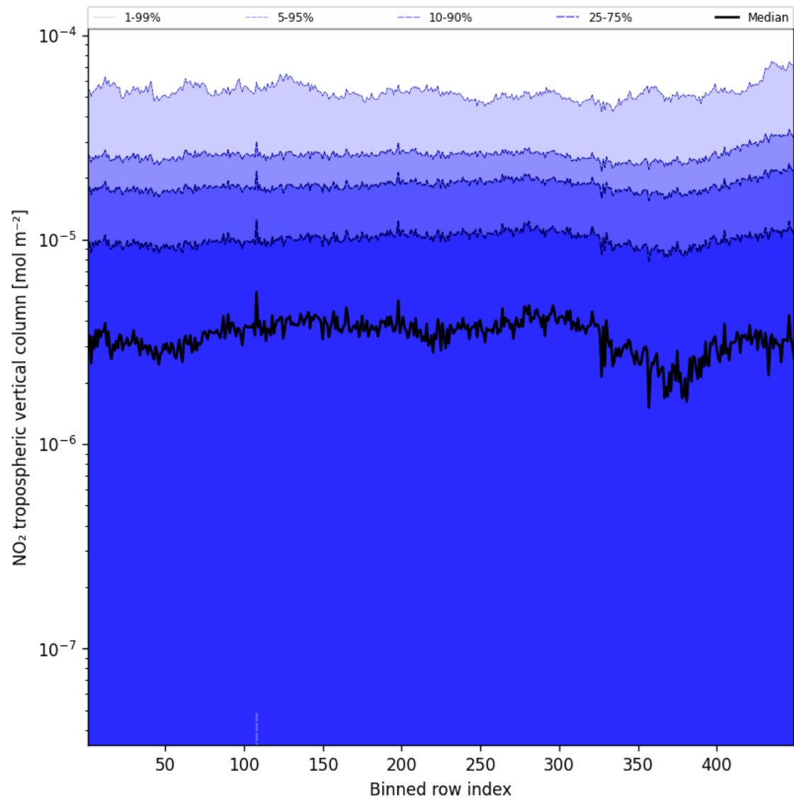
Figure 44: Along track statistics of “NO 2 tropospheric vertical column” for 2025-03-24 to 2025-03-25
