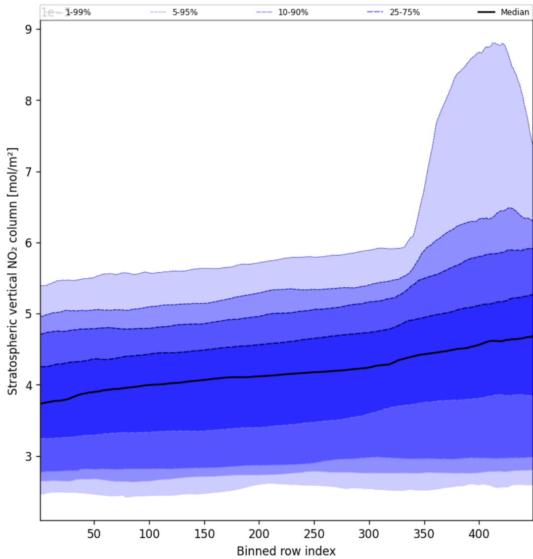
Figure 51: Along track statistics of “Stratospheric vertical NO 2 column” for 2025-03-24 to 2025-03-25
