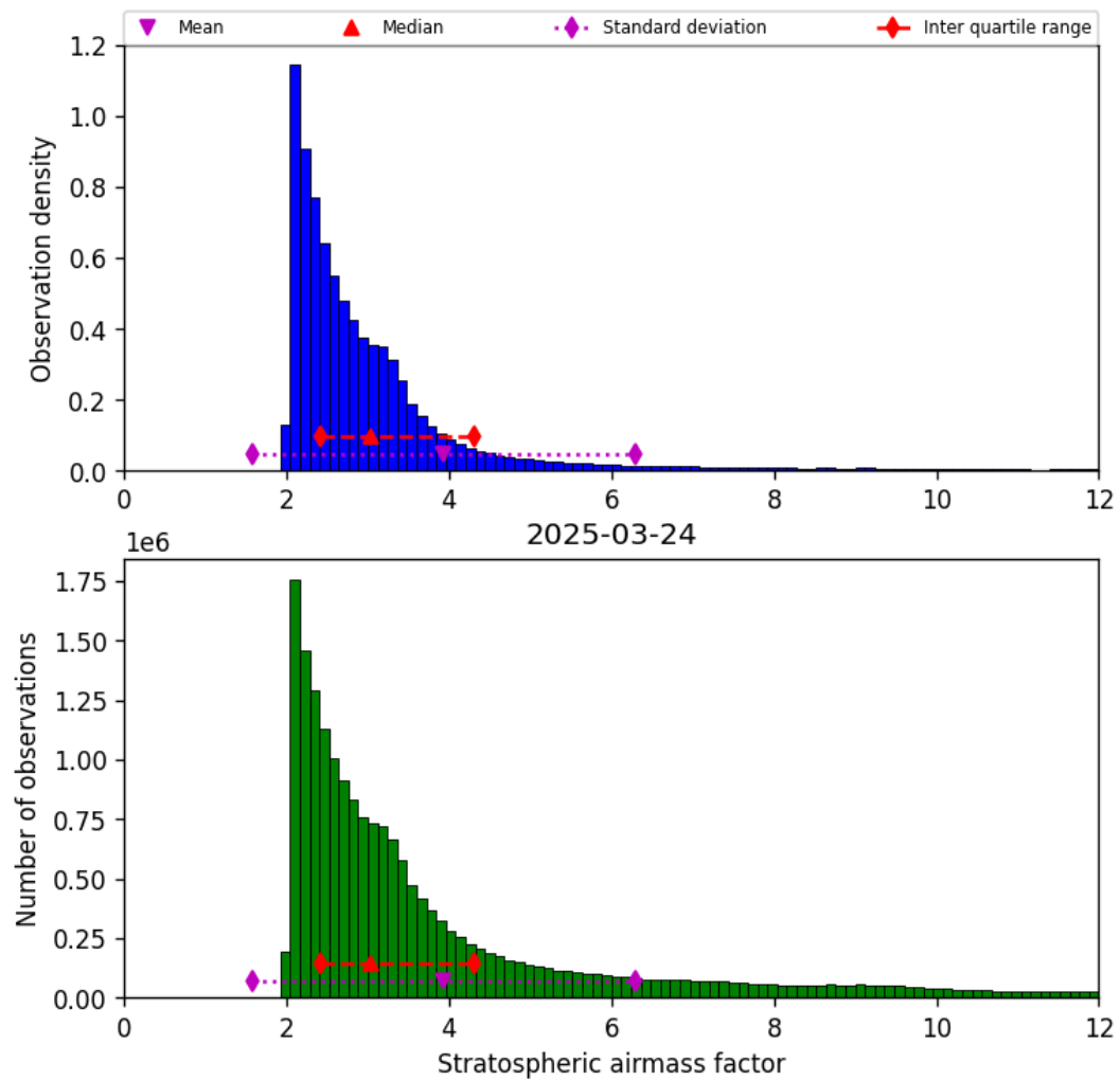
Figure 42: Histogram of “Stratospheric airmass factor” for 2025-03-24 to 2025-03-25
