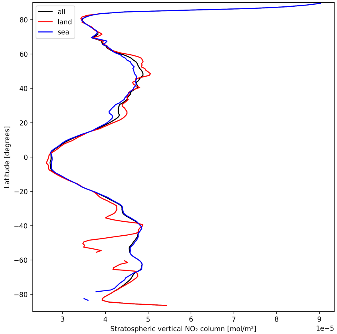
Figure 17: Zonal average of “Stratospheric vertical NO 2 column” for 2025-03-24 to 2025-03-25.
