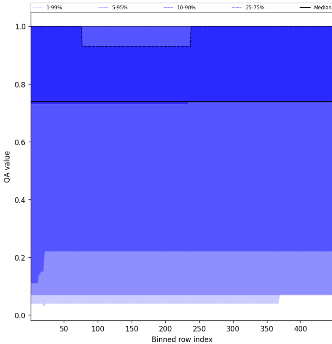
Figure 43: Along track statistics of “QA value” for 2025-03-24 to 2025-03-25
