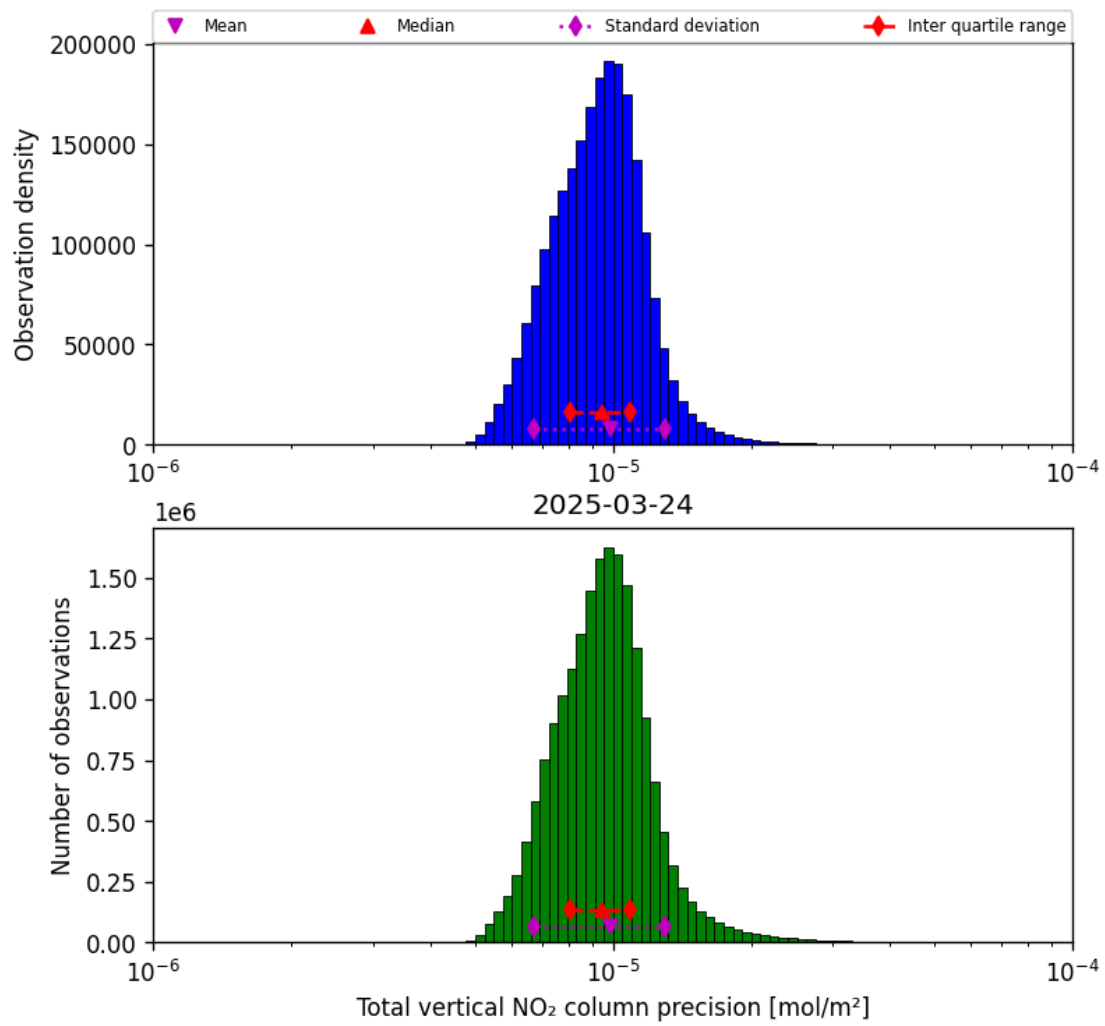
Figure 37: Histogram of “Total vertical NO 2 column precision” for 2025-03-24 to 2025-03-25
