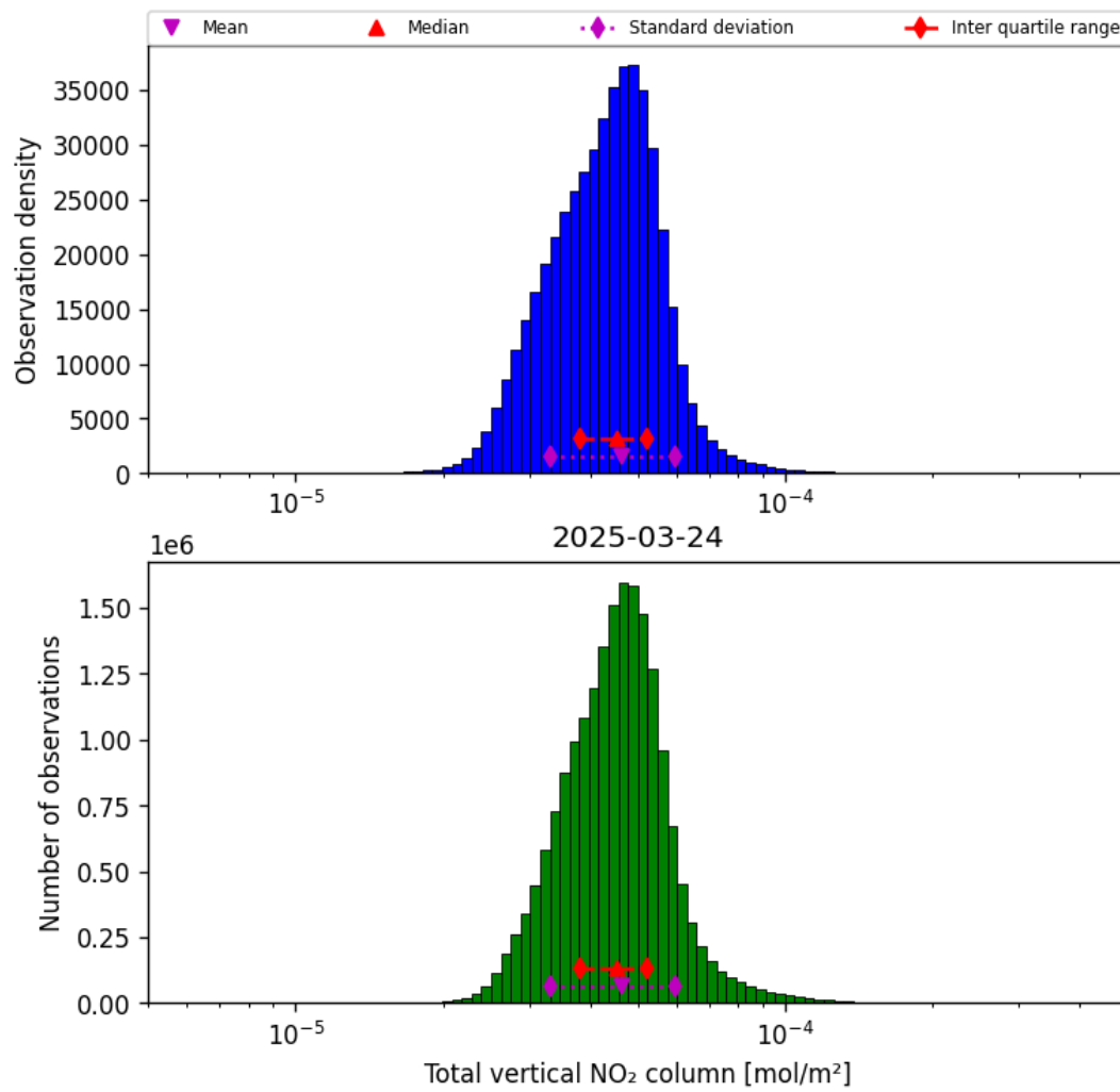
Figure 36: Histogram of “Total vertical NO 2 column” for 2025-03-24 to 2025-03-25
