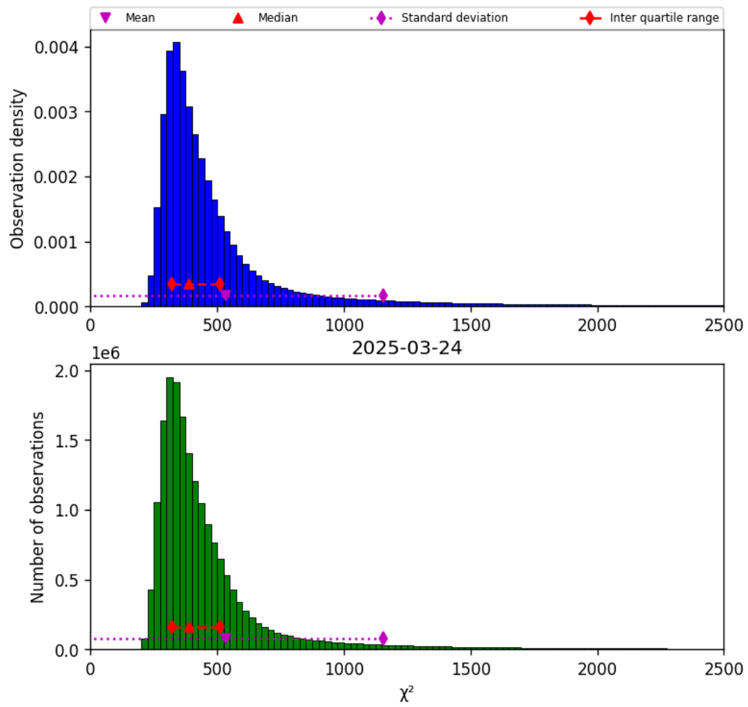
Figure 40: Histogram of “ \chi^2 ” for 2025-03-24 to 2025-03-25
