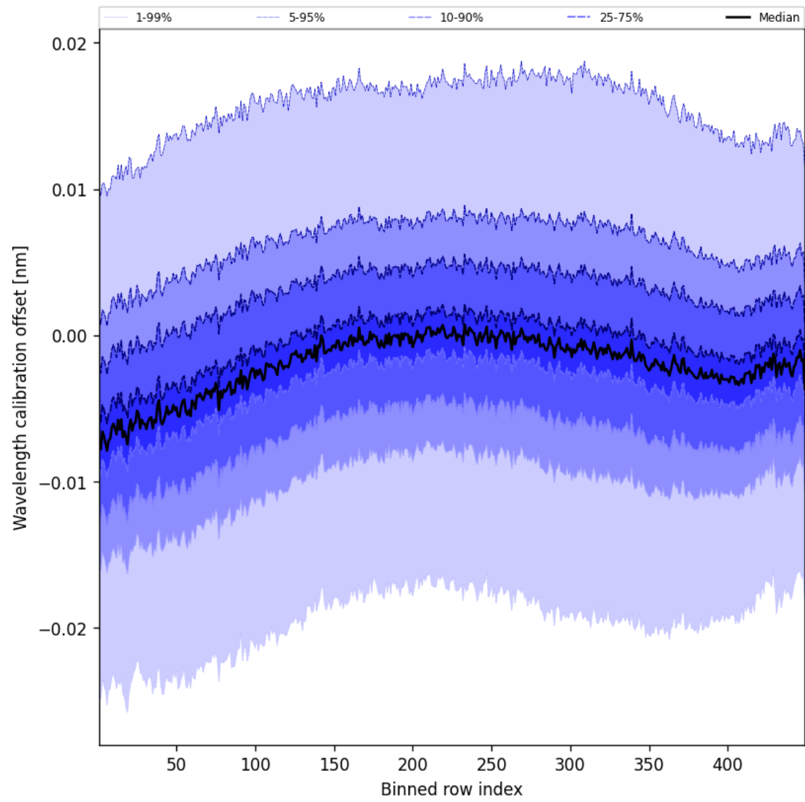
Figure 50: Along track statistics of “Wavelength calibration offset” for 2025-03-25 to 2025-03-26
