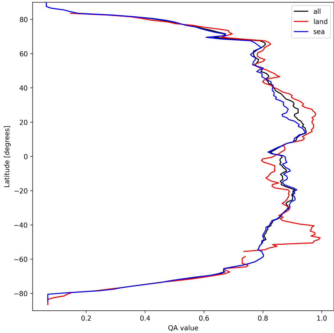
Figure 9: Zonal average of “QA value” for 2025-03-25 to 2025-03-26.
