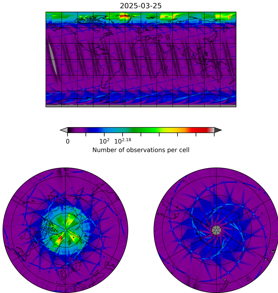
Figure 8: Map of the number of observations for 2025-03-25 to 2025-03-26
