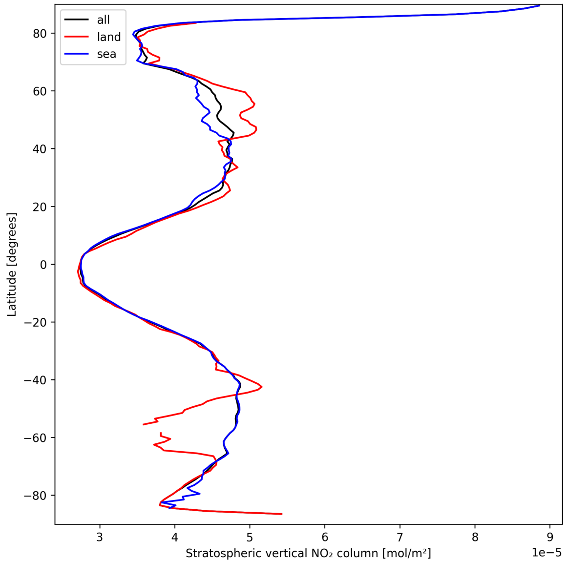
Figure 17: Zonal average of “Stratospheric vertical NO 2 column” for 2025-03-25 to 2025-03-26.
