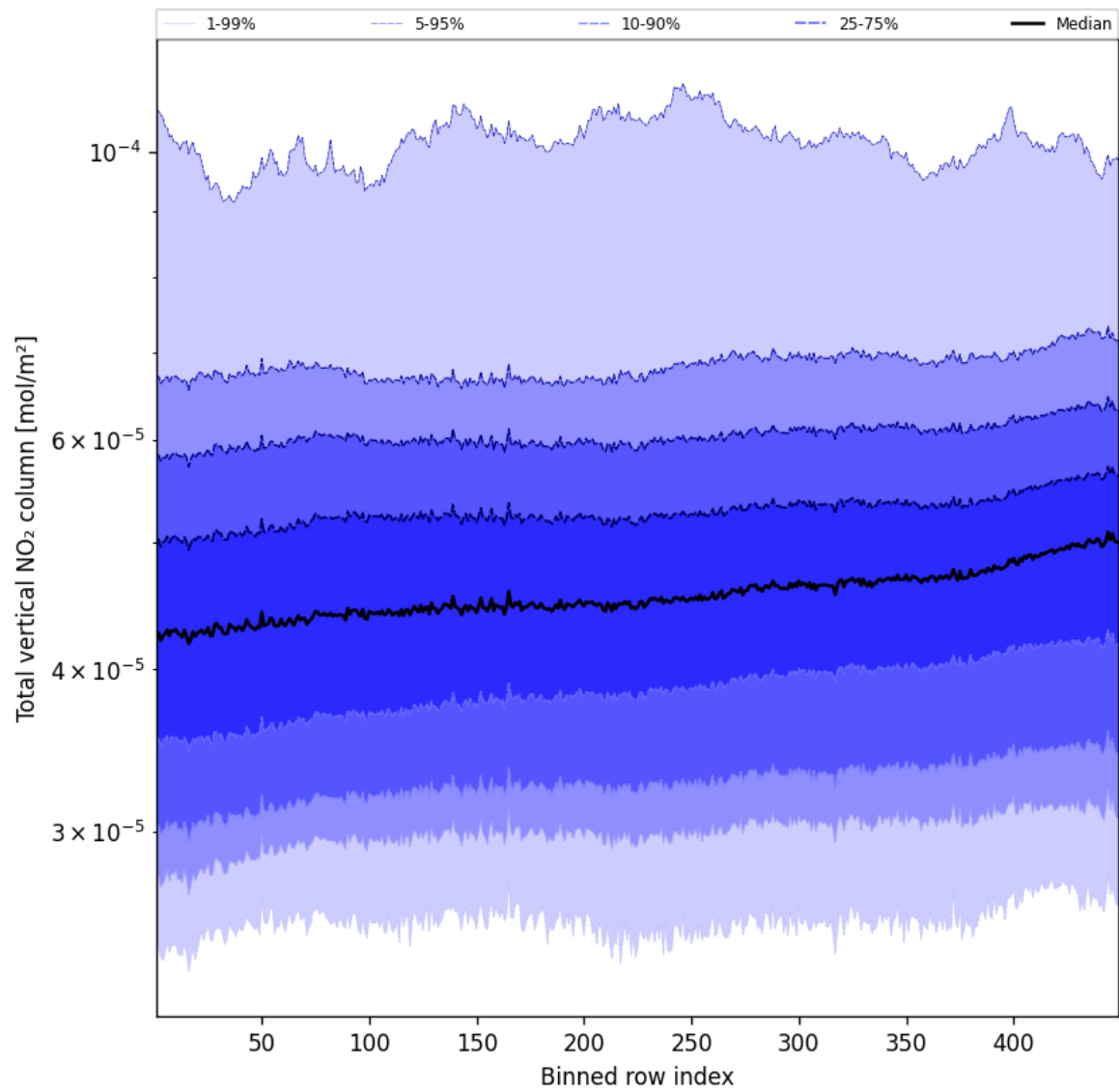
Figure 53: Along track statistics of “Total vertical NO 2 column” for 2025-03-25 to 2025-03-26
