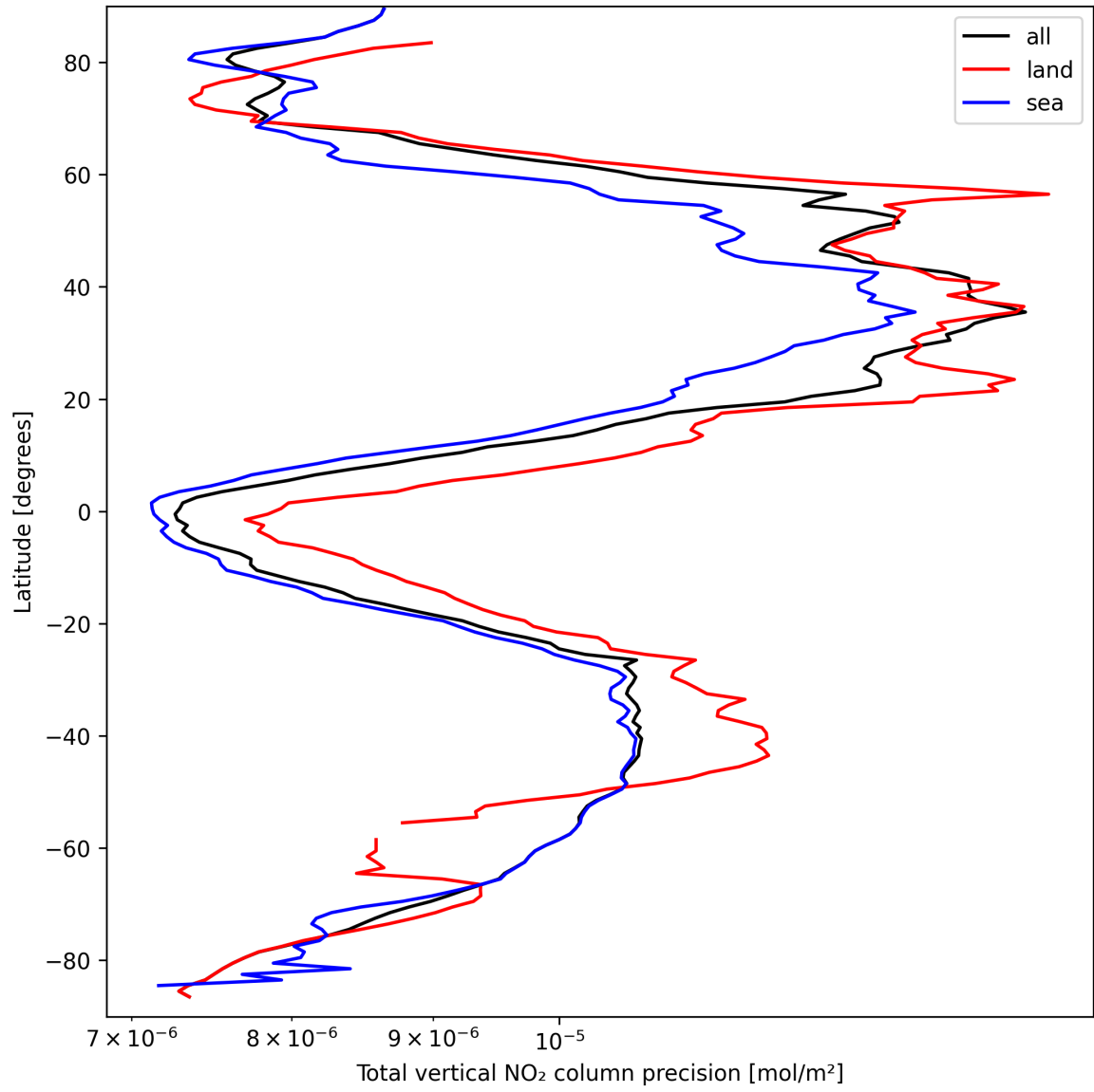
Figure 20: Zonal average of “Total vertical NO 2 column precision” for 2025-03-25 to 2025-03-26.
