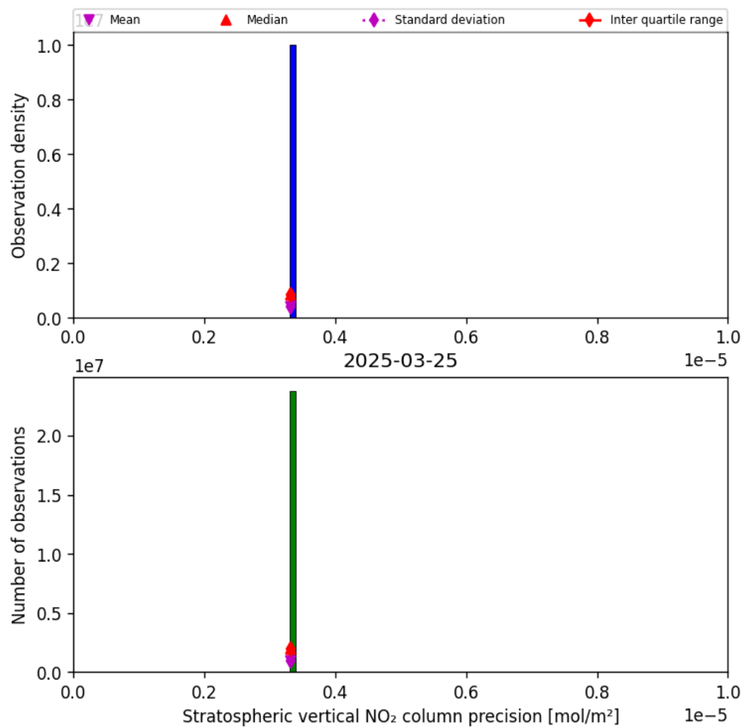
Figure 35: Histogram of “Stratospheric vertical NO 2 column precision” for 2025-03-25 to 2025-03-26
