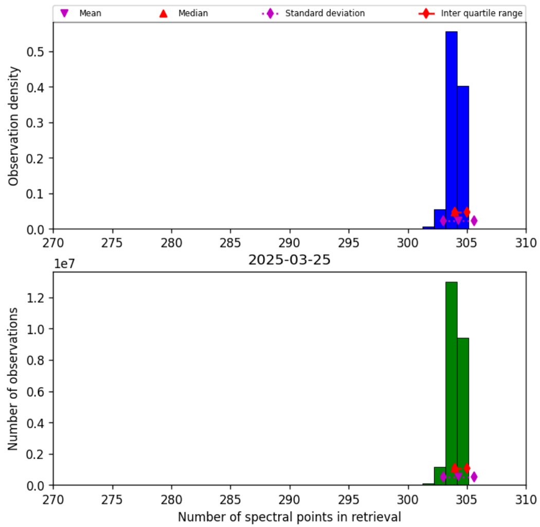
Figure 31: Histogram of “Number of spectral points in retrieval” for 2025-03-25 to 2025-03-26
