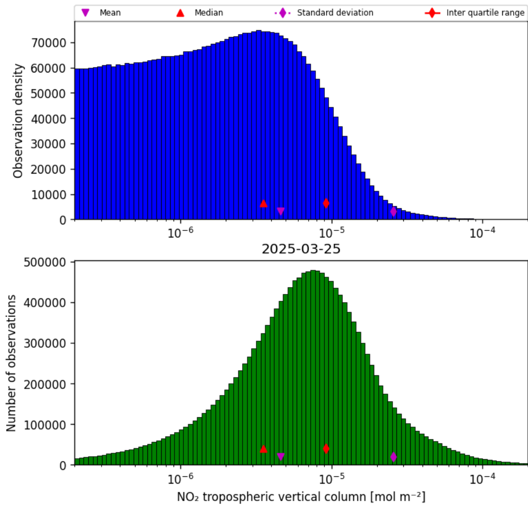
Figure 27: Histogram of “NO 2 tropospheric vertical column” for 2025-03-25 to 2025-03-26
