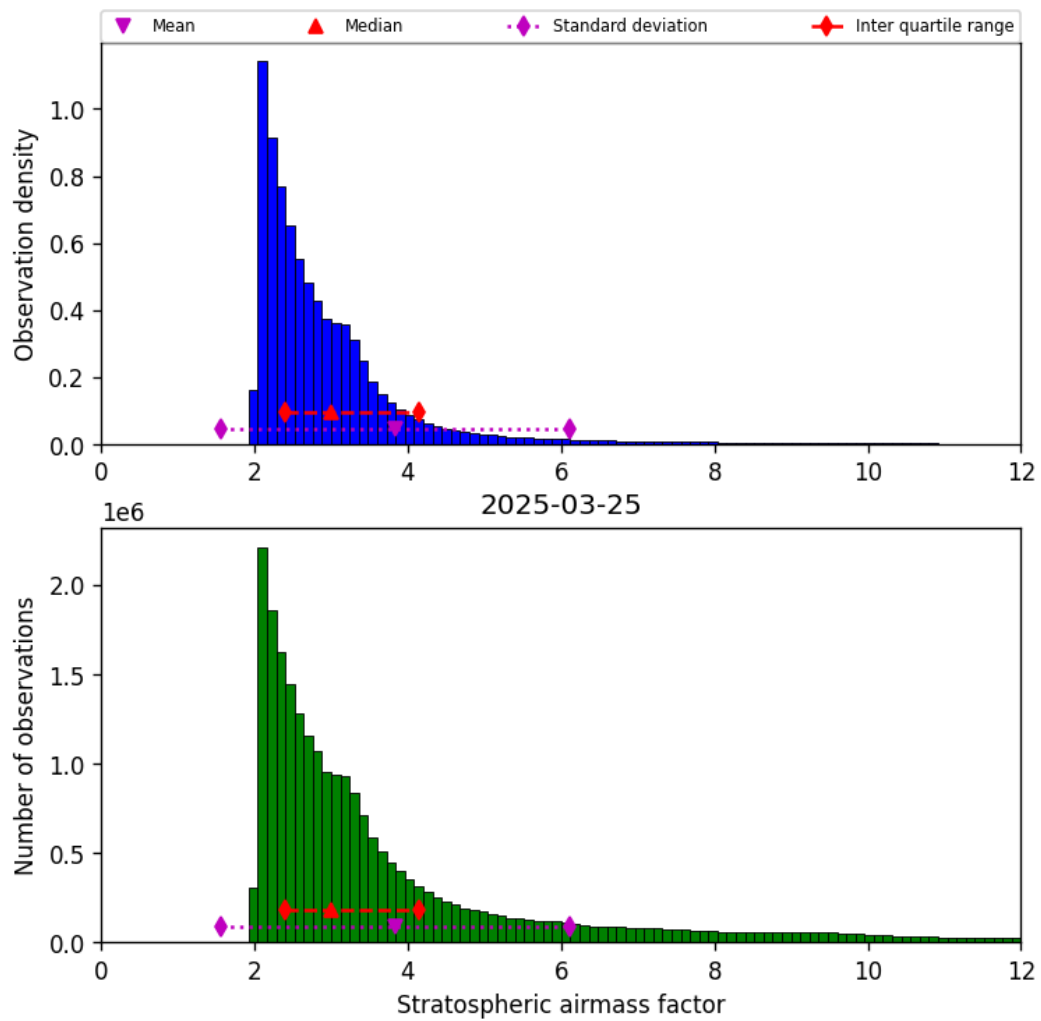
Figure 42: Histogram of “Stratospheric airmass factor” for 2025-03-25 to 2025-03-26
