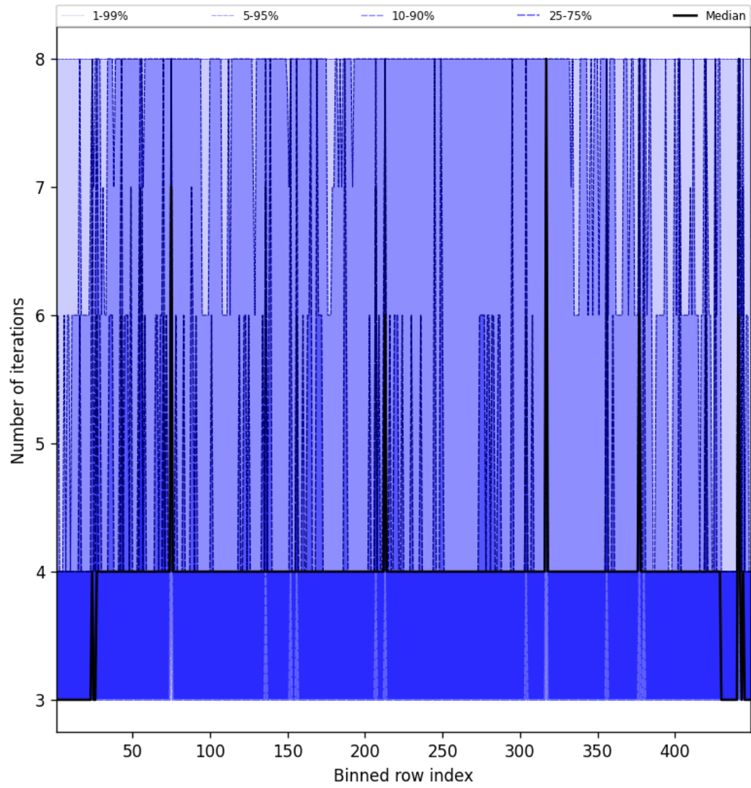
Figure 49: Along track statistics of “Number of iterations” for 2025-03-25 to 2025-03-26
