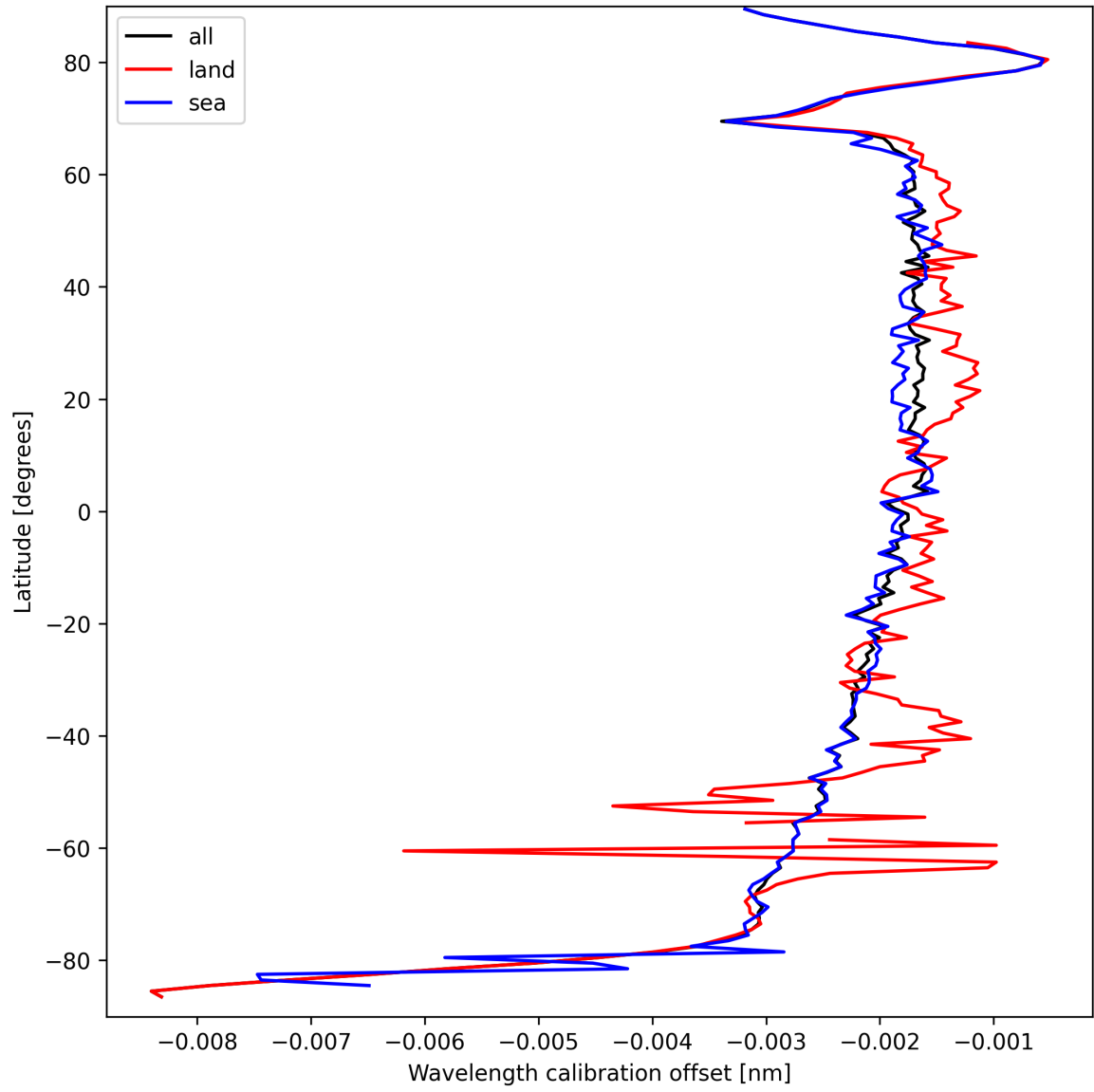
Figure 16: Zonal average of “Wavelength calibration offset” for 2025-03-25 to 2025-03-26.
