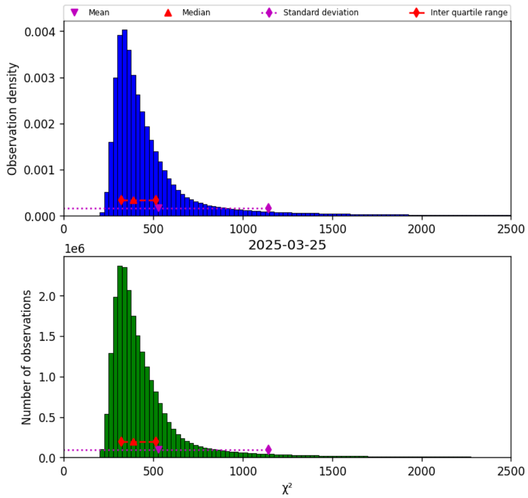
Figure 40: Histogram of “ \chi^2 ” for 2025-03-25 to 2025-03-26
