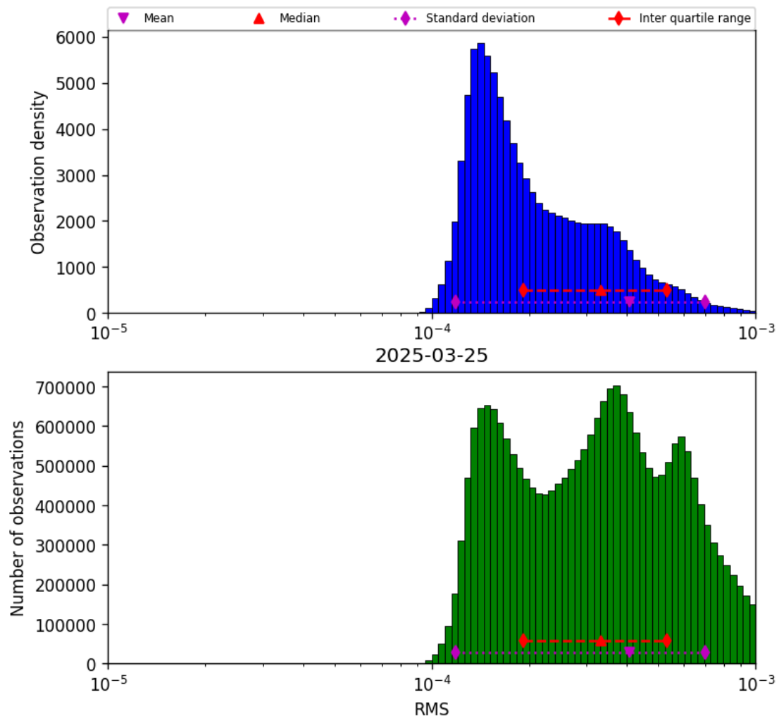
Figure 41: Histogram of “RMS” for 2025-03-25 to 2025-03-26
