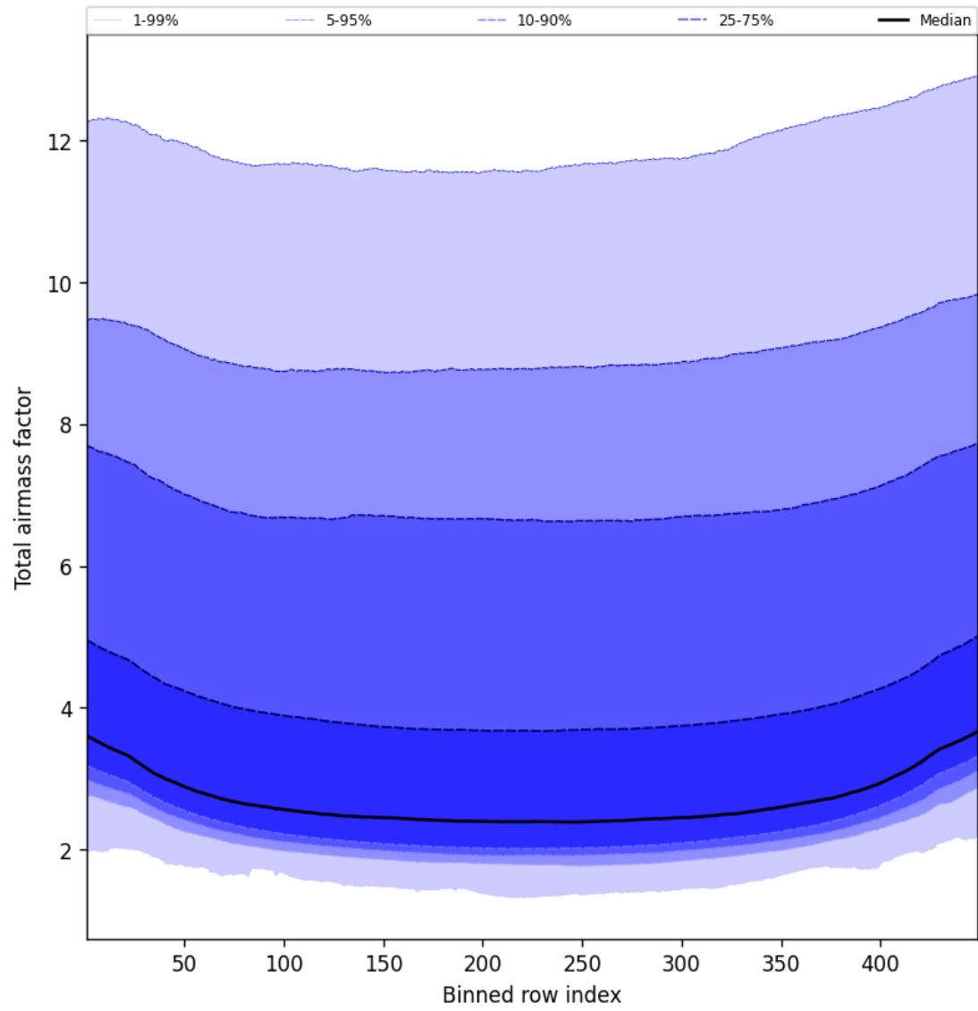
Figure 47: Along track statistics of “Total airmass factor” for 2025-03-25 to 2025-03-26
