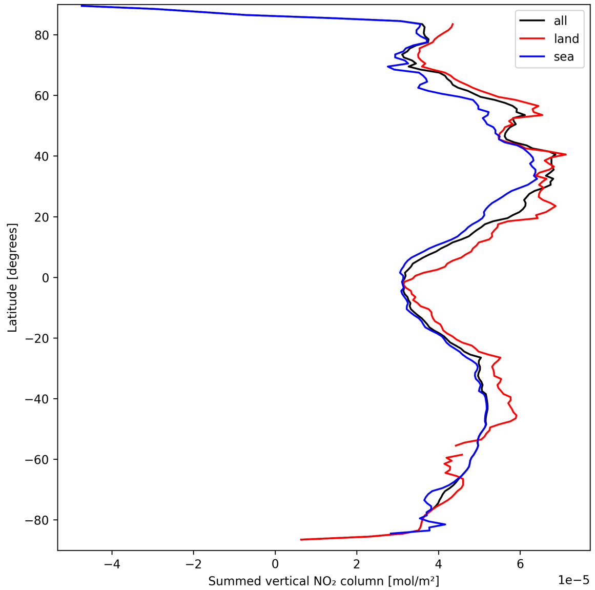
Figure 21: Zonal average of “Summed vertical NO 2 column” for 2025-03-25 to 2025-03-26.
