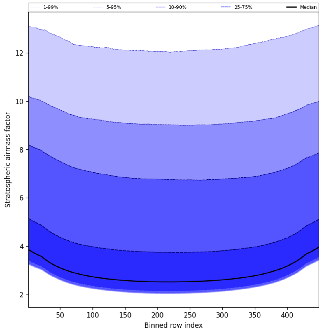
Figure 59: Along track statistics of “Stratospheric airmass factor” for 2025-03-25 to 2025-03-26
