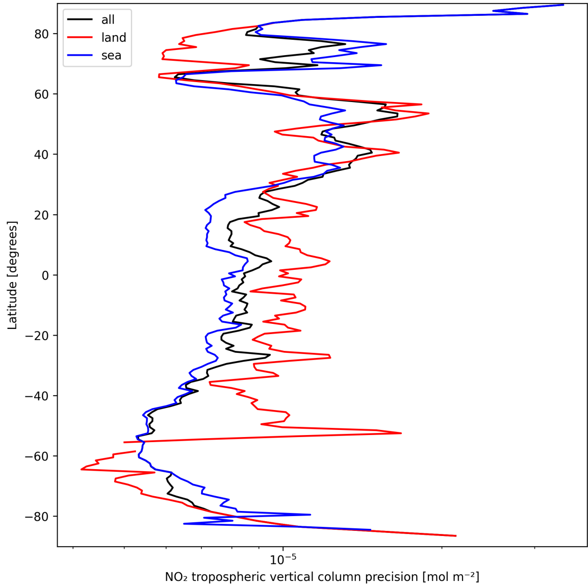
Figure 11: Zonal average of “NO 2 tropospheric vertical column precision” for 2025-03-25 to 2025-03-26.
