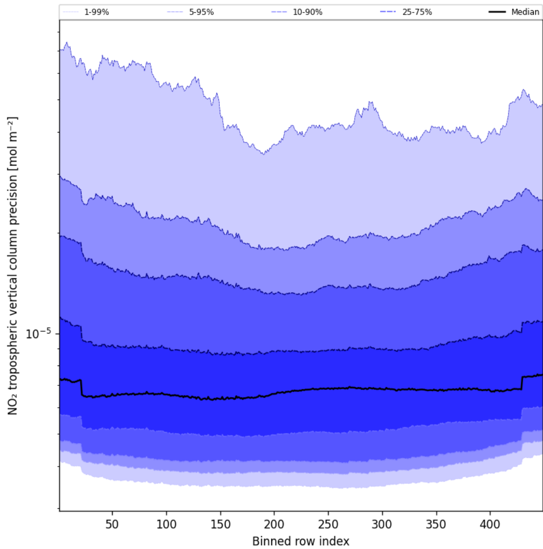
Figure 45: Along track statistics of “NO 2 tropospheric vertical column precision” for 2025-03-25 to 2025-03-26
