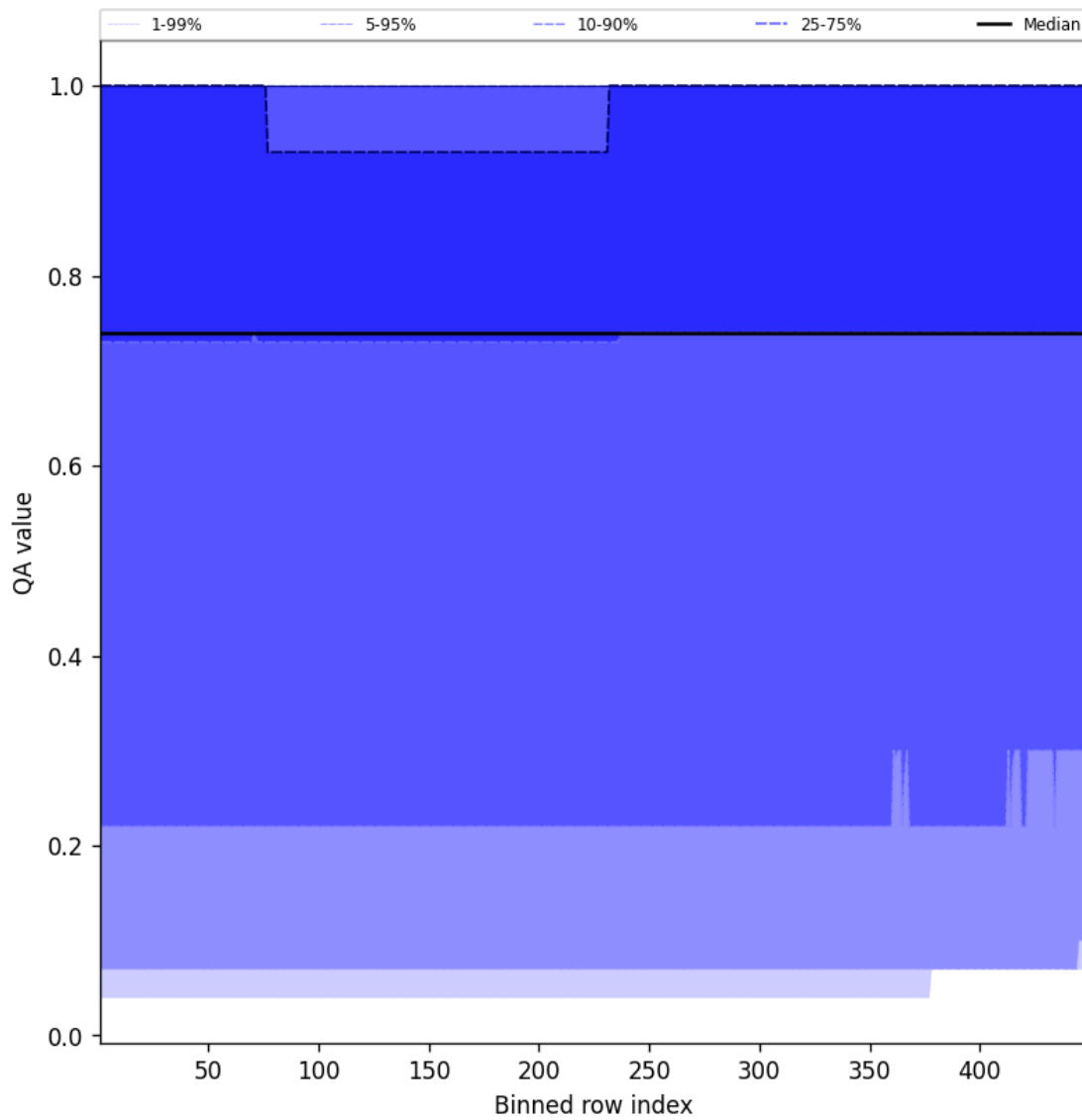
Figure 43: Along track statistics of “QA value” for 2025-03-25 to 2025-03-26
