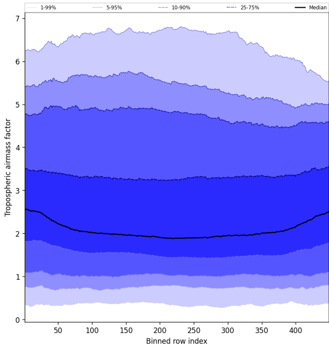
Figure 46: Along track statistics of “Tropospheric airmass factor” for 2025-03-25 to 2025-03-26
