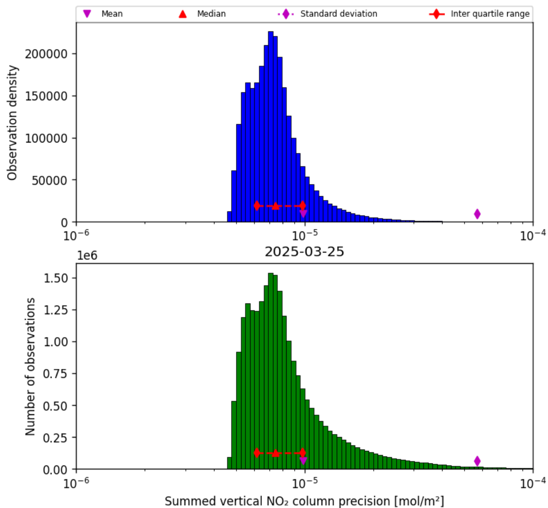
Figure 39: Histogram of "Summed vertical NO 2 column precision" for 2025-03-25 to 2025-03-26
