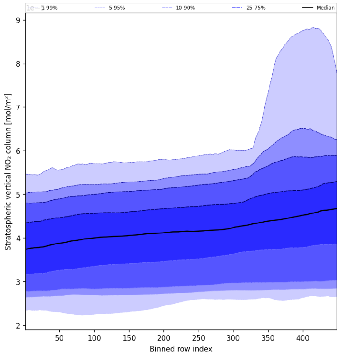
Figure 51: Along track statistics of “Stratospheric vertical NO 2 column” for 2025-03-25 to 2025-03-26
