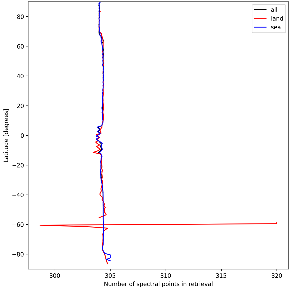
Figure 14: Zonal average of “Number of spectral points in retrieval” for 2025-03-25 to 2025-03-26.
