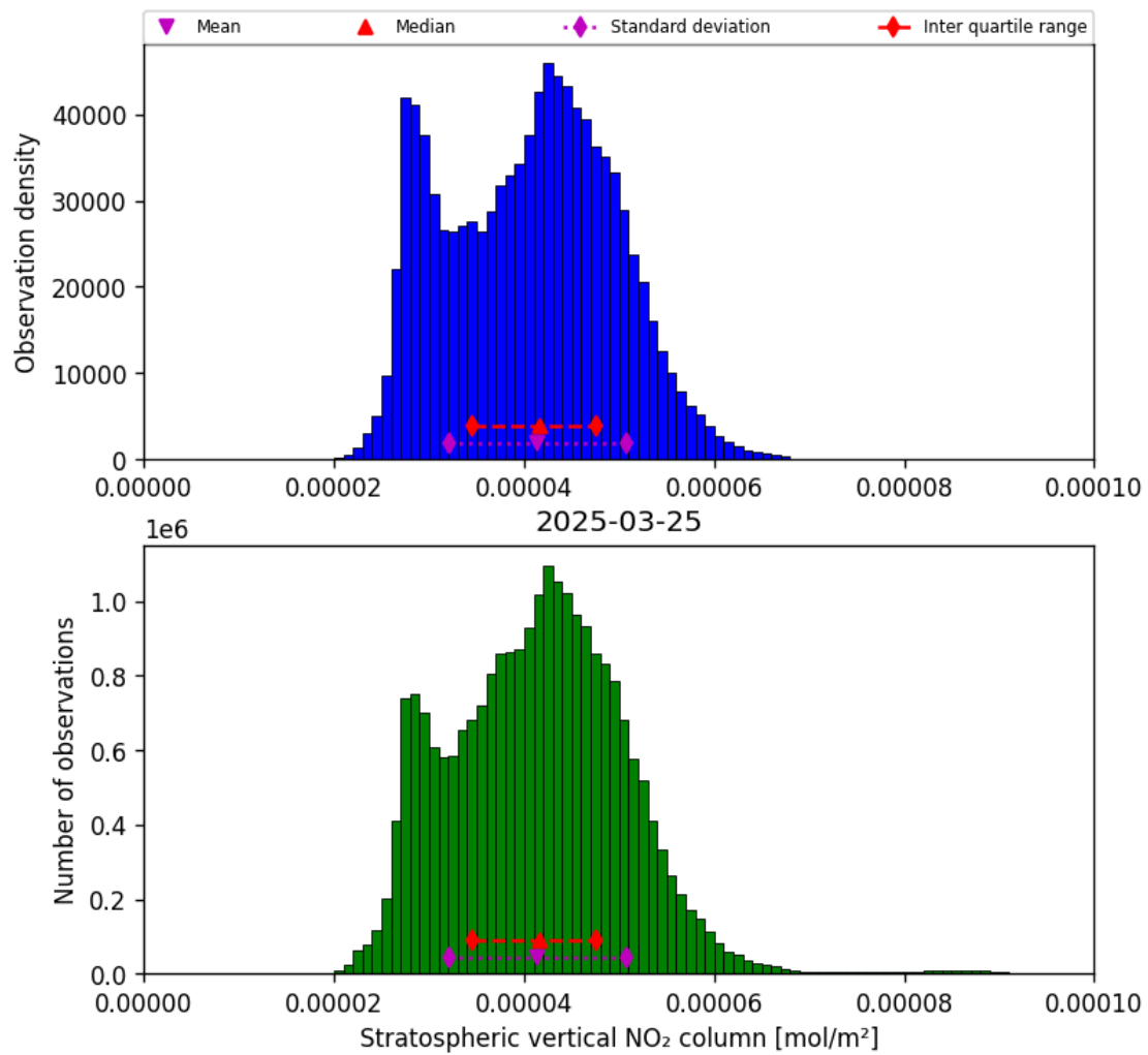
Figure 34: Histogram of “Stratospheric vertical NO 2 column” for 2025-03-25 to 2025-03-26
