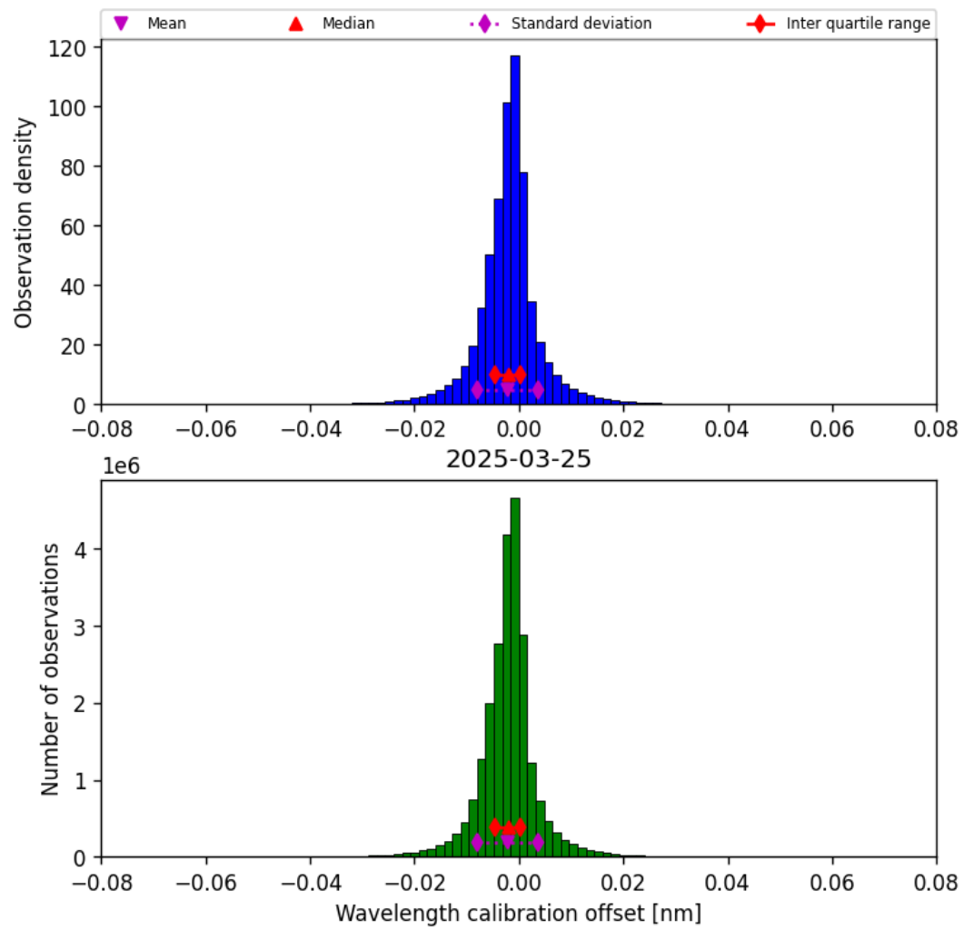
Figure 33: Histogram of “Wavelength calibration offset” for 2025-03-25 to 2025-03-26
