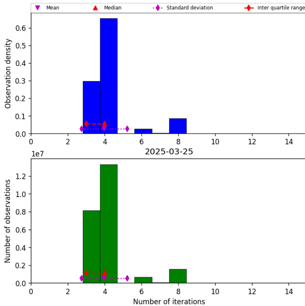
Figure 32: Histogram of “Number of iterations” for 2025-03-25 to 2025-03-26
