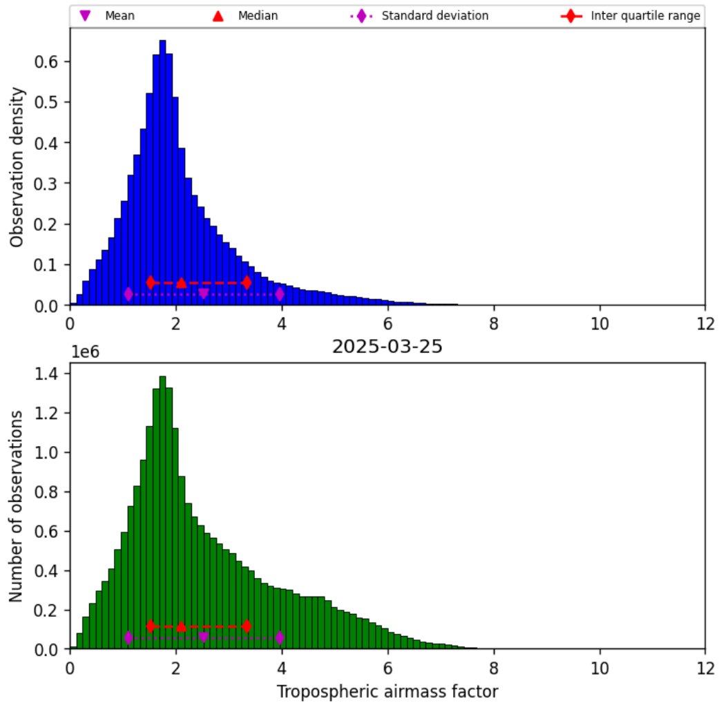
Figure 29: Histogram of “Tropospheric airmass factor” for 2025-03-25 to 2025-03-26
