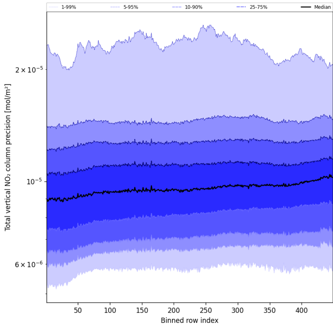
Figure 54: Along track statistics of "Total vertical NO 2 column precision" for 2025-03-25 to 2025-03-26
