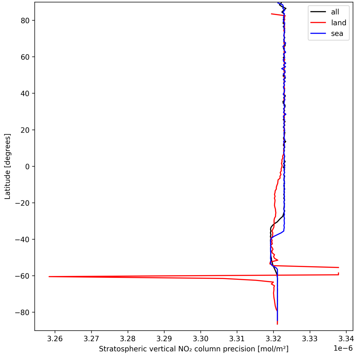
Figure 18: Zonal average of "Stratospheric vertical NO 2 column precision" for 2025-03-25 to 2025-03-26.
