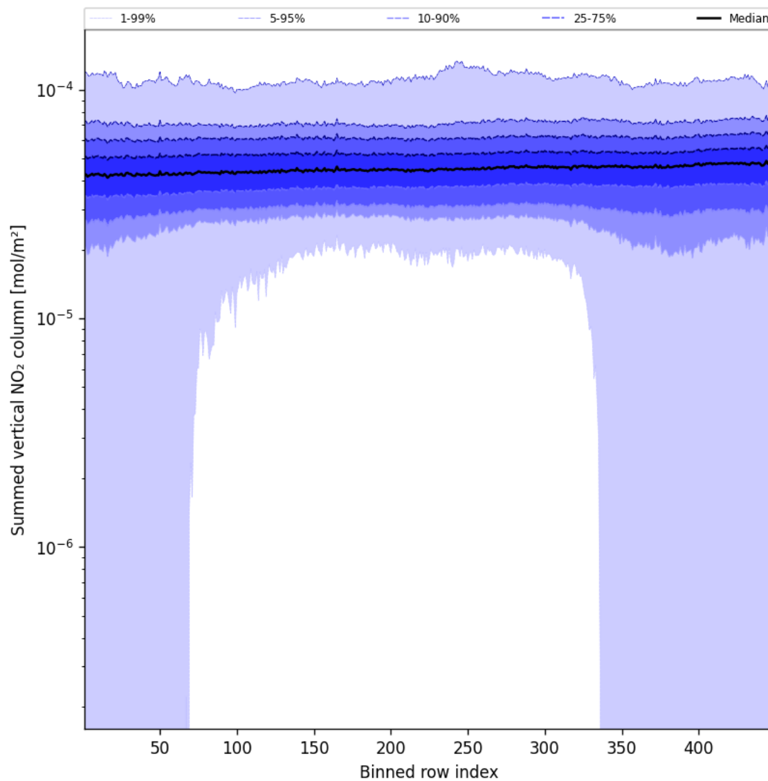
Figure 55: Along track statistics of “Summed vertical NO 2 column” for 2025-03-25 to 2025-03-26
