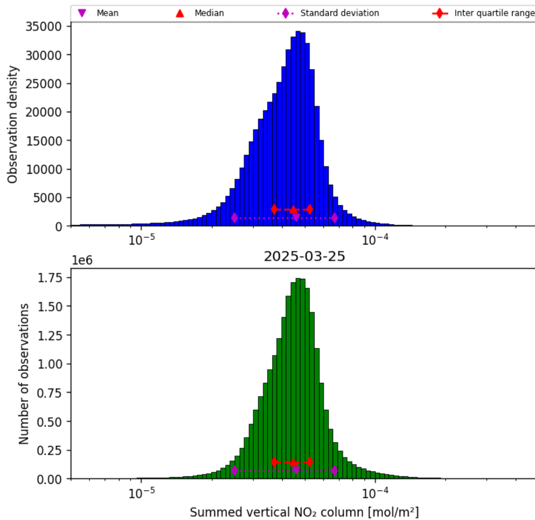
Figure 38: Histogram of “Summed vertical NO 2 column” for 2025-03-25 to 2025-03-26
