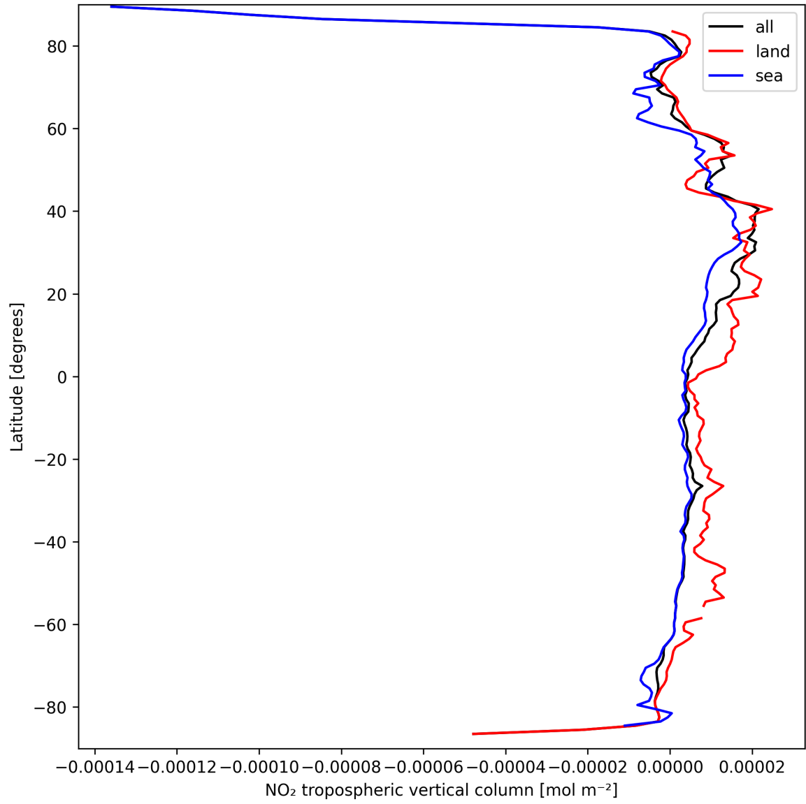
Figure 10: Zonal average of “NO 2 tropospheric vertical column” for 2025-03-25 to 2025-03-26.
