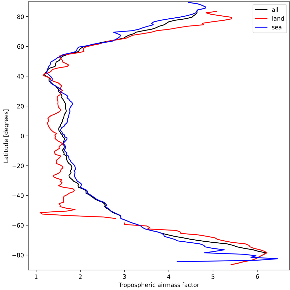
Figure 12: Zonal average of “Tropospheric airmass factor” for 2025-03-25 to 2025-03-26.
