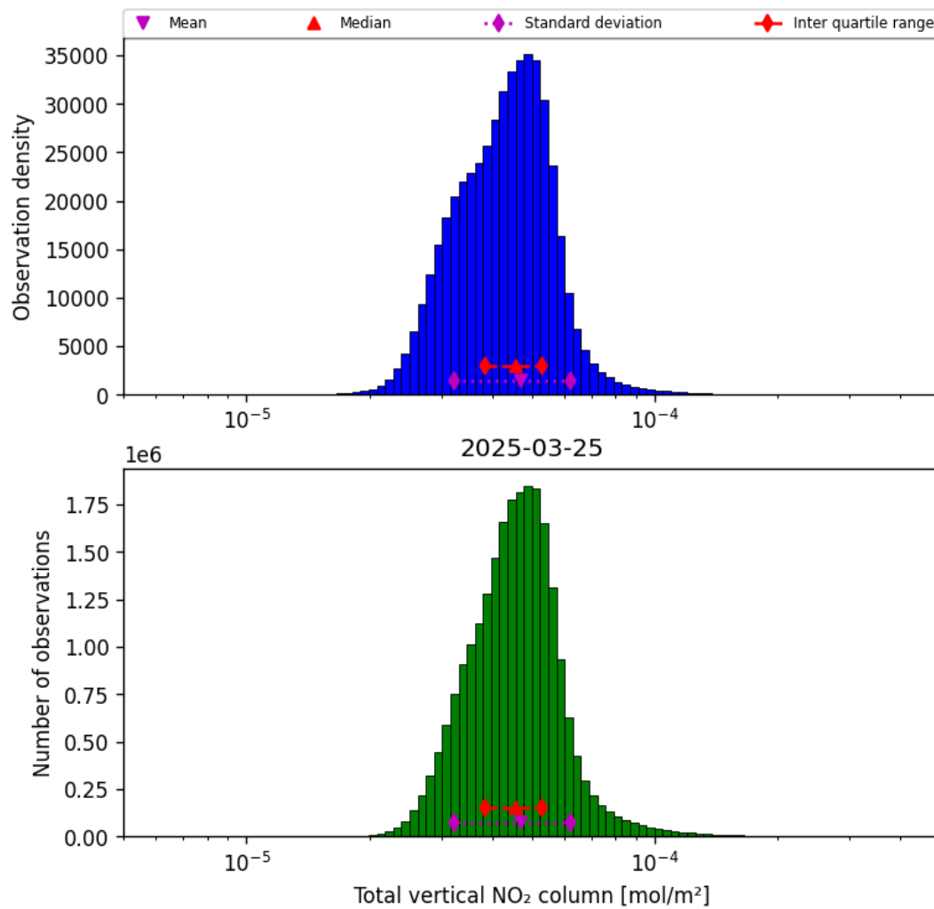
Figure 36: Histogram of "Total vertical NO 2 column" for 2025-03-25 to 2025-03-26
