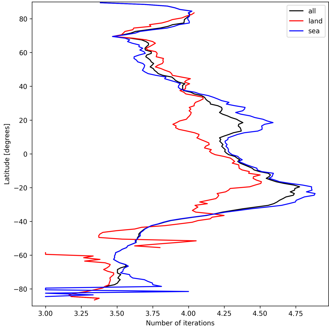
Figure 15: Zonal average of “Number of iterations” for 2025-03-25 to 2025-03-26.
