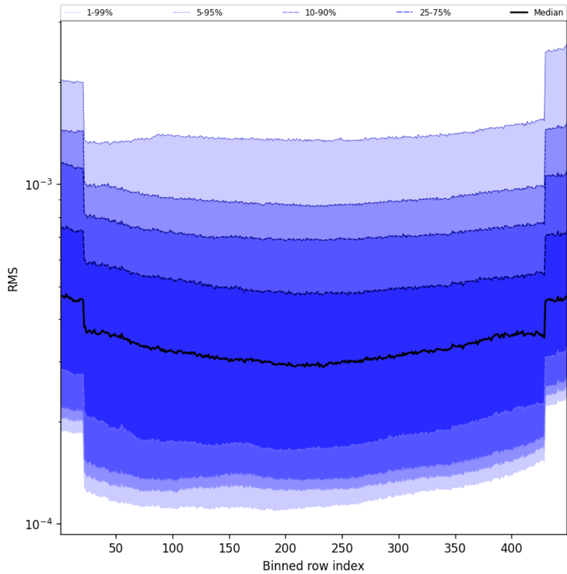
Figure 58: Along track statistics of “RMS” for 2025-03-25 to 2025-03-26
