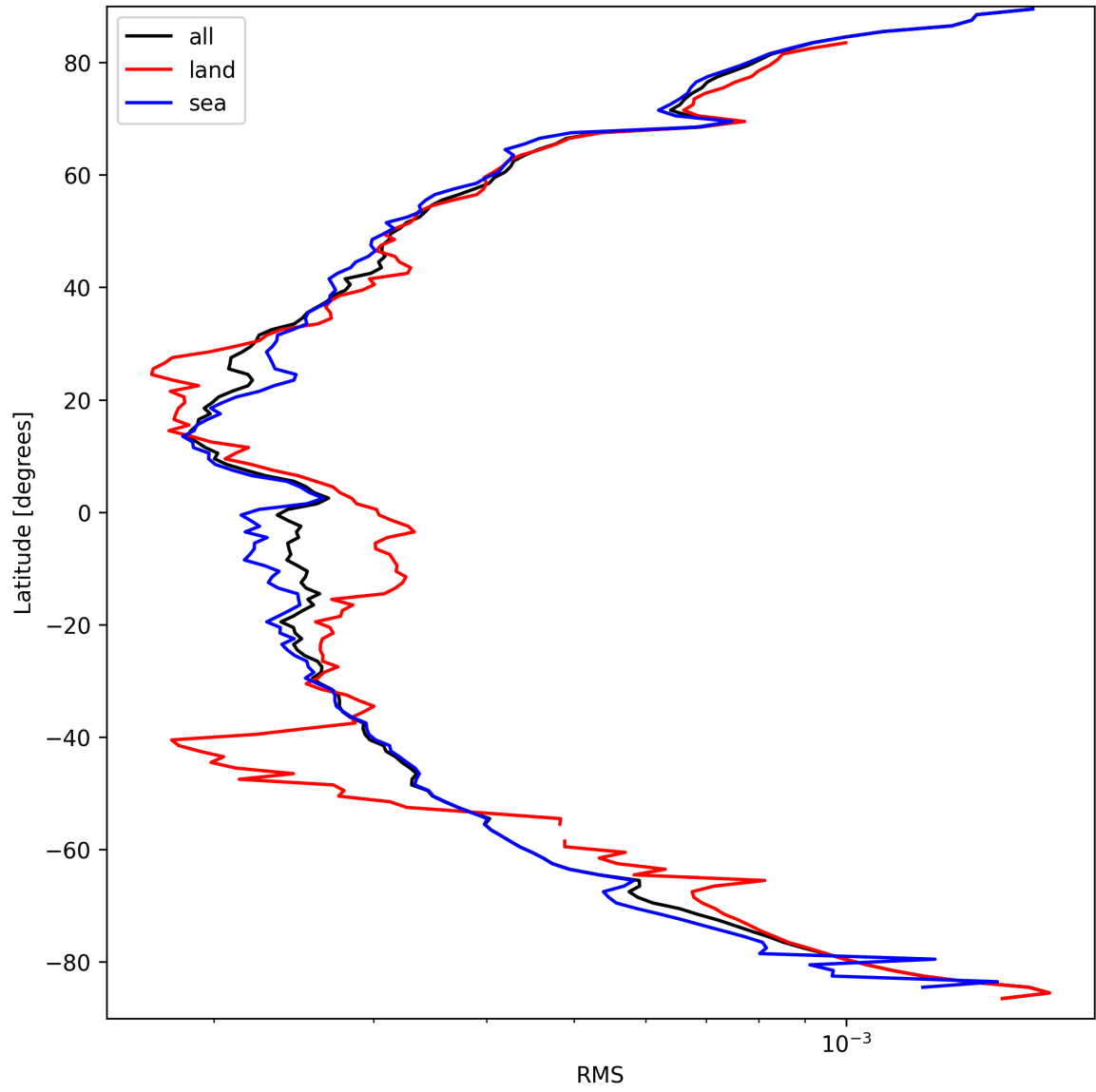
Figure 24: Zonal average of “RMS” for 2025-03-25 to 2025-03-26.
