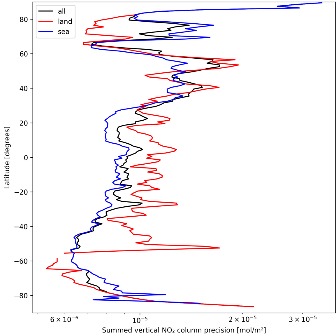
Figure 22: Zonal average of “Summed vertical NO 2 column precision” for 2025-03-25 to 2025-03-26.
