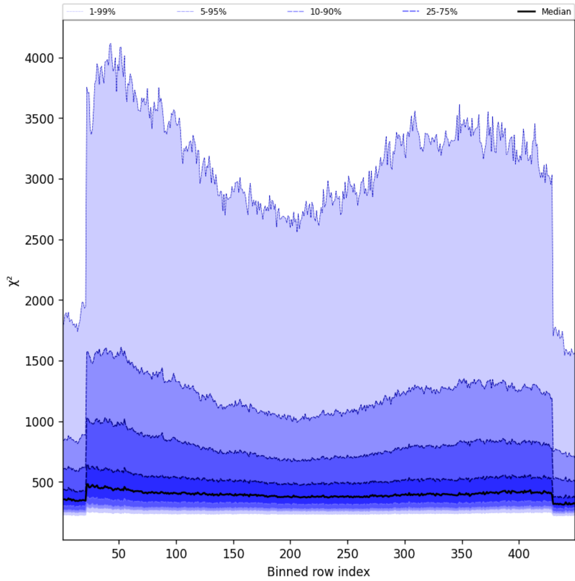
Figure 57: Along track statistics of “ \chi^2 ” for 2025-03-25 to 2025-03-26
