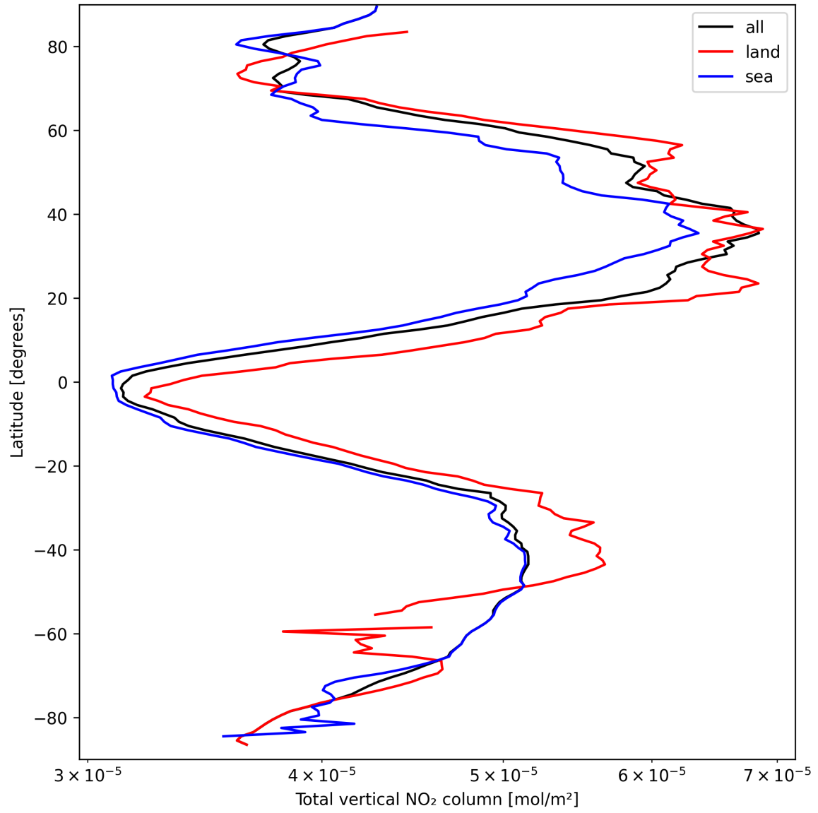
Figure 19: Zonal average of “Total vertical NO 2 column” for 2025-03-25 to 2025-03-26.
