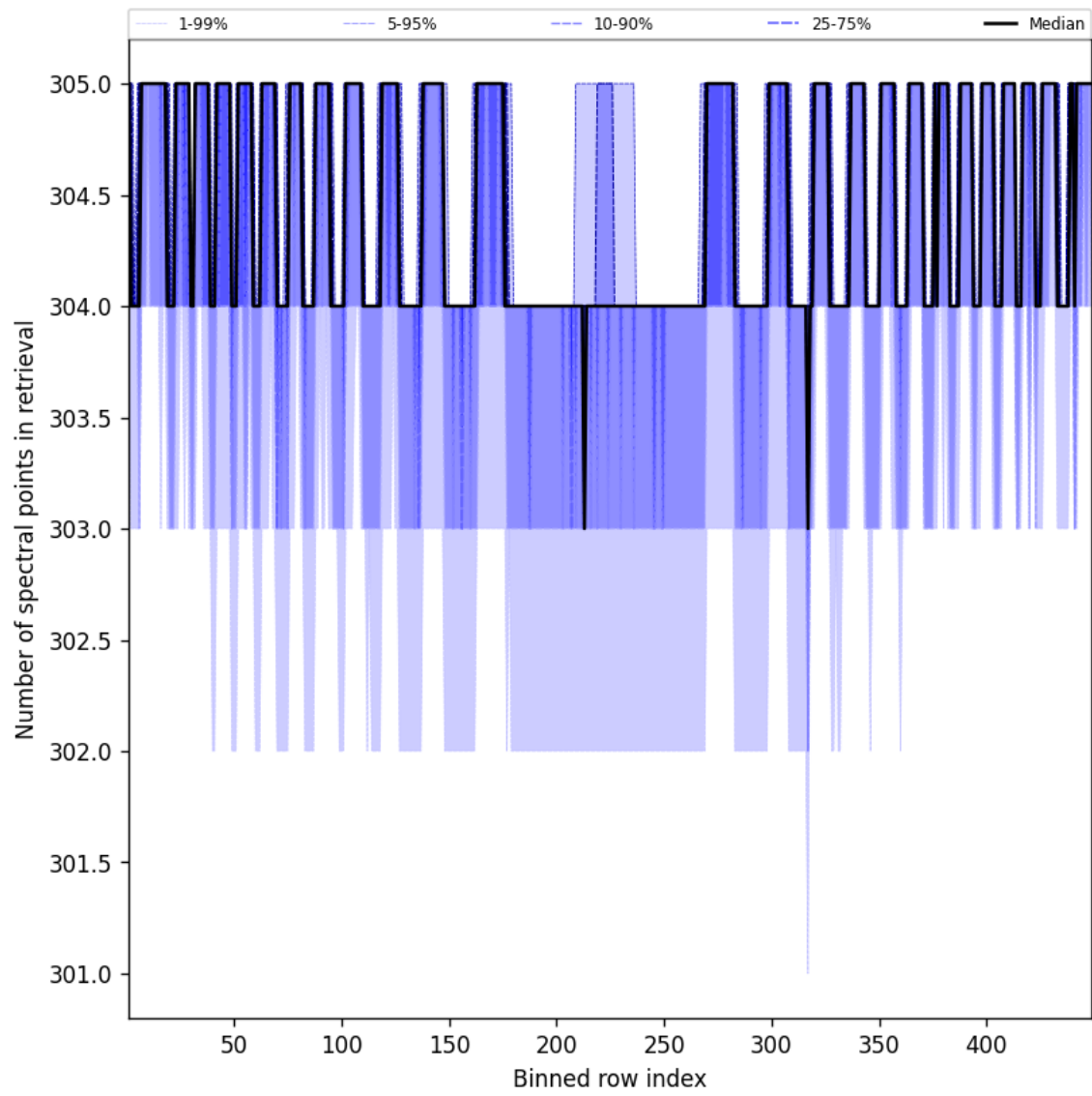
Figure 48: Along track statistics of “Number of spectral points in retrieval” for 2025-03-25 to 2025-03-26
