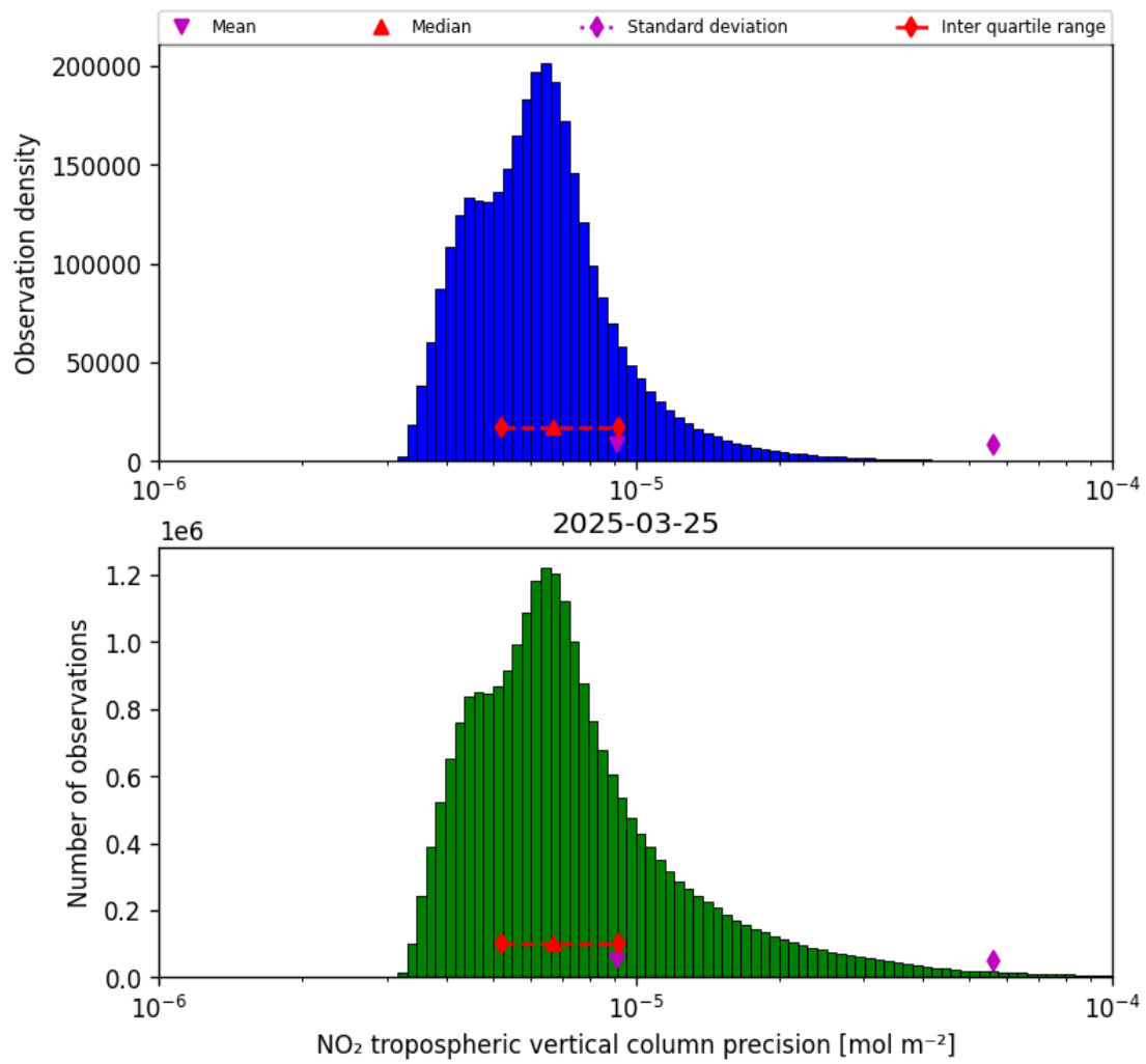
Figure 28: Histogram of “NO 2 tropospheric vertical column precision” for 2025-03-25 to 2025-03-26
