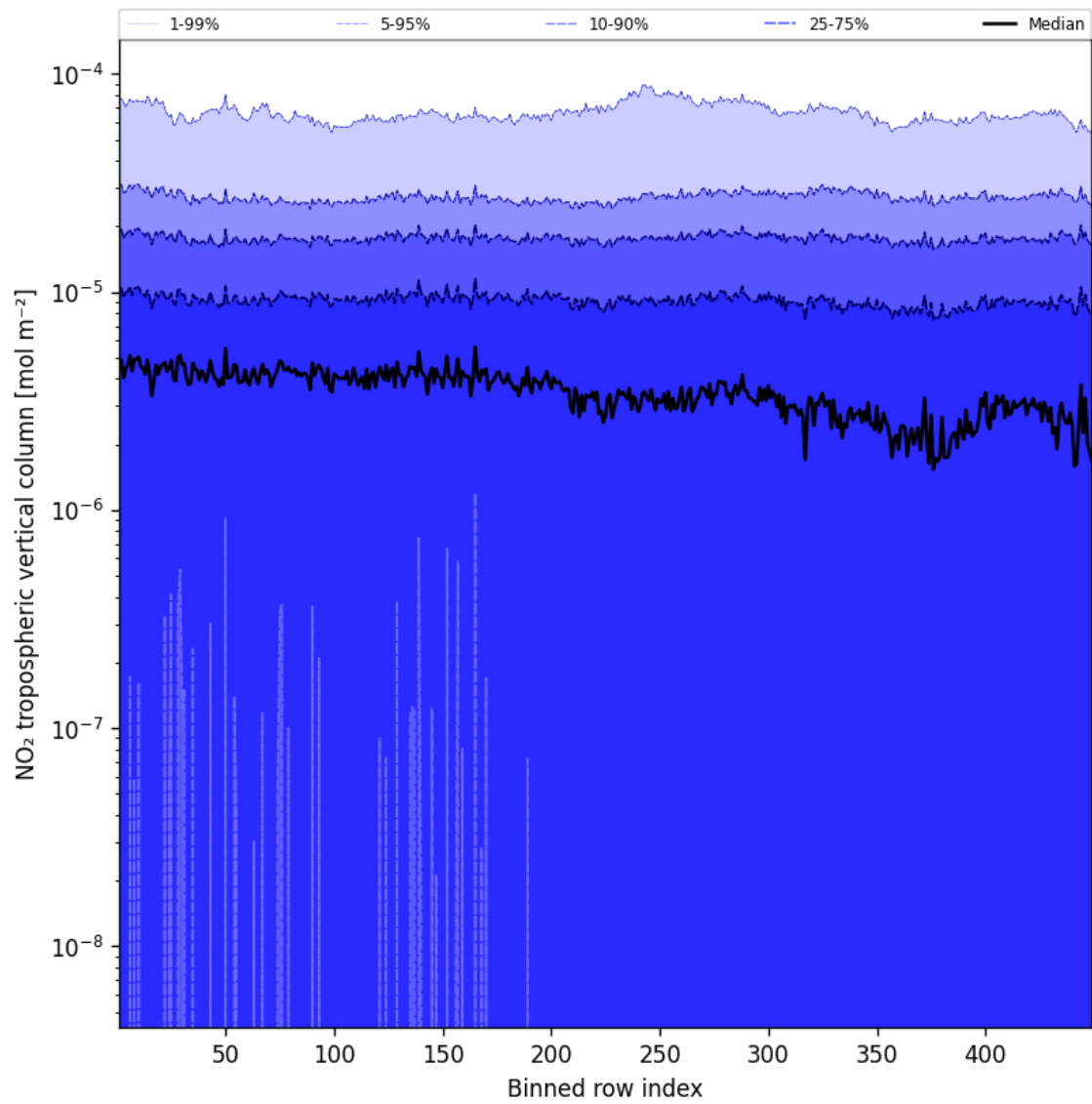
Figure 44: Along track statistics of “NO 2 tropospheric vertical column” for 2025-03-25 to 2025-03-26
