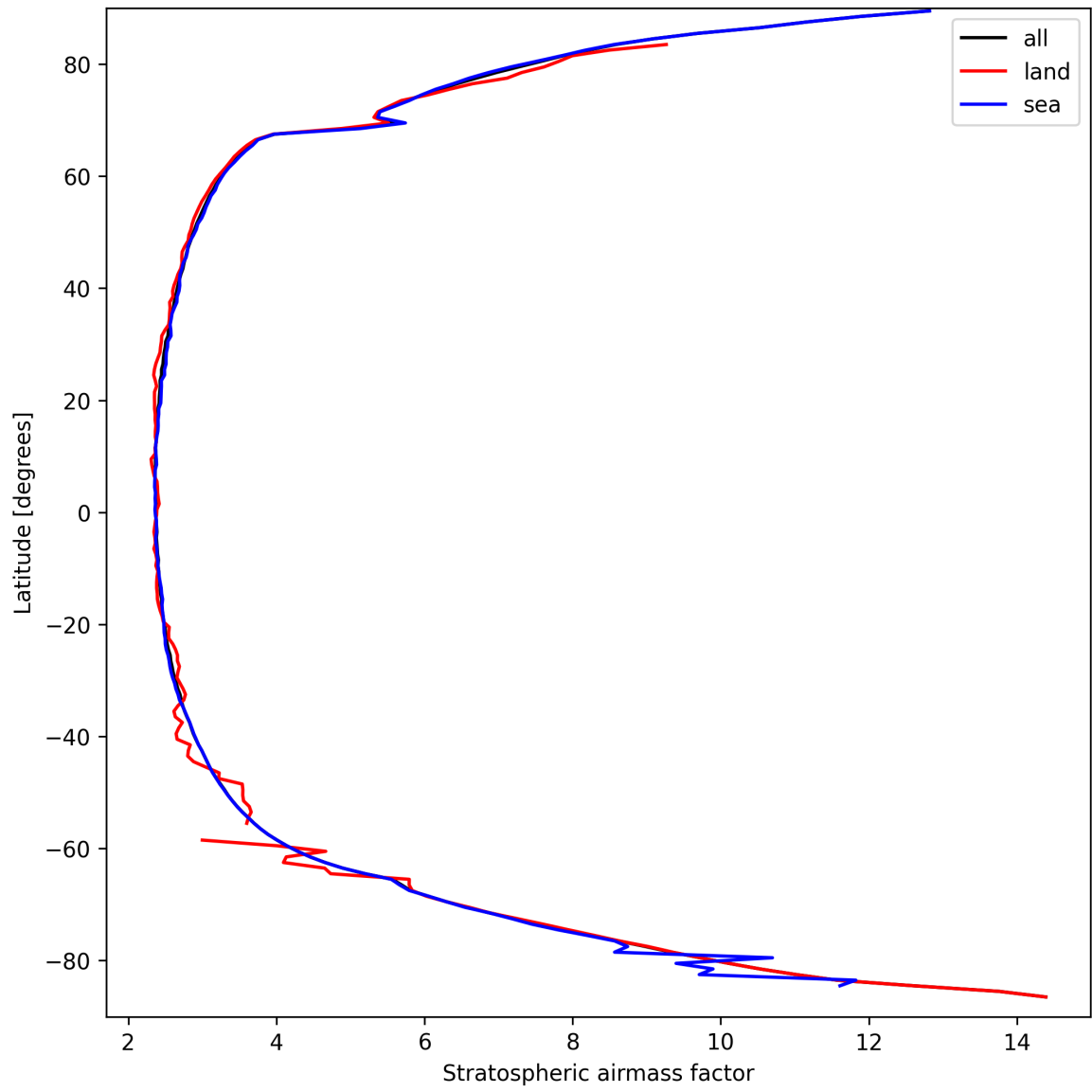
Figure 25: Zonal average of “Stratospheric airmass factor” for 2025-03-25 to 2025-03-26.
