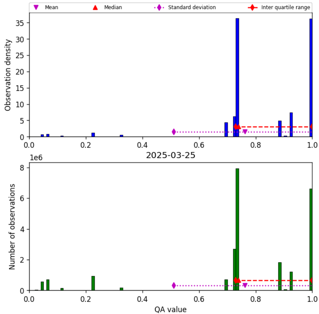
Figure 26: Histogram of “QA value” for 2025-03-25 to 2025-03-26
