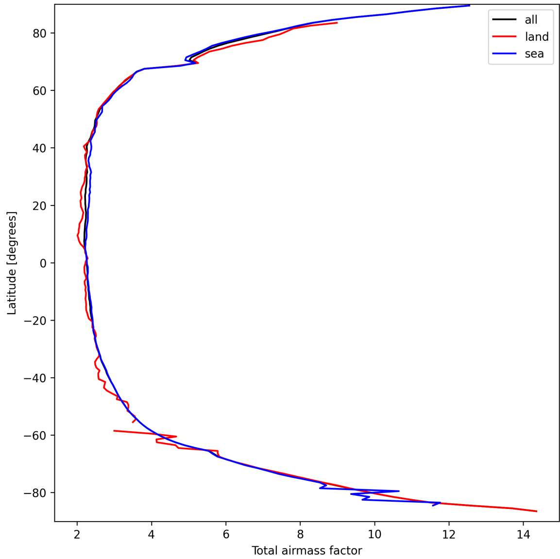
Figure 13: Zonal average of “Total airmass factor” for 2025-03-25 to 2025-03-26.
