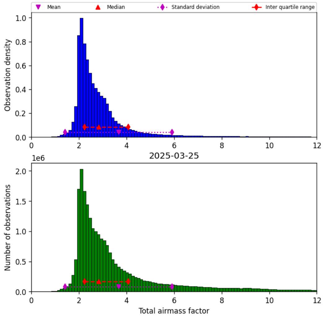
Figure 30: Histogram of “Total airmass factor” for 2025-03-25 to 2025-03-26
