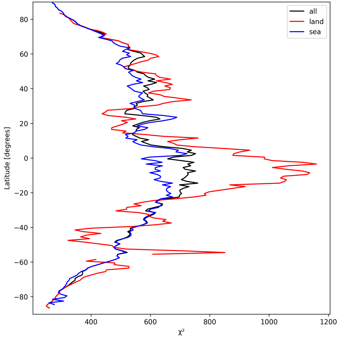
Figure 23: Zonal average of “ \chi^2 ” for 2025-03-25 to 2025-03-26.
