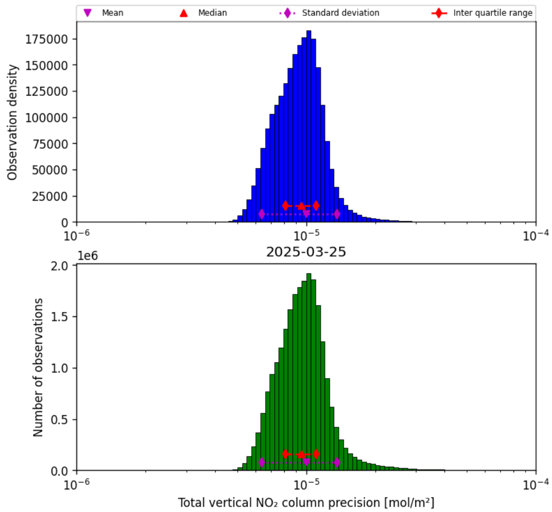
Figure 37: Histogram of "Total vertical NO 2 column precision" for 2025-03-25 to 2025-03-26
