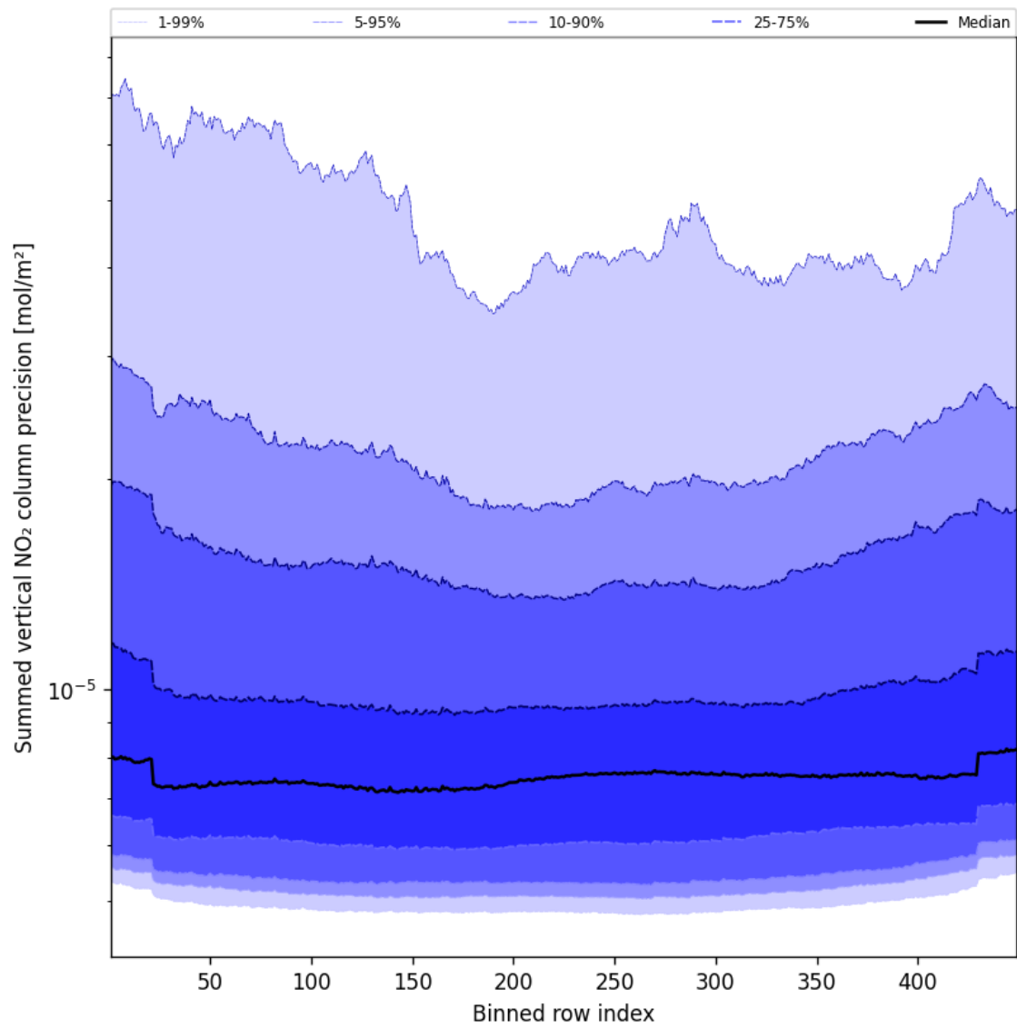
Figure 56: Along track statistics of “Summed vertical NO 2 column precision” for 2025-03-25 to 2025-03-26
