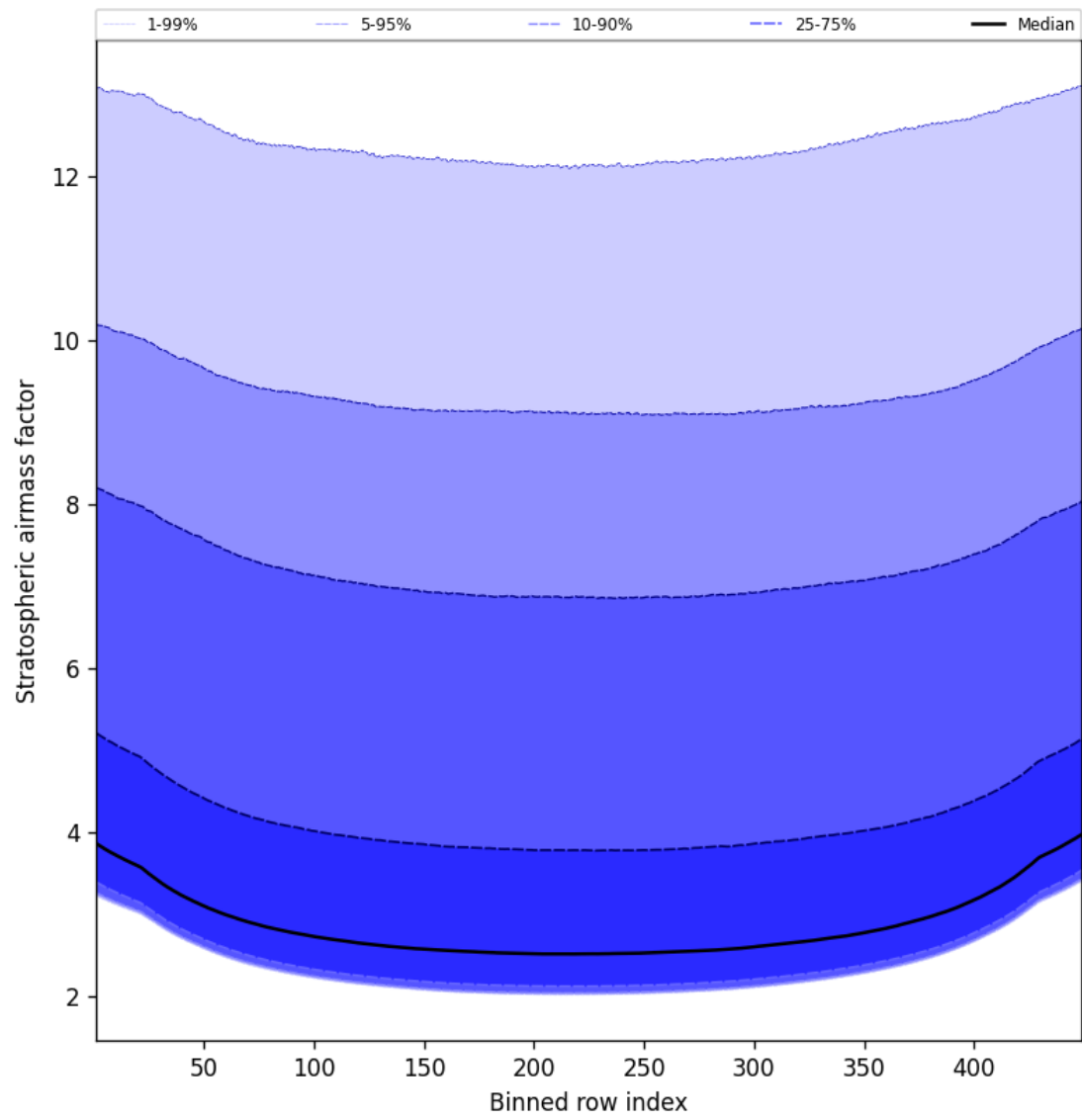
Figure 59: Along track statistics of “Stratospheric airmass factor” for 2025-03-26 to 2025-03-26
