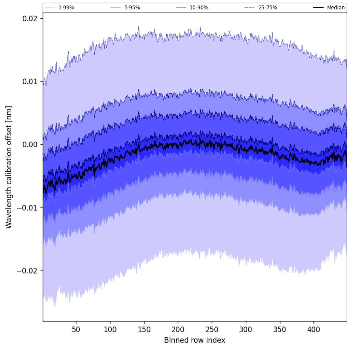
Figure 50: Along track statistics of “Wavelength calibration offset” for 2025-03-26 to 2025-03-26
