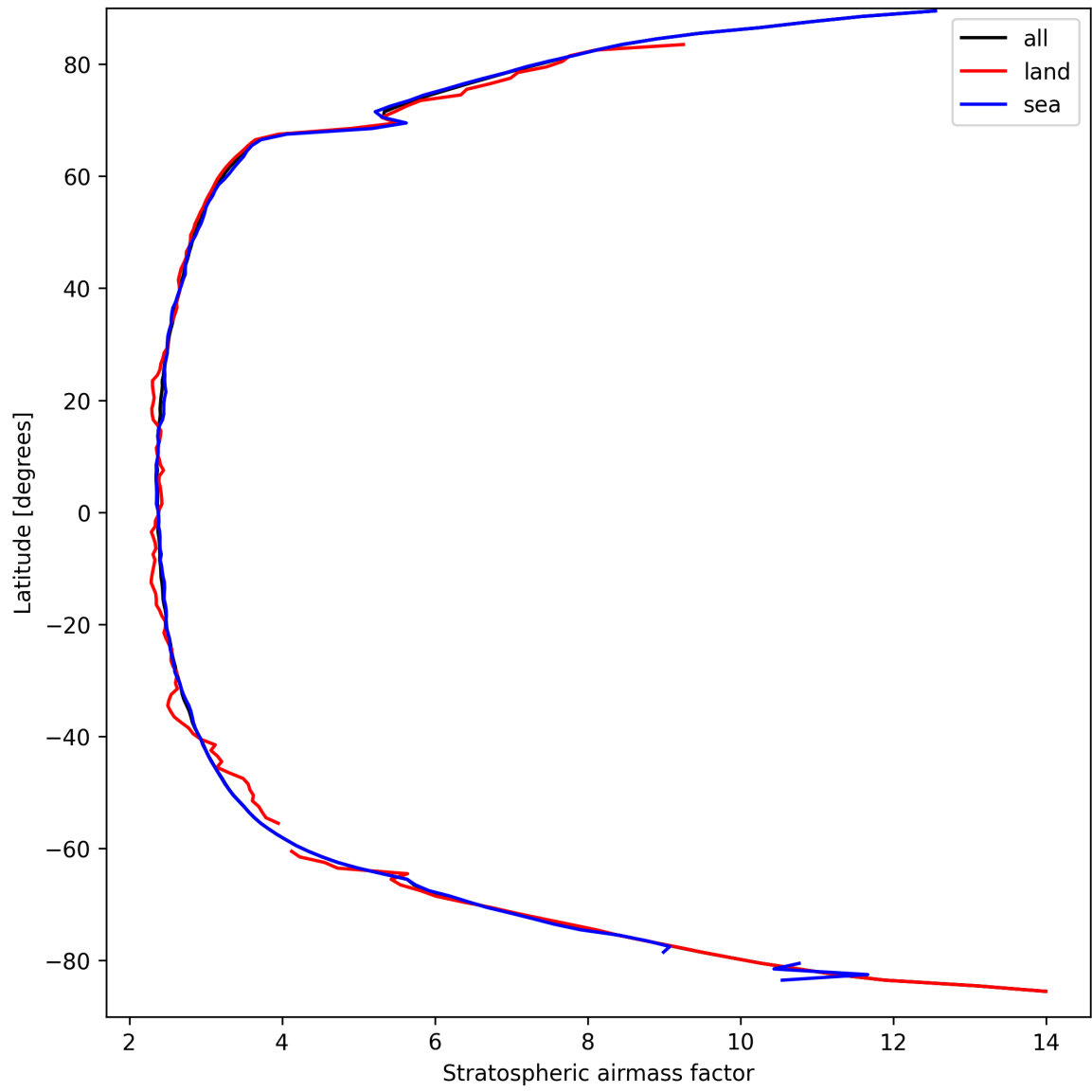
Figure 25: Zonal average of “Stratospheric airmass factor” for 2025-03-26 to 2025-03-26.
