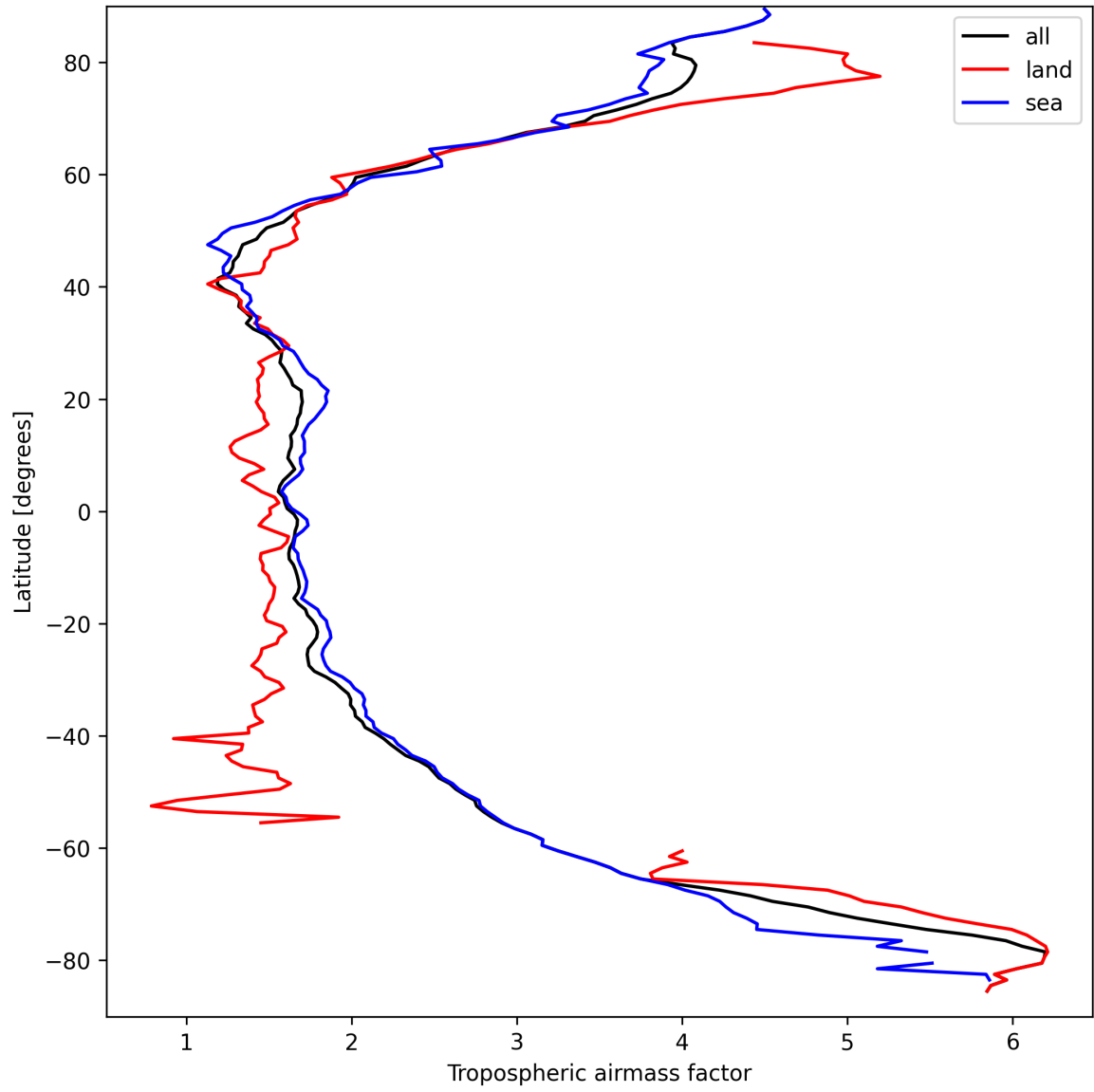
Figure 12: Zonal average of “Tropospheric airmass factor” for 2025-03-26 to 2025-03-26.
