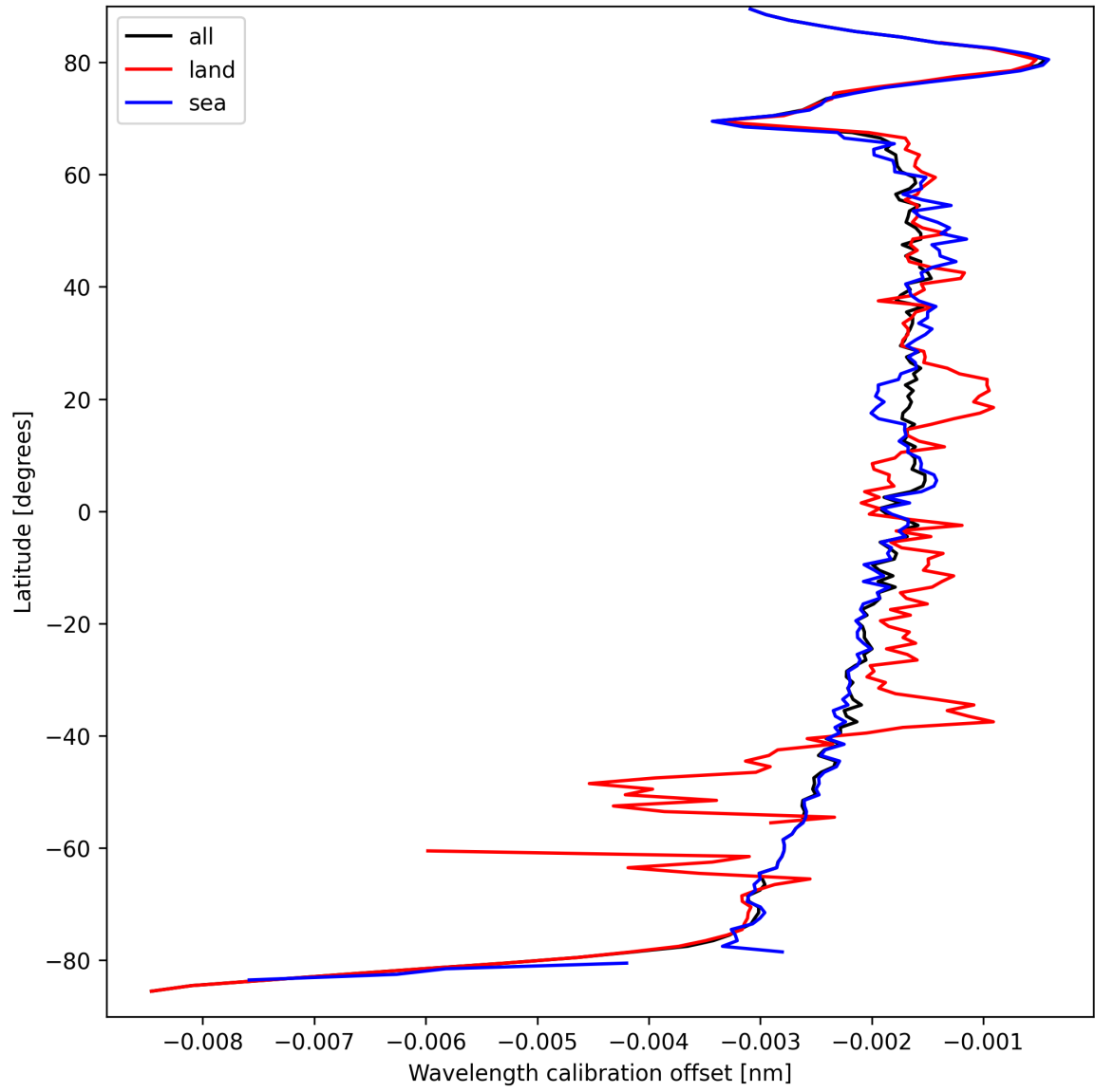
Figure 16: Zonal average of “Wavelength calibration offset” for 2025-03-26 to 2025-03-26.
