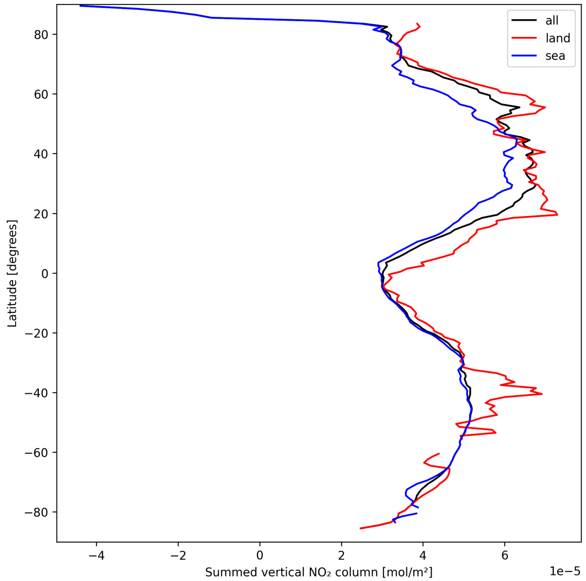
Figure 21: Zonal average of “Summed vertical NO 2 column” for 2025-03-26 to 2025-03-26.
