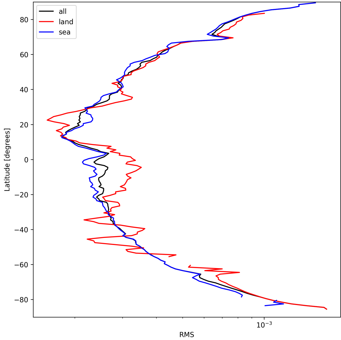
Figure 24: Zonal average of “RMS” for 2025-03-26 to 2025-03-26.
