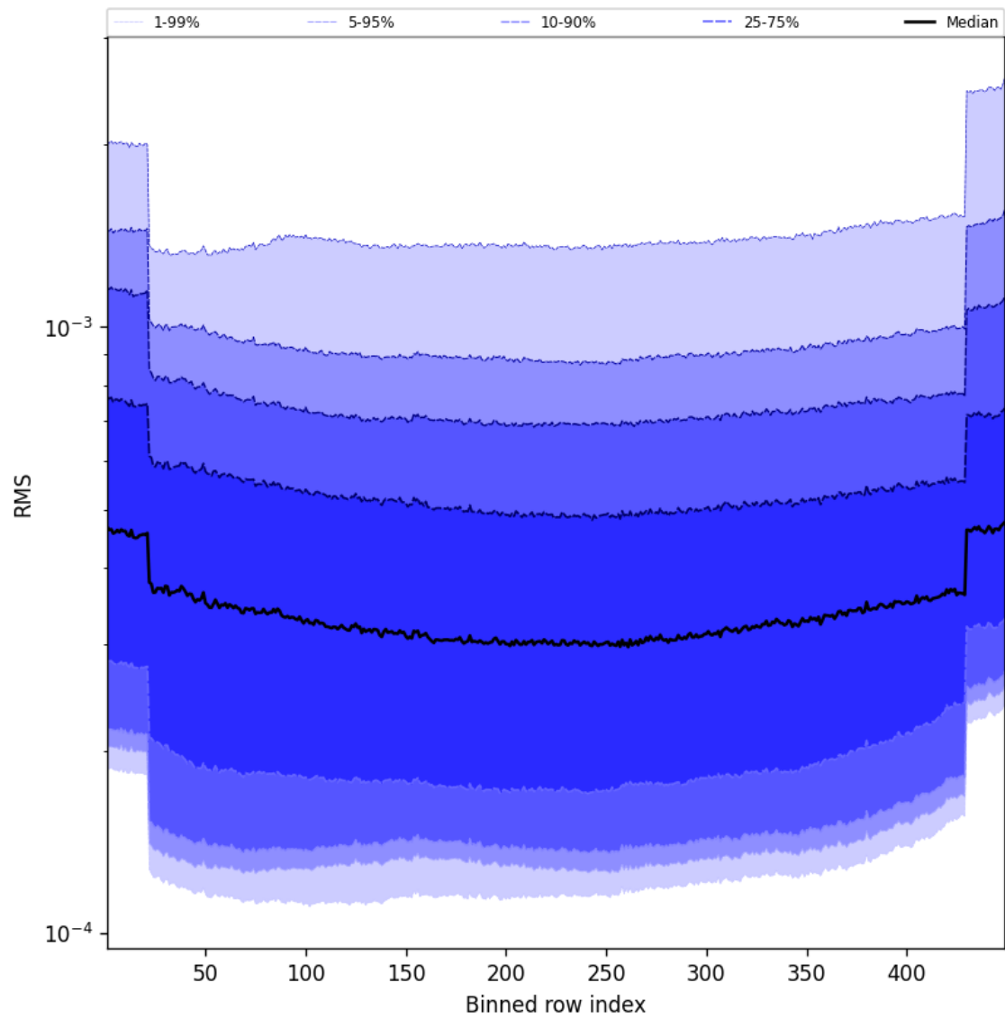
Figure 58: Along track statistics of “RMS” for 2025-03-26 to 2025-03-26
