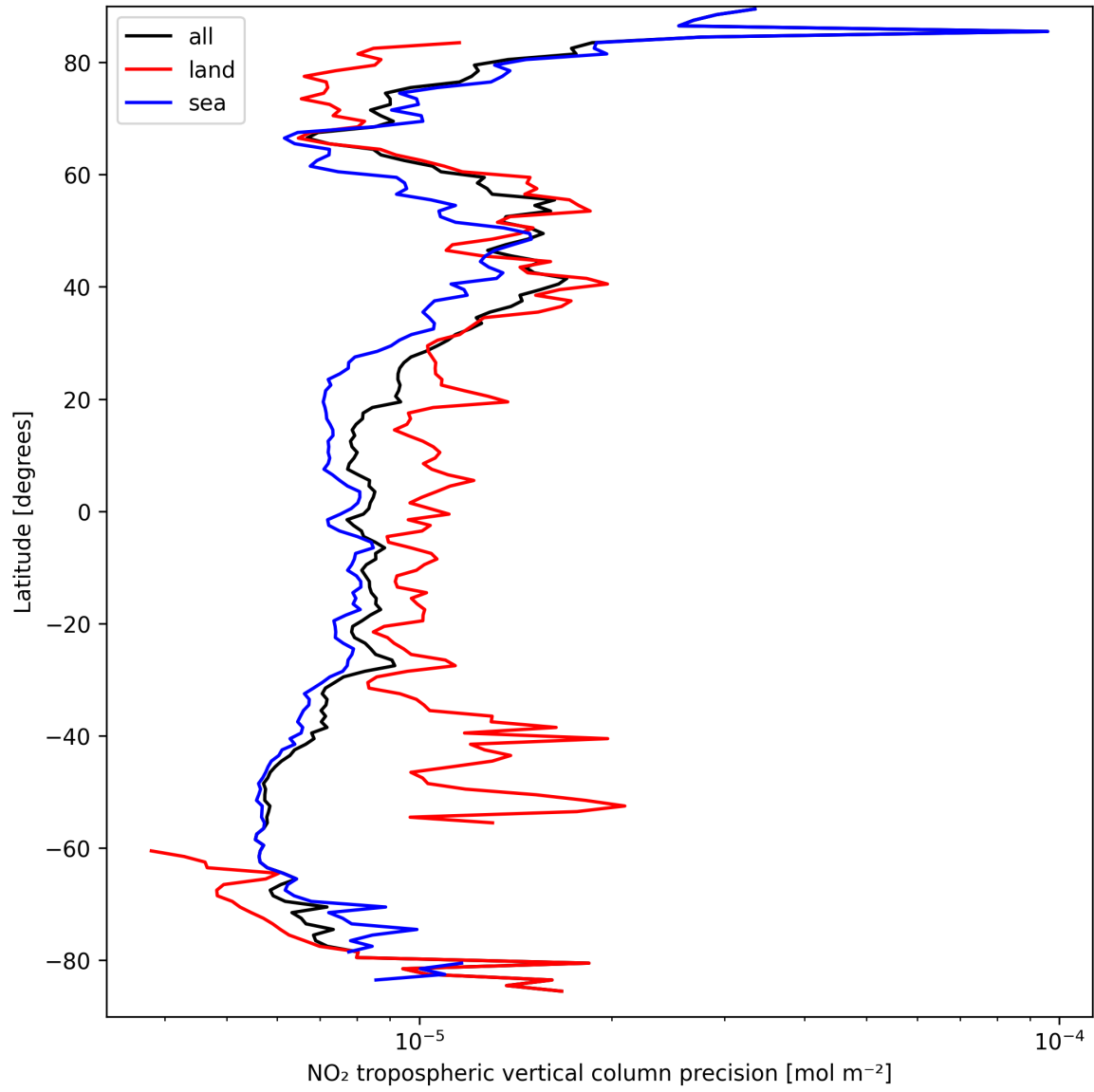
Figure 11: Zonal average of “NO 2 tropospheric vertical column precision” for 2025-03-26 to 2025-03-26.
