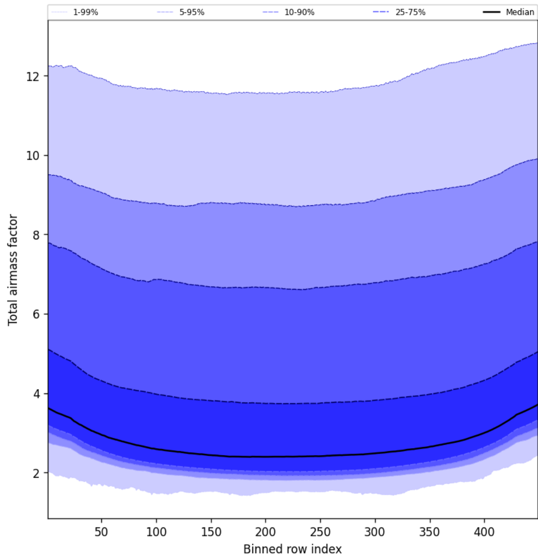
Figure 47: Along track statistics of “Total airmass factor” for 2025-03-26 to 2025-03-26
