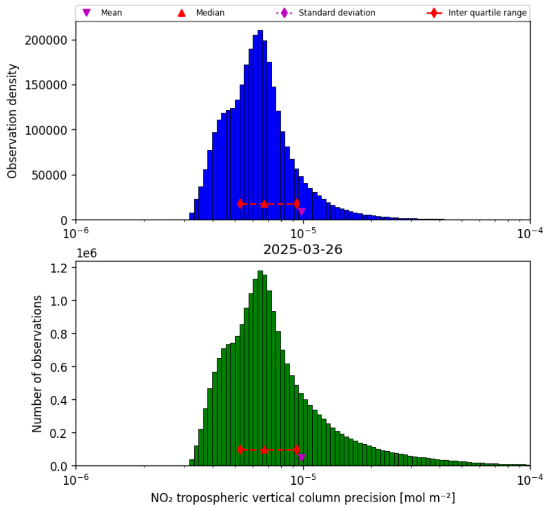
Figure 28: Histogram of “NO 2 tropospheric vertical column precision” for 2025-03-26 to 2025-03-26
