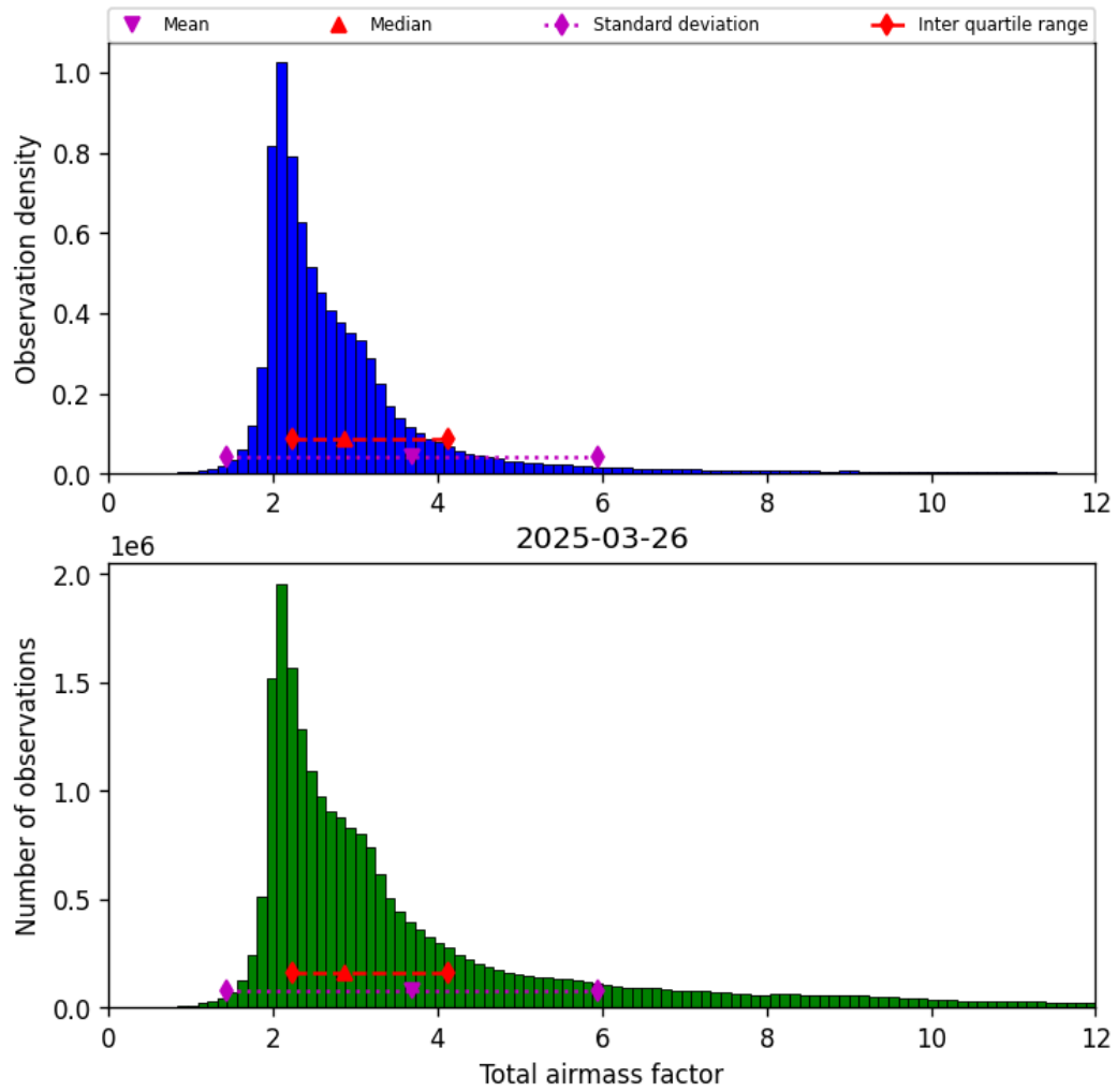
Figure 30: Histogram of “Total airmass factor” for 2025-03-26 to 2025-03-26
