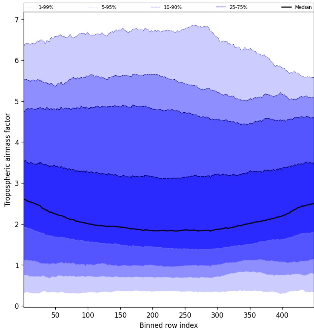
Figure 46: Along track statistics of “Tropospheric airmass factor” for 2025-03-26 to 2025-03-26
