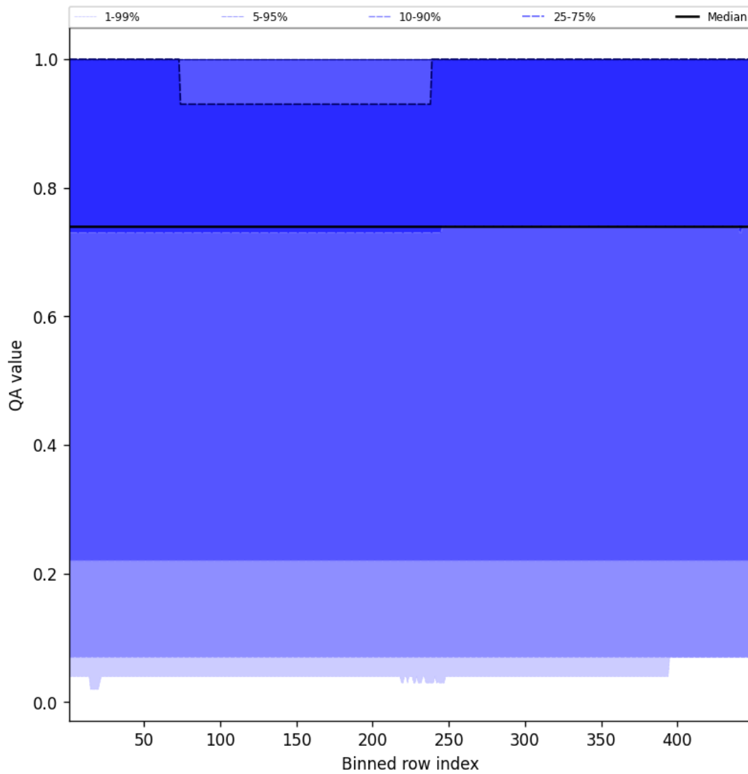
Figure 43: Along track statistics of “QA value” for 2025-03-26 to 2025-03-26
