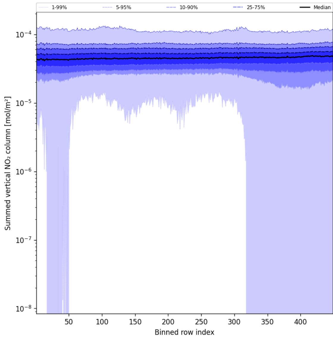
Figure 55: Along track statistics of “Summed vertical NO 2 column” for 2025-03-26 to 2025-03-26
