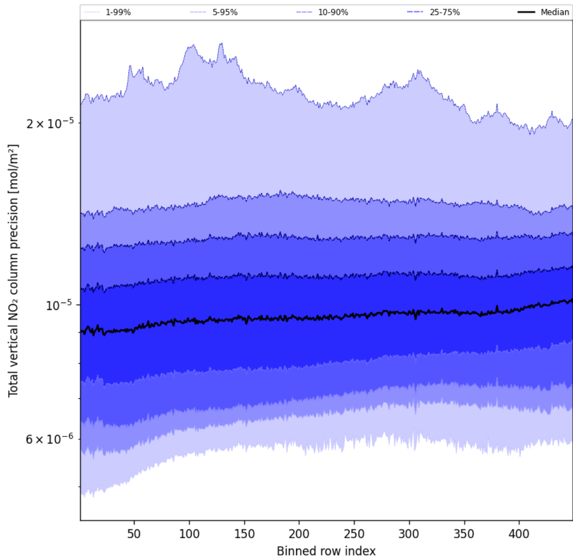
Figure 54: Along track statistics of “Total vertical NO 2 column precision” for 2025-03-26 to 2025-03-26
