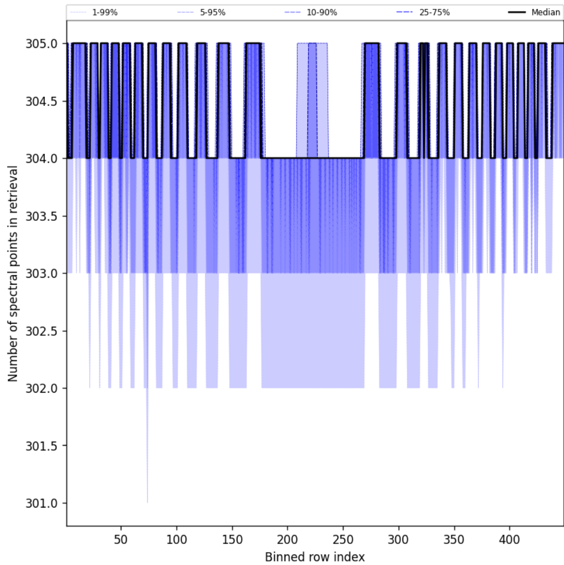
Figure 48: Along track statistics of “Number of spectral points in retrieval” for 2025-03-26 to 2025-03-26
