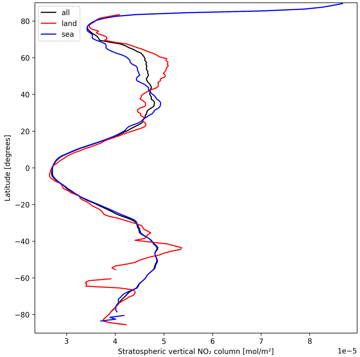
Figure 17: Zonal average of “Stratospheric vertical NO 2 column” for 2025-03-26 to 2025-03-26.
