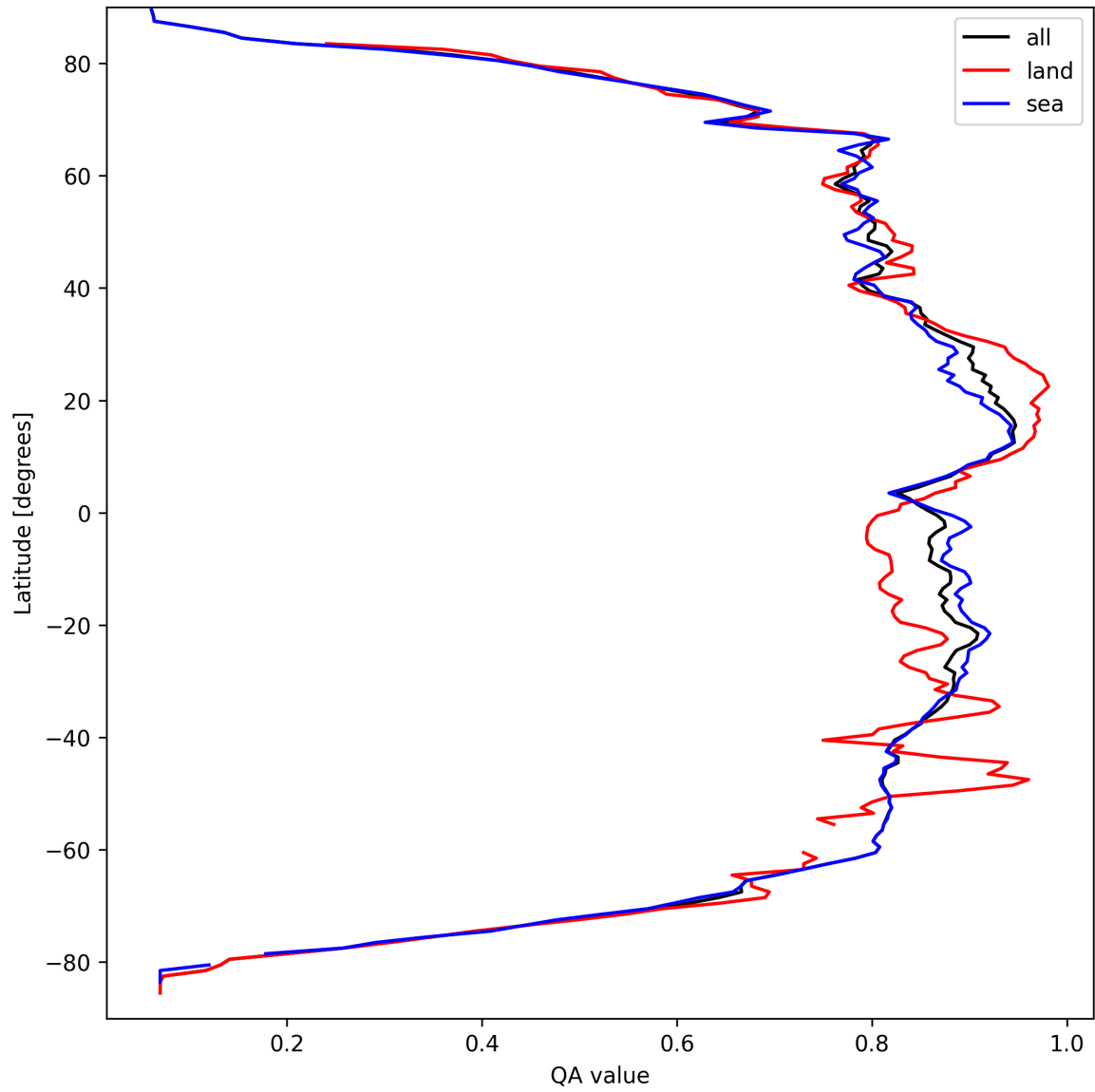
Figure 9: Zonal average of “QA value” for 2025-03-26 to 2025-03-26.
