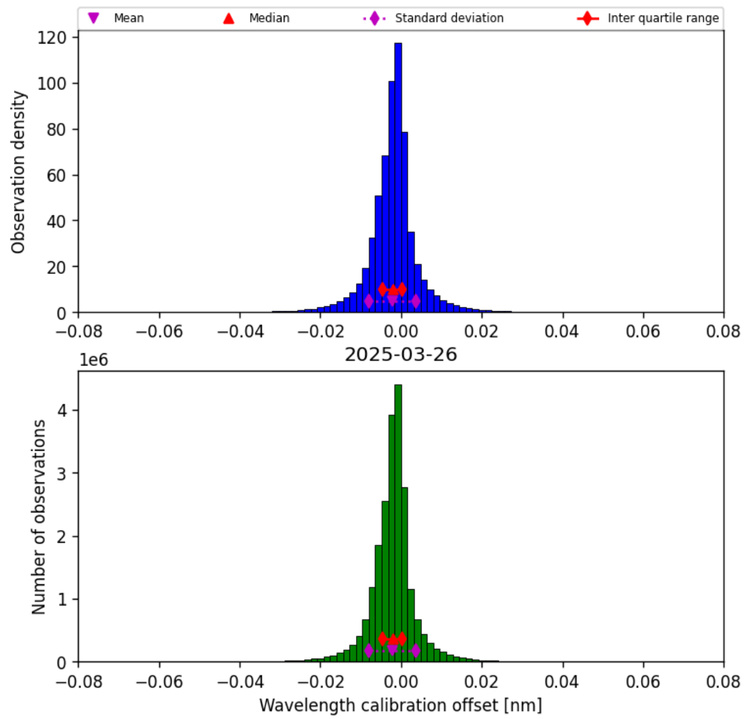
Figure 33: Histogram of “Wavelength calibration offset” for 2025-03-26 to 2025-03-26
