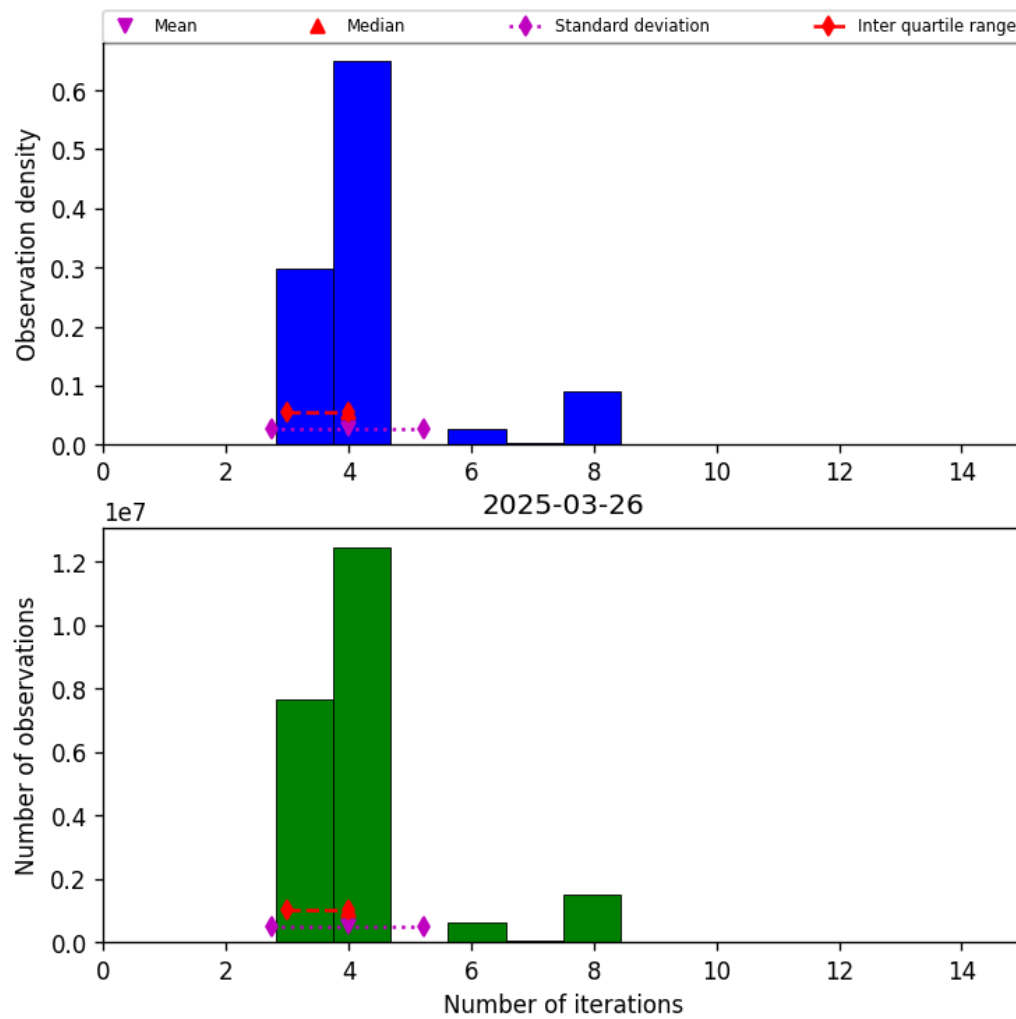
Figure 32: Histogram of “Number of iterations” for 2025-03-26 to 2025-03-26
