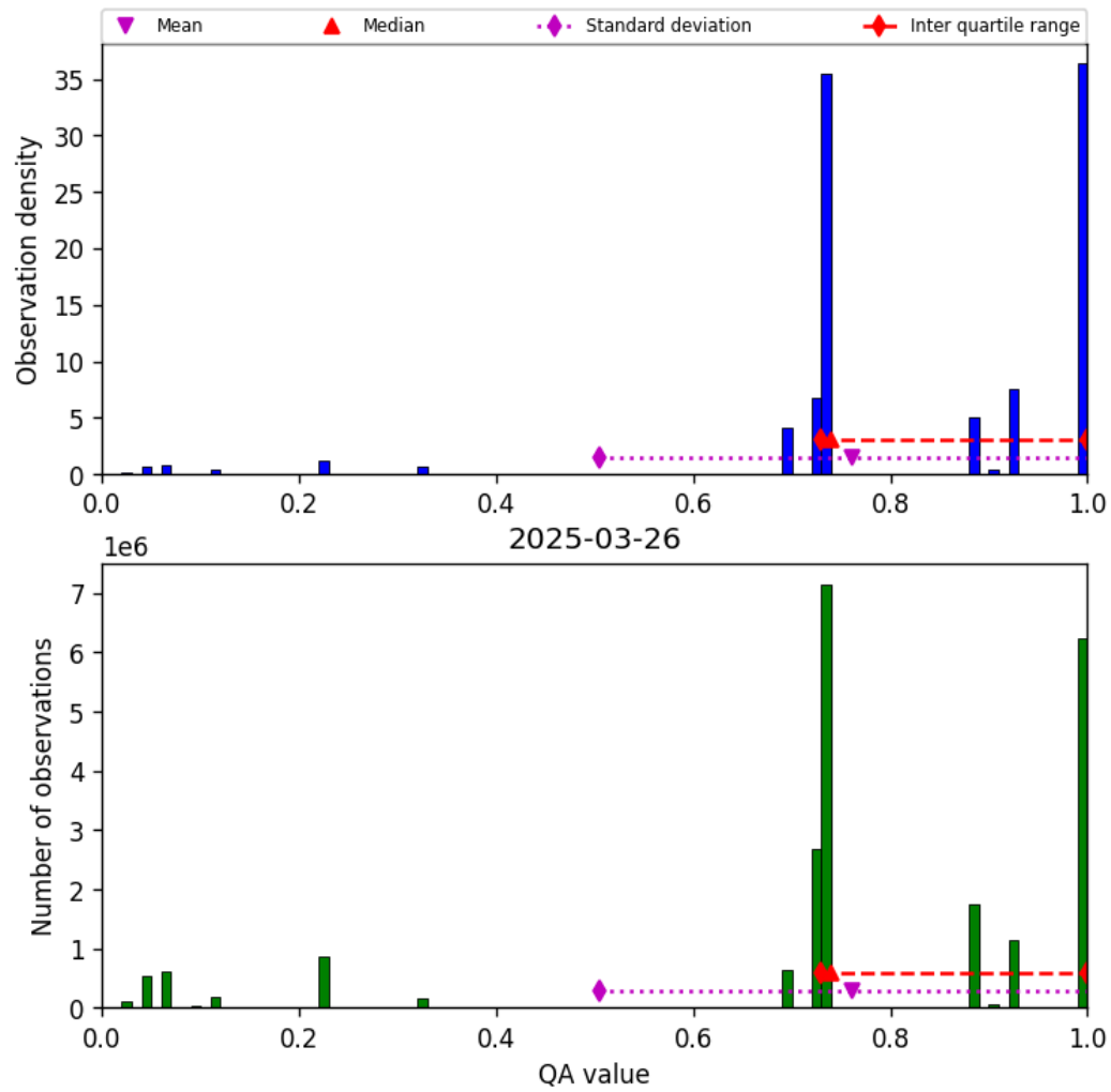
Figure 26: Histogram of “QA value” for 2025-03-26 to 2025-03-26
