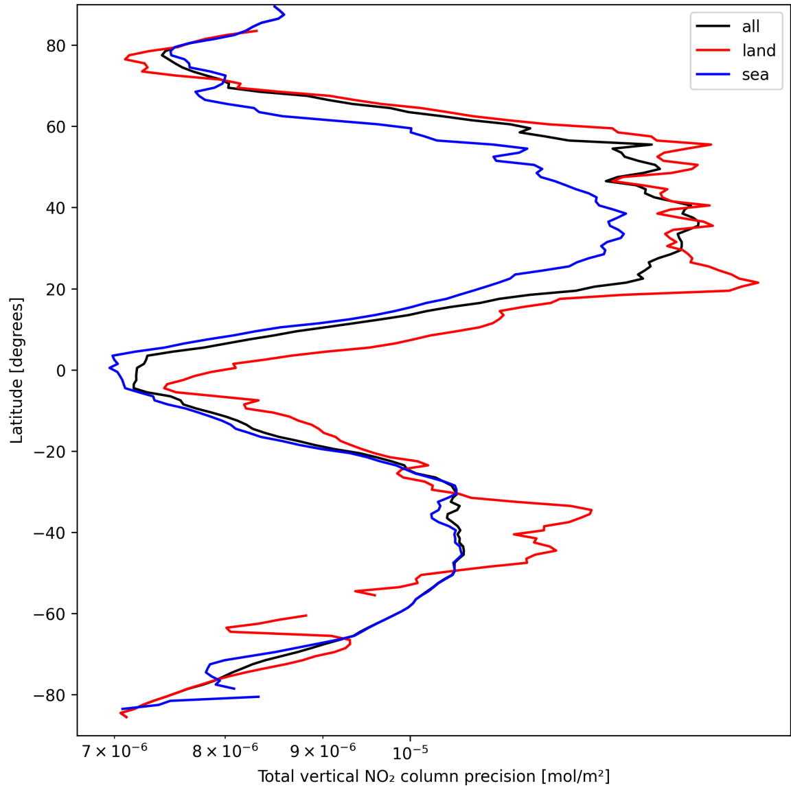
Figure 20: Zonal average of “Total vertical NO 2 column precision” for 2025-03-26 to 2025-03-26.
