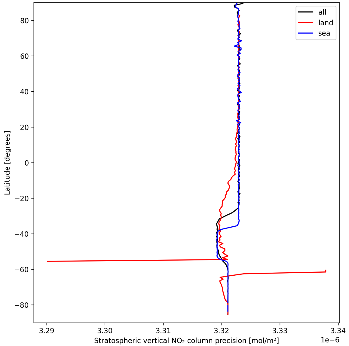
Figure 18: Zonal average of "Stratospheric vertical NO 2 column precision" for 2025-03-26 to 2025-03-26.
