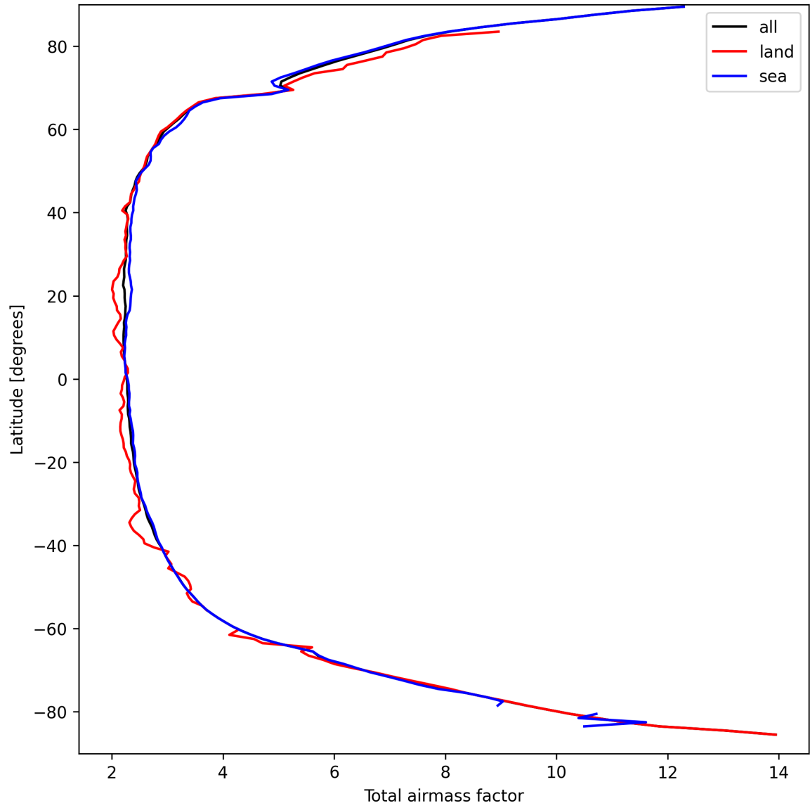
Figure 13: Zonal average of “Total airmass factor” for 2025-03-26 to 2025-03-26.
