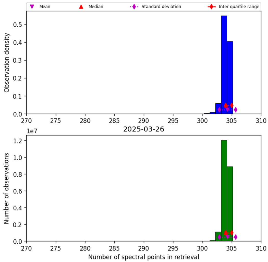
Figure 31: Histogram of “Number of spectral points in retrieval” for 2025-03-26 to 2025-03-26
