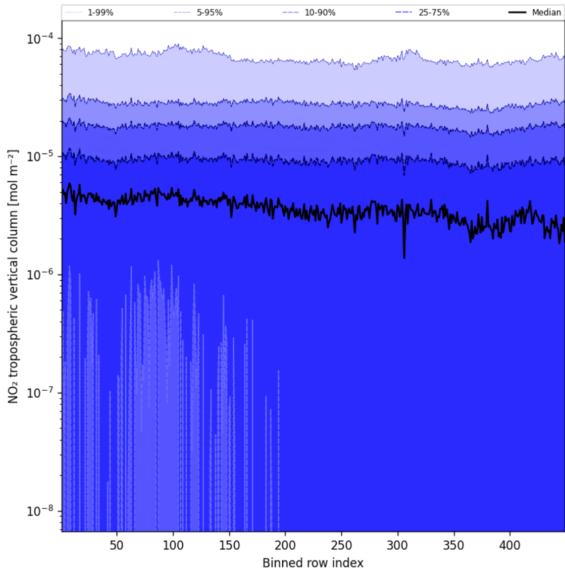
Figure 44: Along track statistics of “NO 2 tropospheric vertical column” for 2025-03-26 to 2025-03-26
