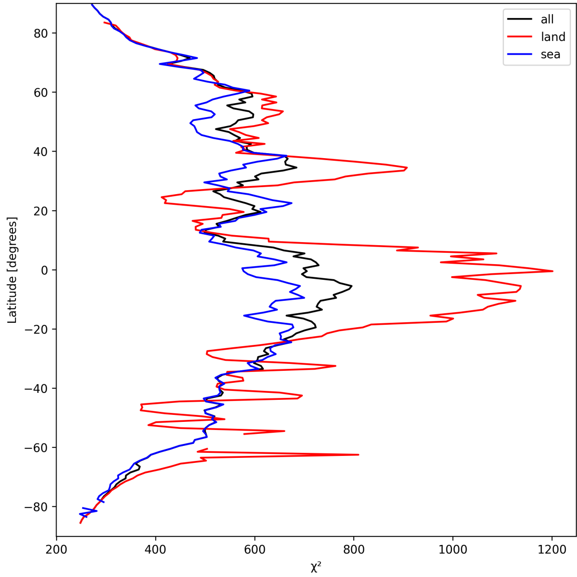
Figure 23: Zonal average of “ \chi^2 ” for 2025-03-26 to 2025-03-26.
