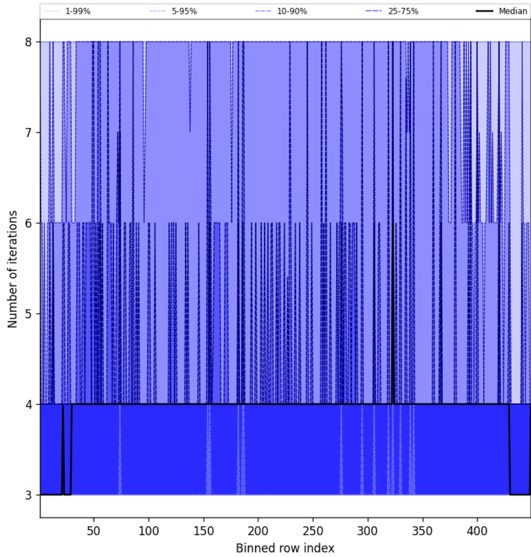
Figure 49: Along track statistics of “Number of iterations” for 2025-03-26 to 2025-03-26
