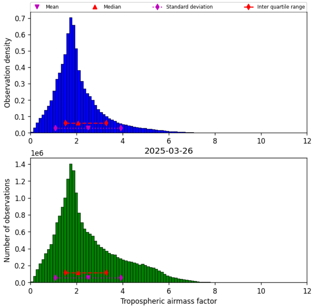
Figure 29: Histogram of “Tropospheric airmass factor” for 2025-03-26 to 2025-03-26
