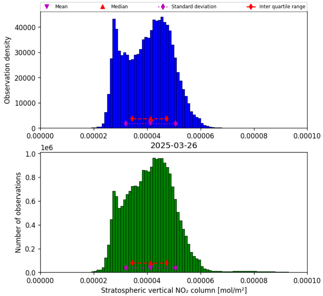
Figure 34: Histogram of “Stratospheric vertical NO 2 column” for 2025-03-26 to 2025-03-26
