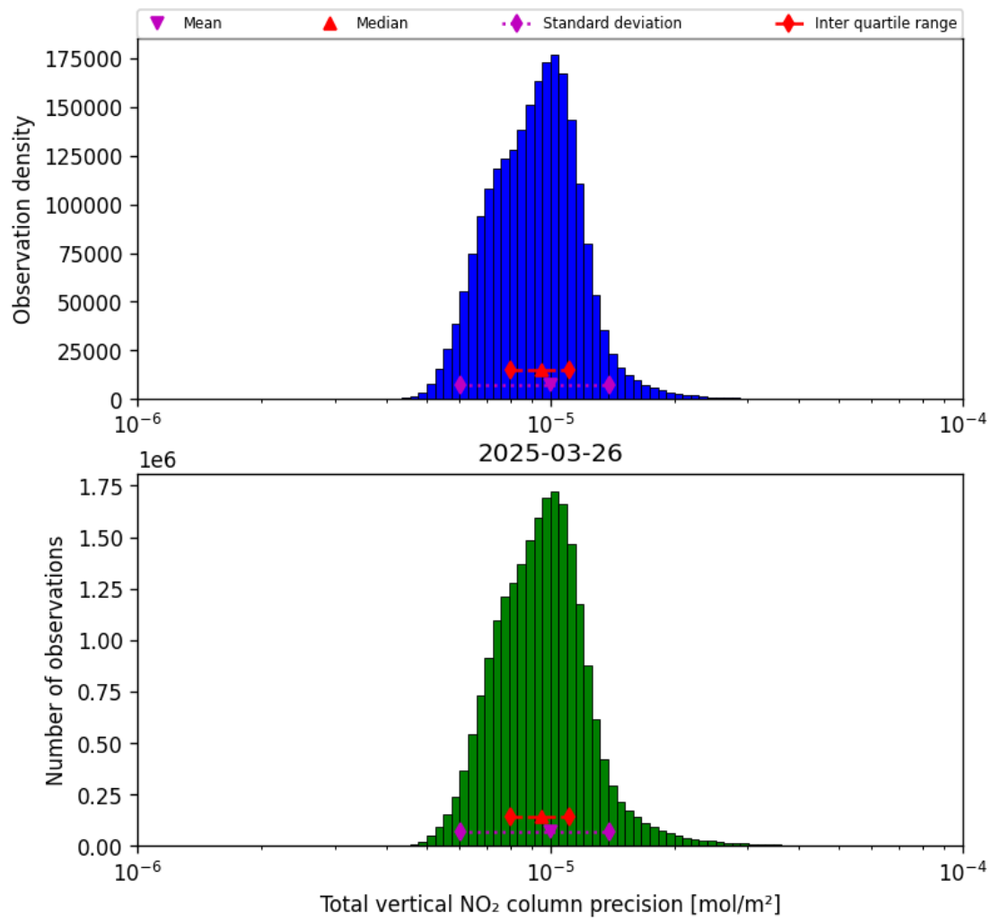
Figure 37: Histogram of "Total vertical NO 2 column precision" for 2025-03-26 to 2025-03-26
