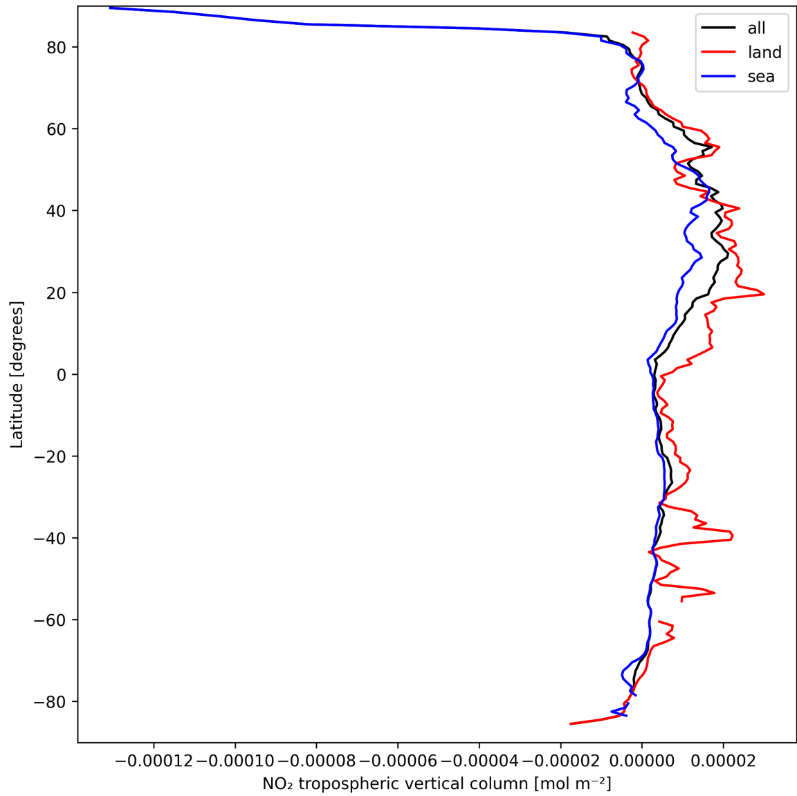
Figure 10: Zonal average of “NO 2 tropospheric vertical column” for 2025-03-26 to 2025-03-26.
