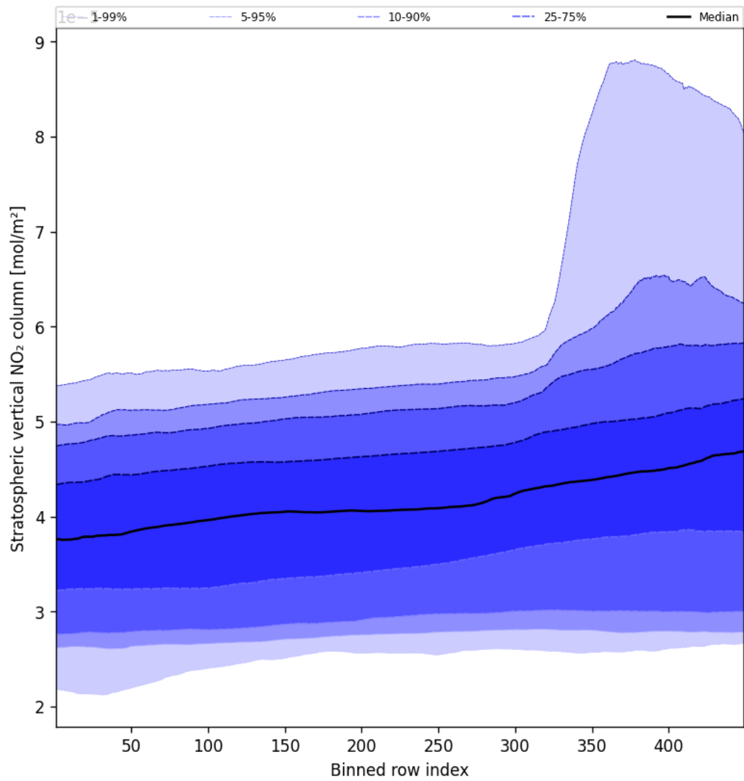
Figure 51: Along track statistics of “Stratospheric vertical NO 2 column” for 2025-03-26 to 2025-03-26
