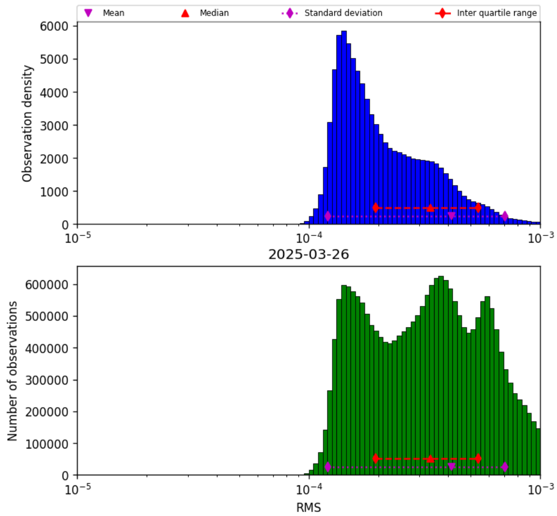
Figure 41: Histogram of “RMS” for 2025-03-26 to 2025-03-26
