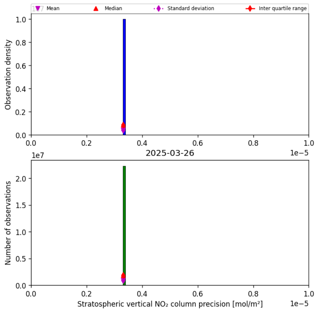
Figure 35: Histogram of “Stratospheric vertical NO 2 column precision” for 2025-03-26 to 2025-03-26
