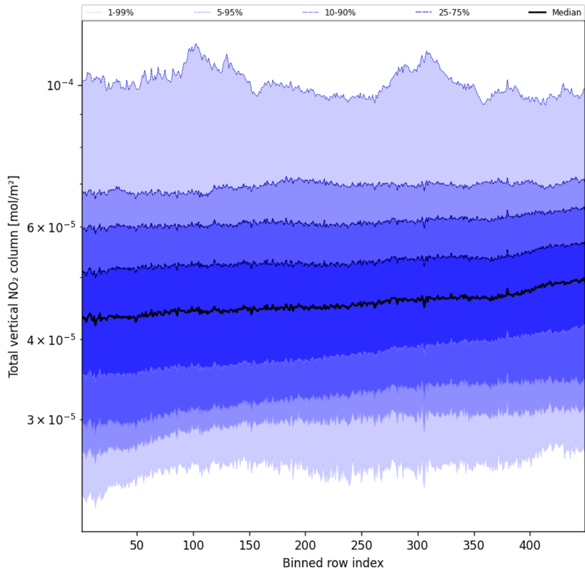
Figure 53: Along track statistics of “Total vertical NO 2 column” for 2025-03-26 to 2025-03-26
