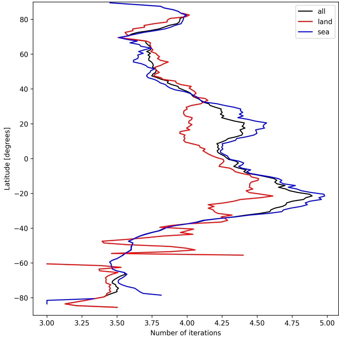
Figure 15: Zonal average of “Number of iterations” for 2025-03-26 to 2025-03-26.
