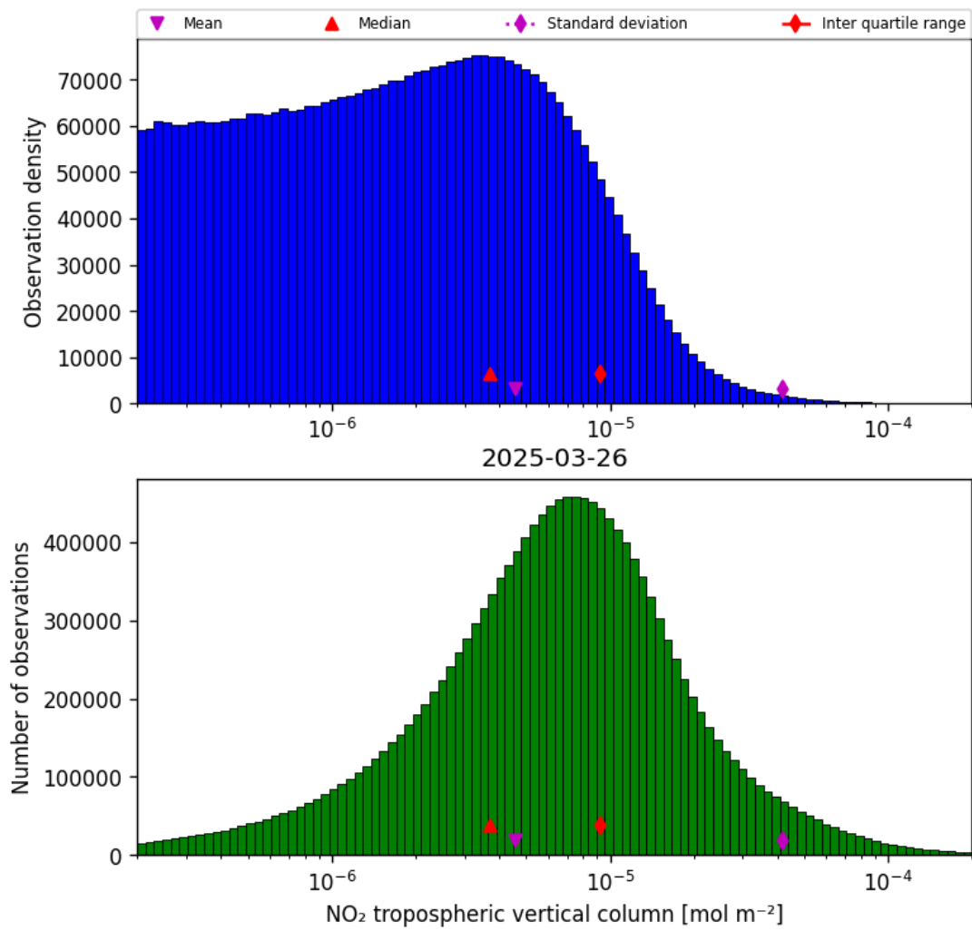
Figure 27: Histogram of “NO 2 tropospheric vertical column” for 2025-03-26 to 2025-03-26
