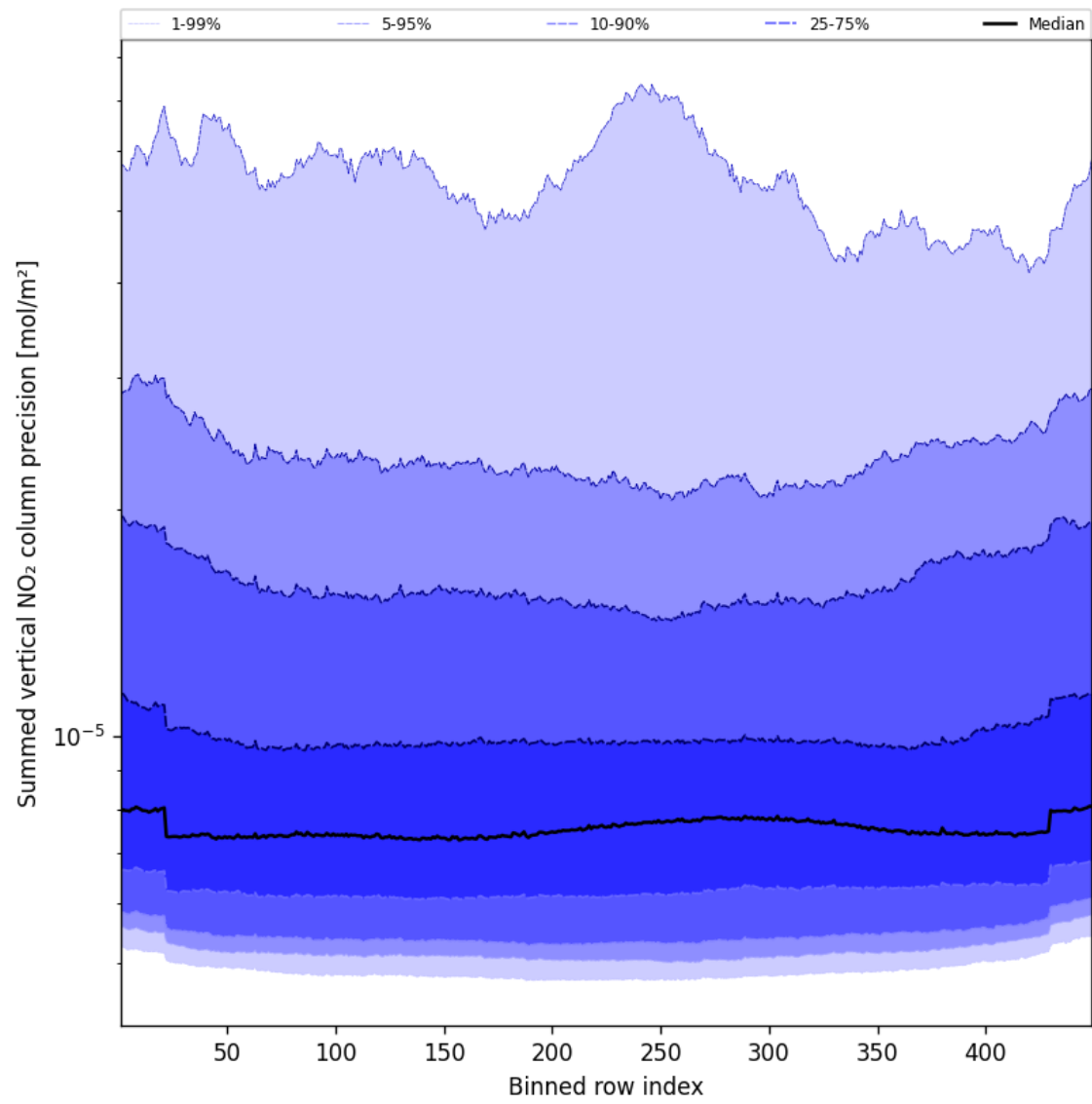
Figure 56: Along track statistics of “Summed vertical NO 2 column precision” for 2025-03-26 to 2025-03-26
