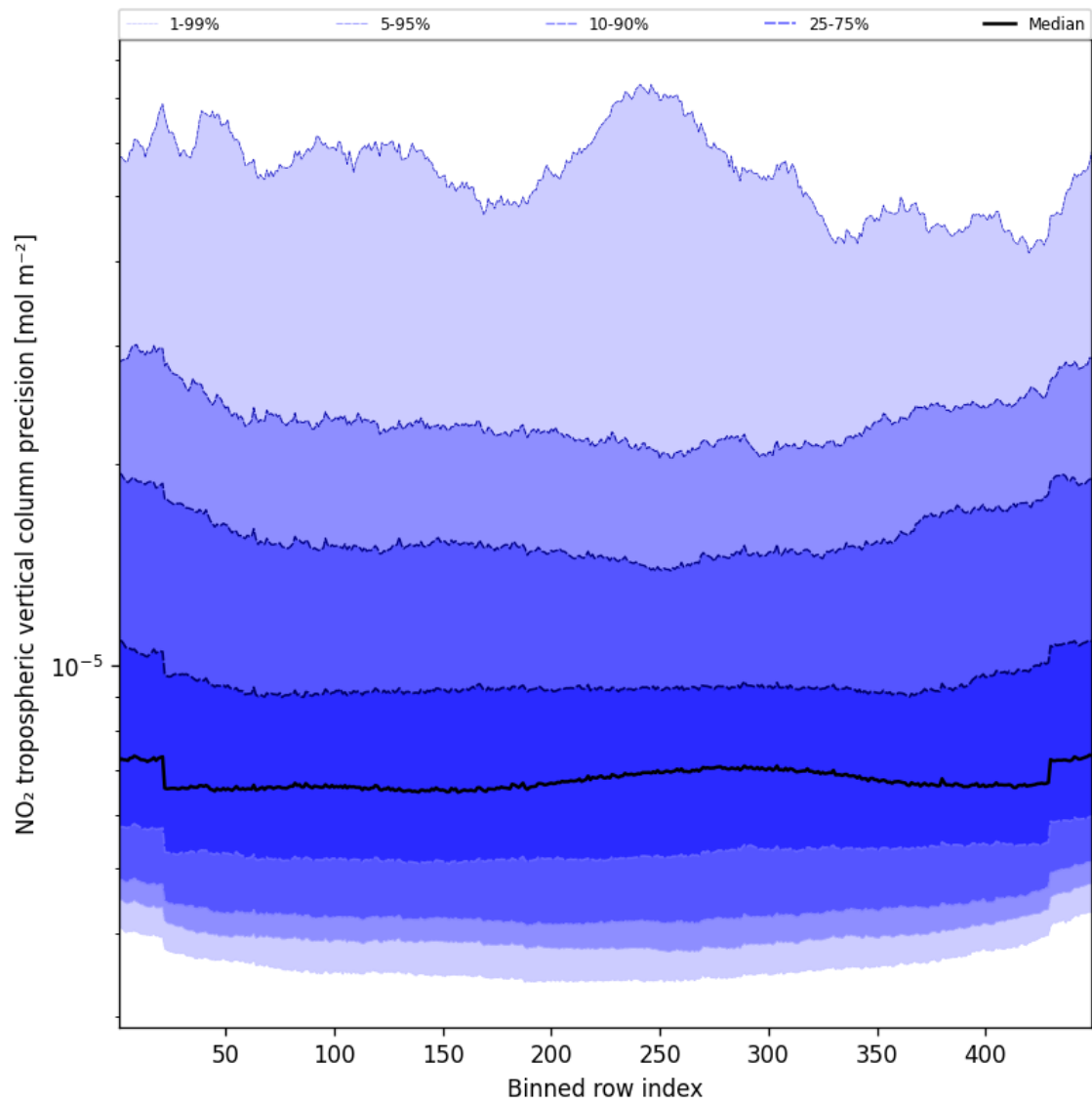
Figure 45: Along track statistics of “NO 2 tropospheric vertical column precision” for 2025-03-26 to 2025-03-26
