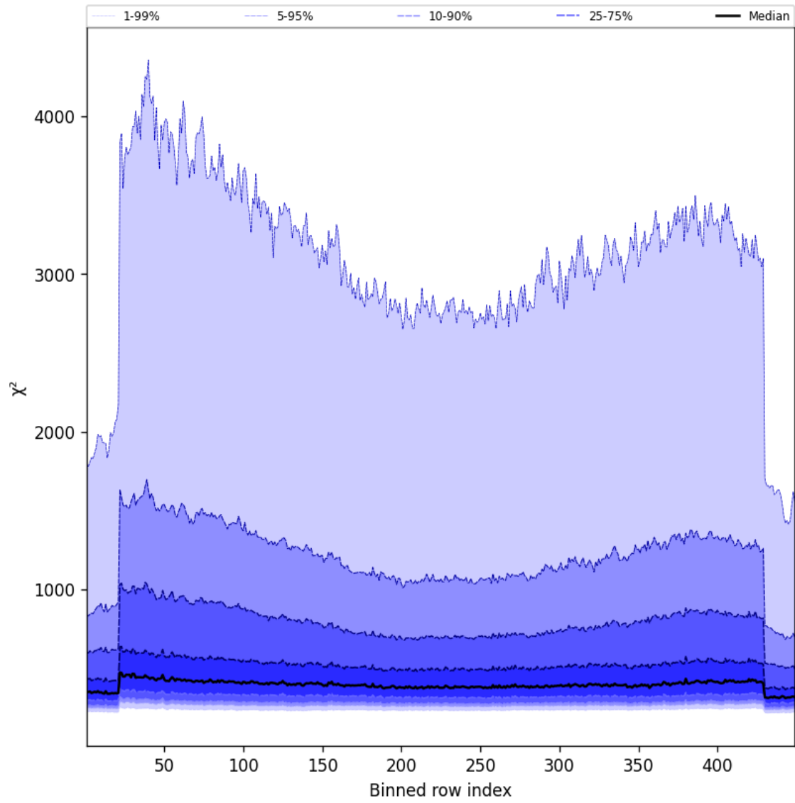
Figure 57: Along track statistics of “ \chi^2 ” for 2025-03-26 to 2025-03-26
