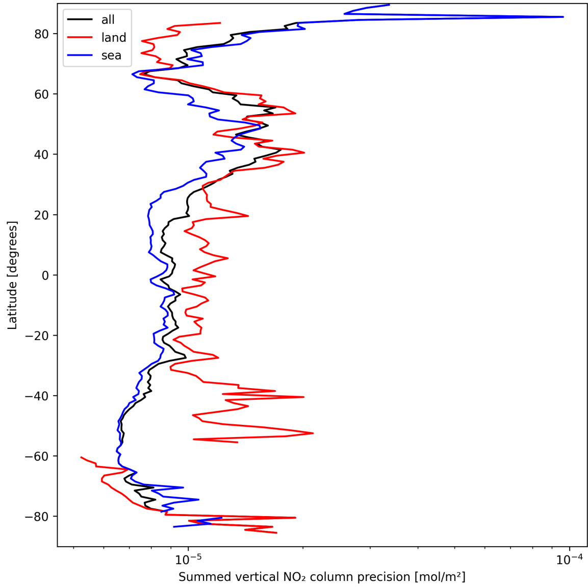
Figure 22: Zonal average of “Summed vertical NO 2 column precision” for 2025-03-26 to 2025-03-26.
