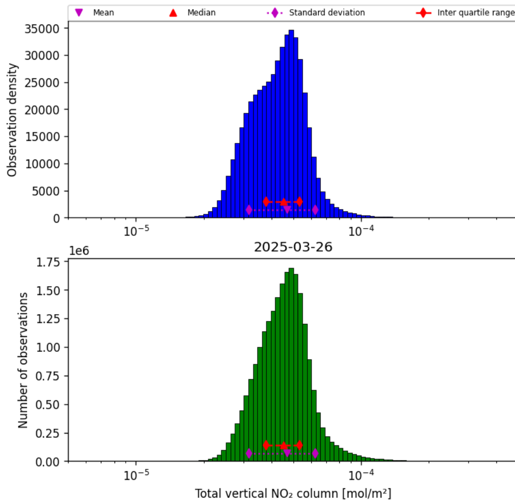
Figure 36: Histogram of "Total vertical NO 2 column" for 2025-03-26 to 2025-03-26
