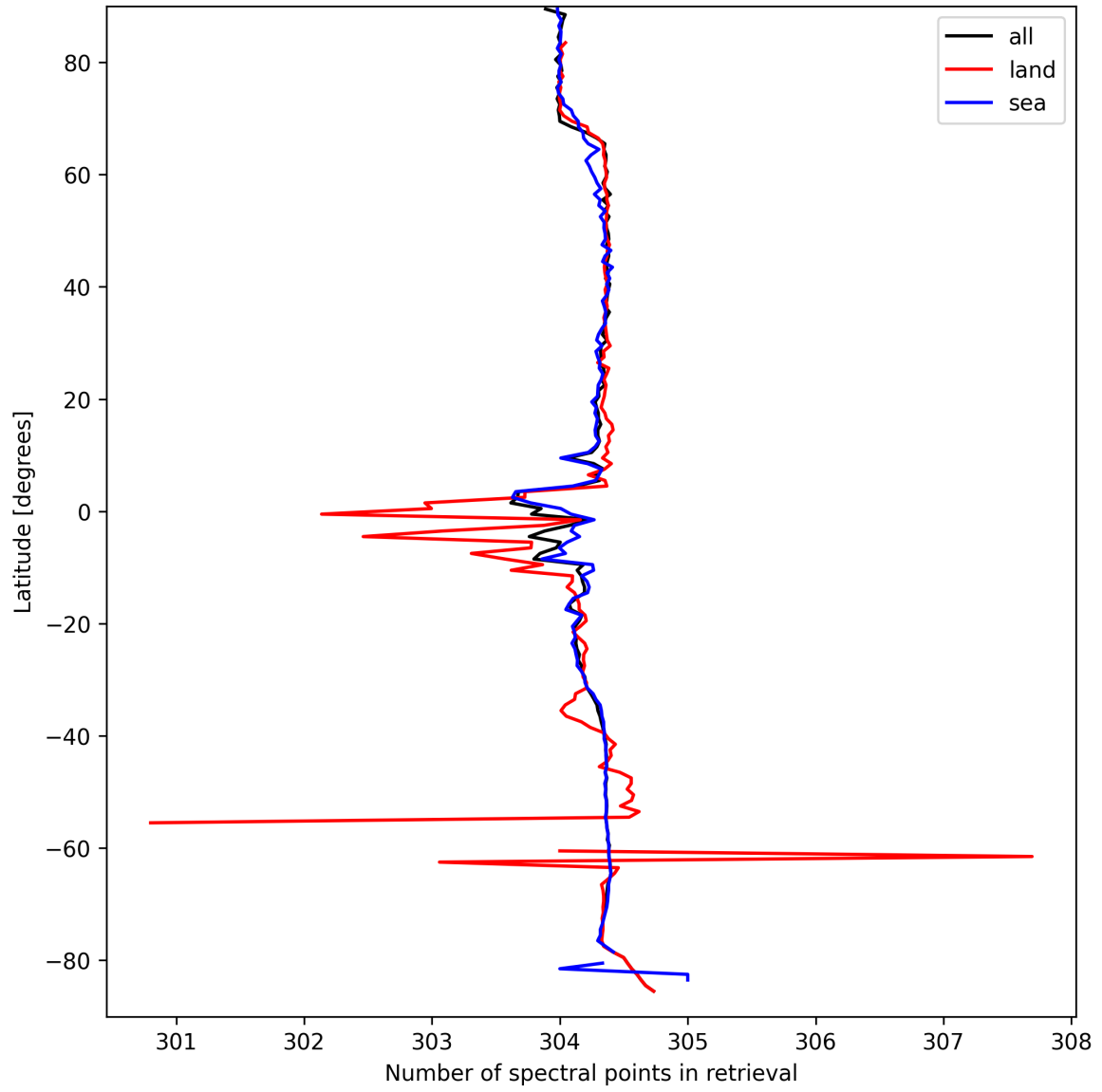
Figure 14: Zonal average of “Number of spectral points in retrieval” for 2025-03-26 to 2025-03-26.
