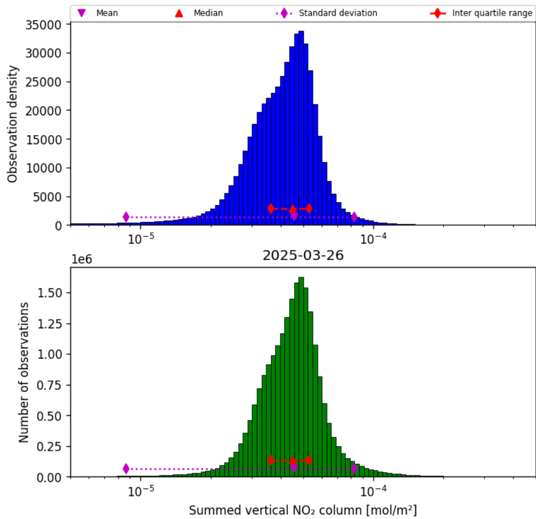
Figure 38: Histogram of “Summed vertical NO 2 column” for 2025-03-26 to 2025-03-26
