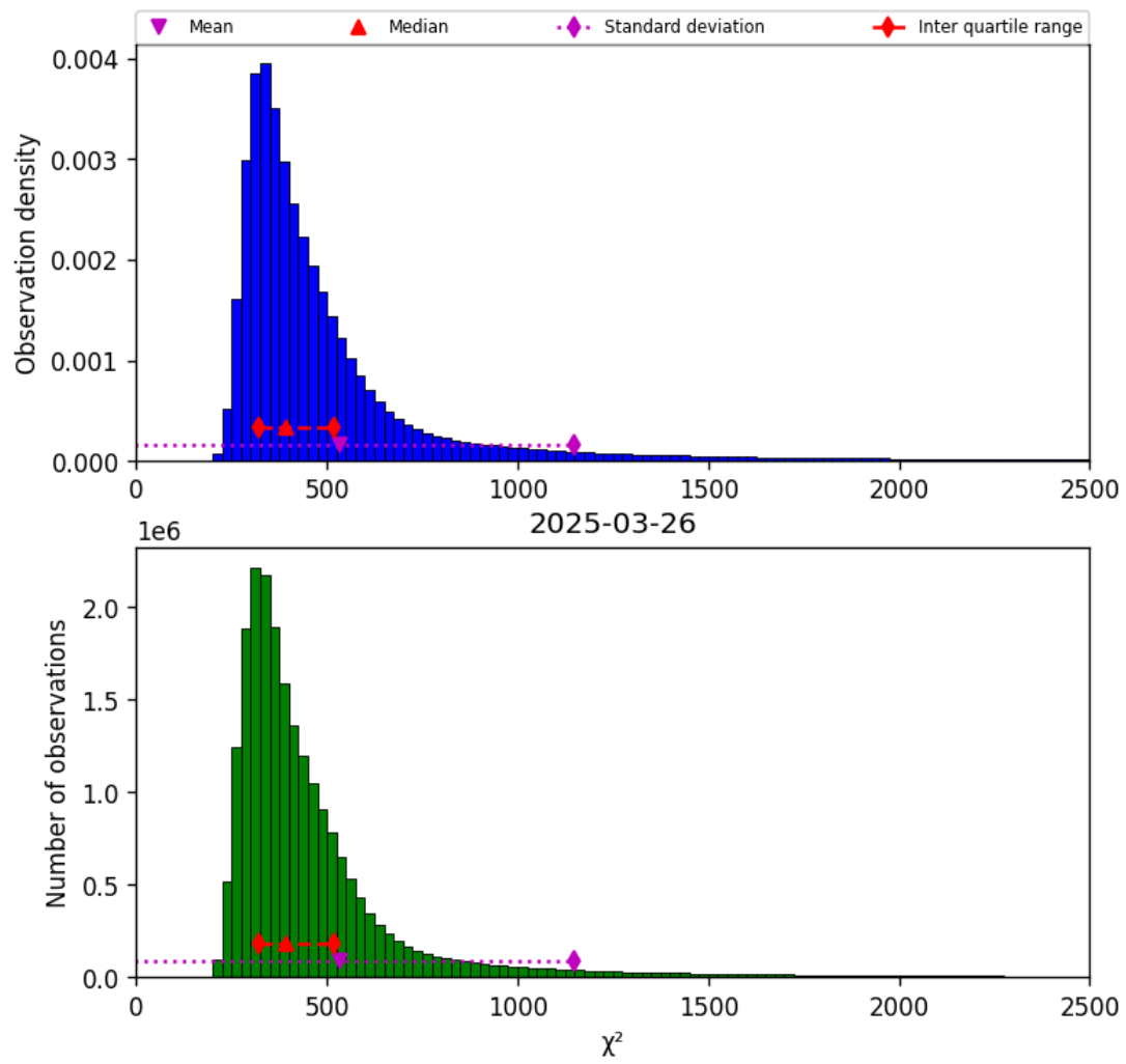
Figure 40: Histogram of " \chi^2 " for 2025-03-26 to 2025-03-26
