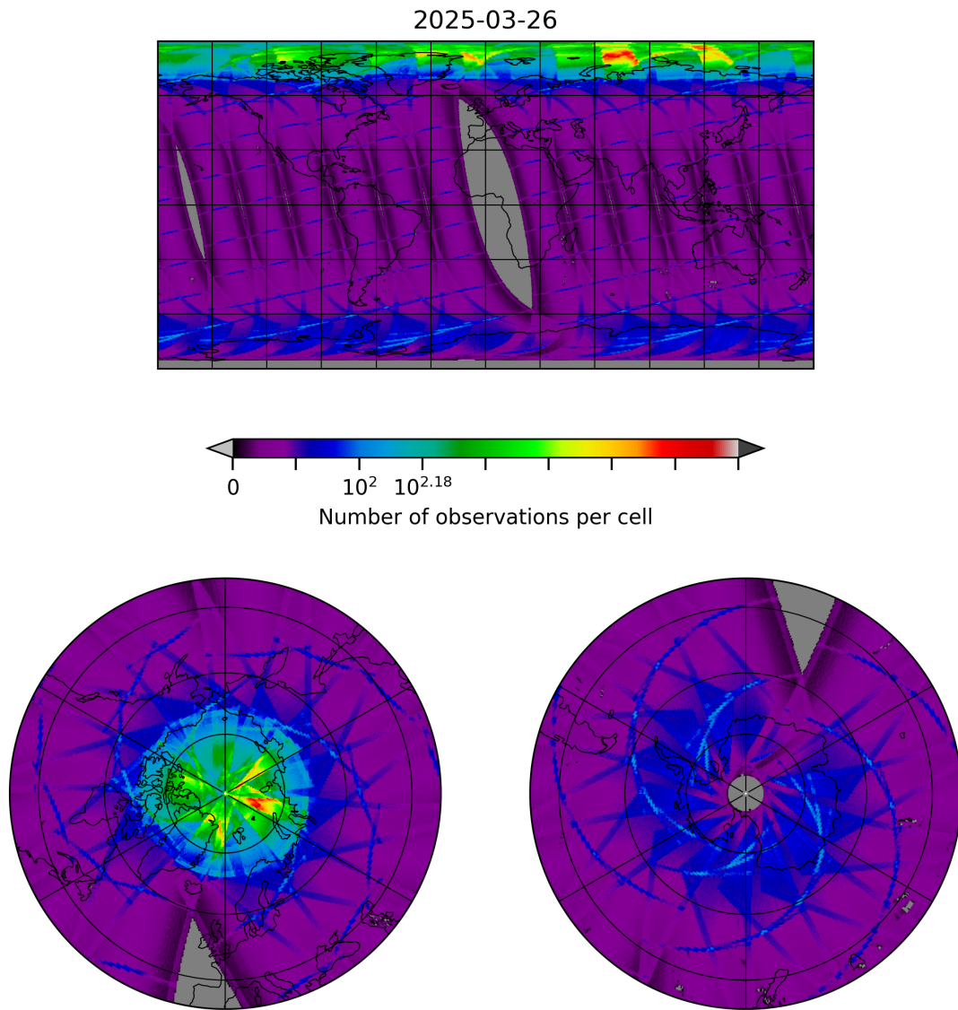
Figure 8: Map of the number of observations for 2025-03-26 to 2025-03-26
