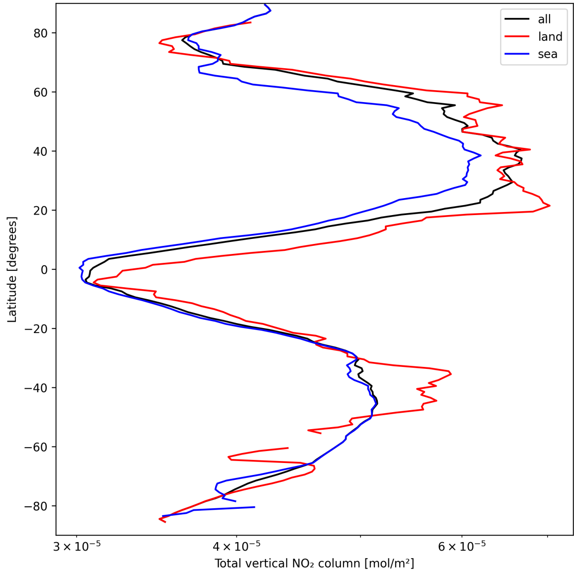
Figure 19: Zonal average of “Total vertical NO 2 column” for 2025-03-26 to 2025-03-26.
