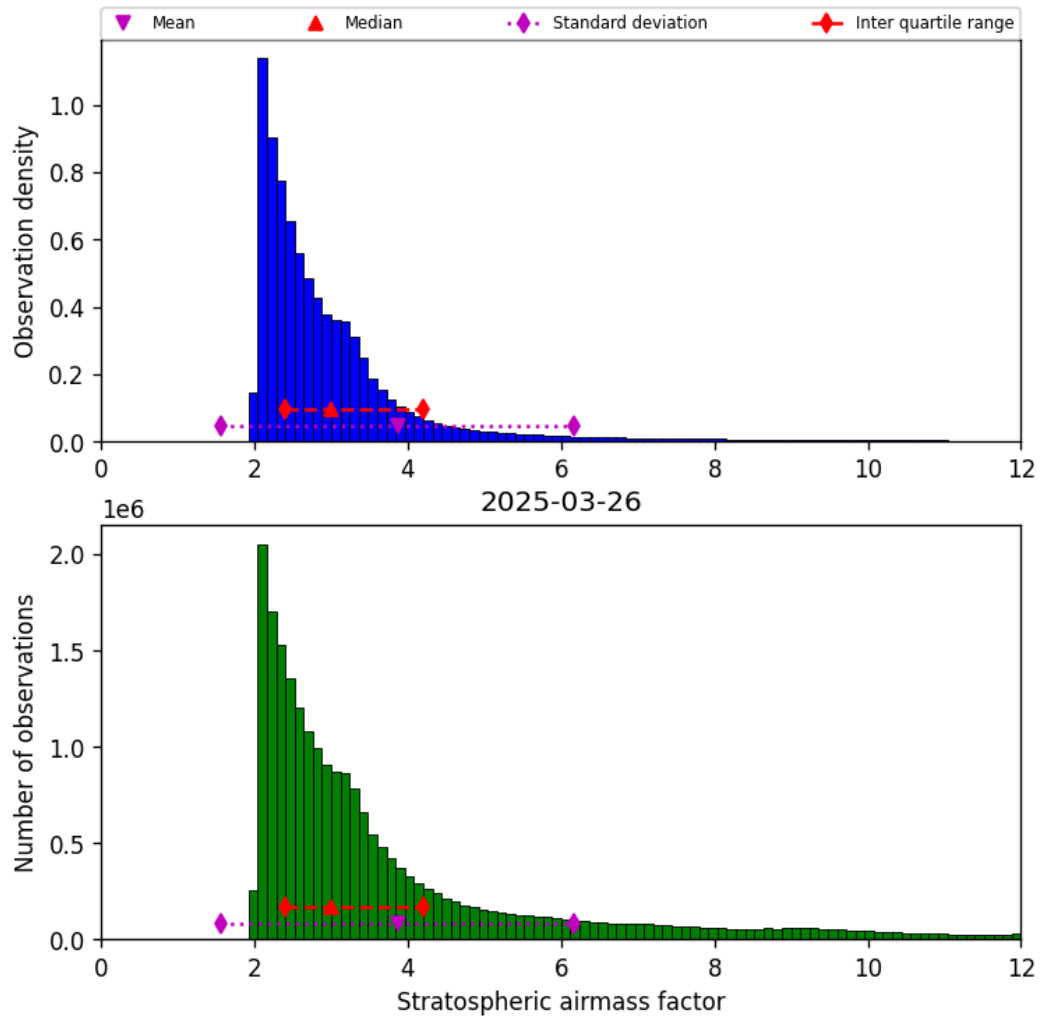
Figure 42: Histogram of “Stratospheric airmass factor” for 2025-03-26 to 2025-03-26
