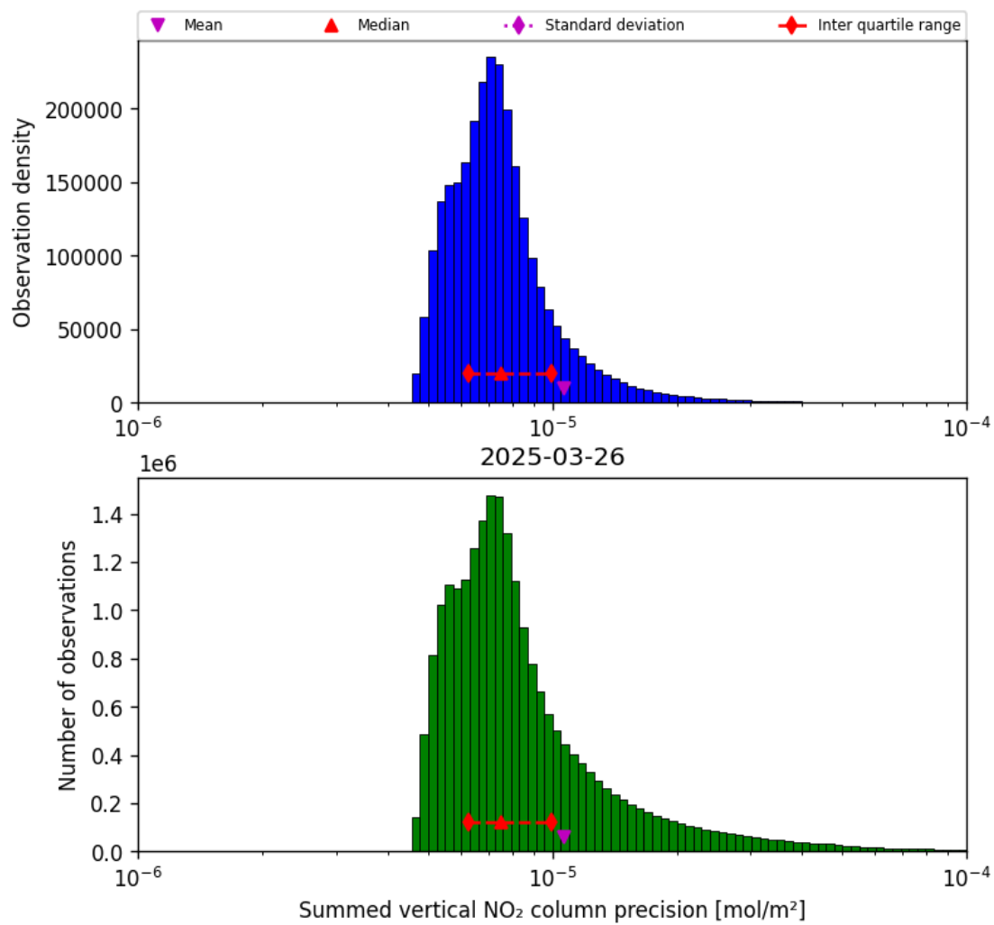
Figure 39: Histogram of "Summed vertical NO 2 column precision" for 2025-03-26 to 2025-03-26
