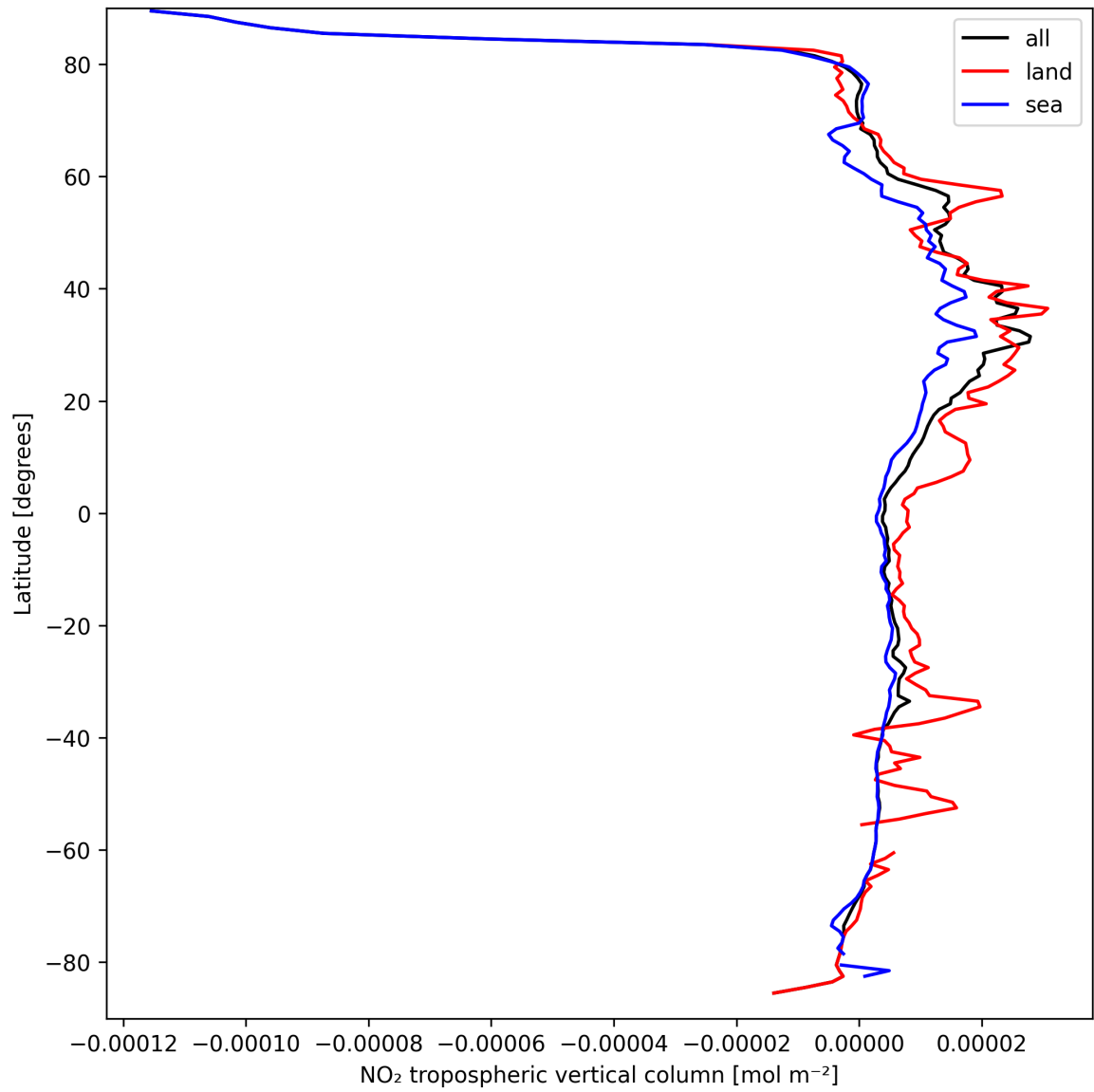
Figure 10: Zonal average of “NO 2 tropospheric vertical column” for 2025-03-27 to 2025-03-28.
