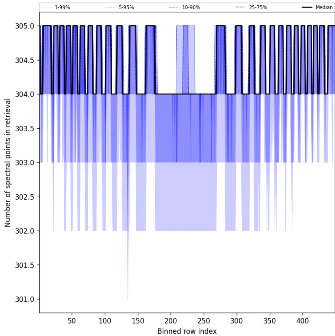
Figure 48: Along track statistics of “Number of spectral points in retrieval” for 2025-03-27 to 2025-03-28
