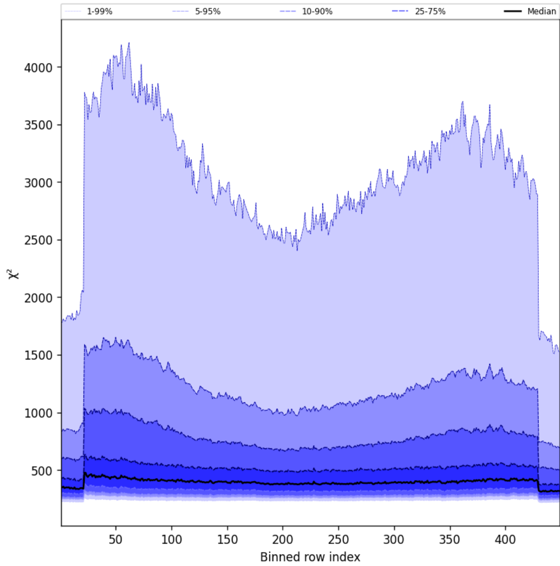
Figure 57: Along track statistics of “ \chi^2 ” for 2025-03-27 to 2025-03-28
