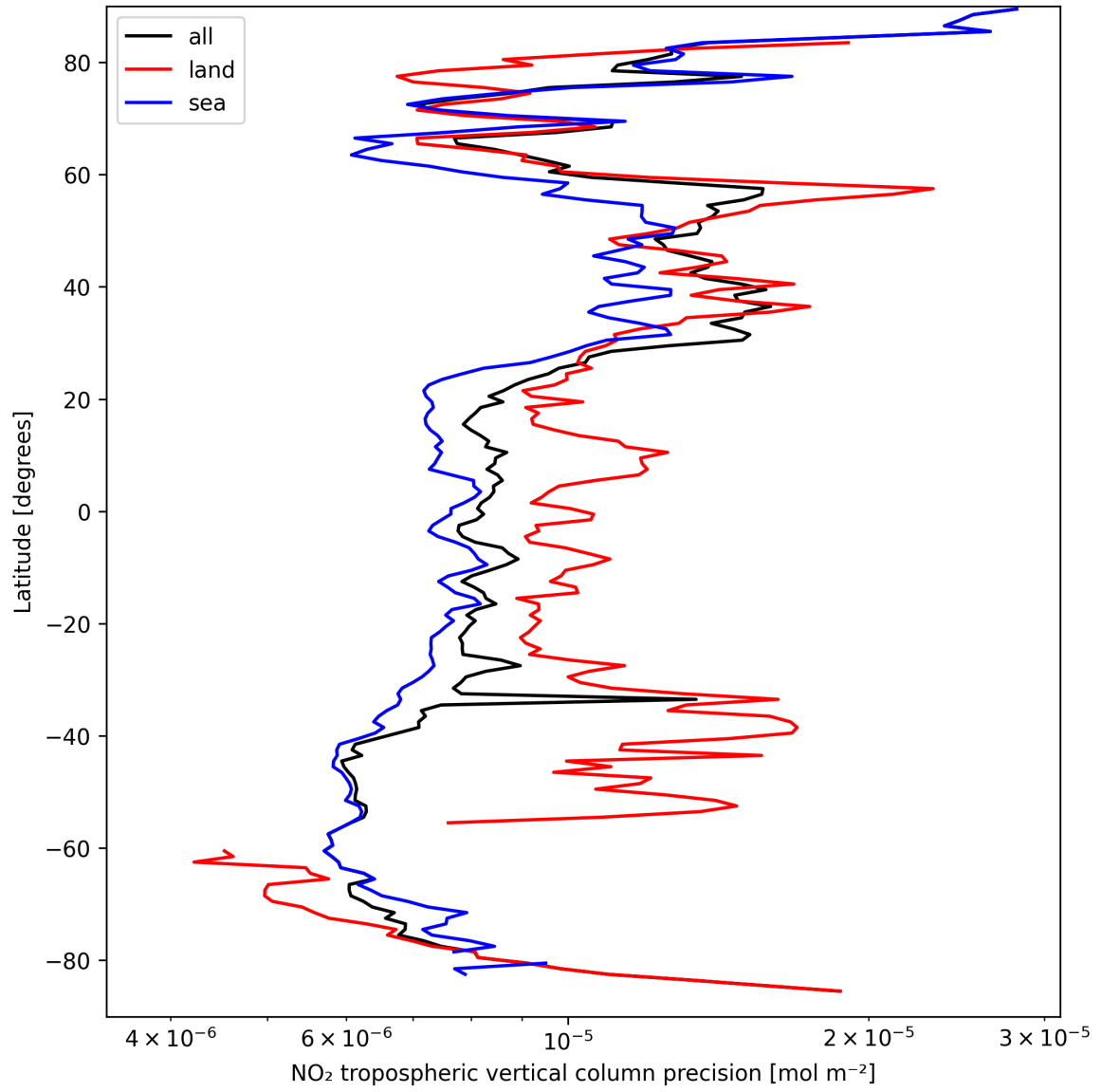
Figure 11: Zonal average of “NO 2 tropospheric vertical column precision” for 2025-03-27 to 2025-03-28.
