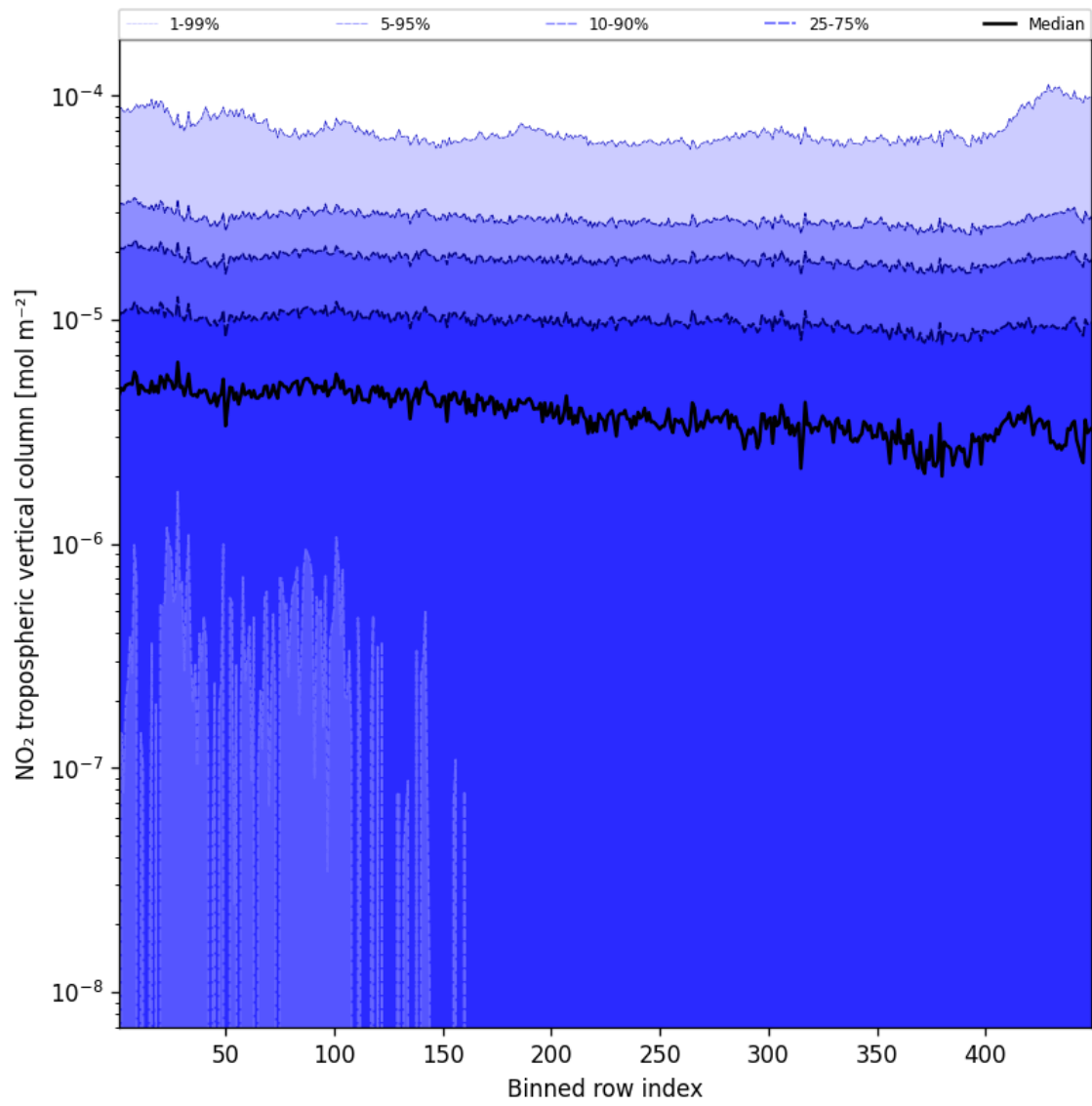
Figure 44: Along track statistics of “NO 2 tropospheric vertical column” for 2025-03-27 to 2025-03-28
