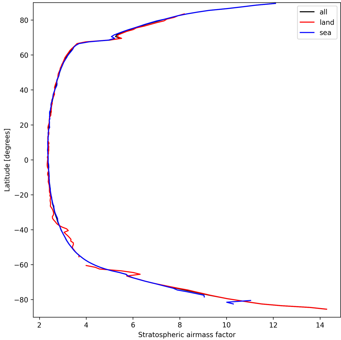
Figure 25: Zonal average of “Stratospheric air mass factor” for 2025-03-27 to 2025-03-28.
