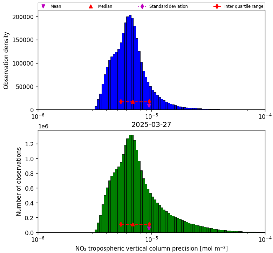
Figure 28: Histogram of “NO 2 tropospheric vertical column precision” for 2025-03-27 to 2025-03-28
