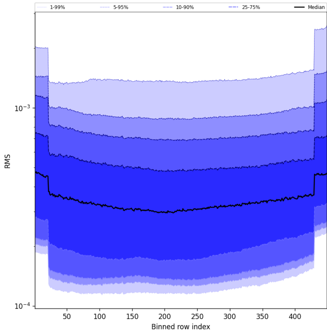
Figure 58: Along track statistics of “RMS” for 2025-03-27 to 2025-03-28
