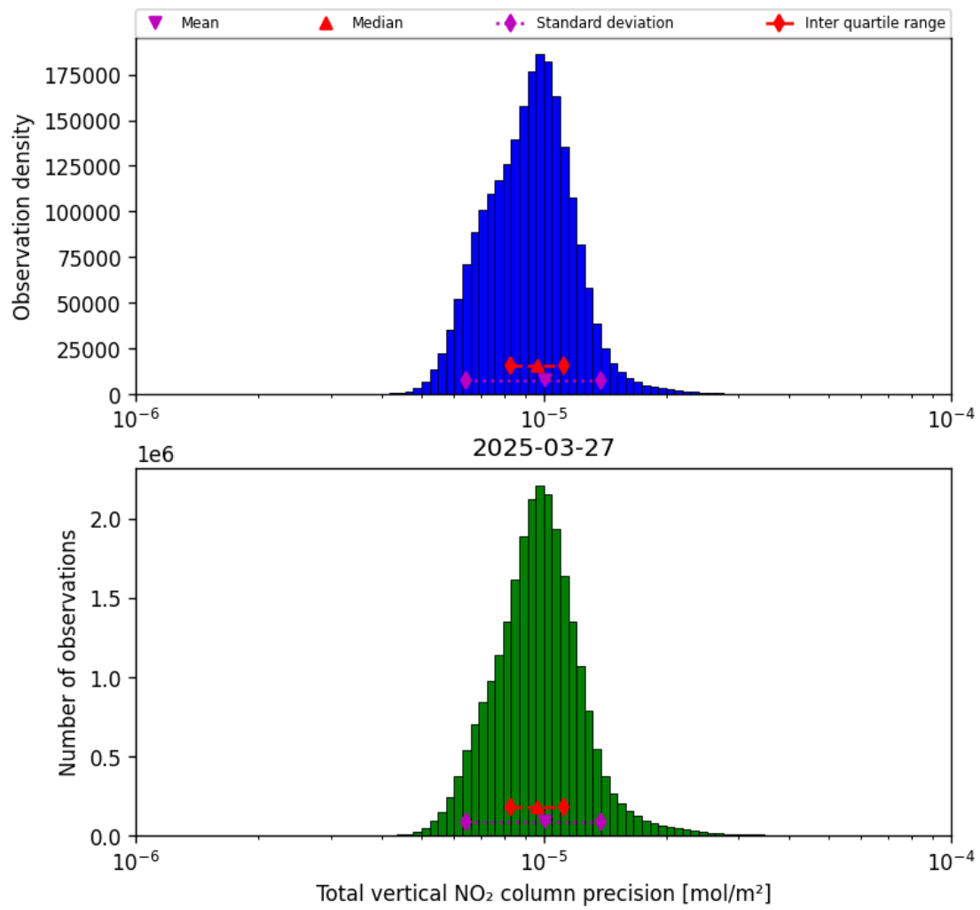
Figure 37: Histogram of “Total vertical NO 2 column precision” for 2025-03-27 to 2025-03-28
