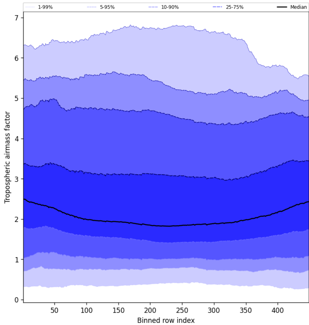
Figure 46: Along track statistics of “Tropospheric airmass factor” for 2025-03-27 to 2025-03-28
