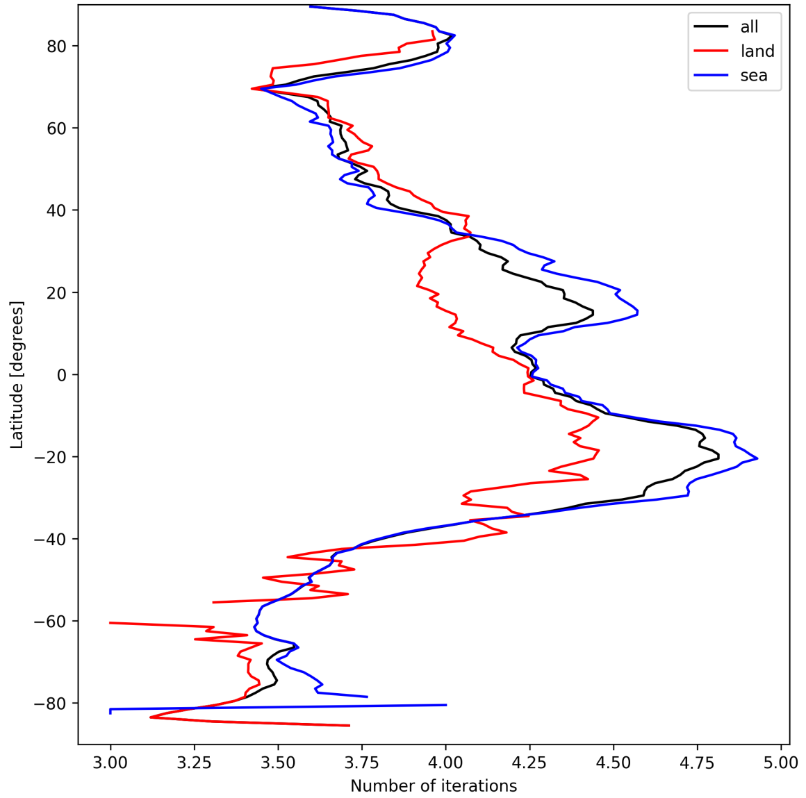
Figure 15: Zonal average of “Number of iterations” for 2025-03-27 to 2025-03-28.
