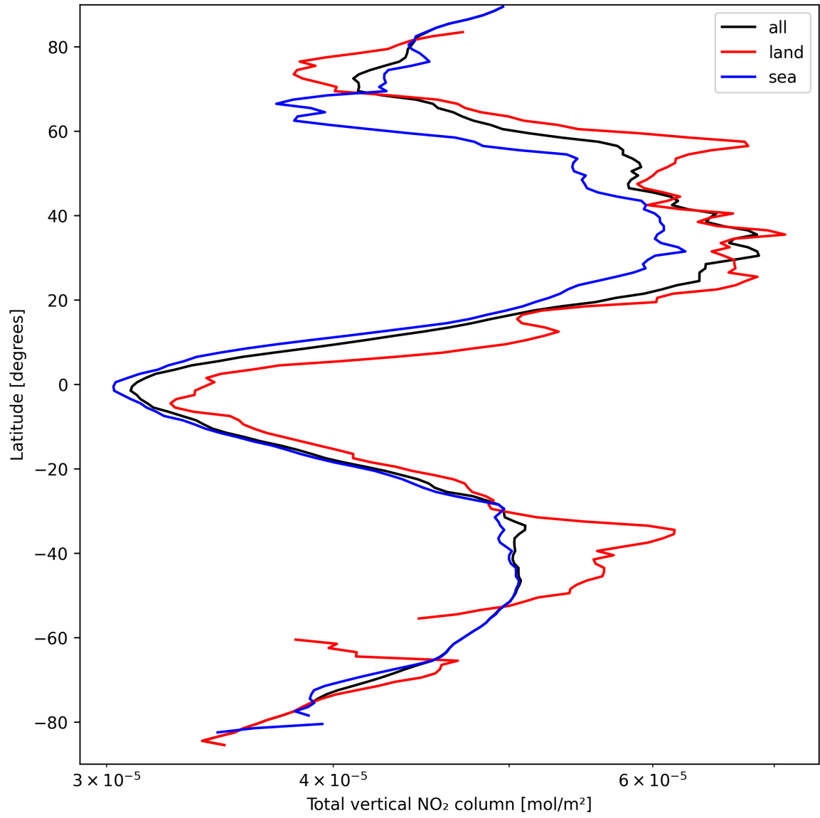
Figure 19: Zonal average of “Total vertical NO 2 column” for 2025-03-27 to 2025-03-28.
