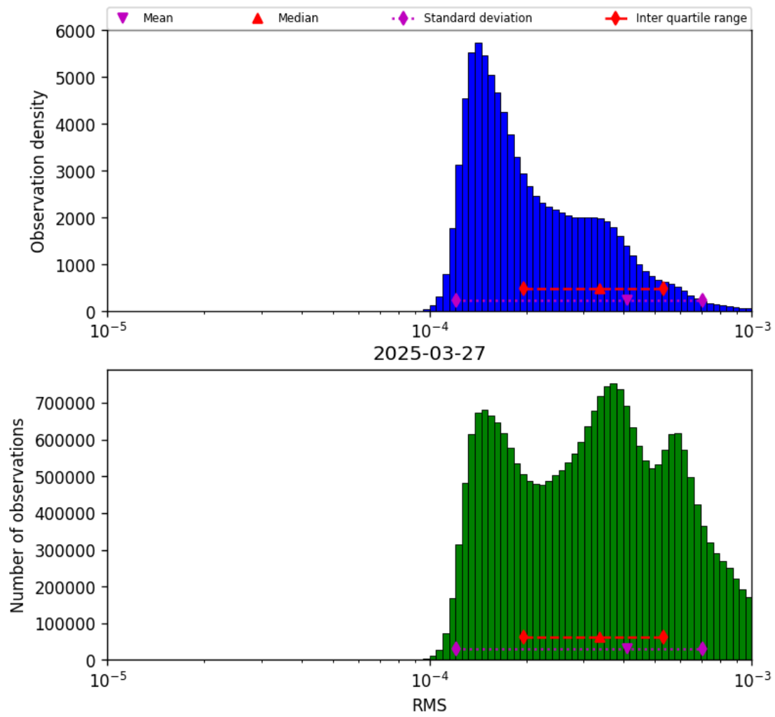
Figure 41: Histogram of “RMS” for 2025-03-27 to 2025-03-28
