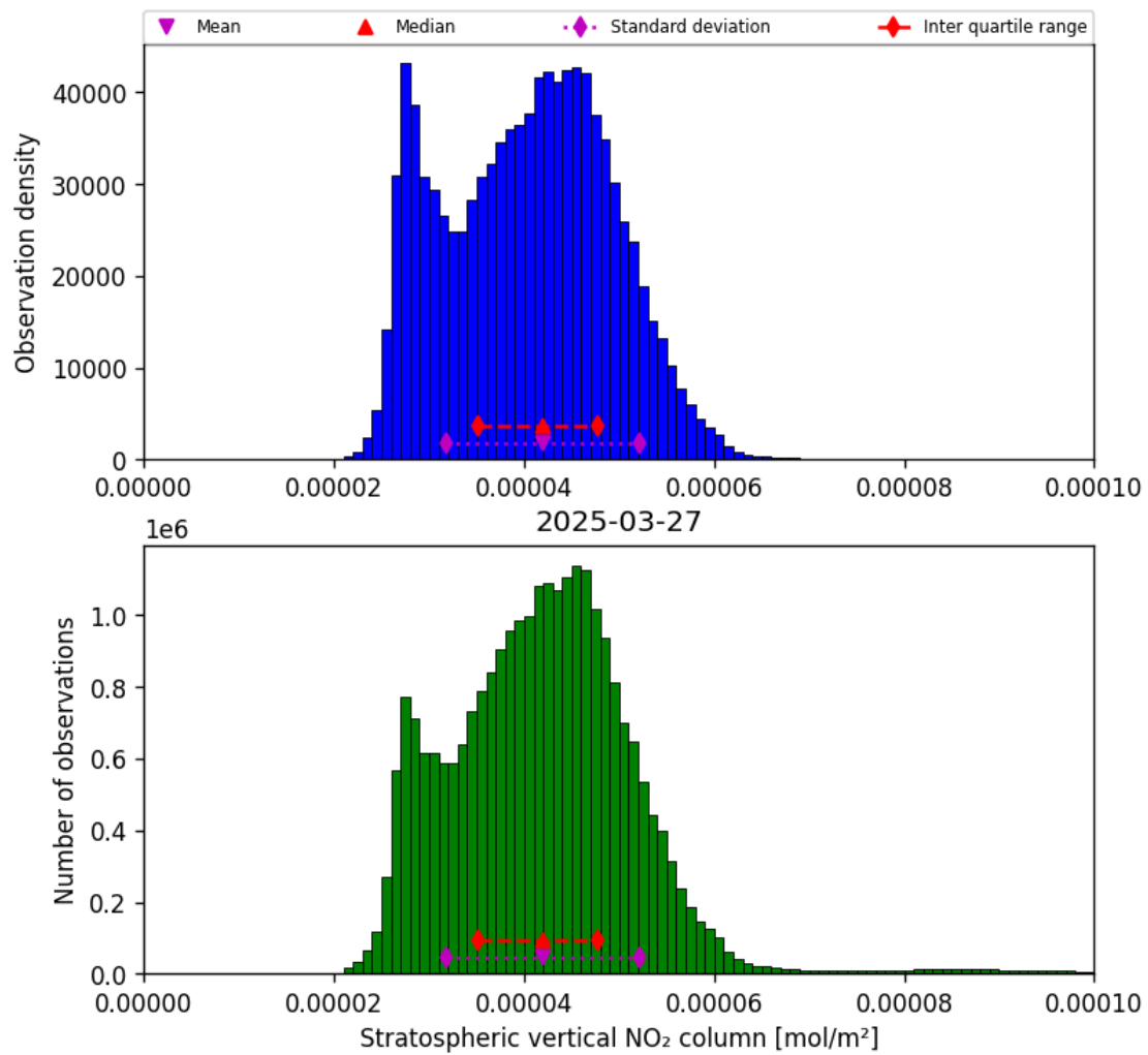
Figure 34: Histogram of “Stratospheric vertical NO 2 column” for 2025-03-27 to 2025-03-28
