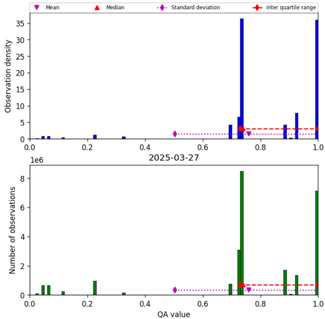
Figure 26: Histogram of “QA value” for 2025-03-27 to 2025-03-28
