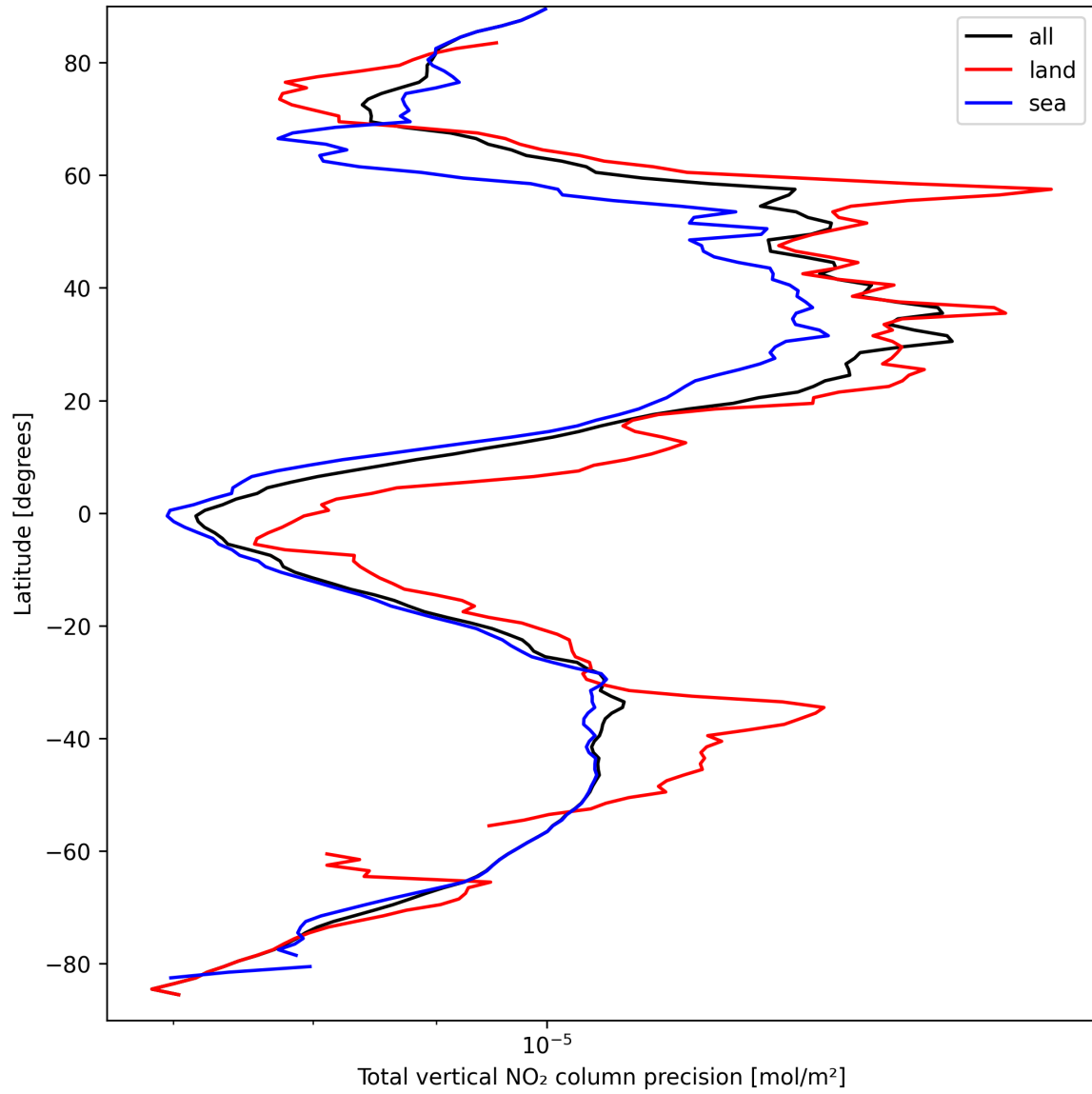
Figure 20: Zonal average of “Total vertical NO 2 column precision” for 2025-03-27 to 2025-03-28.
