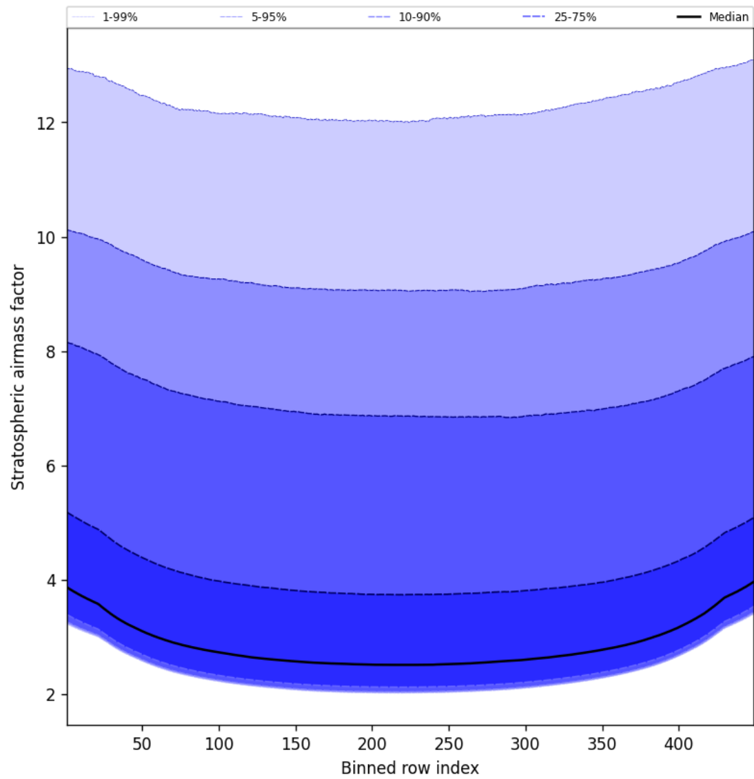
Figure 59: Along track statistics of “Stratospheric airmass factor” for 2025-03-27 to 2025-03-28
