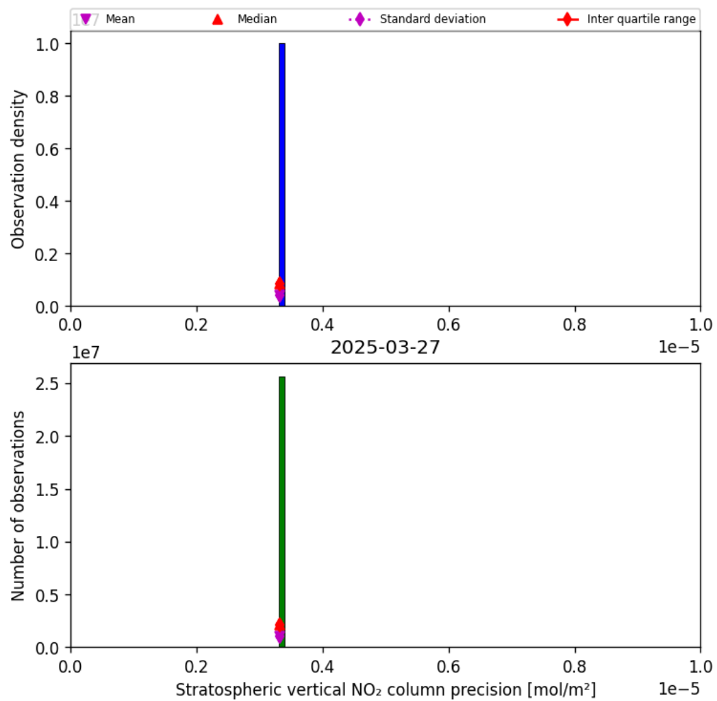
Figure 35: Histogram of “Stratospheric vertical NO 2 column precision” for 2025-03-27 to 2025-03-28
