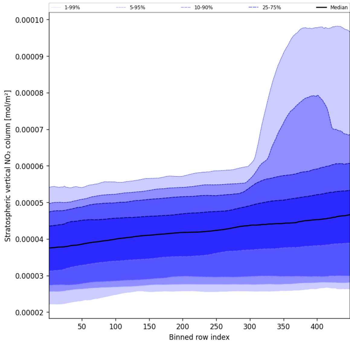
Figure 51: Along track statistics of “Stratospheric vertical NO 2 column” for 2025-03-27 to 2025-03-28
