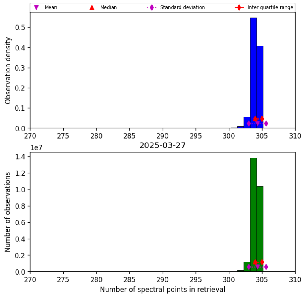
Figure 31: Histogram of “Number of spectral points in retrieval” for 2025-03-27 to 2025-03-28
