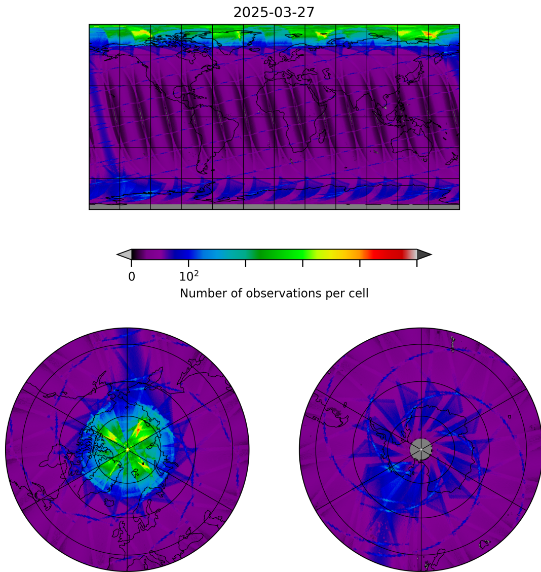
Figure 8: Map of the number of observations for 2025-03-27 to 2025-03-28
