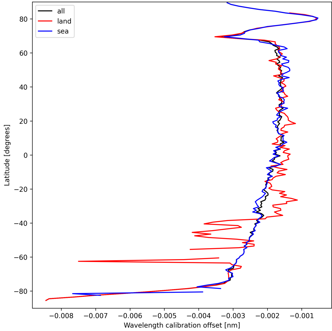
Figure 16: Zonal average of “Wavelength calibration offset” for 2025-03-27 to 2025-03-28.
