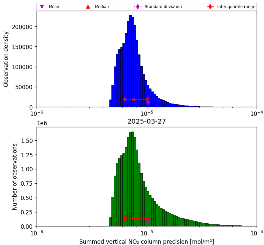
Figure 39: Histogram of “Summed vertical NO 2 column precision” for 2025-03-27 to 2025-03-28
