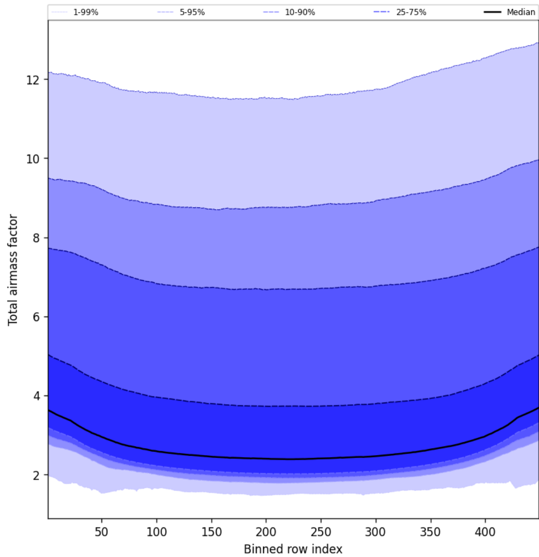
Figure 47: Along track statistics of “Total airmass factor” for 2025-03-27 to 2025-03-28
