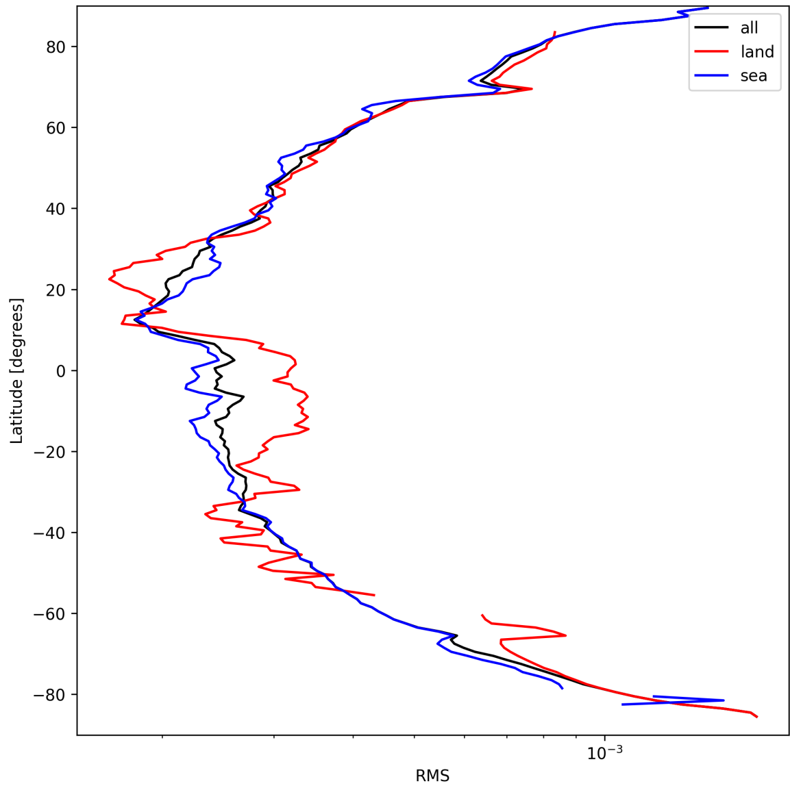
Figure 24: Zonal average of “RMS” for 2025-03-27 to 2025-03-28.
