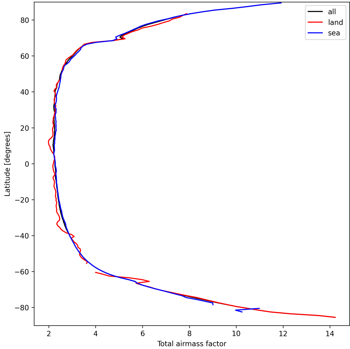
Figure 13: Zonal average of “Total airmass factor” for 2025-03-27 to 2025-03-28.
