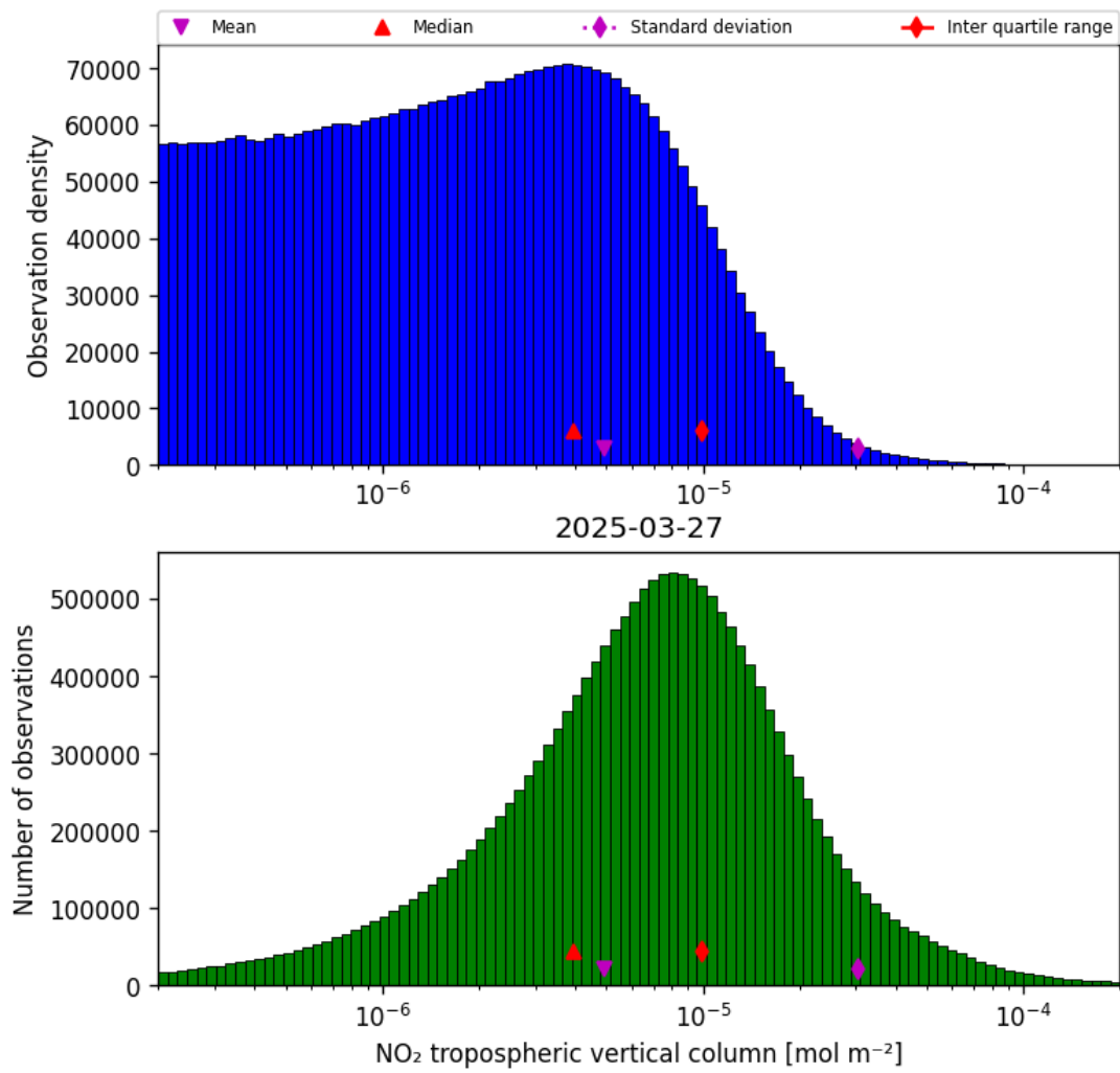
Figure 27: Histogram of “NO 2 tropospheric vertical column” for 2025-03-27 to 2025-03-28
