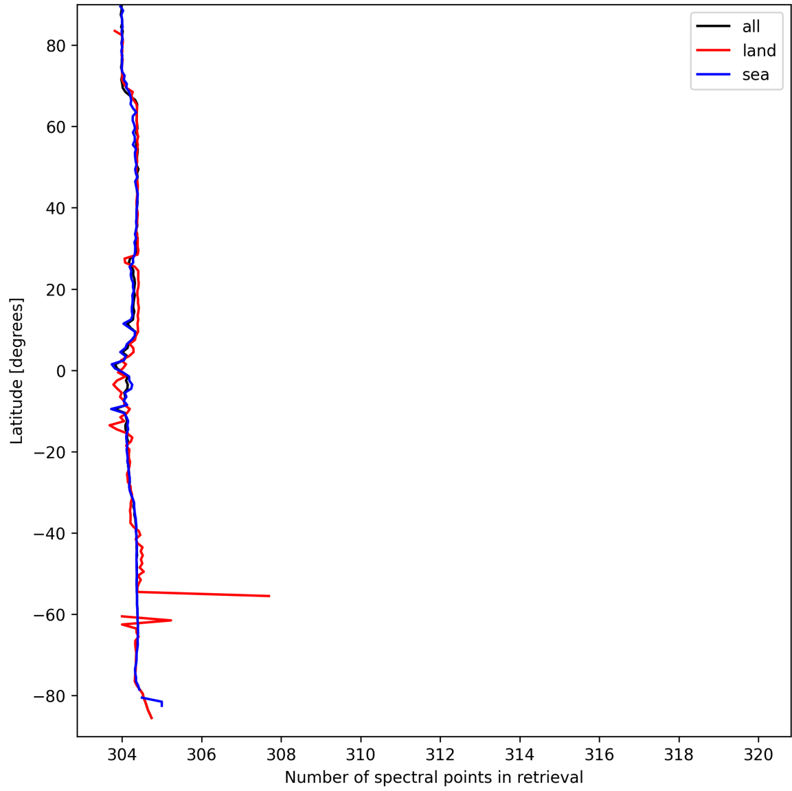
Figure 14: Zonal average of “Number of spectral points in retrieval” for 2025-03-27 to 2025-03-28.
