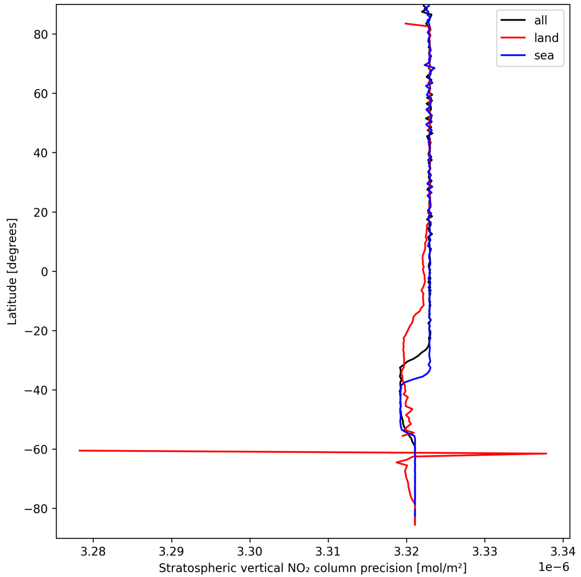
Figure 18: Zonal average of “Stratospheric vertical NO 2 column precision” for 2025-03-27 to 2025-03-28.
