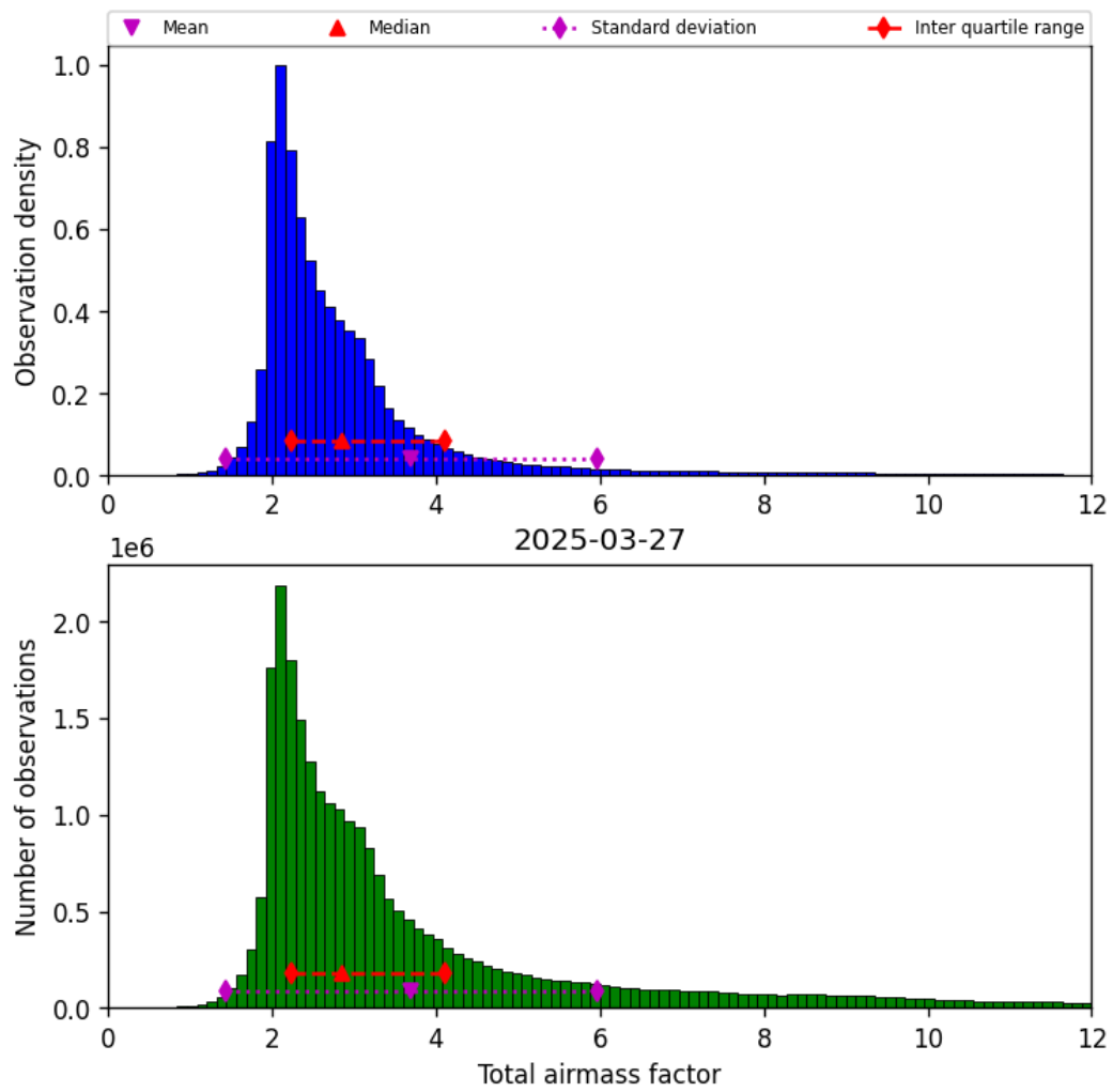
Figure 30: Histogram of “Total airmass factor” for 2025-03-27 to 2025-03-28
