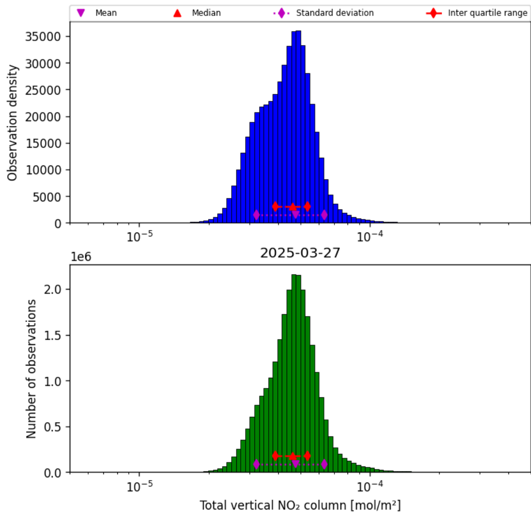
Figure 36: Histogram of “Total vertical NO 2 column” for 2025-03-27 to 2025-03-28
