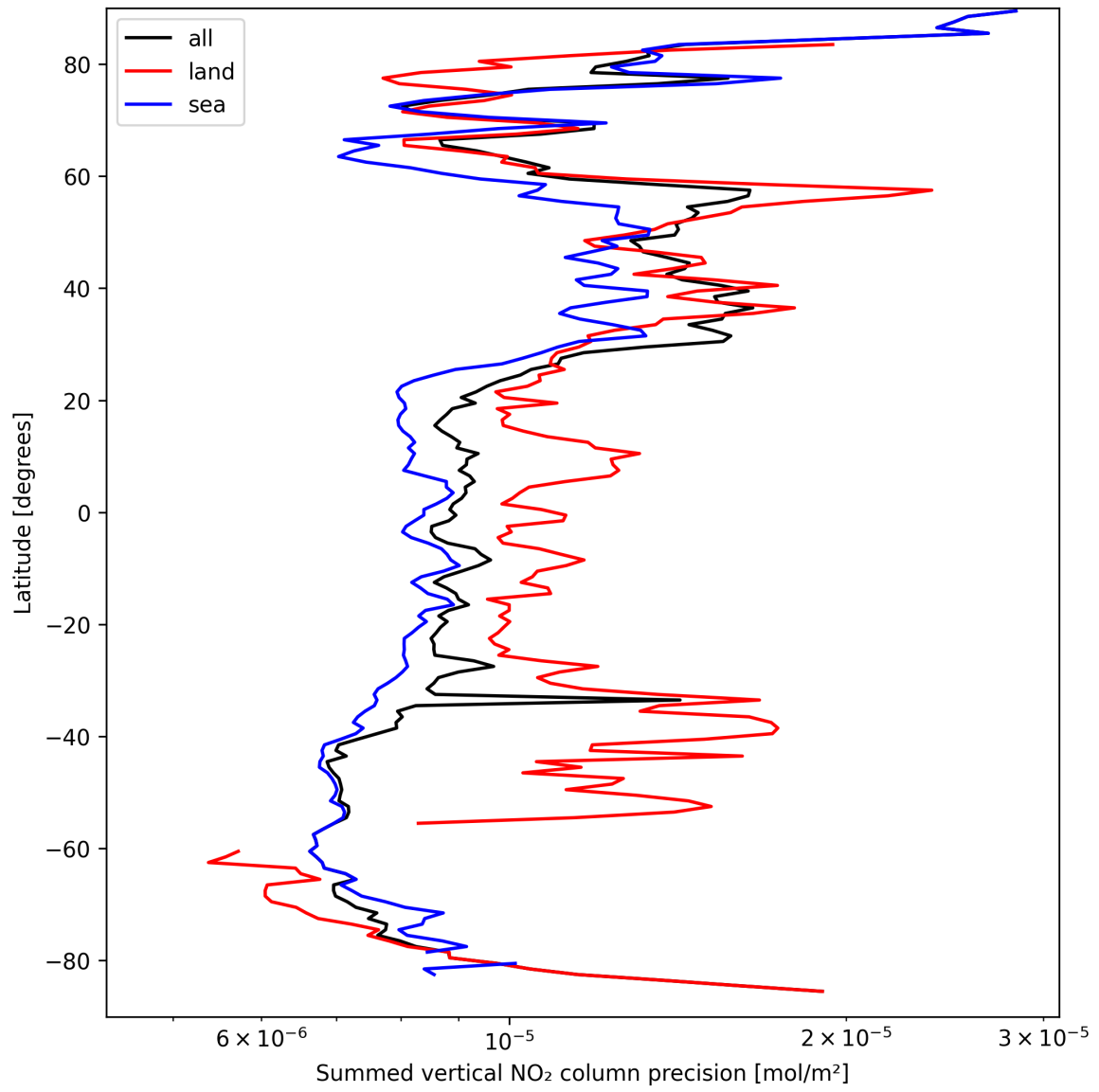
Figure 22: Zonal average of “Summed vertical NO 2 column precision” for 2025-03-27 to 2025-03-28.
