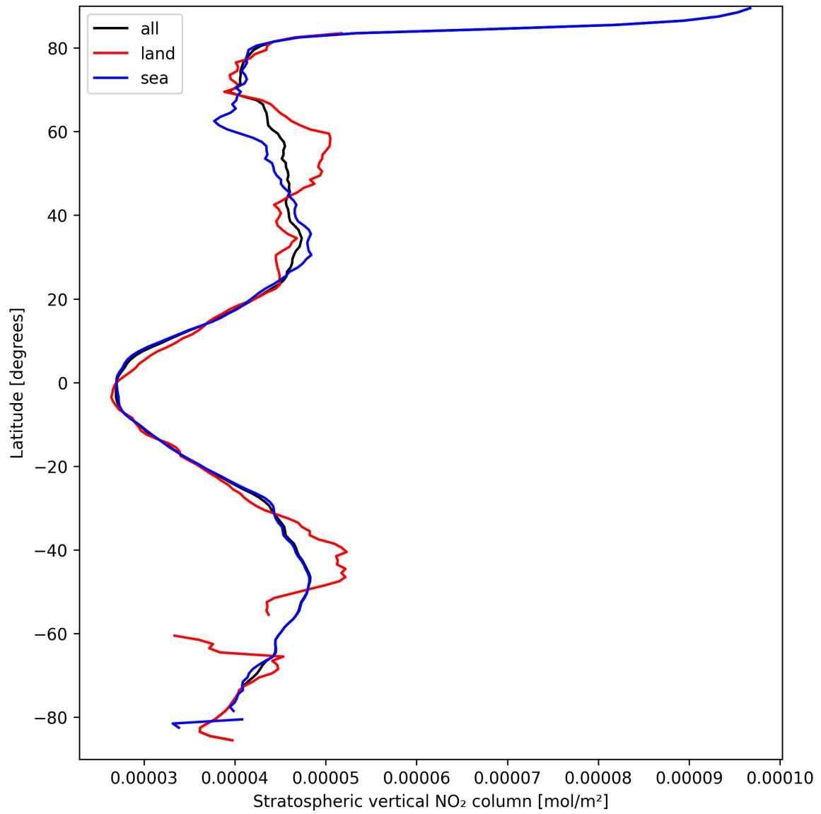
Figure 17: Zonal average of “Stratospheric vertical NO 2 column” for 2025-03-27 to 2025-03-28.
