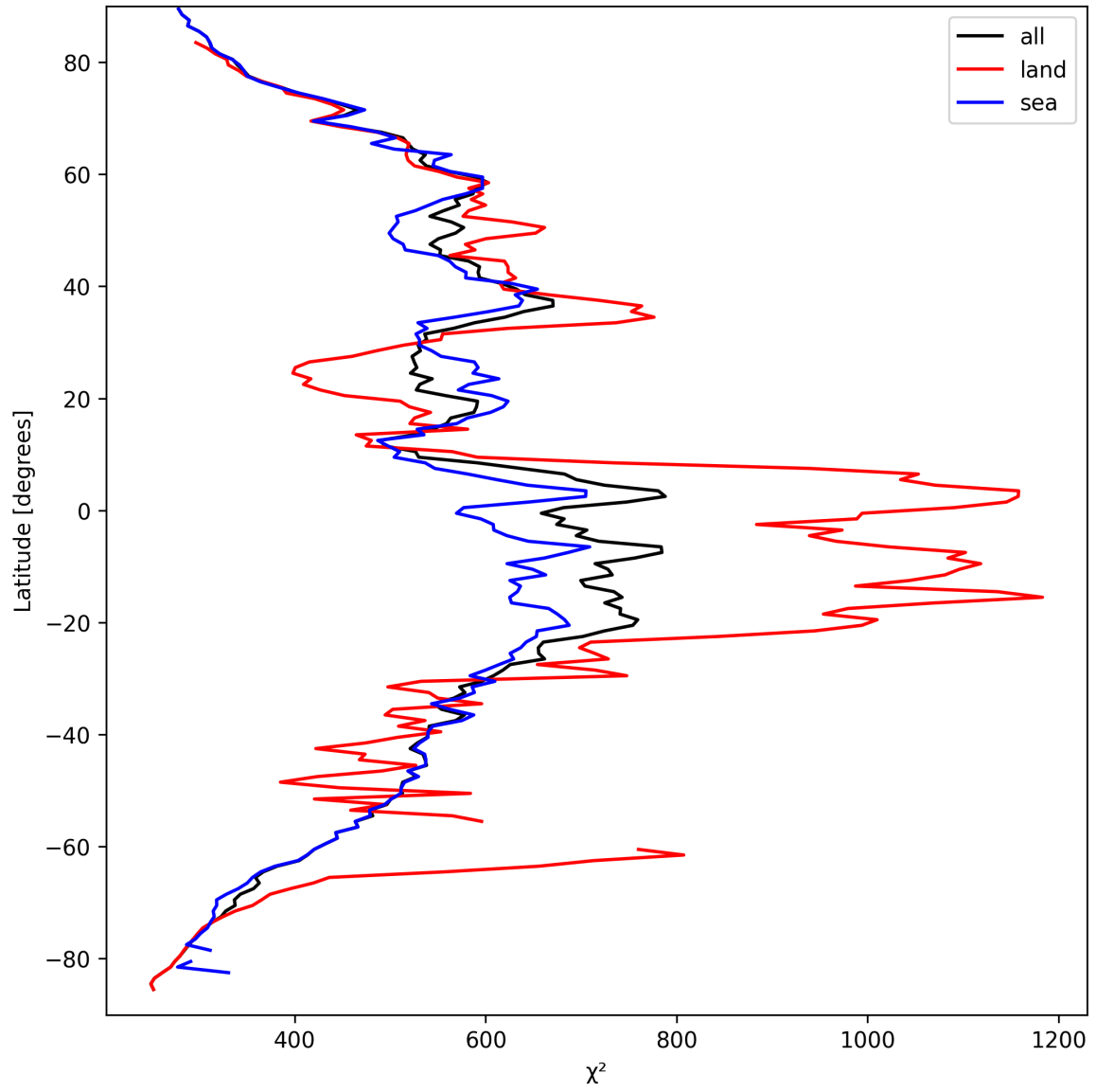
Figure 23: Zonal average of “ \chi^2 ” for 2025-03-27 to 2025-03-28.
