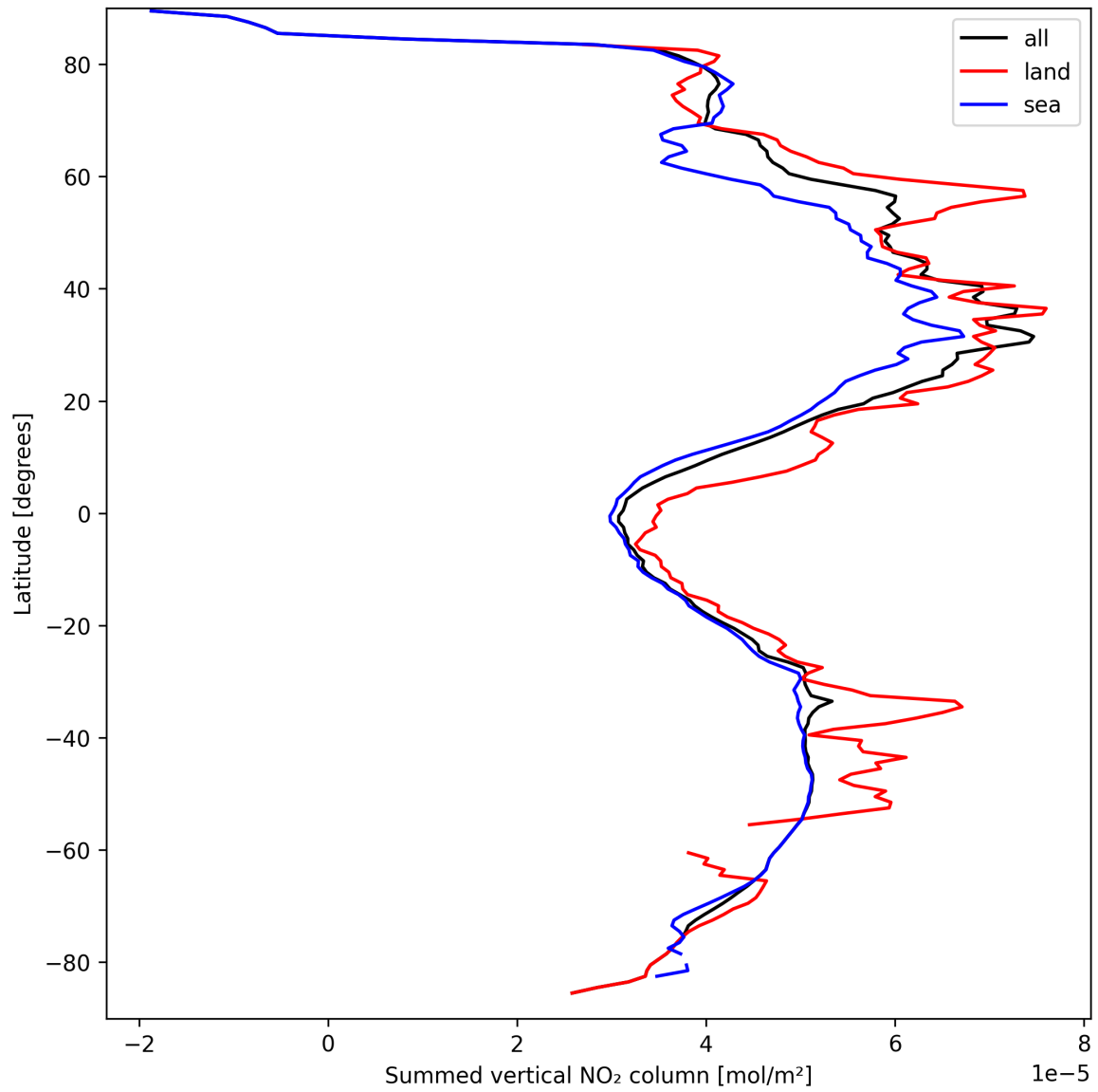
Figure 21: Zonal average of “Summed vertical NO 2 column” for 2025-03-27 to 2025-03-28.
