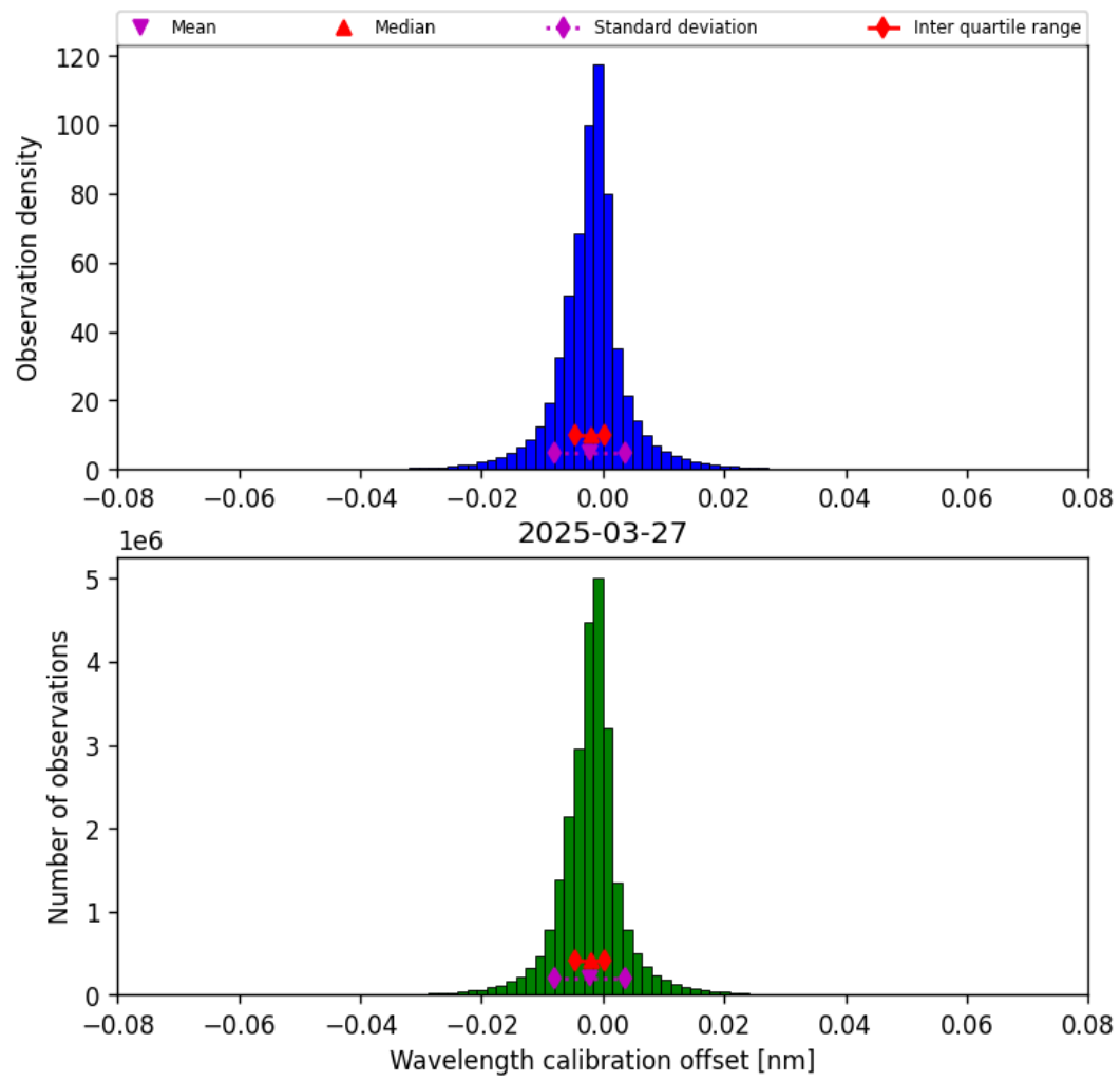
Figure 33: Histogram of “Wavelength calibration offset” for 2025-03-27 to 2025-03-28
