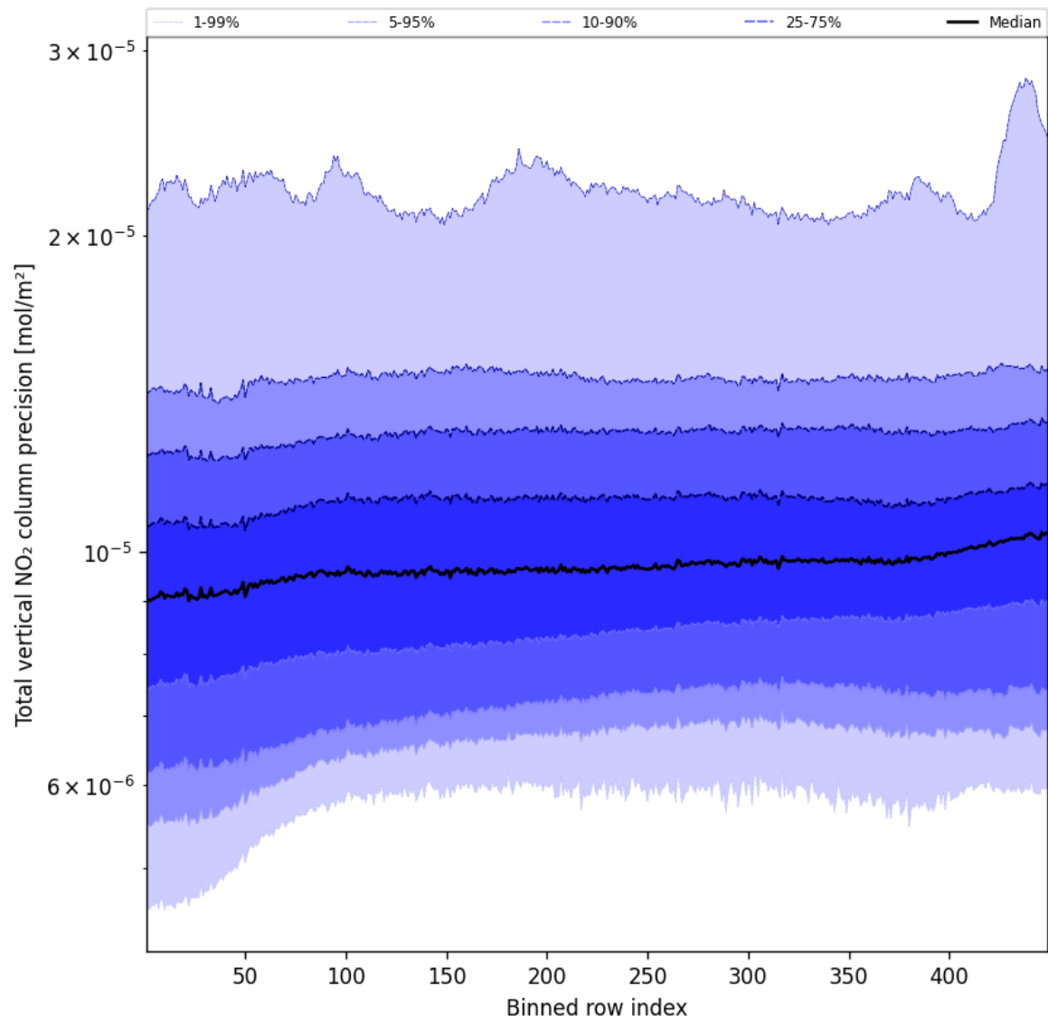
Figure 54: Along track statistics of “Total vertical NO 2 column precision” for 2025-03-27 to 2025-03-28
