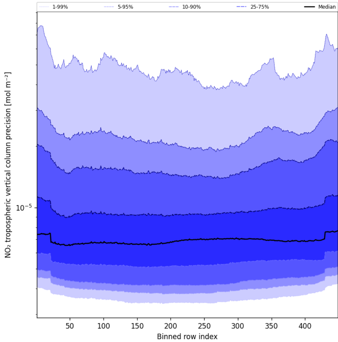
Figure 45: Along track statistics of “NO 2 tropospheric vertical column precision” for 2025-03-27 to 2025-03-28
