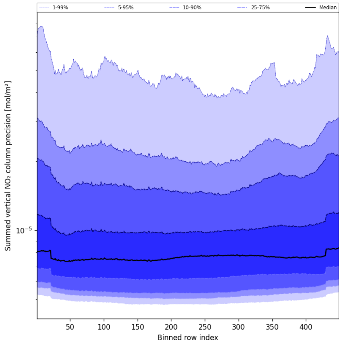
Figure 56: Along track statistics of “Summed vertical NO 2 column precision” for 2025-03-27 to 2025-03-28
