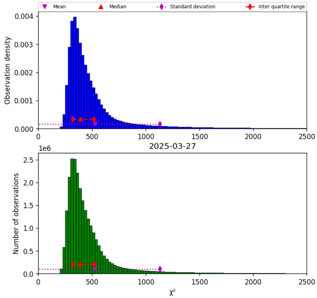
Figure 40: Histogram of “ \chi^2 ” for 2025-03-27 to 2025-03-28
