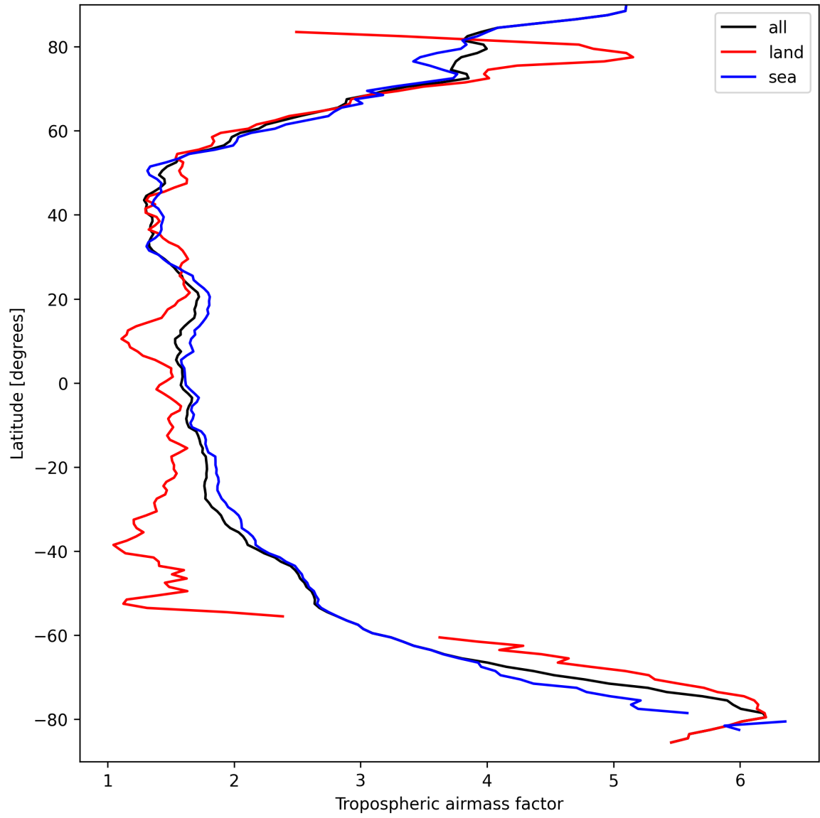
Figure 12: Zonal average of “Tropospheric airmass factor” for 2025-03-27 to 2025-03-28.
