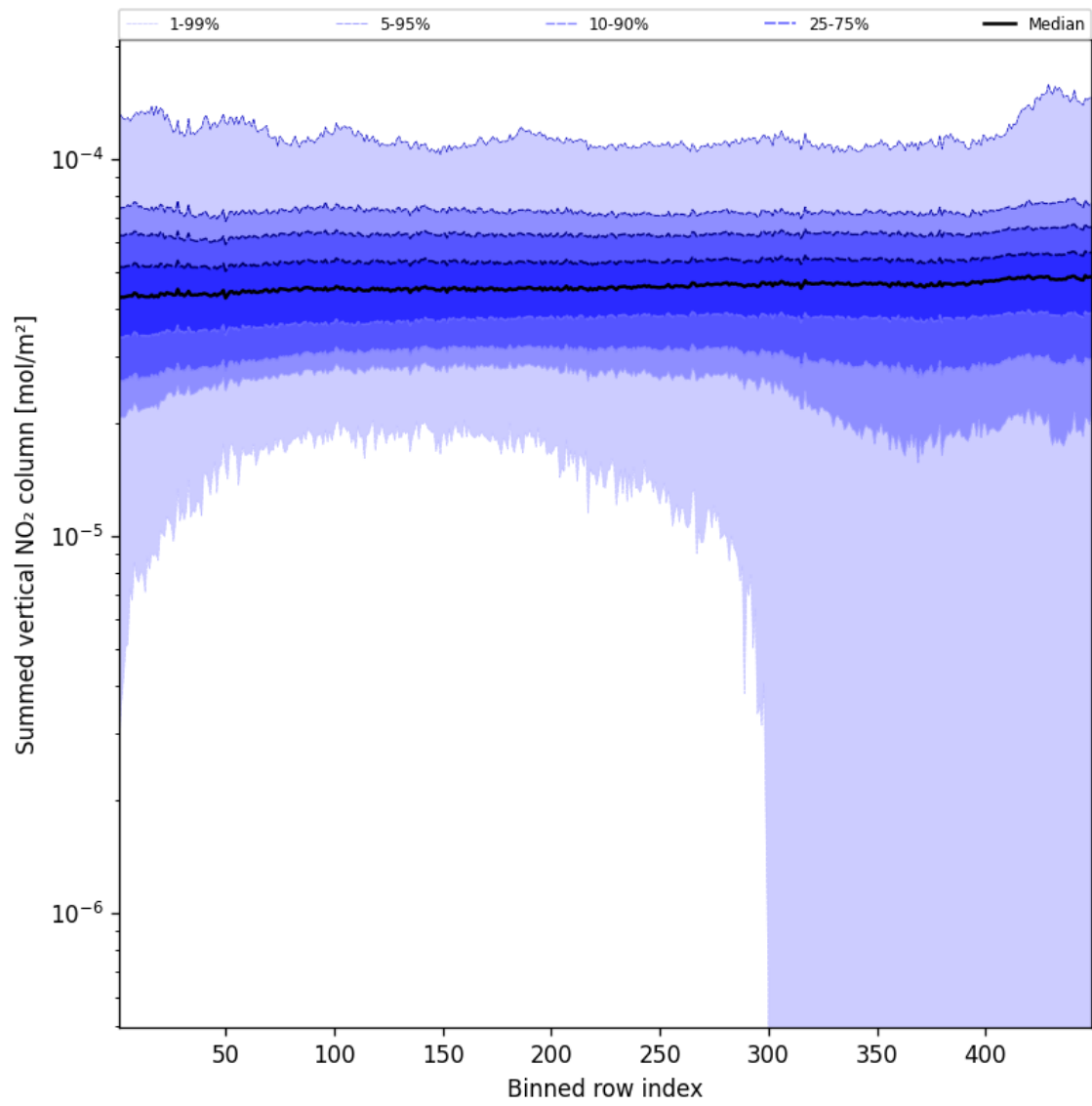
Figure 55: Along track statistics of “Summed vertical NO 2 column” for 2025-03-27 to 2025-03-28
