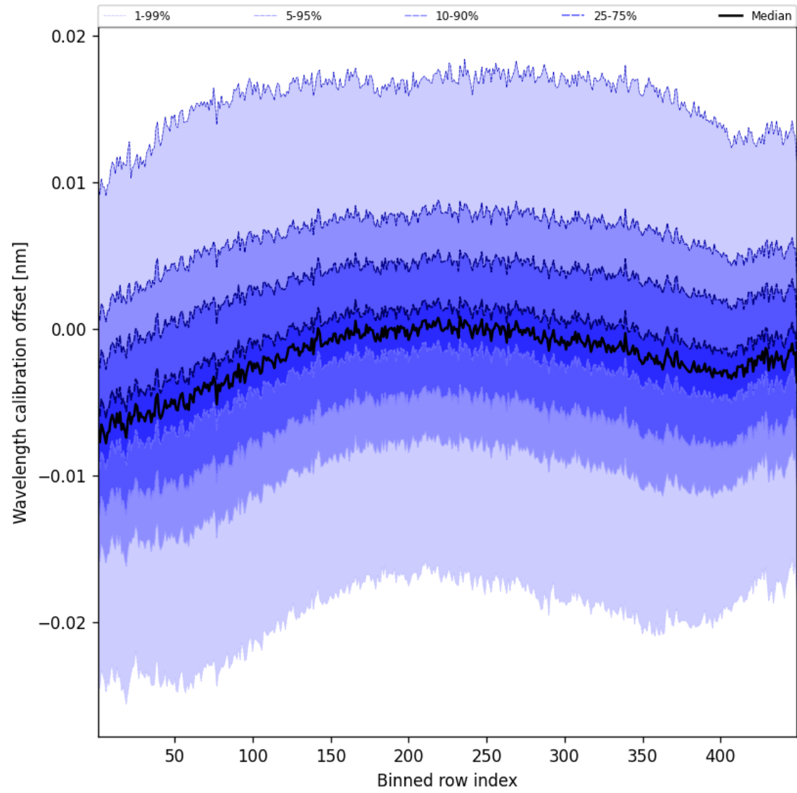
Figure 50: Along track statistics of “Wavelength calibration offset” for 2025-03-27 to 2025-03-28
