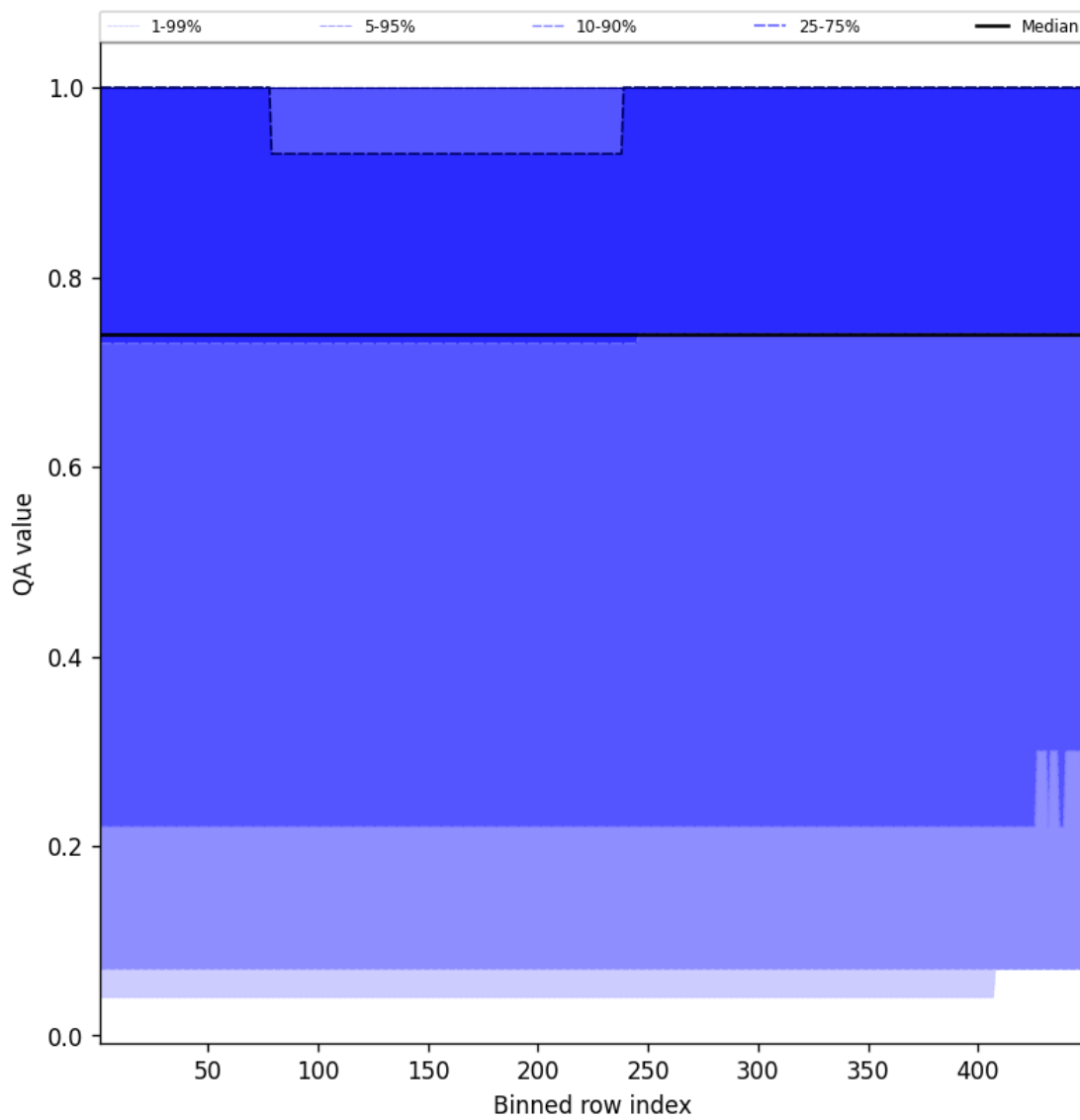
Figure 43: Along track statistics of “QA value” for 2025-03-27 to 2025-03-28
