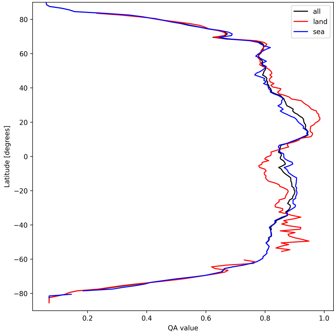
Figure 9: Zonal average of “QA value” for 2025-03-27 to 2025-03-28.
