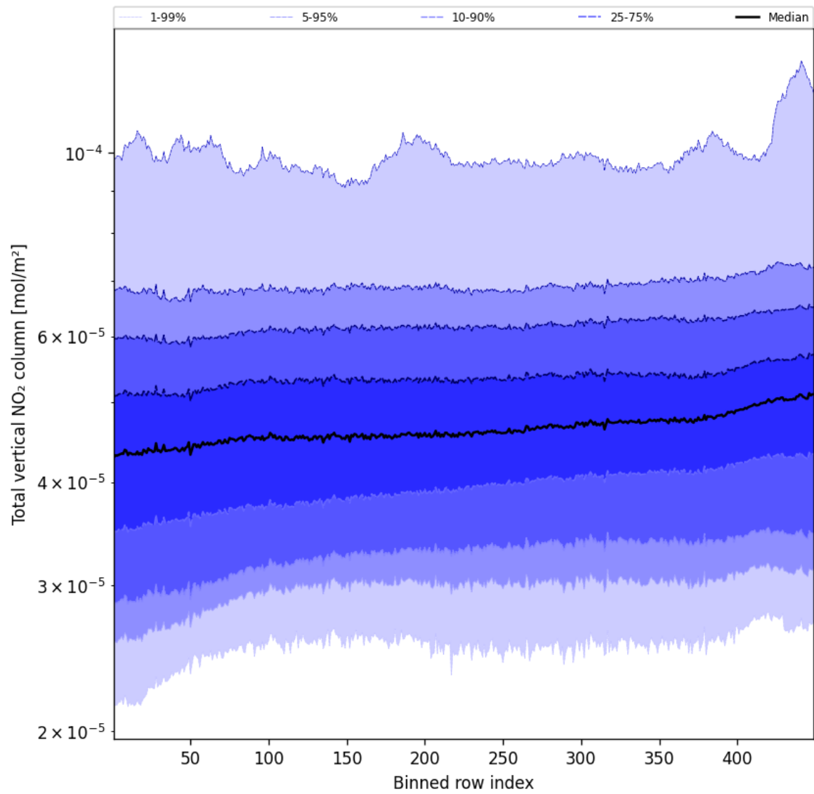
Figure 53: Along track statistics of “Total vertical NO 2 column” for 2025-03-27 to 2025-03-28
