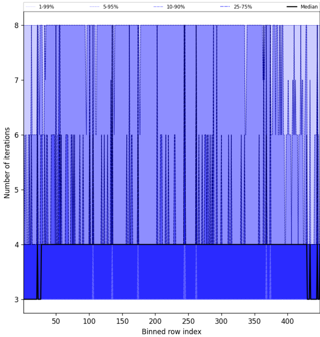
Figure 49: Along track statistics of “Number of iterations” for 2025-03-27 to 2025-03-28
