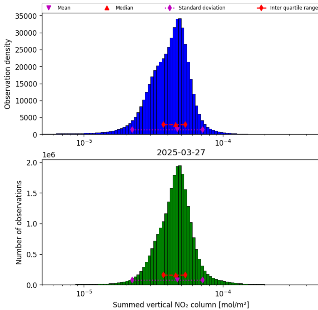
Figure 38: Histogram of “Summed vertical NO 2 column” for 2025-03-27 to 2025-03-28
