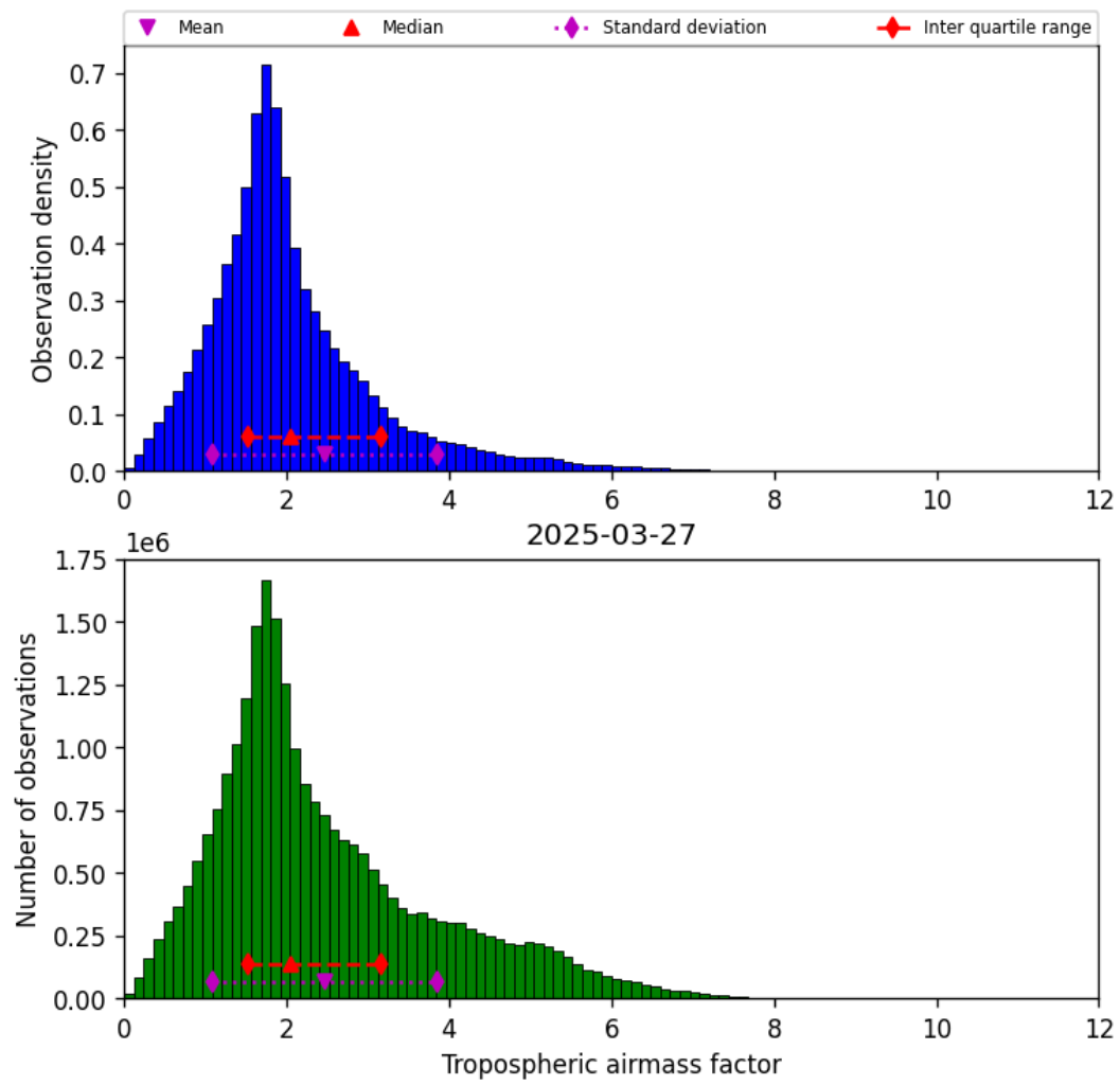
Figure 29: Histogram of “Tropospheric airmass factor” for 2025-03-27 to 2025-03-28
