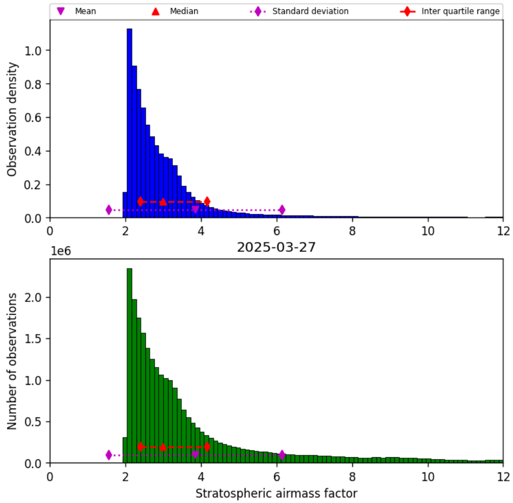
Figure 42: Histogram of “Stratospheric airmass factor” for 2025-03-27 to 2025-03-28
