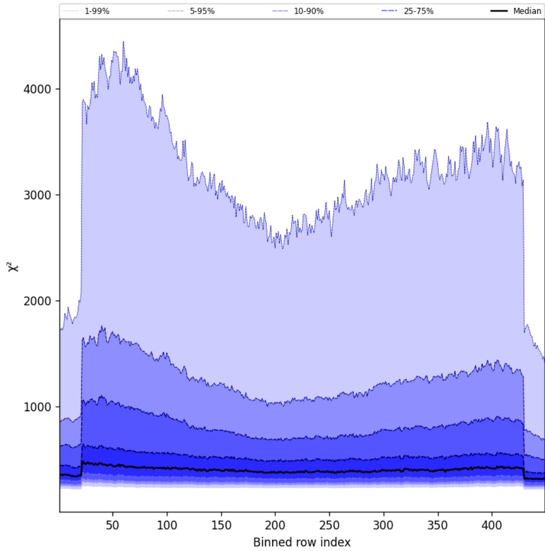
Figure 57: Along track statistics of “ \chi^2 ” for 2025-03-29 to 2025-03-30
