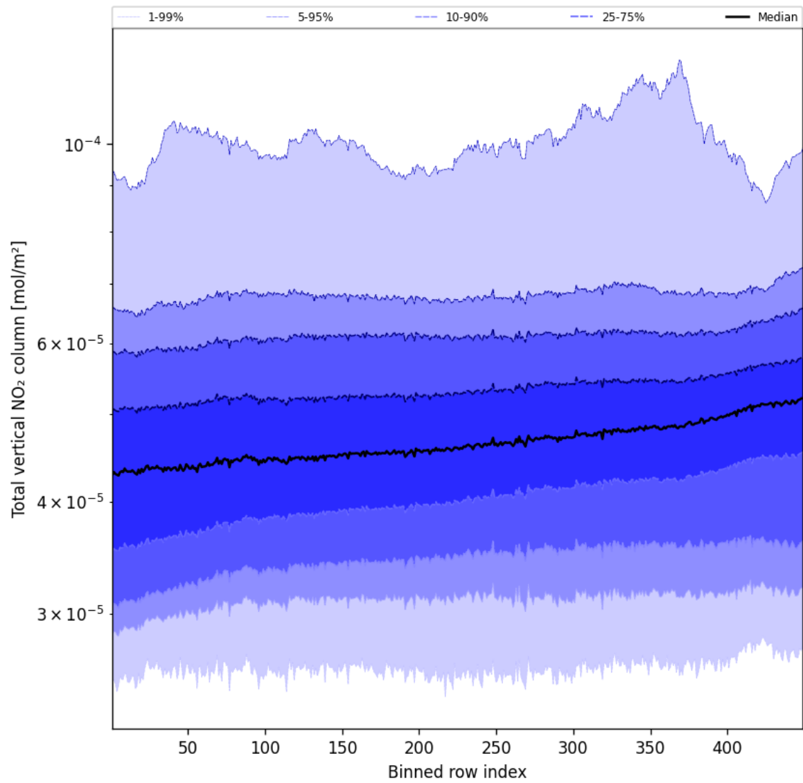
Figure 53: Along track statistics of “Total vertical NO 2 column” for 2025-03-29 to 2025-03-30
