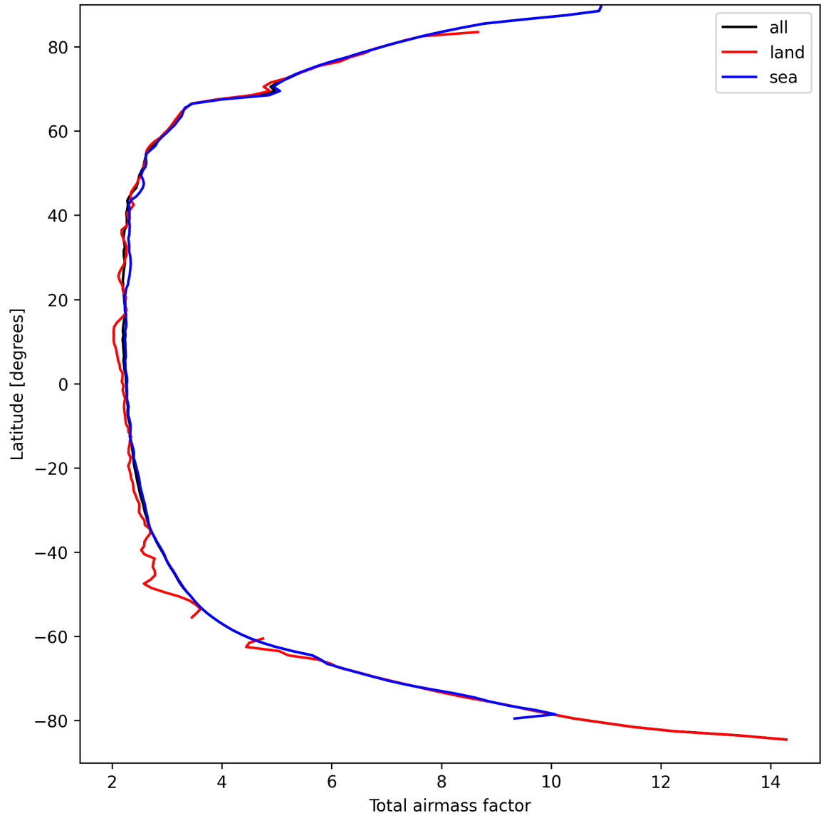
Figure 13: Zonal average of “Total airmass factor” for 2025-03-29 to 2025-03-30.
