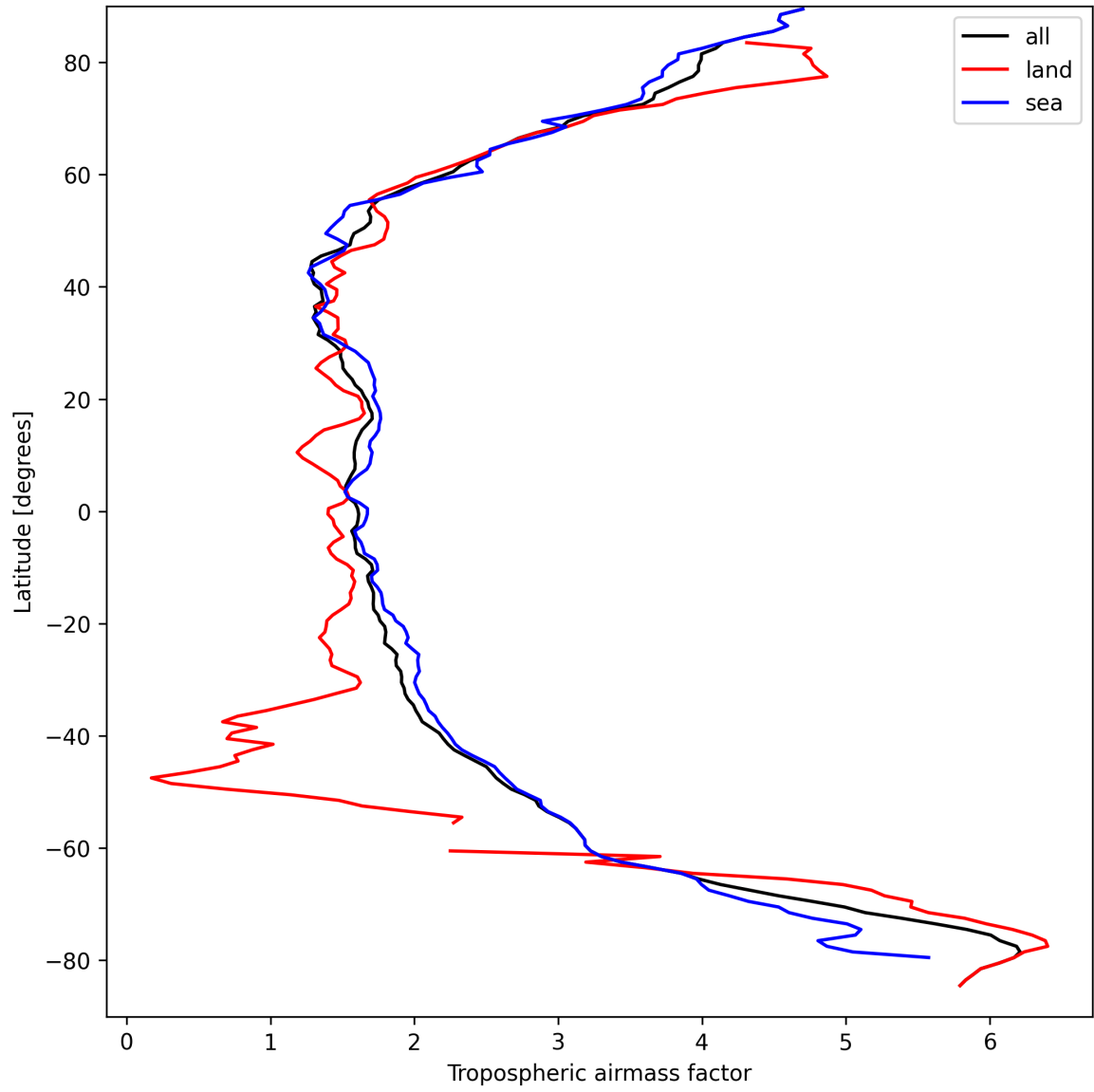
Figure 12: Zonal average of “Tropospheric air mass factor” for 2025-03-29 to 2025-03-30.
