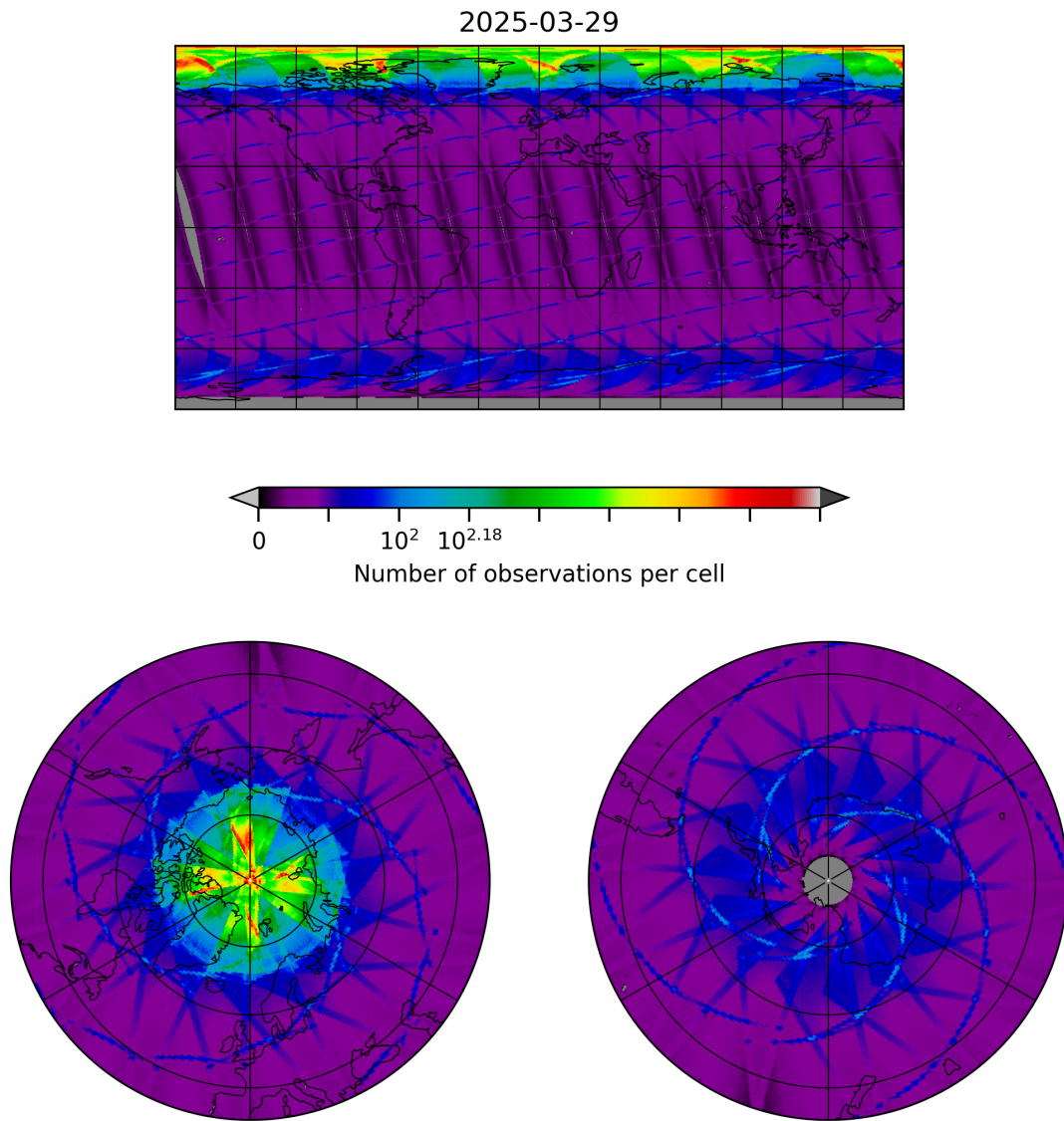
Figure 8: Map of the number of observations for 2025-03-29 to 2025-03-30
