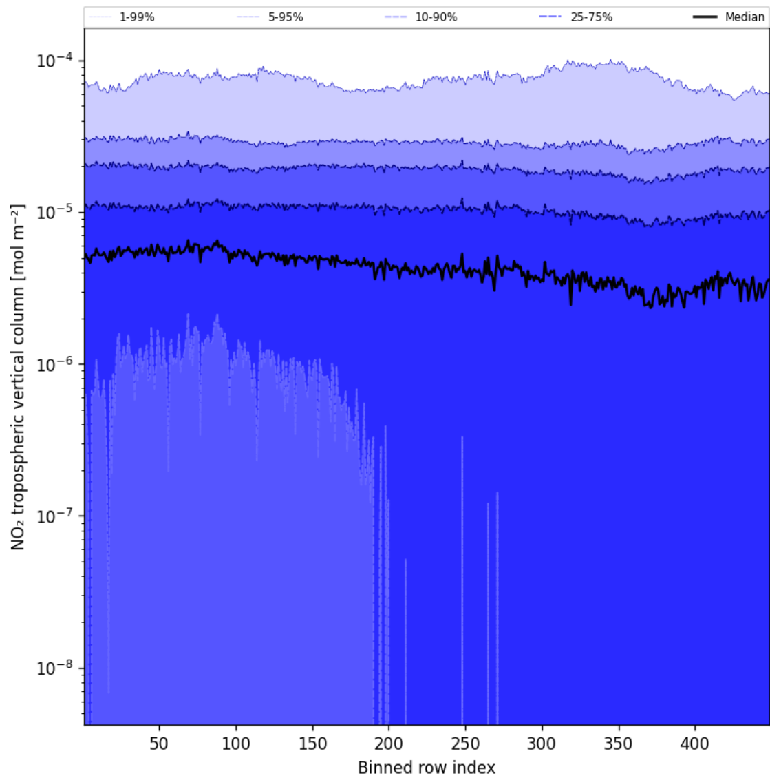
Figure 44: Along track statistics of “NO 2 tropospheric vertical column” for 2025-03-29 to 2025-03-30
