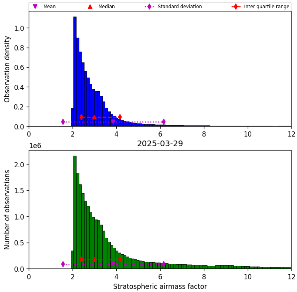
Figure 42: Histogram of “Stratospheric airmass factor” for 2025-03-29 to 2025-03-30
