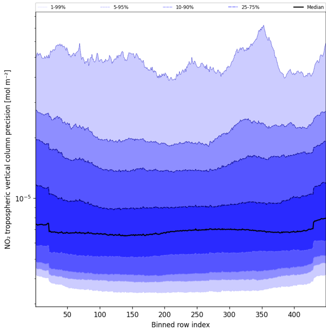
Figure 45: Along track statistics of “NO 2 tropospheric vertical column precision” for 2025-03-29 to 2025-03-30
