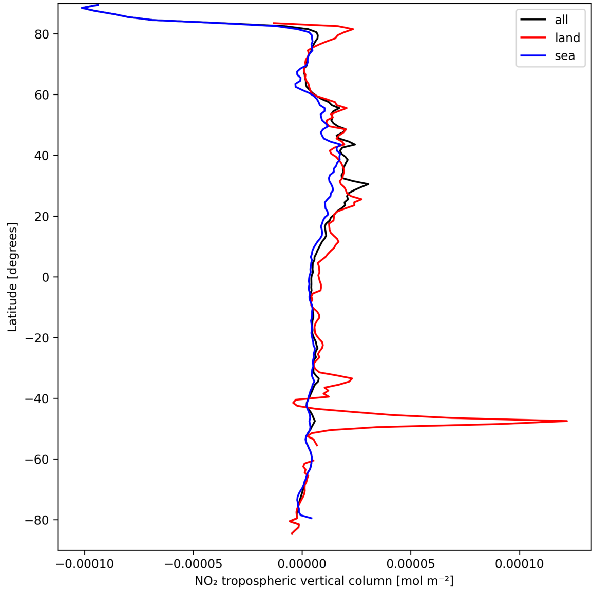
Figure 10: Zonal average of “NO 2 tropospheric vertical column” for 2025-03-29 to 2025-03-30.
