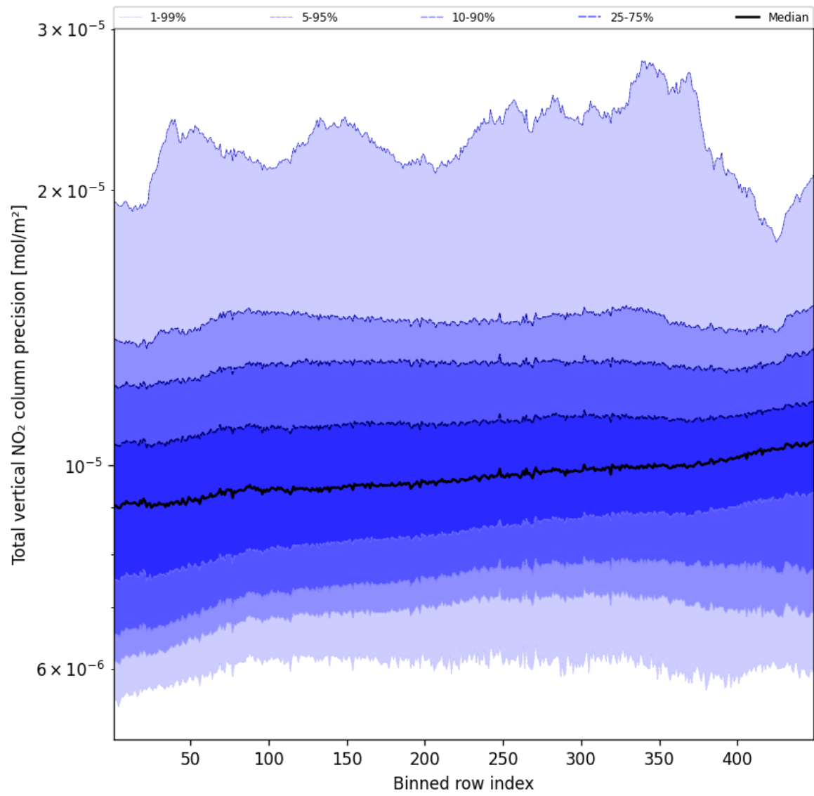
Figure 54: Along track statistics of “Total vertical NO 2 column precision” for 2025-03-29 to 2025-03-30
