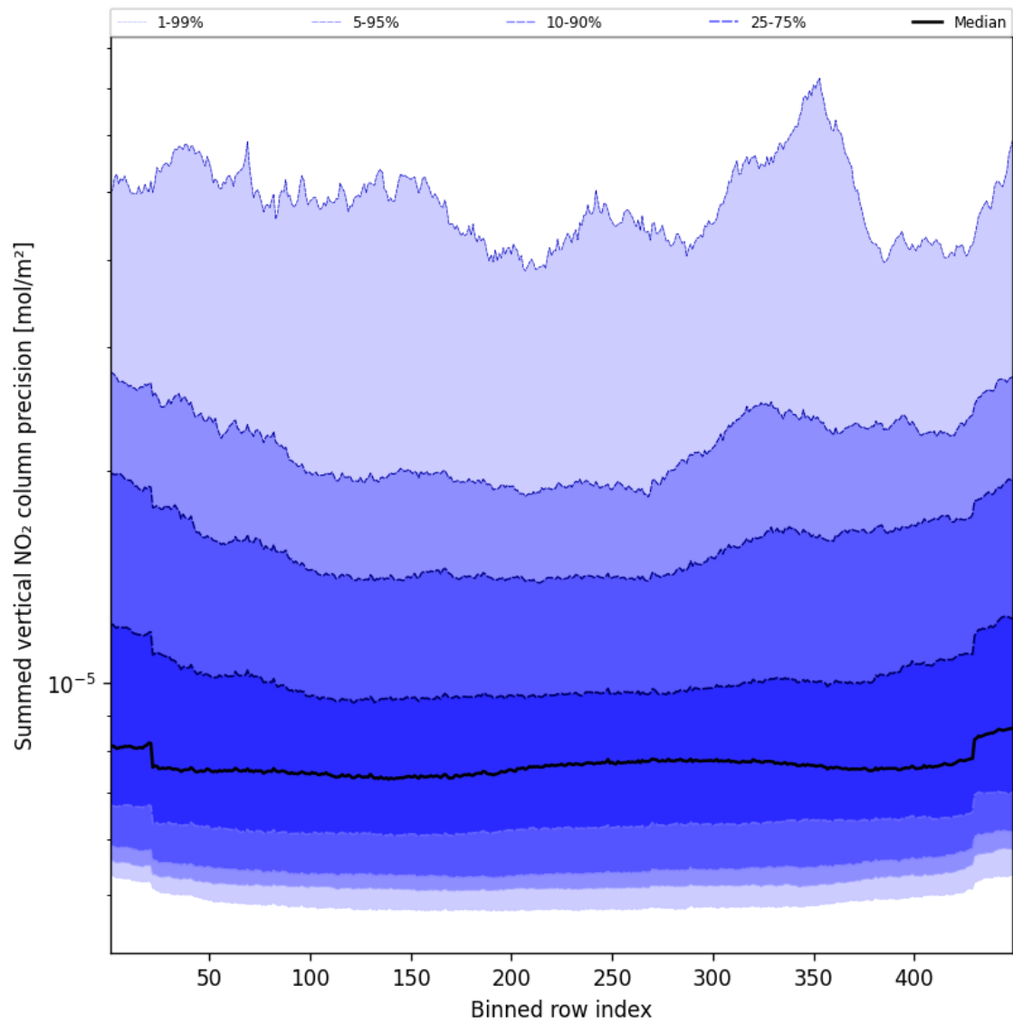
Figure 56: Along track statistics of “Summed vertical NO 2 column precision” for 2025-03-29 to 2025-03-30
