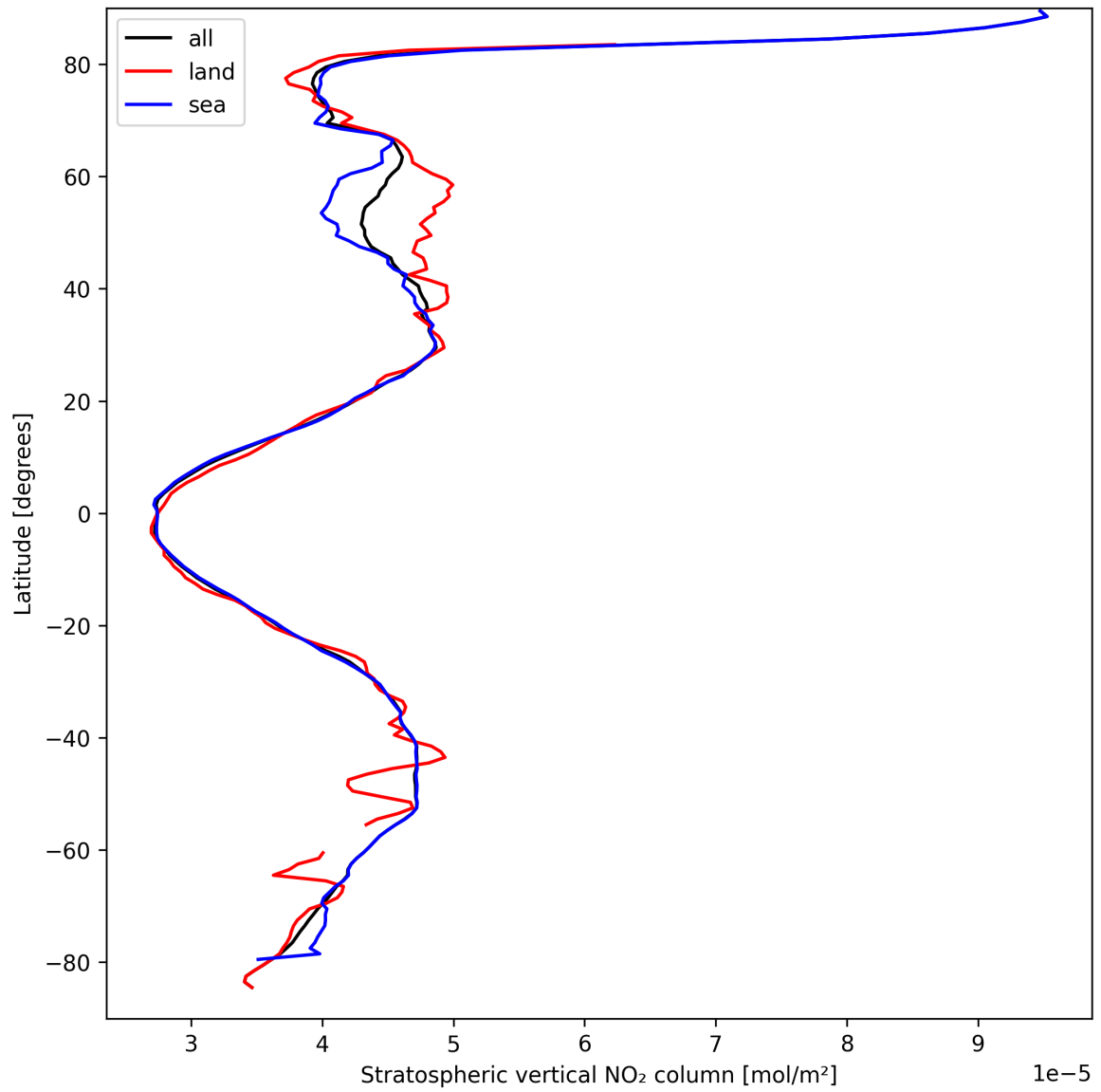
Figure 17: Zonal average of “Stratospheric vertical NO 2 column” for 2025-03-29 to 2025-03-30.
