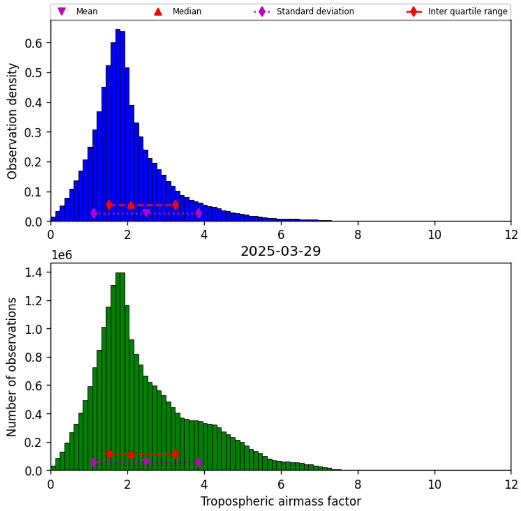
Figure 29: Histogram of “Tropospheric airmass factor” for 2025-03-29 to 2025-03-30
