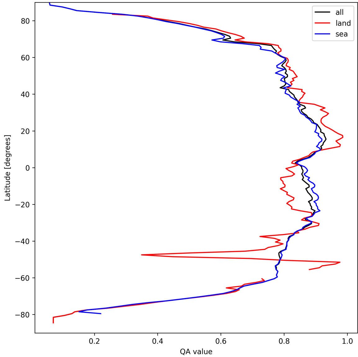
Figure 9: Zonal average of “QA value” for 2025-03-29 to 2025-03-30.
