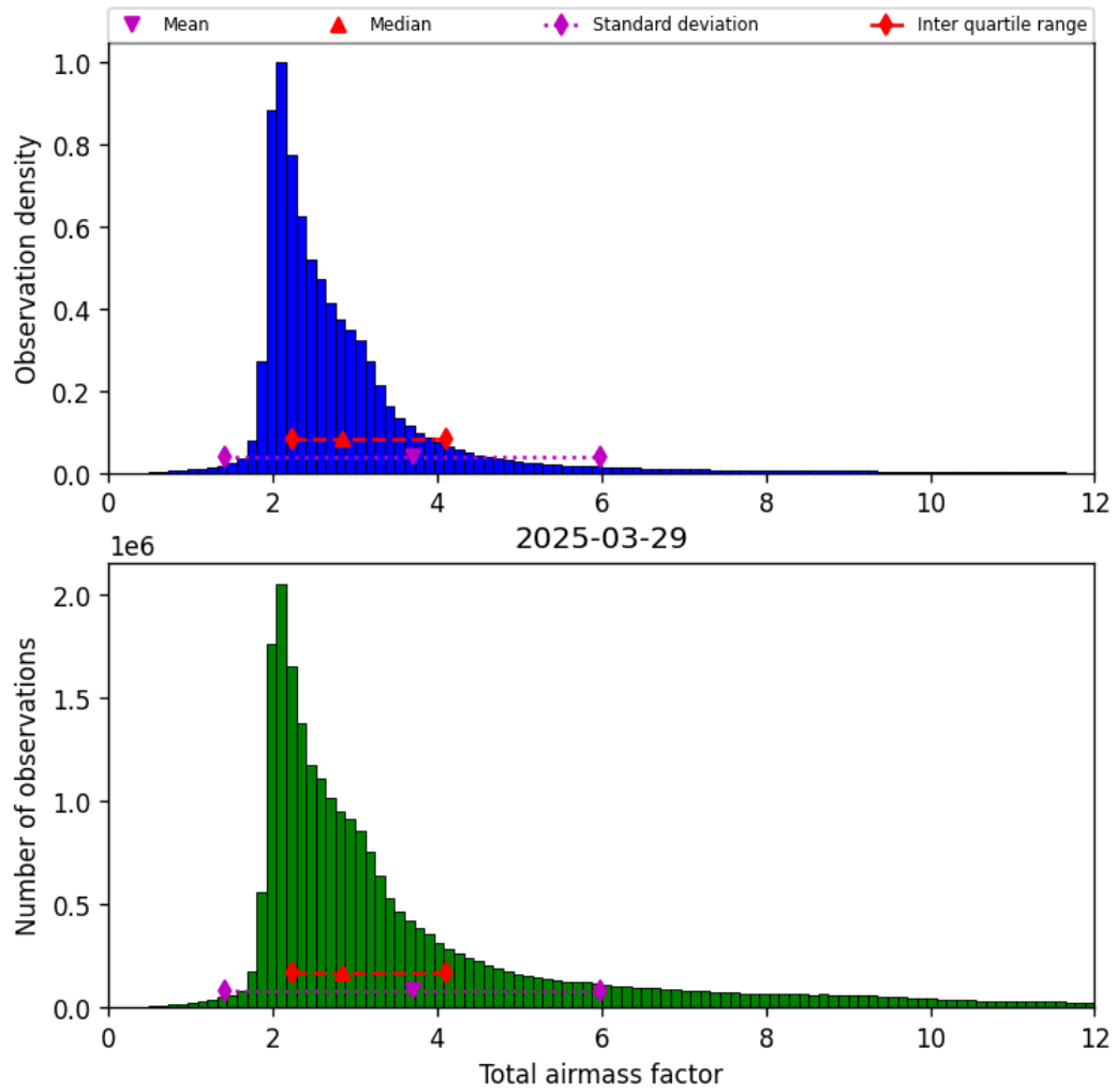
Figure 30: Histogram of “Total airmass factor” for 2025-03-29 to 2025-03-30
