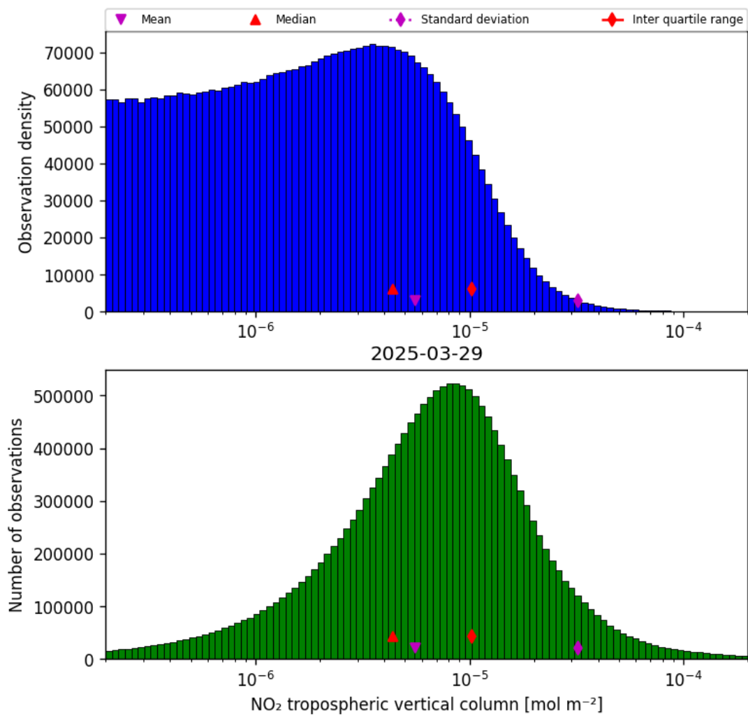
Figure 27: Histogram of “NO 2 tropospheric vertical column” for 2025-03-29 to 2025-03-30
