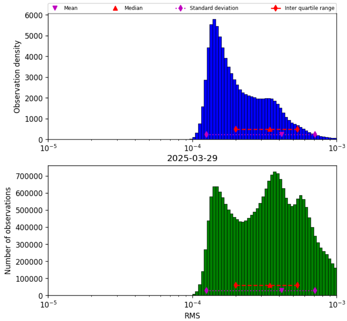
Figure 41: Histogram of “RMS” for 2025-03-29 to 2025-03-30
