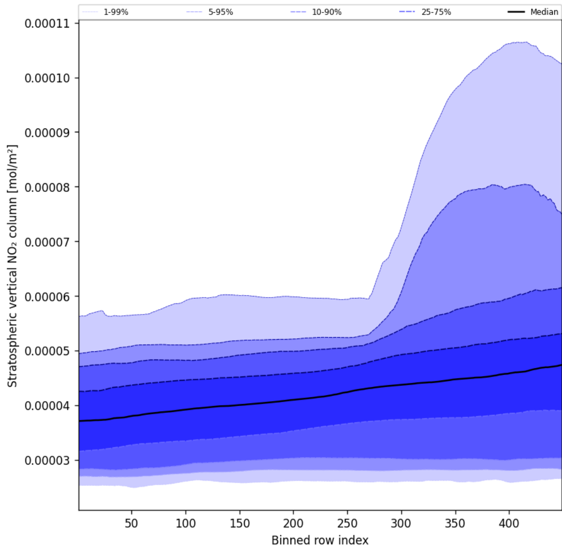
Figure 51: Along track statistics of “Stratospheric vertical NO 2 column” for 2025-03-29 to 2025-03-30
