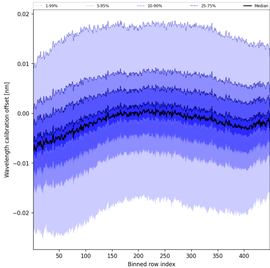
Figure 50: Along track statistics of “Wavelength calibration offset” for 2025-03-29 to 2025-03-30
