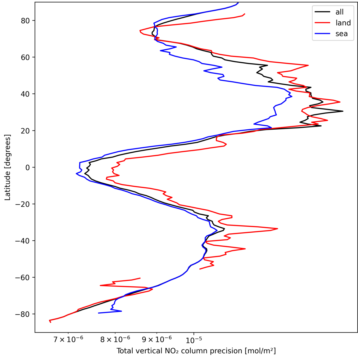
Figure 20: Zonal average of “Total vertical NO 2 column precision” for 2025-03-29 to 2025-03-30.
