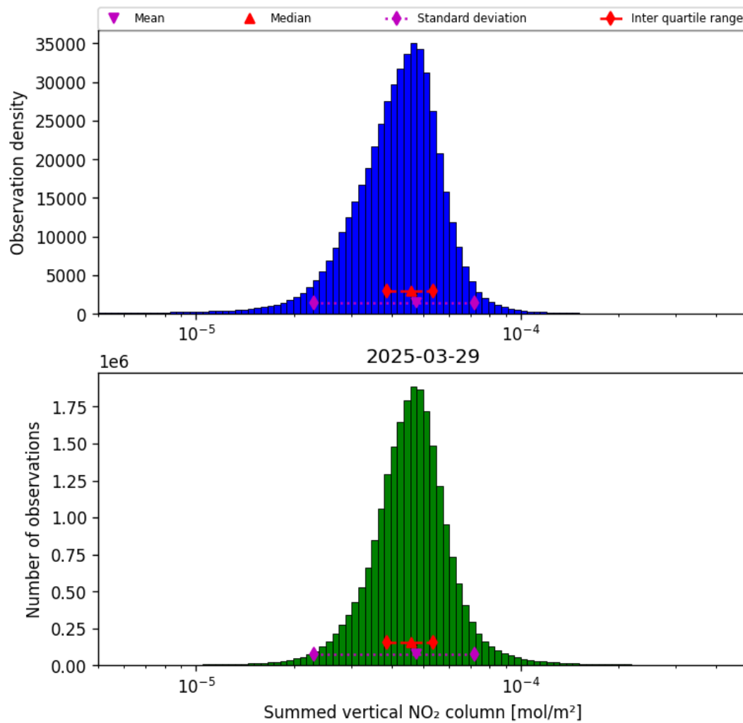
Figure 38: Histogram of “Summed vertical NO 2 column” for 2025-03-29 to 2025-03-30
