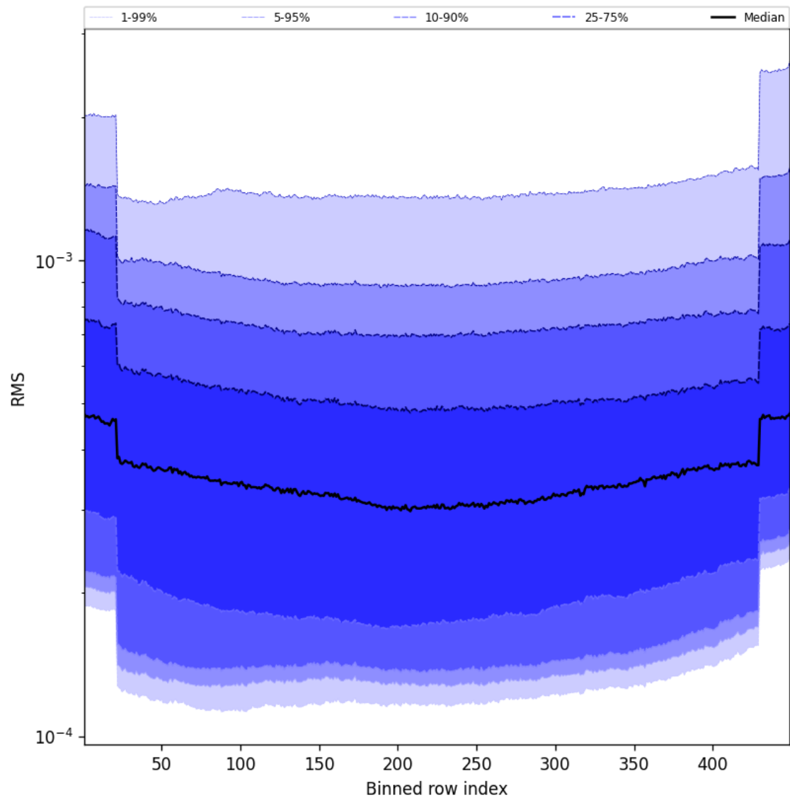
Figure 58: Along track statistics of “RMS” for 2025-03-29 to 2025-03-30
