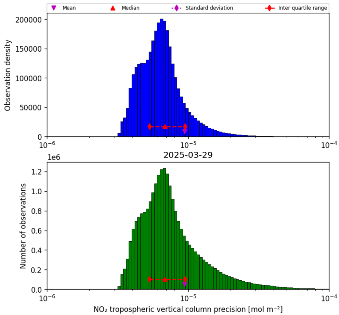
Figure 28: Histogram of “NO 2 tropospheric vertical column precision” for 2025-03-29 to 2025-03-30
