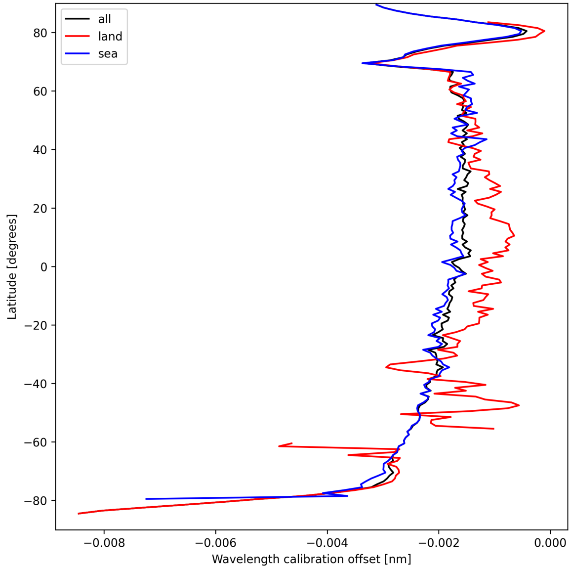
Figure 16: Zonal average of “Wavelength calibration offset” for 2025-03-29 to 2025-03-30.
