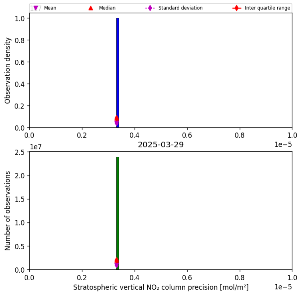
Figure 35: Histogram of “Stratospheric vertical NO 2 column precision” for 2025-03-29 to 2025-03-30
