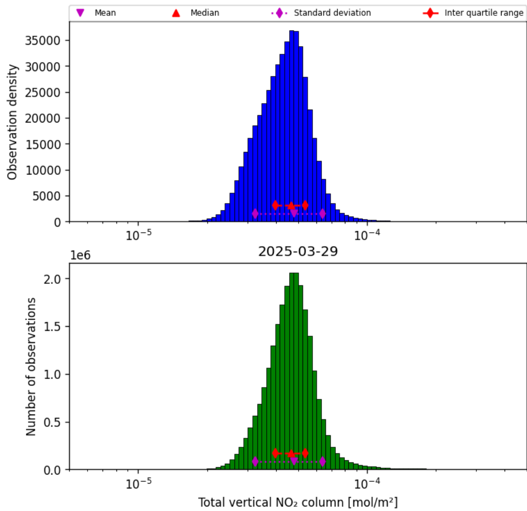
Figure 36: Histogram of “Total vertical NO 2 column” for 2025-03-29 to 2025-03-30
