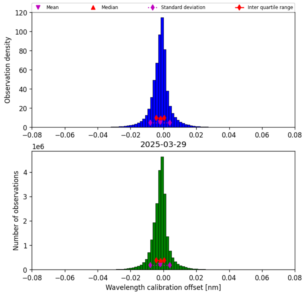
Figure 33: Histogram of “Wavelength calibration offset” for 2025-03-29 to 2025-03-30
