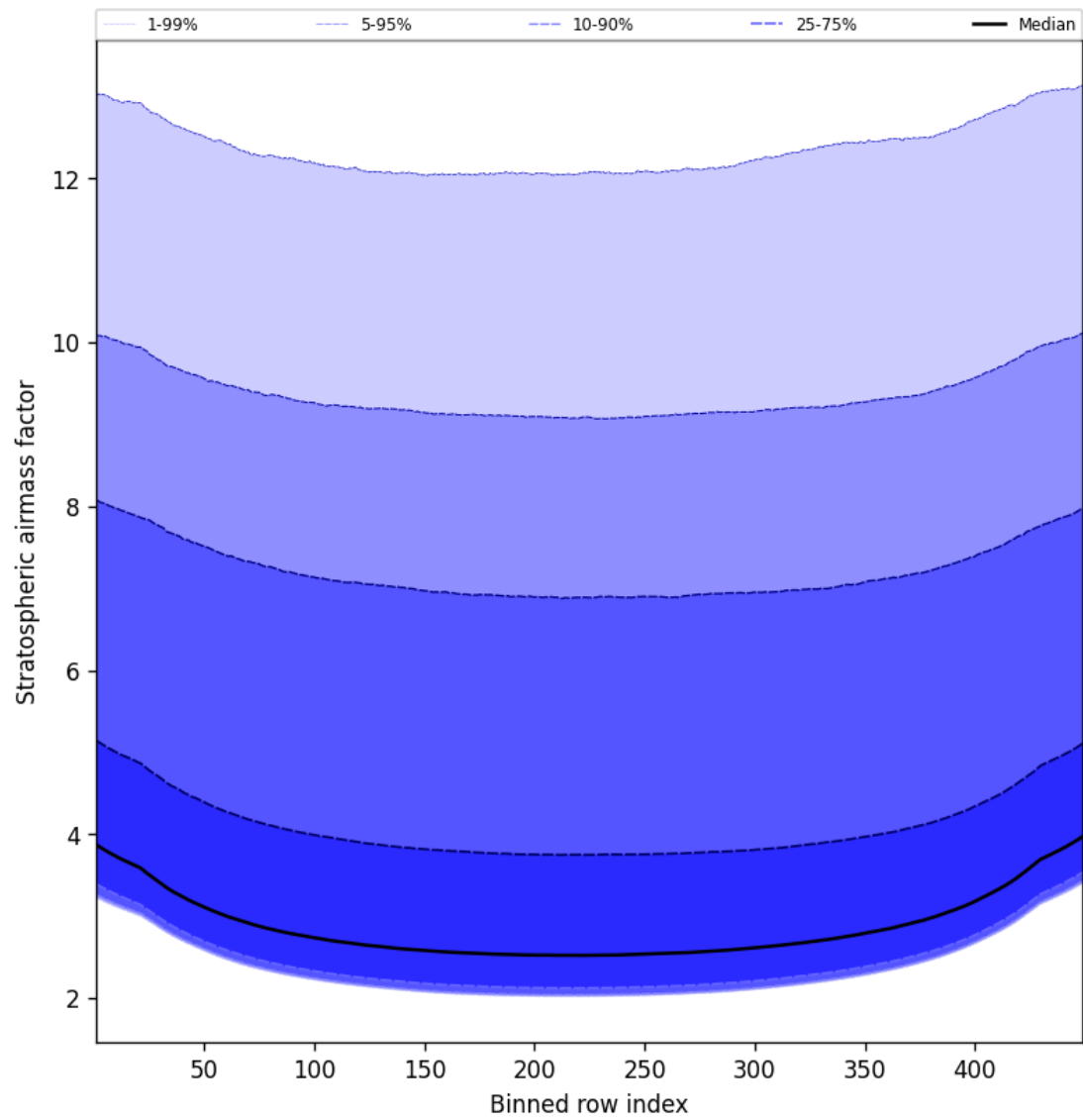
Figure 59: Along track statistics of “Stratospheric airmass factor” for 2025-03-29 to 2025-03-30
