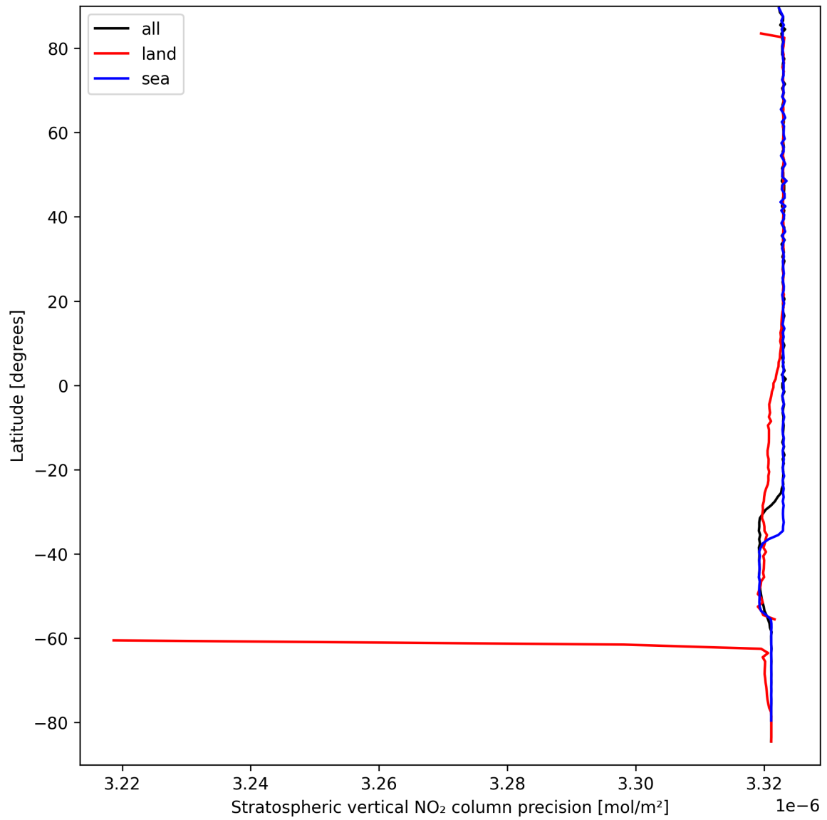
Figure 18: Zonal average of “Stratospheric vertical NO 2 column precision” for 2025-03-29 to 2025-03-30.
