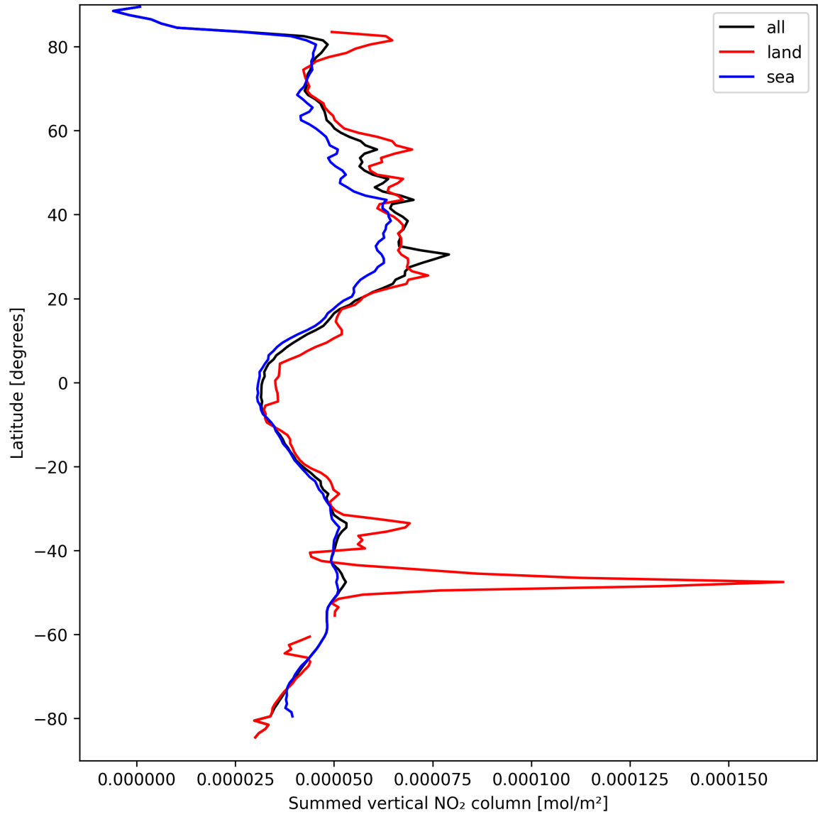
Figure 21: Zonal average of “Summed vertical NO 2 column” for 2025-03-29 to 2025-03-30.
