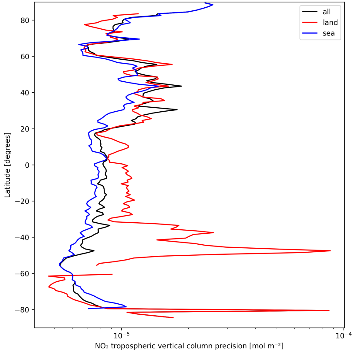
Figure 11: Zonal average of “NO 2 tropospheric vertical column precision” for 2025-03-29 to 2025-03-30.
