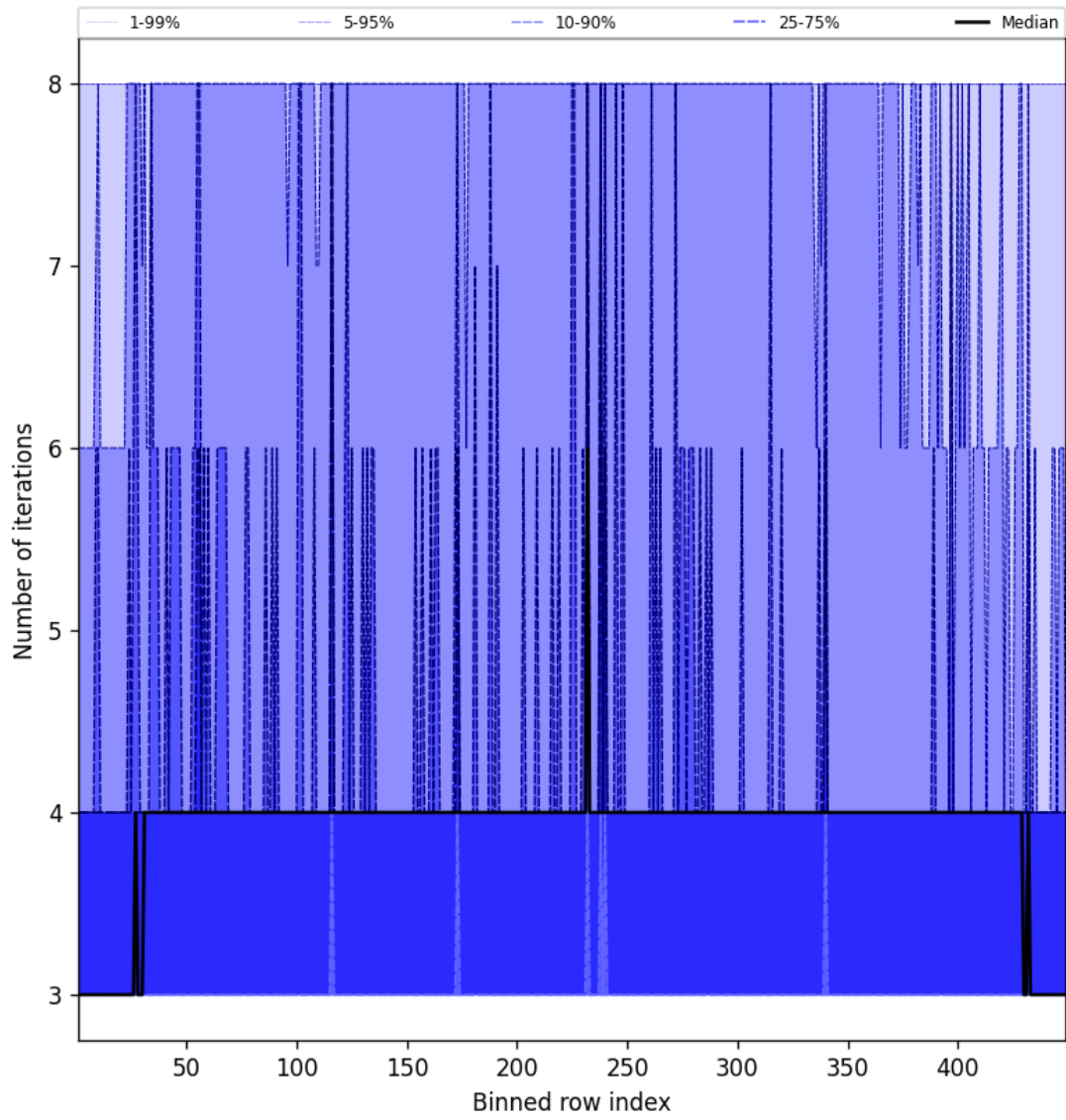
Figure 49: Along track statistics of “Number of iterations” for 2025-03-29 to 2025-03-30
