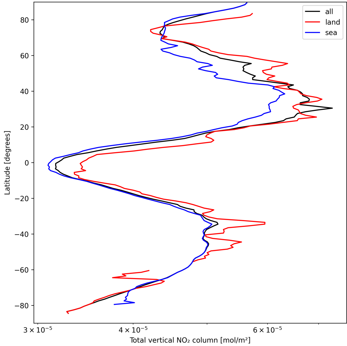
Figure 19: Zonal average of “Total vertical NO 2 column” for 2025-03-29 to 2025-03-30.
