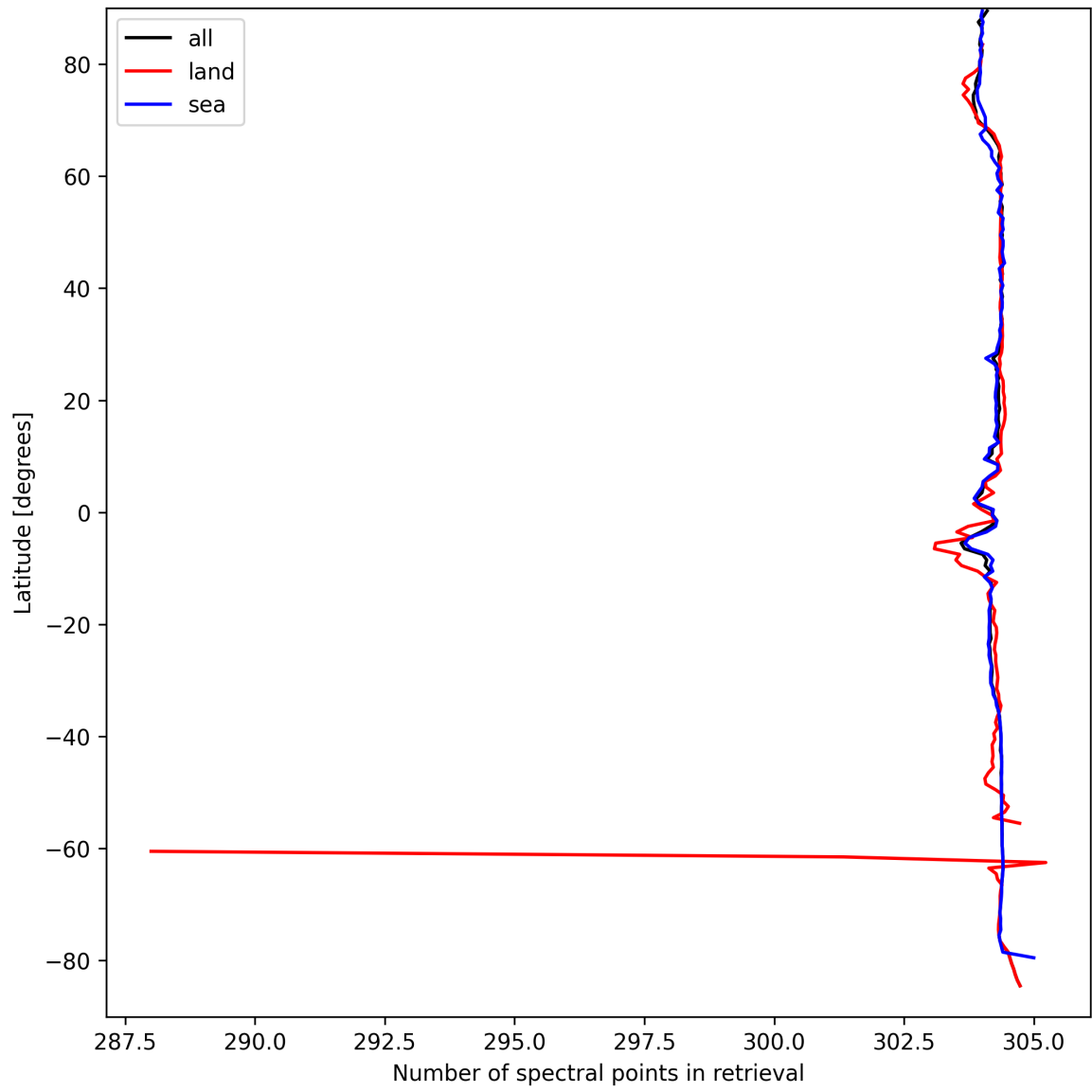
Figure 14: Zonal average of “Number of spectral points in retrieval” for 2025-03-29 to 2025-03-30.
