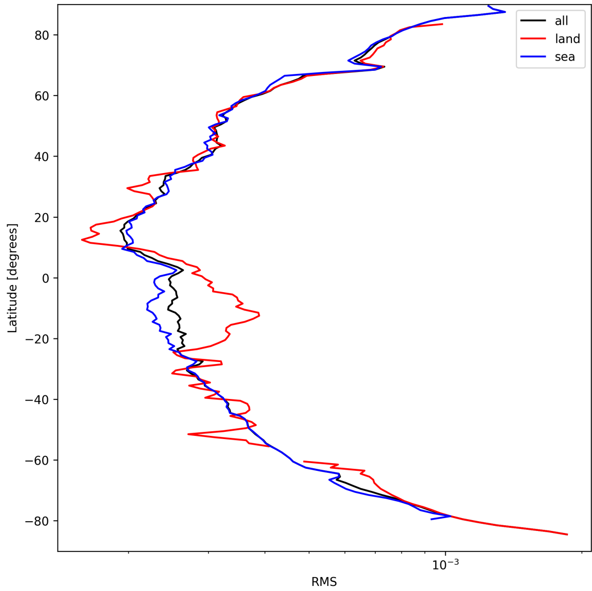
Figure 24: Zonal average of “RMS” for 2025-03-29 to 2025-03-30.
