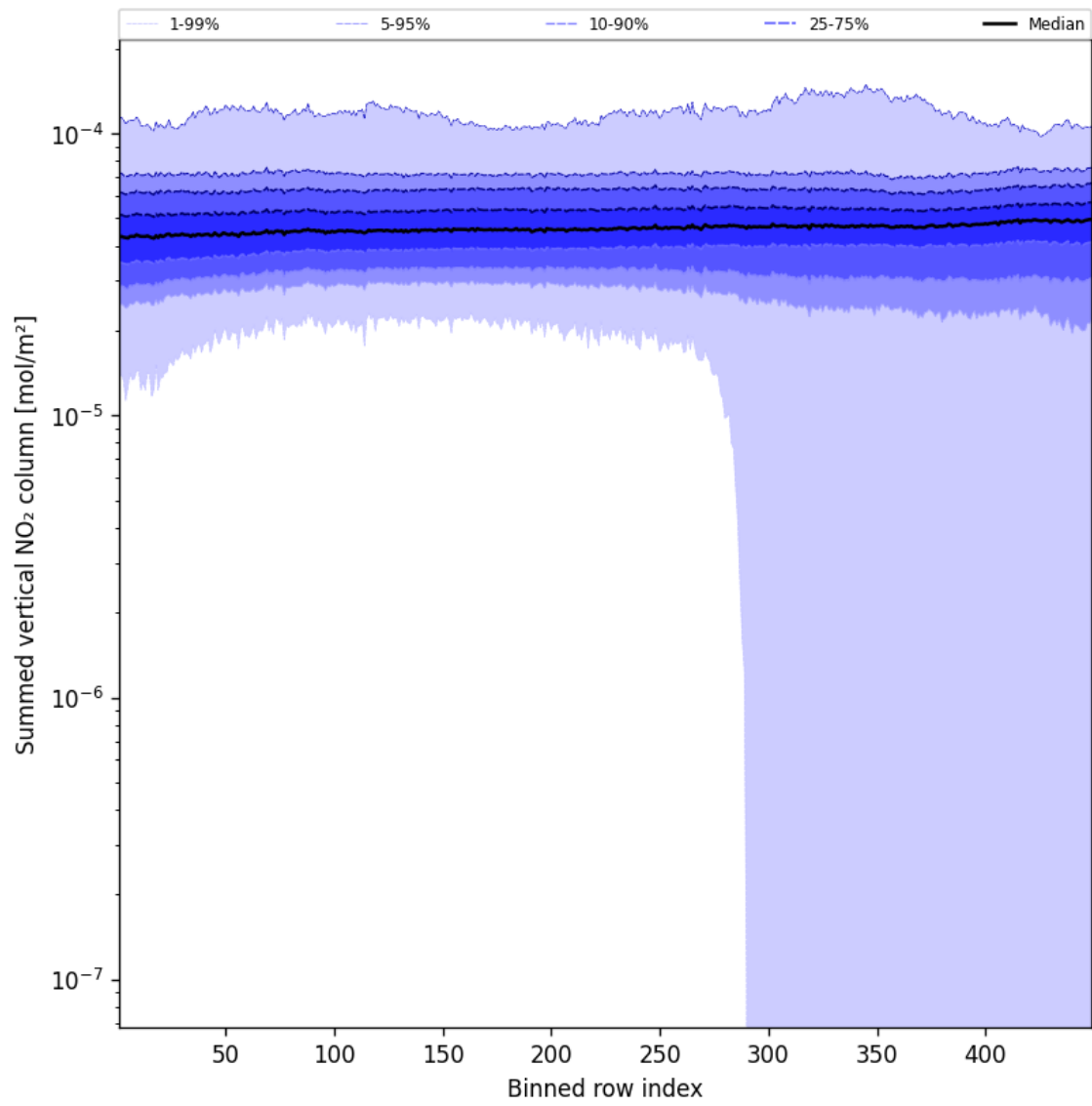
Figure 55: Along track statistics of “Summed vertical NO 2 column” for 2025-03-29 to 2025-03-30
