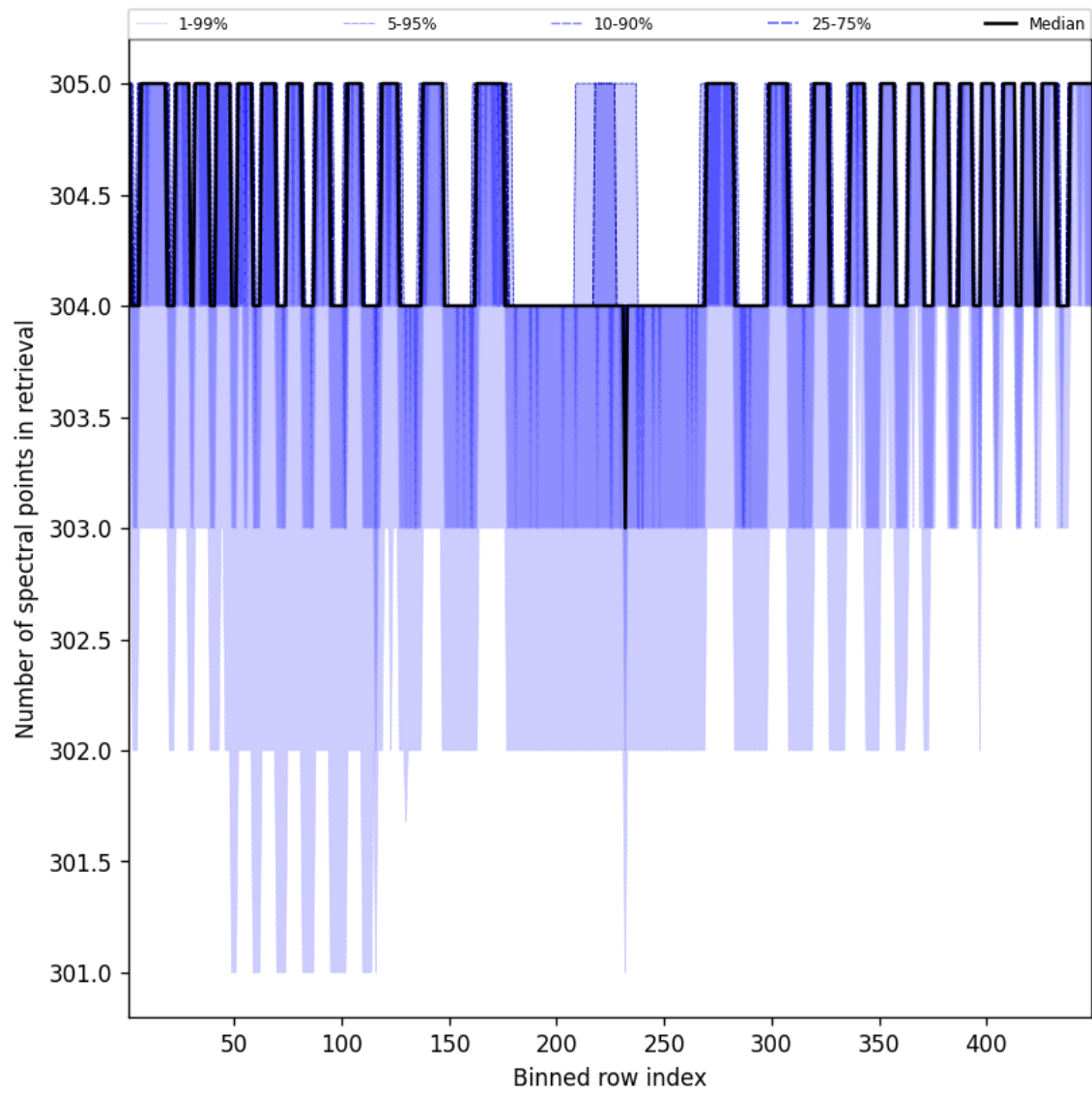
Figure 48: Along track statistics of “Number of spectral points in retrieval” for 2025-03-29 to 2025-03-30
