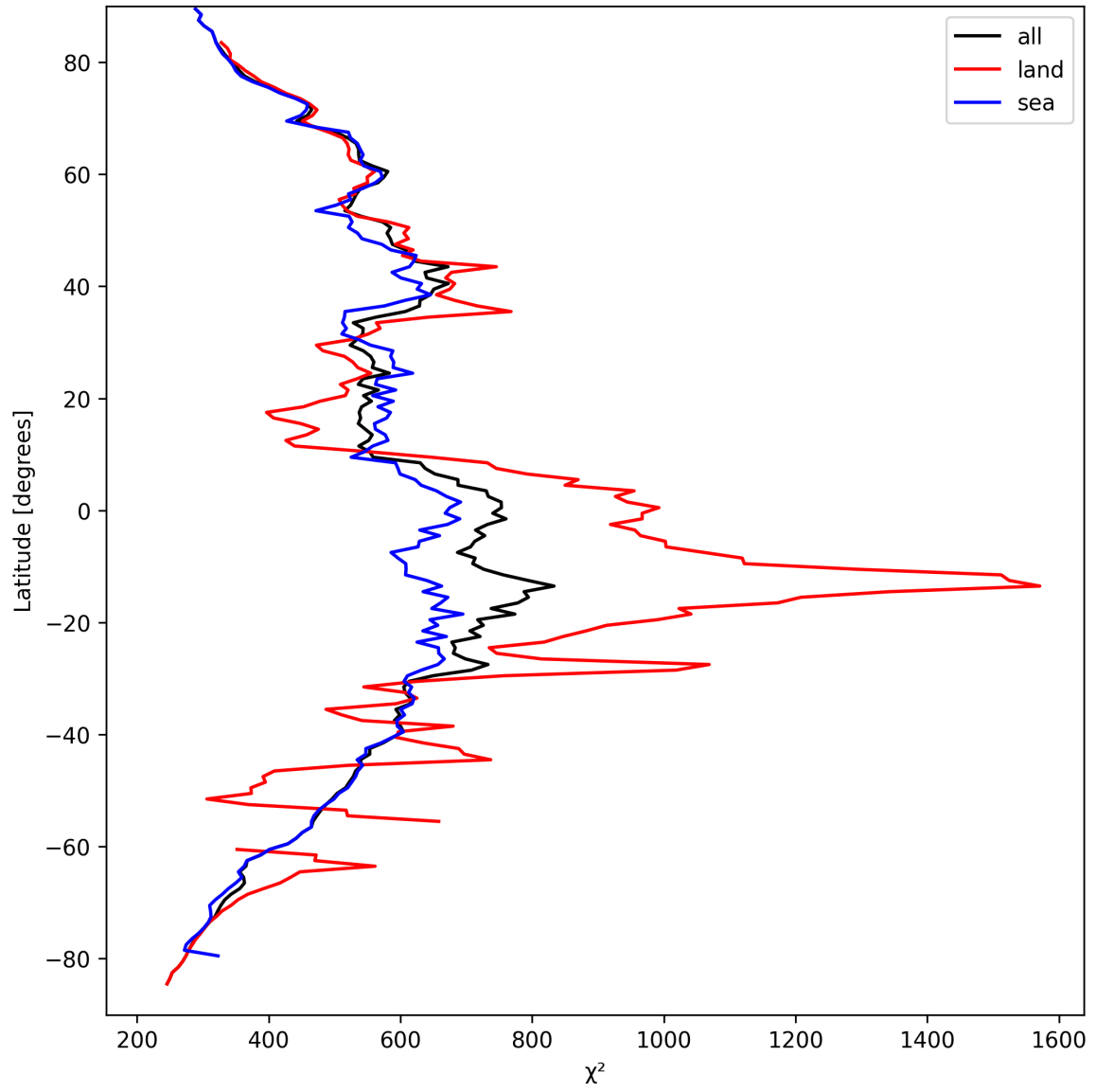
Figure 23: Zonal average of “ \chi^2 ” for 2025-03-29 to 2025-03-30.
