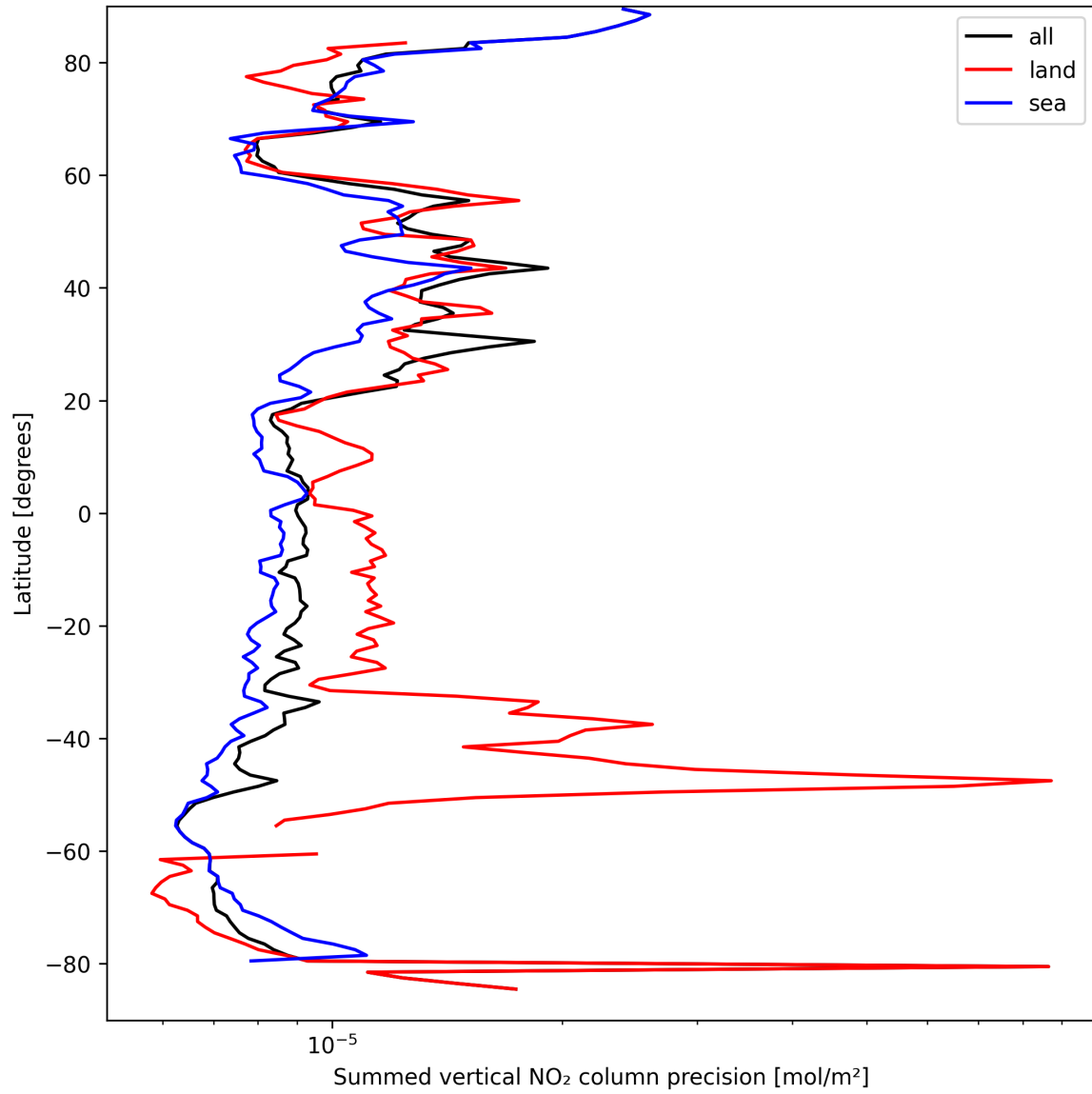
Figure 22: Zonal average of “Summed vertical NO 2 column precision” for 2025-03-29 to 2025-03-30.
