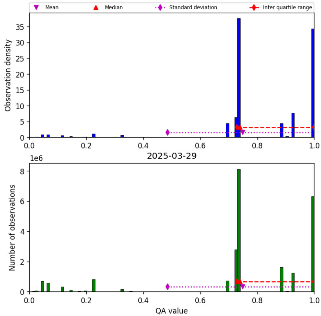
Figure 26: Histogram of “QA value” for 2025-03-29 to 2025-03-30
