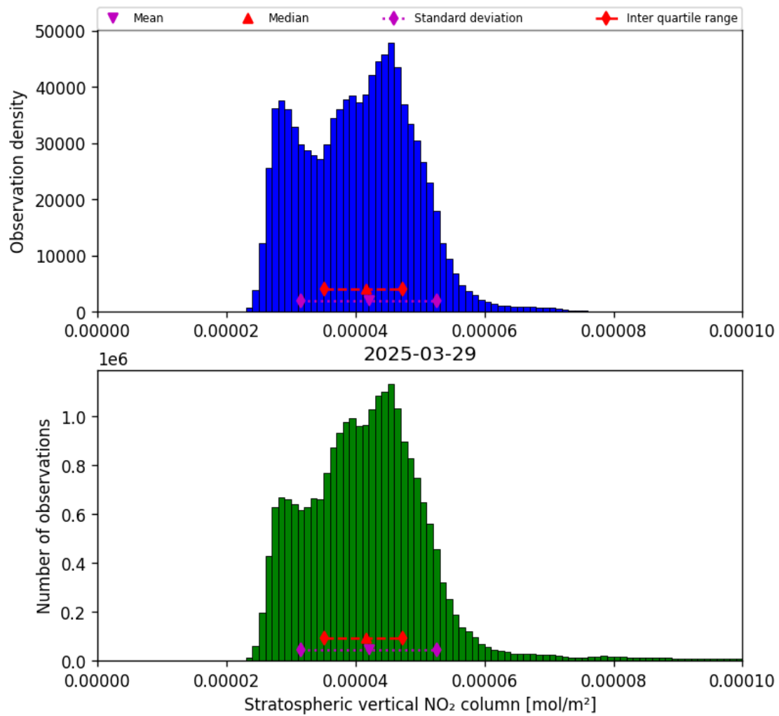
Figure 34: Histogram of “Stratospheric vertical NO 2 column” for 2025-03-29 to 2025-03-30
