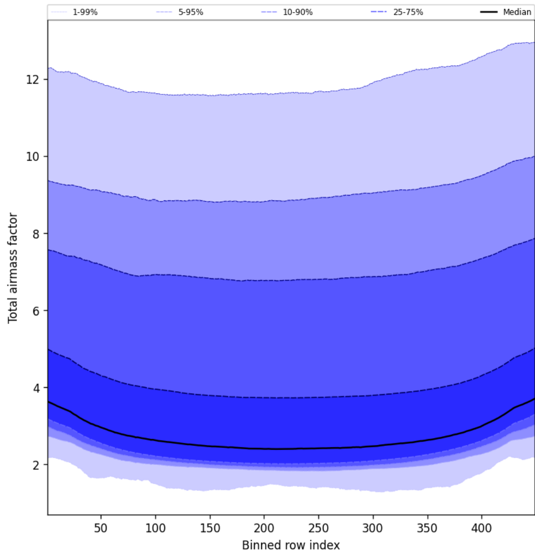
Figure 47: Along track statistics of “Total airmass factor” for 2025-03-29 to 2025-03-30
