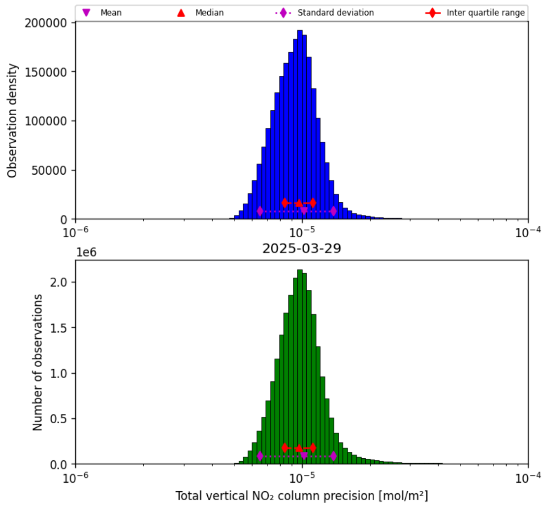
Figure 37: Histogram of "Total vertical NO 2 column precision" for 2025-03-29 to 2025-03-30
