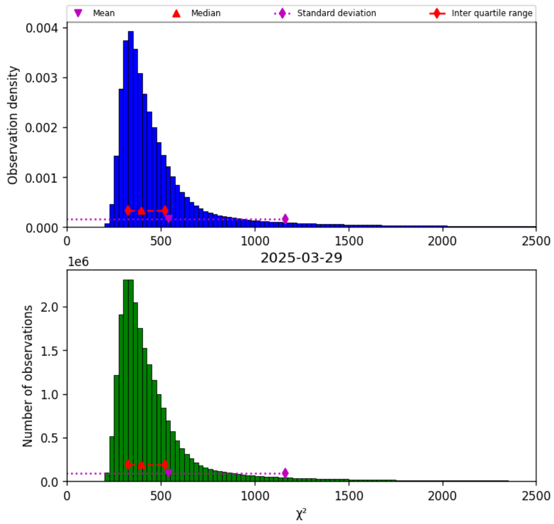
Figure 40: Histogram of “ \chi^2 ” for 2025-03-29 to 2025-03-30
