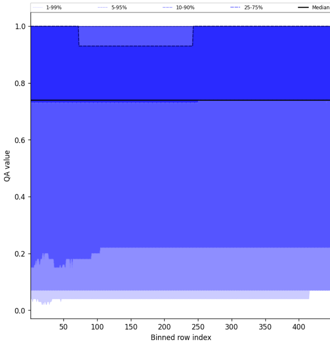
Figure 43: Along track statistics of “QA value” for 2025-03-29 to 2025-03-30
