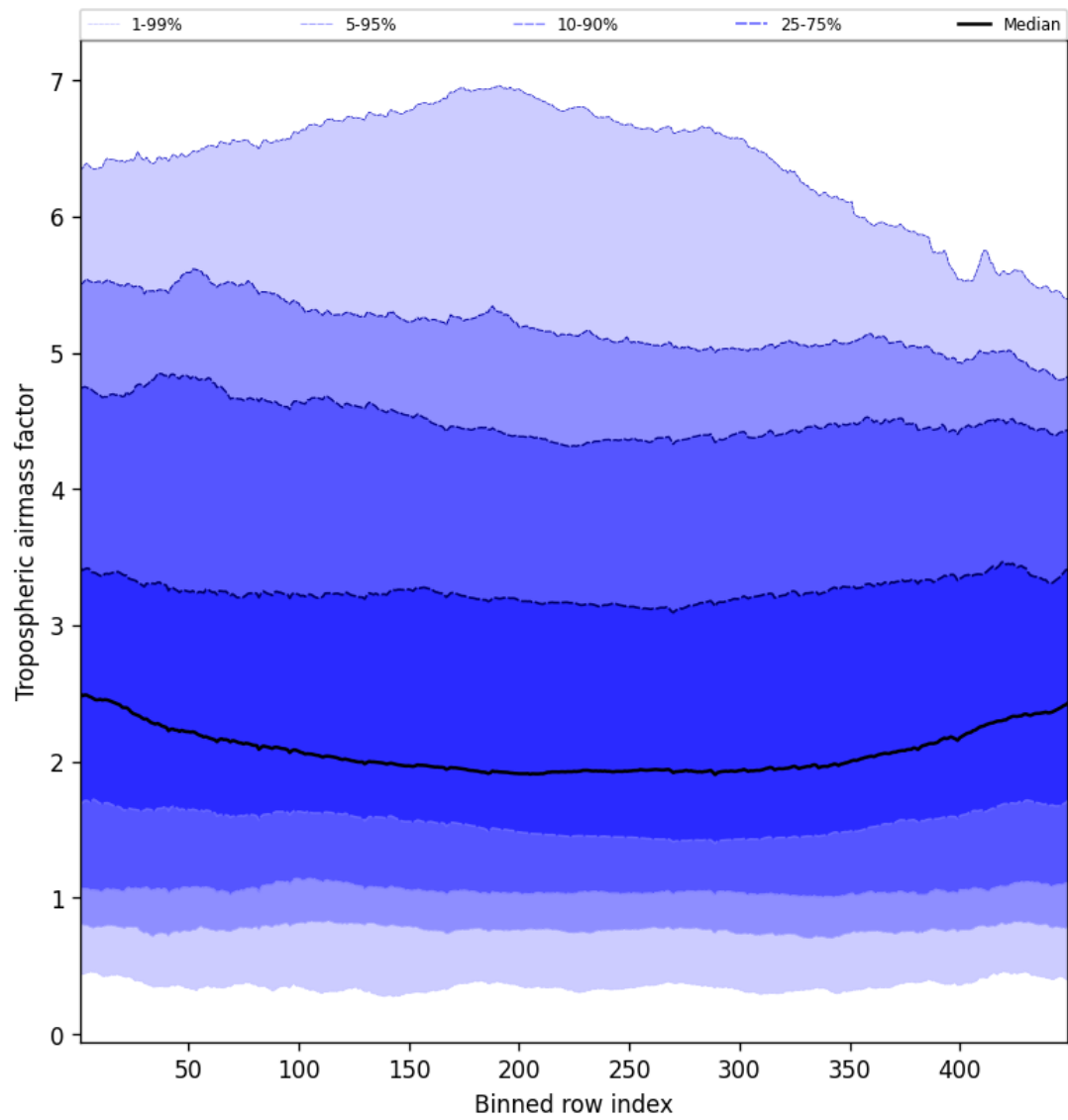
Figure 46: Along track statistics of “Tropospheric airmass factor” for 2025-03-29 to 2025-03-30
