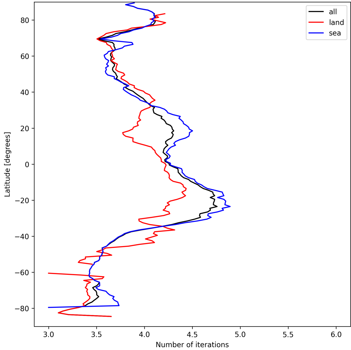
Figure 15: Zonal average of “Number of iterations” for 2025-03-29 to 2025-03-30.
