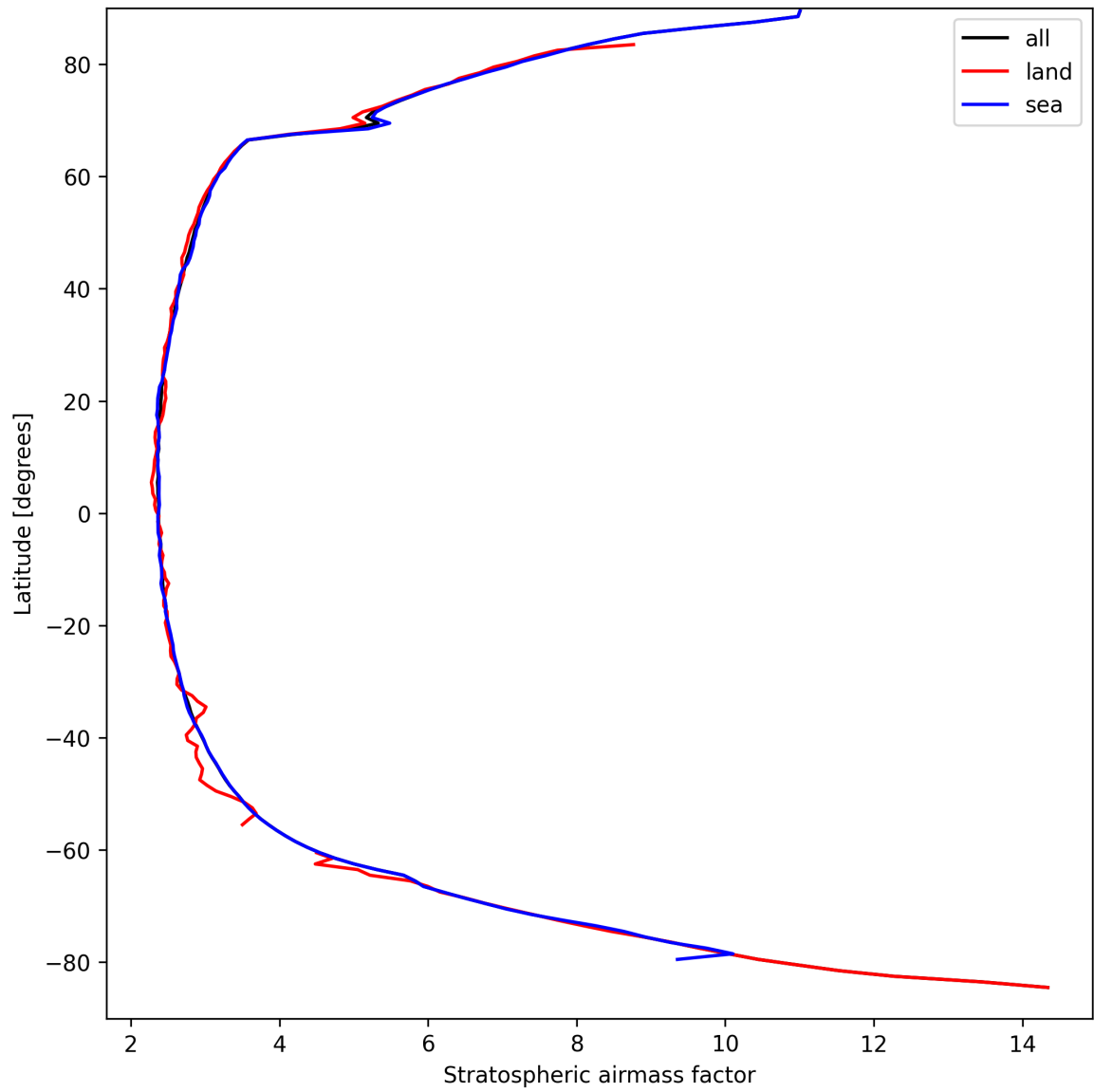
Figure 25: Zonal average of “Stratospheric airmass factor” for 2025-03-29 to 2025-03-30.
