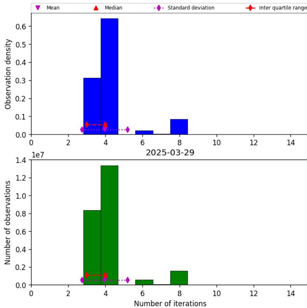
Figure 32: Histogram of “Number of iterations” for 2025-03-29 to 2025-03-30
