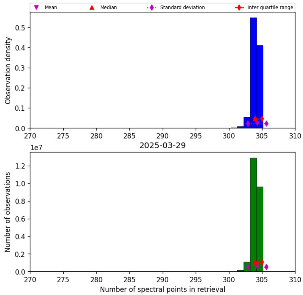
Figure 31: Histogram of “Number of spectral points in retrieval” for 2025-03-29 to 2025-03-30
