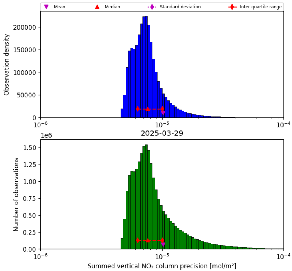
Figure 39: Histogram of "Summed vertical NO 2 column precision" for 2025-03-29 to 2025-03-30
