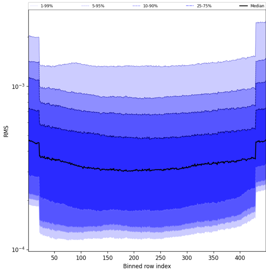
Figure 58: Along track statistics of “RMS” for 2025-03-30 to 2025-03-31
