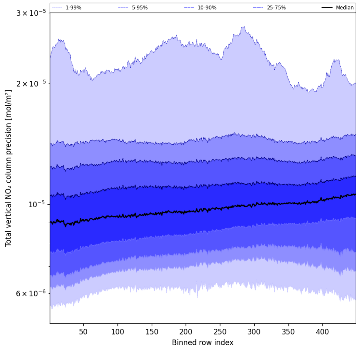
Figure 54: Along track statistics of “Total vertical NO 2 column precision” for 2025-03-30 to 2025-03-31
