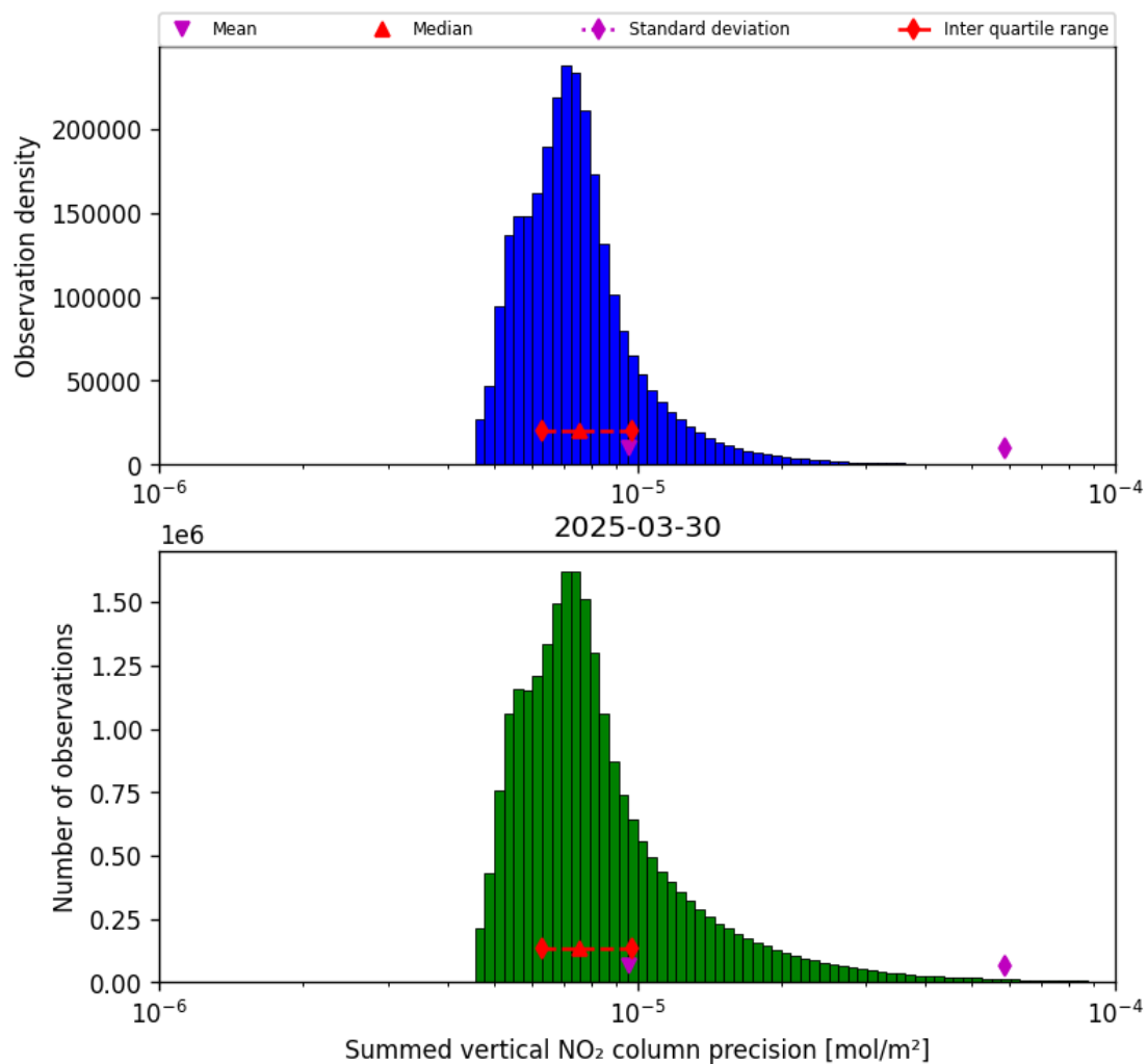
Figure 39: Histogram of “Summed vertical NO 2 column precision” for 2025-03-30 to 2025-03-31
