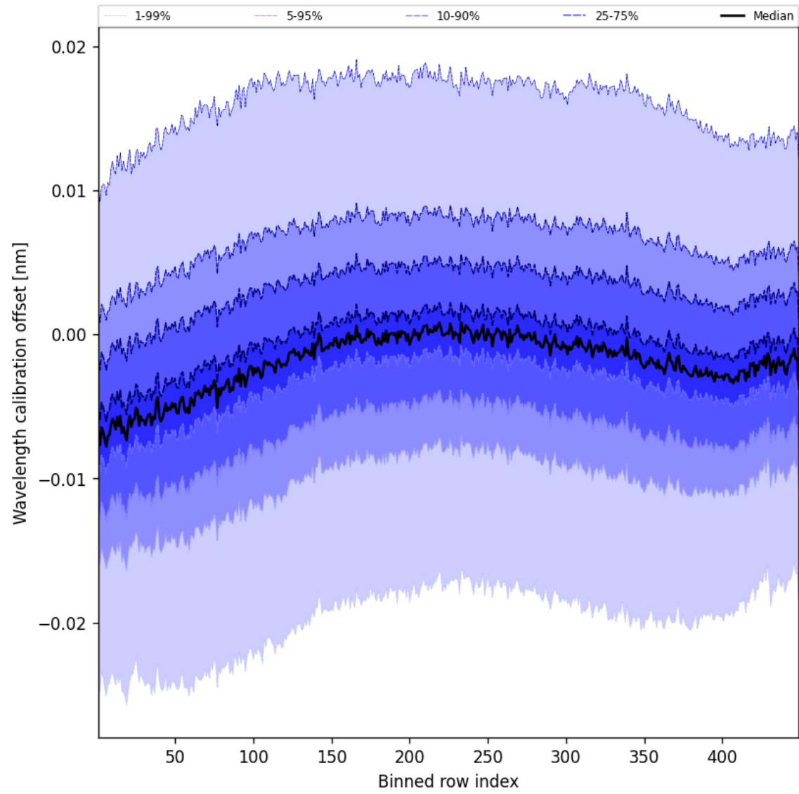
Figure 50: Along track statistics of “Wavelength calibration offset” for 2025-03-30 to 2025-03-31
