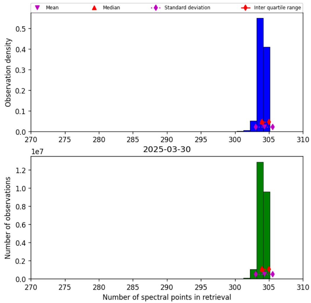
Figure 31: Histogram of “Number of spectral points in retrieval” for 2025-03-30 to 2025-03-31
