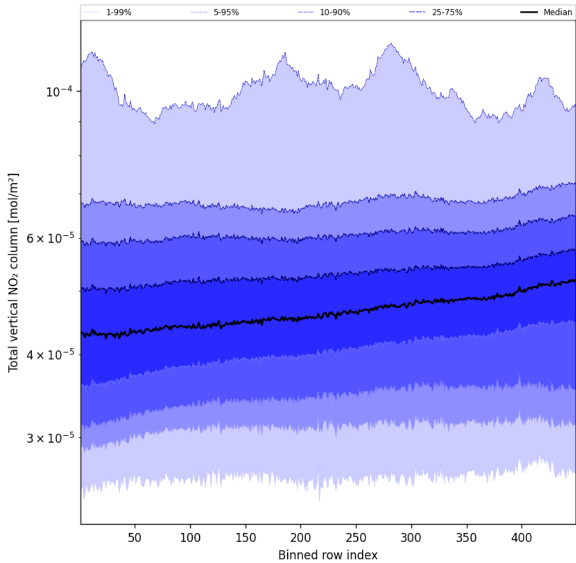
Figure 53: Along track statistics of “Total vertical NO 2 column” for 2025-03-30 to 2025-03-31
