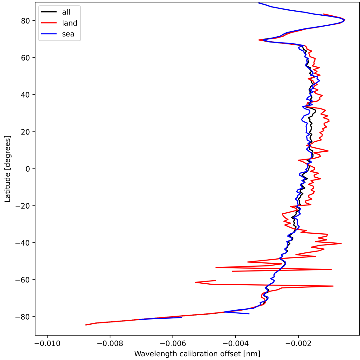
Figure 16: Zonal average of “Wavelength calibration offset” for 2025-03-30 to 2025-03-31.
