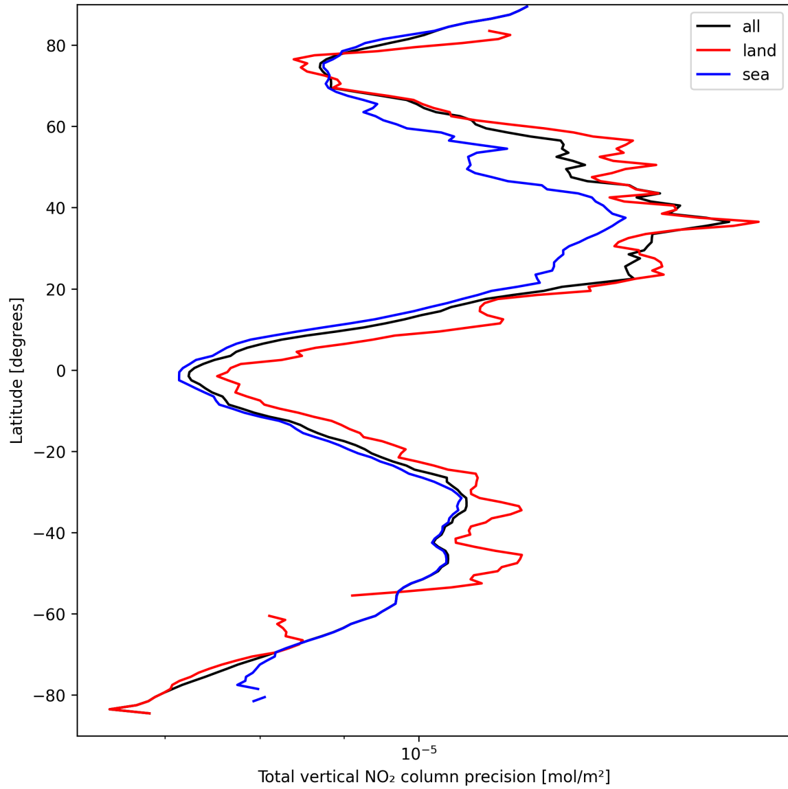
Figure 20: Zonal average of “Total vertical NO 2 column precision” for 2025-03-30 to 2025-03-31.
