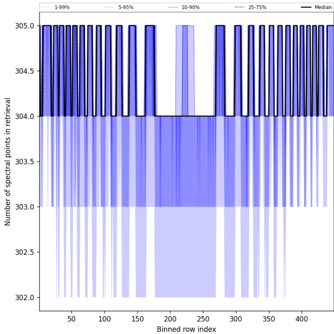
Figure 48: Along track statistics of “Number of spectral points in retrieval” for 2025-03-30 to 2025-03-31
