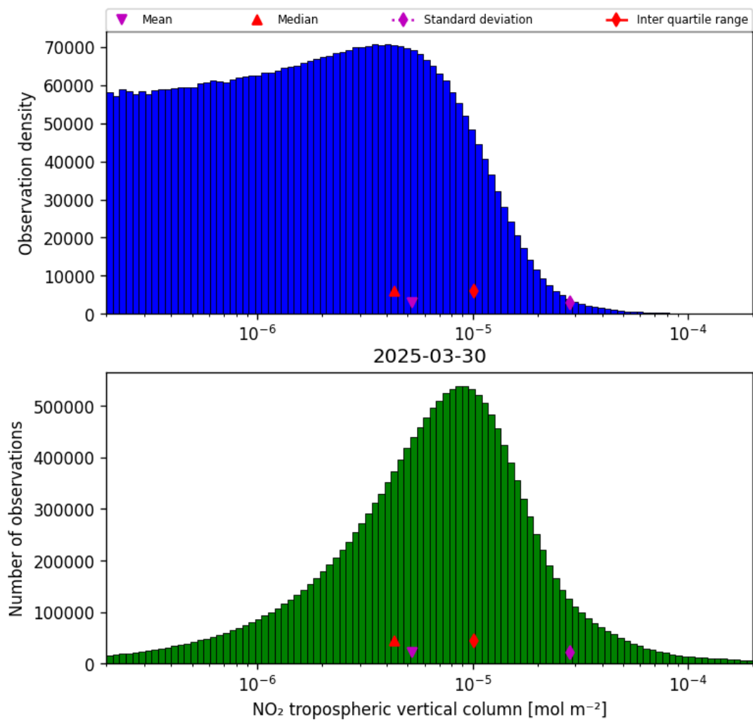
Figure 27: Histogram of “NO 2 tropospheric vertical column” for 2025-03-30 to 2025-03-31
