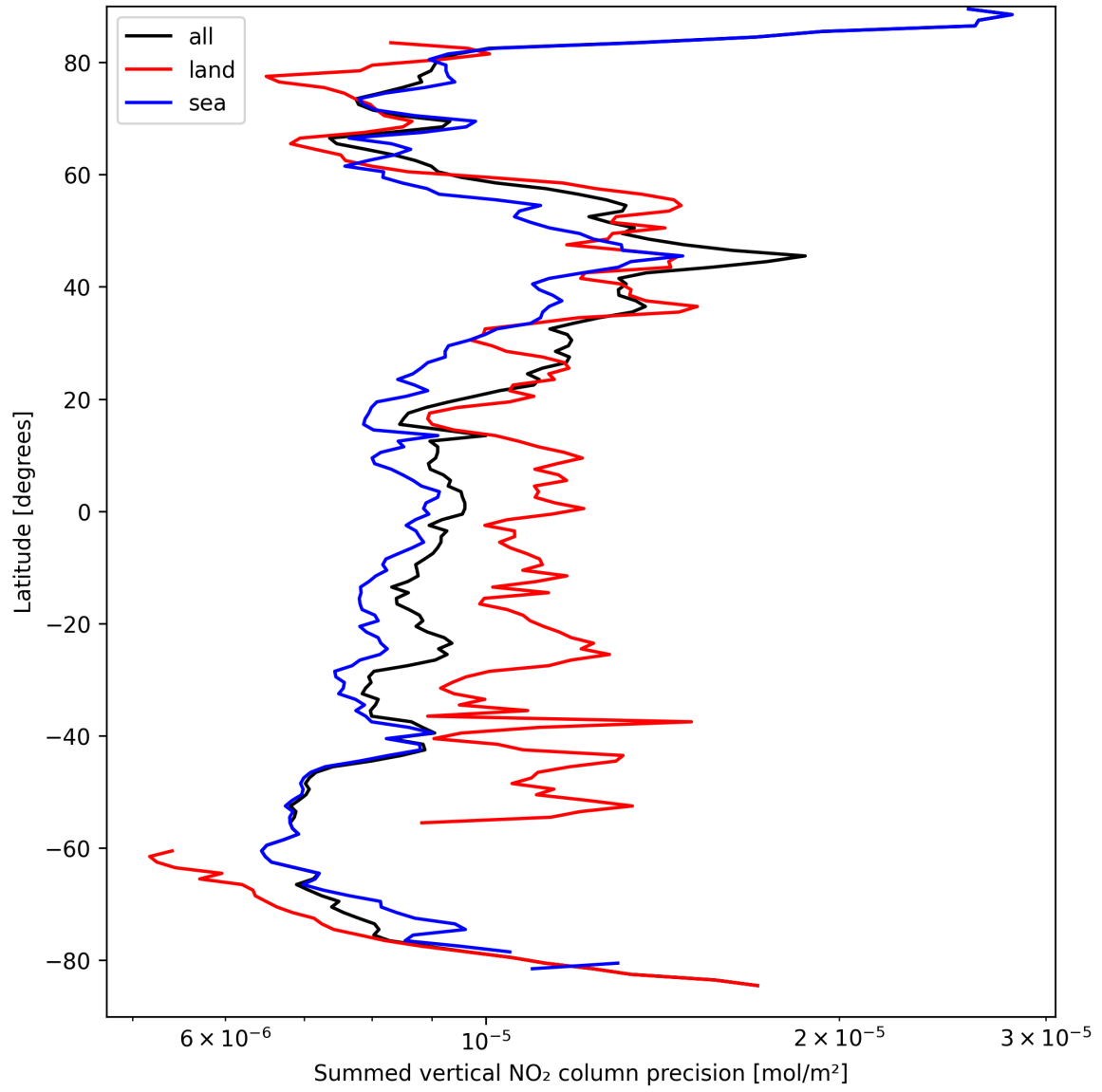
Figure 22: Zonal average of “Summed vertical NO 2 column precision” for 2025-03-30 to 2025-03-31.
