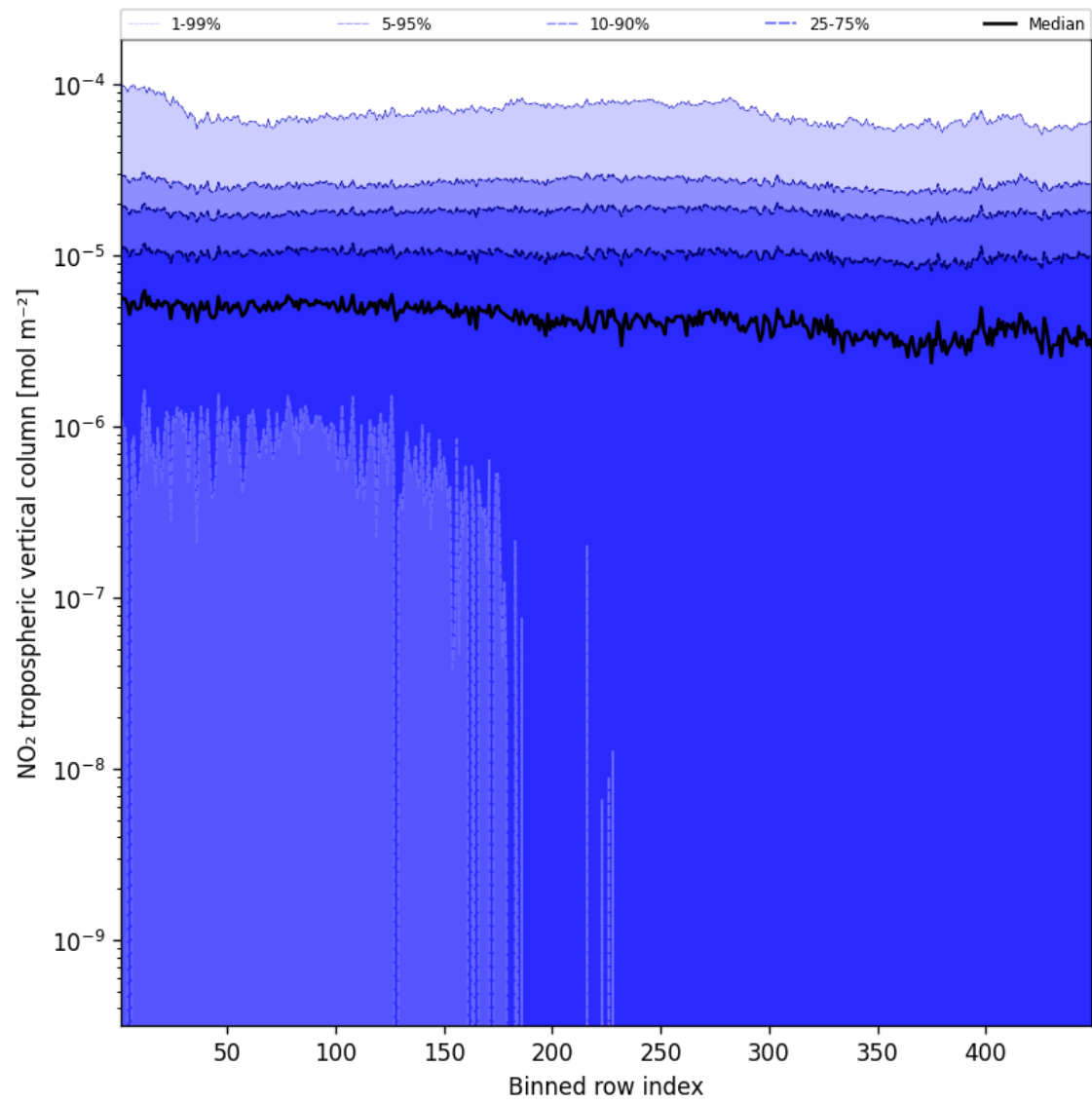
Figure 44: Along track statistics of “NO 2 tropospheric vertical column” for 2025-03-30 to 2025-03-31
