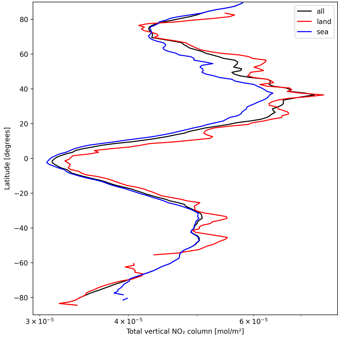
Figure 19: Zonal average of “Total vertical NO 2 column” for 2025-03-30 to 2025-03-31.
