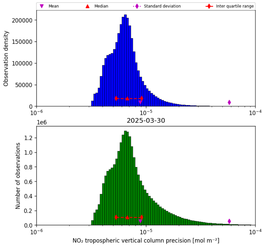
Figure 28: Histogram of “NO 2 tropospheric vertical column precision” for 2025-03-30 to 2025-03-31
