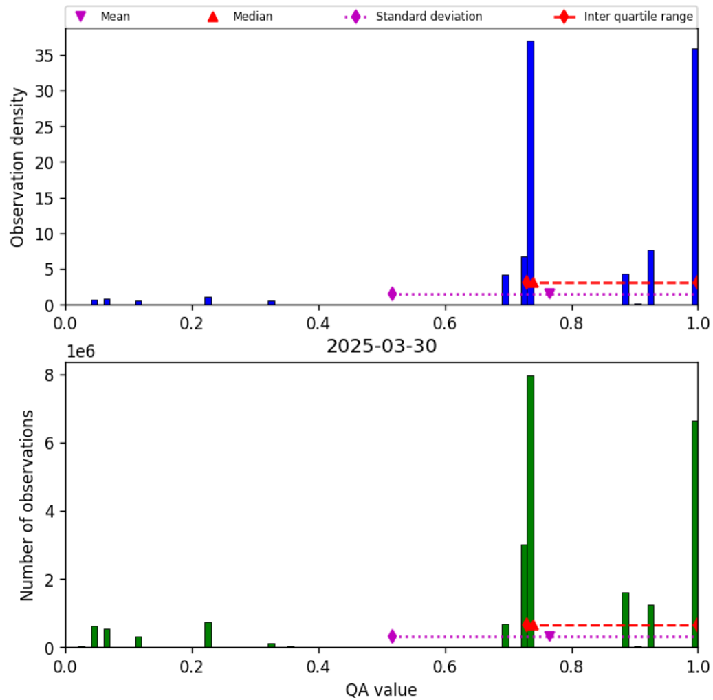
Figure 26: Histogram of “QA value” for 2025-03-30 to 2025-03-31
