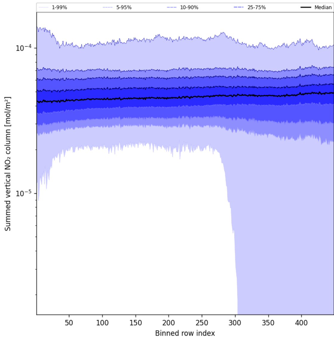
Figure 55: Along track statistics of “Summed vertical NO 2 column” for 2025-03-30 to 2025-03-31
