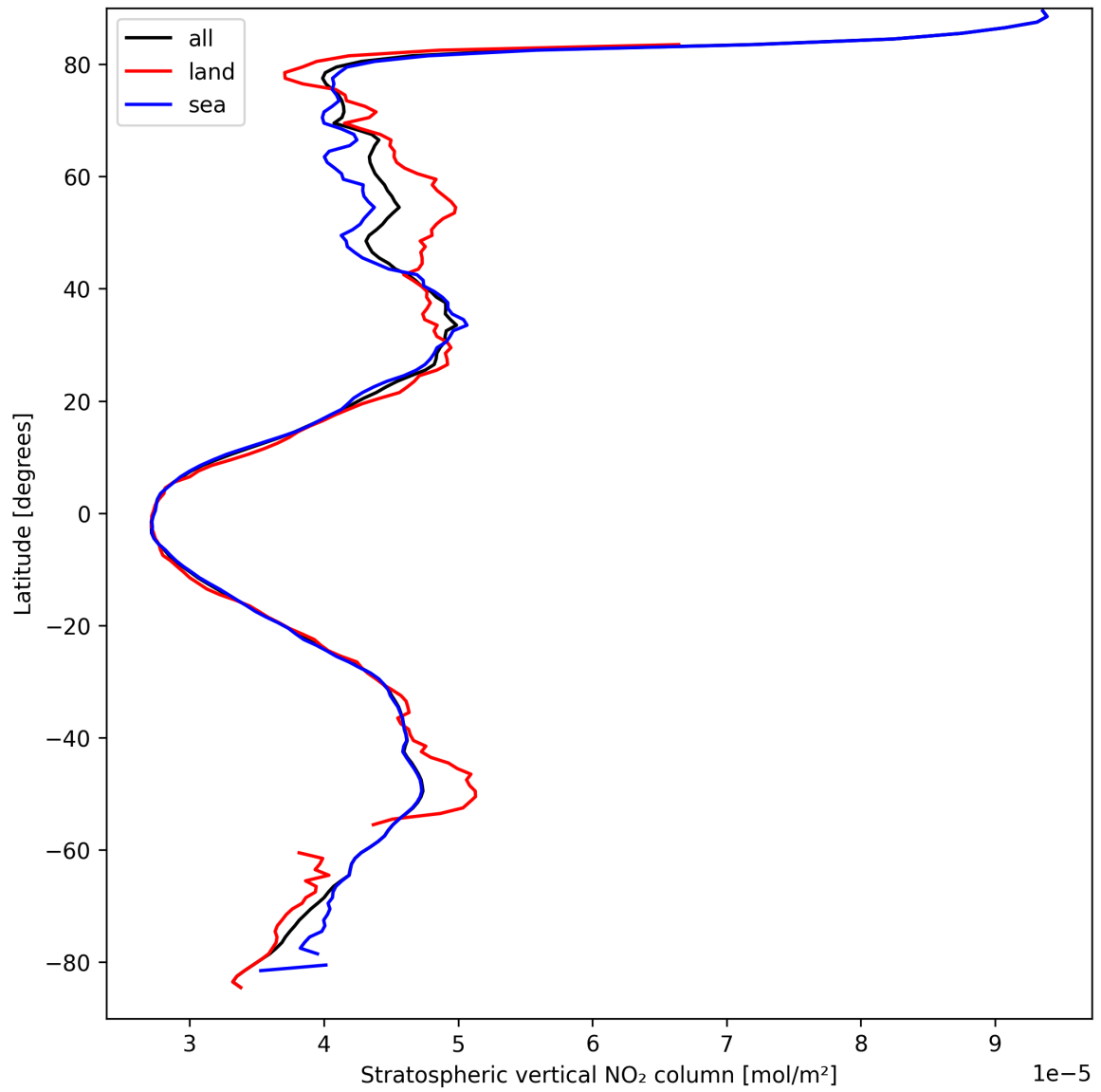
Figure 17: Zonal average of “Stratospheric vertical NO 2 column” for 2025-03-30 to 2025-03-31.
