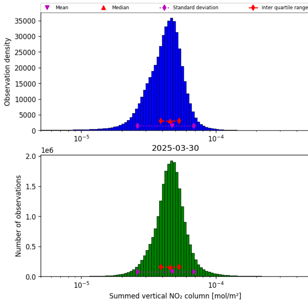
Figure 38: Histogram of "Summed vertical NO 2 column" for 2025-03-30 to 2025-03-31
