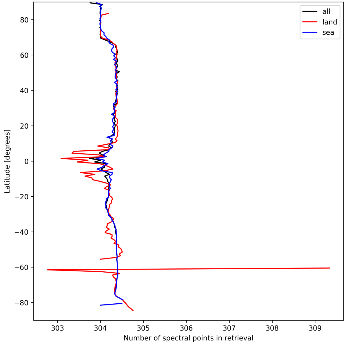
Figure 14: Zonal average of “Number of spectral points in retrieval” for 2025-03-30 to 2025-03-31.
