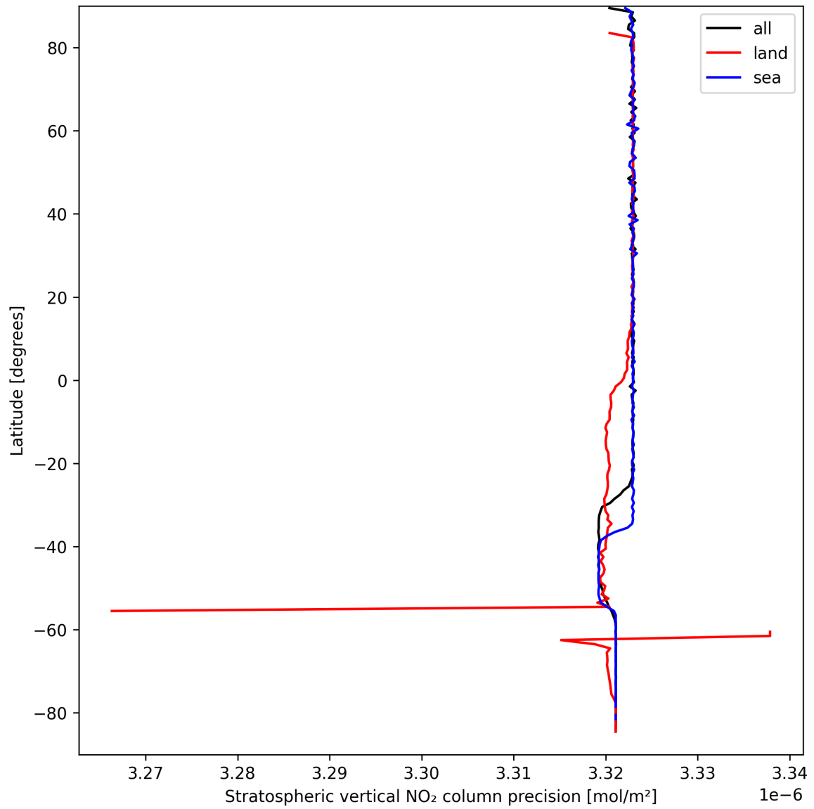
Figure 18: Zonal average of “Stratospheric vertical NO 2 column precision” for 2025-03-30 to 2025-03-31.
