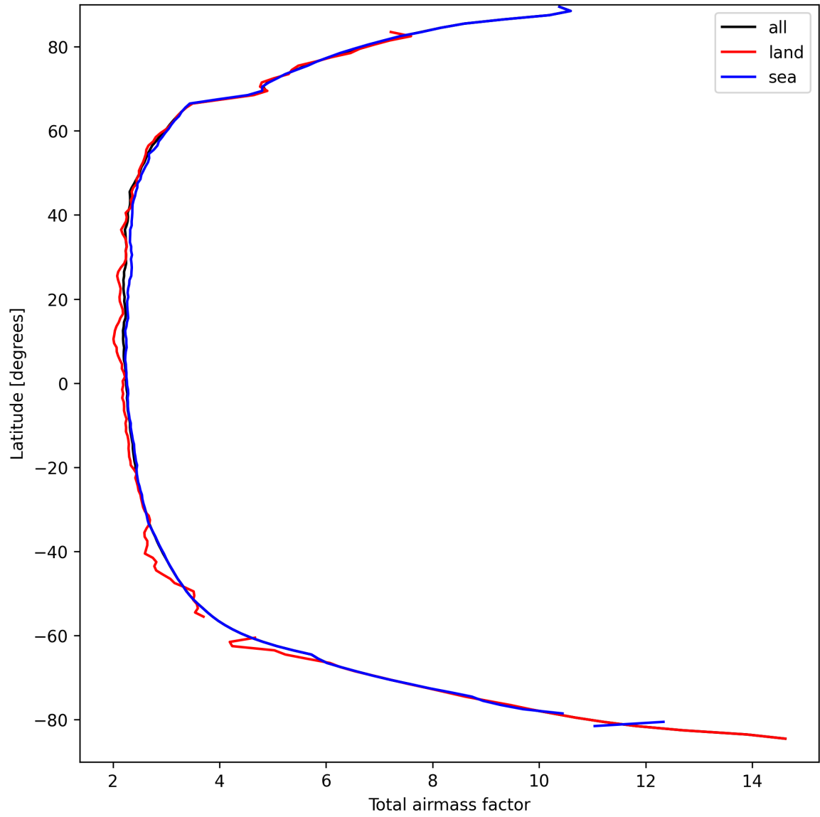
Figure 13: Zonal average of “Total airmass factor” for 2025-03-30 to 2025-03-31.
