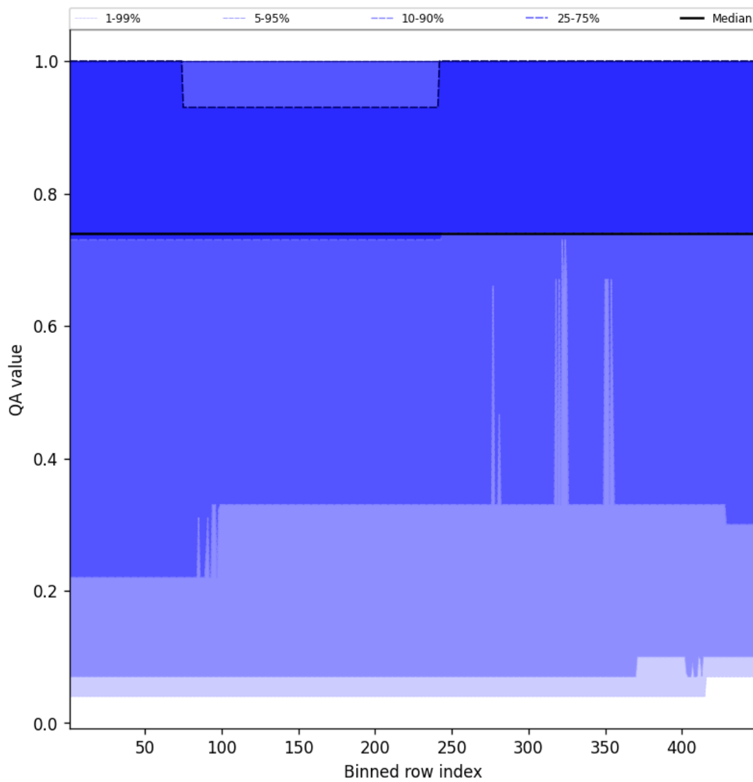
Figure 43: Along track statistics of “QA value” for 2025-03-30 to 2025-03-31
