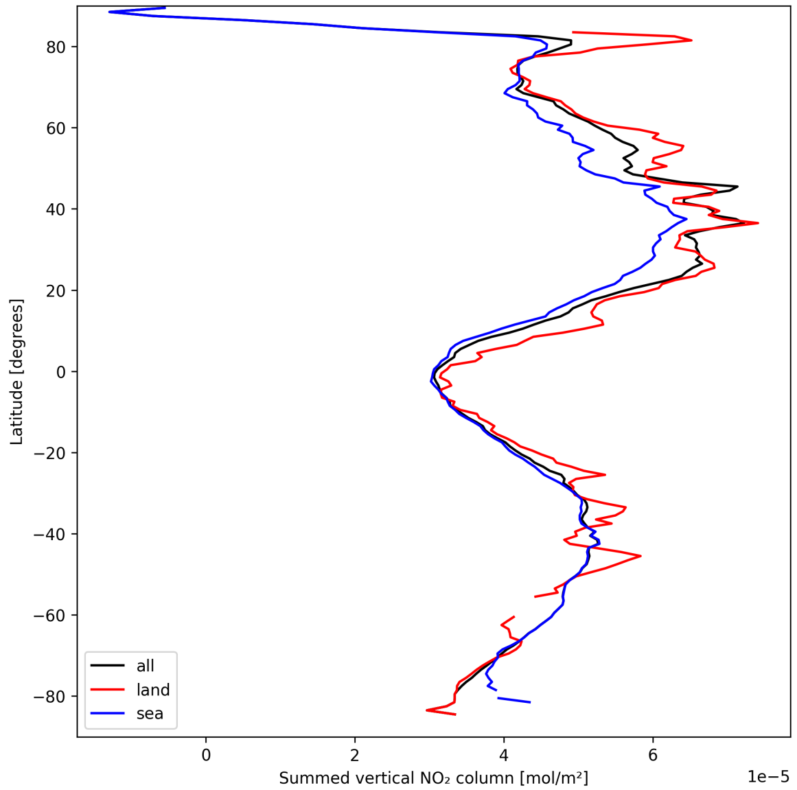
Figure 21: Zonal average of “Summed vertical NO 2 column” for 2025-03-30 to 2025-03-31.
