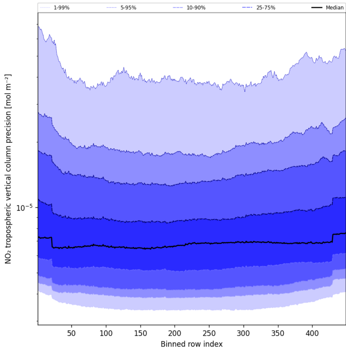
Figure 45: Along track statistics of “NO 2 tropospheric vertical column precision” for 2025-03-30 to 2025-03-31
