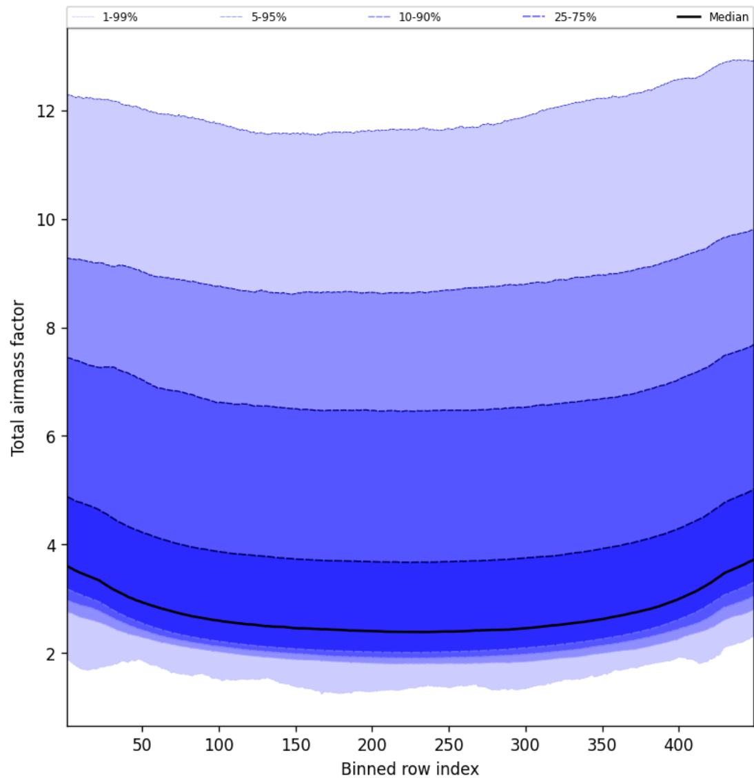
Figure 47: Along track statistics of “Total airmass factor” for 2025-03-30 to 2025-03-31
