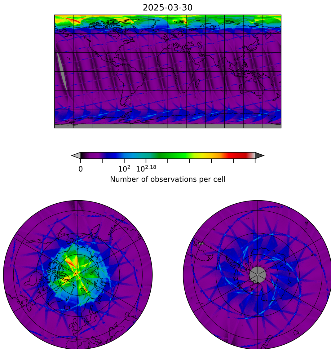
Figure 8: Map of the number of observations for 2025-03-30 to 2025-03-31
