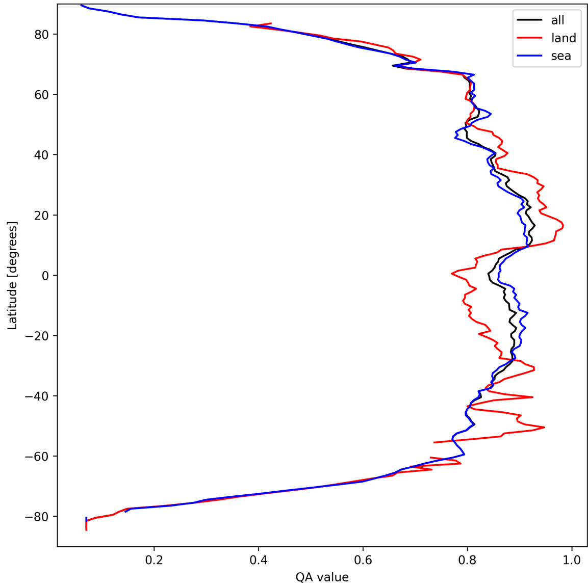
Figure 9: Zonal average of “QA value” for 2025-03-30 to 2025-03-31.
