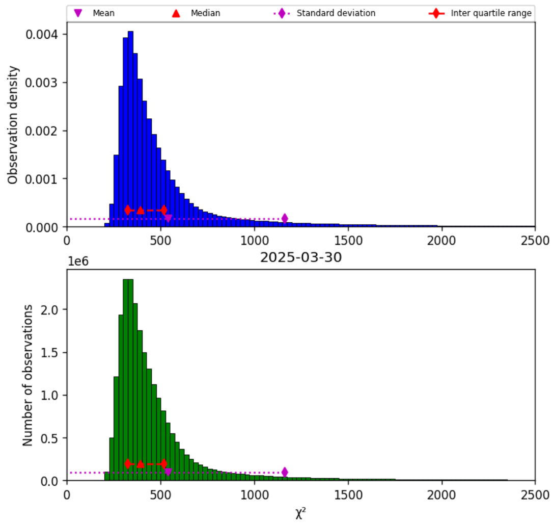
Figure 40: Histogram of “ \chi^2 ” for 2025-03-30 to 2025-03-31
