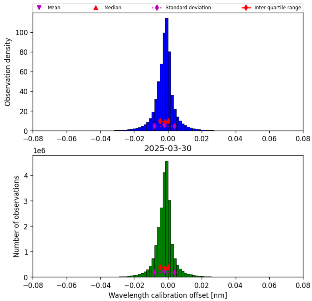
Figure 33: Histogram of “Wavelength calibration offset” for 2025-03-30 to 2025-03-31
