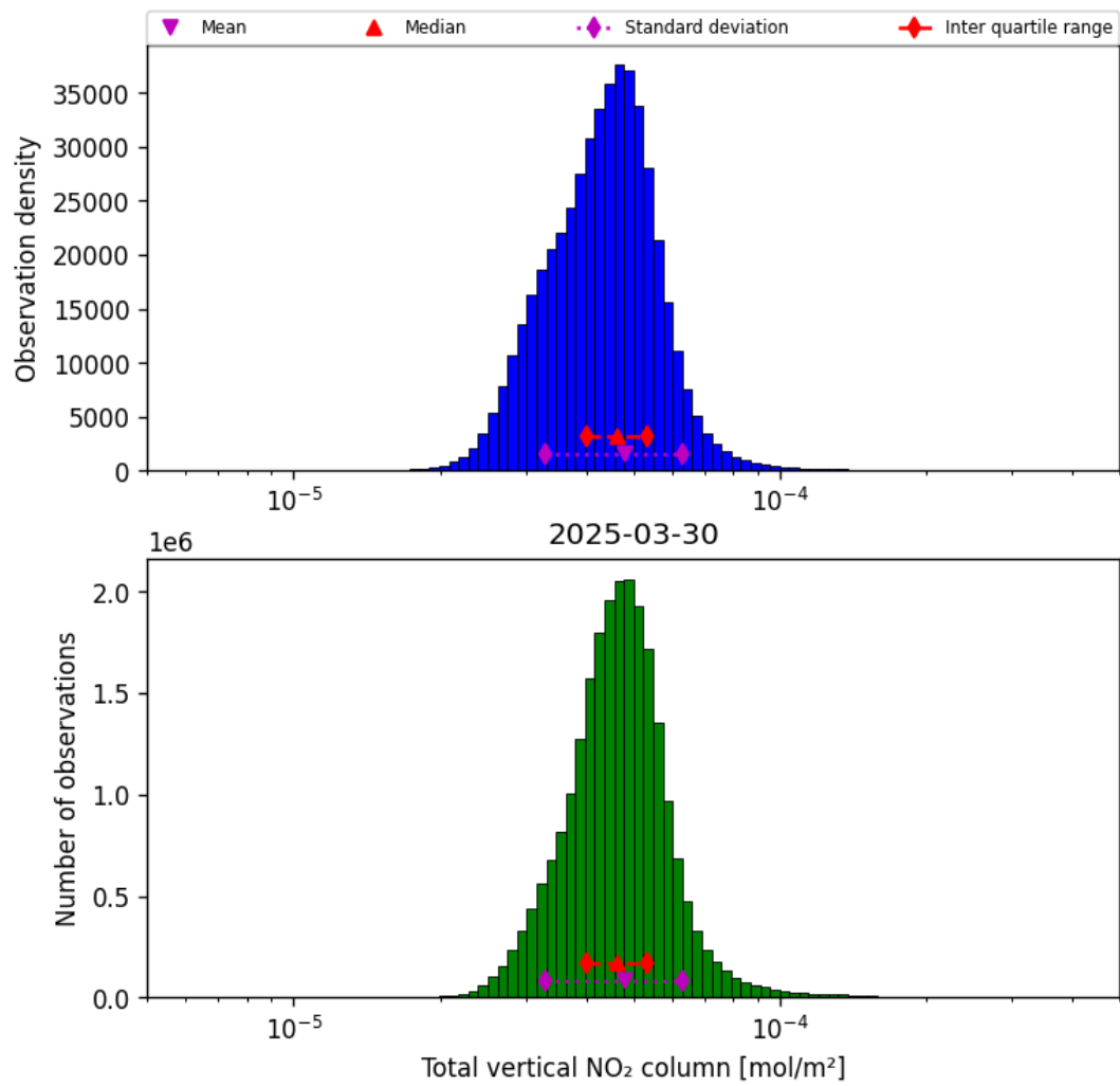
Figure 36: Histogram of "Total vertical NO 2 column" for 2025-03-30 to 2025-03-31
