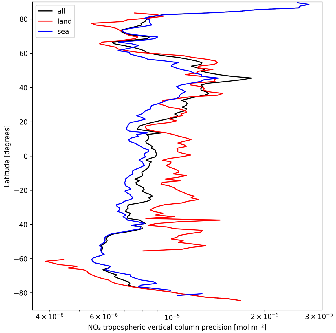
Figure 11: Zonal average of “NO 2 tropospheric vertical column precision” for 2025-03-30 to 2025-03-31.
