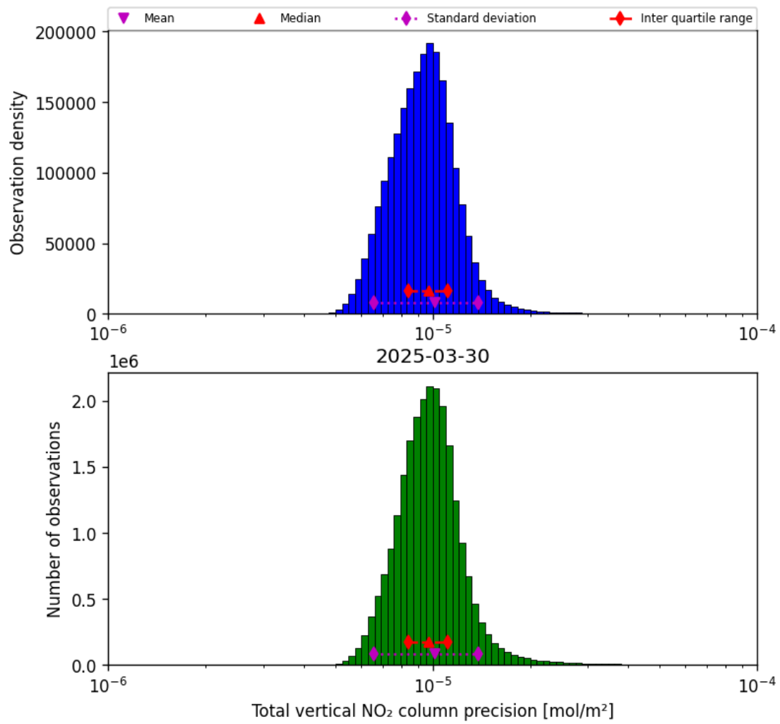
Figure 37: Histogram of "Total vertical NO 2 column precision" for 2025-03-30 to 2025-03-31
