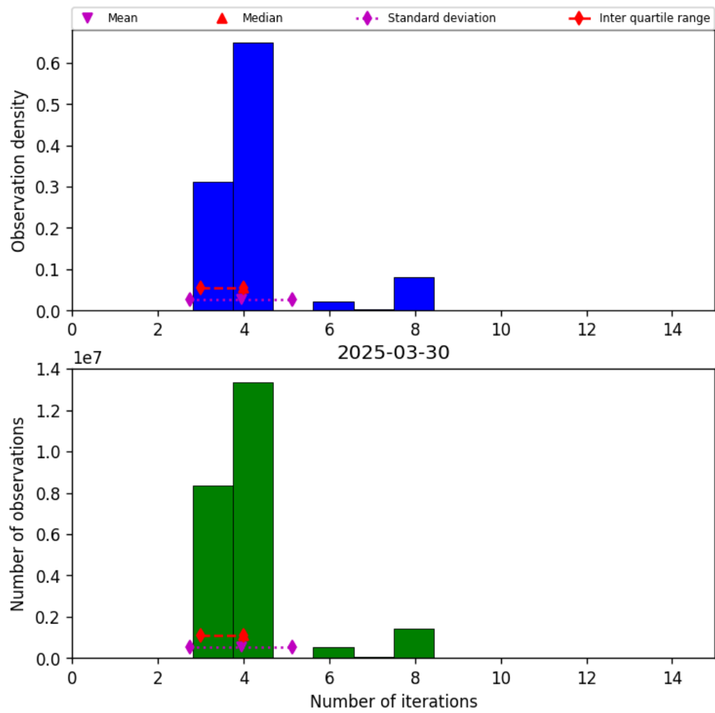
Figure 32: Histogram of “Number of iterations” for 2025-03-30 to 2025-03-31
