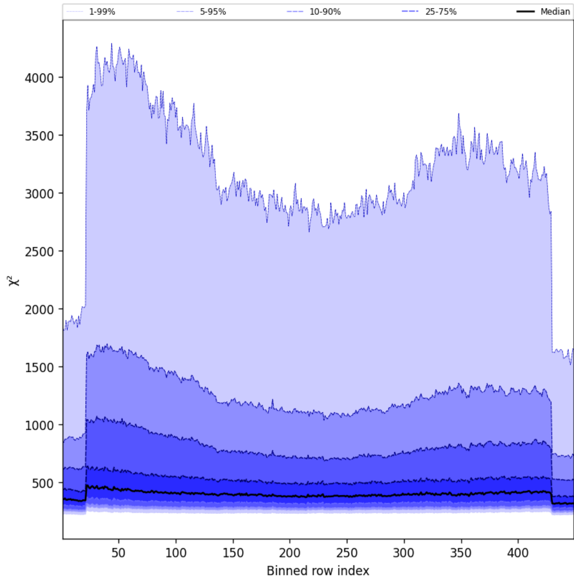
Figure 57: Along track statistics of “ \chi^2 ” for 2025-03-30 to 2025-03-31
