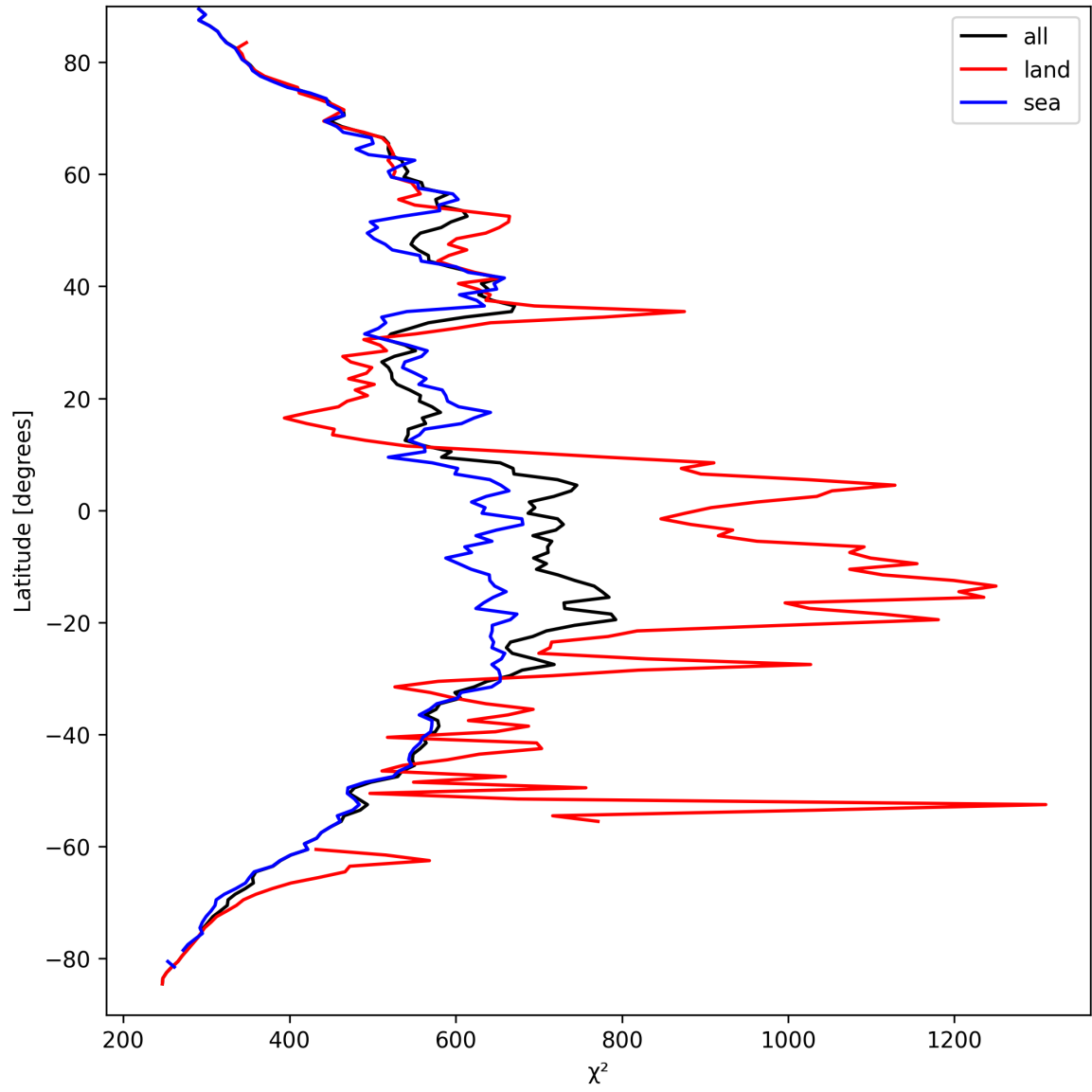
Figure 23: Zonal average of “ \chi^2 ” for 2025-03-30 to 2025-03-31.
