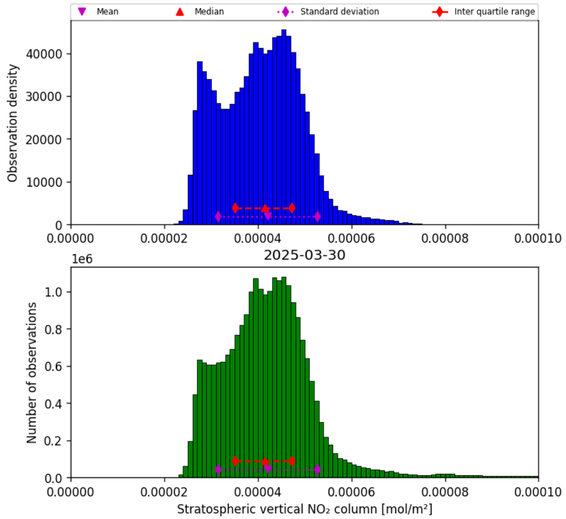
Figure 34: Histogram of “Stratospheric vertical NO 2 column” for 2025-03-30 to 2025-03-31
