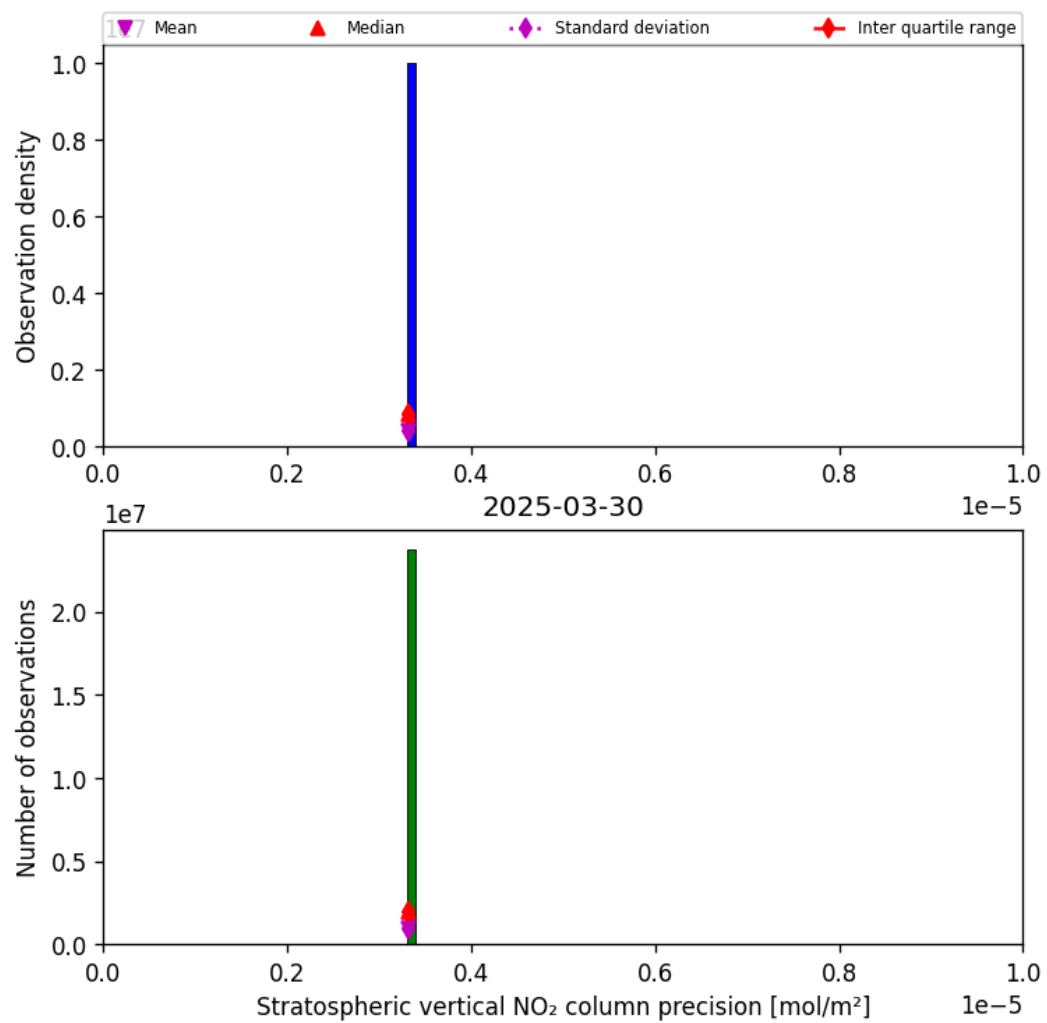
Figure 35: Histogram of “Stratospheric vertical NO 2 column precision” for 2025-03-30 to 2025-03-31
