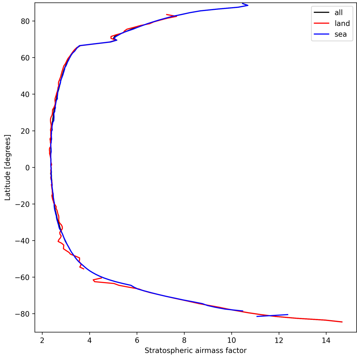
Figure 25: Zonal average of “Stratospheric air mass factor” for 2025-03-30 to 2025-03-31.
