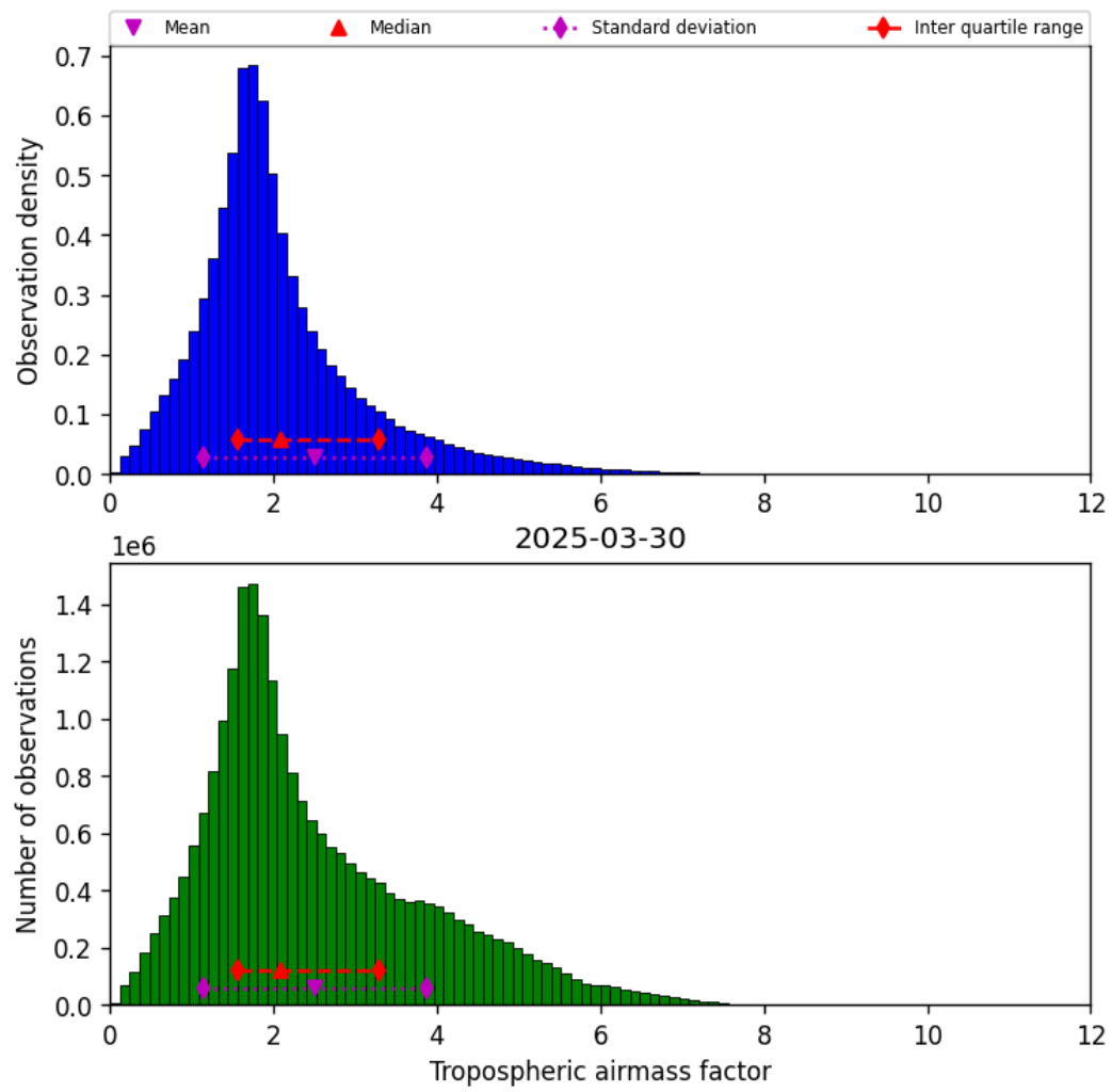
Figure 29: Histogram of “Tropospheric airmass factor” for 2025-03-30 to 2025-03-31
