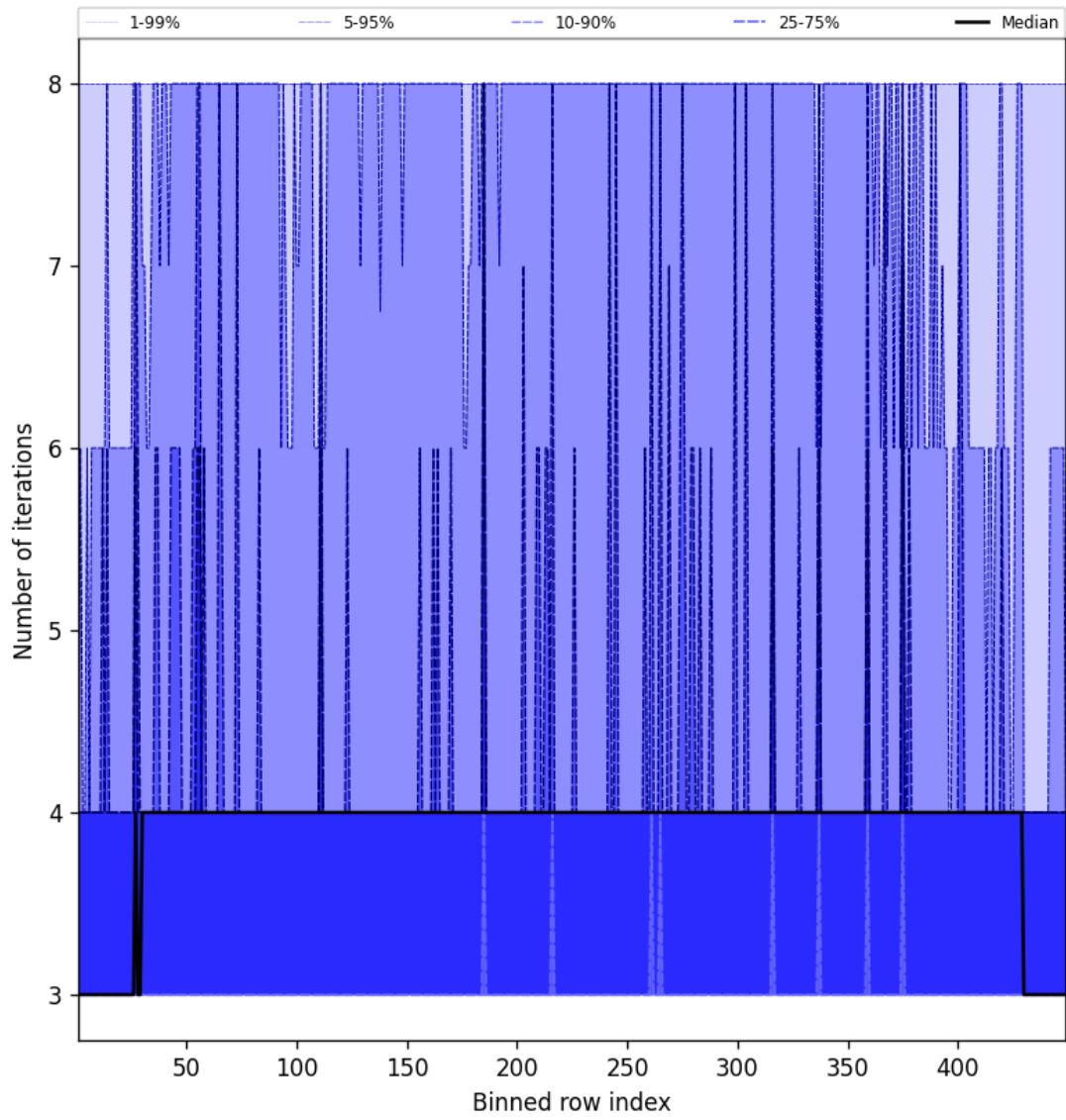
Figure 49: Along track statistics of “Number of iterations” for 2025-03-30 to 2025-03-31
