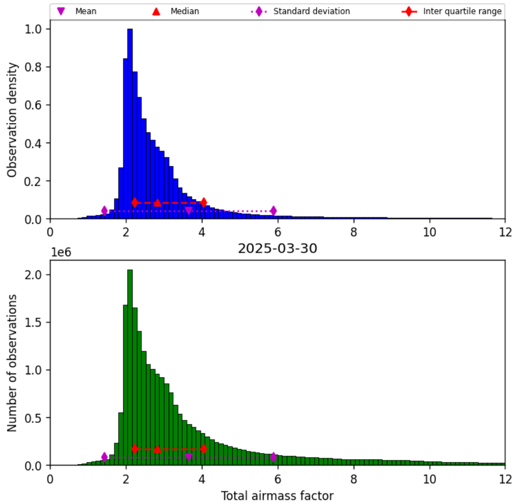
Figure 30: Histogram of “Total airmass factor” for 2025-03-30 to 2025-03-31
