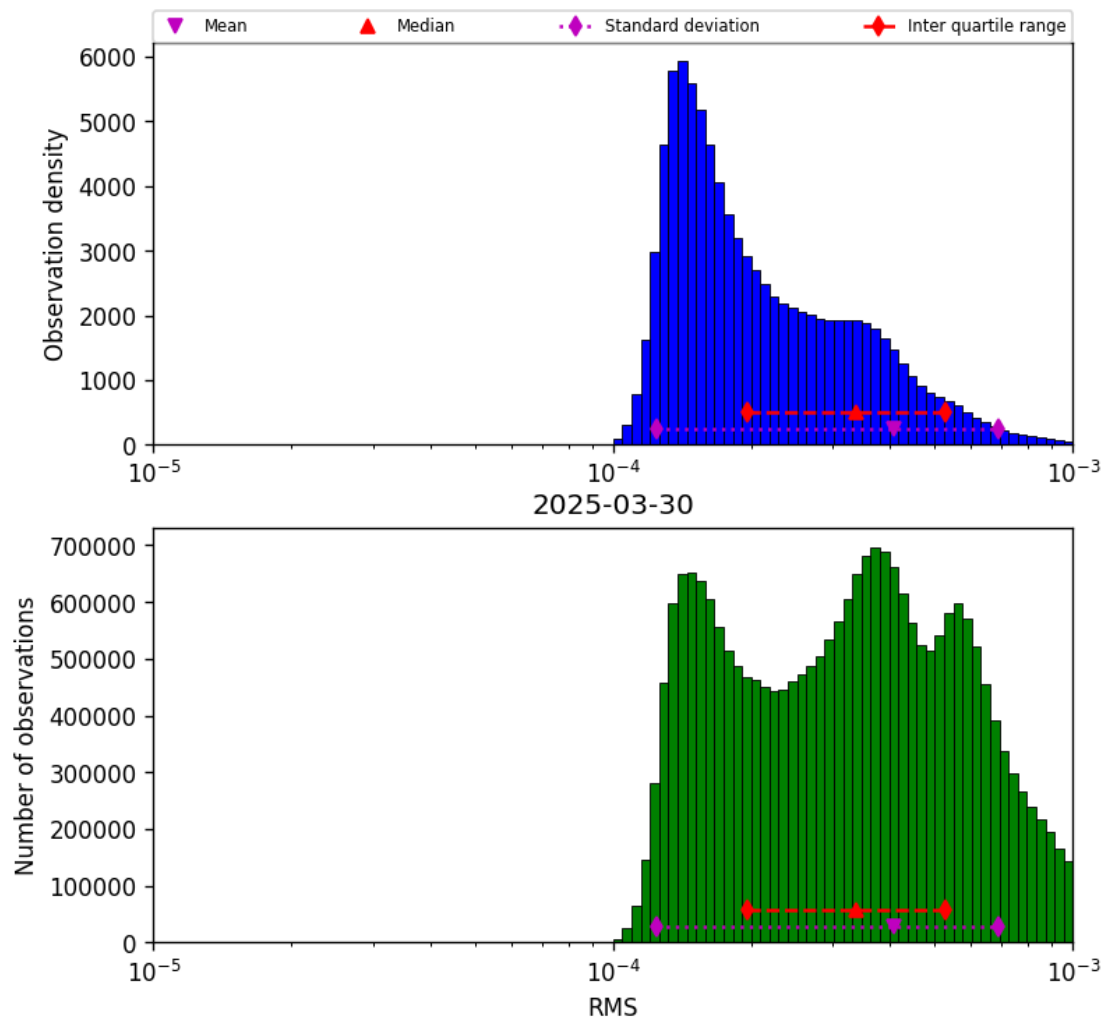
Figure 41: Histogram of “RMS” for 2025-03-30 to 2025-03-31
