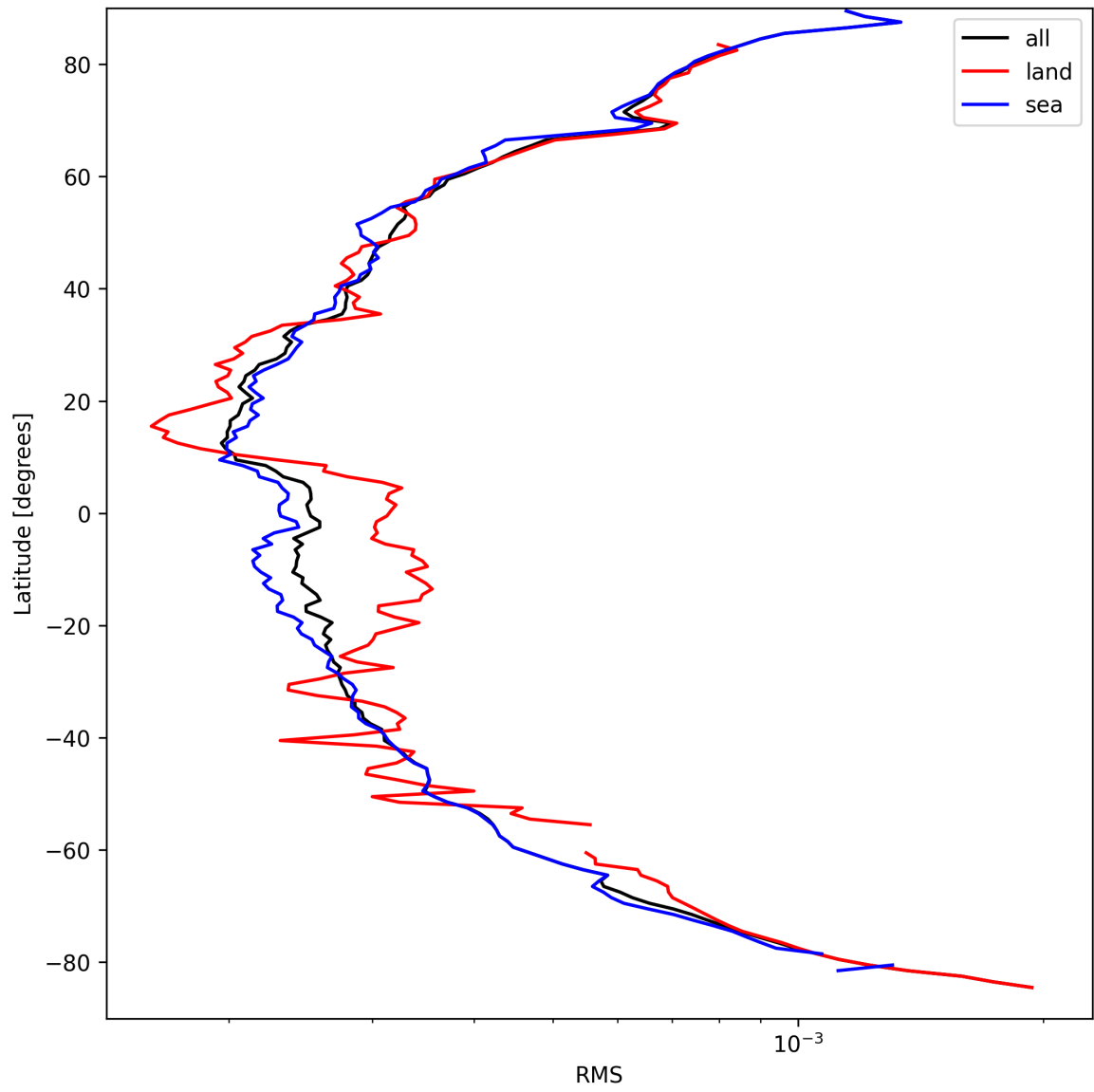
Figure 24: Zonal average of “RMS” for 2025-03-30 to 2025-03-31.
