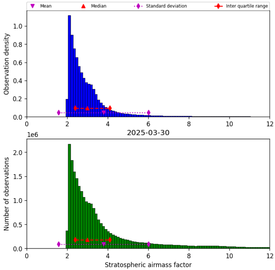
Figure 42: Histogram of “Stratospheric airmass factor” for 2025-03-30 to 2025-03-31
