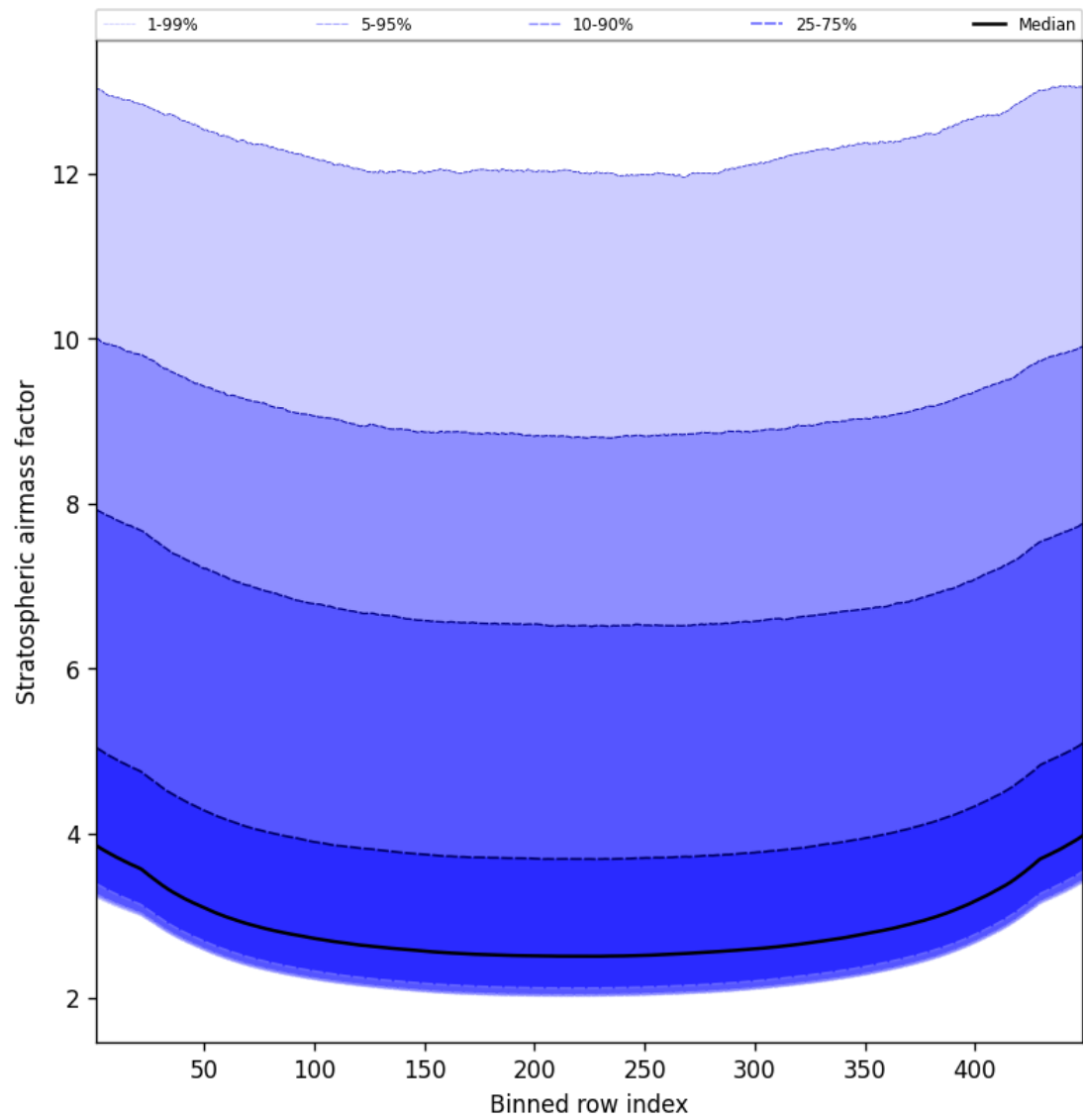
Figure 59: Along track statistics of “Stratospheric airmass factor” for 2025-03-30 to 2025-03-31
