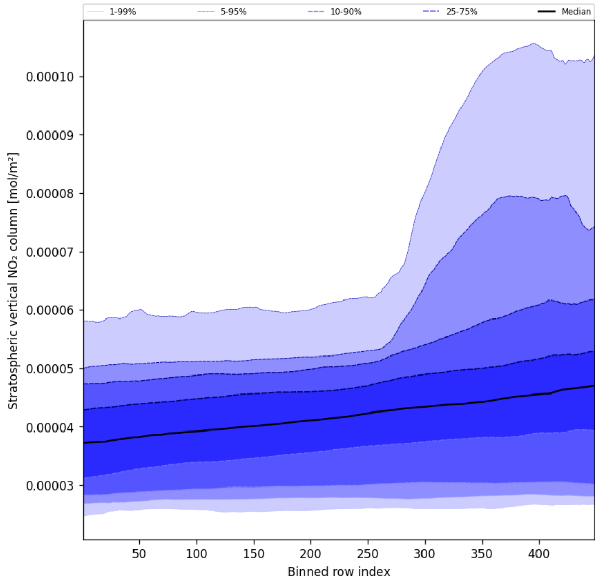
Figure 51: Along track statistics of “Stratospheric vertical NO 2 column” for 2025-03-30 to 2025-03-31
