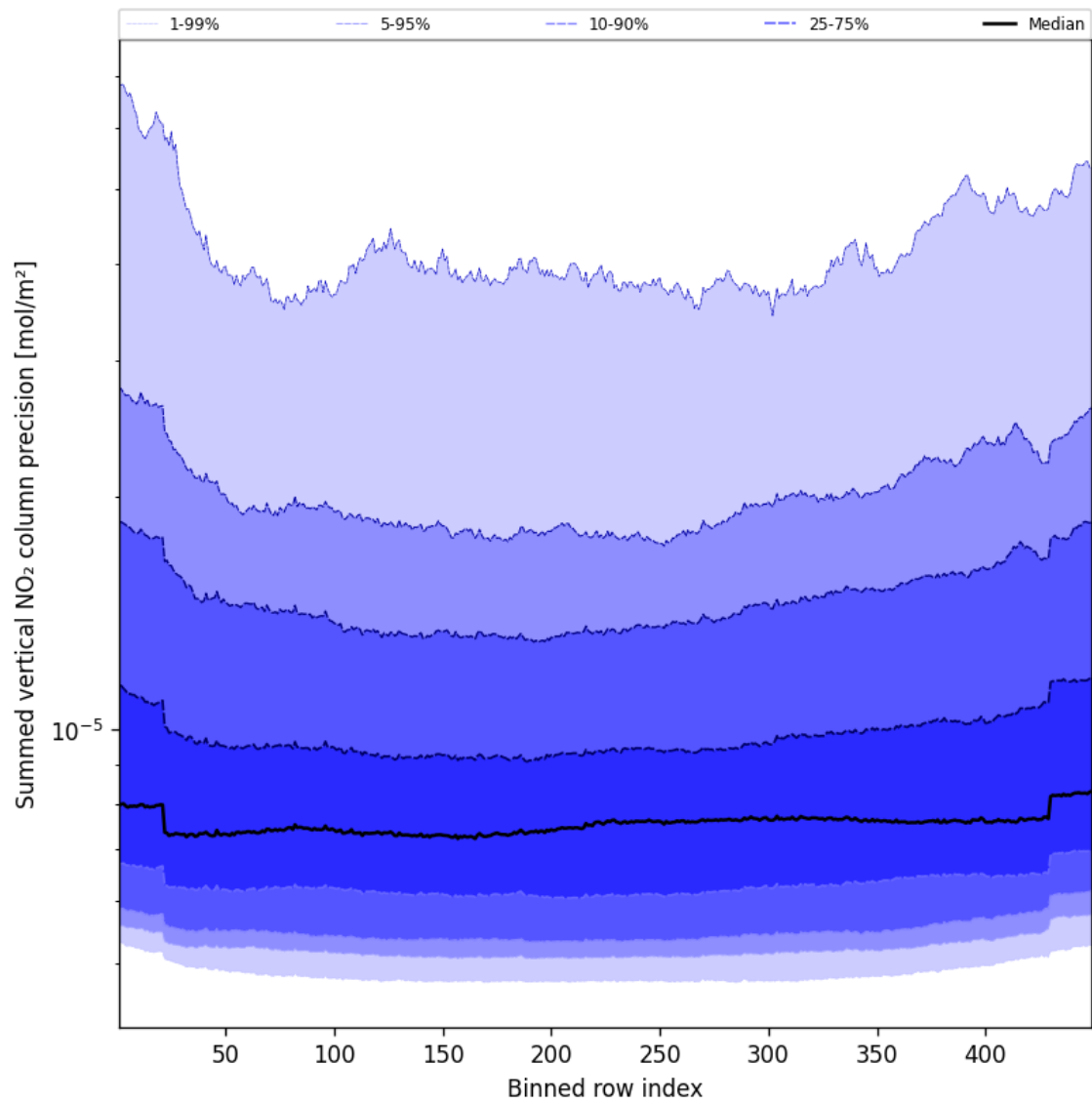
Figure 56: Along track statistics of “Summed vertical NO 2 column precision” for 2025-03-30 to 2025-03-31
