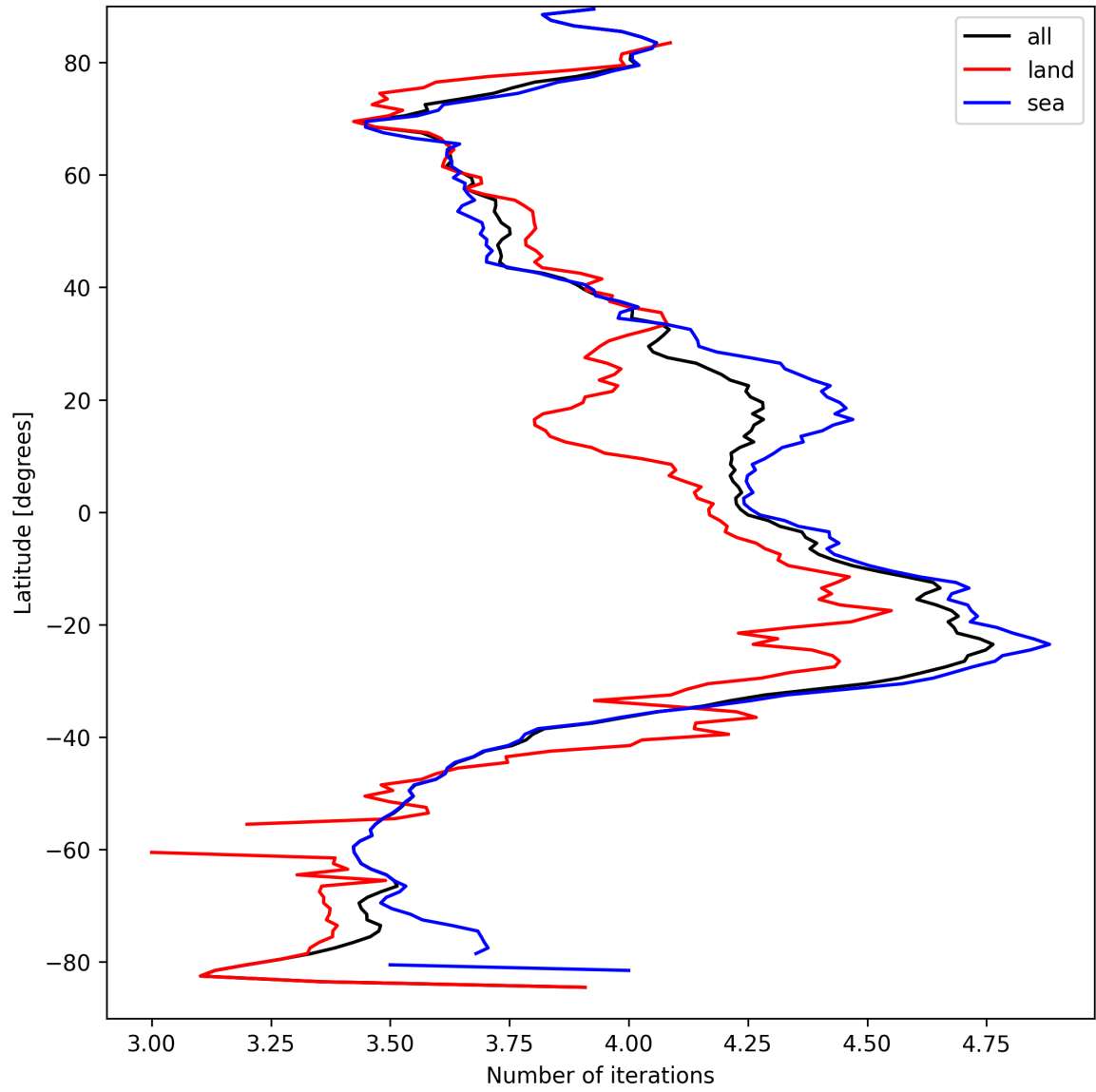
Figure 15: Zonal average of “Number of iterations” for 2025-03-30 to 2025-03-31.
