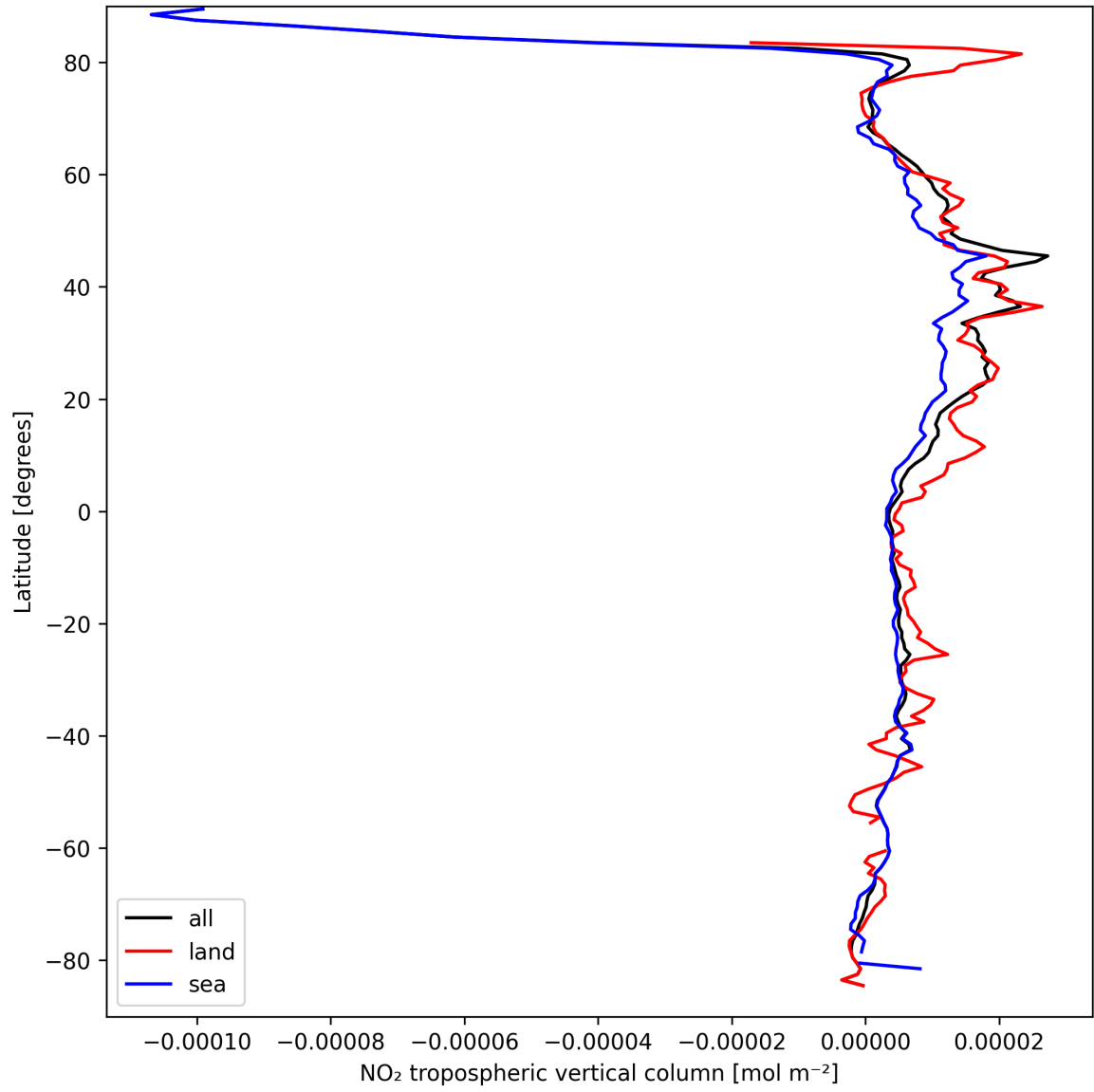
Figure 10: Zonal average of “NO 2 tropospheric vertical column” for 2025-03-30 to 2025-03-31.
