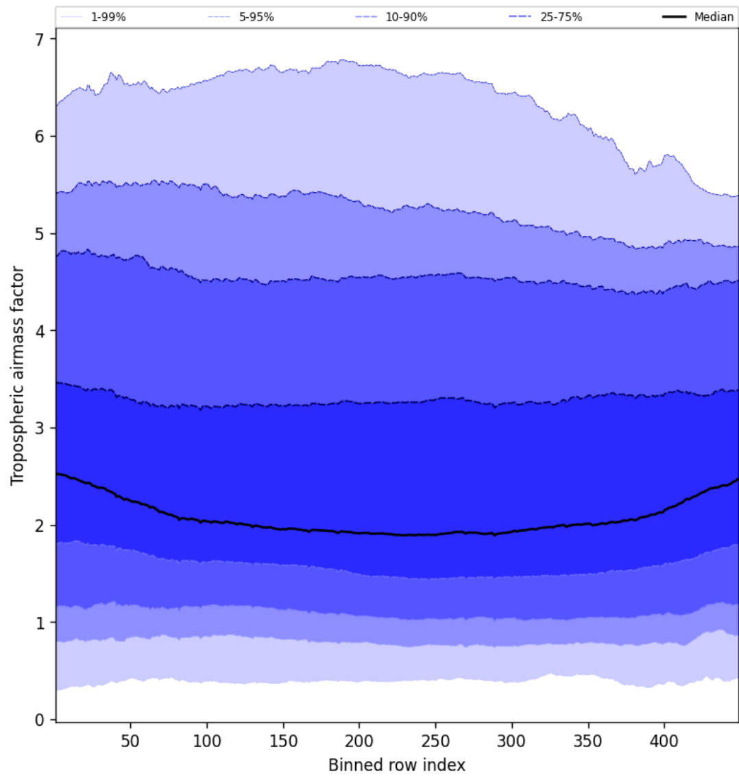
Figure 46: Along track statistics of “Tropospheric airmass factor” for 2025-03-30 to 2025-03-31
