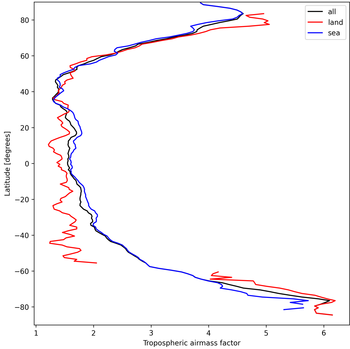
Figure 12: Zonal average of “Tropospheric airmass factor” for 2025-03-30 to 2025-03-31.
