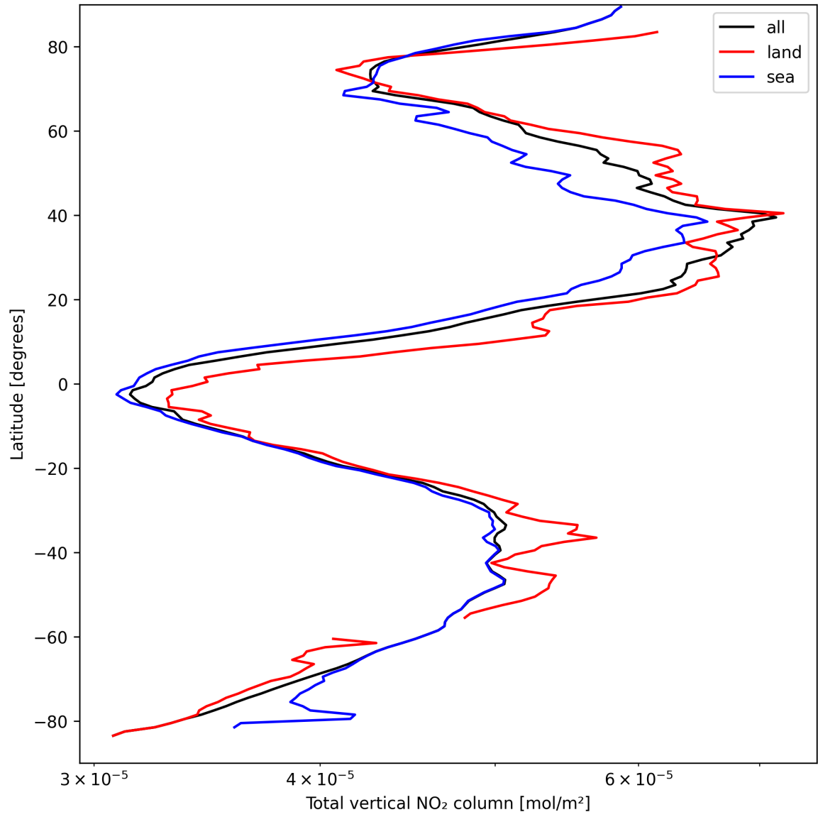
Figure 19: Zonal average of “Total vertical NO 2 column” for 2025-03-31 to 2025-03-31.
