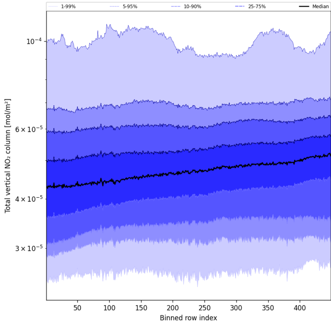
Figure 53: Along track statistics of “Total vertical NO 2 column” for 2025-03-31 to 2025-03-31
