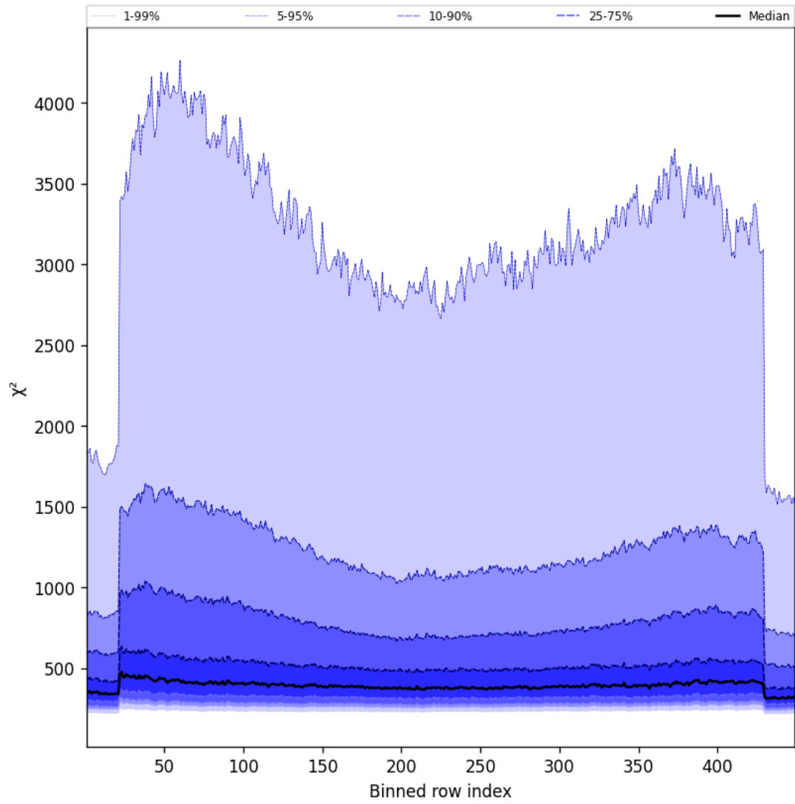
Figure 57: Along track statistics of “ \chi^2 ” for 2025-03-31 to 2025-03-31
