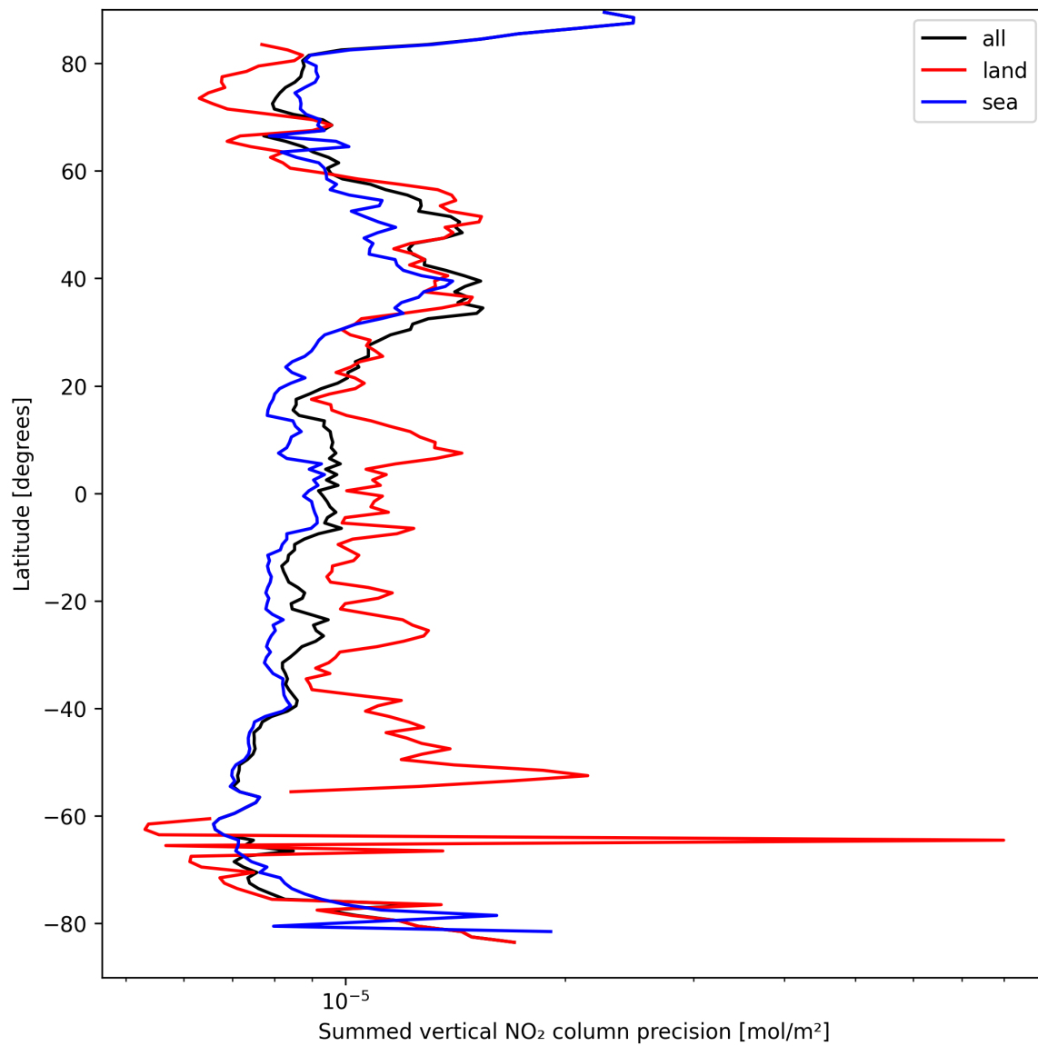
Figure 22: Zonal average of “Summed vertical NO 2 column precision” for 2025-03-31 to 2025-03-31.
