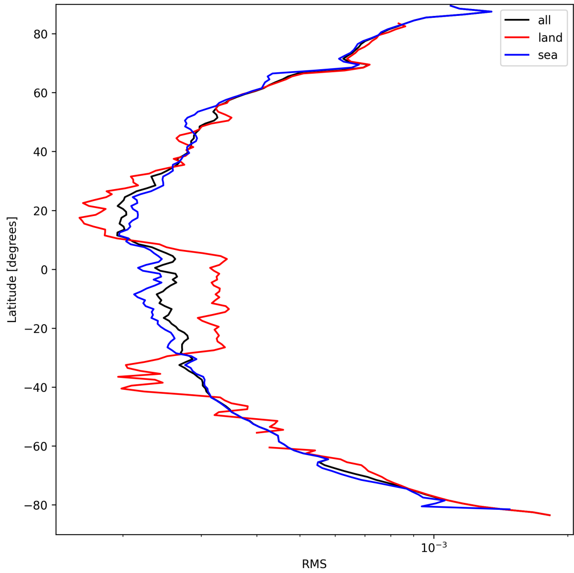
Figure 24: Zonal average of “RMS” for 2025-03-31 to 2025-03-31.
