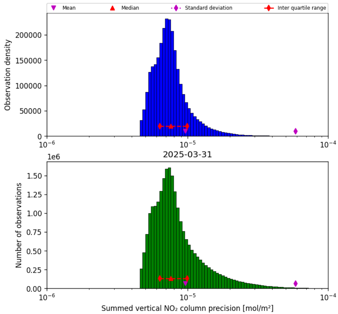
Figure 39: Histogram of "Summed vertical NO 2 column precision" for 2025-03-31 to 2025-03-31
