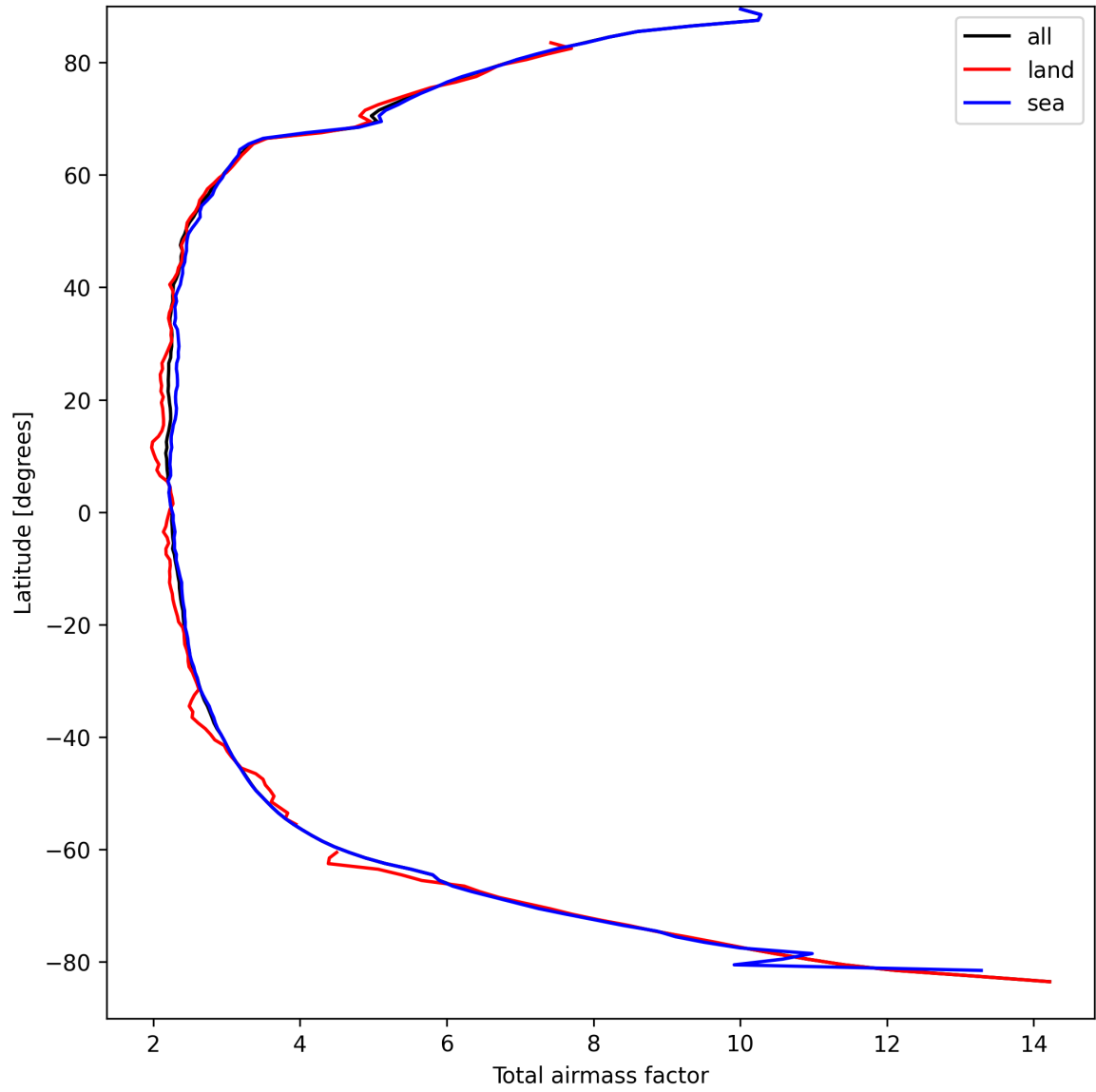
Figure 13: Zonal average of “Total airmass factor” for 2025-03-31 to 2025-03-31.
