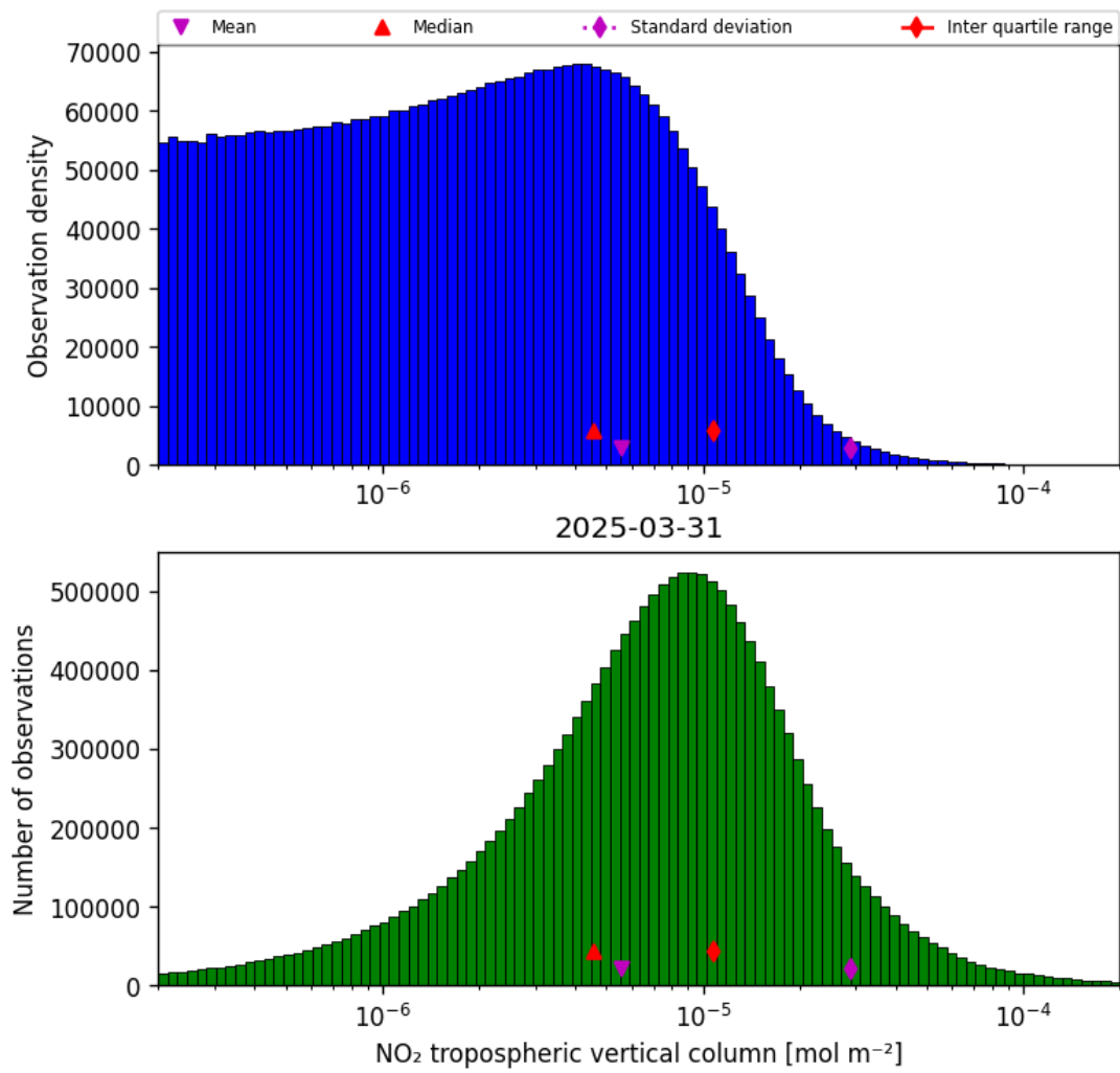
Figure 27: Histogram of "NO 2 tropospheric vertical column" for 2025-03-31 to 2025-03-31
