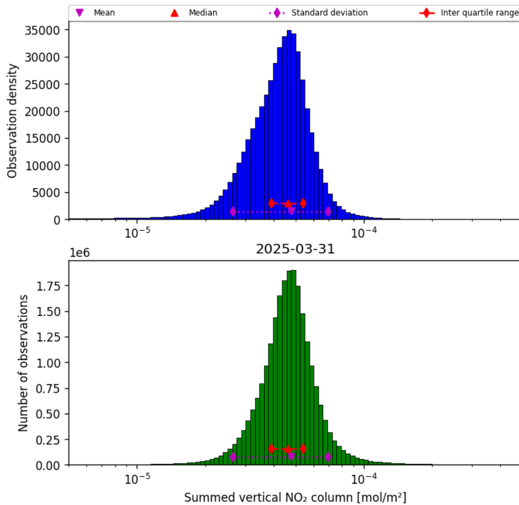
Figure 38: Histogram of “Summed vertical NO 2 column” for 2025-03-31 to 2025-03-31
