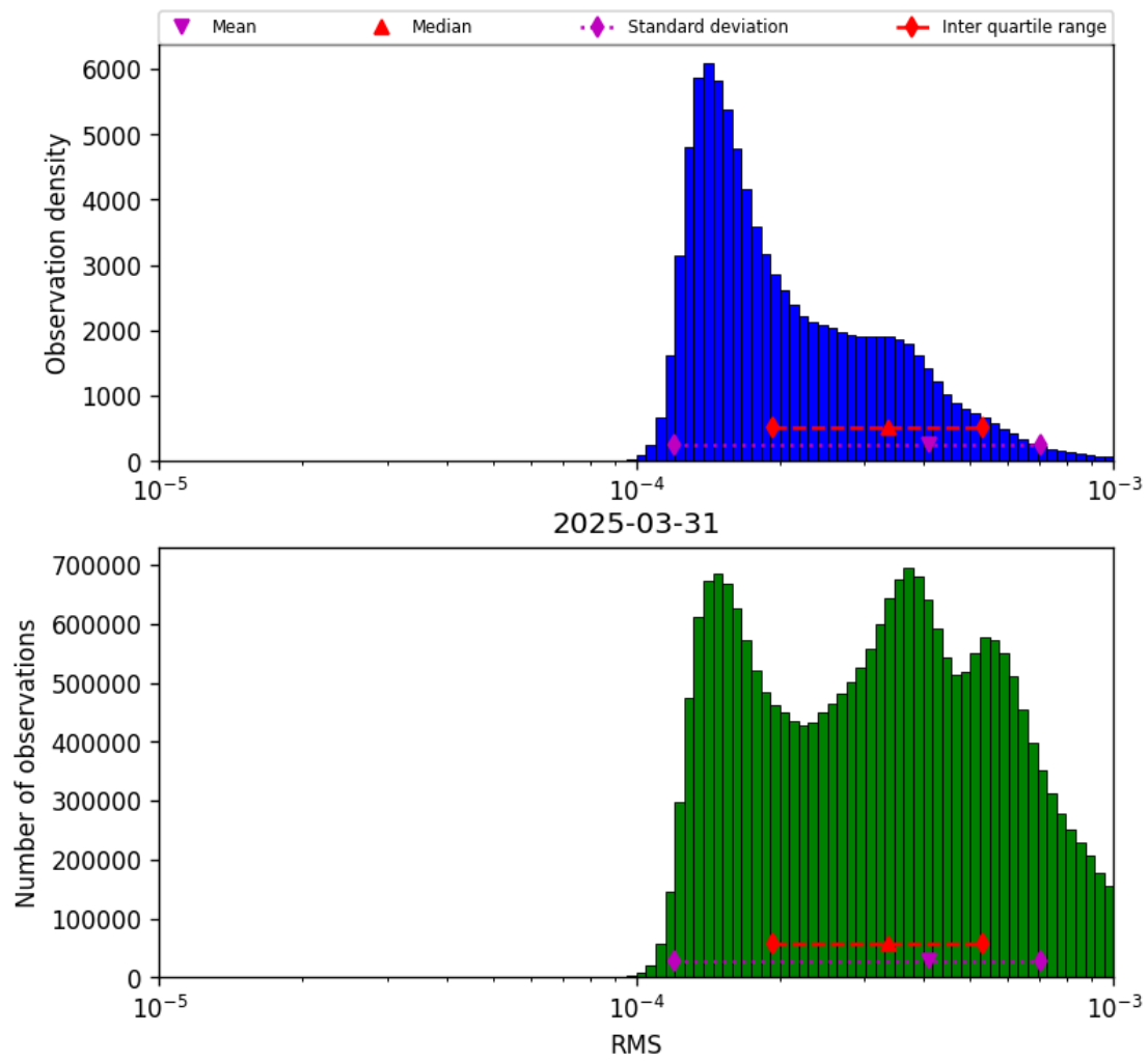
Figure 41: Histogram of “RMS” for 2025-03-31 to 2025-03-31
