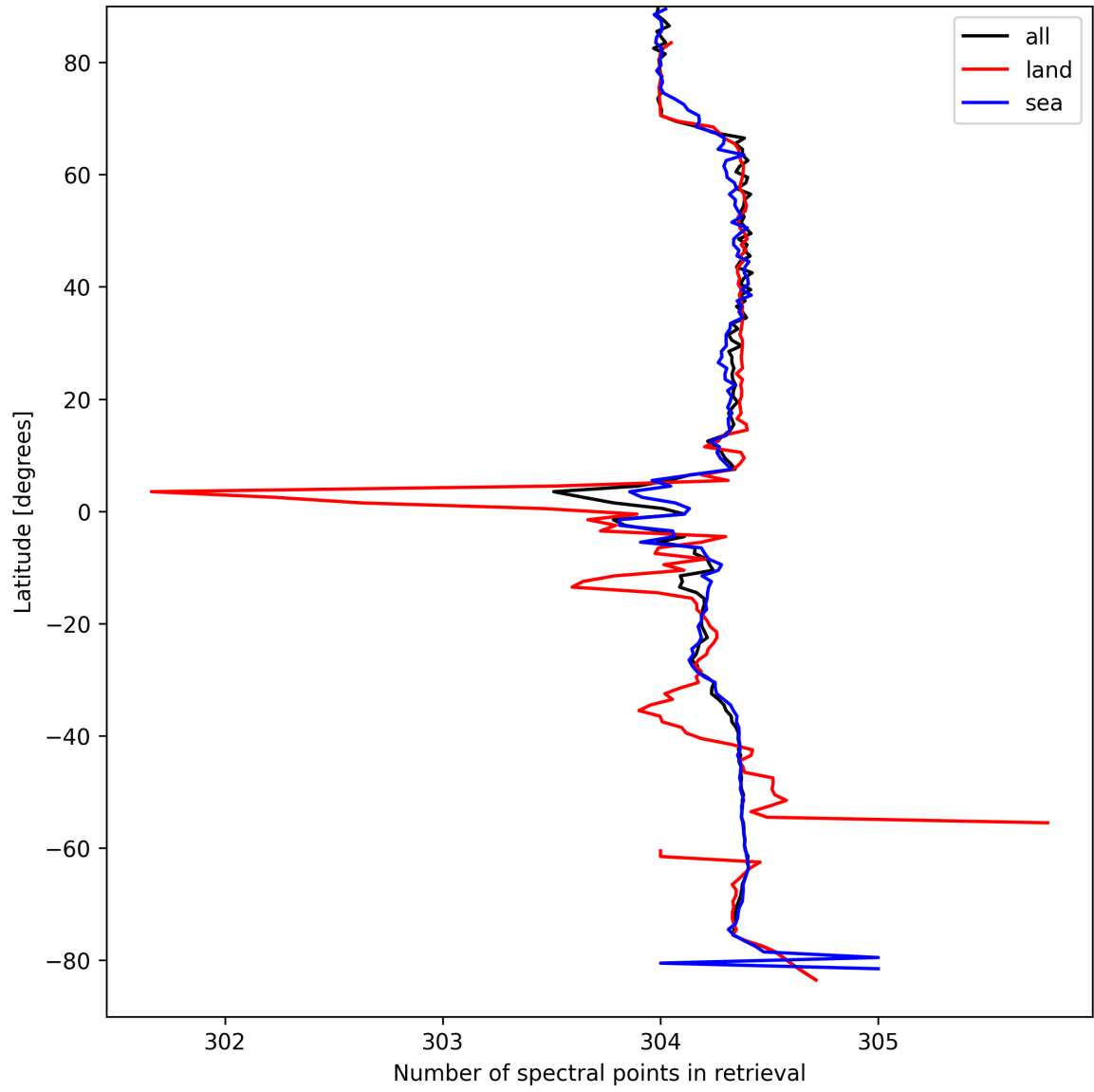
Figure 14: Zonal average of “Number of spectral points in retrieval” for 2025-03-31 to 2025-03-31.
