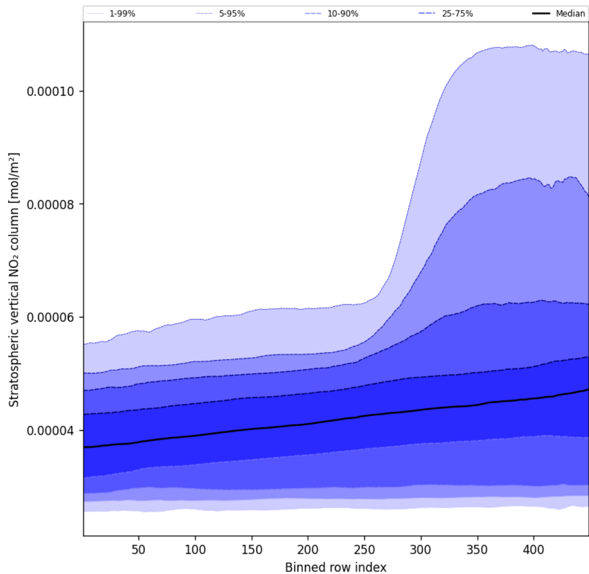
Figure 51: Along track statistics of “Stratospheric vertical NO 2 column” for 2025-03-31 to 2025-03-31
