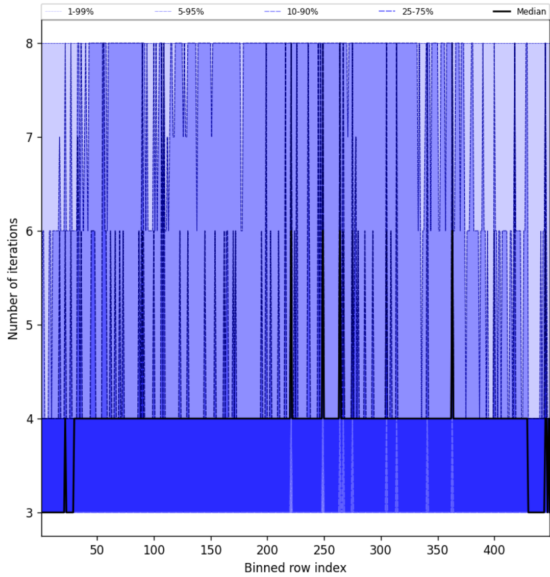
Figure 49: Along track statistics of “Number of iterations” for 2025-03-31 to 2025-03-31
