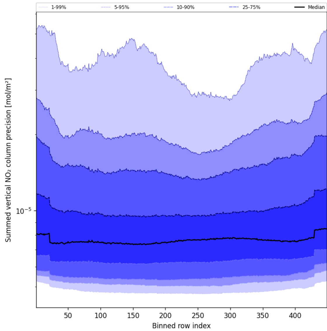
Figure 56: Along track statistics of “Summed vertical NO 2 column precision” for 2025-03-31 to 2025-03-31
