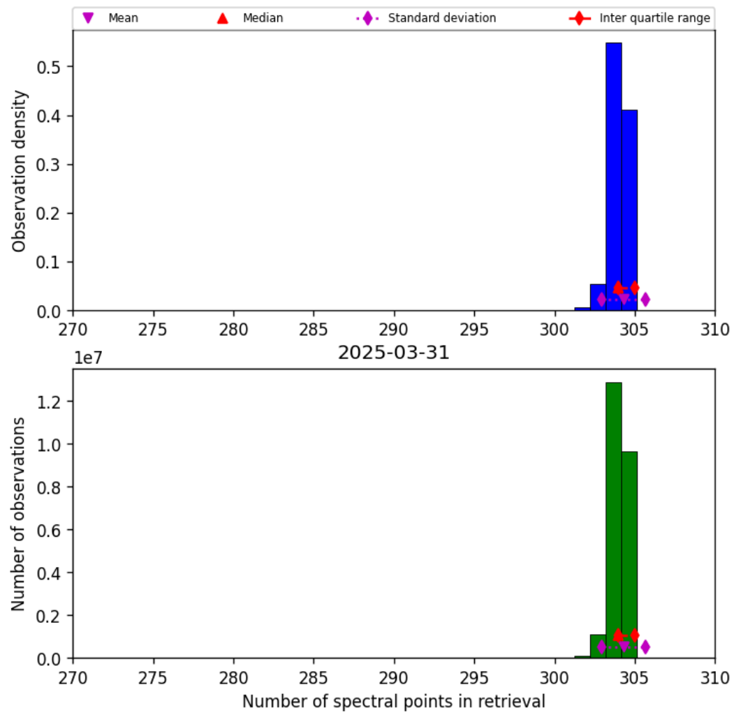
Figure 31: Histogram of “Number of spectral points in retrieval” for 2025-03-31 to 2025-03-31
