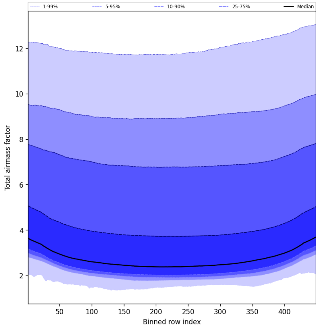
Figure 47: Along track statistics of “Total airmass factor” for 2025-03-31 to 2025-03-31
