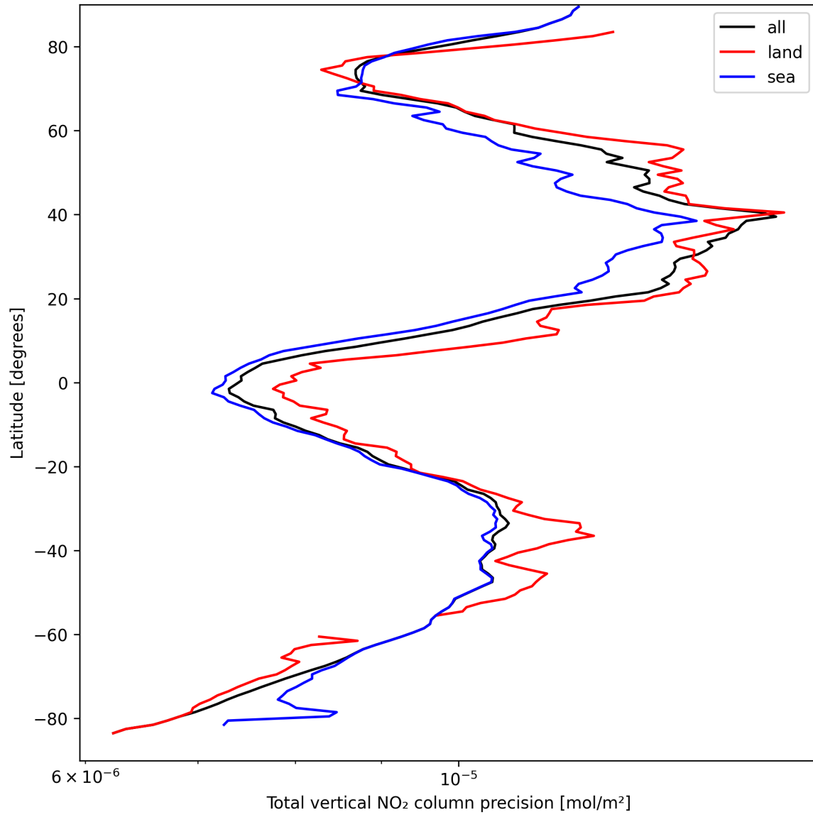
Figure 20: Zonal average of “Total vertical NO 2 column precision” for 2025-03-31 to 2025-03-31.
