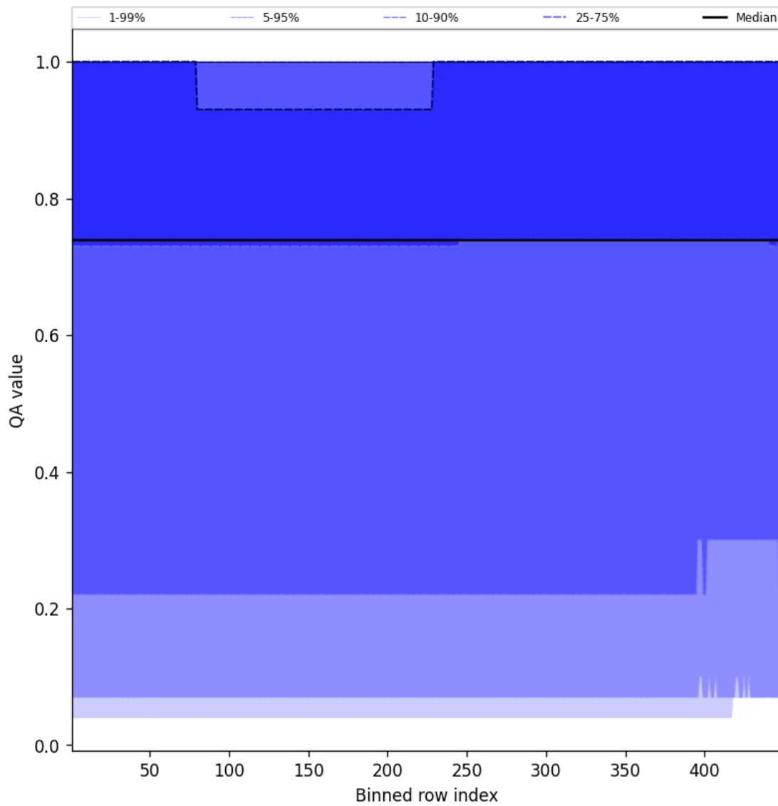
Figure 43: Along track statistics of “QA value” for 2025-03-31 to 2025-03-31
