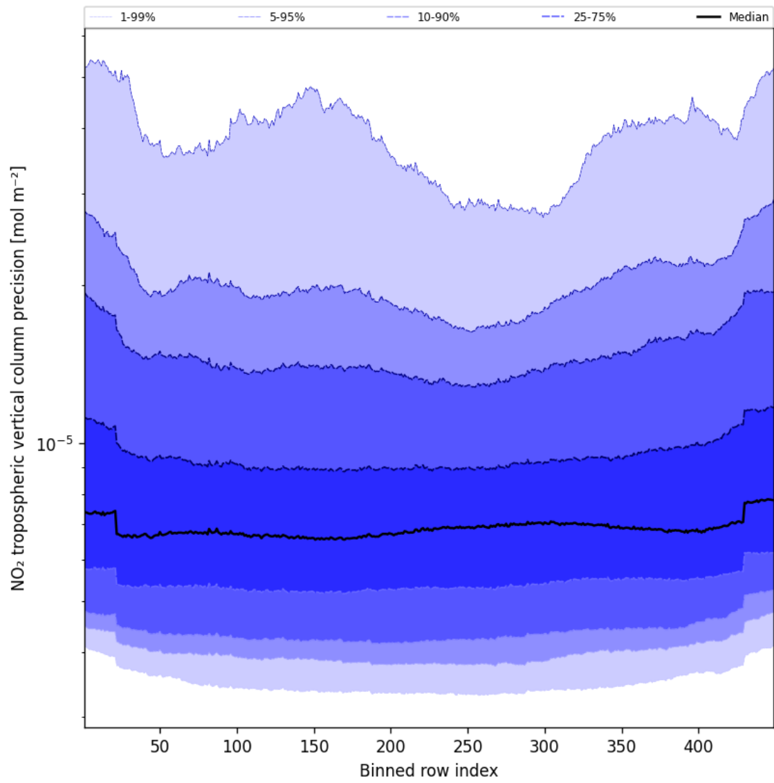
Figure 45: Along track statistics of “NO 2 tropospheric vertical column precision” for 2025-03-31 to 2025-03-31
