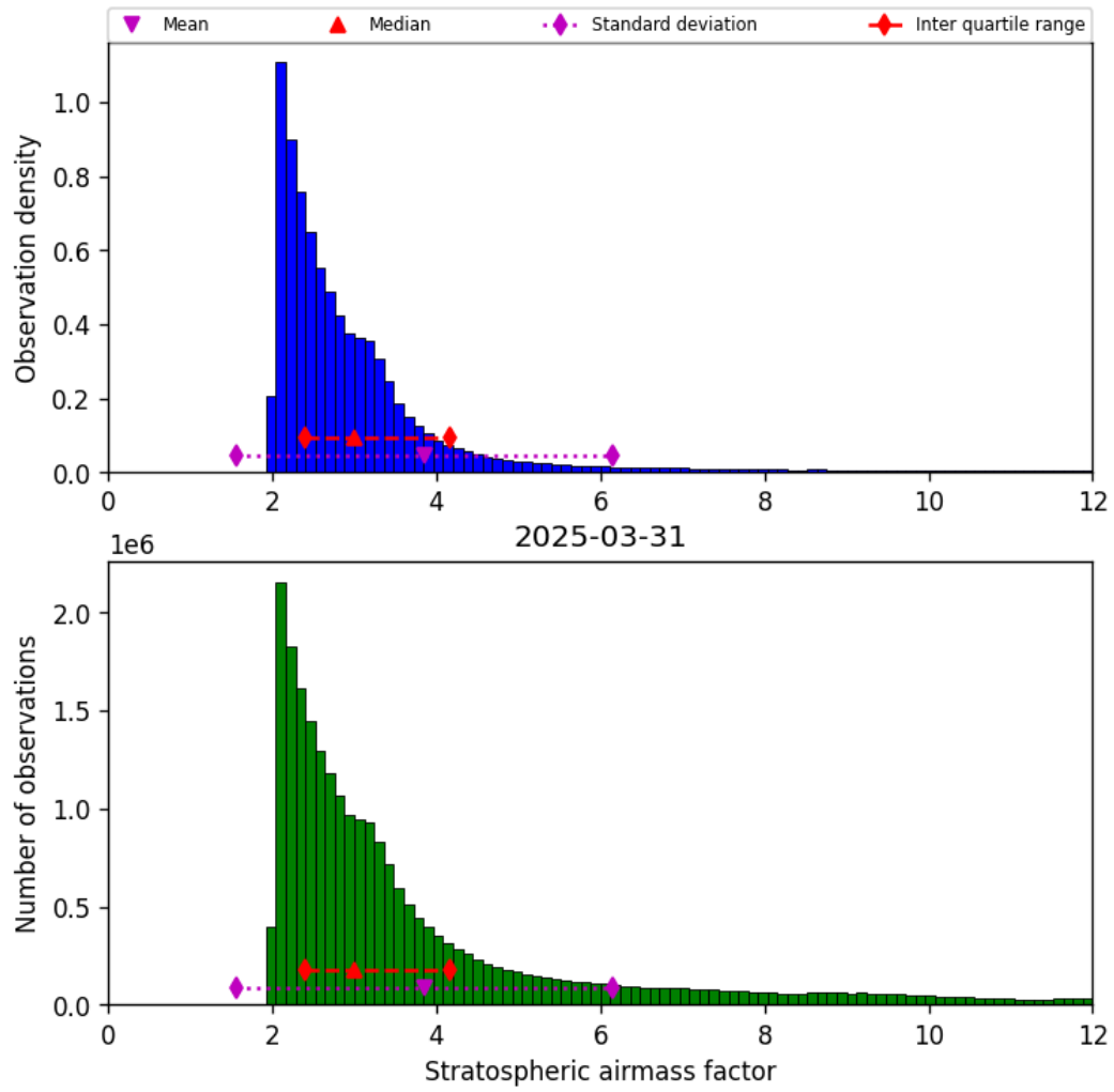
Figure 42: Histogram of “Stratospheric airmass factor” for 2025-03-31 to 2025-03-31
