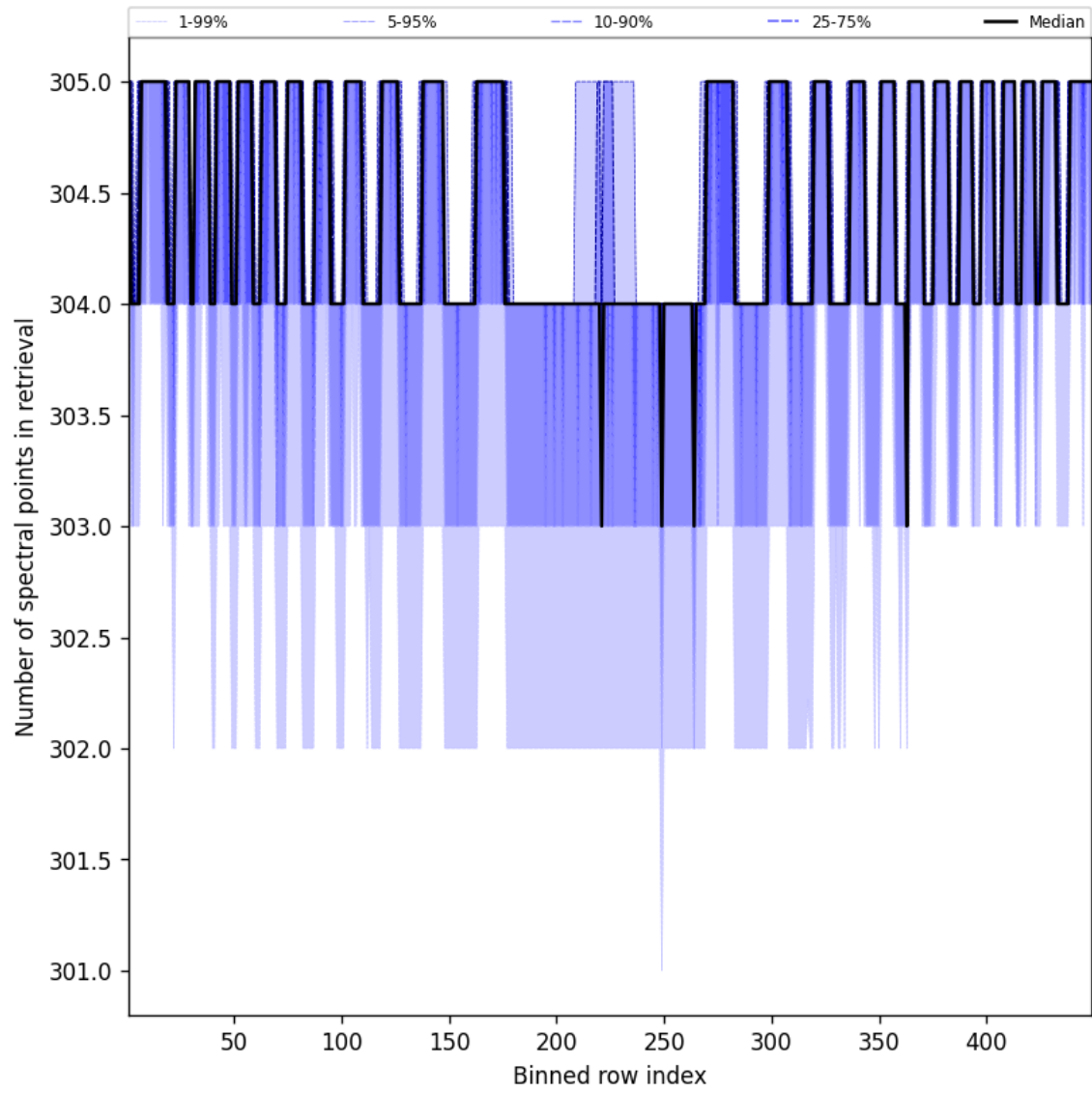
Figure 48: Along track statistics of “Number of spectral points in retrieval” for 2025-03-31 to 2025-03-31
