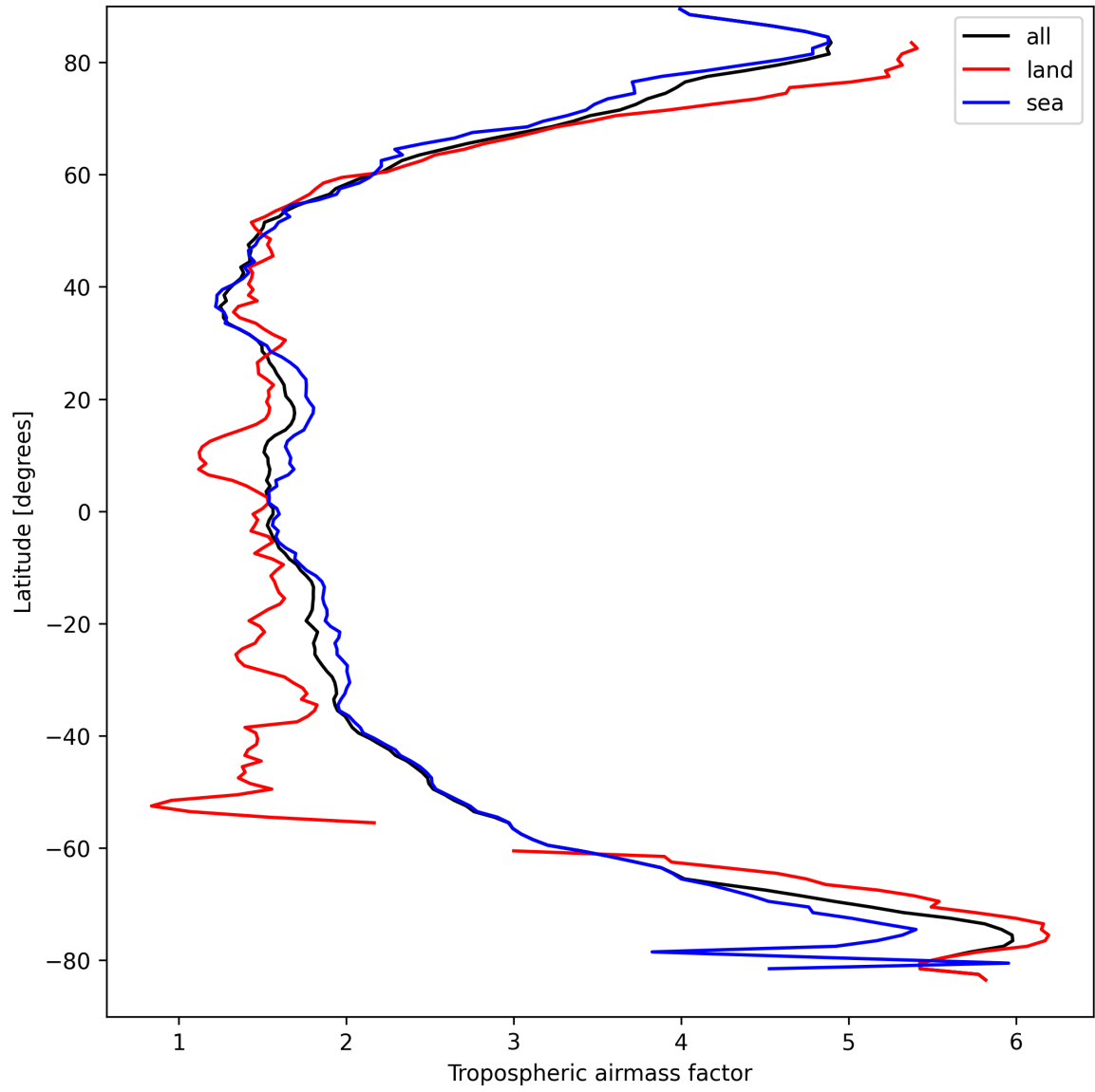
Figure 12: Zonal average of “Tropospheric airmass factor” for 2025-03-31 to 2025-03-31.
