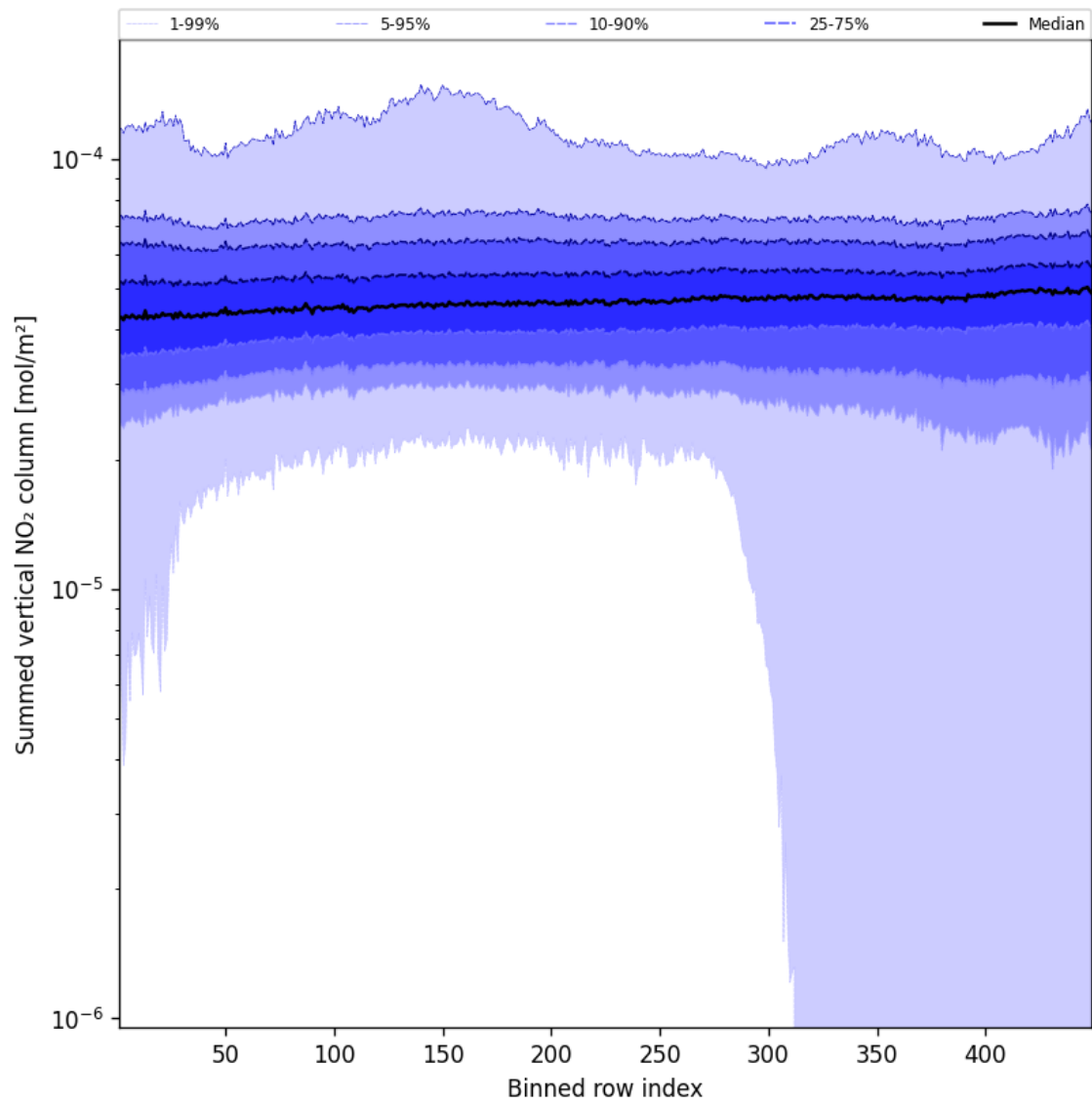
Figure 55: Along track statistics of “Summed vertical NO 2 column” for 2025-03-31 to 2025-03-31
