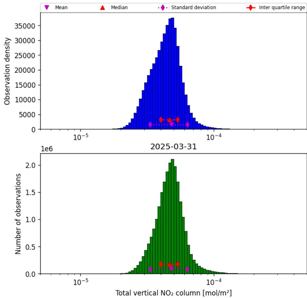
Figure 36: Histogram of “Total vertical NO 2 column” for 2025-03-31 to 2025-03-31
