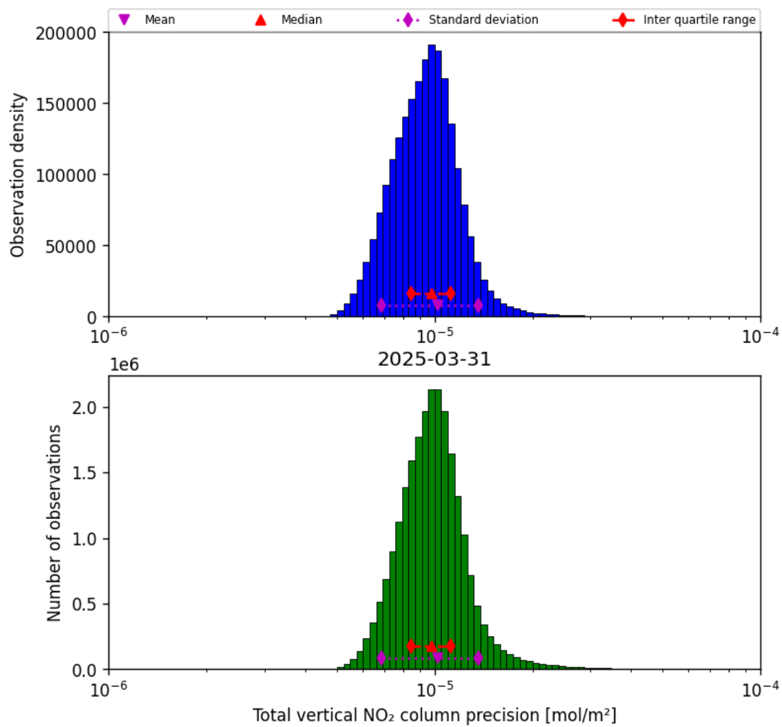
Figure 37: Histogram of "Total vertical NO 2 column precision" for 2025-03-31 to 2025-03-31
