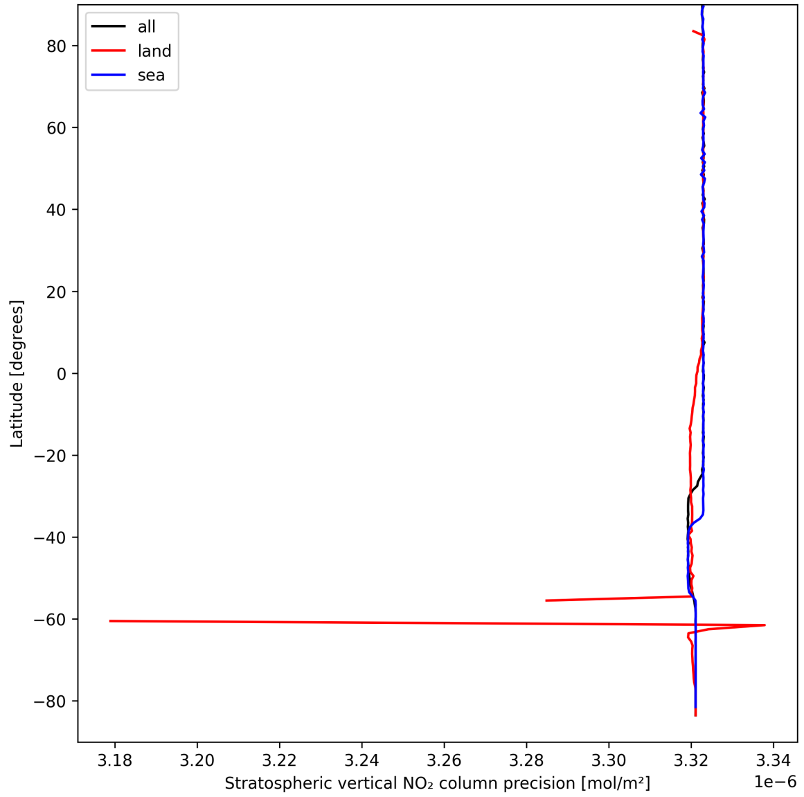
Figure 18: Zonal average of “Stratospheric vertical NO 2 column precision” for 2025-03-31 to 2025-03-31.
