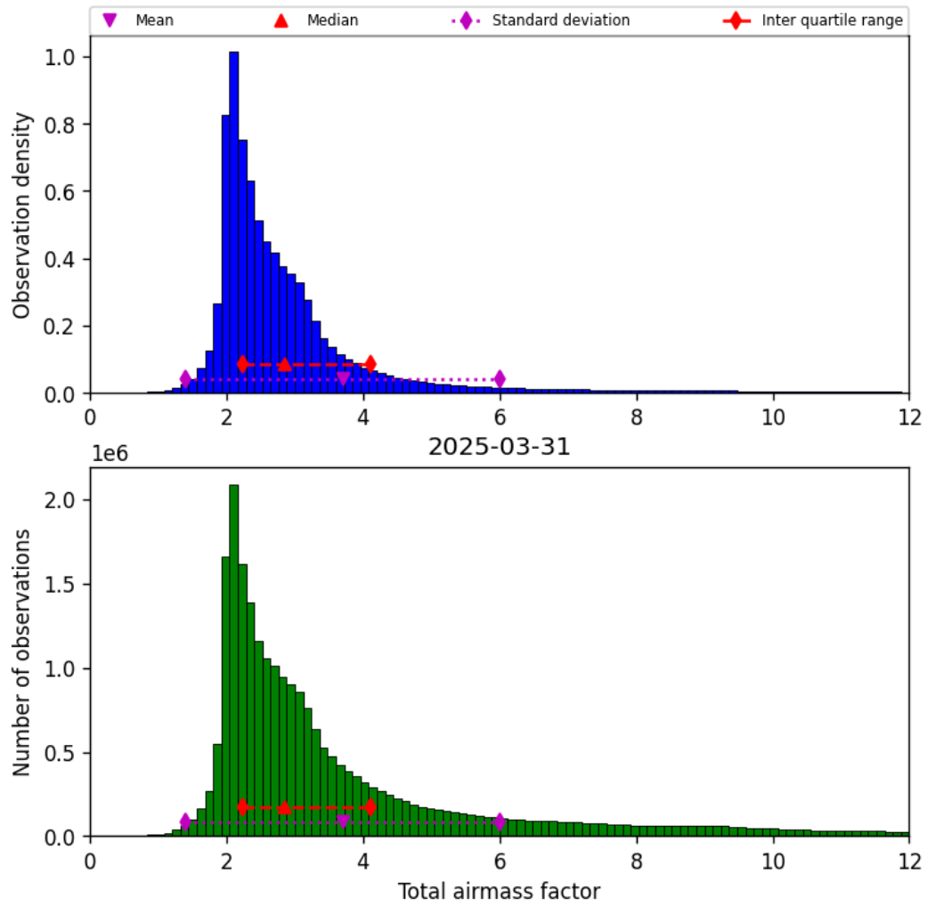
Figure 30: Histogram of “Total airmass factor” for 2025-03-31 to 2025-03-31
