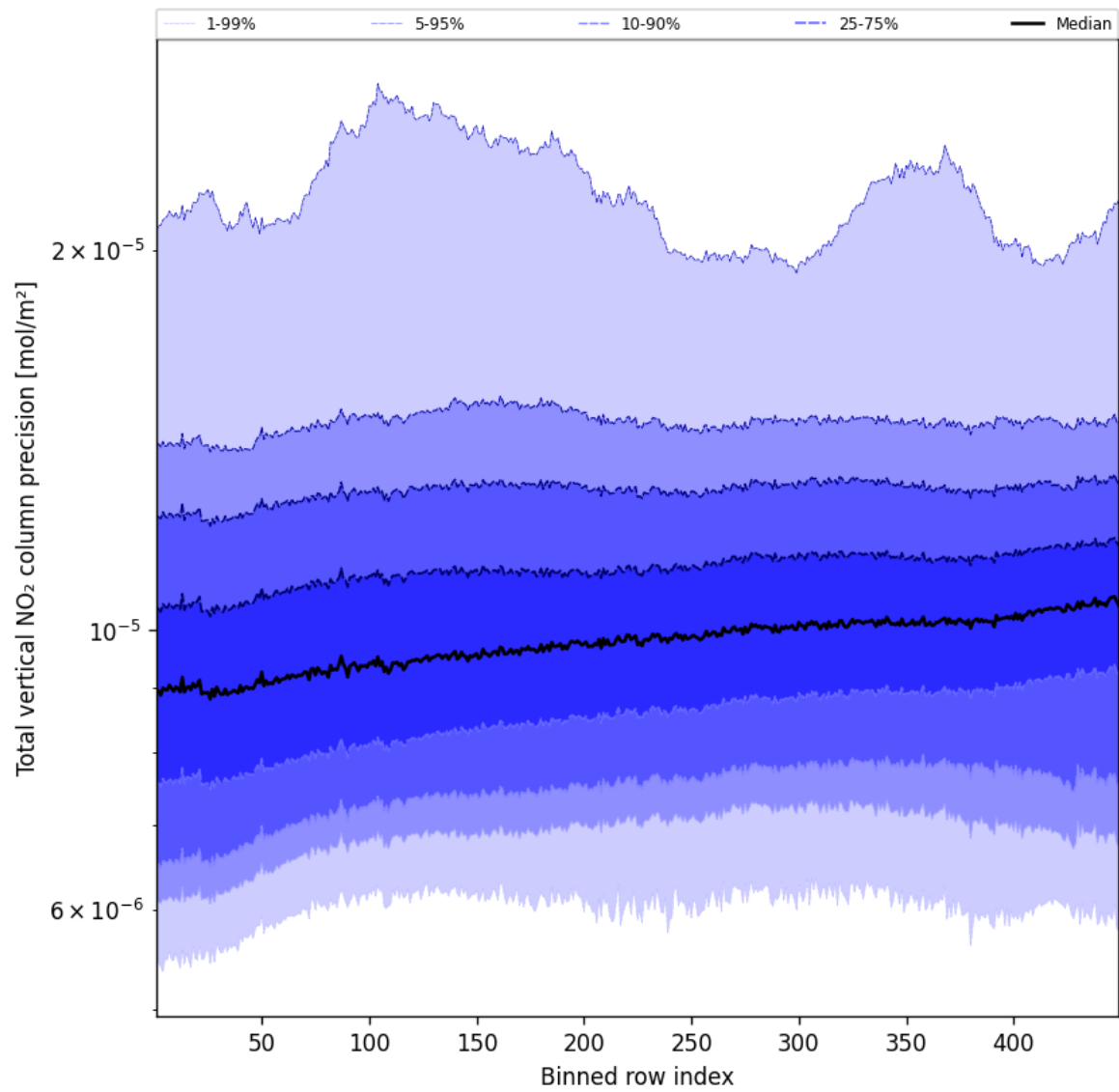
Figure 54: Along track statistics of “Total vertical NO 2 column precision” for 2025-03-31 to 2025-03-31
