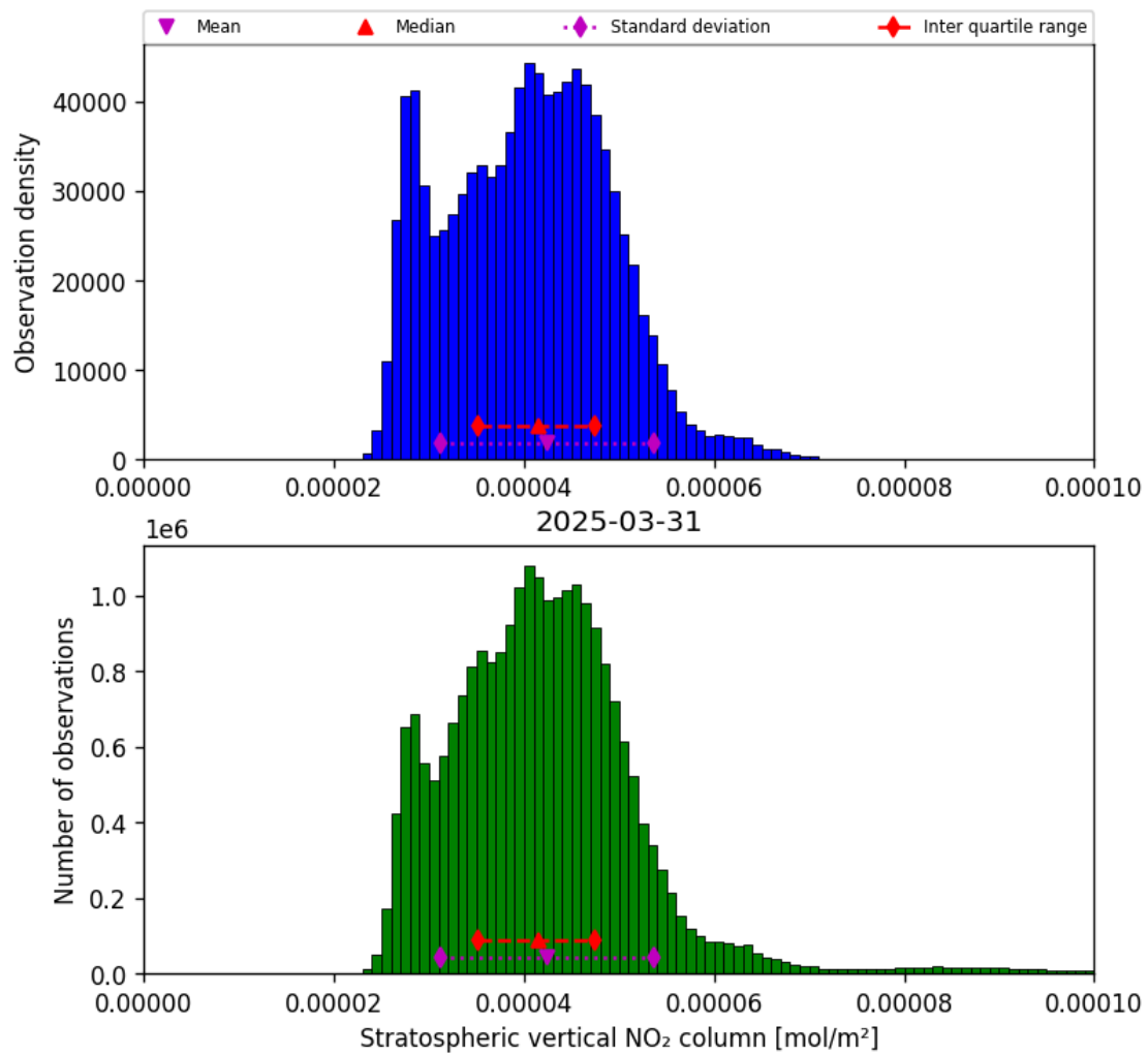
Figure 34: Histogram of “Stratospheric vertical NO 2 column” for 2025-03-31 to 2025-03-31
