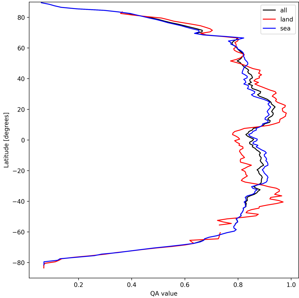
Figure 9: Zonal average of “QA value” for 2025-03-31 to 2025-03-31.
