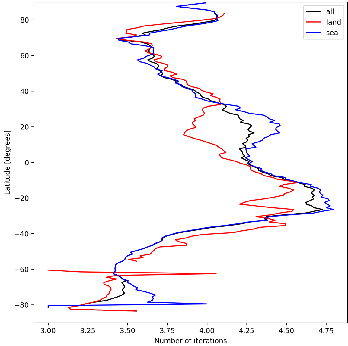
Figure 15: Zonal average of “Number of iterations” for 2025-03-31 to 2025-03-31.
