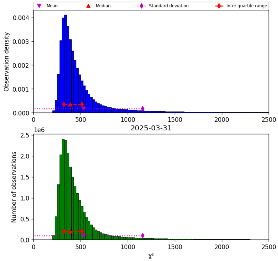
Figure 40: Histogram of “ \chi^2 ” for 2025-03-31 to 2025-03-31
