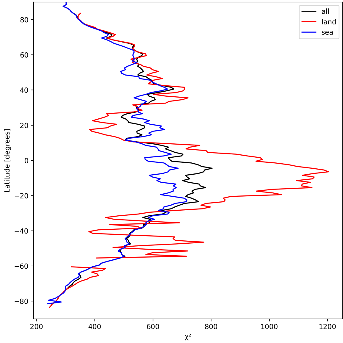
Figure 23: Zonal average of “ \chi^2 ” for 2025-03-31 to 2025-03-31.
