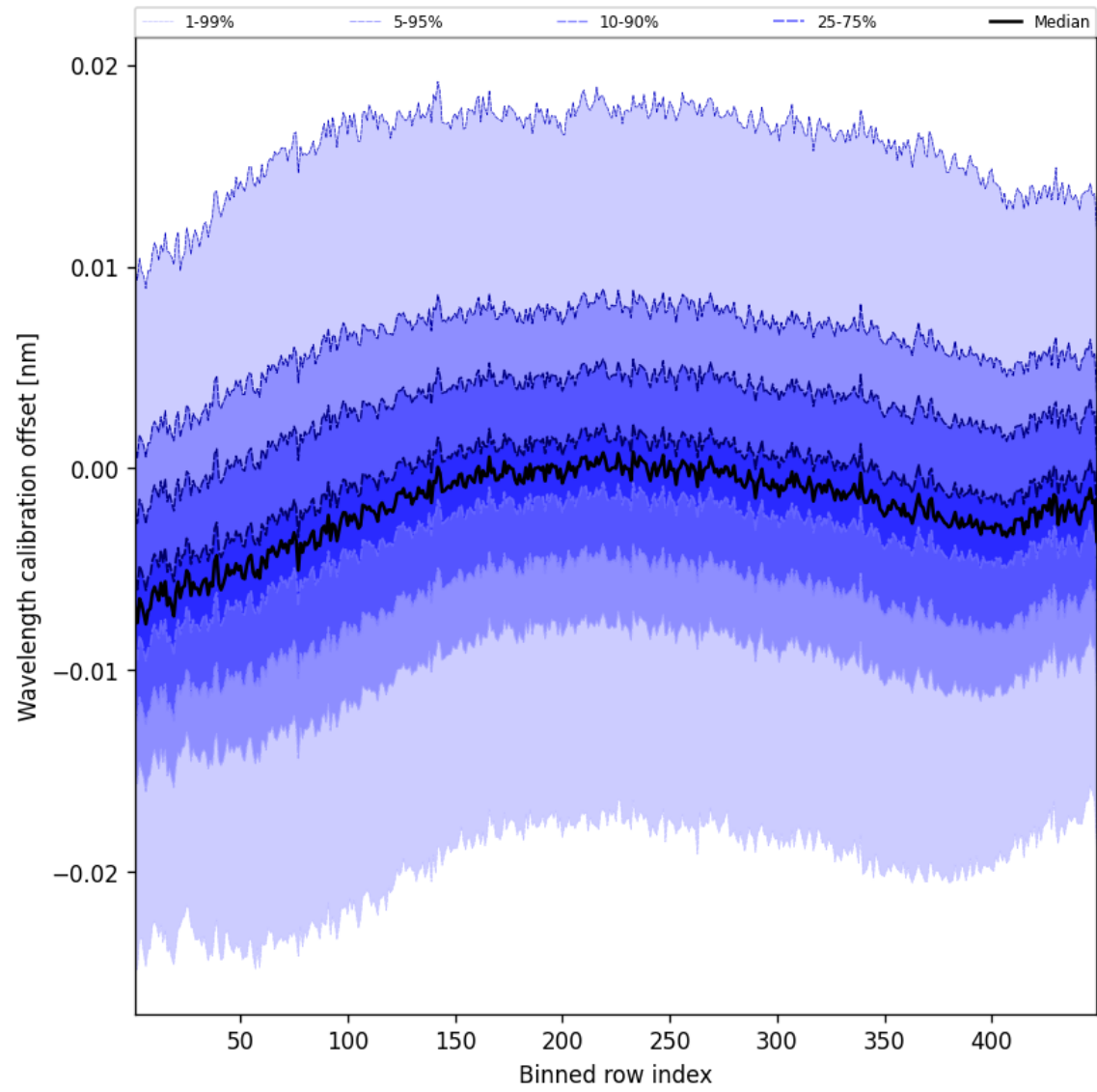
Figure 50: Along track statistics of “Wavelength calibration offset” for 2025-03-31 to 2025-03-31
