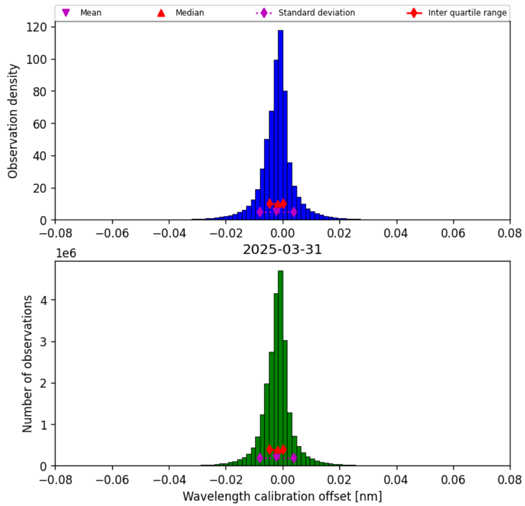
Figure 33: Histogram of “Wavelength calibration offset” for 2025-03-31 to 2025-03-31
