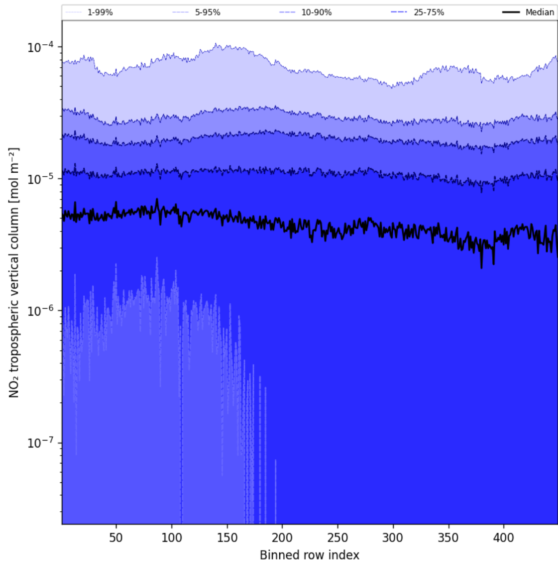
Figure 44: Along track statistics of "NO 2 tropospheric vertical column" for 2025-03-31 to 2025-03-31
