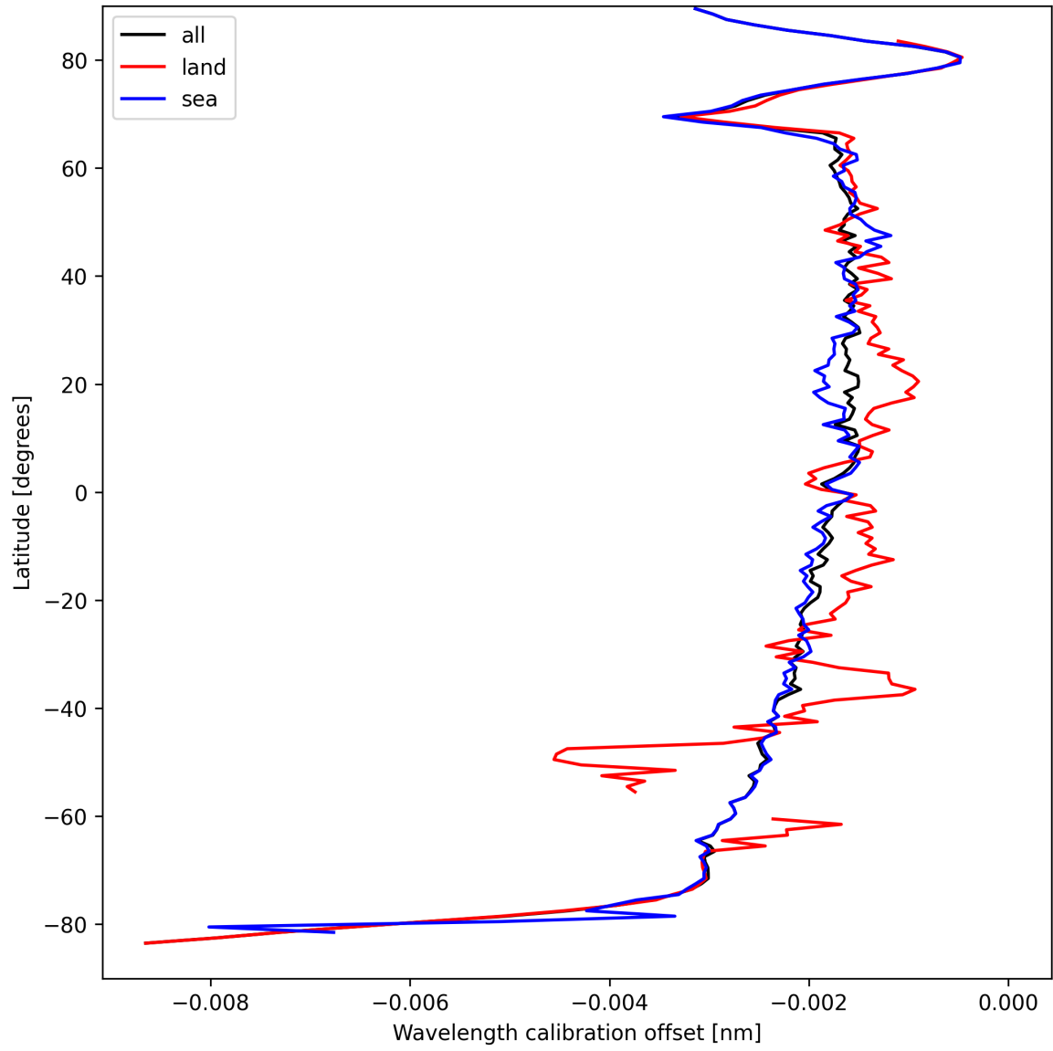
Figure 16: Zonal average of “Wavelength calibration offset” for 2025-03-31 to 2025-03-31.
