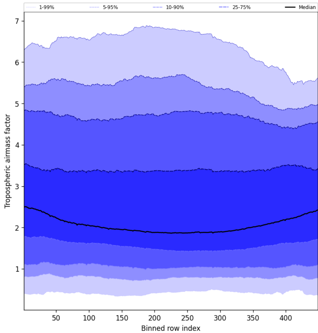
Figure 46: Along track statistics of “Tropospheric airmass factor” for 2025-03-31 to 2025-03-31
