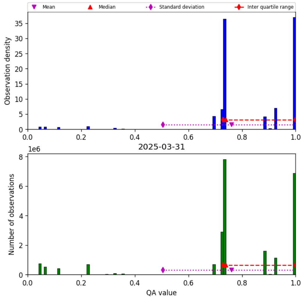
Figure 26: Histogram of “QA value” for 2025-03-31 to 2025-03-31
