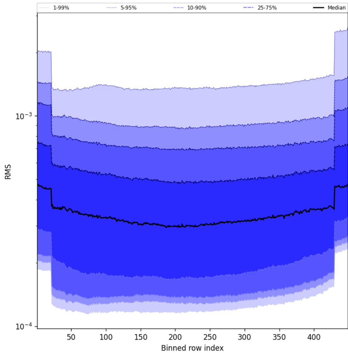
Figure 58: Along track statistics of “RMS” for 2025-03-31 to 2025-03-31
