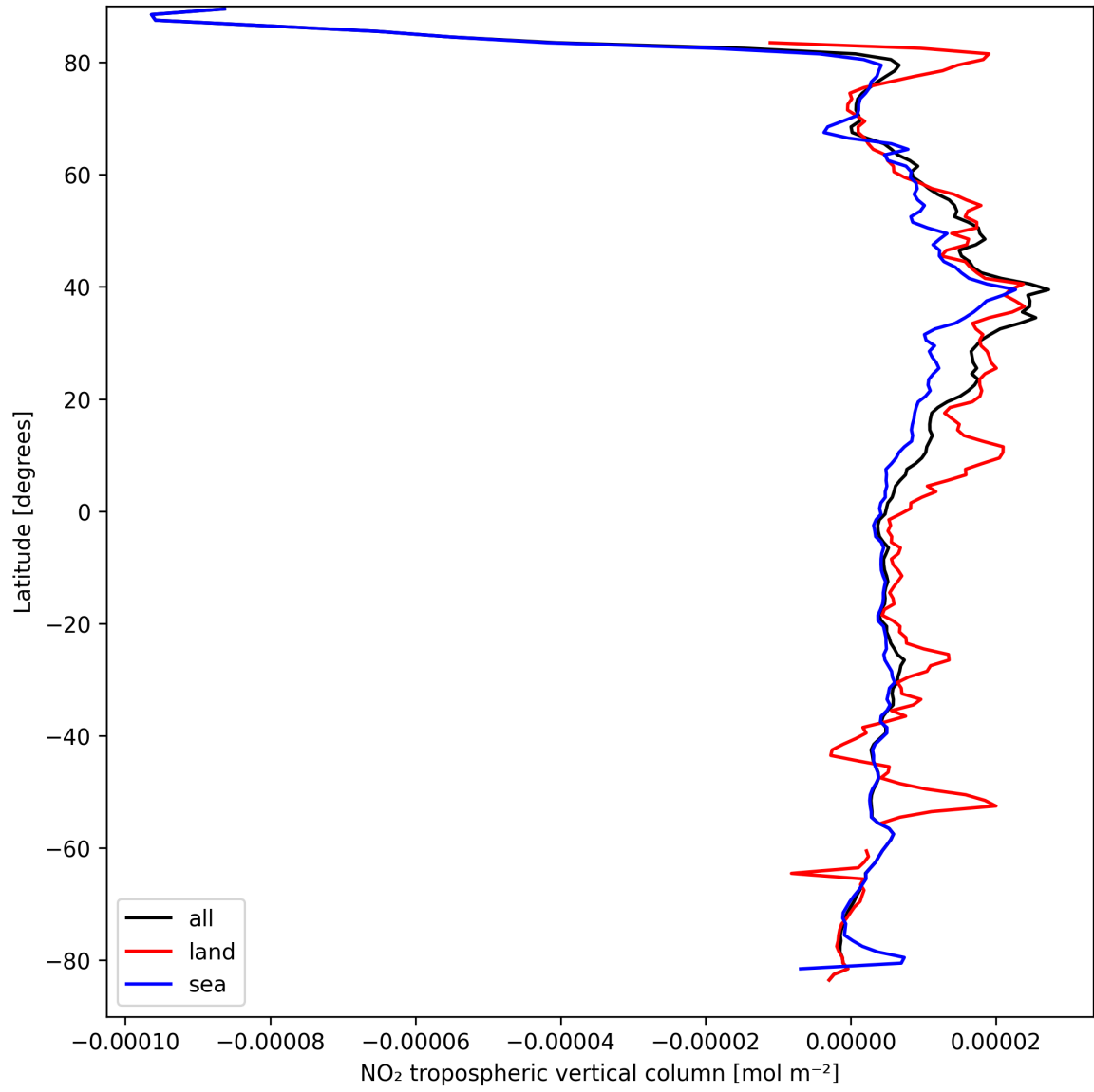
Figure 10: Zonal average of “NO 2 tropospheric vertical column” for 2025-03-31 to 2025-03-31.
