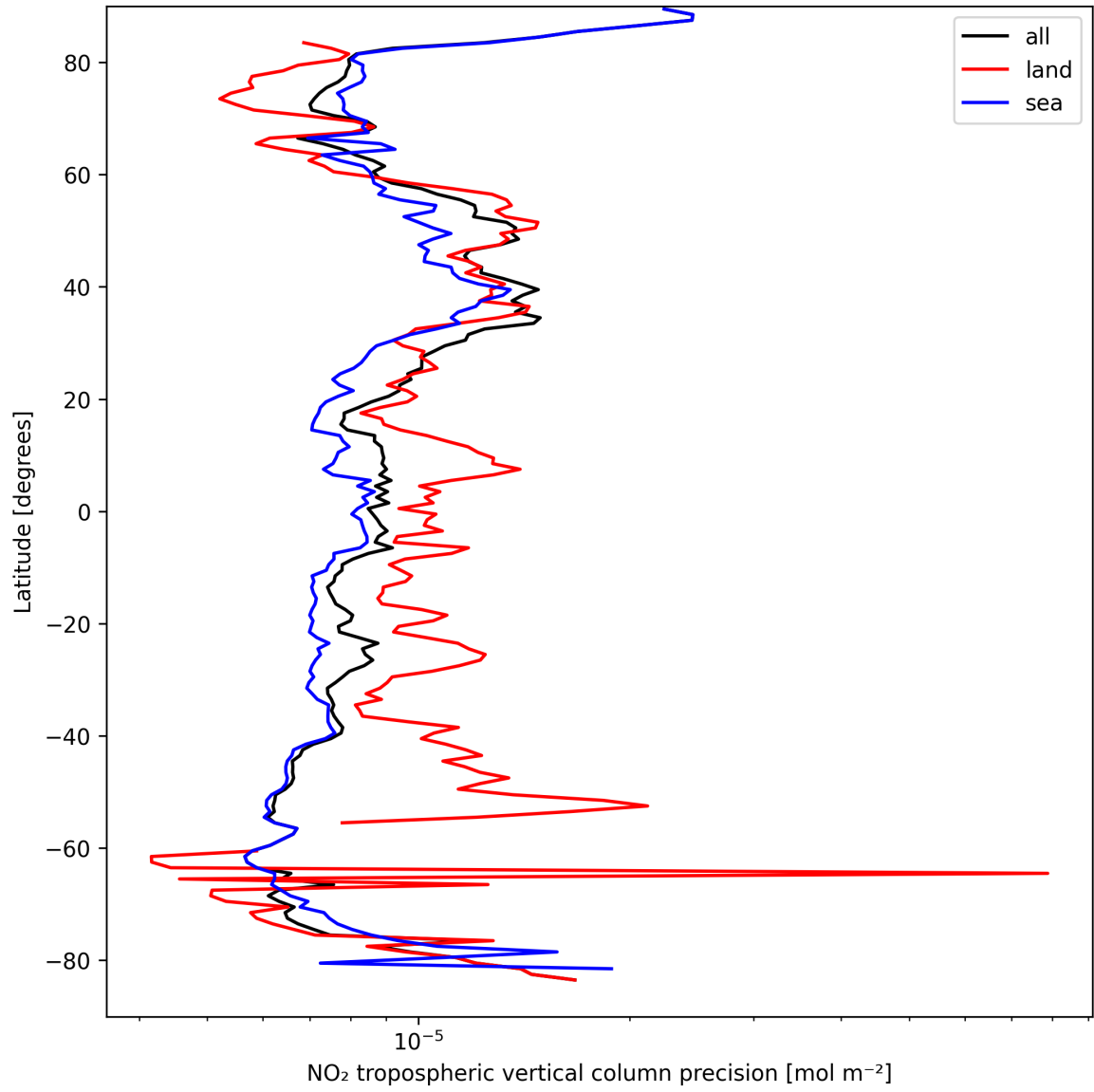
Figure 11: Zonal average of “NO 2 tropospheric vertical column precision” for 2025-03-31 to 2025-03-31.
