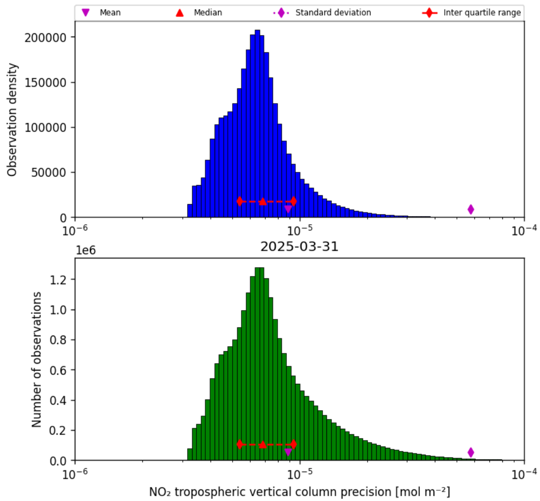
Figure 28: Histogram of "NO 2 tropospheric vertical column precision" for 2025-03-31 to 2025-03-31
