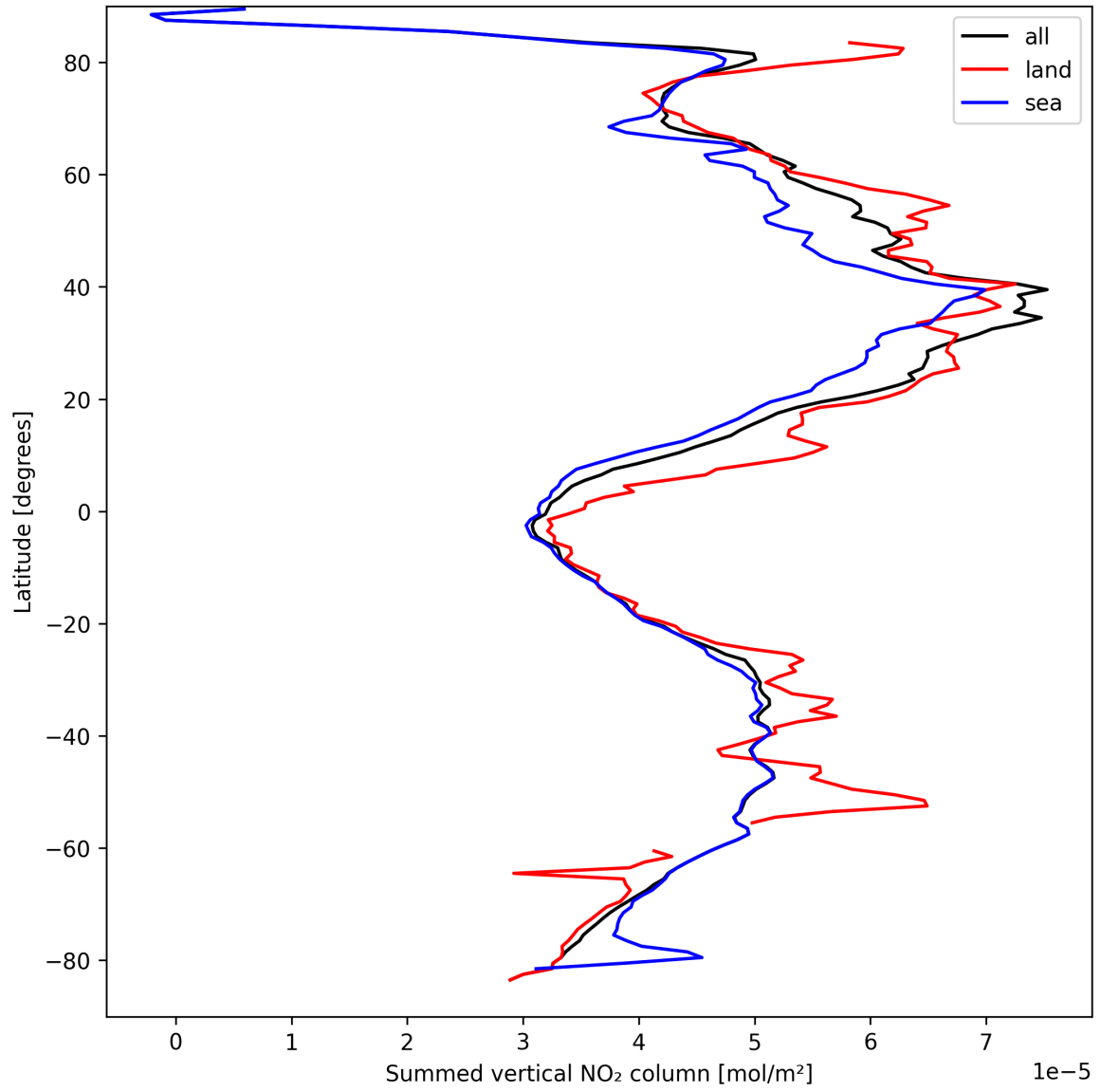
Figure 21: Zonal average of “Summed vertical NO 2 column” for 2025-03-31 to 2025-03-31.
