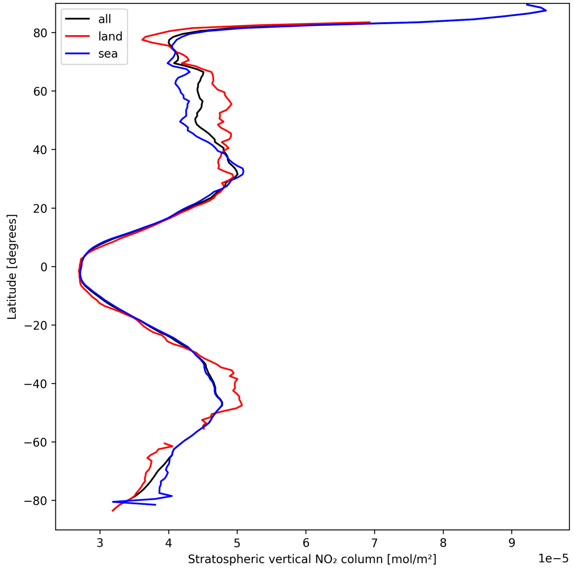
Figure 17: Zonal average of “Stratospheric vertical NO 2 column” for 2025-03-31 to 2025-03-31.
