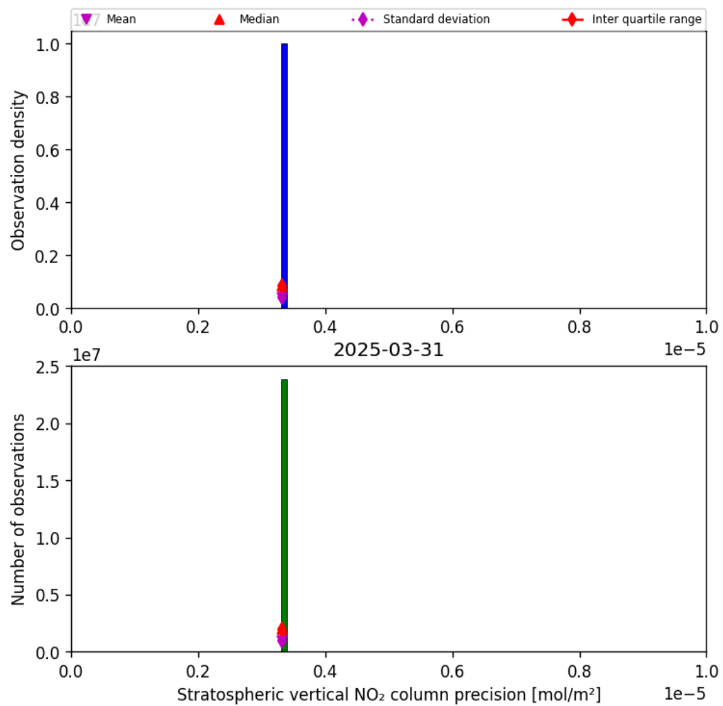
Figure 35: Histogram of “Stratospheric vertical NO 2 column precision” for 2025-03-31 to 2025-03-31
