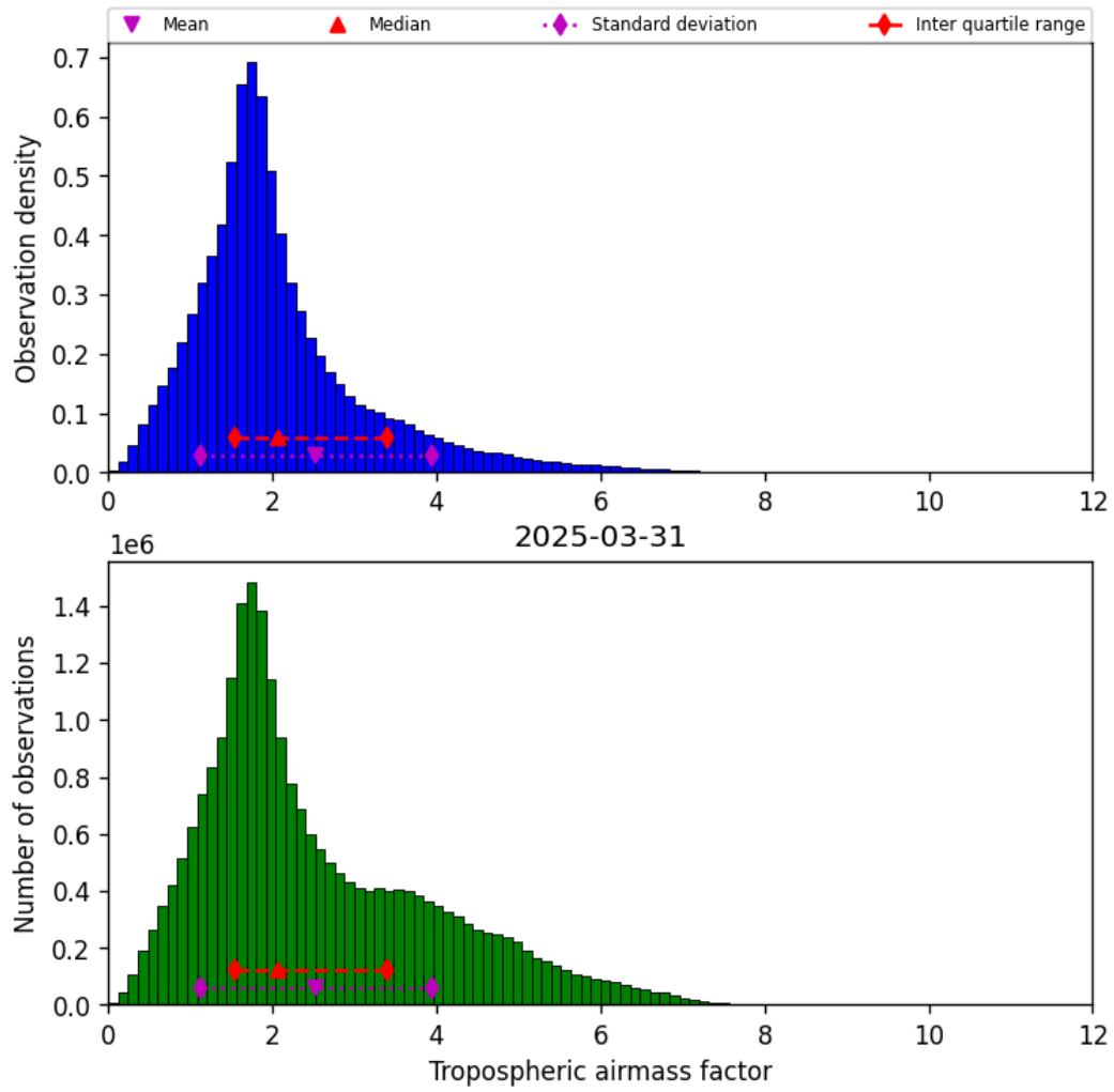
Figure 29: Histogram of “Tropospheric airmass factor” for 2025-03-31 to 2025-03-31
