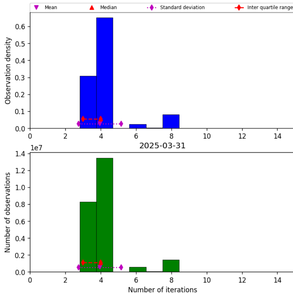
Figure 32: Histogram of “Number of iterations” for 2025-03-31 to 2025-03-31
