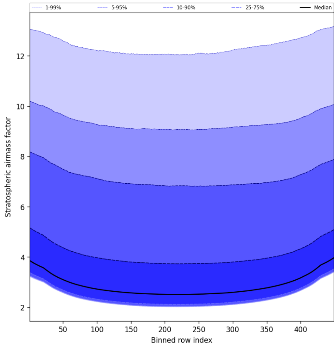
Figure 59: Along track statistics of “Stratospheric airmass factor” for 2025-03-31 to 2025-03-31
