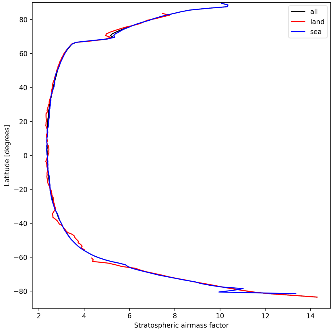
Figure 25: Zonal average of “Stratospheric airmass factor” for 2025-03-31 to 2025-03-31.
