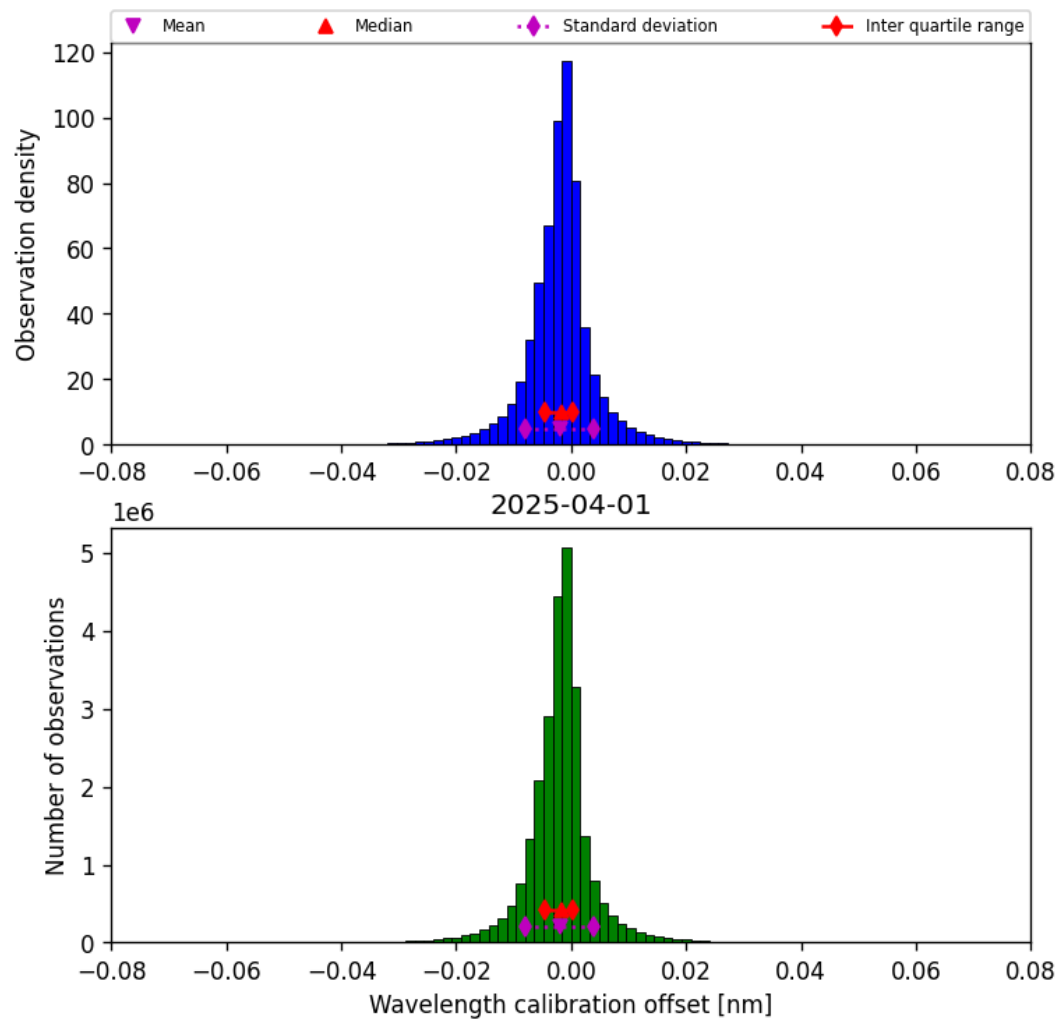
Figure 33: Histogram of “Wavelength calibration offset” for 2025-04-01 to 2025-04-02
