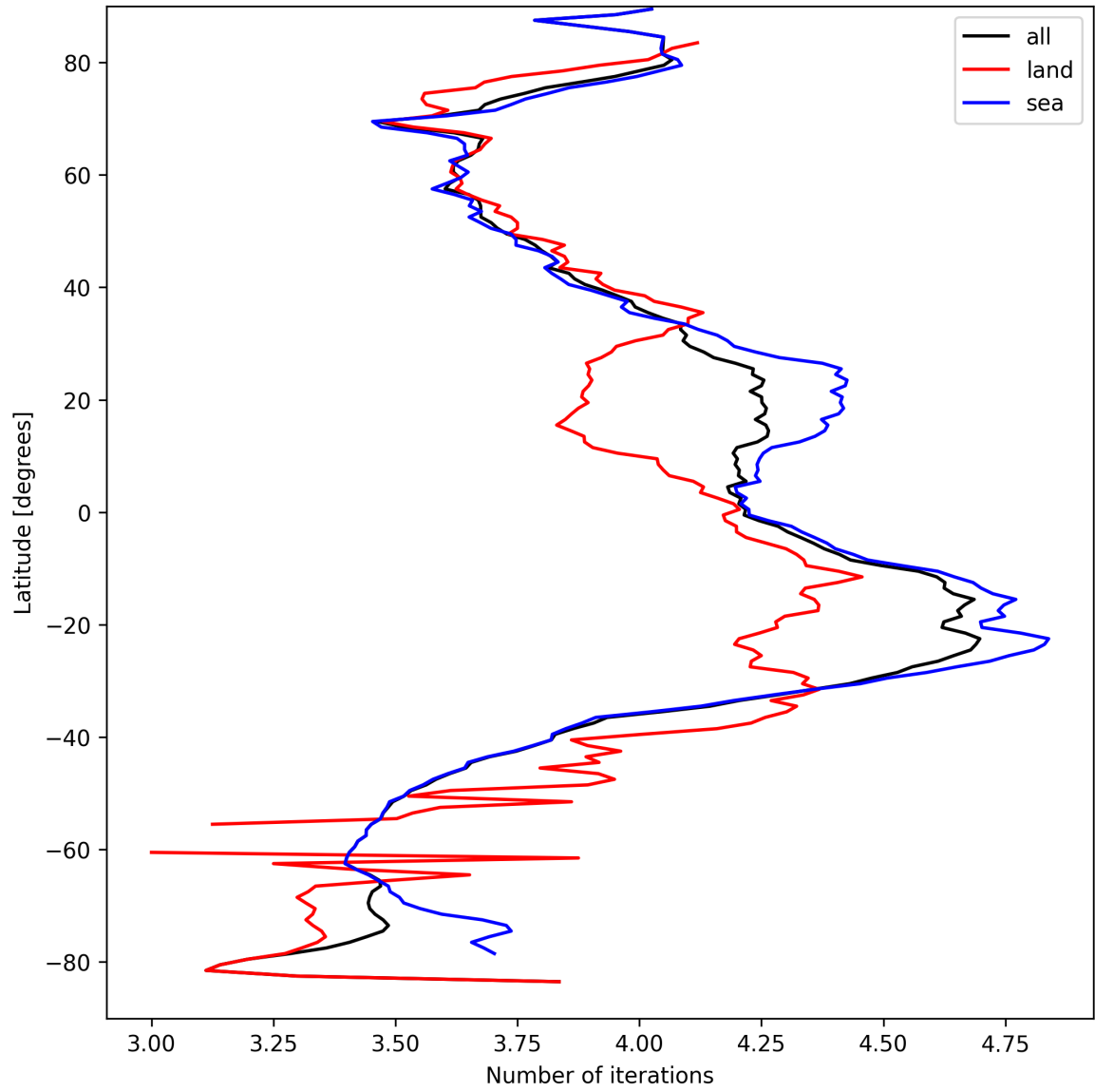
Figure 15: Zonal average of “Number of iterations” for 2025-04-01 to 2025-04-02.
