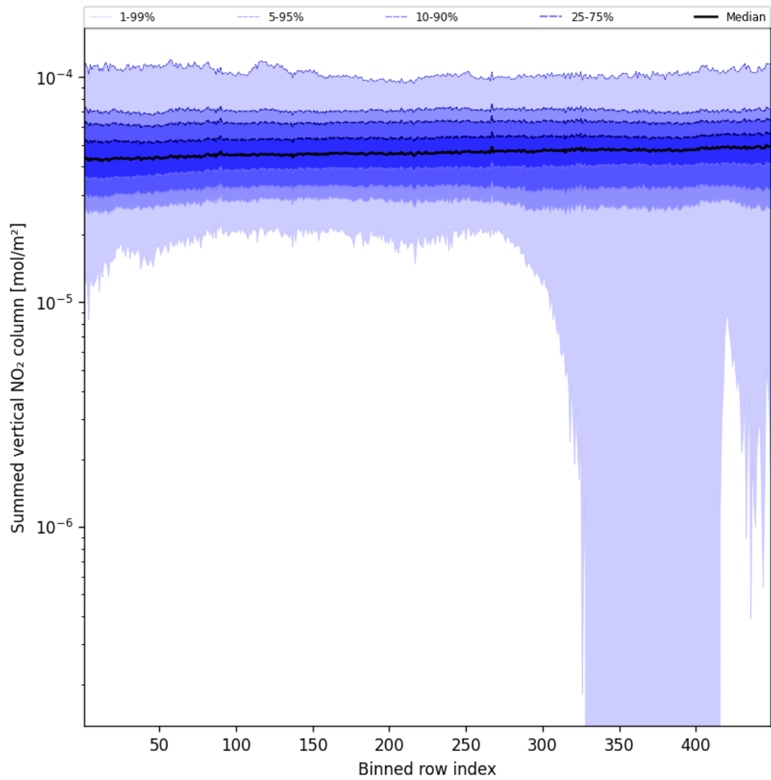
Figure 55: Along track statistics of “Summed vertical NO 2 column” for 2025-04-01 to 2025-04-02
