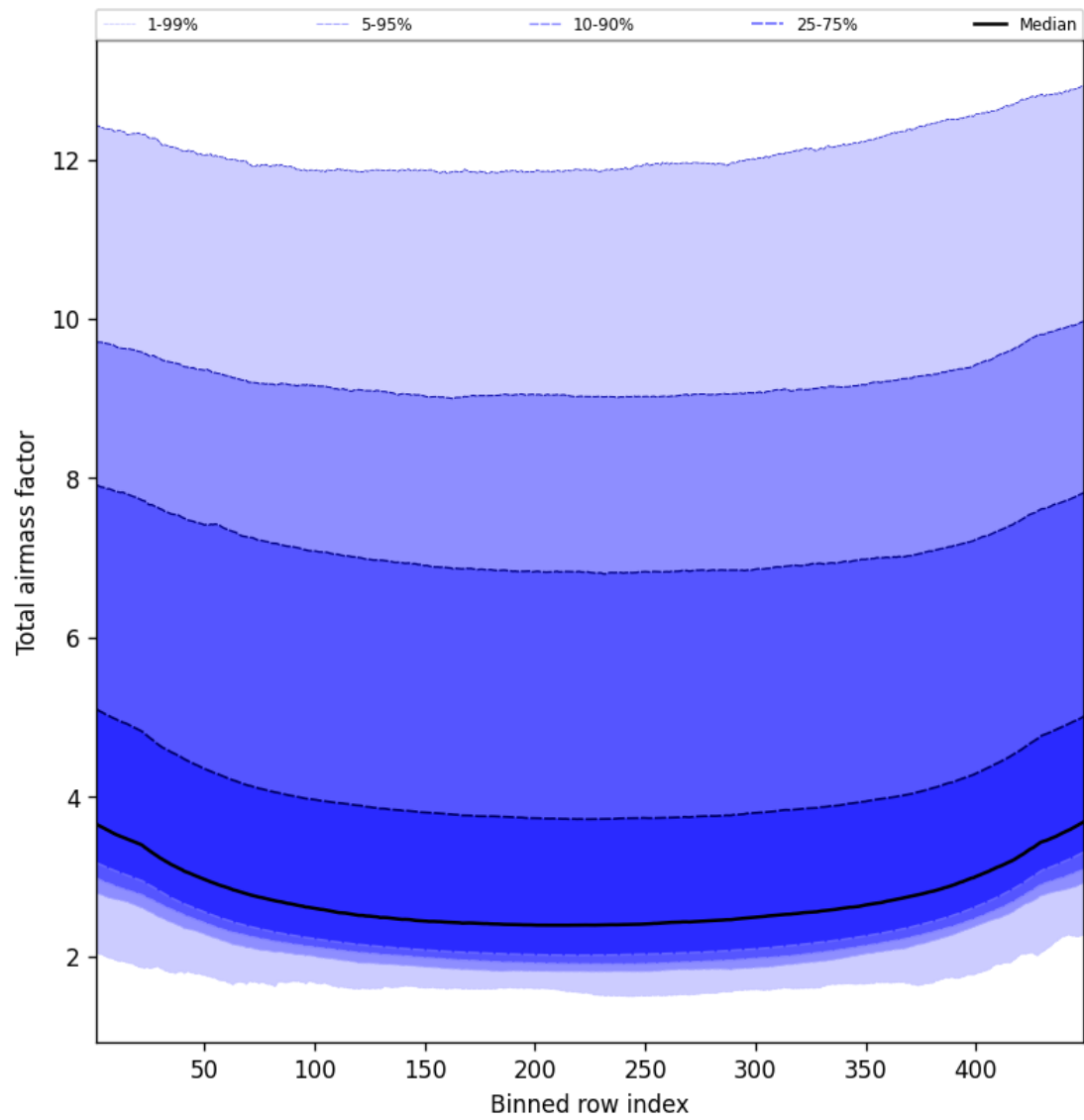
Figure 47: Along track statistics of “Total airmass factor” for 2025-04-01 to 2025-04-02
