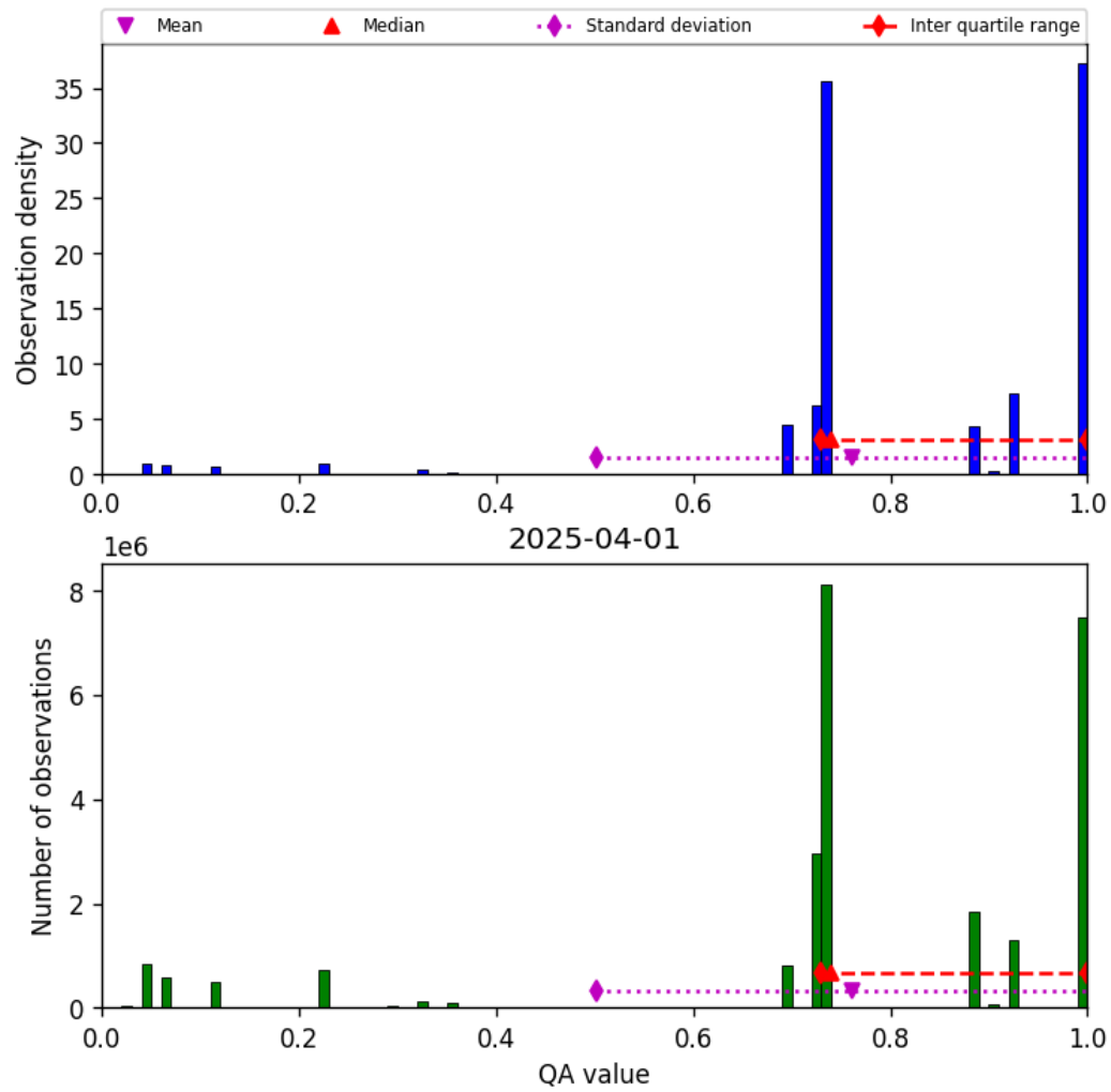
Figure 26: Histogram of “QA value” for 2025-04-01 to 2025-04-02
