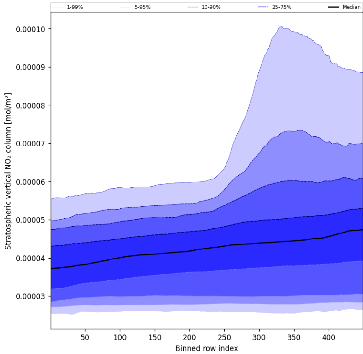
Figure 51: Along track statistics of “Stratospheric vertical NO 2 column” for 2025-04-01 to 2025-04-02
