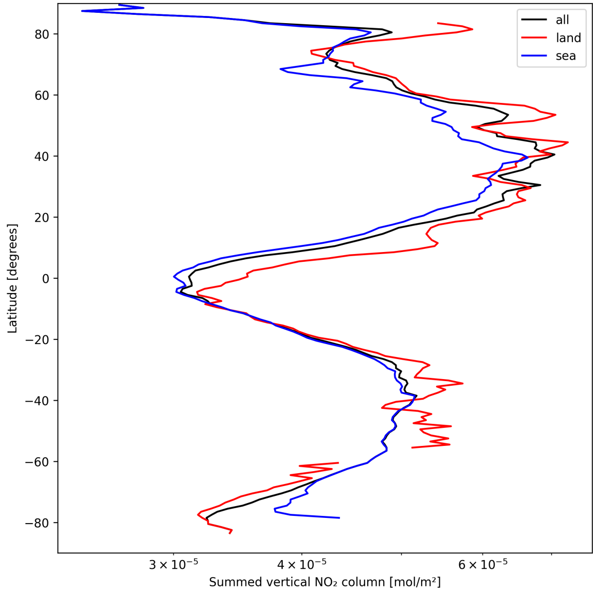
Figure 21: Zonal average of “Summed vertical NO 2 column” for 2025-04-01 to 2025-04-02.
