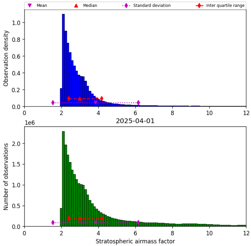
Figure 42: Histogram of “Stratospheric airmass factor” for 2025-04-01 to 2025-04-02
