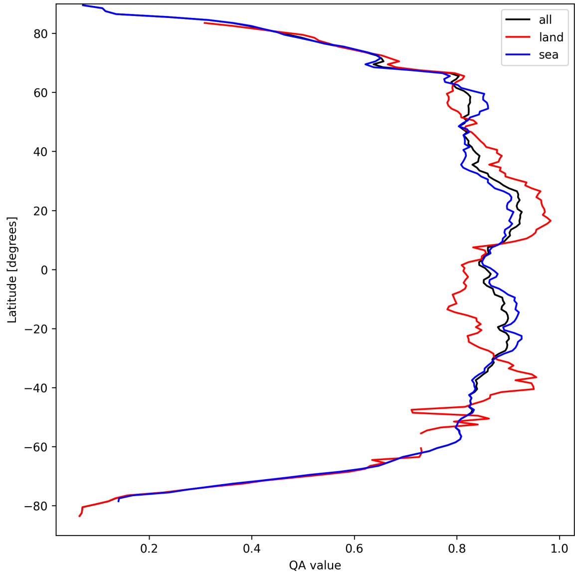
Figure 9: Zonal average of “QA value” for 2025-04-01 to 2025-04-02.
