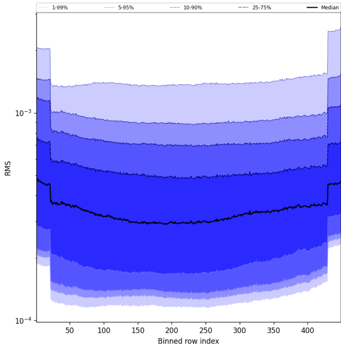
Figure 58: Along track statistics of “RMS” for 2025-04-01 to 2025-04-02
