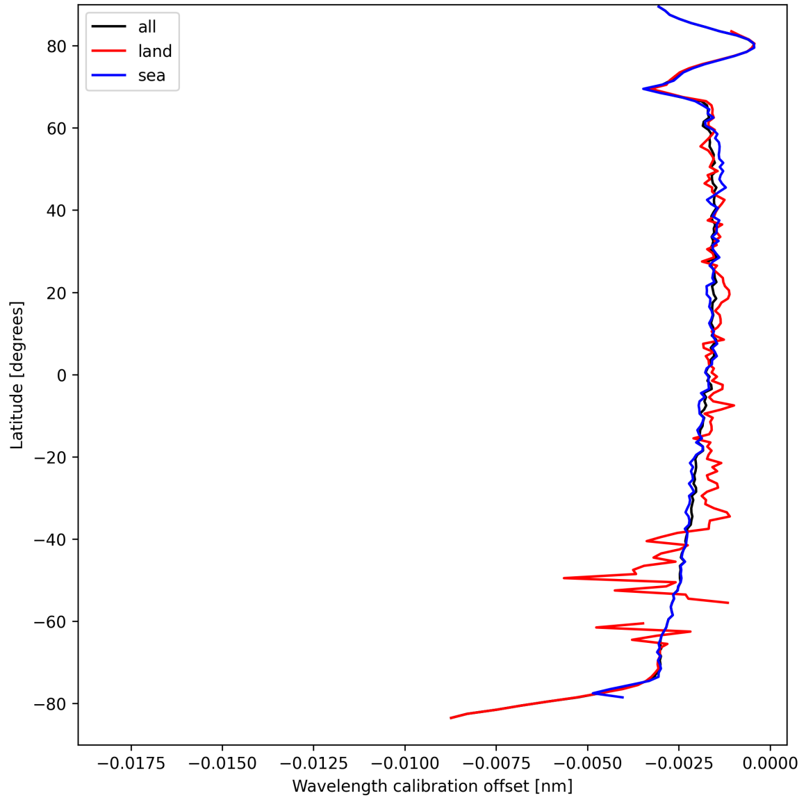
Figure 16: Zonal average of “Wavelength calibration offset” for 2025-04-01 to 2025-04-02.
