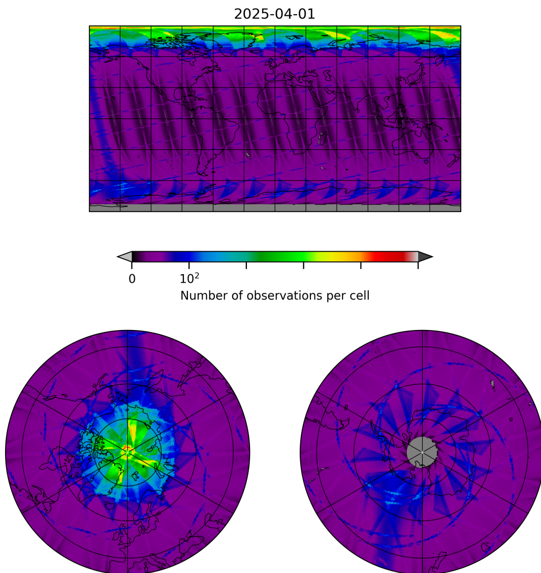
Figure 8: Map of the number of observations for 2025-04-01 to 2025-04-02
