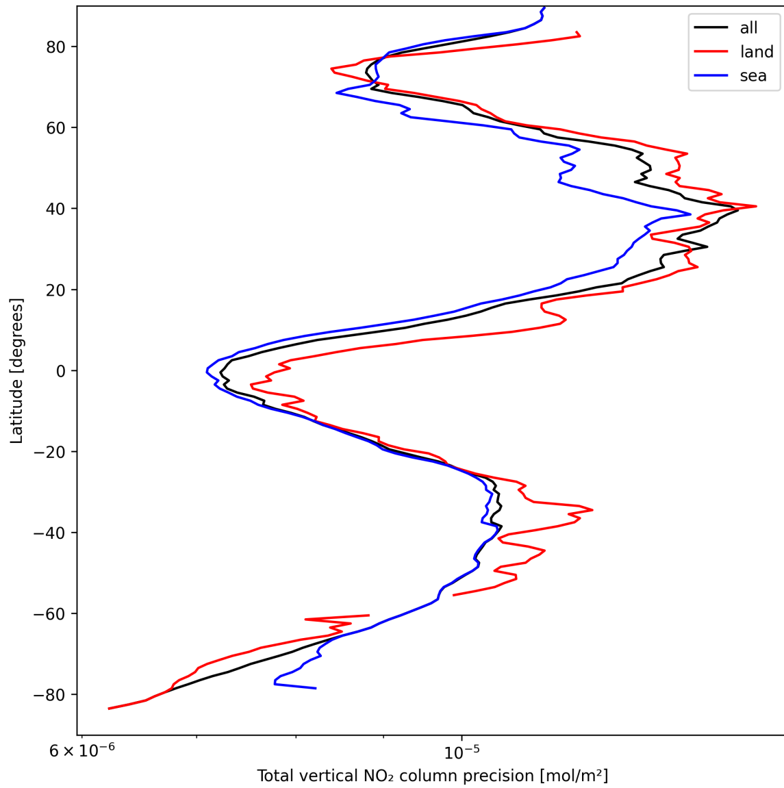
Figure 20: Zonal average of “Total vertical NO 2 column precision” for 2025-04-01 to 2025-04-02.
