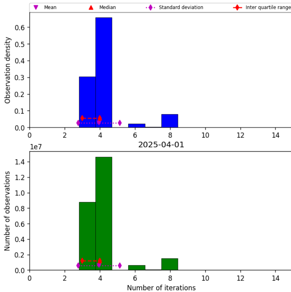
Figure 32: Histogram of “Number of iterations” for 2025-04-01 to 2025-04-02
