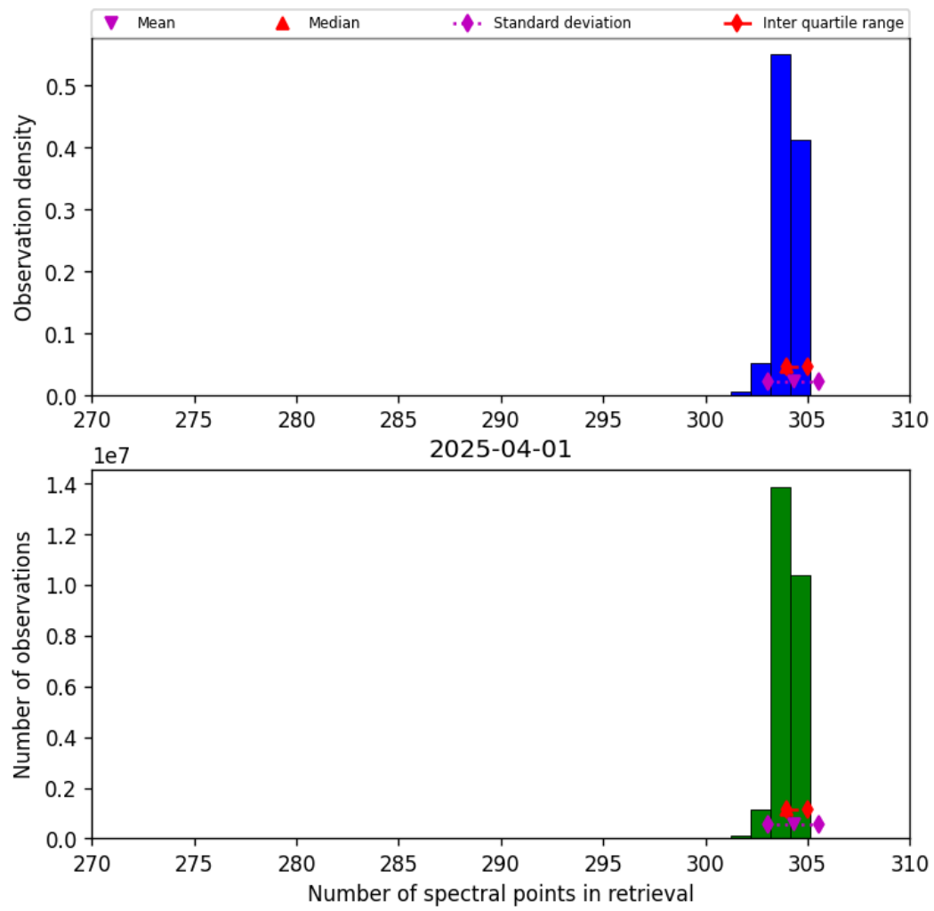
Figure 31: Histogram of “Number of spectral points in retrieval” for 2025-04-01 to 2025-04-02
