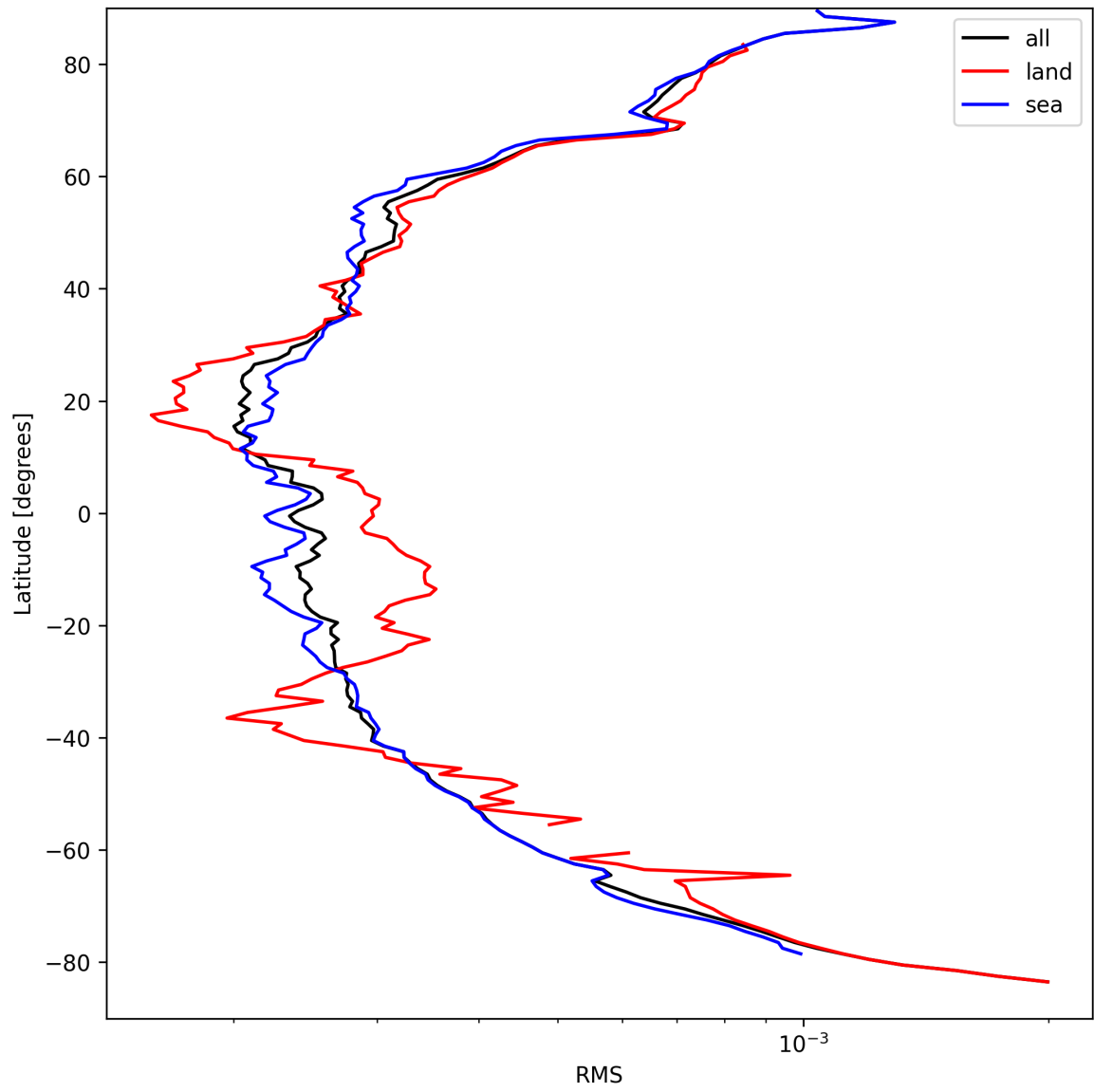
Figure 24: Zonal average of “RMS” for 2025-04-01 to 2025-04-02.
