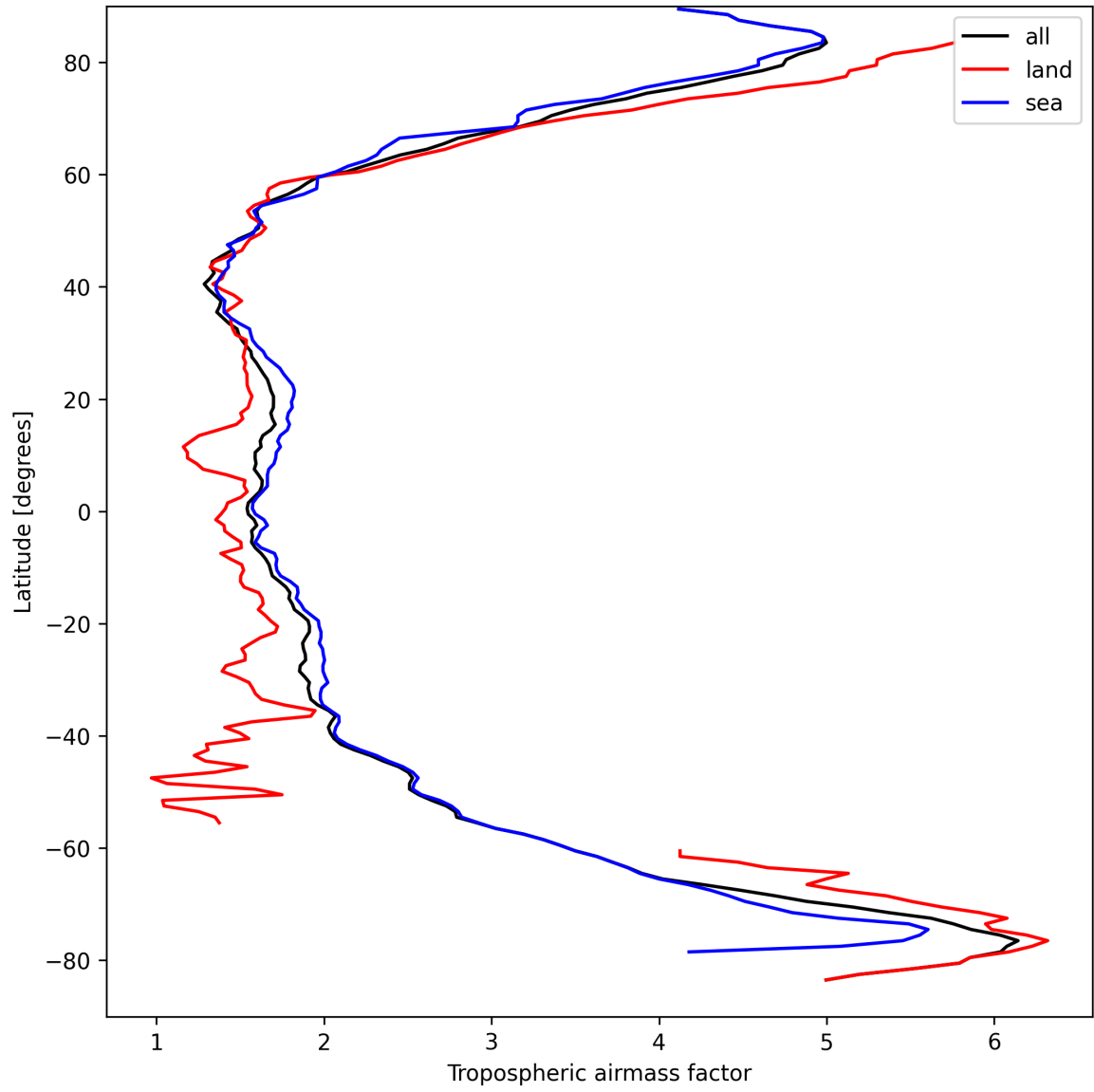
Figure 12: Zonal average of “Tropospheric airmass factor” for 2025-04-01 to 2025-04-02.
