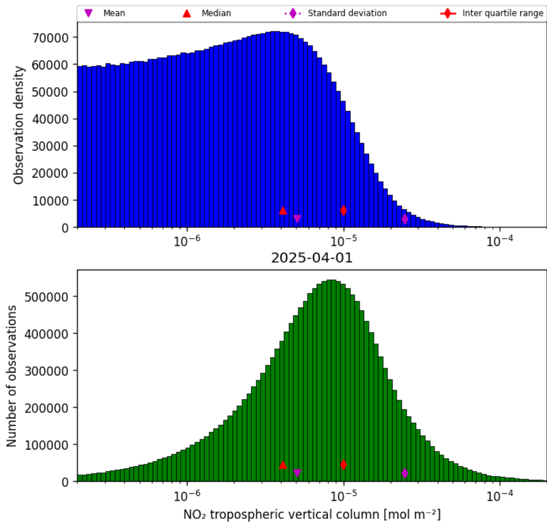
Figure 27: Histogram of “NO 2 tropospheric vertical column” for 2025-04-01 to 2025-04-02
