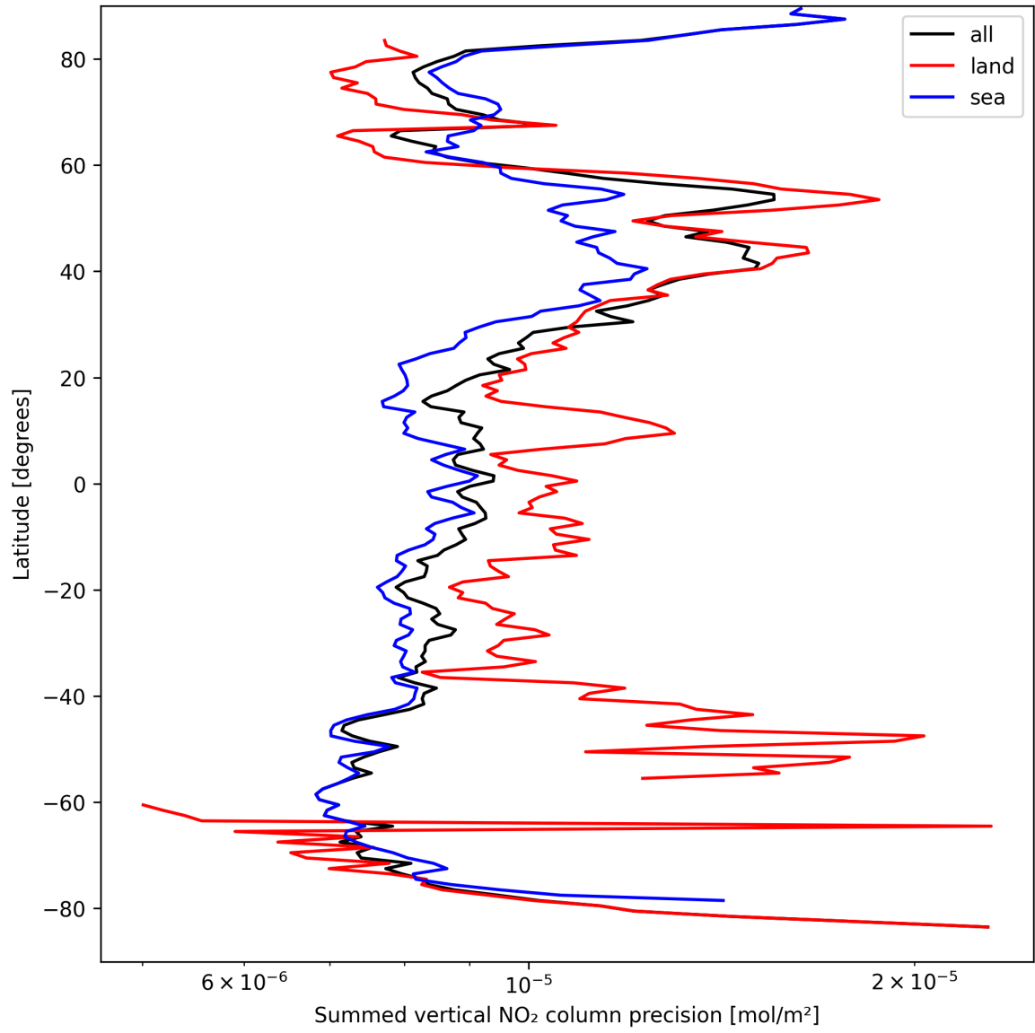
Figure 22: Zonal average of “Summed vertical NO 2 column precision” for 2025-04-01 to 2025-04-02.
