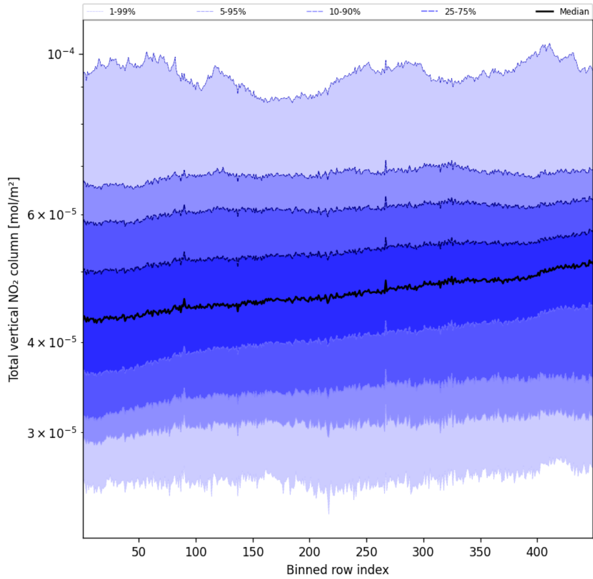
Figure 53: Along track statistics of “Total vertical NO 2 column” for 2025-04-01 to 2025-04-02
