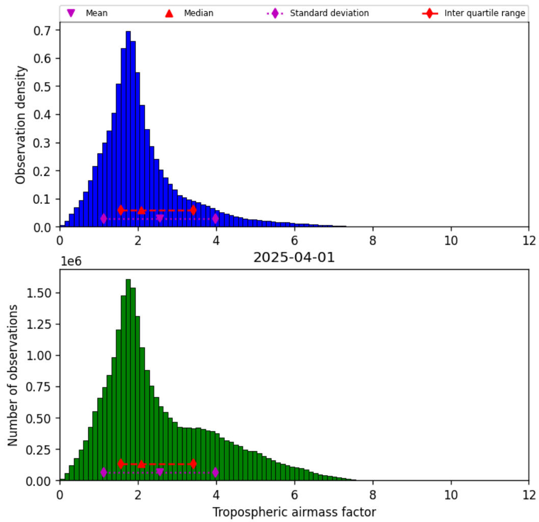
Figure 29: Histogram of “Tropospheric airmass factor” for 2025-04-01 to 2025-04-02
