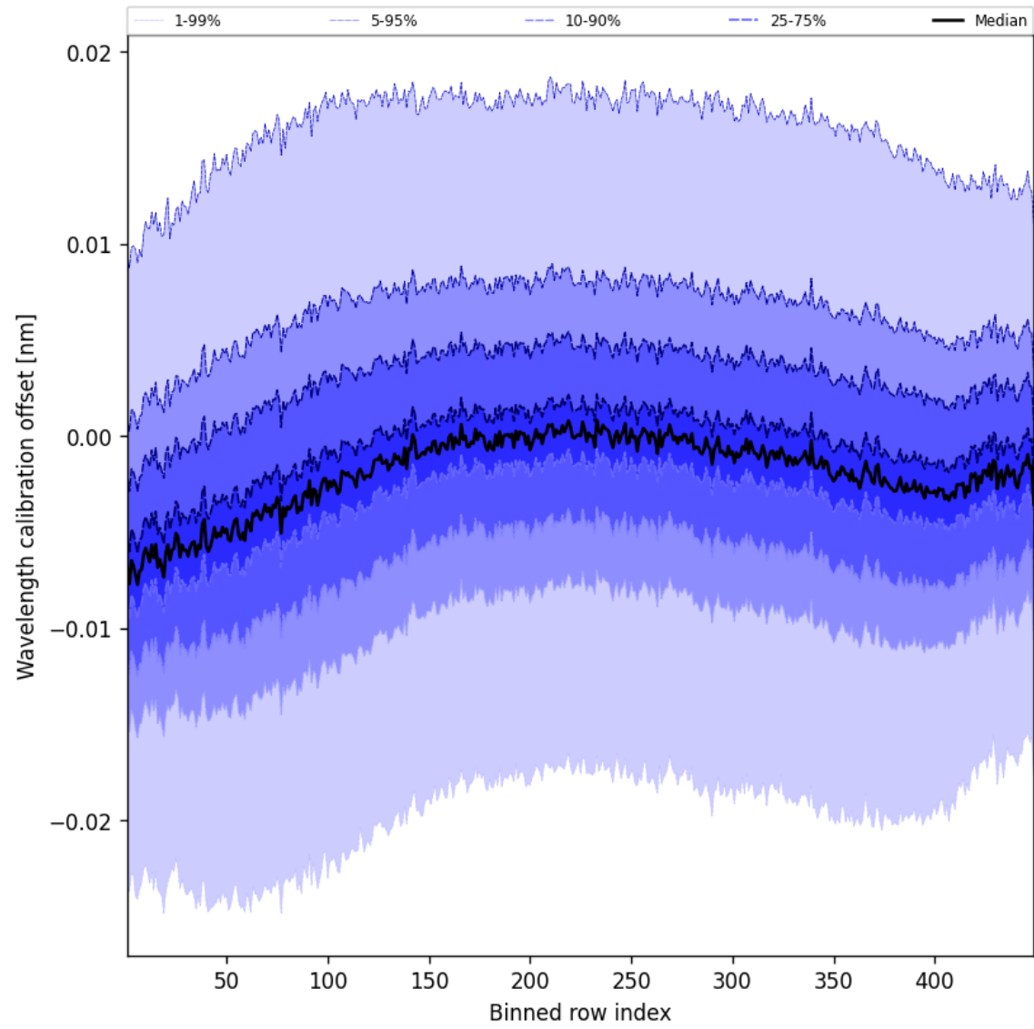
Figure 50: Along track statistics of “Wavelength calibration offset” for 2025-04-01 to 2025-04-02
