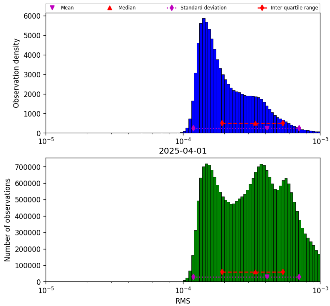
Figure 41: Histogram of “RMS” for 2025-04-01 to 2025-04-02
