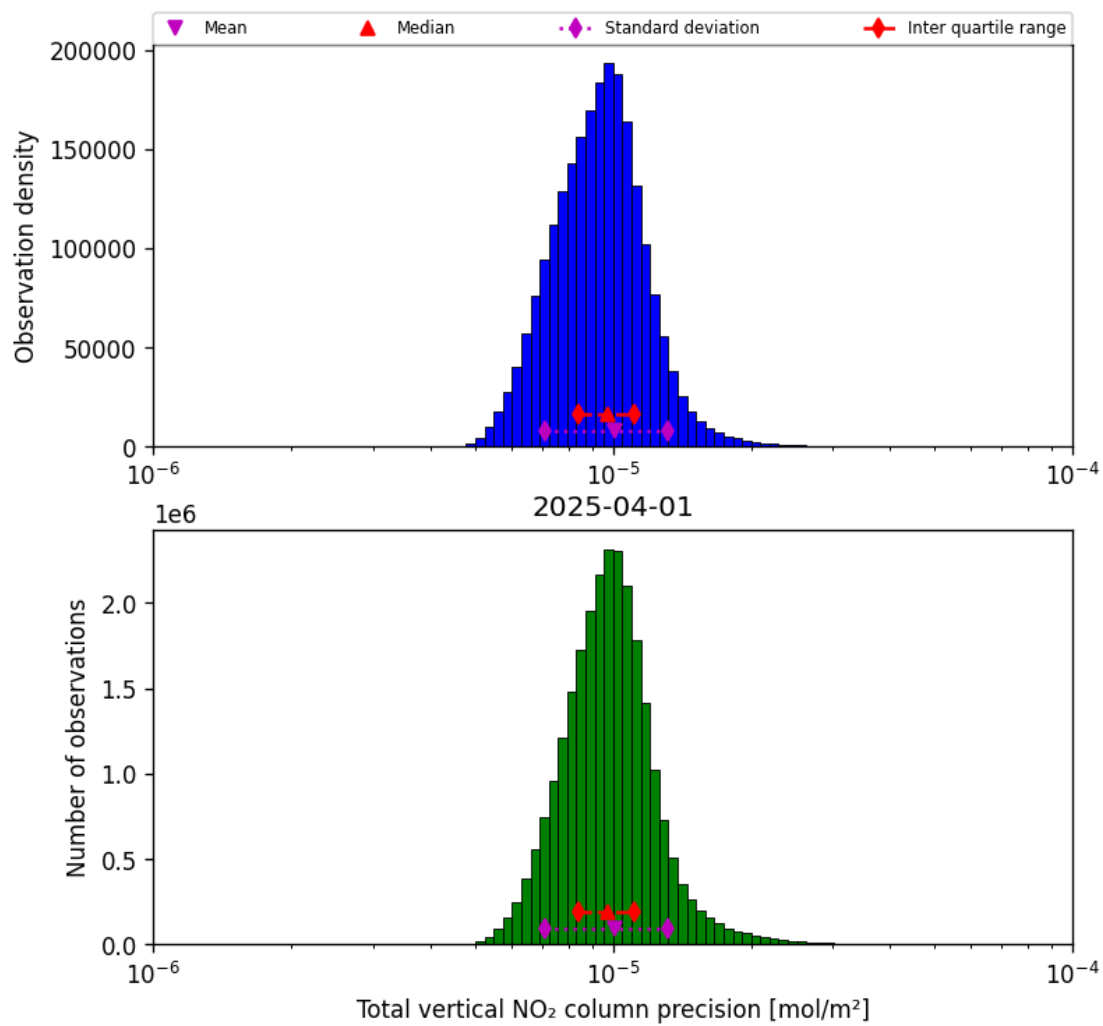
Figure 37: Histogram of “Total vertical NO 2 column precision” for 2025-04-01 to 2025-04-02
