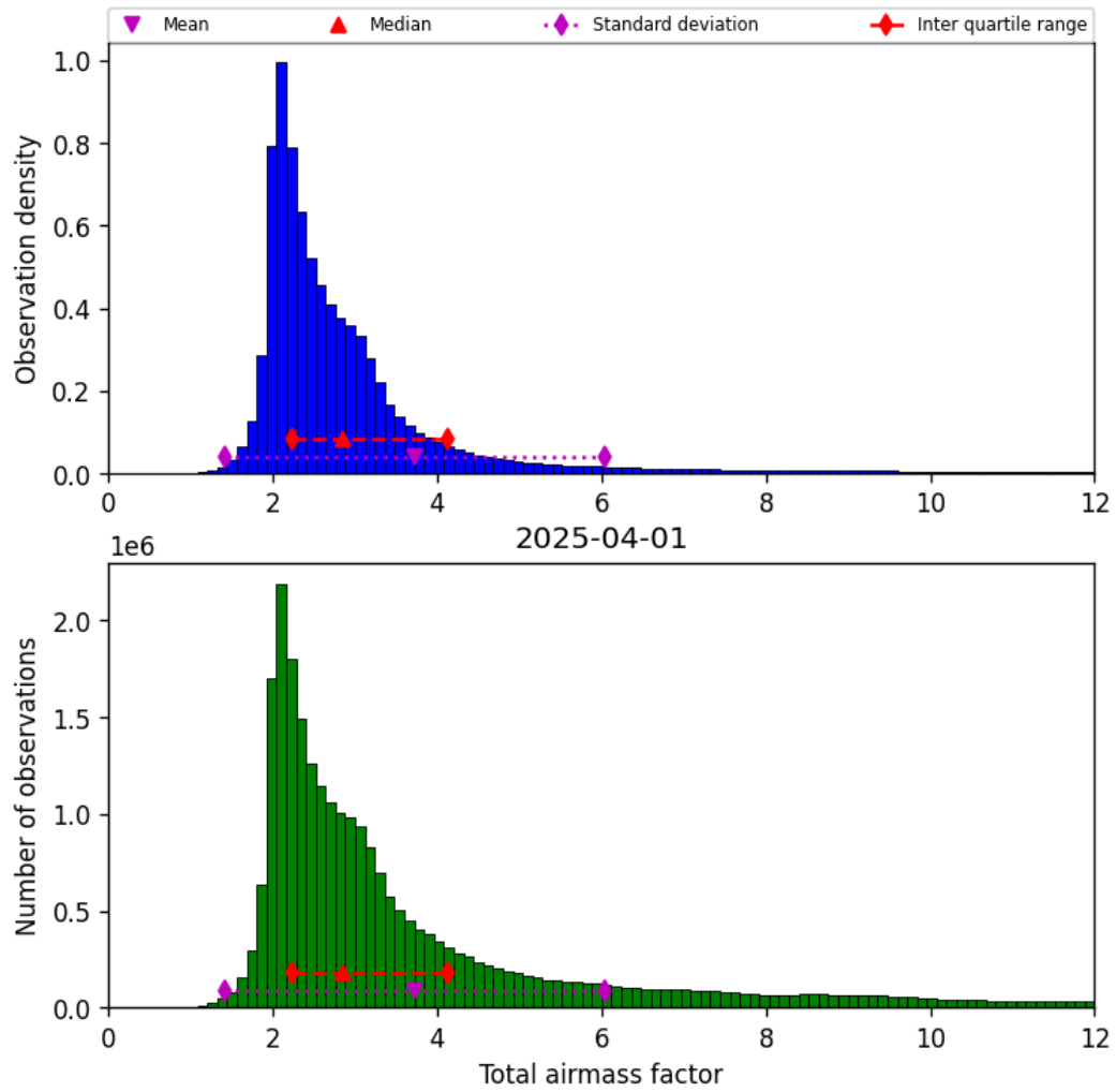
Figure 30: Histogram of “Total airmass factor” for 2025-04-01 to 2025-04-02
