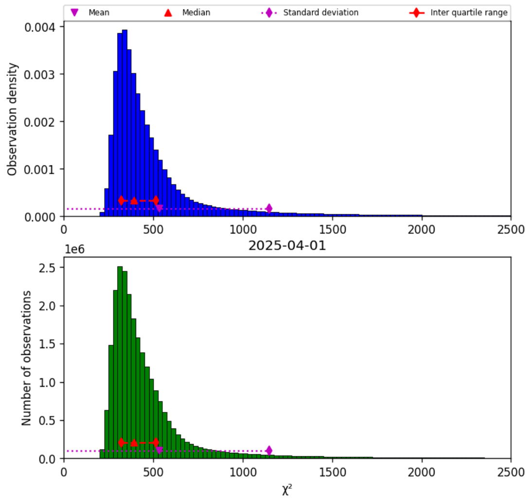
Figure 40: Histogram of “ \chi^2 ” for 2025-04-01 to 2025-04-02
