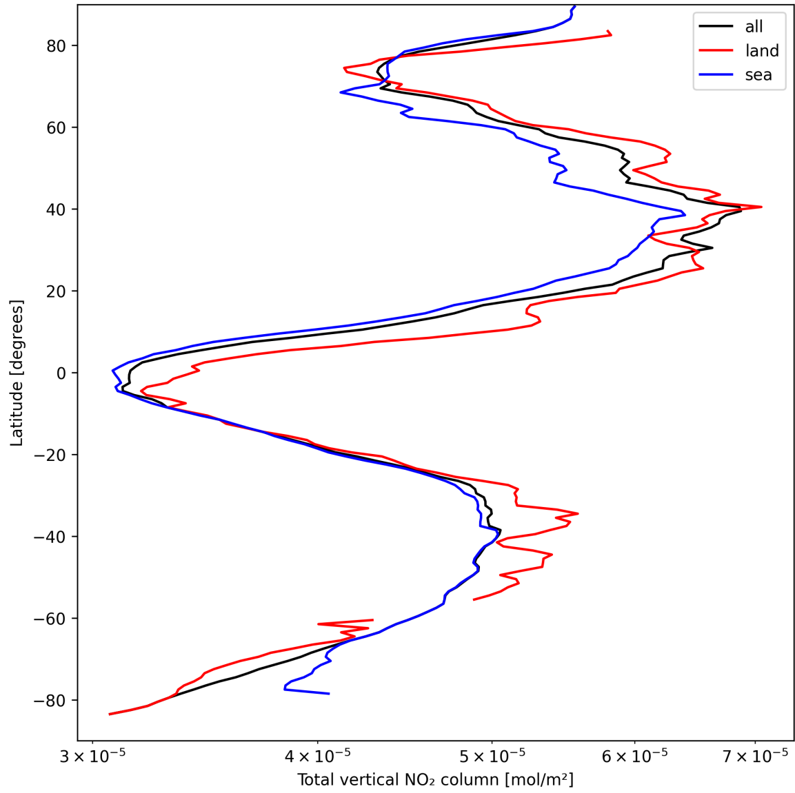
Figure 19: Zonal average of “Total vertical NO 2 column” for 2025-04-01 to 2025-04-02.
