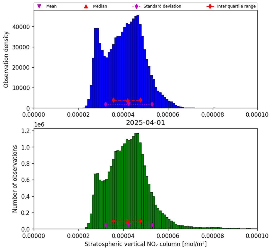
Figure 34: Histogram of “Stratospheric vertical NO 2 column” for 2025-04-01 to 2025-04-02
