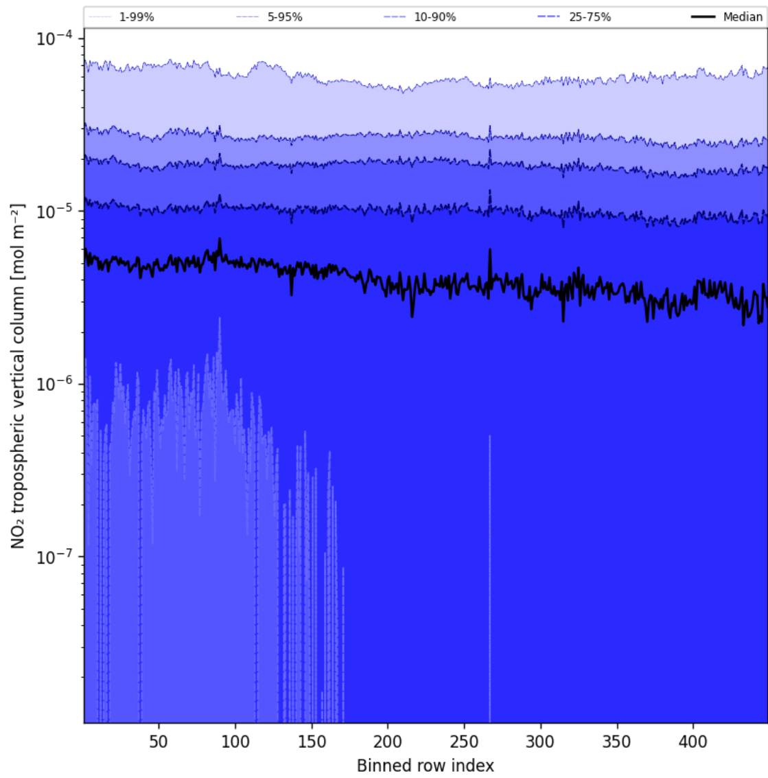
Figure 44: Along track statistics of “NO 2 tropospheric vertical column” for 2025-04-01 to 2025-04-02
