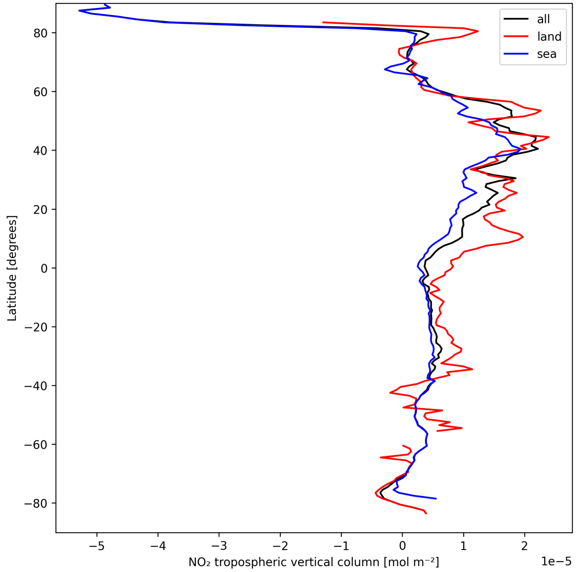
Figure 10: Zonal average of “NO 2 tropospheric vertical column” for 2025-04-01 to 2025-04-02.
