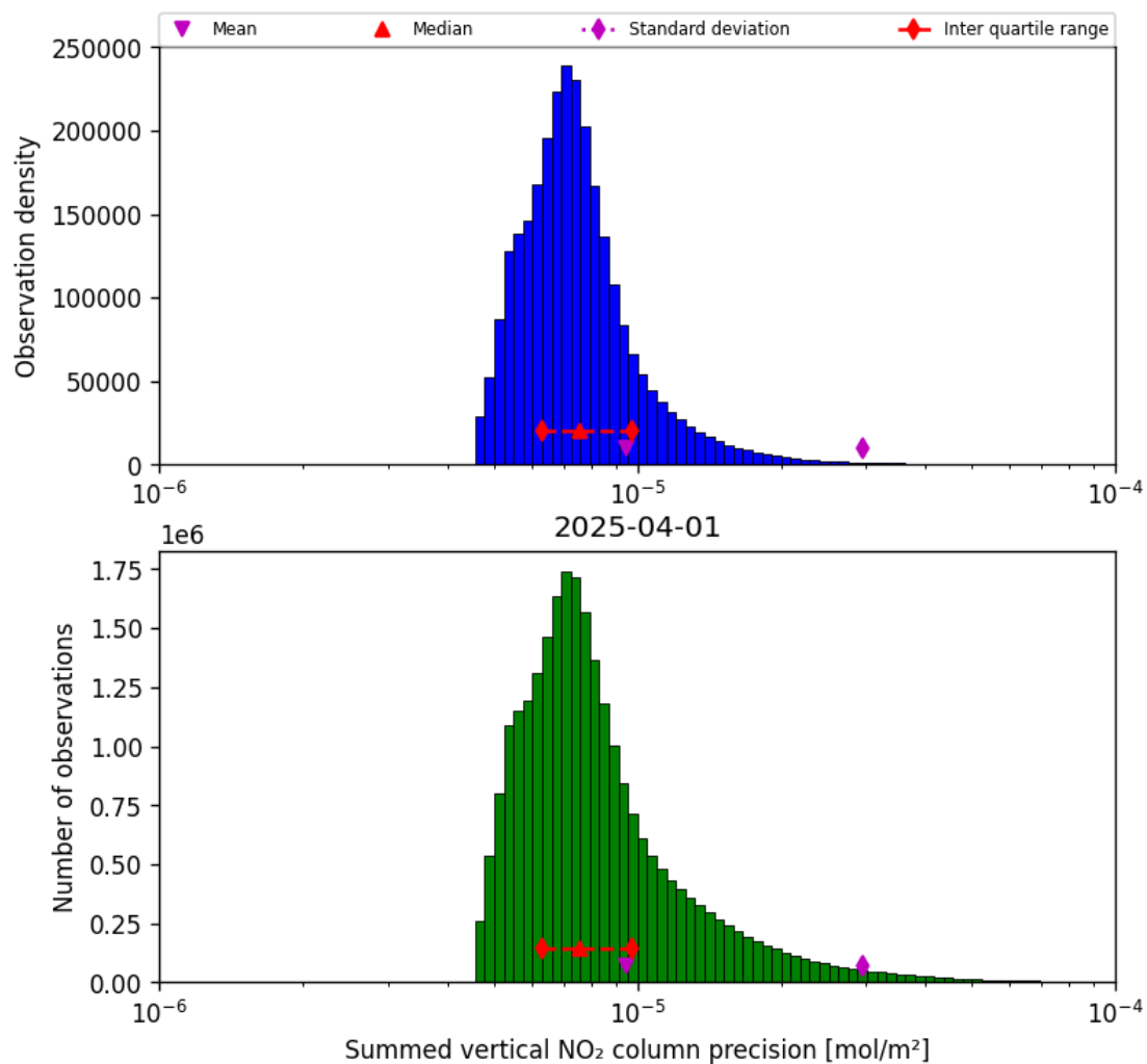
Figure 39: Histogram of “Summed vertical NO 2 column precision” for 2025-04-01 to 2025-04-02
