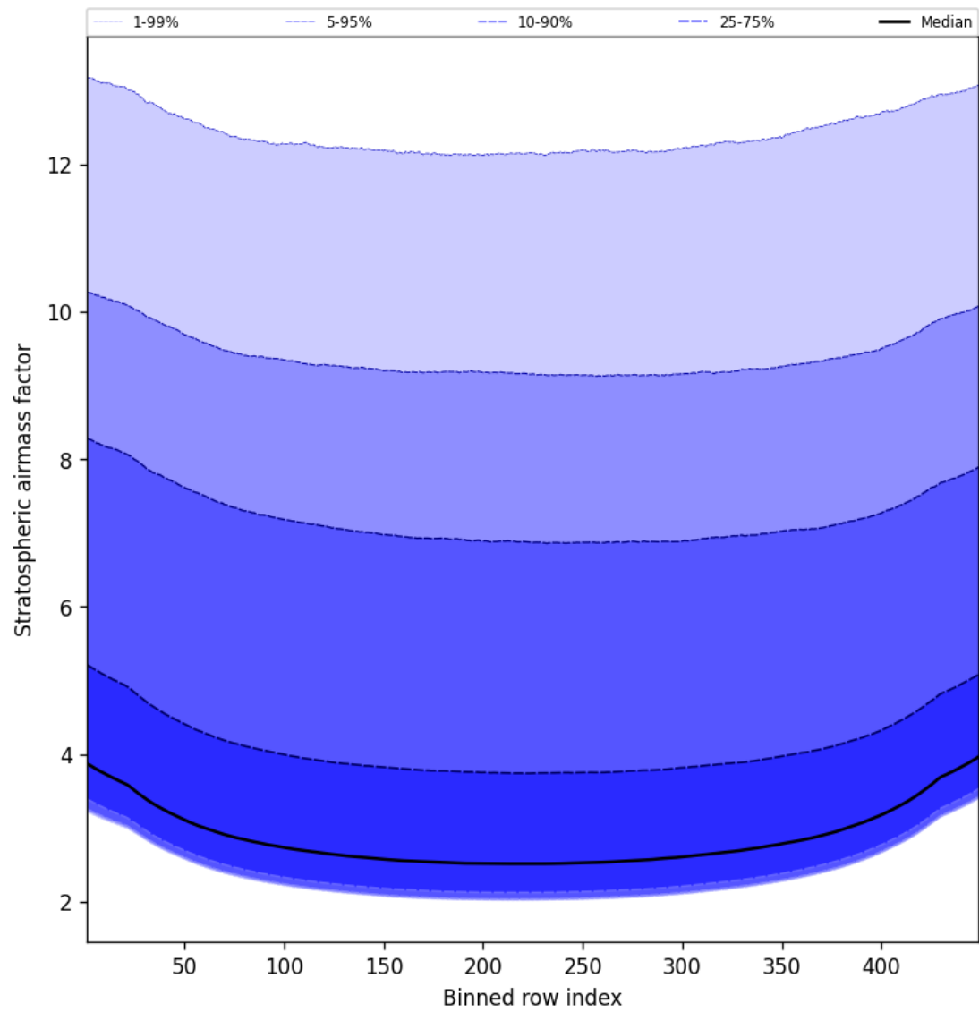
Figure 59: Along track statistics of “Stratospheric air mass factor” for 2025-04-01 to 2025-04-02
