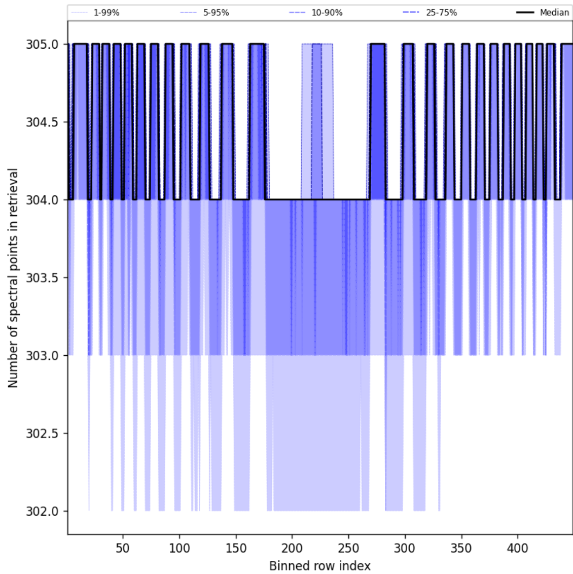
Figure 48: Along track statistics of “Number of spectral points in retrieval” for 2025-04-01 to 2025-04-02
