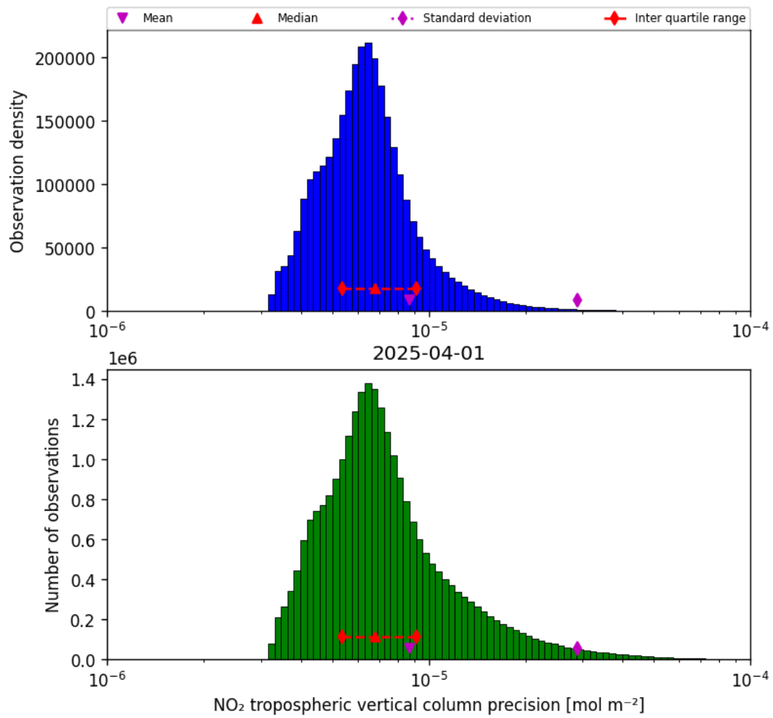
Figure 28: Histogram of “NO 2 tropospheric vertical column precision” for 2025-04-01 to 2025-04-02
