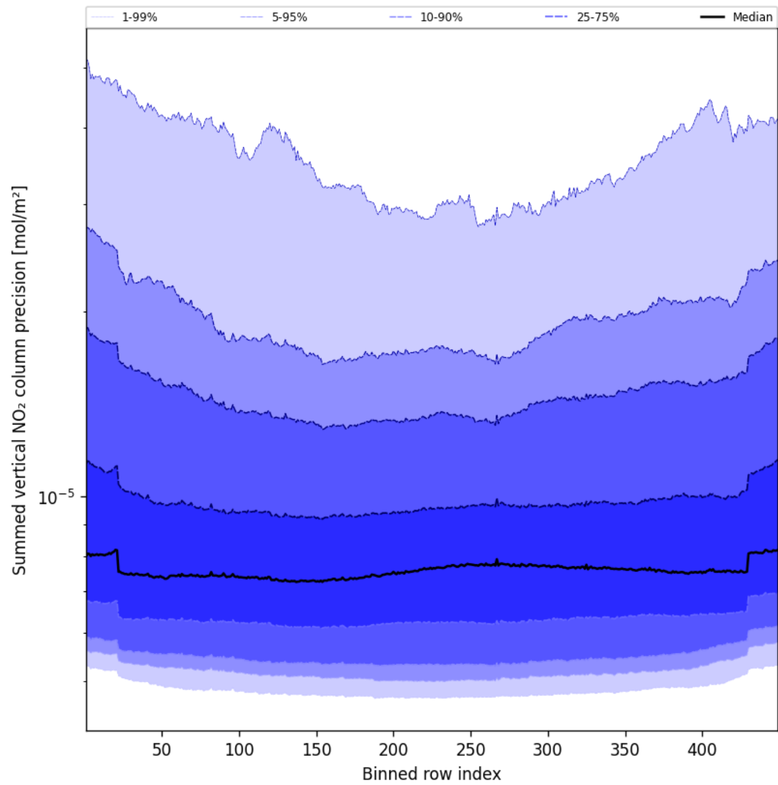
Figure 56: Along track statistics of “Summed vertical NO 2 column precision” for 2025-04-01 to 2025-04-02
