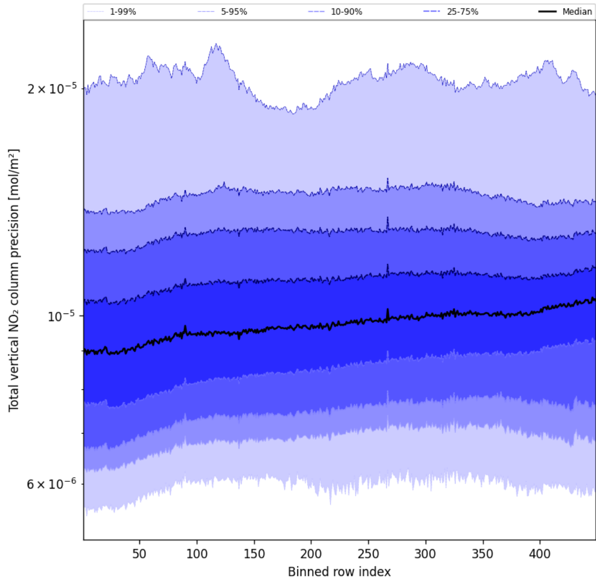
Figure 54: Along track statistics of “Total vertical NO 2 column precision” for 2025-04-01 to 2025-04-02
