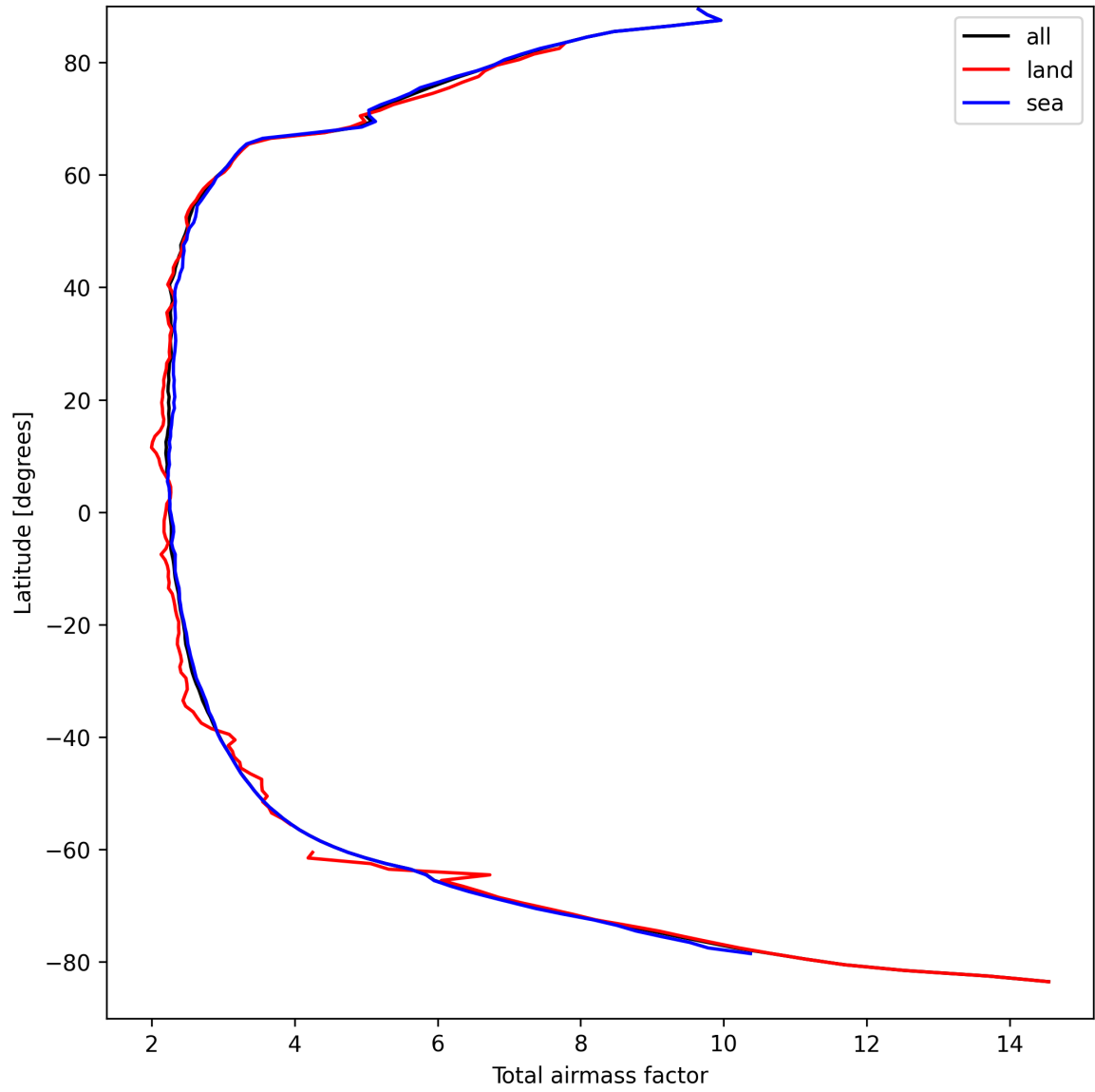
Figure 13: Zonal average of “Total airmass factor” for 2025-04-01 to 2025-04-02.
