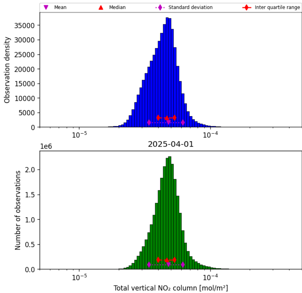
Figure 36: Histogram of “Total vertical NO 2 column” for 2025-04-01 to 2025-04-02
