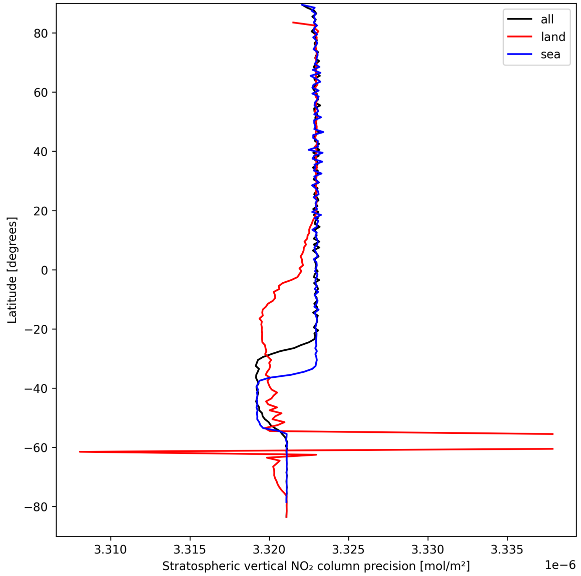
Figure 18: Zonal average of “Stratospheric vertical NO 2 column precision” for 2025-04-01 to 2025-04-02.
