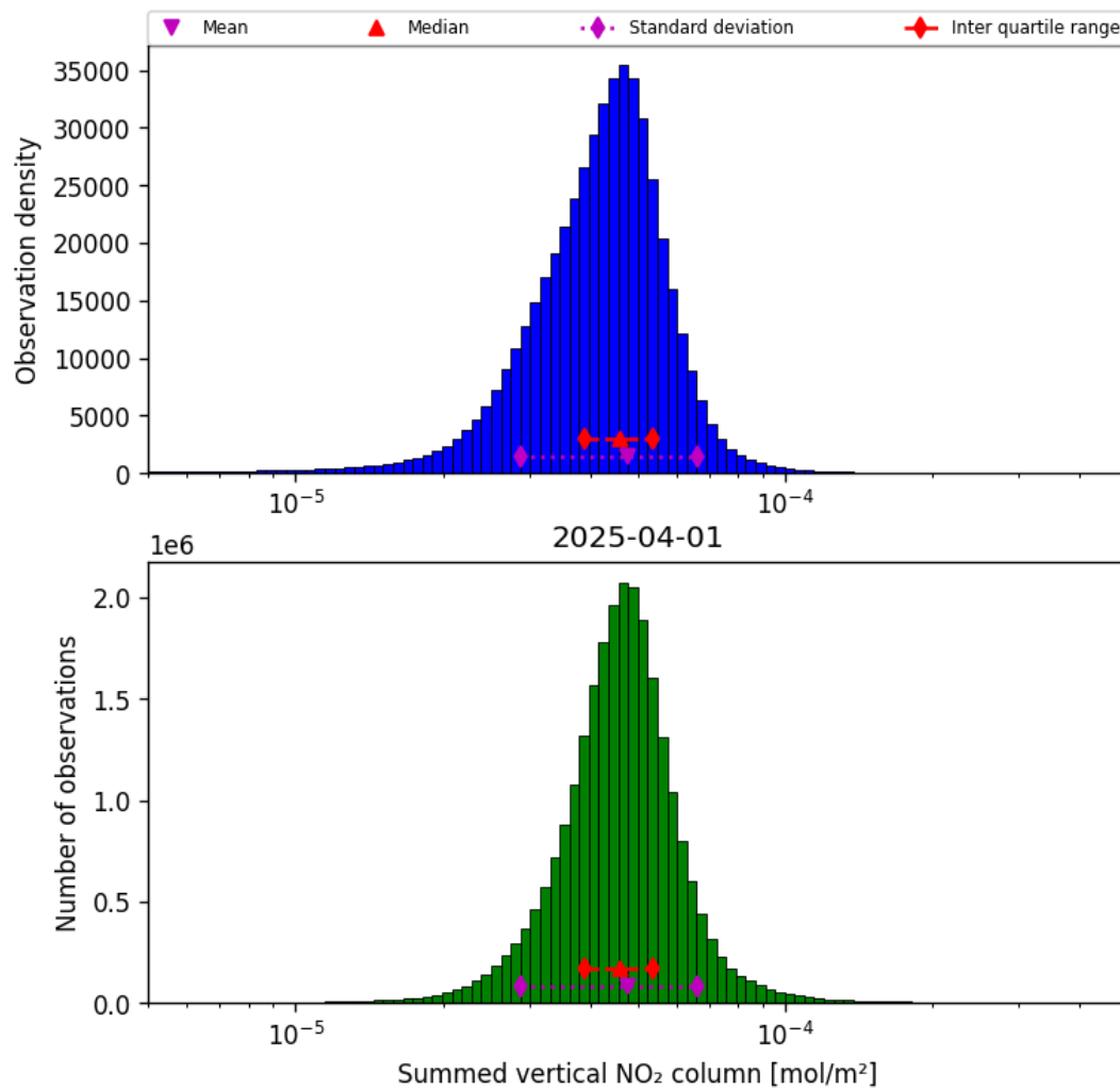
Figure 38: Histogram of “Summed vertical NO 2 column” for 2025-04-01 to 2025-04-02
