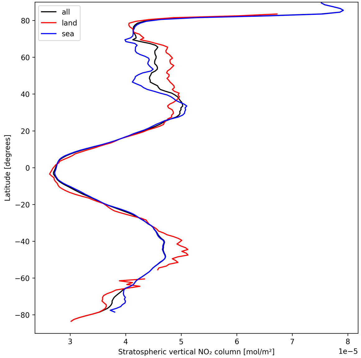
Figure 17: Zonal average of “Stratospheric vertical NO 2 column” for 2025-04-01 to 2025-04-02.
