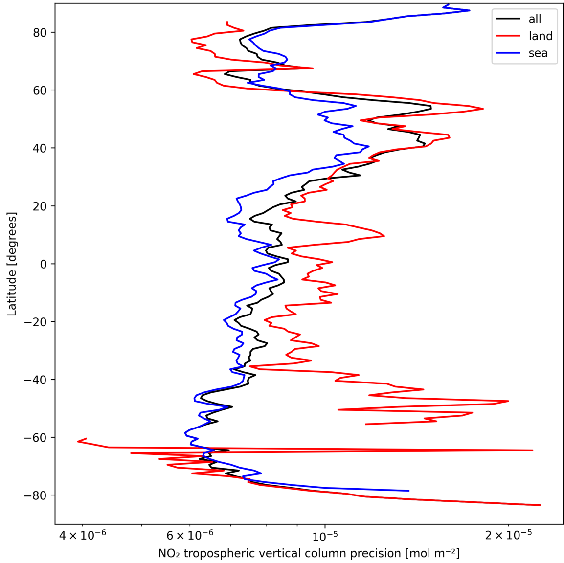
Figure 11: Zonal average of “NO 2 tropospheric vertical column precision” for 2025-04-01 to 2025-04-02.
