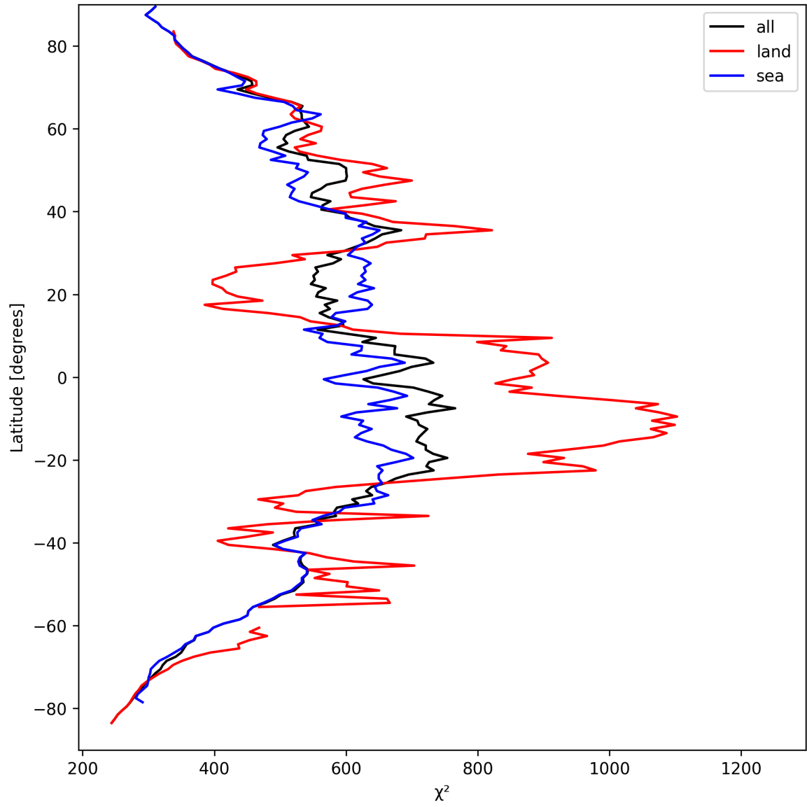
Figure 23: Zonal average of “ \chi^2 ” for 2025-04-01 to 2025-04-02.
