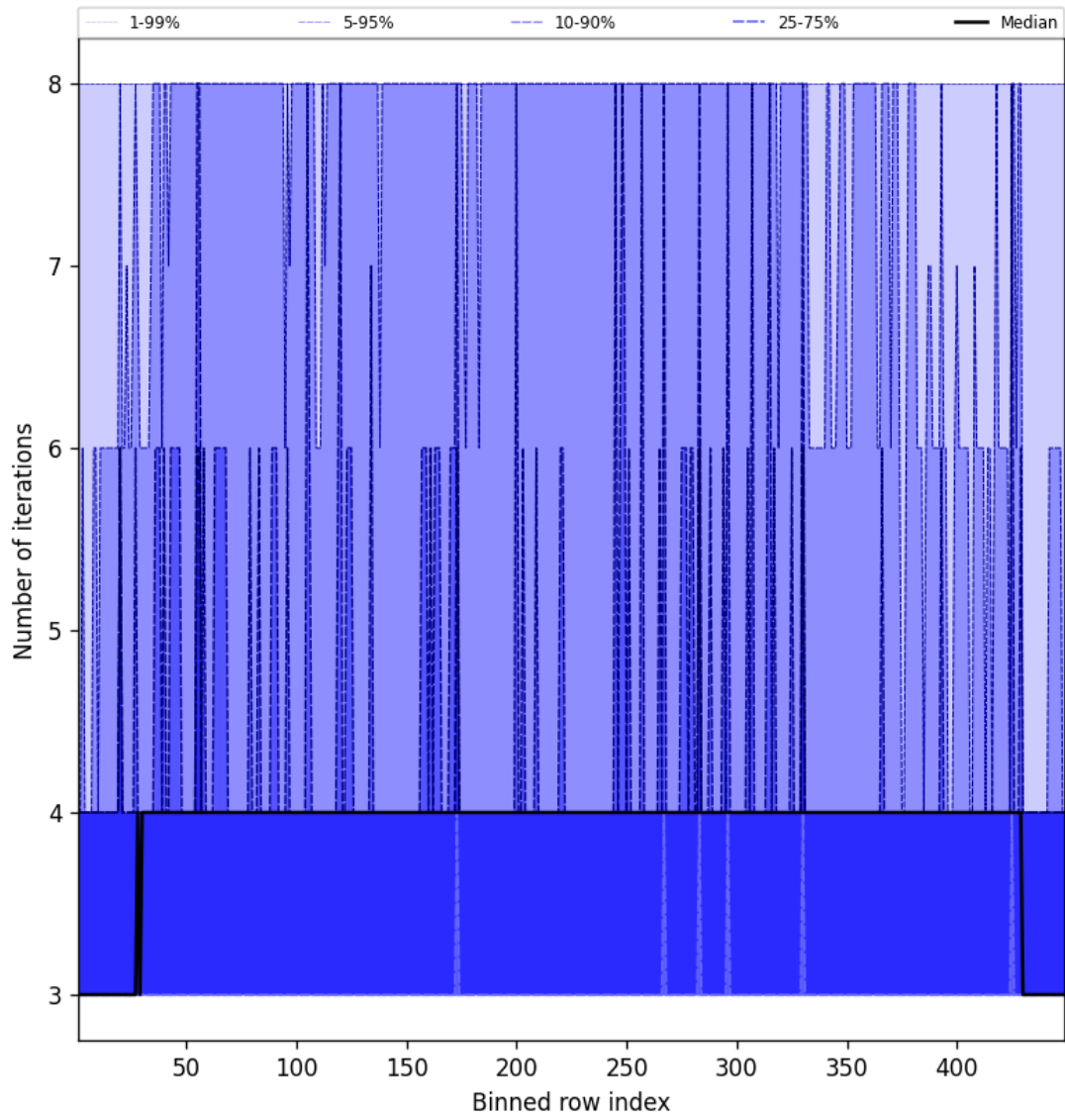
Figure 49: Along track statistics of “Number of iterations” for 2025-04-01 to 2025-04-02
