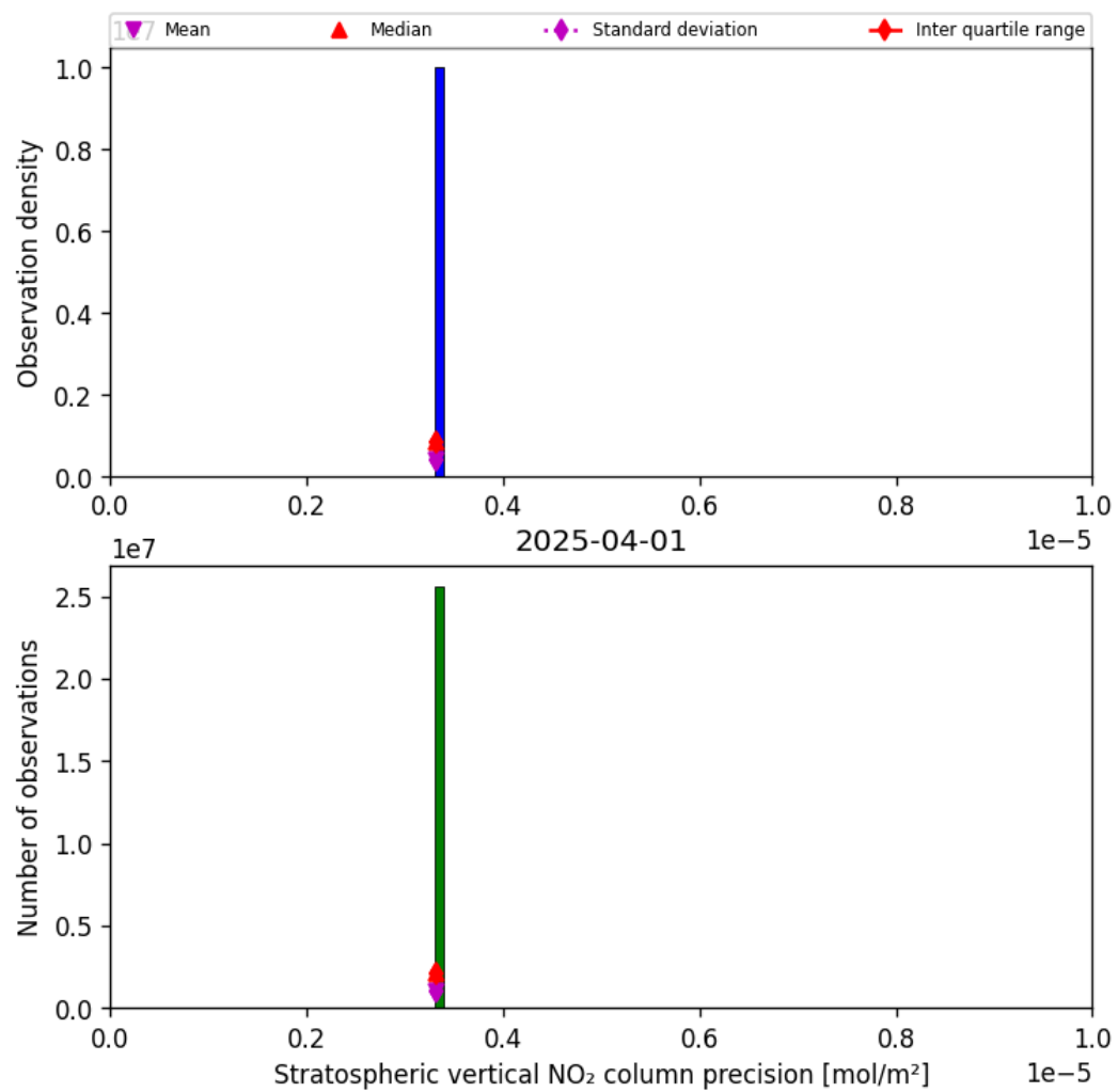
Figure 35: Histogram of “Stratospheric vertical NO 2 column precision” for 2025-04-01 to 2025-04-02
