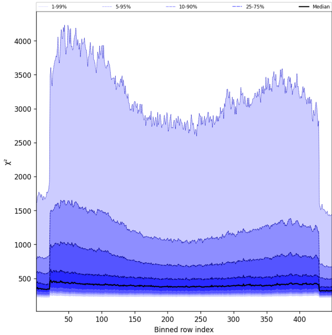
Figure 57: Along track statistics of “ \chi^2 ” for 2025-04-01 to 2025-04-02
