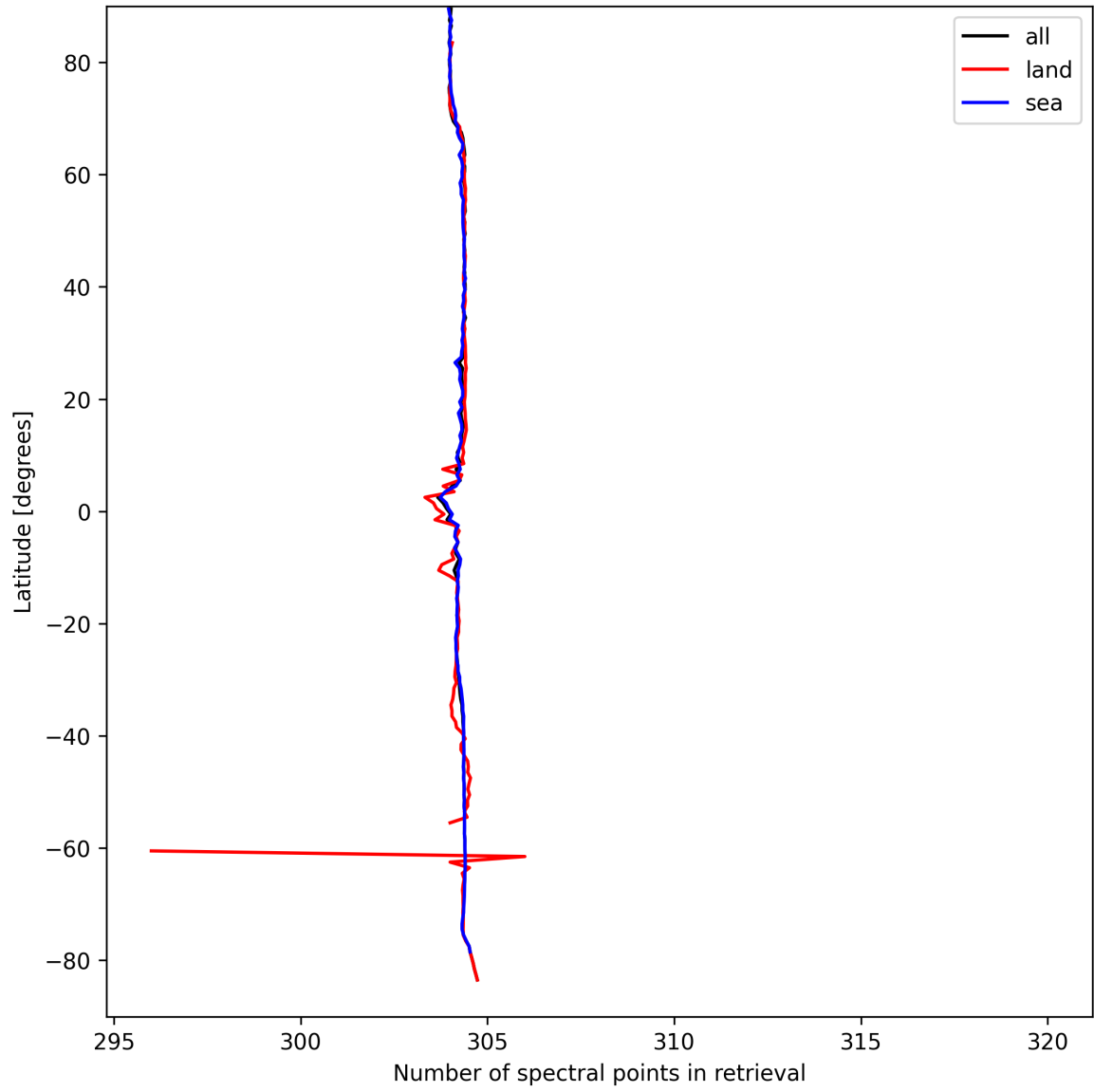
Figure 14: Zonal average of “Number of spectral points in retrieval” for 2025-04-01 to 2025-04-02.
