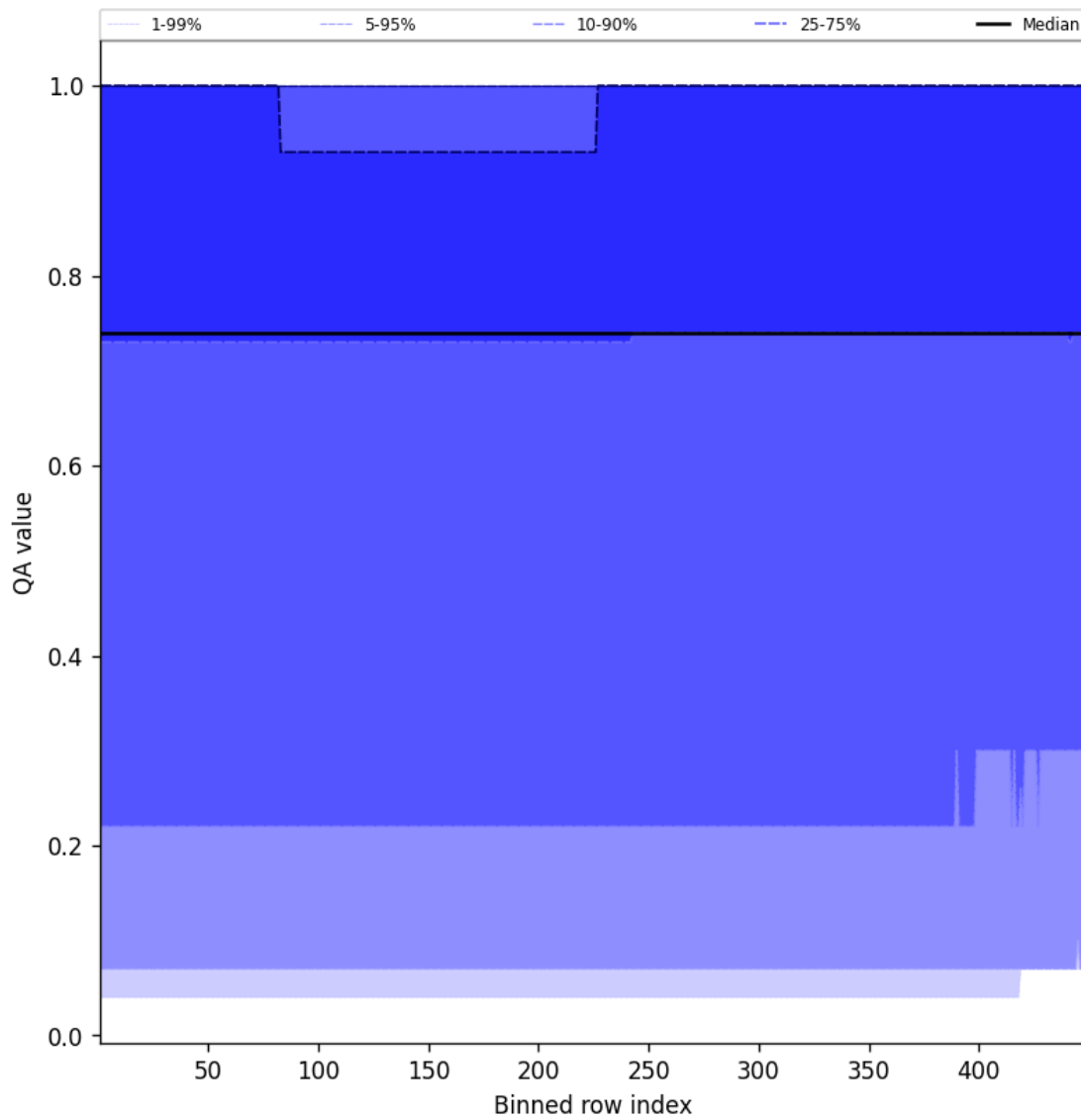
Figure 43: Along track statistics of “QA value” for 2025-04-01 to 2025-04-02
