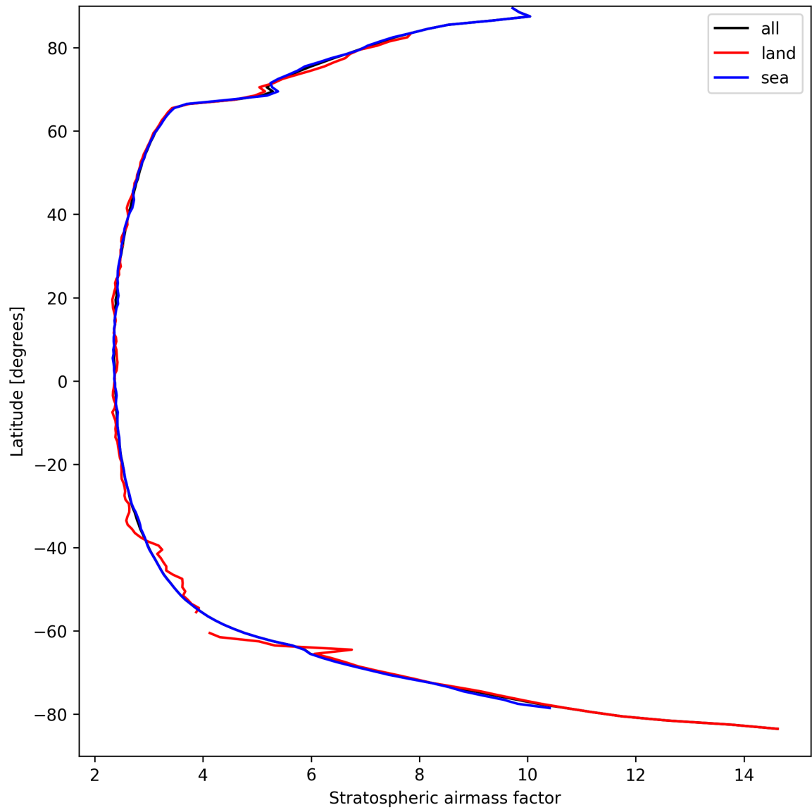
Figure 25: Zonal average of “Stratospheric airmass factor” for 2025-04-01 to 2025-04-02.
