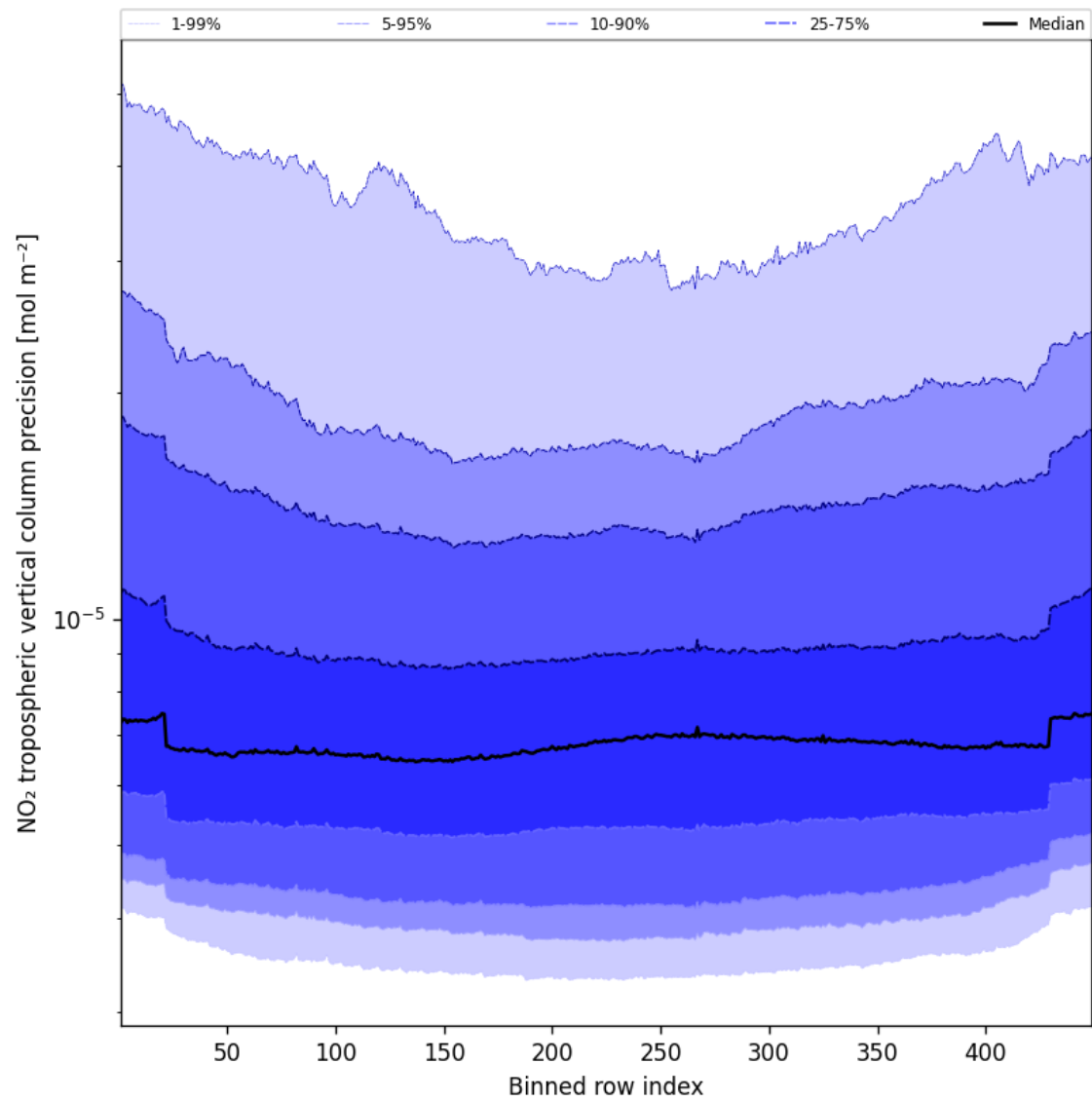
Figure 45: Along track statistics of “NO 2 tropospheric vertical column precision” for 2025-04-01 to 2025-04-02
