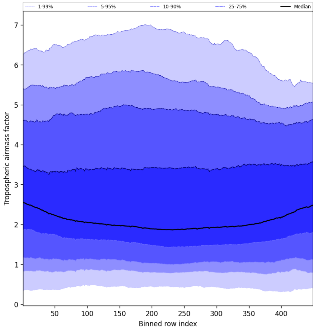
Figure 46: Along track statistics of “Tropospheric airmass factor” for 2025-04-01 to 2025-04-02
