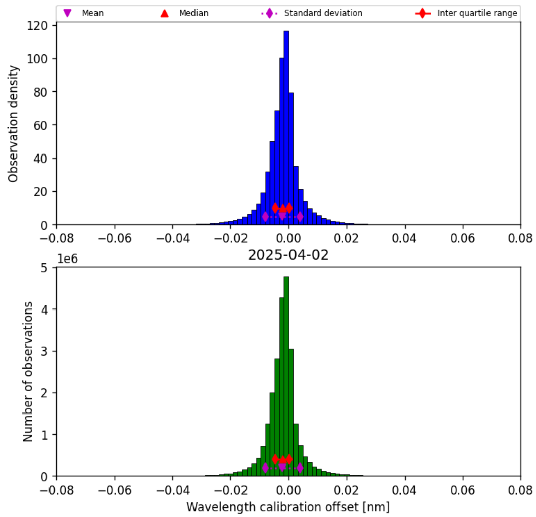
Figure 33: Histogram of “Wavelength calibration offset” for 2025-04-02 to 2025-04-03
