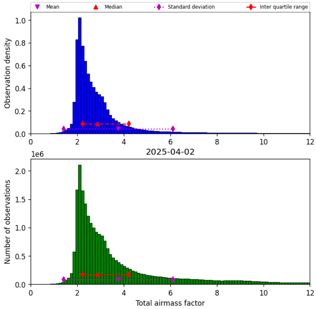
Figure 30: Histogram of “Total airmass factor” for 2025-04-02 to 2025-04-03
