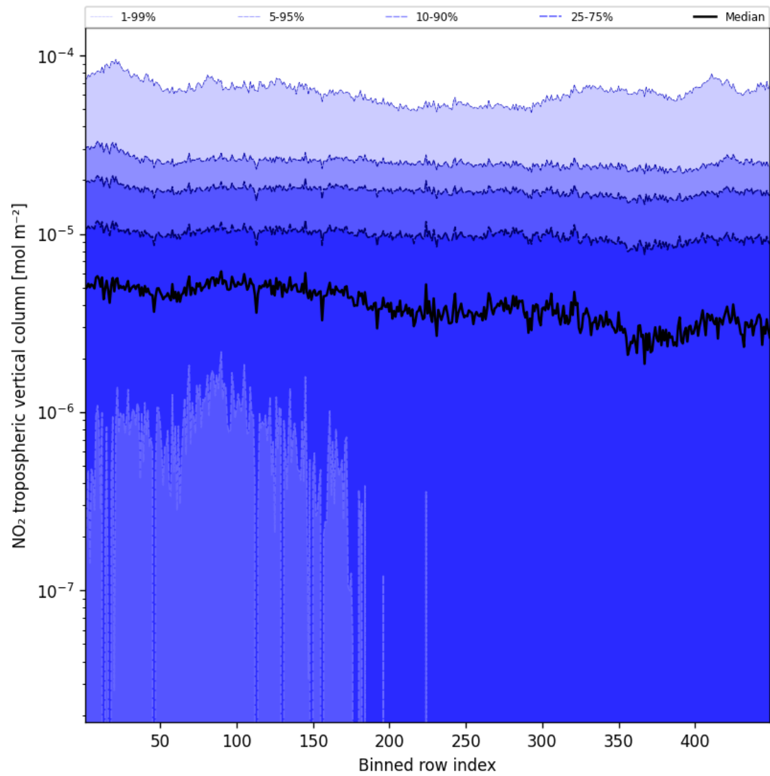
Figure 44: Along track statistics of “NO 2 tropospheric vertical column” for 2025-04-02 to 2025-04-03
