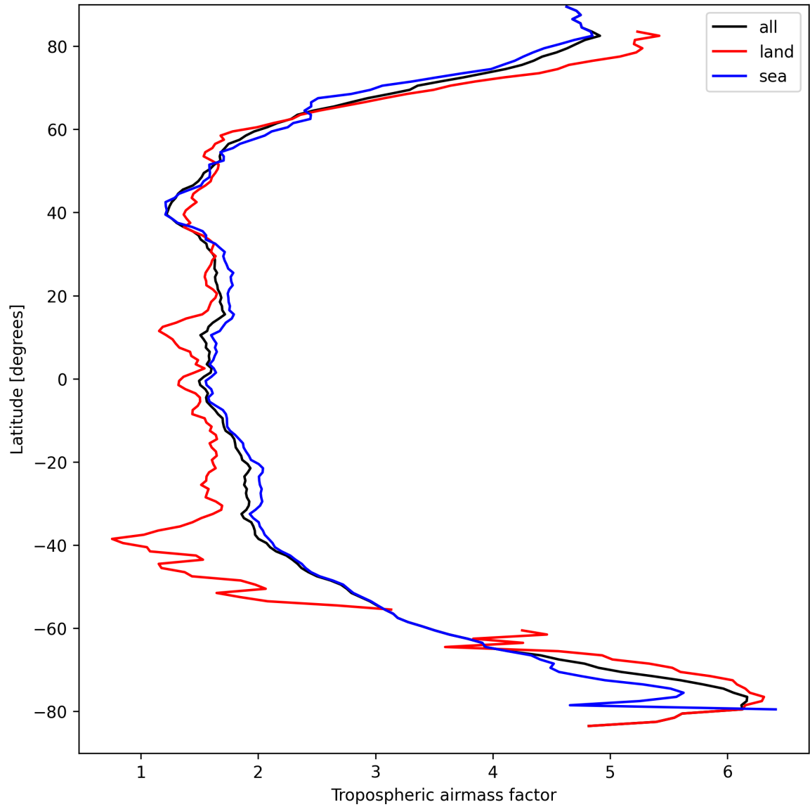
Figure 12: Zonal average of “Tropospheric air mass factor” for 2025-04-02 to 2025-04-03.
