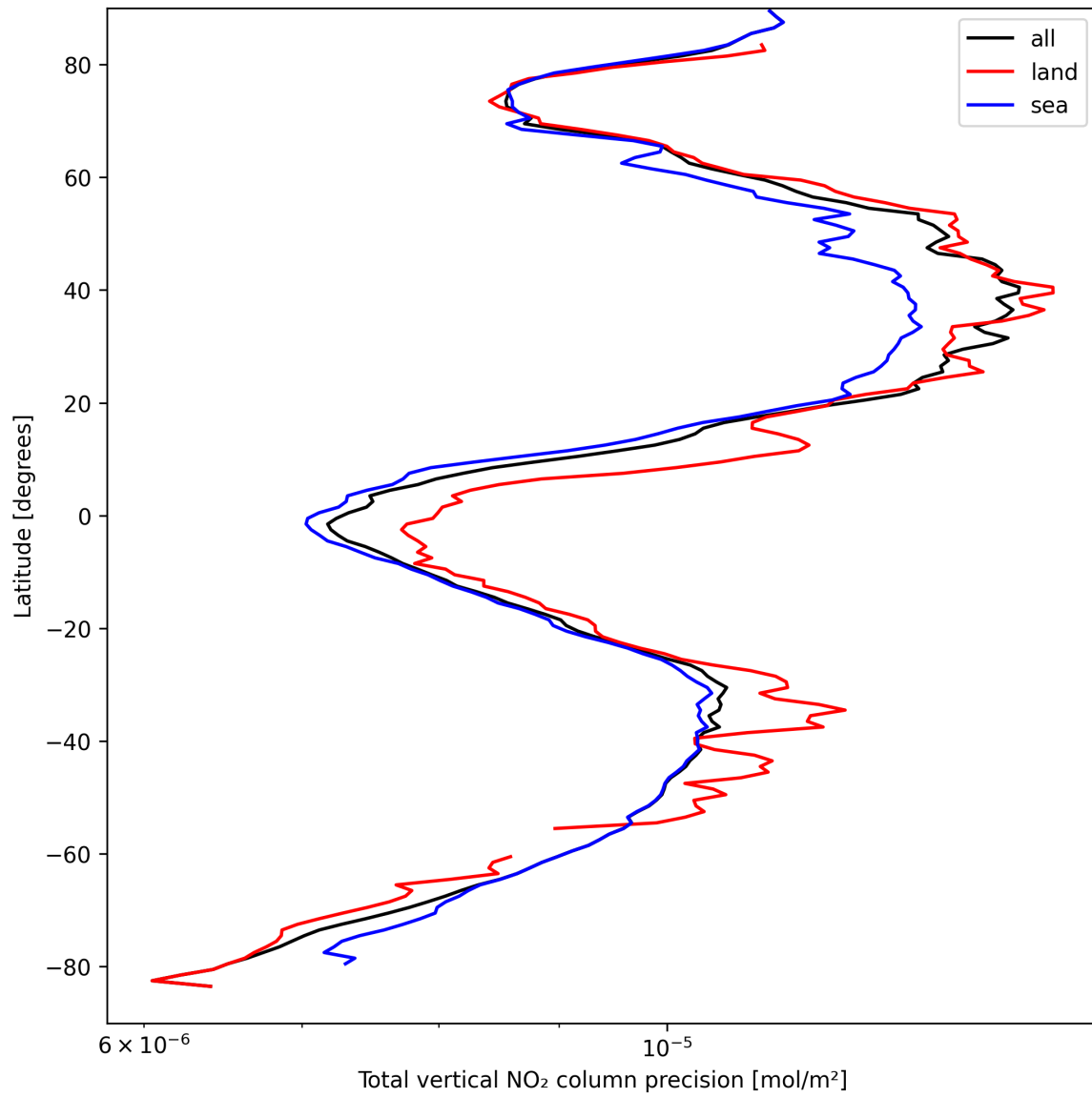
Figure 20: Zonal average of “Total vertical NO 2 column precision” for 2025-04-02 to 2025-04-03.
