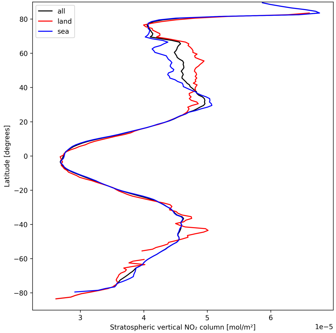
Figure 17: Zonal average of “Stratospheric vertical NO 2 column” for 2025-04-02 to 2025-04-03.
