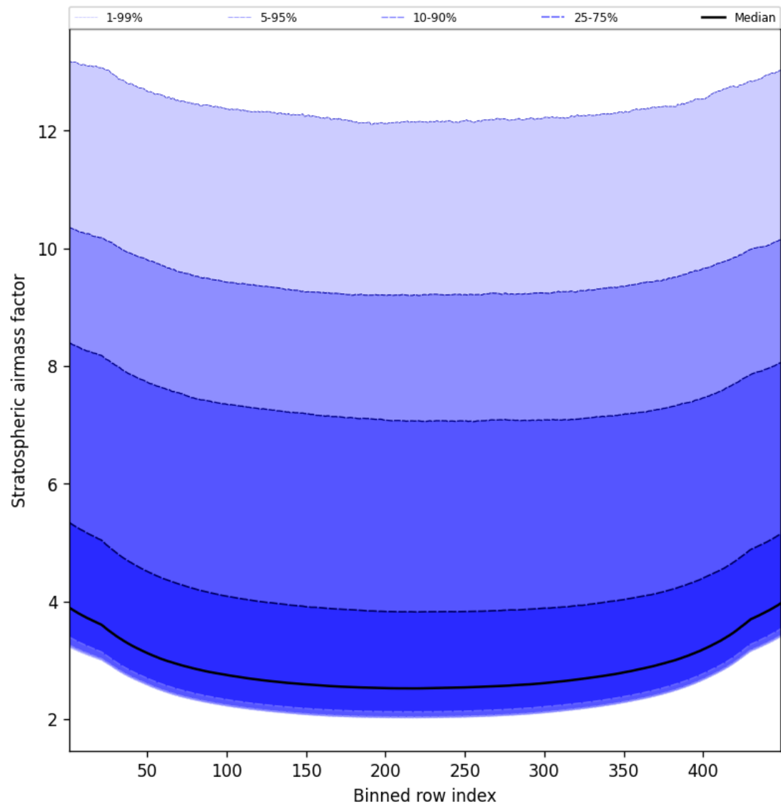
Figure 59: Along track statistics of “Stratospheric airmass factor” for 2025-04-02 to 2025-04-03
