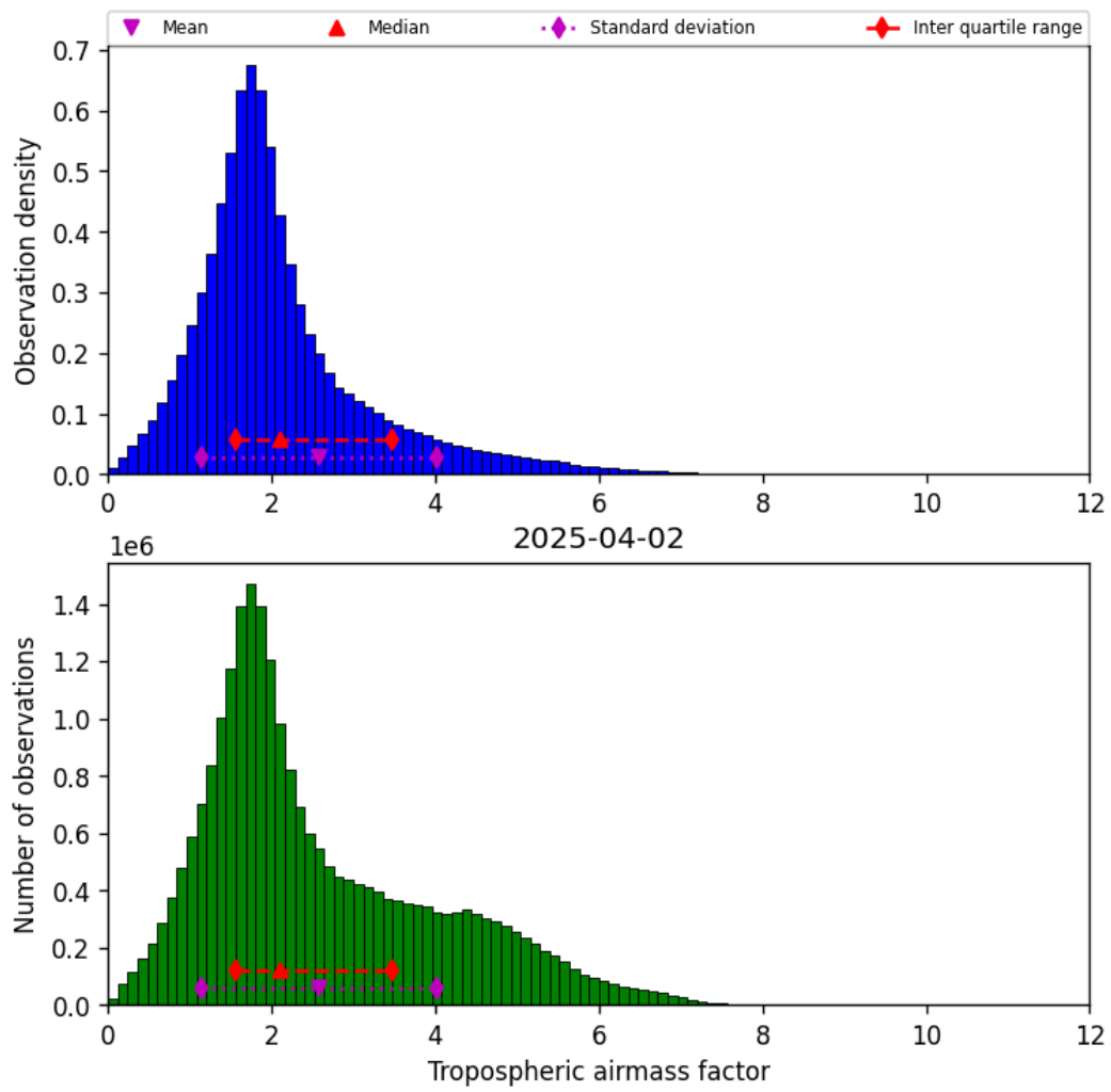
Figure 29: Histogram of “Tropospheric airmass factor” for 2025-04-02 to 2025-04-03
