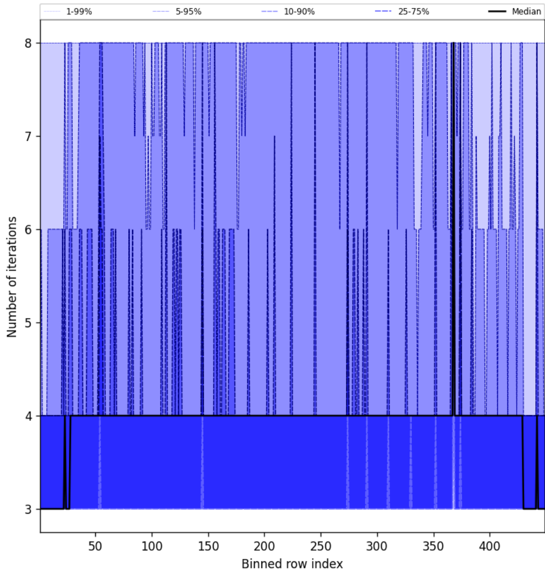
Figure 49: Along track statistics of “Number of iterations” for 2025-04-02 to 2025-04-03
