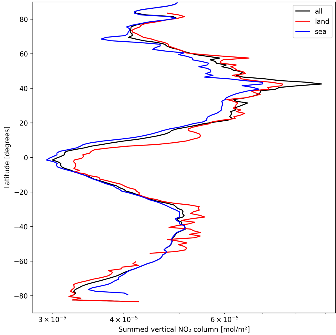
Figure 21: Zonal average of “Summed vertical NO 2 column” for 2025-04-02 to 2025-04-03.
