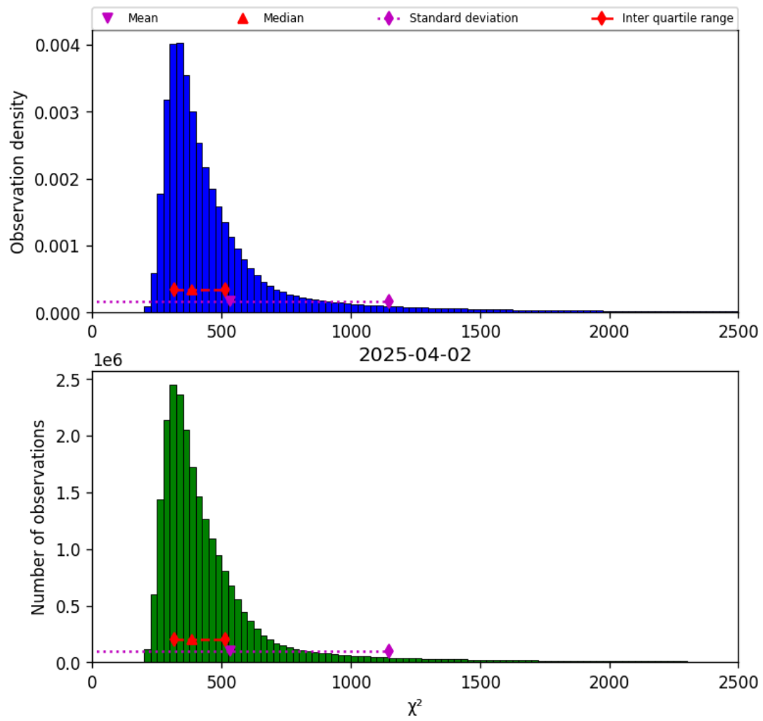
Figure 40: Histogram of “ \chi^2 ” for 2025-04-02 to 2025-04-03
