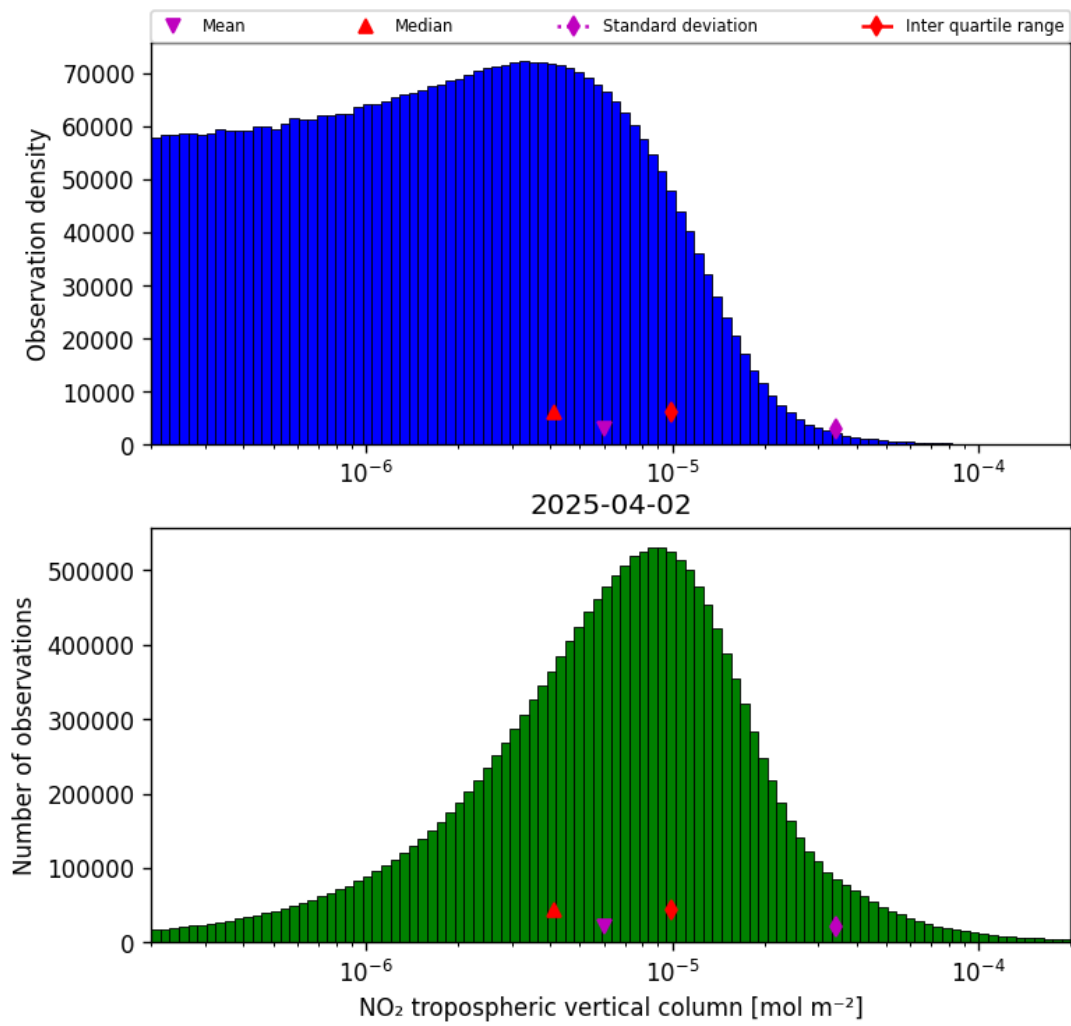
Figure 27: Histogram of “NO 2 tropospheric vertical column” for 2025-04-02 to 2025-04-03
