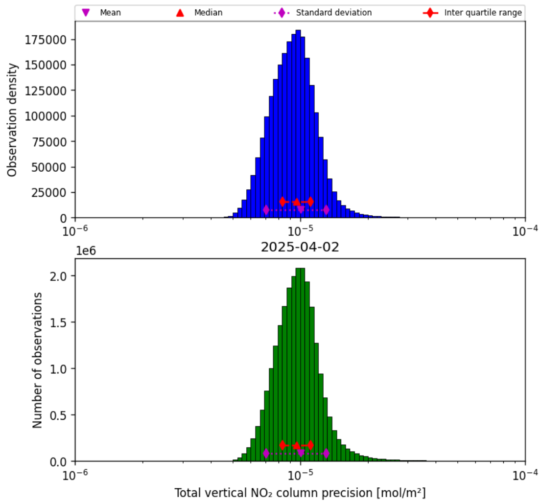
Figure 37: Histogram of “Total vertical NO 2 column precision” for 2025-04-02 to 2025-04-03
