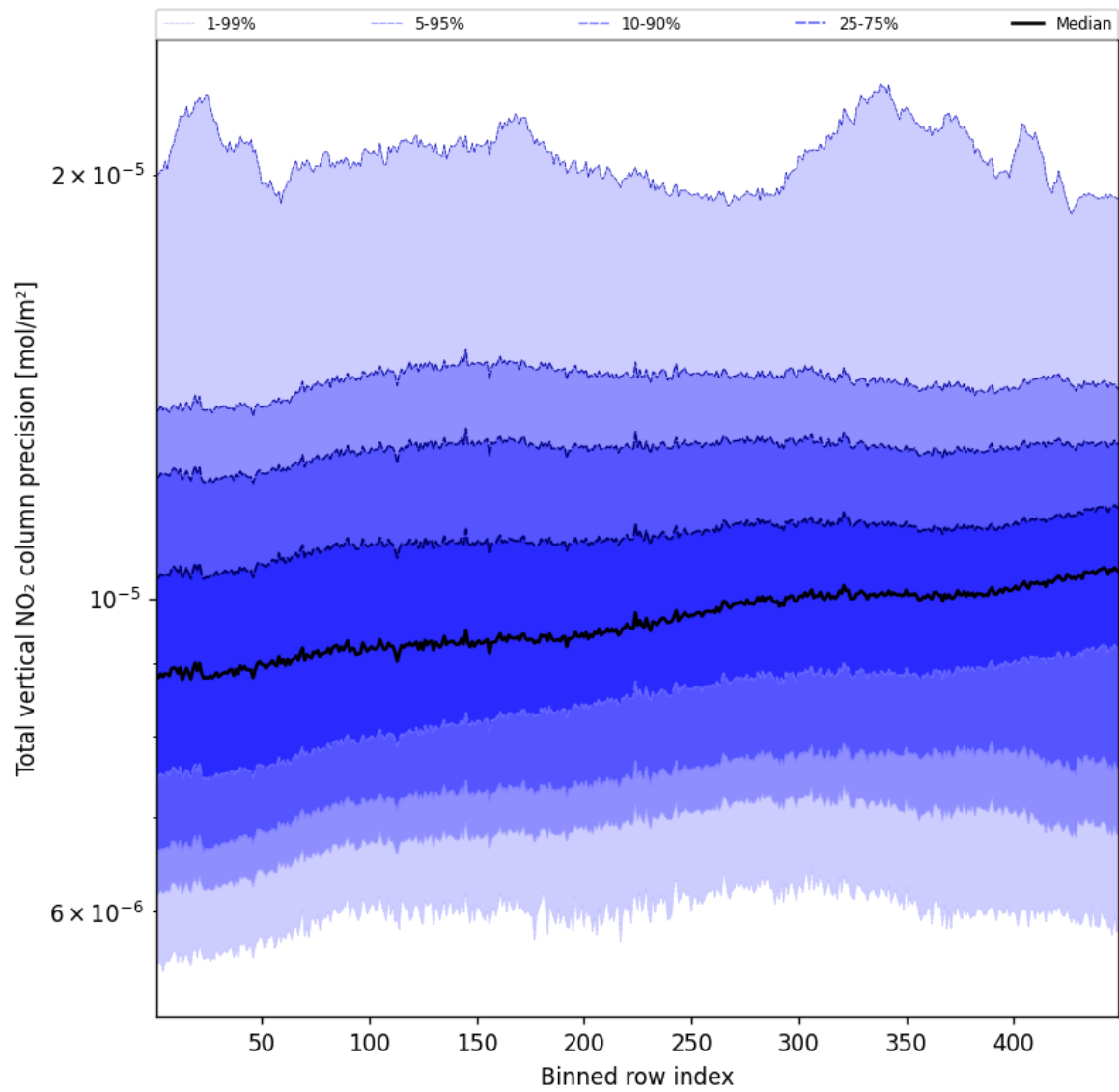
Figure 54: Along track statistics of “Total vertical NO 2 column precision” for 2025-04-02 to 2025-04-03
