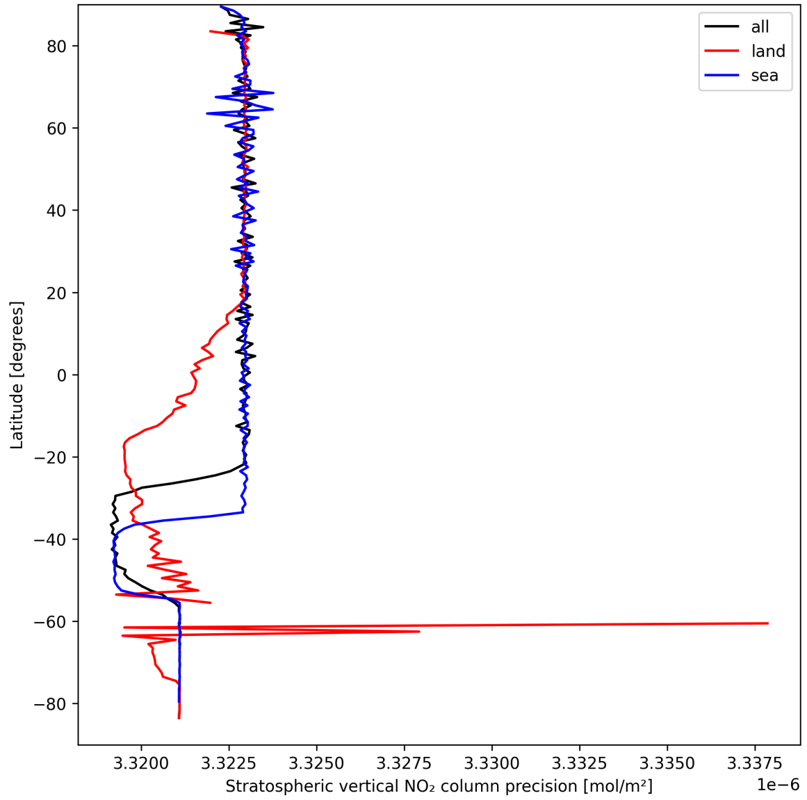
Figure 18: Zonal average of “Stratospheric vertical NO 2 column precision” for 2025-04-02 to 2025-04-03.
