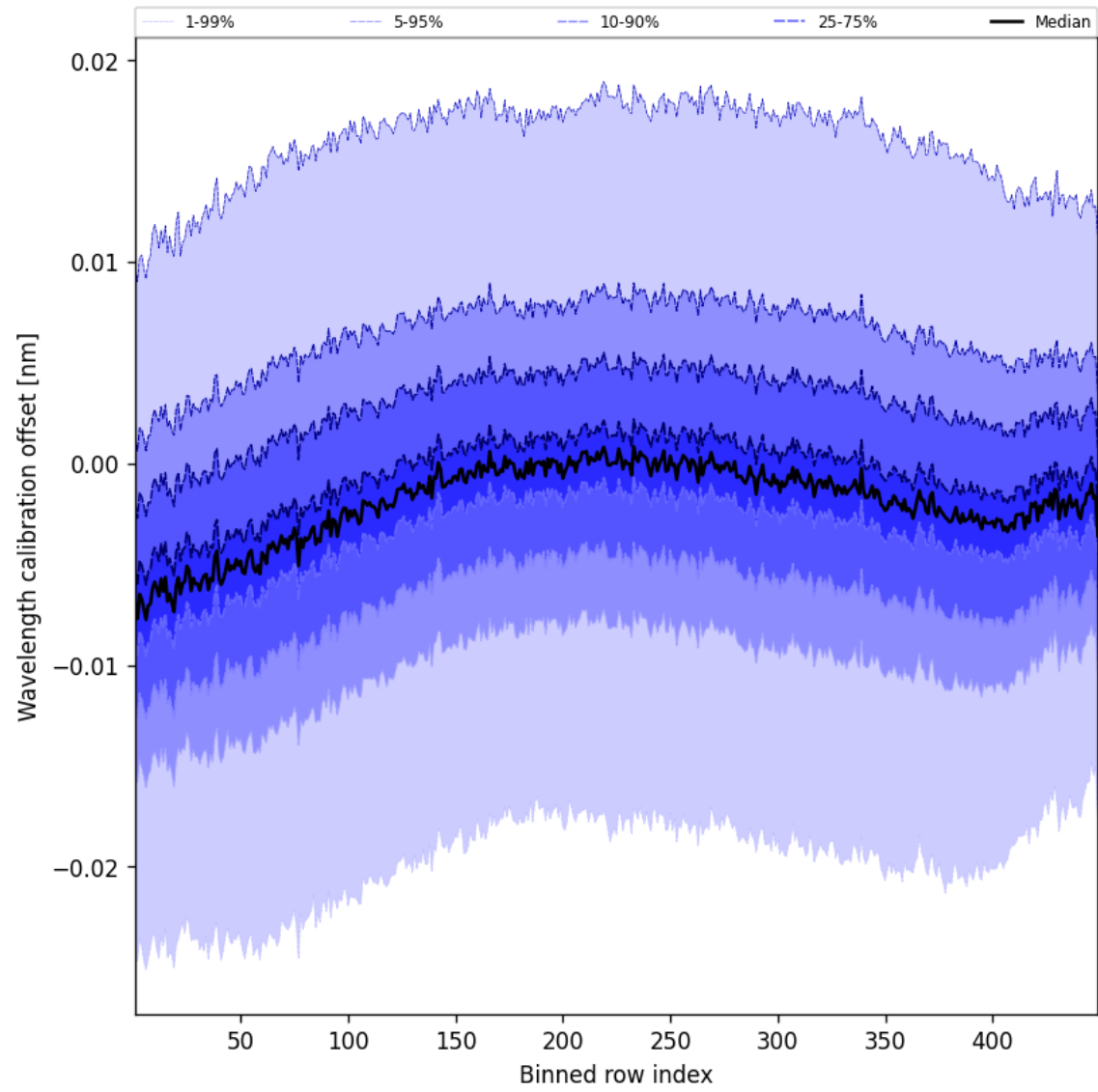
Figure 50: Along track statistics of “Wavelength calibration offset” for 2025-04-02 to 2025-04-03
