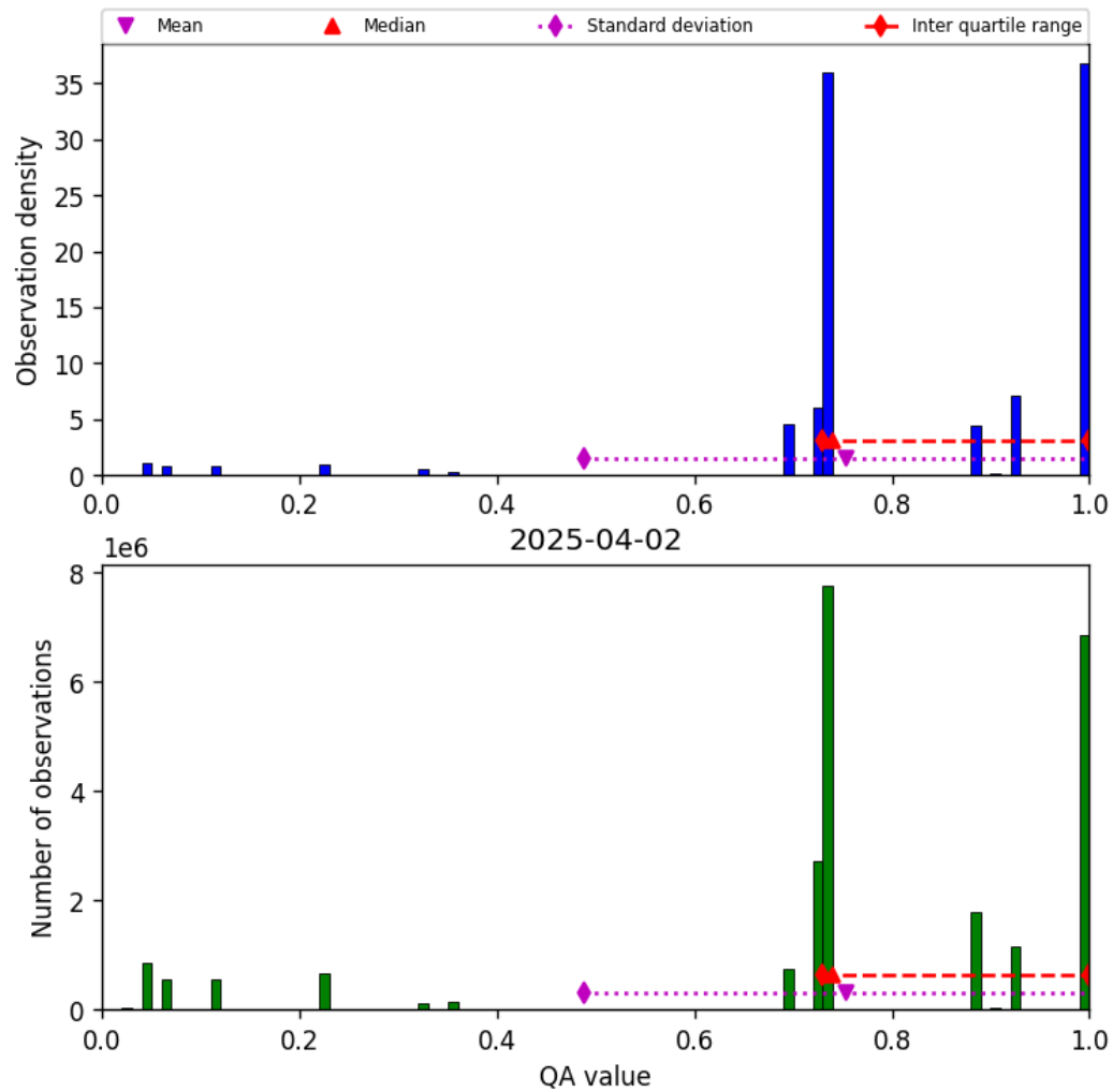
Figure 26: Histogram of “QA value” for 2025-04-02 to 2025-04-03
