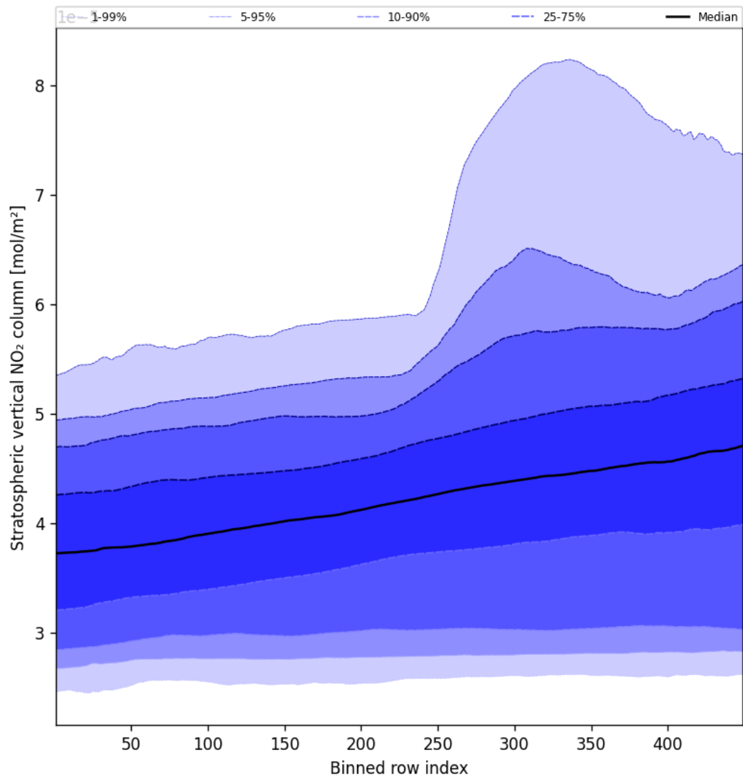
Figure 51: Along track statistics of “Stratospheric vertical NO 2 column” for 2025-04-02 to 2025-04-03
