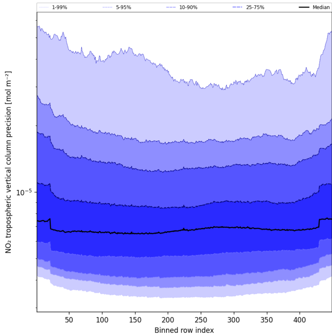
Figure 45: Along track statistics of “NO 2 tropospheric vertical column precision” for 2025-04-02 to 2025-04-03
