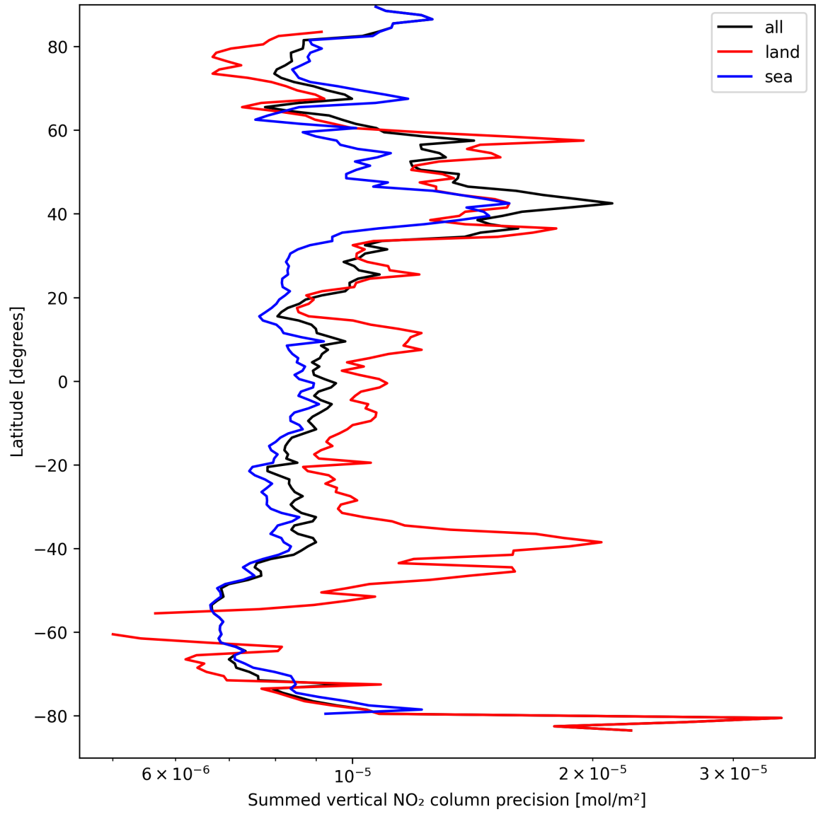
Figure 22: Zonal average of “Summed vertical NO 2 column precision” for 2025-04-02 to 2025-04-03.
