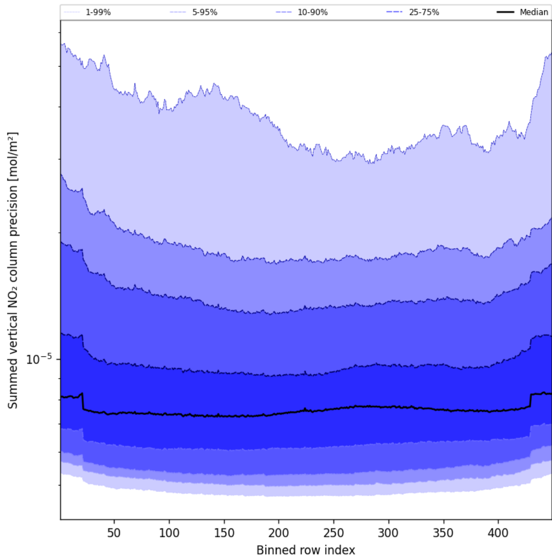
Figure 56: Along track statistics of “Summed vertical NO 2 column precision” for 2025-04-02 to 2025-04-03
