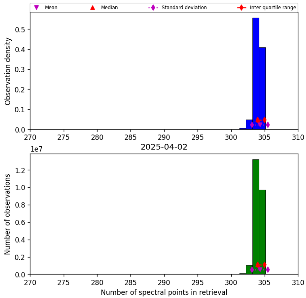
Figure 31: Histogram of “Number of spectral points in retrieval” for 2025-04-02 to 2025-04-03
