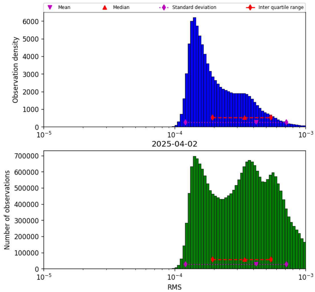
Figure 41: Histogram of “RMS” for 2025-04-02 to 2025-04-03
