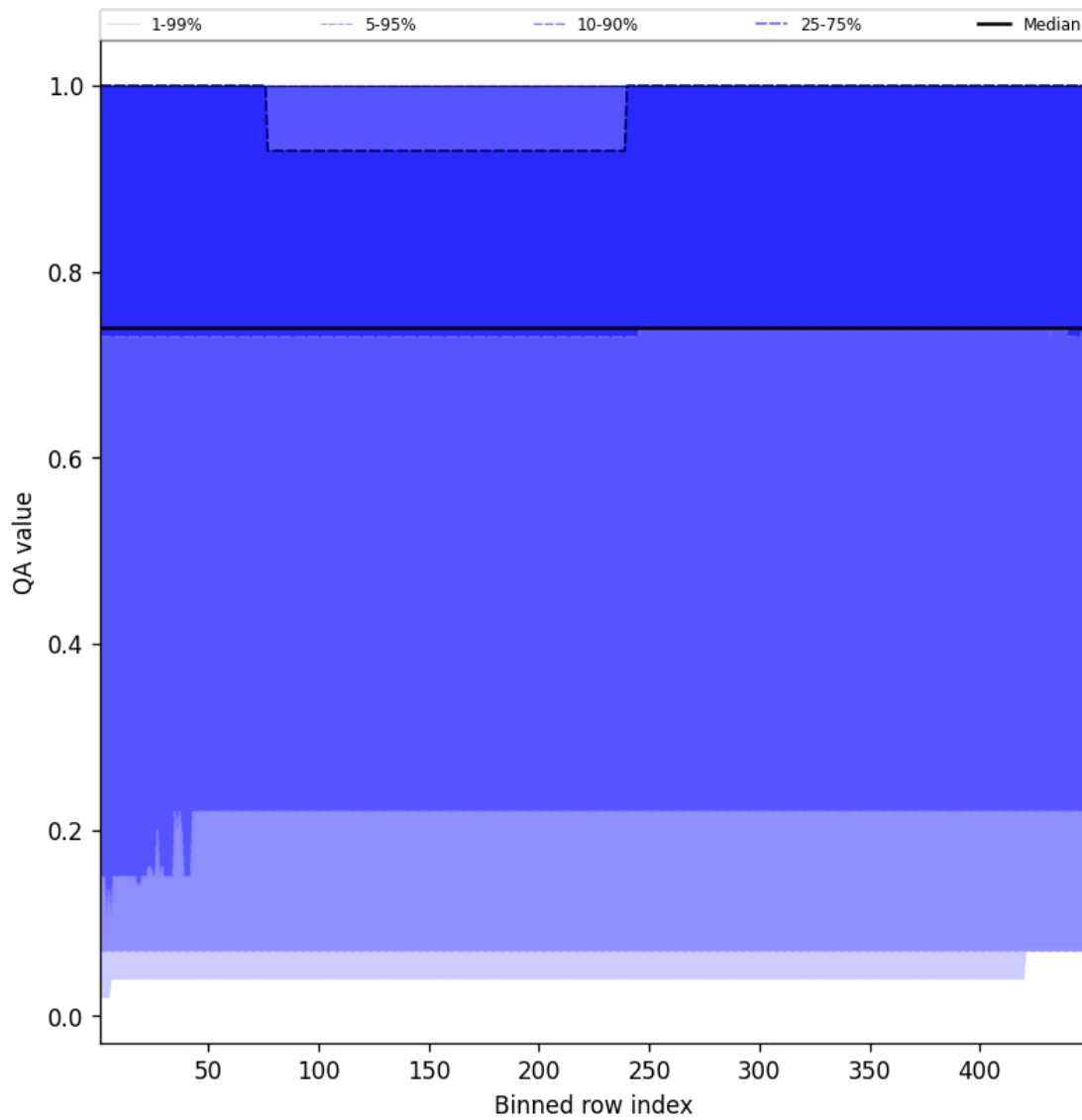
Figure 43: Along track statistics of "QA value" for 2025-04-02 to 2025-04-03
