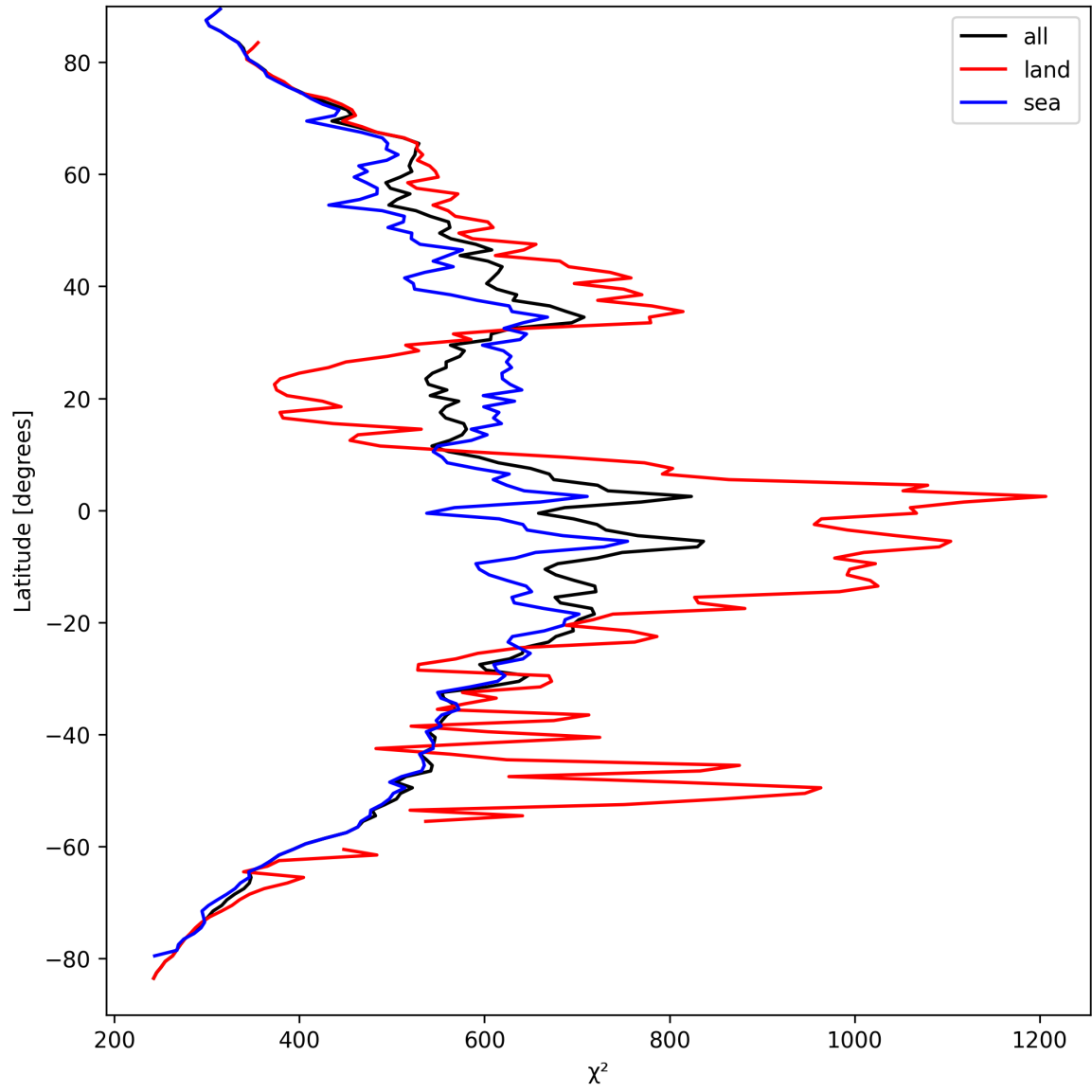
Figure 23: Zonal average of “ \chi^2 ” for 2025-04-02 to 2025-04-03.
