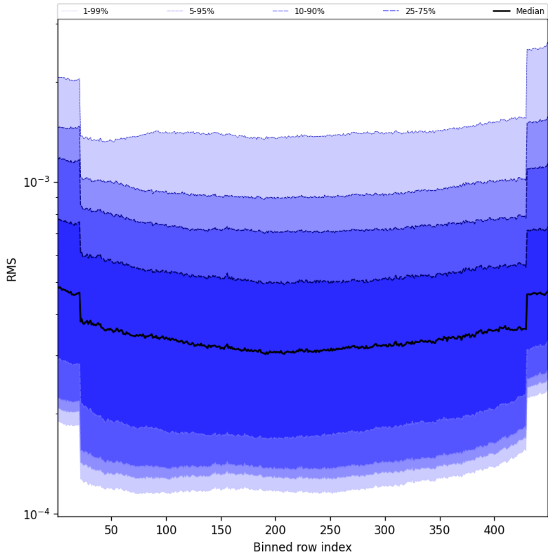
Figure 58: Along track statistics of “RMS” for 2025-04-02 to 2025-04-03
