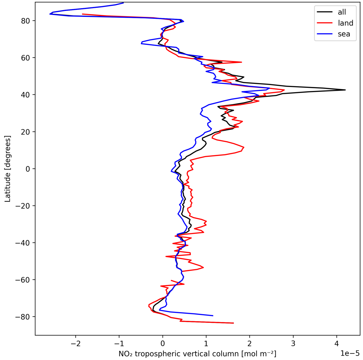
Figure 10: Zonal average of “NO 2 tropospheric vertical column” for 2025-04-02 to 2025-04-03.
