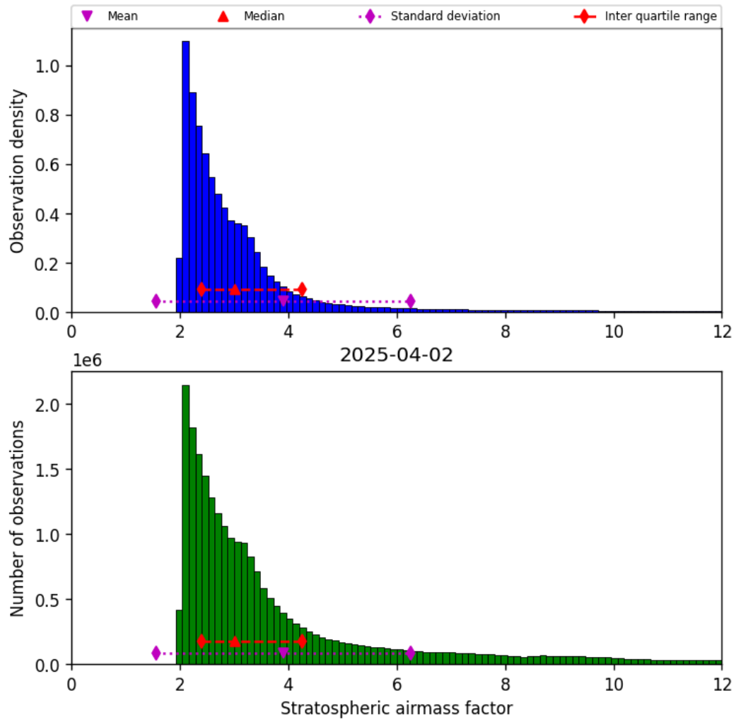
Figure 42: Histogram of “Stratospheric airmass factor” for 2025-04-02 to 2025-04-03
