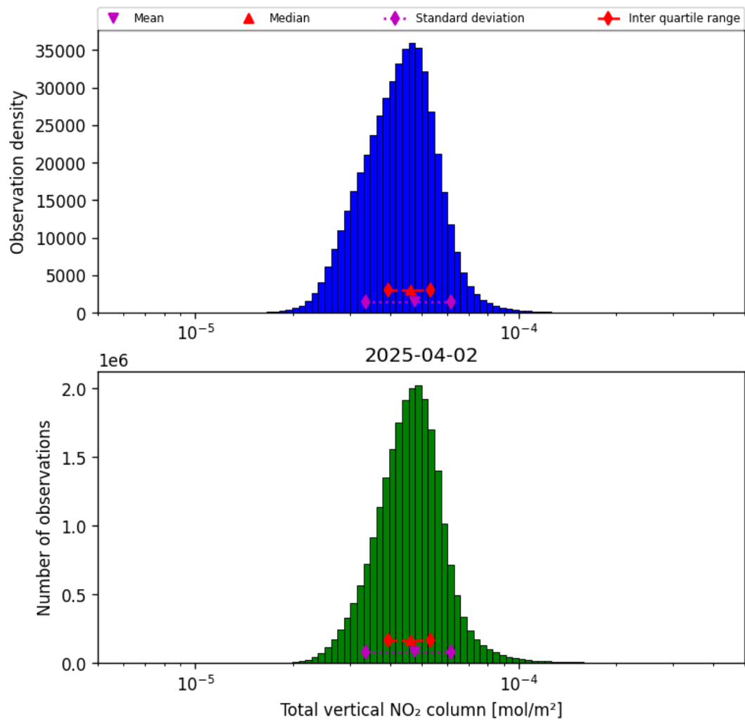
Figure 36: Histogram of “Total vertical NO 2 column” for 2025-04-02 to 2025-04-03
