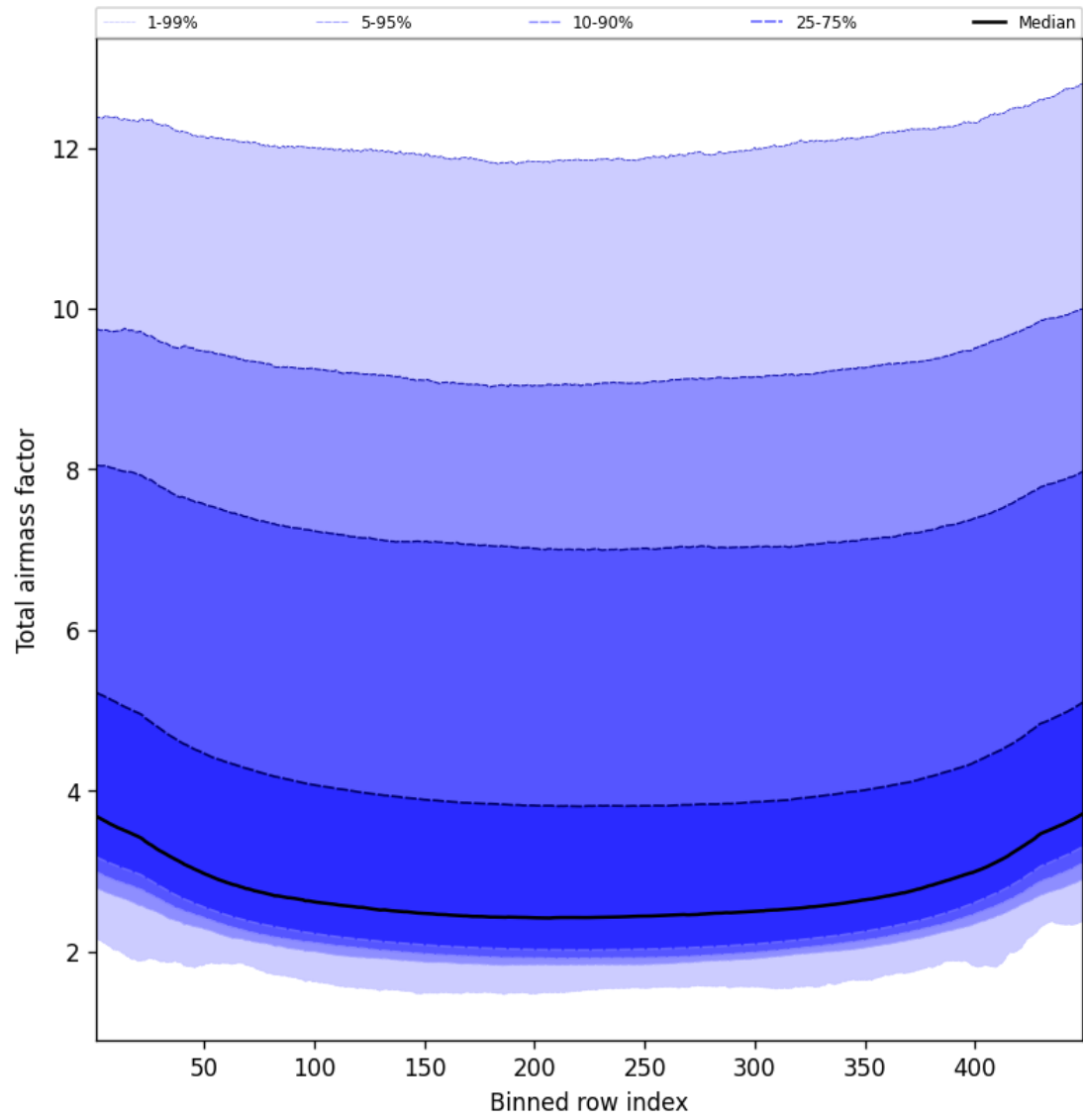
Figure 47: Along track statistics of “Total airmass factor” for 2025-04-02 to 2025-04-03
