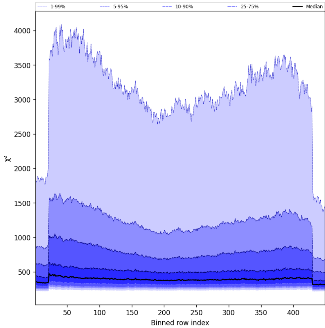
Figure 57: Along track statistics of “ \chi^2 ” for 2025-04-02 to 2025-04-03
