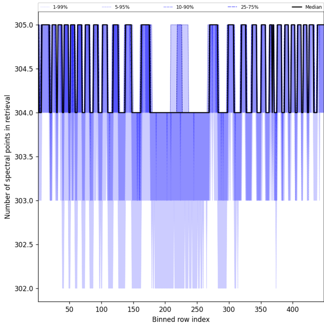
Figure 48: Along track statistics of “Number of spectral points in retrieval” for 2025-04-02 to 2025-04-03
