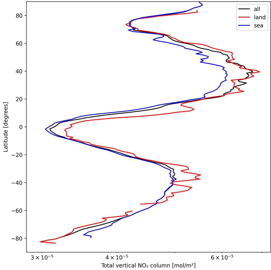
Figure 19: Zonal average of “Total vertical NO 2 column” for 2025-04-02 to 2025-04-03.
