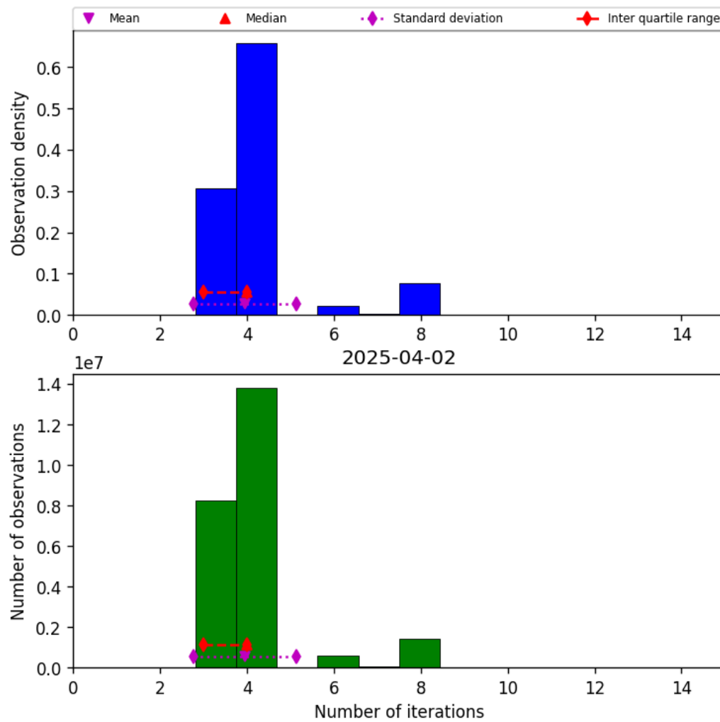
Figure 32: Histogram of “Number of iterations” for 2025-04-02 to 2025-04-03
