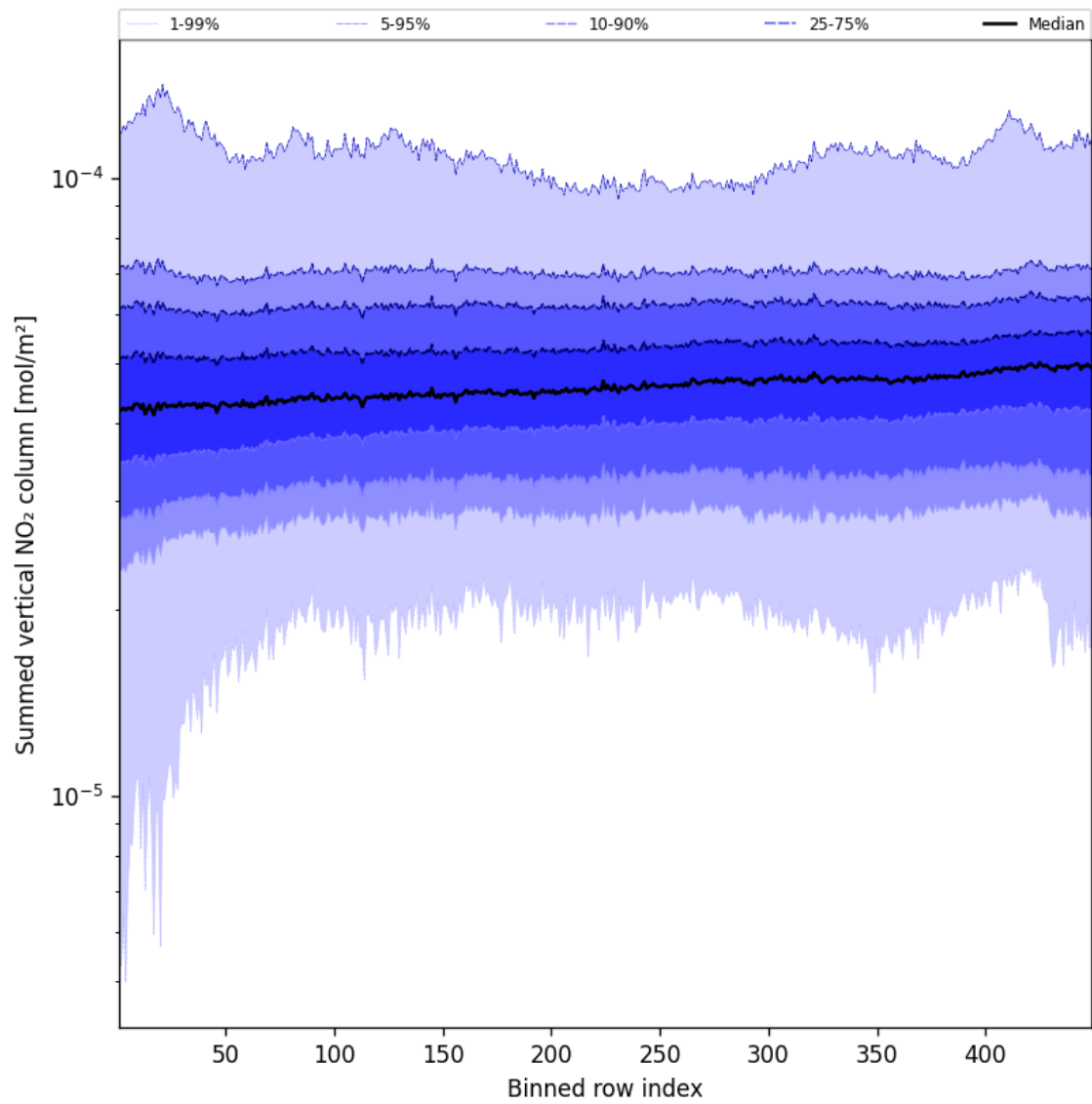
Figure 55: Along track statistics of “Summed vertical NO 2 column” for 2025-04-02 to 2025-04-03
