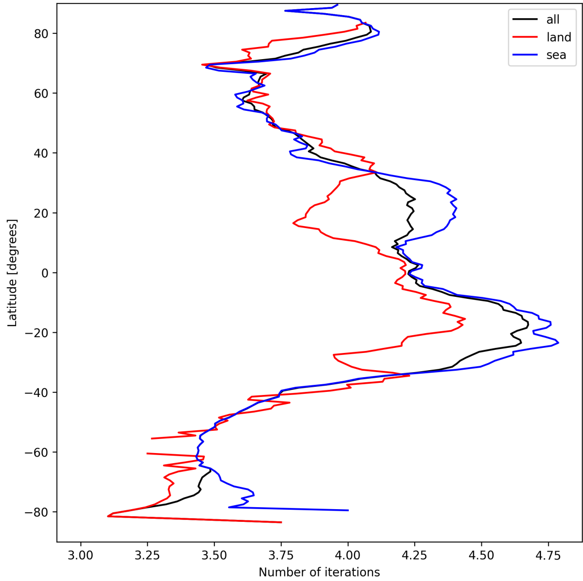
Figure 15: Zonal average of “Number of iterations” for 2025-04-02 to 2025-04-03.
