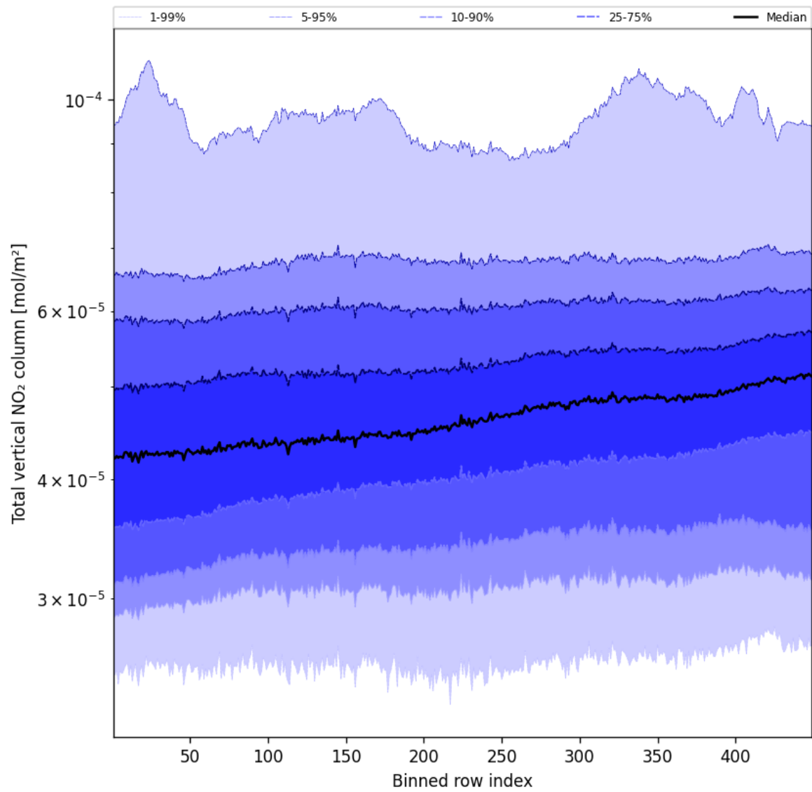
Figure 53: Along track statistics of “Total vertical NO 2 column” for 2025-04-02 to 2025-04-03
