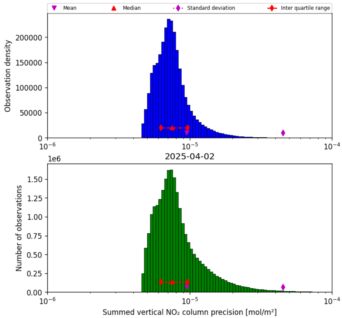
Figure 39: Histogram of “Summed vertical NO 2 column precision” for 2025-04-02 to 2025-04-03
