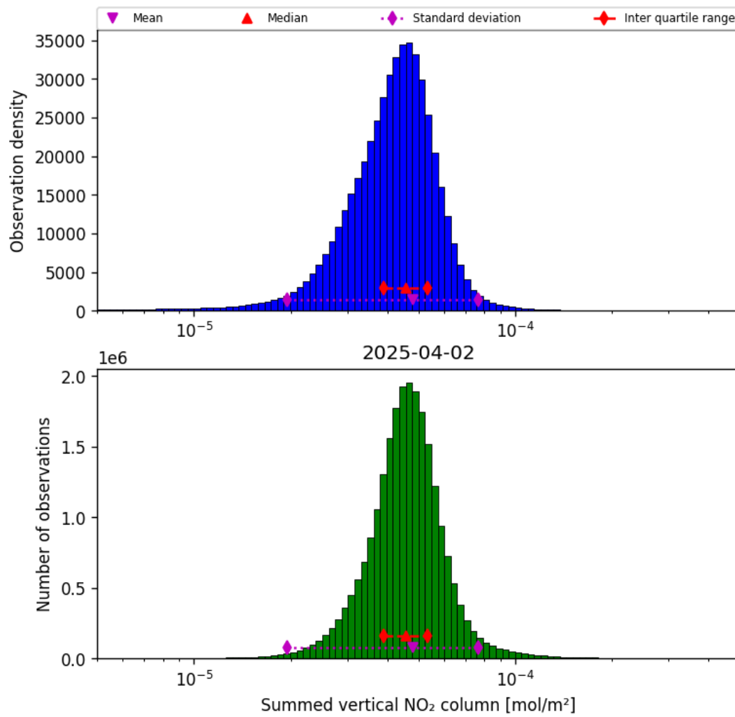
Figure 38: Histogram of “Summed vertical NO 2 column” for 2025-04-02 to 2025-04-03
