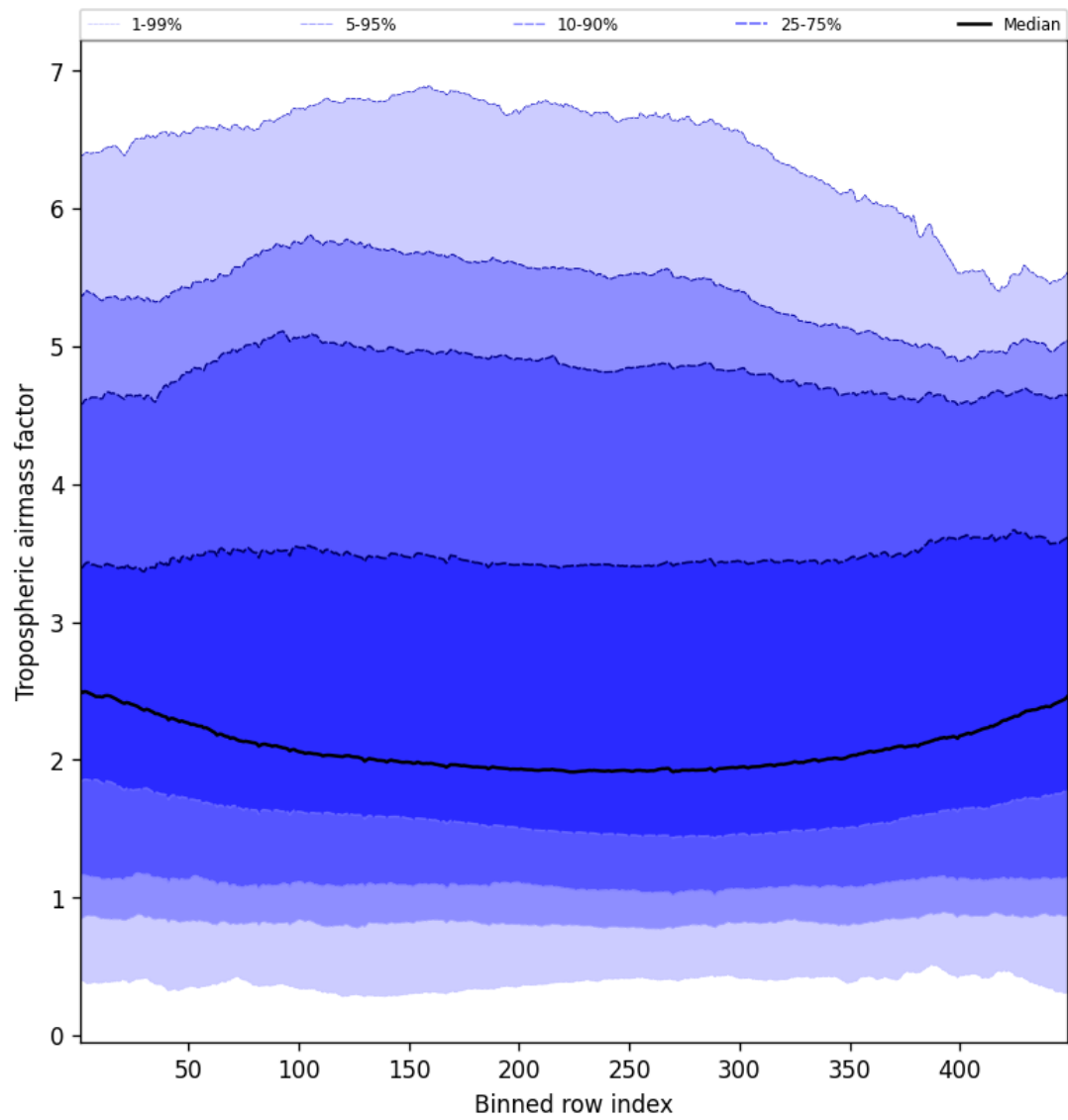
Figure 46: Along track statistics of “Tropospheric airmass factor” for 2025-04-02 to 2025-04-03
