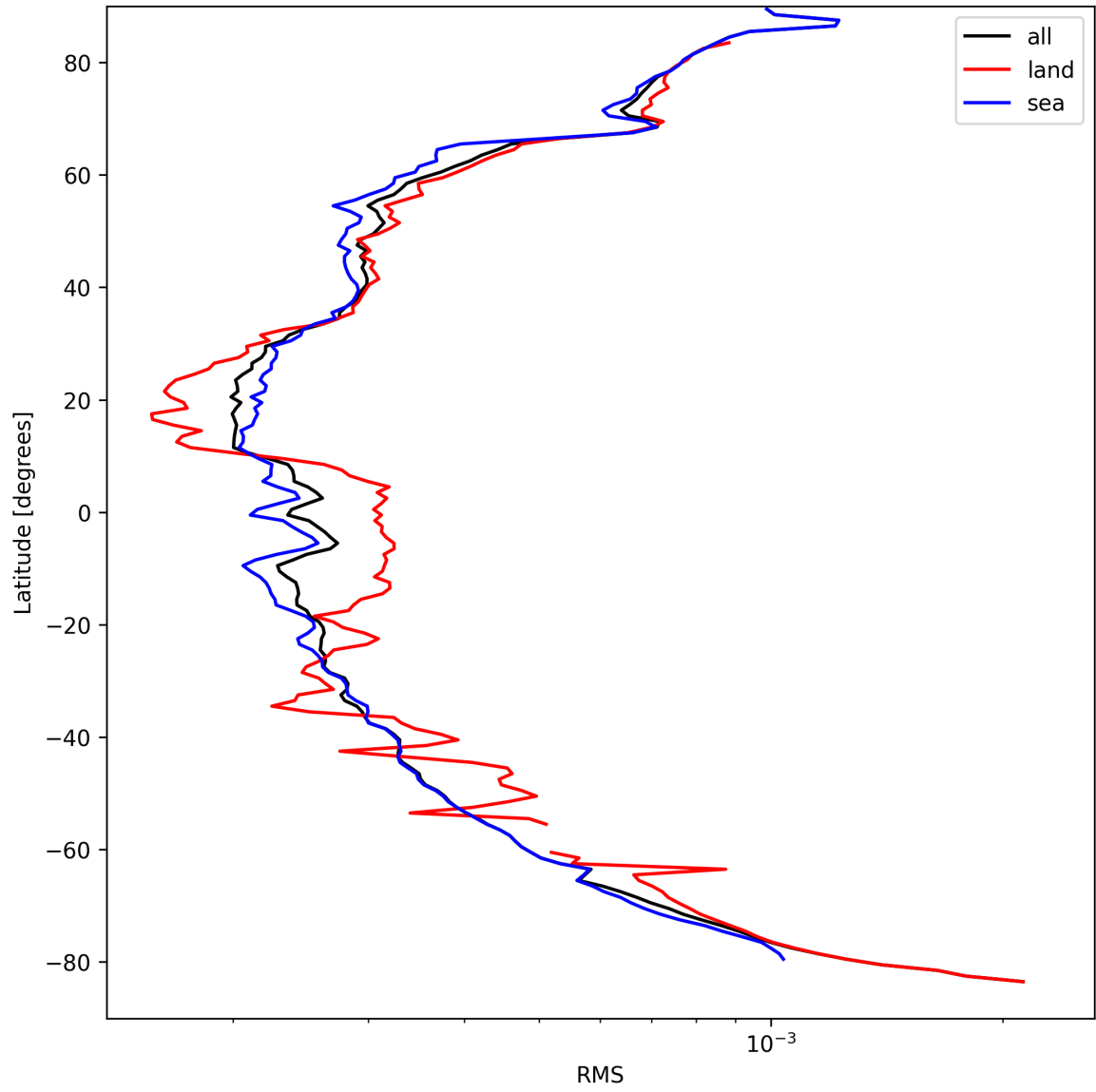
Figure 24: Zonal average of “RMS” for 2025-04-02 to 2025-04-03.
