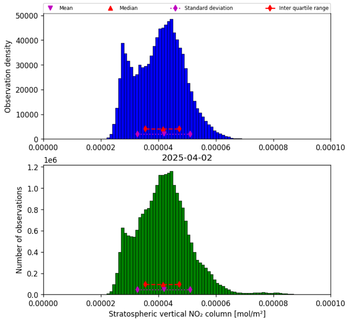
Figure 34: Histogram of “Stratospheric vertical NO 2 column” for 2025-04-02 to 2025-04-03
