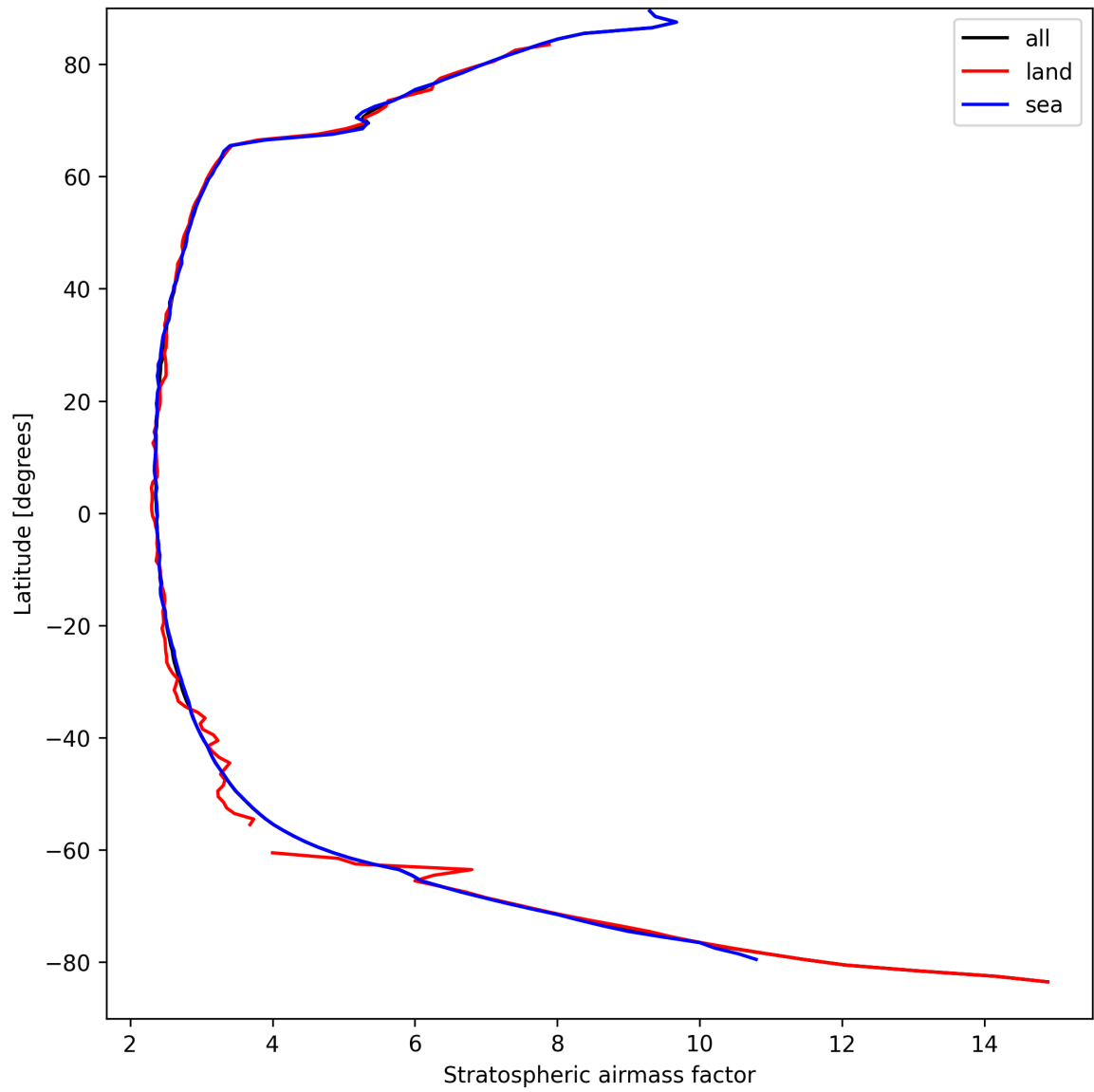
Figure 25: Zonal average of “Stratospheric airmass factor” for 2025-04-02 to 2025-04-03.
