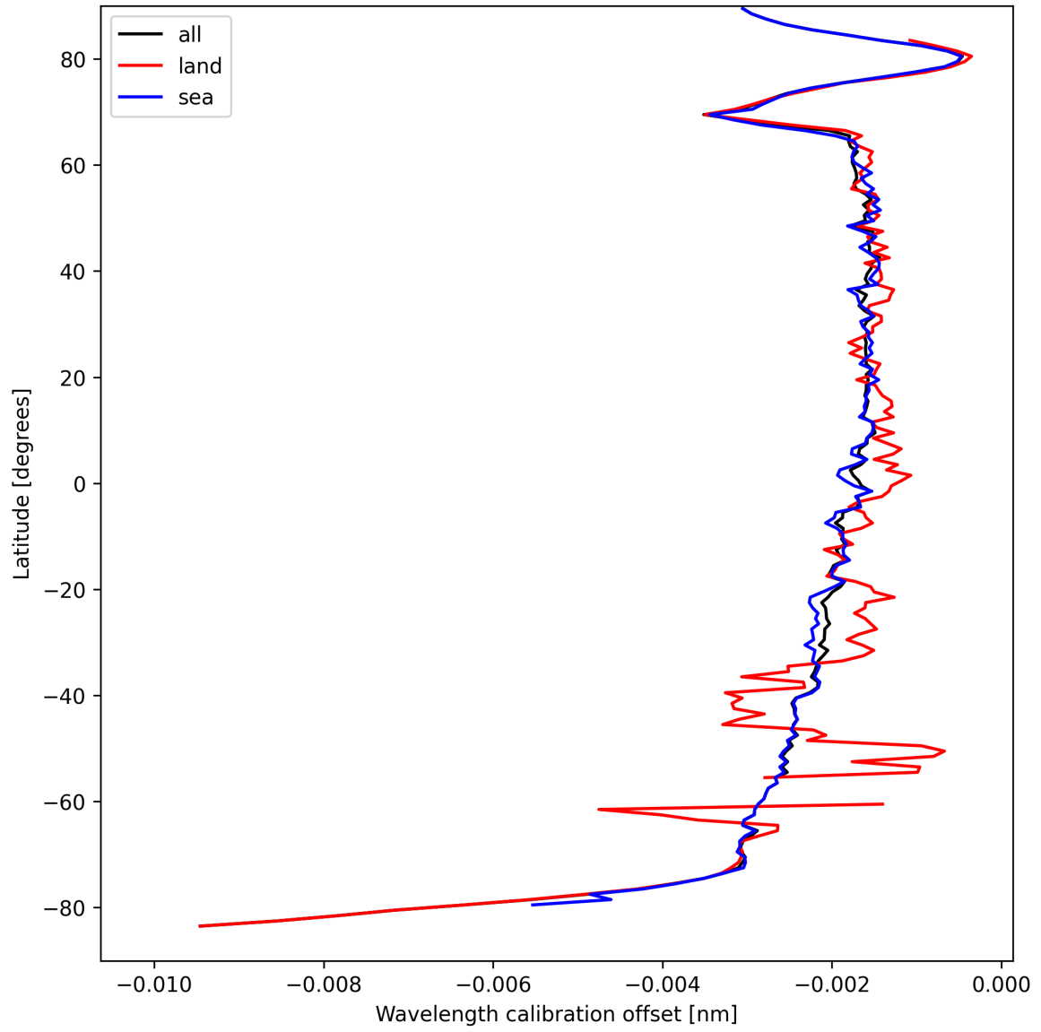
Figure 16: Zonal average of “Wavelength calibration offset” for 2025-04-02 to 2025-04-03.
