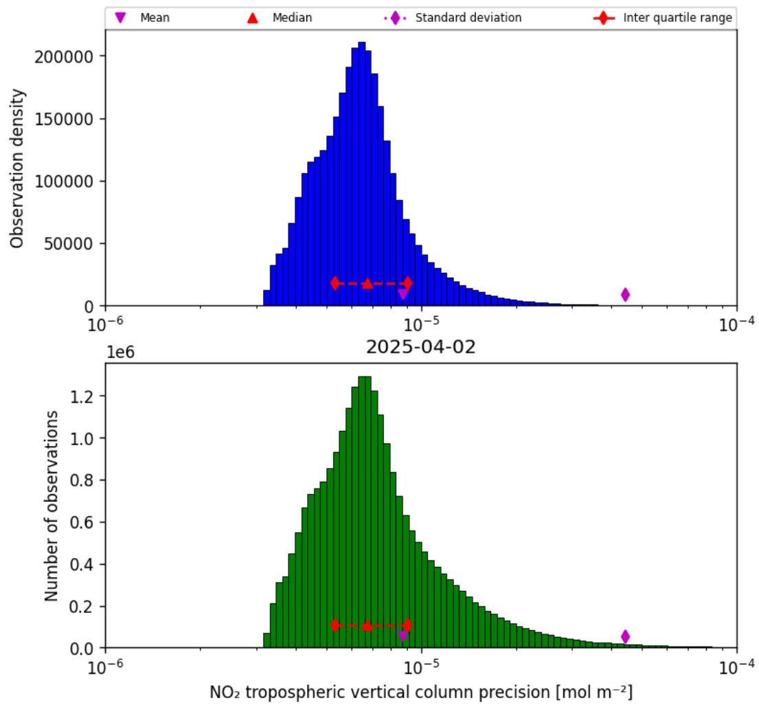
Figure 28: Histogram of “NO 2 tropospheric vertical column precision” for 2025-04-02 to 2025-04-03
