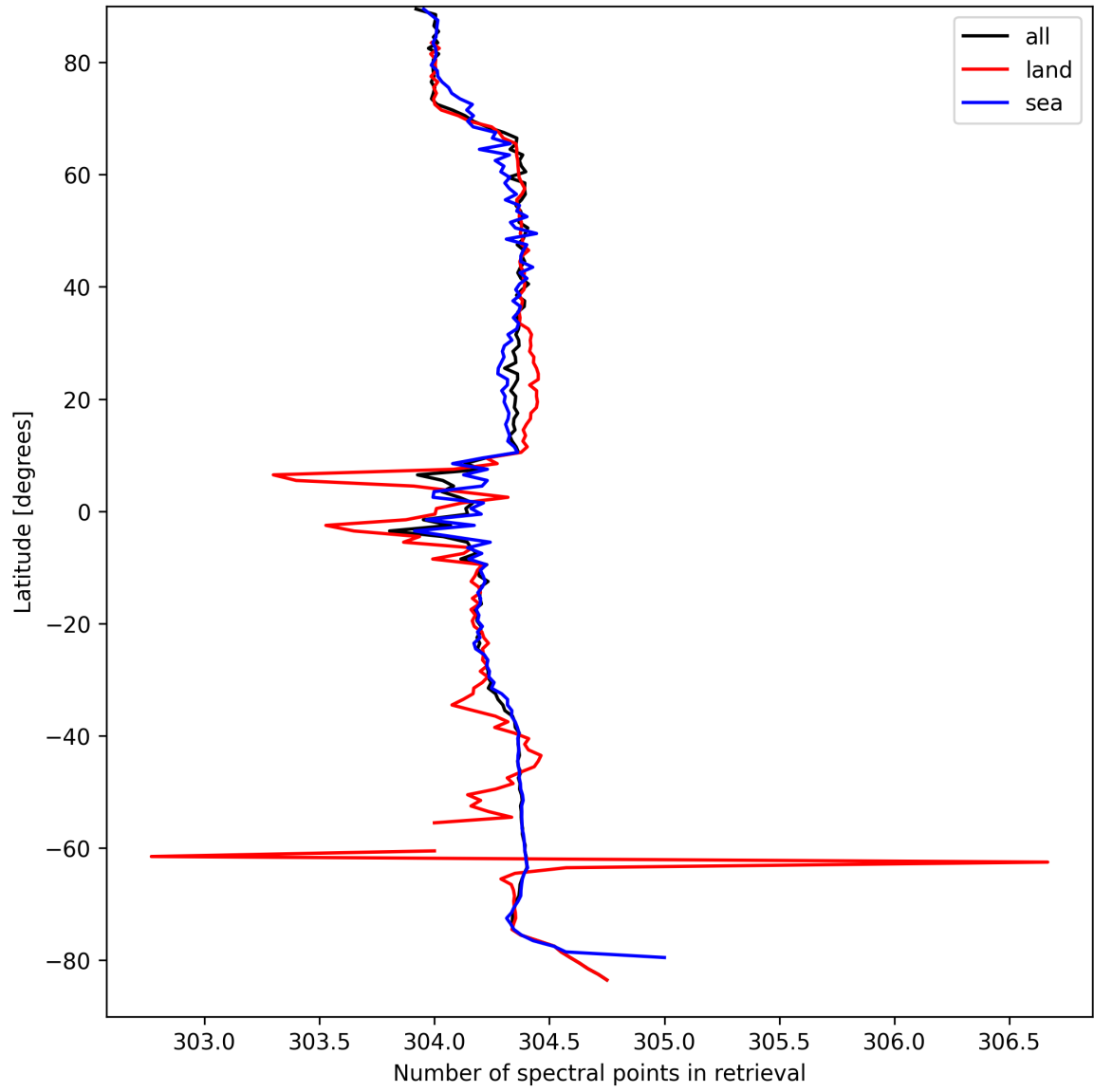
Figure 14: Zonal average of “Number of spectral points in retrieval” for 2025-04-02 to 2025-04-03.
