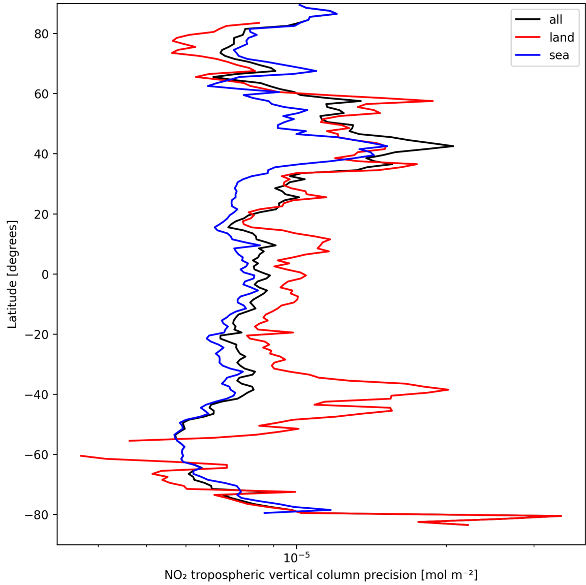
Figure 11: Zonal average of "NO 2 tropospheric vertical column precision" for 2025-04-02 to 2025-04-03.
