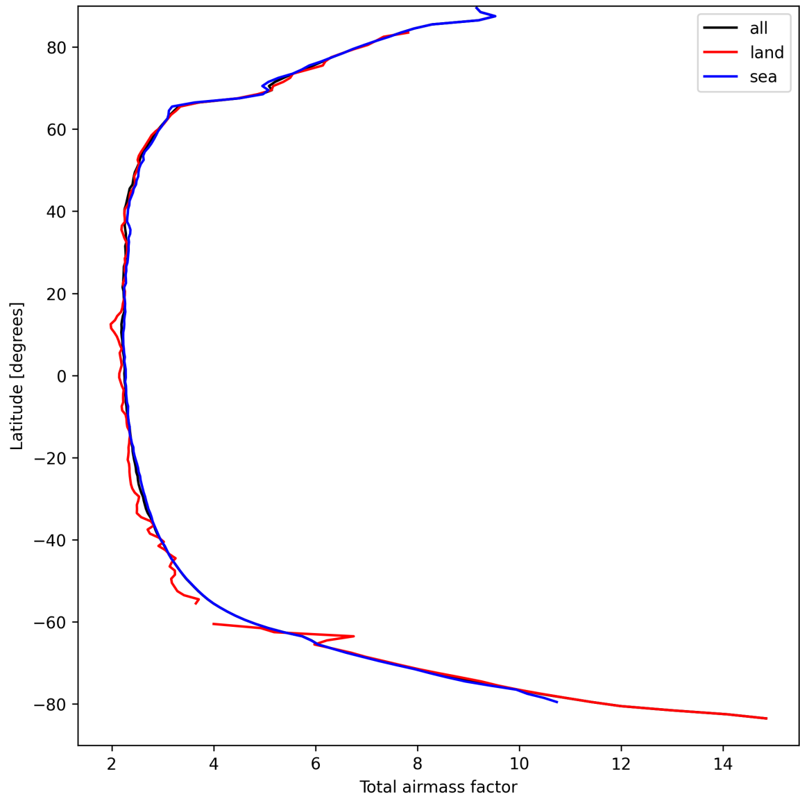
Figure 13: Zonal average of “Total airmass factor” for 2025-04-02 to 2025-04-03.
