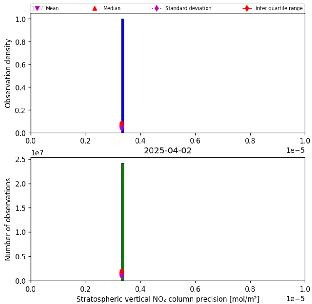
Figure 35: Histogram of “Stratospheric vertical NO 2 column precision” for 2025-04-02 to 2025-04-03
