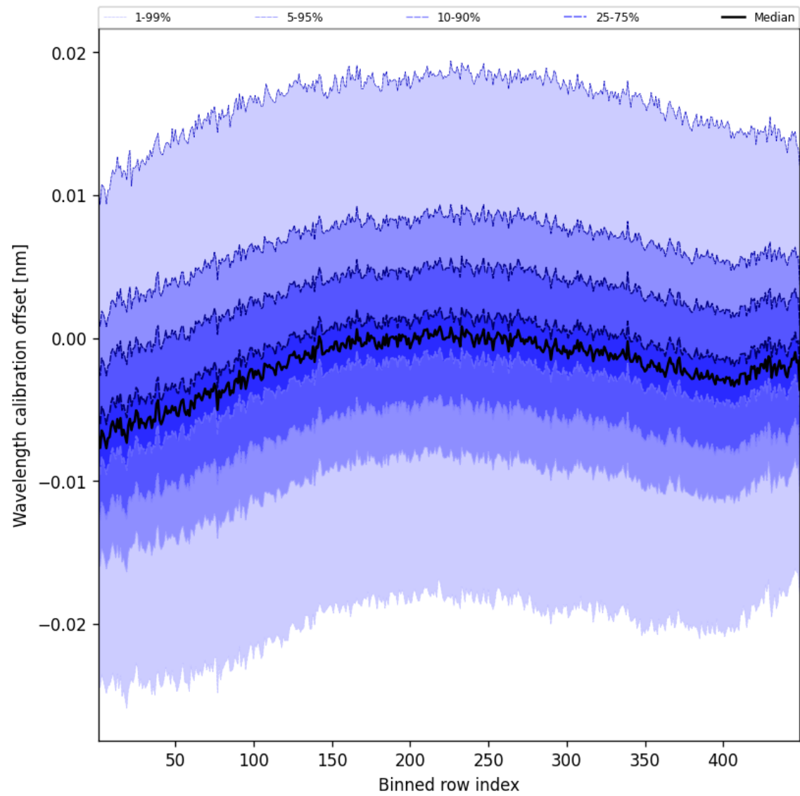
Figure 50: Along track statistics of “Wavelength calibration offset” for 2025-04-03 to 2025-04-04
