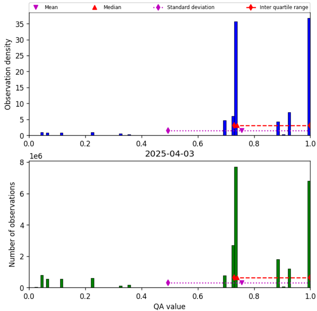
Figure 26: Histogram of “QA value” for 2025-04-03 to 2025-04-04
