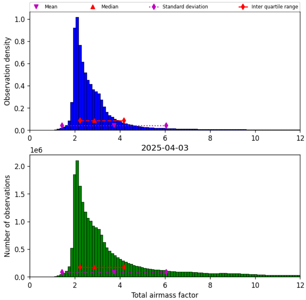
Figure 30: Histogram of “Total airmass factor” for 2025-04-03 to 2025-04-04
