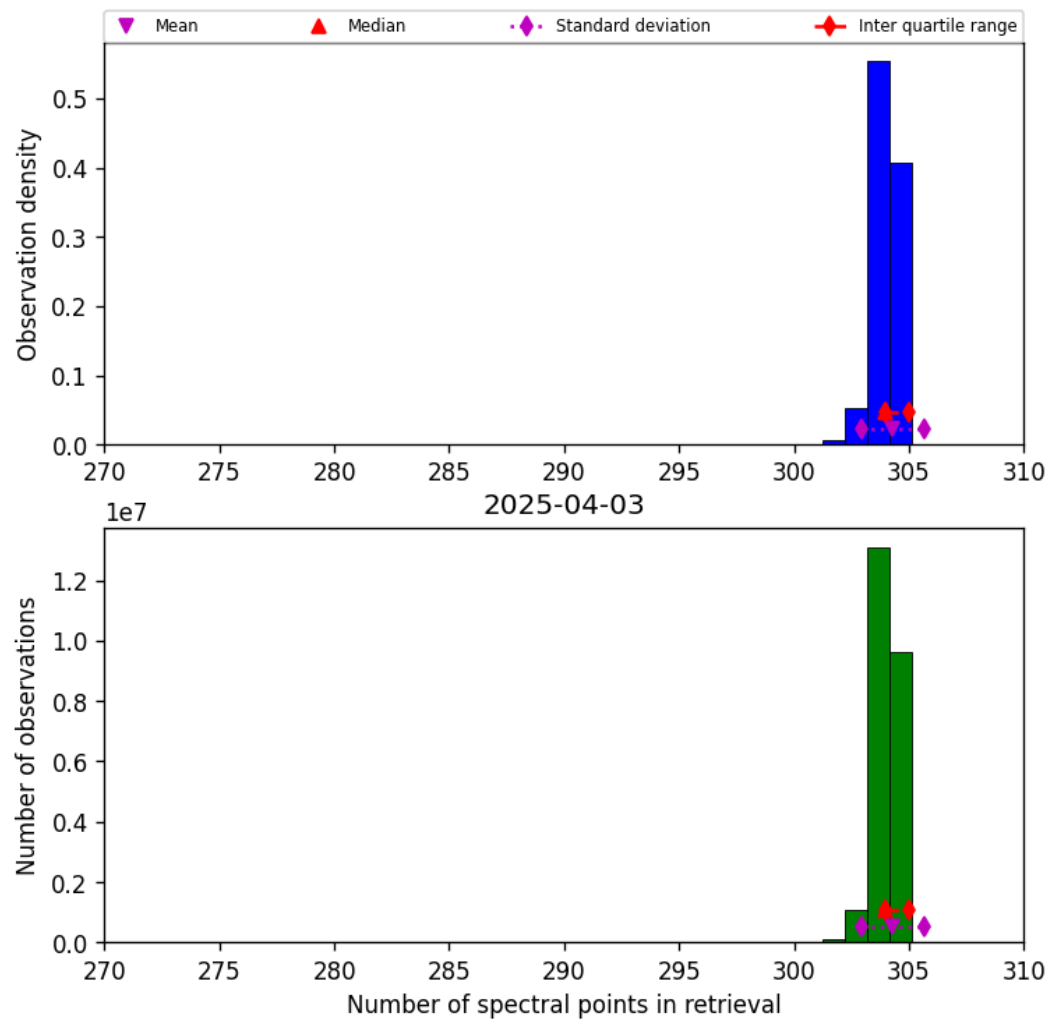
Figure 31: Histogram of “Number of spectral points in retrieval” for 2025-04-03 to 2025-04-04
