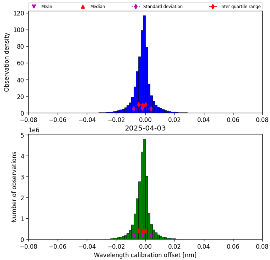
Figure 33: Histogram of “Wavelength calibration offset” for 2025-04-03 to 2025-04-04
