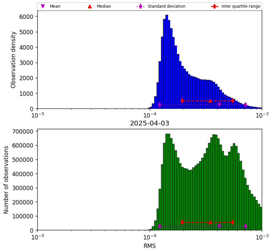
Figure 41: Histogram of “RMS” for 2025-04-03 to 2025-04-04
