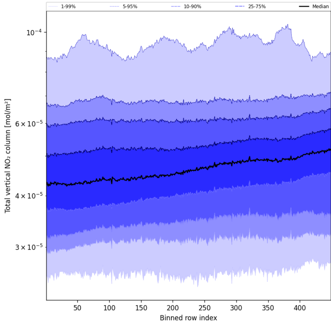
Figure 53: Along track statistics of “Total vertical NO 2 column” for 2025-04-03 to 2025-04-04
