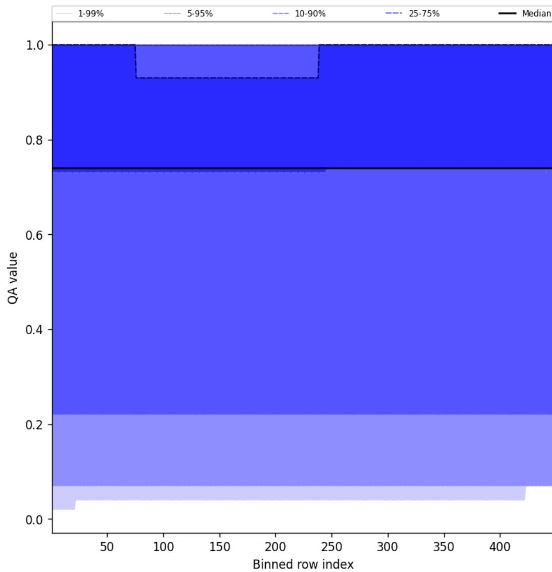
Figure 43: Along track statistics of “QA value” for 2025-04-03 to 2025-04-04
