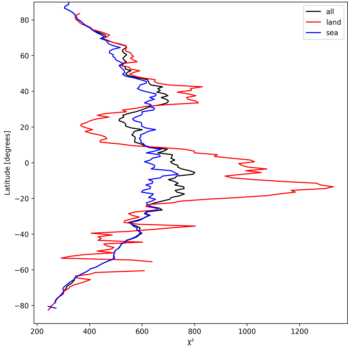
Figure 23: Zonal average of “ \chi^2 ” for 2025-04-03 to 2025-04-04.
