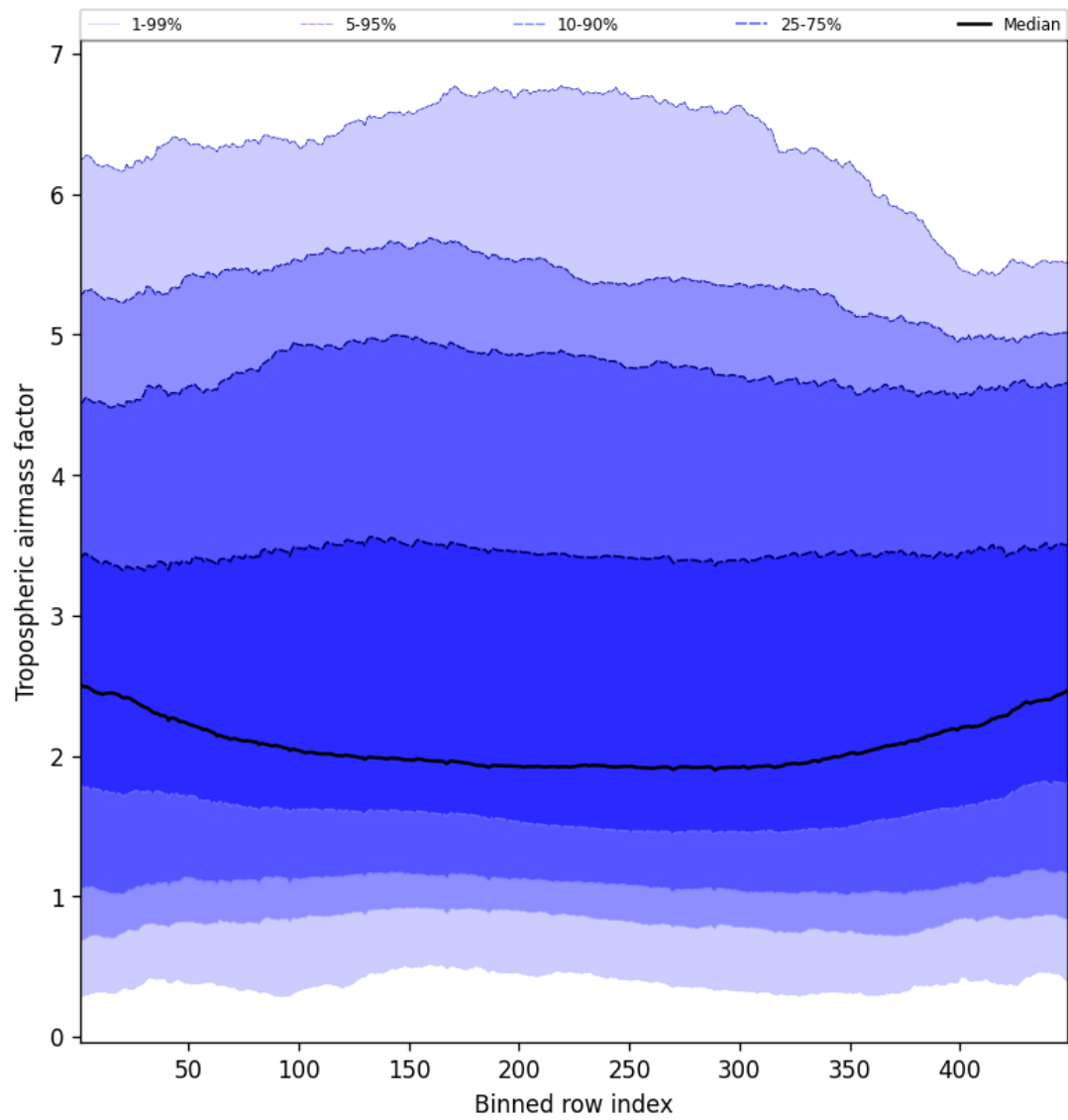
Figure 46: Along track statistics of “Tropospheric airmass factor” for 2025-04-03 to 2025-04-04
