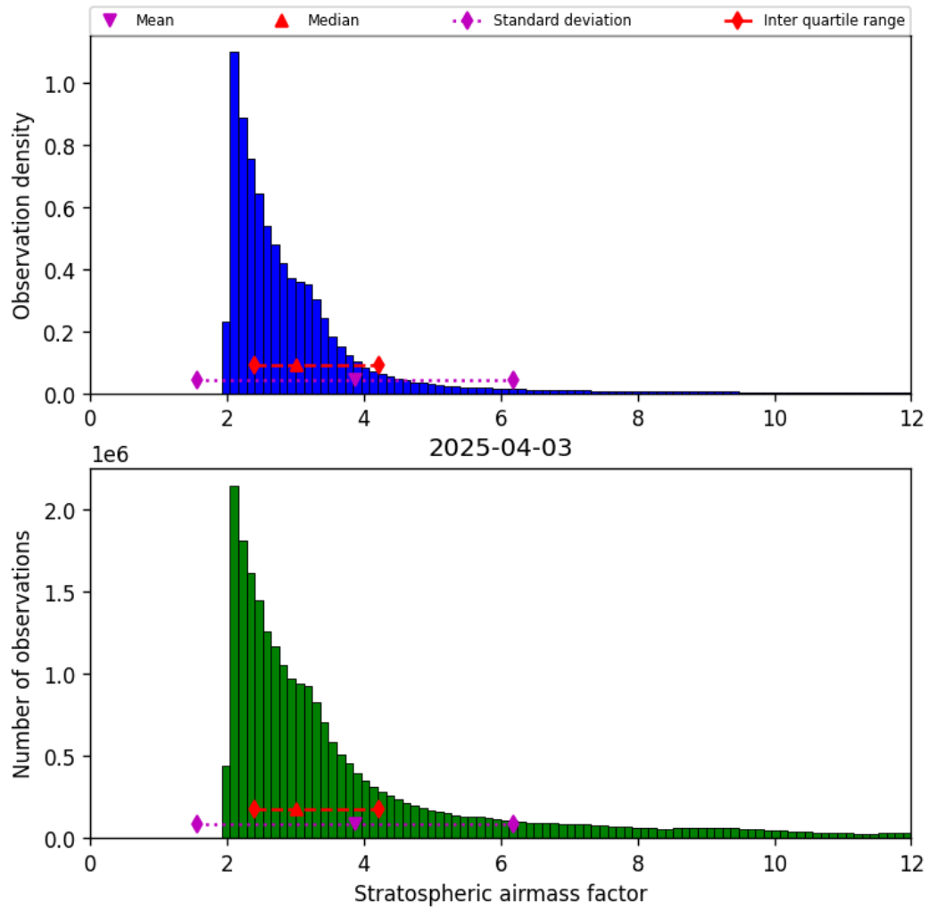
Figure 42: Histogram of "Stratospheric airmass factor" for 2025-04-03 to 2025-04-04
