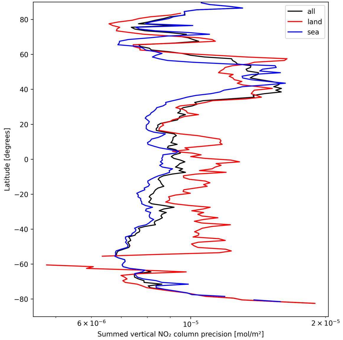
Figure 22: Zonal average of “Summed vertical NO 2 column precision” for 2025-04-03 to 2025-04-04.
