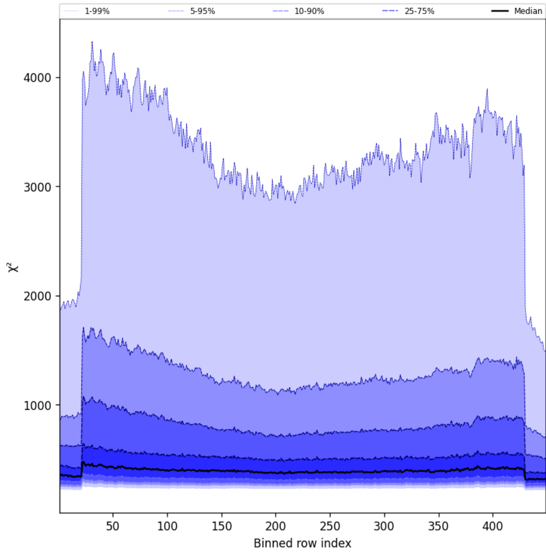
Figure 57: Along track statistics of “ \chi^2 ” for 2025-04-03 to 2025-04-04
