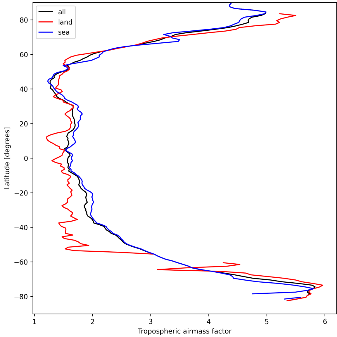
Figure 12: Zonal average of “Tropospheric air mass factor” for 2025-04-03 to 2025-04-04.
