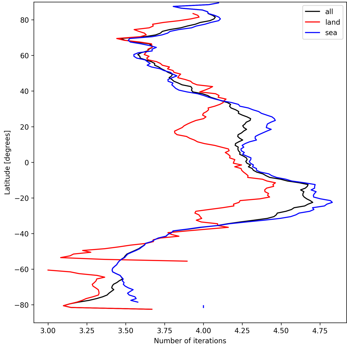
Figure 15: Zonal average of “Number of iterations” for 2025-04-03 to 2025-04-04.
