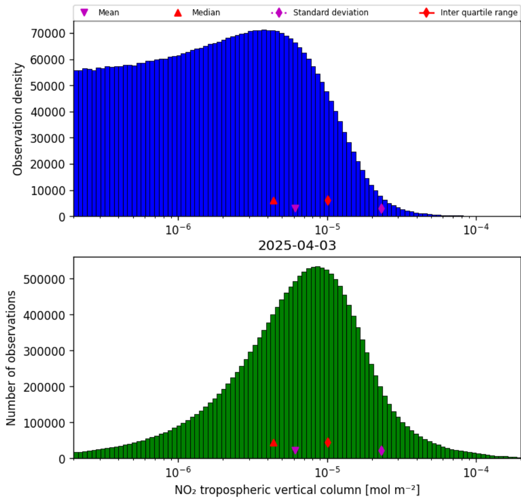
Figure 27: Histogram of “NO 2 tropospheric vertical column” for 2025-04-03 to 2025-04-04
