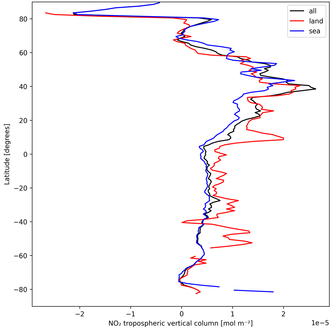
Figure 10: Zonal average of “NO 2 tropospheric vertical column” for 2025-04-03 to 2025-04-04.
