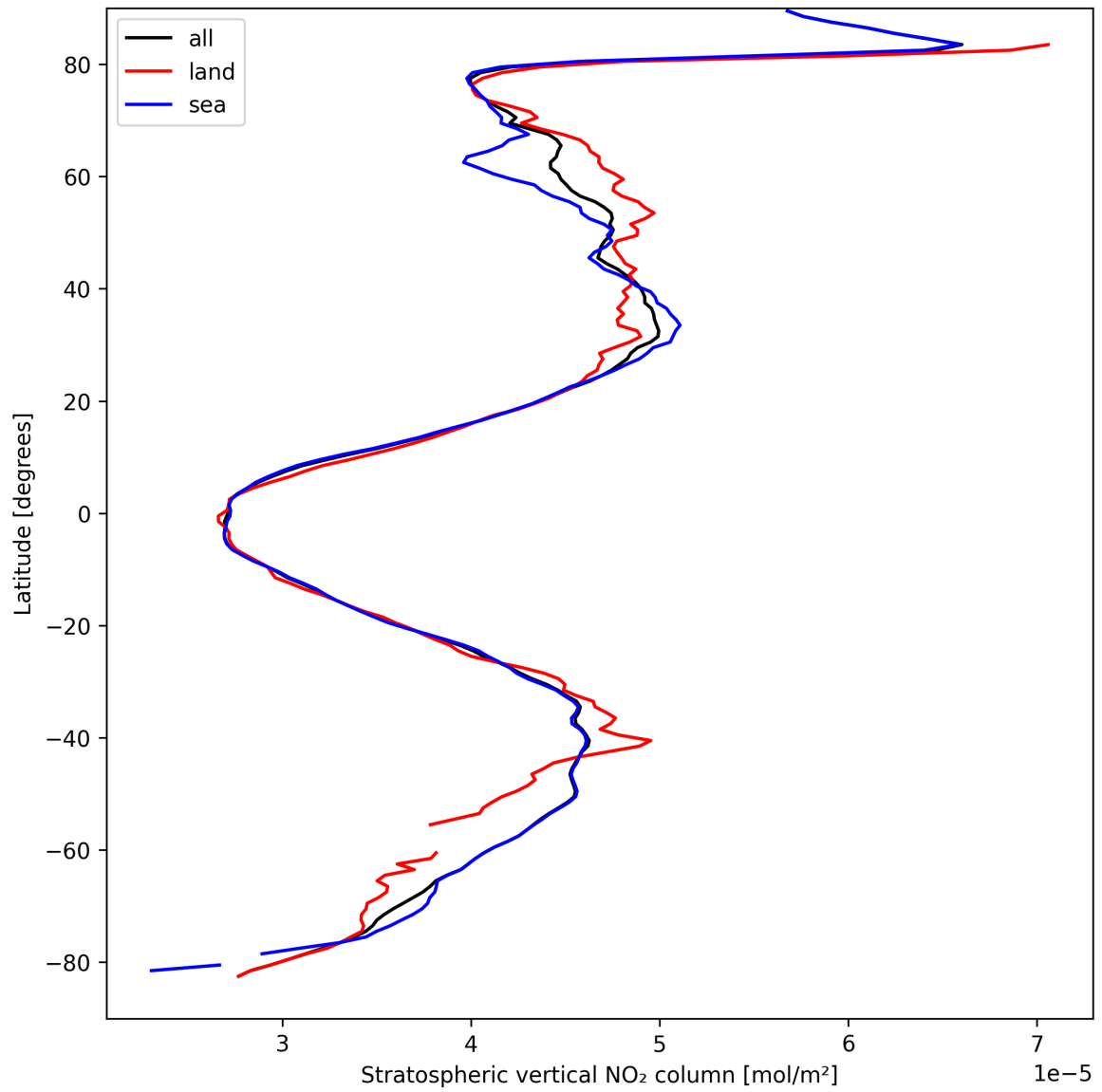
Figure 17: Zonal average of “Stratospheric vertical NO 2 column” for 2025-04-03 to 2025-04-04.
