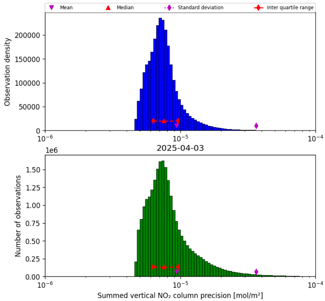
Figure 39: Histogram of “Summed vertical NO 2 column precision” for 2025-04-03 to 2025-04-04
