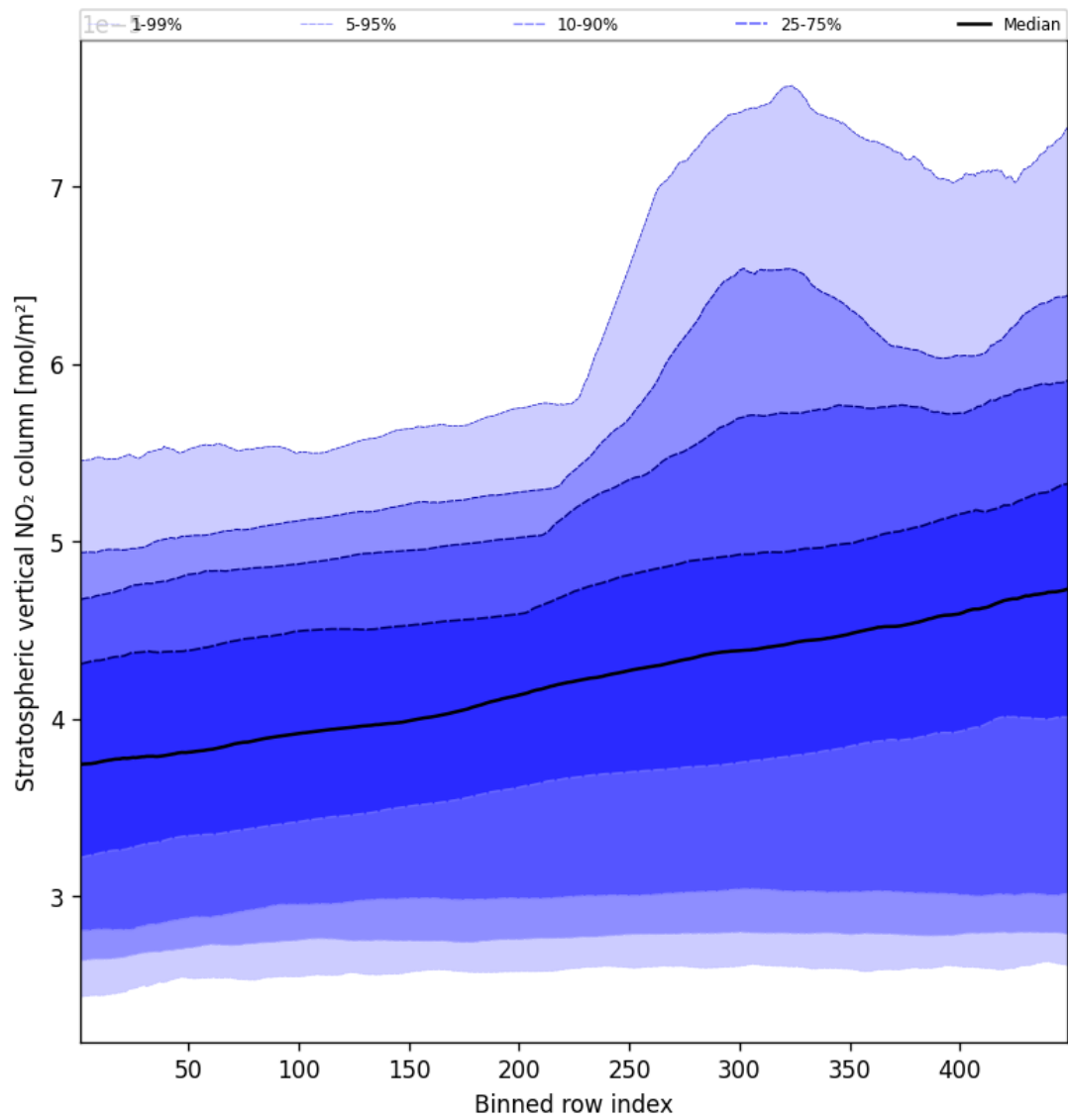
Figure 51: Along track statistics of "Stratospheric vertical NO 2 column" for 2025-04-03 to 2025-04-04
