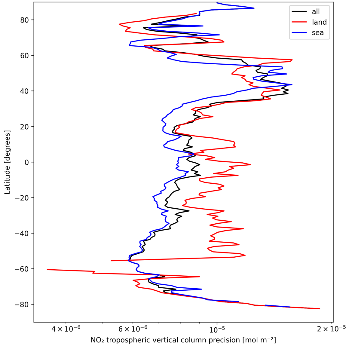
Figure 11: Zonal average of “NO 2 tropospheric vertical column precision” for 2025-04-03 to 2025-04-04.
