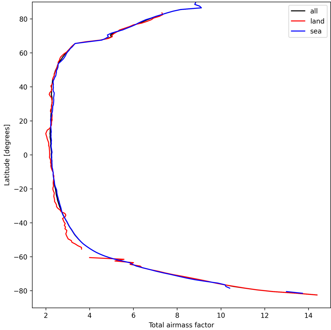
Figure 13: Zonal average of “Total airmass factor” for 2025-04-03 to 2025-04-04.
