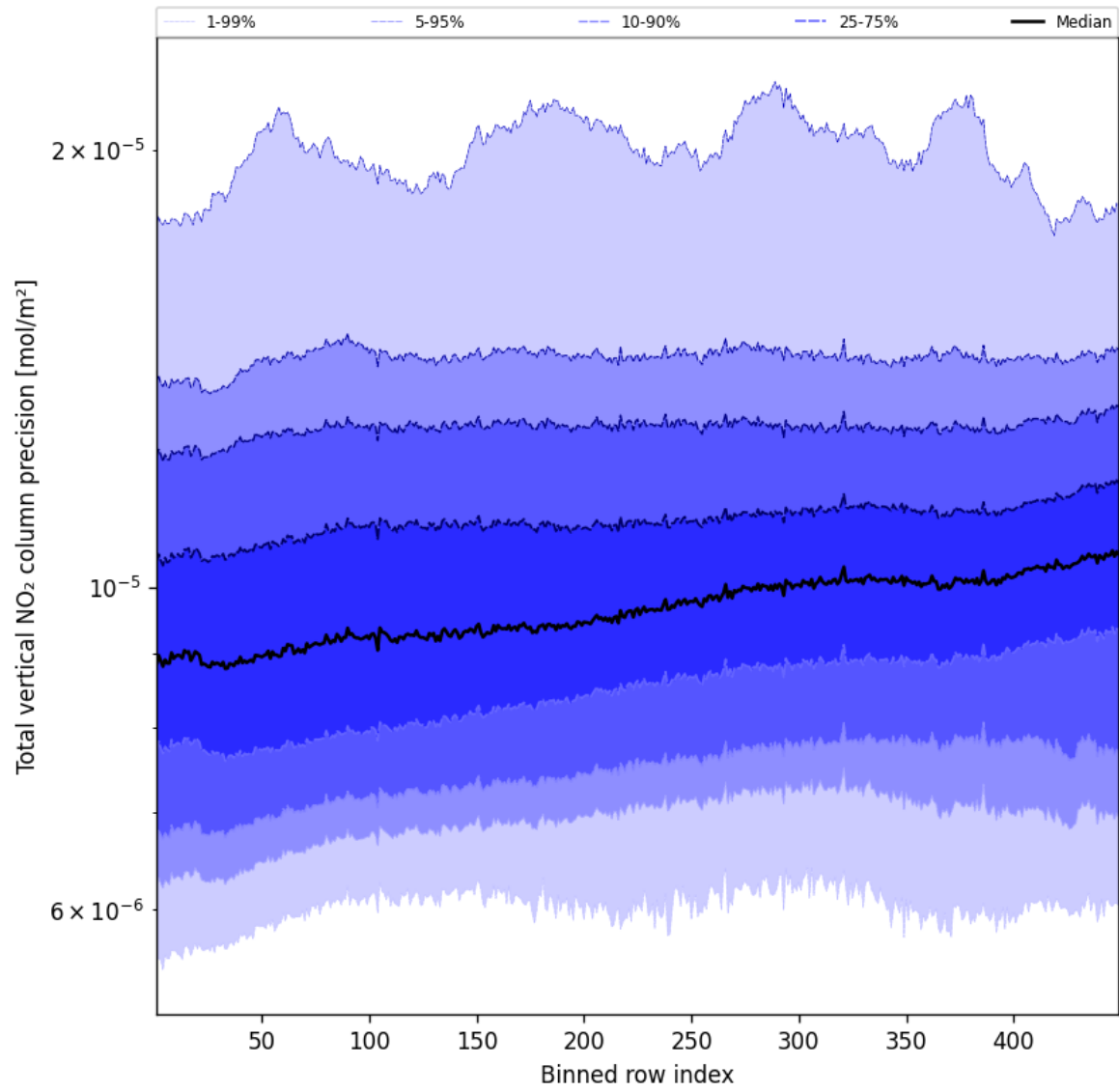
Figure 54: Along track statistics of "Total vertical NO 2 column precision" for 2025-04-03 to 2025-04-04
