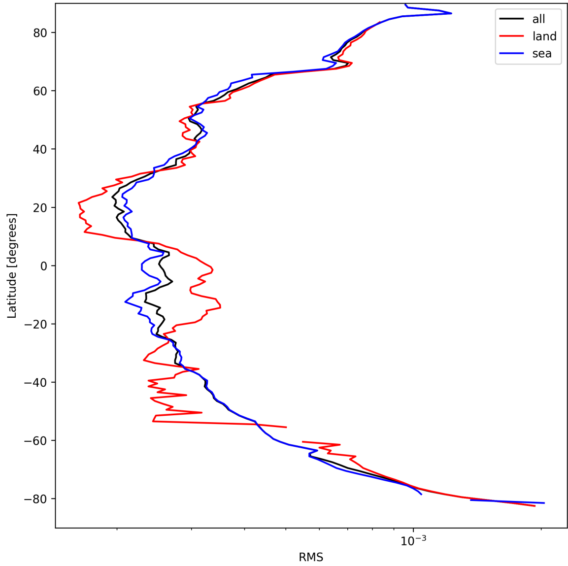
Figure 24: Zonal average of “RMS” for 2025-04-03 to 2025-04-04.
