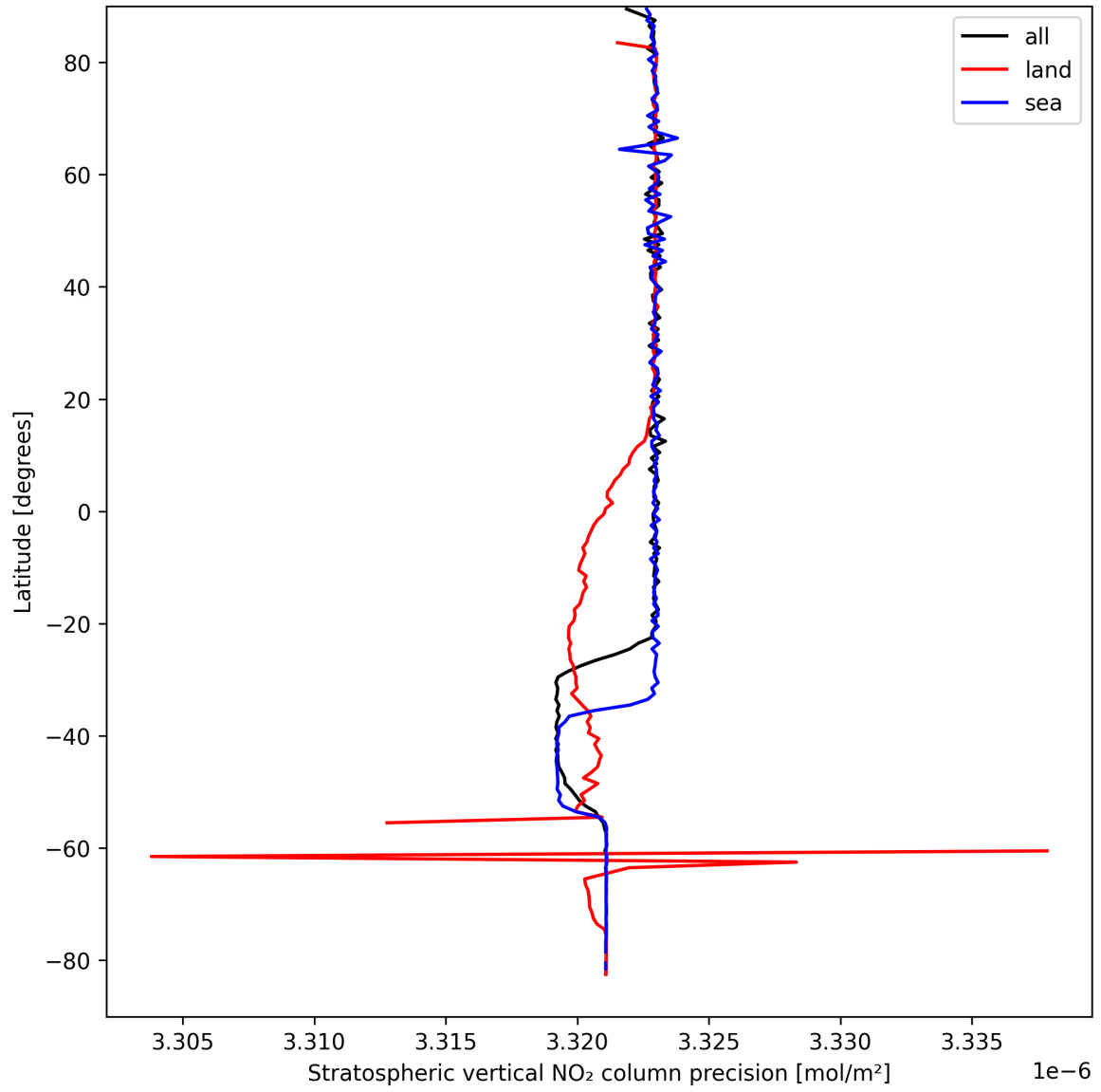
Figure 18: Zonal average of “Stratospheric vertical NO 2 column precision” for 2025-04-03 to 2025-04-04.
