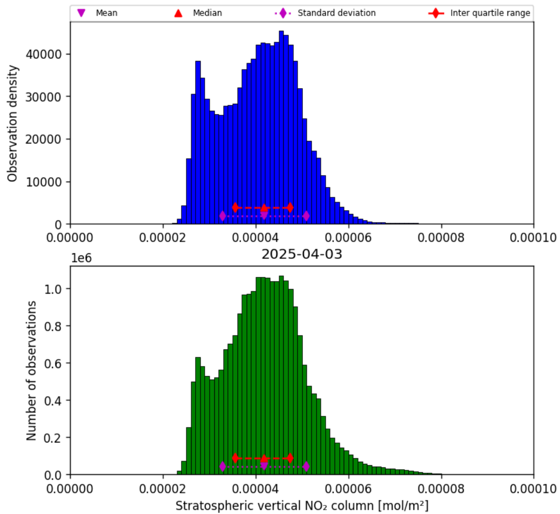
Figure 34: Histogram of “Stratospheric vertical NO 2 column” for 2025-04-03 to 2025-04-04
