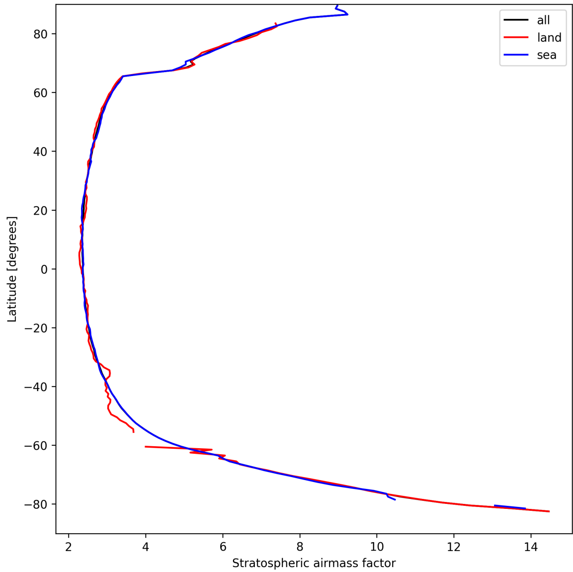
Figure 25: Zonal average of “Stratospheric airmass factor” for 2025-04-03 to 2025-04-04.
