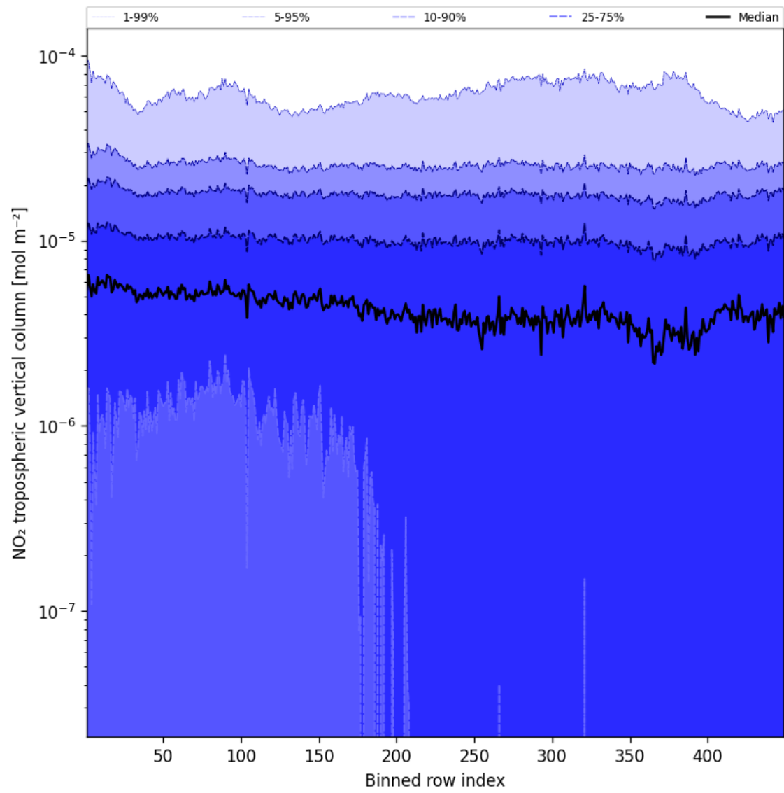
Figure 44: Along track statistics of “NO 2 tropospheric vertical column” for 2025-04-03 to 2025-04-04
