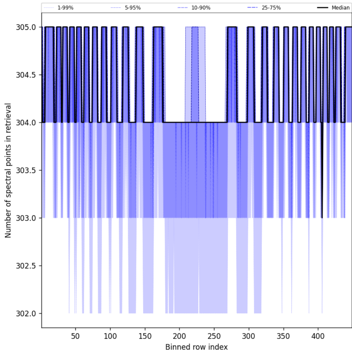
Figure 48: Along track statistics of “Number of spectral points in retrieval” for 2025-04-03 to 2025-04-04
