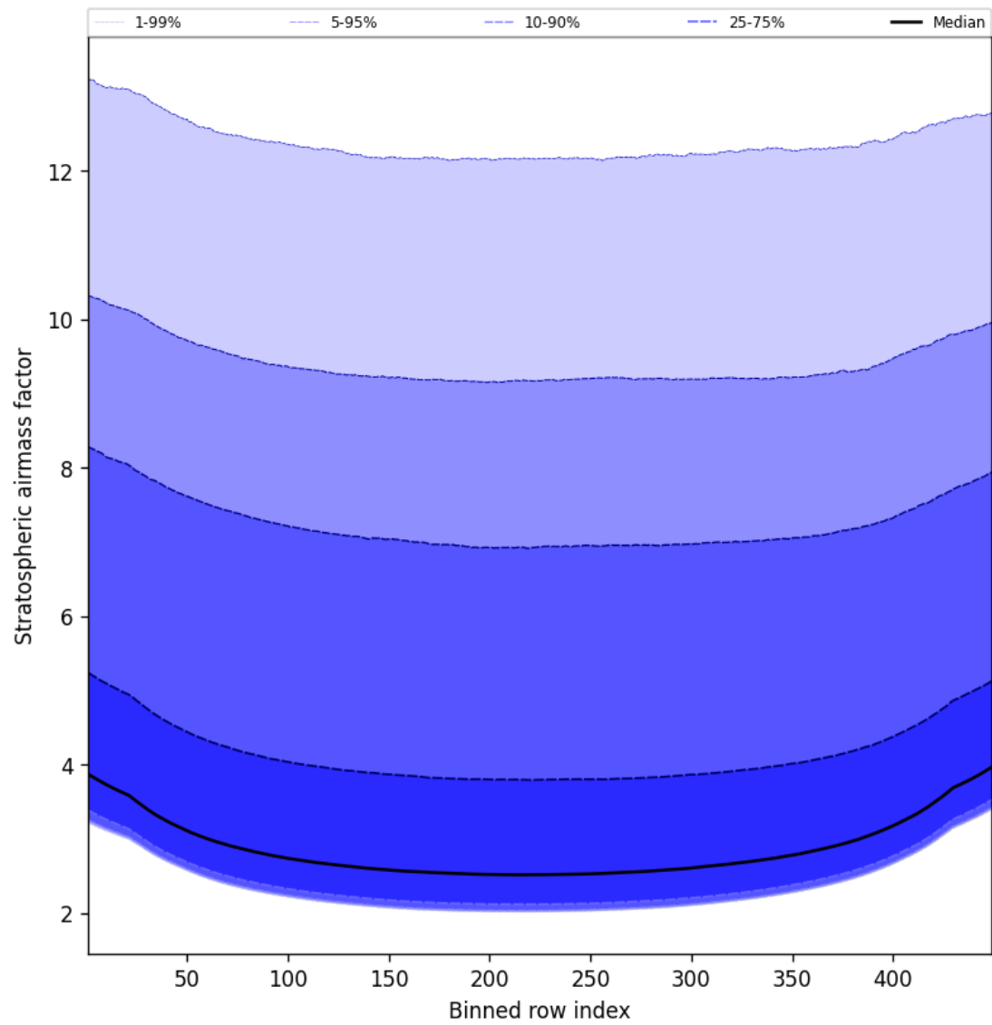
Figure 59: Along track statistics of “Stratospheric airmass factor” for 2025-04-03 to 2025-04-04
