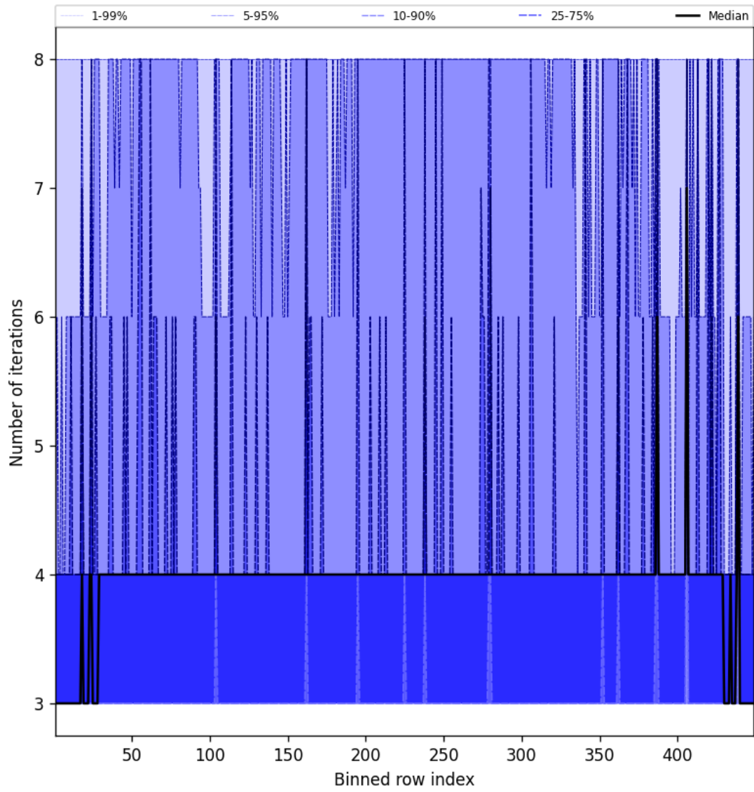
Figure 49: Along track statistics of “Number of iterations” for 2025-04-03 to 2025-04-04
