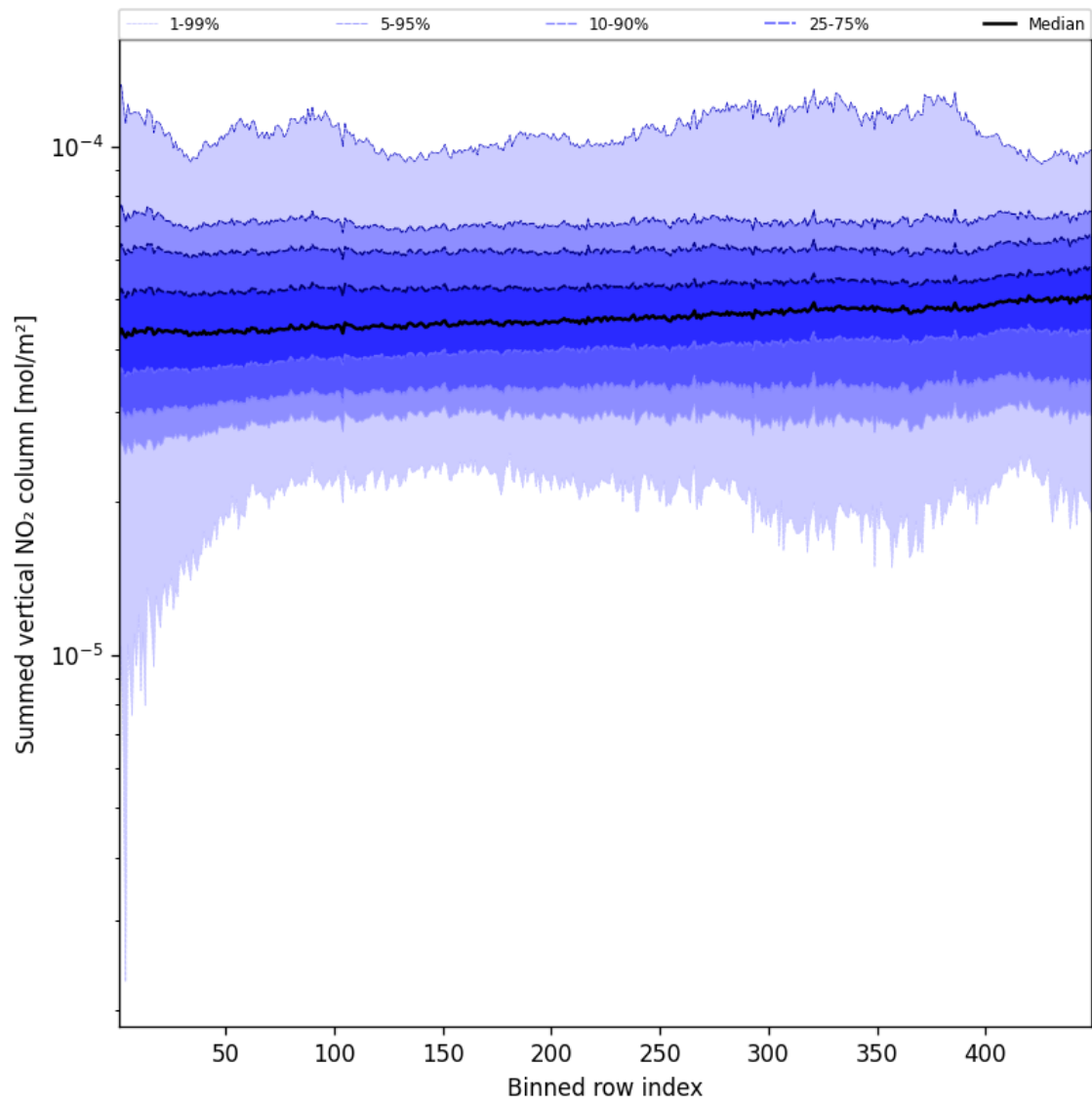
Figure 55: Along track statistics of “Summed vertical NO 2 column” for 2025-04-03 to 2025-04-04
