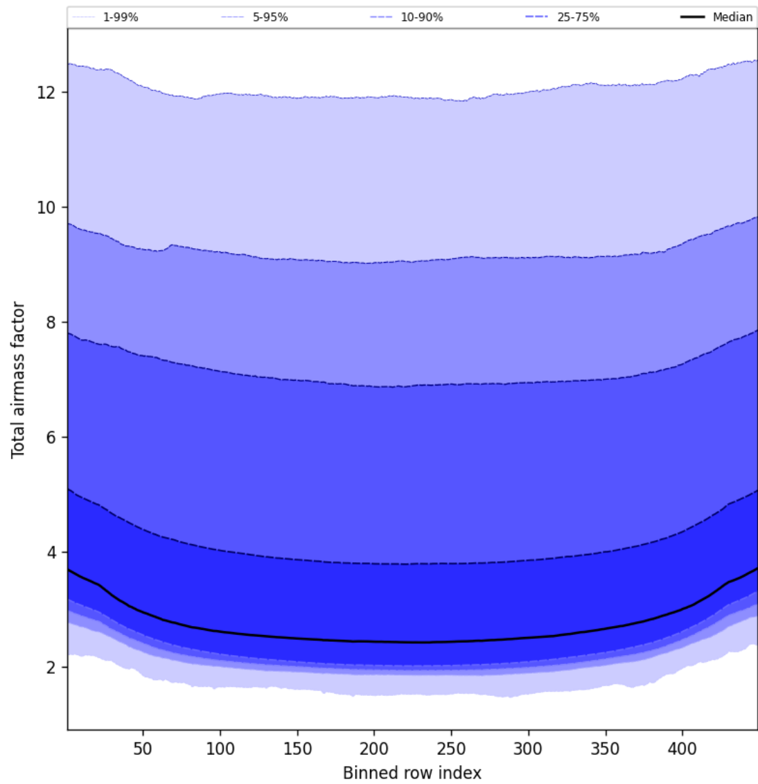
Figure 47: Along track statistics of “Total airmass factor” for 2025-04-03 to 2025-04-04
