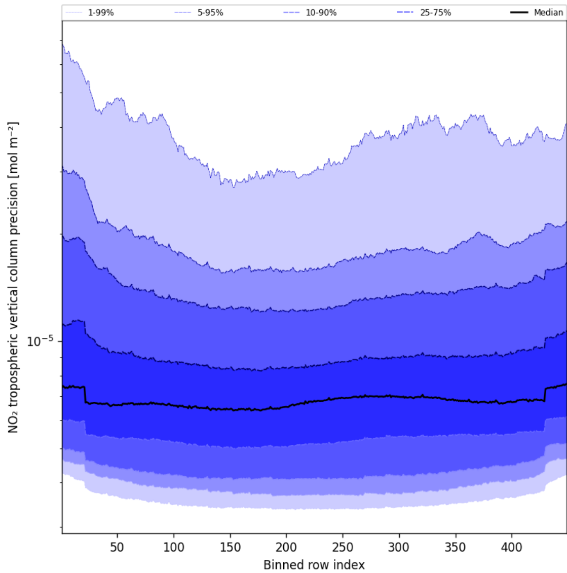
Figure 45: Along track statistics of “NO 2 tropospheric vertical column precision” for 2025-04-03 to 2025-04-04
