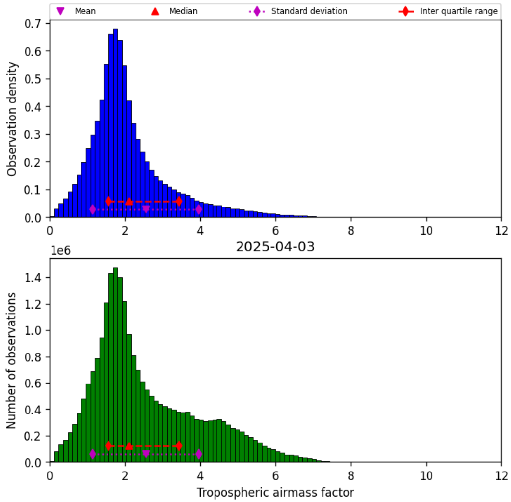
Figure 29: Histogram of “Tropospheric airmass factor” for 2025-04-03 to 2025-04-04
