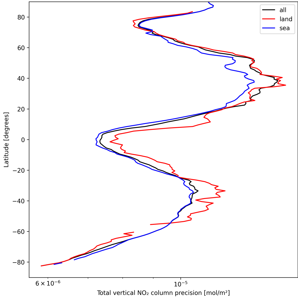
Figure 20: Zonal average of “Total vertical NO 2 column precision” for 2025-04-03 to 2025-04-04.
