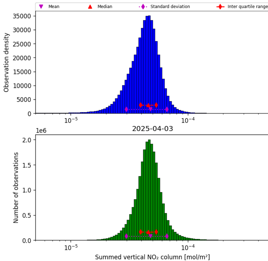
Figure 38: Histogram of “Summed vertical NO 2 column” for 2025-04-03 to 2025-04-04
