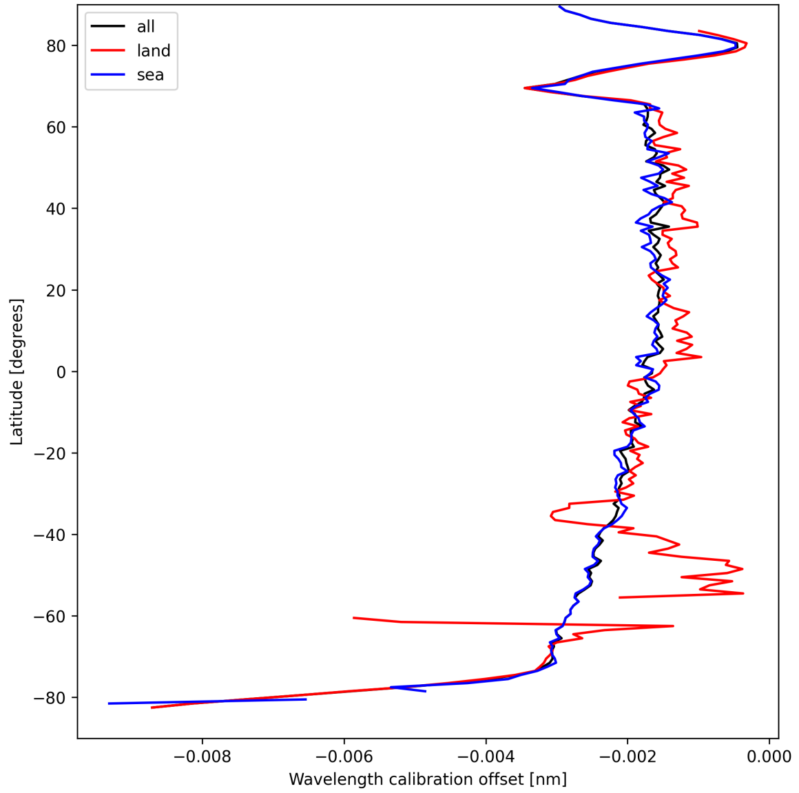
Figure 16: Zonal average of “Wavelength calibration offset” for 2025-04-03 to 2025-04-04.
