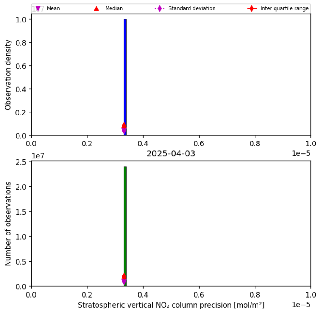
Figure 35: Histogram of “Stratospheric vertical NO 2 column precision” for 2025-04-03 to 2025-04-04
