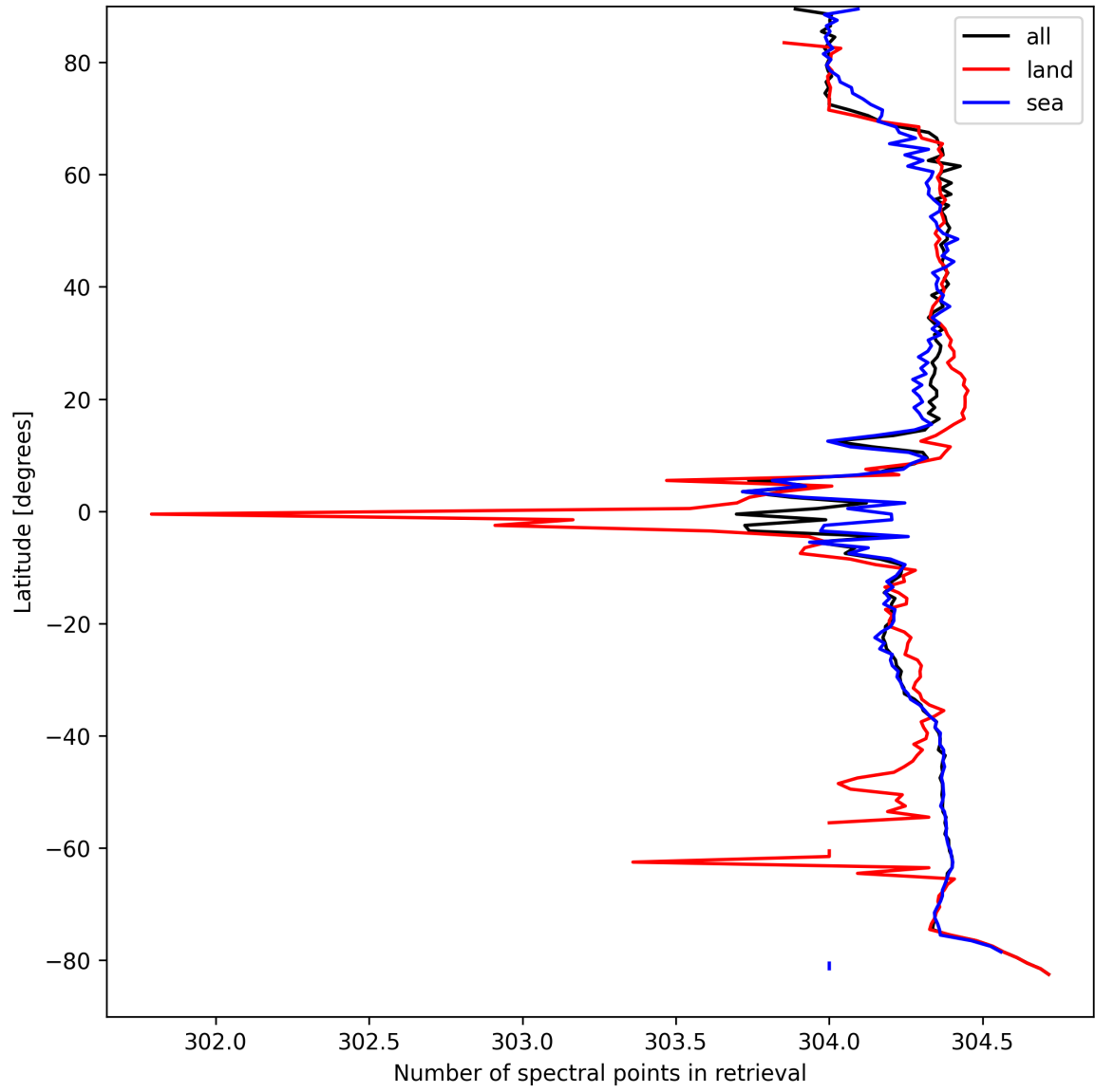
Figure 14: Zonal average of “Number of spectral points in retrieval” for 2025-04-03 to 2025-04-04.
