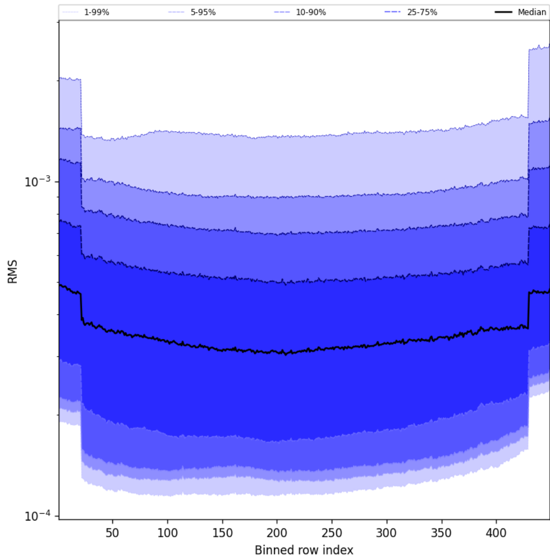
Figure 58: Along track statistics of “RMS” for 2025-04-03 to 2025-04-04
