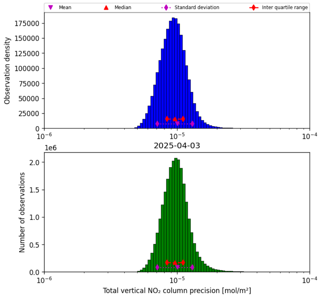
Figure 37: Histogram of “Total vertical NO 2 column precision” for 2025-04-03 to 2025-04-04
