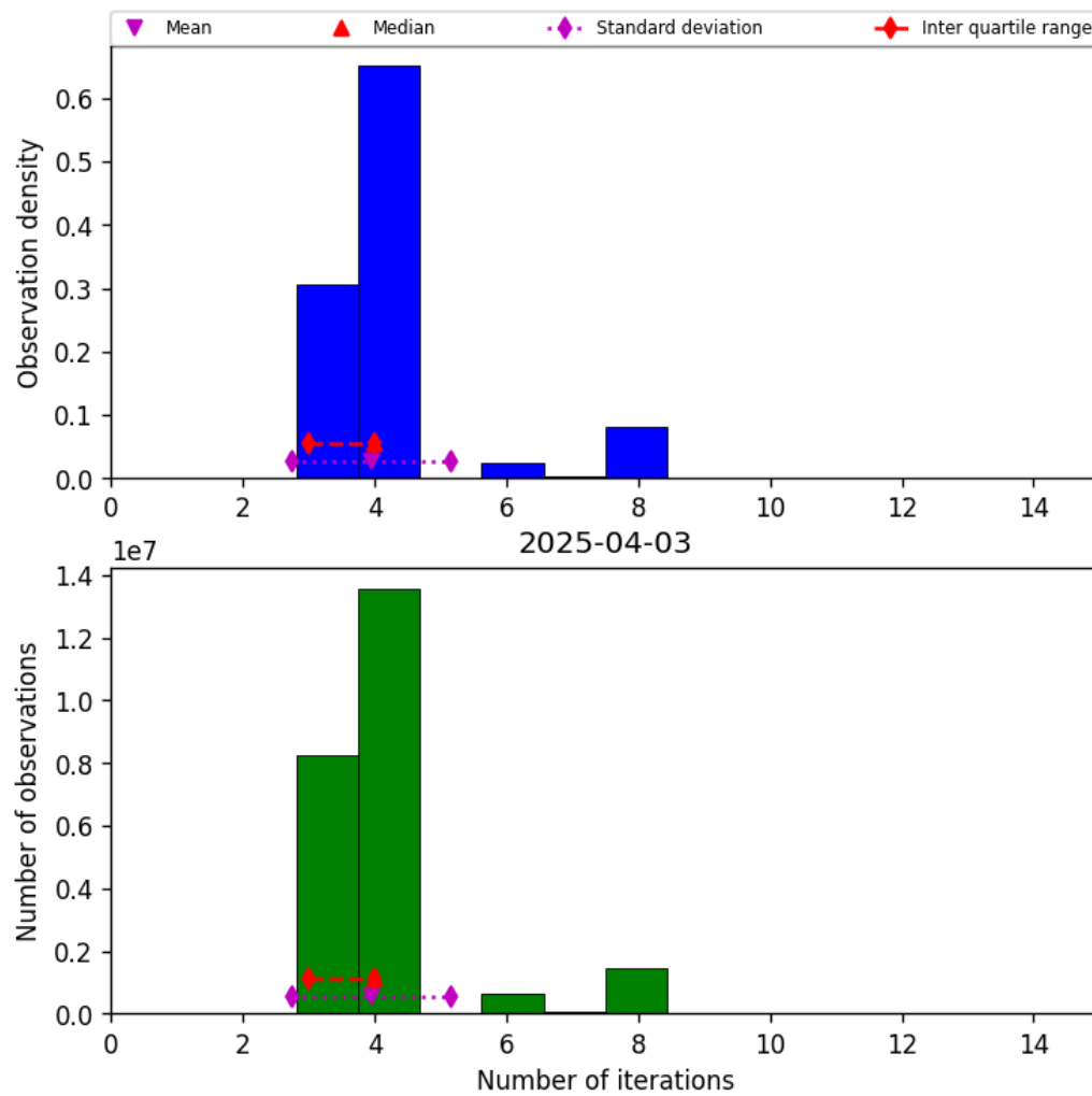
Figure 32: Histogram of “Number of iterations” for 2025-04-03 to 2025-04-04
