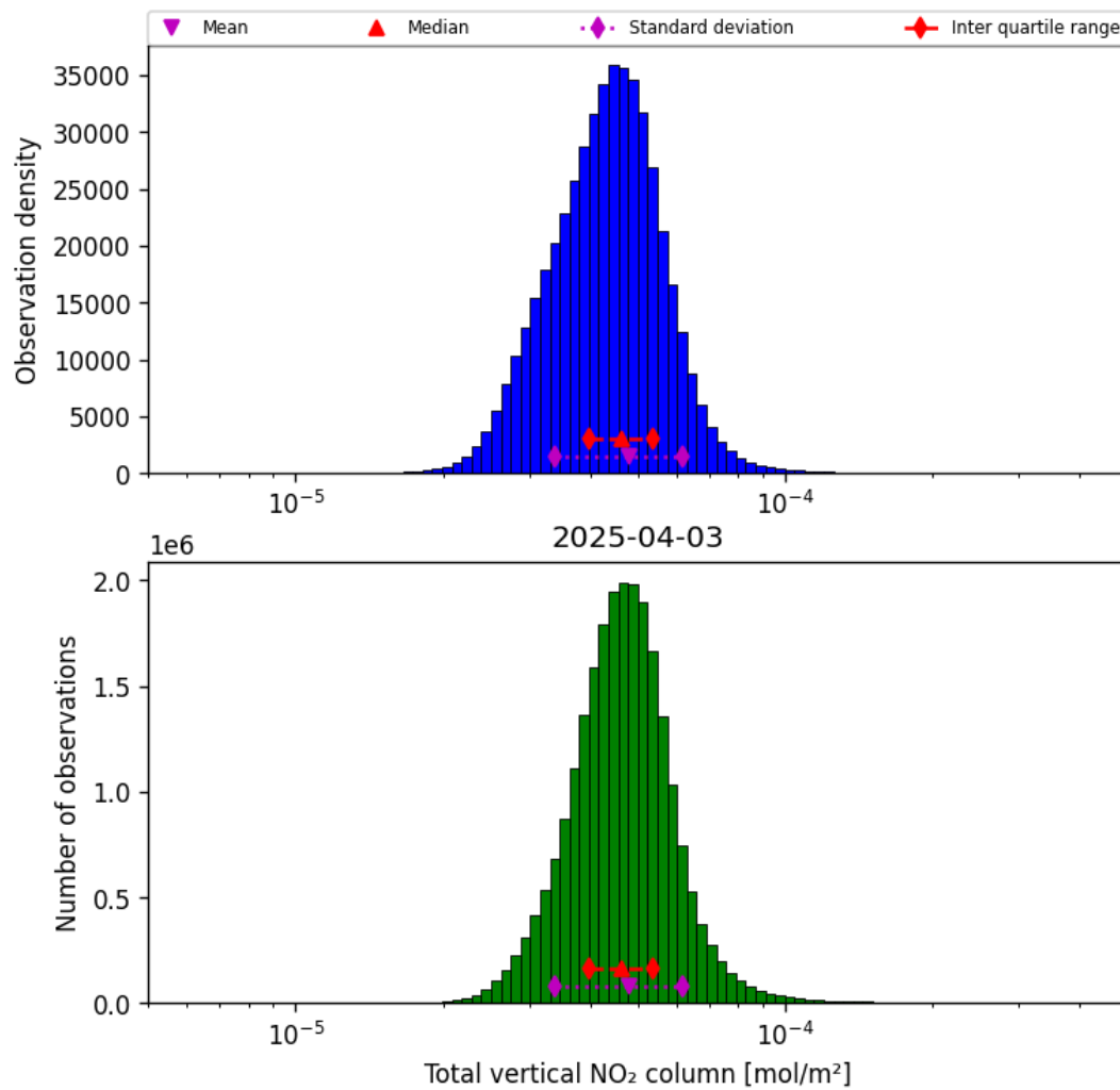
Figure 36: Histogram of “Total vertical NO 2 column” for 2025-04-03 to 2025-04-04
