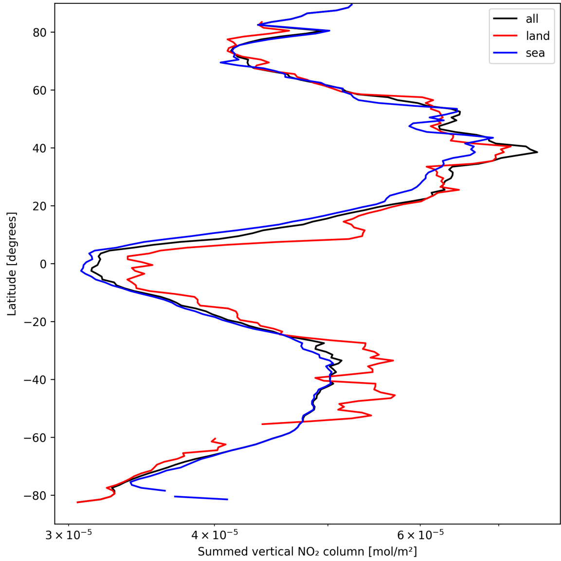
Figure 21: Zonal average of “Summed vertical NO 2 column” for 2025-04-03 to 2025-04-04.
