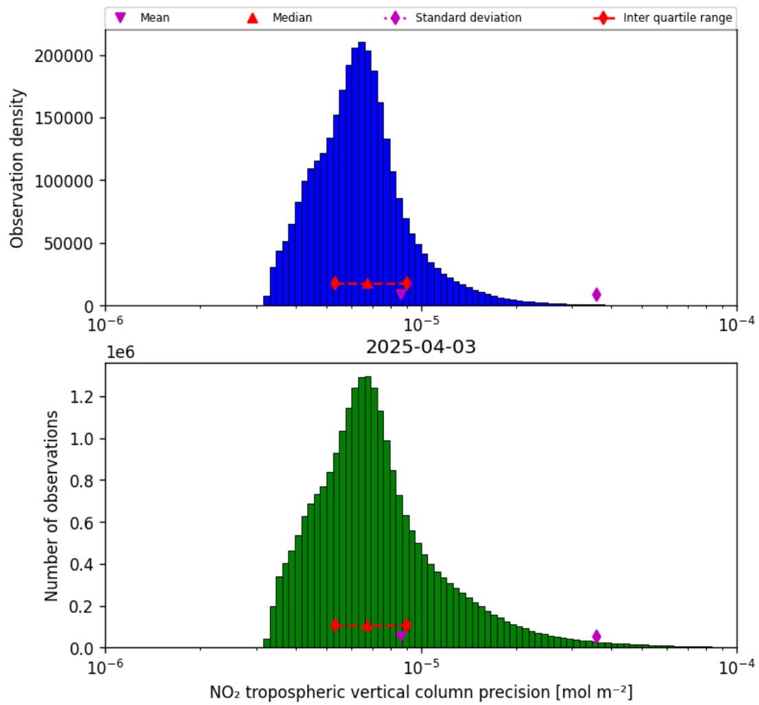
Figure 28: Histogram of “NO 2 tropospheric vertical column precision” for 2025-04-03 to 2025-04-04
