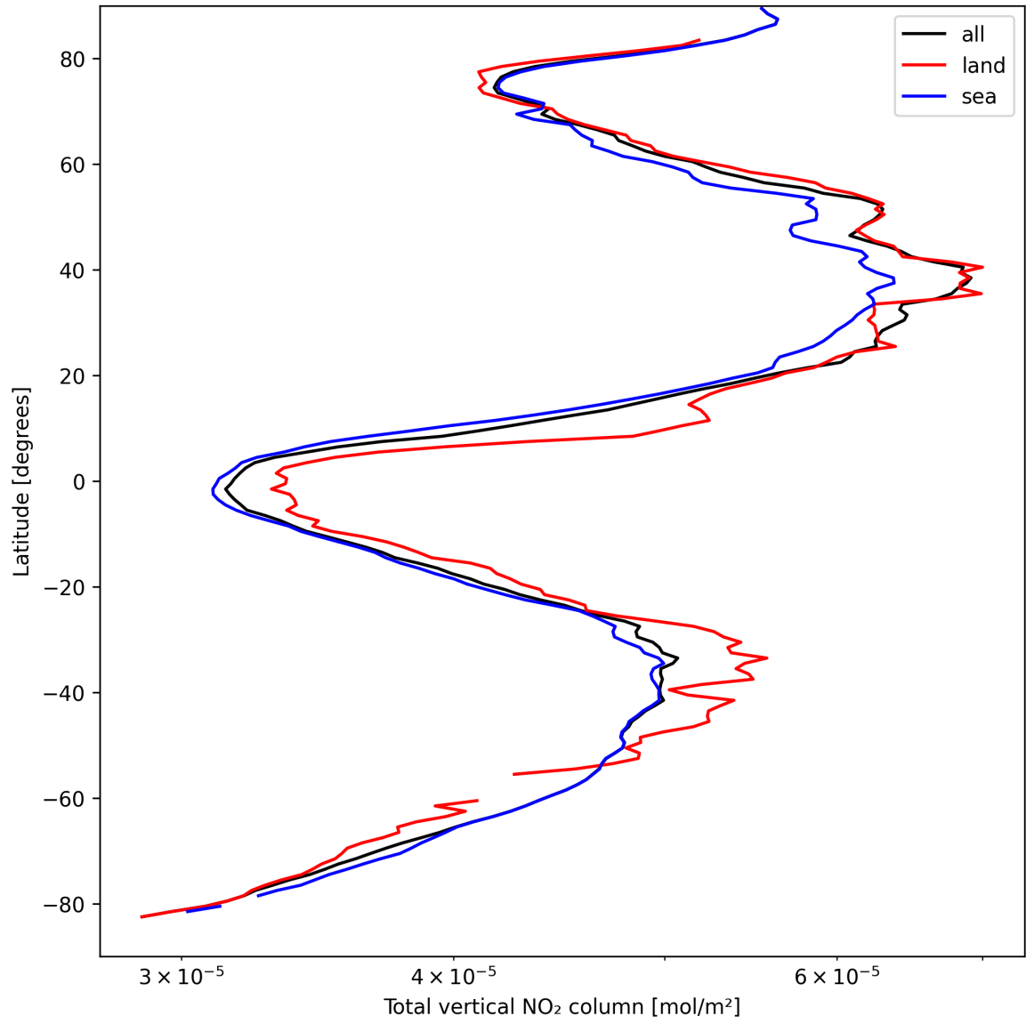
Figure 19: Zonal average of “Total vertical NO 2 column” for 2025-04-03 to 2025-04-04.
