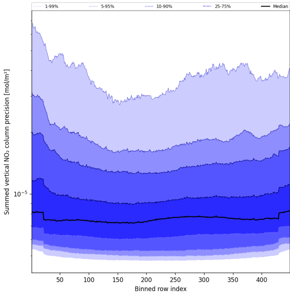
Figure 56: Along track statistics of “Summed vertical NO 2 column precision” for 2025-04-03 to 2025-04-04
