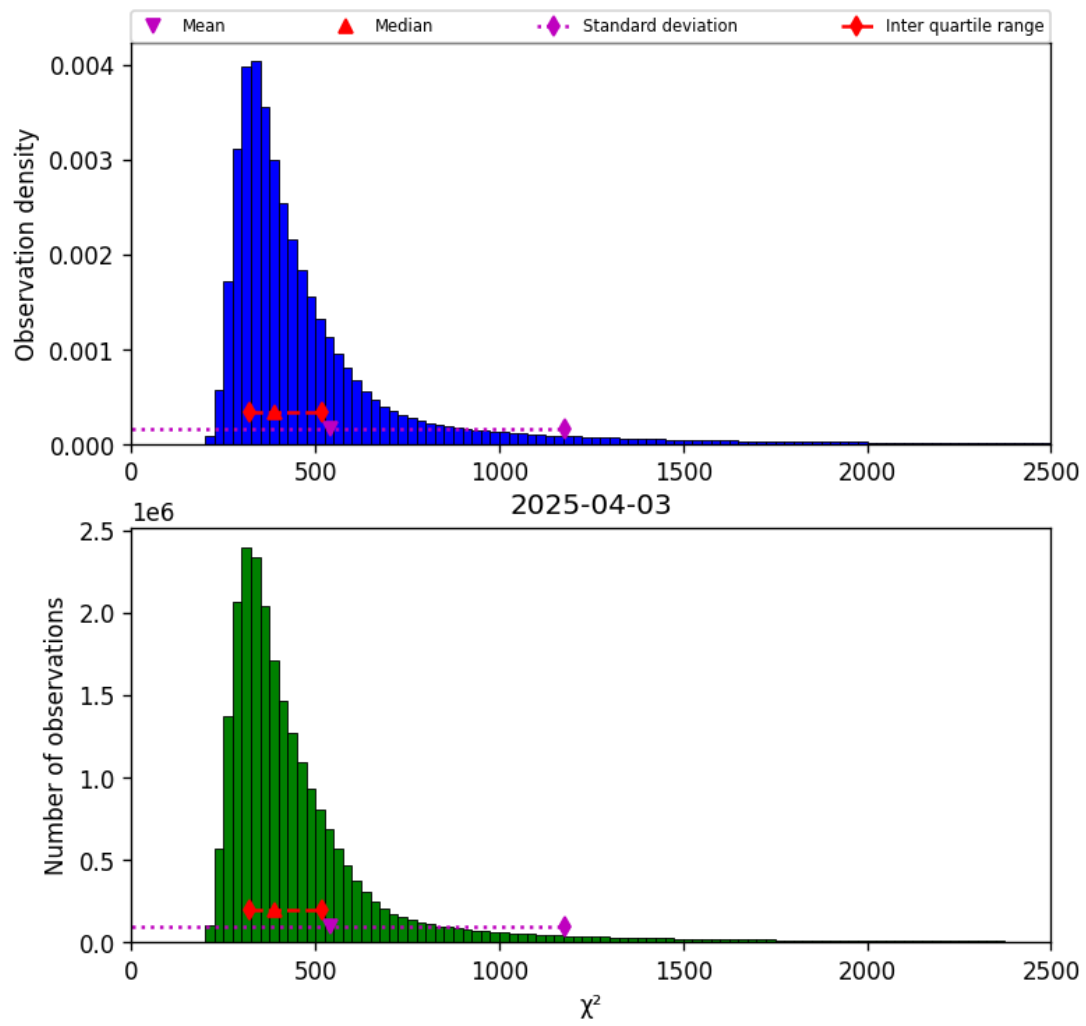
Figure 40: Histogram of “ \chi^2 ” for 2025-04-03 to 2025-04-04
