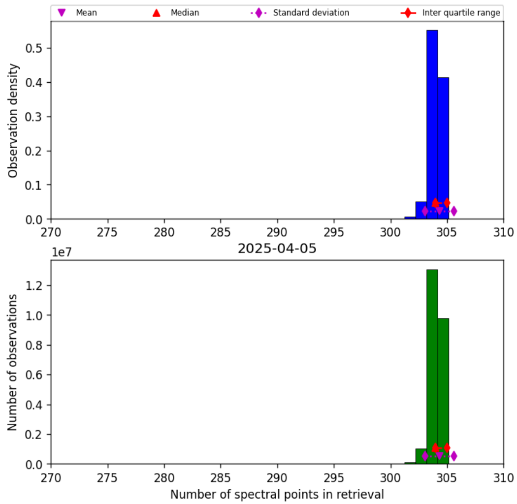
Figure 31: Histogram of “Number of spectral points in retrieval” for 2025-04-05 to 2025-04-06
