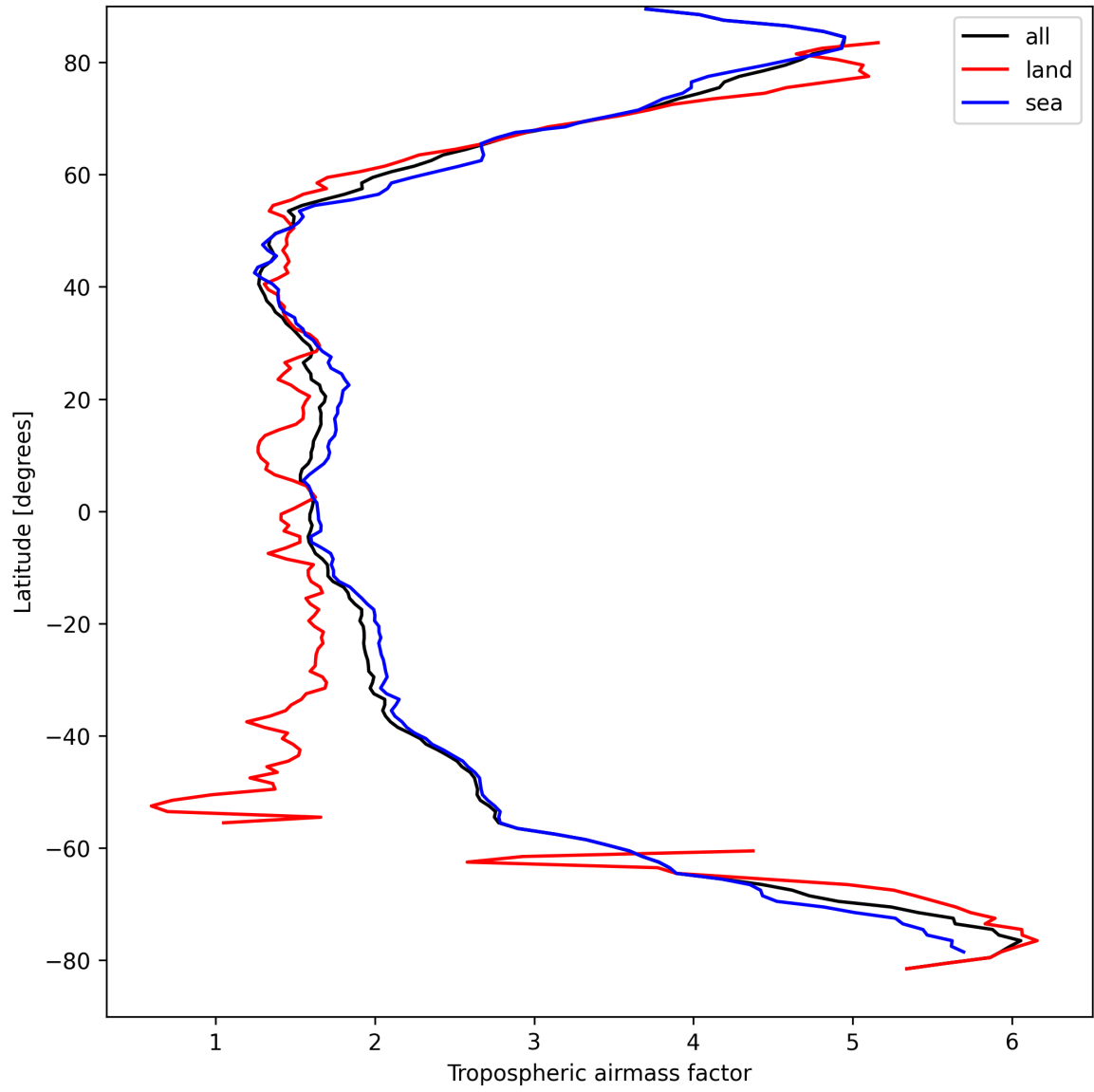
Figure 12: Zonal average of “Tropospheric air mass factor” for 2025-04-05 to 2025-04-06.
