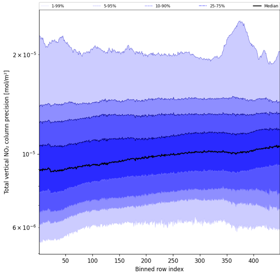
Figure 54: Along track statistics of “Total vertical NO 2 column precision” for 2025-04-05 to 2025-04-06
