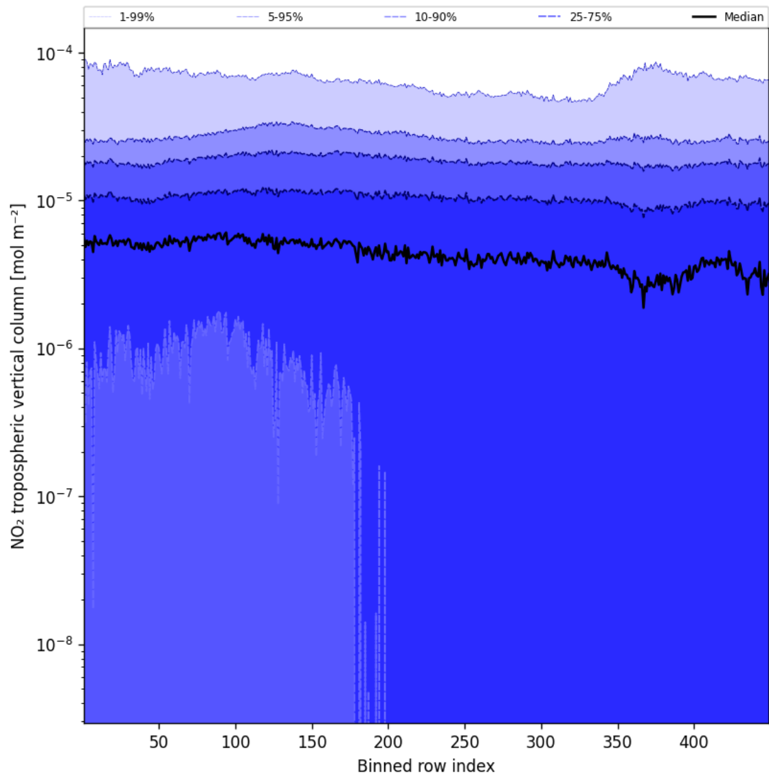
Figure 44: Along track statistics of “NO 2 tropospheric vertical column” for 2025-04-05 to 2025-04-06
