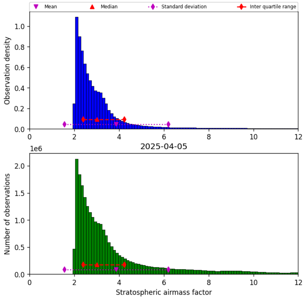
Figure 42: Histogram of “Stratospheric airmass factor” for 2025-04-05 to 2025-04-06
