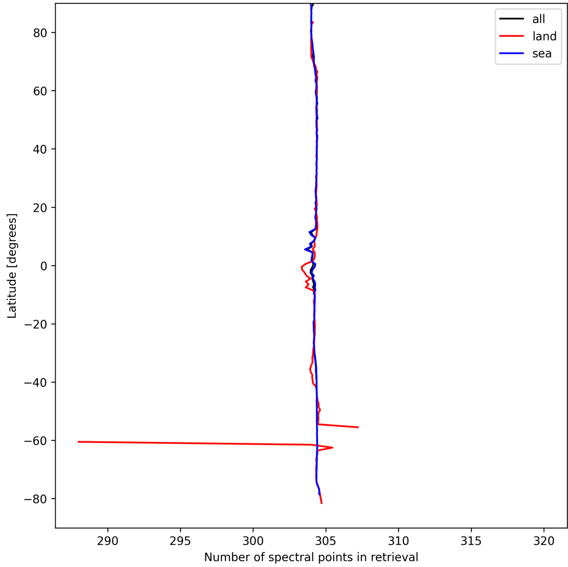
Figure 14: Zonal average of “Number of spectral points in retrieval” for 2025-04-05 to 2025-04-06.
