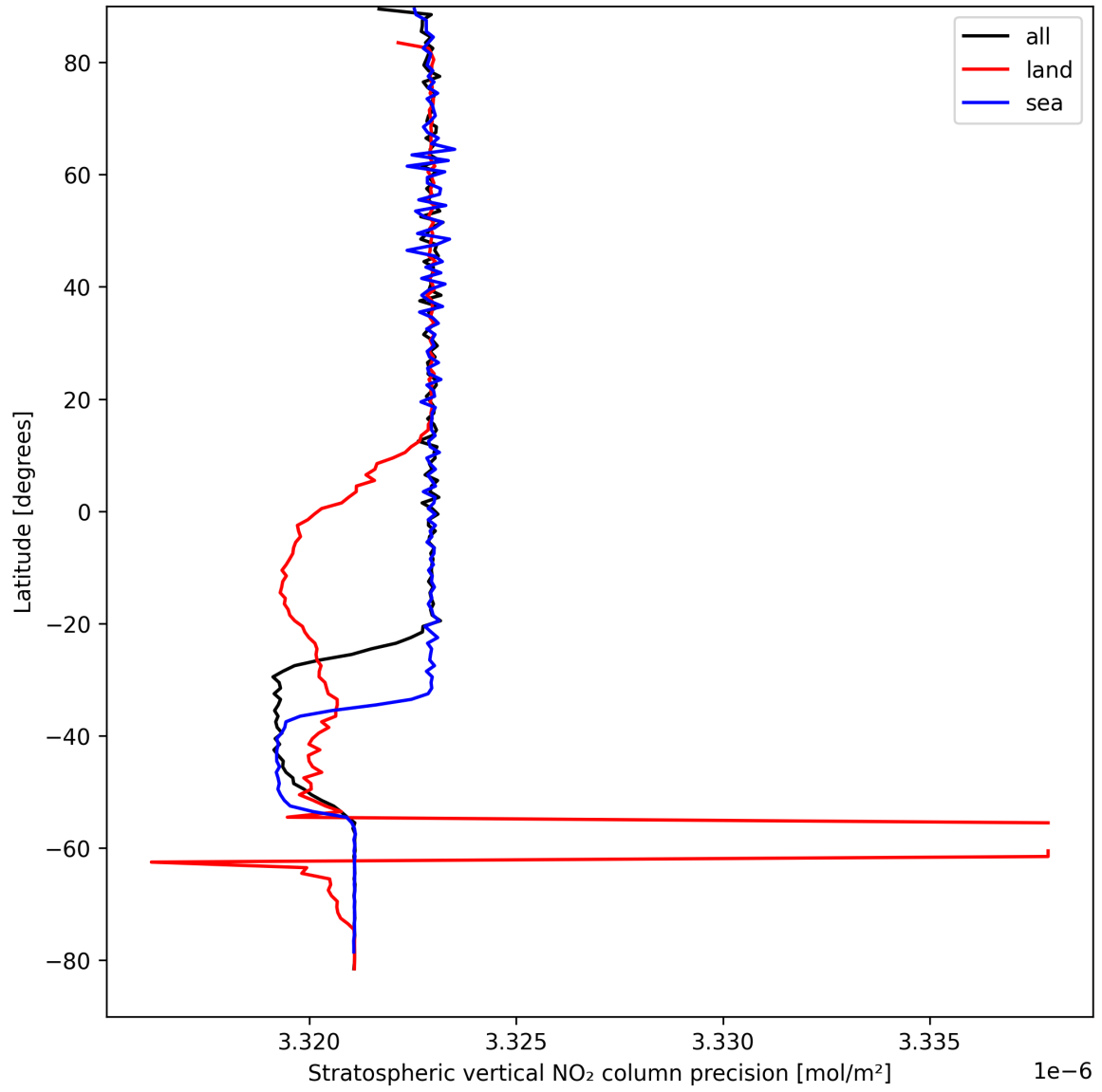
Figure 18: Zonal average of “Stratospheric vertical NO 2 column precision” for 2025-04-05 to 2025-04-06.
