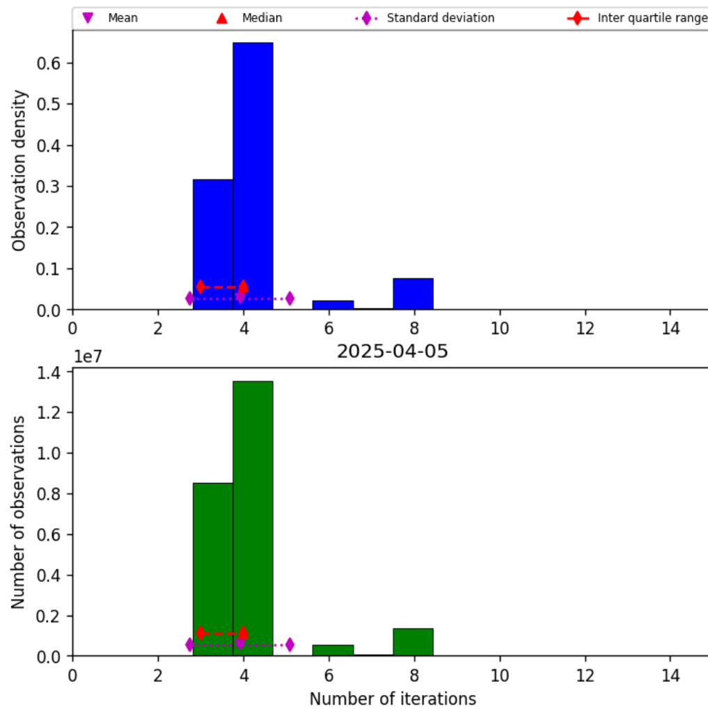
Figure 32: Histogram of “Number of iterations” for 2025-04-05 to 2025-04-06
