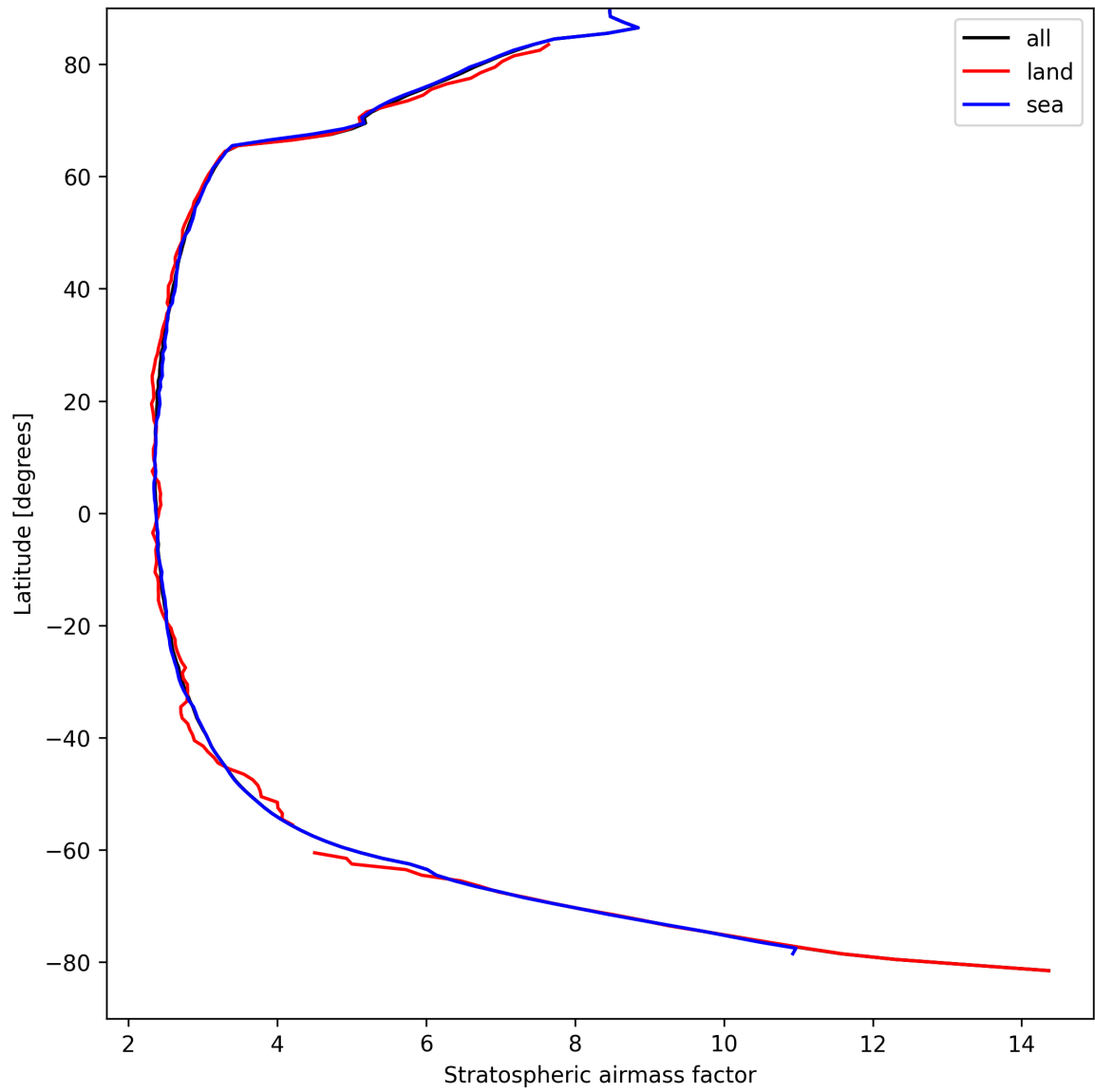
Figure 25: Zonal average of “Stratospheric air mass factor” for 2025-04-05 to 2025-04-06.
