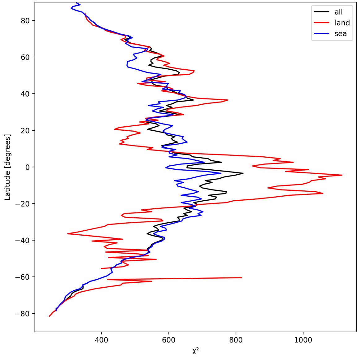
Figure 23: Zonal average of “ \chi^2 ” for 2025-04-05 to 2025-04-06.
