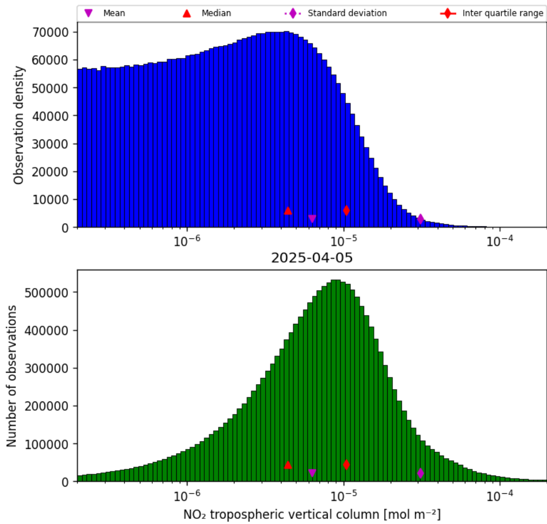
Figure 27: Histogram of “NO 2 tropospheric vertical column” for 2025-04-05 to 2025-04-06
