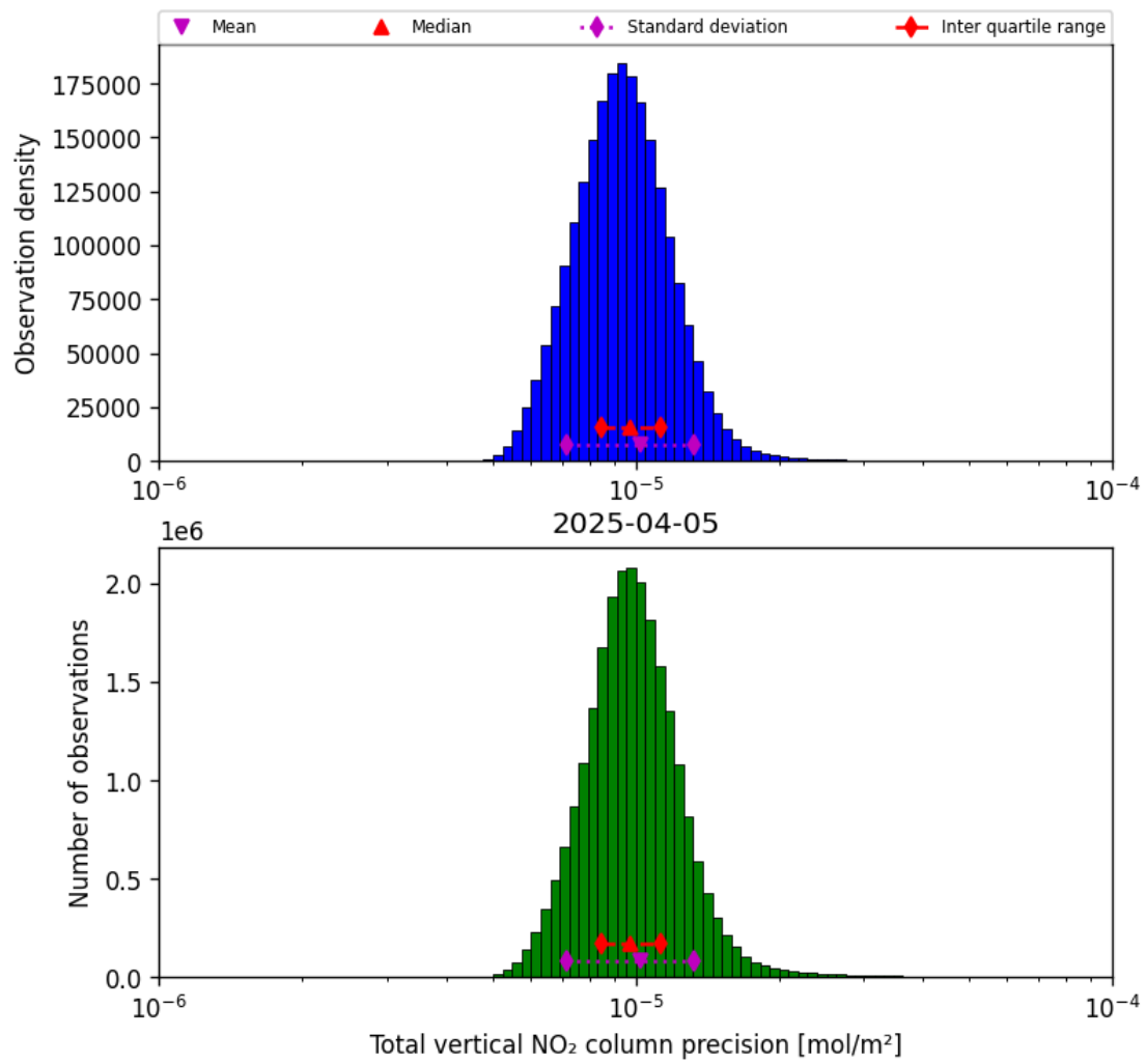
Figure 37: Histogram of “Total vertical NO 2 column precision” for 2025-04-05 to 2025-04-06
