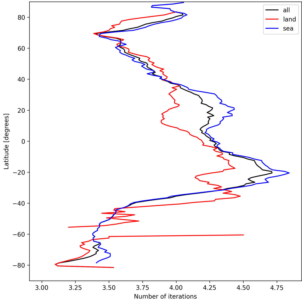
Figure 15: Zonal average of “Number of iterations” for 2025-04-05 to 2025-04-06.
