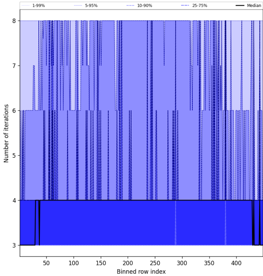
Figure 49: Along track statistics of “Number of iterations” for 2025-04-05 to 2025-04-06
