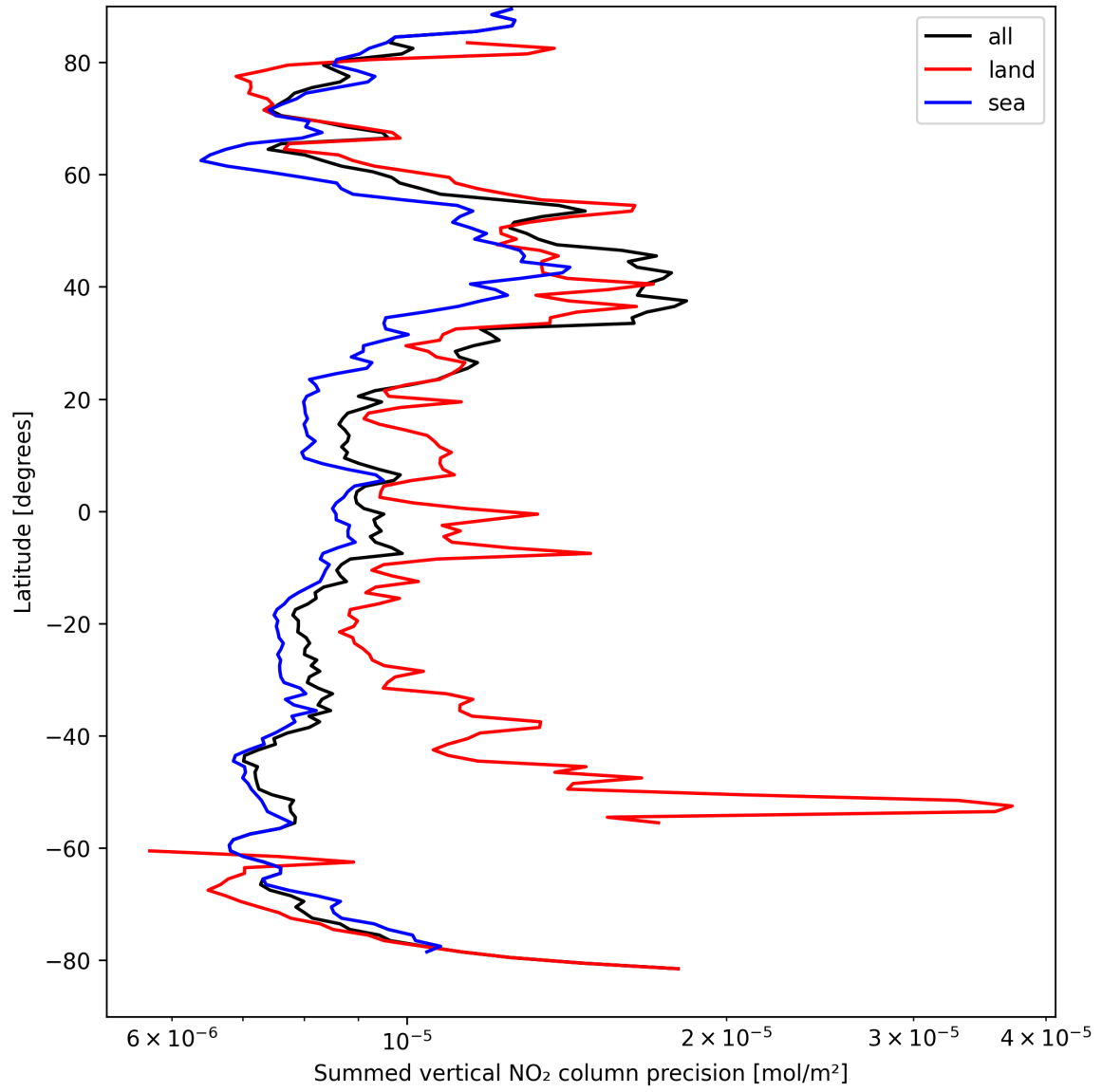
Figure 22: Zonal average of “Summed vertical NO 2 column precision” for 2025-04-05 to 2025-04-06.
