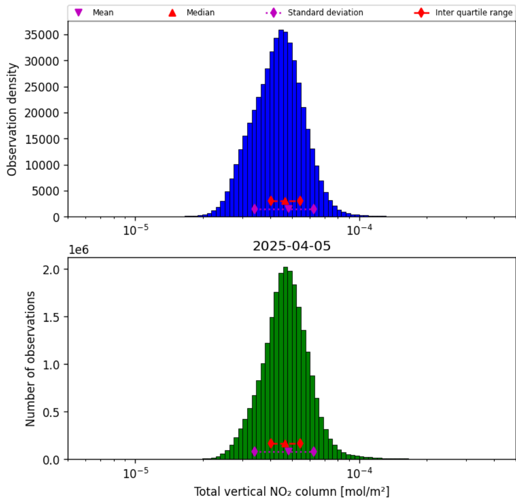
Figure 36: Histogram of “Total vertical NO 2 column” for 2025-04-05 to 2025-04-06
