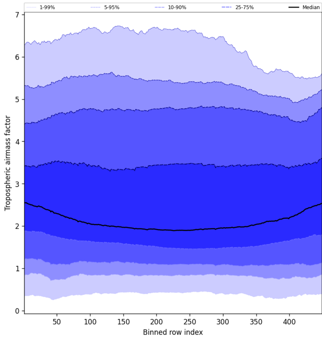
Figure 46: Along track statistics of “Tropospheric airmass factor” for 2025-04-05 to 2025-04-06
