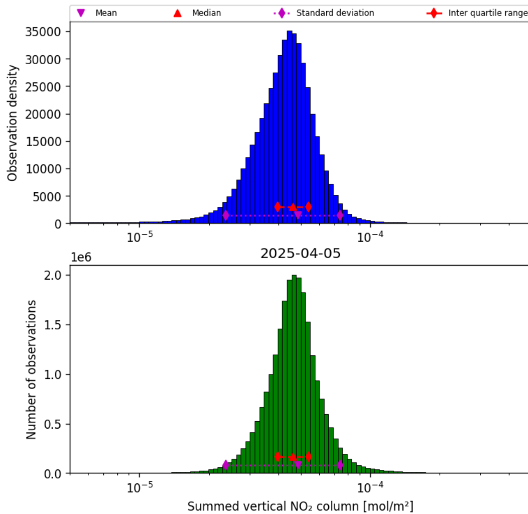
Figure 38: Histogram of "Summed vertical NO 2 column" for 2025-04-05 to 2025-04-06
