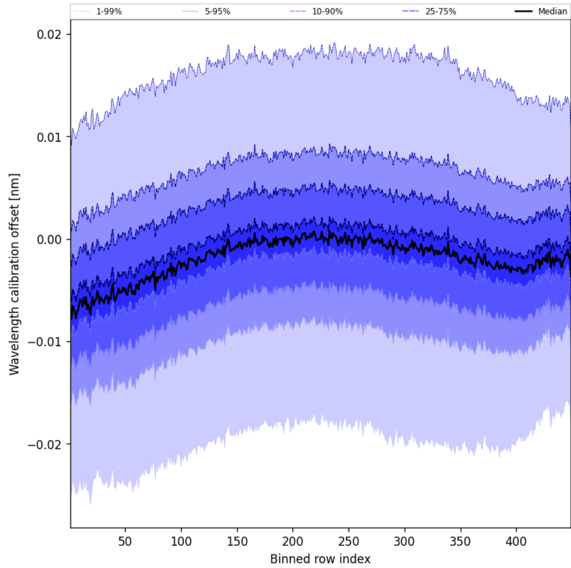
Figure 50: Along track statistics of “Wavelength calibration offset” for 2025-04-05 to 2025-04-06
