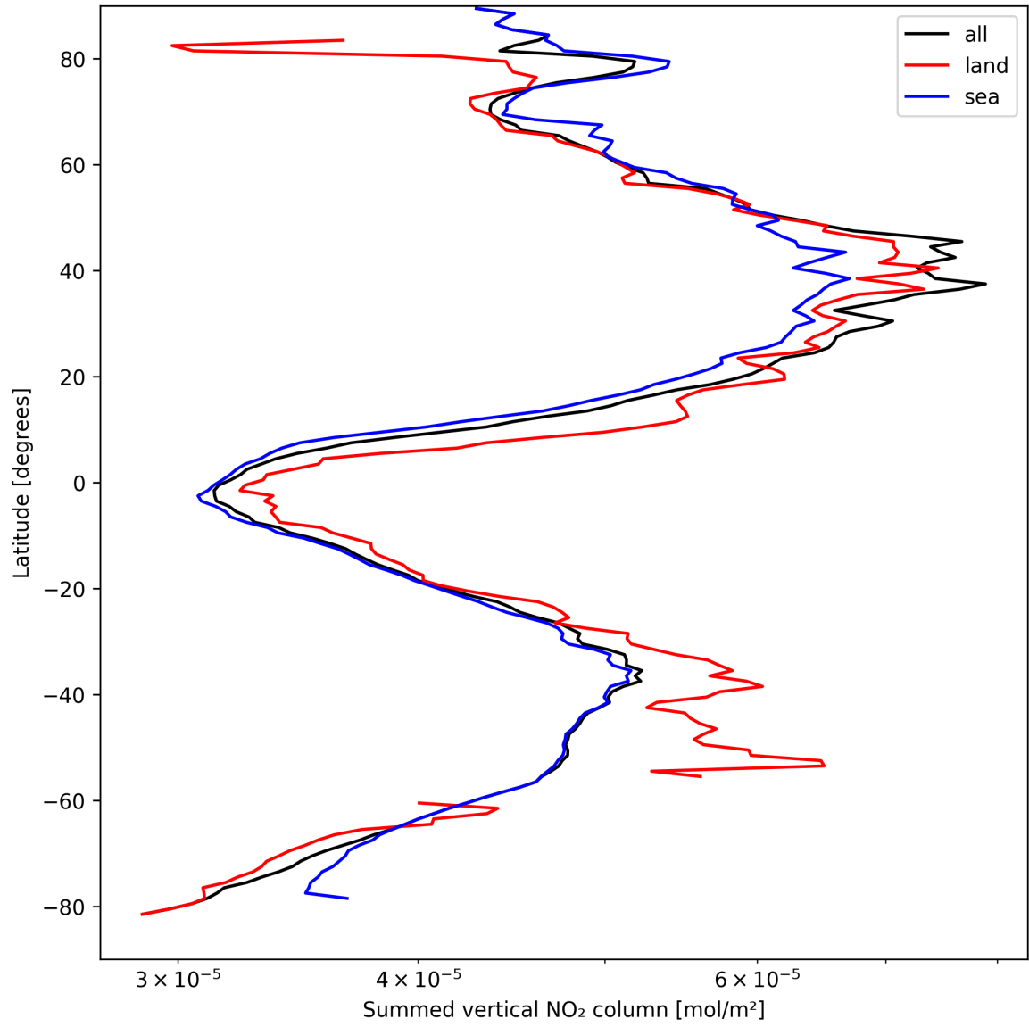
Figure 21: Zonal average of “Summed vertical NO 2 column” for 2025-04-05 to 2025-04-06.
