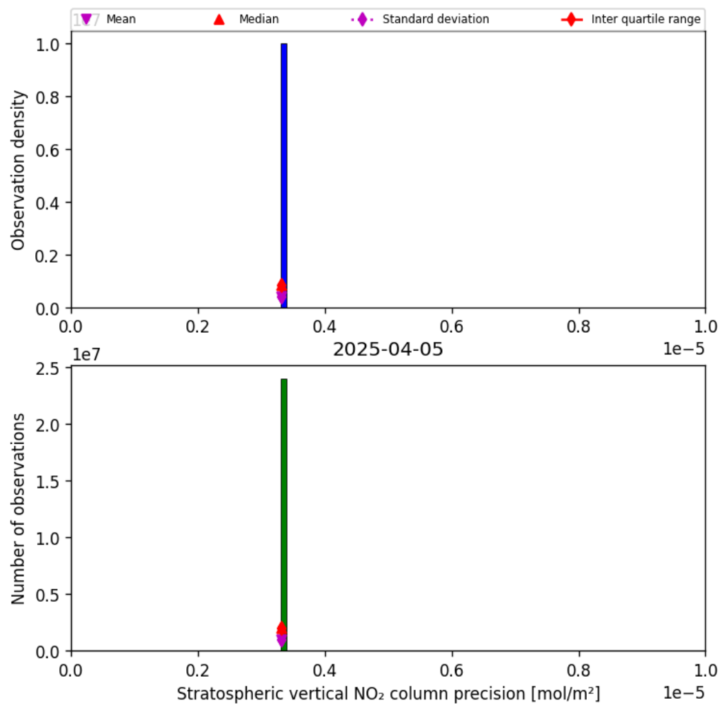
Figure 35: Histogram of “Stratospheric vertical NO 2 column precision” for 2025-04-05 to 2025-04-06
