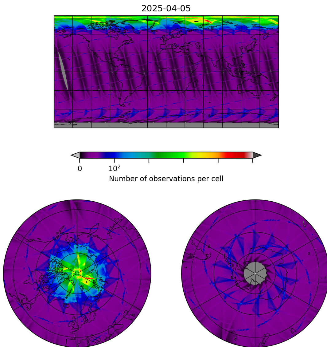
Figure 8: Map of the number of observations for 2025-04-05 to 2025-04-06
