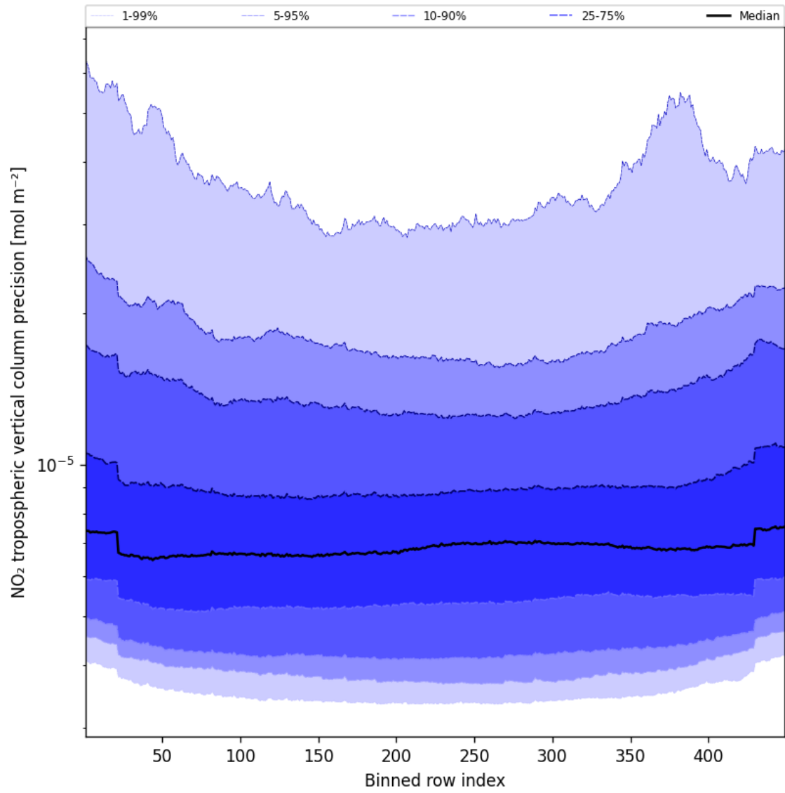
Figure 45: Along track statistics of “NO 2 tropospheric vertical column precision” for 2025-04-05 to 2025-04-06
