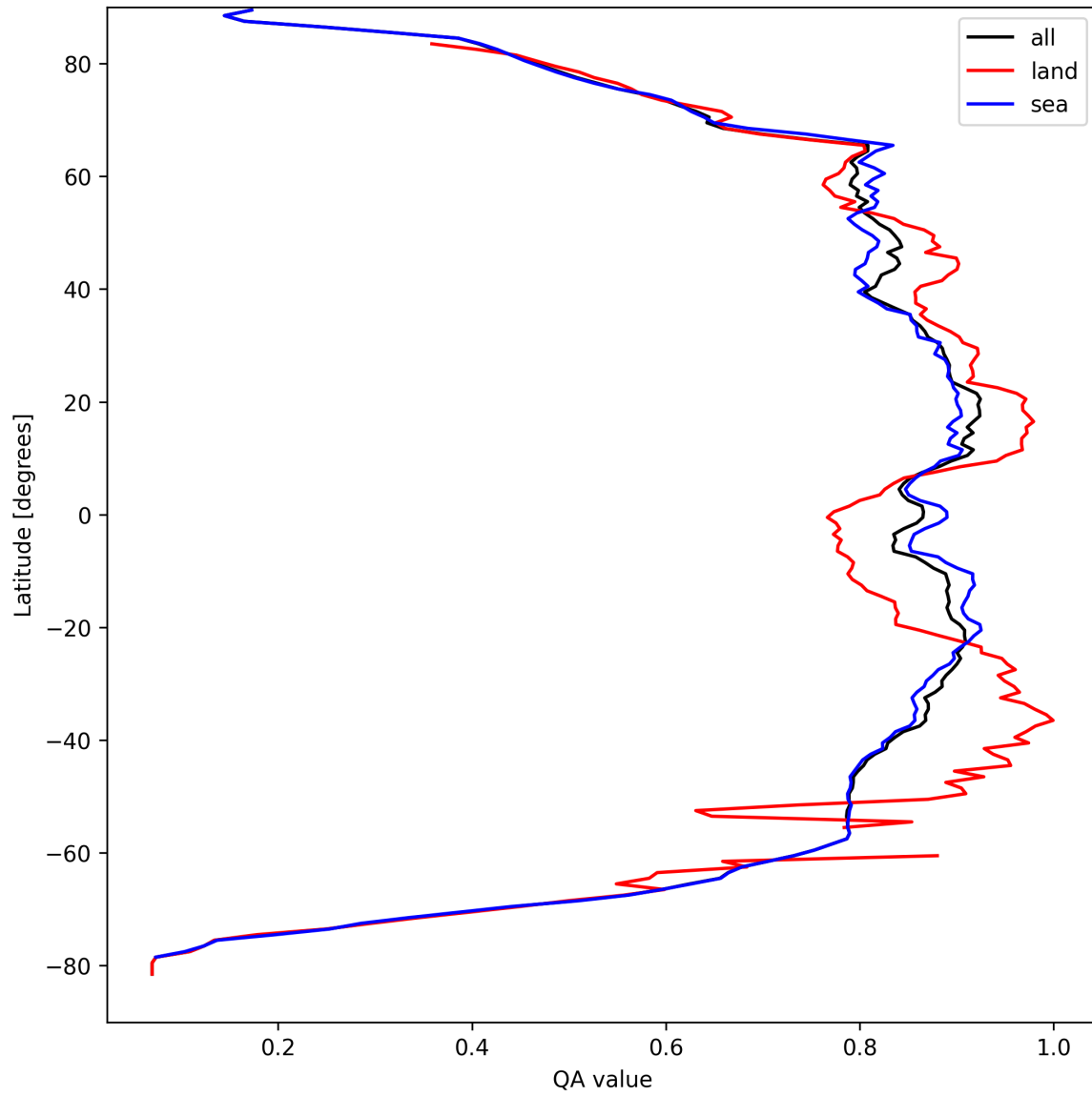
Figure 9: Zonal average of “QA value” for 2025-04-05 to 2025-04-06.
