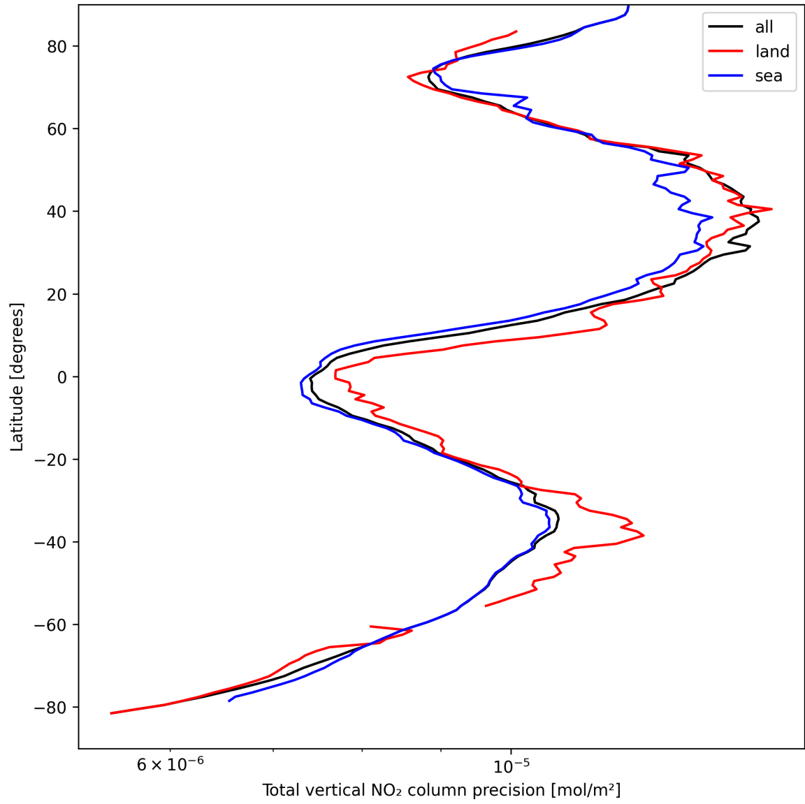
Figure 20: Zonal average of “Total vertical NO 2 column precision” for 2025-04-05 to 2025-04-06.
