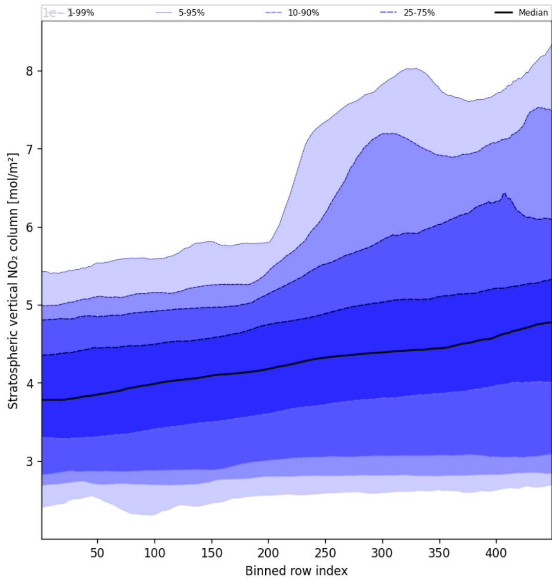
Figure 51: Along track statistics of “Stratospheric vertical NO 2 column” for 2025-04-05 to 2025-04-06
