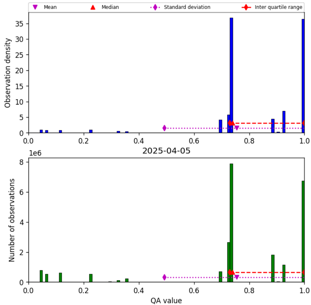
Figure 26: Histogram of “QA value” for 2025-04-05 to 2025-04-06
