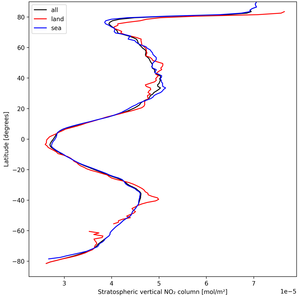
Figure 17: Zonal average of “Stratospheric vertical NO 2 column” for 2025-04-05 to 2025-04-06.
