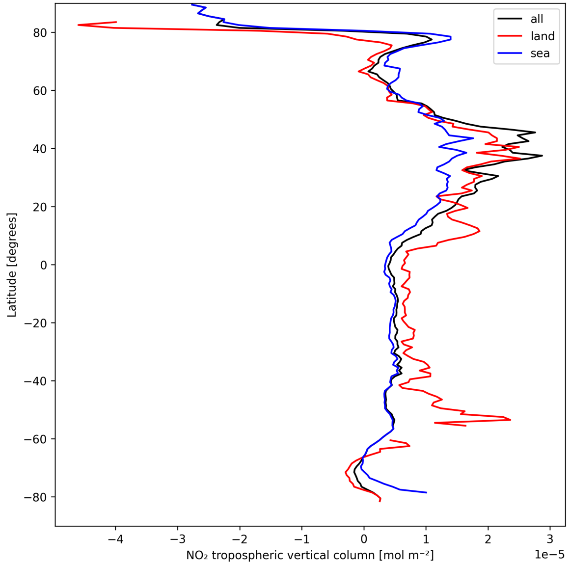
Figure 10: Zonal average of “NO 2 tropospheric vertical column” for 2025-04-05 to 2025-04-06.
