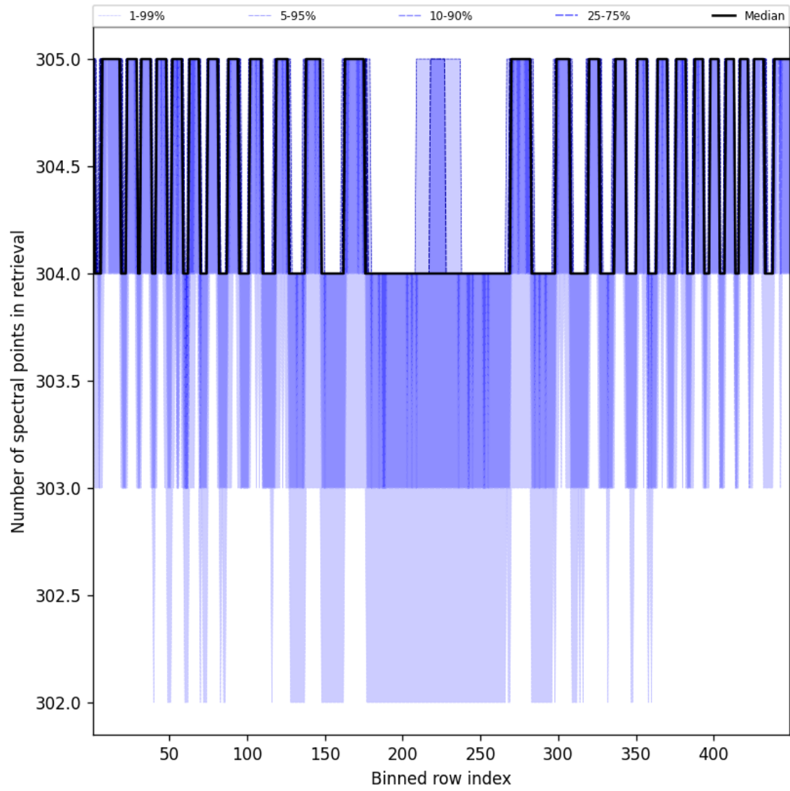
Figure 48: Along track statistics of “Number of spectral points in retrieval” for 2025-04-05 to 2025-04-06
