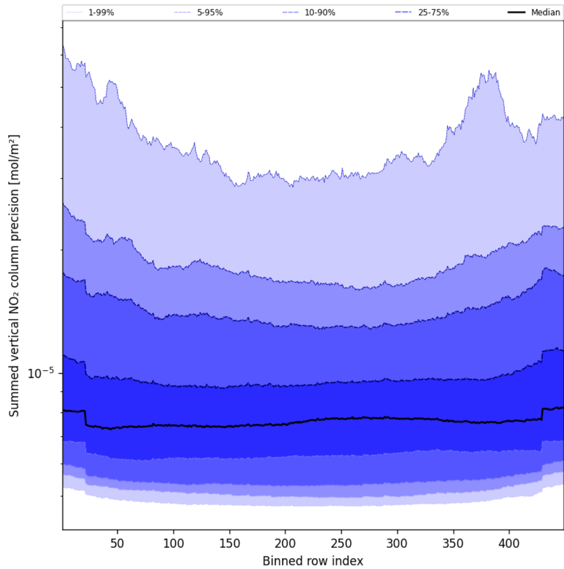
Figure 56: Along track statistics of “Summed vertical NO 2 column precision” for 2025-04-05 to 2025-04-06
