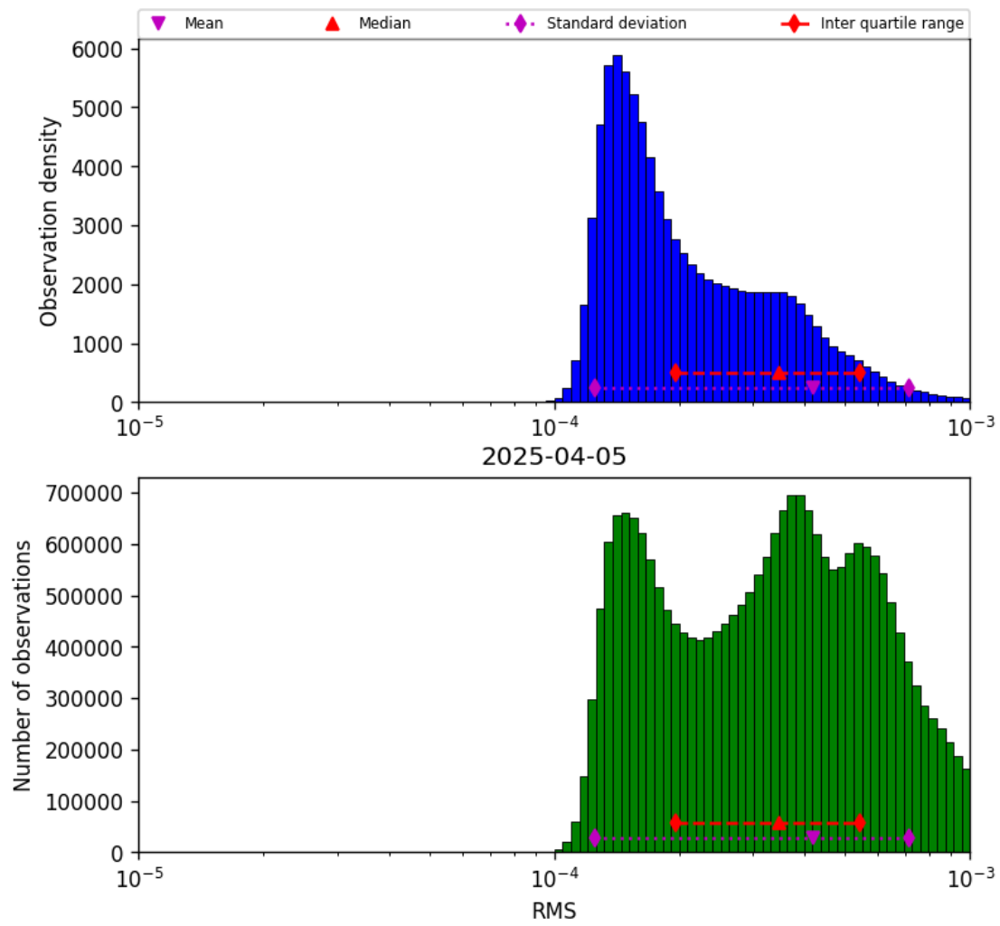
Figure 41: Histogram of “RMS” for 2025-04-05 to 2025-04-06
