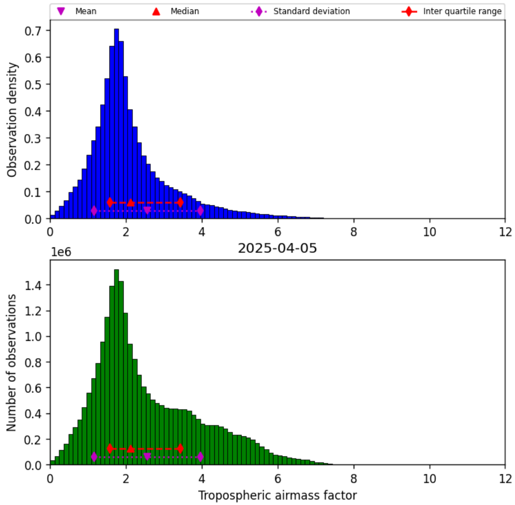
Figure 29: Histogram of “Tropospheric airmass factor” for 2025-04-05 to 2025-04-06
