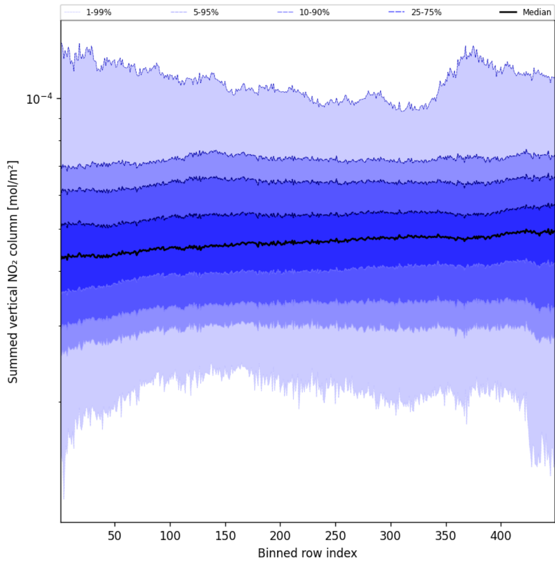
Figure 55: Along track statistics of “Summed vertical NO 2 column” for 2025-04-05 to 2025-04-06
