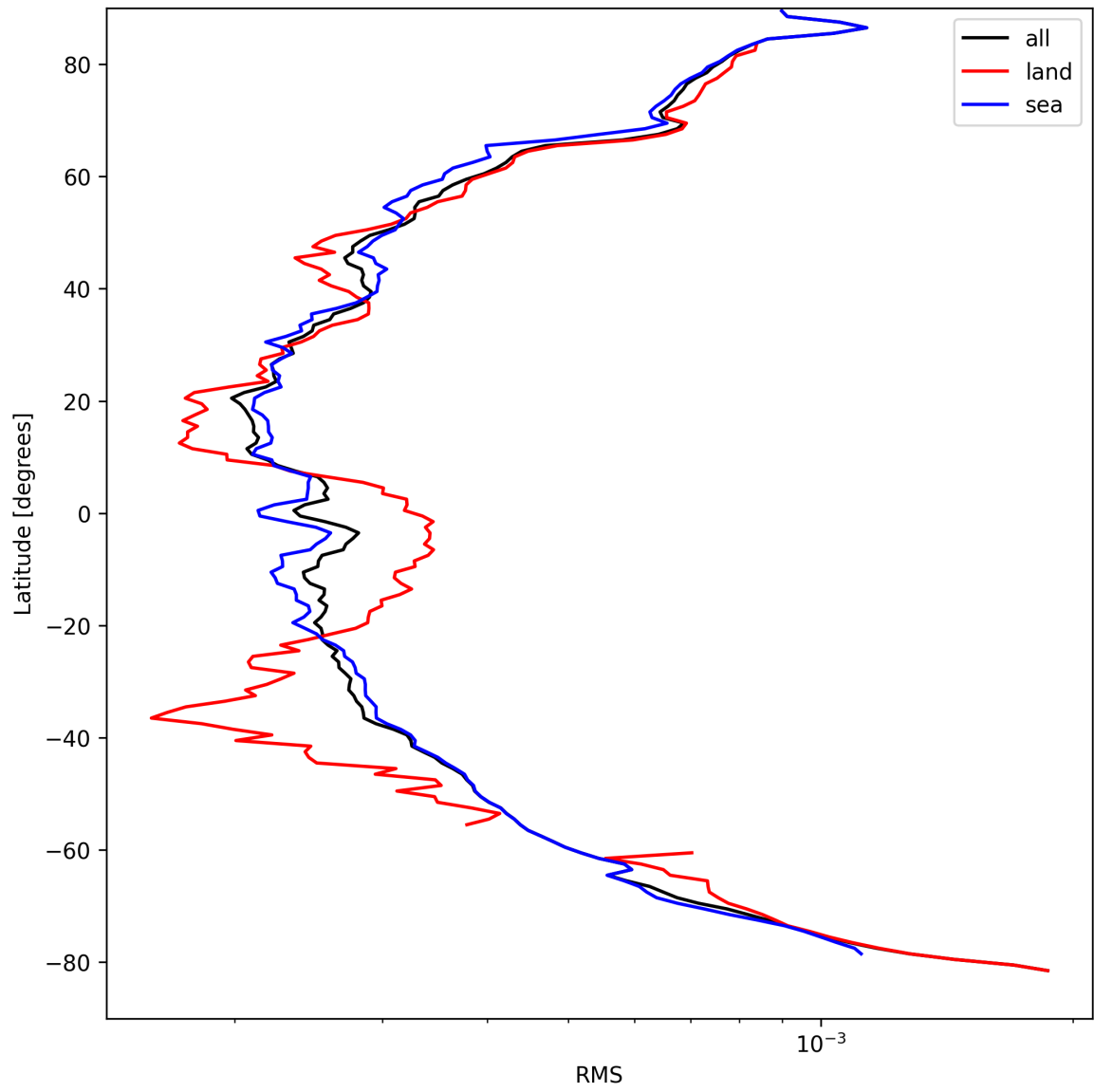
Figure 24: Zonal average of “RMS” for 2025-04-05 to 2025-04-06.
