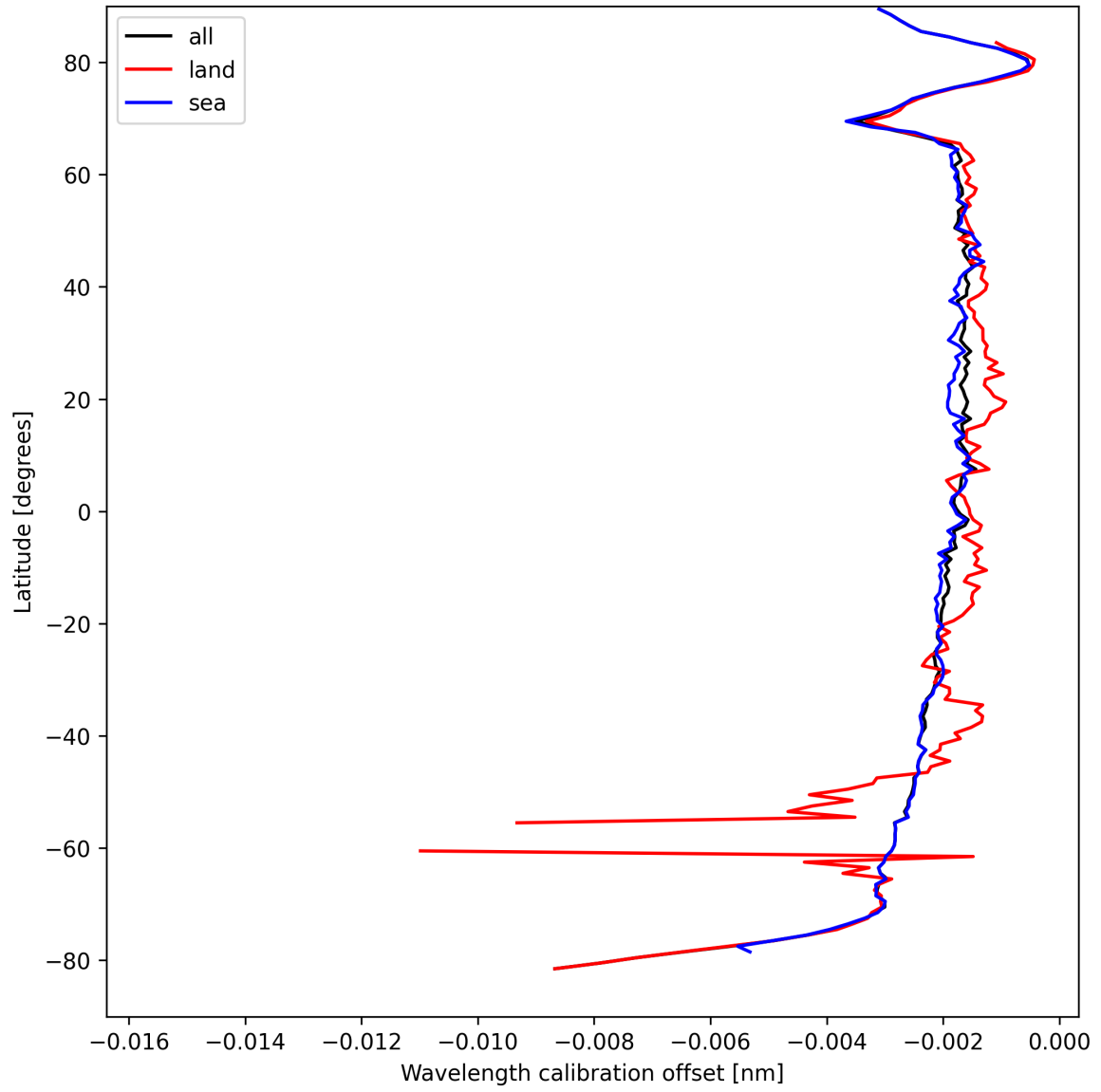
Figure 16: Zonal average of “Wavelength calibration offset” for 2025-04-05 to 2025-04-06.
