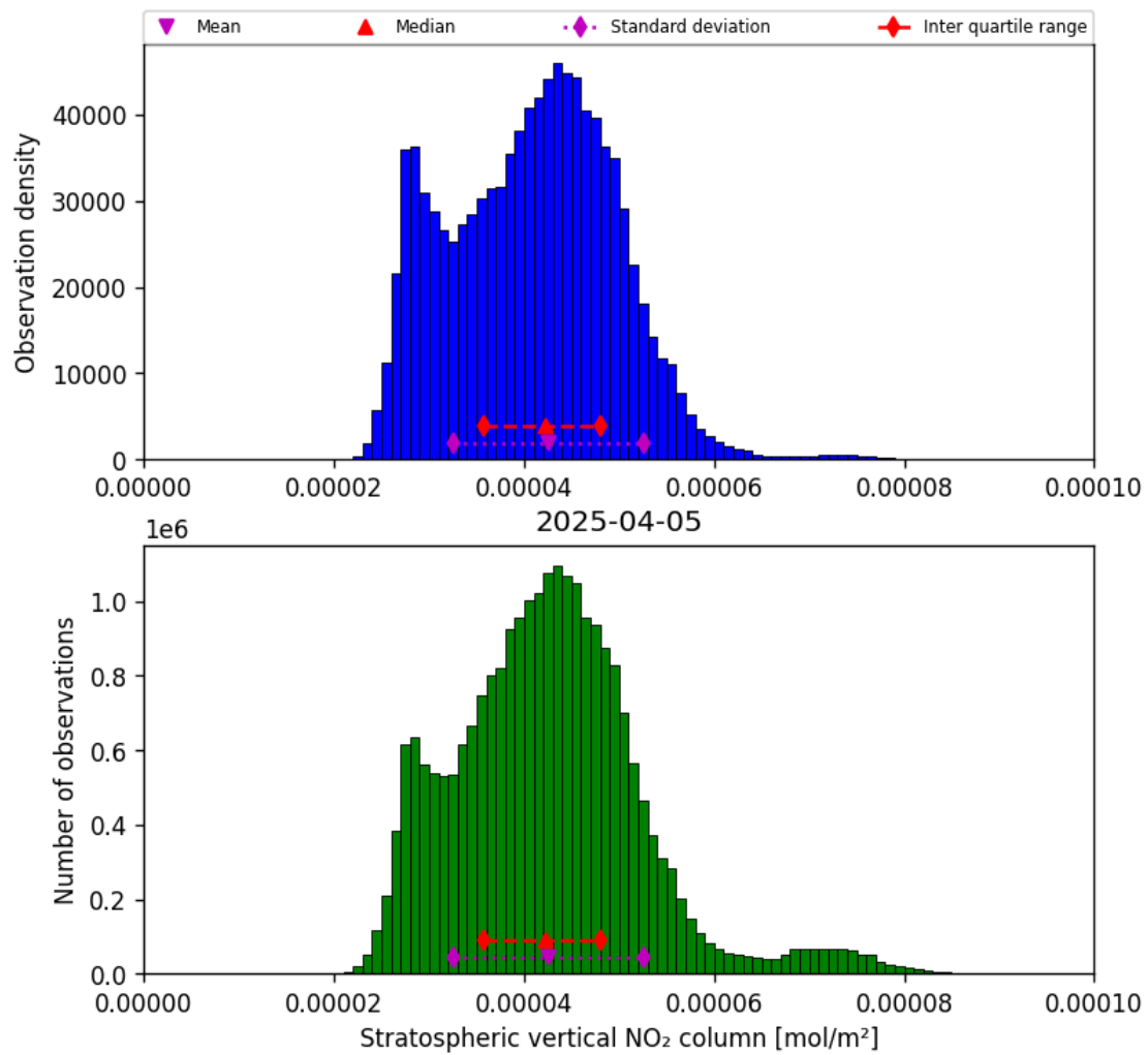
Figure 34: Histogram of “Stratospheric vertical NO 2 column” for 2025-04-05 to 2025-04-06
