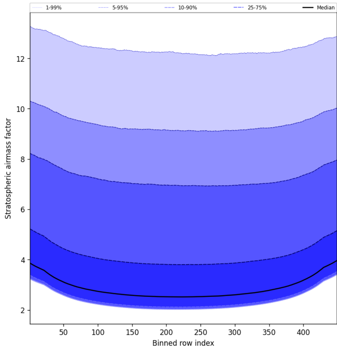
Figure 59: Along track statistics of “Stratospheric airmass factor” for 2025-04-05 to 2025-04-06
