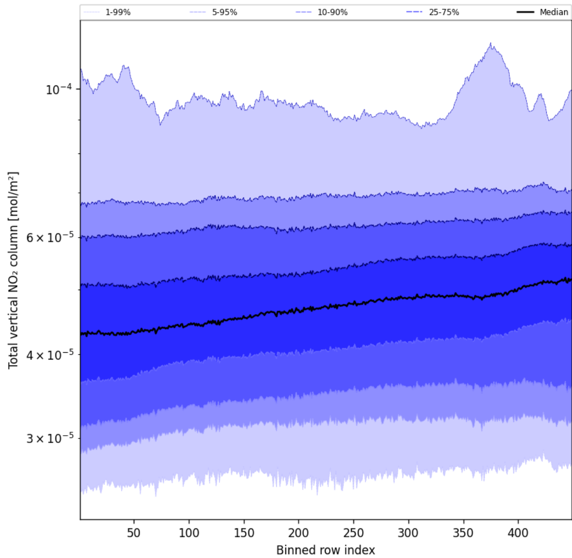
Figure 53: Along track statistics of “Total vertical NO 2 column” for 2025-04-05 to 2025-04-06
