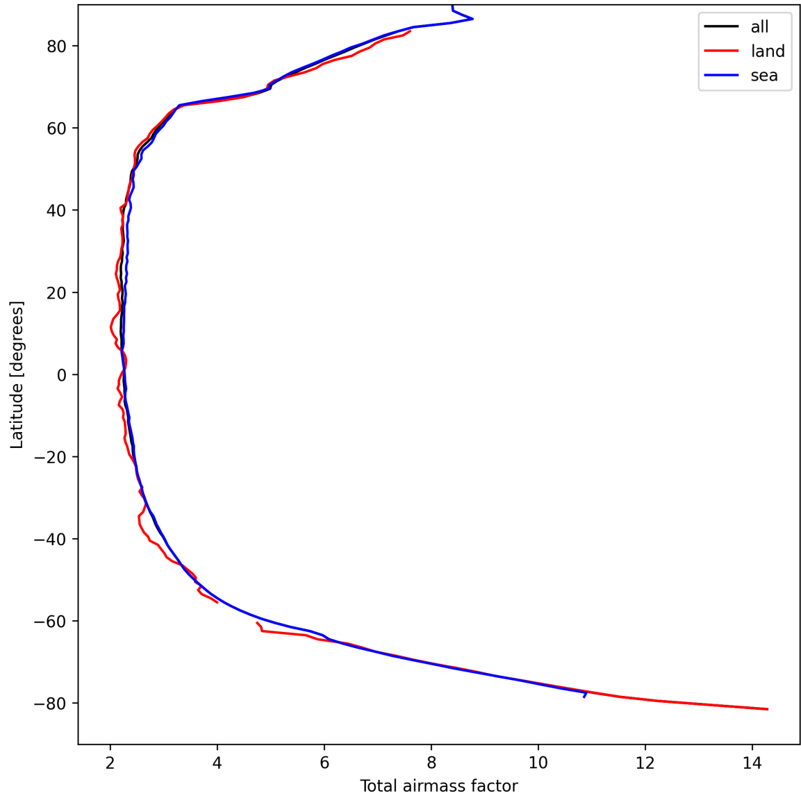
Figure 13: Zonal average of “Total airmass factor” for 2025-04-05 to 2025-04-06.
