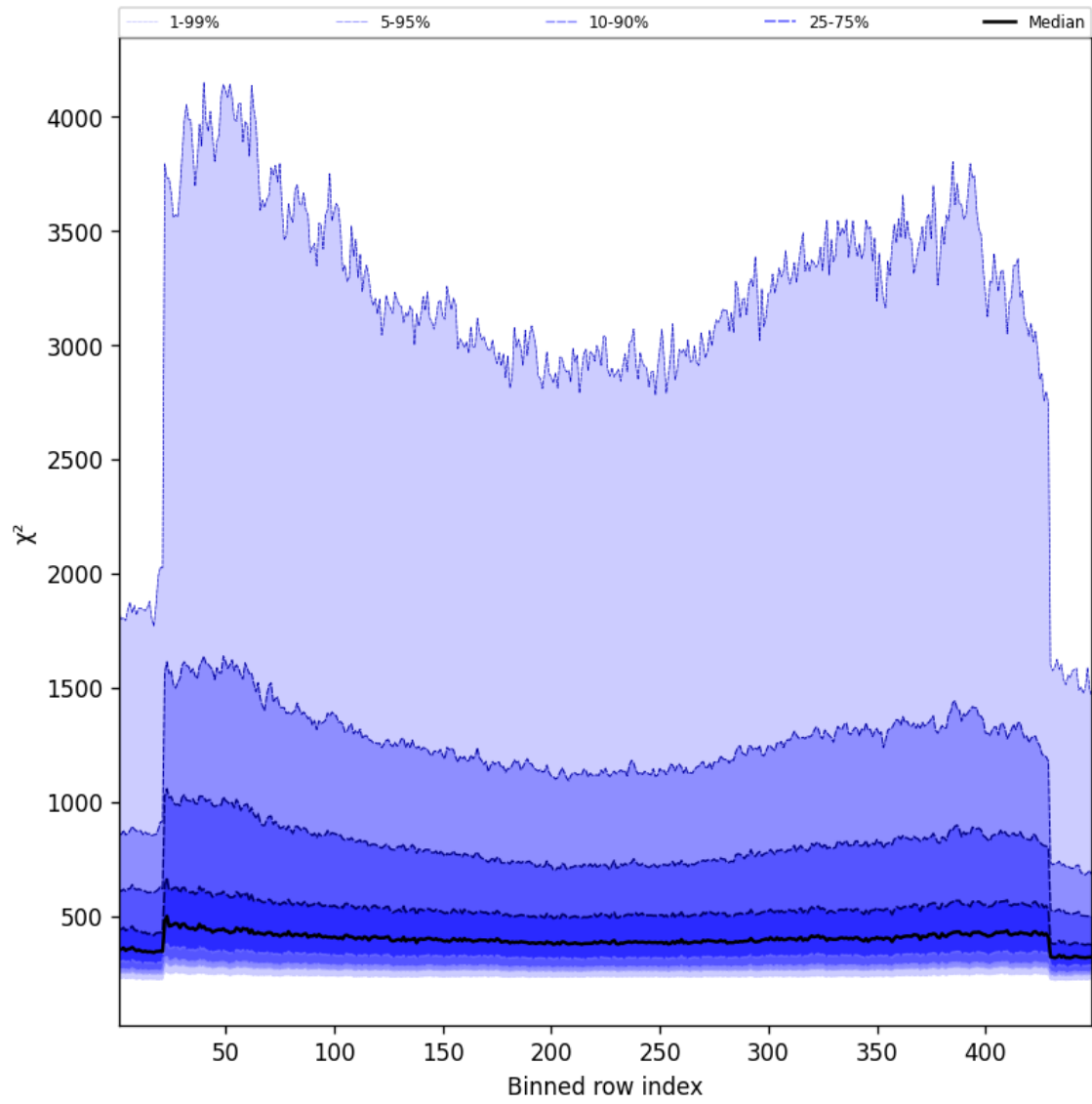
Figure 57: Along track statistics of “ \chi^2 ” for 2025-04-05 to 2025-04-06
