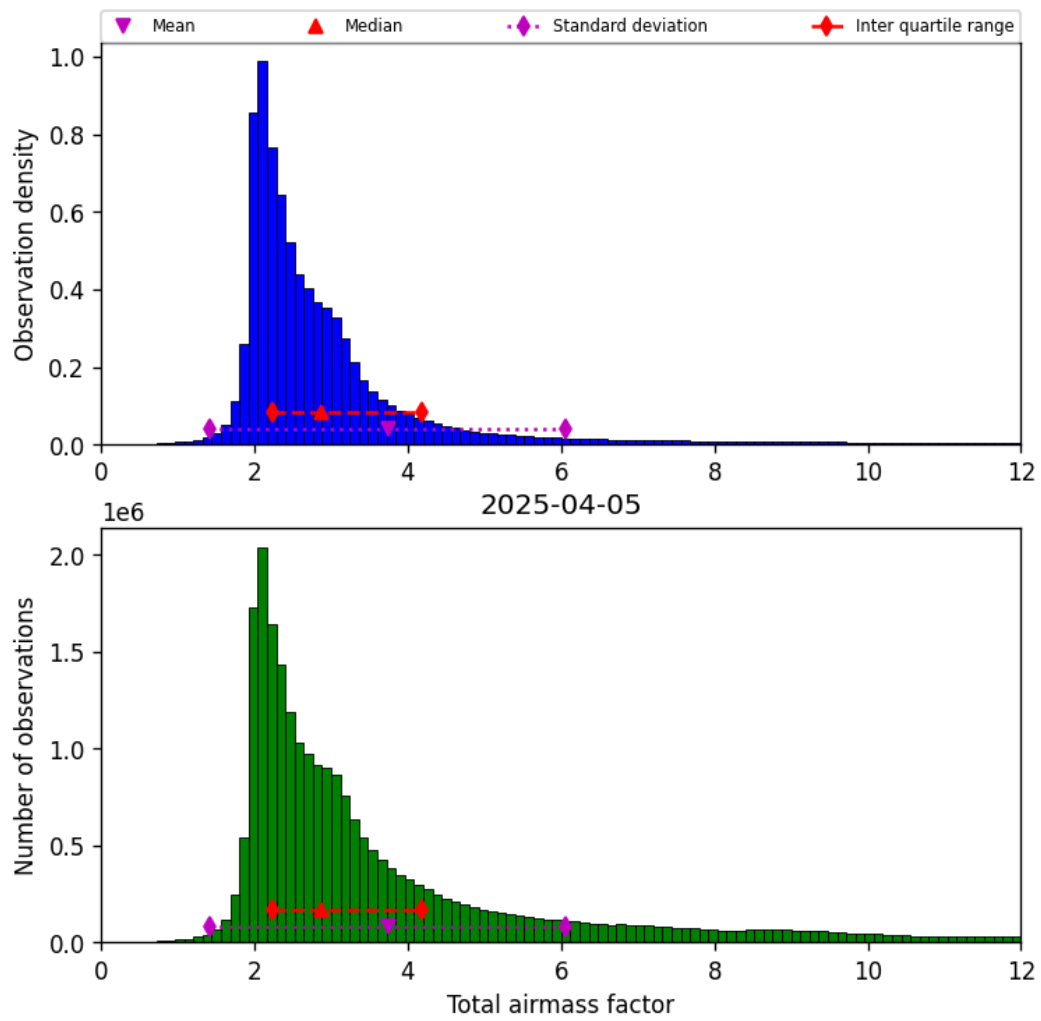
Figure 30: Histogram of “Total airmass factor” for 2025-04-05 to 2025-04-06
