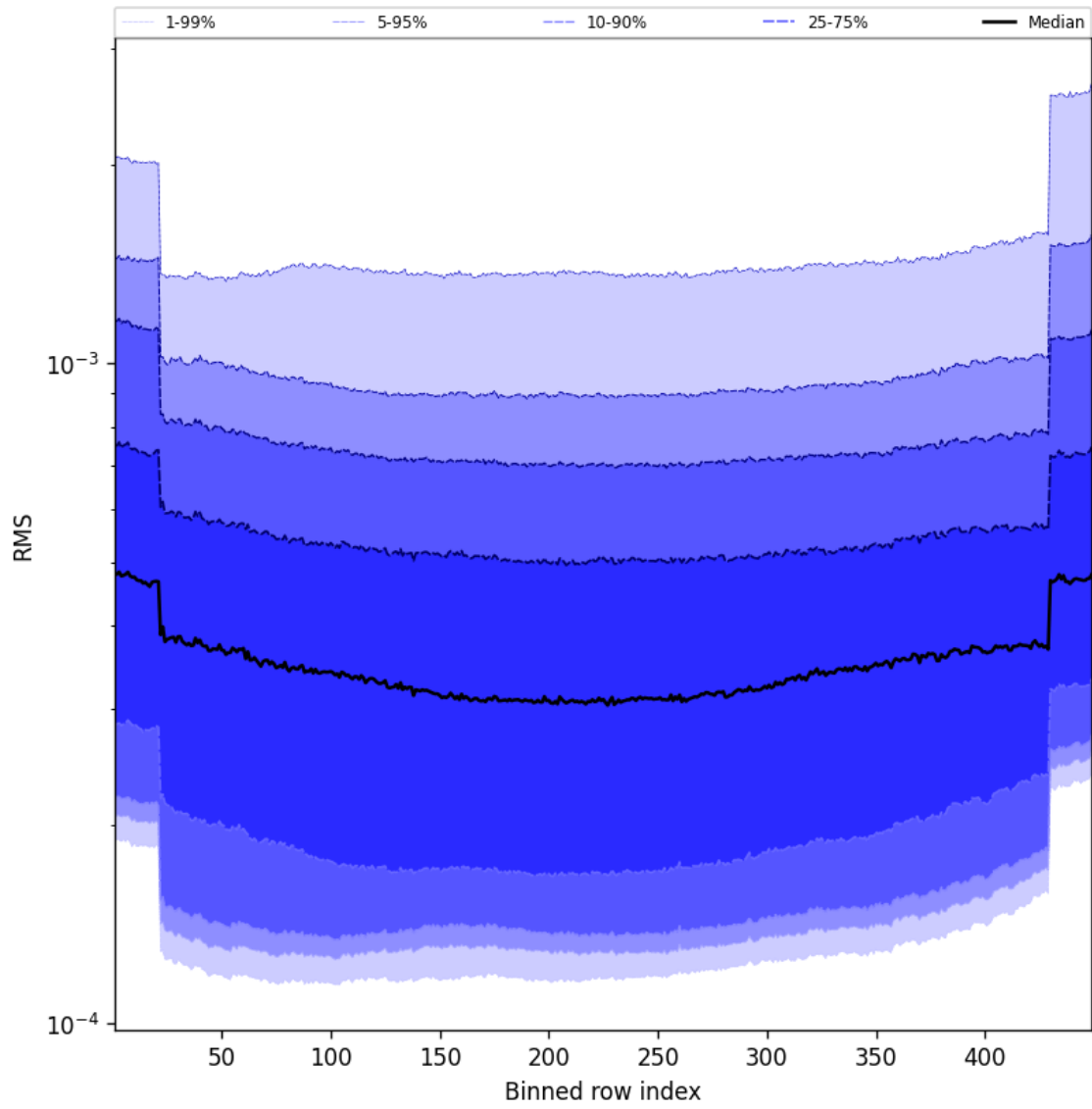
Figure 58: Along track statistics of “RMS” for 2025-04-05 to 2025-04-06
