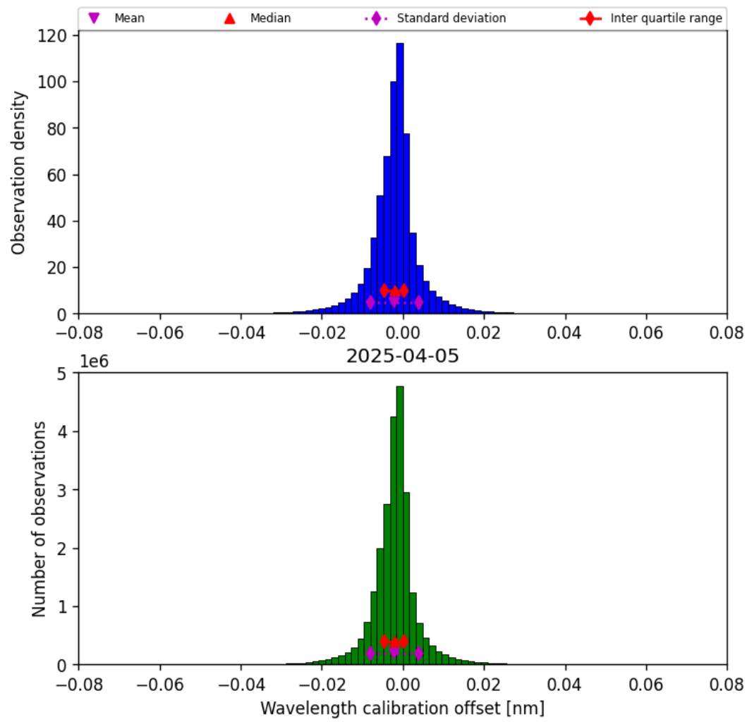
Figure 33: Histogram of “Wavelength calibration offset” for 2025-04-05 to 2025-04-06
