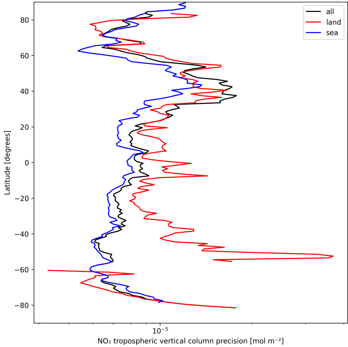
Figure 11: Zonal average of “NO 2 tropospheric vertical column precision” for 2025-04-05 to 2025-04-06.
