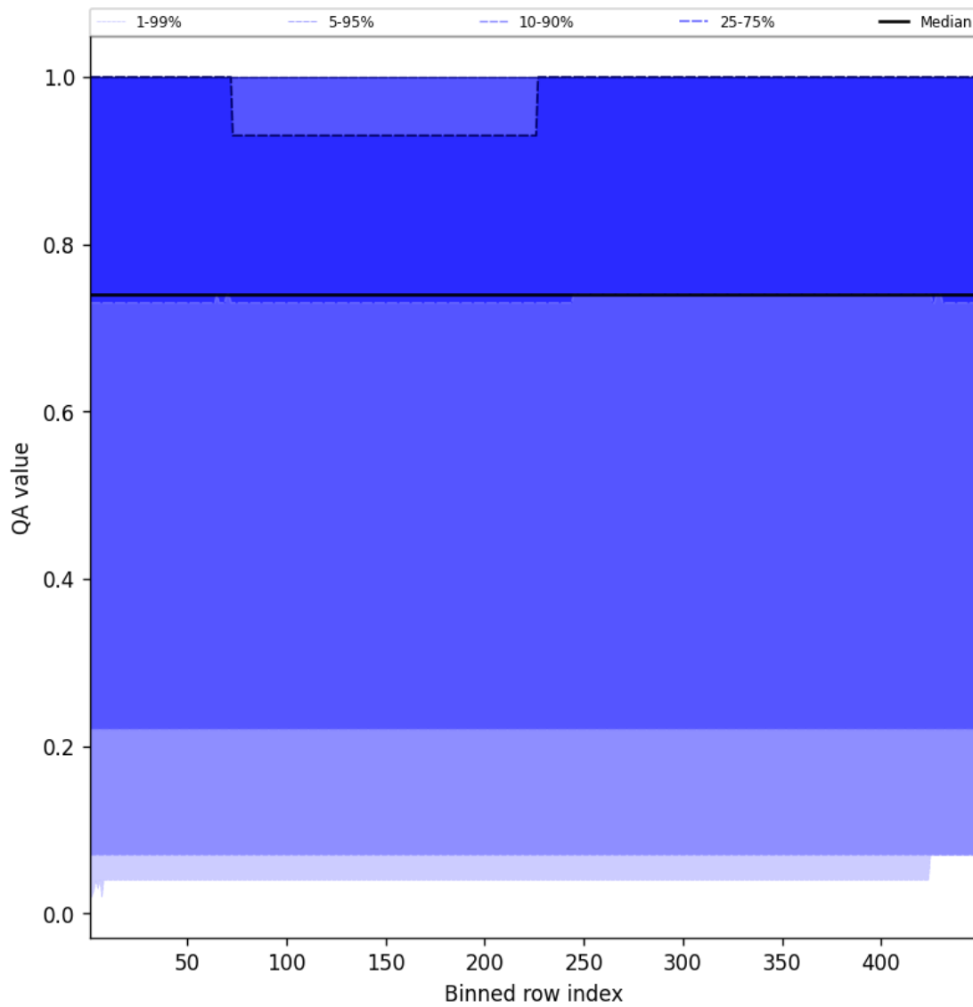
Figure 43: Along track statistics of “QA value” for 2025-04-05 to 2025-04-06
