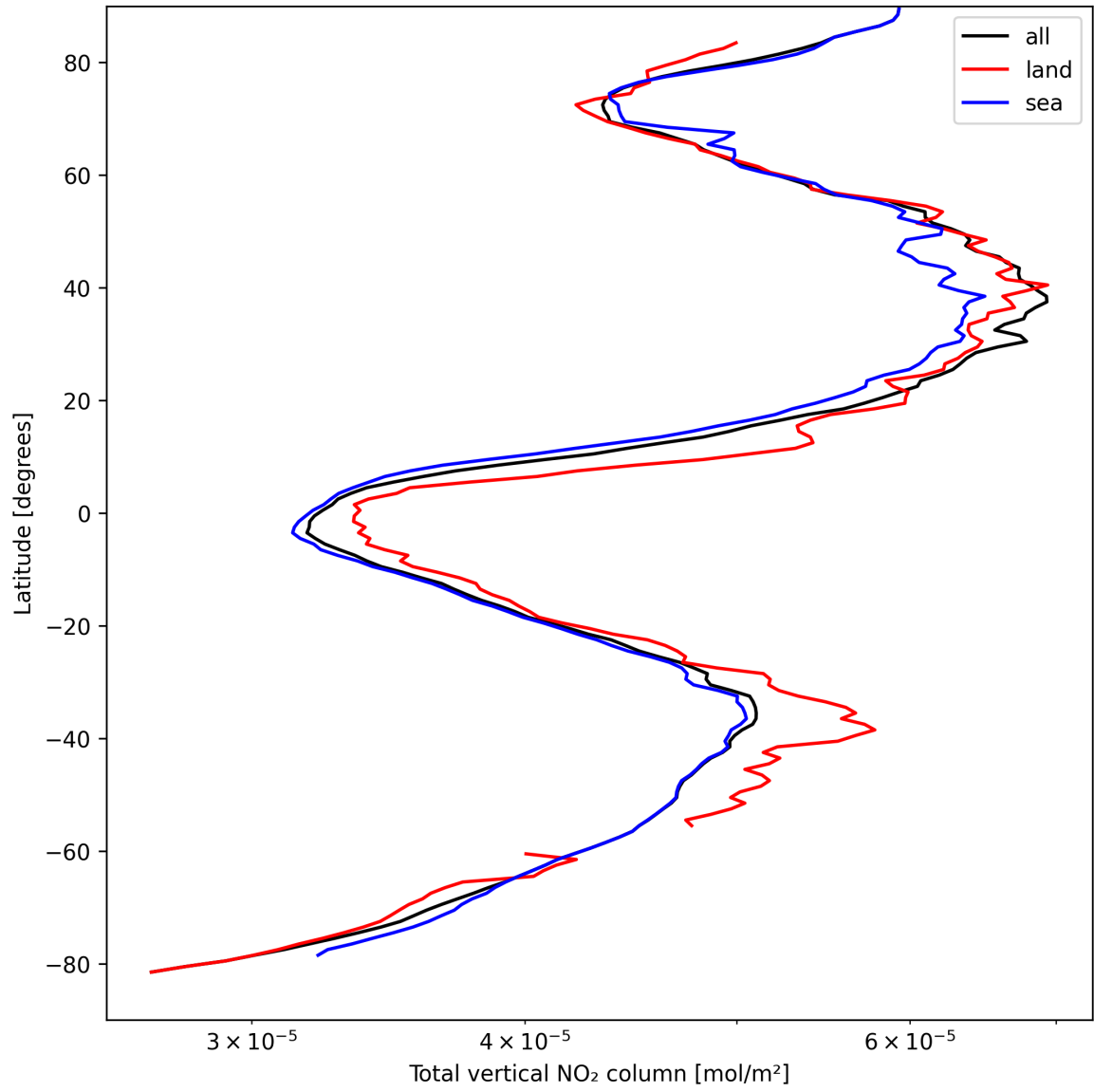
Figure 19: Zonal average of “Total vertical NO 2 column” for 2025-04-05 to 2025-04-06.
