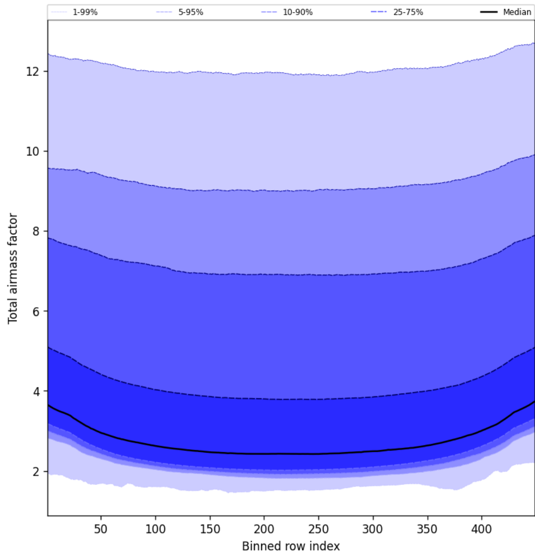
Figure 47: Along track statistics of “Total airmass factor” for 2025-04-05 to 2025-04-06
