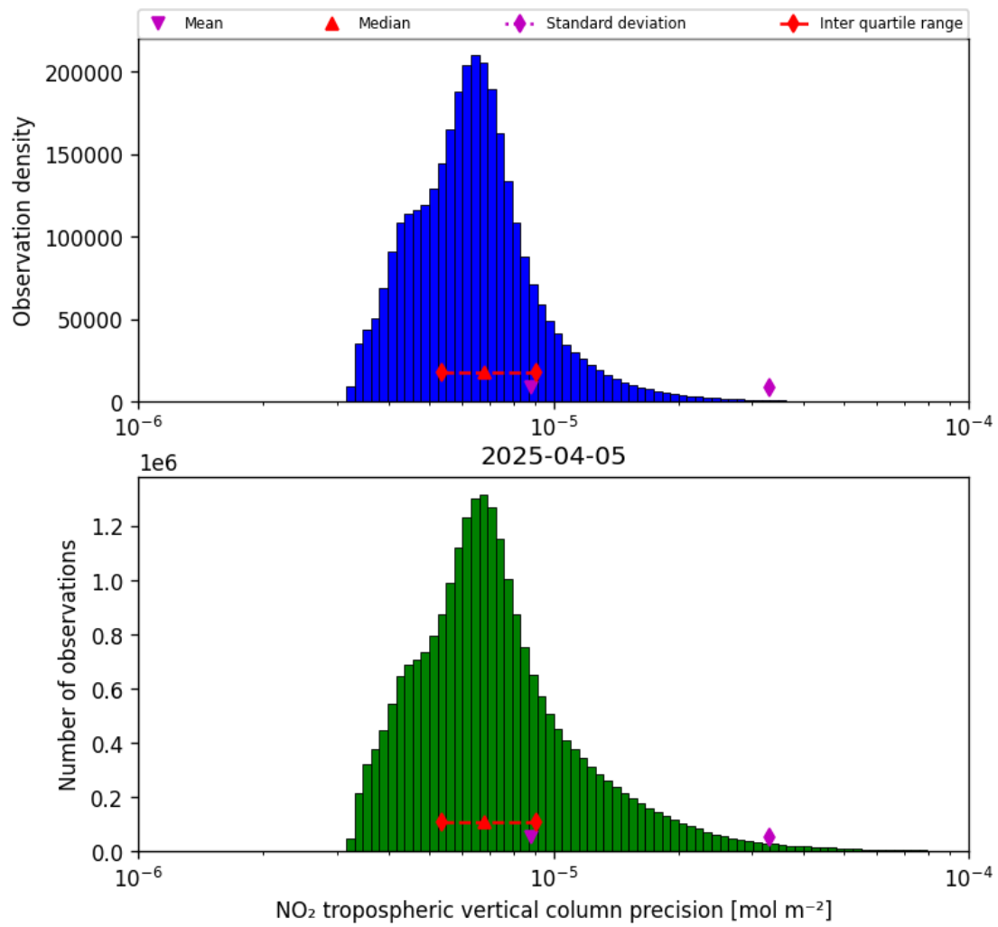
Figure 28: Histogram of “NO 2 tropospheric vertical column precision” for 2025-04-05 to 2025-04-06
