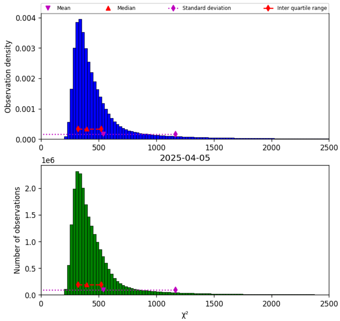
Figure 40: Histogram of “ \chi^2 ” for 2025-04-05 to 2025-04-06
