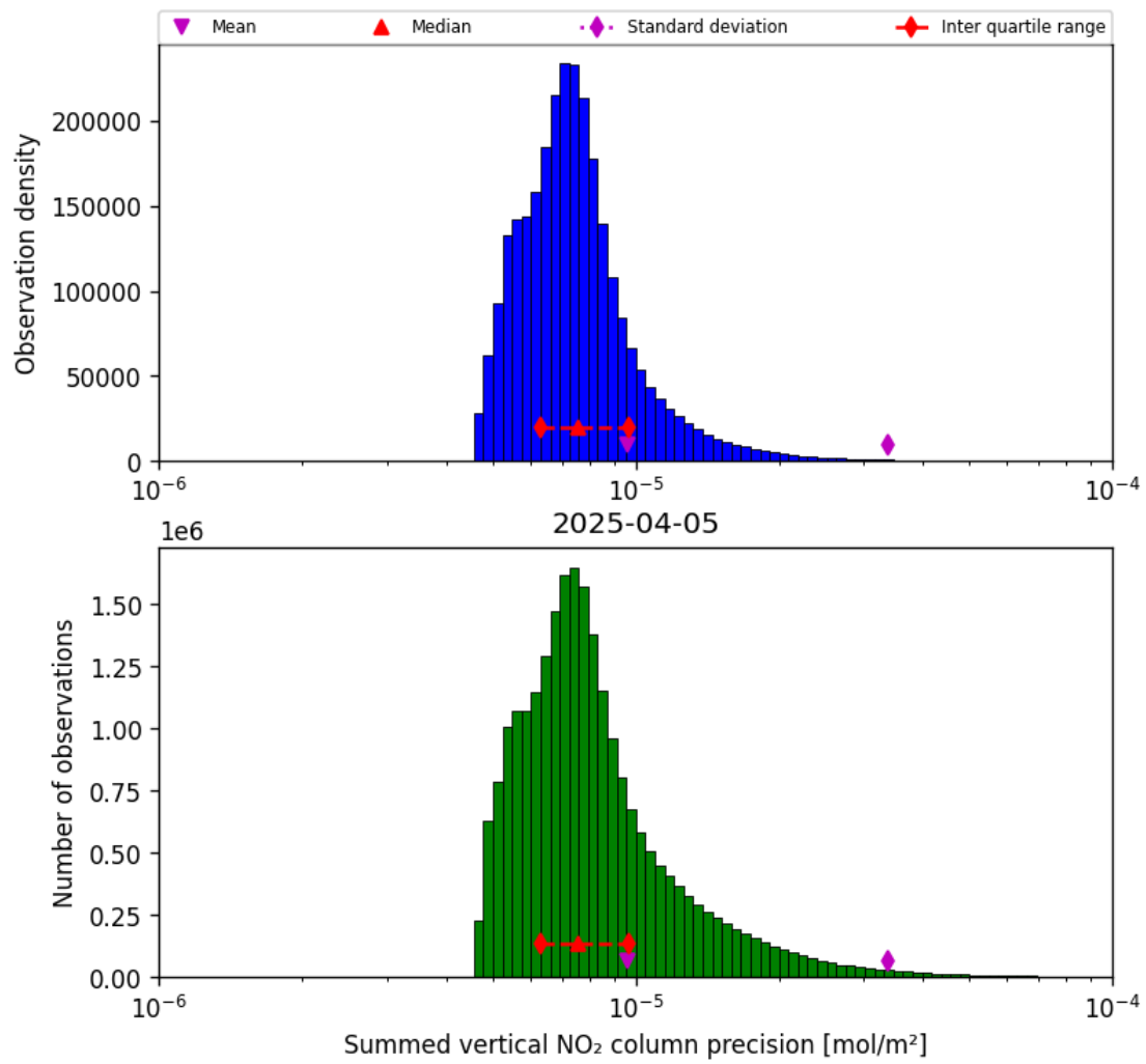
Figure 39: Histogram of "Summed vertical NO 2 column precision" for 2025-04-05 to 2025-04-06
