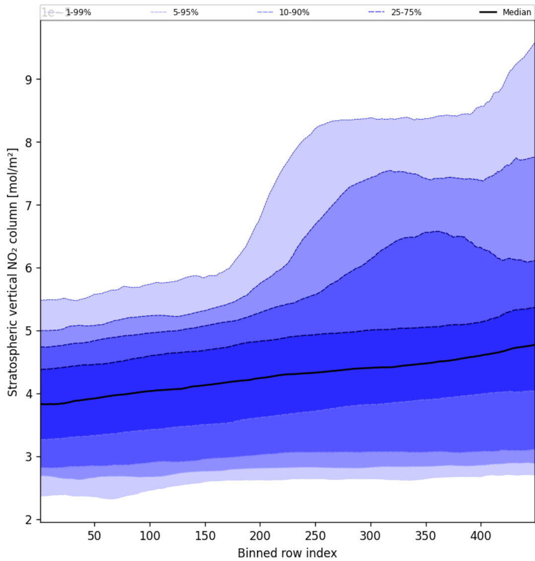
Figure 51: Along track statistics of “Stratospheric vertical NO 2 column” for 2025-04-06 to 2025-04-06
