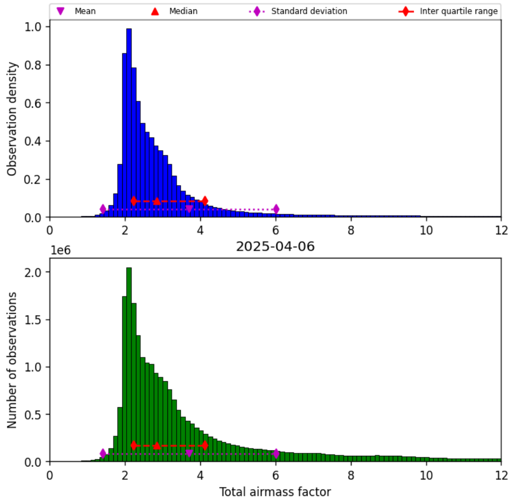
Figure 30: Histogram of “Total airmass factor” for 2025-04-06 to 2025-04-06
