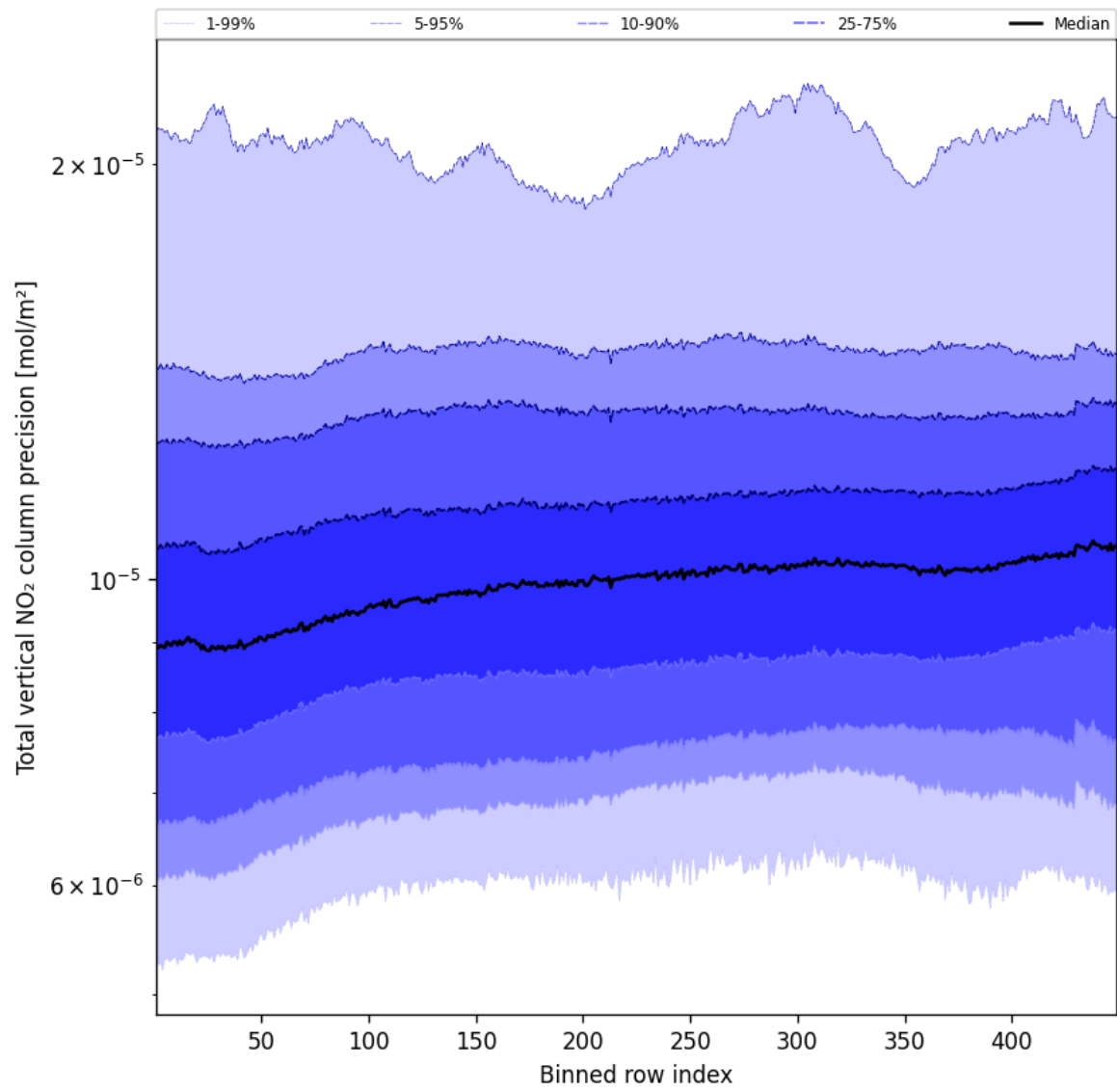
Figure 54: Along track statistics of “Total vertical NO 2 column precision” for 2025-04-06 to 2025-04-06
