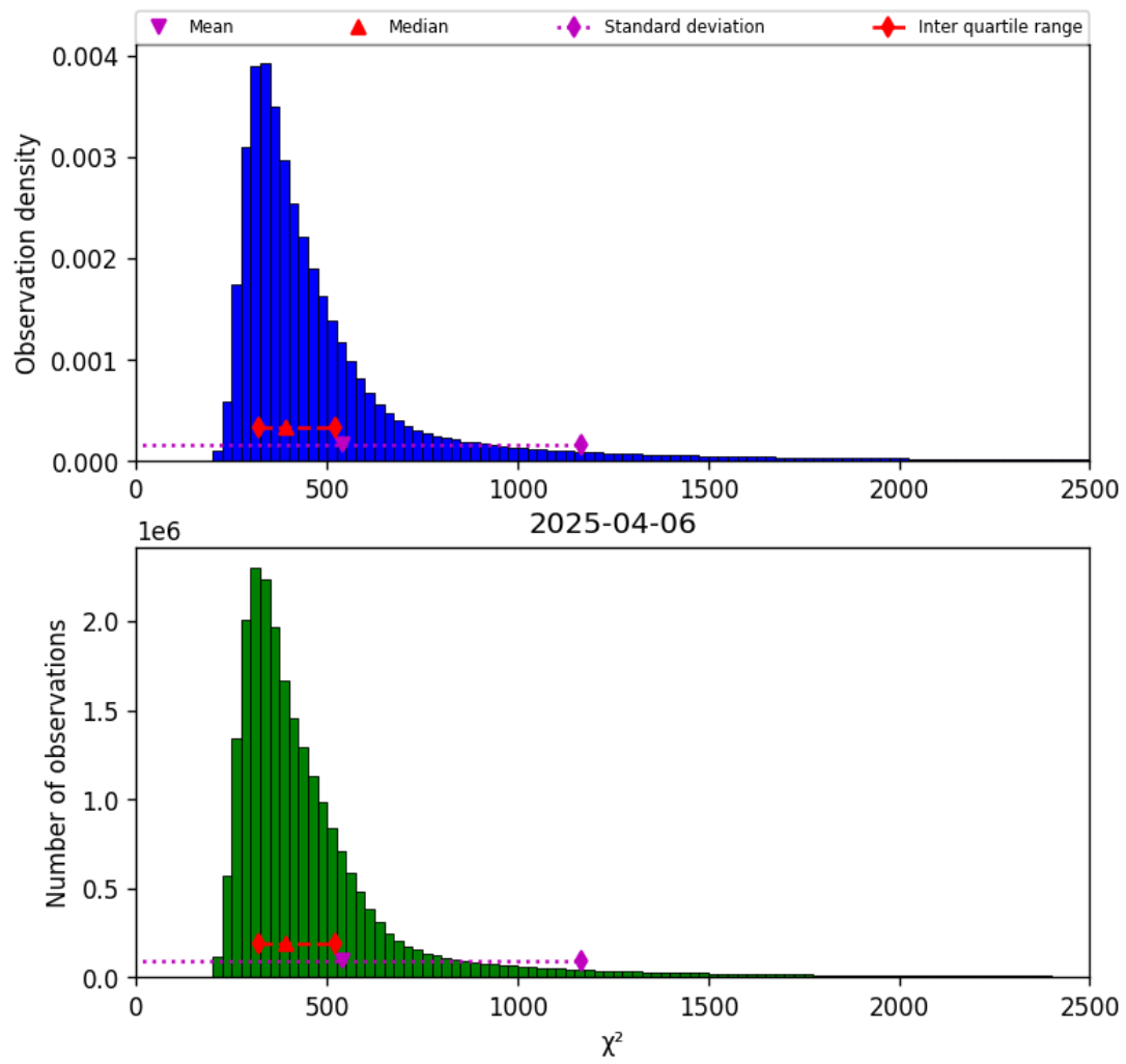
Figure 40: Histogram of " \chi^2 " for 2025-04-06 to 2025-04-06
