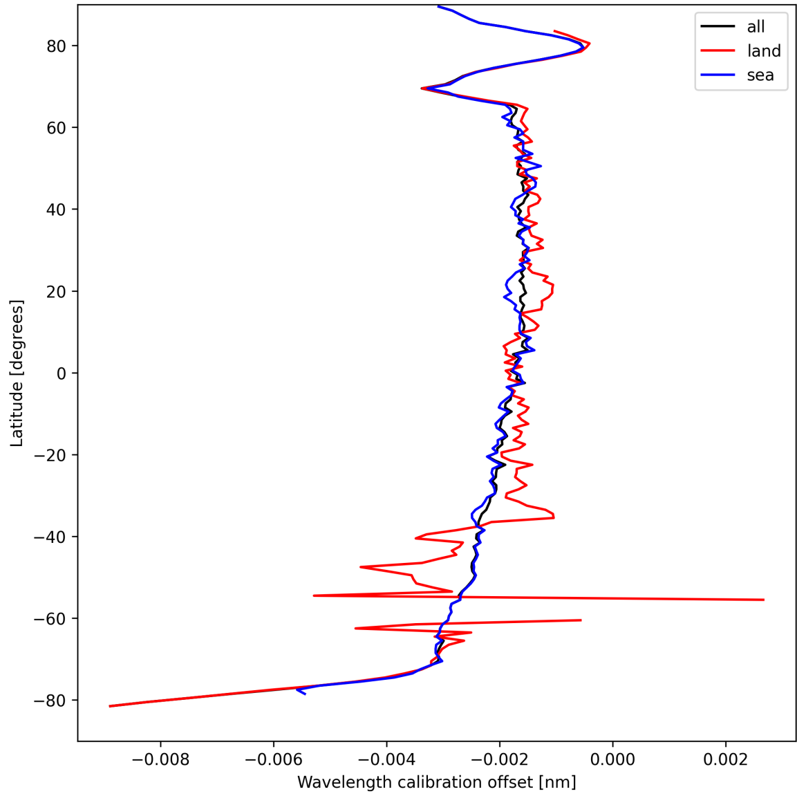
Figure 16: Zonal average of “Wavelength calibration offset” for 2025-04-06 to 2025-04-06.
