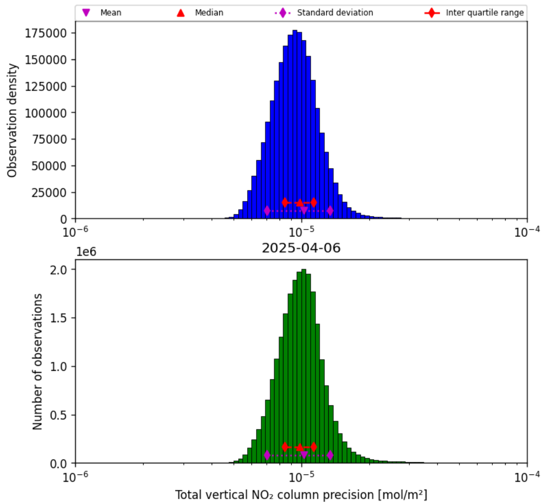
Figure 37: Histogram of "Total vertical NO 2 column precision" for 2025-04-06 to 2025-04-06
