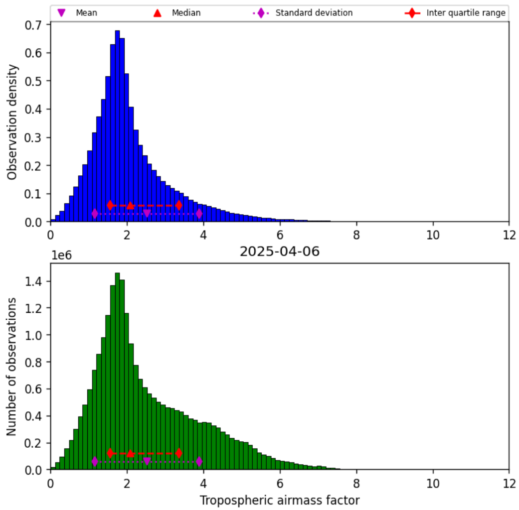
Figure 29: Histogram of “Tropospheric airmass factor” for 2025-04-06 to 2025-04-06
