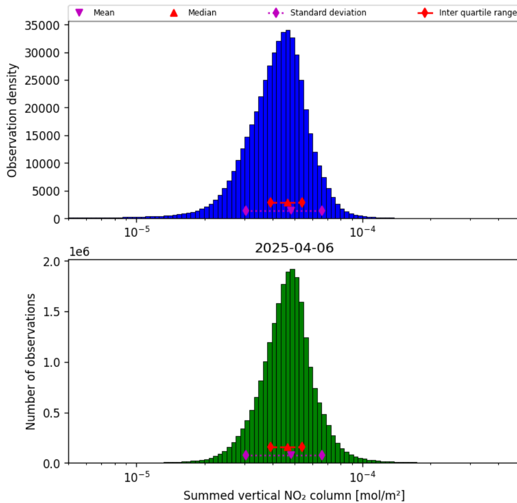
Figure 38: Histogram of “Summed vertical NO 2 column” for 2025-04-06 to 2025-04-06
