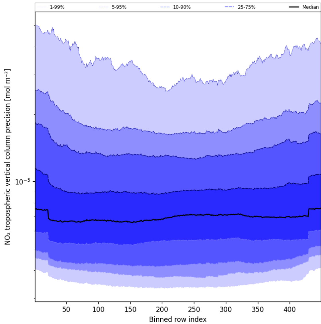
Figure 45: Along track statistics of “NO 2 tropospheric vertical column precision” for 2025-04-06 to 2025-04-06
