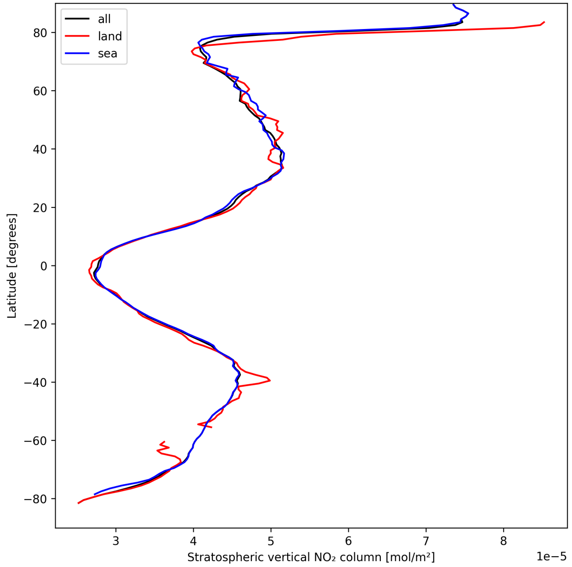
Figure 17: Zonal average of “Stratospheric vertical NO 2 column” for 2025-04-06 to 2025-04-06.
