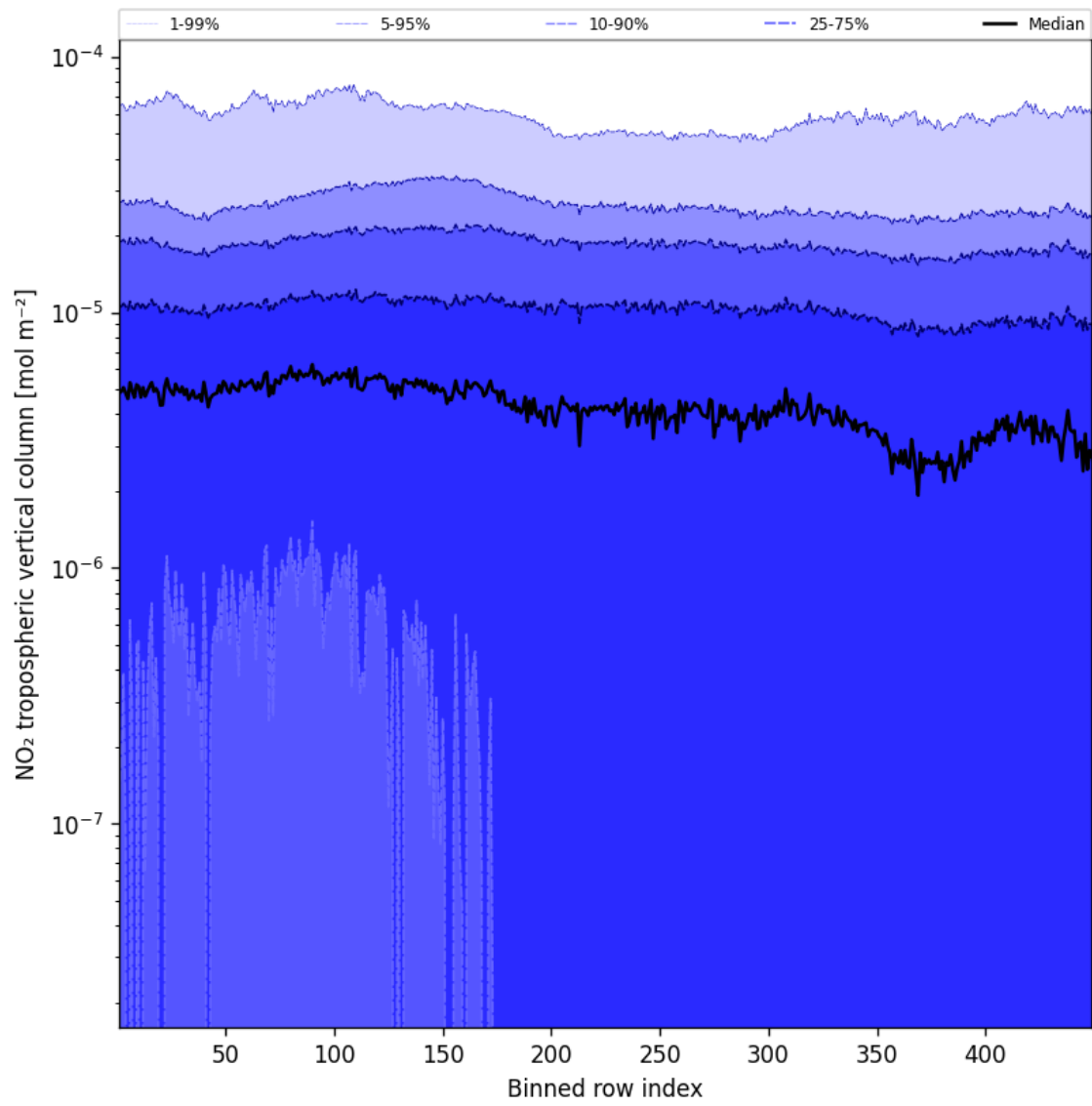
Figure 44: Along track statistics of “NO 2 tropospheric vertical column” for 2025-04-06 to 2025-04-06
