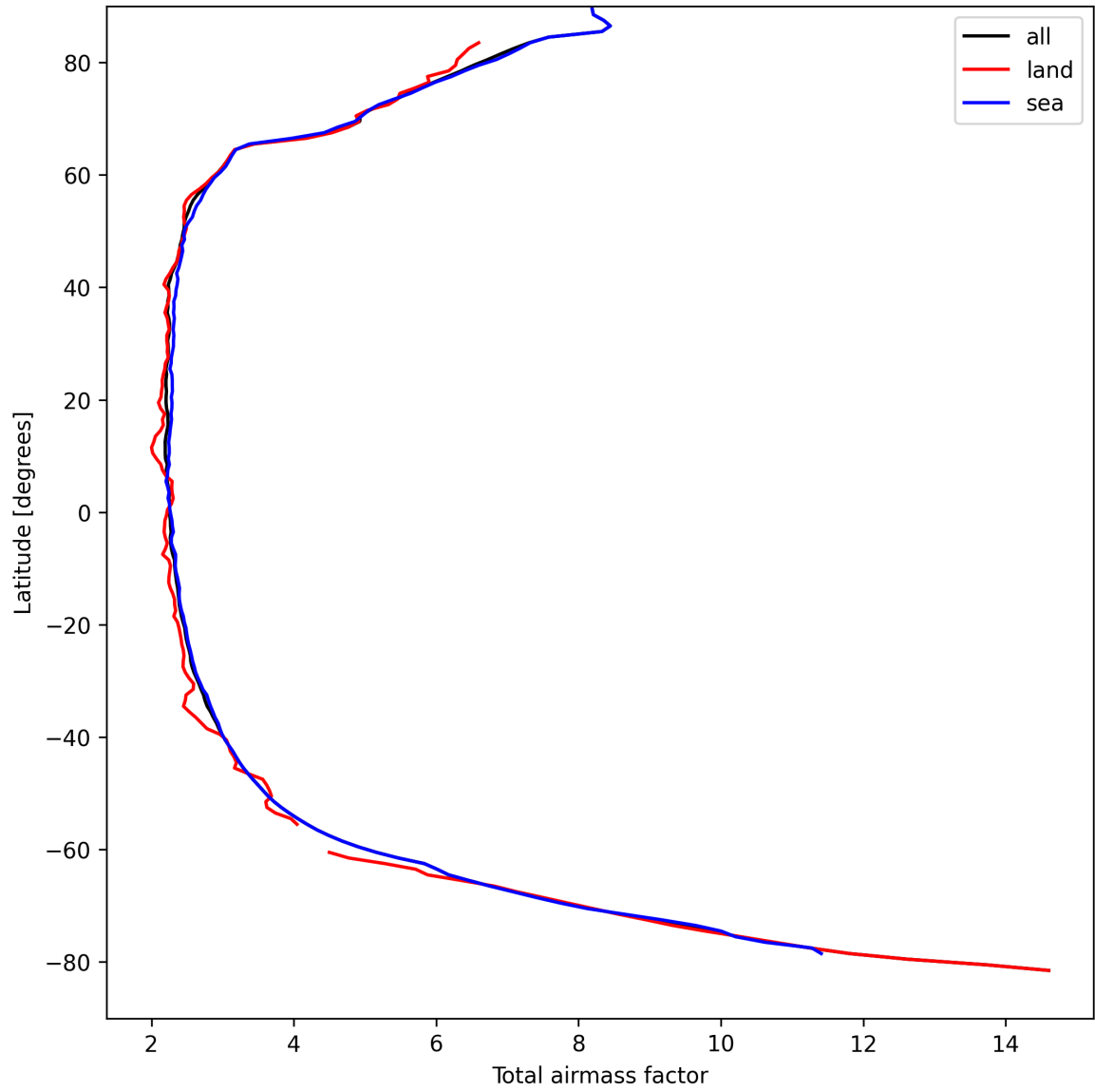
Figure 13: Zonal average of “Total airmass factor” for 2025-04-06 to 2025-04-06.
