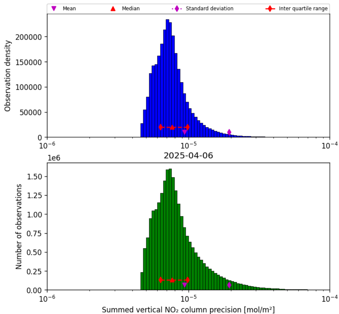
Figure 39: Histogram of "Summed vertical NO 2 column precision" for 2025-04-06 to 2025-04-06
