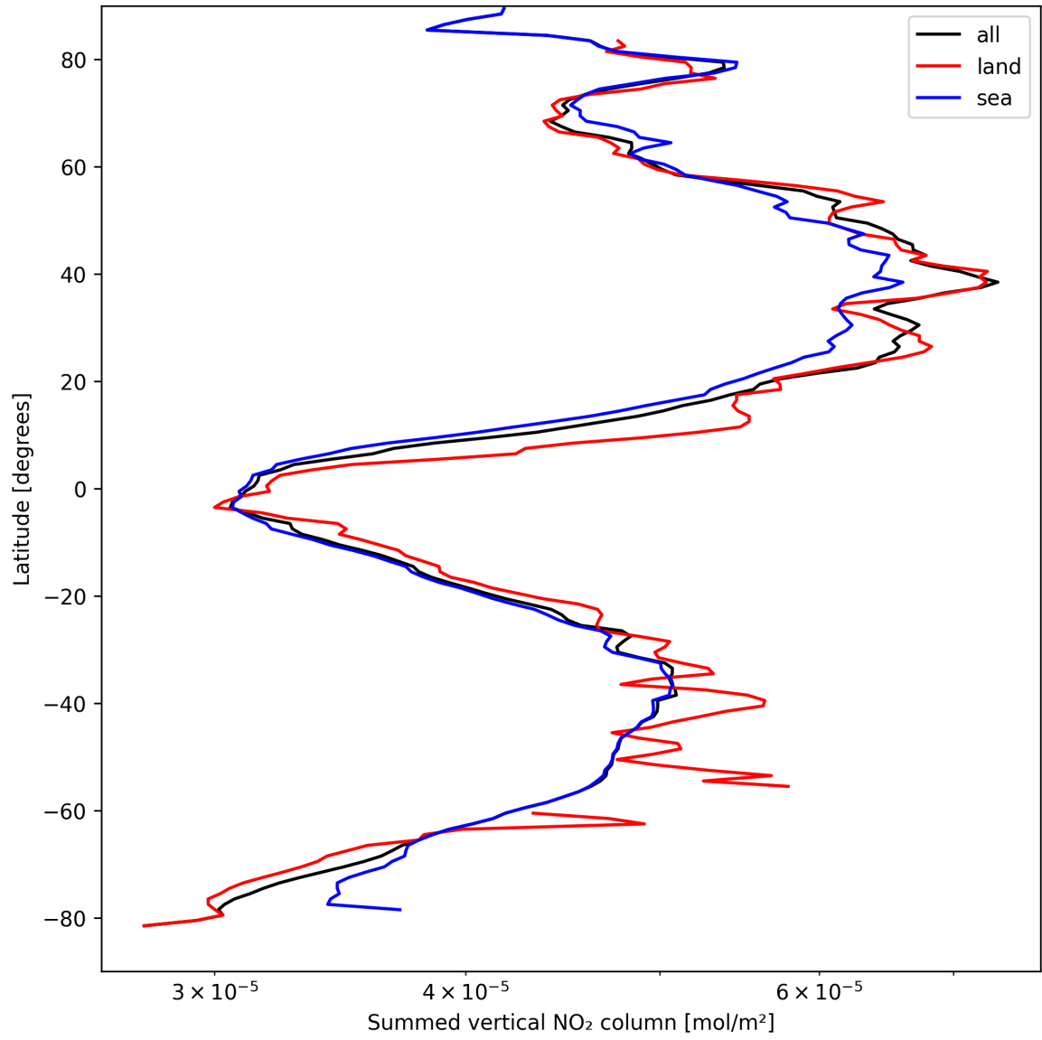
Figure 21: Zonal average of “Summed vertical NO 2 column” for 2025-04-06 to 2025-04-06.
