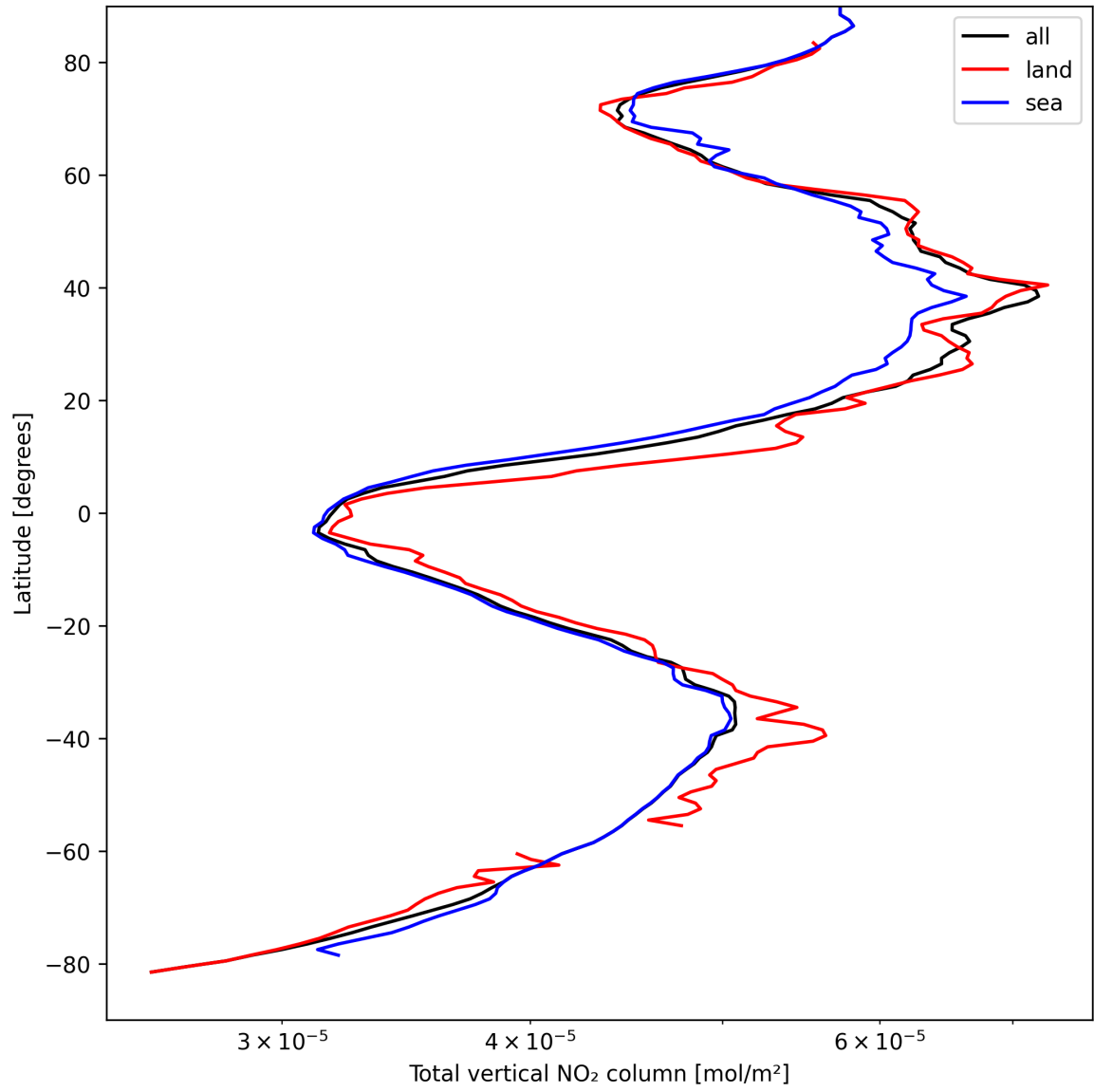
Figure 19: Zonal average of “Total vertical NO 2 column” for 2025-04-06 to 2025-04-06.
