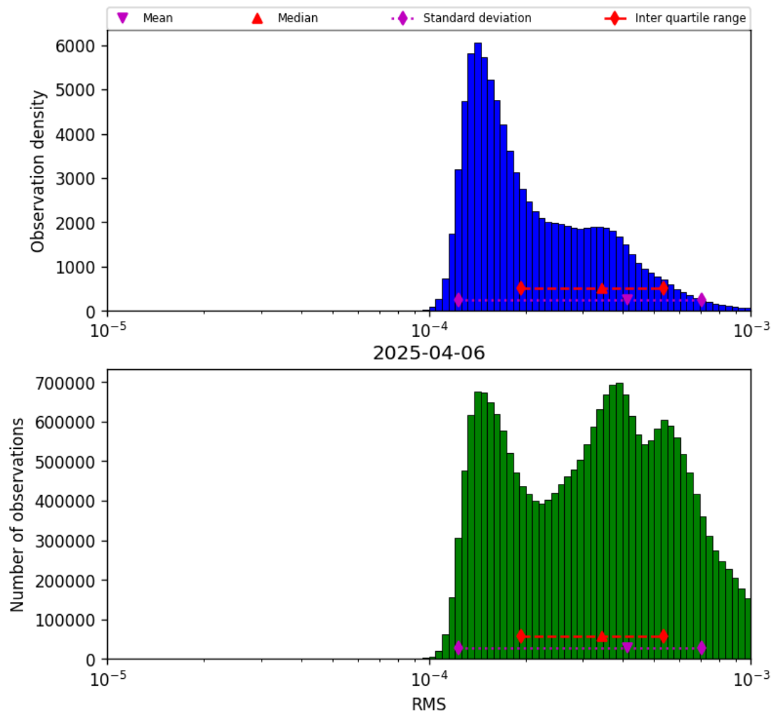
Figure 41: Histogram of “RMS” for 2025-04-06 to 2025-04-06
