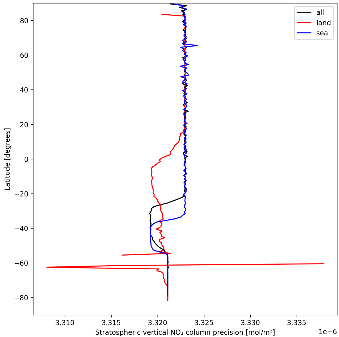
Figure 18: Zonal average of “Stratospheric vertical NO 2 column precision” for 2025-04-06 to 2025-04-06.
