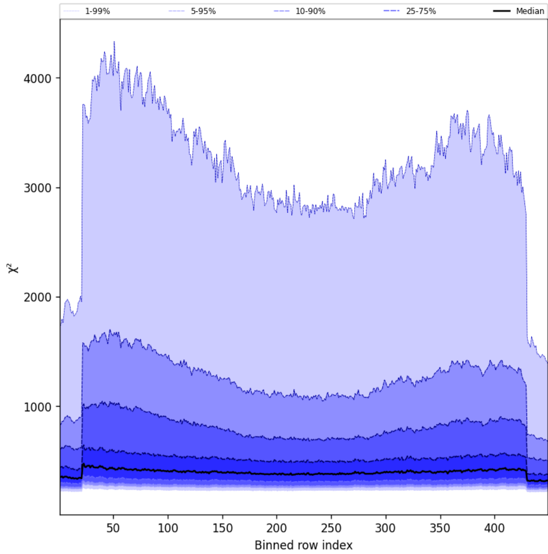
Figure 57: Along track statistics of “ \chi^2 ” for 2025-04-06 to 2025-04-06
