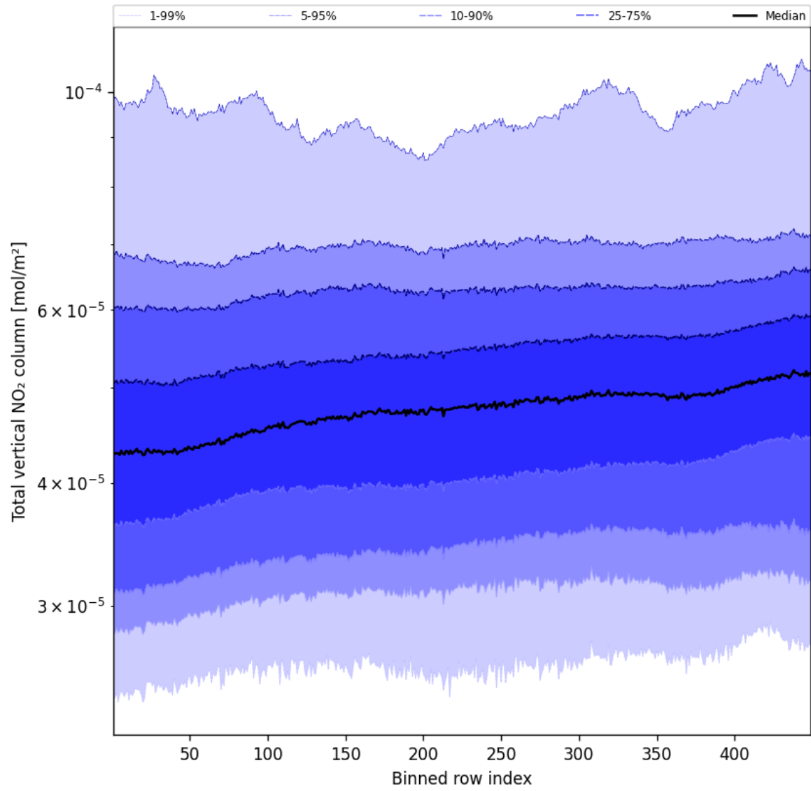
Figure 53: Along track statistics of “Total vertical NO 2 column” for 2025-04-06 to 2025-04-06
