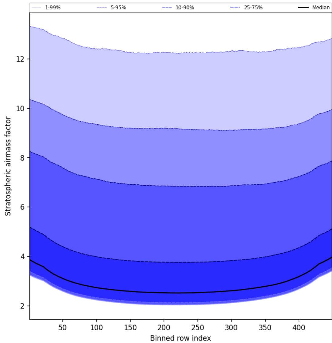
Figure 59: Along track statistics of “Stratospheric airmass factor” for 2025-04-06 to 2025-04-06
