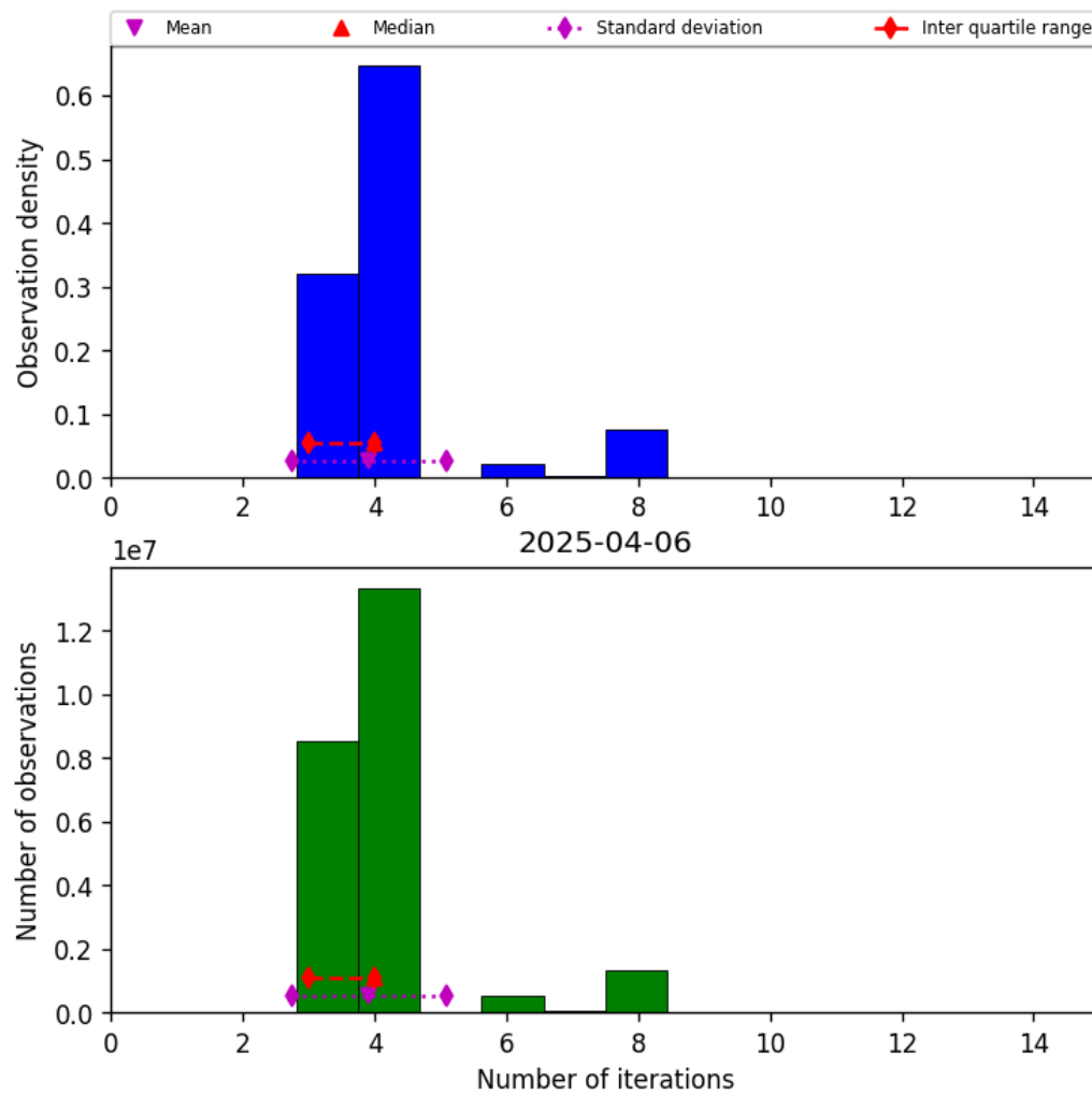
Figure 32: Histogram of “Number of iterations” for 2025-04-06 to 2025-04-06
