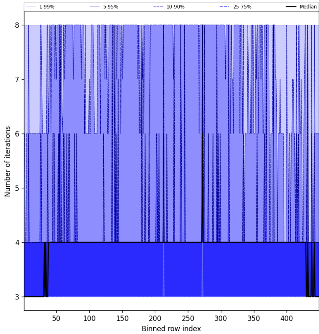
Figure 49: Along track statistics of “Number of iterations” for 2025-04-06 to 2025-04-06
