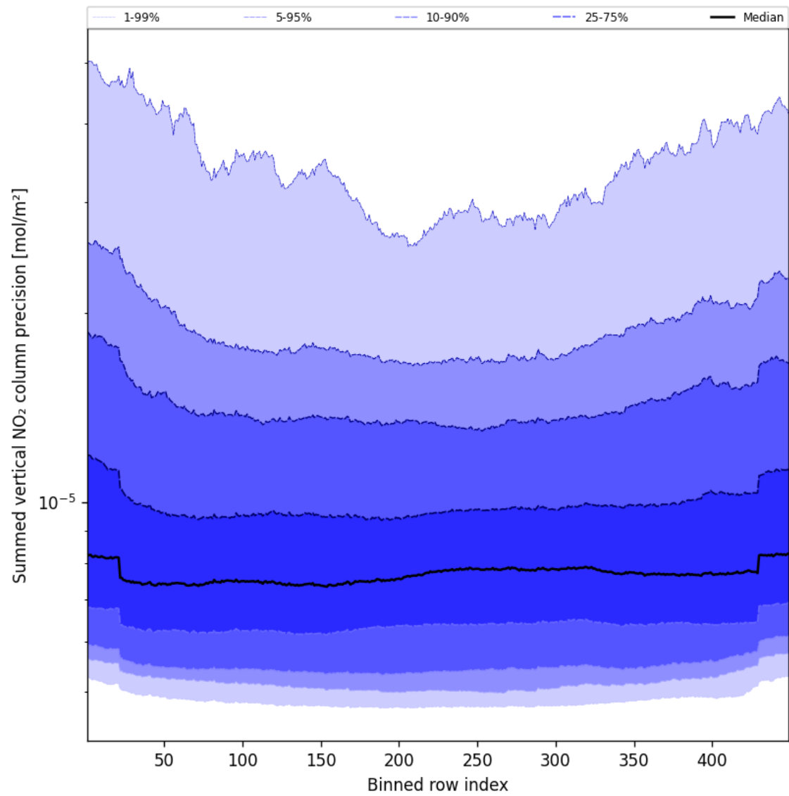
Figure 56: Along track statistics of “Summed vertical NO 2 column precision” for 2025-04-06 to 2025-04-06
