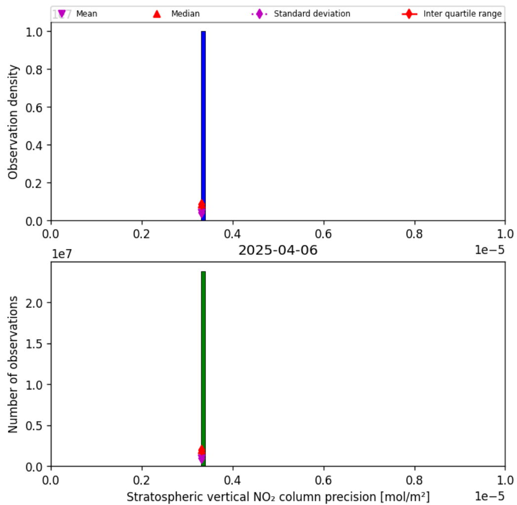
Figure 35: Histogram of “Stratospheric vertical NO 2 column precision” for 2025-04-06 to 2025-04-06
