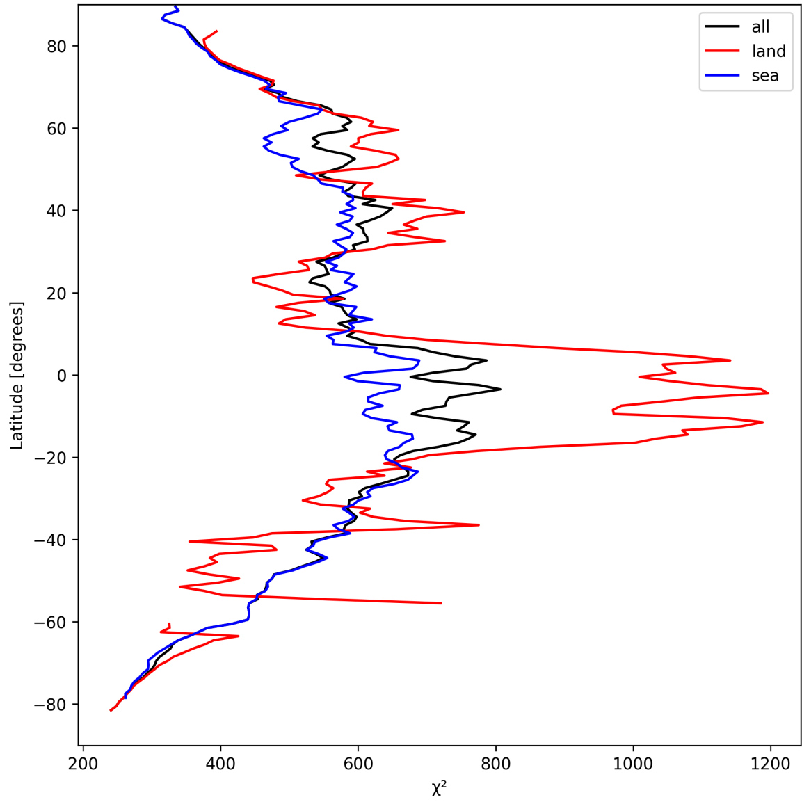
Figure 23: Zonal average of “ \chi^2 ” for 2025-04-06 to 2025-04-06.
