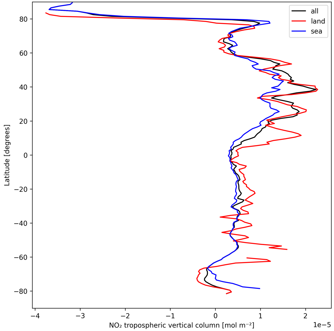
Figure 10: Zonal average of “NO 2 tropospheric vertical column” for 2025-04-06 to 2025-04-06.
