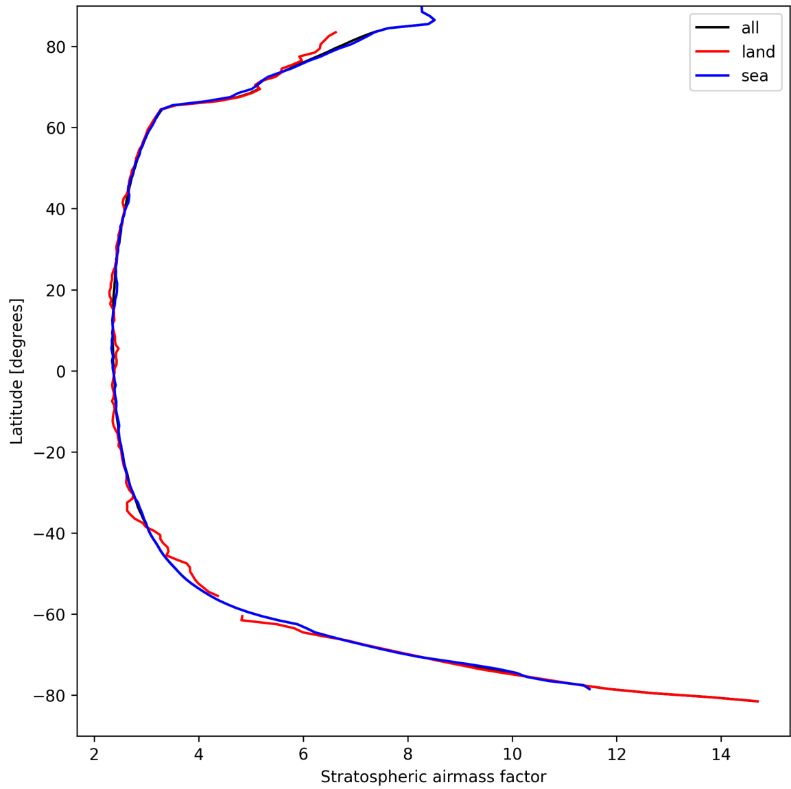
Figure 25: Zonal average of “Stratospheric airmass factor” for 2025-04-06 to 2025-04-06.
