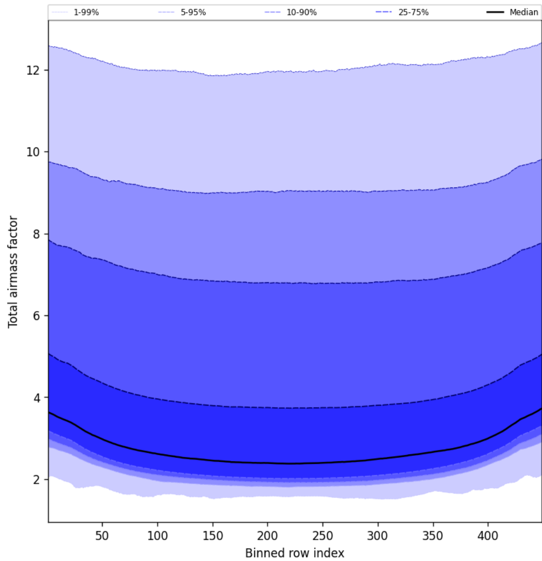
Figure 47: Along track statistics of “Total airmass factor” for 2025-04-06 to 2025-04-06
