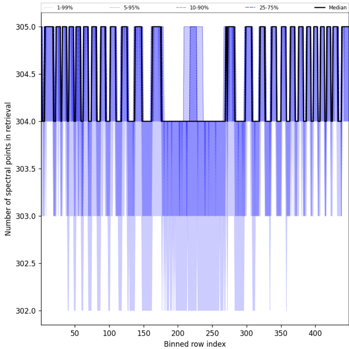
Figure 48: Along track statistics of “Number of spectral points in retrieval” for 2025-04-06 to 2025-04-06
