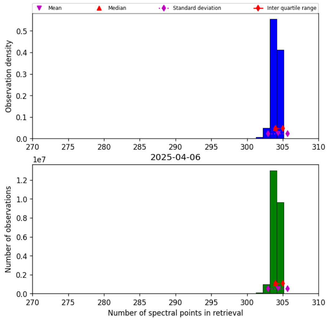
Figure 31: Histogram of “Number of spectral points in retrieval” for 2025-04-06 to 2025-04-06
