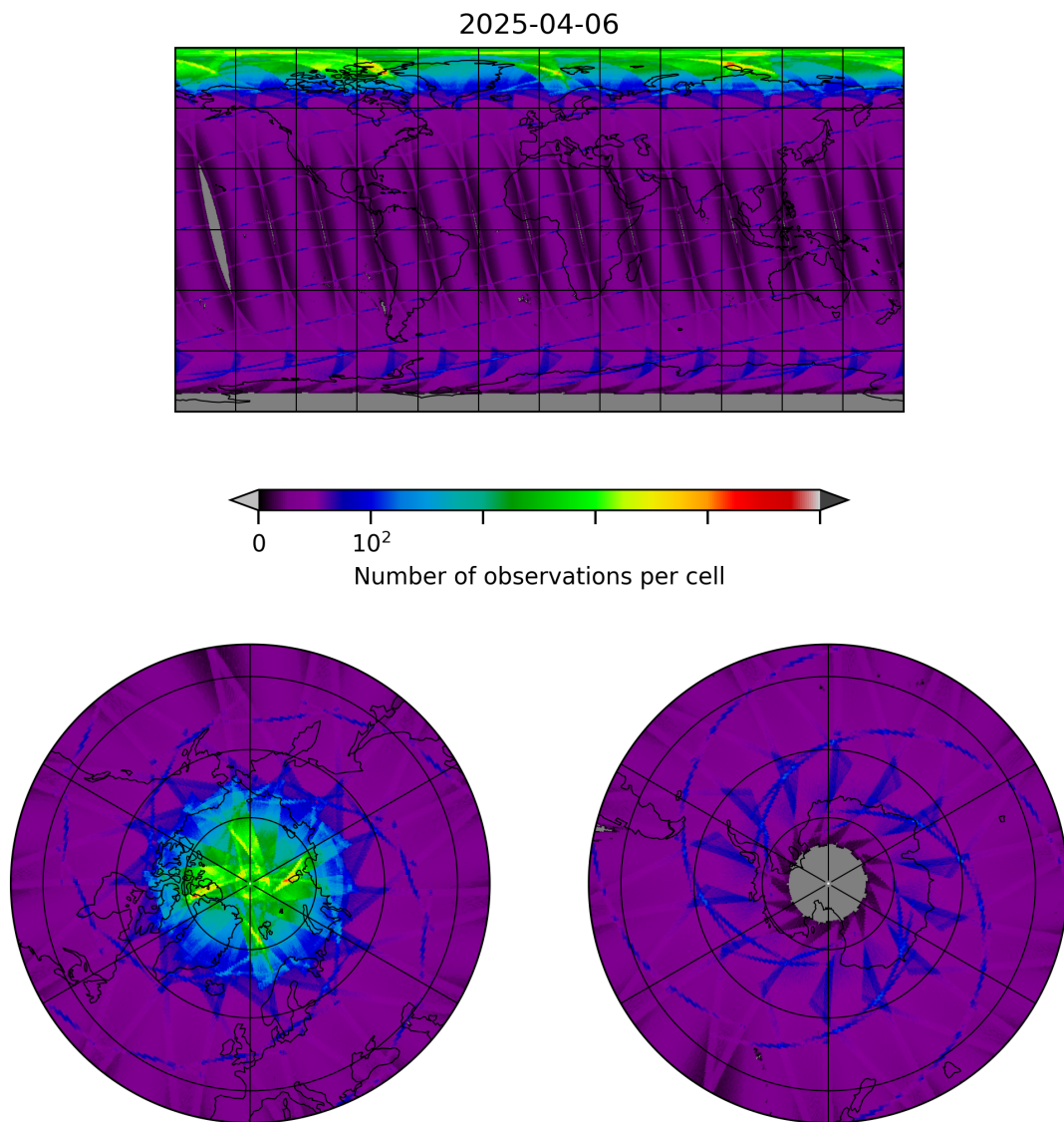
Figure 8: Map of the number of observations for 2025-04-06 to 2025-04-06
