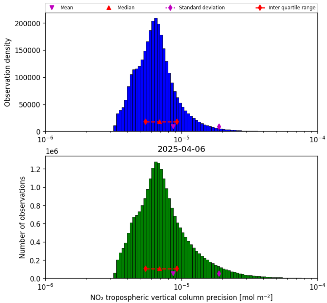
Figure 28: Histogram of “NO 2 tropospheric vertical column precision” for 2025-04-06 to 2025-04-06
