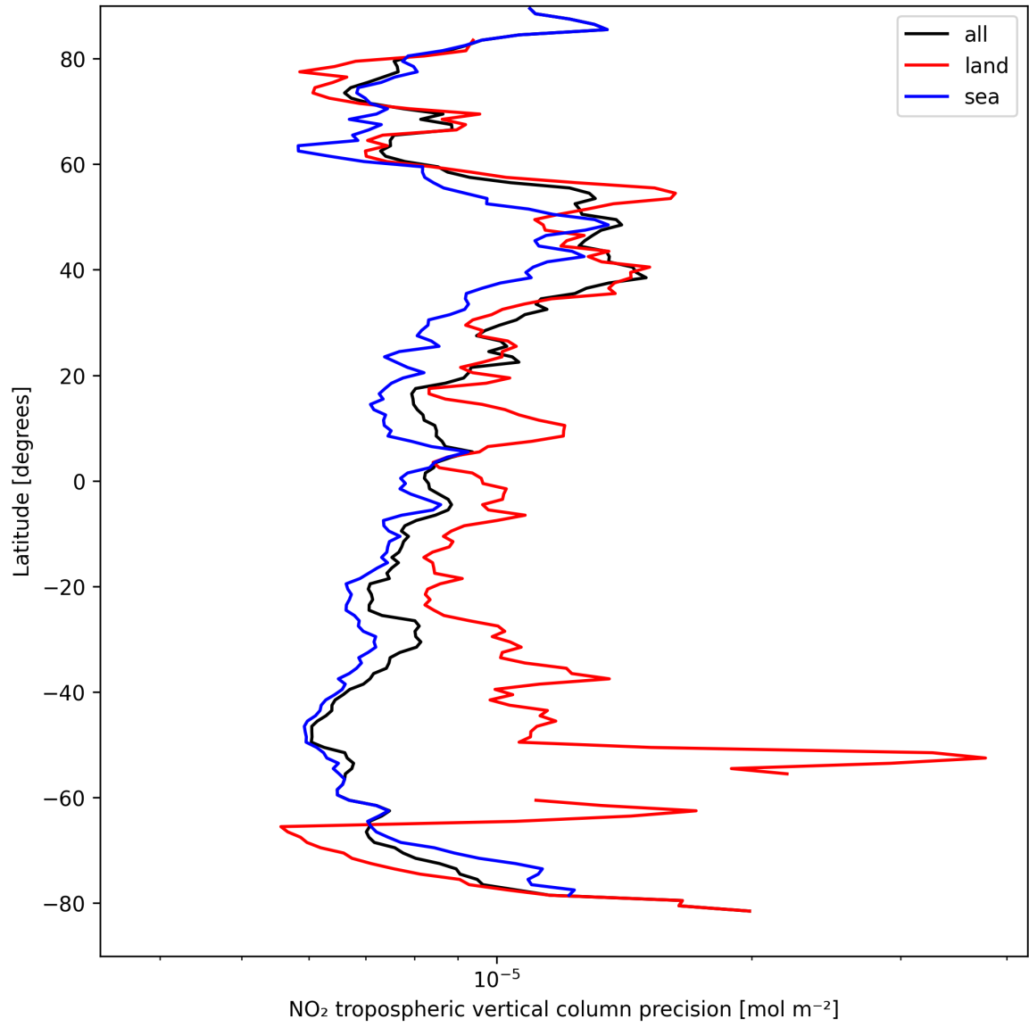
Figure 11: Zonal average of “NO 2 tropospheric vertical column precision” for 2025-04-06 to 2025-04-06.
