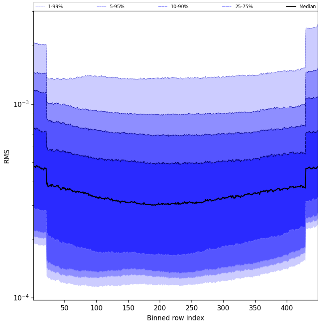
Figure 58: Along track statistics of “RMS” for 2025-04-06 to 2025-04-06
