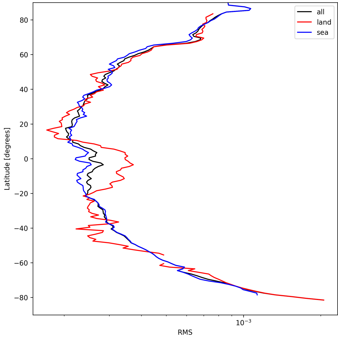
Figure 24: Zonal average of “RMS” for 2025-04-06 to 2025-04-06.
