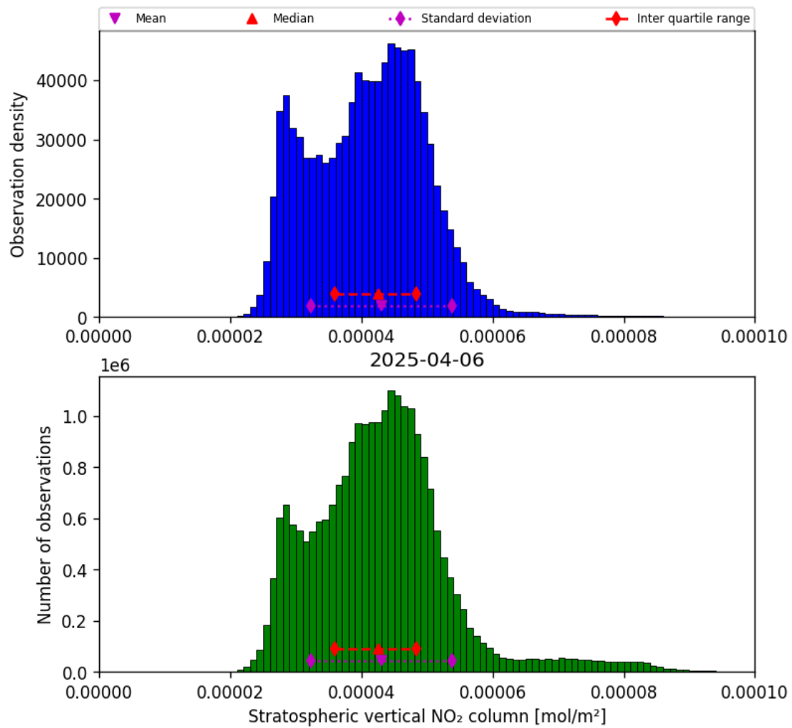
Figure 34: Histogram of “Stratospheric vertical NO 2 column” for 2025-04-06 to 2025-04-06
