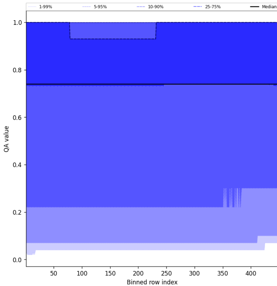
Figure 43: Along track statistics of “QA value” for 2025-04-06 to 2025-04-06
