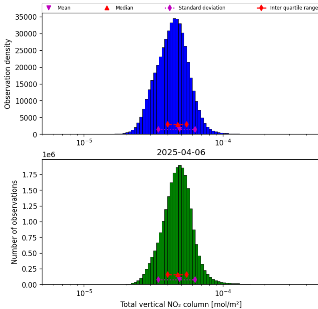
Figure 36: Histogram of "Total vertical NO 2 column" for 2025-04-06 to 2025-04-06
