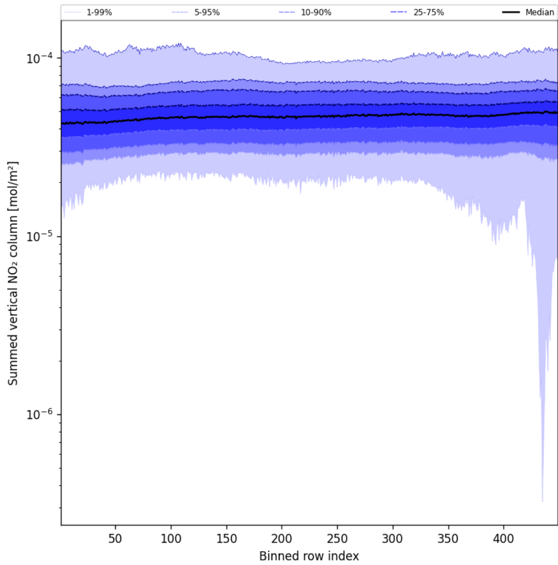
Figure 55: Along track statistics of “Summed vertical NO 2 column” for 2025-04-06 to 2025-04-06
