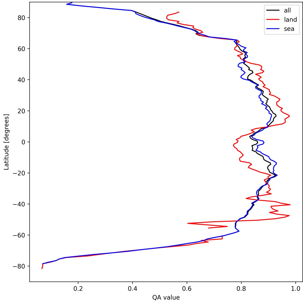
Figure 9: Zonal average of “QA value” for 2025-04-06 to 2025-04-06.
