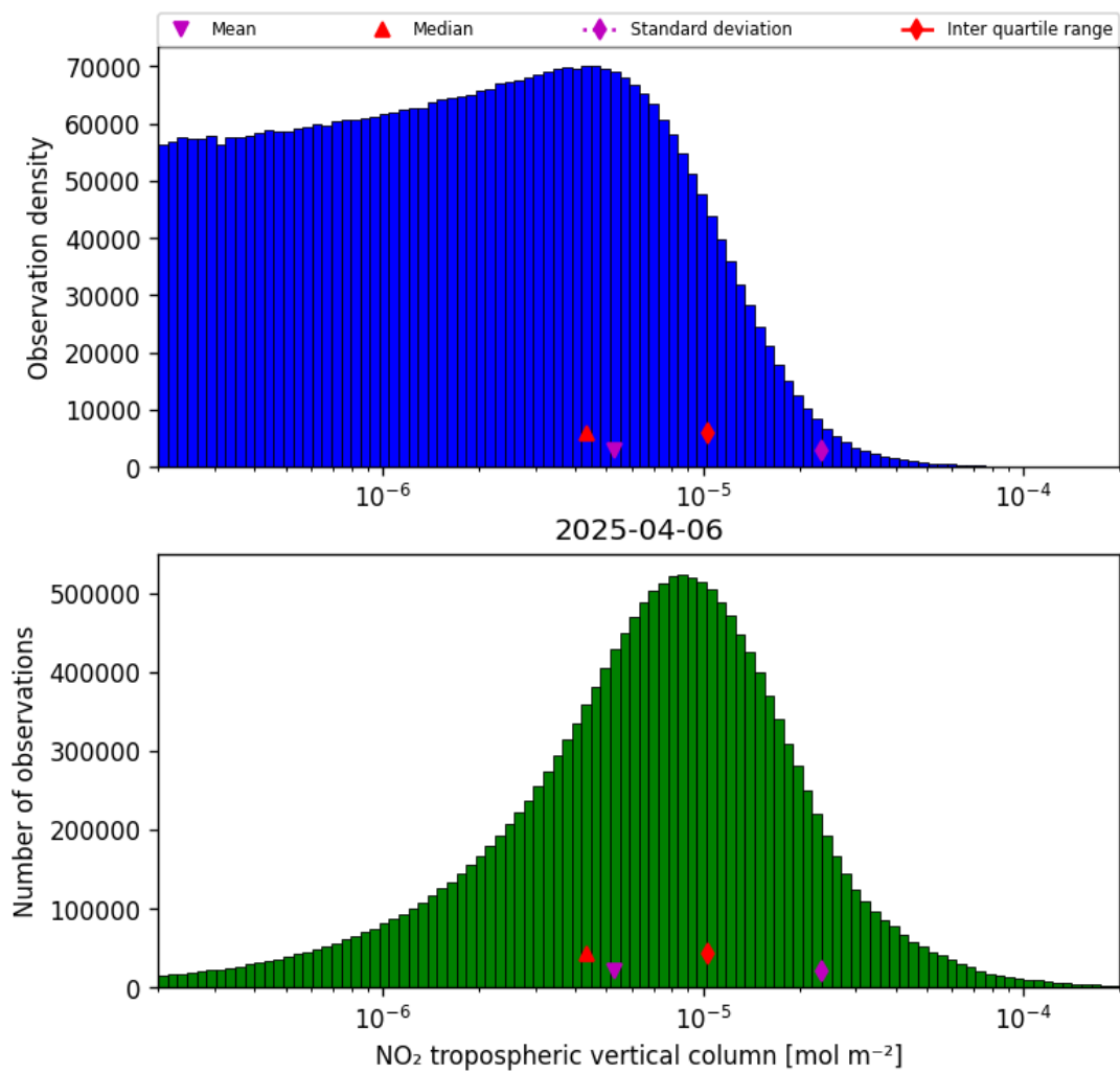
Figure 27: Histogram of “NO 2 tropospheric vertical column” for 2025-04-06 to 2025-04-06
