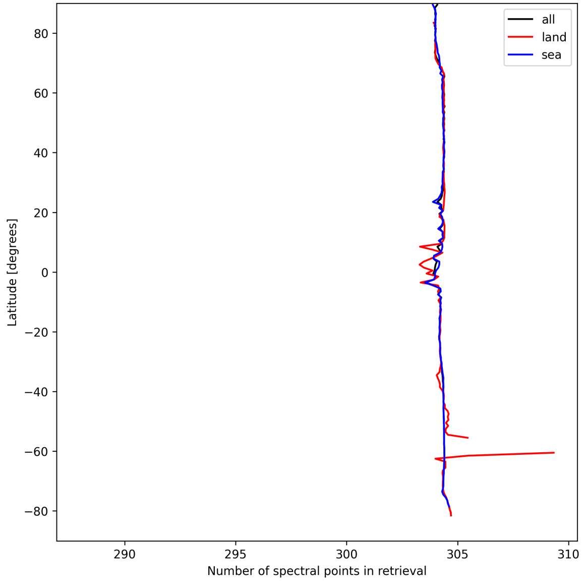
Figure 14: Zonal average of “Number of spectral points in retrieval” for 2025-04-06 to 2025-04-06.
