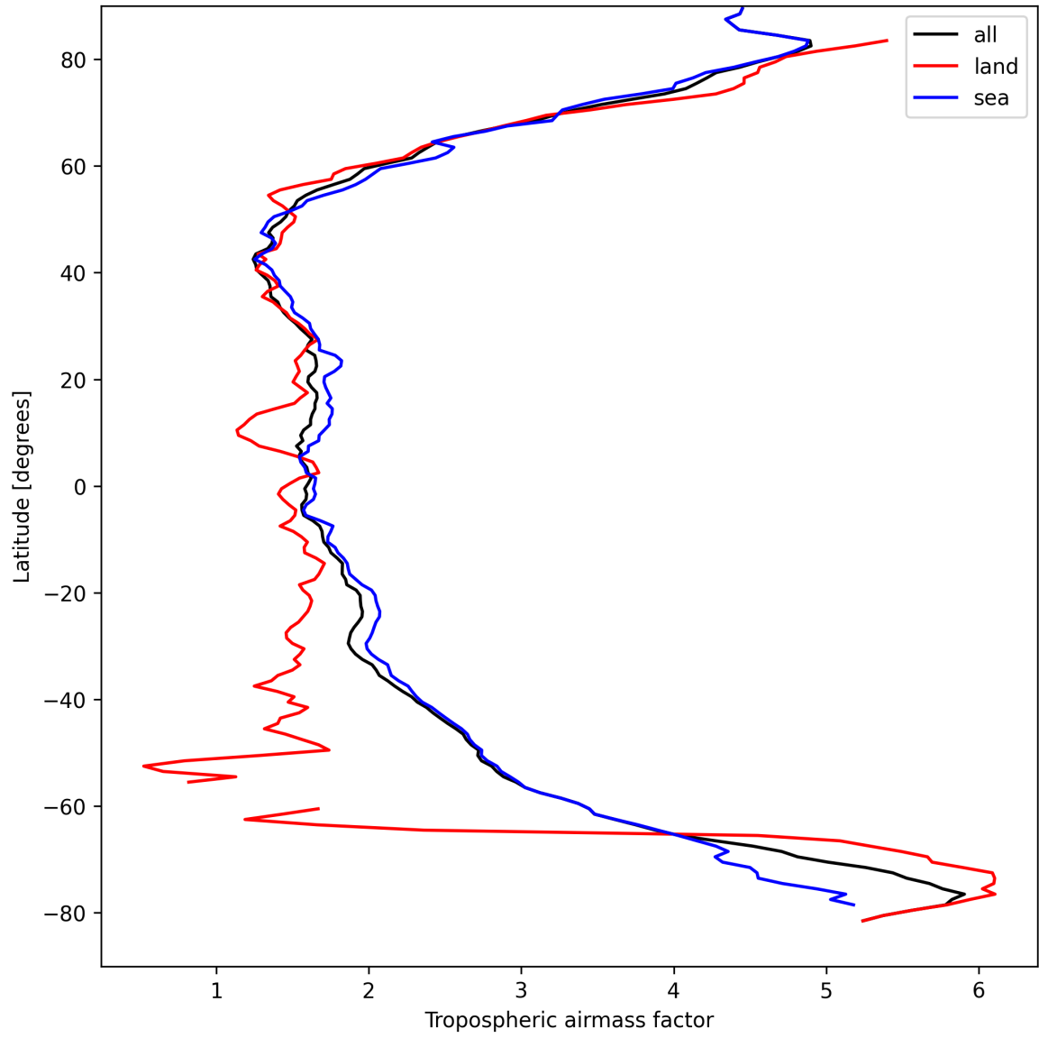
Figure 12: Zonal average of “Tropospheric airmass factor” for 2025-04-06 to 2025-04-06.
