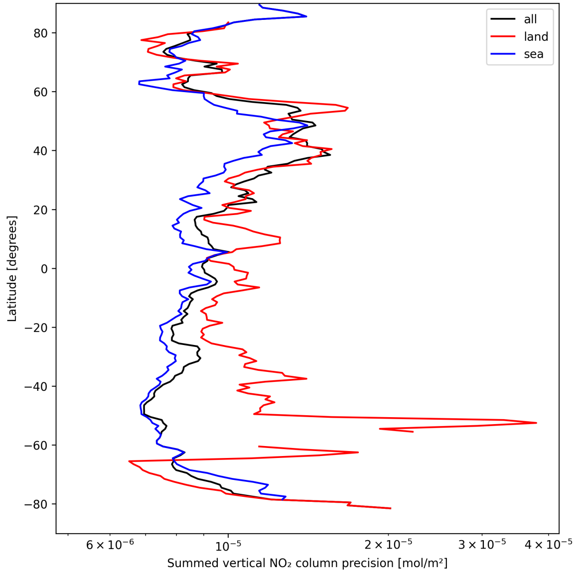
Figure 22: Zonal average of “Summed vertical NO 2 column precision” for 2025-04-06 to 2025-04-06.
