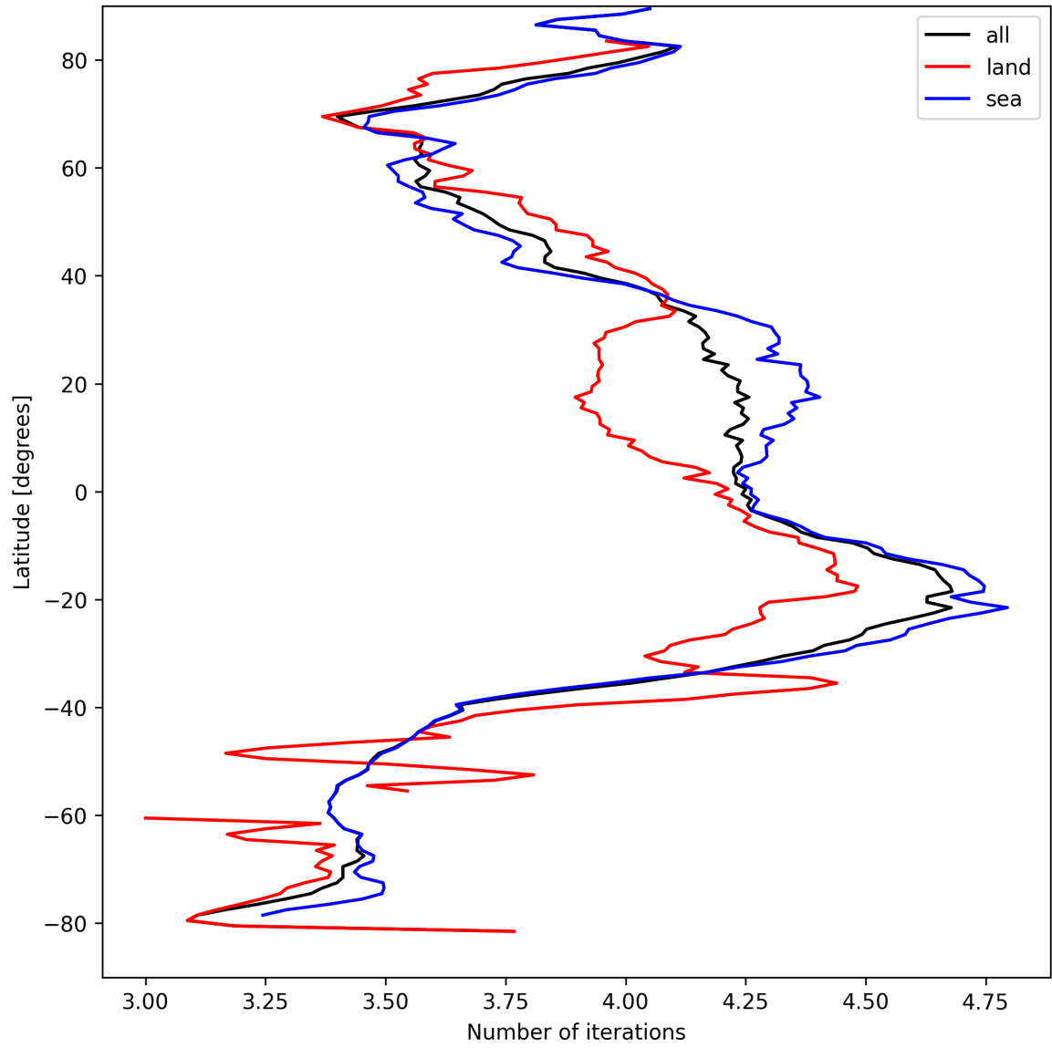
Figure 15: Zonal average of “Number of iterations” for 2025-04-06 to 2025-04-06.
