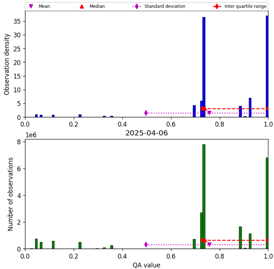
Figure 26: Histogram of “QA value” for 2025-04-06 to 2025-04-06
