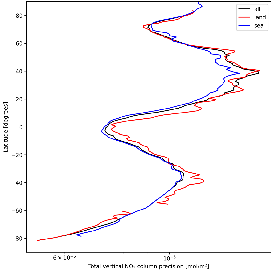
Figure 20: Zonal average of “Total vertical NO 2 column precision” for 2025-04-06 to 2025-04-06.
