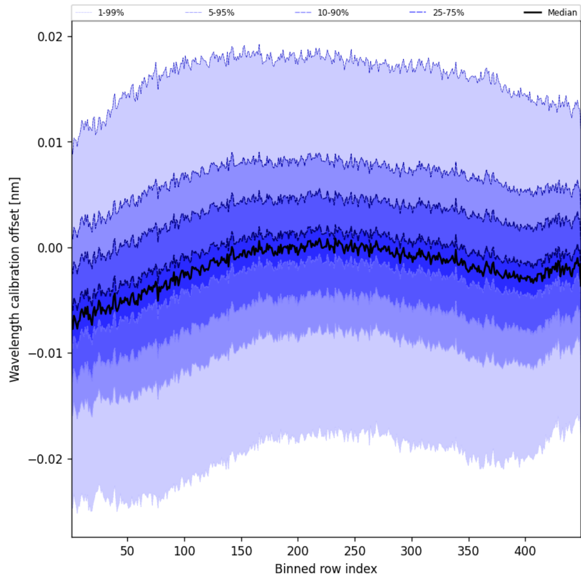
Figure 50: Along track statistics of “Wavelength calibration offset” for 2025-04-06 to 2025-04-06
