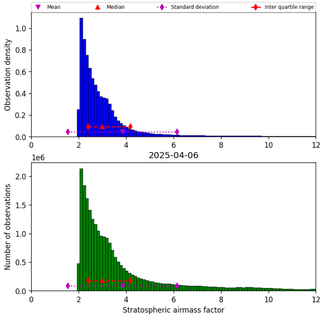
Figure 42: Histogram of “Stratospheric airmass factor” for 2025-04-06 to 2025-04-06
