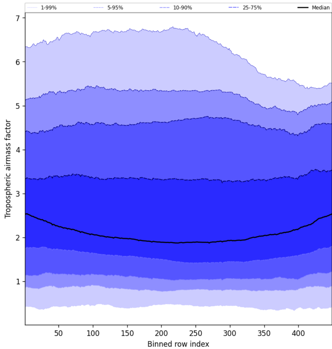
Figure 46: Along track statistics of “Tropospheric airmass factor” for 2025-04-06 to 2025-04-06
