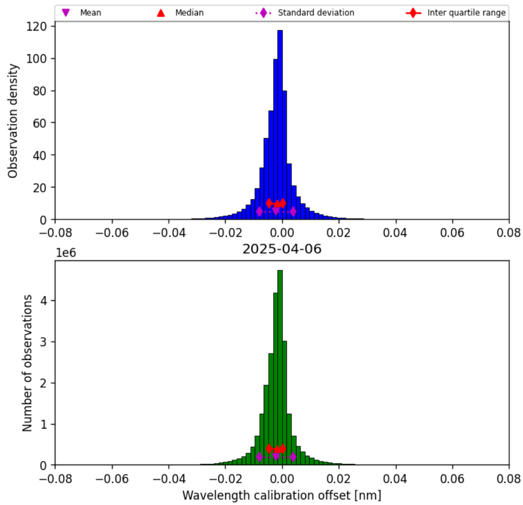
Figure 33: Histogram of “Wavelength calibration offset” for 2025-04-06 to 2025-04-06
