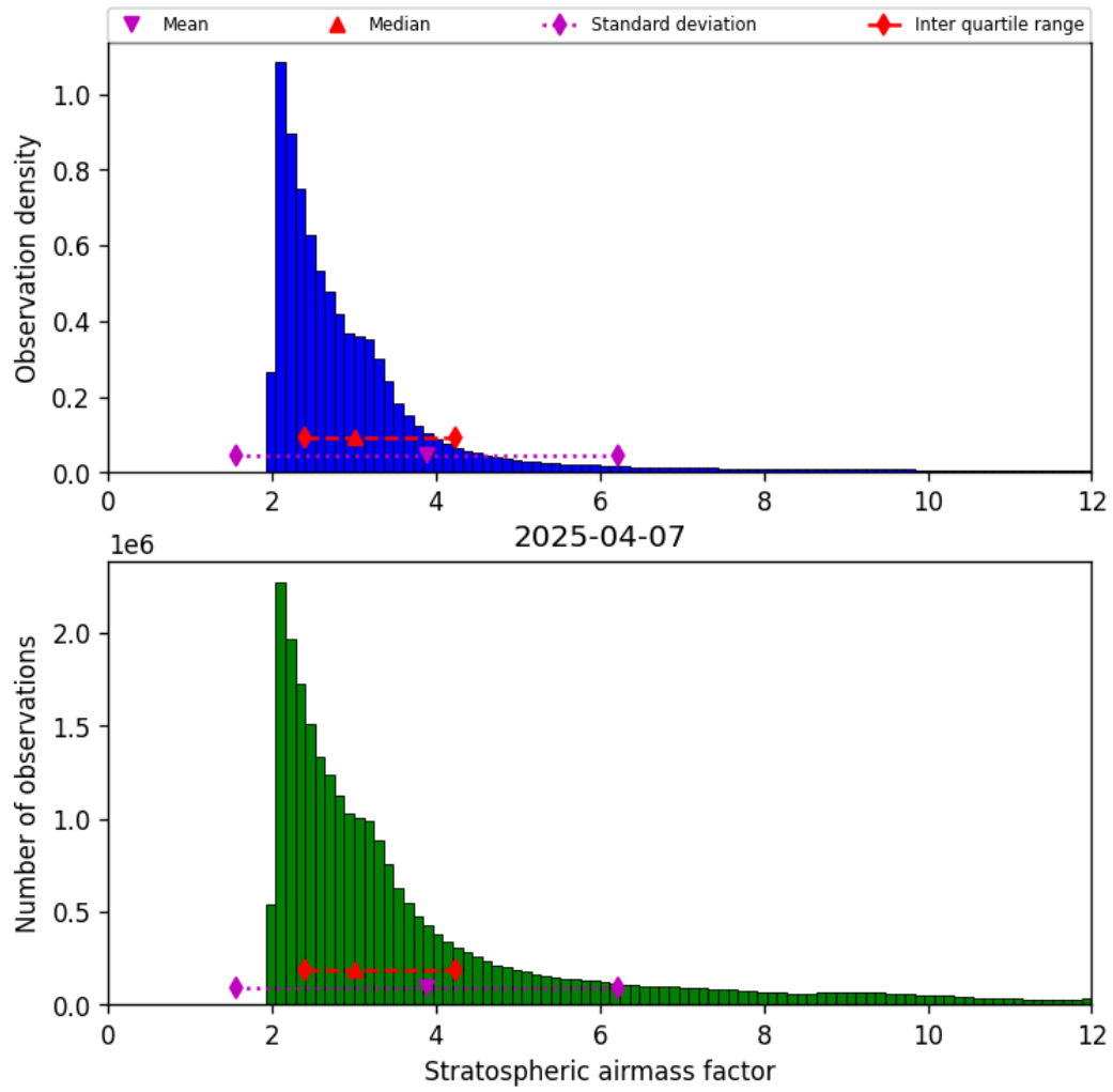
Figure 42: Histogram of “Stratospheric airmass factor” for 2025-04-07 to 2025-04-08
