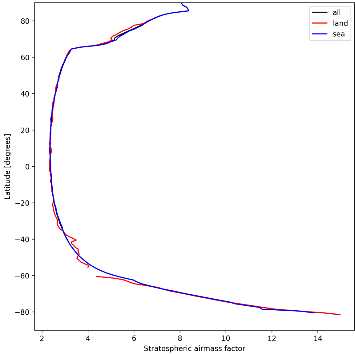
Figure 25: Zonal average of “Stratospheric air mass factor” for 2025-04-07 to 2025-04-08.
