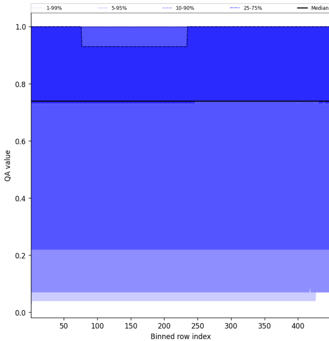
Figure 43: Along track statistics of “QA value” for 2025-04-07 to 2025-04-08
