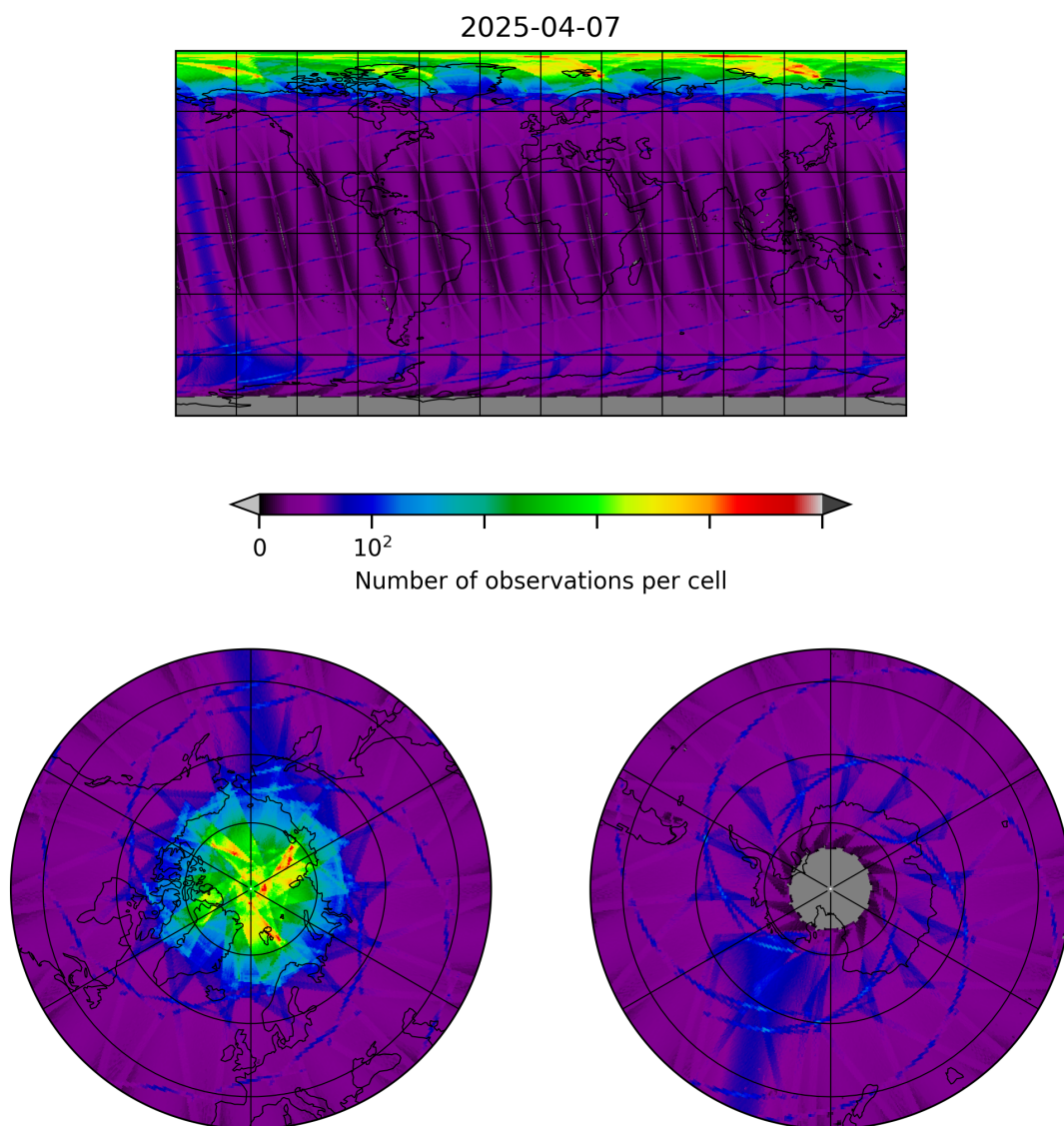
Figure 8: Map of the number of observations for 2025-04-07 to 2025-04-08
