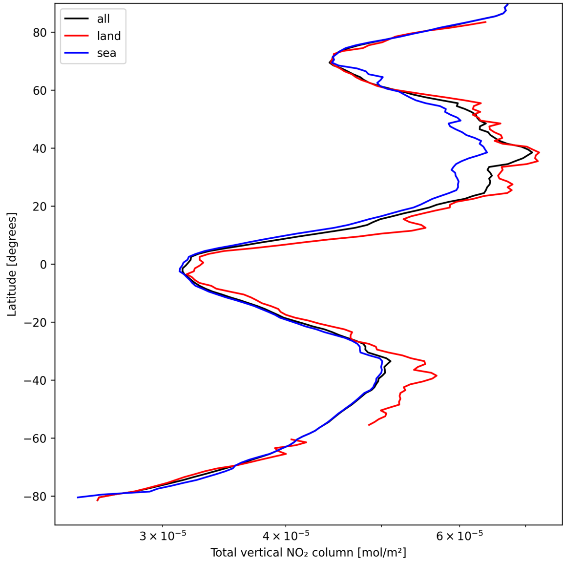
Figure 19: Zonal average of “Total vertical NO 2 column” for 2025-04-07 to 2025-04-08.
