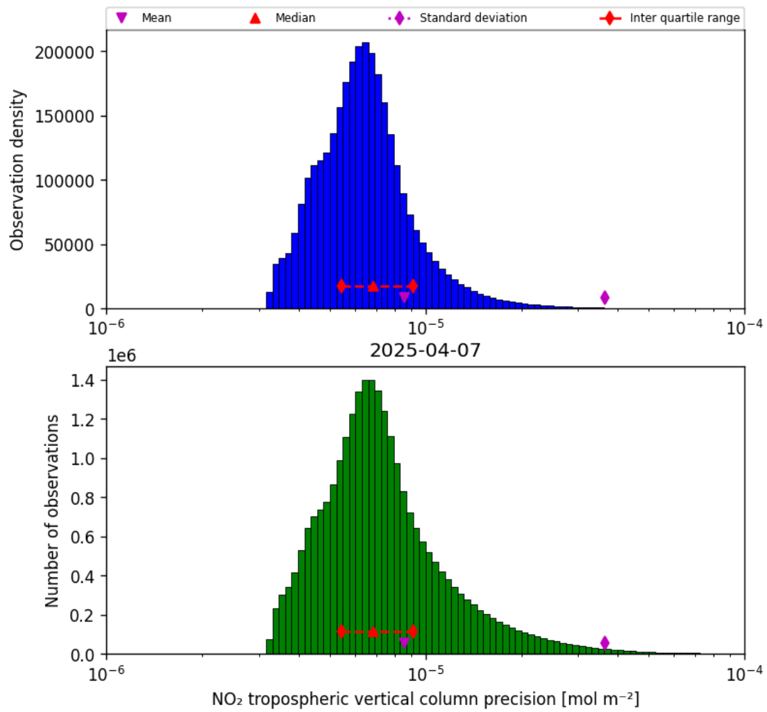
Figure 28: Histogram of “NO 2 tropospheric vertical column precision” for 2025-04-07 to 2025-04-08
