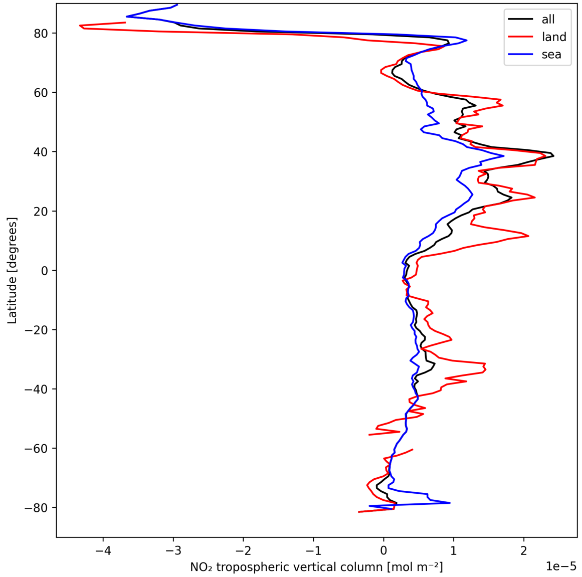
Figure 10: Zonal average of “NO 2 tropospheric vertical column” for 2025-04-07 to 2025-04-08.
