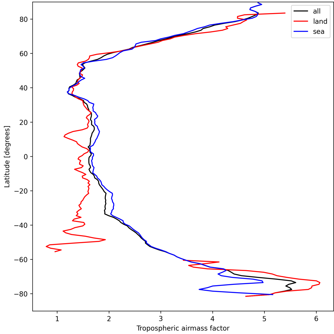
Figure 12: Zonal average of “Tropospheric airmass factor” for 2025-04-07 to 2025-04-08.
