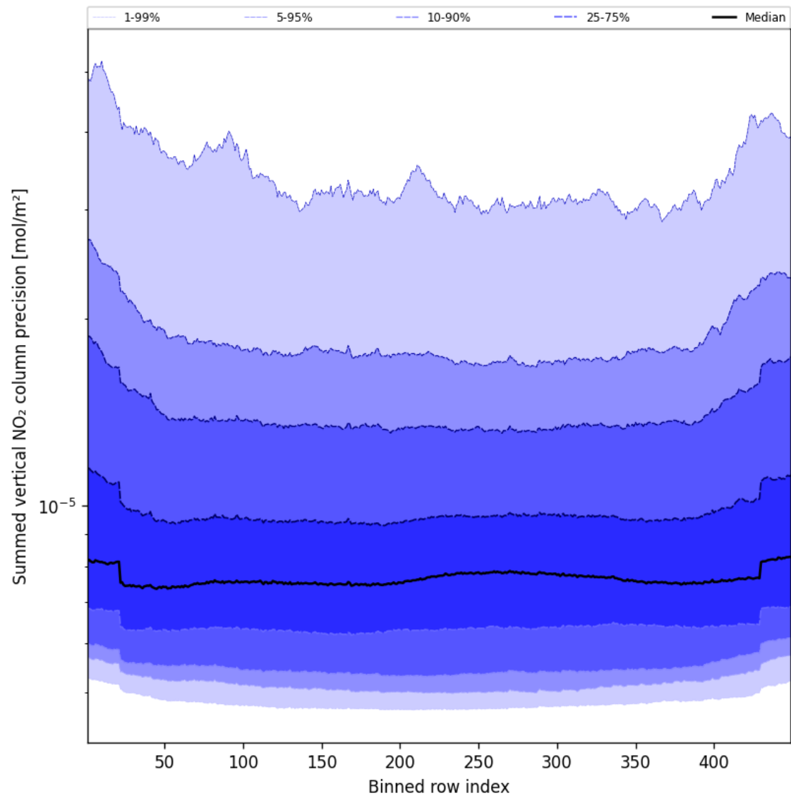
Figure 56: Along track statistics of “Summed vertical NO 2 column precision” for 2025-04-07 to 2025-04-08
