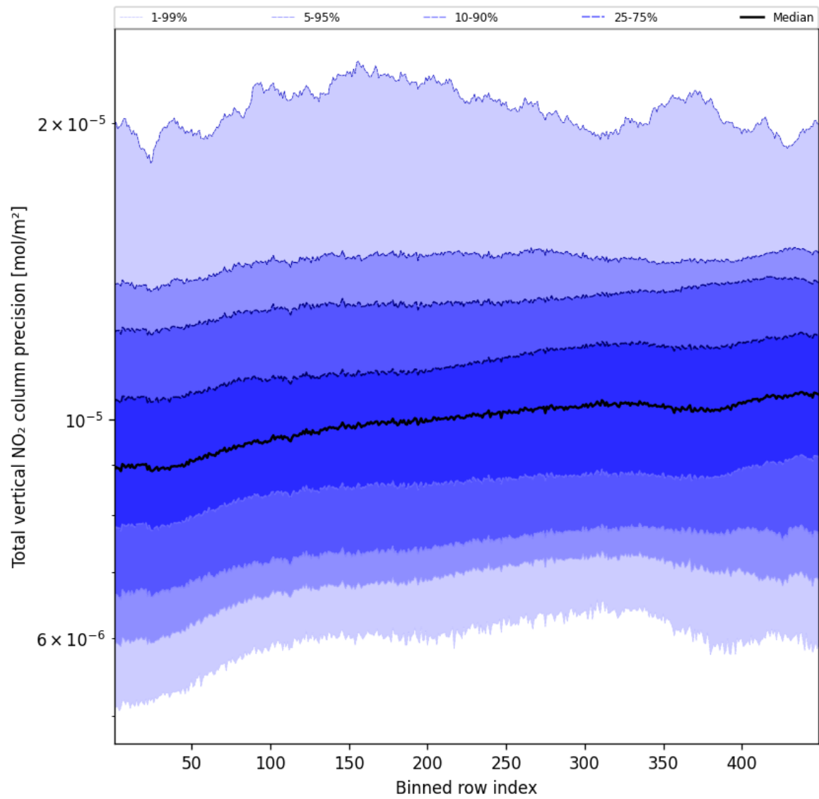
Figure 54: Along track statistics of "Total vertical NO 2 column precision" for 2025-04-07 to 2025-04-08
