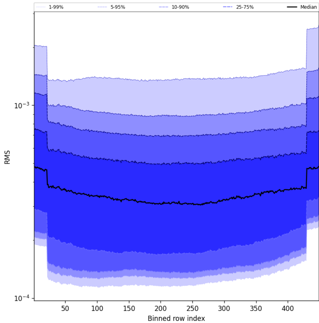
Figure 58: Along track statistics of “RMS” for 2025-04-07 to 2025-04-08
