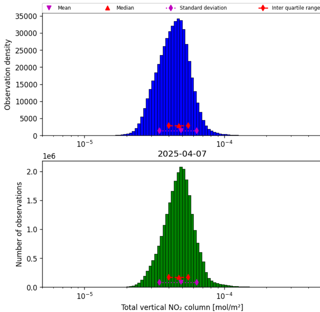
Figure 36: Histogram of “Total vertical NO 2 column” for 2025-04-07 to 2025-04-08
