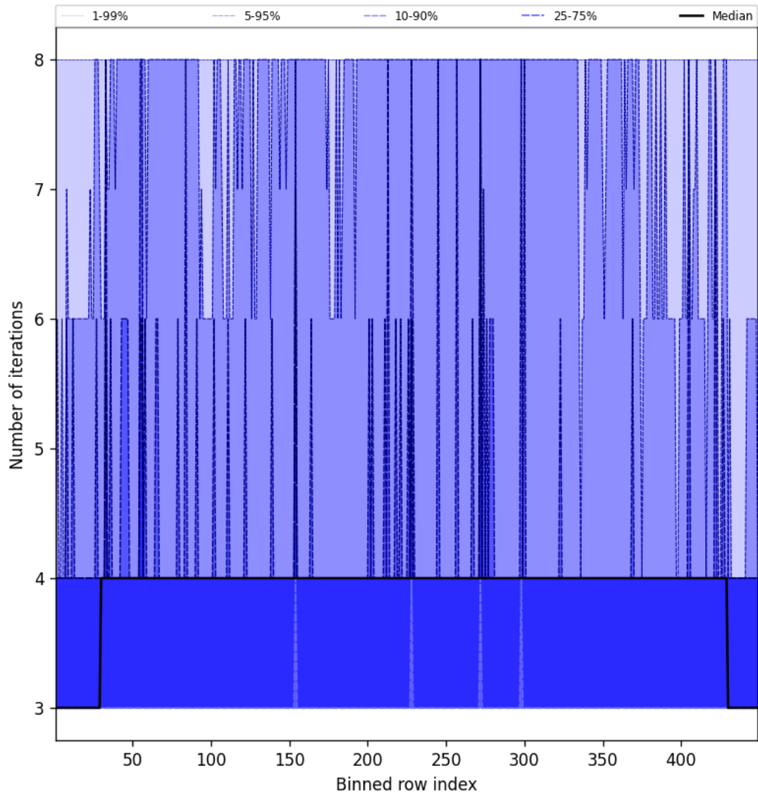
Figure 49: Along track statistics of “Number of iterations” for 2025-04-07 to 2025-04-08
