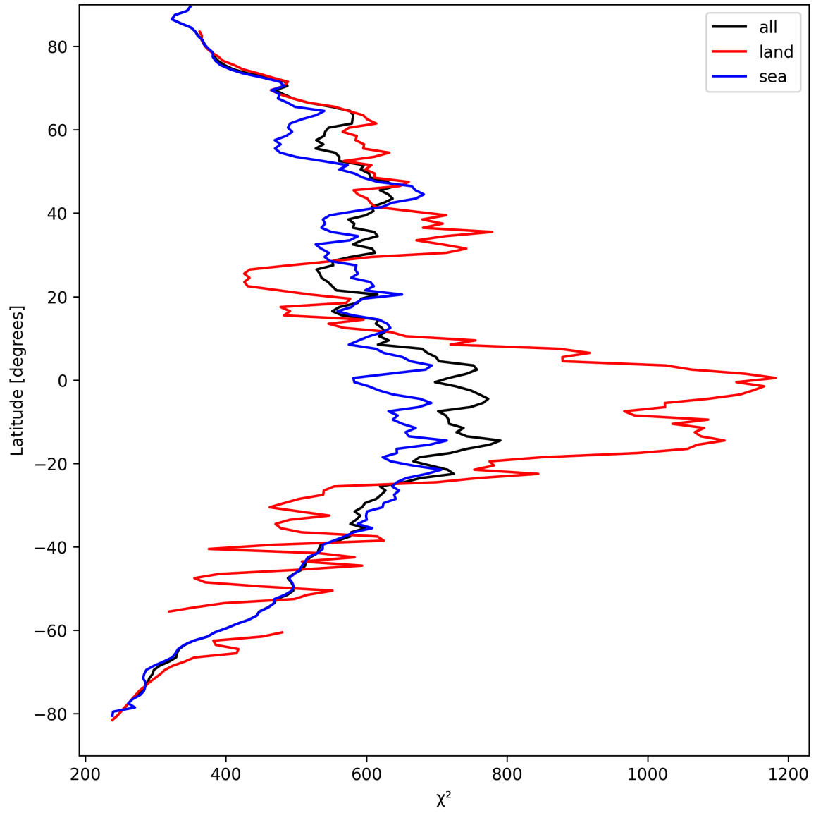
Figure 23: Zonal average of “ \chi^2 ” for 2025-04-07 to 2025-04-08.
