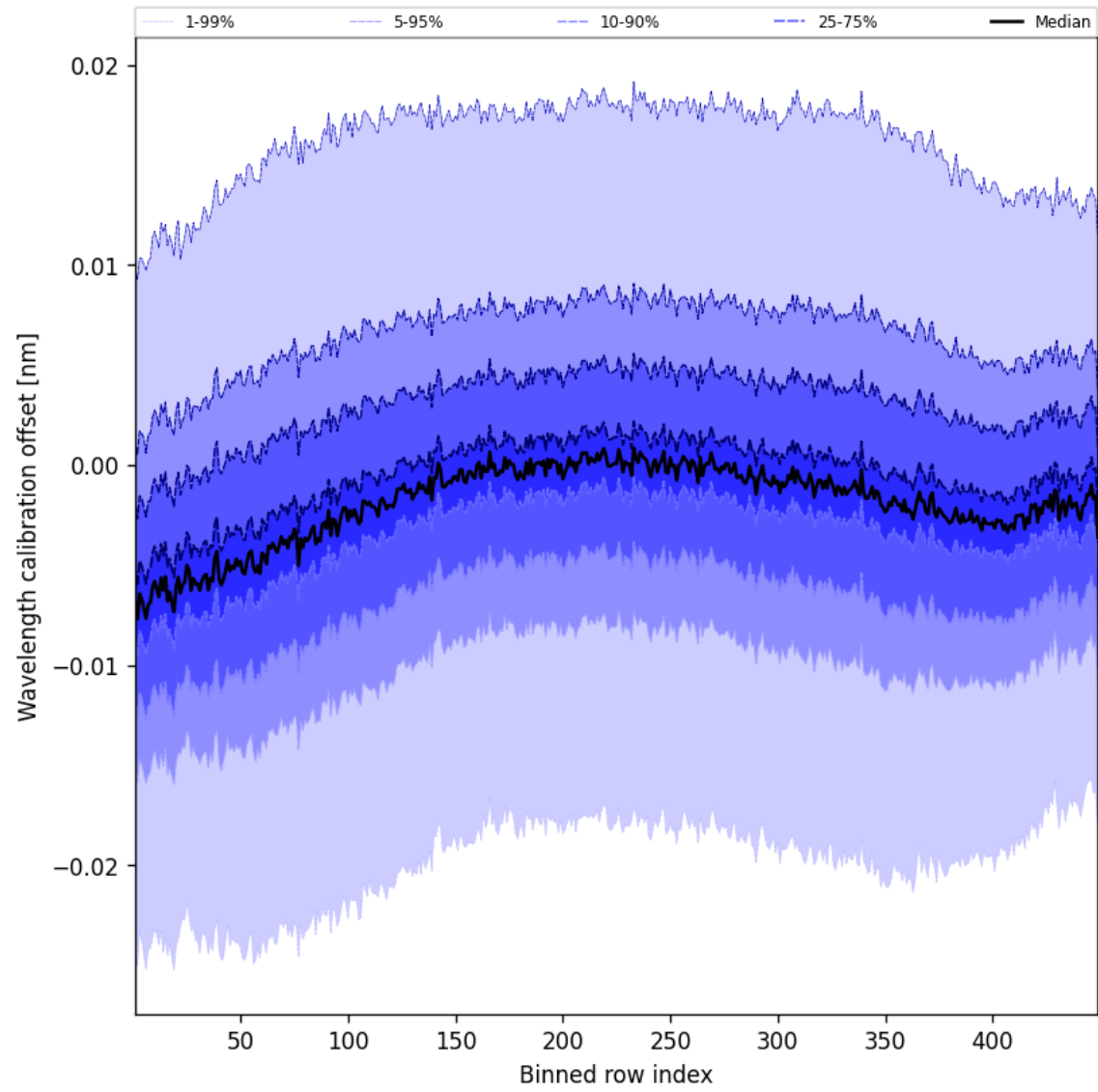
Figure 50: Along track statistics of “Wavelength calibration offset” for 2025-04-07 to 2025-04-08
