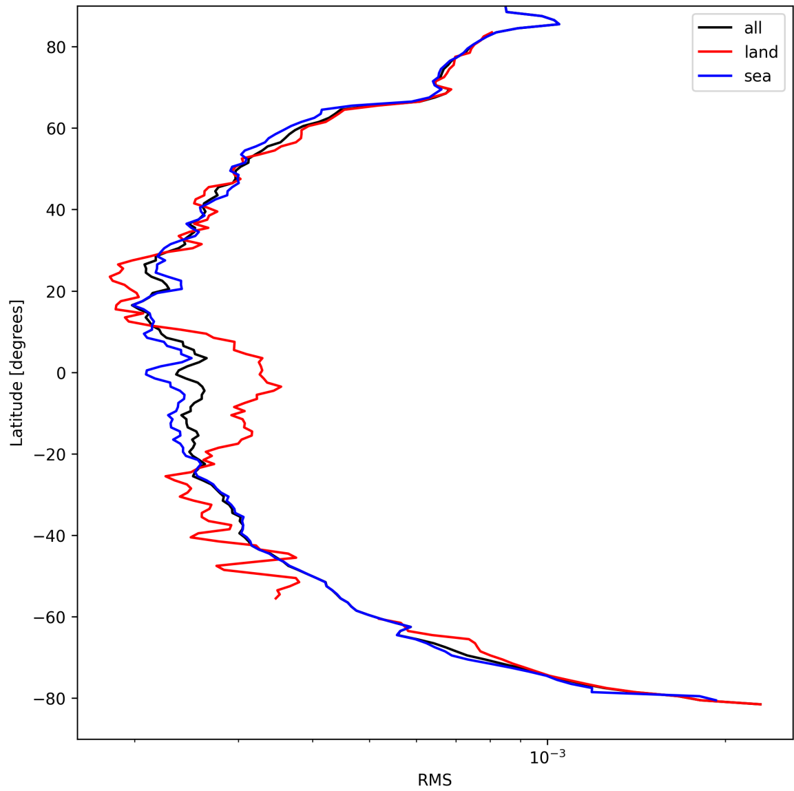
Figure 24: Zonal average of “RMS” for 2025-04-07 to 2025-04-08.
