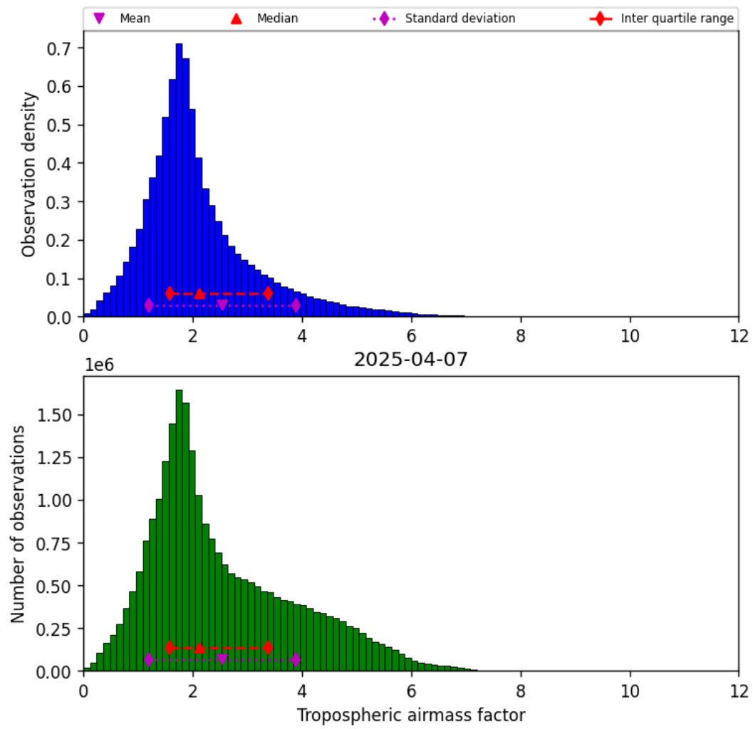
Figure 29: Histogram of “Tropospheric air mass factor” for 2025-04-07 to 2025-04-08
