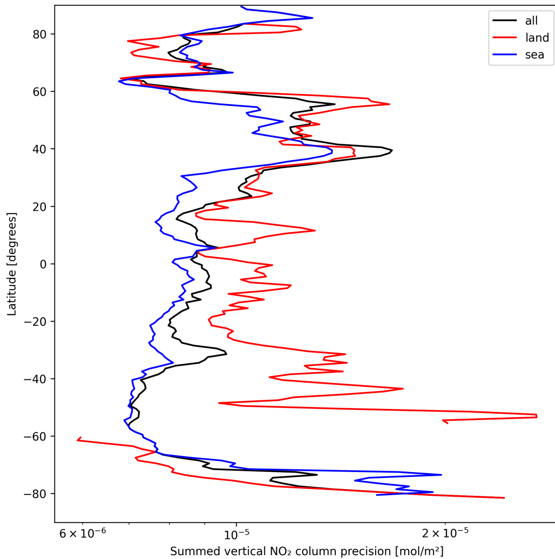
Figure 22: Zonal average of “Summed vertical NO 2 column precision” for 2025-04-07 to 2025-04-08.
