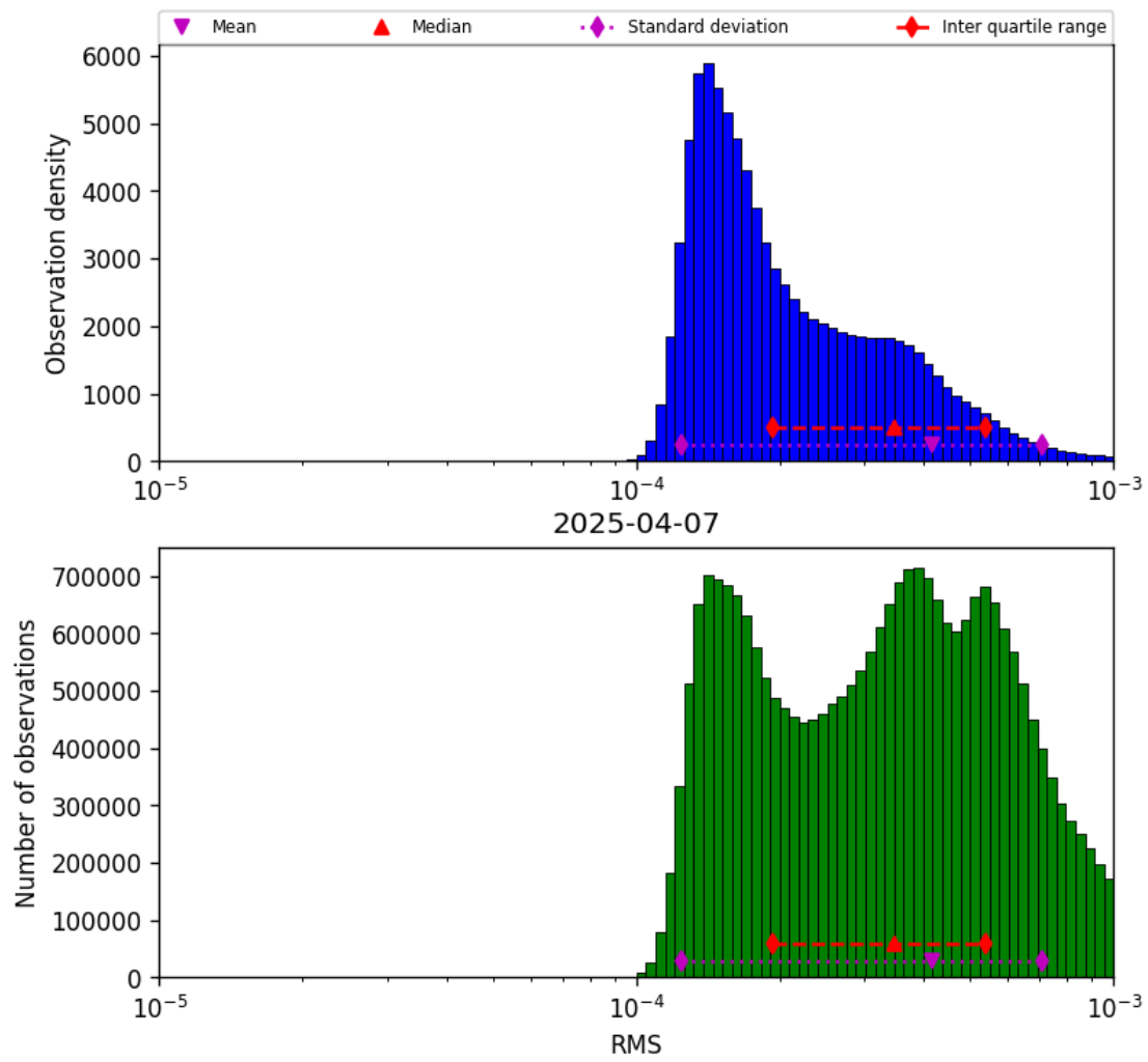
Figure 41: Histogram of “RMS” for 2025-04-07 to 2025-04-08
