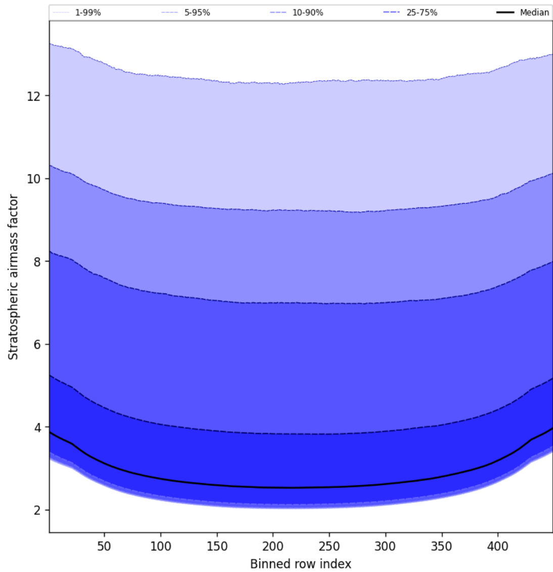
Figure 59: Along track statistics of “Stratospheric airmass factor” for 2025-04-07 to 2025-04-08
