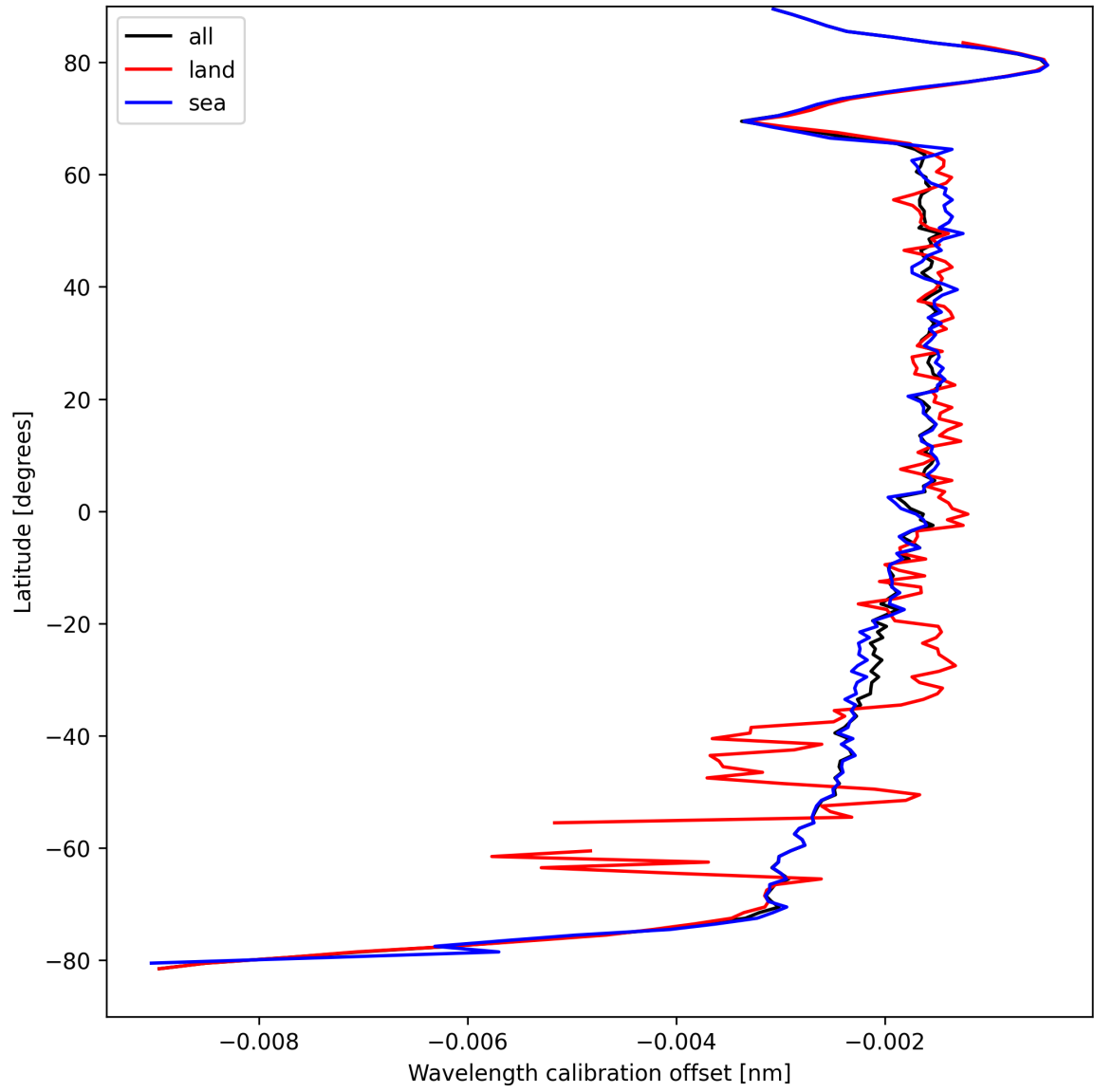
Figure 16: Zonal average of “Wavelength calibration offset” for 2025-04-07 to 2025-04-08.
