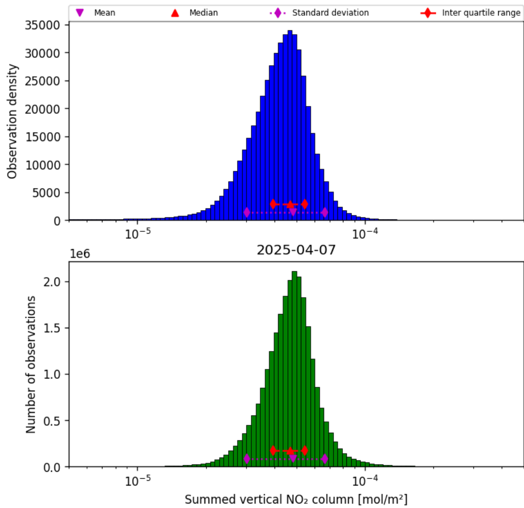
Figure 38: Histogram of “Summed vertical NO 2 column” for 2025-04-07 to 2025-04-08
