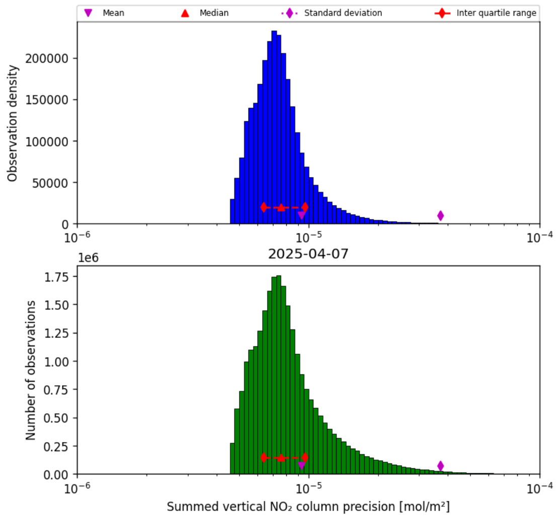
Figure 39: Histogram of “Summed vertical NO 2 column precision” for 2025-04-07 to 2025-04-08
