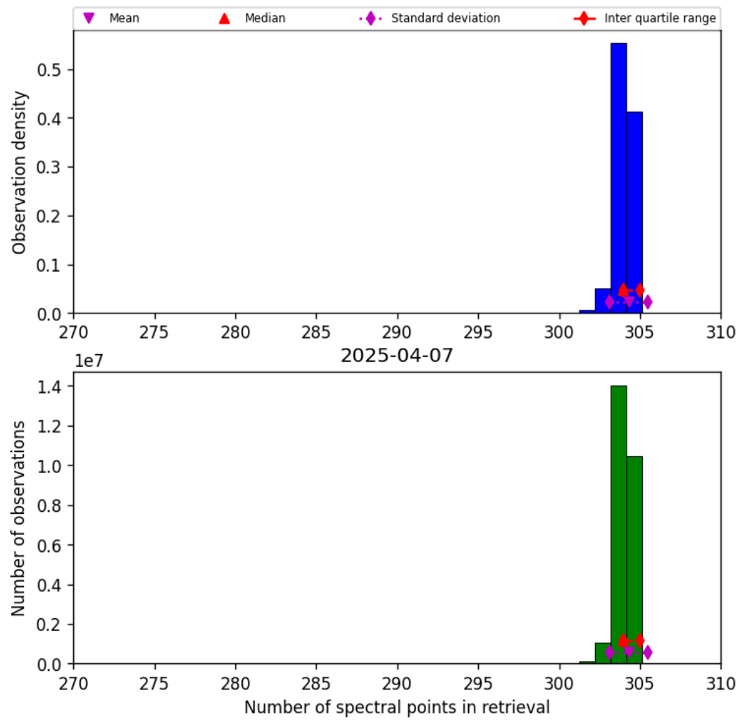
Figure 31: Histogram of “Number of spectral points in retrieval” for 2025-04-07 to 2025-04-08
