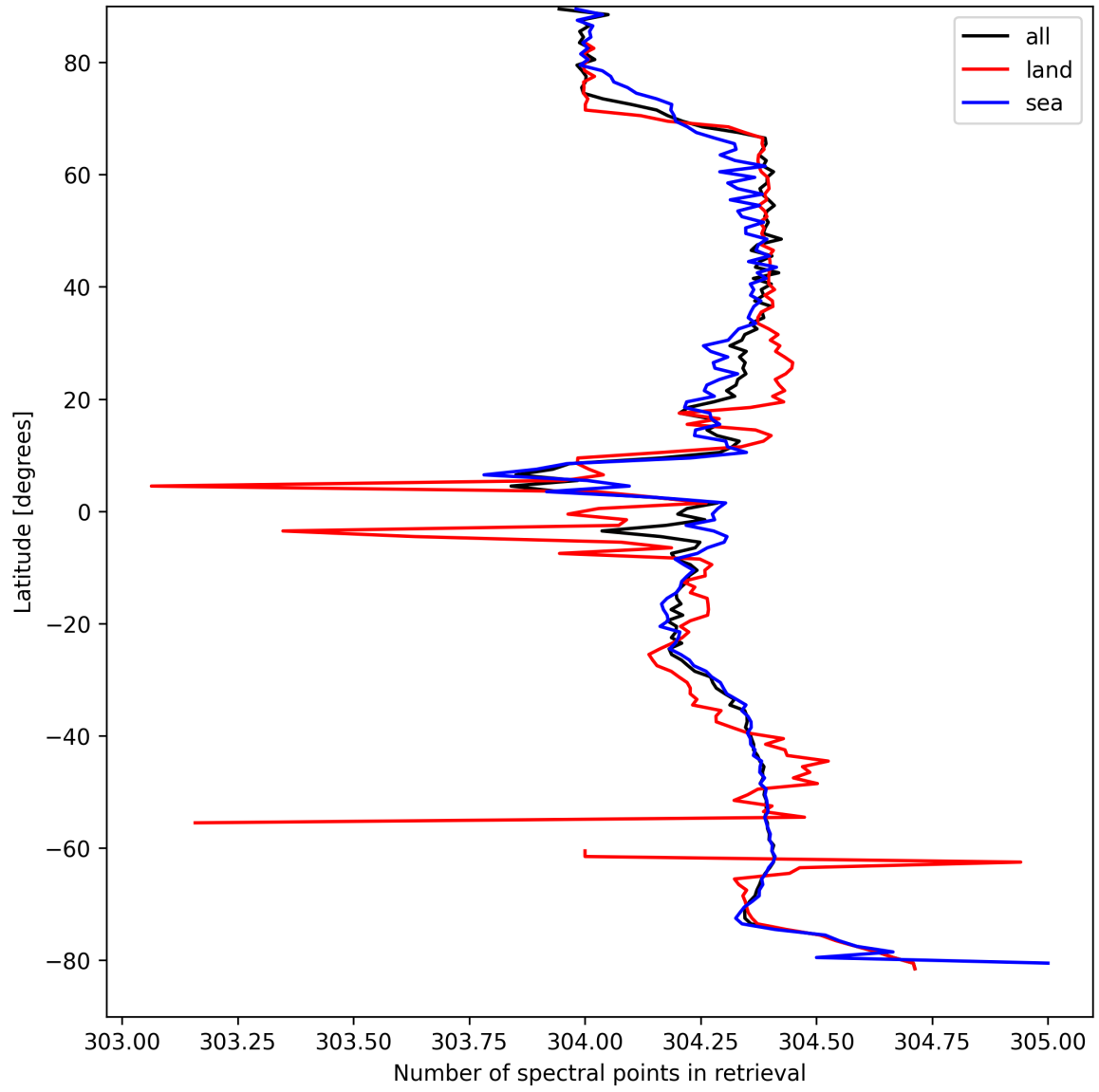
Figure 14: Zonal average of “Number of spectral points in retrieval” for 2025-04-07 to 2025-04-08.
