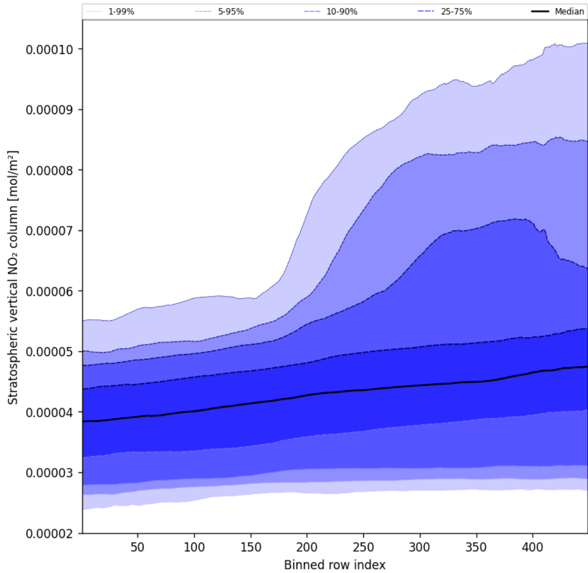
Figure 51: Along track statistics of “Stratospheric vertical NO 2 column” for 2025-04-07 to 2025-04-08
