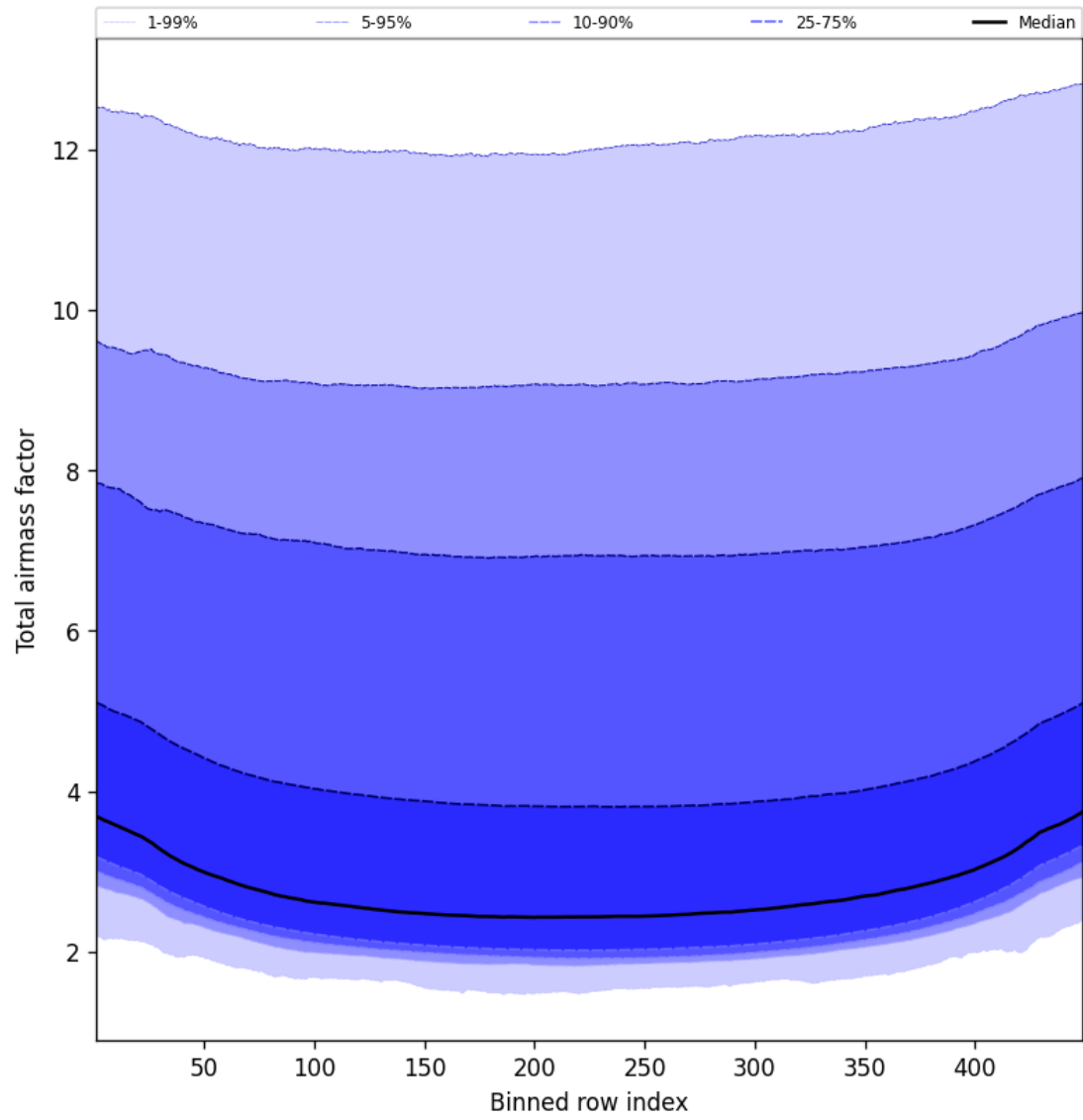
Figure 47: Along track statistics of “Total airmass factor” for 2025-04-07 to 2025-04-08
