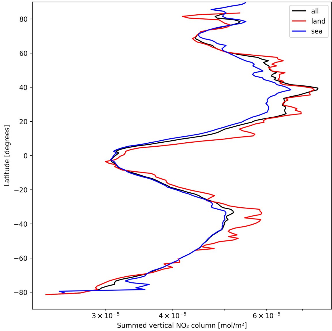
Figure 21: Zonal average of “Summed vertical NO 2 column” for 2025-04-07 to 2025-04-08.
