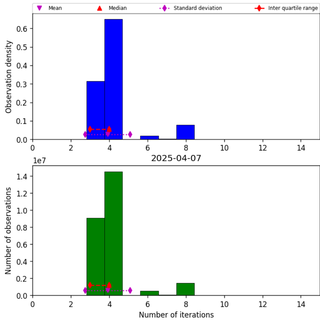
Figure 32: Histogram of “Number of iterations” for 2025-04-07 to 2025-04-08
