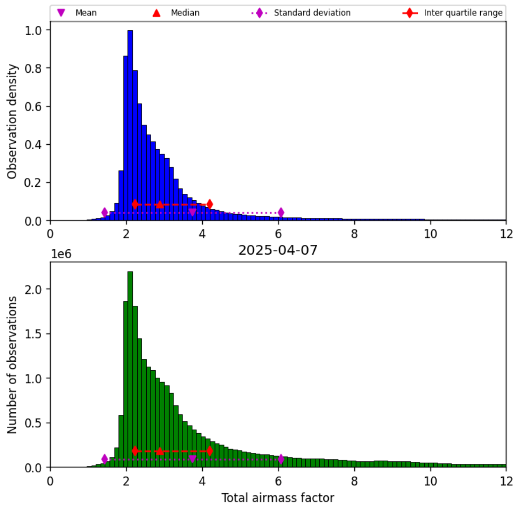
Figure 30: Histogram of “Total airmass factor” for 2025-04-07 to 2025-04-08
