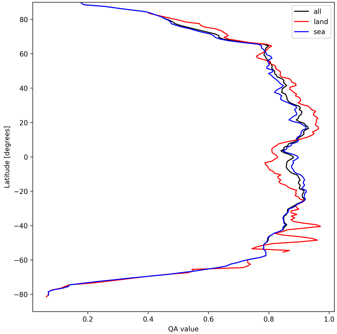
Figure 9: Zonal average of “QA value” for 2025-04-07 to 2025-04-08.
