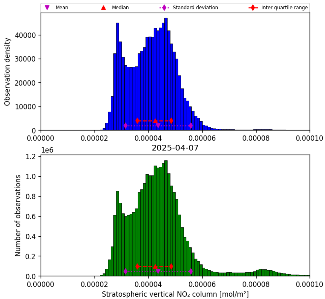
Figure 34: Histogram of “Stratospheric vertical NO 2 column” for 2025-04-07 to 2025-04-08
