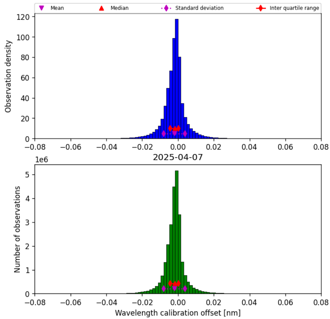
Figure 33: Histogram of “Wavelength calibration offset” for 2025-04-07 to 2025-04-08
