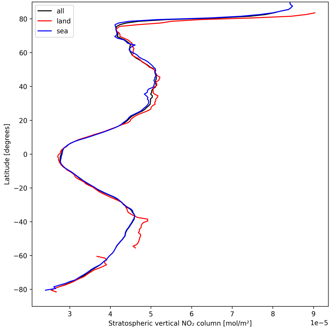
Figure 17: Zonal average of “Stratospheric vertical NO 2 column” for 2025-04-07 to 2025-04-08.
