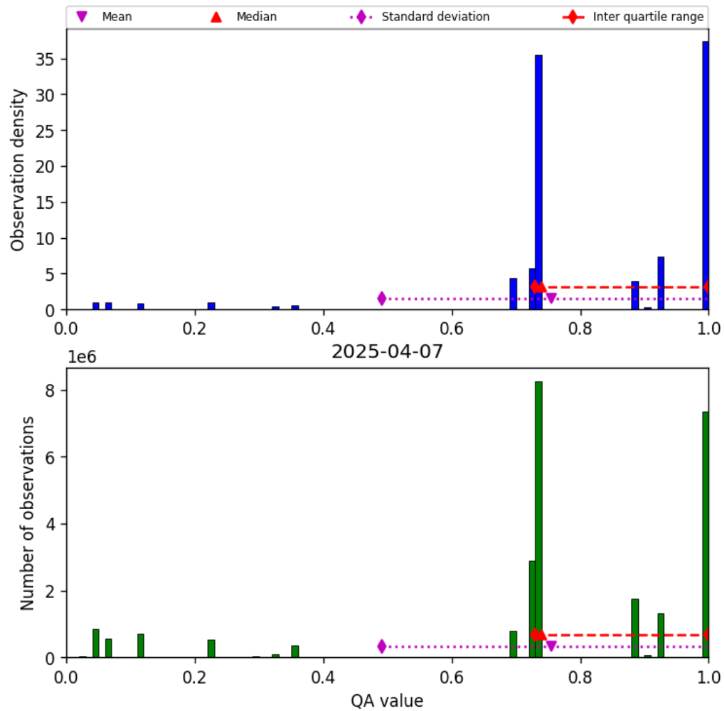
Figure 26: Histogram of “QA value” for 2025-04-07 to 2025-04-08
