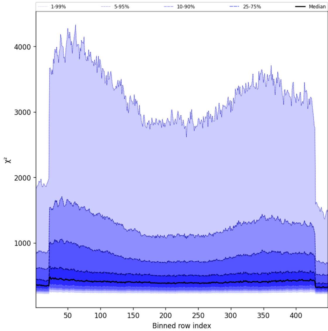
Figure 57: Along track statistics of “ \chi^2 ” for 2025-04-07 to 2025-04-08
