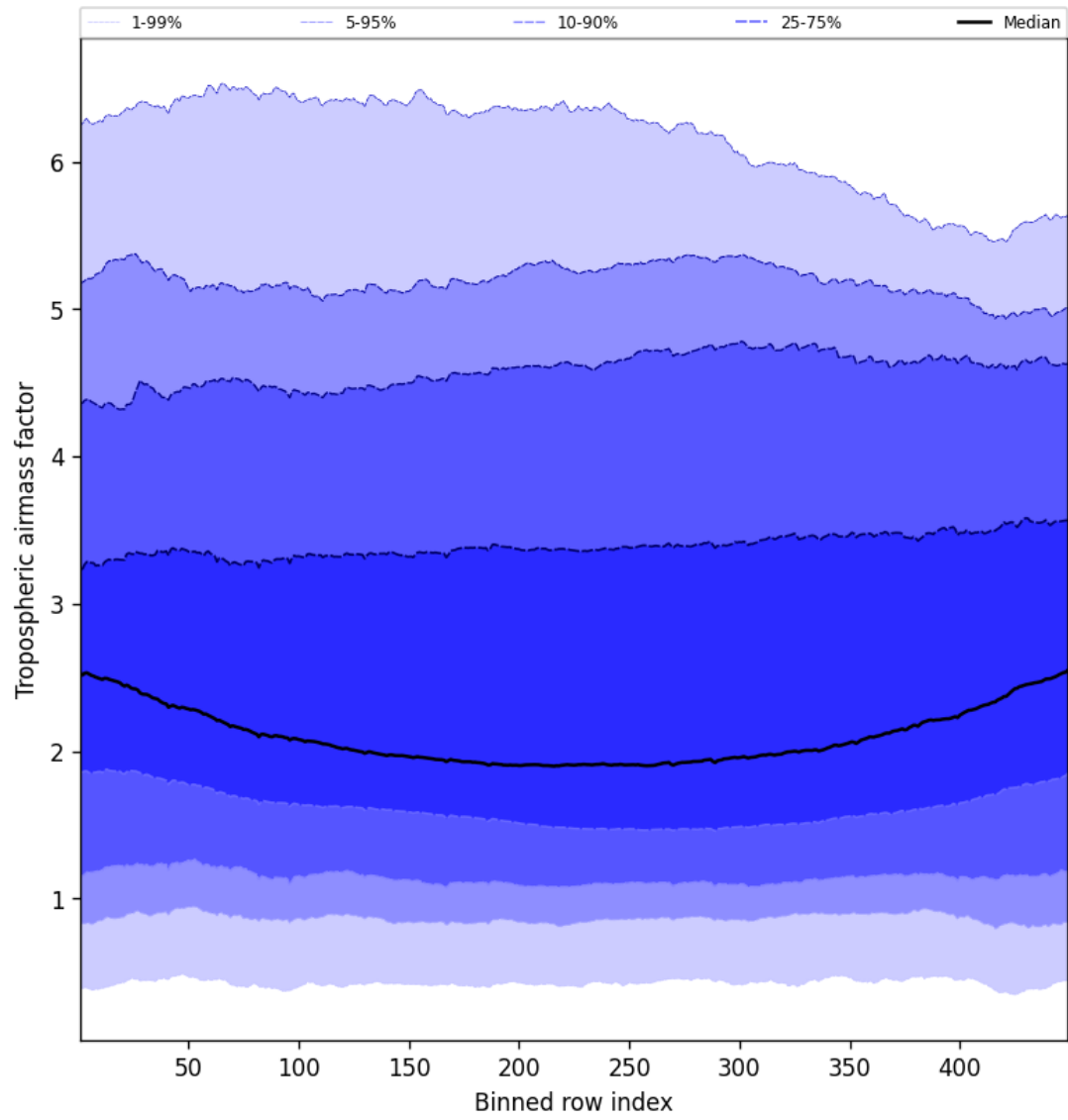
Figure 46: Along track statistics of “Tropospheric airmass factor” for 2025-04-07 to 2025-04-08
