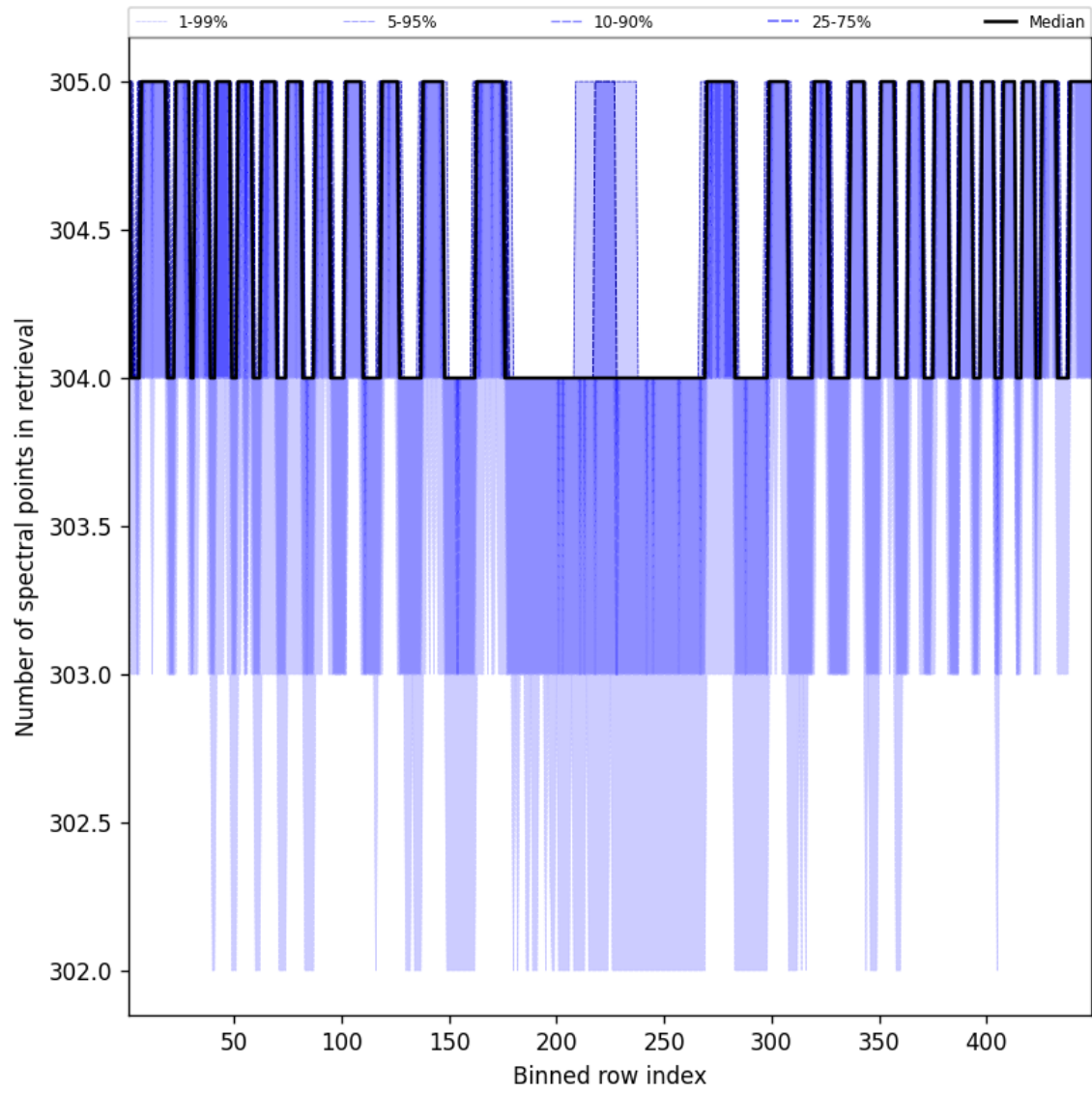
Figure 48: Along track statistics of “Number of spectral points in retrieval” for 2025-04-07 to 2025-04-08
