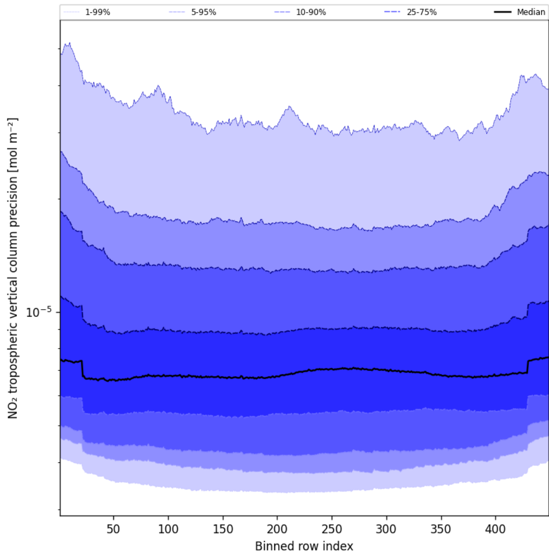
Figure 45: Along track statistics of “NO 2 tropospheric vertical column precision” for 2025-04-07 to 2025-04-08
