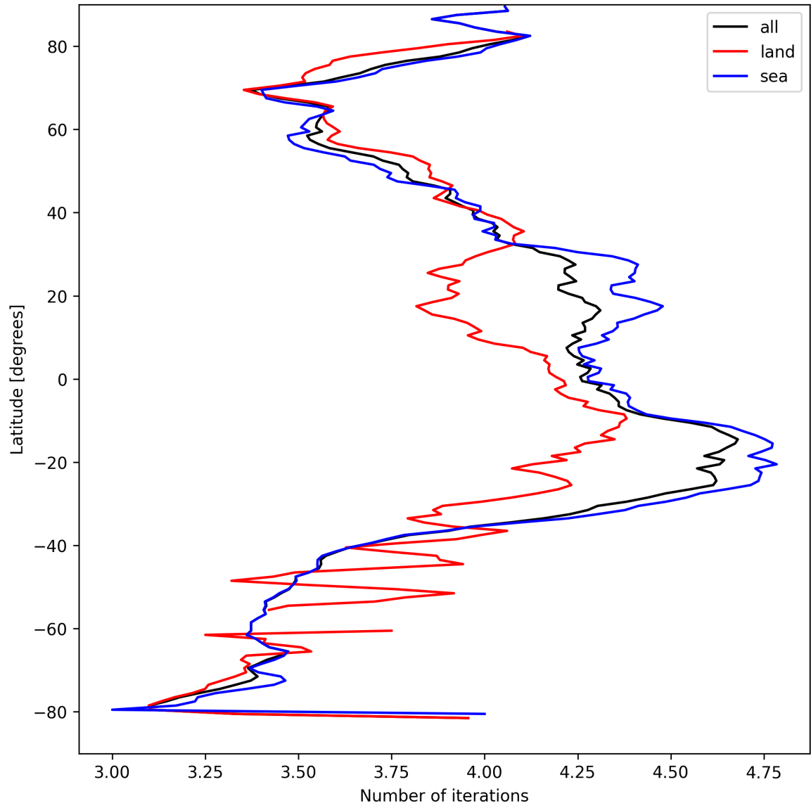
Figure 15: Zonal average of “Number of iterations” for 2025-04-07 to 2025-04-08.
