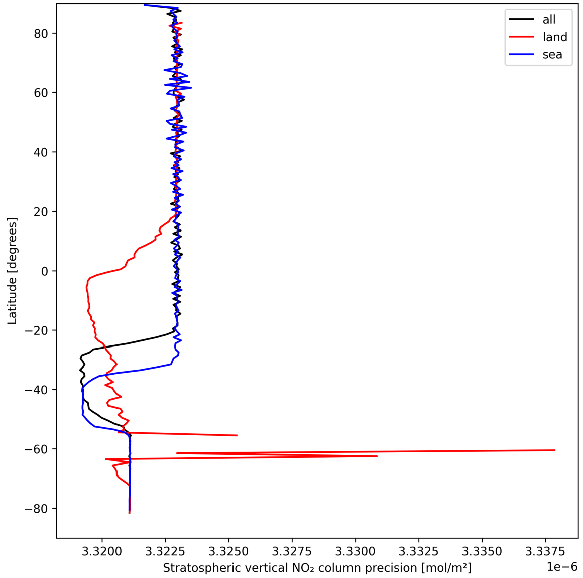
Figure 18: Zonal average of “Stratospheric vertical NO 2 column precision” for 2025-04-07 to 2025-04-08.
