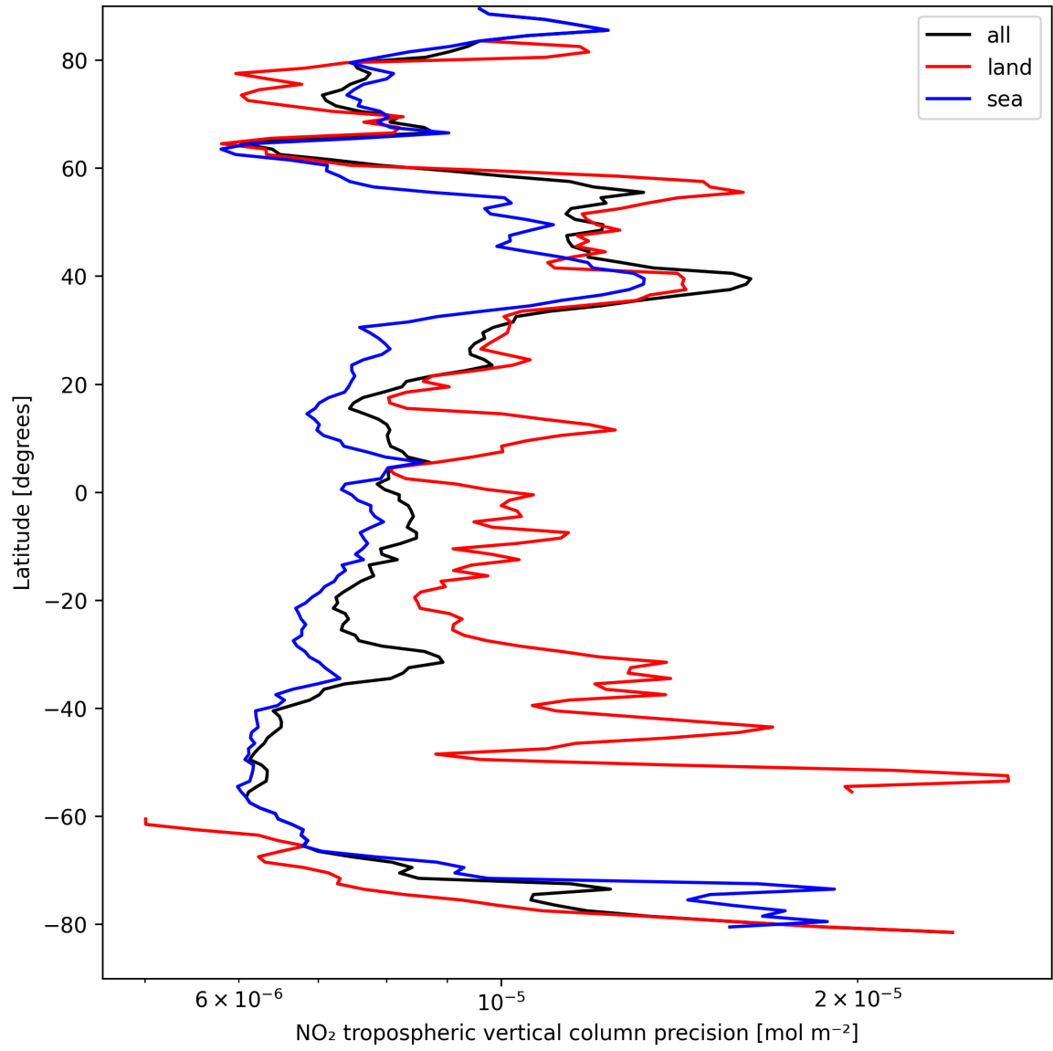
Figure 11: Zonal average of “NO 2 tropospheric vertical column precision” for 2025-04-07 to 2025-04-08.
