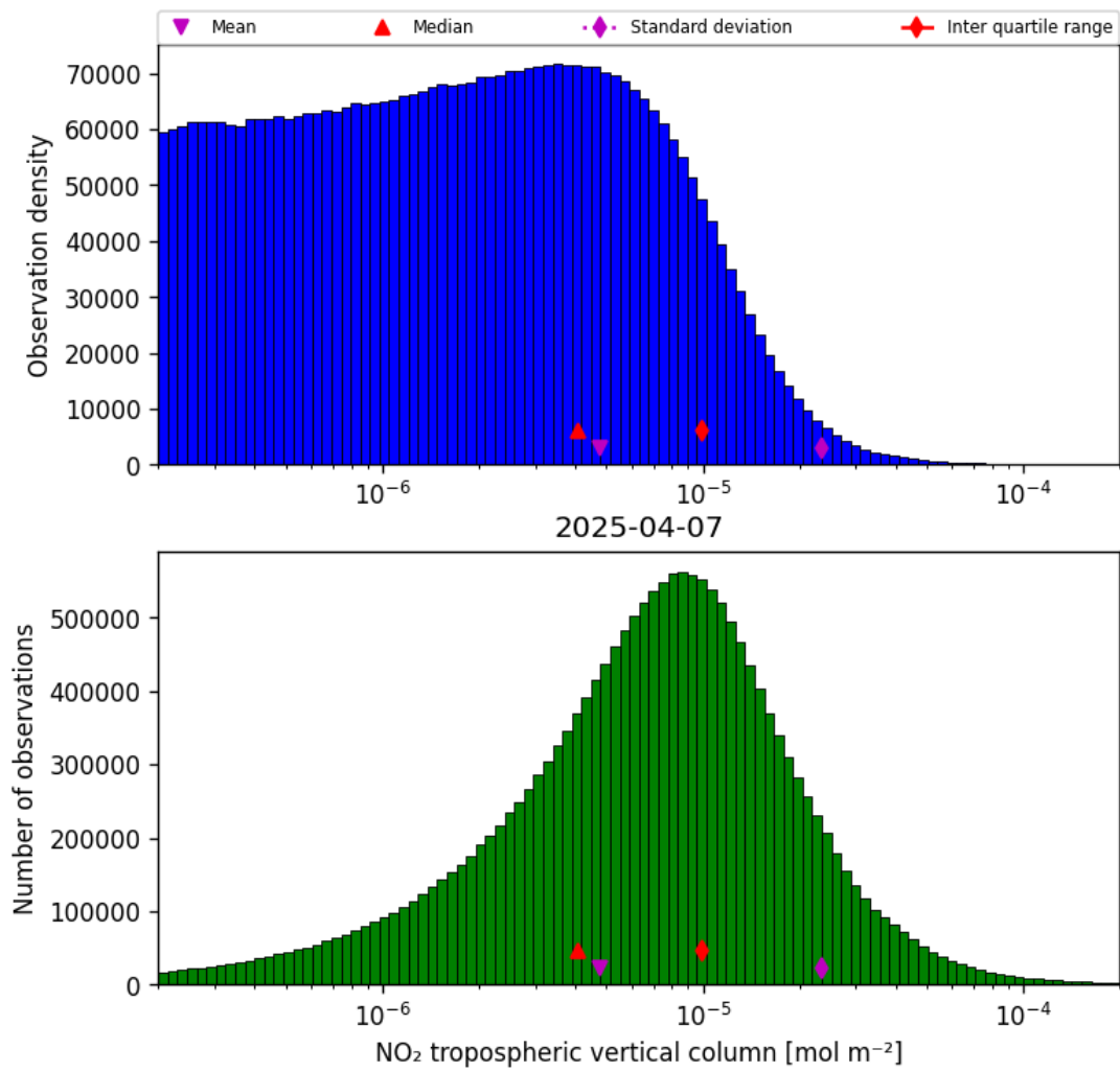
Figure 27: Histogram of “NO 2 tropospheric vertical column” for 2025-04-07 to 2025-04-08
