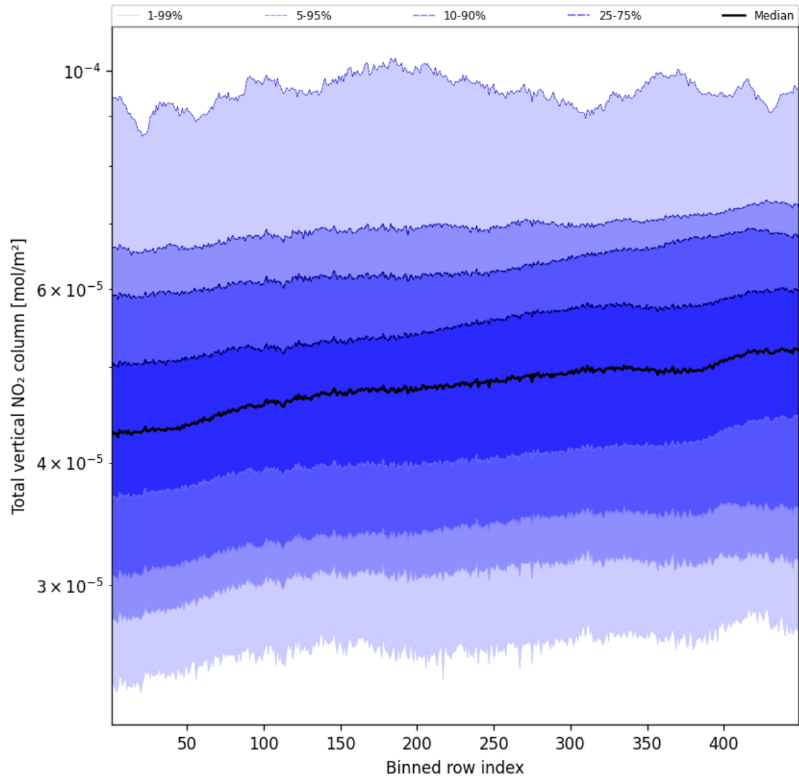
Figure 53: Along track statistics of “Total vertical NO 2 column” for 2025-04-07 to 2025-04-08
