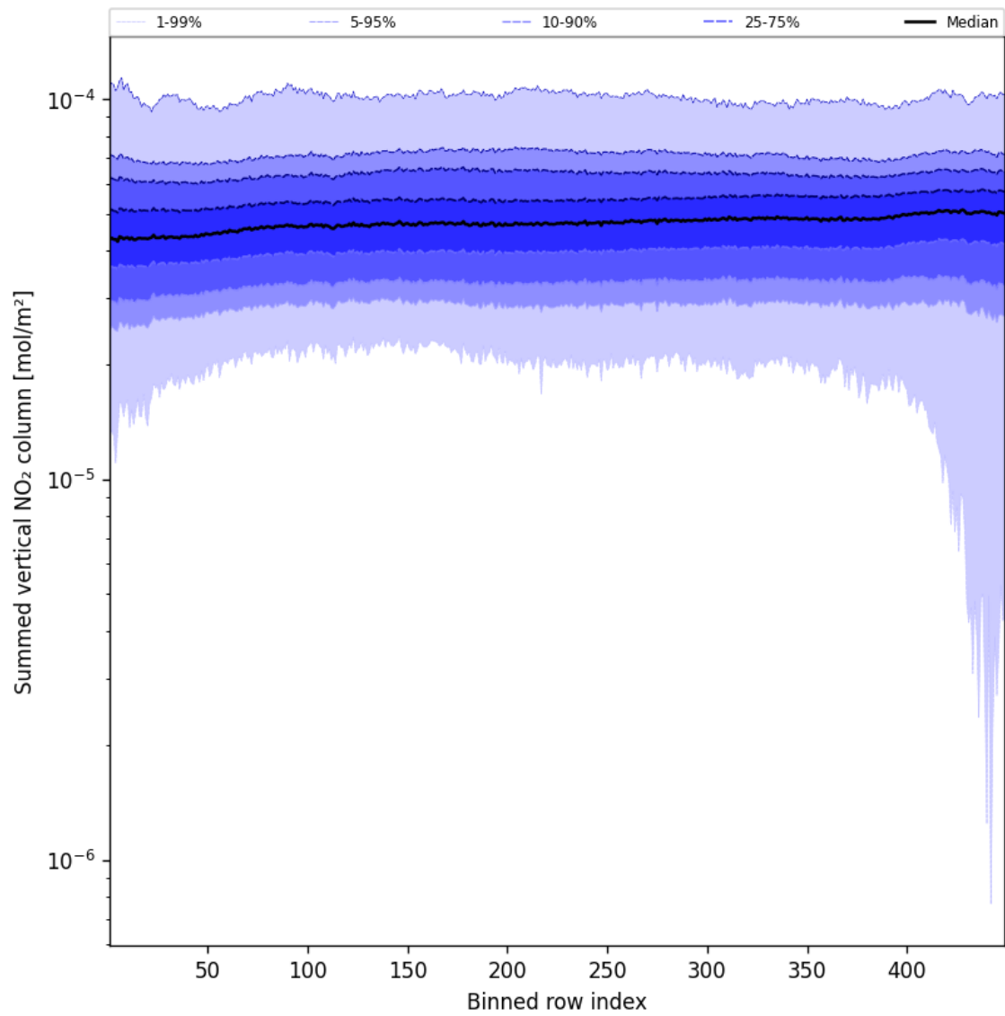
Figure 55: Along track statistics of “Summed vertical NO 2 column” for 2025-04-07 to 2025-04-08
