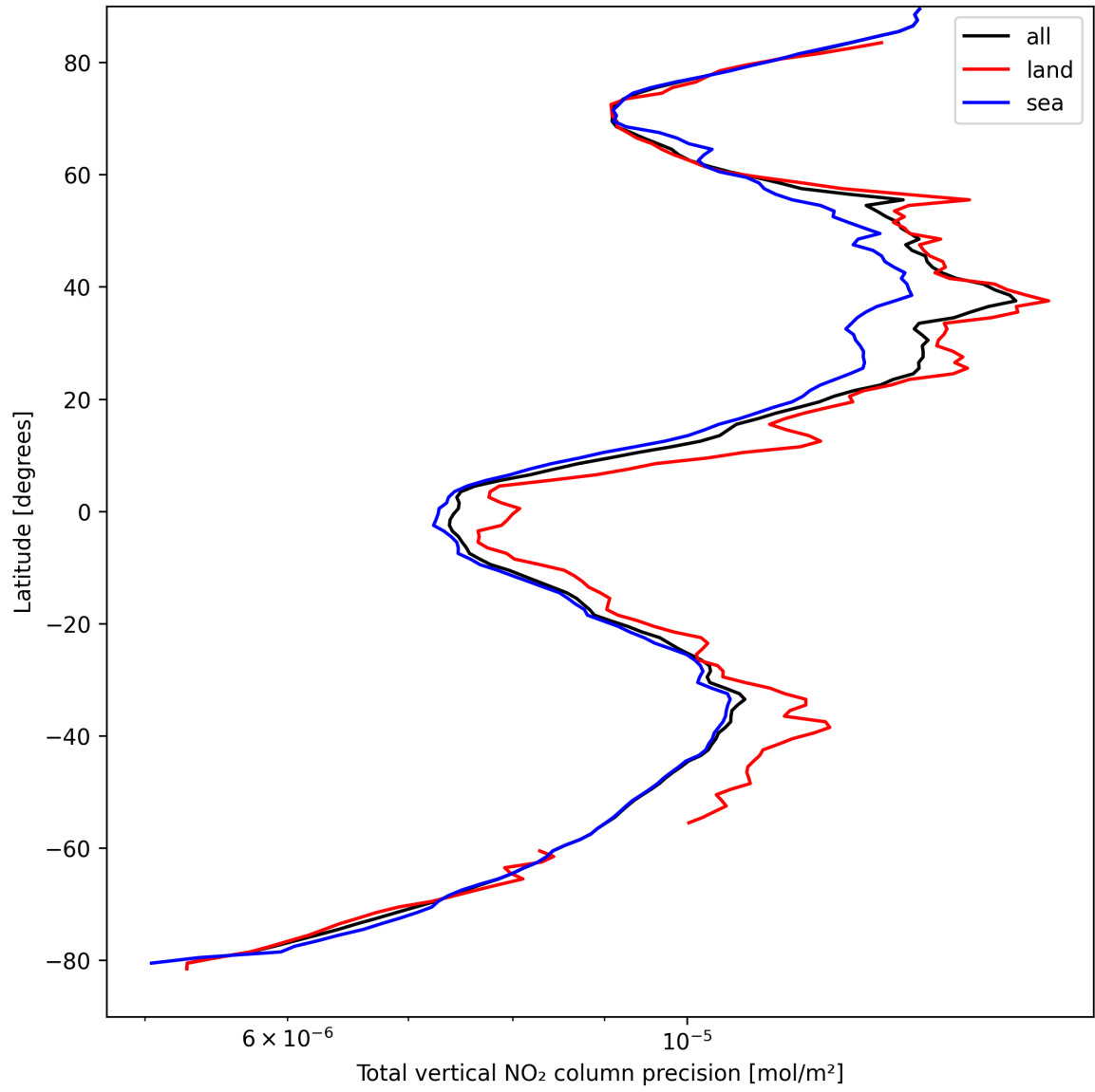
Figure 20: Zonal average of “Total vertical NO 2 column precision” for 2025-04-07 to 2025-04-08.
