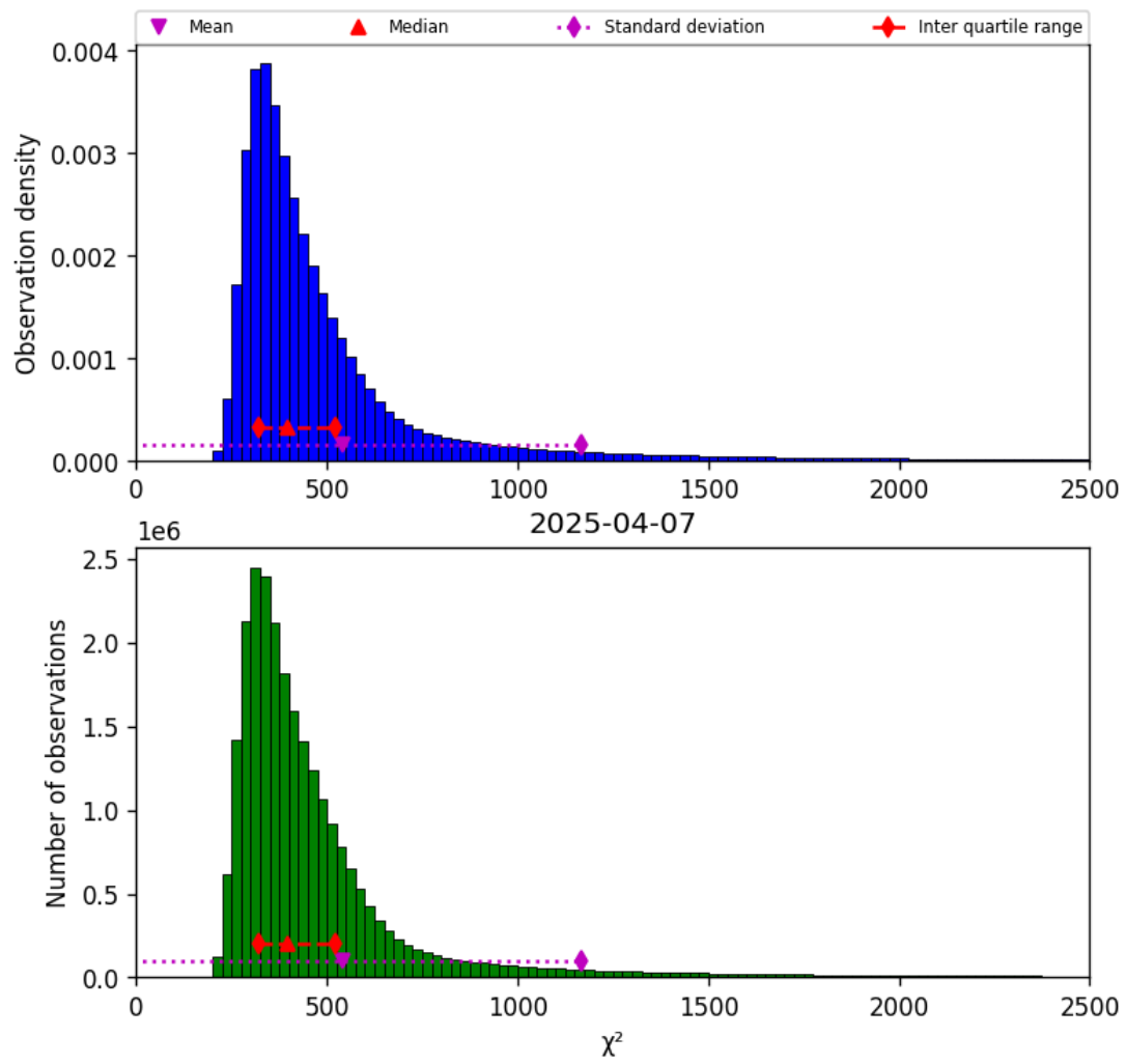
Figure 40: Histogram of “ \chi^2 ” for 2025-04-07 to 2025-04-08
