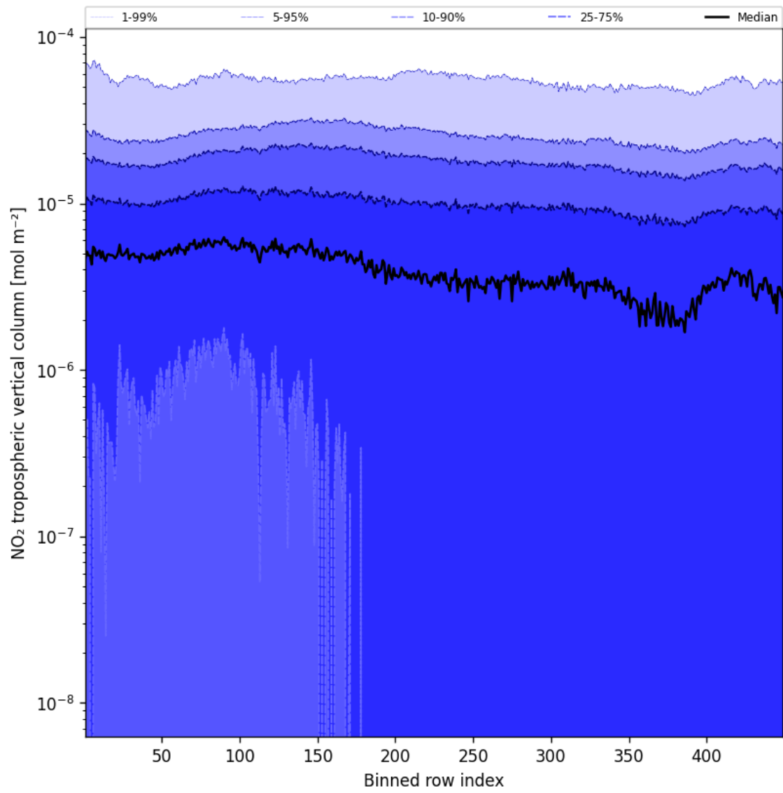
Figure 44: Along track statistics of “NO 2 tropospheric vertical column” for 2025-04-07 to 2025-04-08
