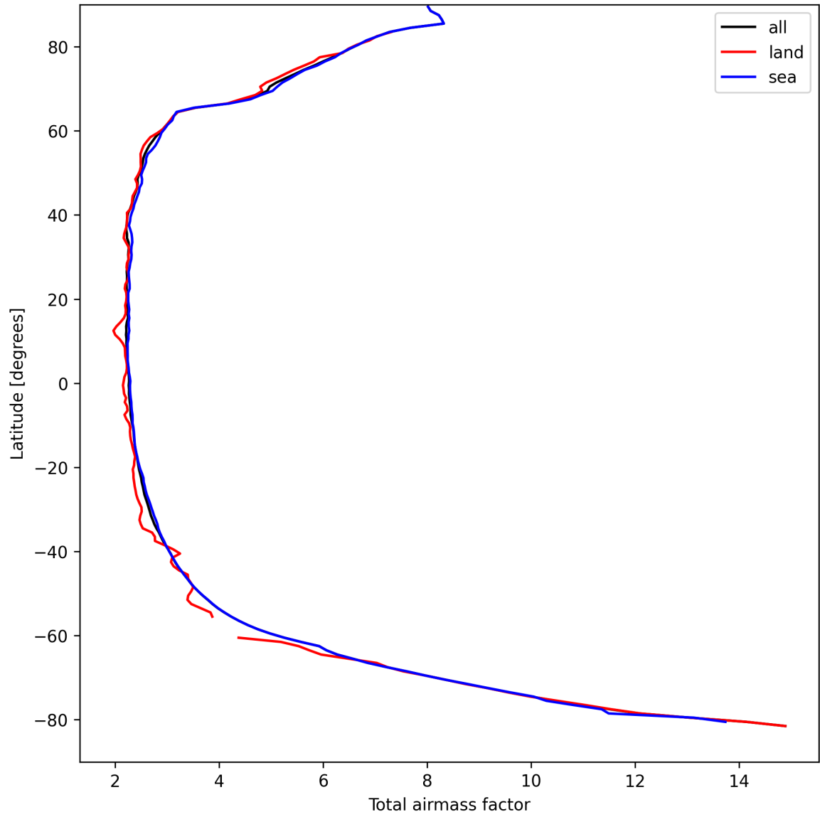
Figure 13: Zonal average of “Total airmass factor” for 2025-04-07 to 2025-04-08.
