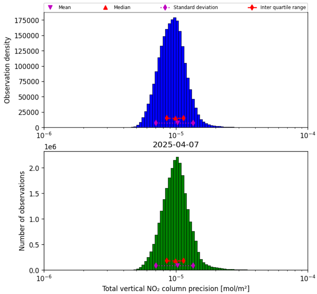
Figure 37: Histogram of “Total vertical NO 2 column precision” for 2025-04-07 to 2025-04-08
