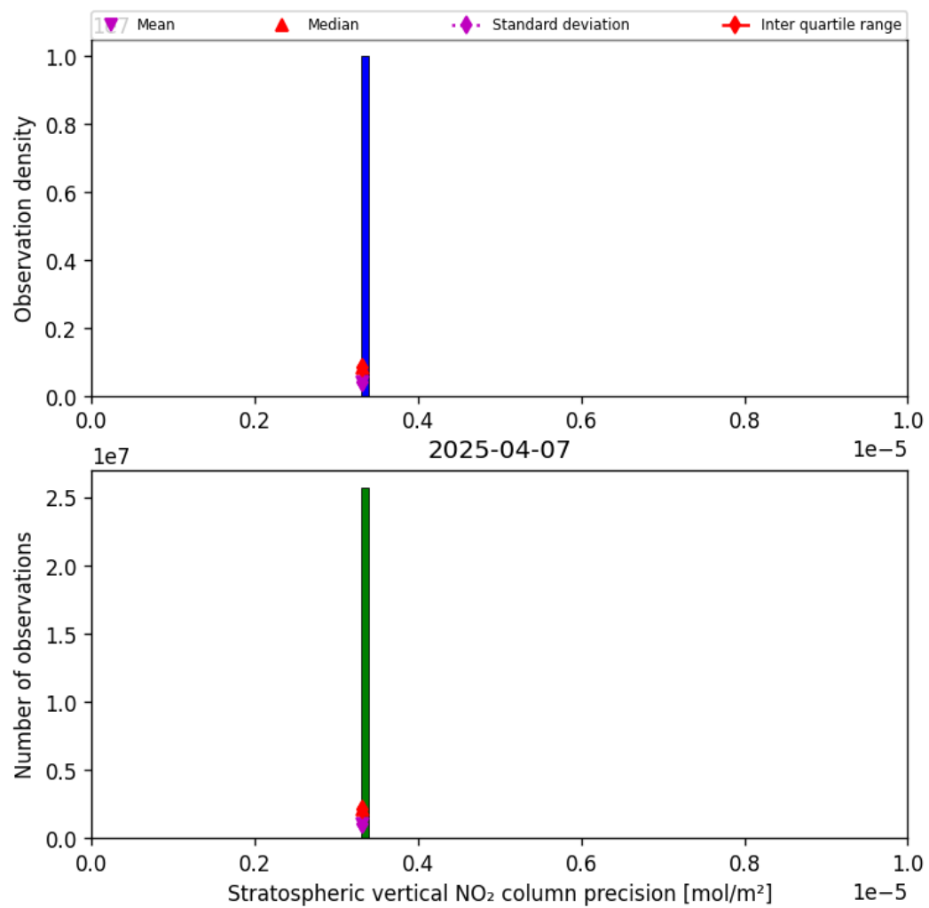
Figure 35: Histogram of “Stratospheric vertical NO 2 column precision” for 2025-04-07 to 2025-04-08
